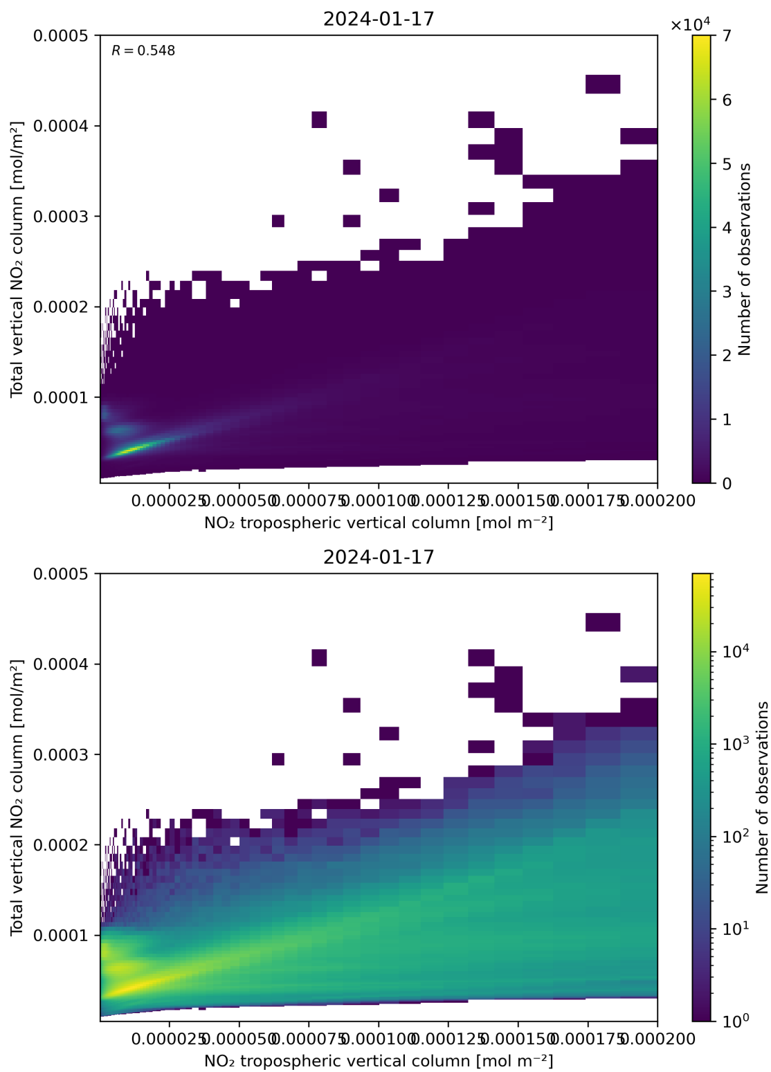
Figure 128: Scatter density plot of “NO 2 tropospheric vertical column” against “Total vertical NO 2 column” for 2024-01-16 to 2024-01-18.
