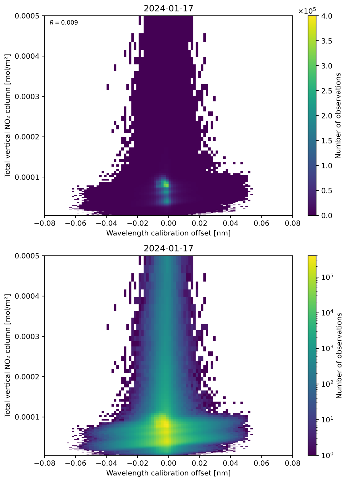
Figure 179: Scatter density plot of “Wavelength calibration offset” against “Total vertical NO 2 column” for 2024-01-16 to 2024-01-18.
