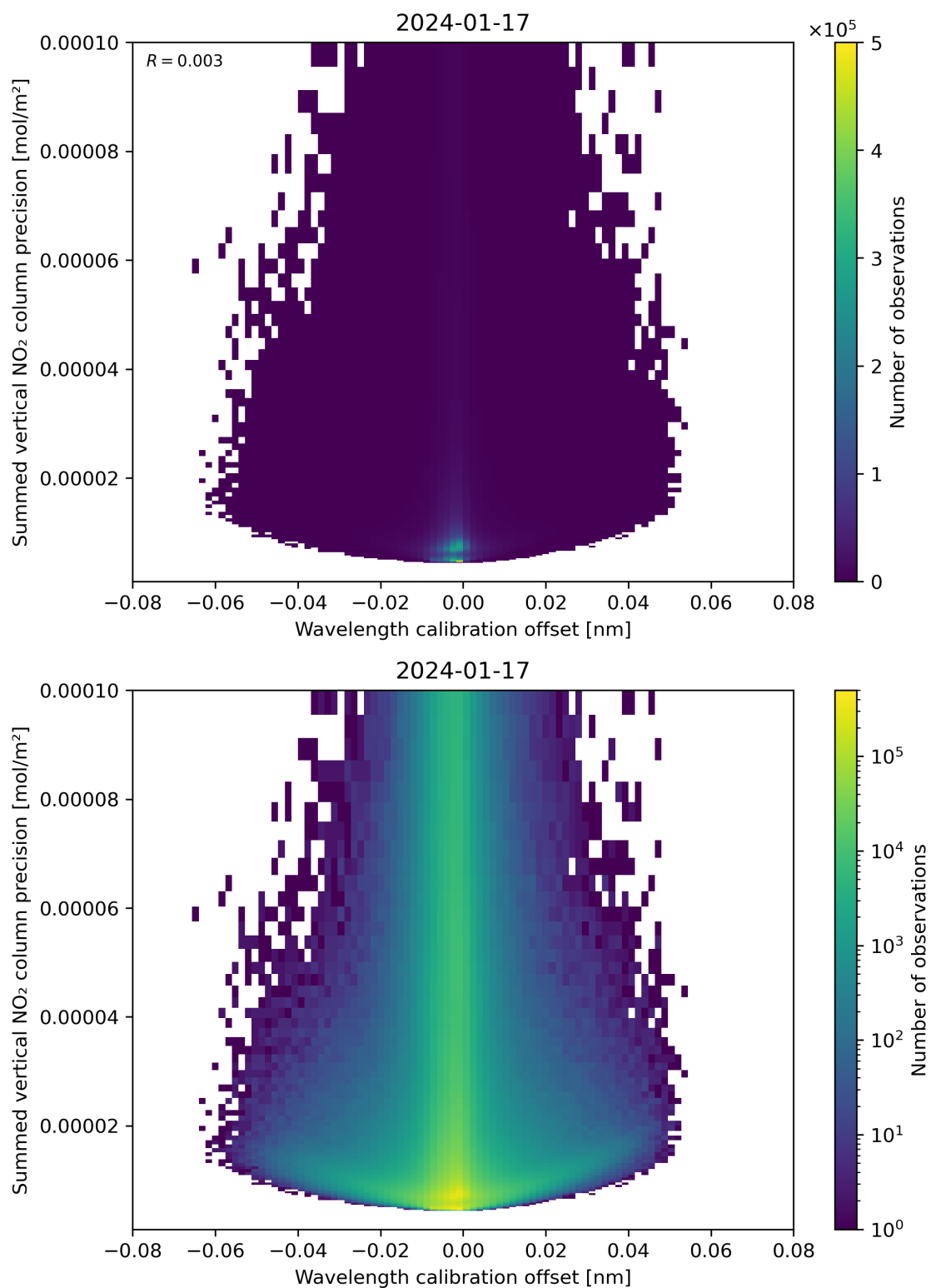
Figure 178: Scatter density plot of “Wavelength calibration offset” against “Summed vertical NO 2 column precision” for 2024-01-16 to 2024-01-18.
