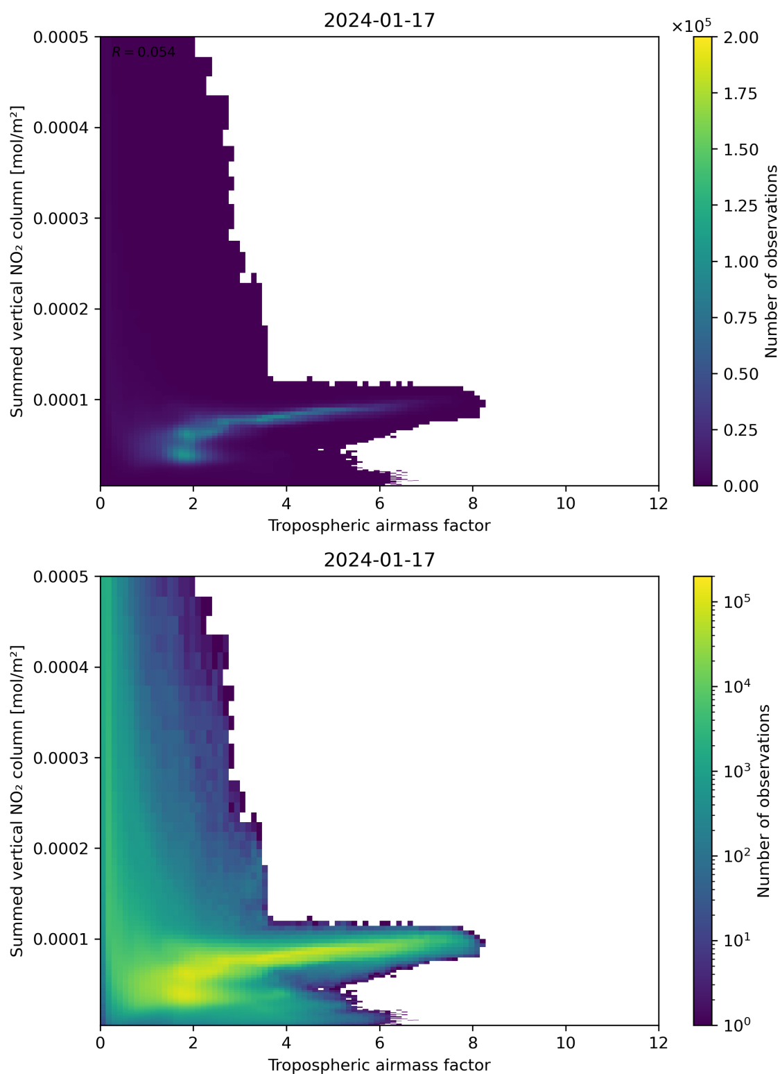
Figure 75: Scatter density plot of “Tropospheric airmass factor” against “Summed vertical NO 2 column” for 2024-01-16 to 2024-01-18.
