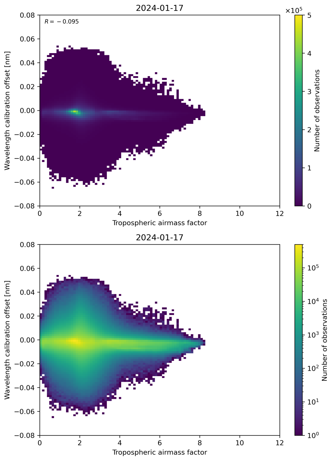
Figure 80: Scatter density plot of “Tropospheric air mass factor” against “Wavelength calibration offset” for 2024-01-16 to 2024-01-18.
