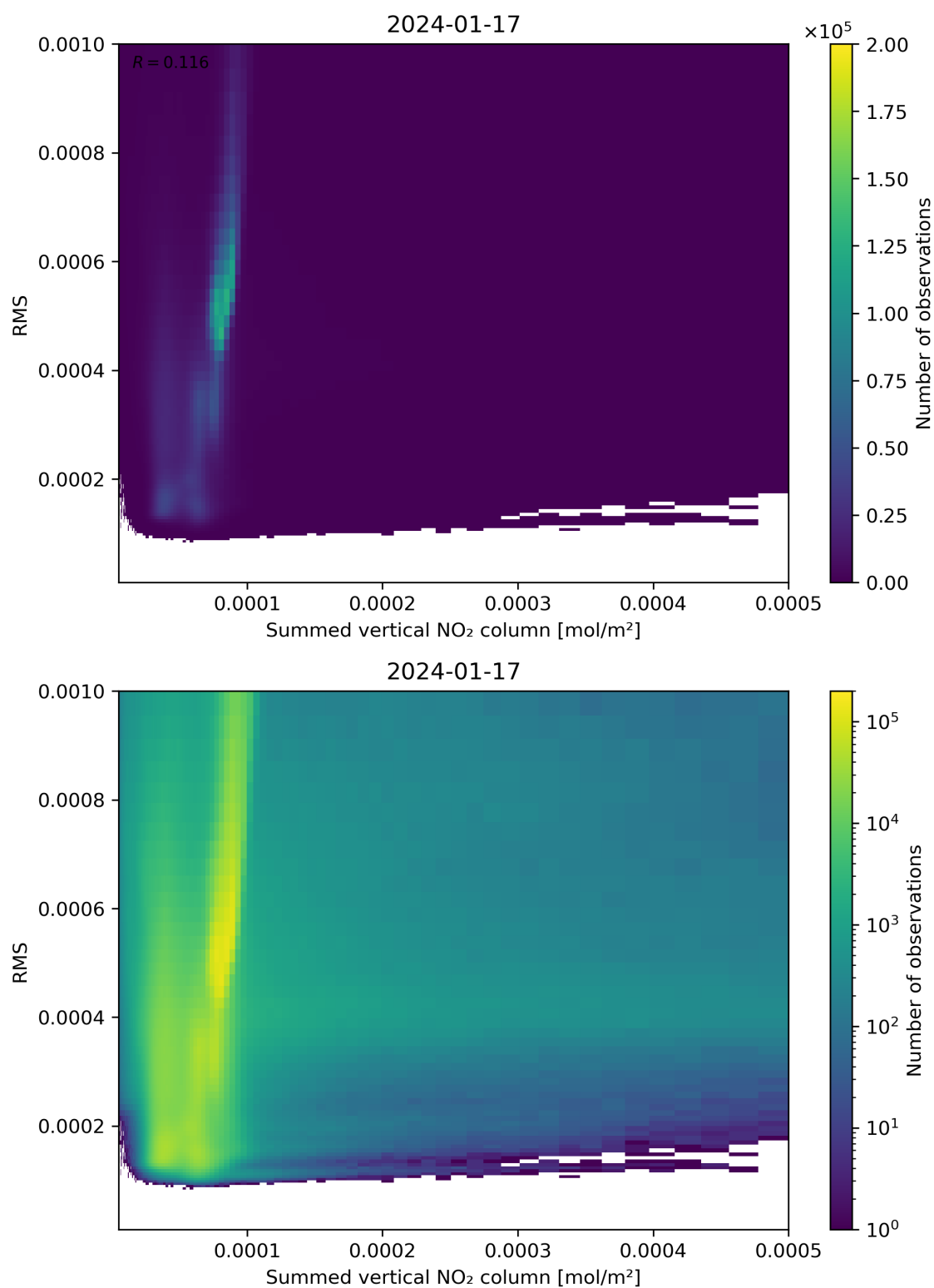
Figure 109: Scatter density plot of “Summed vertical NO 2 column” against “RMS” for 2024-01-16 to 2024-01-18.
