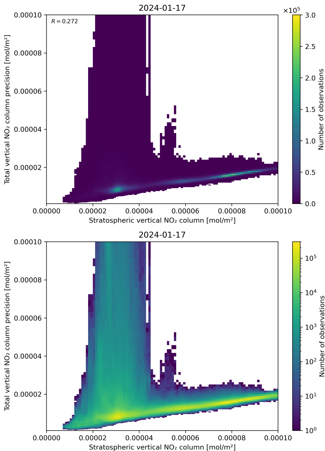
Figure 101: Scatter density plot of “Stratospheric vertical NO 2 column” against “Total vertical NO 2 column precision” for 2024-01-16 to 2024-01-18.
