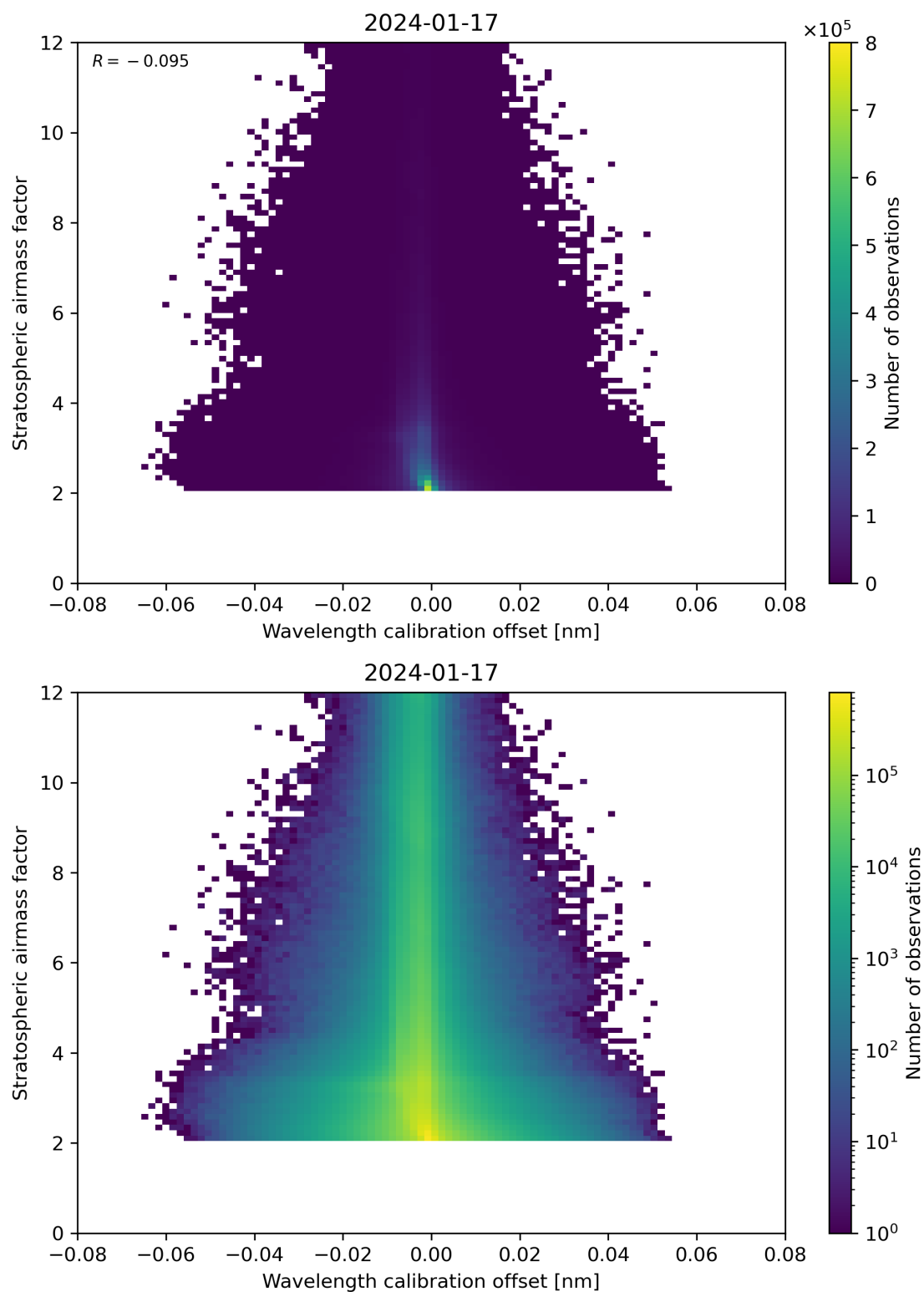
Figure 174: Scatter density plot of “Wavelength calibration offset” against “Stratospheric airmass factor” for 2024-01-16 to 2024-01-18.
