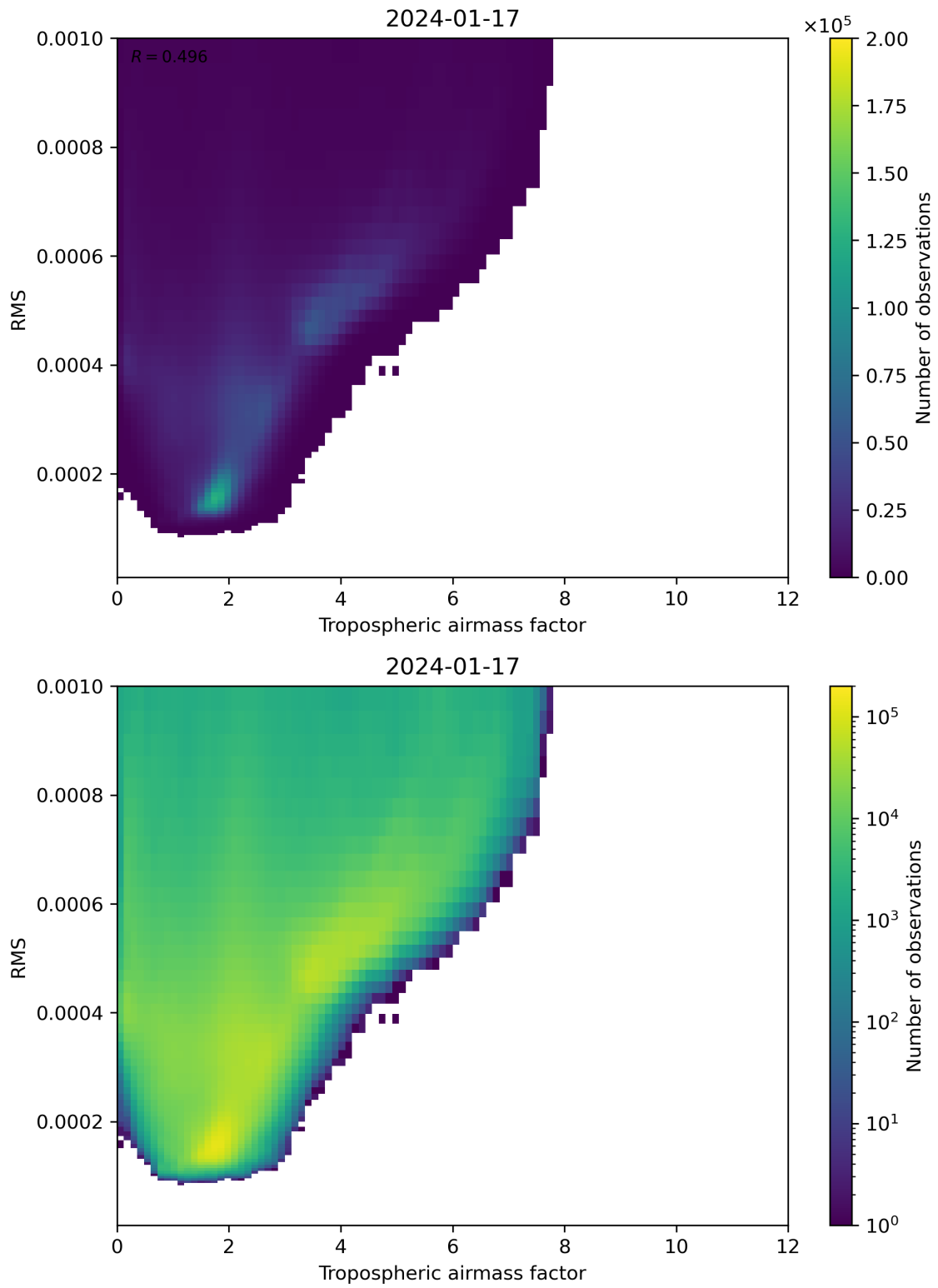
Figure 79: Scatter density plot of “Tropospheric airmass factor” against “RMS” for 2024-01-16 to 2024-01-18.
