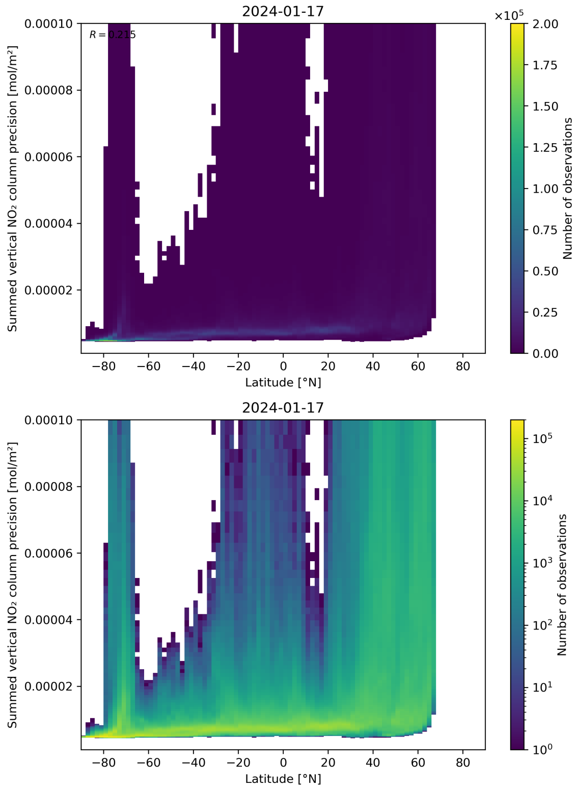
Figure 89: Scatter density plot of “Latitude” against “Summed vertical NO 2 column precision” for 2024-01-16 to 2024-01-18.
