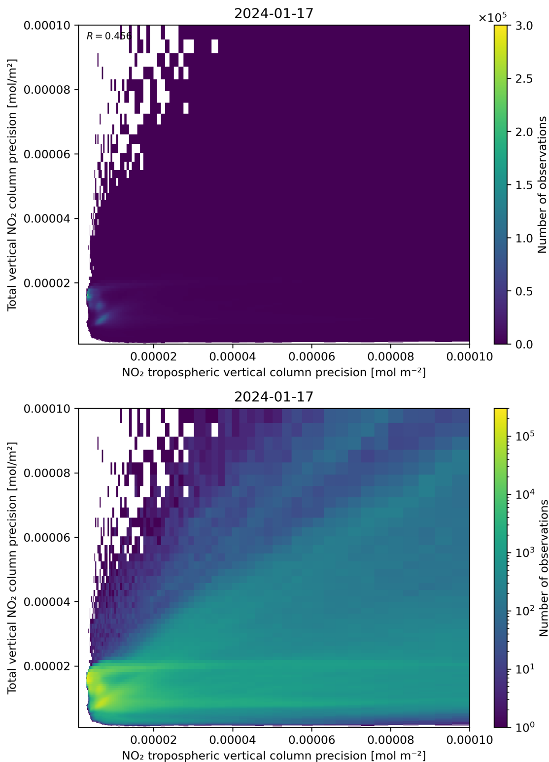
Figure 139: Scatter density plot of “NO 2 tropospheric vertical column precision” against “Total vertical NO 2 column precision” for 2024-01-16 to 2024-01-18.
