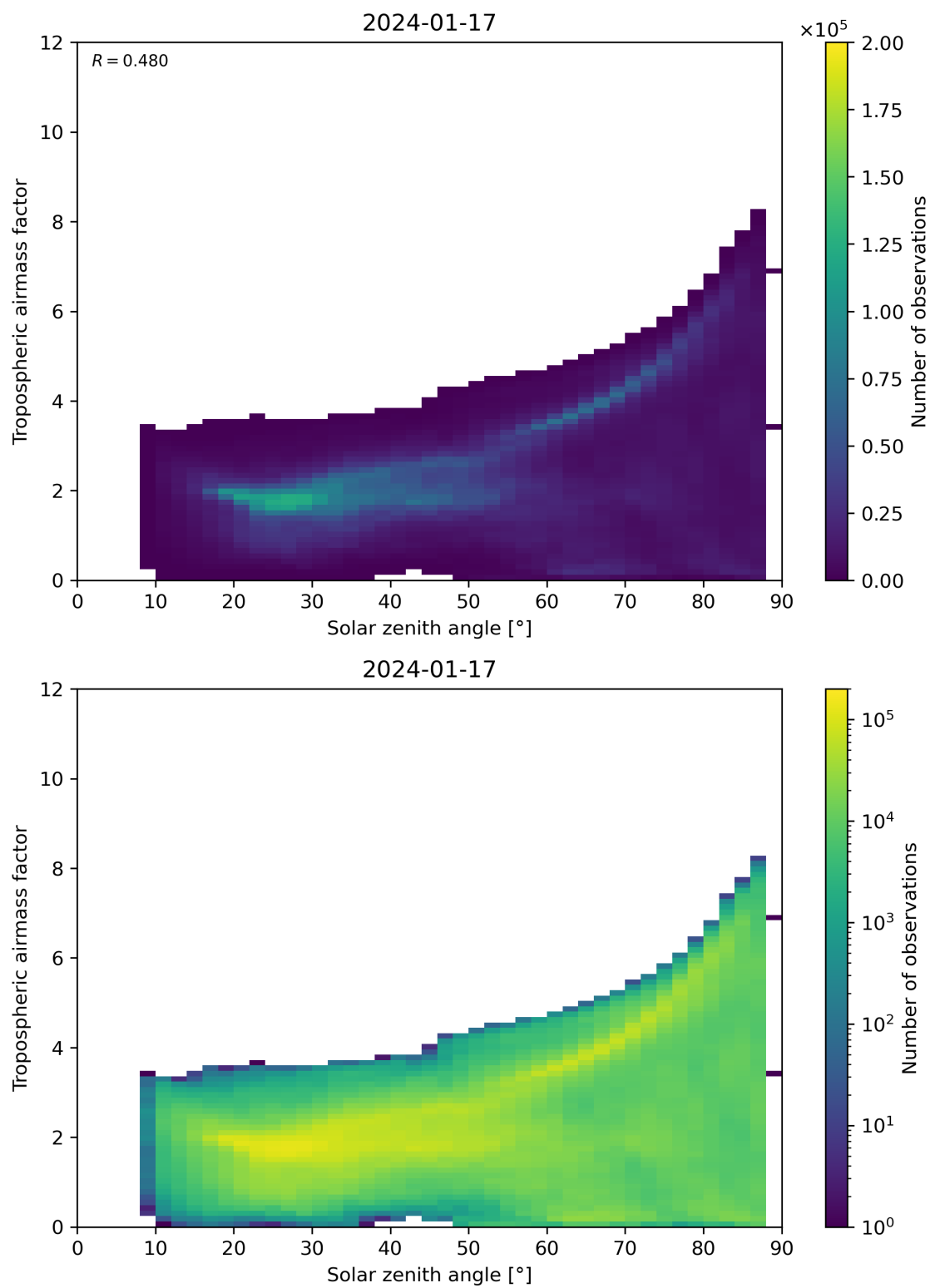
Figure 147: Scatter density plot of “Solar zenith angle” against “Tropospheric airmass factor” for 2024-01-16 to 2024-01-18.
