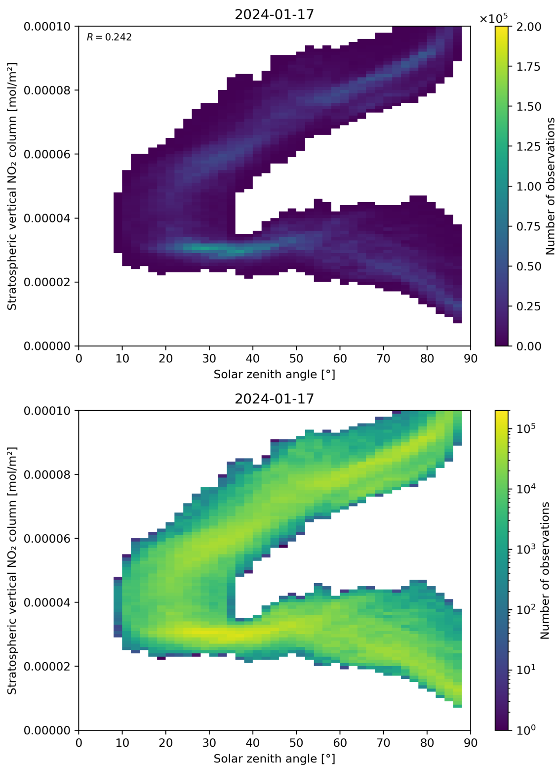
Figure 150: Scatter density plot of “Solar zenith angle” against “Stratospheric vertical NO 2 column” for 2024-01-16 to 2024-01-18.
