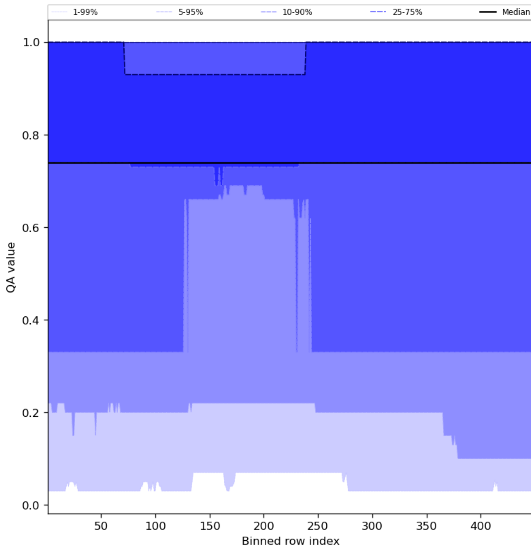
Figure 45: Along track statistics of “QA value” for 2024-01-16 to 2024-01-18
