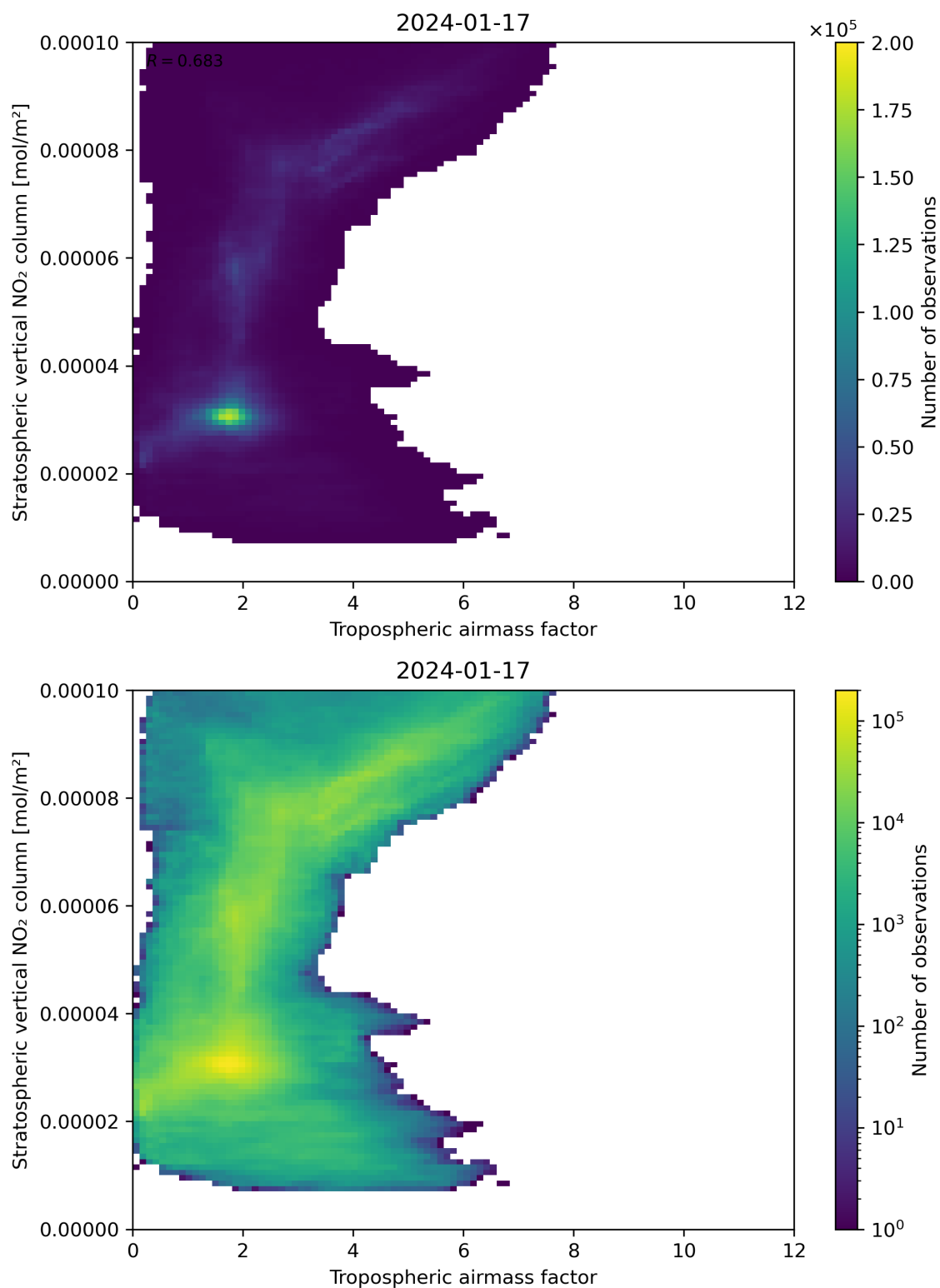
Figure 74: Scatter density plot of “Tropospheric air mass factor” against “Stratospheric vertical NO 2 column” for 2024-01-16 to 2024-01-18.
