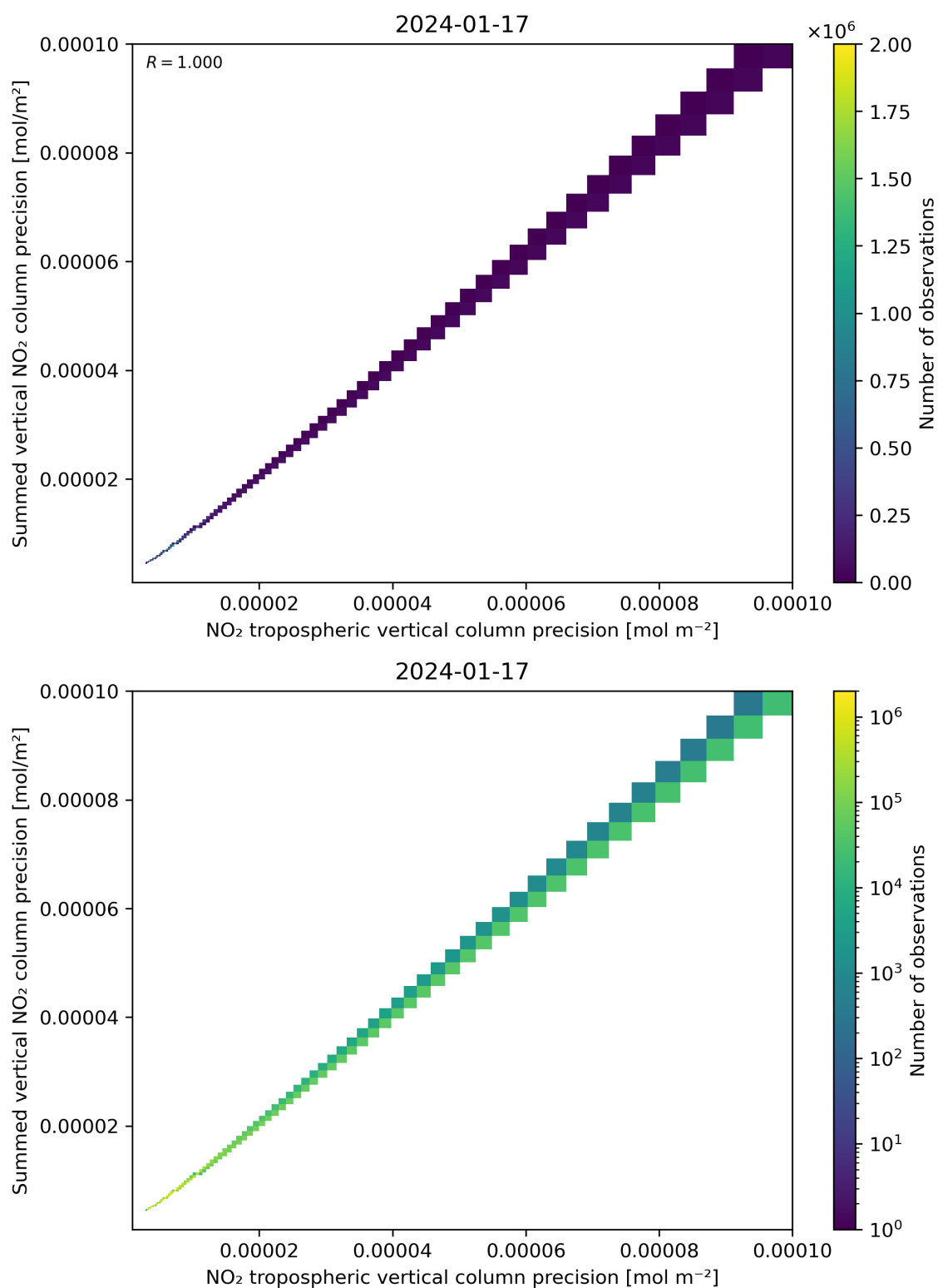
Figure 137: Scatter density plot of “NO 2 tropospheric vertical column precision” against “Summed vertical NO 2 column precision” for 2024-01-16 to 2024-01-18.
