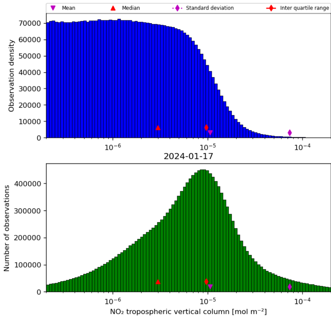
Figure 29: Histogram of “ \text{NO}_2 tropospheric vertical column” for 2024-01-16 to 2024-01-18
