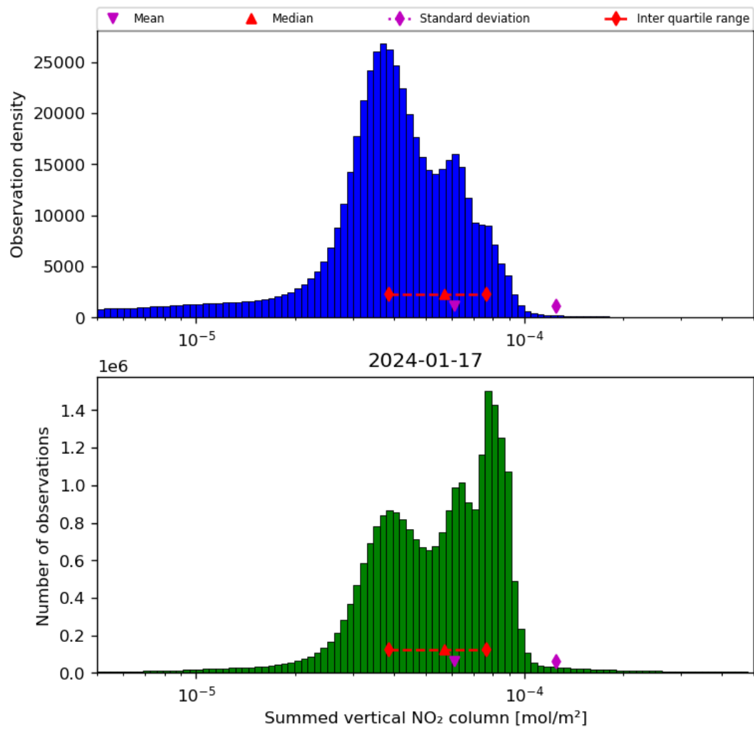
Figure 40: Histogram of “Summed vertical NO 2 column” for 2024-01-16 to 2024-01-18
