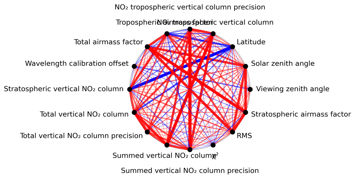
Figure 1: Map of correlation graph for 2024-01-16 to 2024-01-18.
