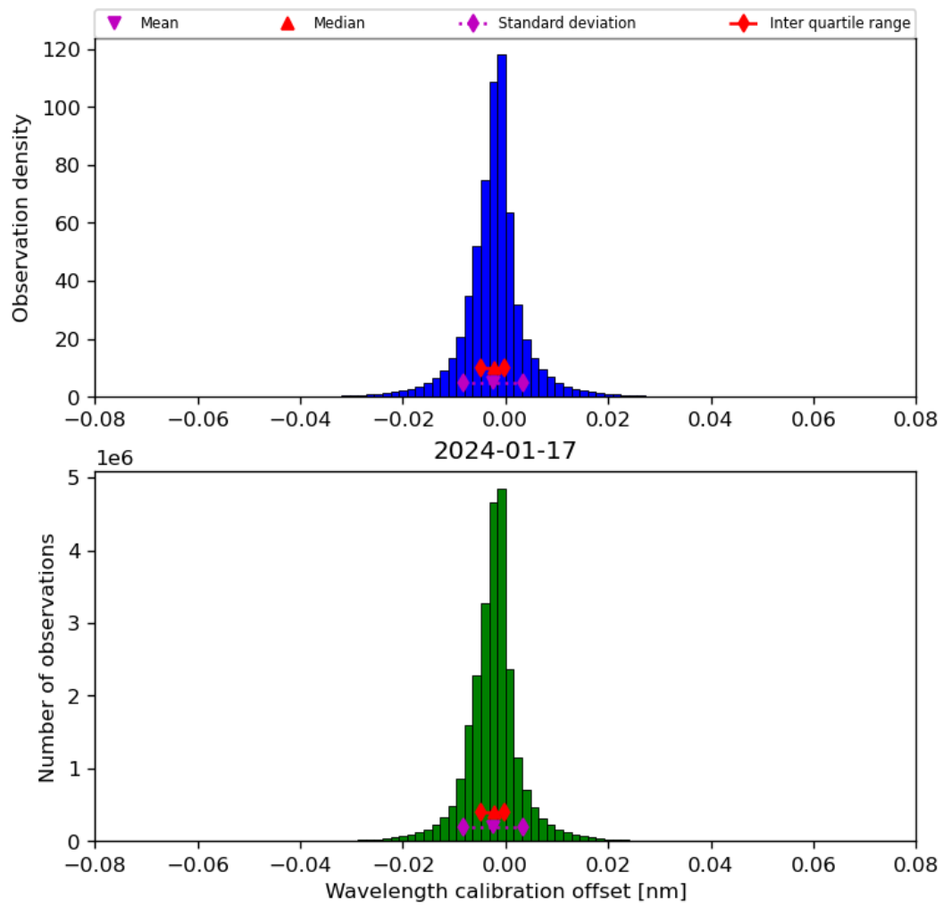
Figure 35: Histogram of “Wavelength calibration offset” for 2024-01-16 to 2024-01-18
