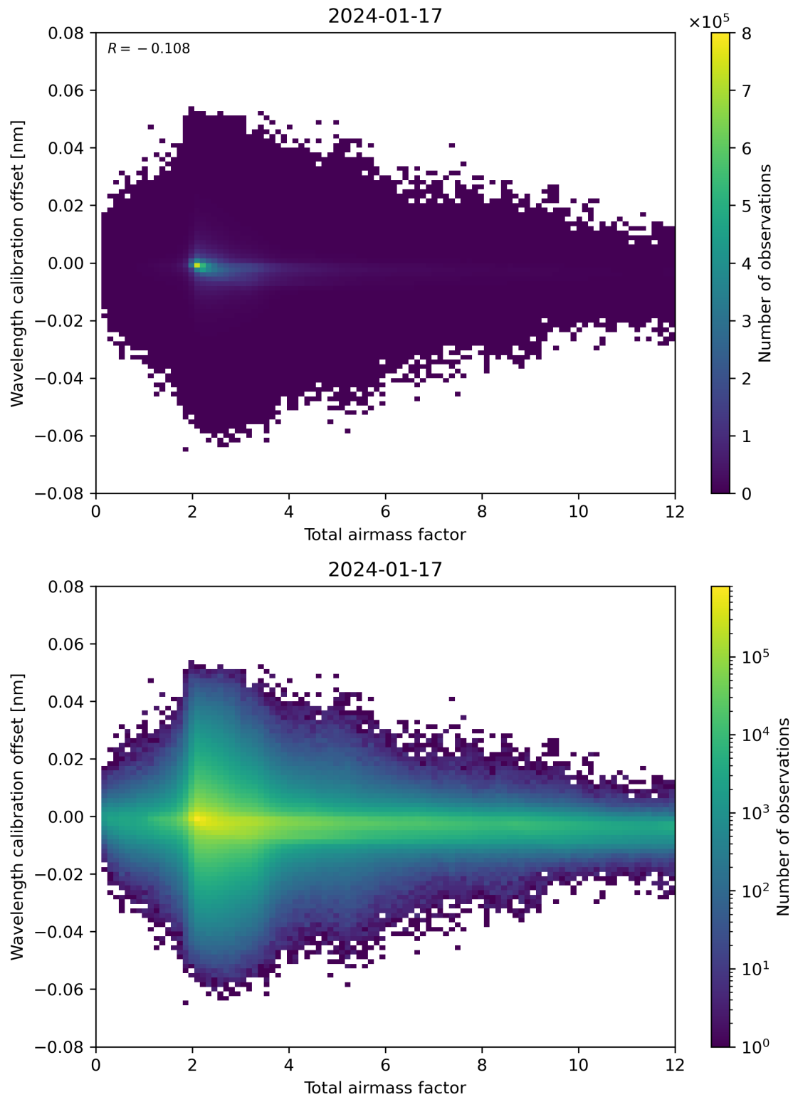
Figure 70: Scatter density plot of “Total airmass factor” against “Wavelength calibration offset” for 2024-01-16 to 2024-01-18.
