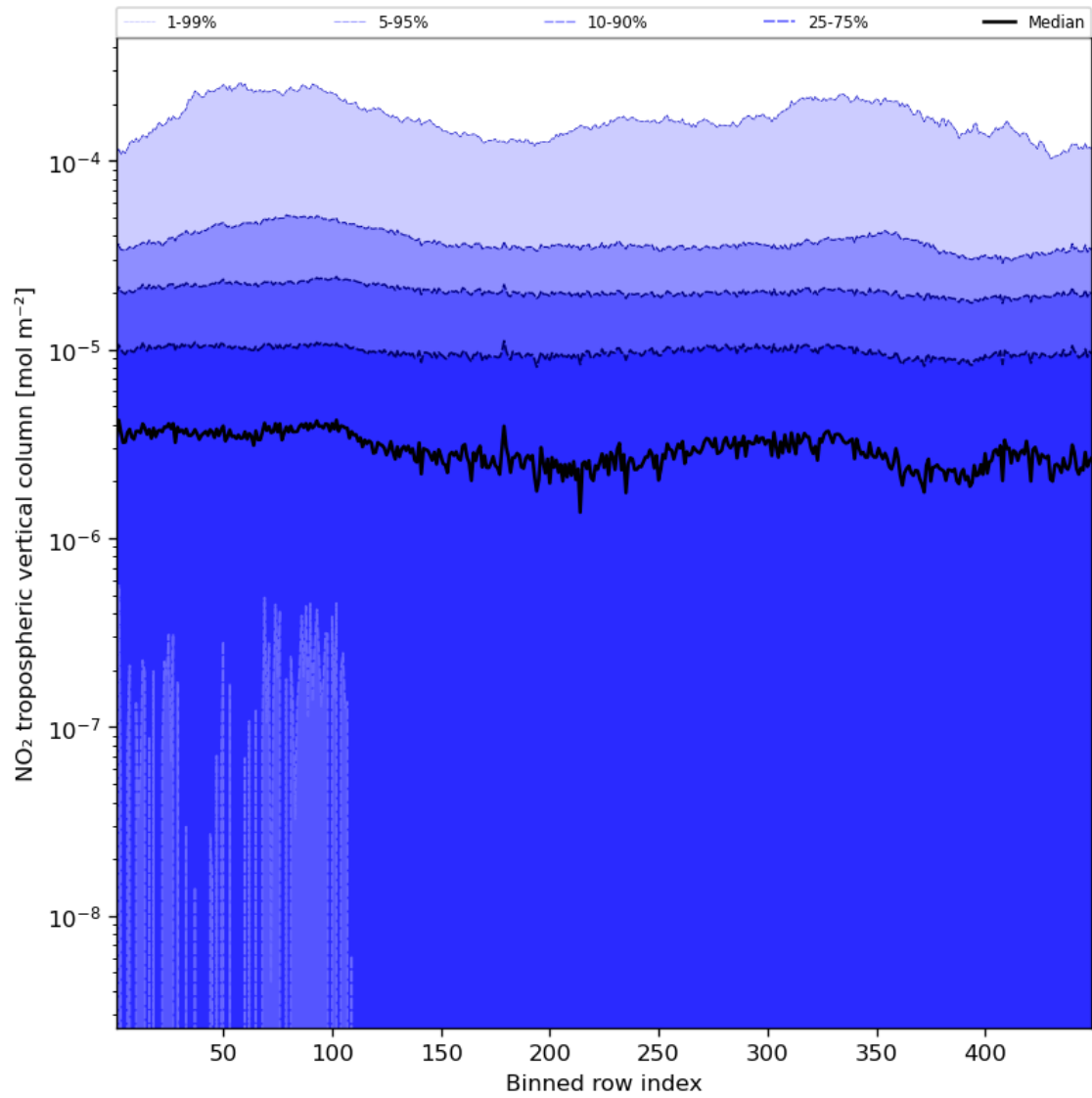
Figure 46: Along track statistics of “NO 2 tropospheric vertical column” for 2024-01-16 to 2024-01-18
