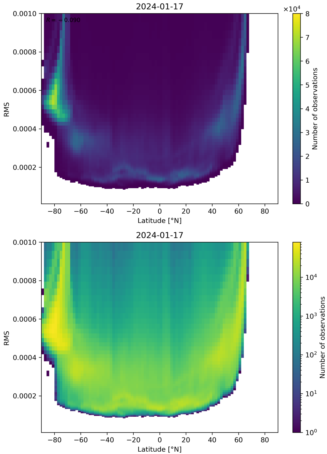
Figure 94: Scatter density plot of “Latitude” against “RMS” for 2024-01-16 to 2024-01-18.
