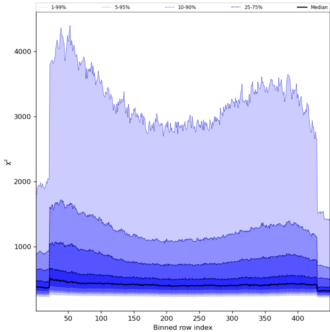
Figure 59: Along track statistics of “ \chi^2 ” for 2024-01-16 to 2024-01-18
