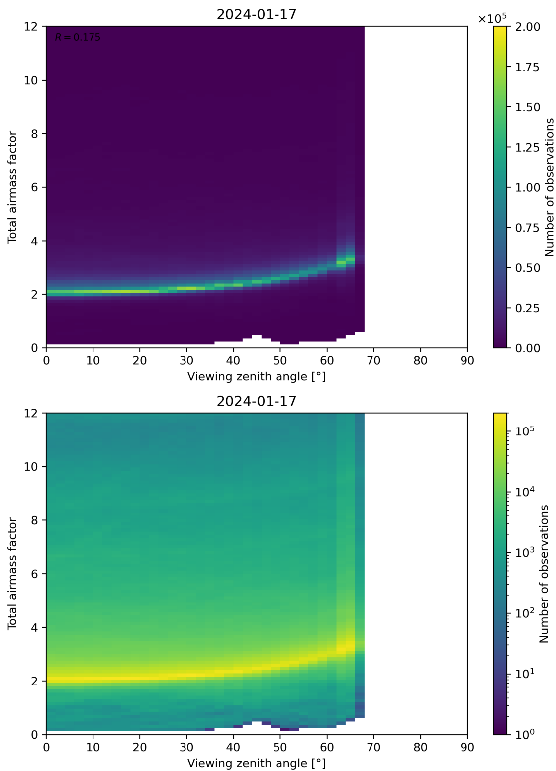
Figure 160: Scatter density plot of “Viewing zenith angle” against “Total airmass factor” for 2024-01-16 to 2024-01-18.
