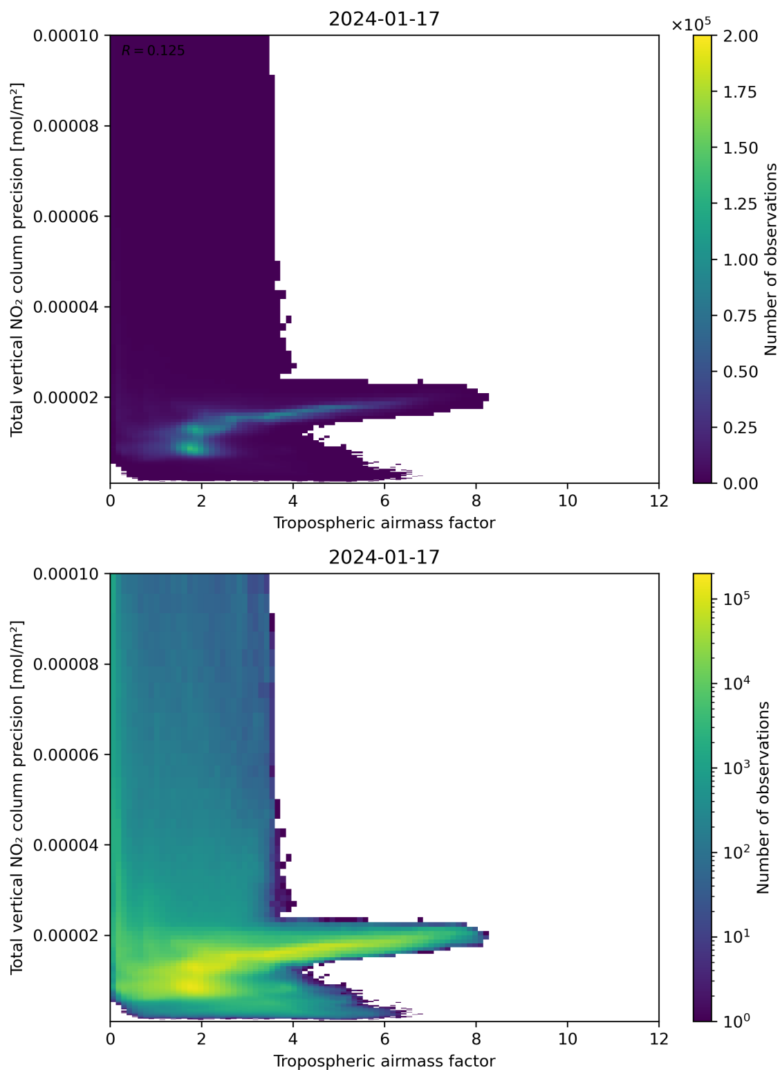
Figure 78: Scatter density plot of “Tropospheric air mass factor” against “Total vertical NO 2 column precision” for 2024-01-16 to 2024-01-18.
