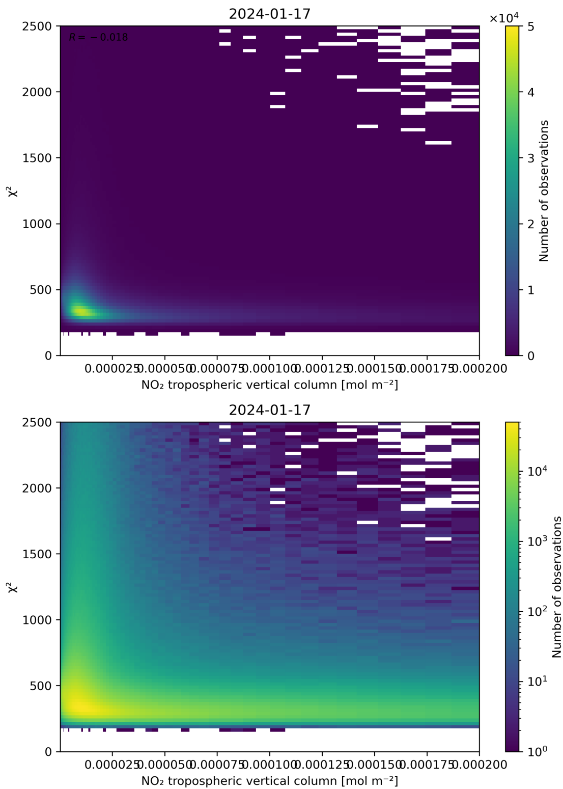
Figure 124: Scatter density plot of “NO 2 tropospheric vertical column” against “ \chi^2 ” for 2024-01-16 to 2024-01-18.
