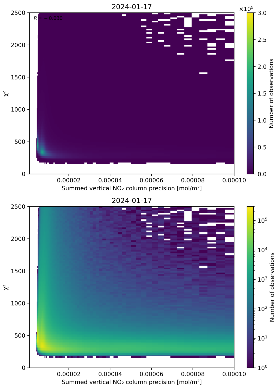
Figure 107: Scatter density plot of “Summed vertical NO 2 column precision” against “ \chi^2 ” for 2024-01-16 to 2024-01-18.
