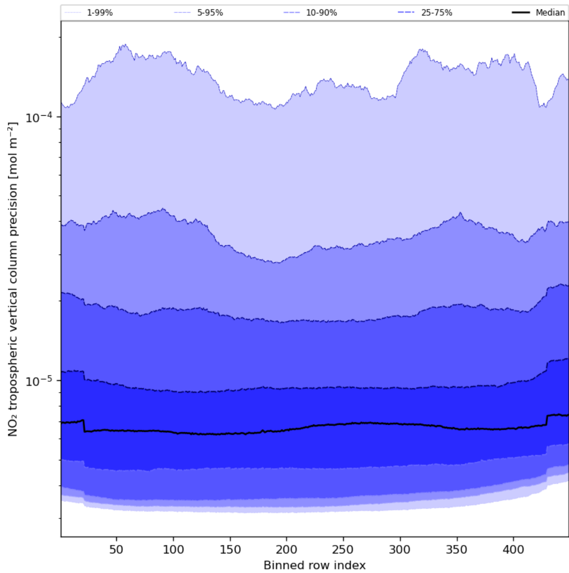
Figure 47: Along track statistics of “NO 2 tropospheric vertical column precision” for 2024-01-16 to 2024-01-18
