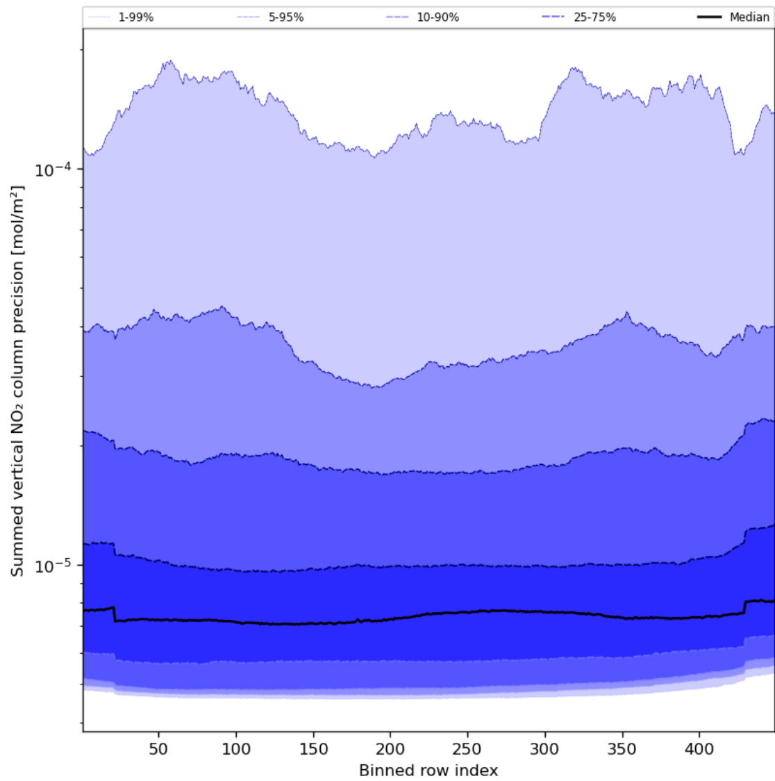
Figure 58: Along track statistics of “Summed vertical NO 2 column precision” for 2024-01-16 to 2024-01-18
