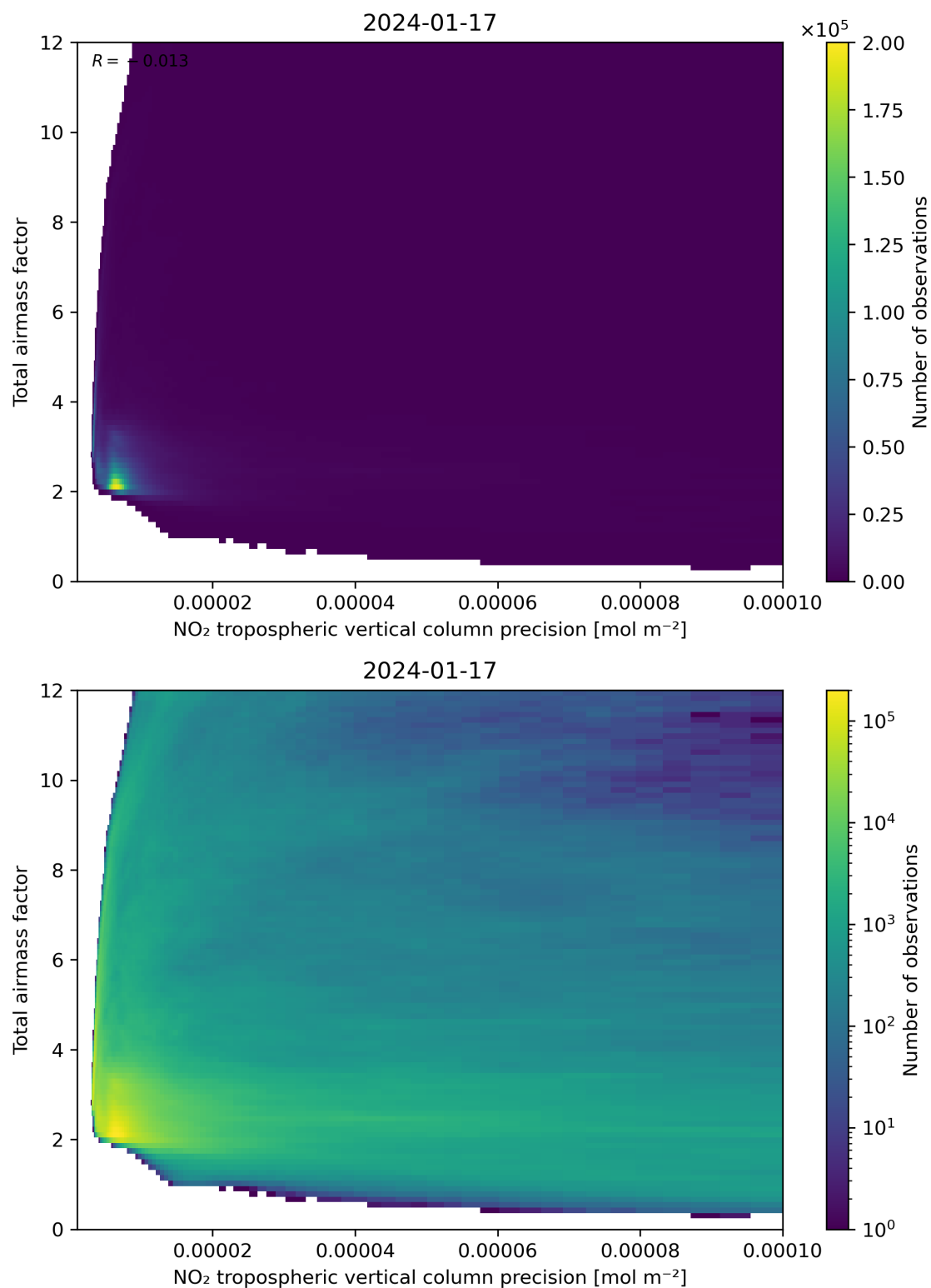
Figure 132: Scatter density plot of “NO 2 tropospheric vertical column precision” against “Total air mass factor” for 2024-01-16 to 2024-01-18.
