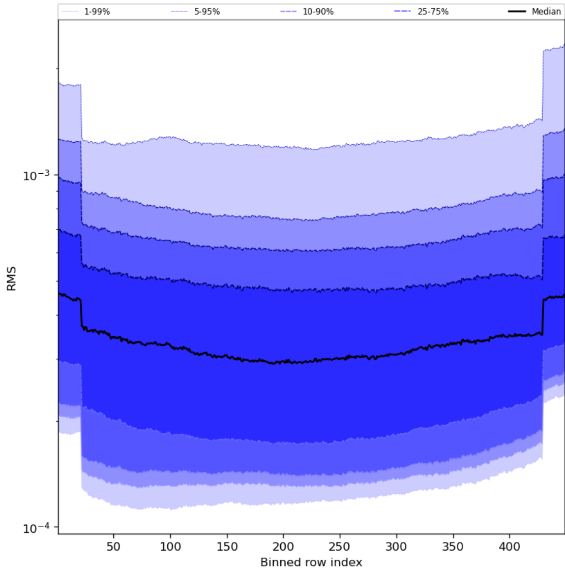
Figure 60: Along track statistics of “RMS” for 2024-01-16 to 2024-01-18
