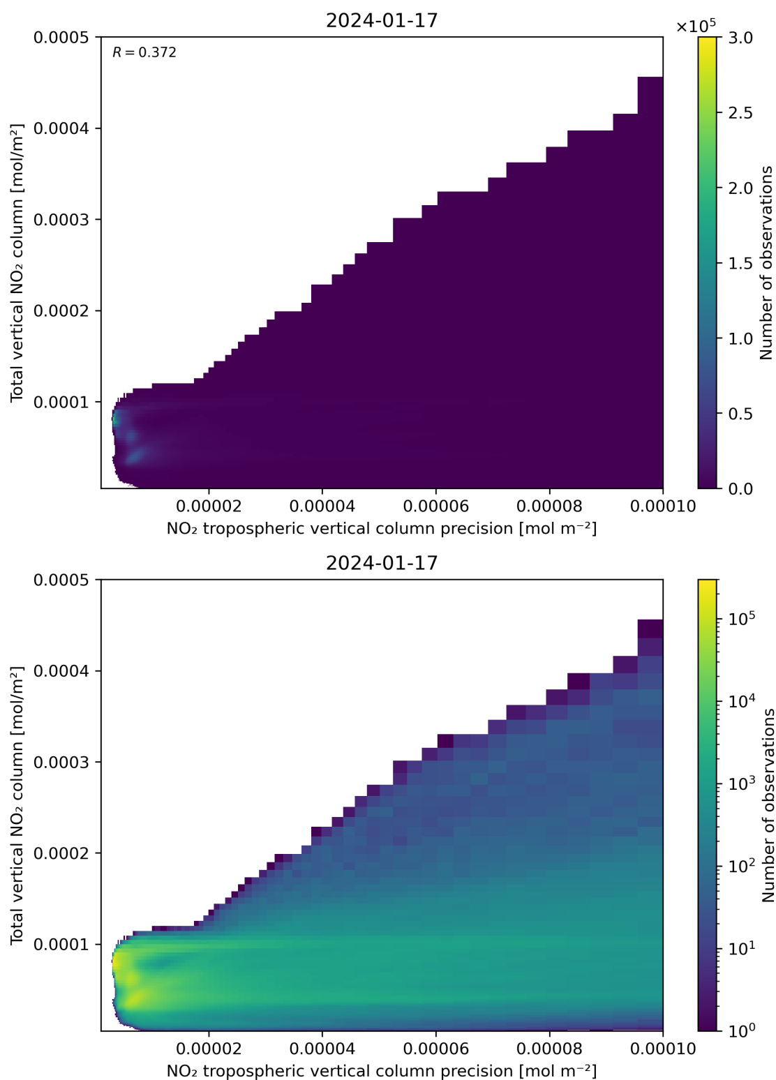
Figure 138: Scatter density plot of “NO 2 tropospheric vertical column precision” against “Total vertical NO 2 column” for 2024-01-16 to 2024-01-18.
