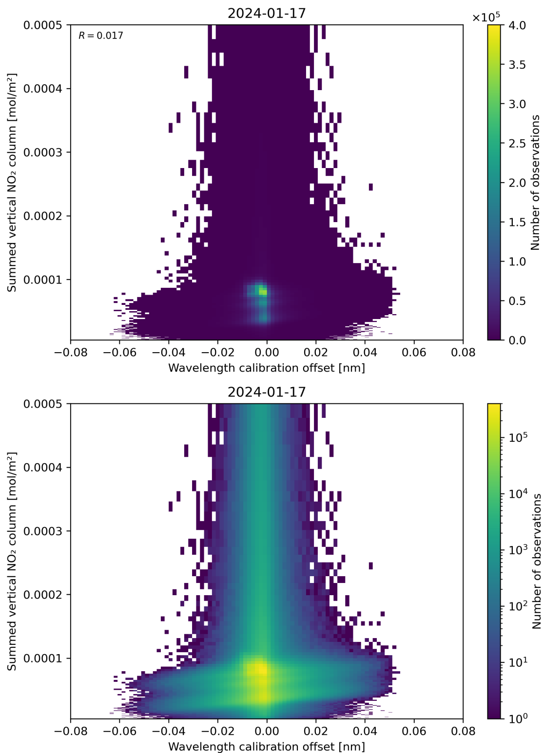
Figure 177: Scatter density plot of “Wavelength calibration offset” against “Summed vertical NO 2 column” for 2024-01-16 to 2024-01-18.
