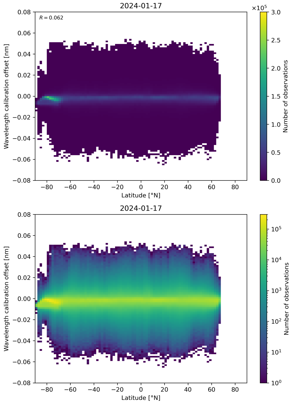
Figure 95: Scatter density plot of “Latitude” against “Wavelength calibration offset” for 2024-01-16 to 2024-01-18.
