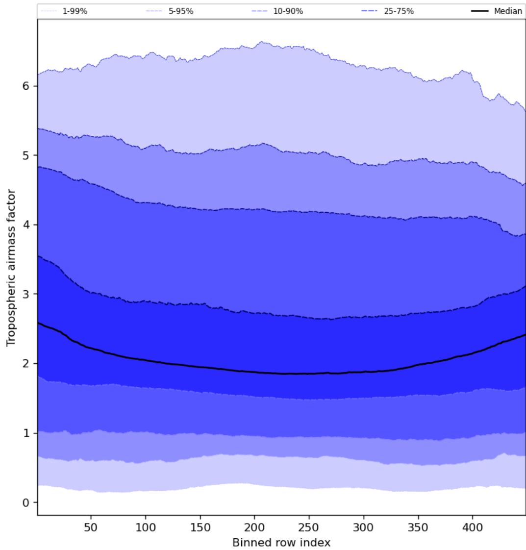
Figure 48: Along track statistics of “Tropospheric airmass factor” for 2024-01-16 to 2024-01-18
