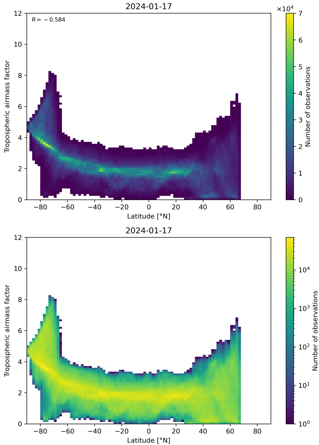
Figure 85: Scatter density plot of “Latitude” against “Tropospheric airmass factor” for 2024-01-16 to 2024-01-18.
