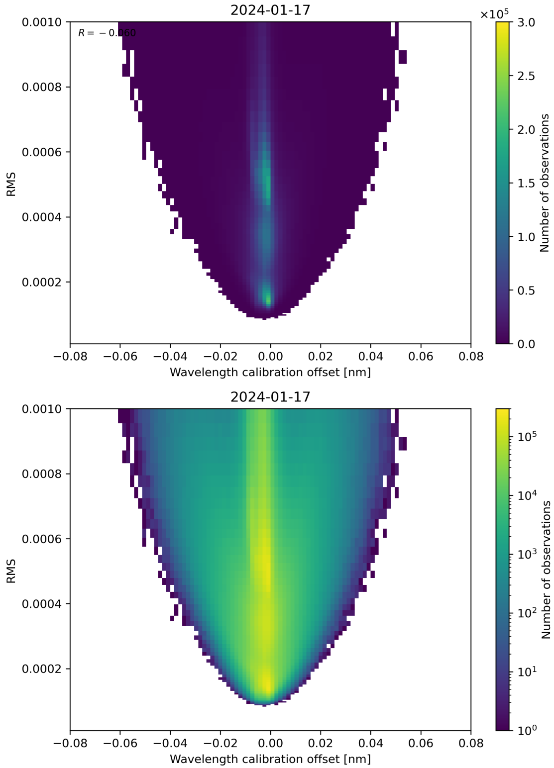
Figure 181: Scatter density plot of “Wavelength calibration offset” against “RMS” for 2024-01-16 to 2024-01-18.
