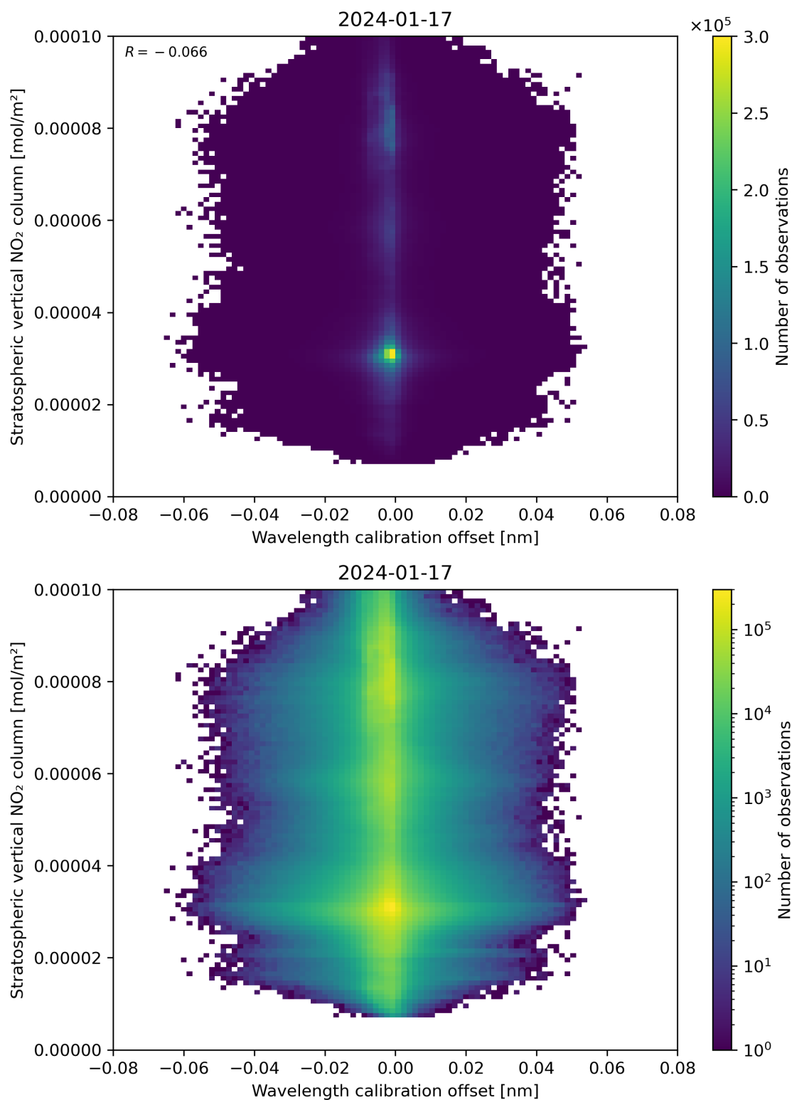
Figure 176: Scatter density plot of “Wavelength calibration offset” against “Stratospheric vertical NO 2 column” for 2024-01-16 to 2024-01-18.
