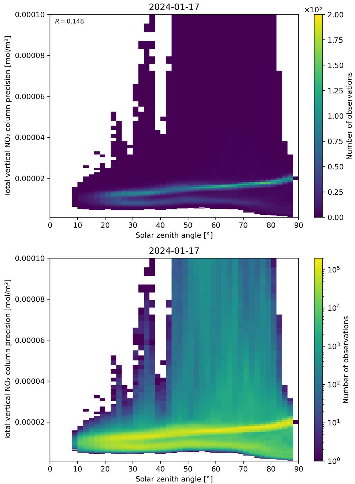
Figure 154: Scatter density plot of “Solar zenith angle” against “Total vertical NO 2 column precision” for 2024-01-16 to 2024-01-18.
