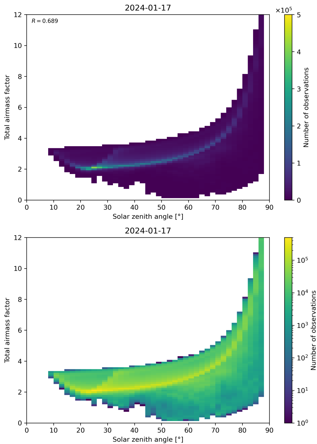
Figure 146: Scatter density plot of “Solar zenith angle” against “Total air mass factor” for 2024-01-16 to 2024-01-18.
