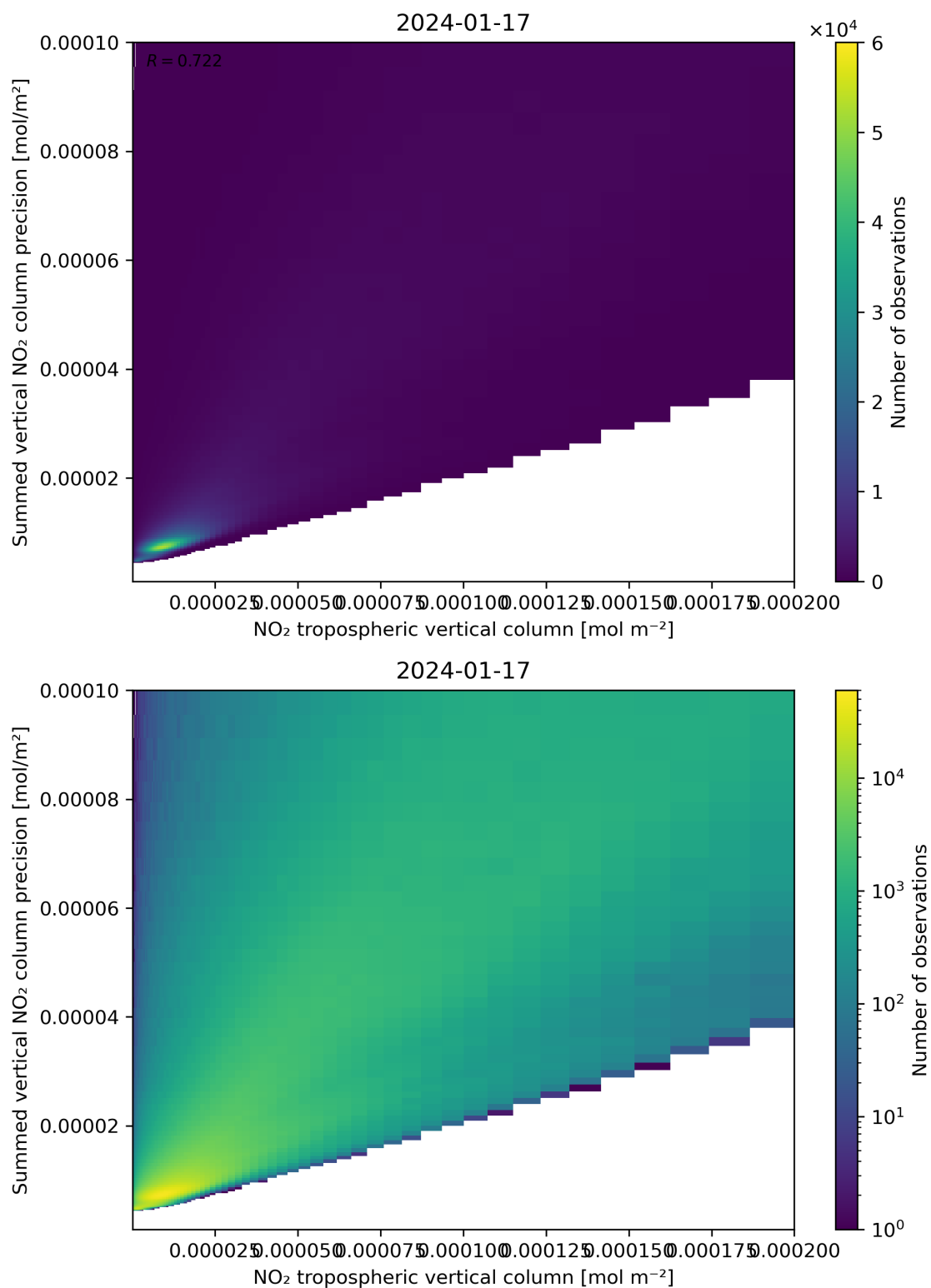
Figure 127: Scatter density plot of “NO 2 tropospheric vertical column” against “Summed vertical NO 2 column precision” for 2024-01-16 to 2024-01-18.
