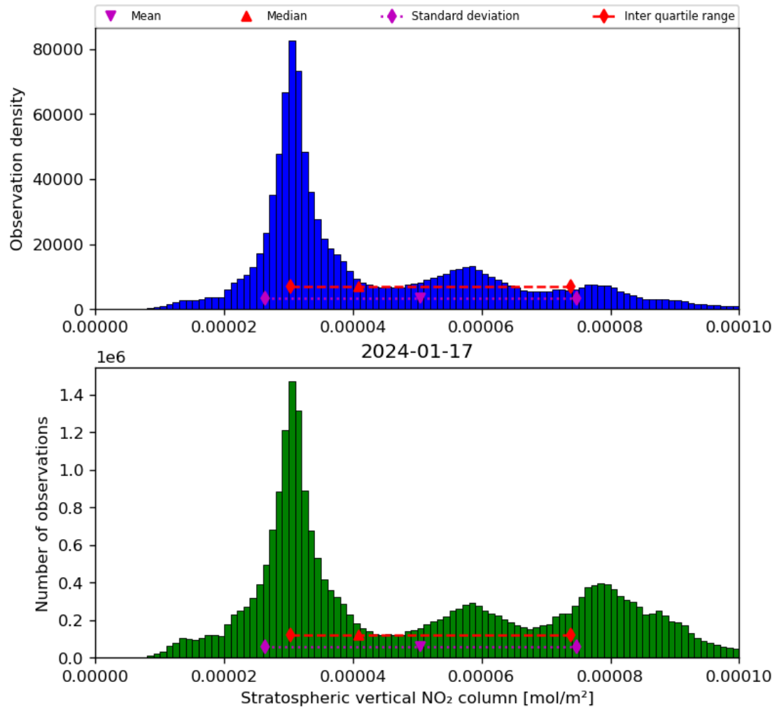
Figure 36: Histogram of “Stratospheric vertical NO 2 column” for 2024-01-16 to 2024-01-18
