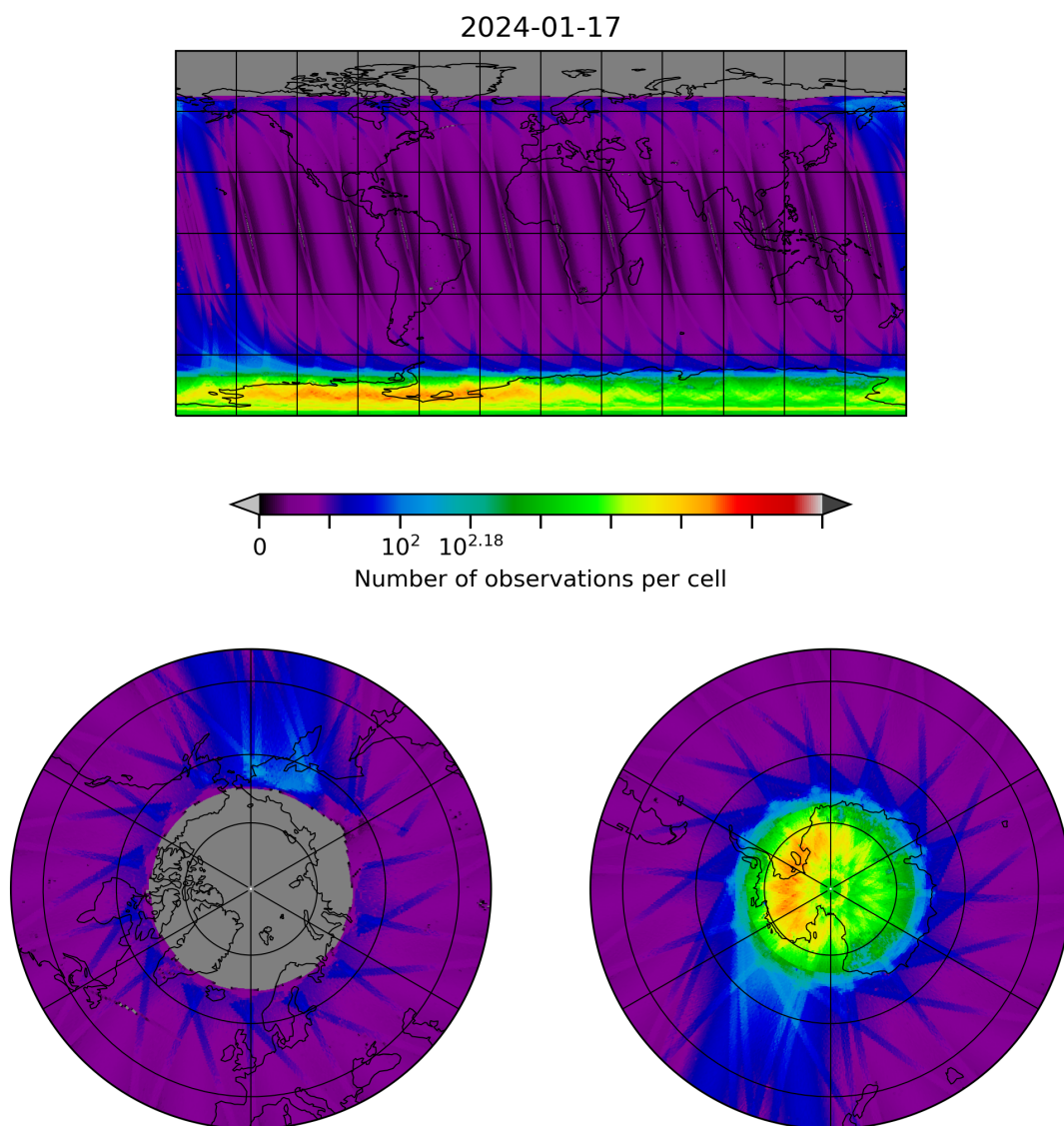
Figure 10: Map of the number of observations for 2024-01-16 to 2024-01-18
