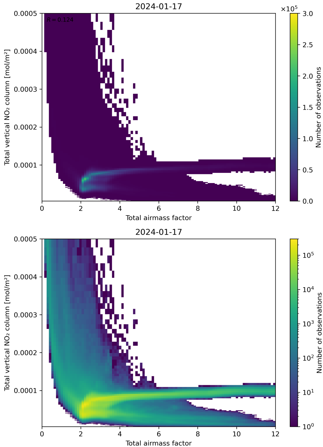
Figure 67: Scatter density plot of “Total airmass factor” against “Total vertical NO 2 column” for 2024-01-16 to 2024-01-18.
