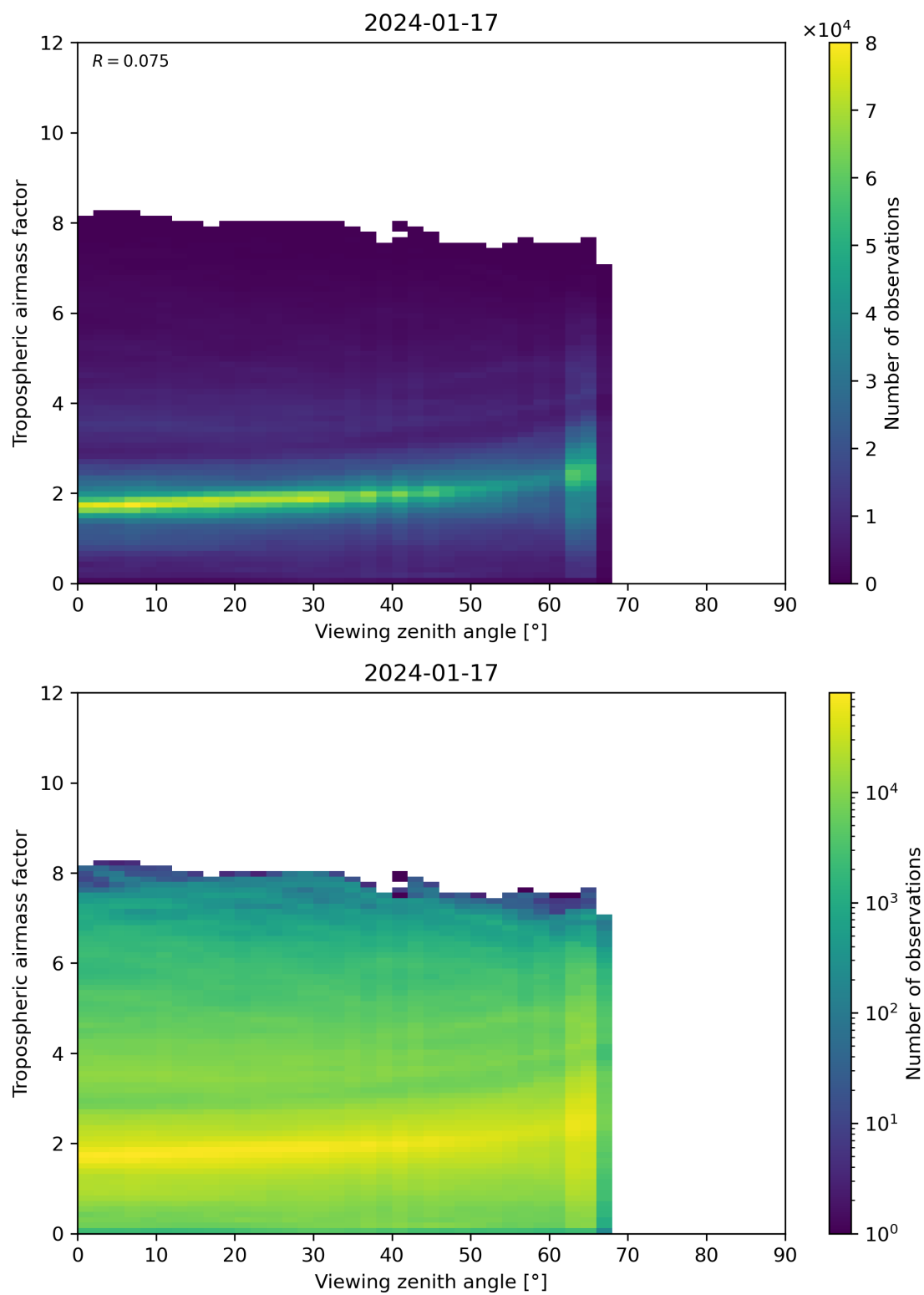
Figure 161: Scatter density plot of “Viewing zenith angle” against “Tropospheric airmass factor” for 2024-01-16 to 2024-01-18.
