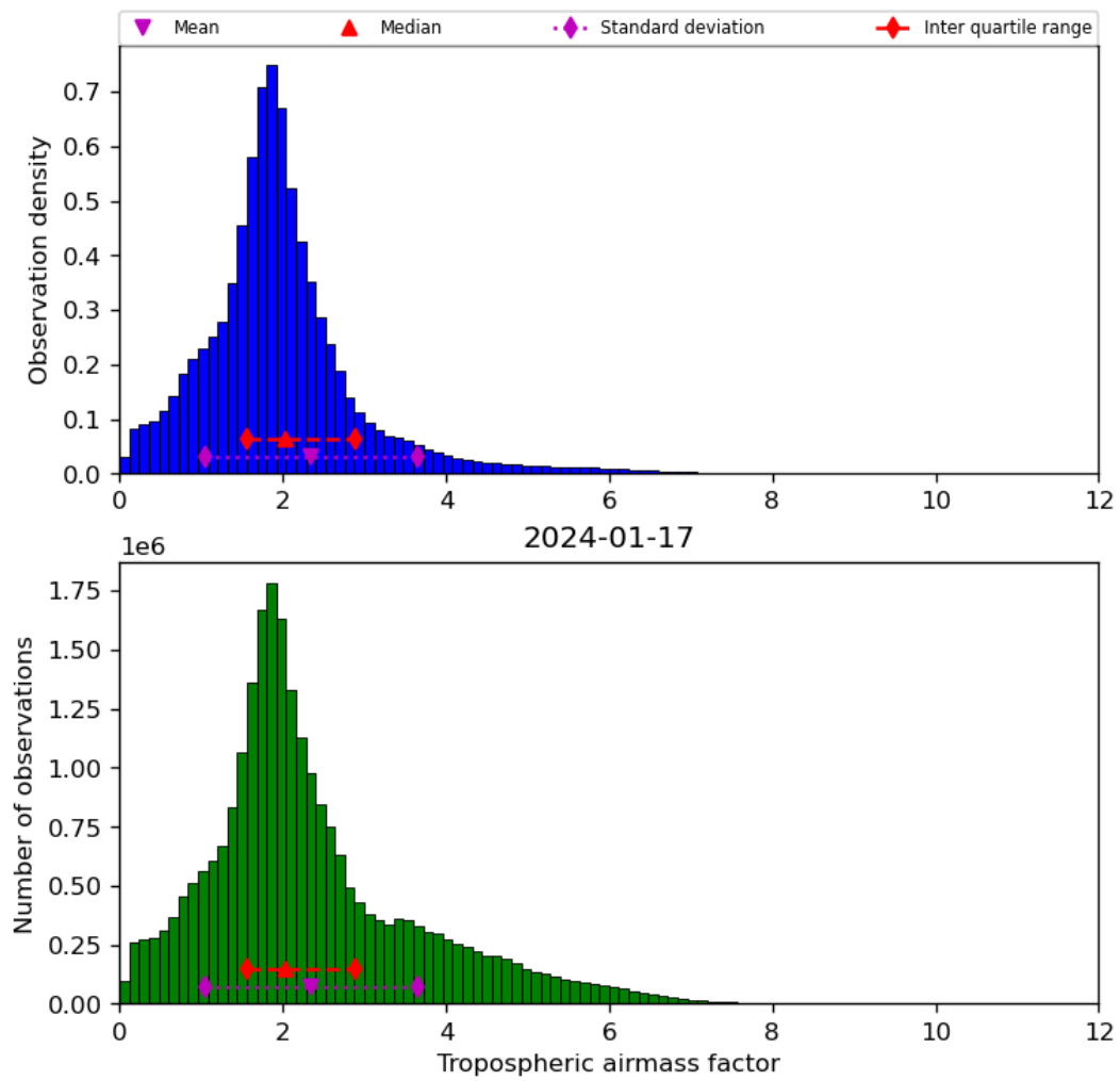
Figure 31: Histogram of “Tropospheric airmass factor” for 2024-01-16 to 2024-01-18
