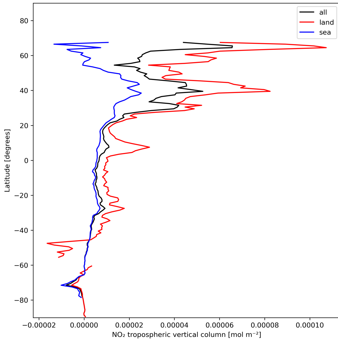
Figure 12: Zonal average of “NO 2 tropospheric vertical column” for 2024-01-16 to 2024-01-18.
