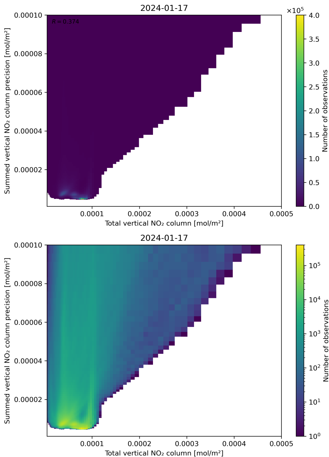
Figure 113: Scatter density plot of “Total vertical NO 2 column” against “Summed vertical NO 2 column precision” for 2024-01-16 to 2024-01-18.
