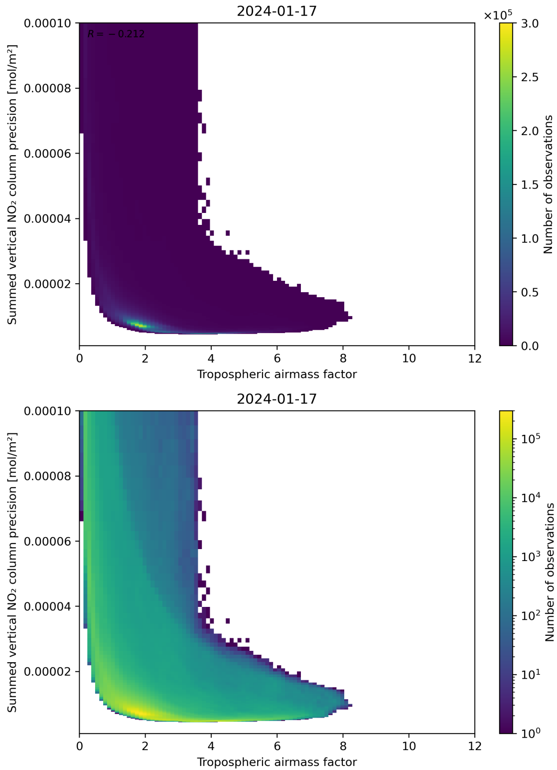
Figure 76: Scatter density plot of “Tropospheric air mass factor” against “Summed vertical NO 2 column precision” for 2024-01-16 to 2024-01-18.
