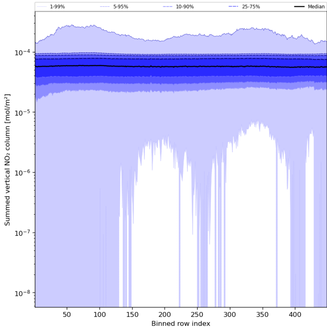
Figure 57: Along track statistics of “Summed vertical NO 2 column” for 2024-01-16 to 2024-01-18
