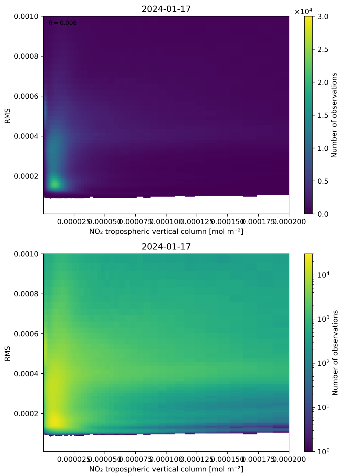
Figure 142: Scatter density plot of “NO 2 tropospheric vertical column” against “RMS” for 2024-01-16 to 2024-01-18.
