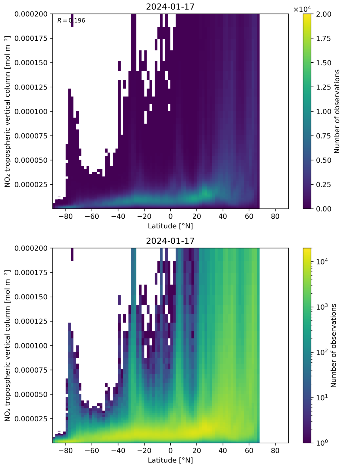
Figure 92: Scatter density plot of “Latitude” against “NO 2 tropospheric vertical column” for 2024-01-16 to 2024-01-18.
