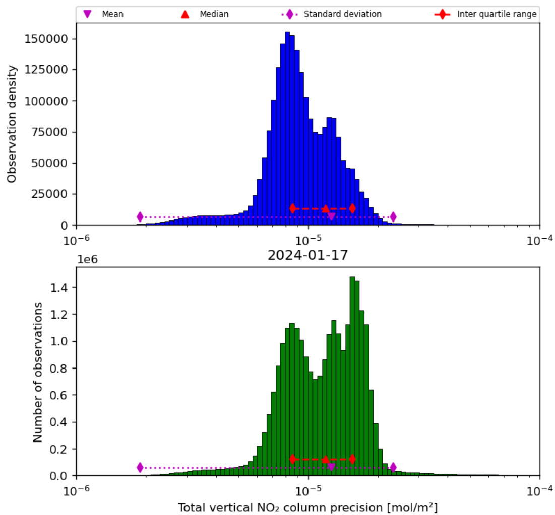
Figure 39: Histogram of “Total vertical NO 2 column precision” for 2024-01-16 to 2024-01-18
