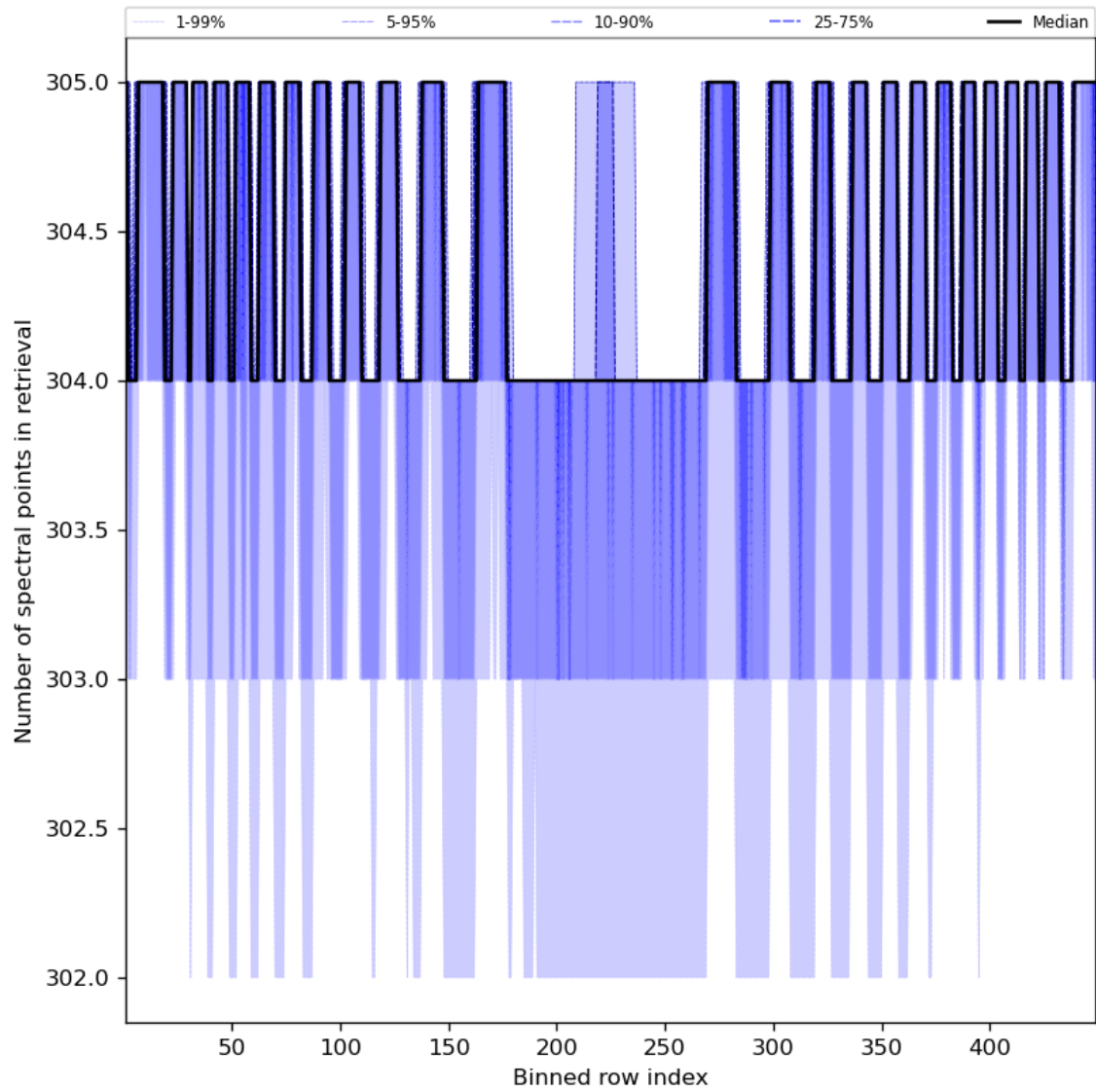
Figure 50: Along track statistics of “Number of spectral points in retrieval” for 2024-01-16 to 2024-01-18
