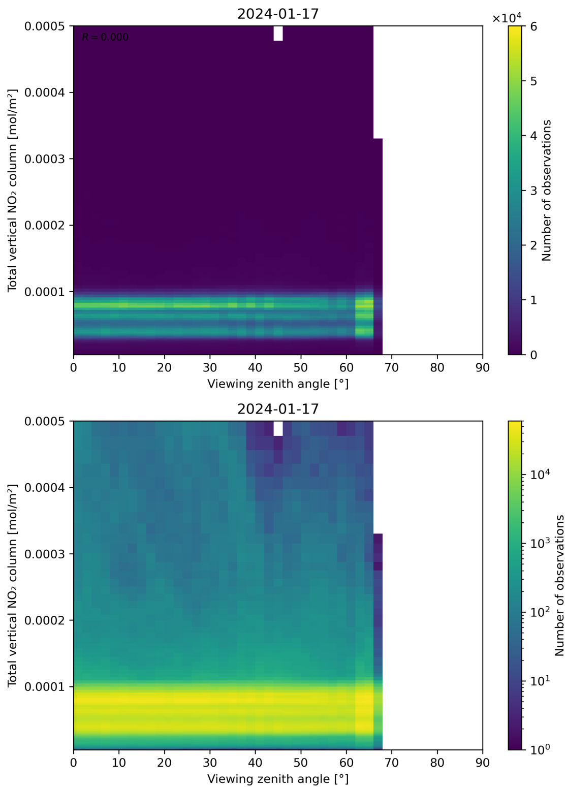
Figure 167: Scatter density plot of “Viewing zenith angle” against “Total vertical NO 2 column” for 2024-01-16 to 2024-01-18.
