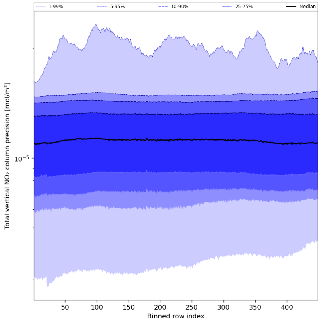
Figure 56: Along track statistics of “Total vertical NO 2 column precision” for 2024-01-16 to 2024-01-18
