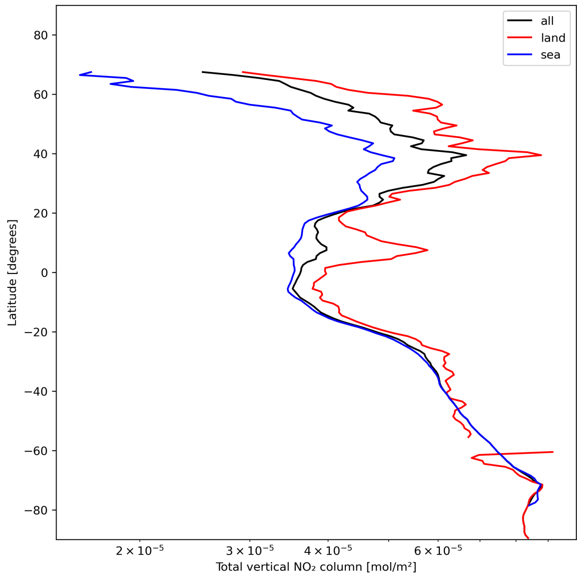
Figure 21: Zonal average of “Total vertical NO 2 column” for 2024-01-16 to 2024-01-18.
