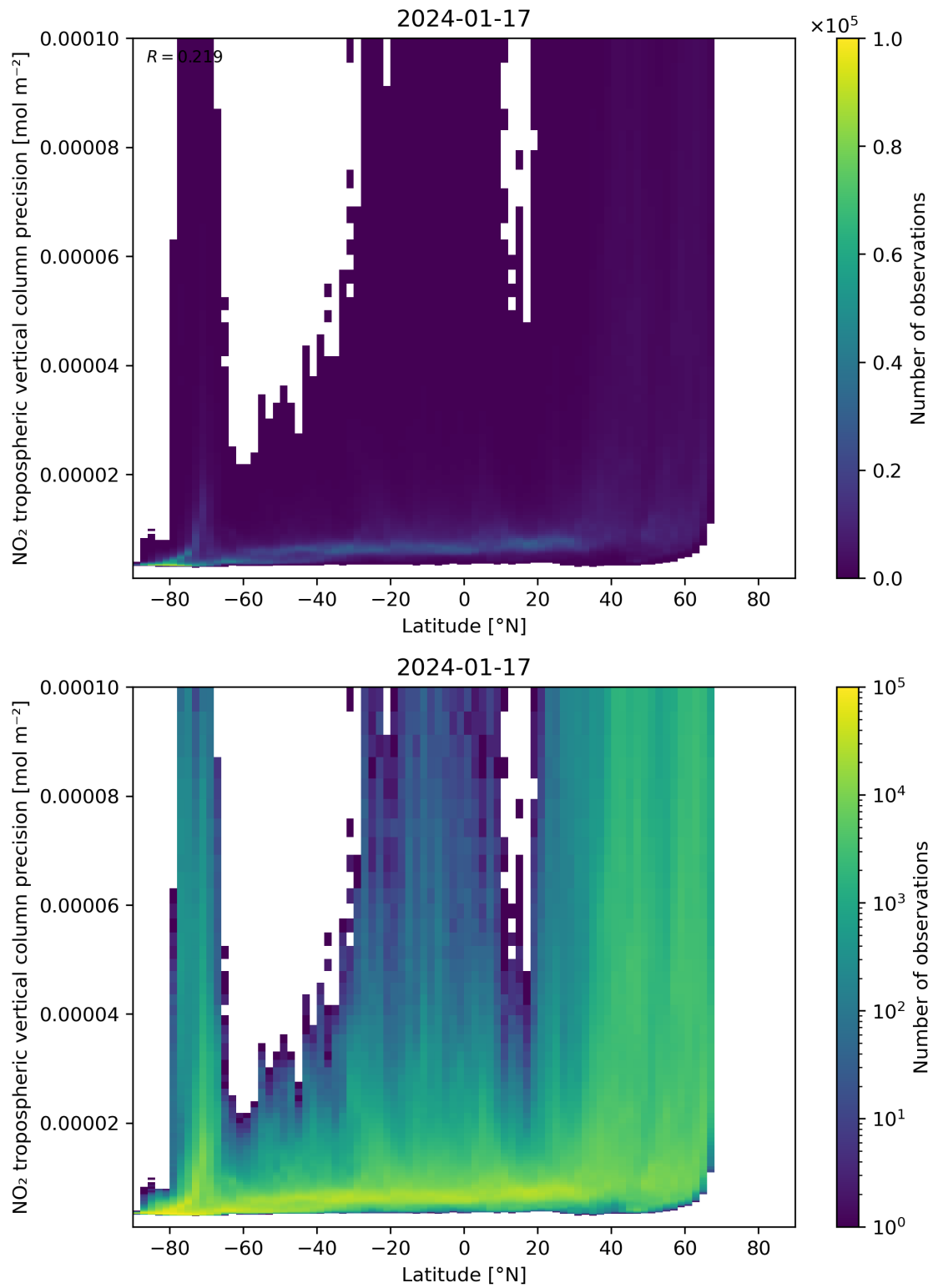
Figure 93: Scatter density plot of “Latitude” against “NO 2 tropospheric vertical column precision” for 2024-01-16 to 2024-01-18.
