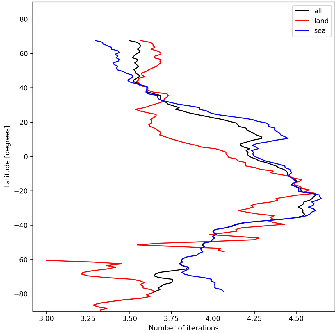
Figure 17: Zonal average of “Number of iterations” for 2024-01-16 to 2024-01-18.
