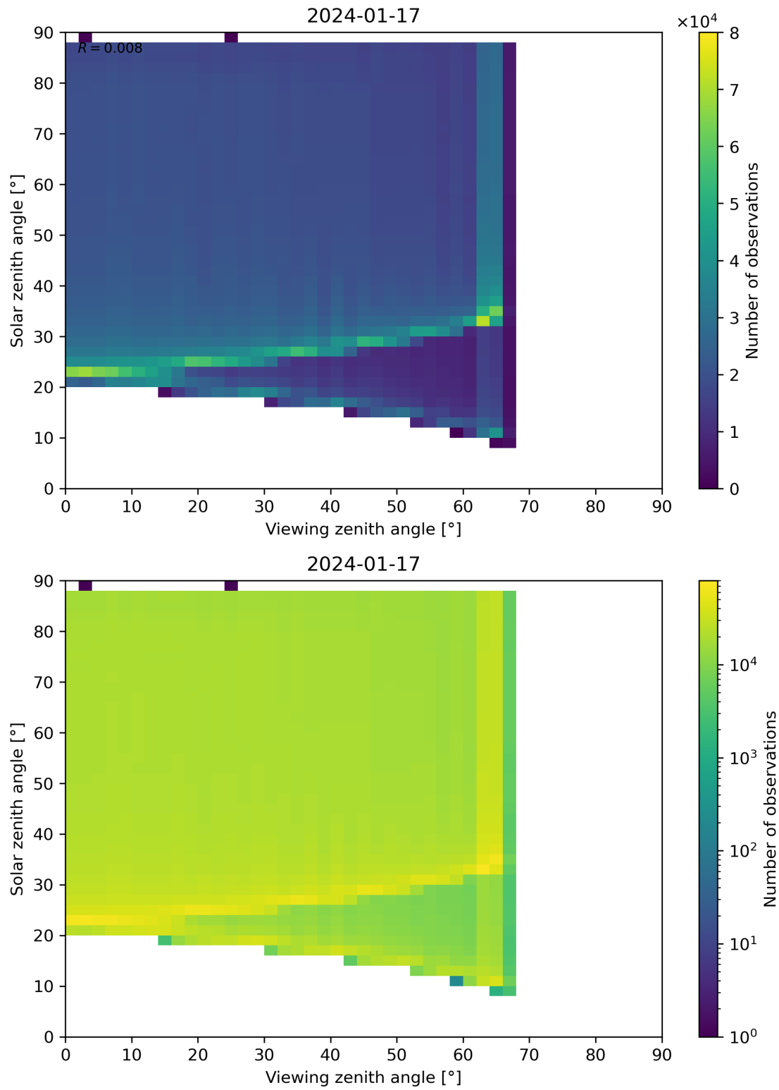
Figure 172: Scatter density plot of “Viewing zenith angle” against “Solar zenith angle” for 2024-01-16 to 2024-01-18.
