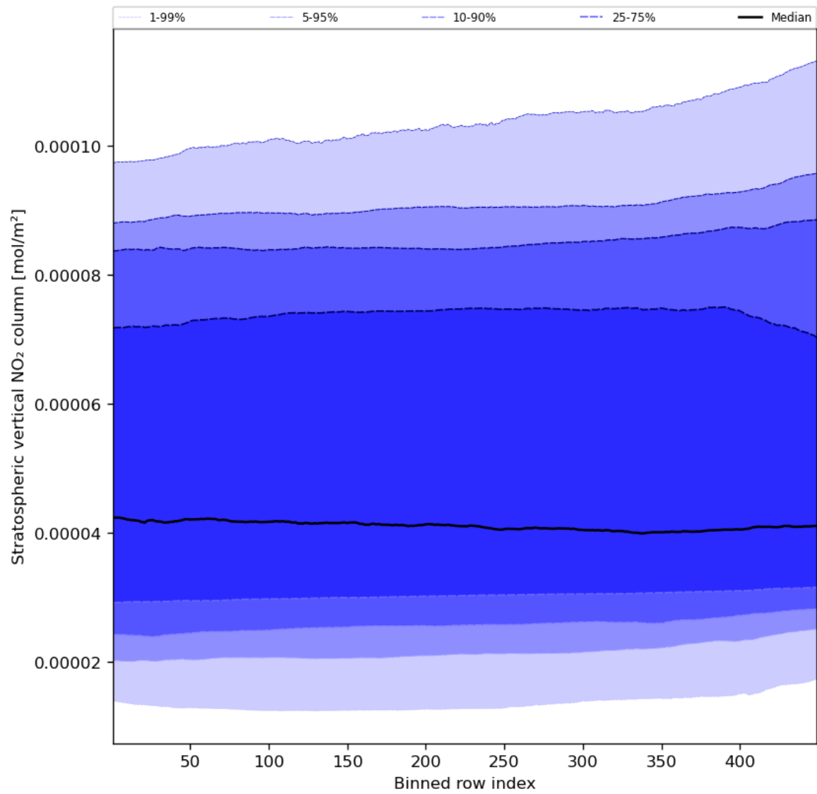
Figure 53: Along track statistics of “Stratospheric vertical NO 2 column” for 2024-01-16 to 2024-01-18
