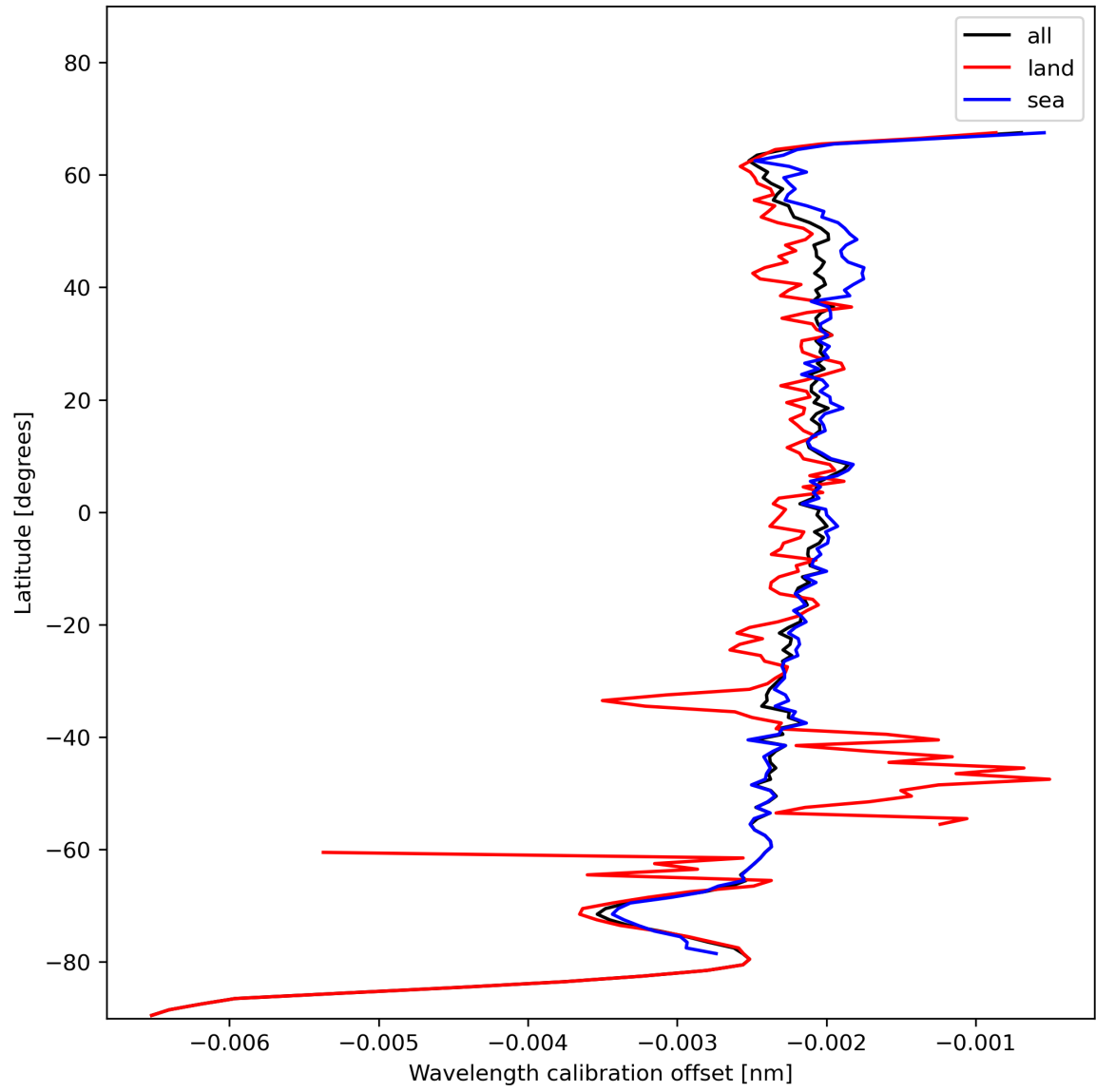
Figure 18: Zonal average of “Wavelength calibration offset” for 2024-01-16 to 2024-01-18.
