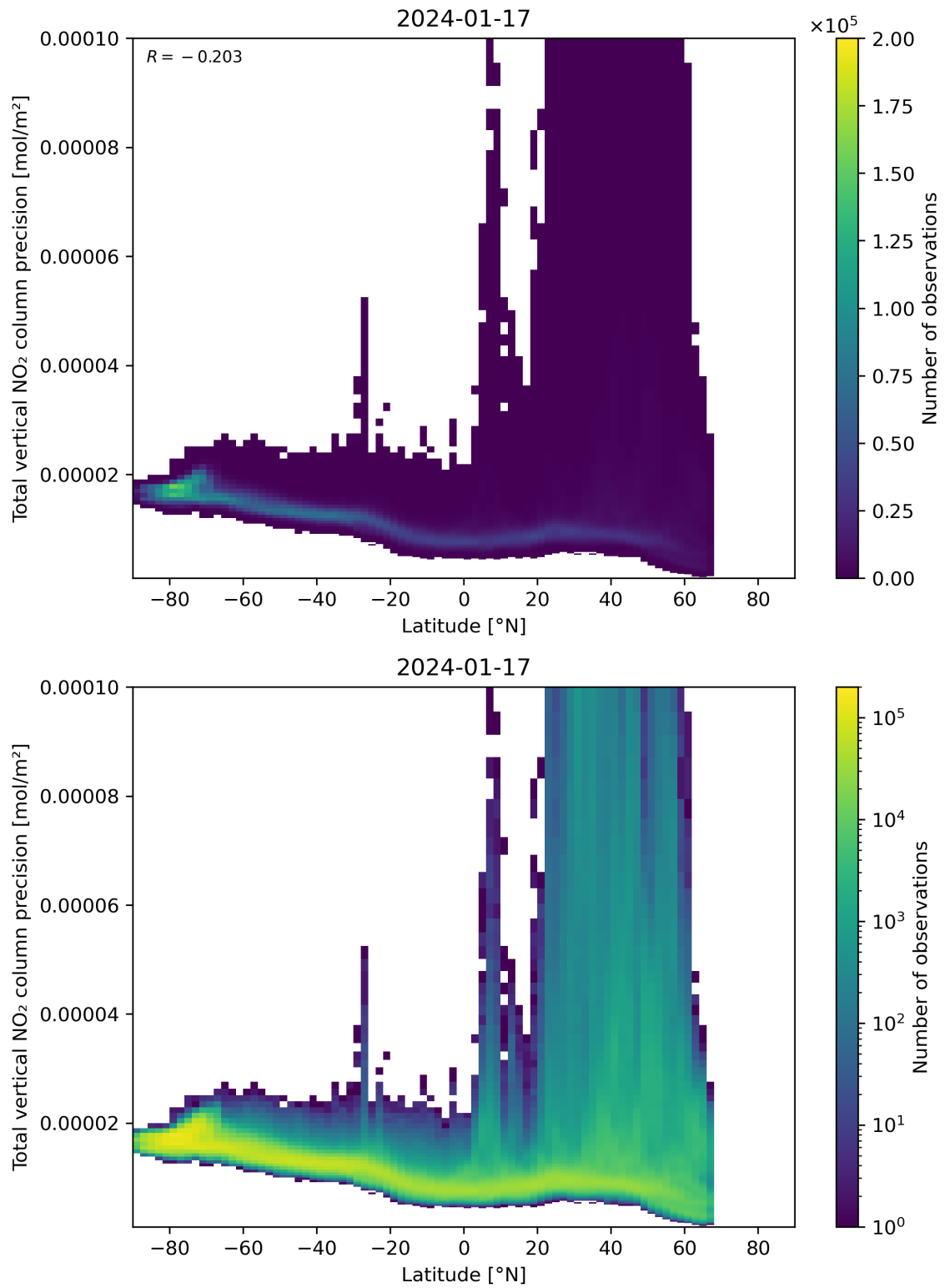
Figure 91: Scatter density plot of “Latitude” against “Total vertical NO 2 column precision” for 2024-01-16 to 2024-01-18.
