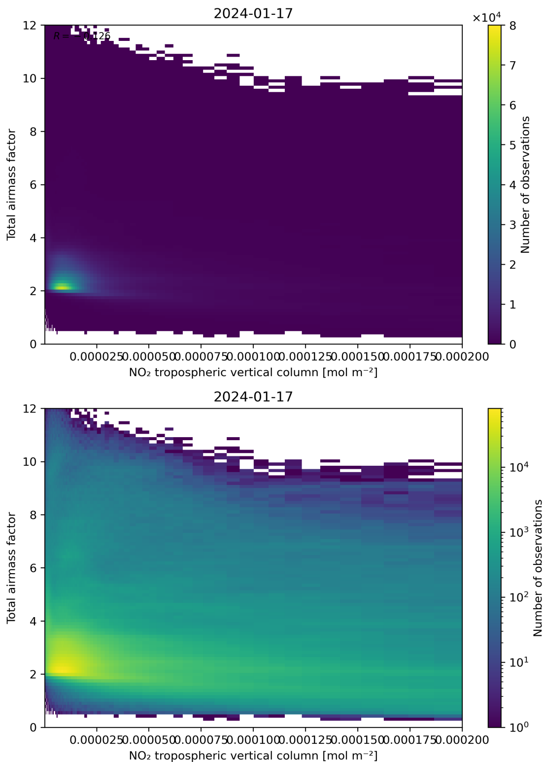
Figure 122: Scatter density plot of “NO 2 tropospheric vertical column” against “Total air mass factor” for 2024-01-16 to 2024-01-18.
