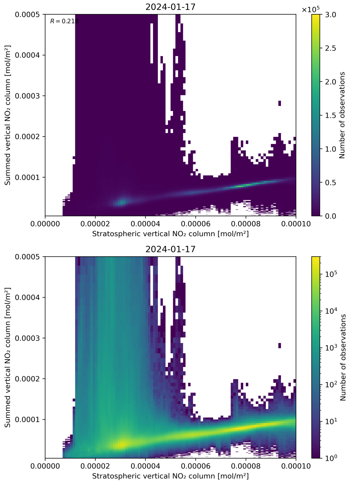
Figure 98: Scatter density plot of “Stratospheric vertical NO 2 column” against “Summed vertical NO 2 column” for 2024-01-16 to 2024-01-18.
