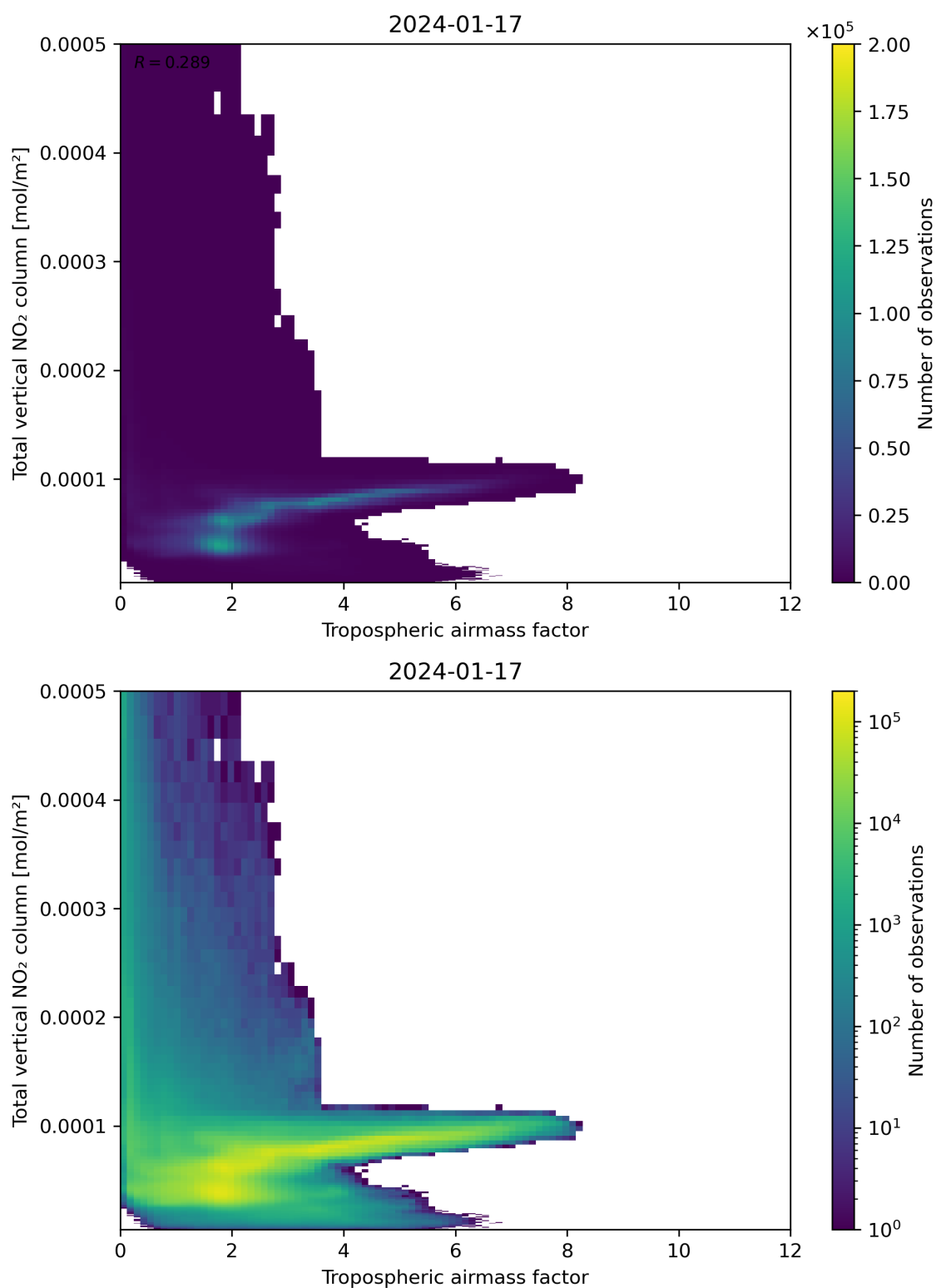
Figure 77: Scatter density plot of “Tropospheric airmass factor” against “Total vertical \text{NO}_2 column” for 2024-01-16 to 2024-01-18.
