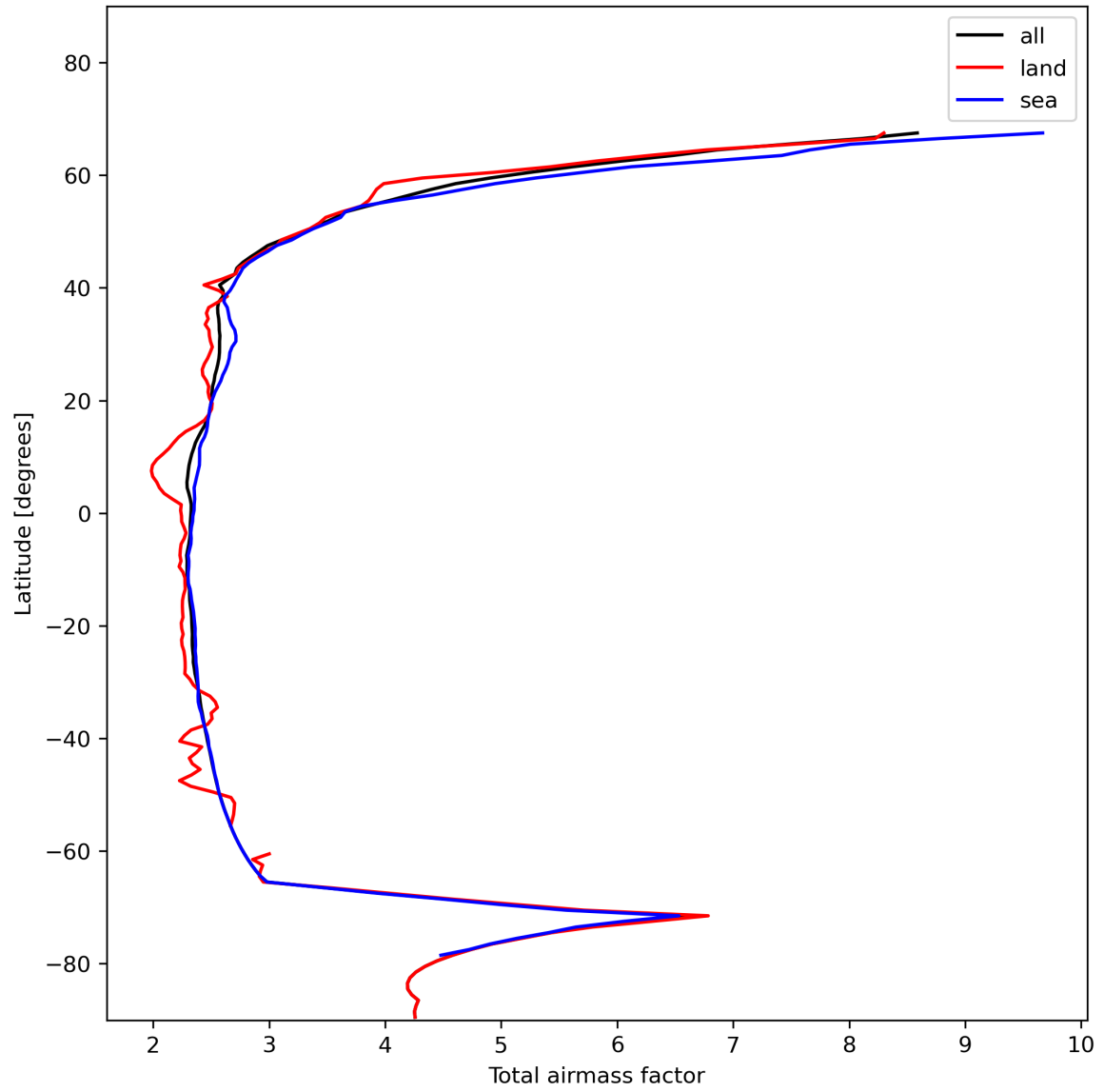
Figure 15: Zonal average of “Total airmass factor” for 2024-01-16 to 2024-01-18.
