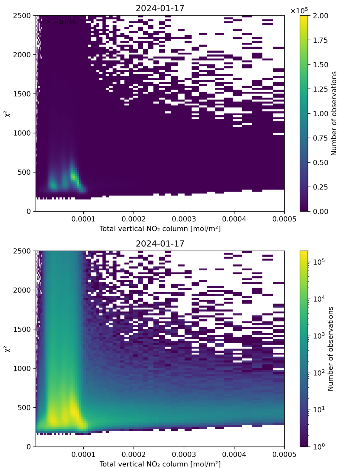
Figure 111: Scatter density plot of “Total vertical NO 2 column” against “ \chi^2 ” for 2024-01-16 to 2024-01-18.
