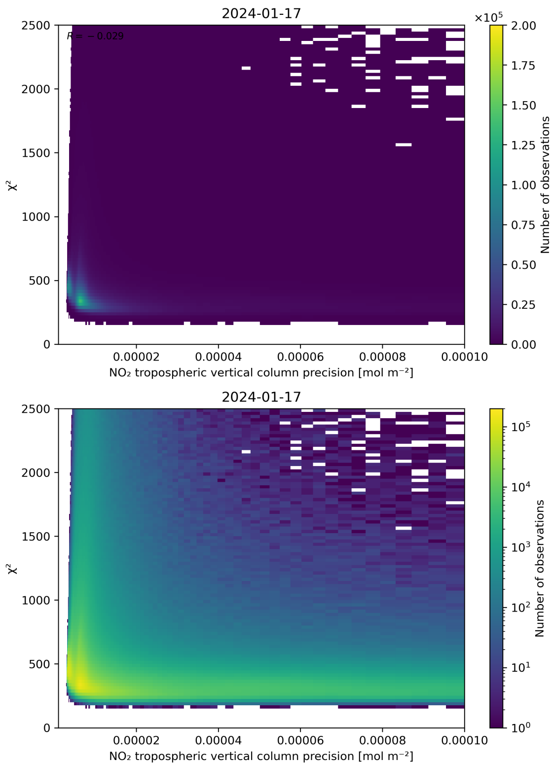
Figure 134: Scatter density plot of “NO 2 tropospheric vertical column precision” against “ \chi^2 ” for 2024-01-16 to 2024-01-18.
