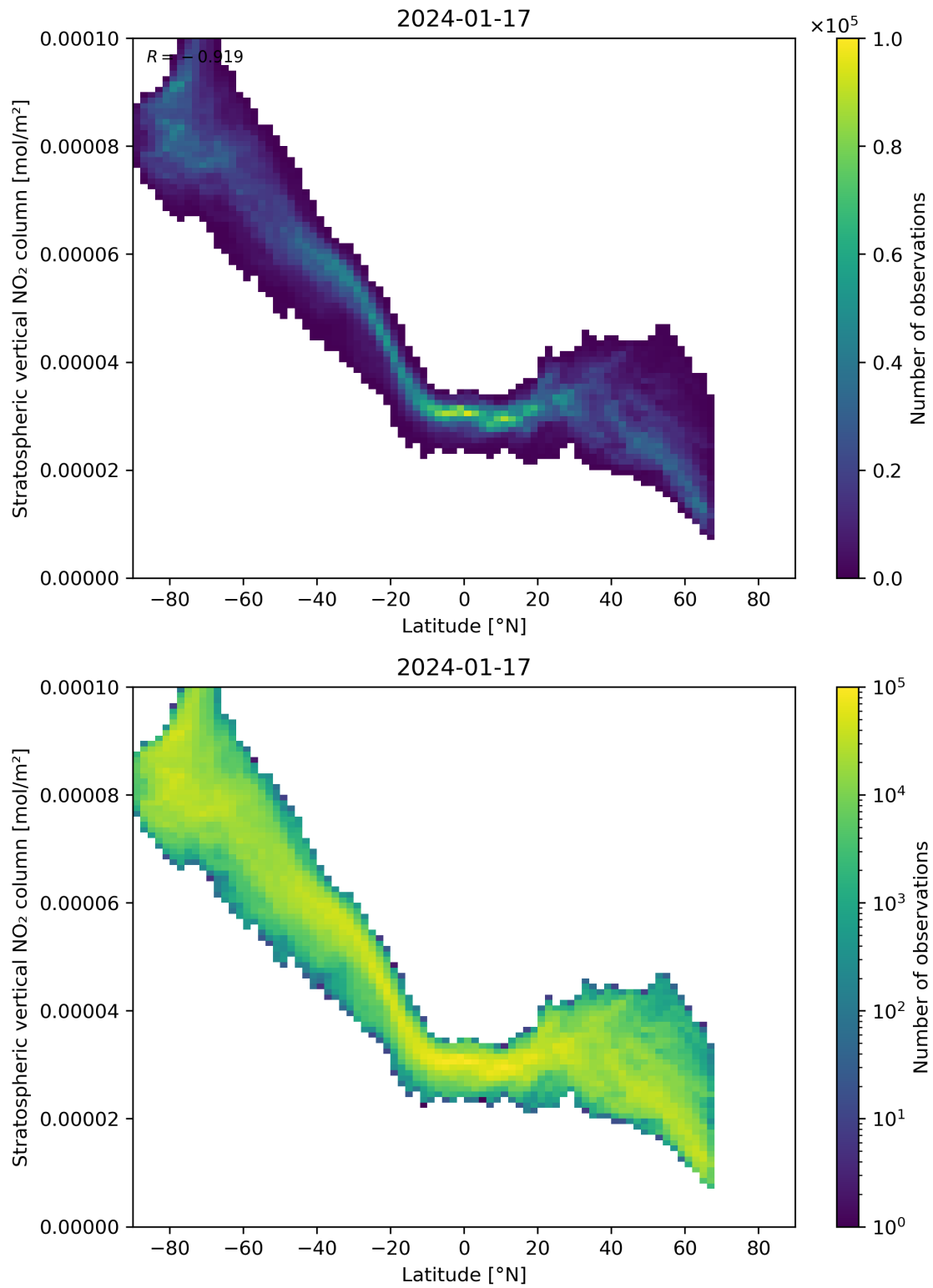
Figure 87: Scatter density plot of “Latitude” against “Stratospheric vertical NO 2 column” for 2024-01-16 to 2024-01-18.
