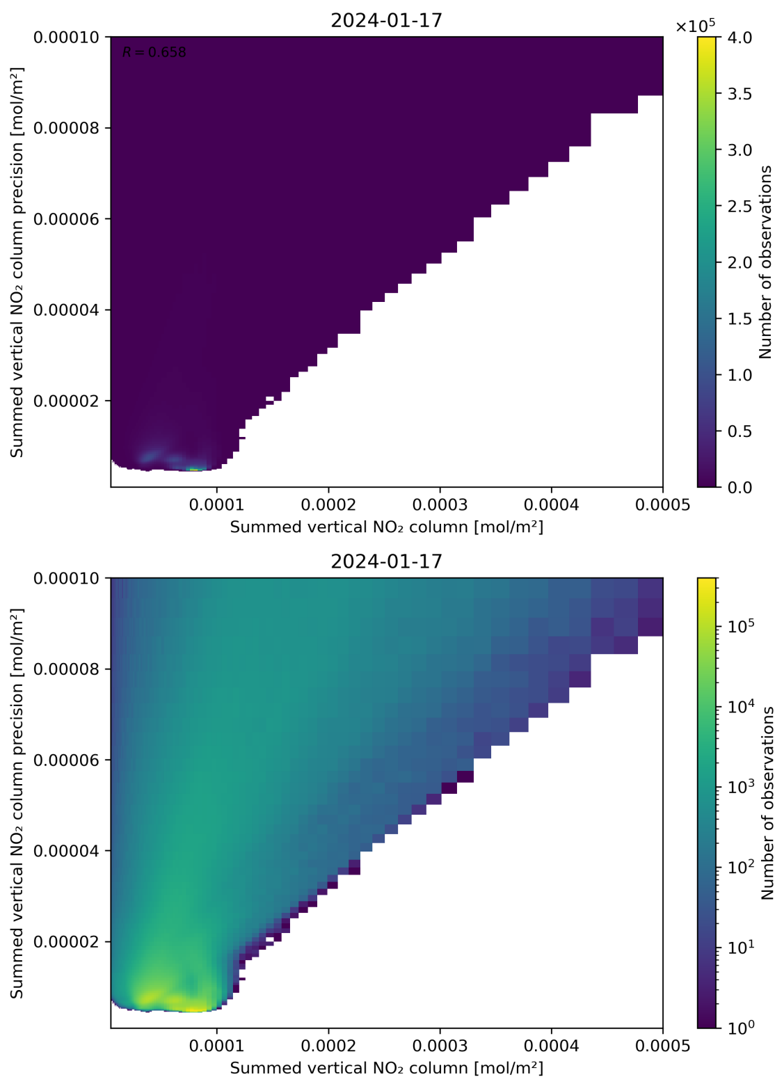
Figure 105: Scatter density plot of “Summed vertical NO 2 column” against “Summed vertical NO 2 column precision” for 2024-01-16 to 2024-01-18.
