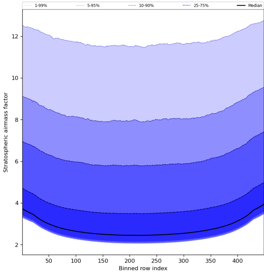
Figure 61: Along track statistics of “Stratospheric airmass factor” for 2024-01-16 to 2024-01-18
