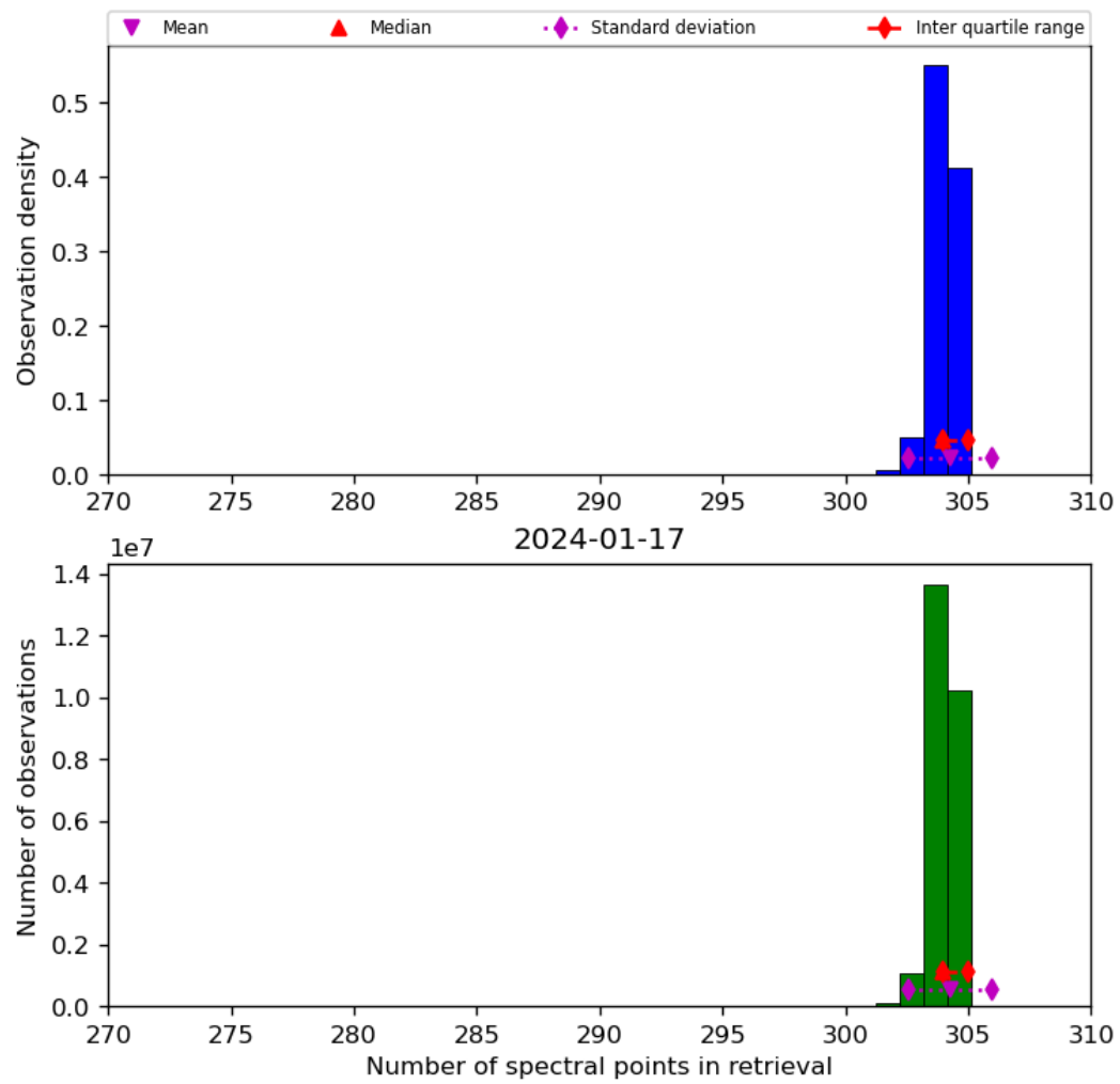
Figure 33: Histogram of “Number of spectral points in retrieval” for 2024-01-16 to 2024-01-18
