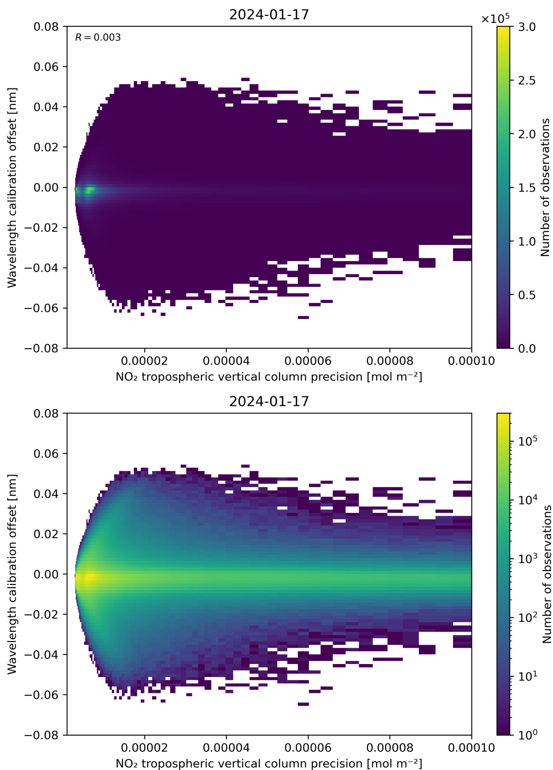
Figure 141: Scatter density plot of “NO 2 tropospheric vertical column precision” against “Wavelength calibration offset” for 2024-01-16 to 2024-01-18.
