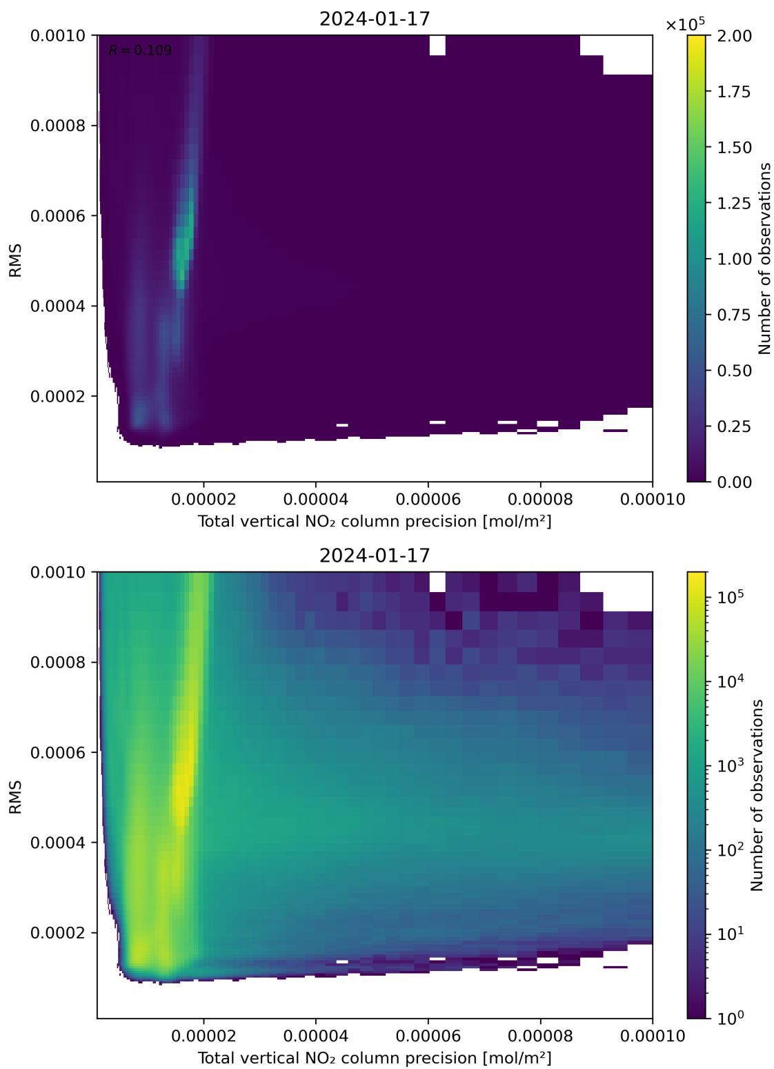
Figure 119: Scatter density plot of “Total vertical NO 2 column precision” against “RMS” for 2024-01-16 to 2024-01-18.
