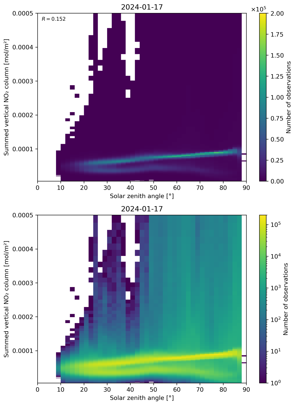
Figure 151: Scatter density plot of “Solar zenith angle” against “Summed vertical NO 2 column” for 2024-01-16 to 2024-01-18.
