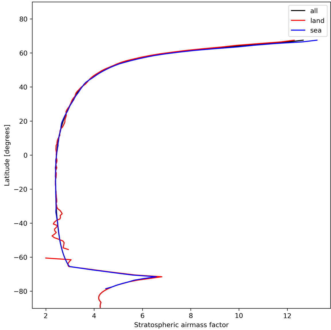
Figure 27: Zonal average of “Stratospheric air mass factor” for 2024-01-16 to 2024-01-18.
