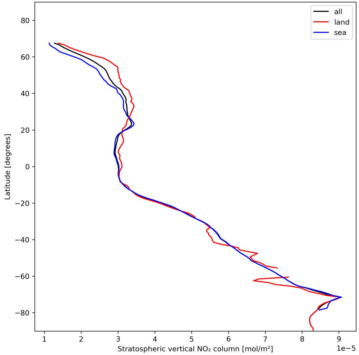
Figure 19: Zonal average of “Stratospheric vertical NO 2 column” for 2024-01-16 to 2024-01-18.
