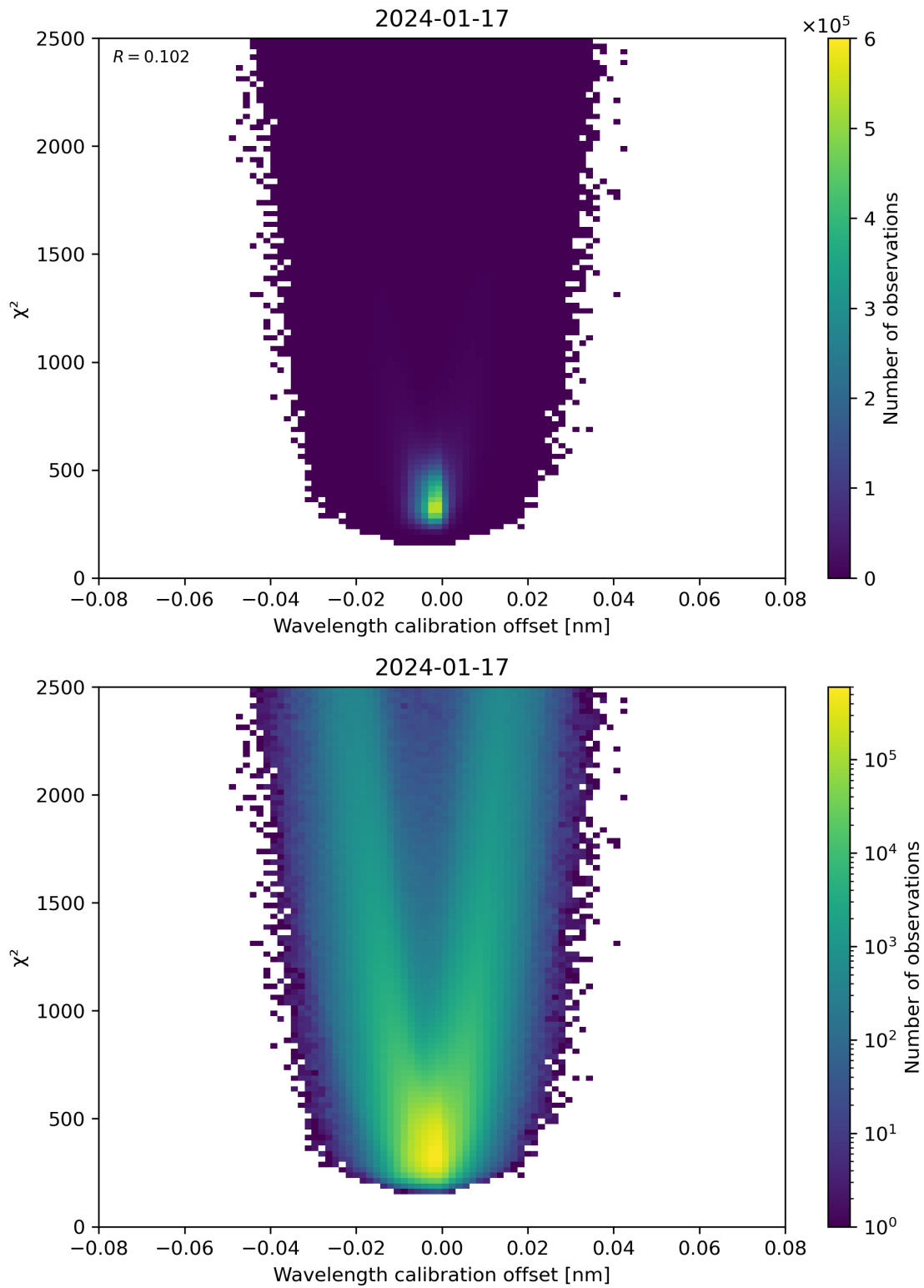
Figure 175: Scatter density plot of “Wavelength calibration offset” against “ \chi^2 ” for 2024-01-16 to 2024-01-18.
