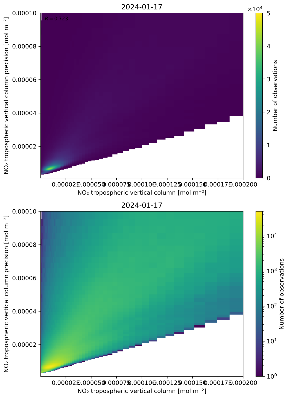
Figure 130: Scatter density plot of “NO 2 tropospheric vertical column” against “NO 2 tropospheric vertical column precision” for 2024-01-16 to 2024-01-18.
