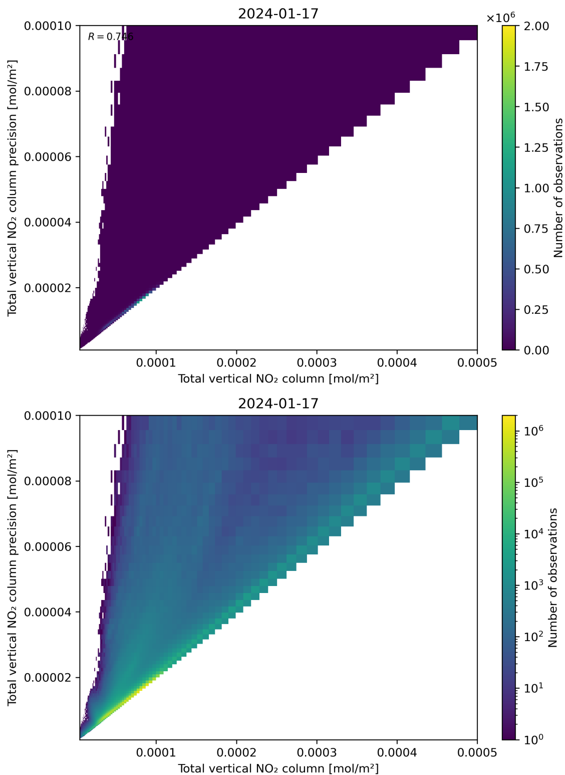
Figure 114: Scatter density plot of “Total vertical NO 2 column” against “Total vertical NO 2 column precision” for 2024-01-16 to 2024-01-18.
