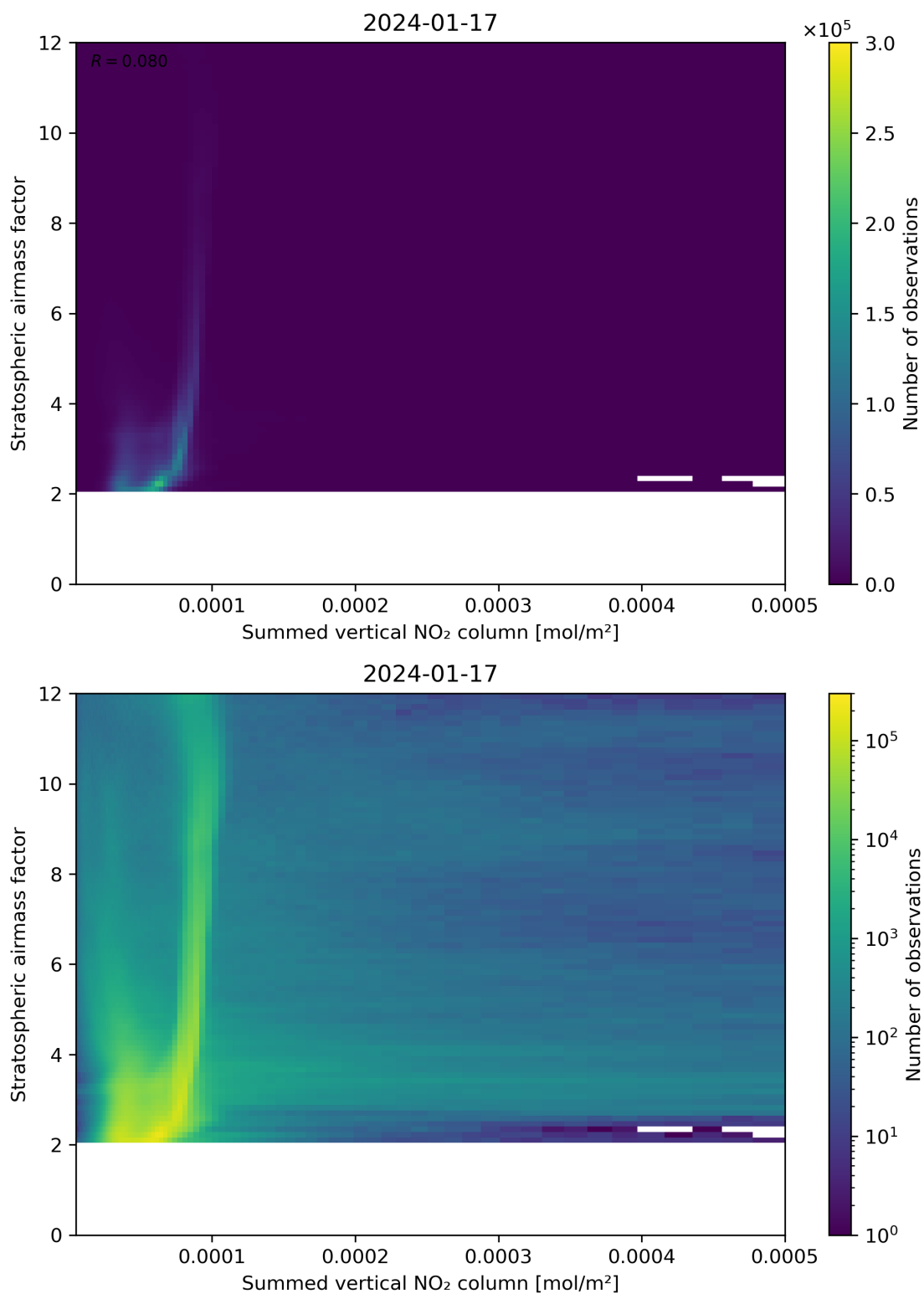
Figure 103: Scatter density plot of “Summed vertical NO 2 column” against “Stratospheric airmass factor” for 2024-01-16 to 2024-01-18.
