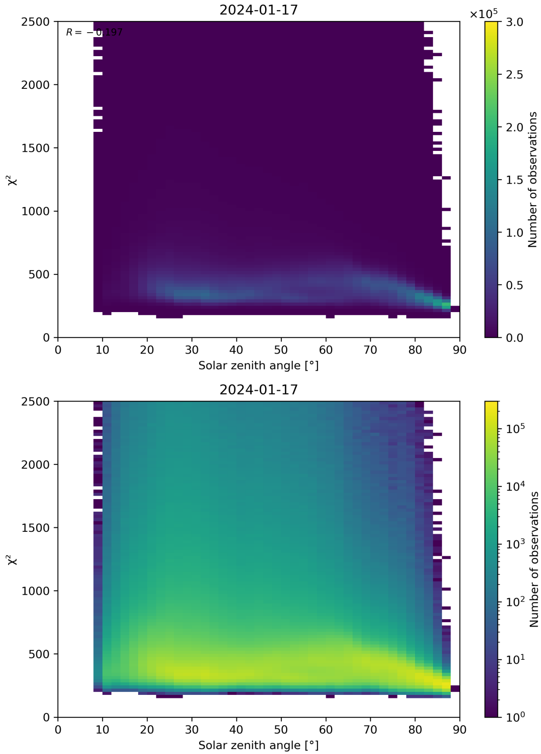
Figure 148: Scatter density plot of “Solar zenith angle” against “ \chi^2 ” for 2024-01-16 to 2024-01-18.
