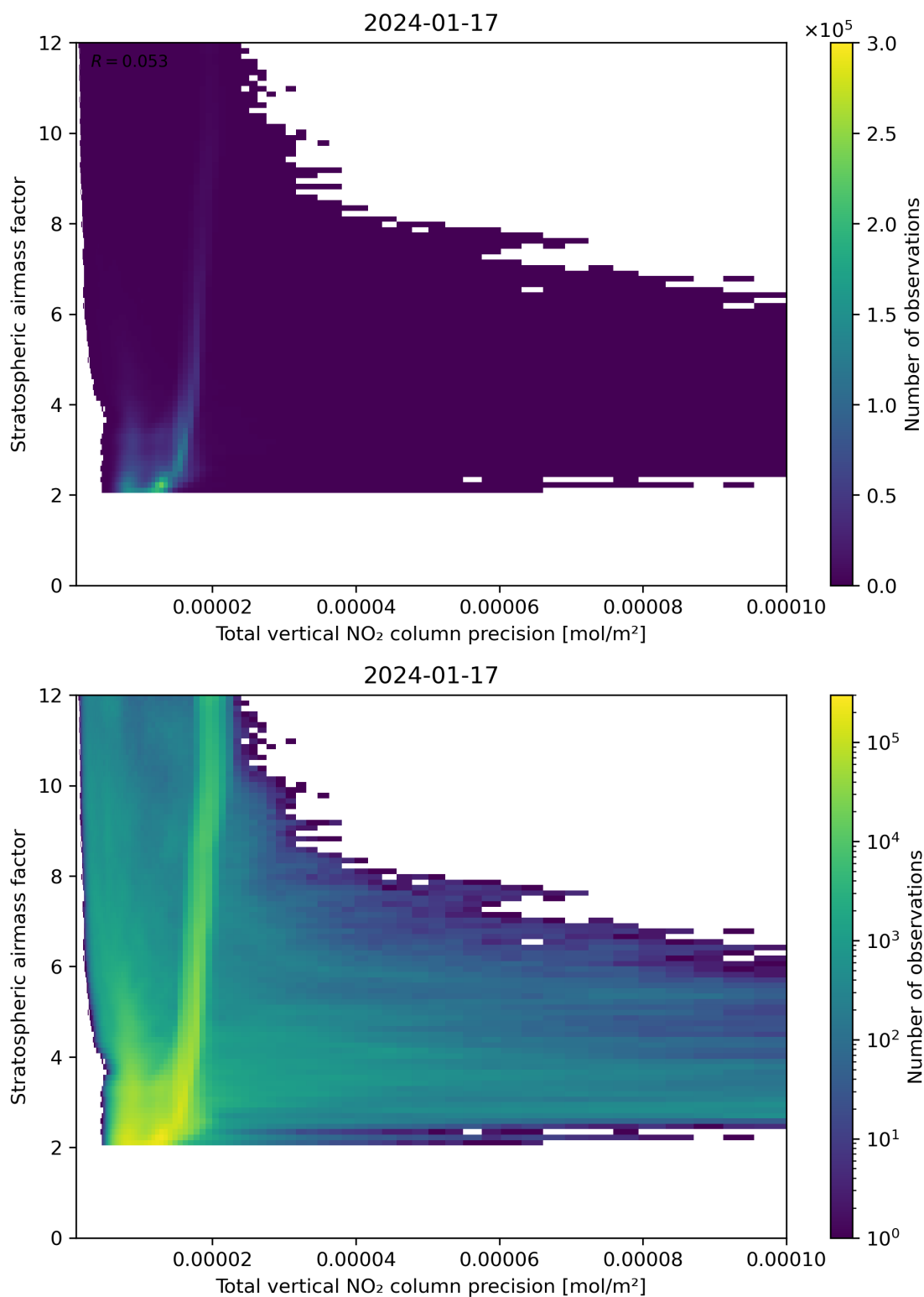
Figure 115: Scatter density plot of “Total vertical NO 2 column precision” against “Stratospheric air mass factor” for 2024-01-16 to 2024-01-18.
