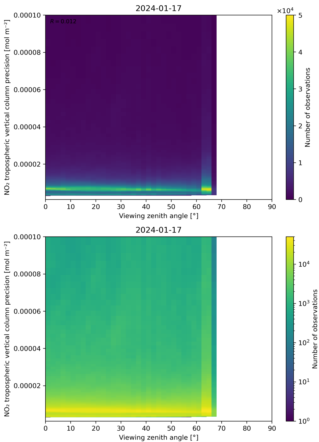
Figure 170: Scatter density plot of “Viewing zenith angle” against “NO 2 tropospheric vertical column precision” for 2024-01-16 to 2024-01-18.
