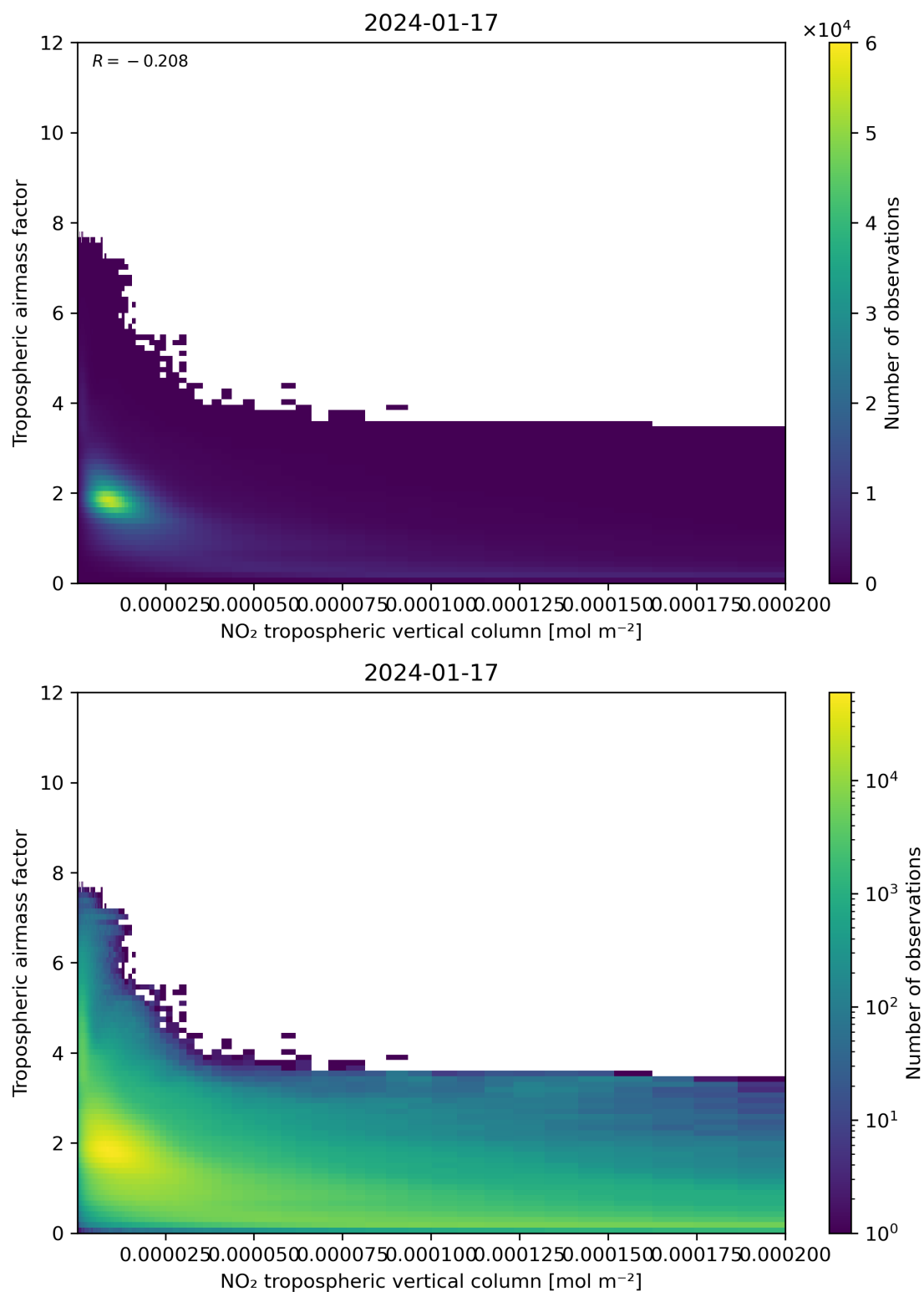
Figure 123: Scatter density plot of “NO 2 tropospheric vertical column” against “Tropospheric air mass factor” for 2024-01-16 to 2024-01-18.
