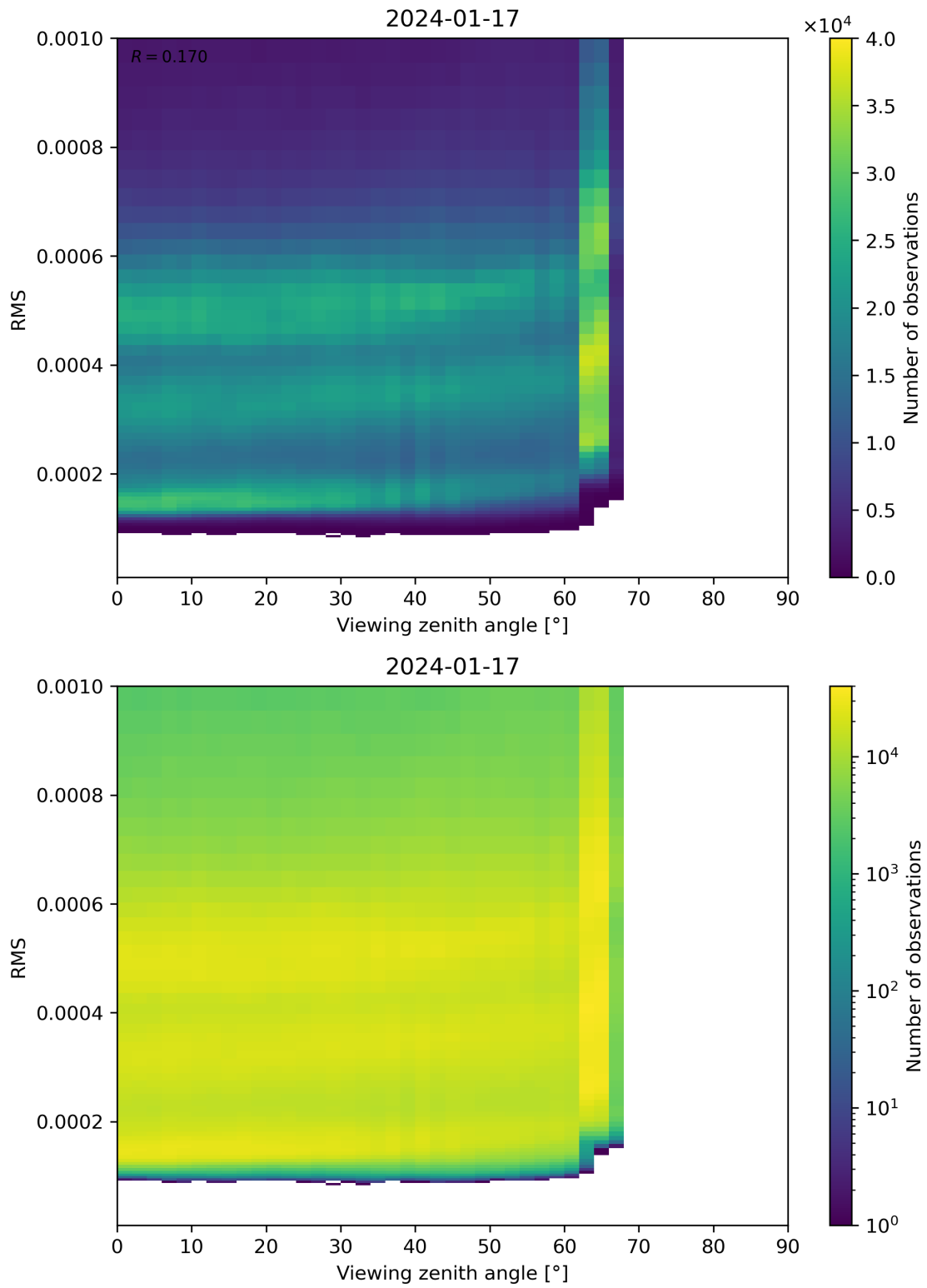
Figure 171: Scatter density plot of “Viewing zenith angle” against “RMS” for 2024-01-16 to 2024-01-18.
