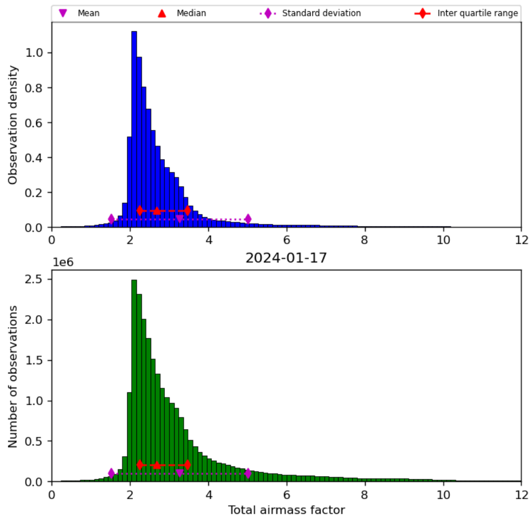
Figure 32: Histogram of “Total airmass factor” for 2024-01-16 to 2024-01-18
