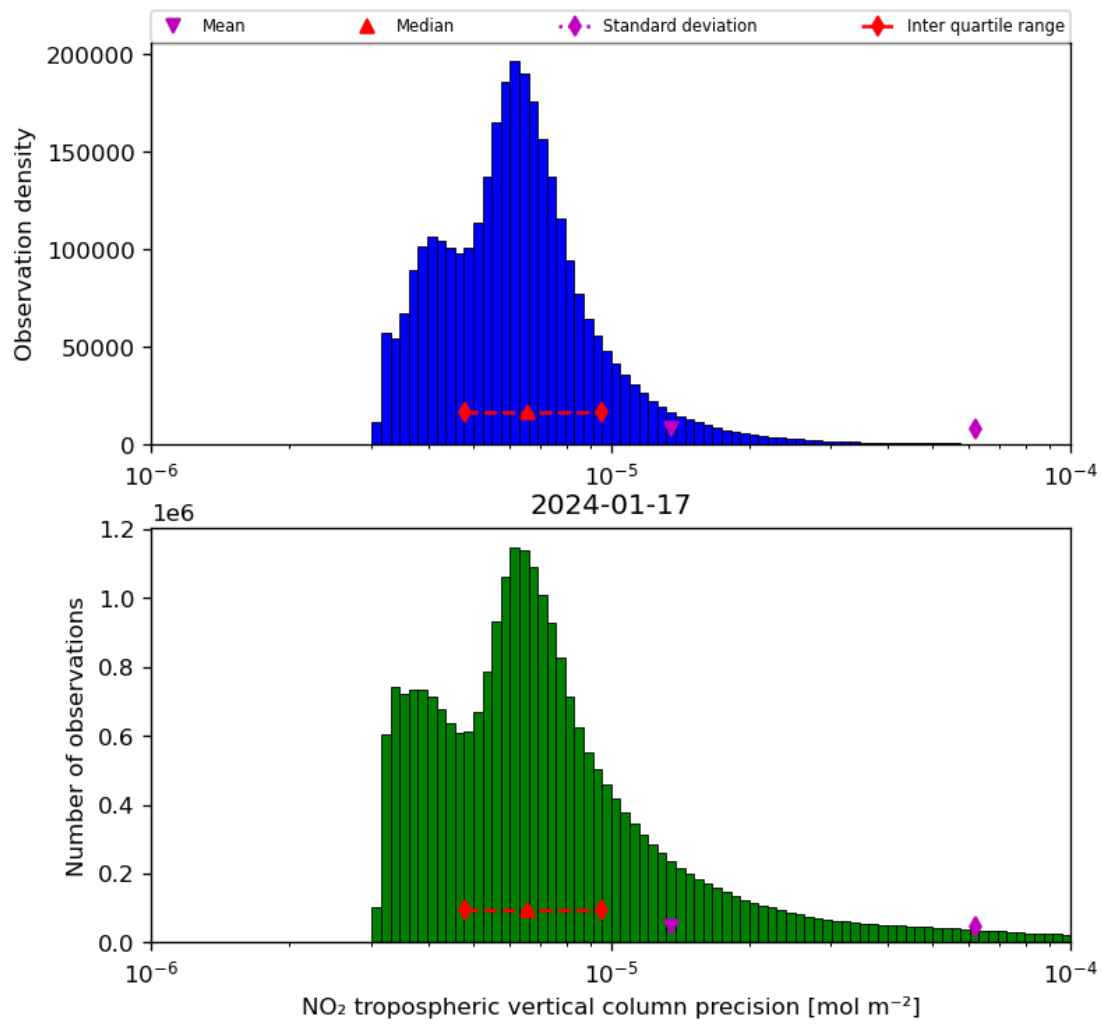
Figure 30: Histogram of “NO 2 tropospheric vertical column precision” for 2024-01-16 to 2024-01-18
