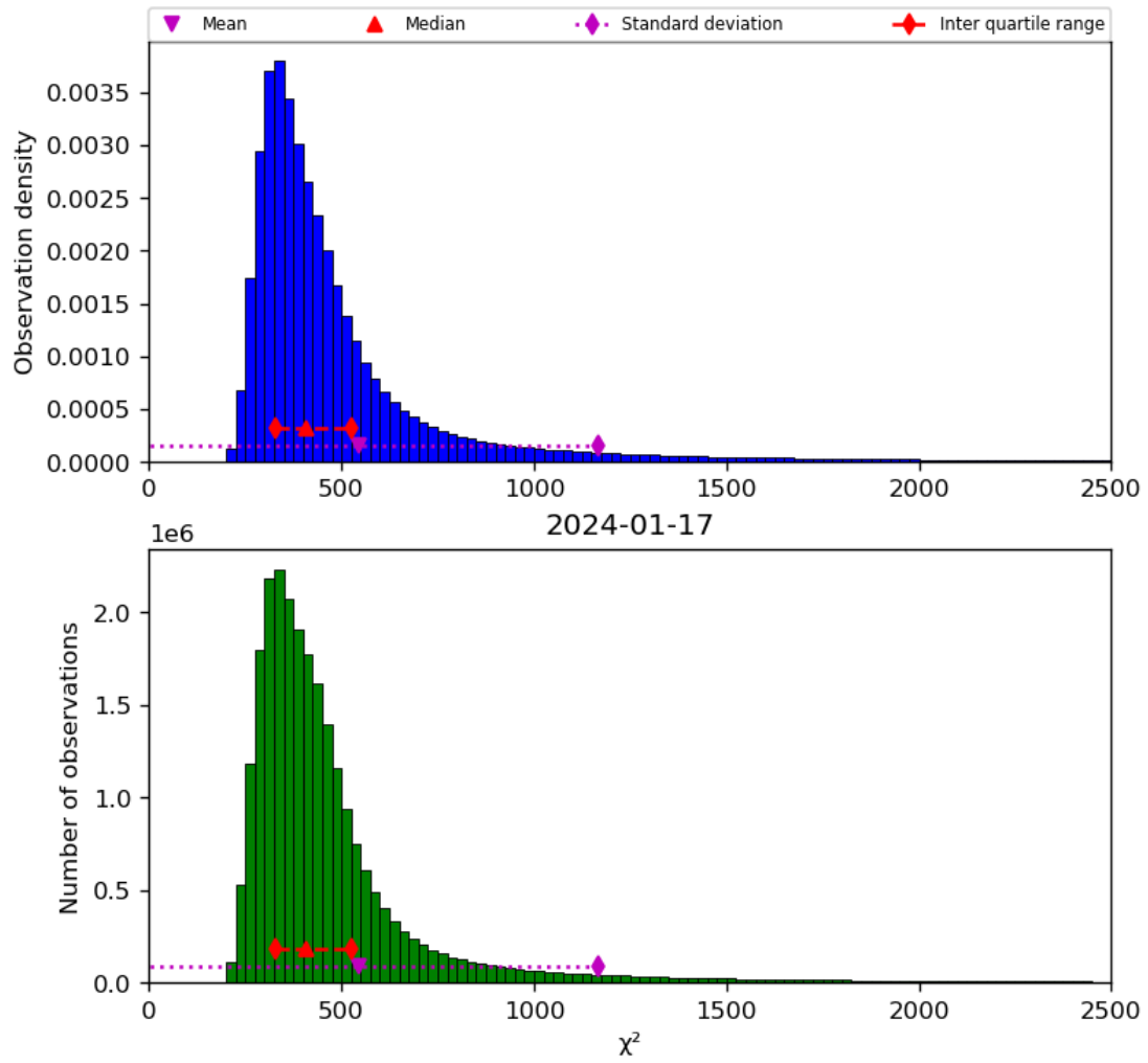
Figure 42: Histogram of “ \chi^2 ” for 2024-01-16 to 2024-01-18
