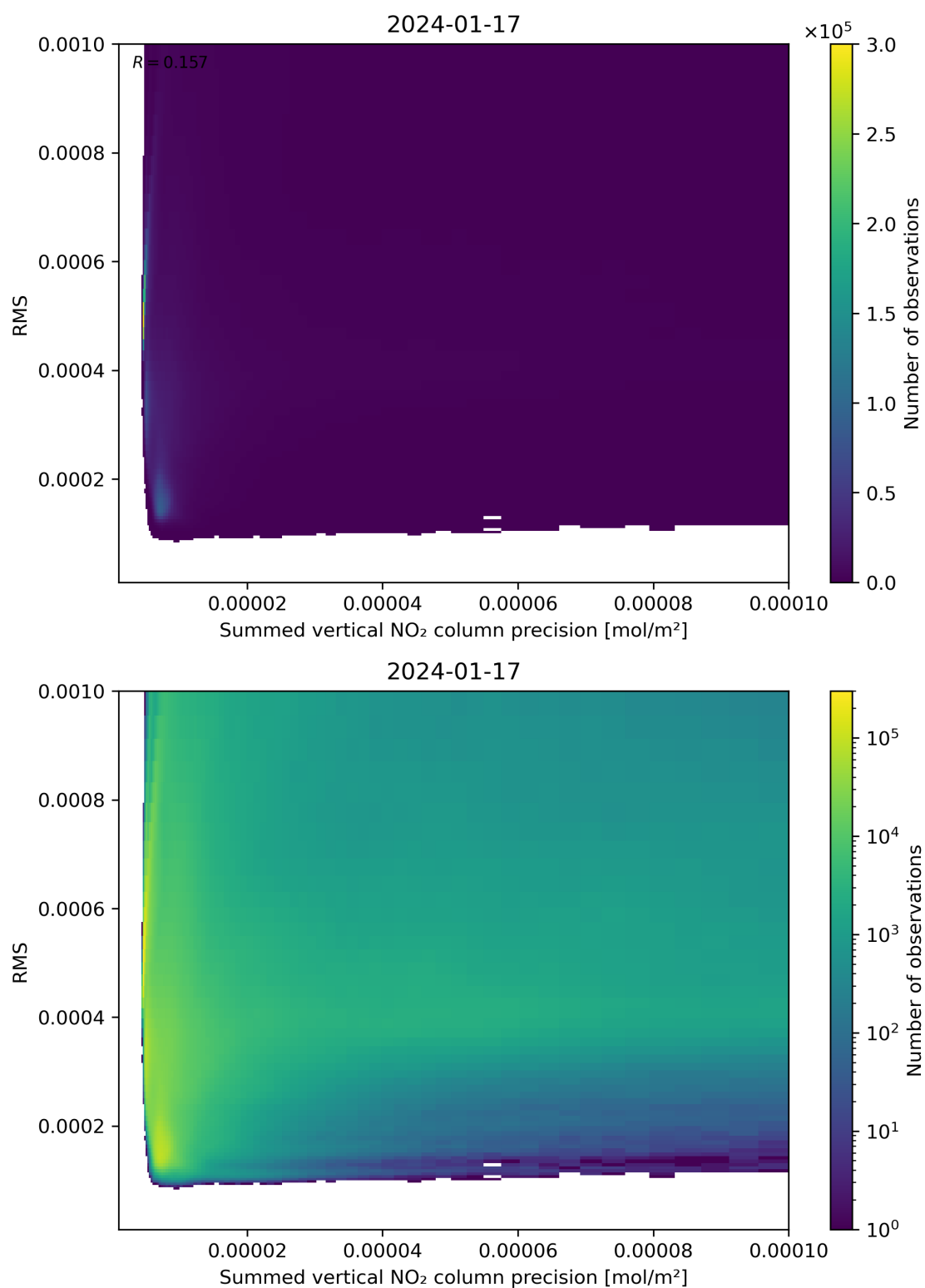
Figure 108: Scatter density plot of “Summed vertical NO 2 column precision” against “RMS” for 2024-01-16 to 2024-01-18.
