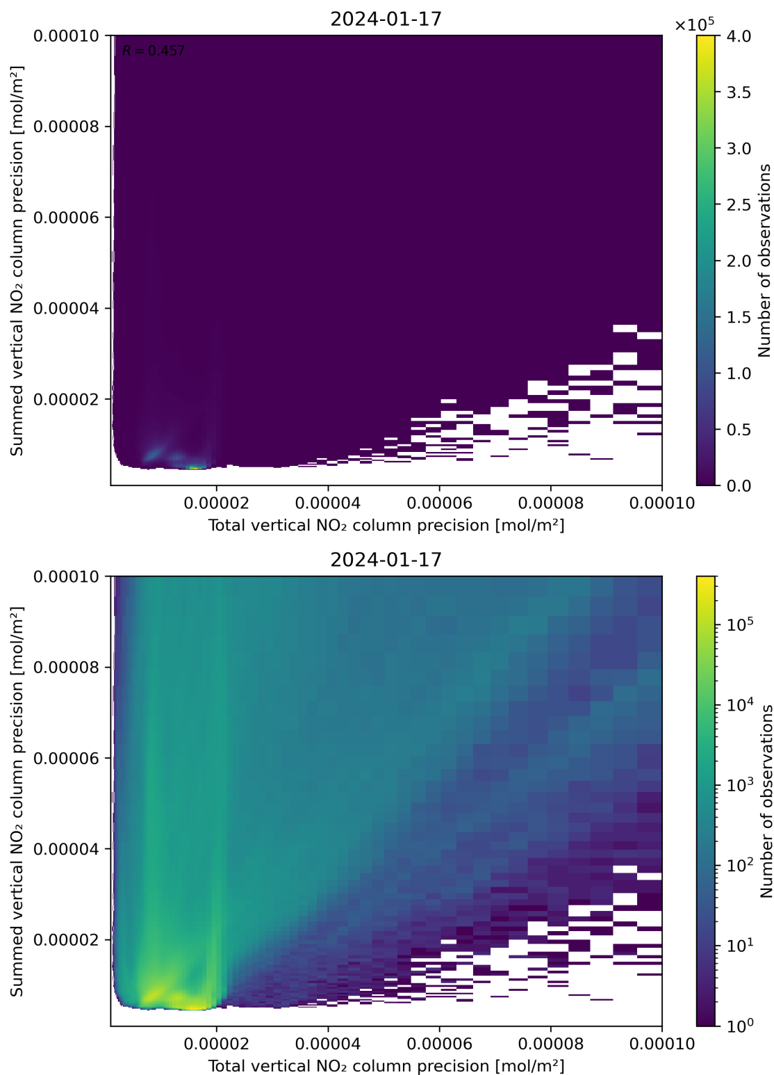
Figure 118: Scatter density plot of “Total vertical NO 2 column precision” against “Summed vertical NO 2 column precision” for 2024-01-16 to 2024-01-18.
