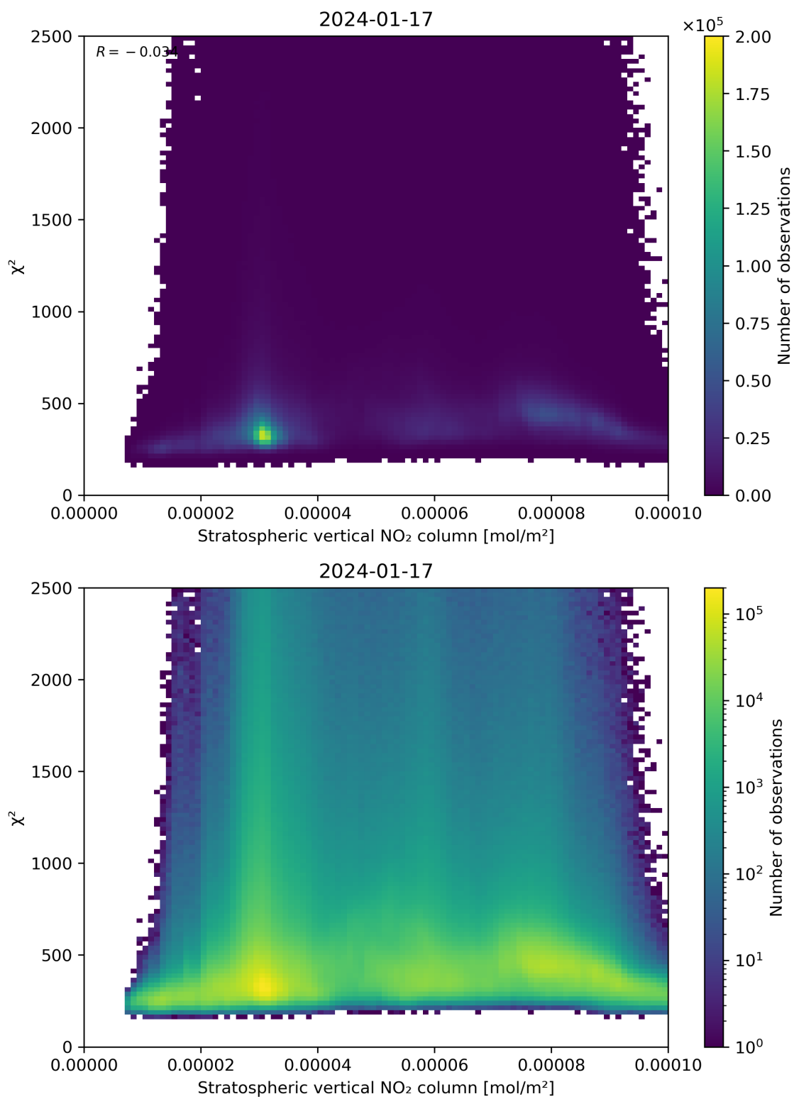
Figure 97: Scatter density plot of “Stratospheric vertical NO 2 column” against “ \chi^2 ” for 2024-01-16 to 2024-01-18.
