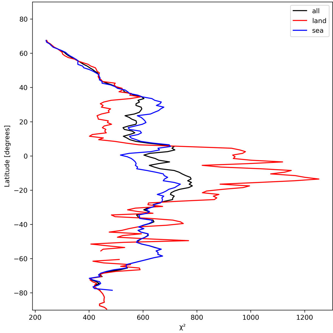
Figure 25: Zonal average of “ \chi^2 ” for 2024-01-16 to 2024-01-18.
