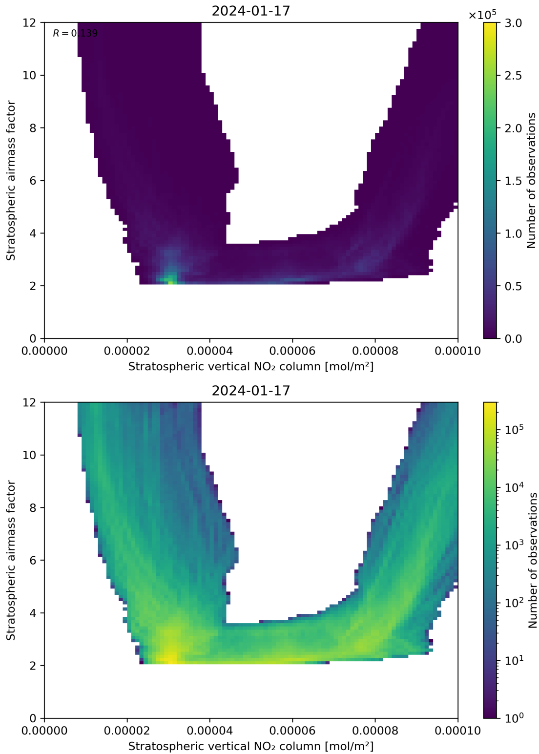
Figure 96: Scatter density plot of “Stratospheric vertical NO 2 column” against “Stratospheric airmass factor” for 2024-01-16 to 2024-01-18.
