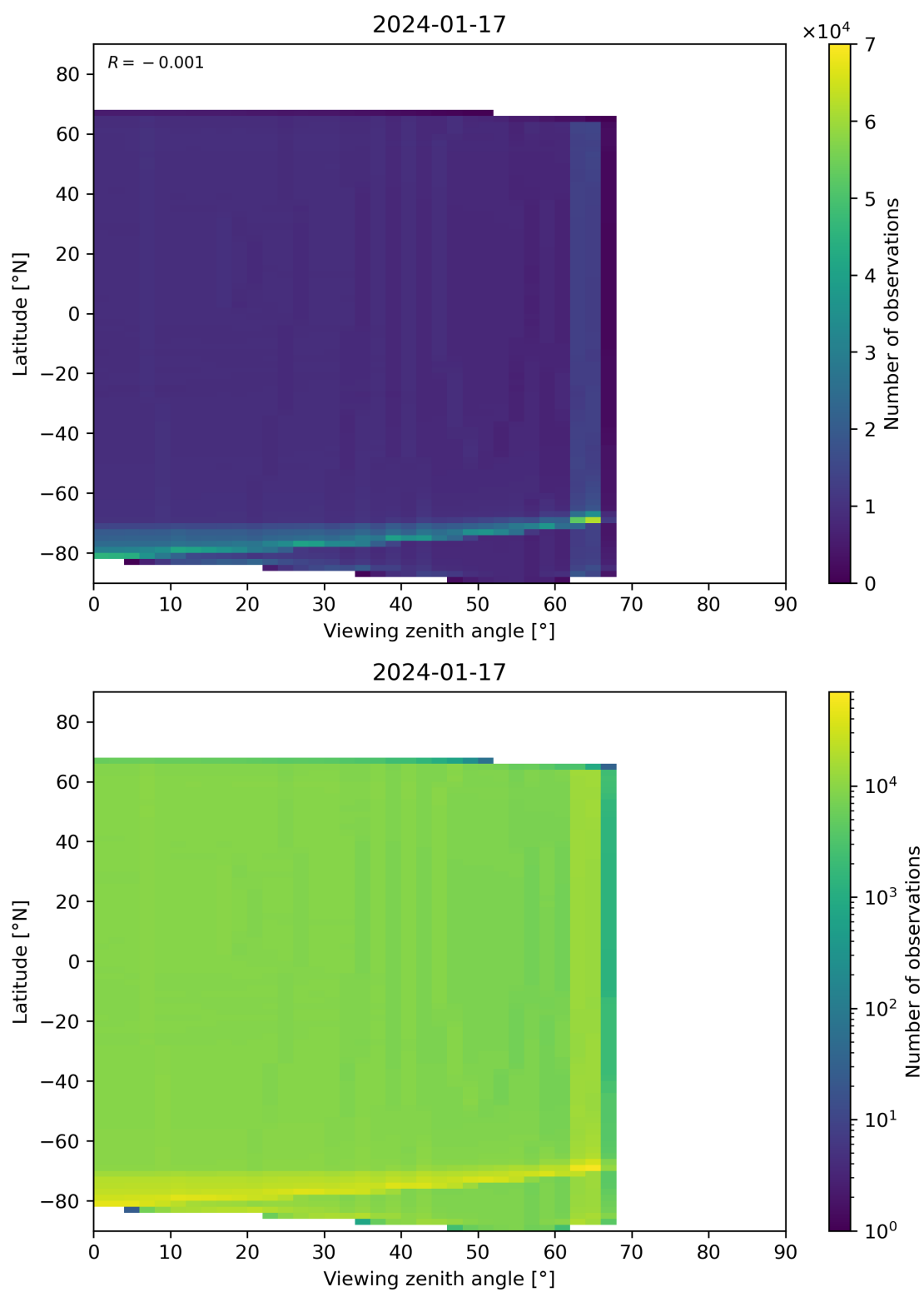
Figure 163: Scatter density plot of “Viewing zenith angle” against “Latitude” for 2024-01-16 to 2024-01-18.
