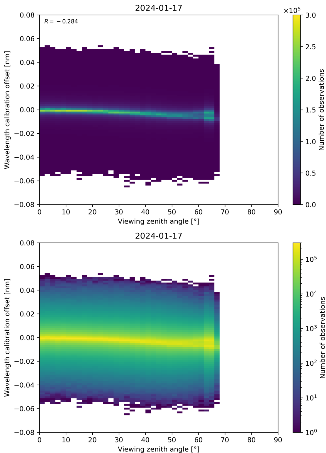
Figure 173: Scatter density plot of “Viewing zenith angle” against “Wavelength calibration offset” for 2024-01-16 to 2024-01-18.
