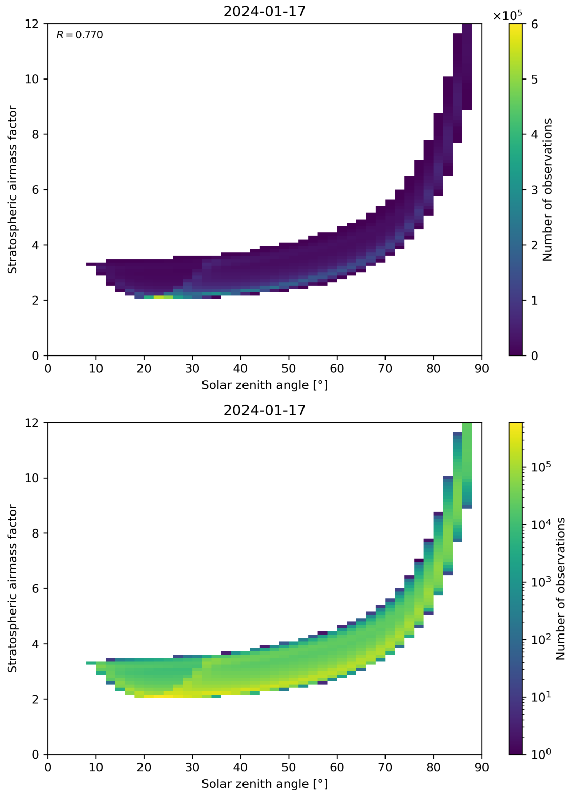
Figure 145: Scatter density plot of “Solar zenith angle” against “Stratospheric airmass factor” for 2024-01-16 to 2024-01-18.
