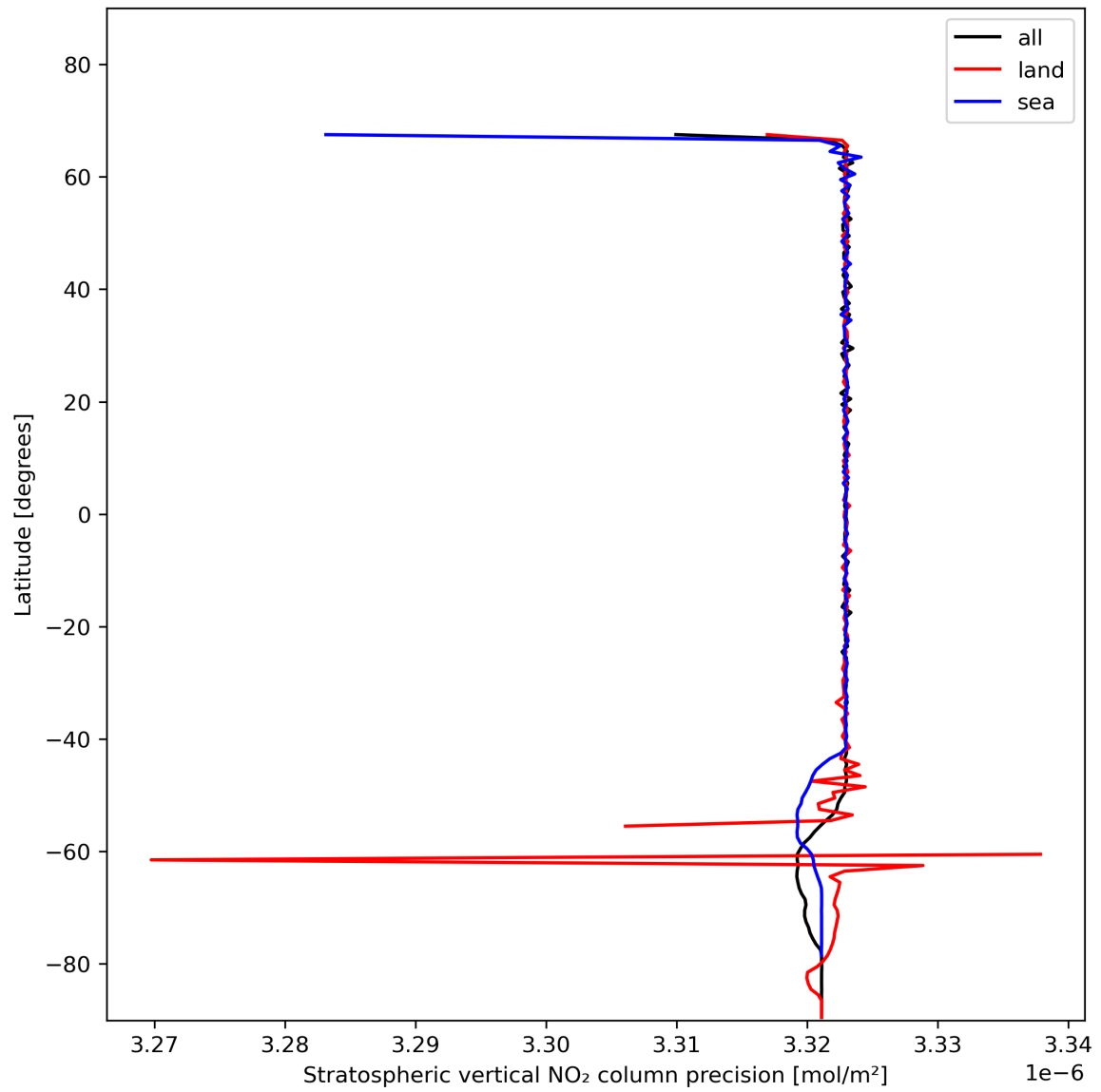
Figure 20: Zonal average of "Stratospheric vertical NO 2 column precision" for 2024-01-16 to 2024-01-18.
