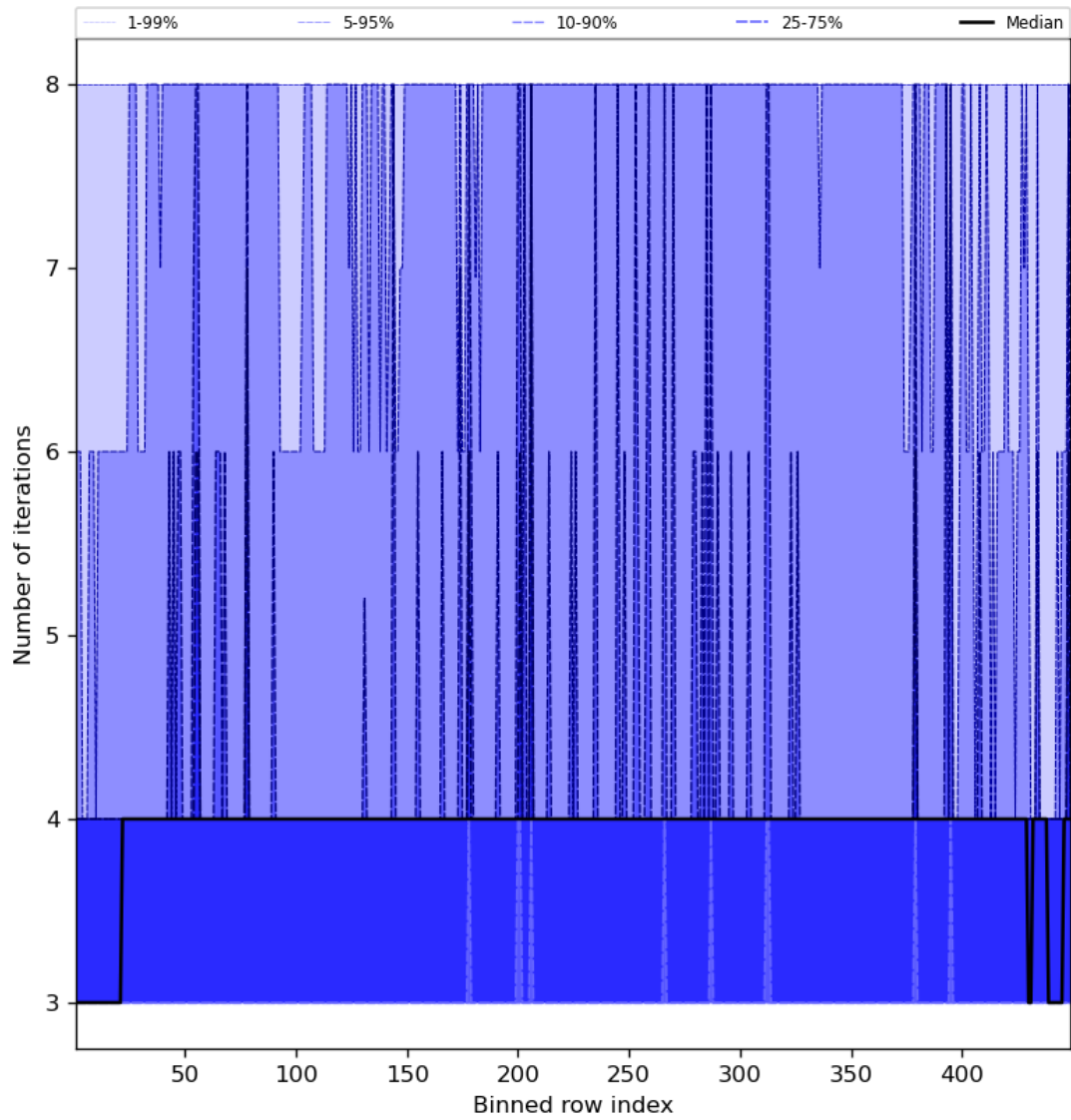
Figure 51: Along track statistics of “Number of iterations” for 2024-01-16 to 2024-01-18
