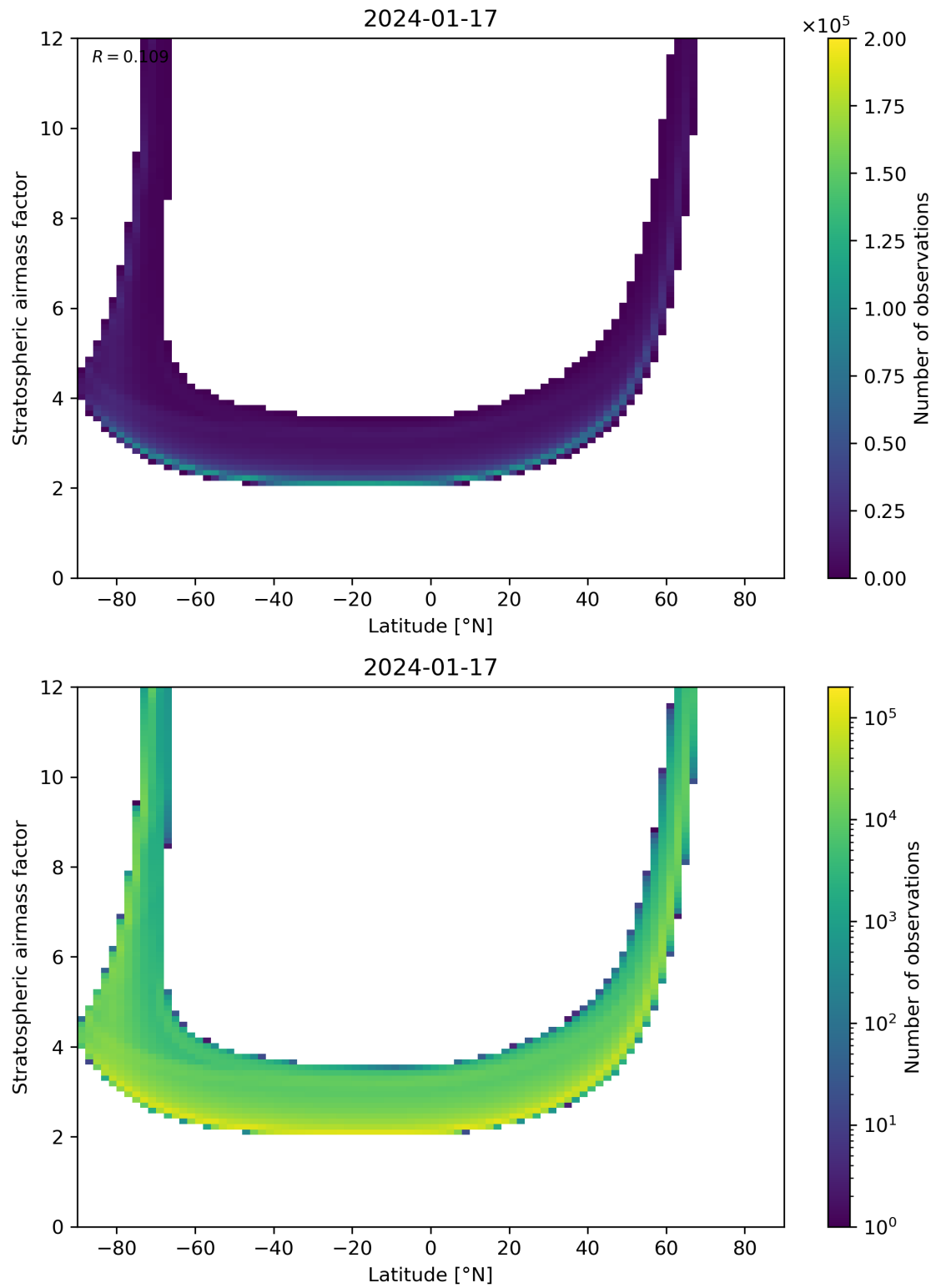
Figure 83: Scatter density plot of “Latitude” against “Stratospheric air mass factor” for 2024-01-16 to 2024-01-18.
