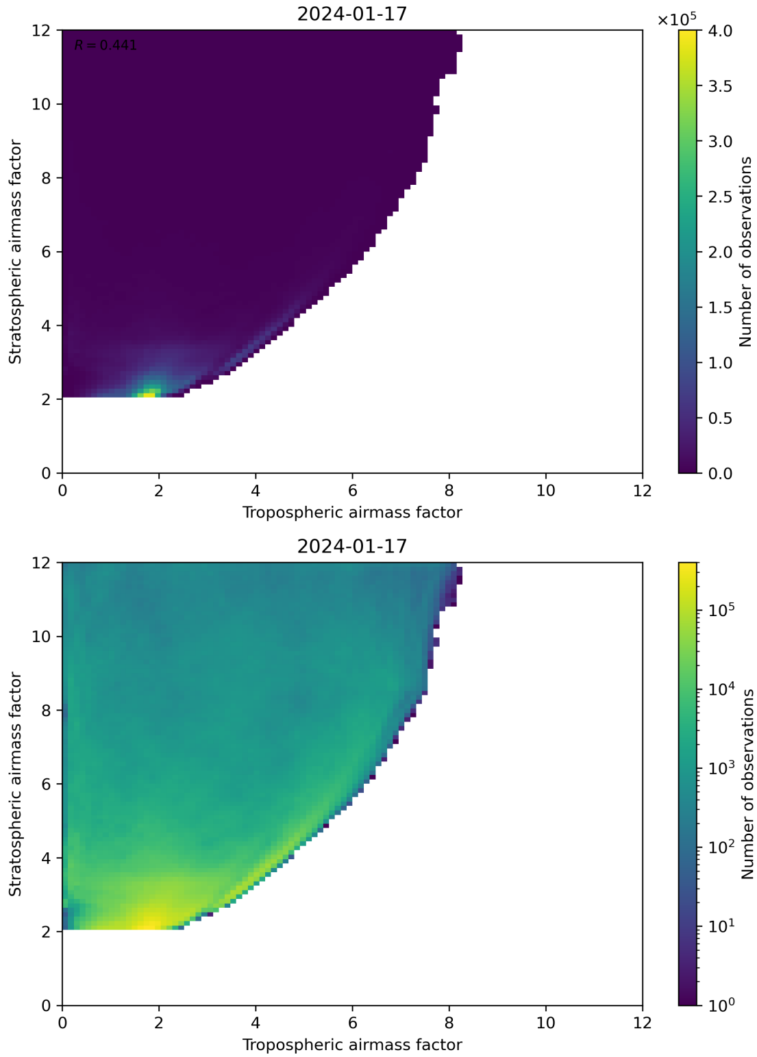
Figure 71: Scatter density plot of “Tropospheric airmass factor” against “Stratospheric airmass factor” for 2024-01-16 to 2024-01-18.
