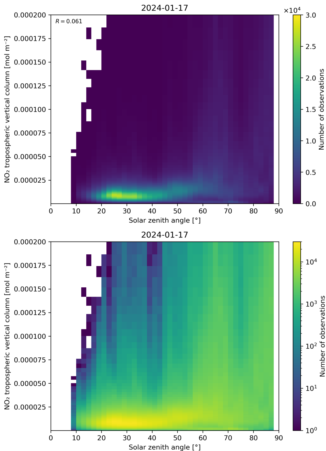
Figure 155: Scatter density plot of “Solar zenith angle” against “NO 2 tropospheric vertical column” for 2024-01-16 to 2024-01-18.
