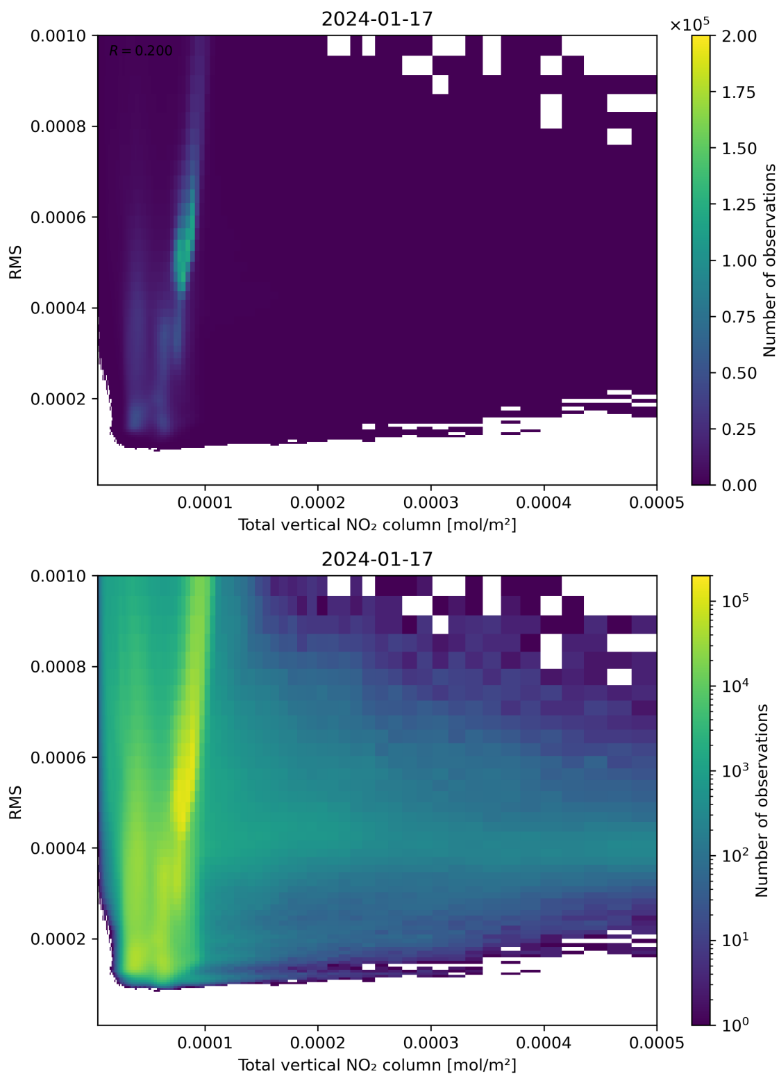
Figure 120: Scatter density plot of “Total vertical NO 2 column” against “RMS” for 2024-01-16 to 2024-01-18.
