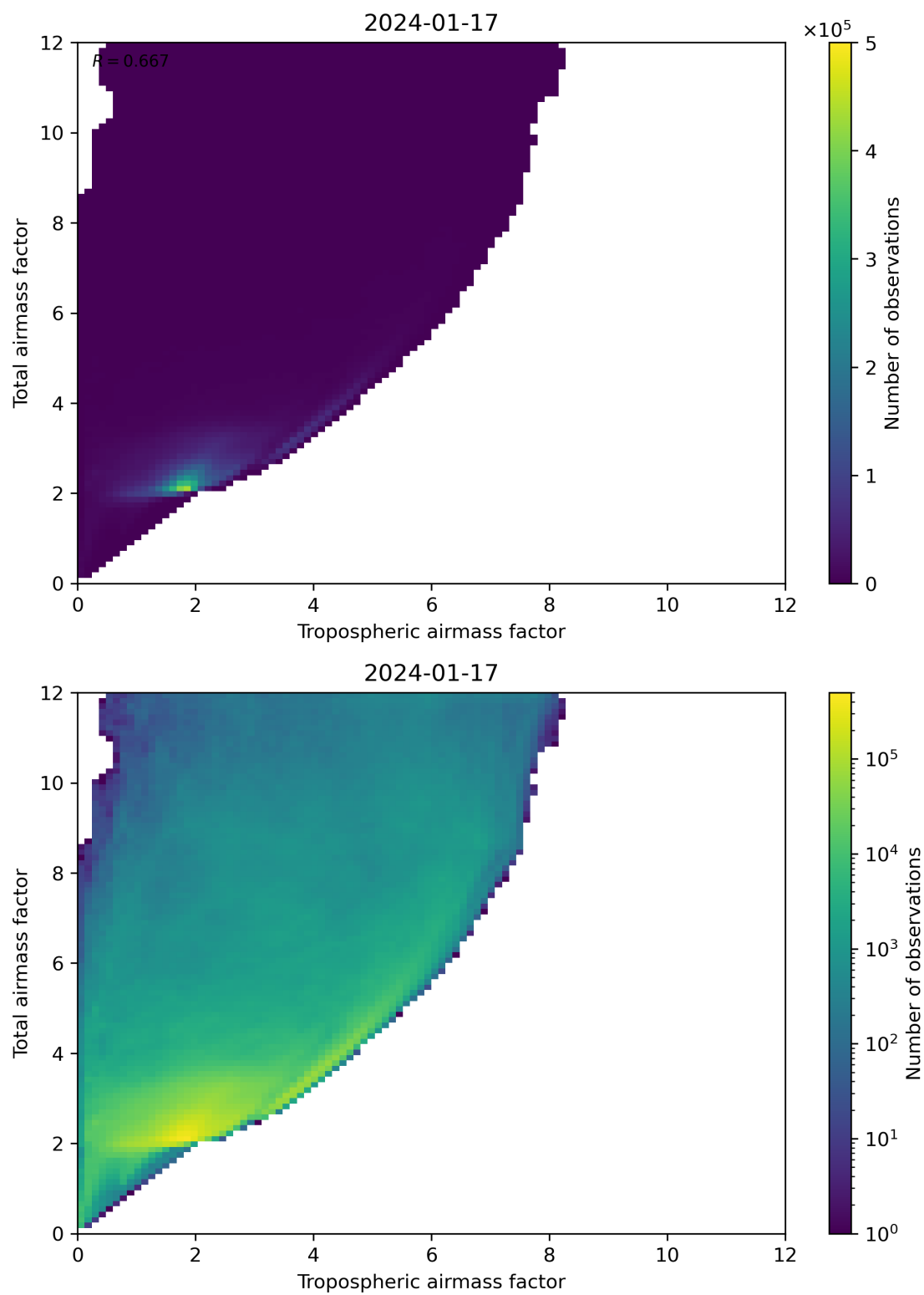
Figure 72: Scatter density plot of “Tropospheric airmass factor” against “Total airmass factor” for 2024-01-16 to 2024-01-18.
