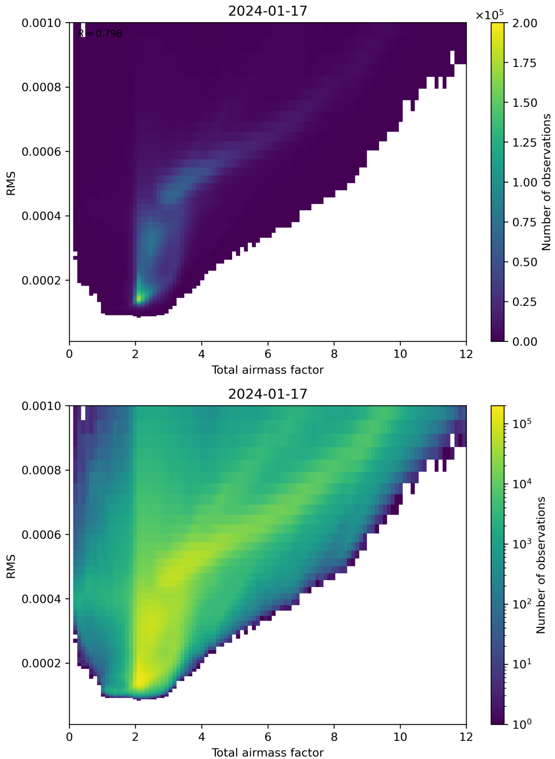
Figure 69: Scatter density plot of “Total airmass factor” against “RMS” for 2024-01-16 to 2024-01-18.
