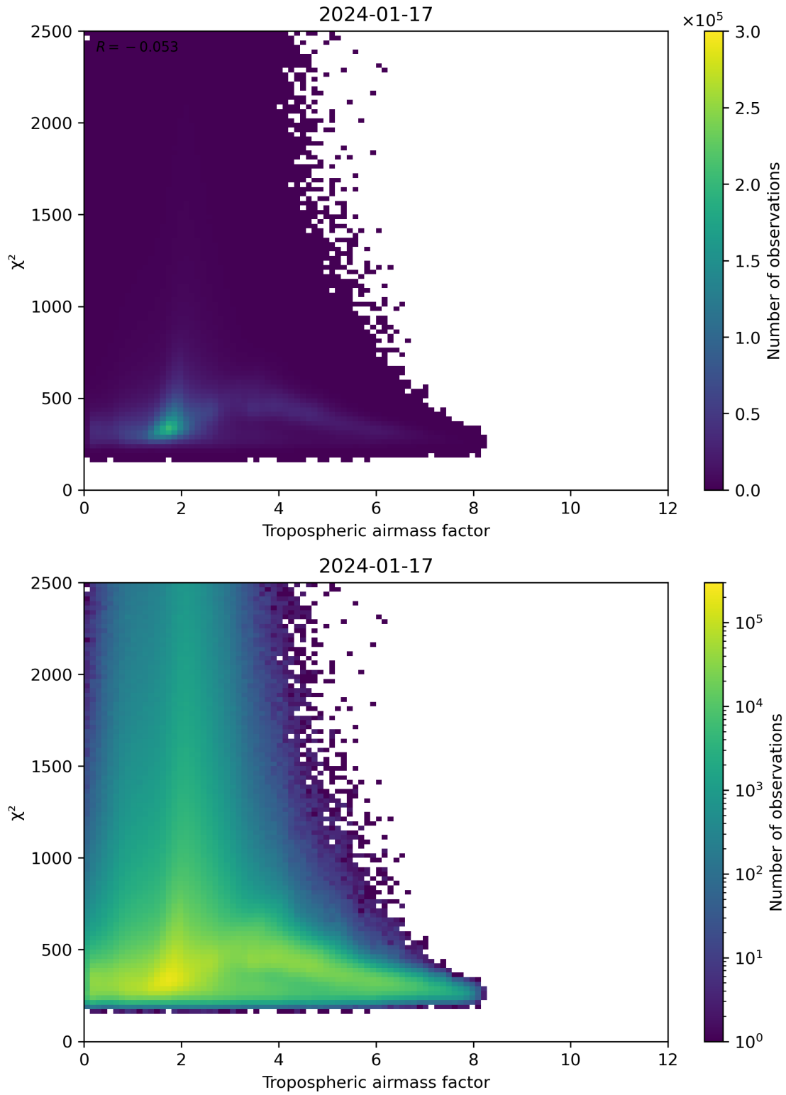
Figure 73: Scatter density plot of “Tropospheric airmass factor” against “ \chi^2 ” for 2024-01-16 to 2024-01-18.
