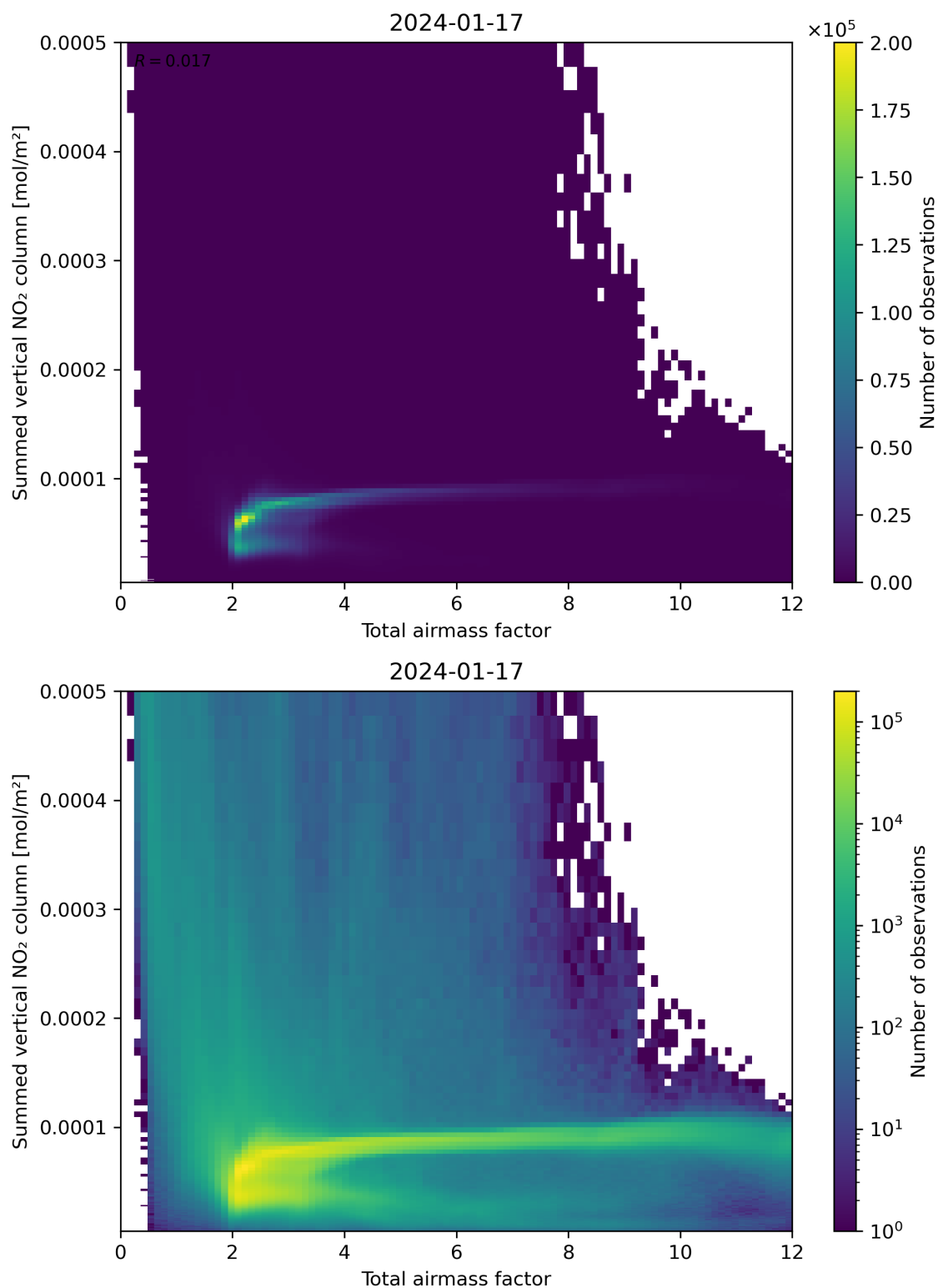
Figure 65: Scatter density plot of “Total airmass factor” against “Summed vertical NO 2 column” for 2024-01-16 to 2024-01-18.
