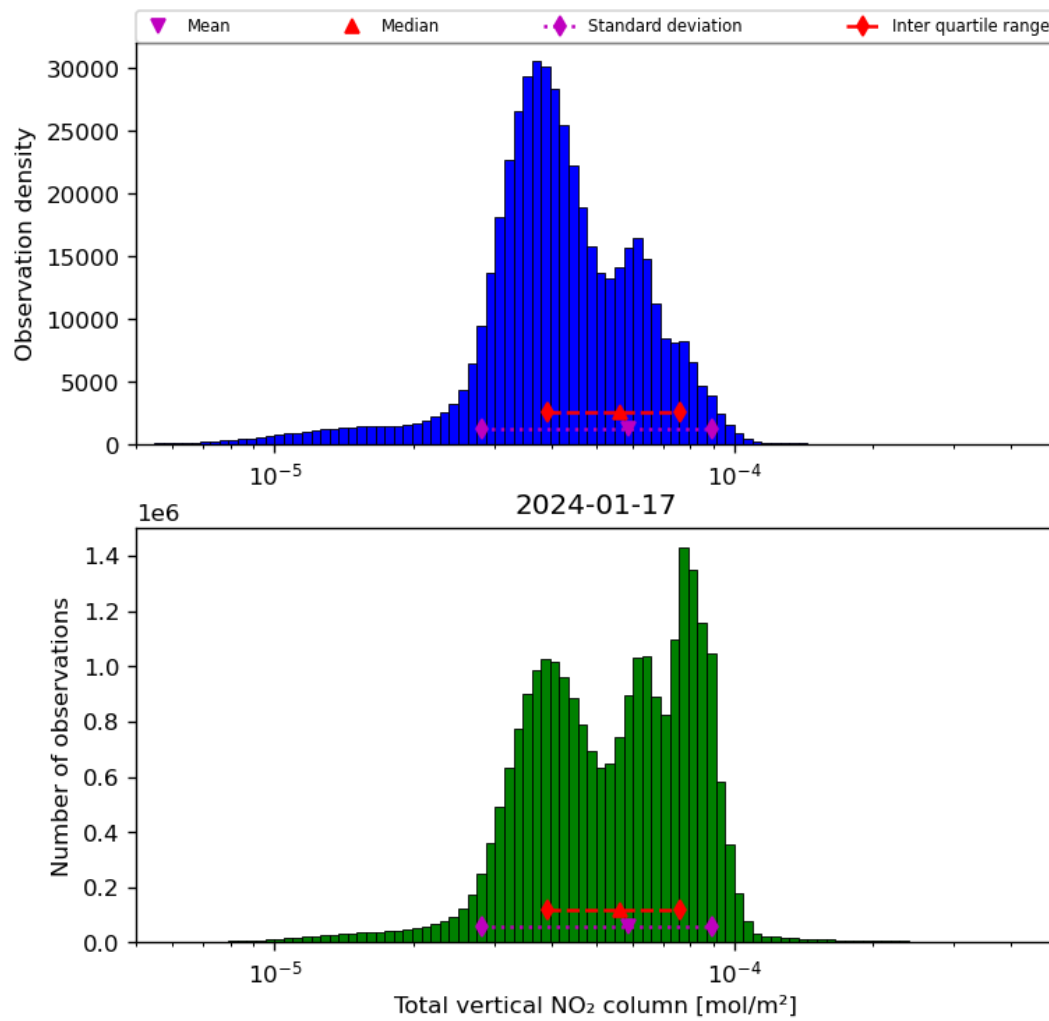
Figure 38: Histogram of “Total vertical NO 2 column” for 2024-01-16 to 2024-01-18
