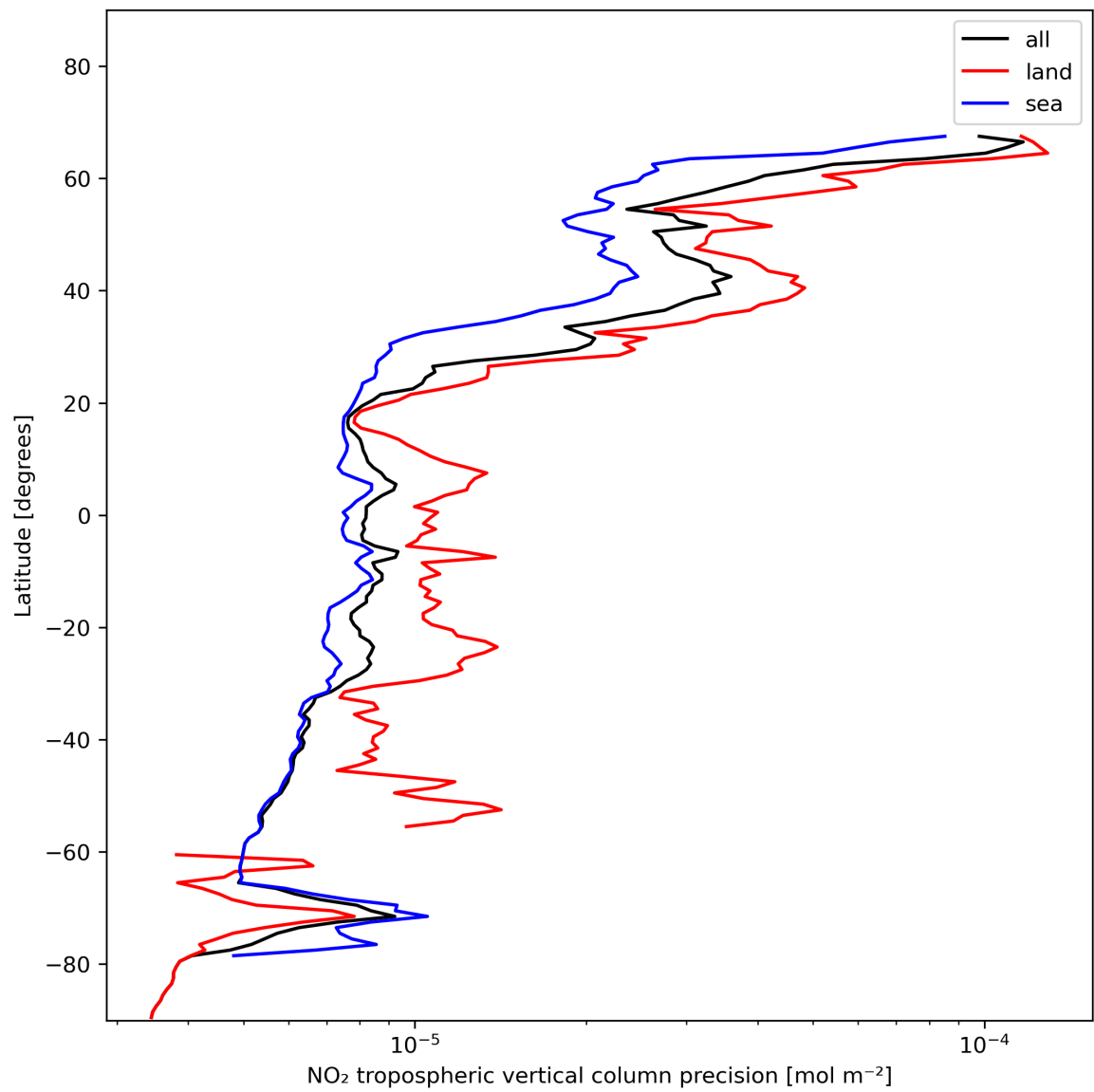
Figure 13: Zonal average of “NO 2 tropospheric vertical column precision” for 2024-01-16 to 2024-01-18.
