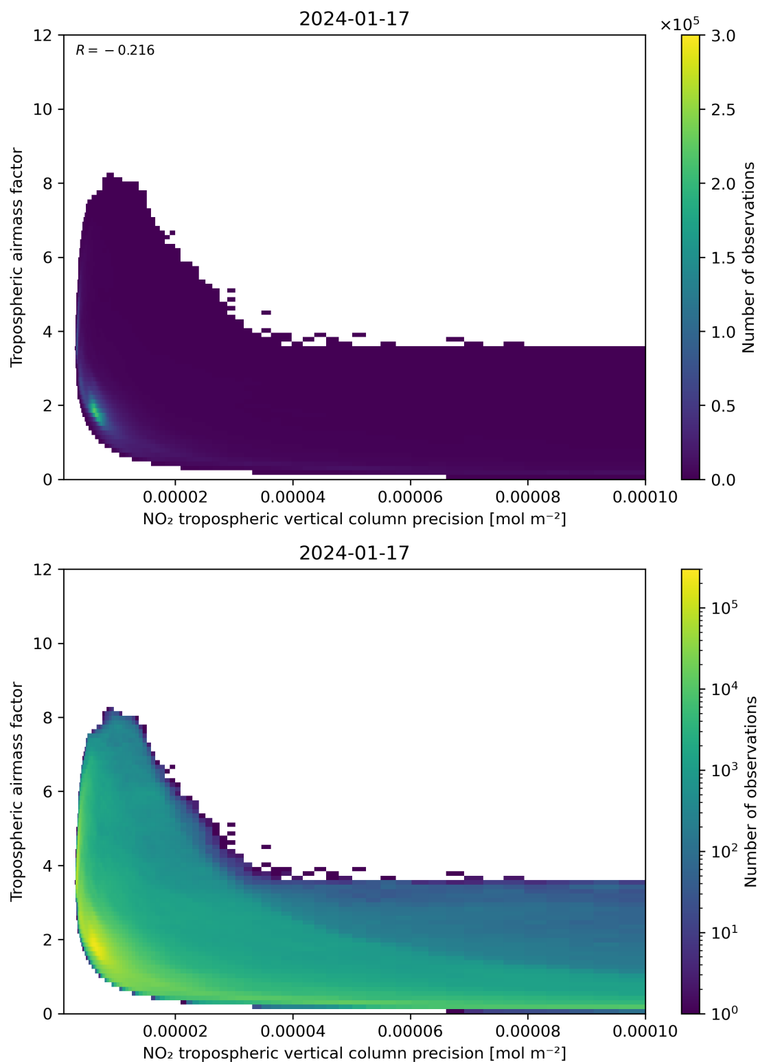
Figure 133: Scatter density plot of “NO 2 tropospheric vertical column precision” against “Tropospheric airmass factor” for 2024-01-16 to 2024-01-18.
