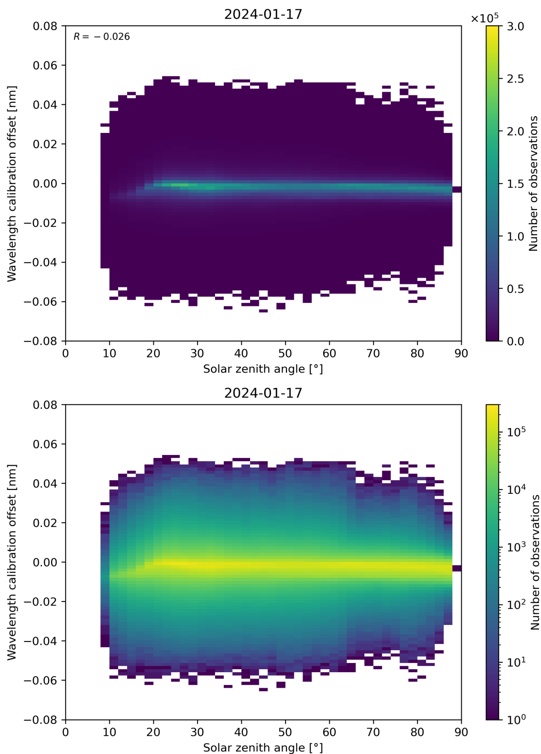
Figure 158: Scatter density plot of “Solar zenith angle” against “Wavelength calibration offset” for 2024-01-16 to 2024-01-18.
