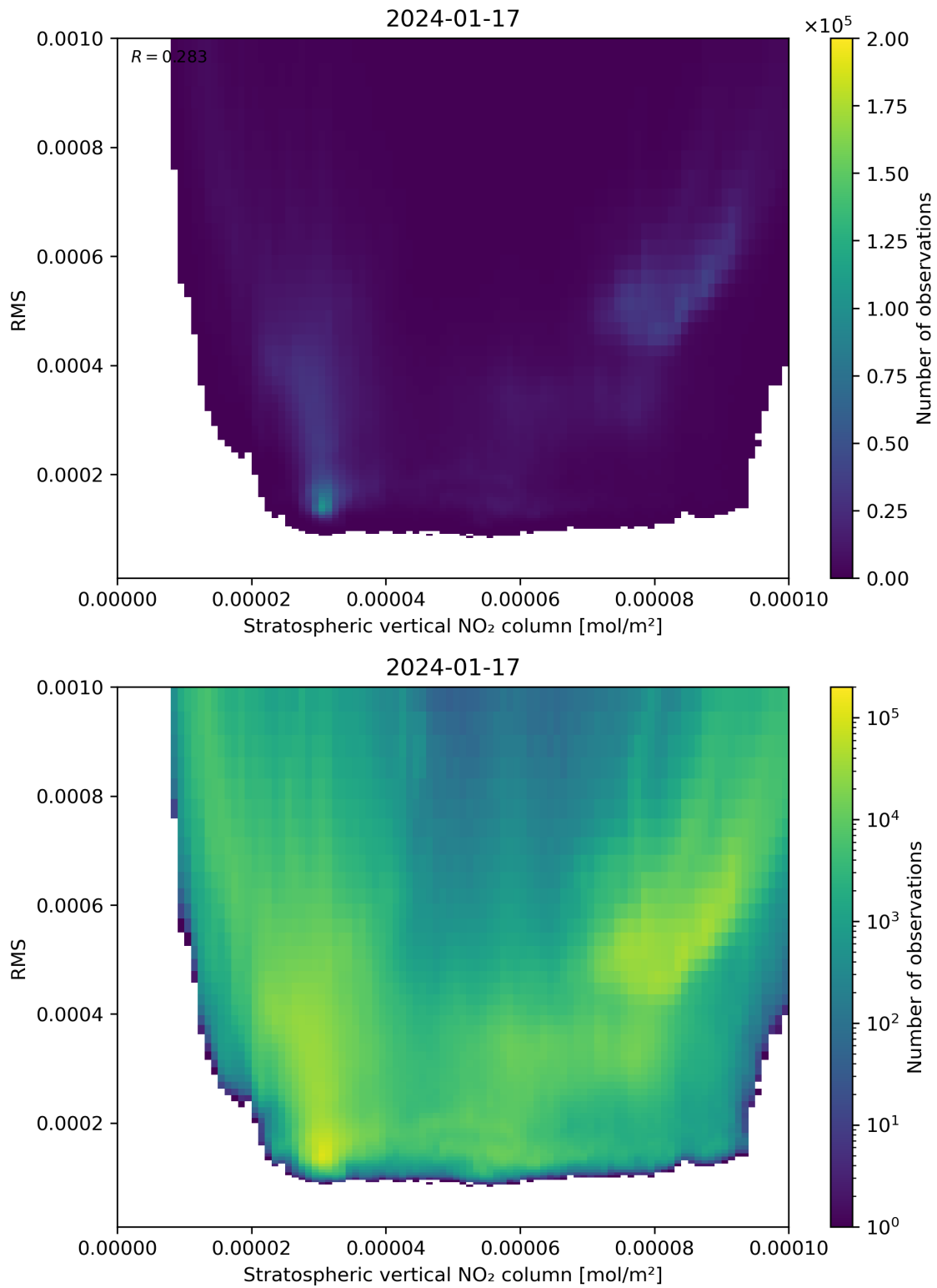
Figure 102: Scatter density plot of “Stratospheric vertical NO 2 column” against “RMS” for 2024-01-16 to 2024-01-18.
