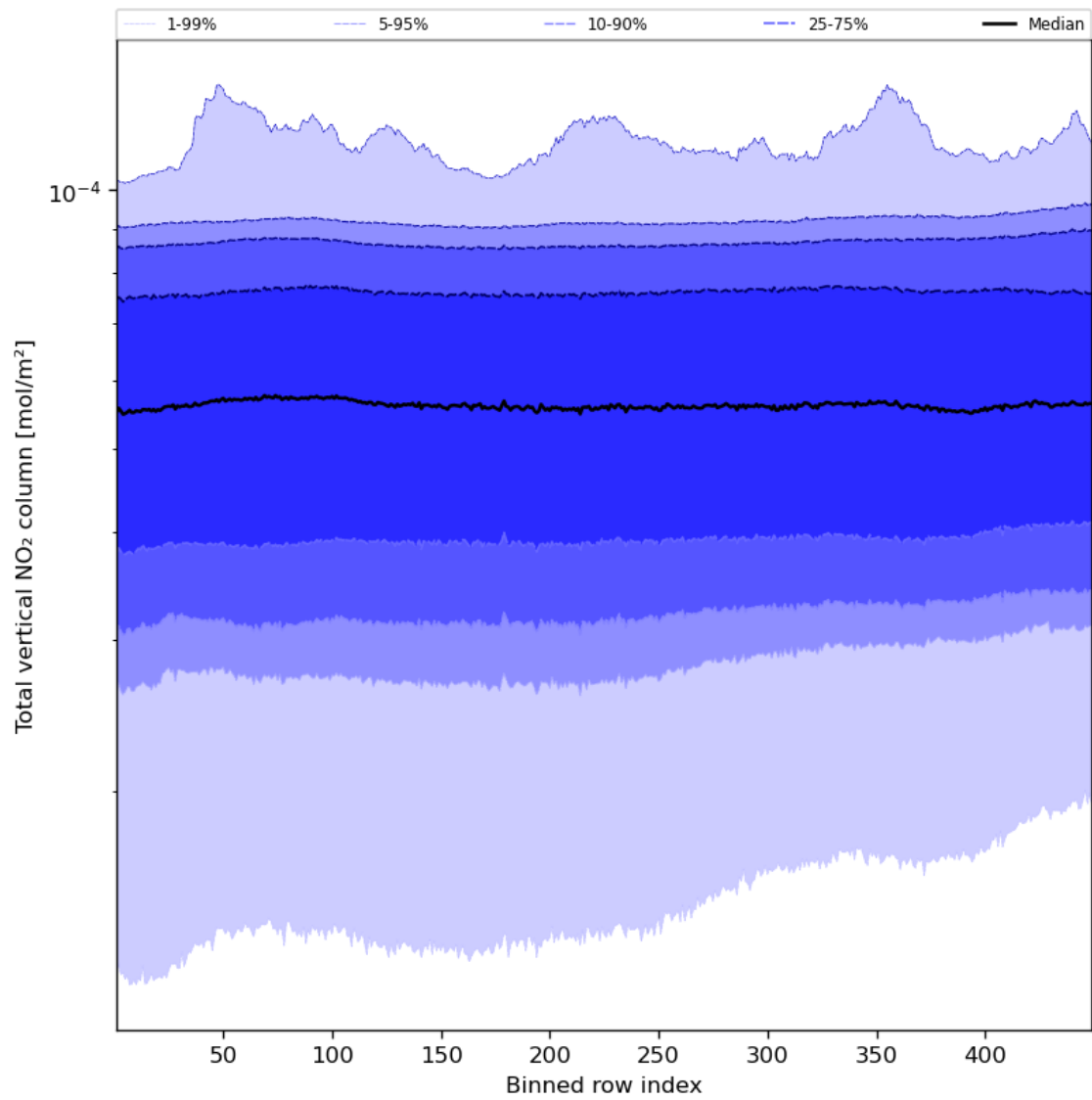
Figure 55: Along track statistics of “Total vertical NO 2 column” for 2024-01-16 to 2024-01-18
