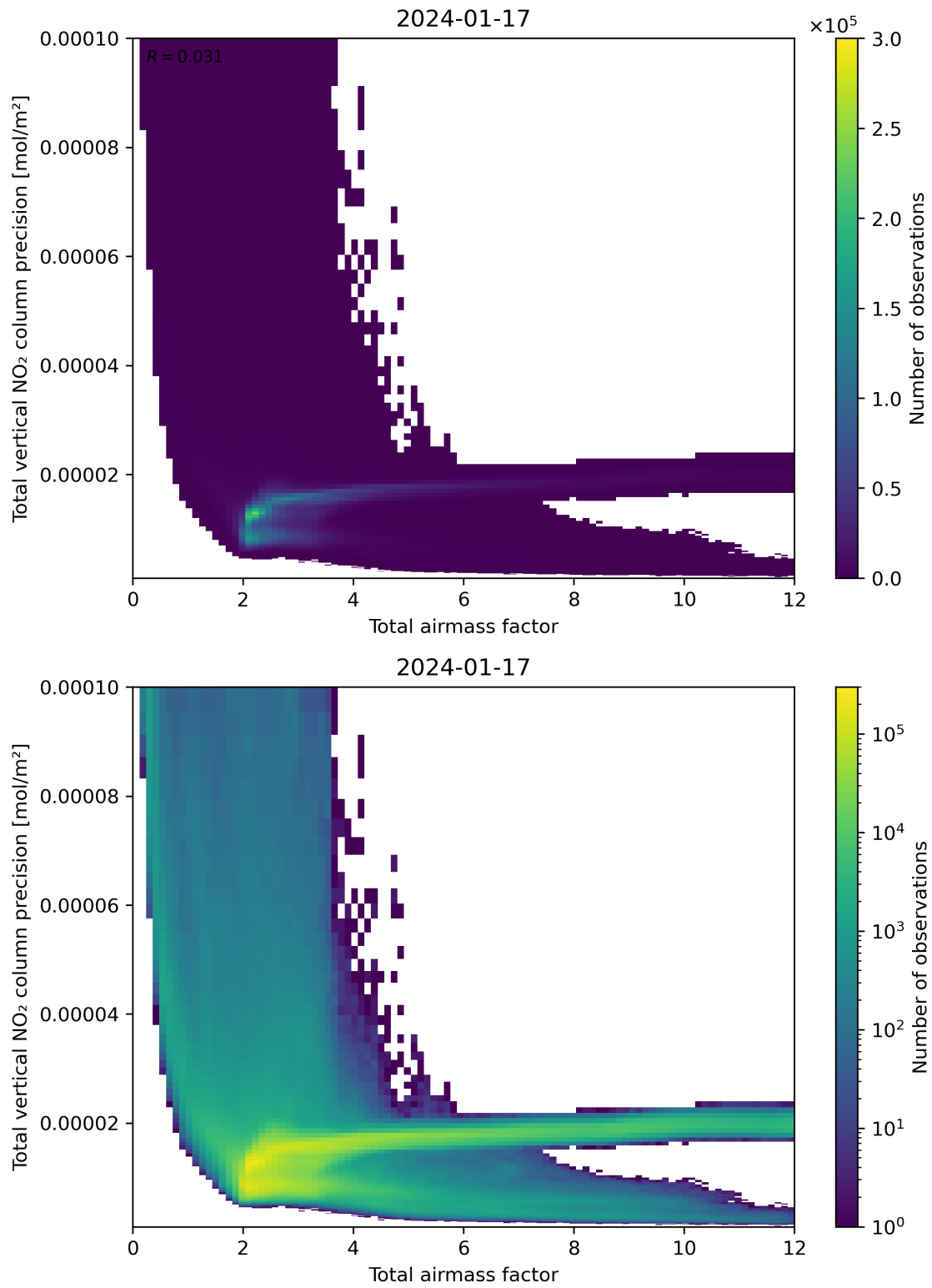
Figure 68: Scatter density plot of “Total airmass factor” against “Total vertical NO 2 column precision” for 2024-01-16 to 2024-01-18.
