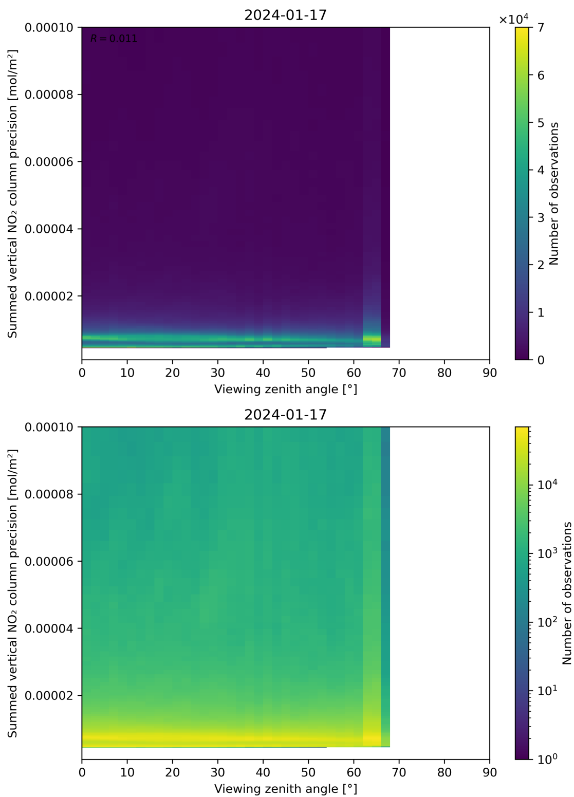
Figure 166: Scatter density plot of “Viewing zenith angle” against “Summed vertical NO 2 column precision” for 2024-01-16 to 2024-01-18.
