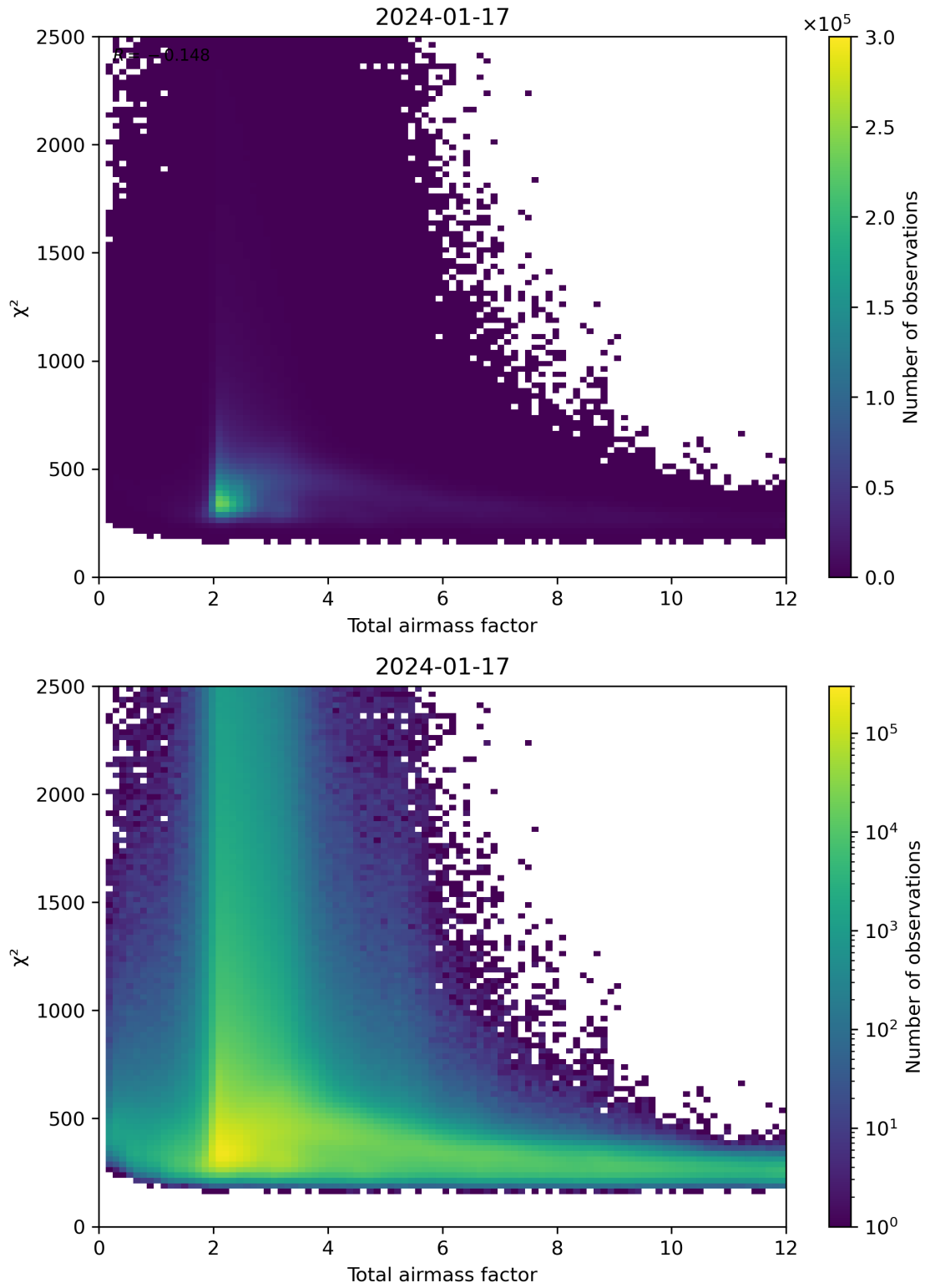
Figure 63: Scatter density plot of “Total airmass factor” against “ \chi^2 ” for 2024-01-16 to 2024-01-18.
