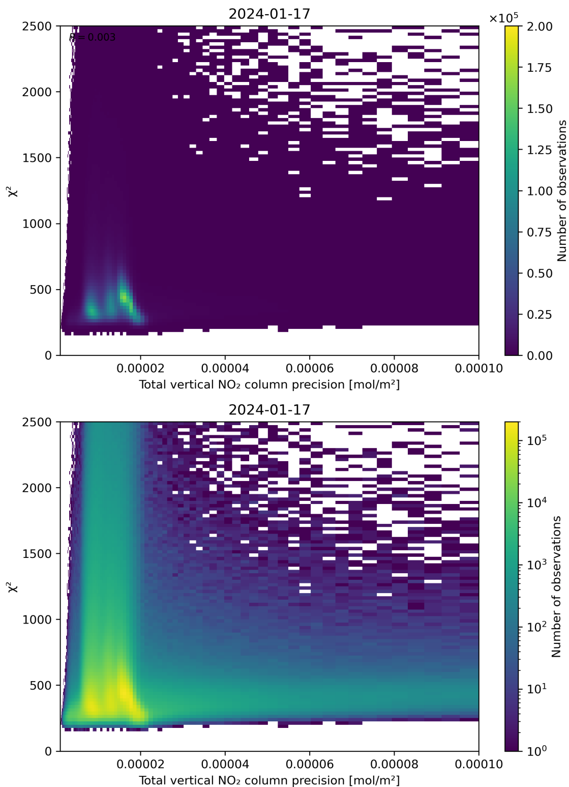
Figure 116: Scatter density plot of “Total vertical NO 2 column precision” against “ \chi^2 ” for 2024-01-16 to 2024-01-18.
