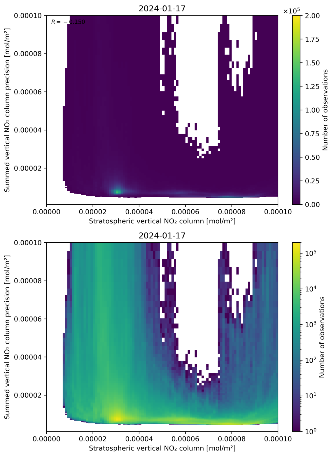
Figure 99: Scatter density plot of “Stratospheric vertical NO 2 column” against “Summed vertical NO 2 column precision” for 2024-01-16 to 2024-01-18.
