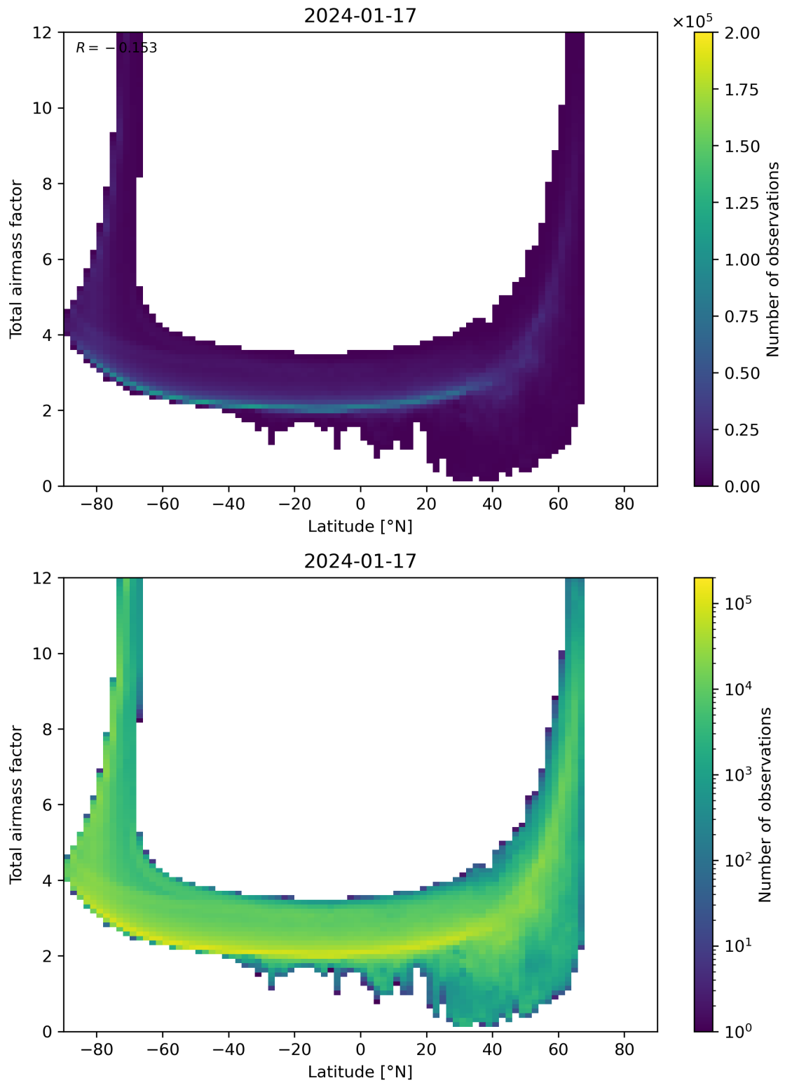
Figure 84: Scatter density plot of “Latitude” against “Total airmass factor” for 2024-01-16 to 2024-01-18.
