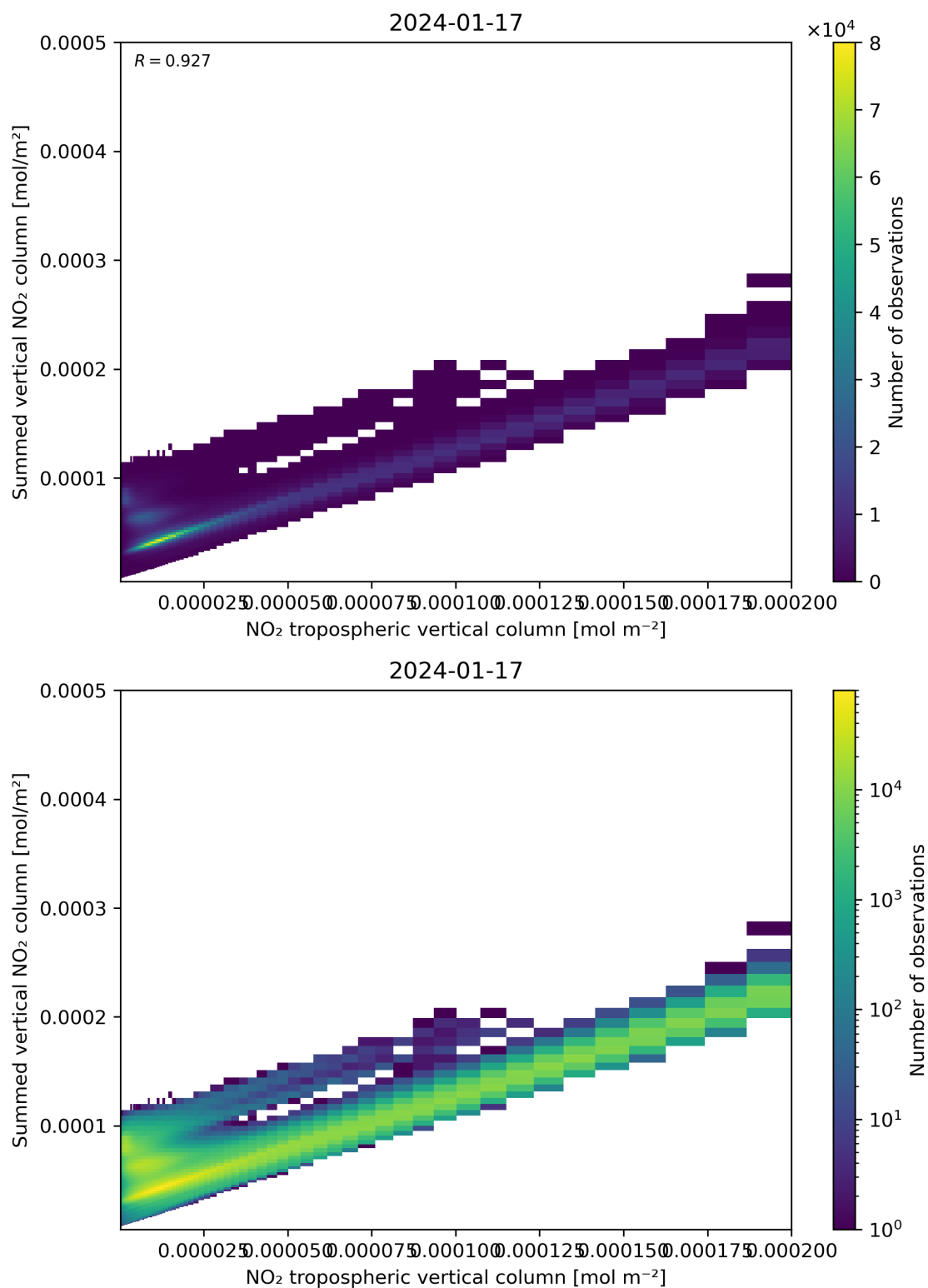
Figure 126: Scatter density plot of “NO 2 tropospheric vertical column” against “Summed vertical NO 2 column” for 2024-01-16 to 2024-01-18.
