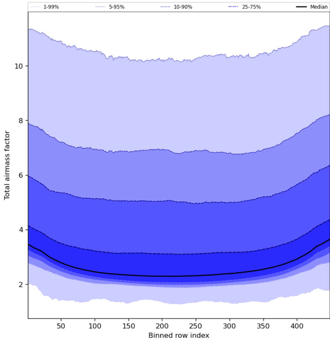
Figure 49: Along track statistics of “Total airmass factor” for 2024-01-16 to 2024-01-18
