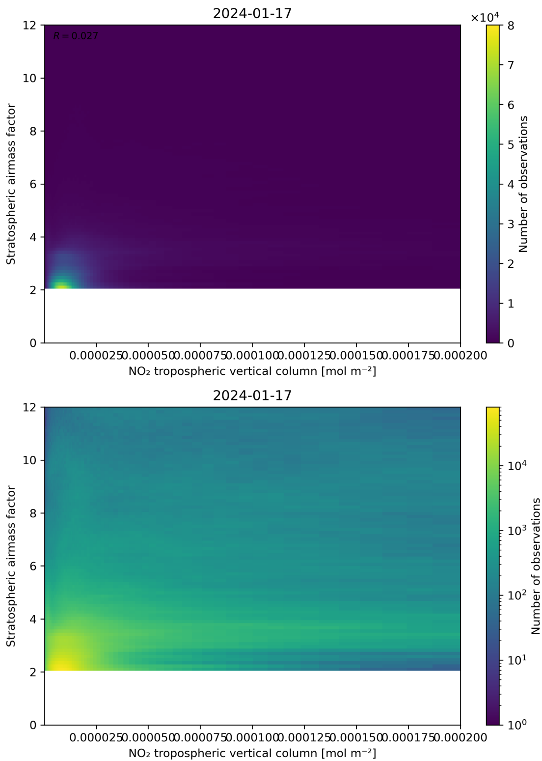
Figure 121: Scatter density plot of “NO 2 tropospheric vertical column” against “Stratospheric airmass factor” for 2024-01-16 to 2024-01-18.
