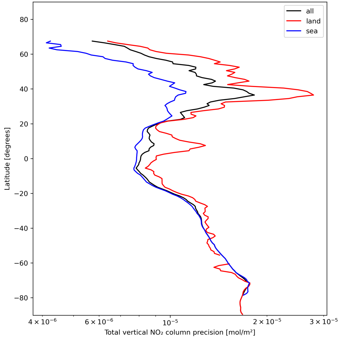
Figure 22: Zonal average of “Total vertical NO 2 column precision” for 2024-01-16 to 2024-01-18.
