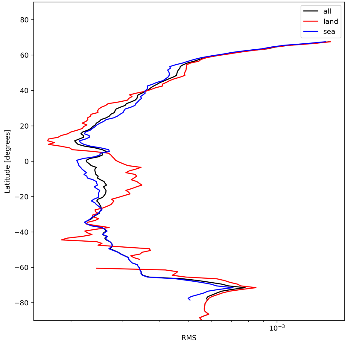
Figure 26: Zonal average of “RMS” for 2024-01-16 to 2024-01-18.
