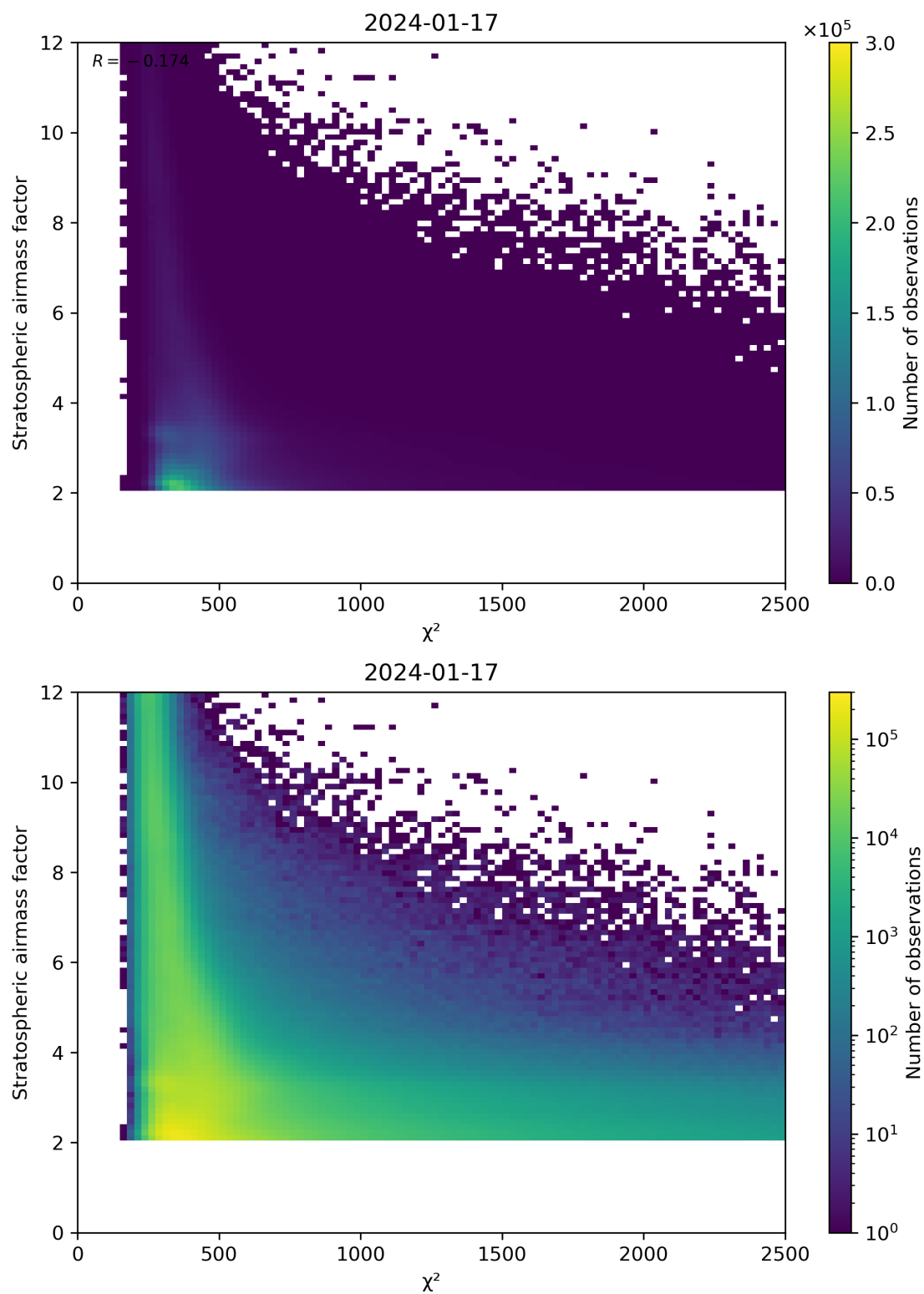
Figure 81: Scatter density plot of “ \chi^2 ” against “Stratospheric airmass factor” for 2024-01-16 to 2024-01-18.
