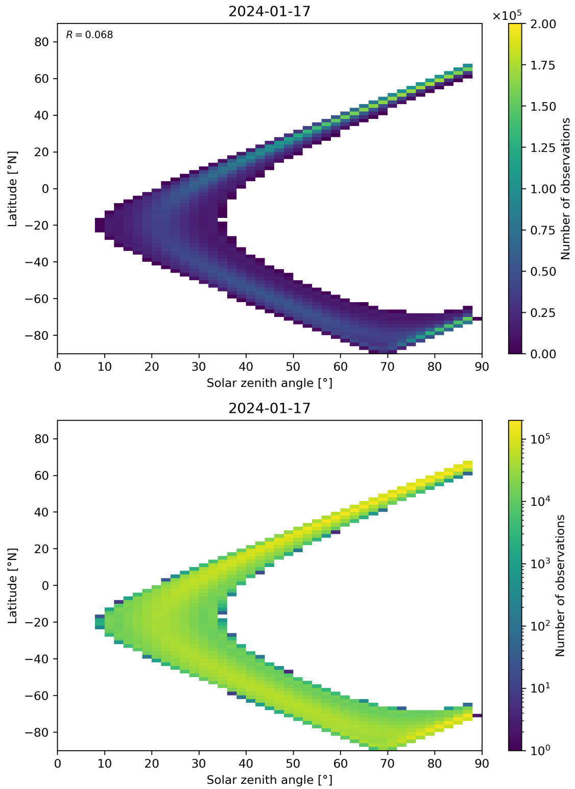
Figure 149: Scatter density plot of “Solar zenith angle” against “Latitude” for 2024-01-16 to 2024-01-18.
