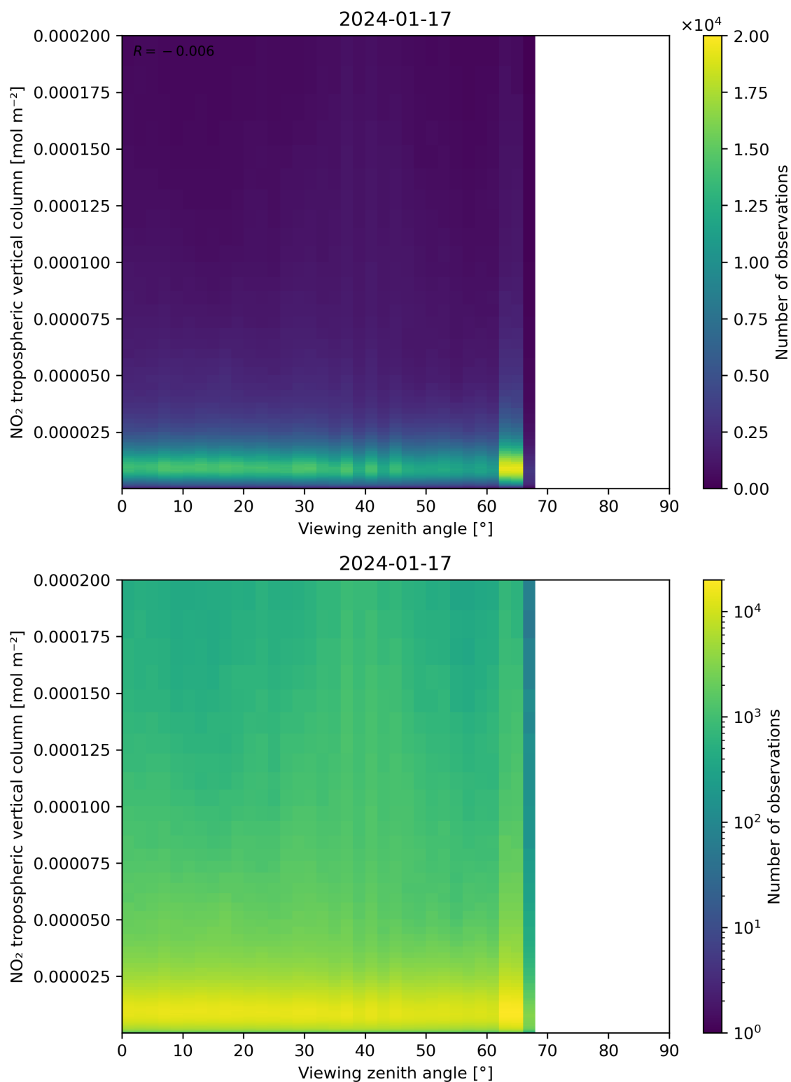
Figure 169: Scatter density plot of “Viewing zenith angle” against “NO 2 tropospheric vertical column” for 2024-01-16 to 2024-01-18.
