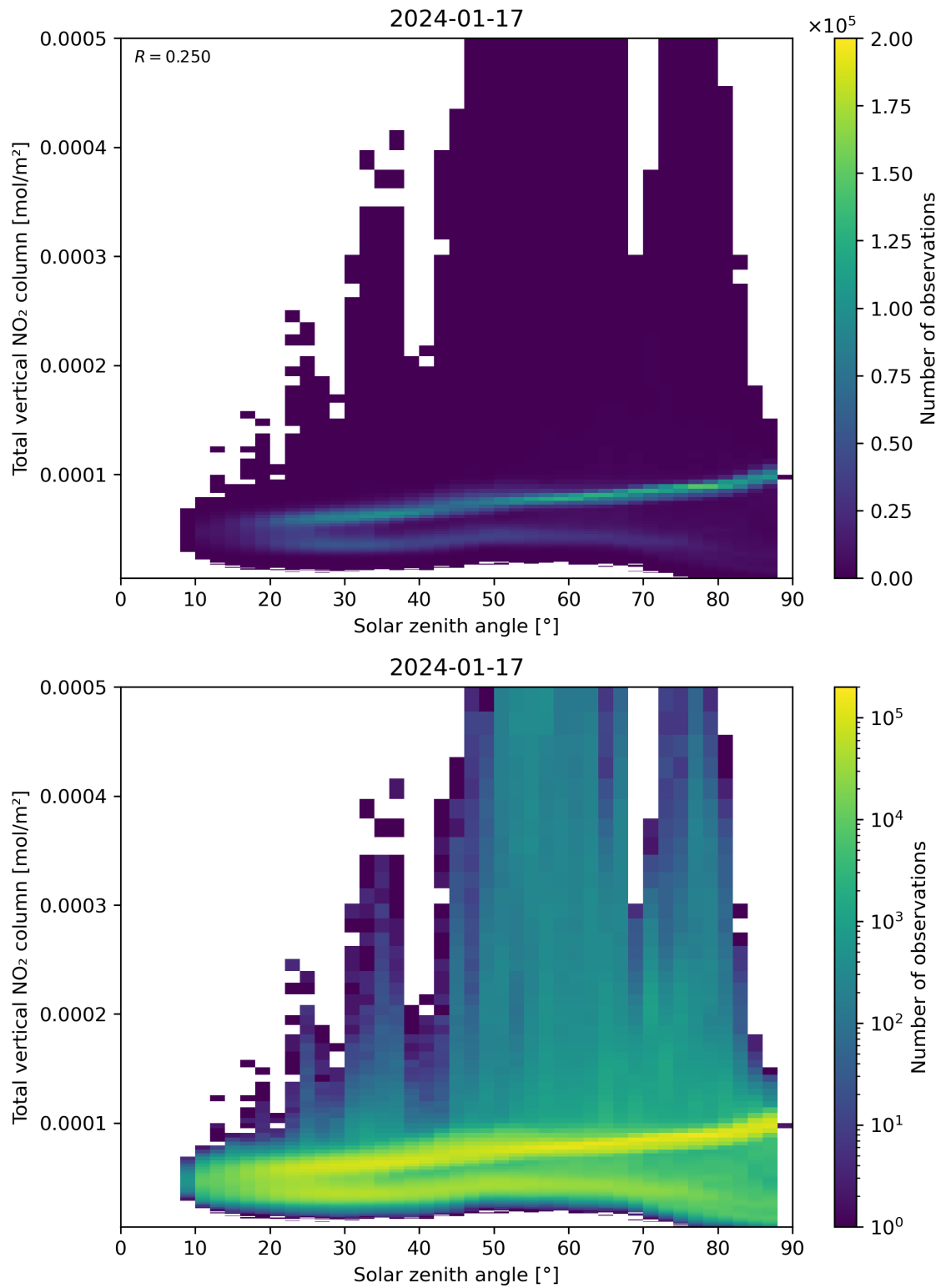
Figure 153: Scatter density plot of “Solar zenith angle” against “Total vertical NO 2 column” for 2024-01-16 to 2024-01-18.
