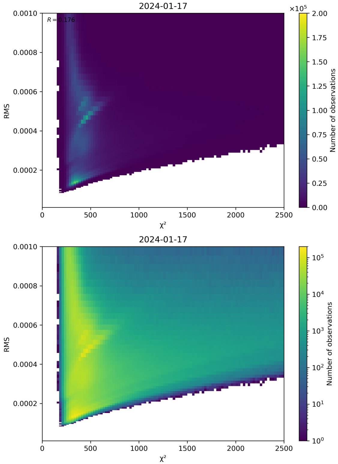
Figure 82: Scatter density plot of “ \chi^2 ” against “RMS” for 2024-01-16 to 2024-01-18.
