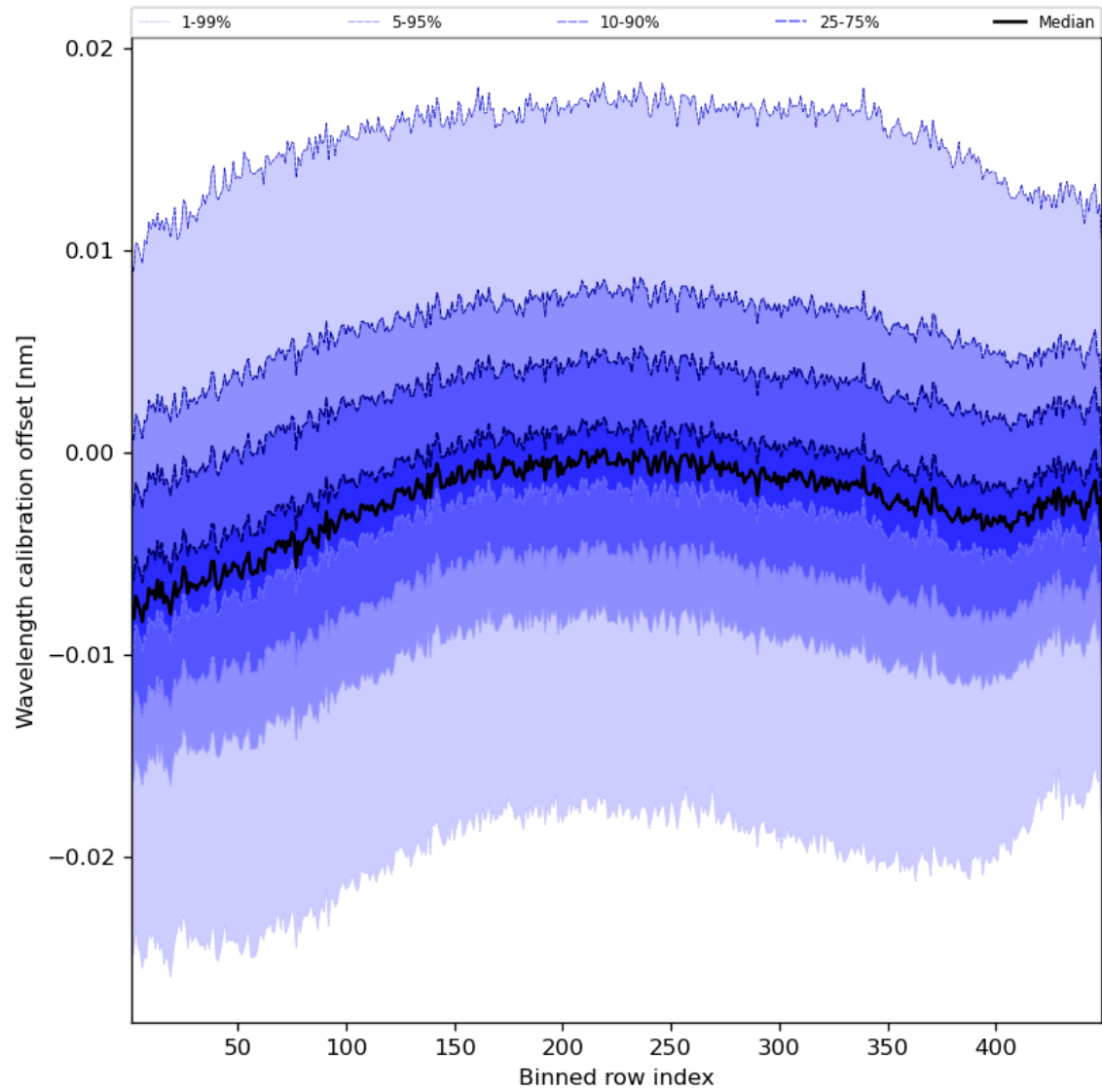
Figure 52: Along track statistics of “Wavelength calibration offset” for 2024-01-16 to 2024-01-18
