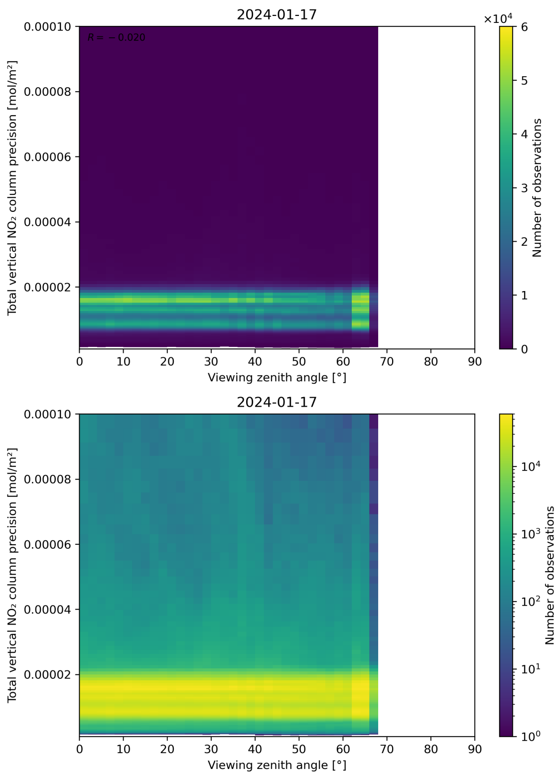
Figure 168: Scatter density plot of “Viewing zenith angle” against “Total vertical NO 2 column precision” for 2024-01-16 to 2024-01-18.
