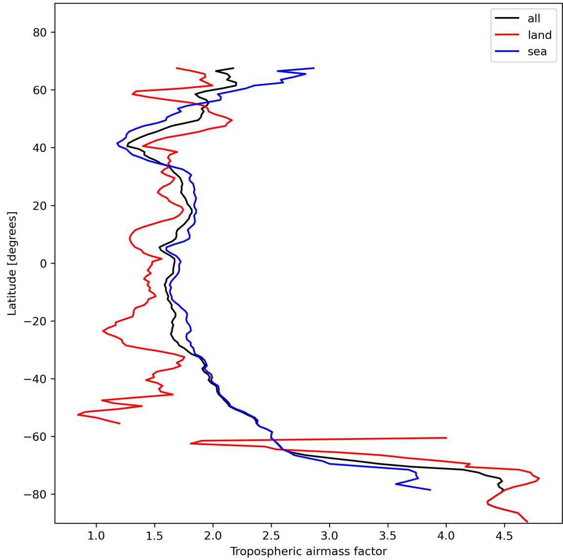
Figure 14: Zonal average of “Tropospheric airmass factor” for 2024-01-16 to 2024-01-18.
