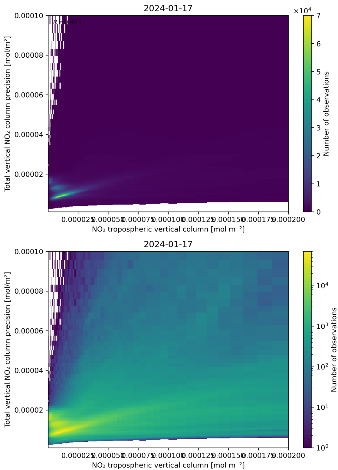
Figure 129: Scatter density plot of “NO 2 tropospheric vertical column” against “Total vertical NO 2 column precision” for 2024-01-16 to 2024-01-18.
