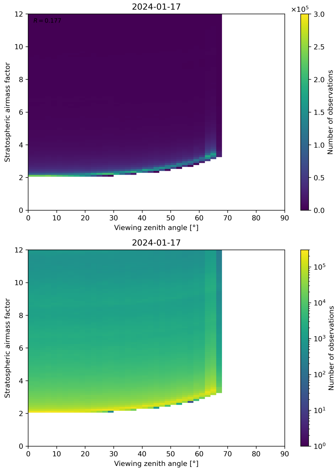
Figure 159: Scatter density plot of “Viewing zenith angle” against “Stratospheric airmass factor” for 2024-01-16 to 2024-01-18.
