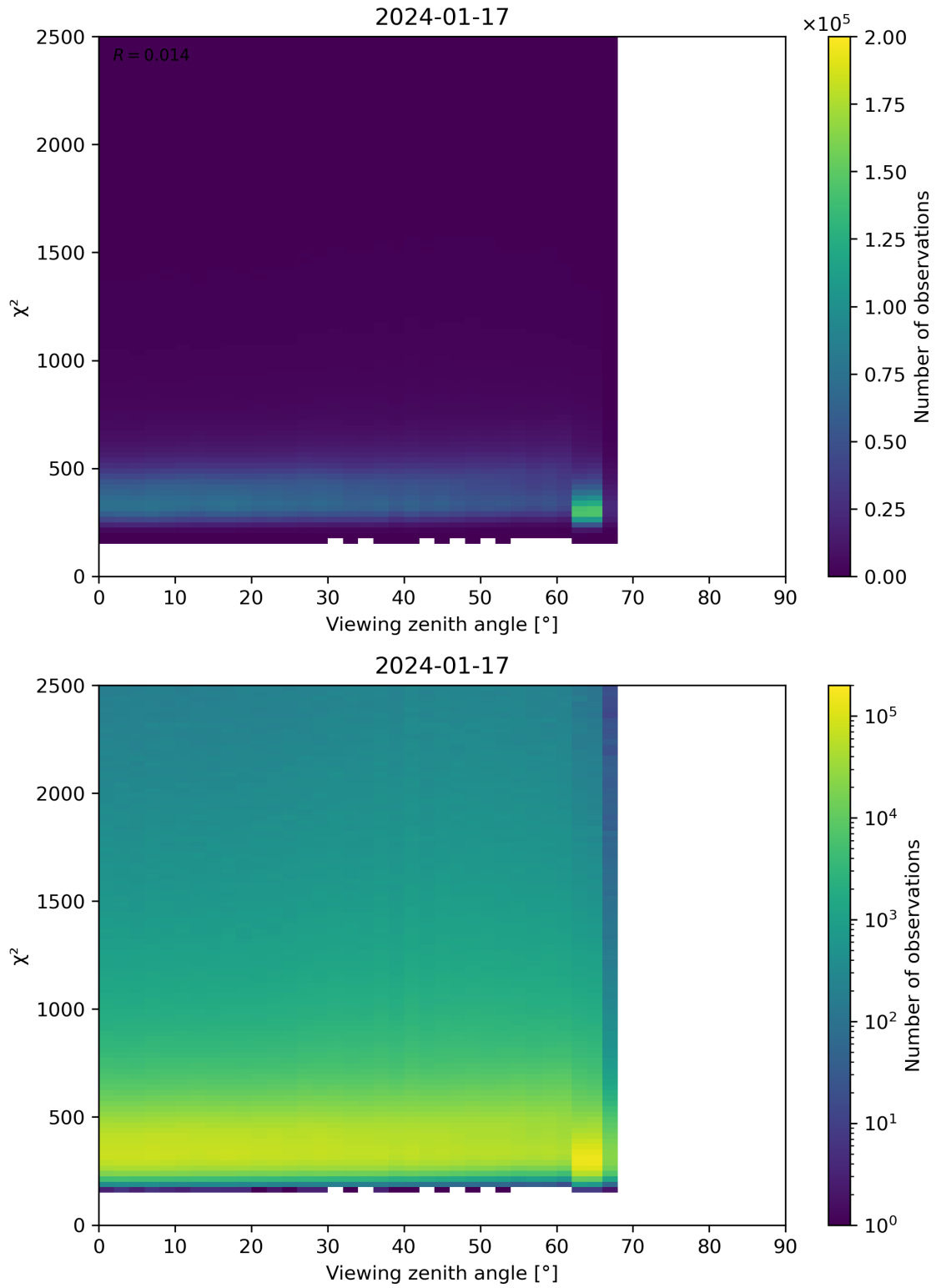
Figure 162: Scatter density plot of “Viewing zenith angle” against “ \chi^2 ” for 2024-01-16 to 2024-01-18.
