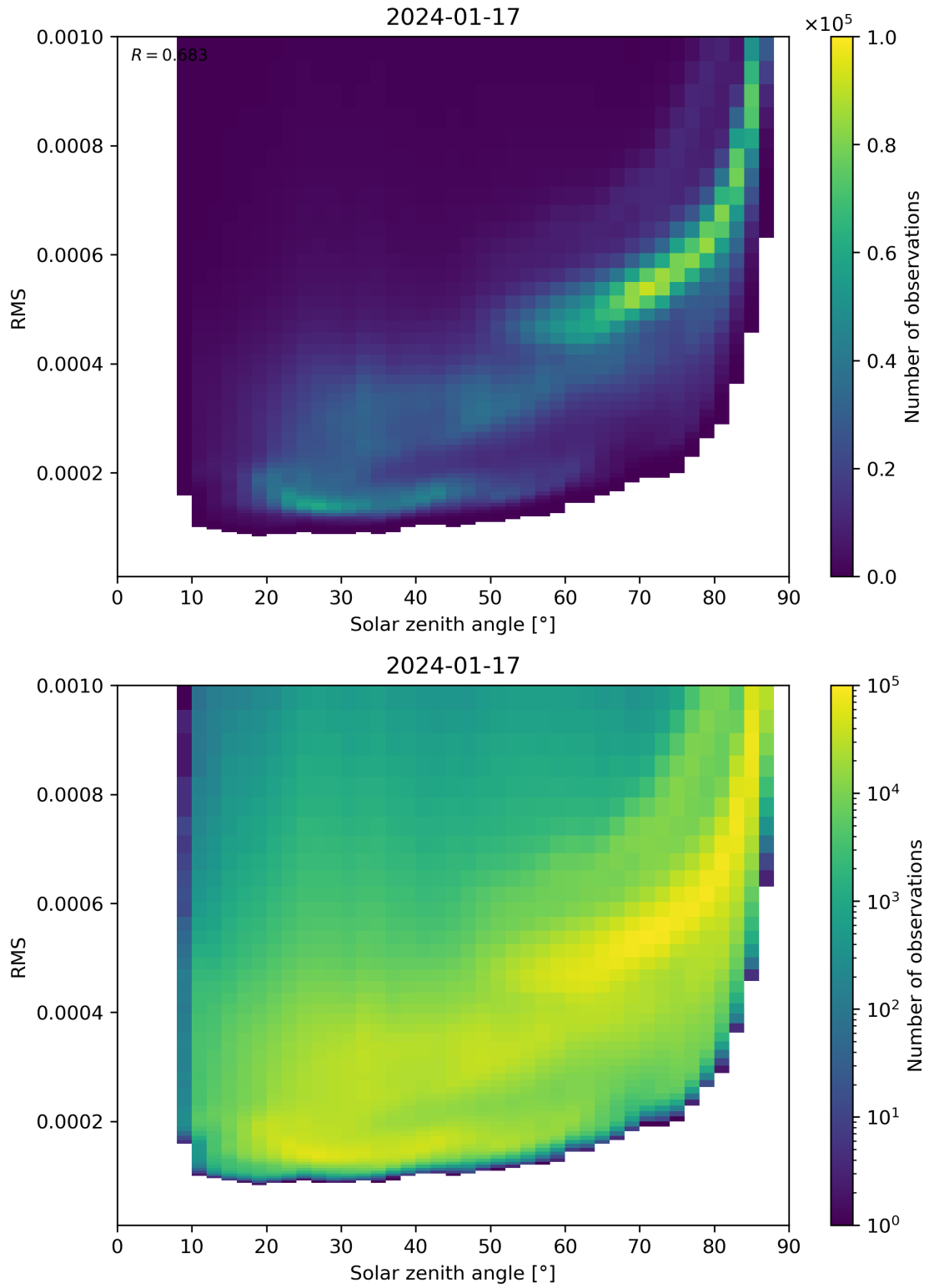
Figure 157: Scatter density plot of “Solar zenith angle” against “RMS” for 2024-01-16 to 2024-01-18.
