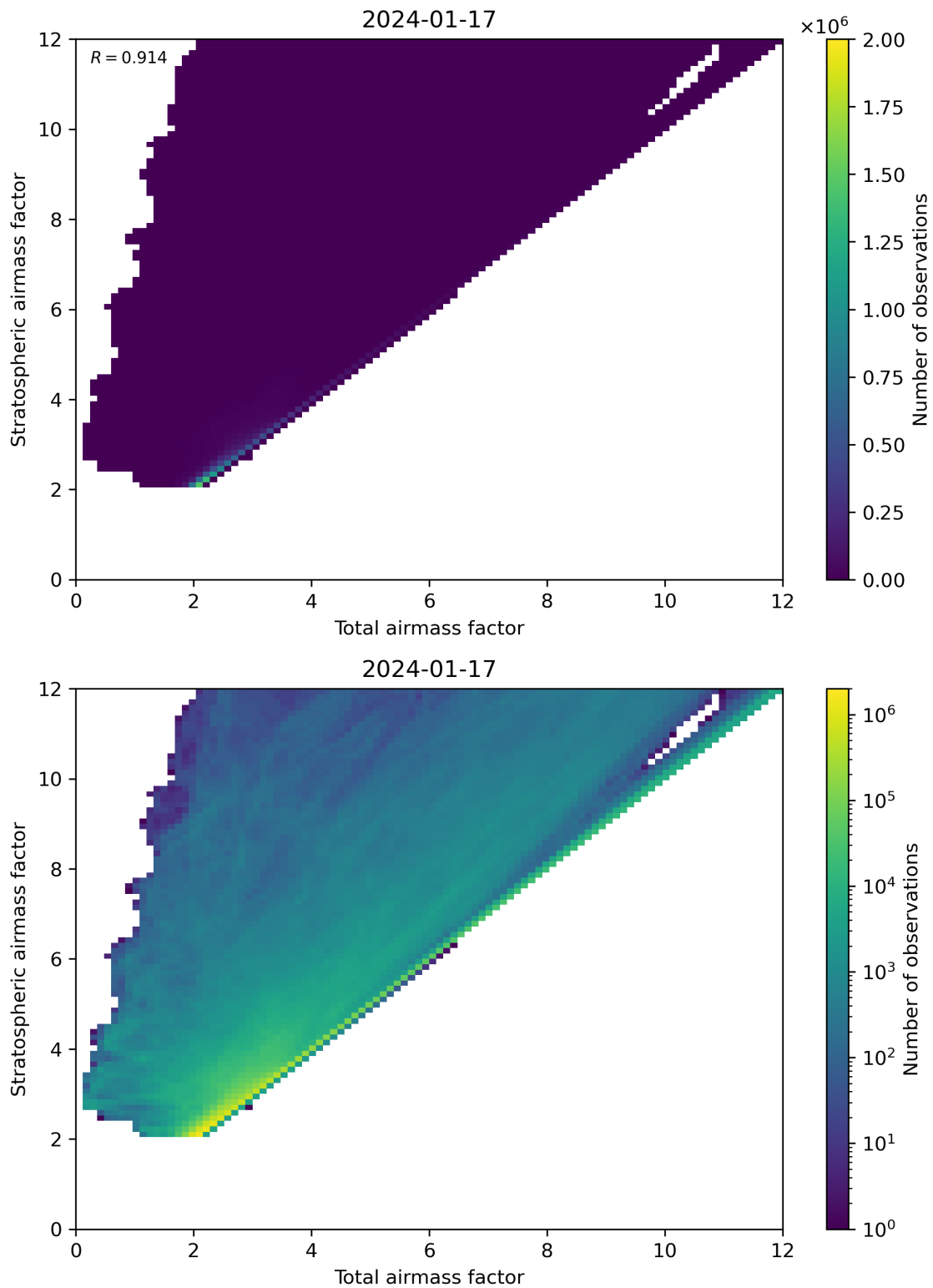
Figure 62: Scatter density plot of “Total airmass factor” against “Stratospheric airmass factor” for 2024-01-16 to 2024-01-18.
