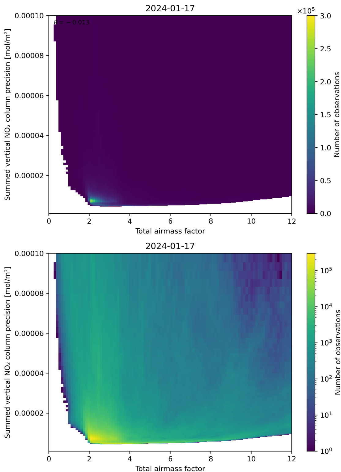
Figure 66: Scatter density plot of “Total airmass factor” against “Summed vertical NO 2 column precision” for 2024-01-16 to 2024-01-18.
