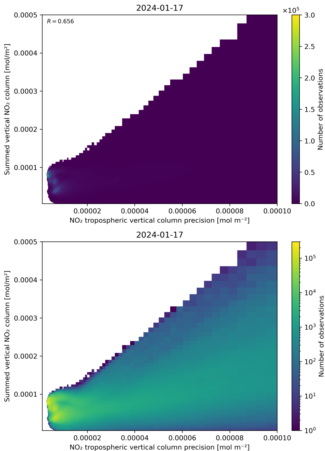
Figure 136: Scatter density plot of “NO 2 tropospheric vertical column precision” against “Summed vertical NO 2 column” for 2024-01-16 to 2024-01-18.
