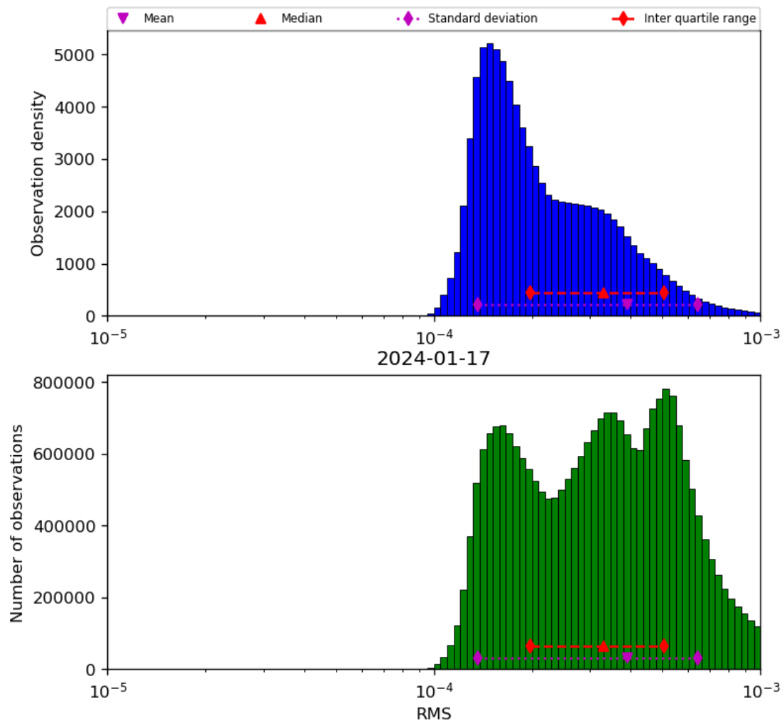
Figure 43: Histogram of “RMS” for 2024-01-16 to 2024-01-18
