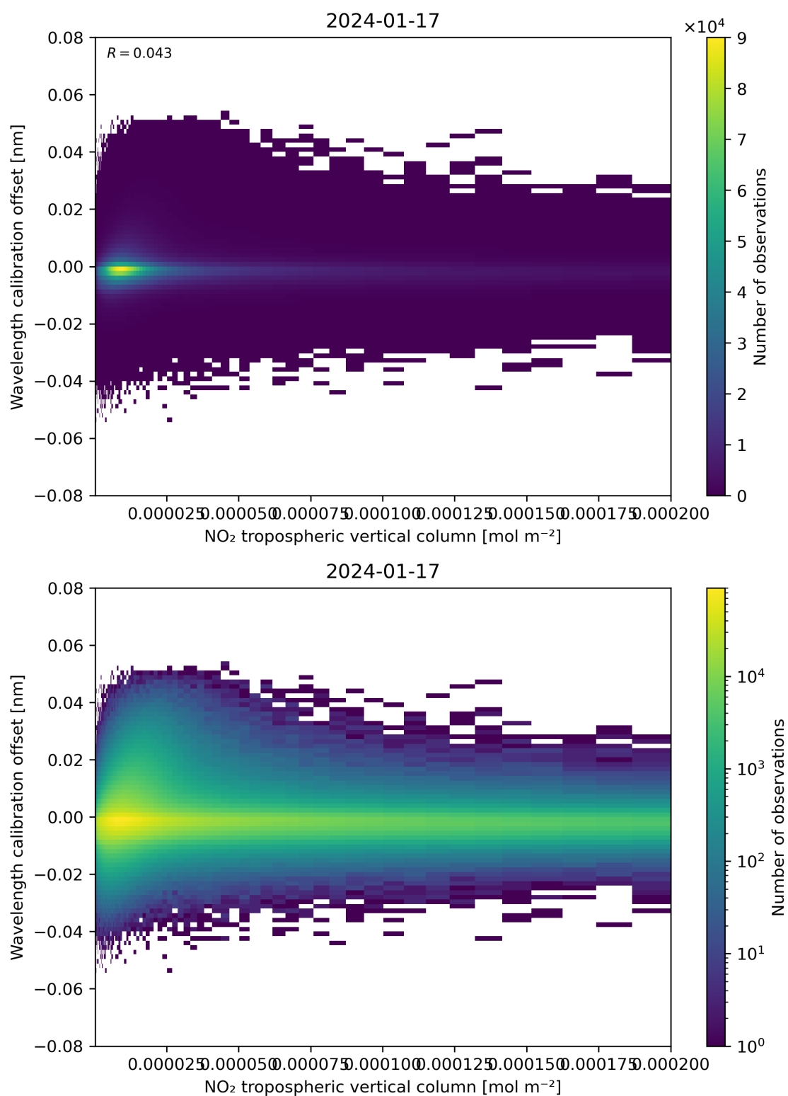
Figure 143: Scatter density plot of “NO 2 tropospheric vertical column” against “Wavelength calibration offset” for 2024-01-16 to 2024-01-18.
