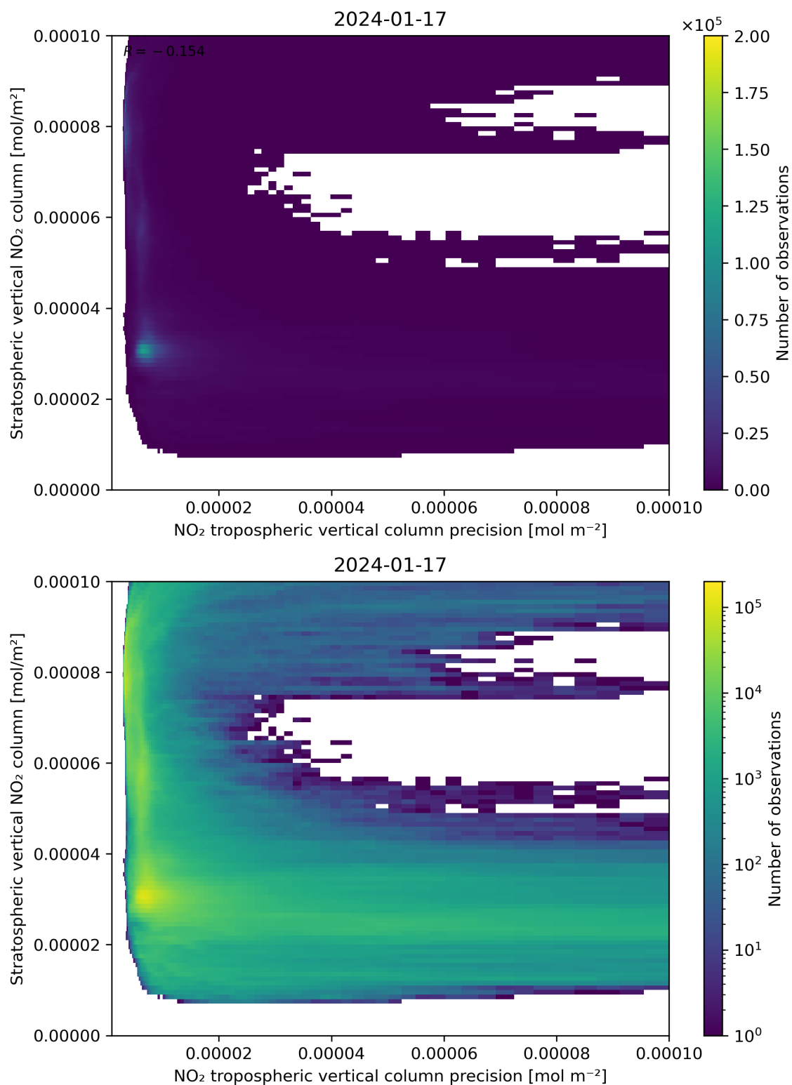
Figure 135: Scatter density plot of “NO 2 tropospheric vertical column precision” against “Stratospheric vertical NO 2 column” for 2024-01-16 to 2024-01-18.
