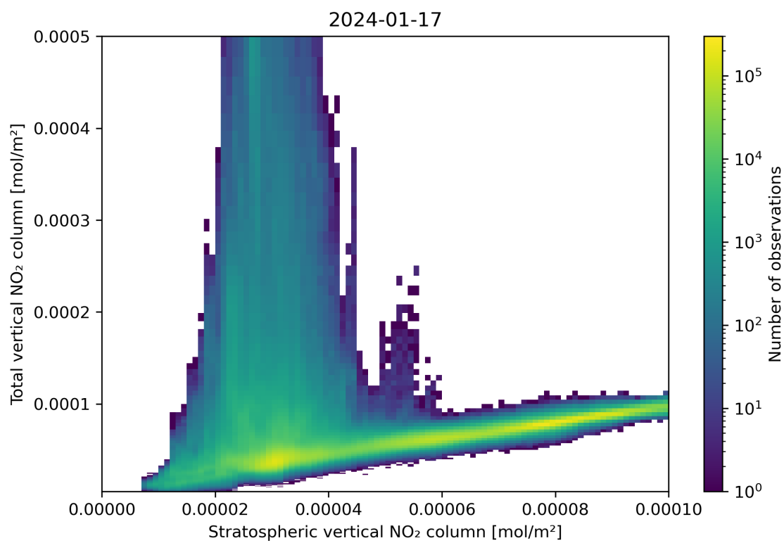
Figure 100: Scatter density plot of “Stratospheric vertical NO 2 column” against “Total vertical NO 2 column” for 2024-01-16 to 2024-01-18.
