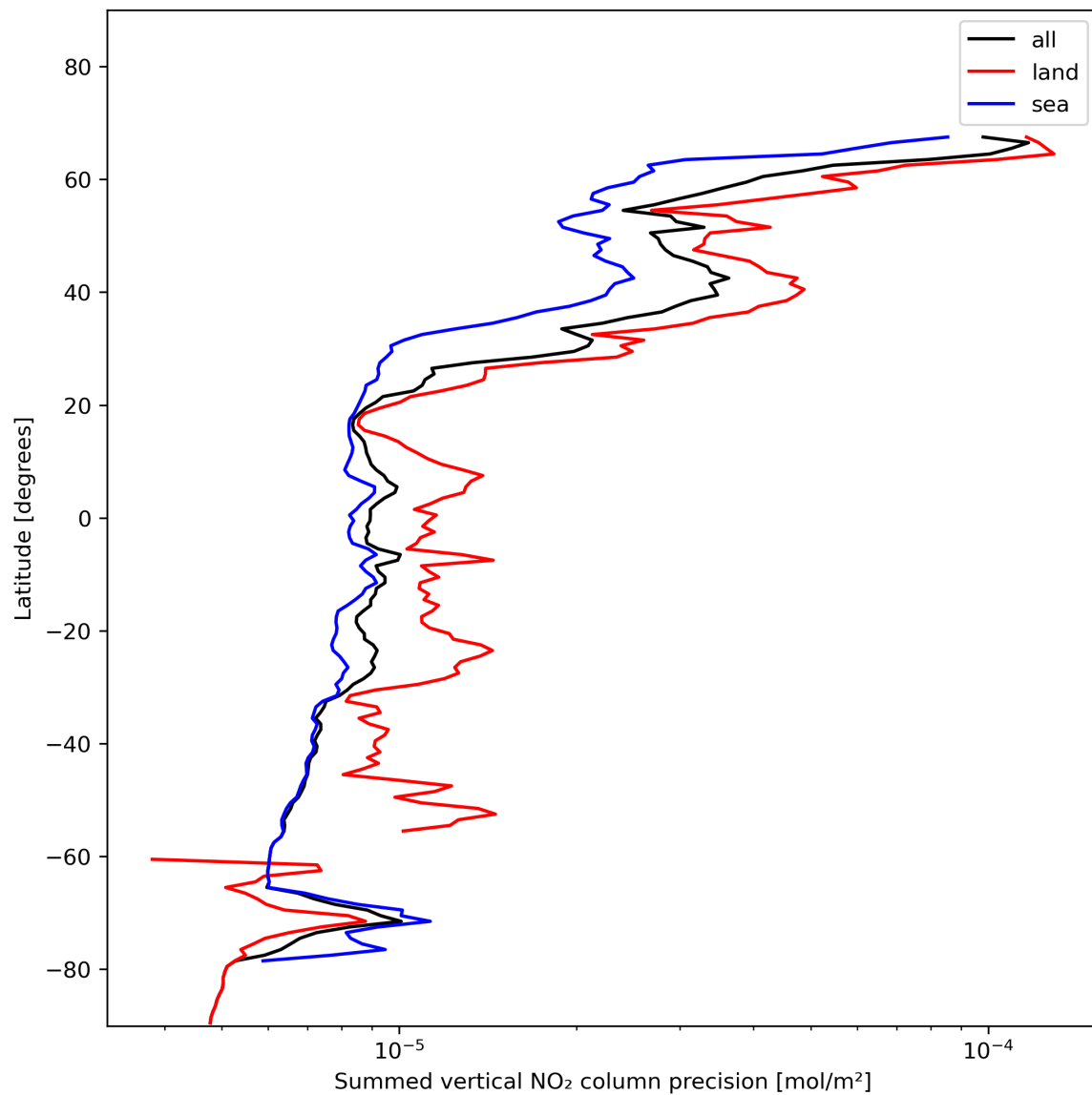
Figure 24: Zonal average of “Summed vertical NO 2 column precision” for 2024-01-16 to 2024-01-18.
