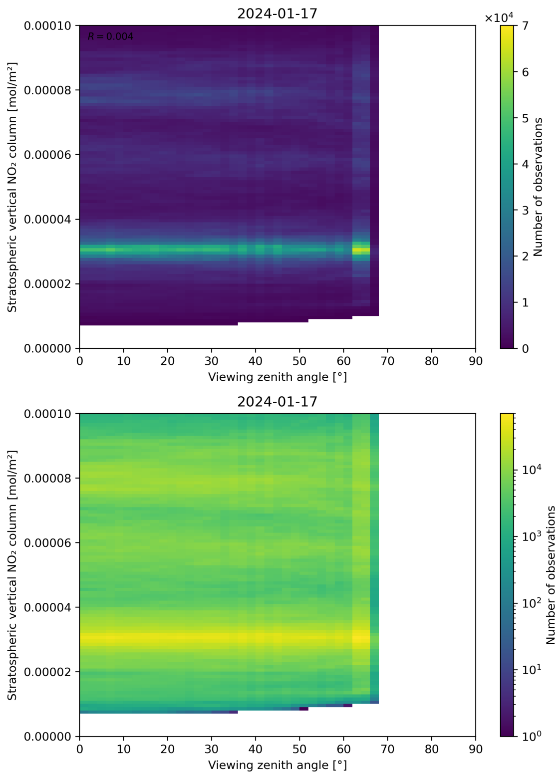
Figure 164: Scatter density plot of “Viewing zenith angle” against “Stratospheric vertical NO 2 column” for 2024-01-16 to 2024-01-18.
