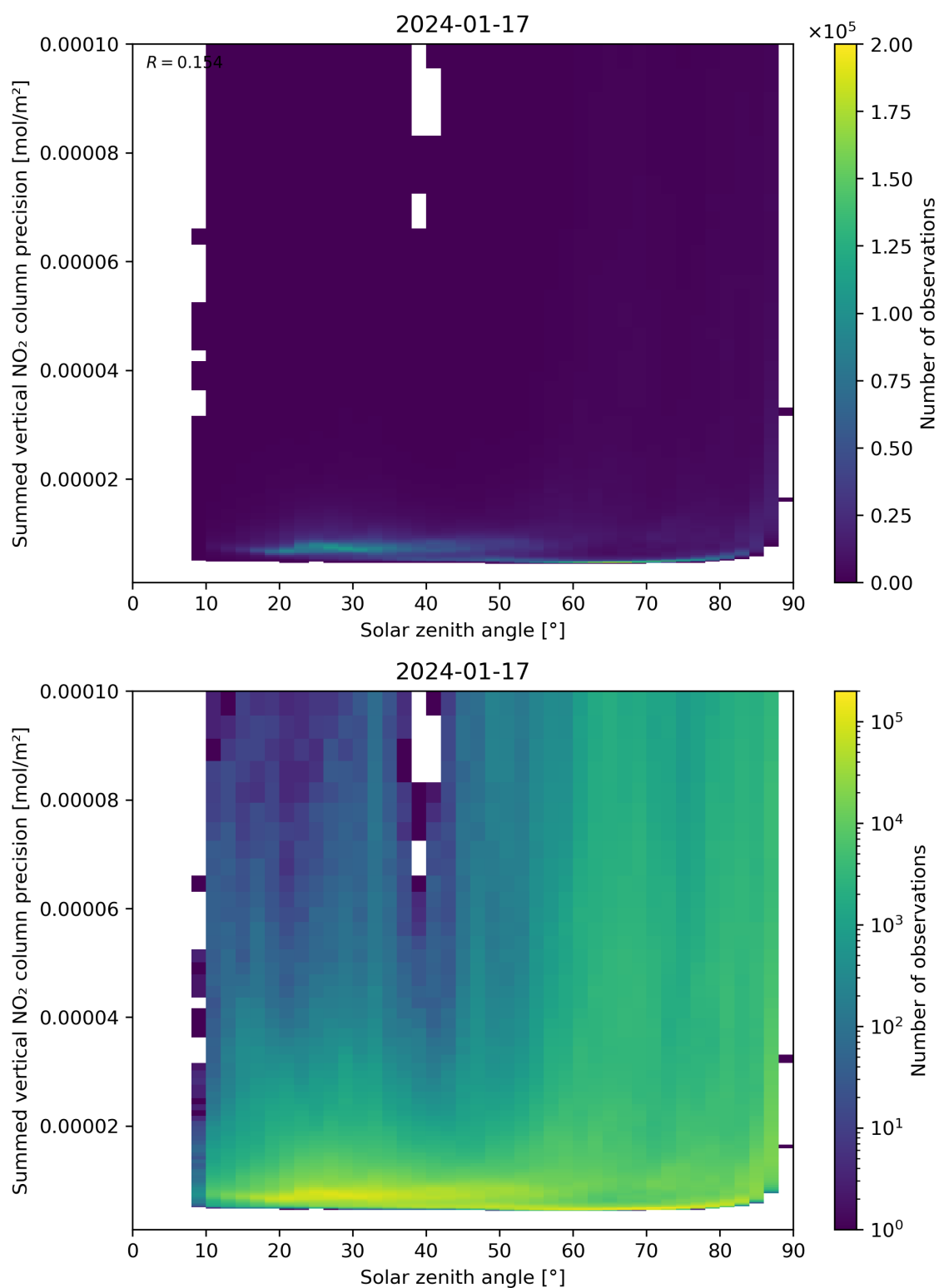
Figure 152: Scatter density plot of “Solar zenith angle” against “Summed vertical NO 2 column precision” for 2024-01-16 to 2024-01-18.
