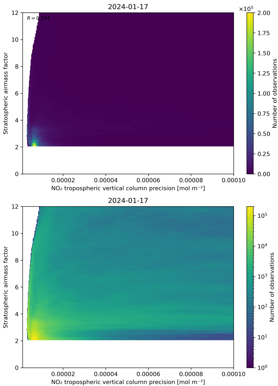
Figure 131: Scatter density plot of “NO 2 tropospheric vertical column precision” against “Stratospheric airmass factor” for 2024-01-16 to 2024-01-18.
