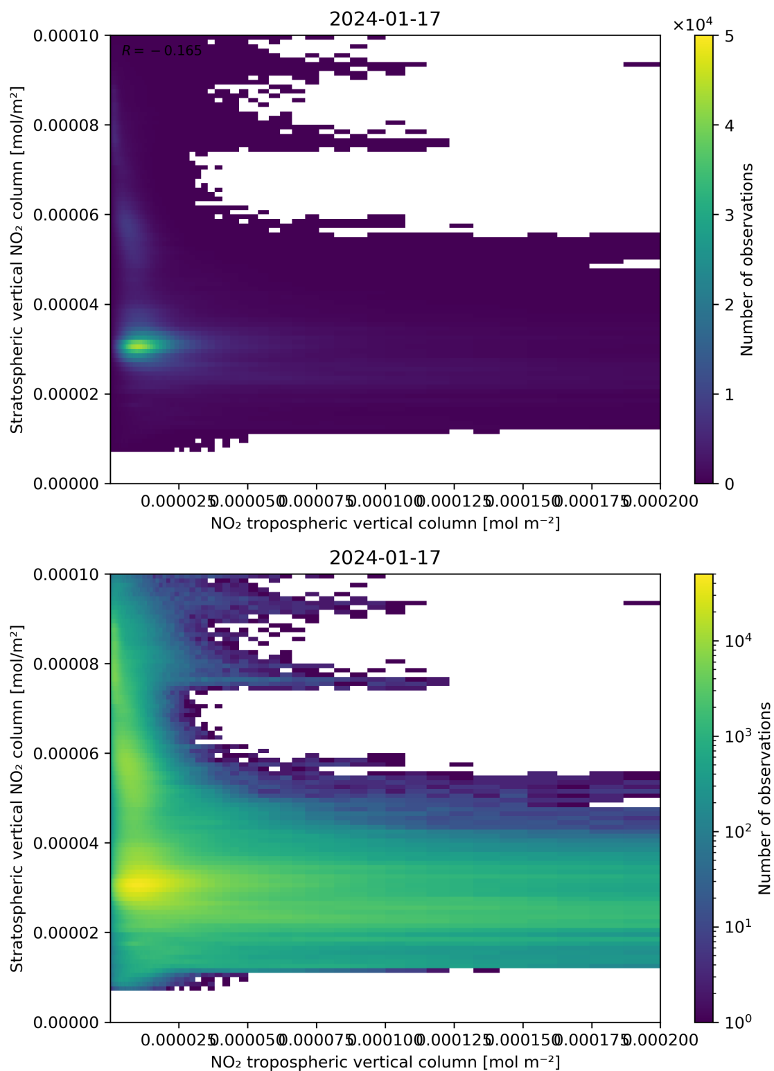
Figure 125: Scatter density plot of “NO 2 tropospheric vertical column” against “Stratospheric vertical NO 2 column” for 2024-01-16 to 2024-01-18.
