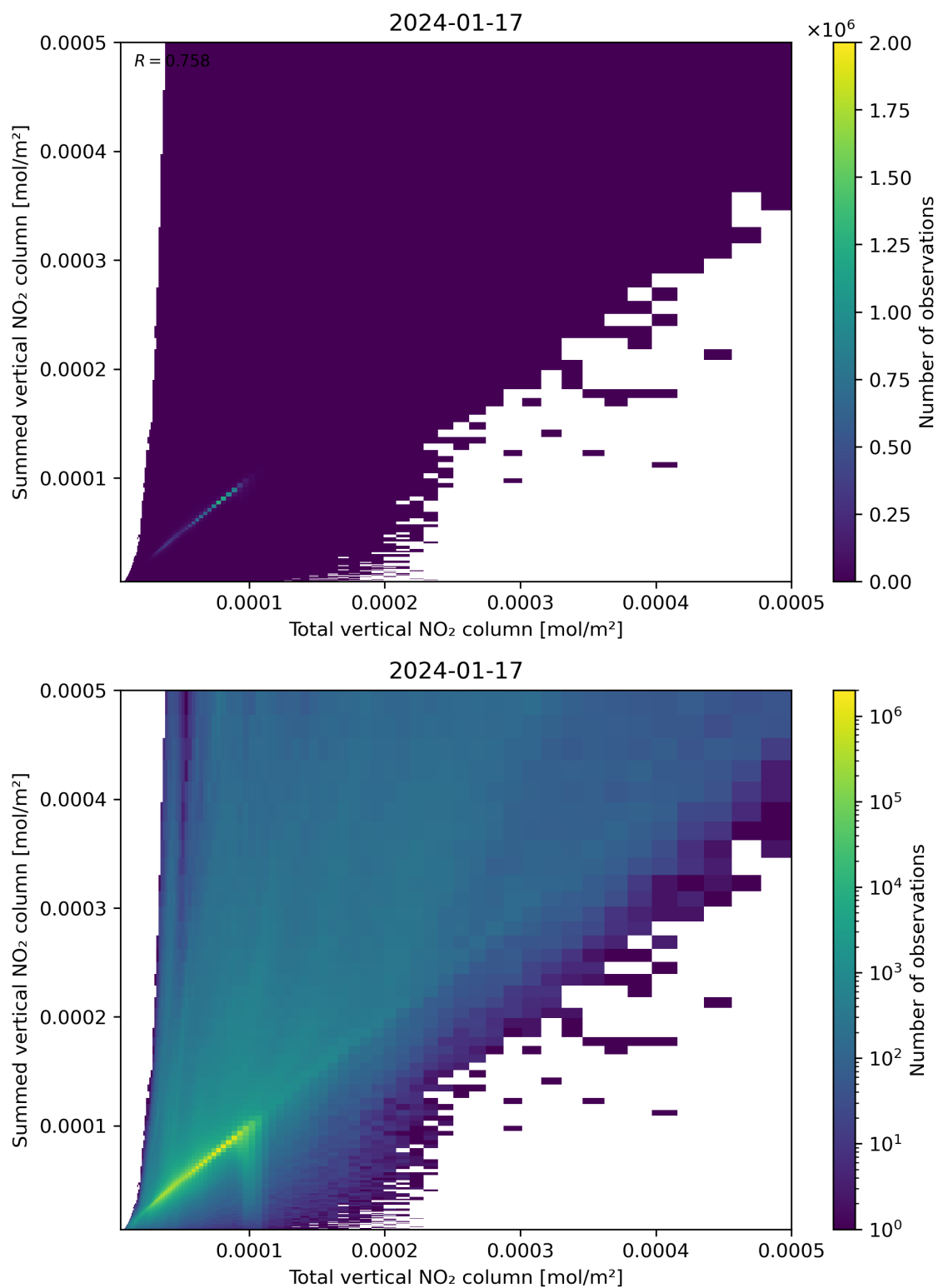
Figure 112: Scatter density plot of “Total vertical NO 2 column” against “Summed vertical NO 2 column” for 2024-01-16 to 2024-01-18.
