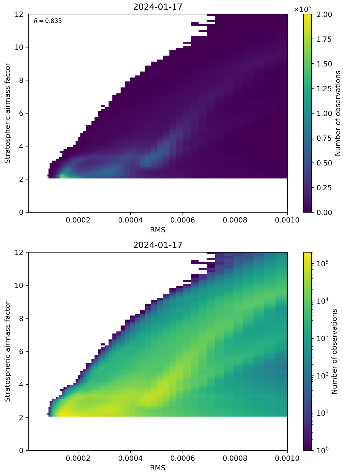
Figure 144: Scatter density plot of “RMS” against “Stratospheric airmass factor” for 2024-01-16 to 2024-01-18.
