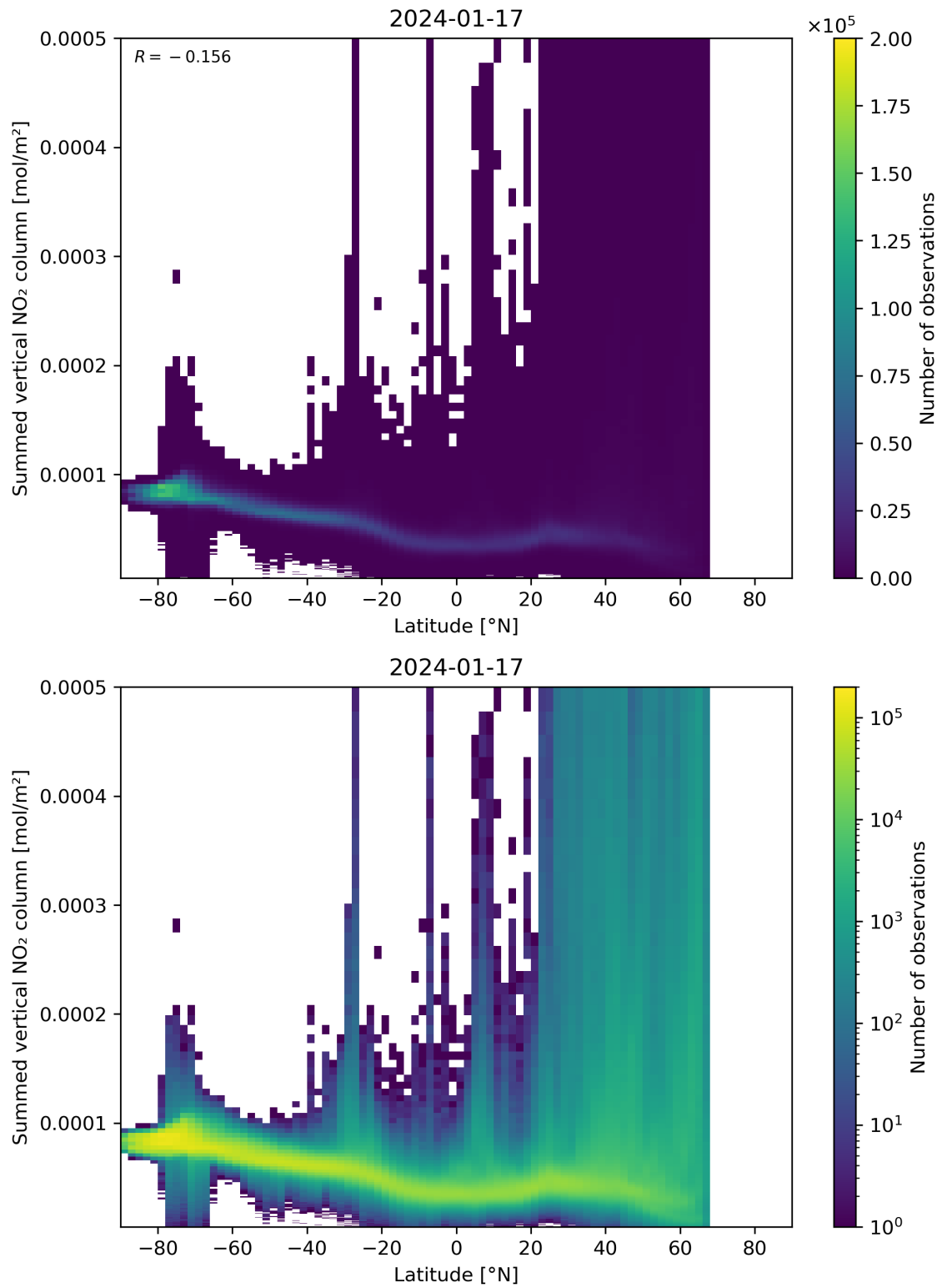
Figure 88: Scatter density plot of “Latitude” against “Summed vertical NO 2 column” for 2024-01-16 to 2024-01-18.
