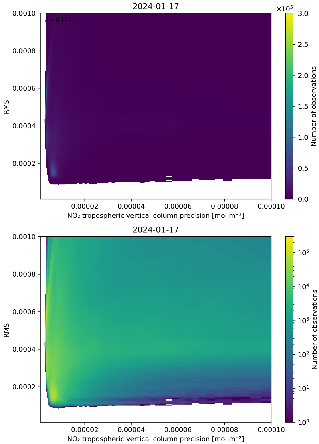
Figure 140: Scatter density plot of “NO 2 tropospheric vertical column precision” against “RMS” for 2024-01-16 to 2024-01-18.
