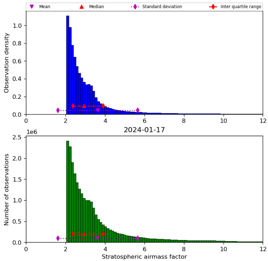
Figure 44: Histogram of “Stratospheric airmass factor” for 2024-01-16 to 2024-01-18
