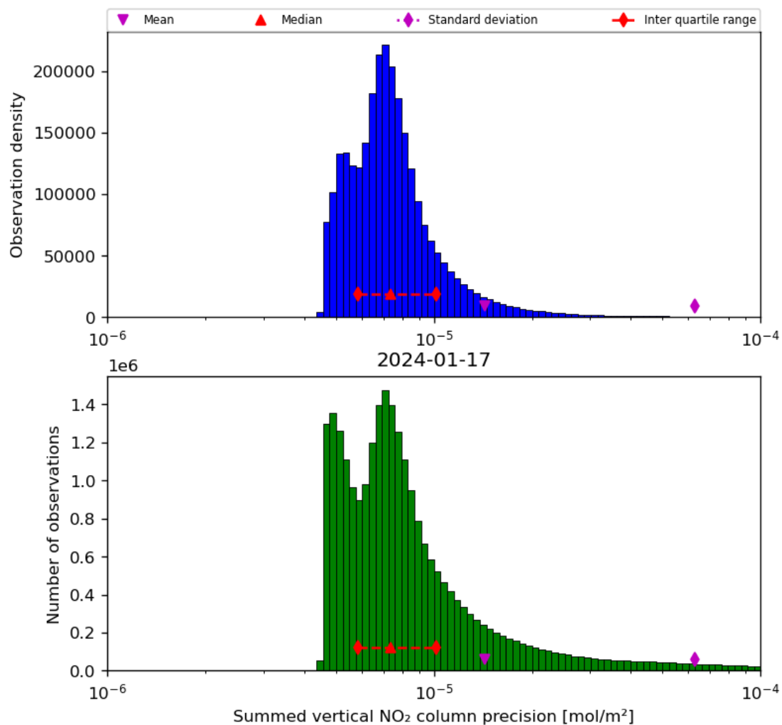
Figure 41: Histogram of “Summed vertical NO 2 column precision” for 2024-01-16 to 2024-01-18
