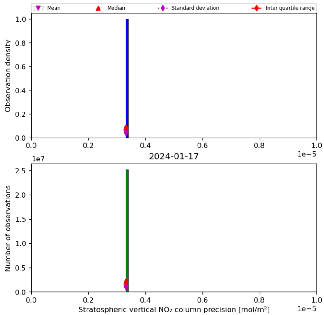
Figure 37: Histogram of “Stratospheric vertical NO 2 column precision” for 2024-01-16 to 2024-01-18
