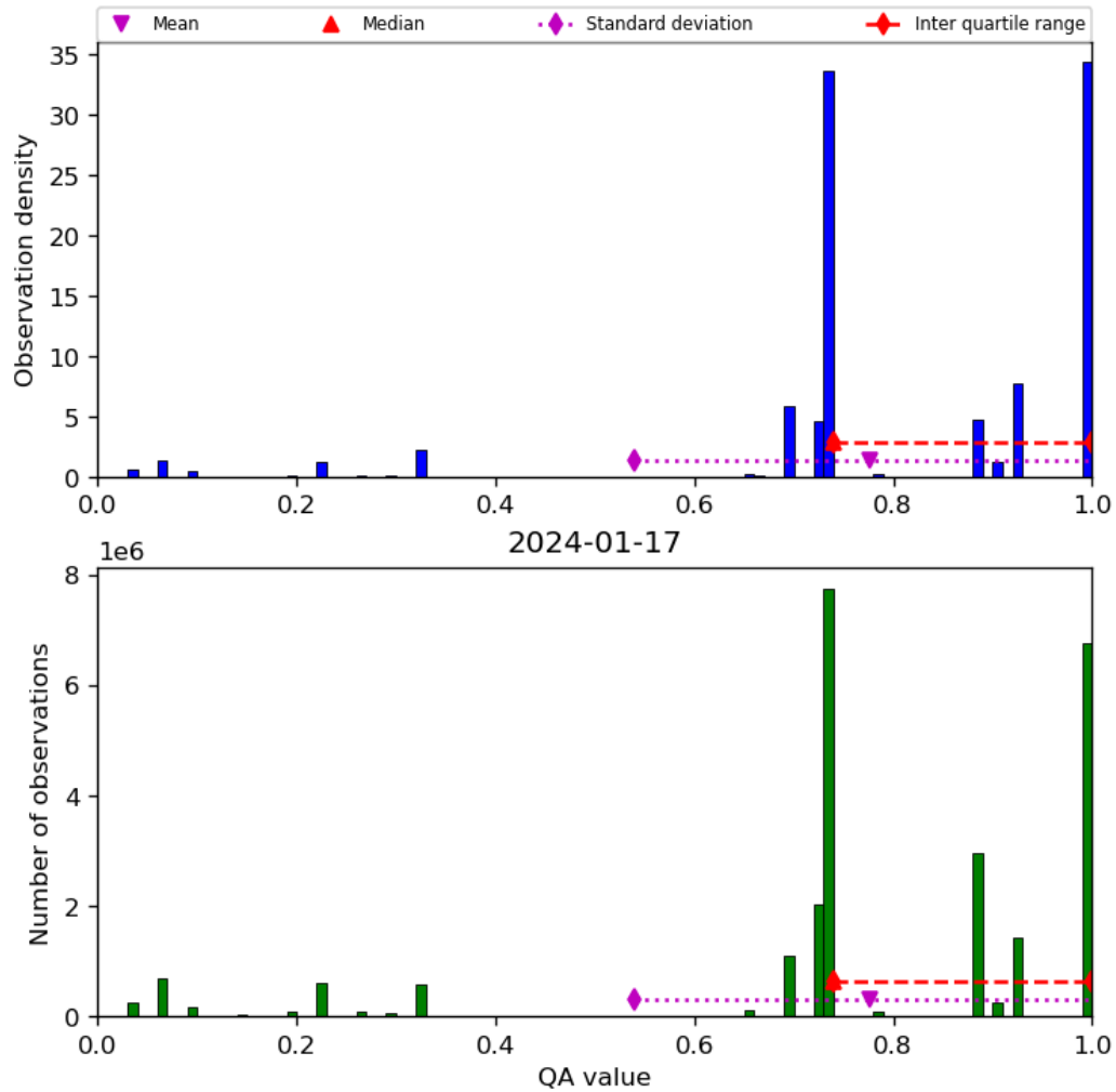
Figure 28: Histogram of “QA value” for 2024-01-16 to 2024-01-18
