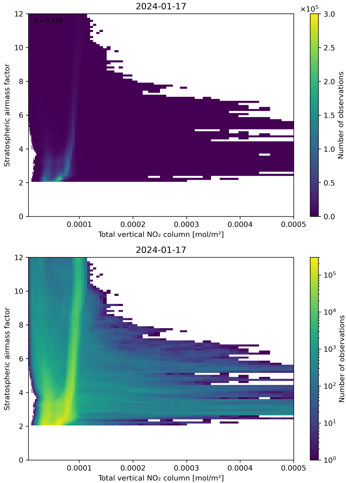
Figure 110: Scatter density plot of “Total vertical NO 2 column” against “Stratospheric airmass factor” for 2024-01-16 to 2024-01-18.
