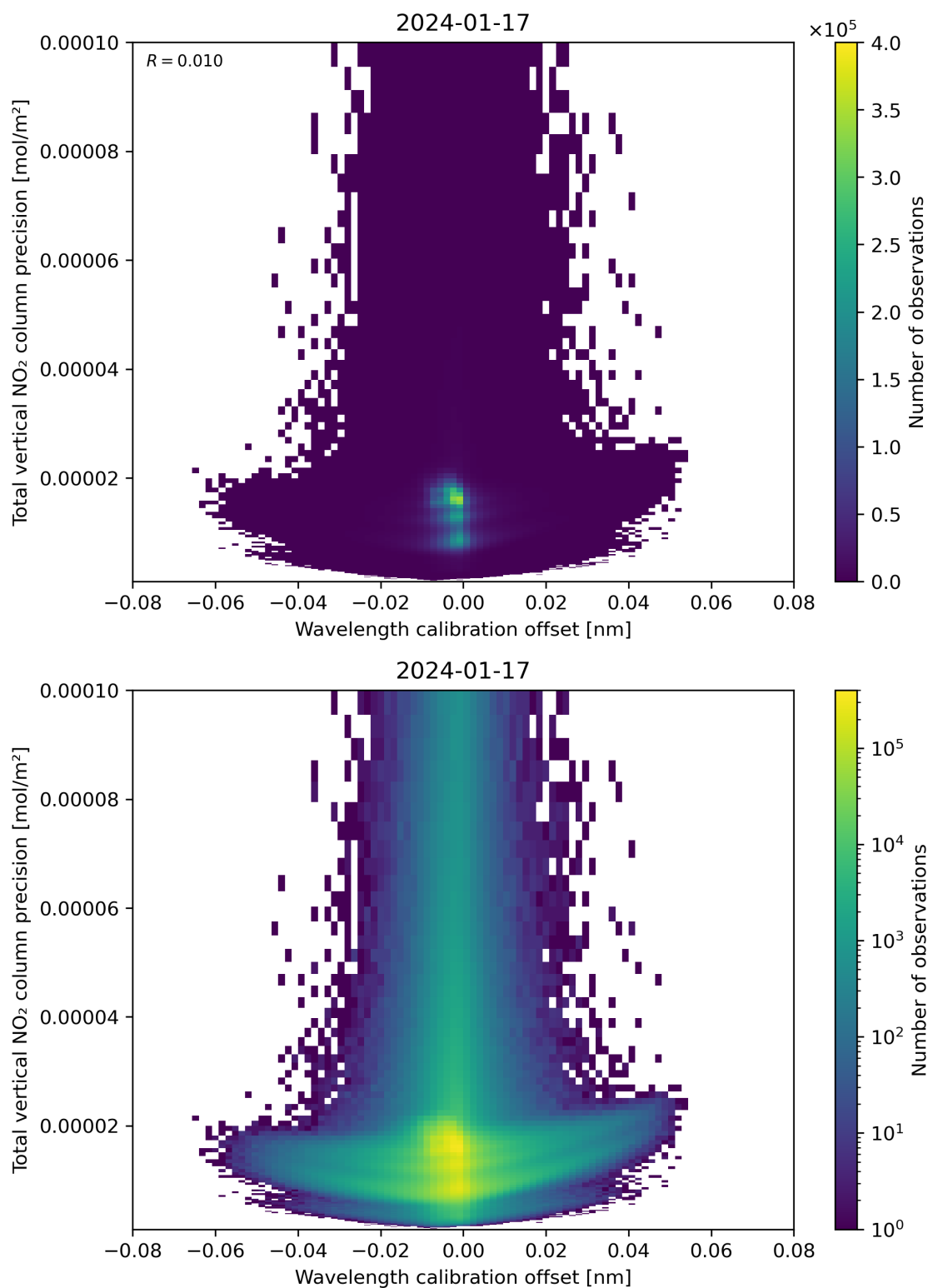
Figure 180: Scatter density plot of “Wavelength calibration offset” against “Total vertical NO 2 column precision” for 2024-01-16 to 2024-01-18.
