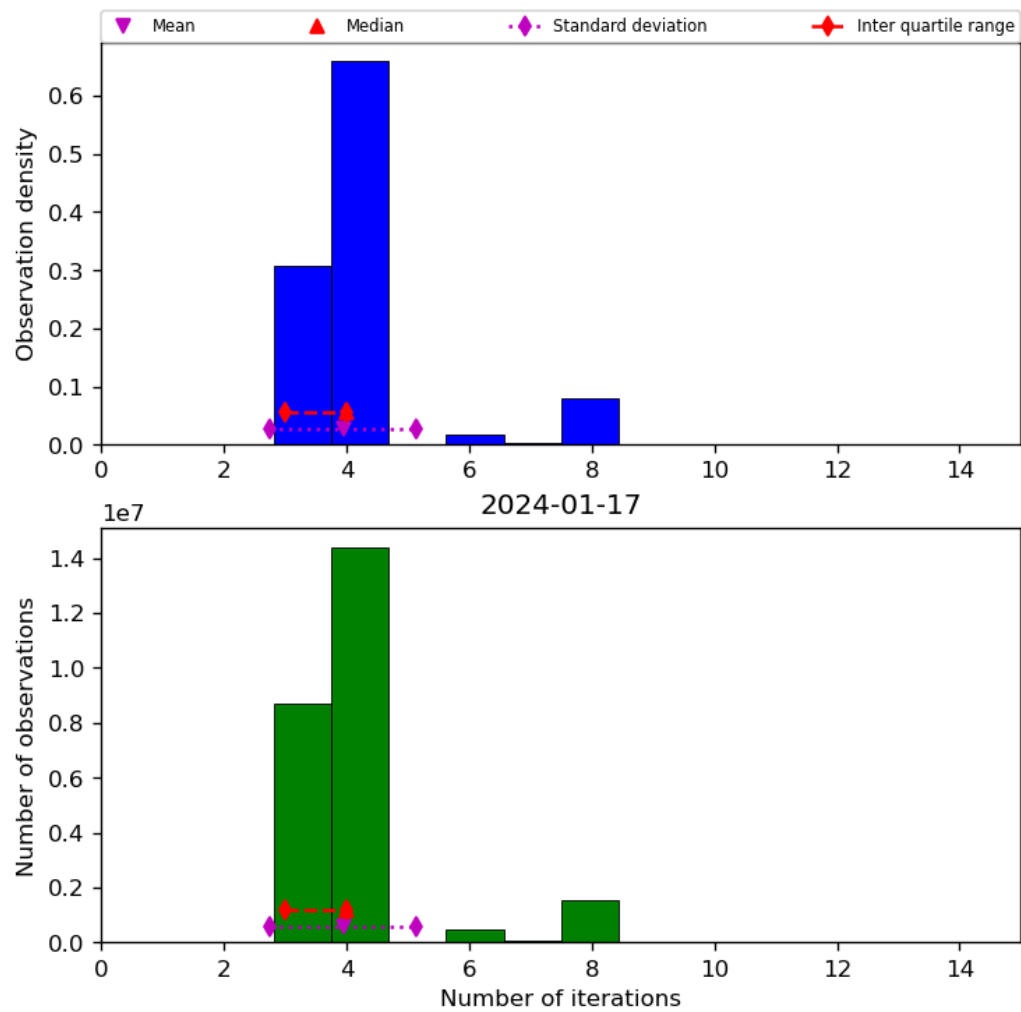
Figure 34: Histogram of “Number of iterations” for 2024-01-16 to 2024-01-18
