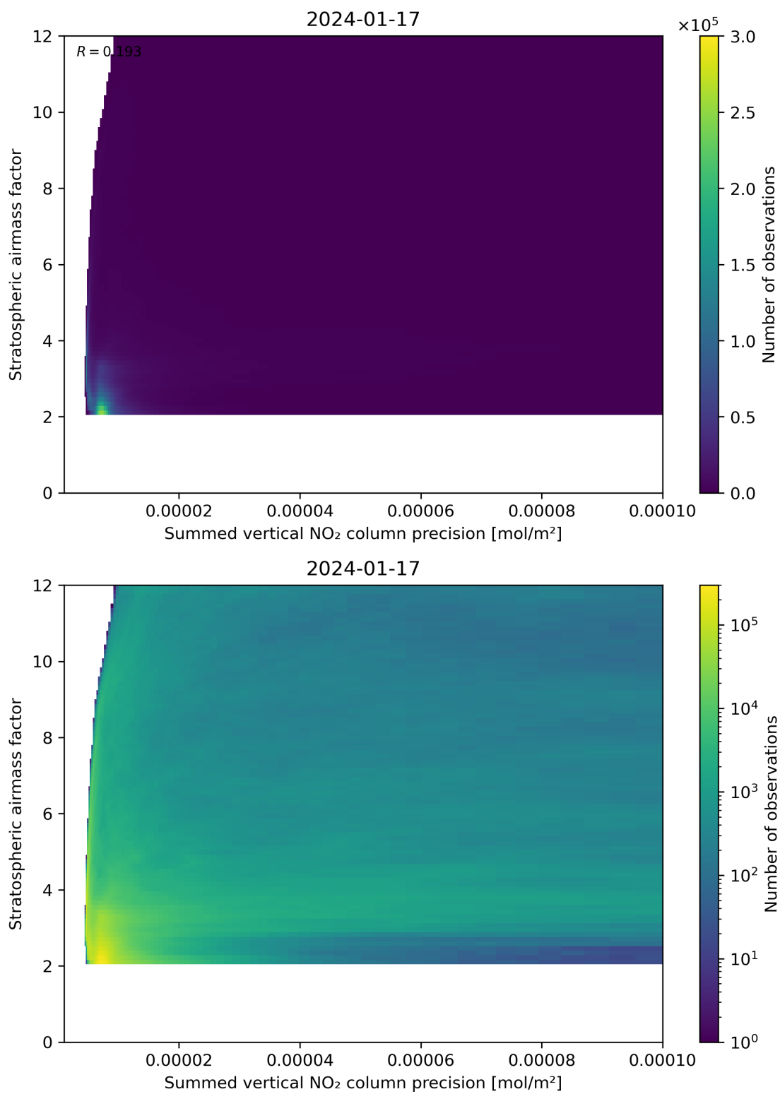
Figure 106: Scatter density plot of “Summed vertical NO 2 column precision” against “Stratospheric airmass factor” for 2024-01-16 to 2024-01-18.
