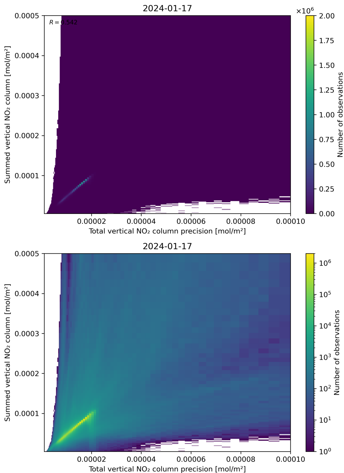
Figure 117: Scatter density plot of “Total vertical NO 2 column precision” against “Summed vertical NO 2 column” for 2024-01-16 to 2024-01-18.
