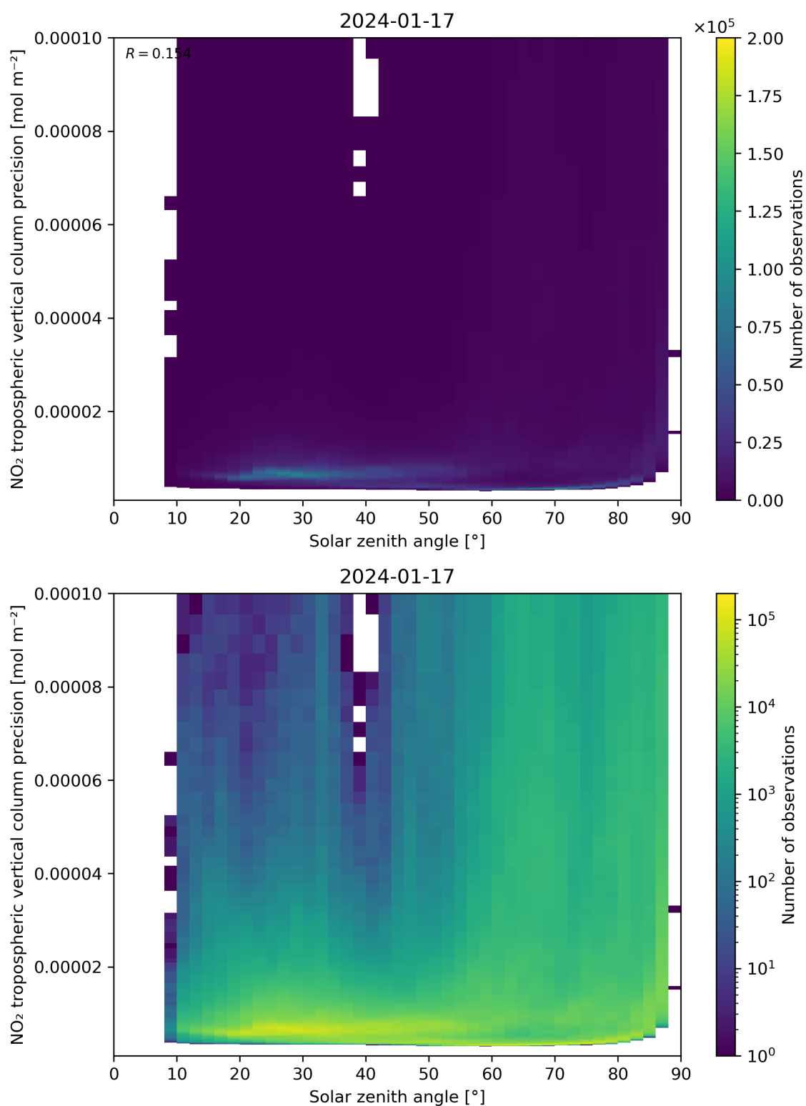
Figure 156: Scatter density plot of “Solar zenith angle” against “NO 2 tropospheric vertical column precision” for 2024-01-16 to 2024-01-18.
