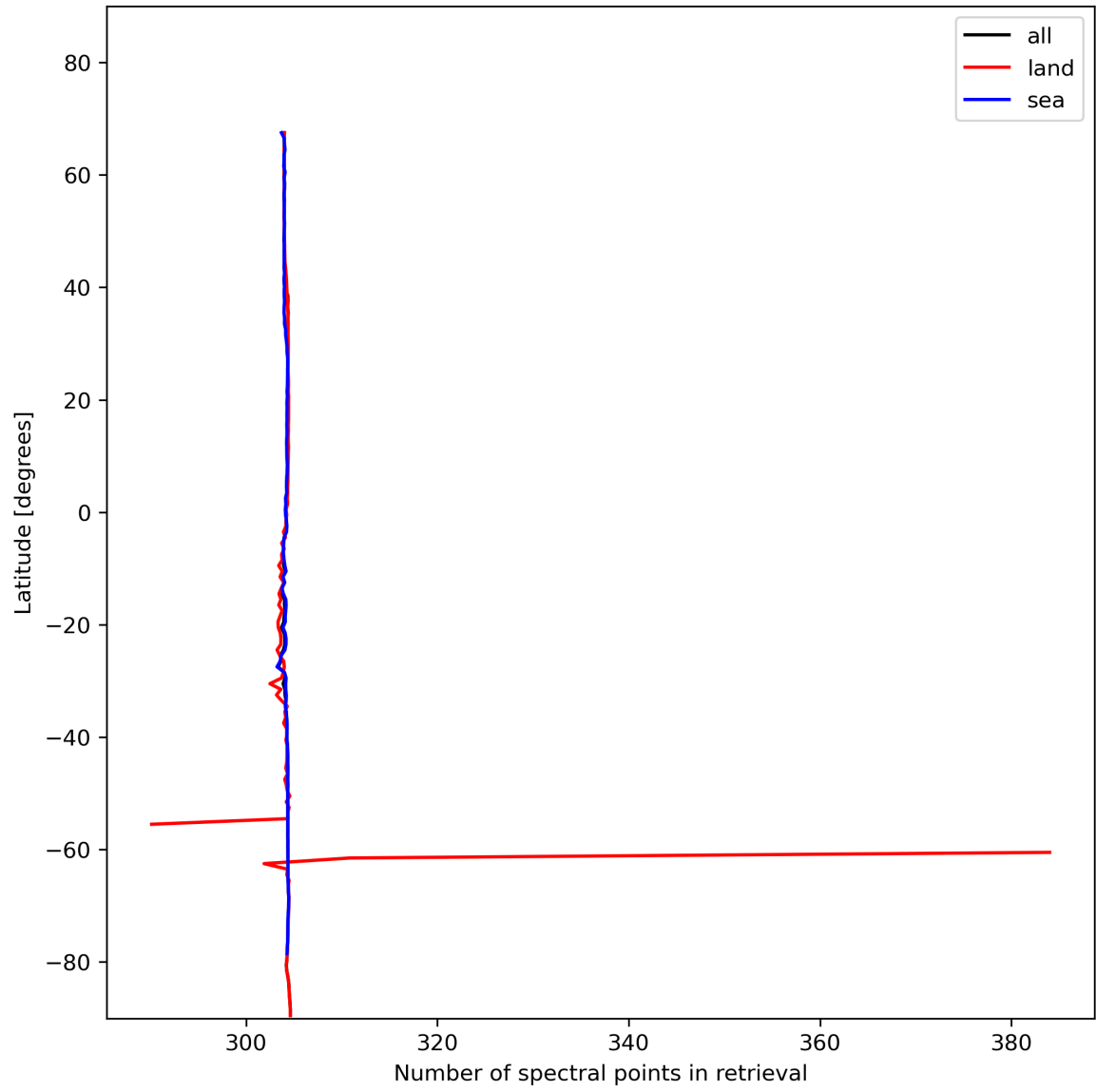
Figure 16: Zonal average of “Number of spectral points in retrieval” for 2024-01-16 to 2024-01-18.
