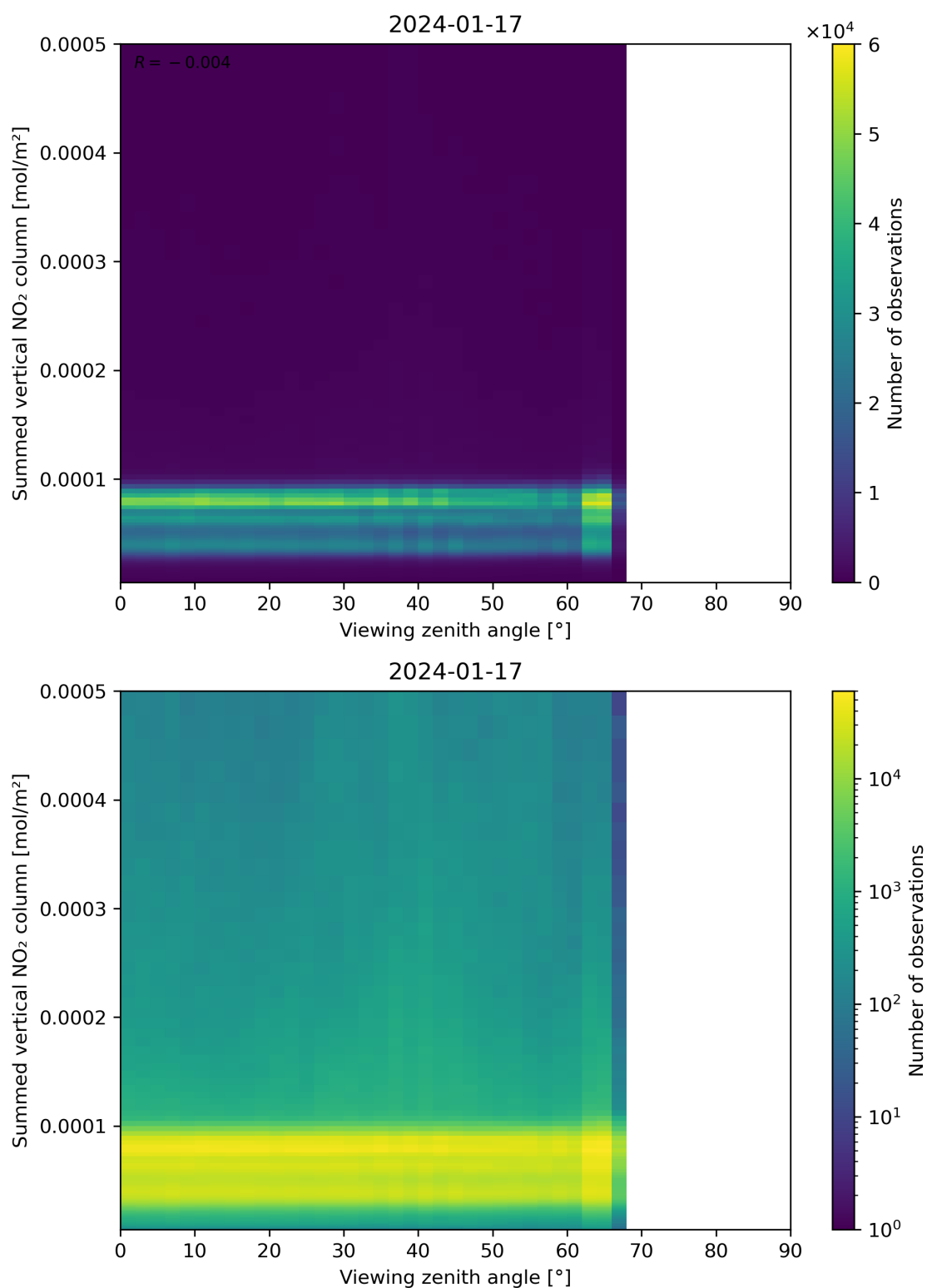
Figure 165: Scatter density plot of “Viewing zenith angle” against “Summed vertical NO 2 column” for 2024-01-16 to 2024-01-18.
