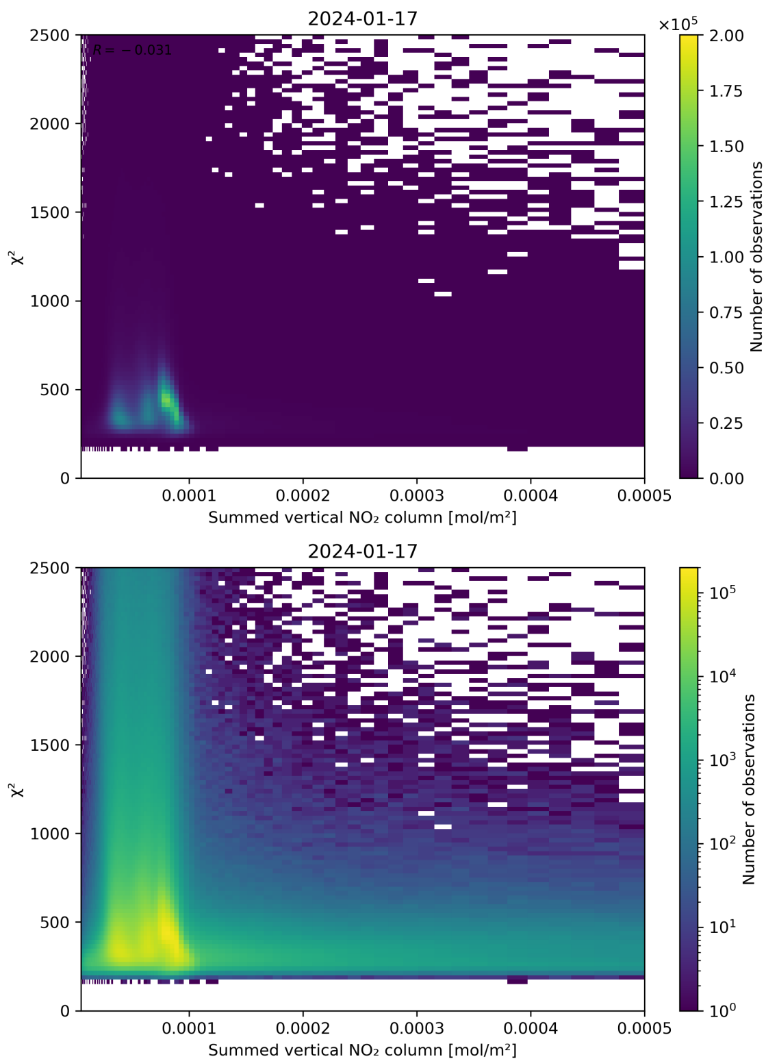
Figure 104: Scatter density plot of “Summed vertical NO 2 column” against “ \chi^2 ” for 2024-01-16 to 2024-01-18.
