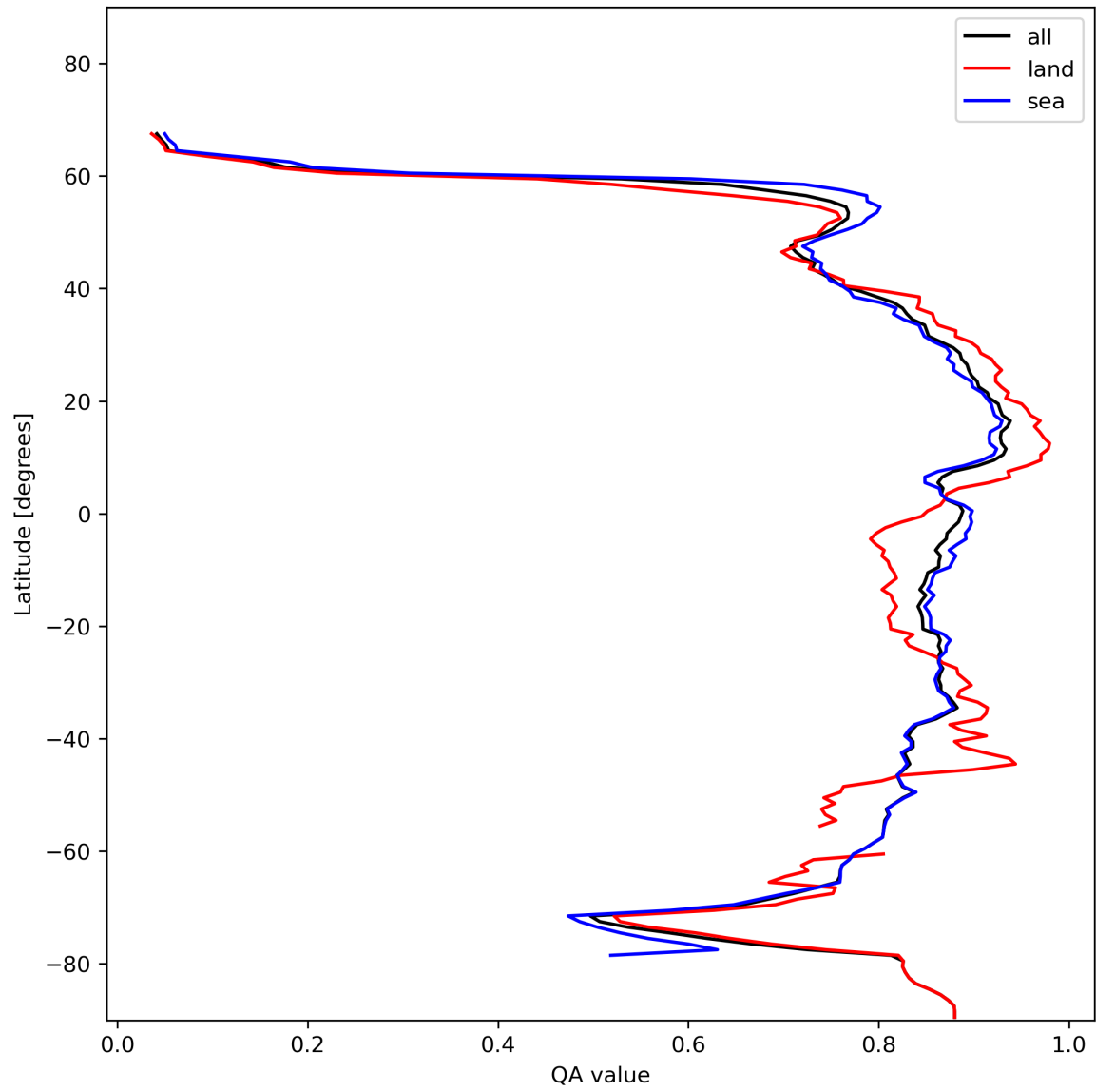
Figure 11: Zonal average of “QA value” for 2024-01-16 to 2024-01-18.
