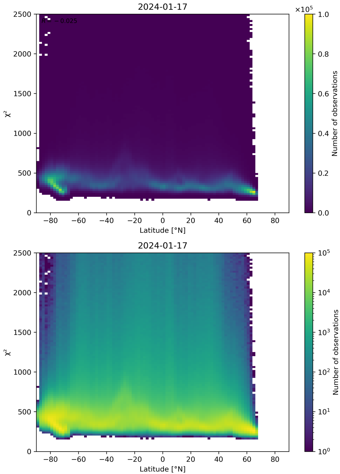
Figure 86: Scatter density plot of “Latitude” against “ \chi^2 ” for 2024-01-16 to 2024-01-18.
