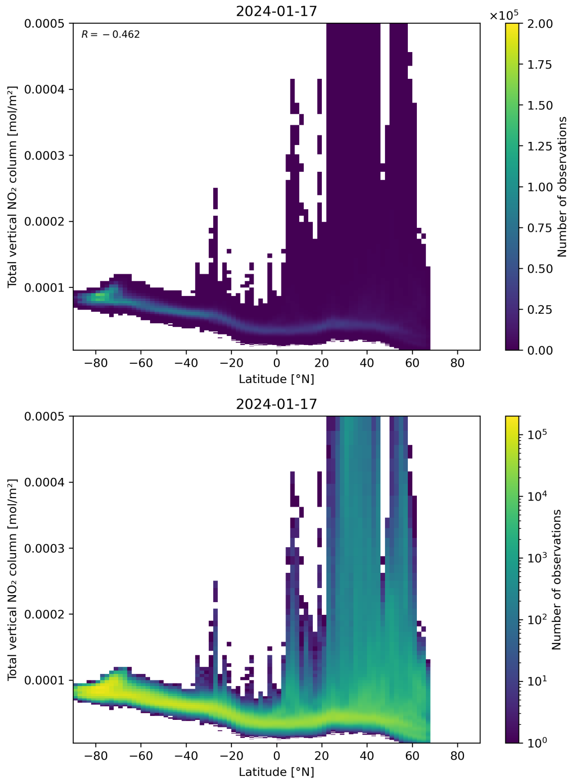
Figure 90: Scatter density plot of “Latitude” against “Total vertical NO 2 column” for 2024-01-16 to 2024-01-18.
