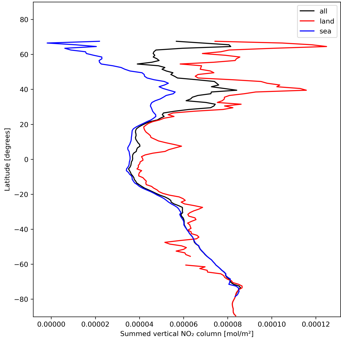
Figure 23: Zonal average of “Summed vertical NO 2 column” for 2024-01-16 to 2024-01-18.
