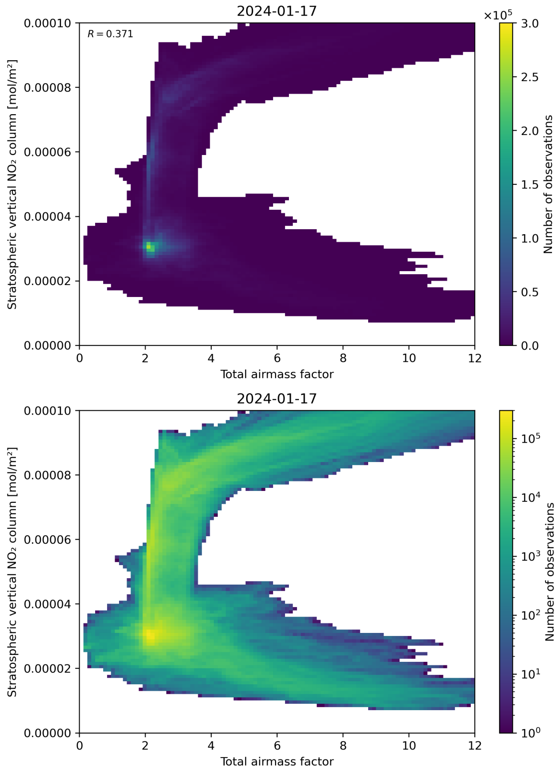
Figure 64: Scatter density plot of “Total airmass factor” against “Stratospheric vertical NO 2 column” for 2024-01-16 to 2024-01-18.
