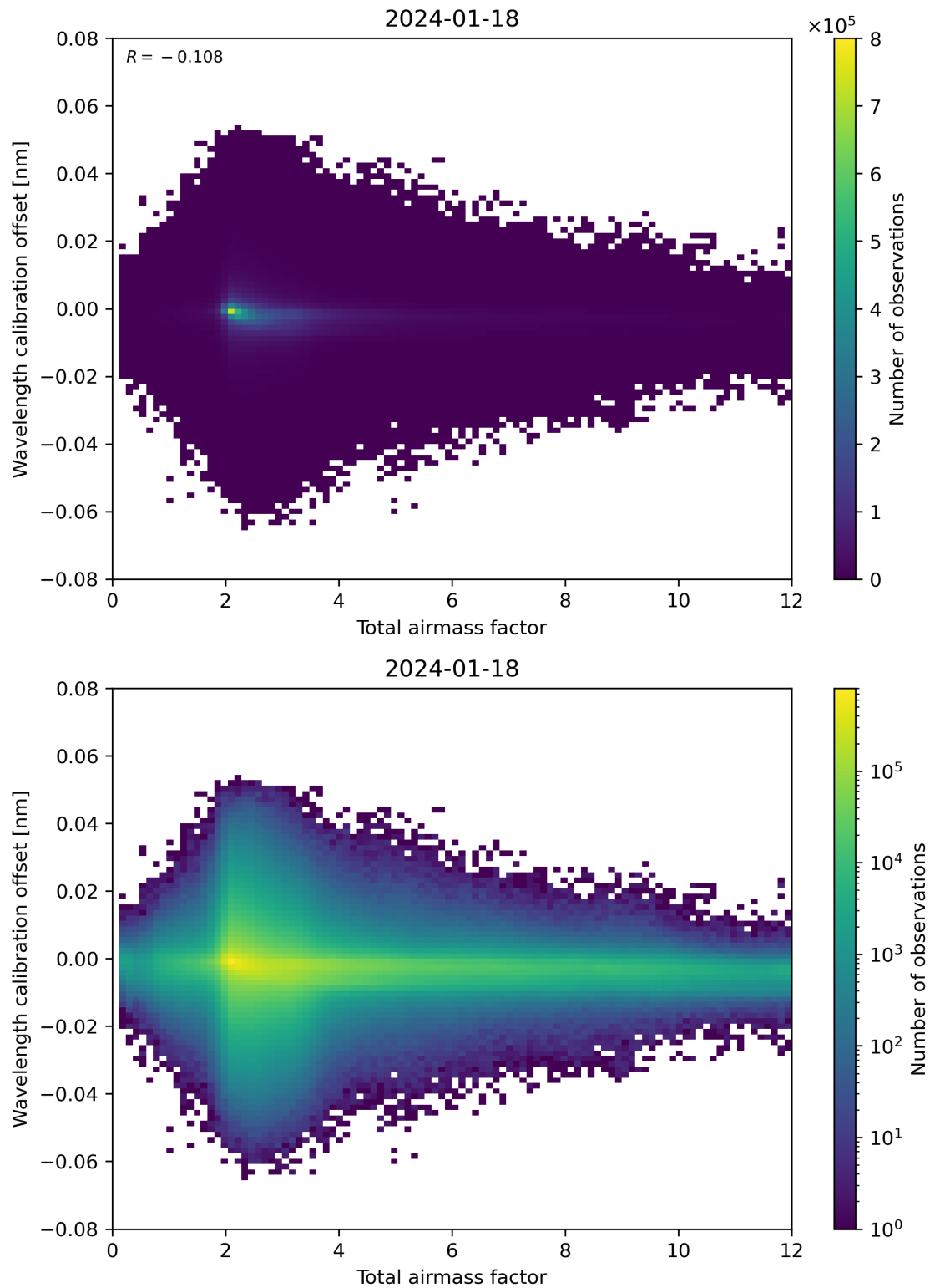
Figure 70: Scatter density plot of “Total airmass factor” against “Wavelength calibration offset” for 2024-01-17 to 2024-01-19.
