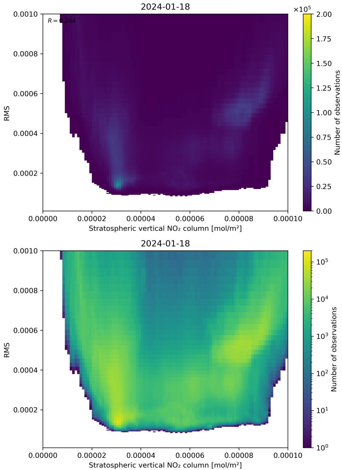
Figure 102: Scatter density plot of “Stratospheric vertical NO 2 column” against “RMS” for 2024-01-17 to 2024-01-19.
