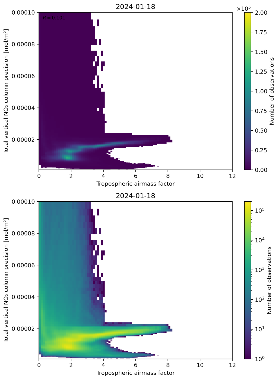
Figure 78: Scatter density plot of “Tropospheric air mass factor” against “Total vertical NO 2 column precision” for 2024-01-17 to 2024-01-19.
