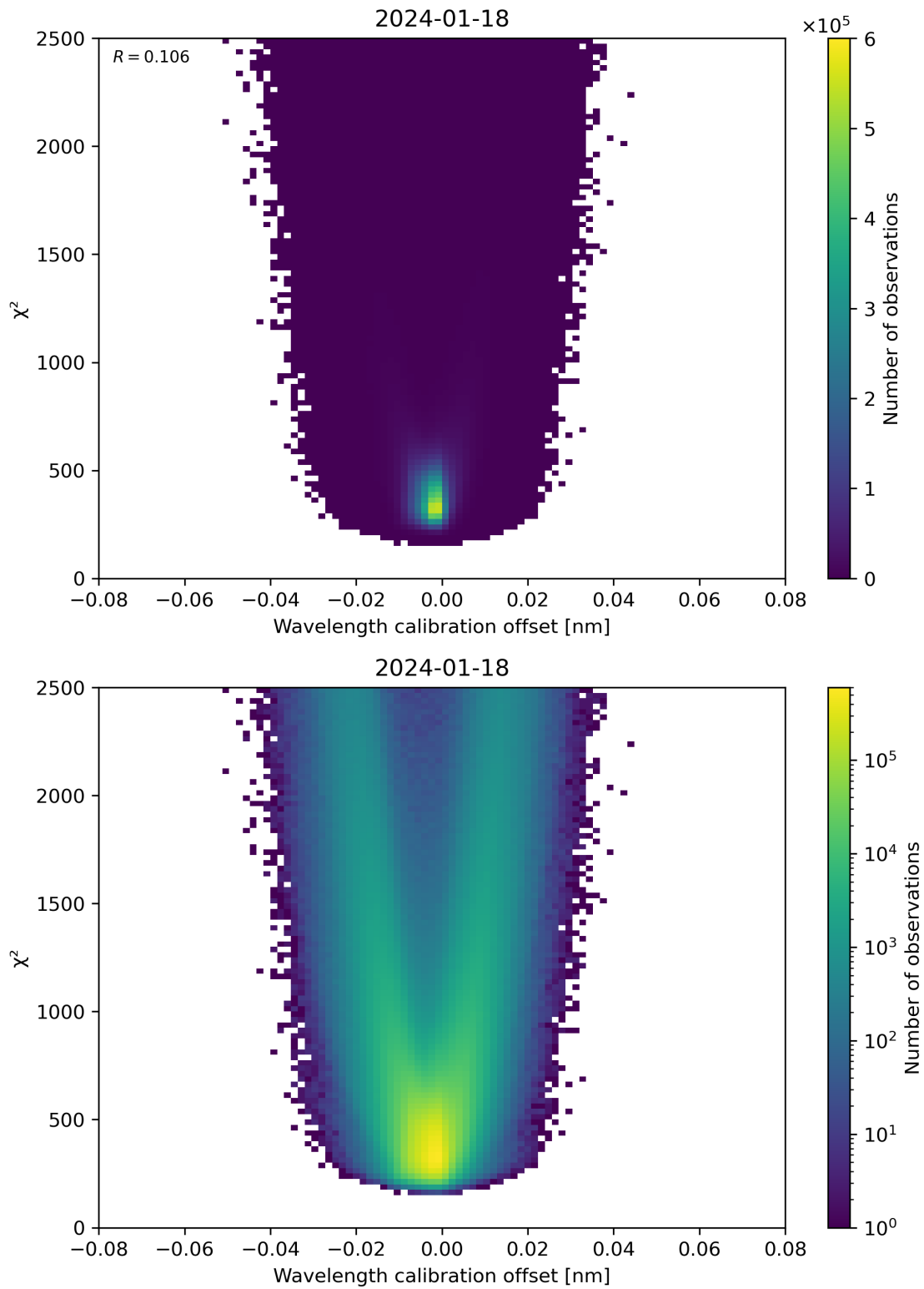
Figure 175: Scatter density plot of “Wavelength calibration offset” against “ \chi^2 ” for 2024-01-17 to 2024-01-19.
