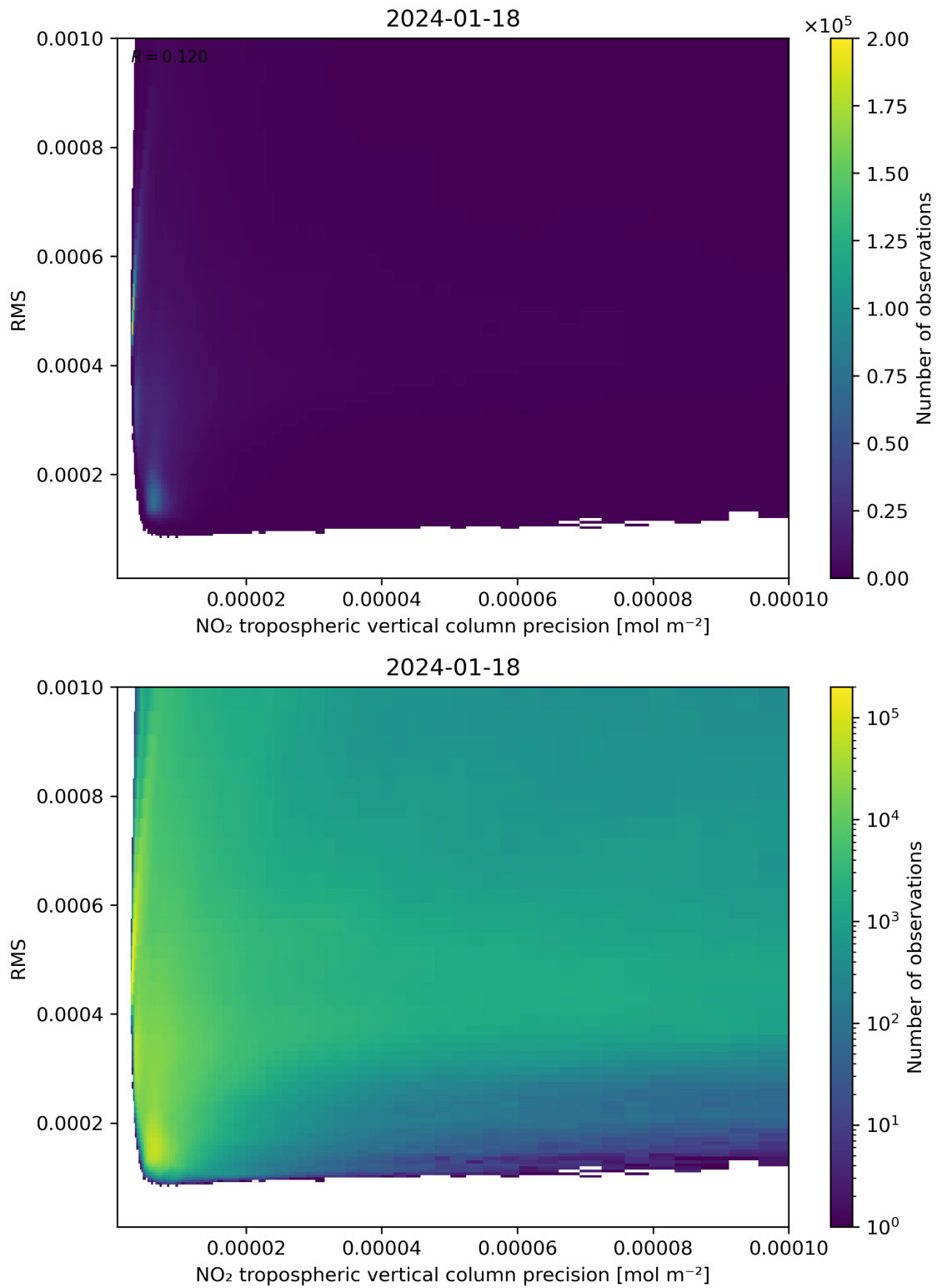
Figure 140: Scatter density plot of “NO 2 tropospheric vertical column precision” against “RMS” for 2024-01-17 to 2024-01-19.
