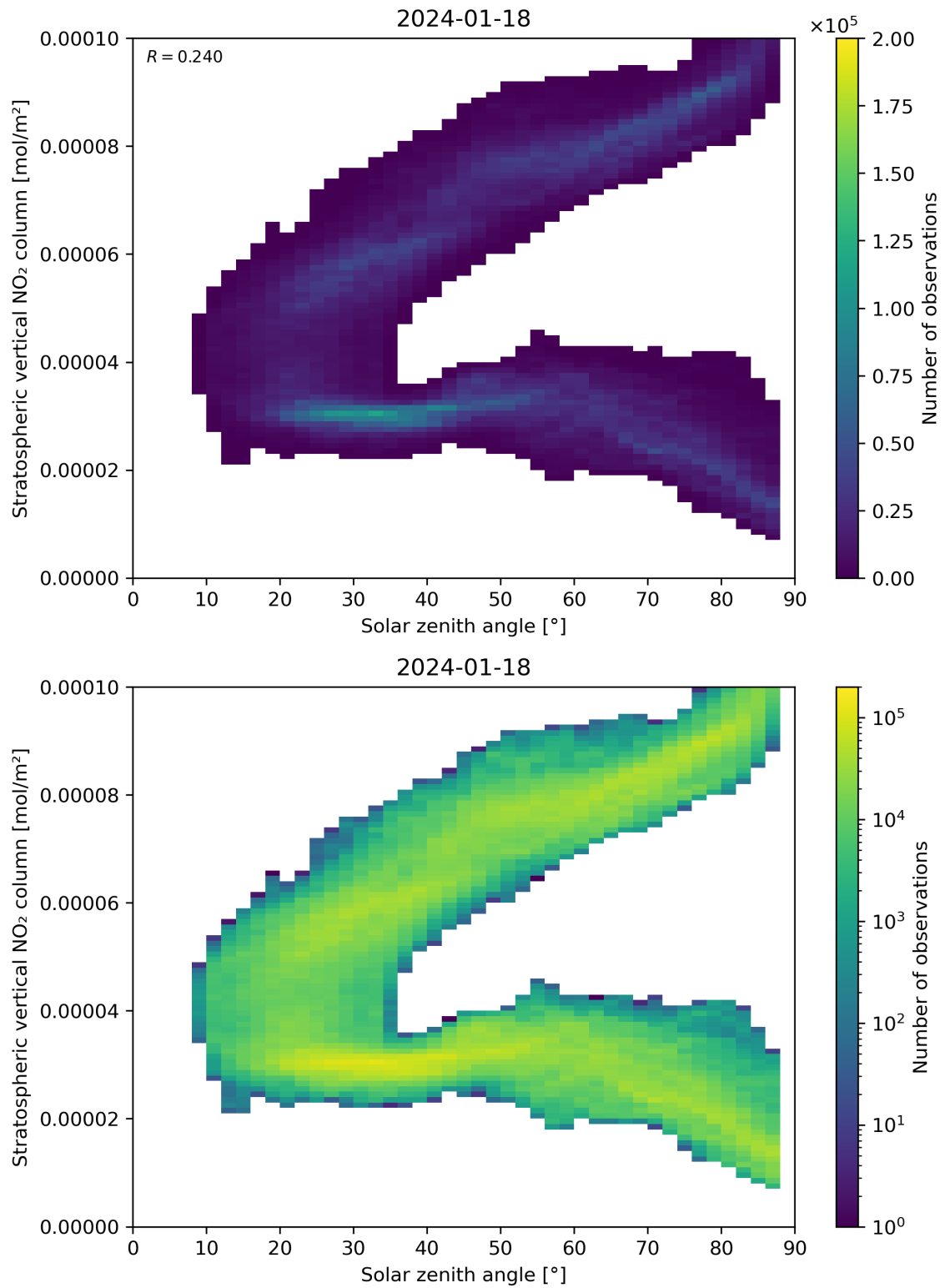
Figure 150: Scatter density plot of “Solar zenith angle” against “Stratospheric vertical NO 2 column” for 2024-01-17 to 2024-01-19.
