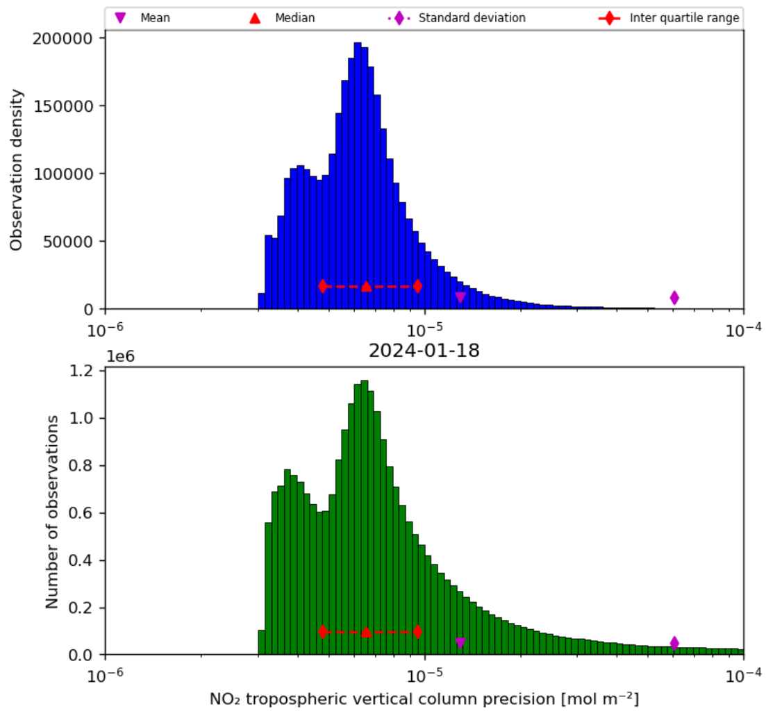
Figure 30: Histogram of “NO 2 tropospheric vertical column precision” for 2024-01-17 to 2024-01-19
