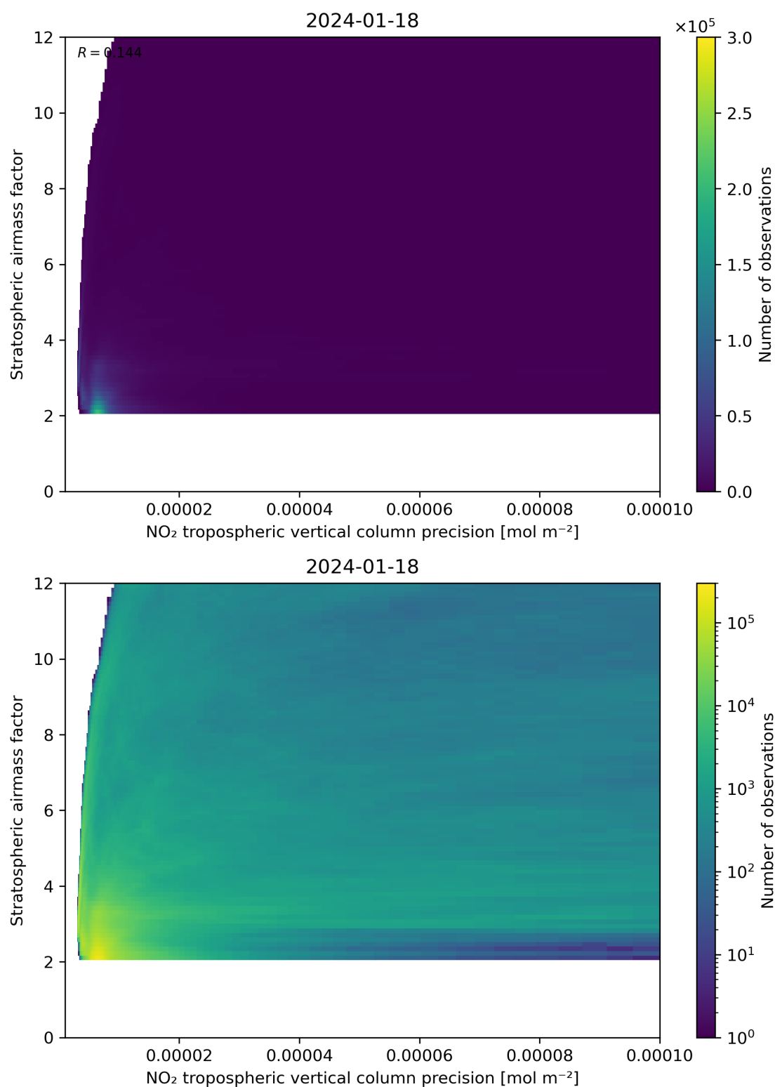
Figure 131: Scatter density plot of “NO 2 tropospheric vertical column precision” against “Stratospheric airmass factor” for 2024-01-17 to 2024-01-19.
