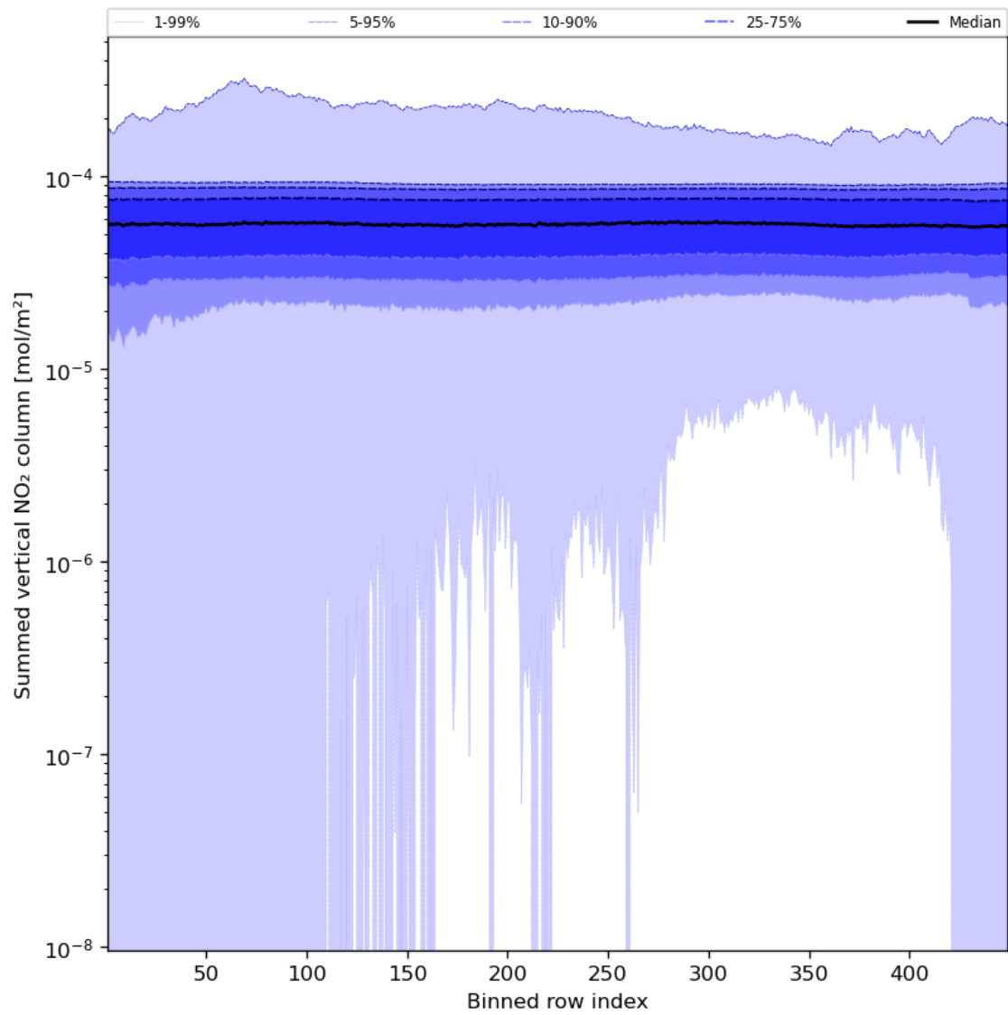
Figure 57: Along track statistics of “Summed vertical NO 2 column” for 2024-01-17 to 2024-01-19
