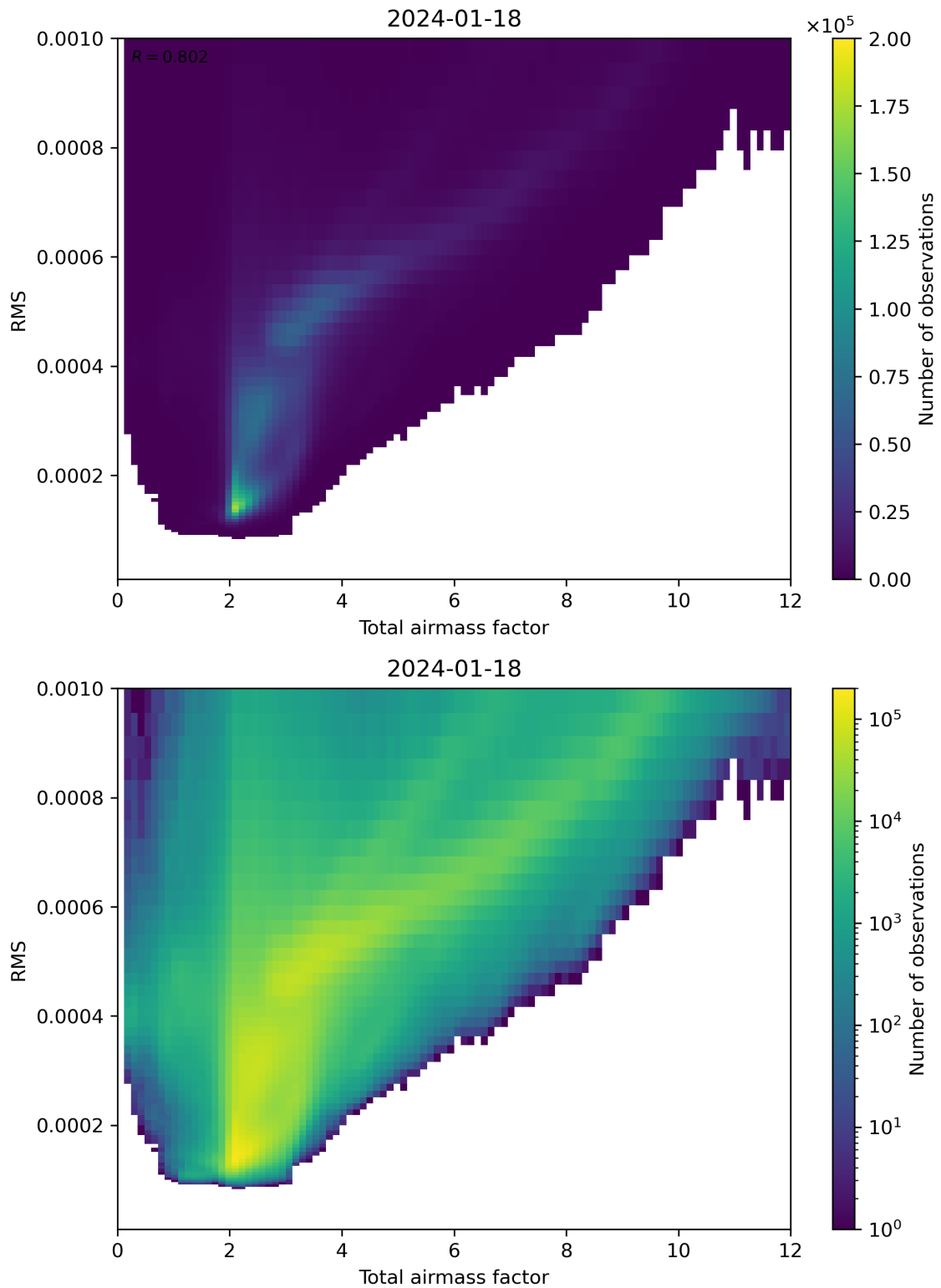
Figure 69: Scatter density plot of “Total airmass factor” against “RMS” for 2024-01-17 to 2024-01-19.
