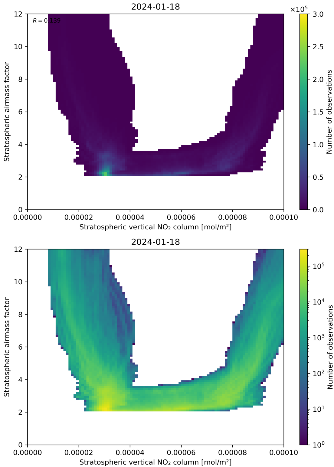
Figure 96: Scatter density plot of “Stratospheric vertical NO 2 column” against “Stratospheric airmass factor” for 2024-01-17 to 2024-01-19.
