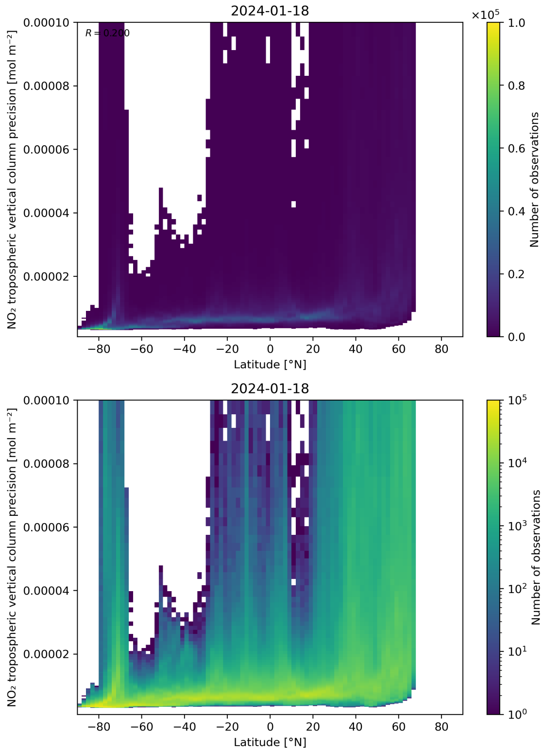
Figure 93: Scatter density plot of “Latitude” against “NO 2 tropospheric vertical column precision” for 2024-01-17 to 2024-01-19.
