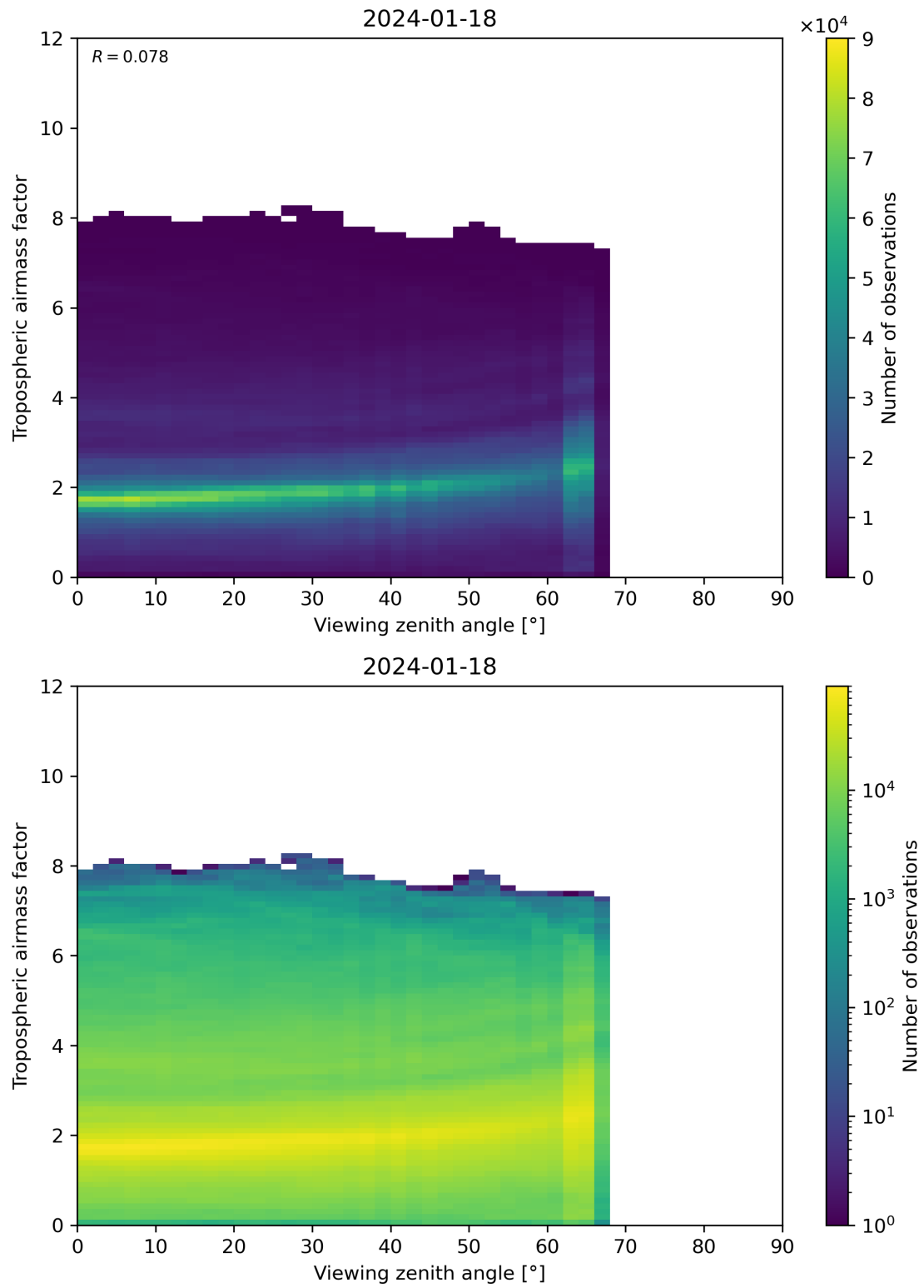
Figure 161: Scatter density plot of “Viewing zenith angle” against “Tropospheric airmass factor” for 2024-01-17 to 2024-01-19.
