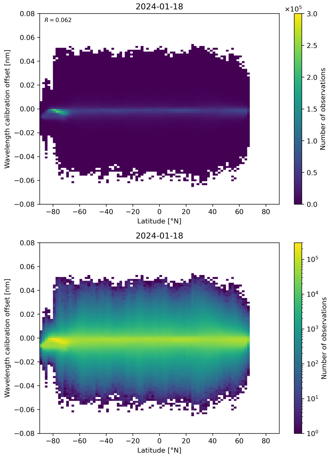
Figure 95: Scatter density plot of “Latitude” against “Wavelength calibration offset” for 2024-01-17 to 2024-01-19.
