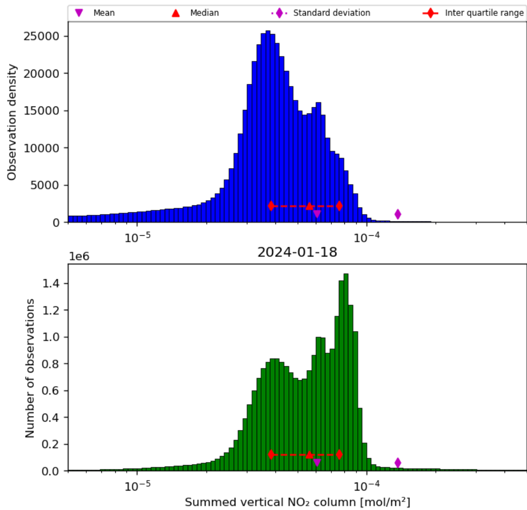
Figure 40: Histogram of “Summed vertical NO 2 column” for 2024-01-17 to 2024-01-19
