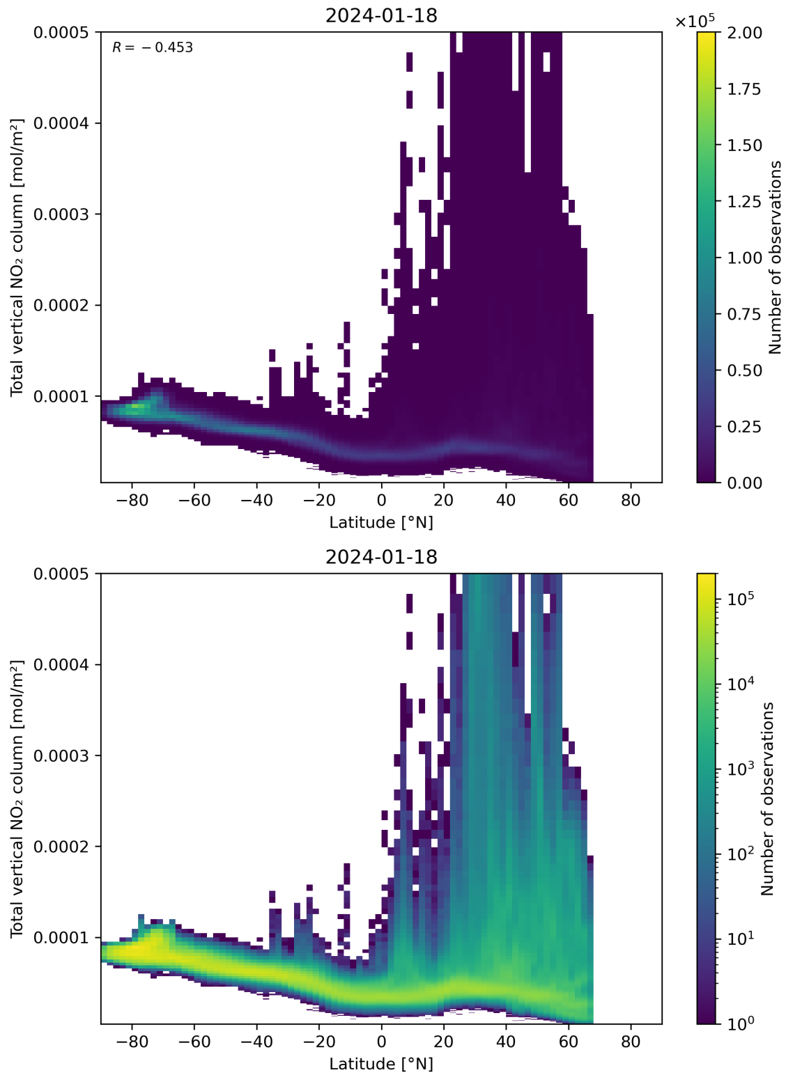
Figure 90: Scatter density plot of “Latitude” against “Total vertical NO 2 column” for 2024-01-17 to 2024-01-19.
