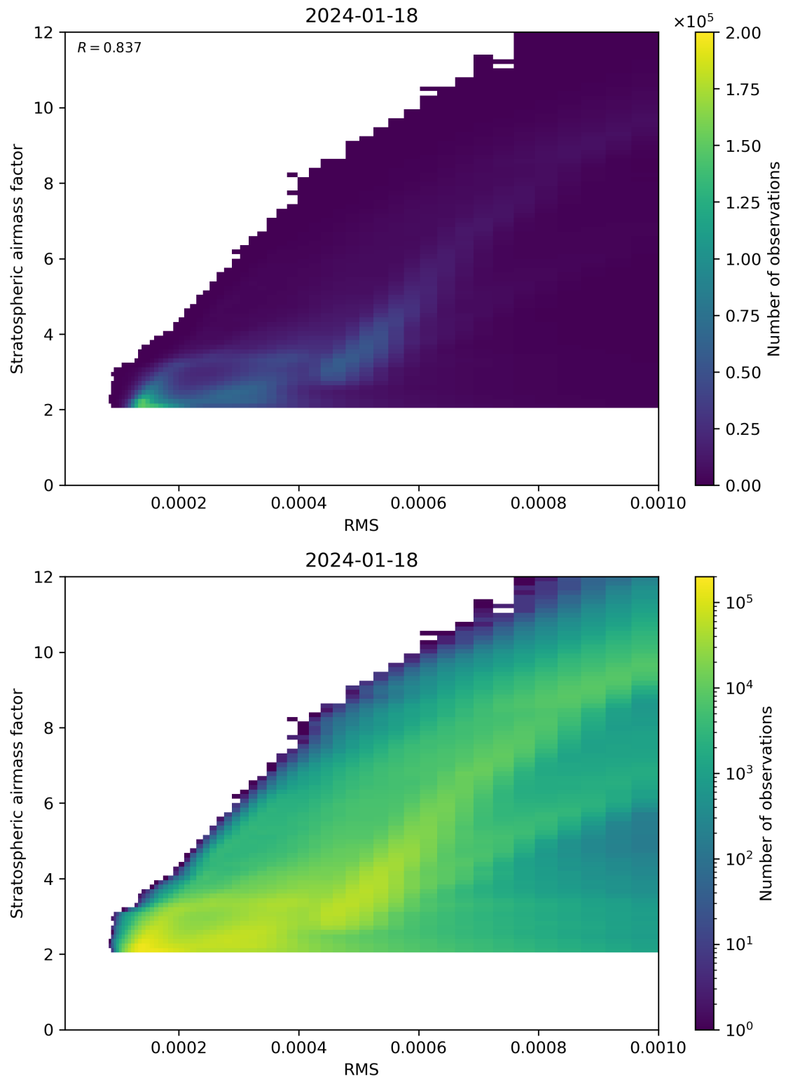
Figure 144: Scatter density plot of “RMS” against “Stratospheric airmass factor” for 2024-01-17 to 2024-01-19.
