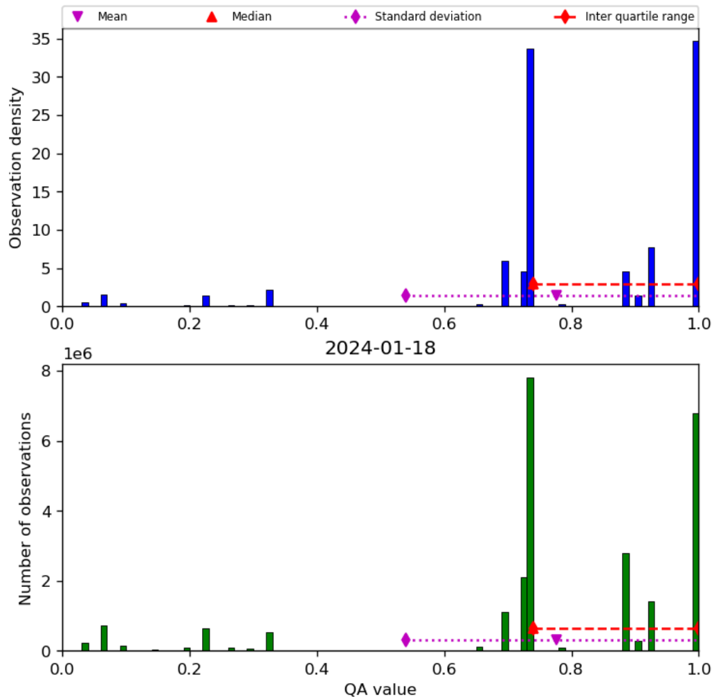
Figure 28: Histogram of “QA value” for 2024-01-17 to 2024-01-19
