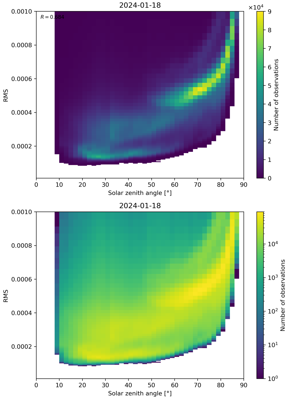
Figure 157: Scatter density plot of “Solar zenith angle” against “RMS” for 2024-01-17 to 2024-01-19.
