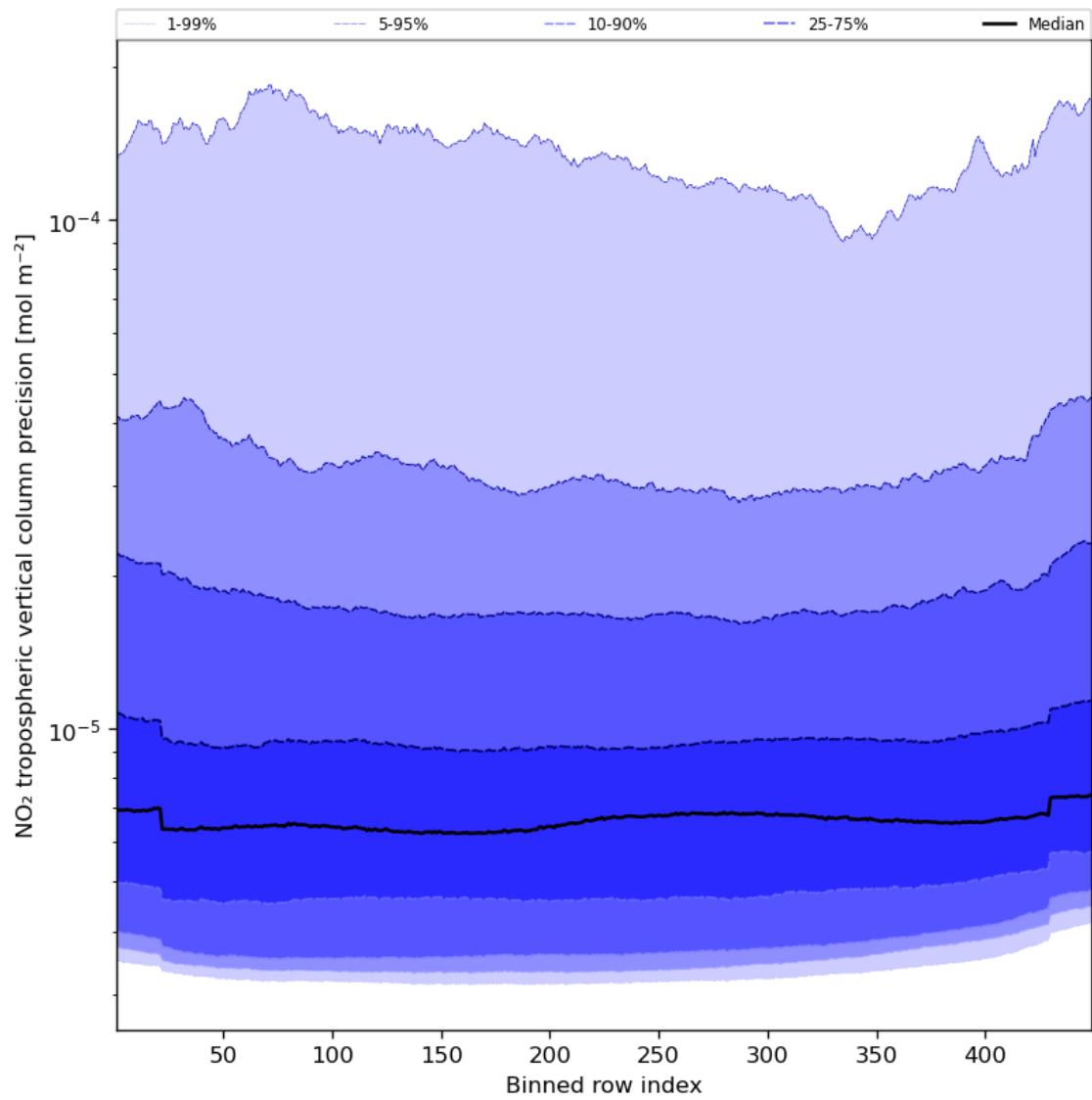
Figure 47: Along track statistics of “NO 2 tropospheric vertical column precision” for 2024-01-17 to 2024-01-19
