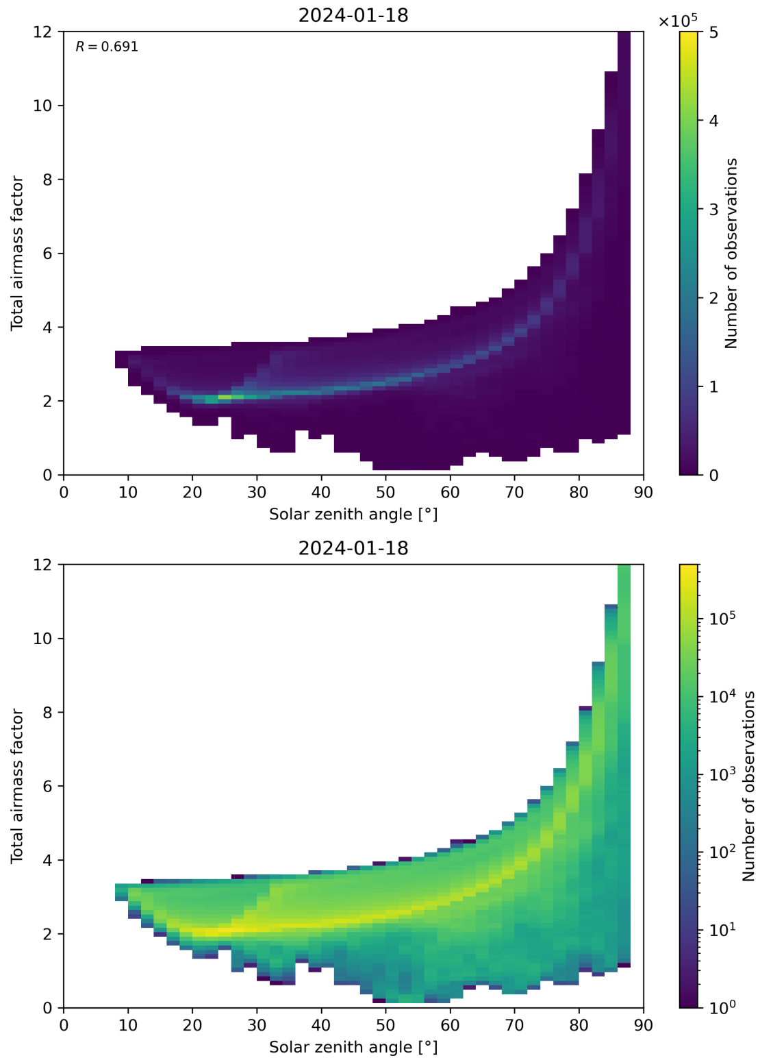
Figure 146: Scatter density plot of “Solar zenith angle” against “Total air mass factor” for 2024-01-17 to 2024-01-19.
