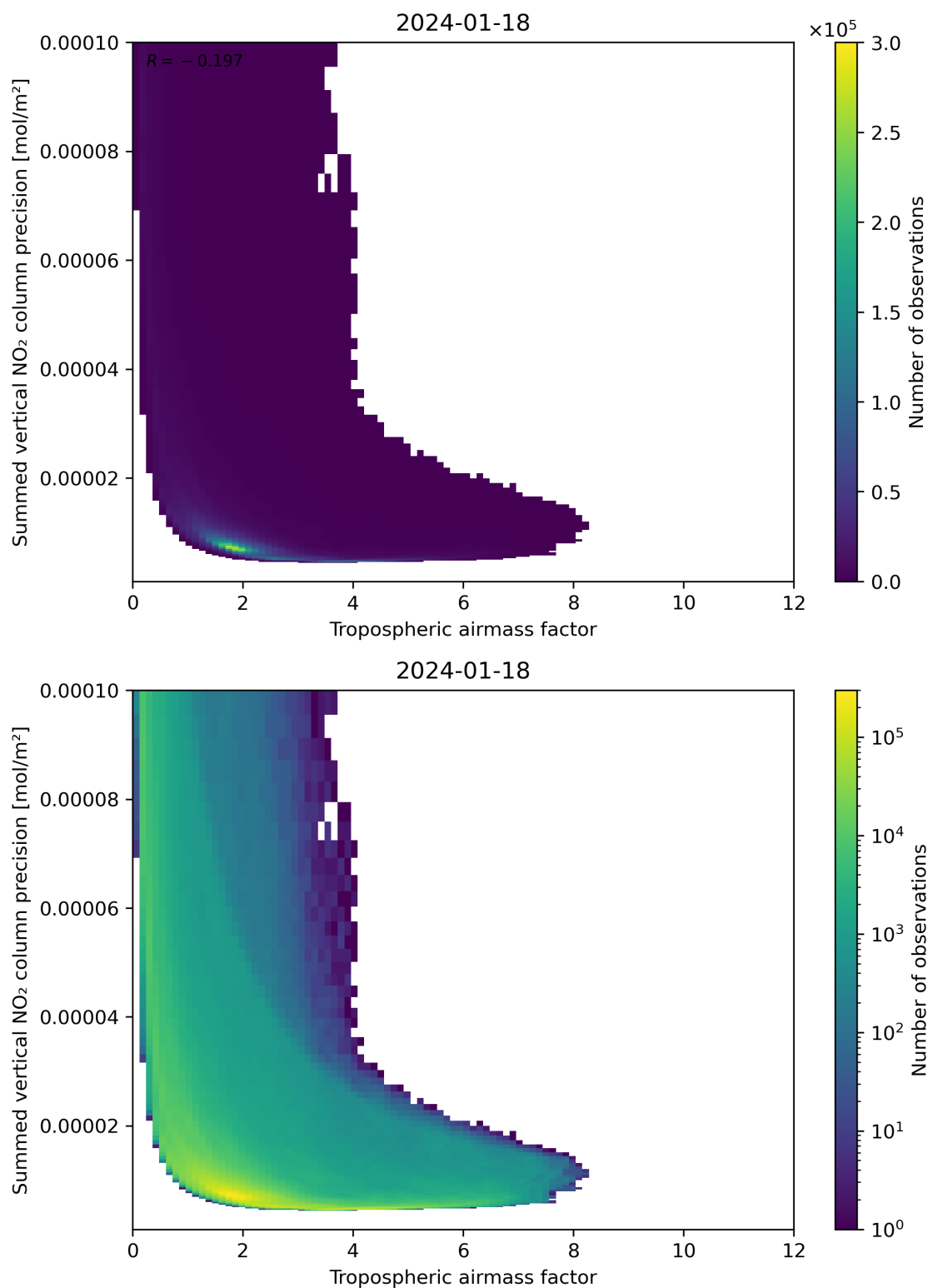
Figure 76: Scatter density plot of “Tropospheric airmass factor” against “Summed vertical NO 2 column precision” for 2024-01-17 to 2024-01-19.
