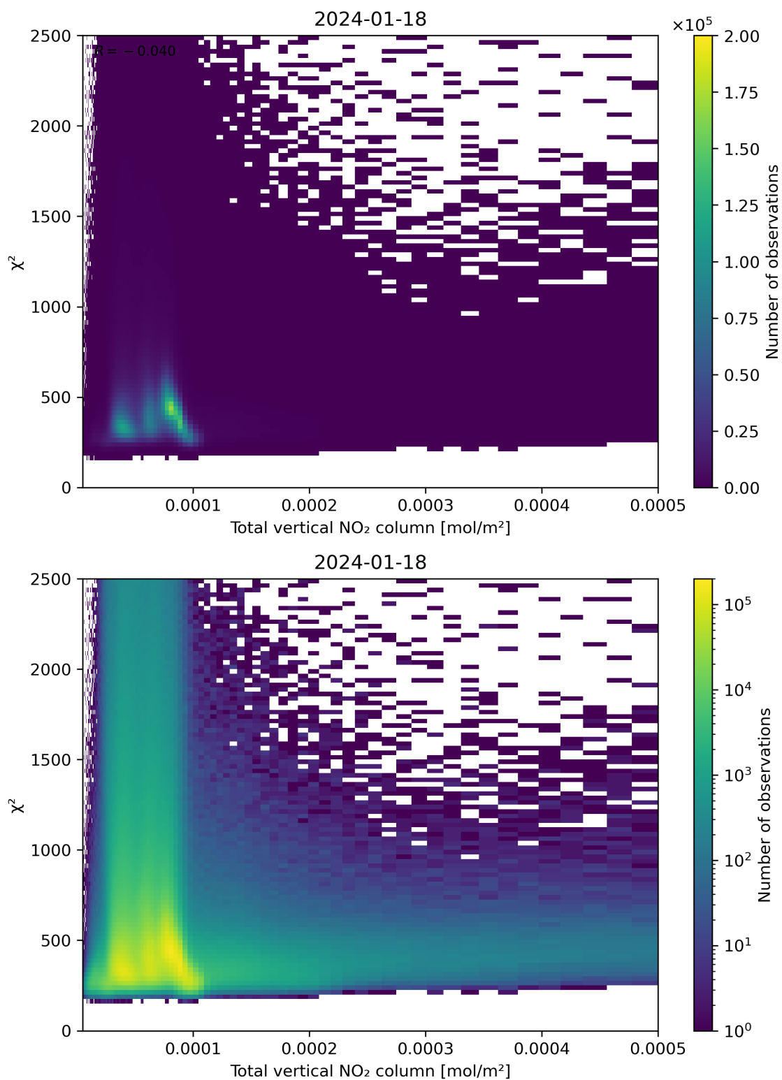
Figure 111: Scatter density plot of “Total vertical NO 2 column” against “ \chi^2 ” for 2024-01-17 to 2024-01-19.
