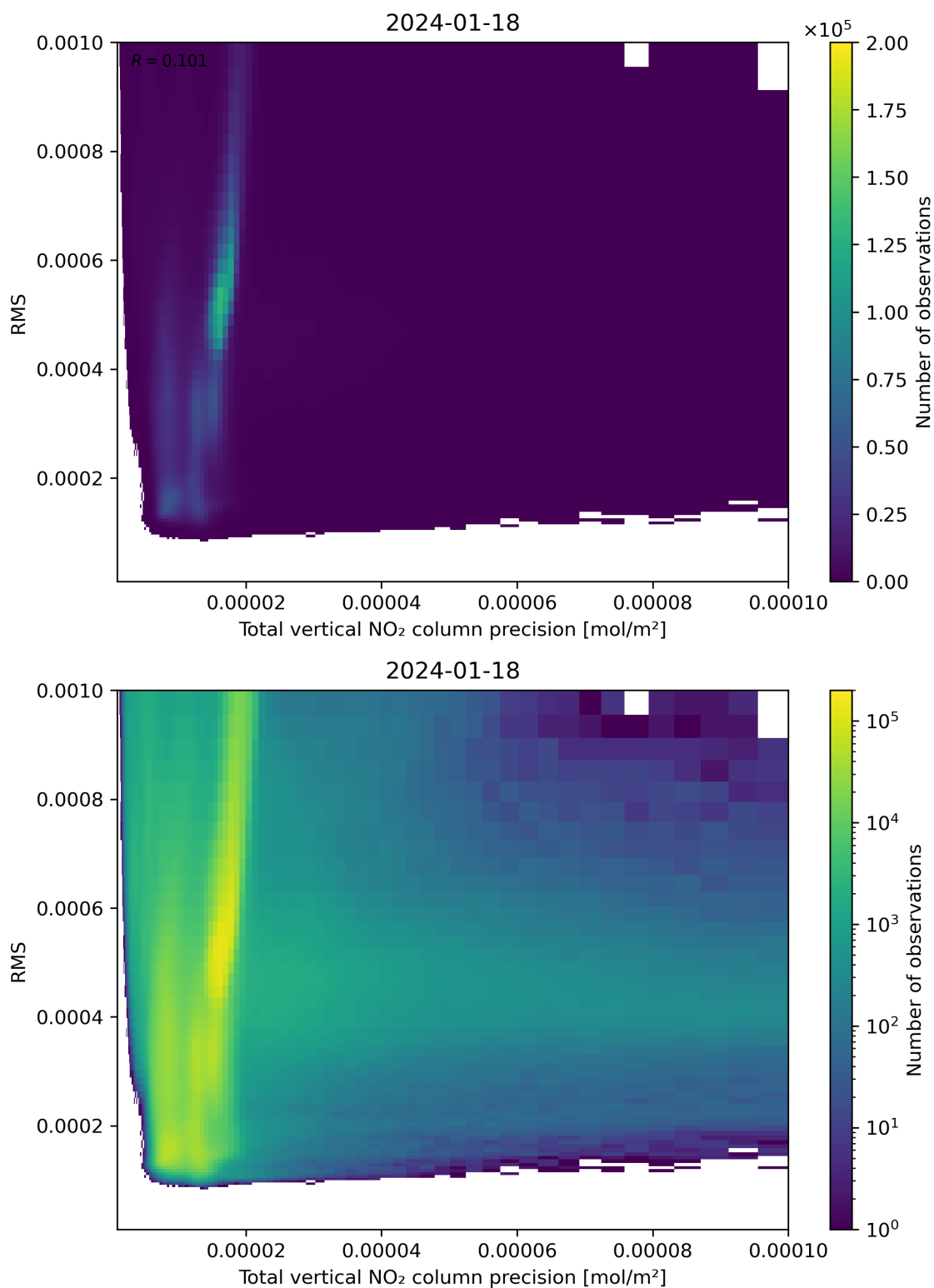
Figure 119: Scatter density plot of “Total vertical NO 2 column precision” against “RMS” for 2024-01-17 to 2024-01-19.
