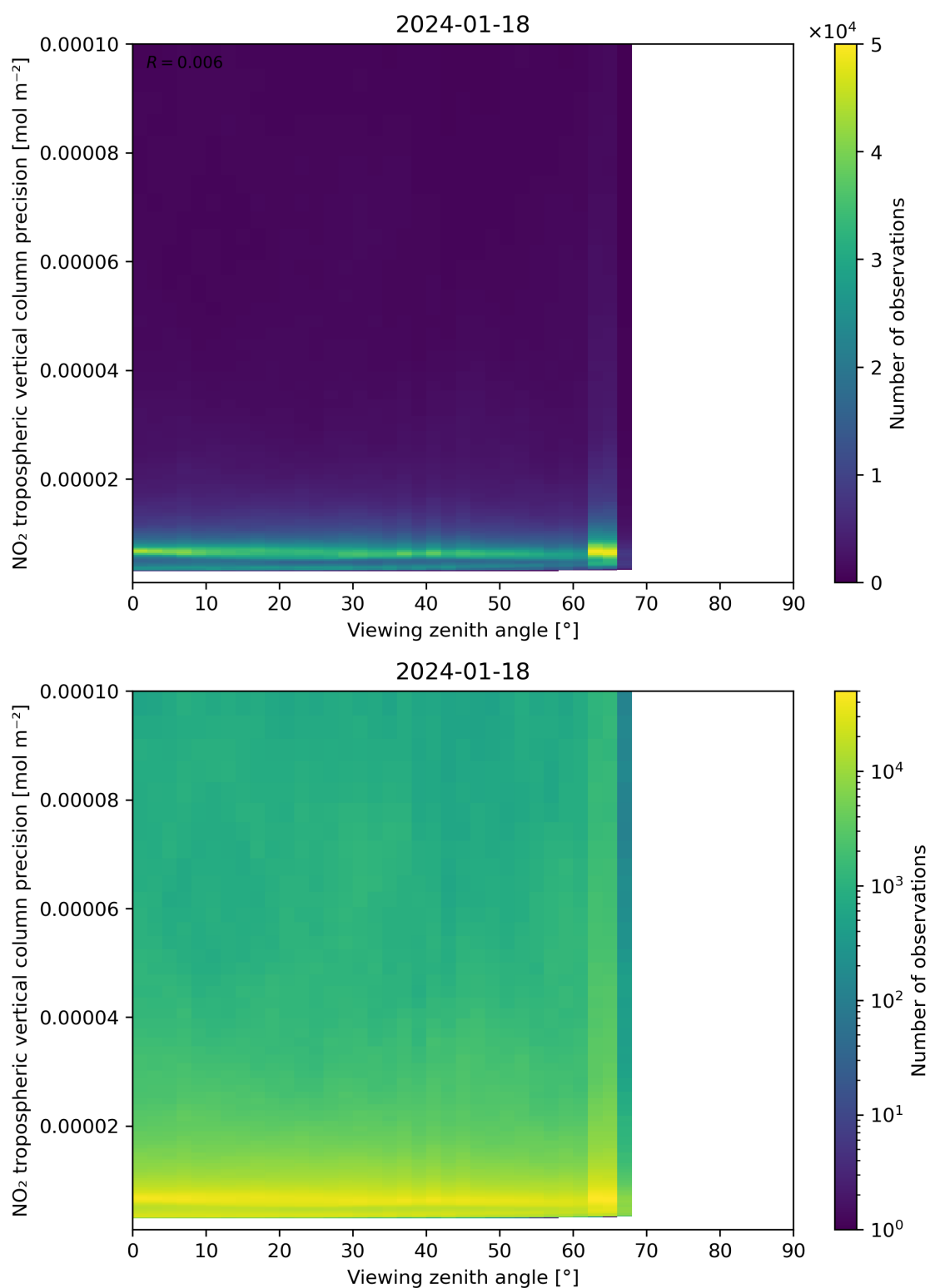
Figure 170: Scatter density plot of “Viewing zenith angle” against “NO 2 tropospheric vertical column precision” for 2024-01-17 to 2024-01-19.
