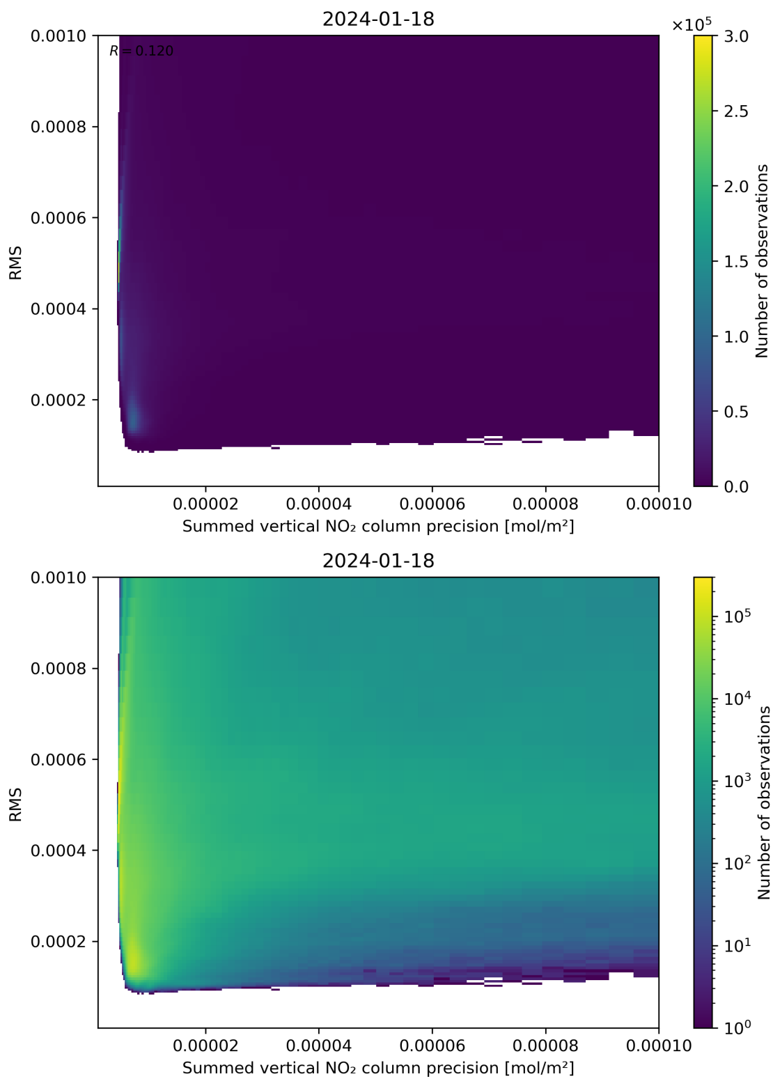
Figure 108: Scatter density plot of “Summed vertical NO 2 column precision” against “RMS” for 2024-01-17 to 2024-01-19.
