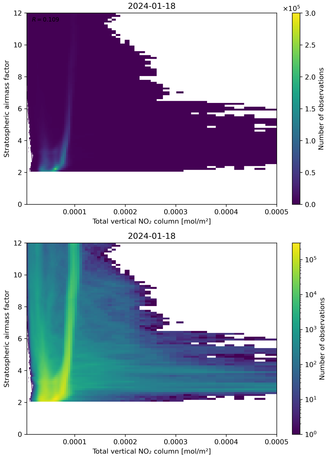
Figure 110: Scatter density plot of “Total vertical NO 2 column” against “Stratospheric air mass factor” for 2024-01-17 to 2024-01-19.
