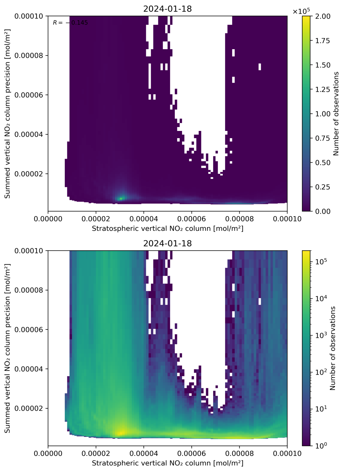
Figure 99: Scatter density plot of “Stratospheric vertical NO 2 column” against “Summed vertical NO 2 column precision” for 2024-01-17 to 2024-01-19.
