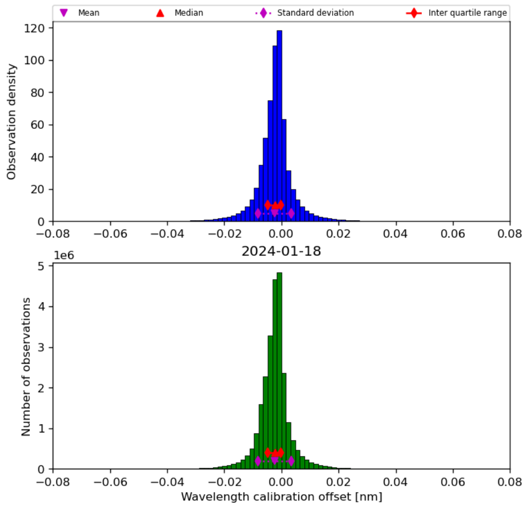
Figure 35: Histogram of “Wavelength calibration offset” for 2024-01-17 to 2024-01-19
