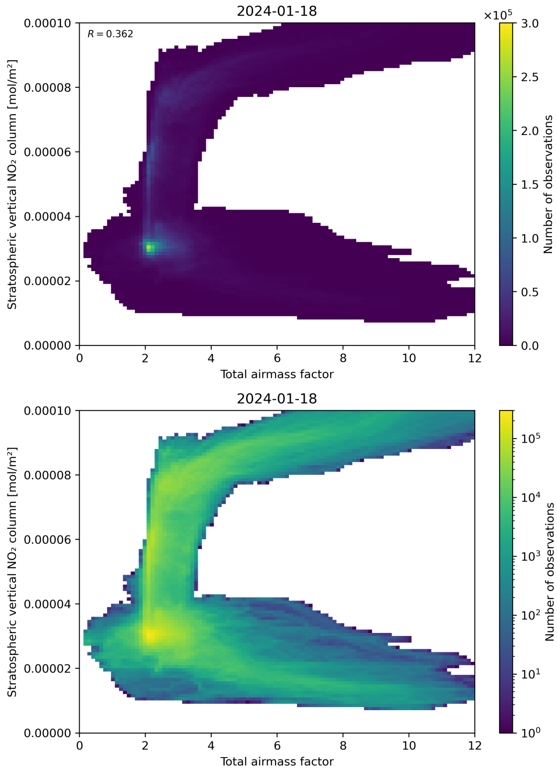
Figure 64: Scatter density plot of “Total airmass factor” against “Stratospheric vertical NO 2 column” for 2024-01-17 to 2024-01-19.
