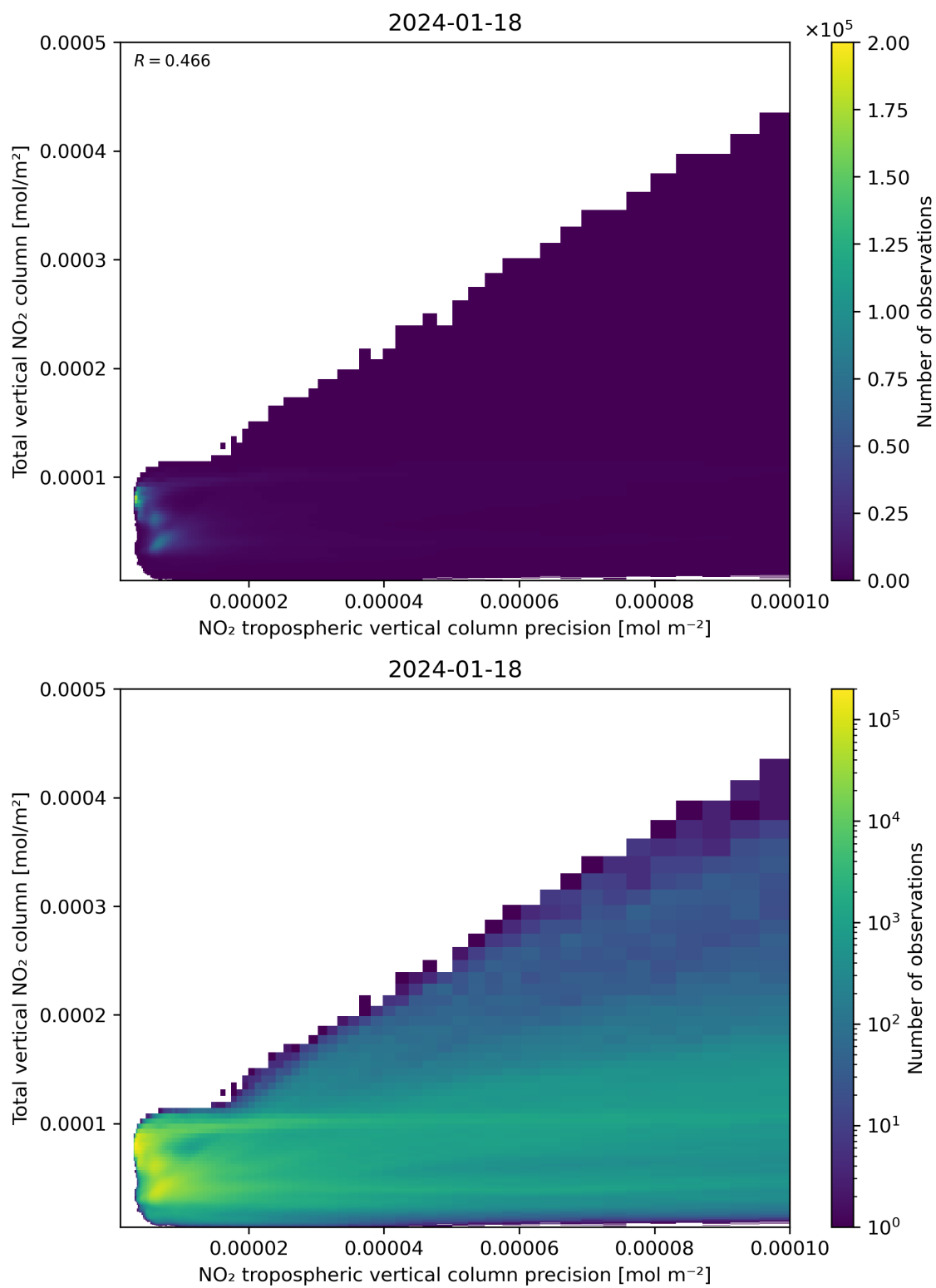
Figure 138: Scatter density plot of “NO 2 tropospheric vertical column precision” against “Total vertical NO 2 column” for 2024-01-17 to 2024-01-19.
