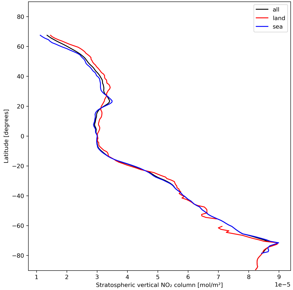
Figure 19: Zonal average of “Stratospheric vertical NO 2 column” for 2024-01-17 to 2024-01-19.
