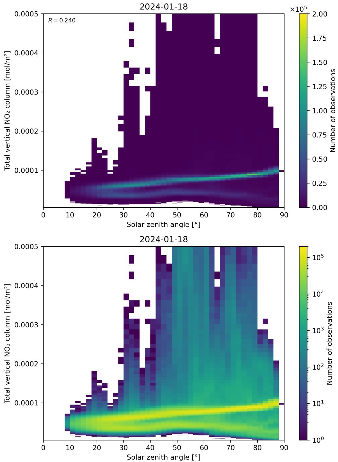
Figure 153: Scatter density plot of “Solar zenith angle” against “Total vertical NO 2 column” for 2024-01-17 to 2024-01-19.
