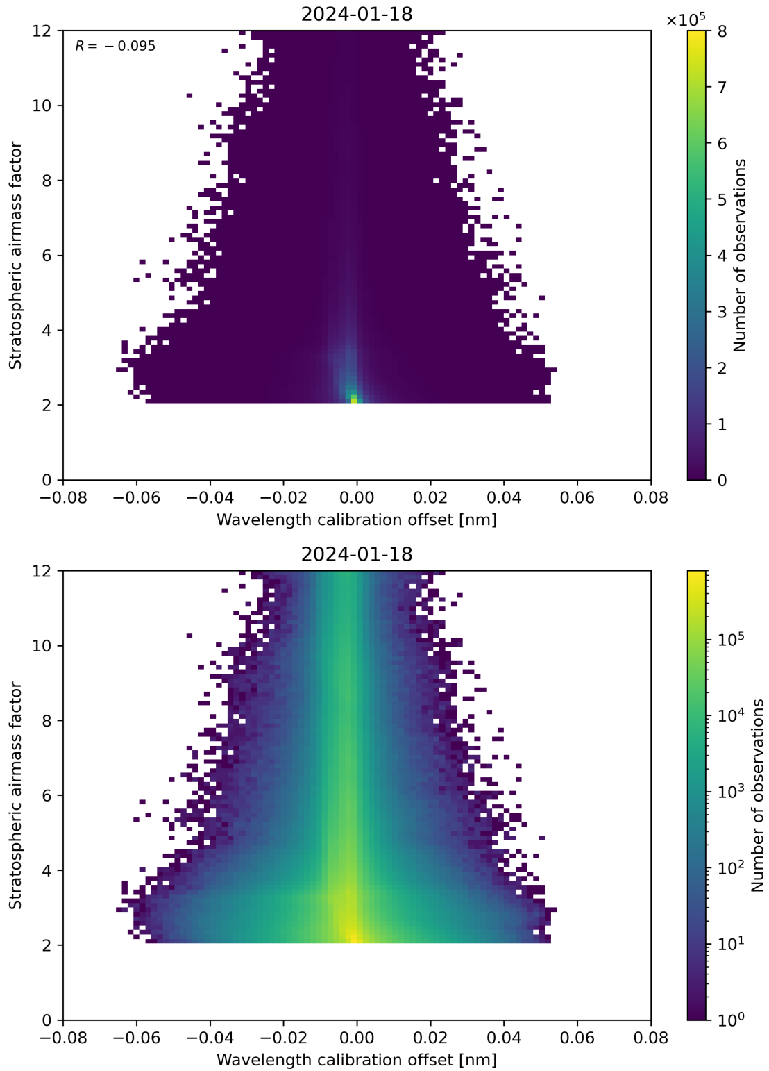
Figure 174: Scatter density plot of “Wavelength calibration offset” against “Stratospheric airmass factor” for 2024-01-17 to 2024-01-19.
