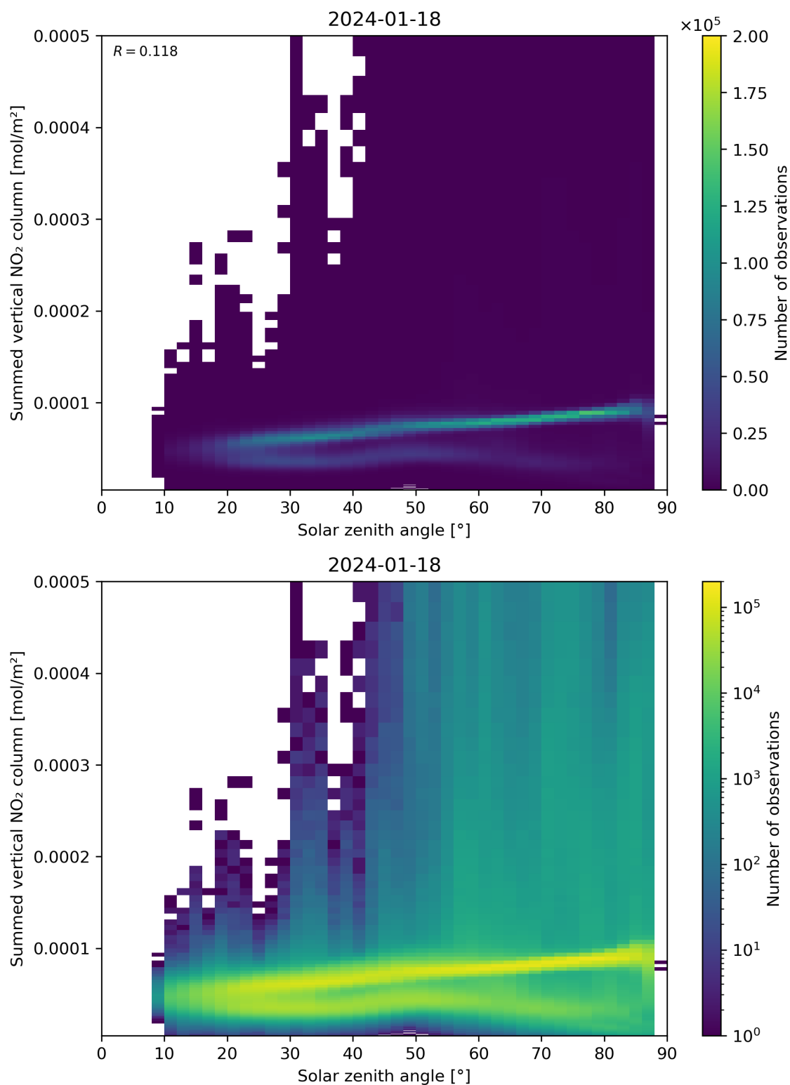
Figure 151: Scatter density plot of “Solar zenith angle” against “Summed vertical NO 2 column” for 2024-01-17 to 2024-01-19.
