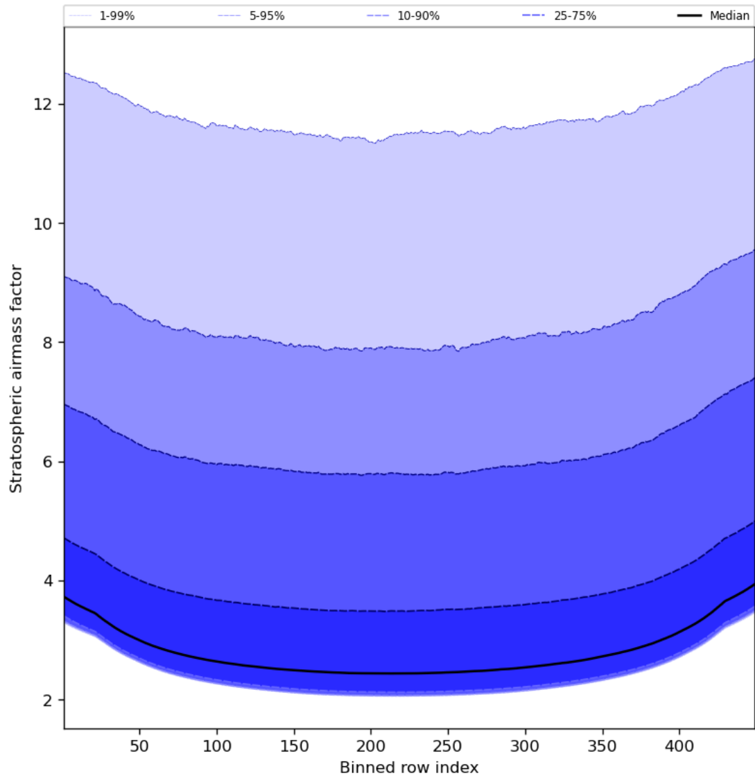
Figure 61: Along track statistics of “Stratospheric airmass factor” for 2024-01-17 to 2024-01-19
