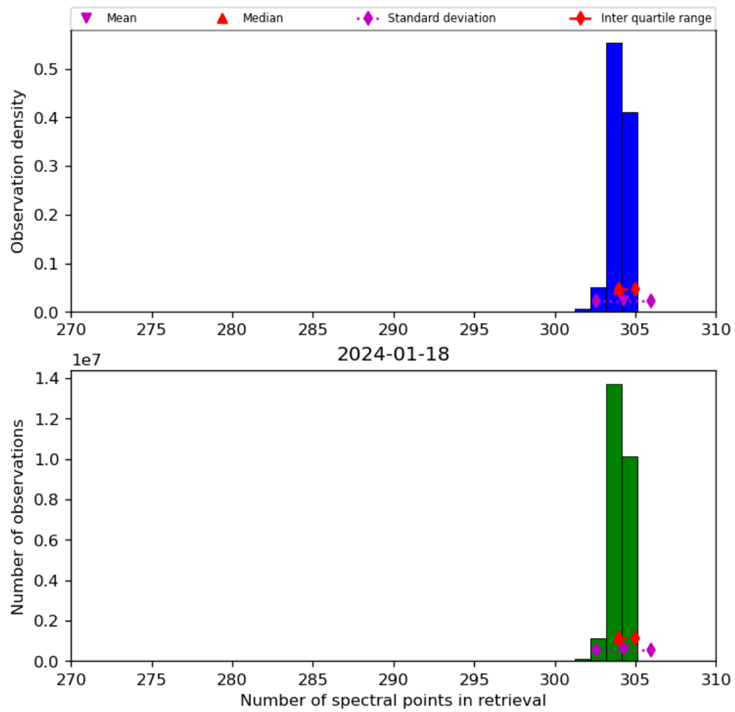
Figure 33: Histogram of “Number of spectral points in retrieval” for 2024-01-17 to 2024-01-19
