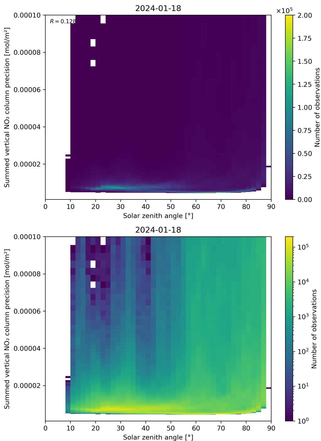
Figure 152: Scatter density plot of “Solar zenith angle” against “Summed vertical NO 2 column precision” for 2024-01-17 to 2024-01-19.
