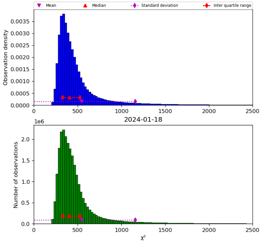
Figure 42: Histogram of “ \chi^2 ” for 2024-01-17 to 2024-01-19
