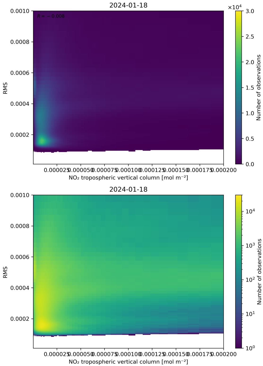
Figure 142: Scatter density plot of “NO 2 tropospheric vertical column” against “RMS” for 2024-01-17 to 2024-01-19.
