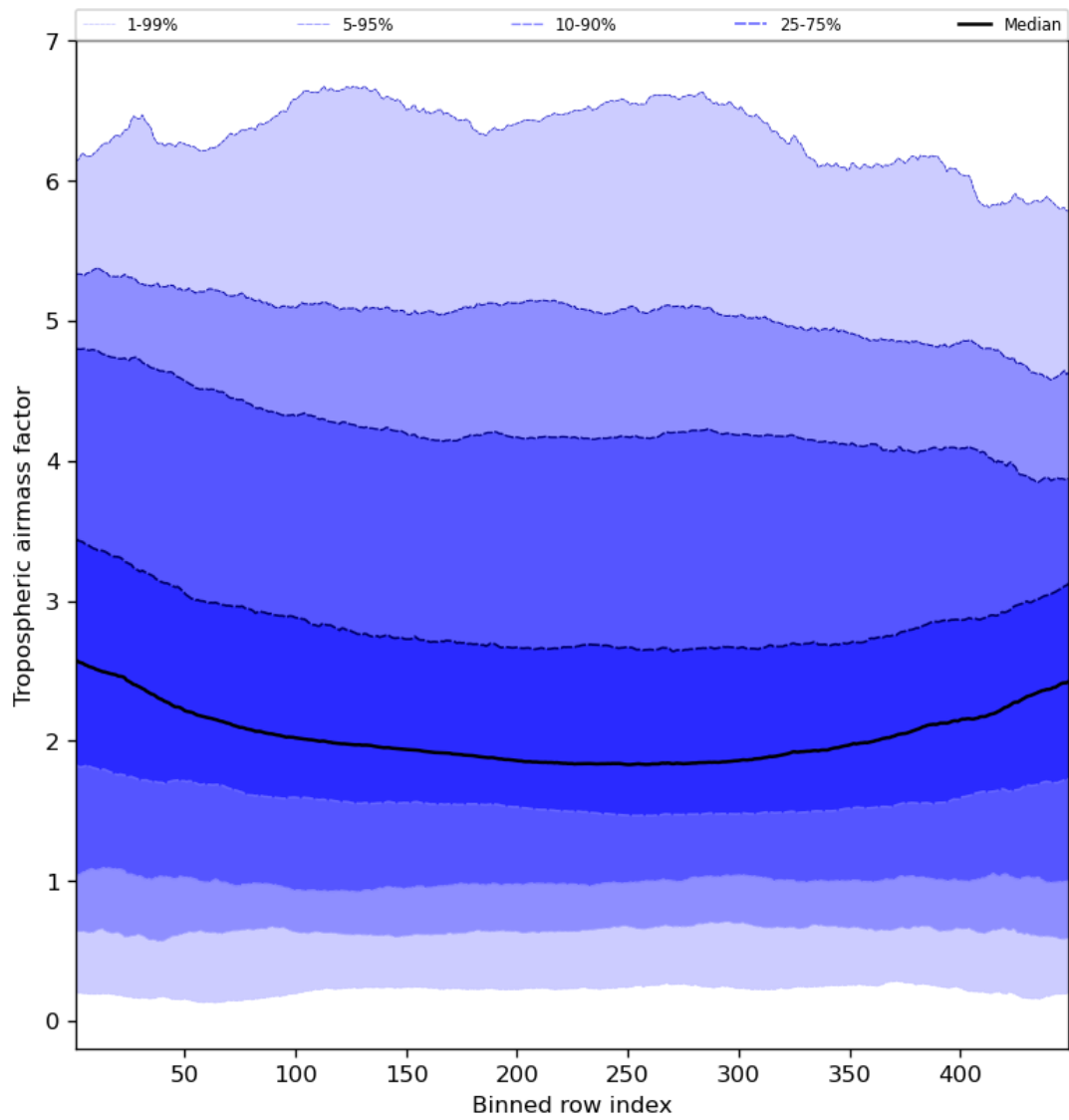
Figure 48: Along track statistics of “Tropospheric airmass factor” for 2024-01-17 to 2024-01-19
