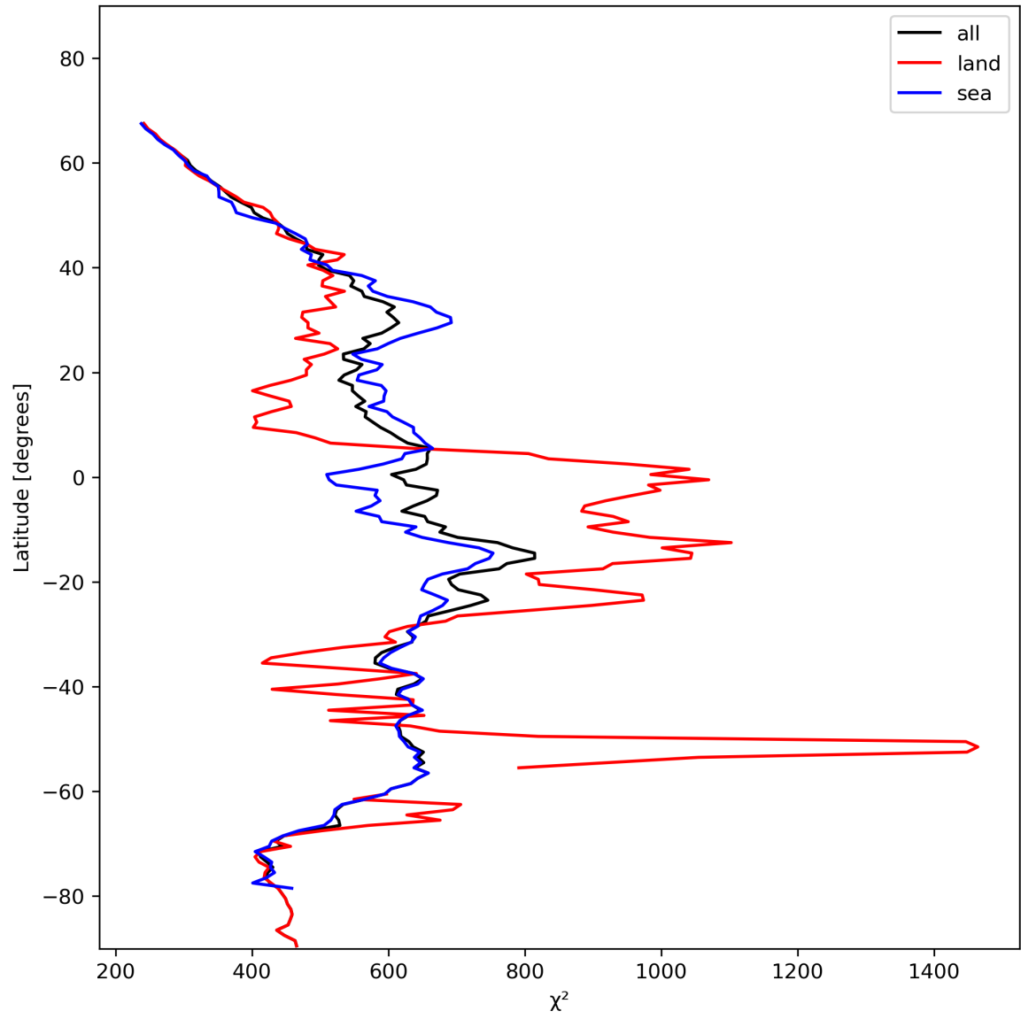
Figure 25: Zonal average of “ \chi^2 ” for 2024-01-17 to 2024-01-19.
