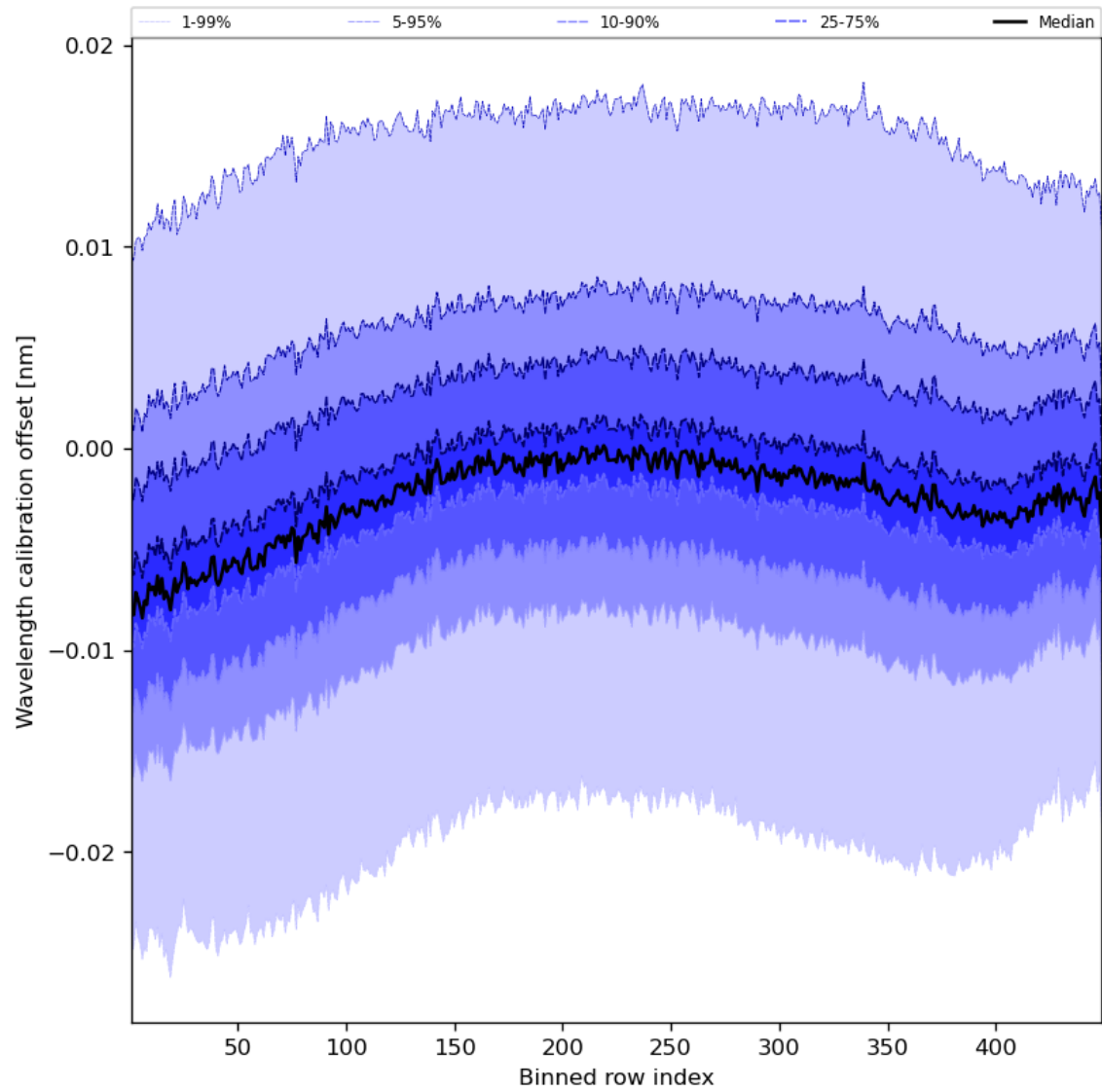
Figure 52: Along track statistics of “Wavelength calibration offset” for 2024-01-17 to 2024-01-19
