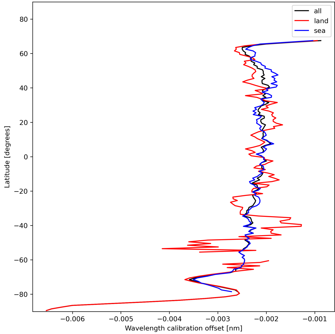
Figure 18: Zonal average of “Wavelength calibration offset” for 2024-01-17 to 2024-01-19.
