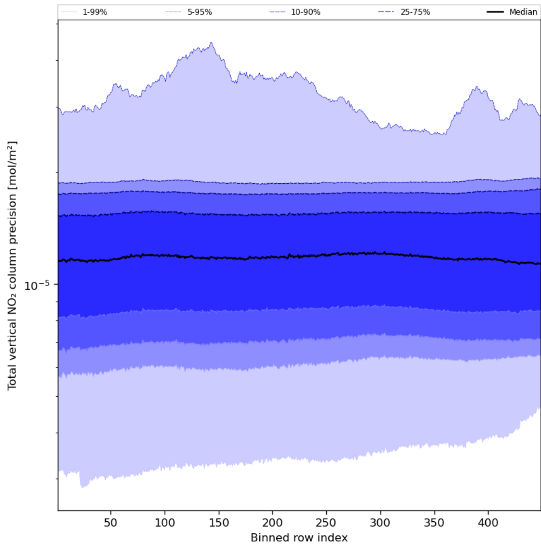
Figure 56: Along track statistics of “Total vertical NO 2 column precision” for 2024-01-17 to 2024-01-19
