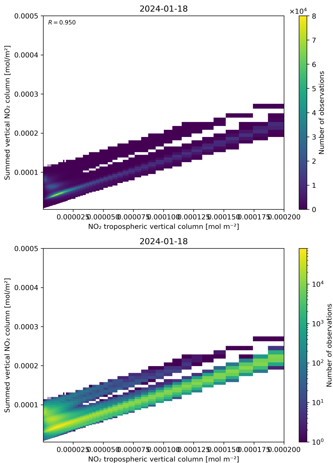
Figure 126: Scatter density plot of “NO 2 tropospheric vertical column” against “Summed vertical NO 2 column” for 2024-01-17 to 2024-01-19.
