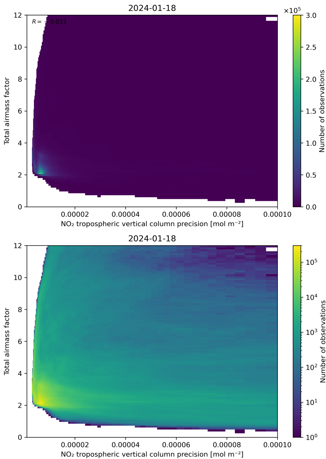
Figure 132: Scatter density plot of “NO 2 tropospheric vertical column precision” against “Total air mass factor” for 2024-01-17 to 2024-01-19.
