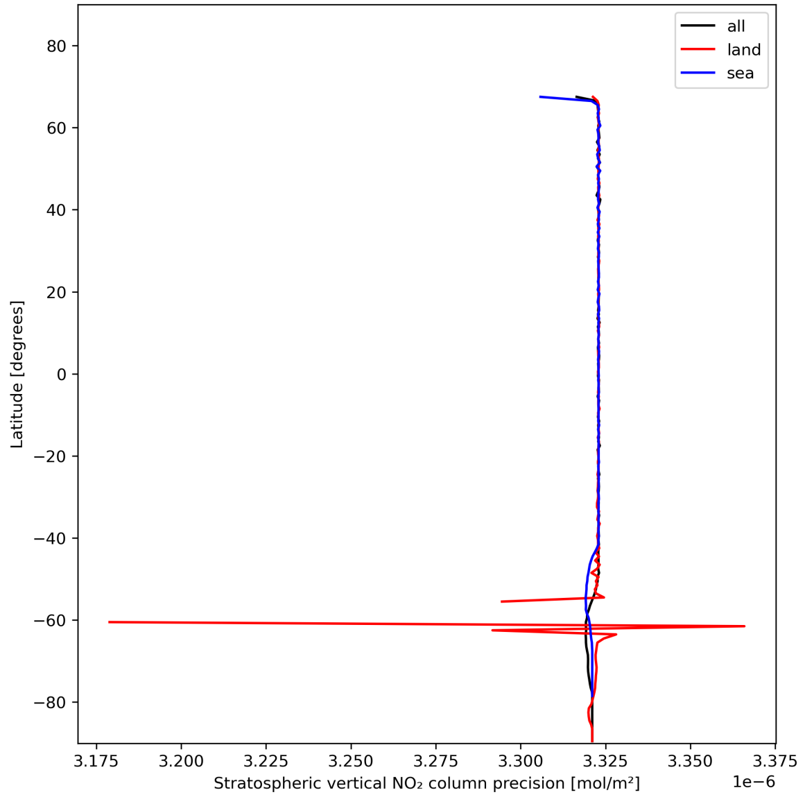
Figure 20: Zonal average of “Stratospheric vertical NO 2 column precision” for 2024-01-17 to 2024-01-19.
