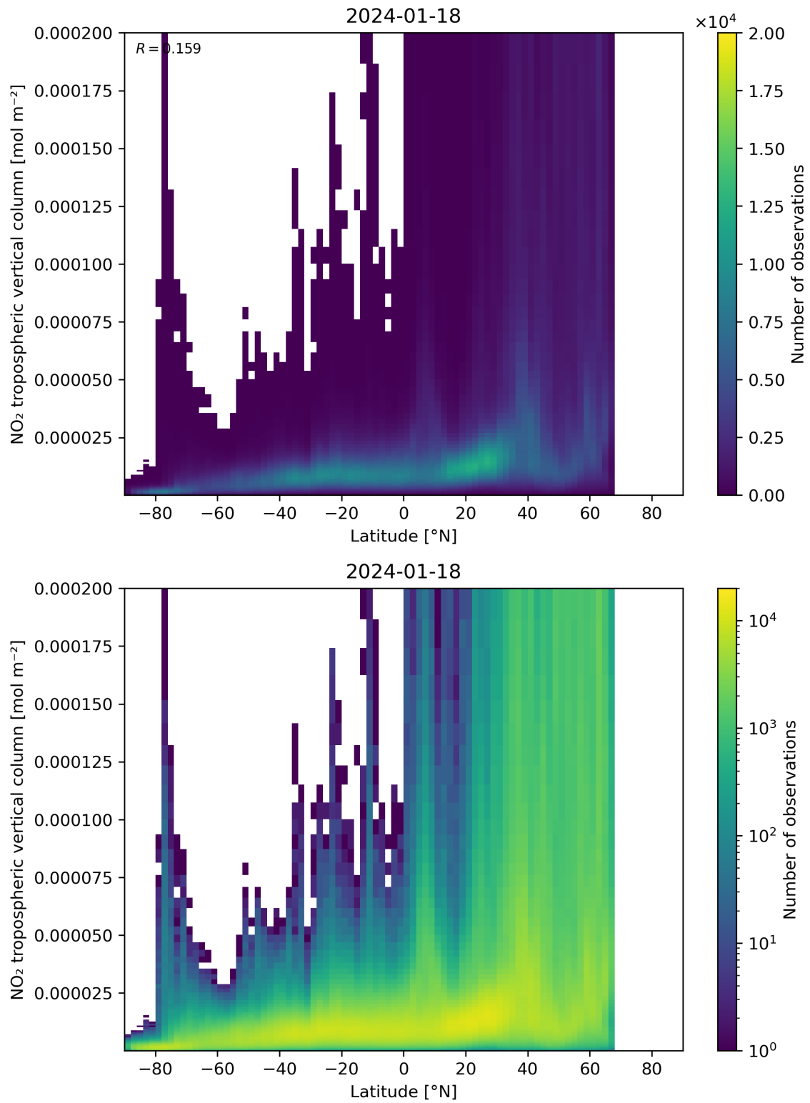
Figure 92: Scatter density plot of “Latitude” against “NO 2 tropospheric vertical column” for 2024-01-17 to 2024-01-19.
