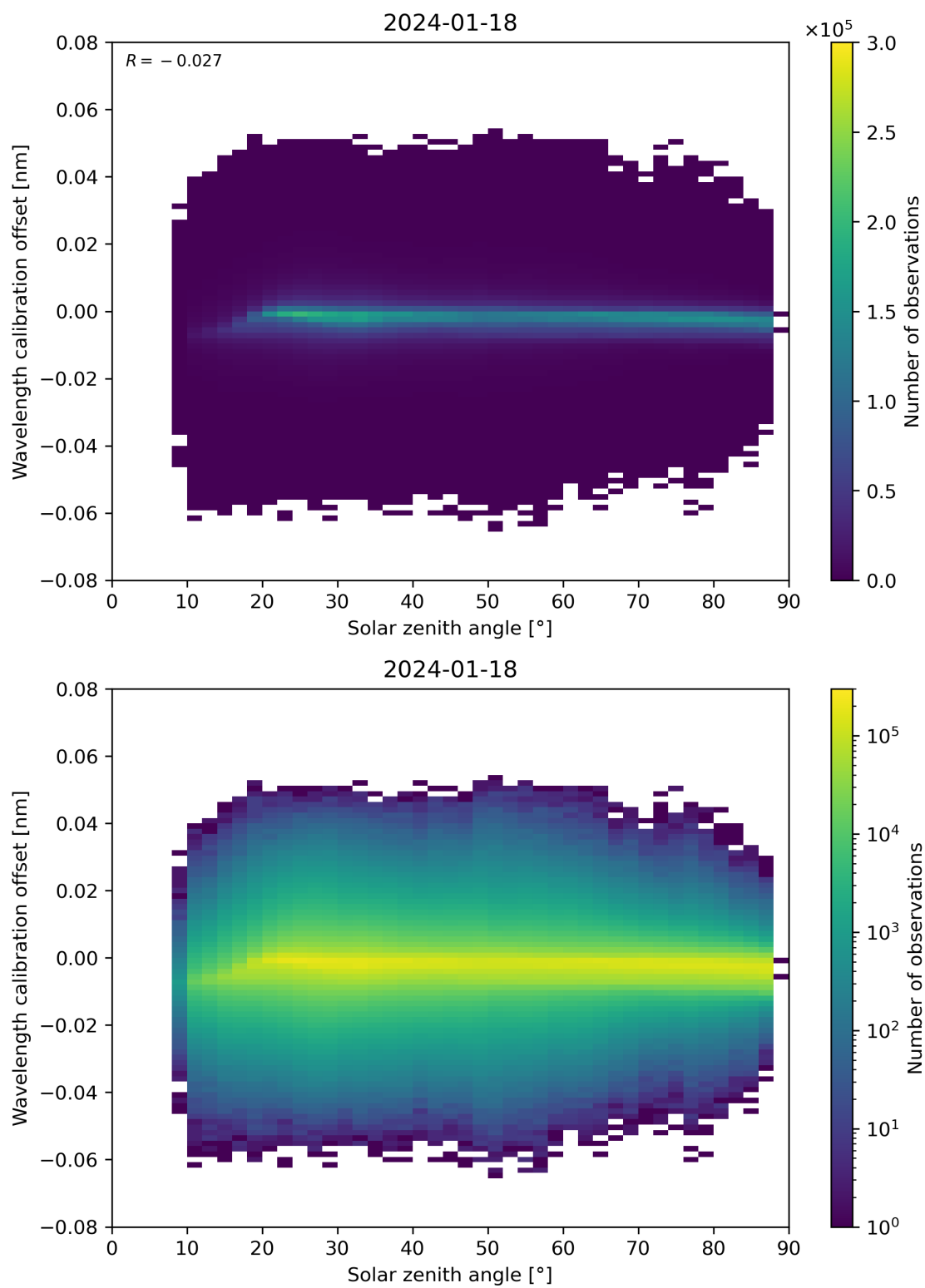
Figure 158: Scatter density plot of “Solar zenith angle” against “Wavelength calibration offset” for 2024-01-17 to 2024-01-19.
