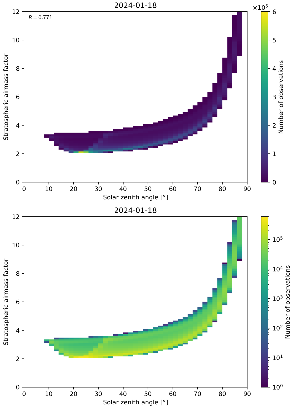
Figure 145: Scatter density plot of “Solar zenith angle” against “Stratospheric airmass factor” for 2024-01-17 to 2024-01-19.
