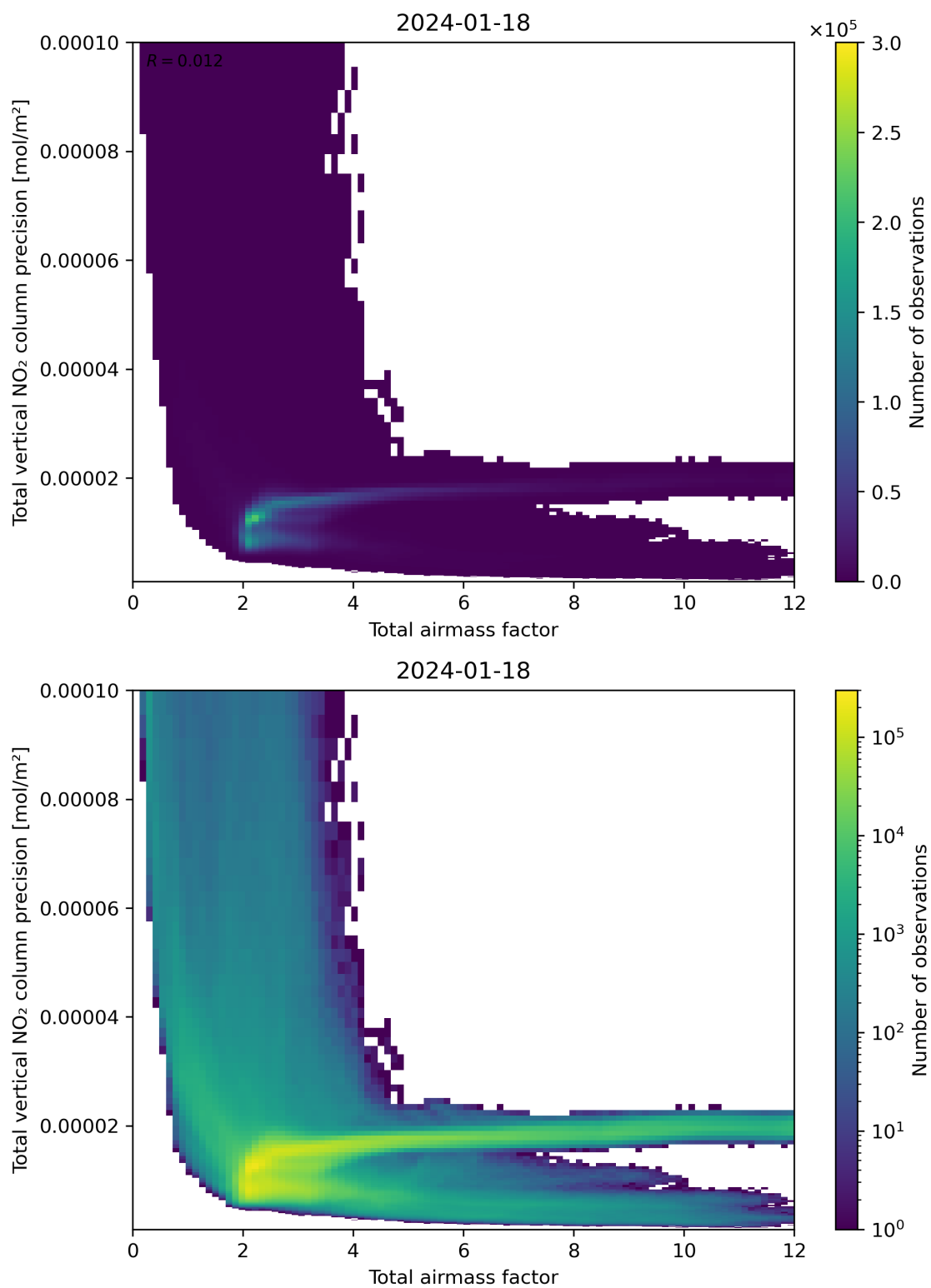
Figure 68: Scatter density plot of “Total airmass factor” against “Total vertical NO 2 column precision” for 2024-01-17 to 2024-01-19.
