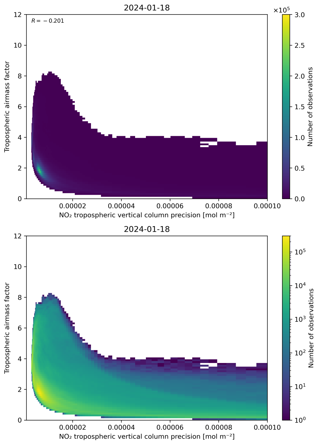
Figure 133: Scatter density plot of “NO 2 tropospheric vertical column precision” against “Tropospheric airmass factor” for 2024-01-17 to 2024-01-19.
