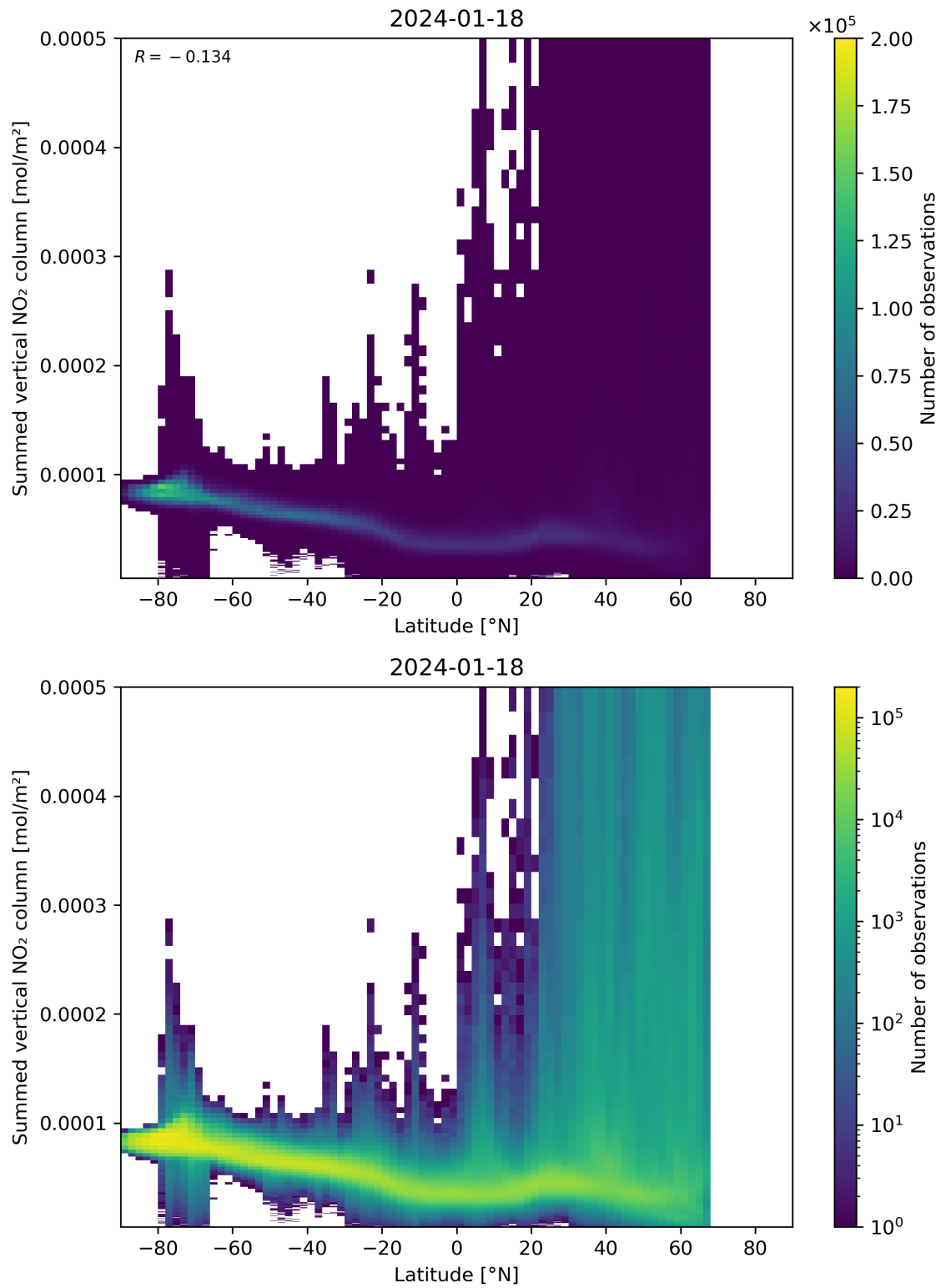
Figure 88: Scatter density plot of “Latitude” against “Summed vertical NO 2 column” for 2024-01-17 to 2024-01-19.
