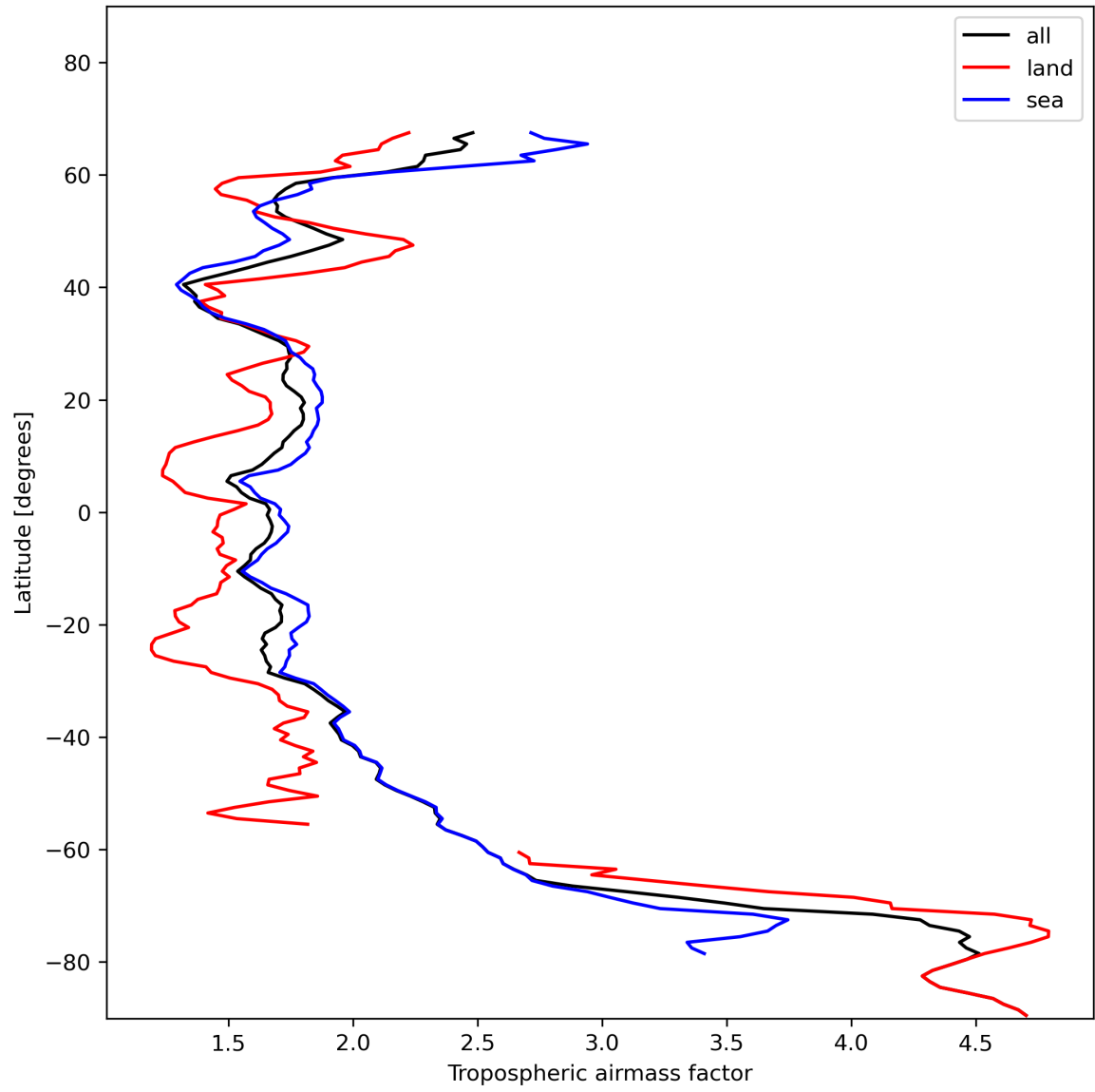
Figure 14: Zonal average of “Tropospheric airmass factor” for 2024-01-17 to 2024-01-19.
