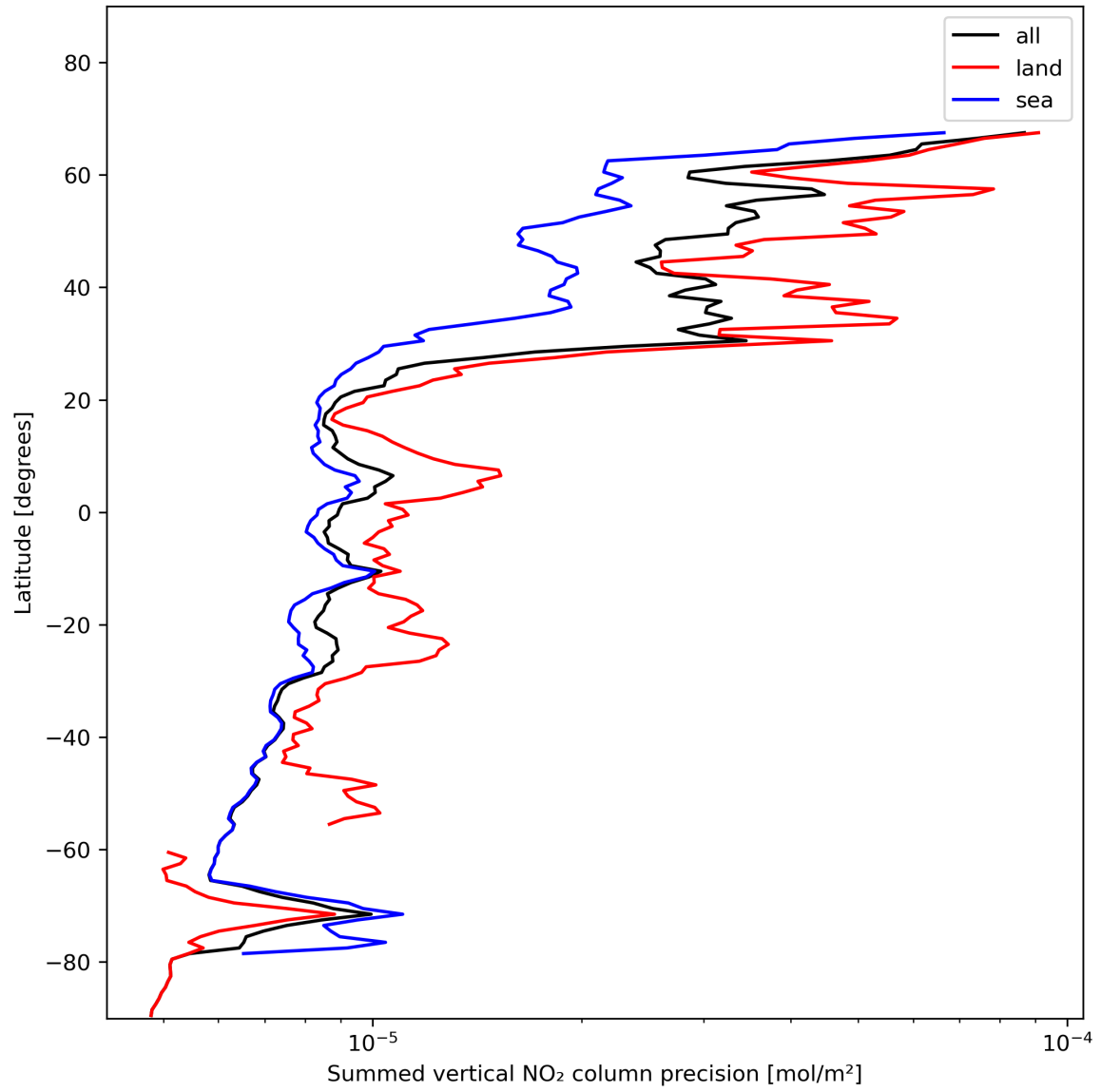
Figure 24: Zonal average of “Summed vertical NO 2 column precision” for 2024-01-17 to 2024-01-19.
