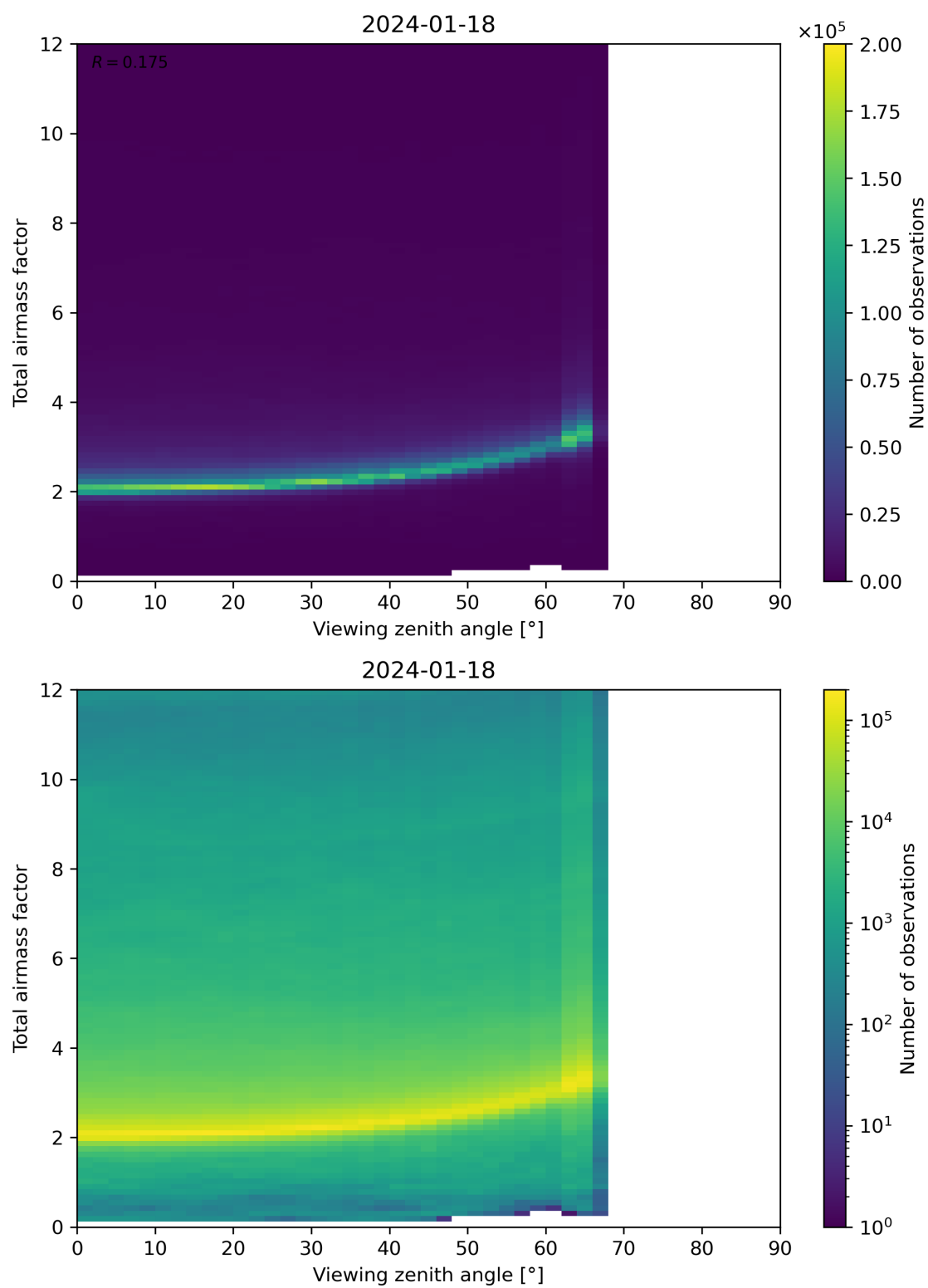
Figure 160: Scatter density plot of “Viewing zenith angle” against “Total airmass factor” for 2024-01-17 to 2024-01-19.
