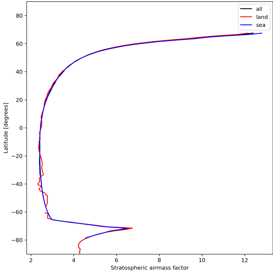
Figure 27: Zonal average of “Stratospheric airmass factor” for 2024-01-17 to 2024-01-19.
