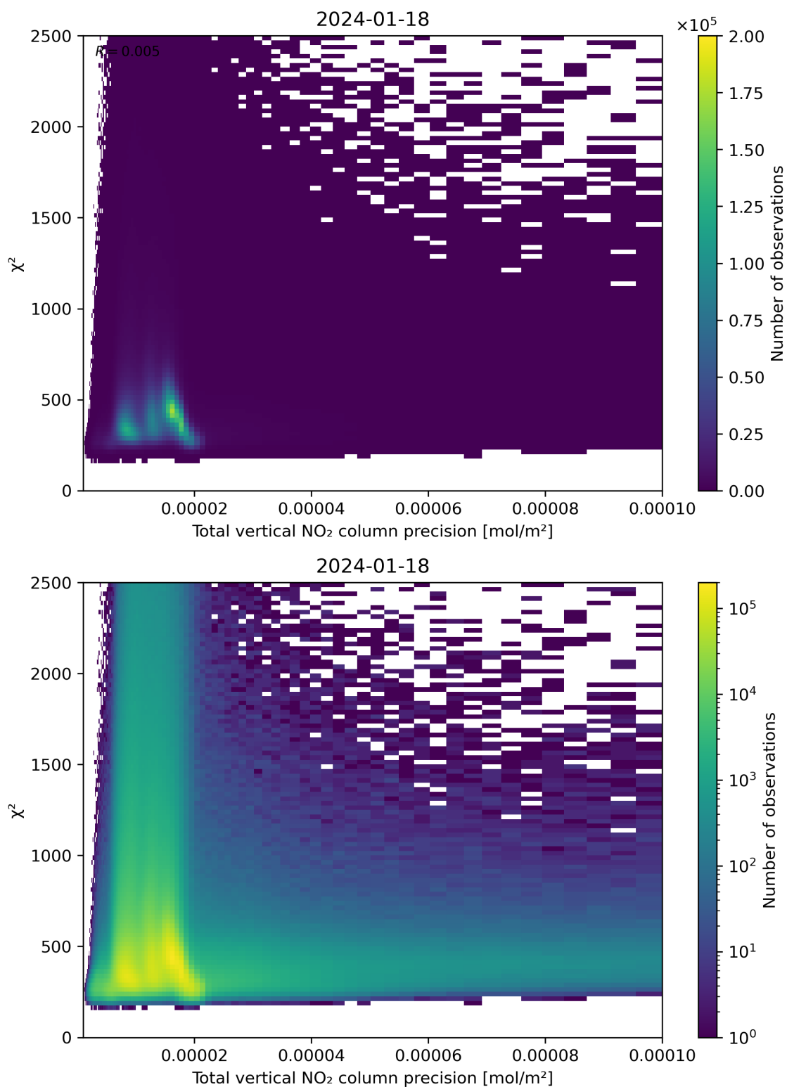
Figure 116: Scatter density plot of “Total vertical NO 2 column precision” against “ \chi^2 ” for 2024-01-17 to 2024-01-19.
