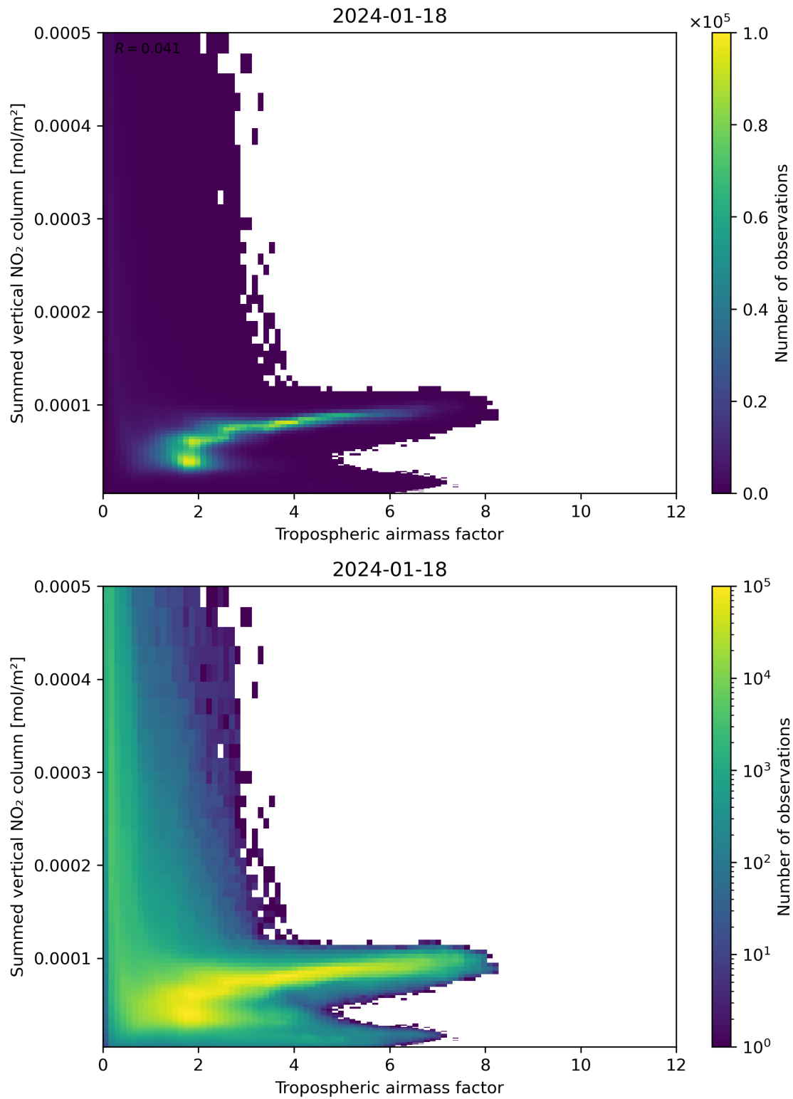
Figure 75: Scatter density plot of “Tropospheric airmass factor” against “Summed vertical NO 2 column” for 2024-01-17 to 2024-01-19.
