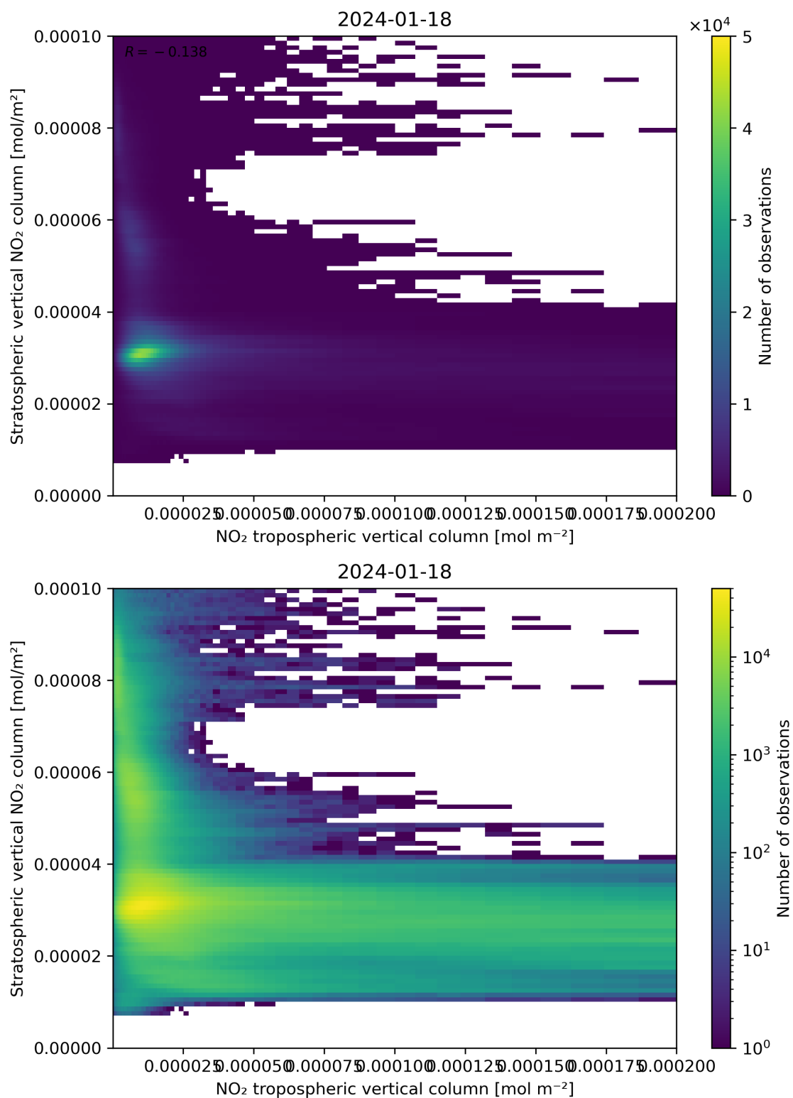
Figure 125: Scatter density plot of “NO 2 tropospheric vertical column” against “Stratospheric vertical NO 2 column” for 2024-01-17 to 2024-01-19.
