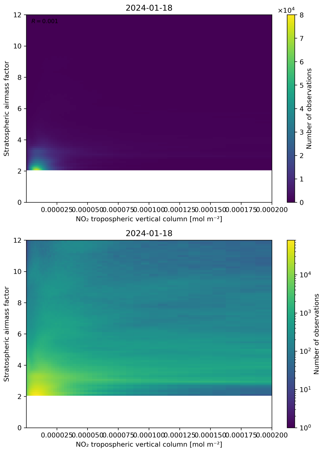
Figure 121: Scatter density plot of “NO 2 tropospheric vertical column” against “Stratospheric airmass factor” for 2024-01-17 to 2024-01-19.
