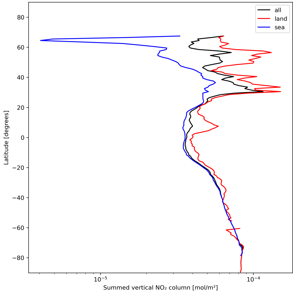
Figure 23: Zonal average of “Summed vertical NO 2 column” for 2024-01-17 to 2024-01-19.
