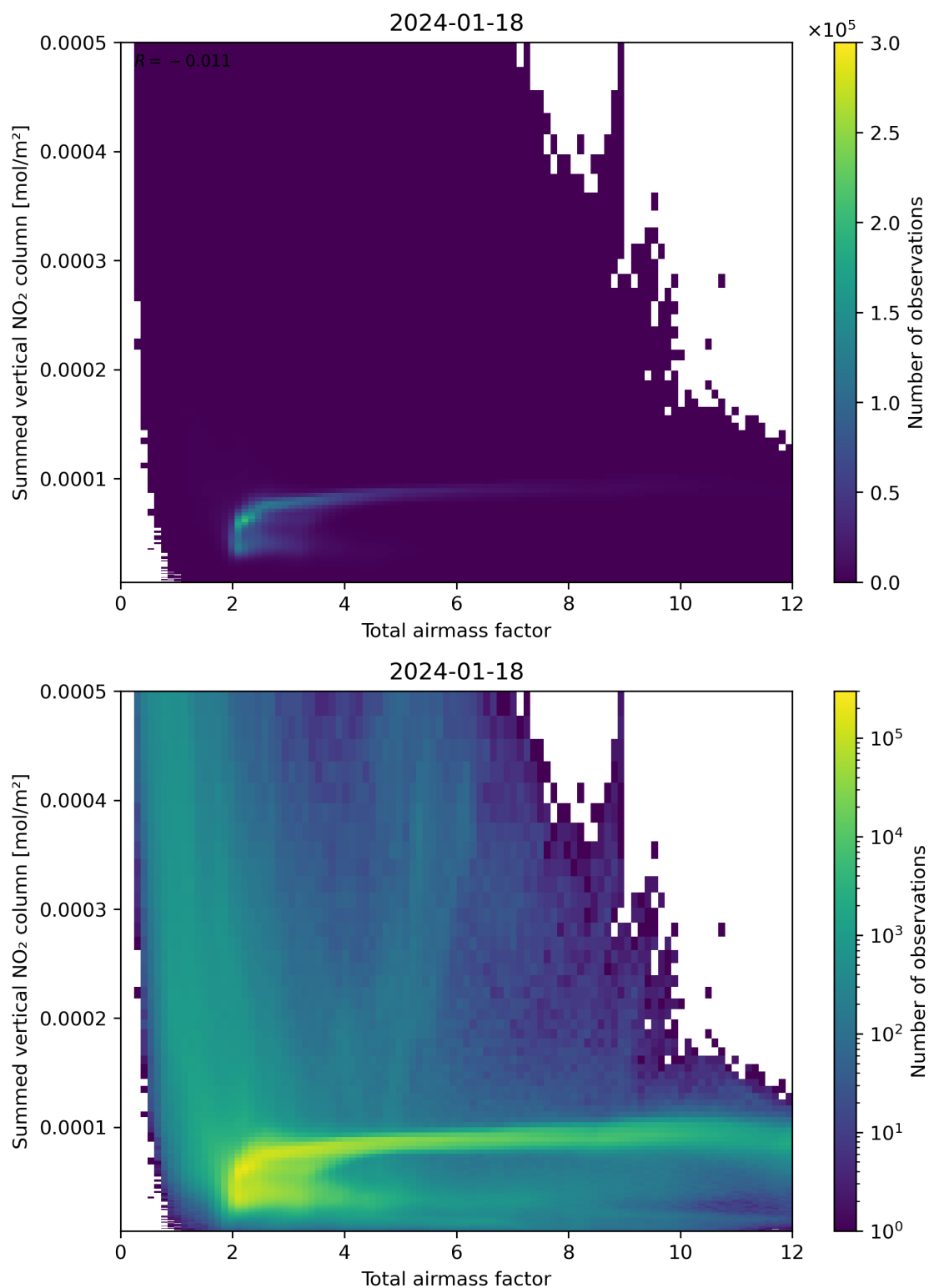
Figure 65: Scatter density plot of “Total airmass factor” against “Summed vertical NO 2 column” for 2024-01-17 to 2024-01-19.
