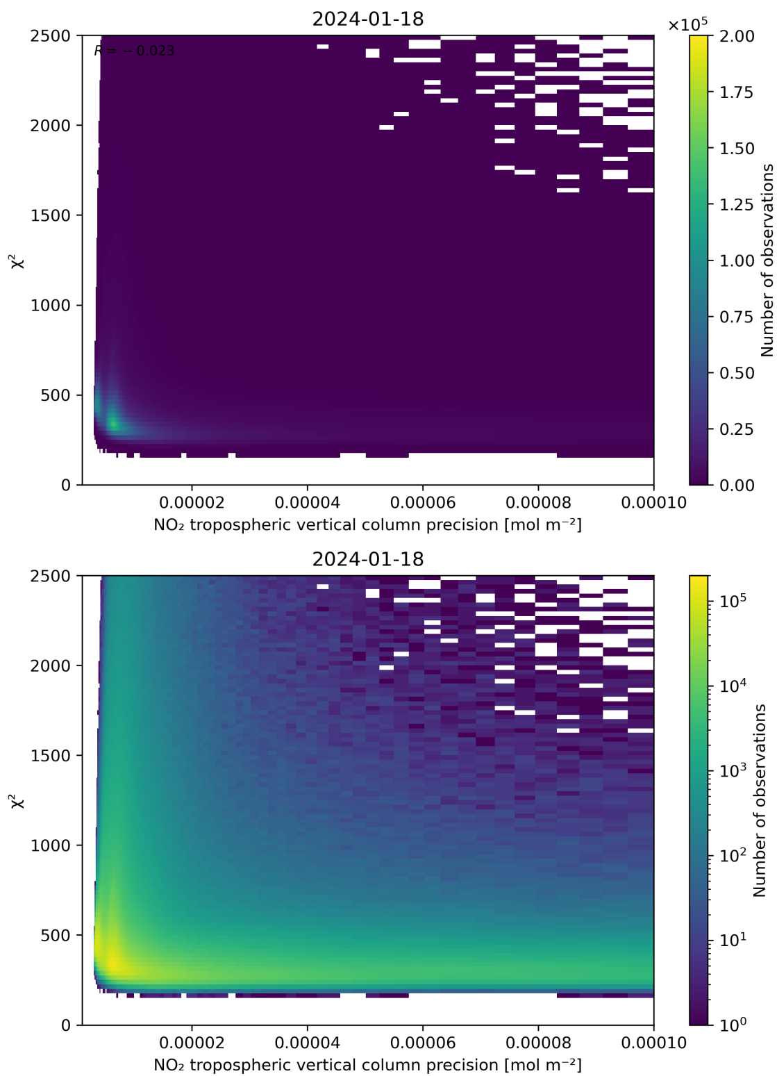
Figure 134: Scatter density plot of “NO 2 tropospheric vertical column precision” against “ \chi^2 ” for 2024-01-17 to 2024-01-19.
