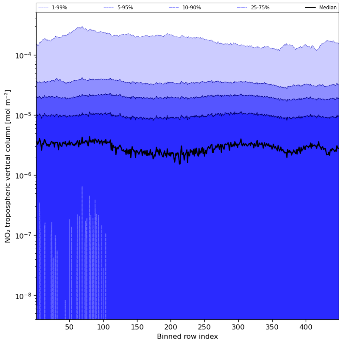
Figure 46: Along track statistics of “NO 2 tropospheric vertical column” for 2024-01-17 to 2024-01-19
