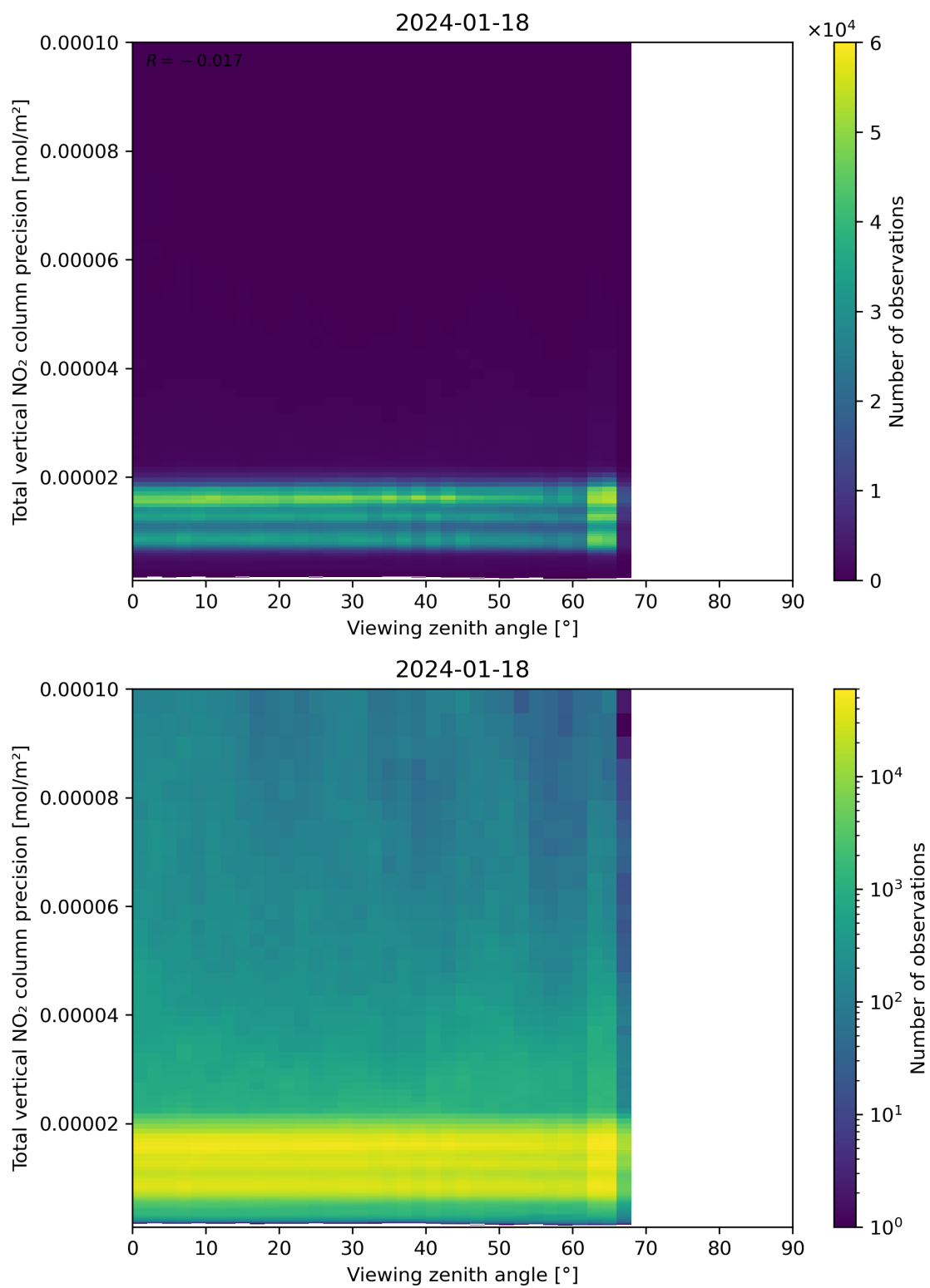
Figure 168: Scatter density plot of “Viewing zenith angle” against “Total vertical NO 2 column precision” for 2024-01-17 to 2024-01-19.
