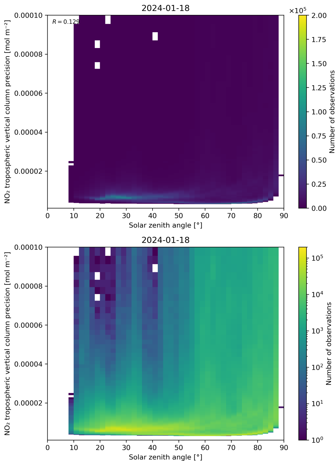
Figure 156: Scatter density plot of “Solar zenith angle” against “NO 2 tropospheric vertical column precision” for 2024-01-17 to 2024-01-19.
