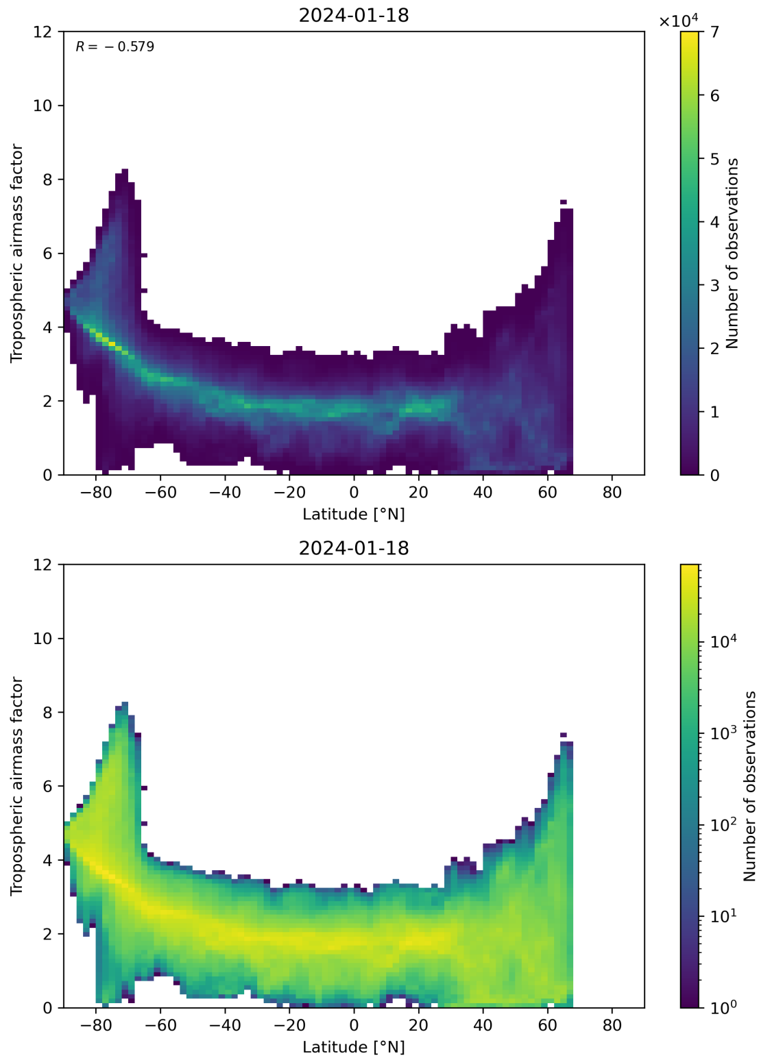
Figure 85: Scatter density plot of “Latitude” against “Tropospheric airmass factor” for 2024-01-17 to 2024-01-19.
