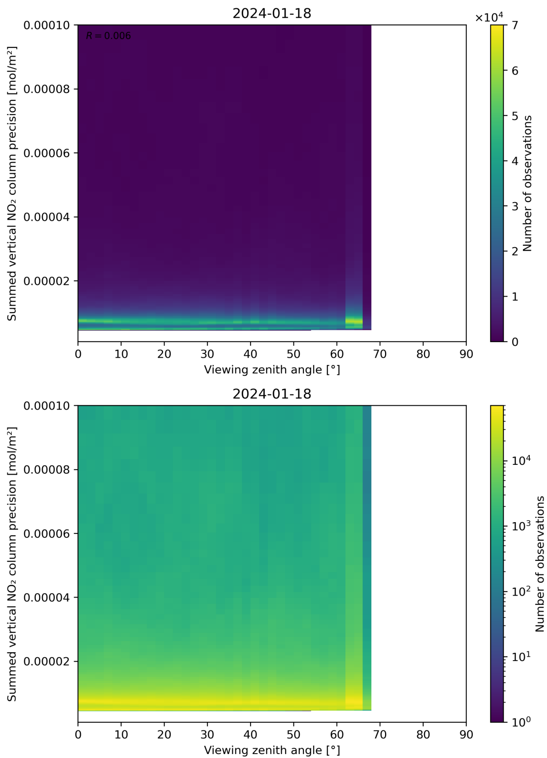
Figure 166: Scatter density plot of “Viewing zenith angle” against “Summed vertical NO 2 column precision” for 2024-01-17 to 2024-01-19.
