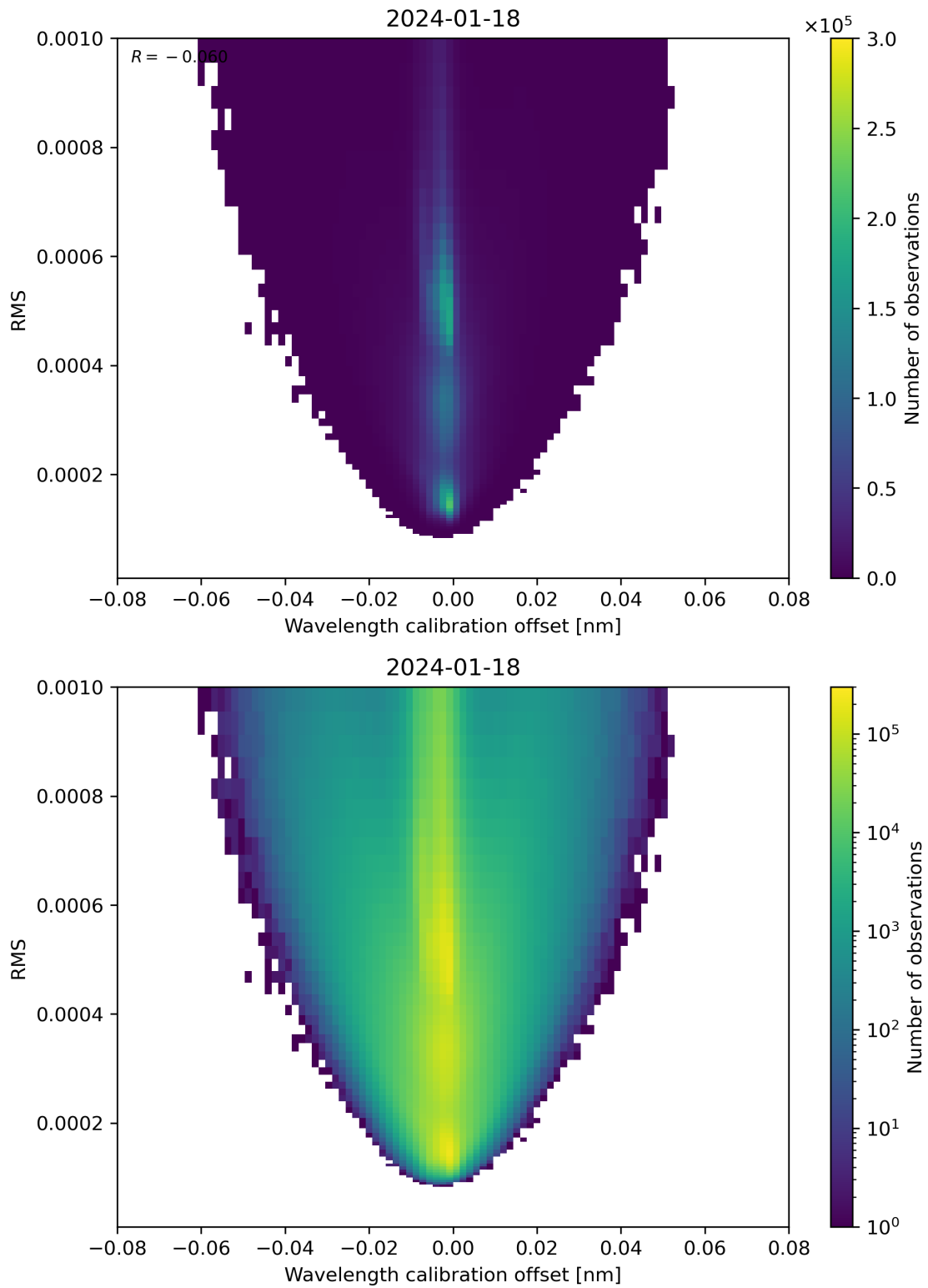
Figure 181: Scatter density plot of “Wavelength calibration offset” against “RMS” for 2024-01-17 to 2024-01-19.
