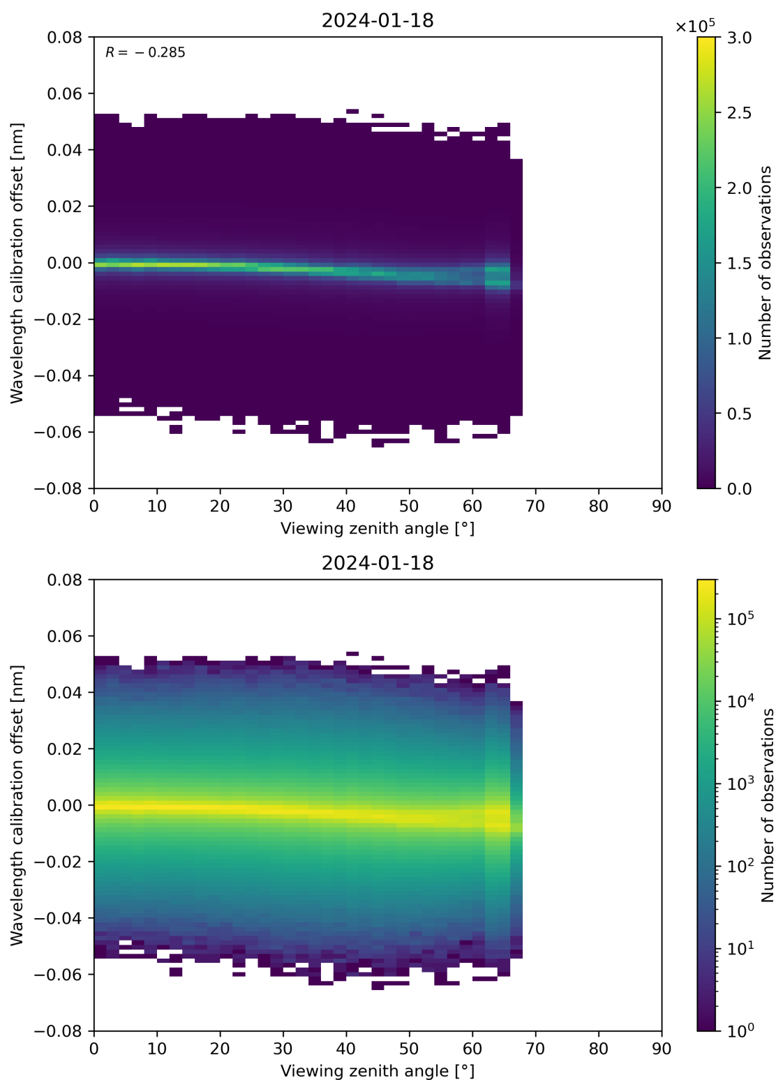
Figure 173: Scatter density plot of “Viewing zenith angle” against “Wavelength calibration offset” for 2024-01-17 to 2024-01-19.
