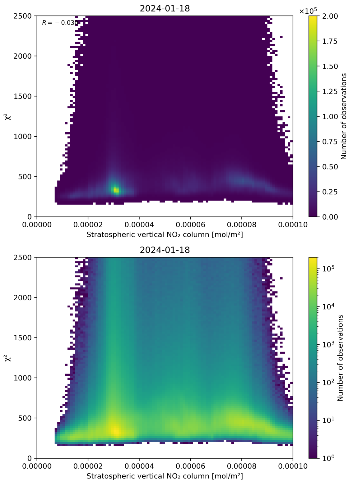
Figure 97: Scatter density plot of “Stratospheric vertical NO 2 column” against “ \chi^2 ” for 2024-01-17 to 2024-01-19.
