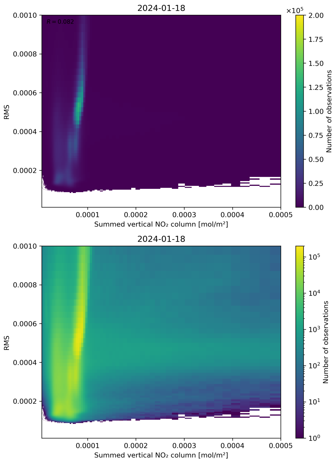
Figure 109: Scatter density plot of “Summed vertical NO 2 column” against “RMS” for 2024-01-17 to 2024-01-19.
