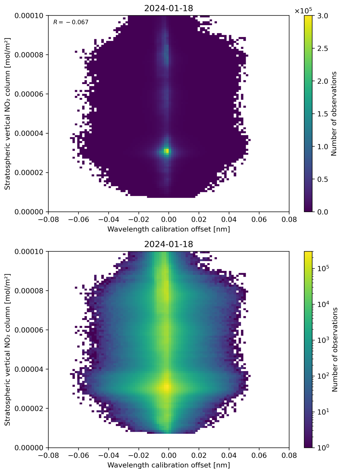
Figure 176: Scatter density plot of “Wavelength calibration offset” against “Stratospheric vertical NO 2 column” for 2024-01-17 to 2024-01-19.
