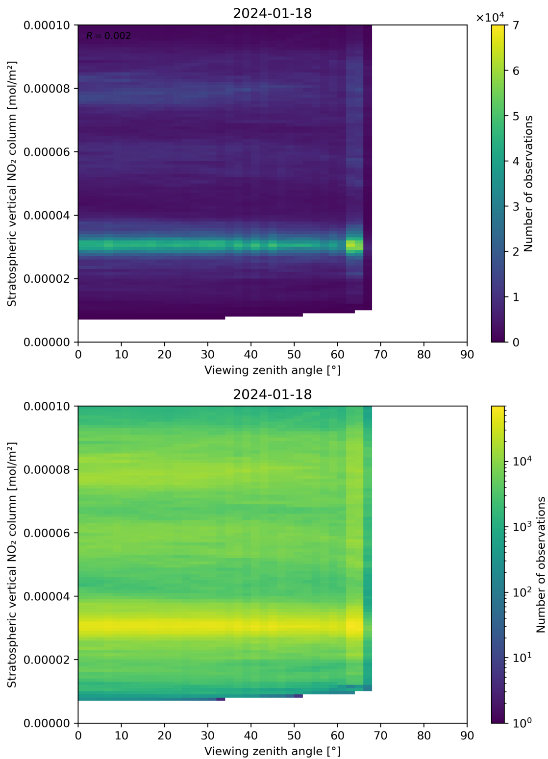
Figure 164: Scatter density plot of “Viewing zenith angle” against “Stratospheric vertical NO 2 column” for 2024-01-17 to 2024-01-19.
