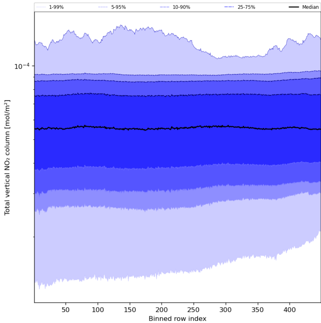
Figure 55: Along track statistics of “Total vertical NO 2 column” for 2024-01-17 to 2024-01-19
