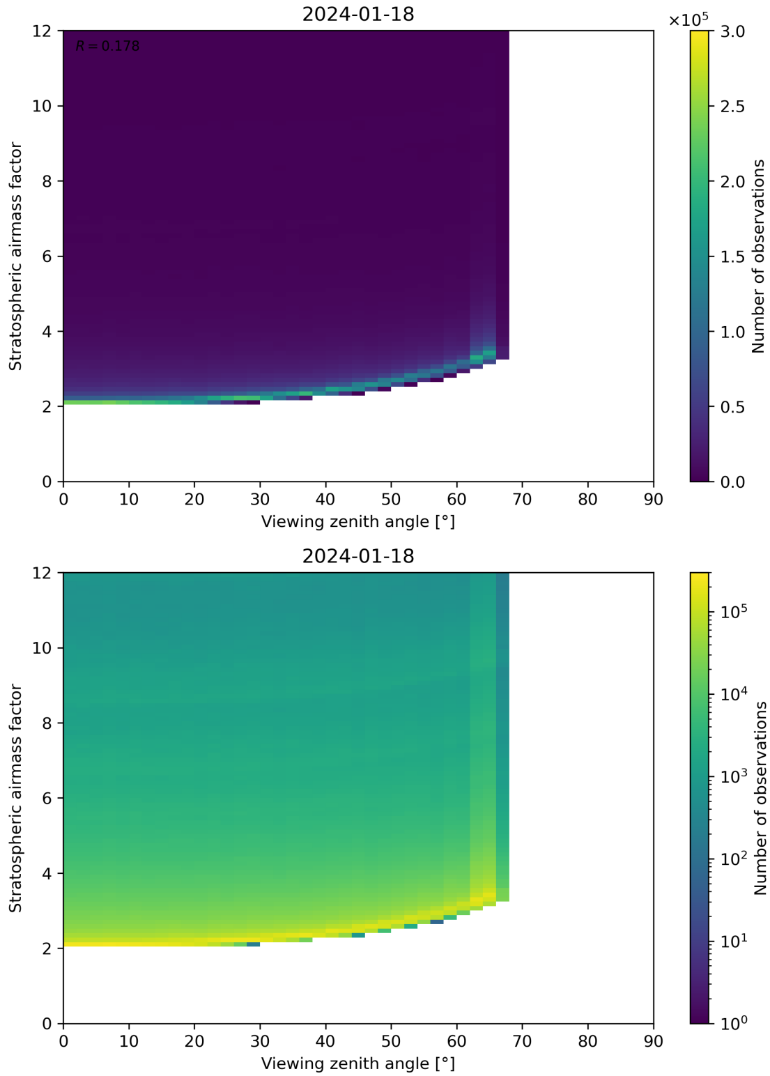
Figure 159: Scatter density plot of “Viewing zenith angle” against “Stratospheric airmass factor” for 2024-01-17 to 2024-01-19.
