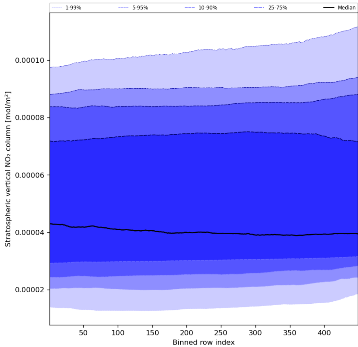
Figure 53: Along track statistics of “Stratospheric vertical NO 2 column” for 2024-01-17 to 2024-01-19
