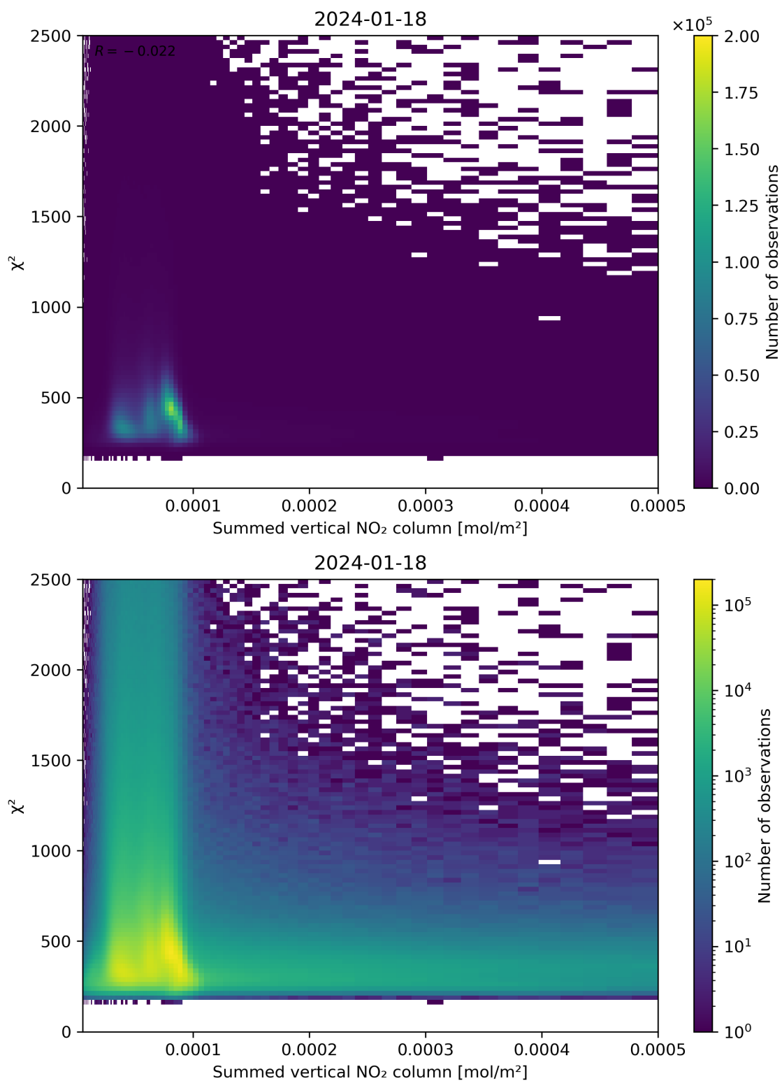
Figure 104: Scatter density plot of “Summed vertical NO 2 column” against “ \chi^2 ” for 2024-01-17 to 2024-01-19.
