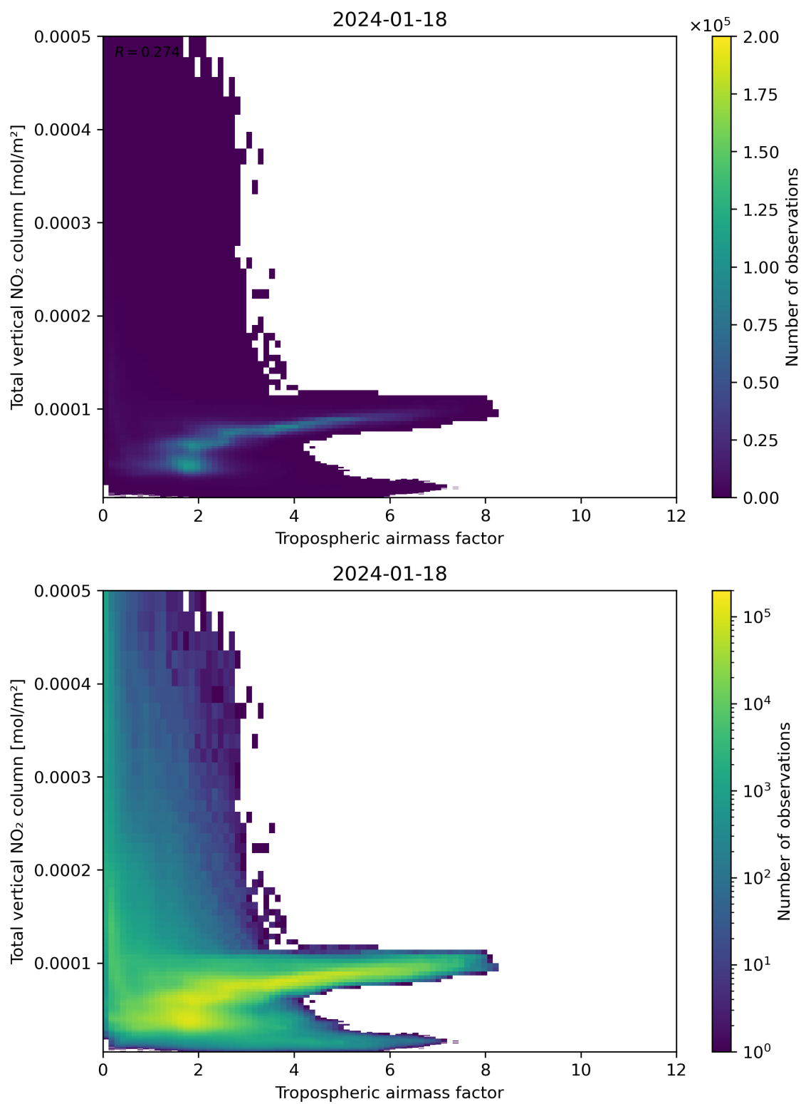
Figure 77: Scatter density plot of “Tropospheric airmass factor” against “Total vertical NO 2 column” for 2024-01-17 to 2024-01-19.
