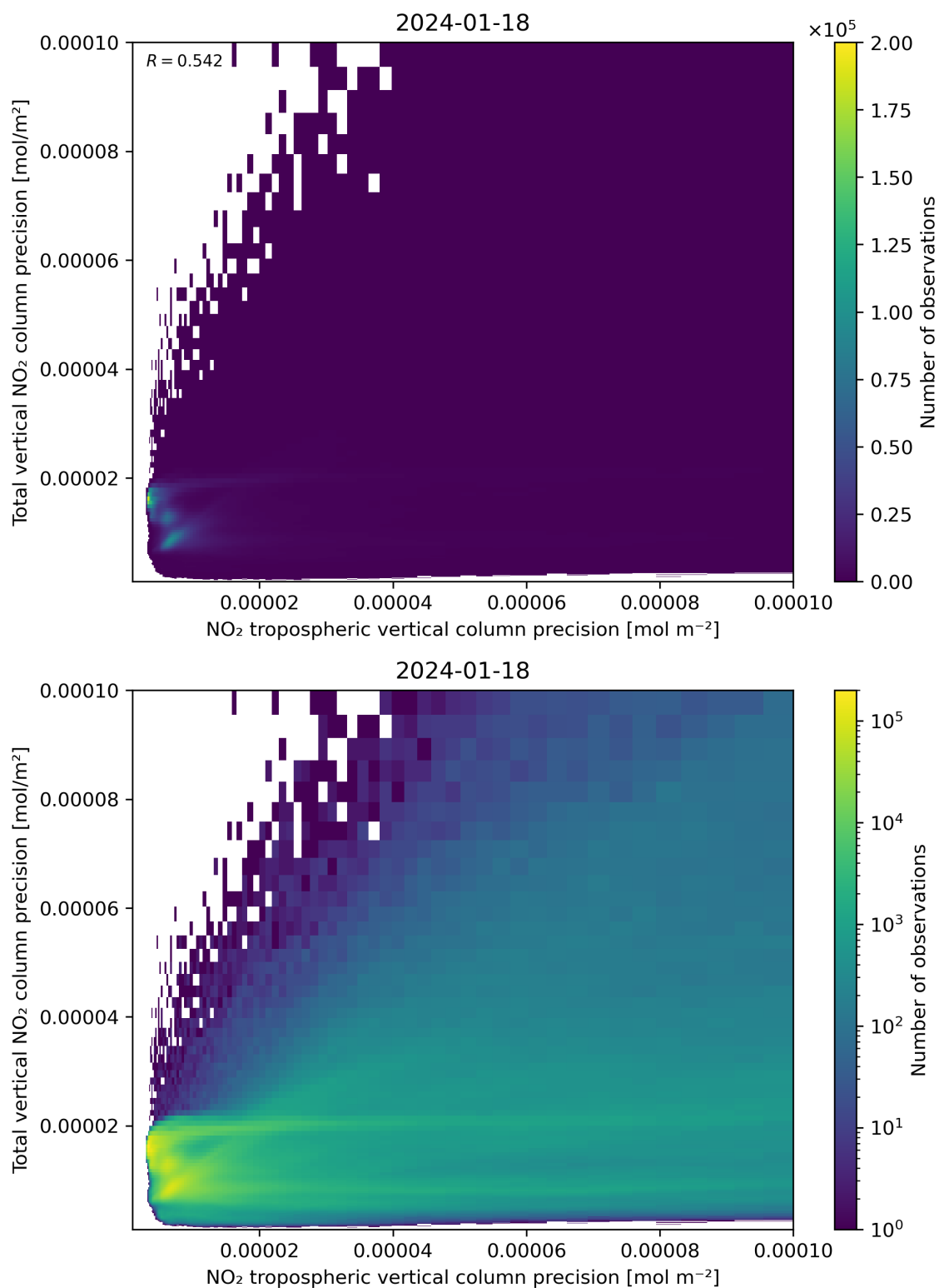
Figure 139: Scatter density plot of “NO 2 tropospheric vertical column precision” against “Total vertical NO 2 column precision” for 2024-01-17 to 2024-01-19.
