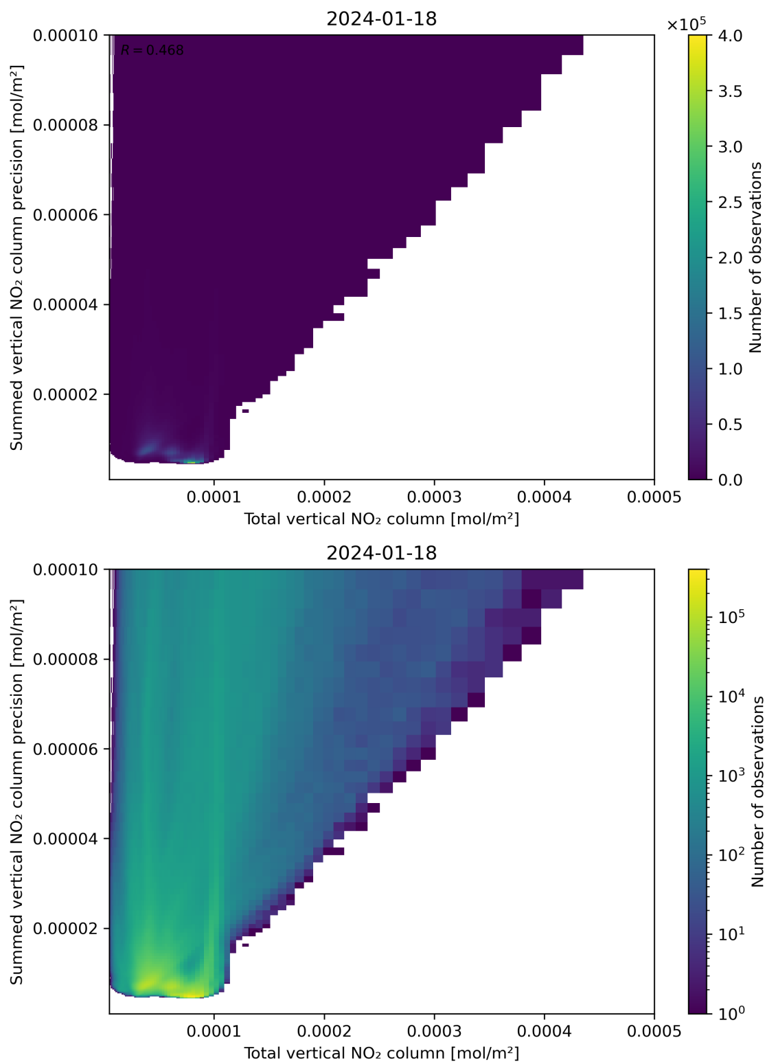
Figure 113: Scatter density plot of “Total vertical NO 2 column” against “Summed vertical NO 2 column precision” for 2024-01-17 to 2024-01-19.
