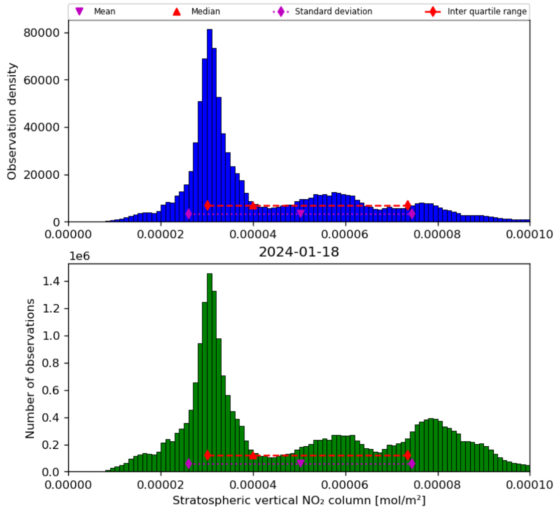
Figure 36: Histogram of “Stratospheric vertical NO 2 column” for 2024-01-17 to 2024-01-19
