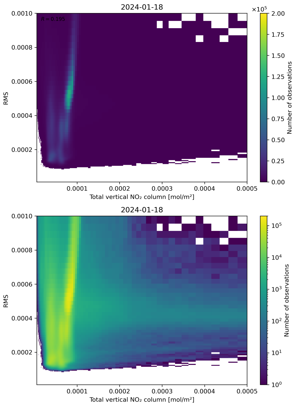
Figure 120: Scatter density plot of “Total vertical NO 2 column” against “RMS” for 2024-01-17 to 2024-01-19.
