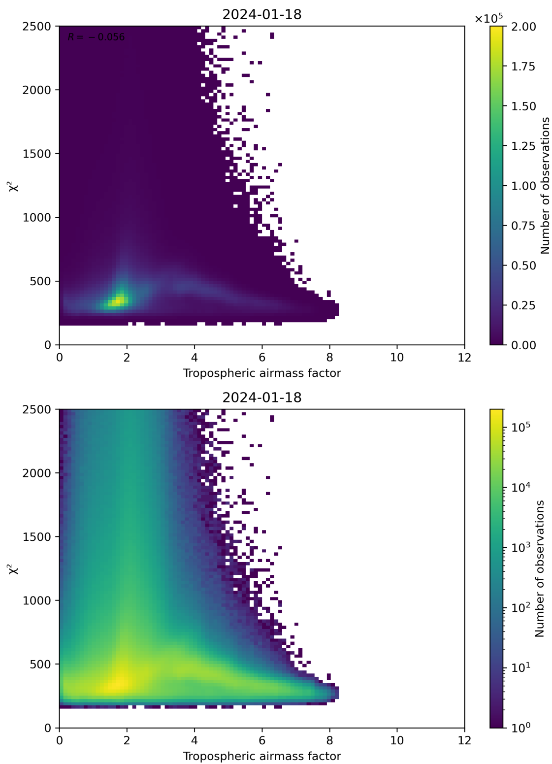
Figure 73: Scatter density plot of “Tropospheric airmass factor” against “ \chi^2 ” for 2024-01-17 to 2024-01-19.
