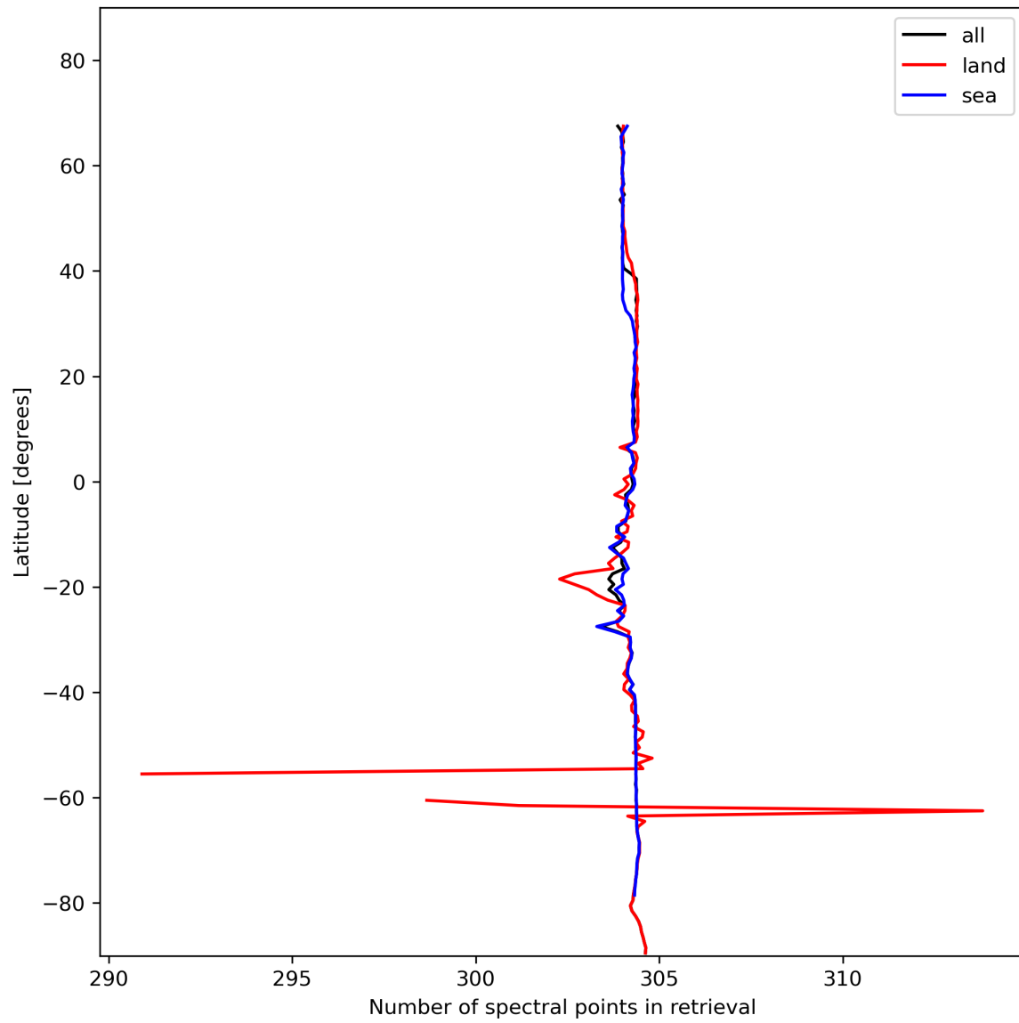
Figure 16: Zonal average of “Number of spectral points in retrieval” for 2024-01-17 to 2024-01-19.
