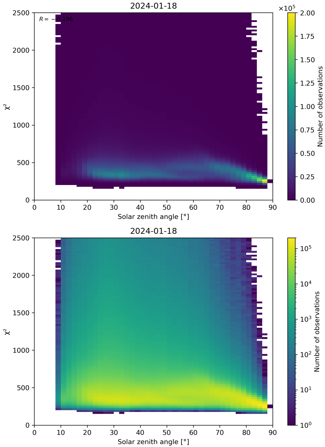
Figure 148: Scatter density plot of “Solar zenith angle” against “ \chi^2 ” for 2024-01-17 to 2024-01-19.
