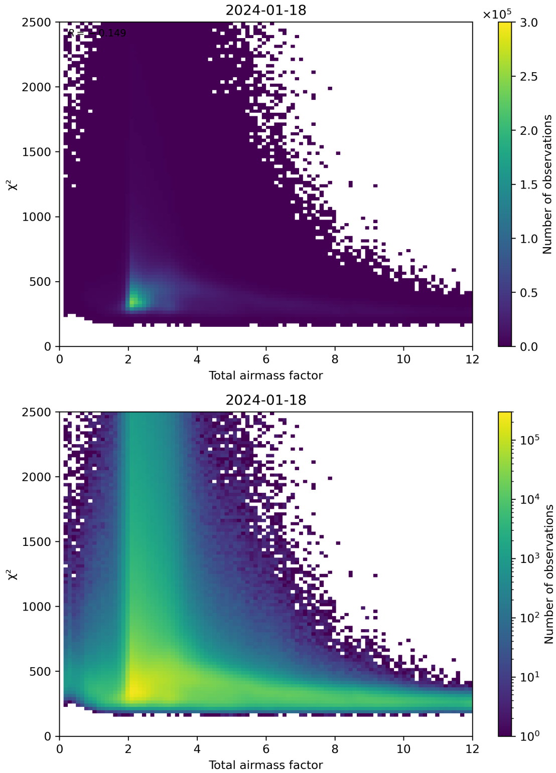
Figure 63: Scatter density plot of “Total airmass factor” against “ \chi^2 ” for 2024-01-17 to 2024-01-19.
