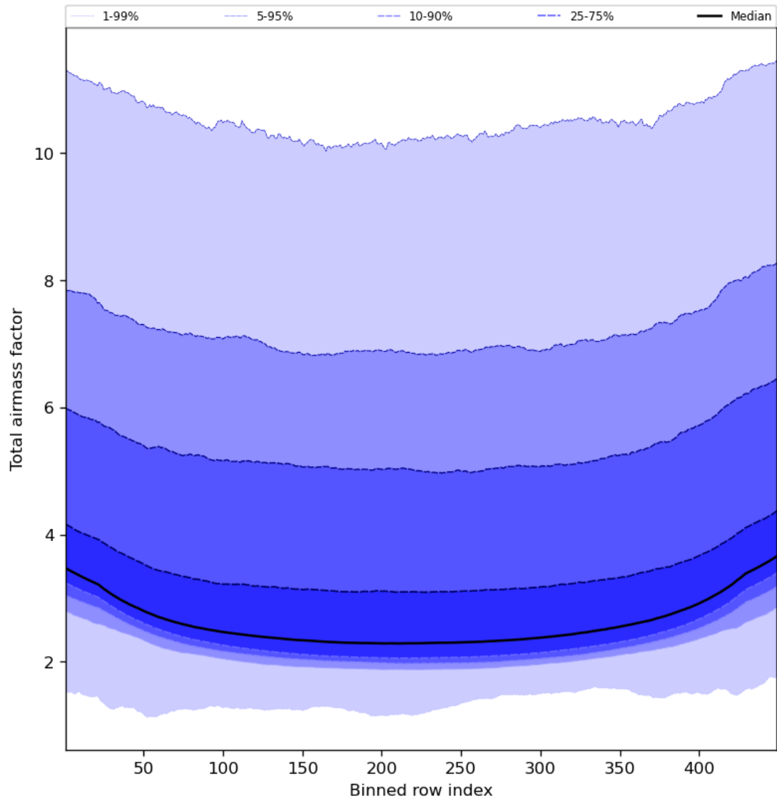
Figure 49: Along track statistics of “Total airmass factor” for 2024-01-17 to 2024-01-19
