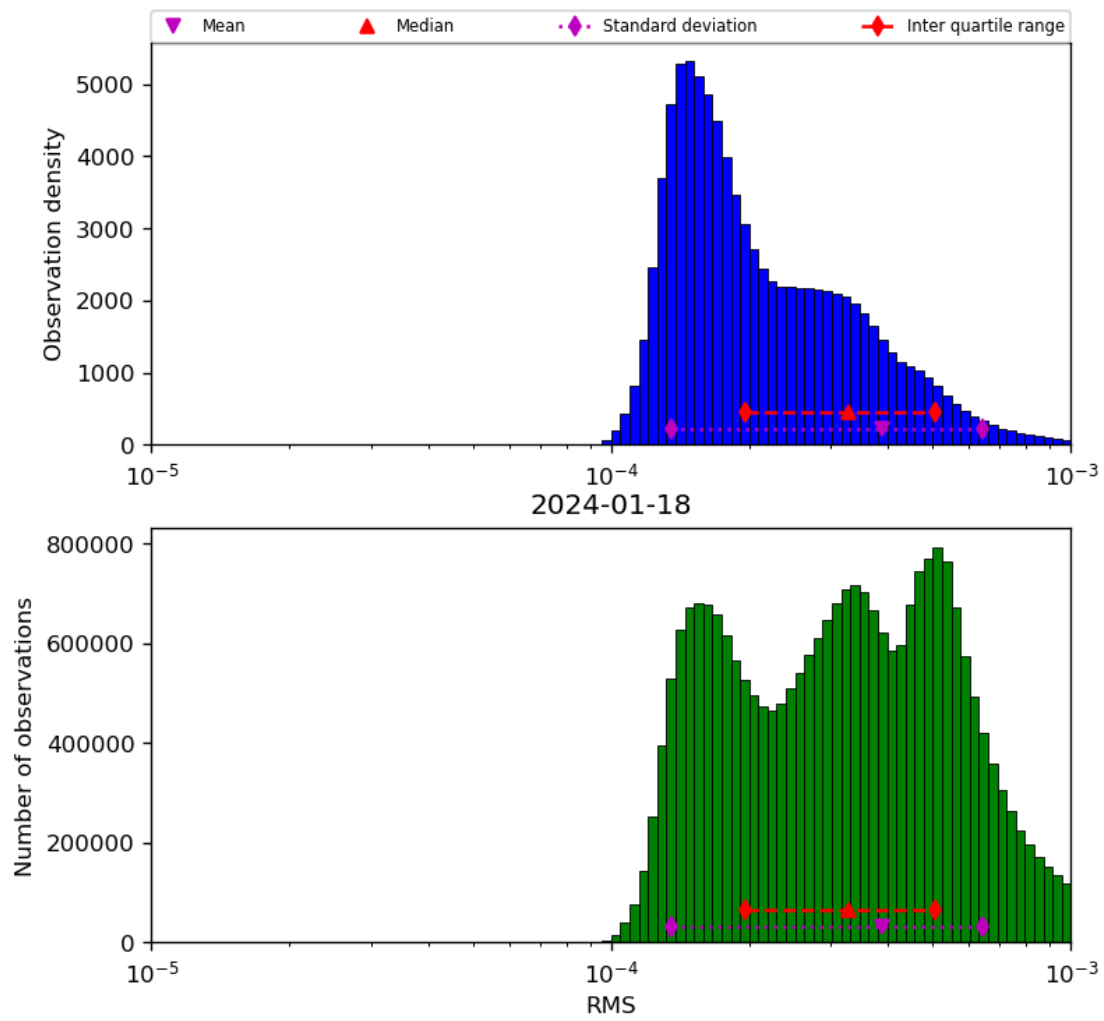
Figure 43: Histogram of “RMS” for 2024-01-17 to 2024-01-19
