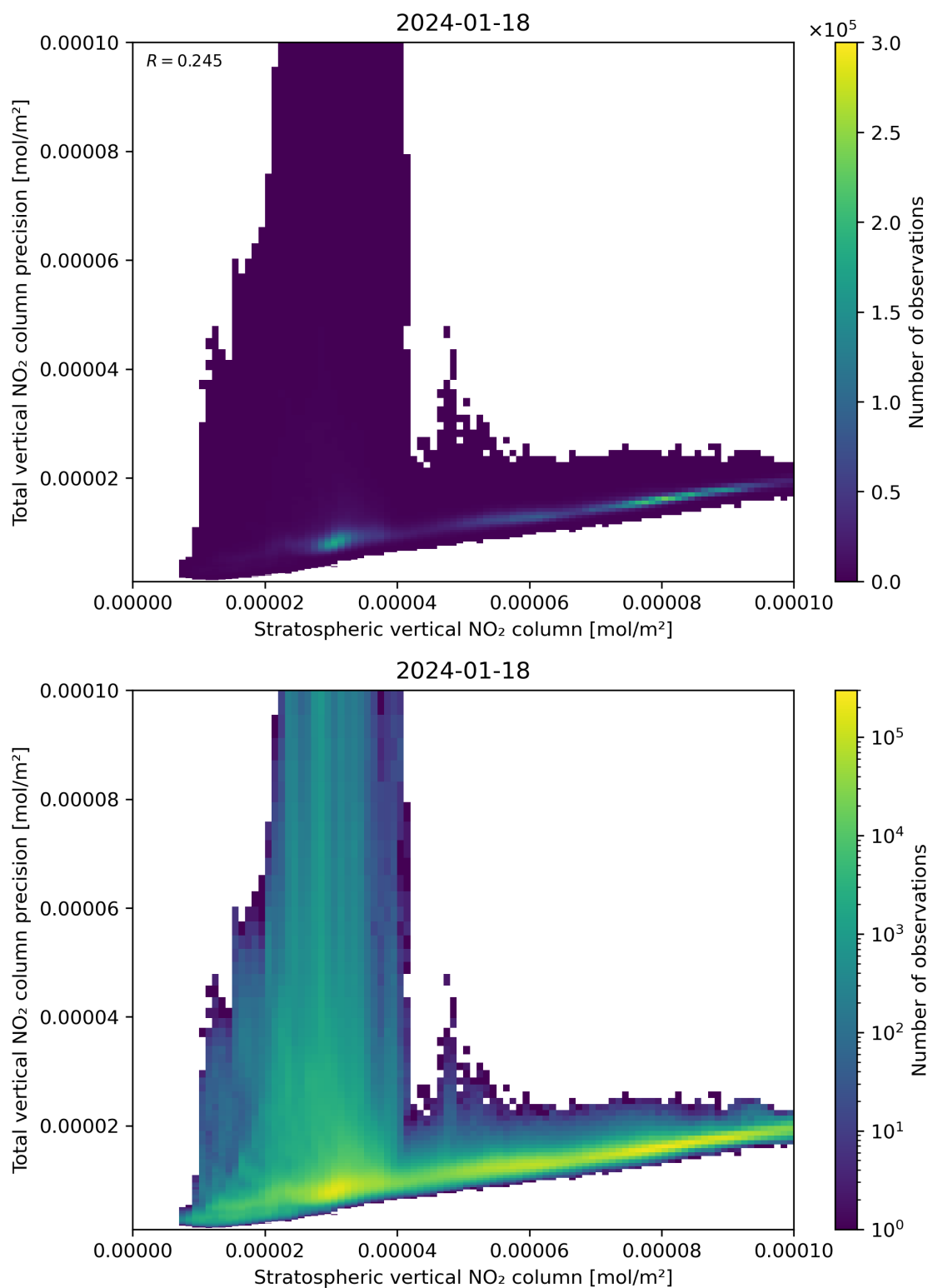
Figure 101: Scatter density plot of “Stratospheric vertical NO 2 column” against “Total vertical NO 2 column precision” for 2024-01-17 to 2024-01-19.
