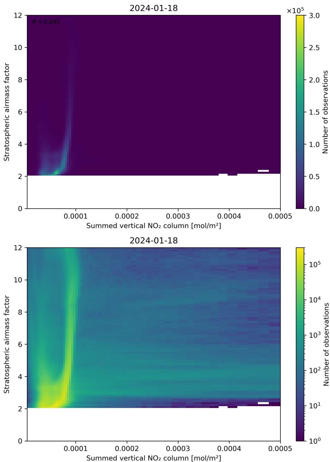
Figure 103: Scatter density plot of “Summed vertical NO 2 column” against “Stratospheric airmass factor” for 2024-01-17 to 2024-01-19.
