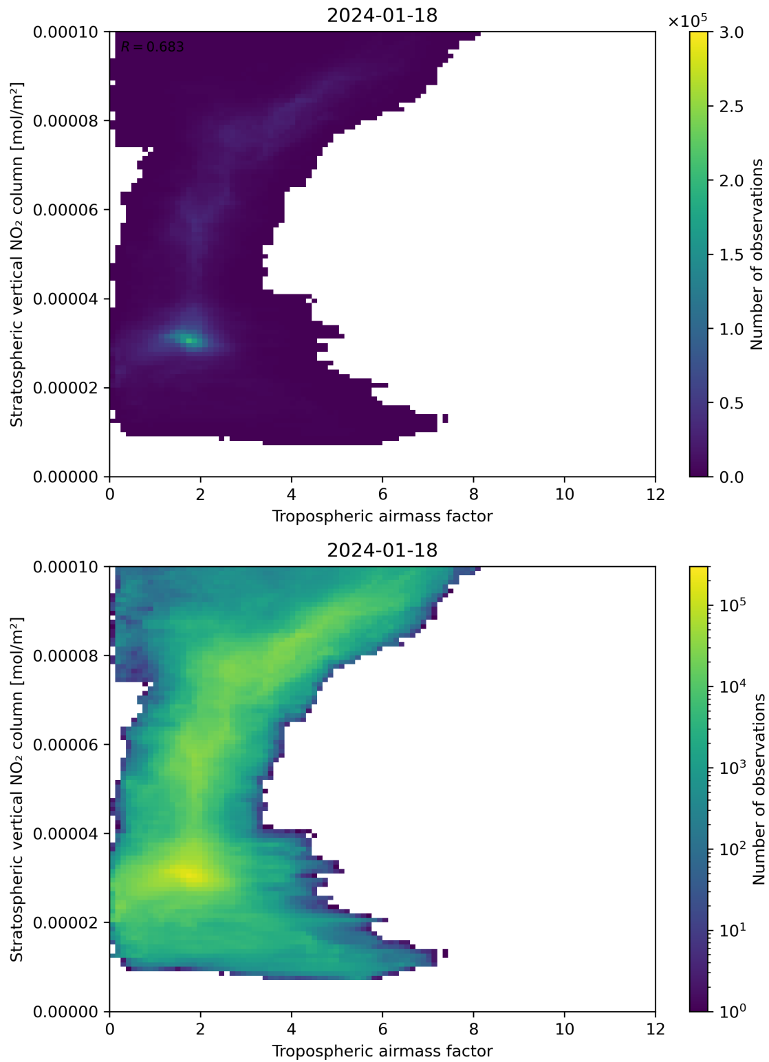
Figure 74: Scatter density plot of “Tropospheric air mass factor” against “Stratospheric vertical NO 2 column” for 2024-01-17 to 2024-01-19.
