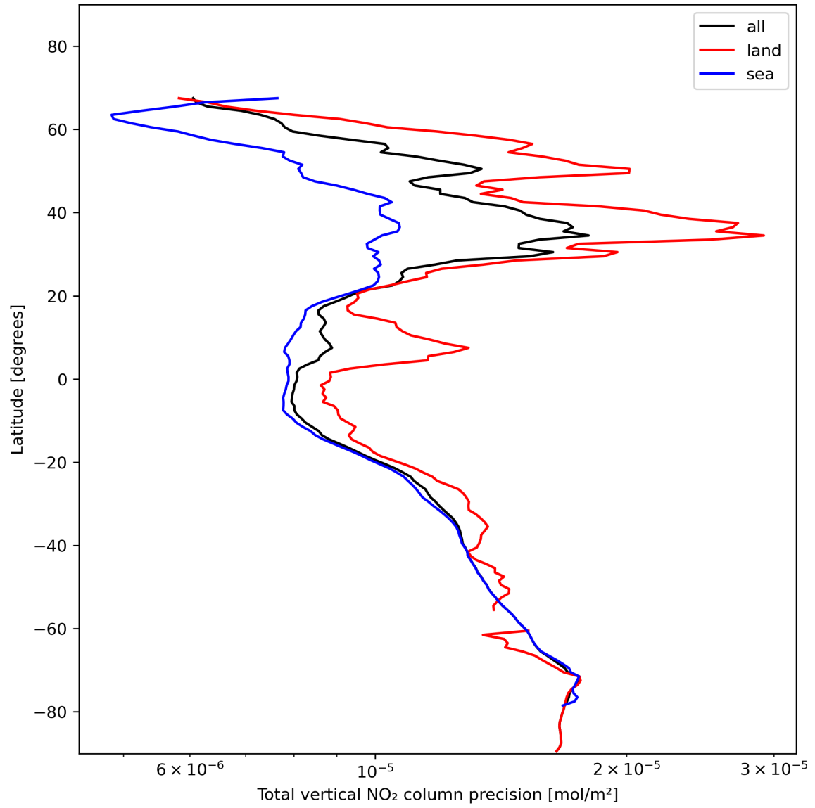
Figure 22: Zonal average of “Total vertical NO 2 column precision” for 2024-01-17 to 2024-01-19.
