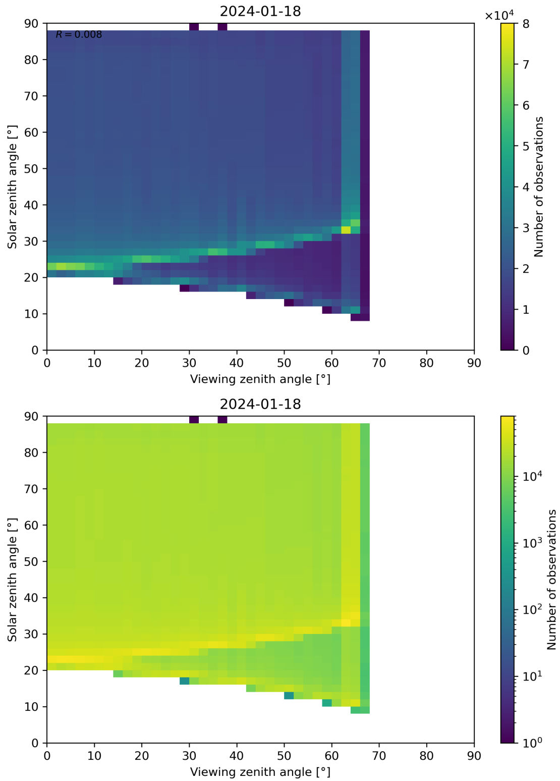
Figure 172: Scatter density plot of “Viewing zenith angle” against “Solar zenith angle” for 2024-01-17 to 2024-01-19.
