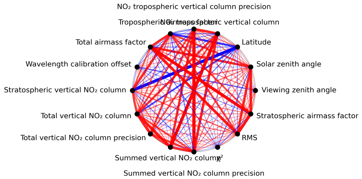
Figure 1: Map of correlation graph for 2024-01-17 to 2024-01-19.
