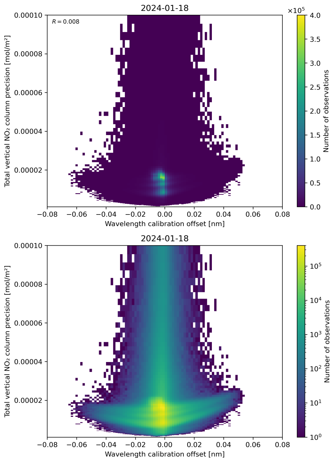
Figure 180: Scatter density plot of “Wavelength calibration offset” against “Total vertical NO 2 column precision” for 2024-01-17 to 2024-01-19.
