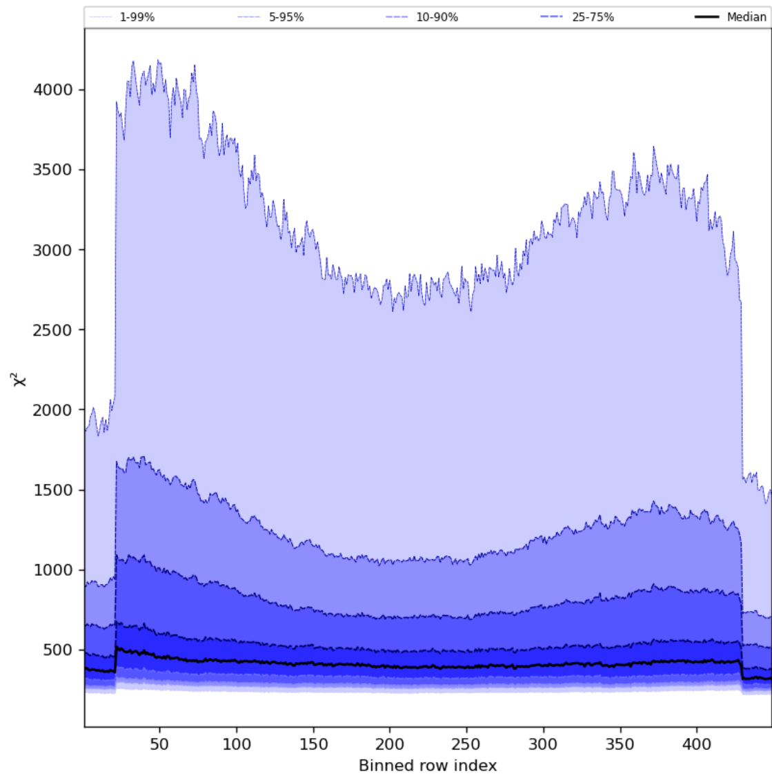
Figure 59: Along track statistics of “ \chi^2 ” for 2024-01-17 to 2024-01-19
