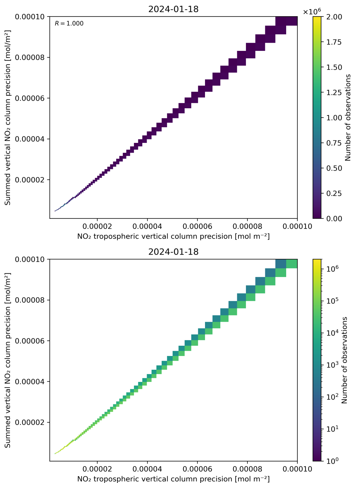
Figure 137: Scatter density plot of “NO 2 tropospheric vertical column precision” against “Summed vertical NO 2 column precision” for 2024-01-17 to 2024-01-19.
