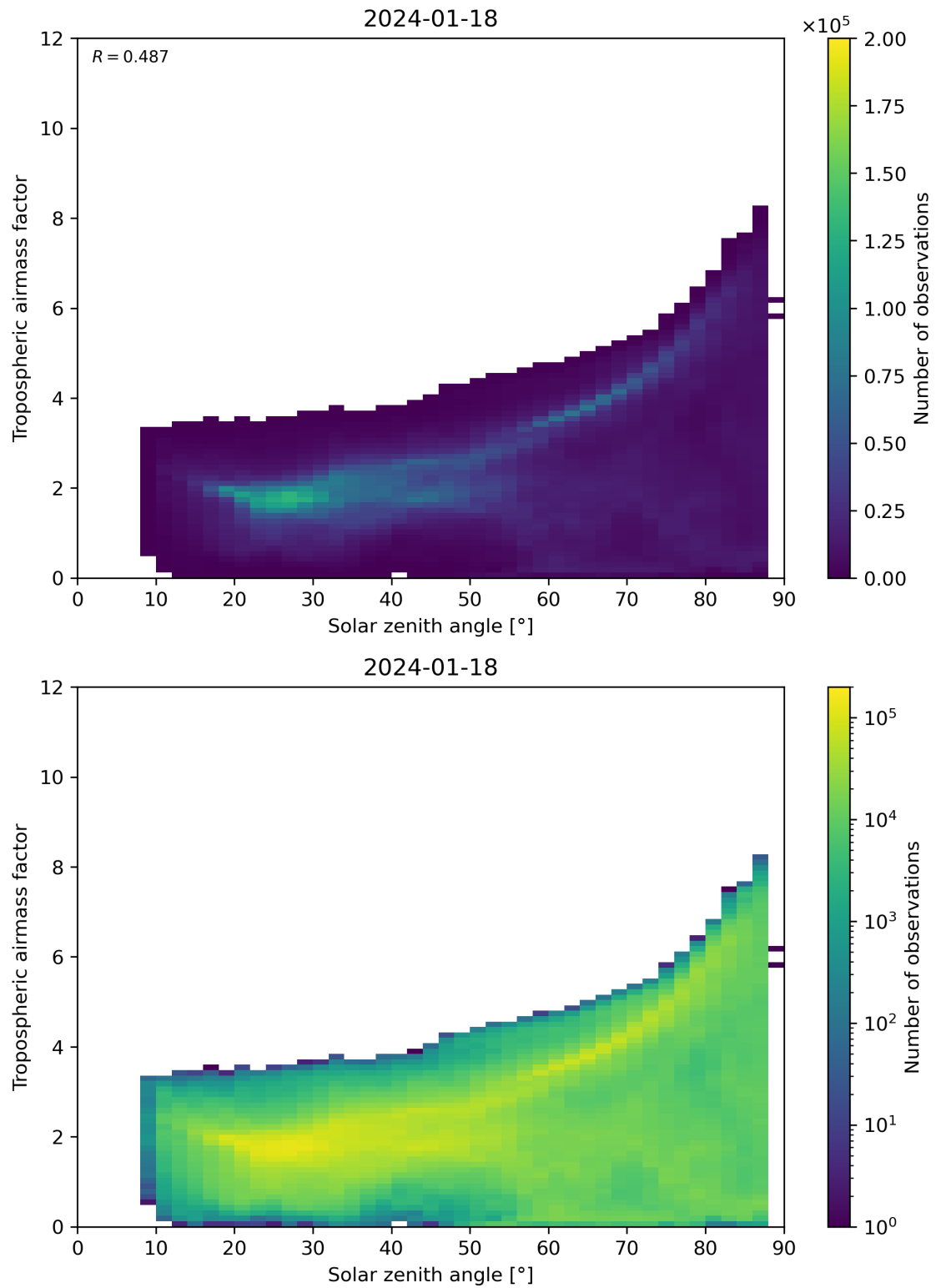
Figure 147: Scatter density plot of “Solar zenith angle” against “Tropospheric airmass factor” for 2024-01-17 to 2024-01-19.
