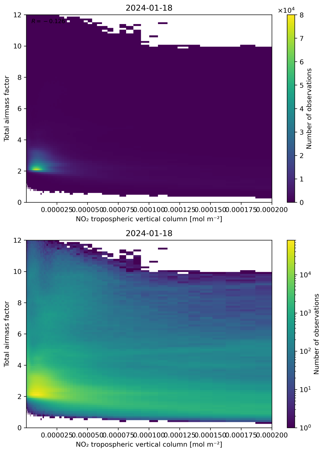
Figure 122: Scatter density plot of “NO 2 tropospheric vertical column” against “Total air mass factor” for 2024-01-17 to 2024-01-19.
