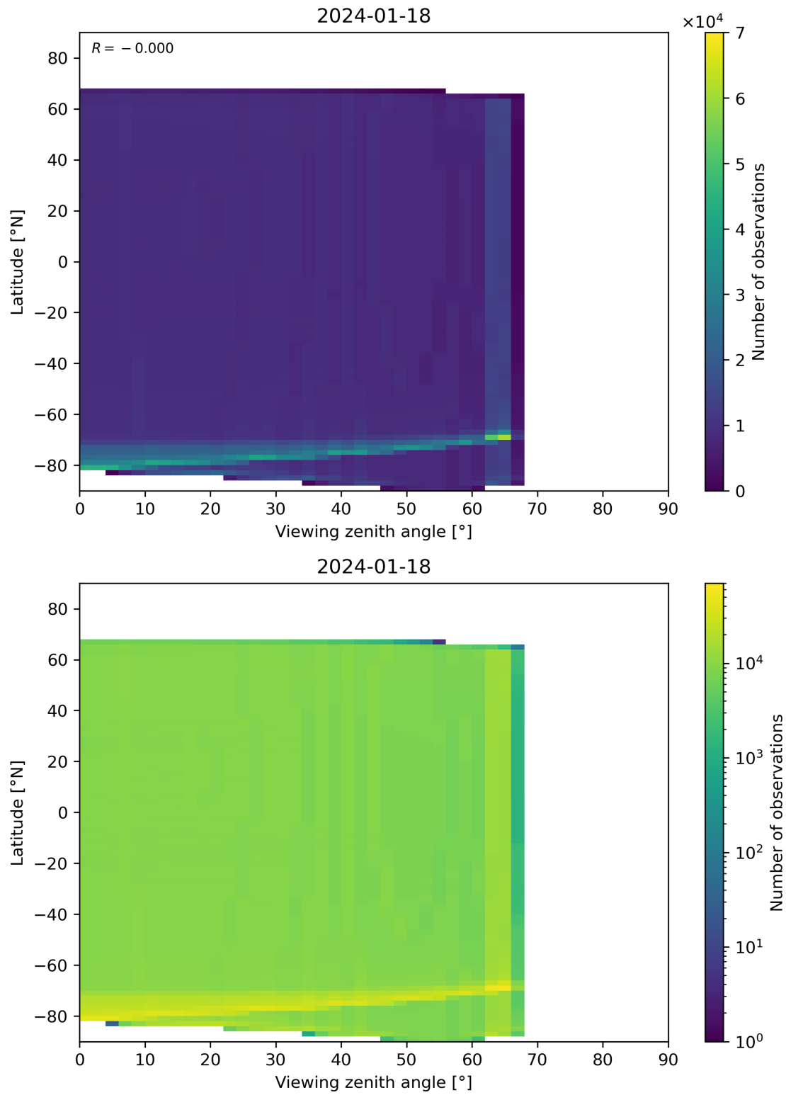
Figure 163: Scatter density plot of “Viewing zenith angle” against “Latitude” for 2024-01-17 to 2024-01-19.
