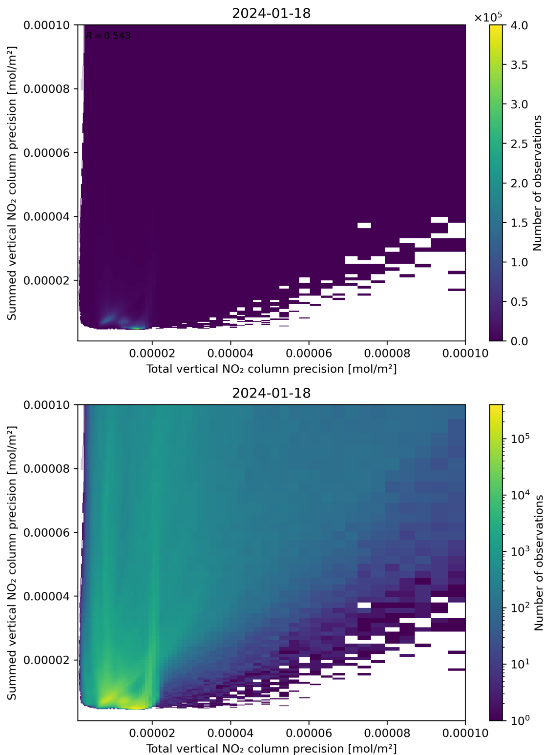
Figure 118: Scatter density plot of “Total vertical NO 2 column precision” against “Summed vertical NO 2 column precision” for 2024-01-17 to 2024-01-19.
