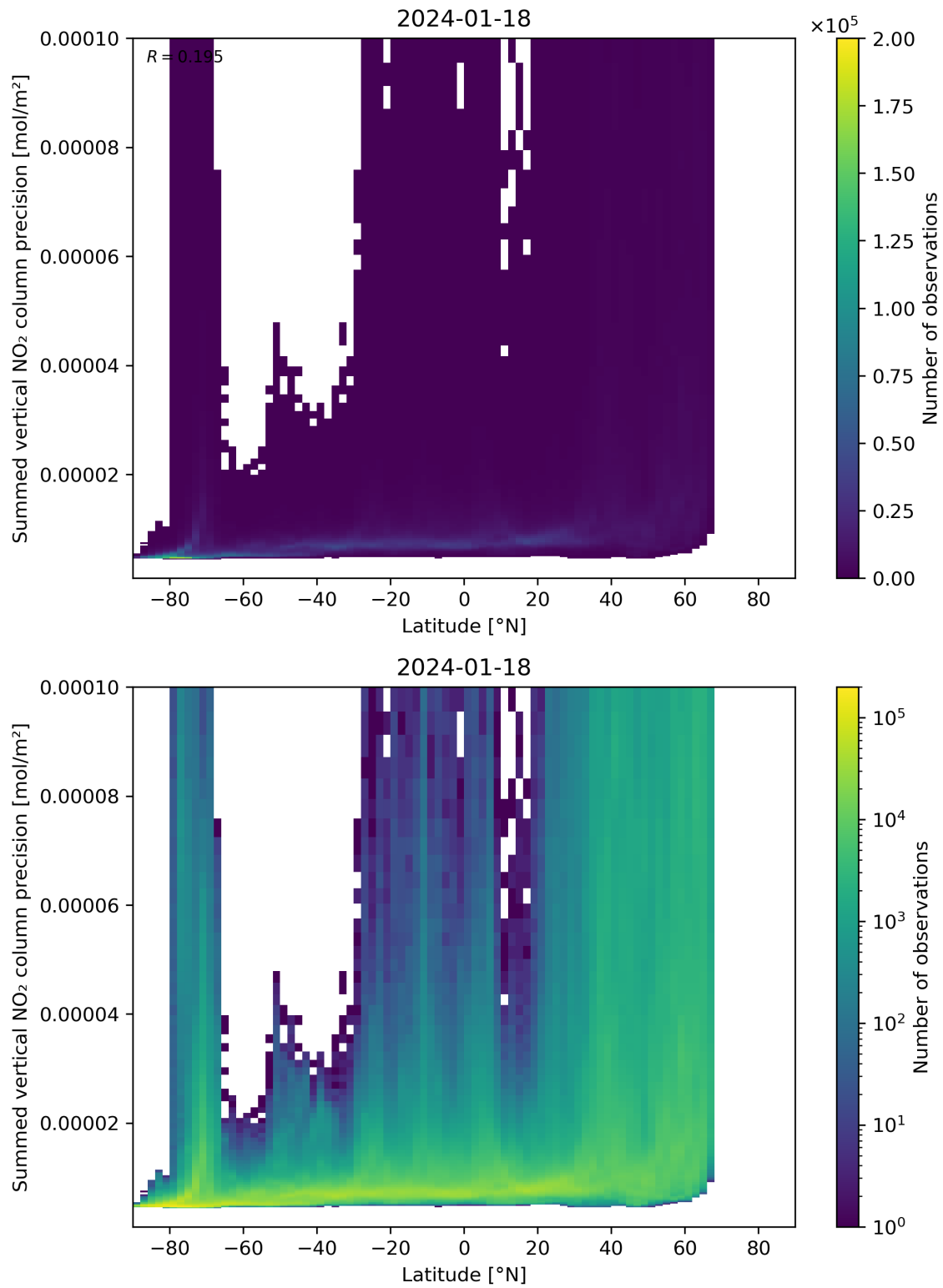
Figure 89: Scatter density plot of “Latitude” against “Summed vertical NO 2 column precision” for 2024-01-17 to 2024-01-19.
