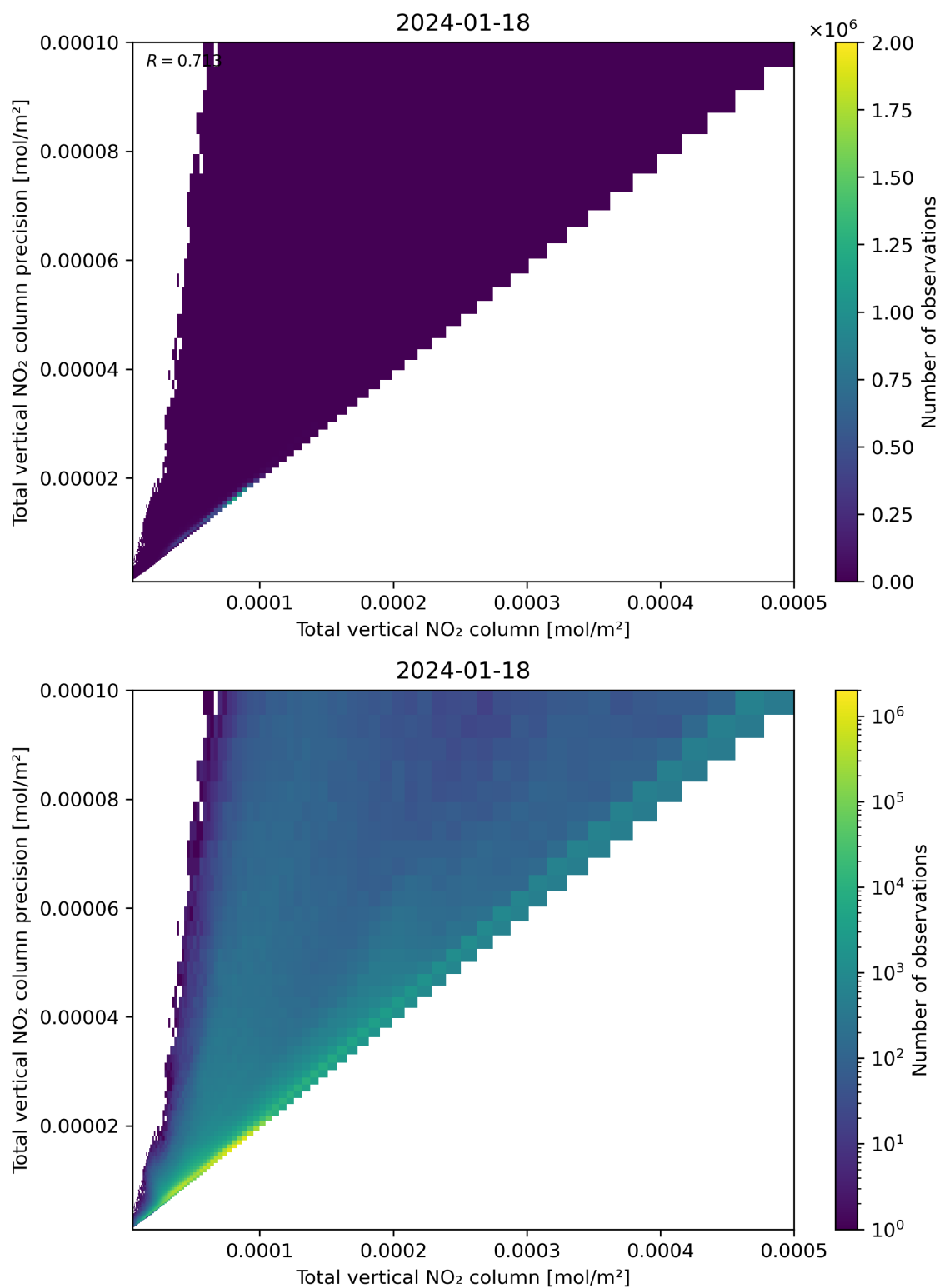
Figure 114: Scatter density plot of “Total vertical NO 2 column” against “Total vertical NO 2 column precision” for 2024-01-17 to 2024-01-19.
