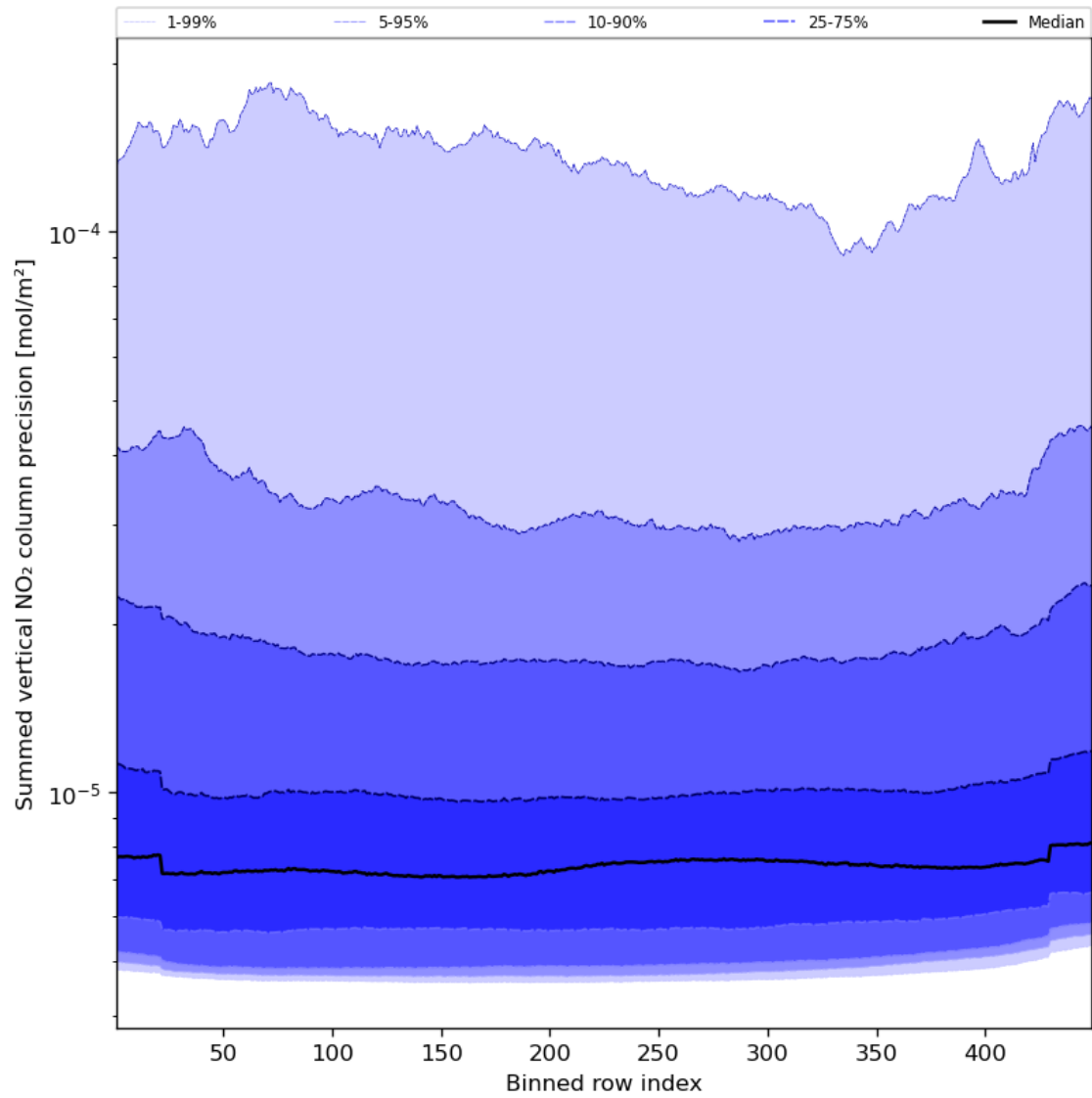
Figure 58: Along track statistics of “Summed vertical NO 2 column precision” for 2024-01-17 to 2024-01-19
