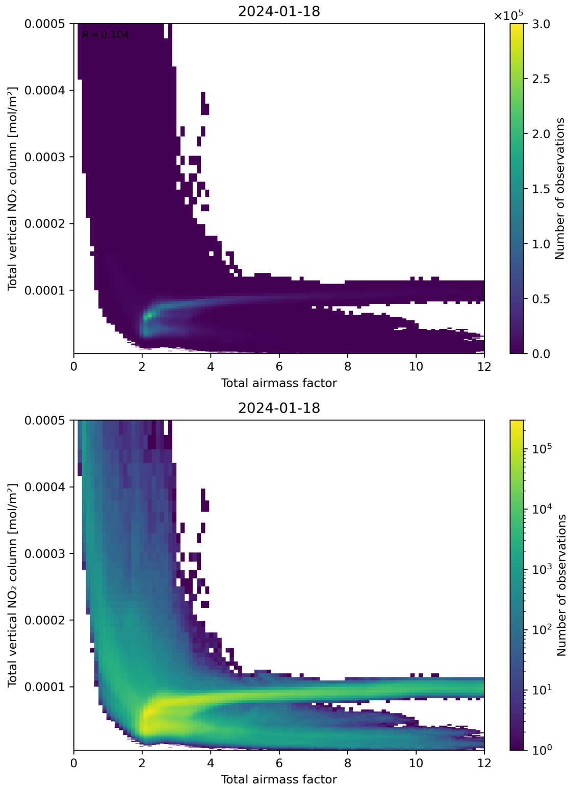
Figure 67: Scatter density plot of “Total air mass factor” against “Total vertical NO 2 column” for 2024-01-17 to 2024-01-19.
