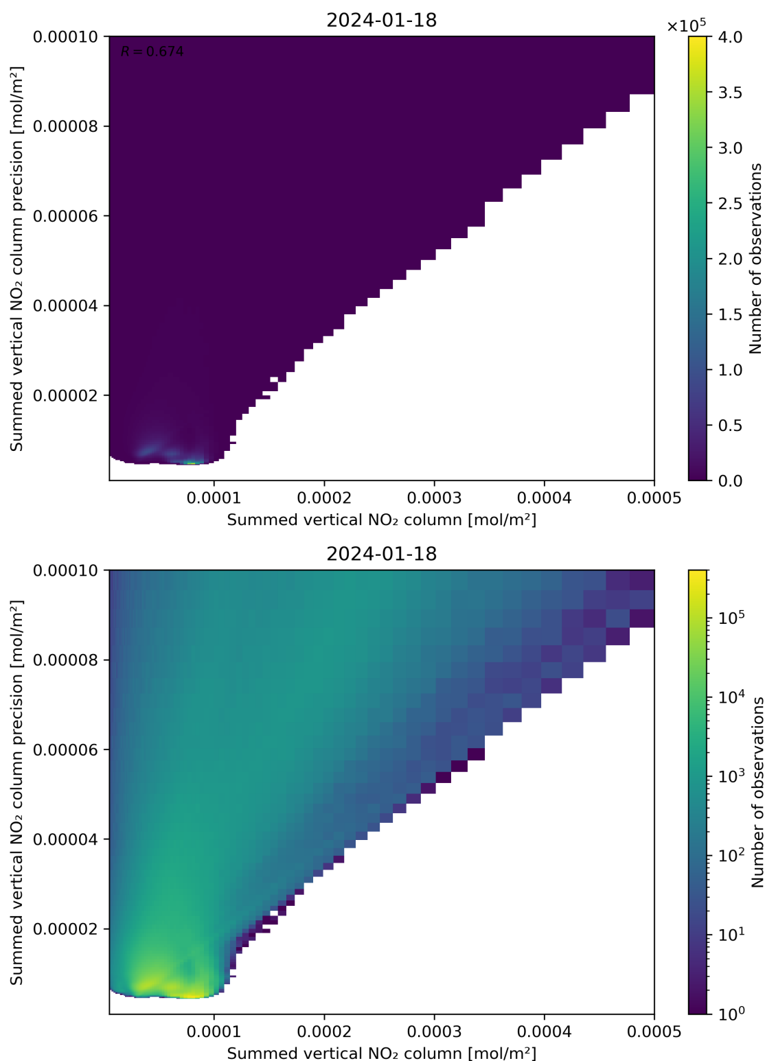
Figure 105: Scatter density plot of “Summed vertical NO 2 column” against “Summed vertical NO 2 column precision” for 2024-01-17 to 2024-01-19.
