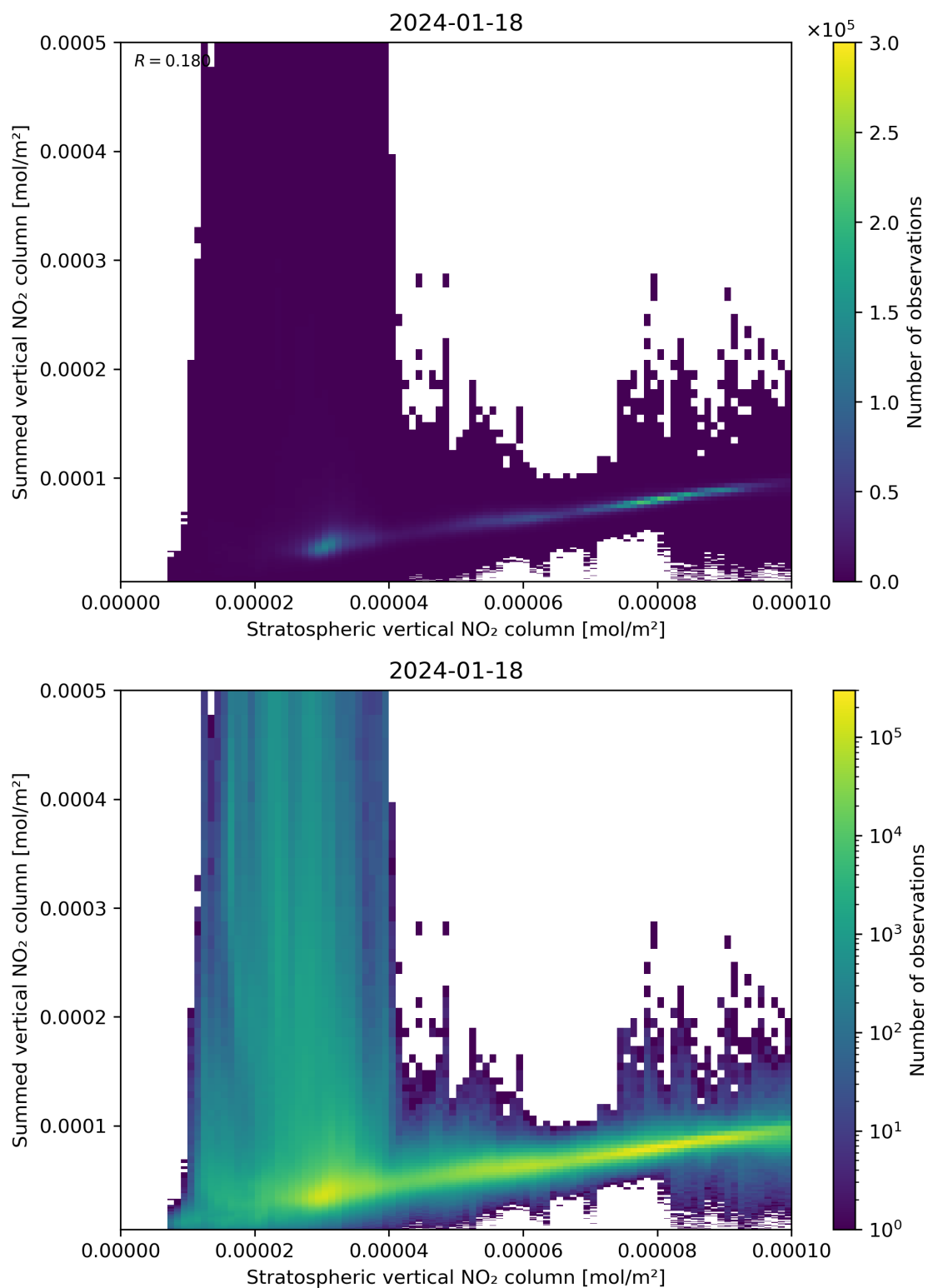
Figure 98: Scatter density plot of “Stratospheric vertical NO 2 column” against “Summed vertical NO 2 column” for 2024-01-17 to 2024-01-19.
