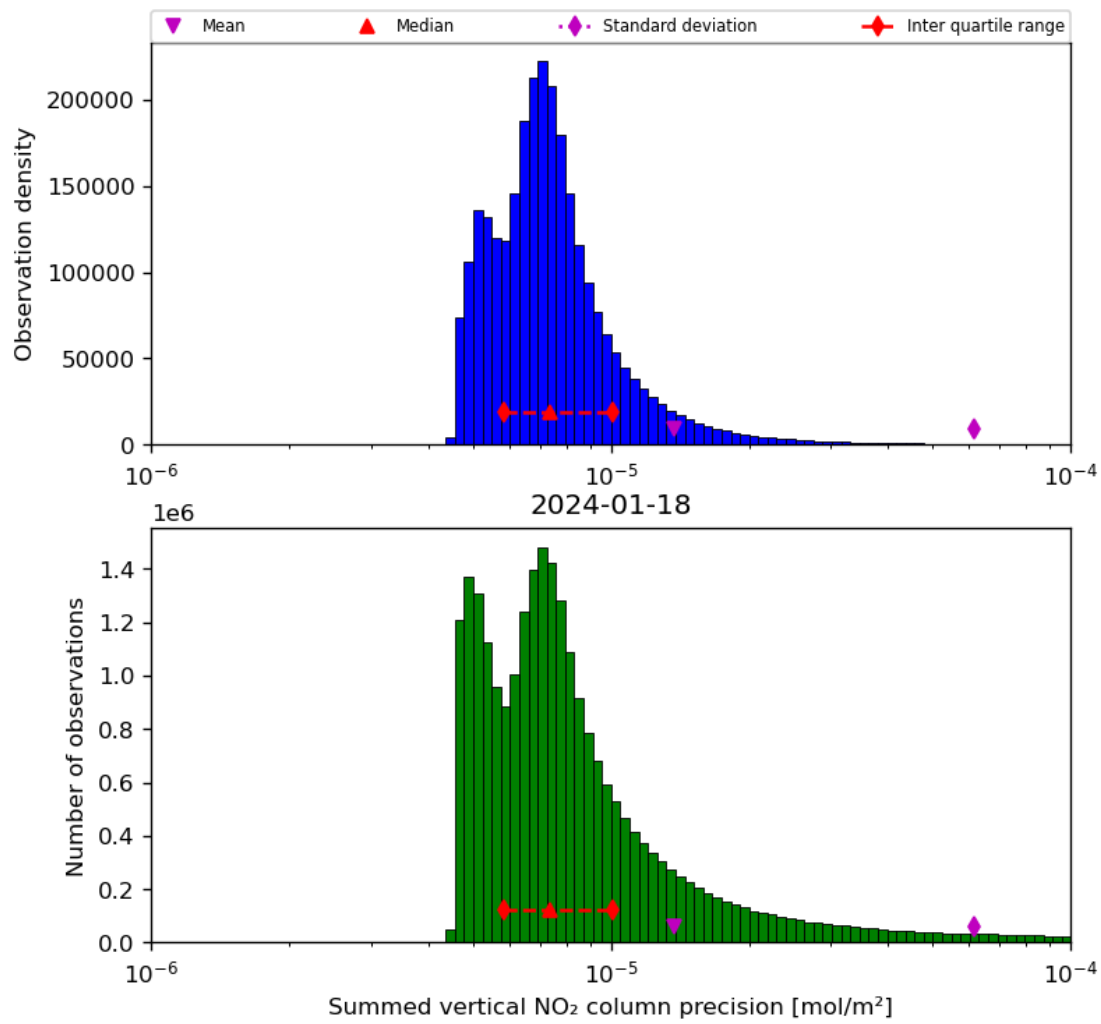
Figure 41: Histogram of “Summed vertical NO 2 column precision” for 2024-01-17 to 2024-01-19
