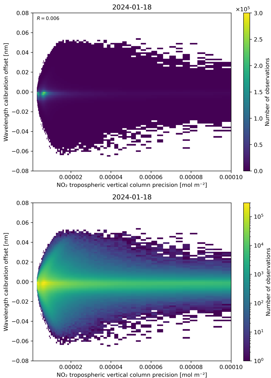
Figure 141: Scatter density plot of “NO 2 tropospheric vertical column precision” against “Wavelength calibration offset” for 2024-01-17 to 2024-01-19.
