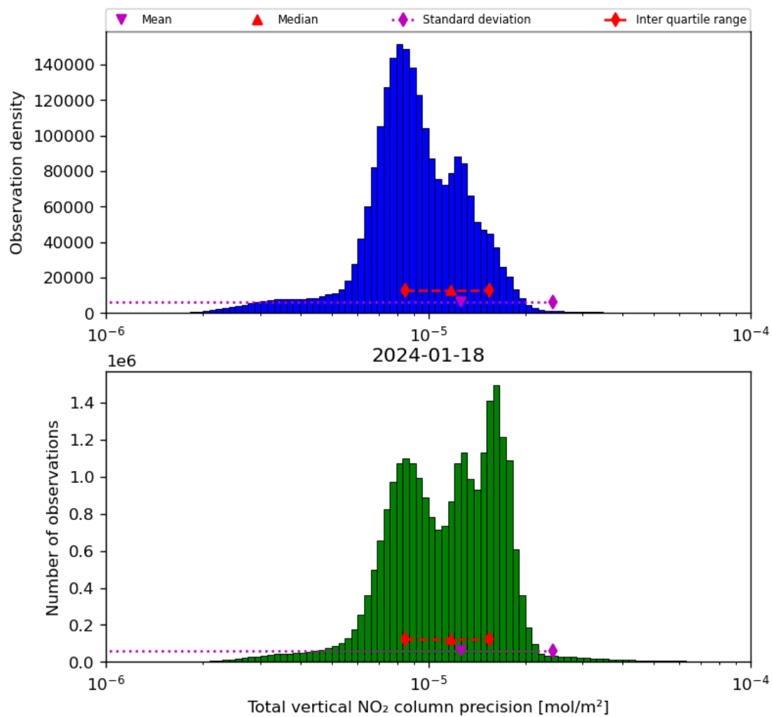
Figure 39: Histogram of “Total vertical NO 2 column precision” for 2024-01-17 to 2024-01-19
