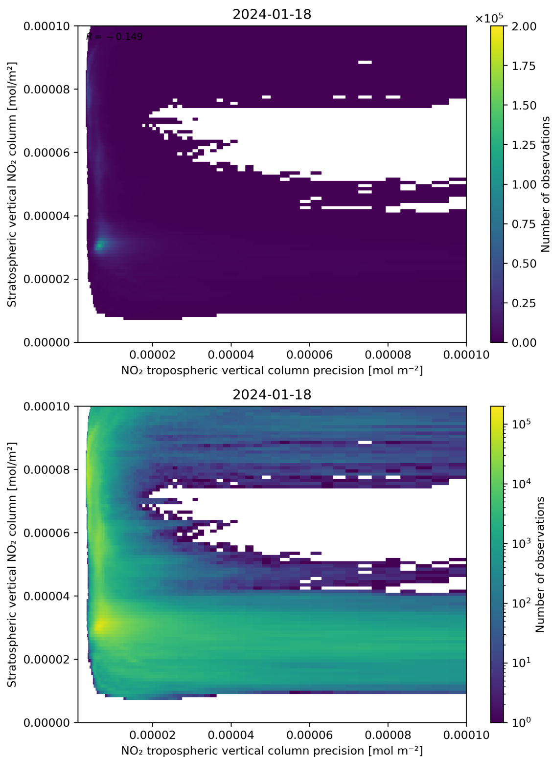
Figure 135: Scatter density plot of “NO 2 tropospheric vertical column precision” against “Stratospheric vertical NO 2 column” for 2024-01-17 to 2024-01-19.
