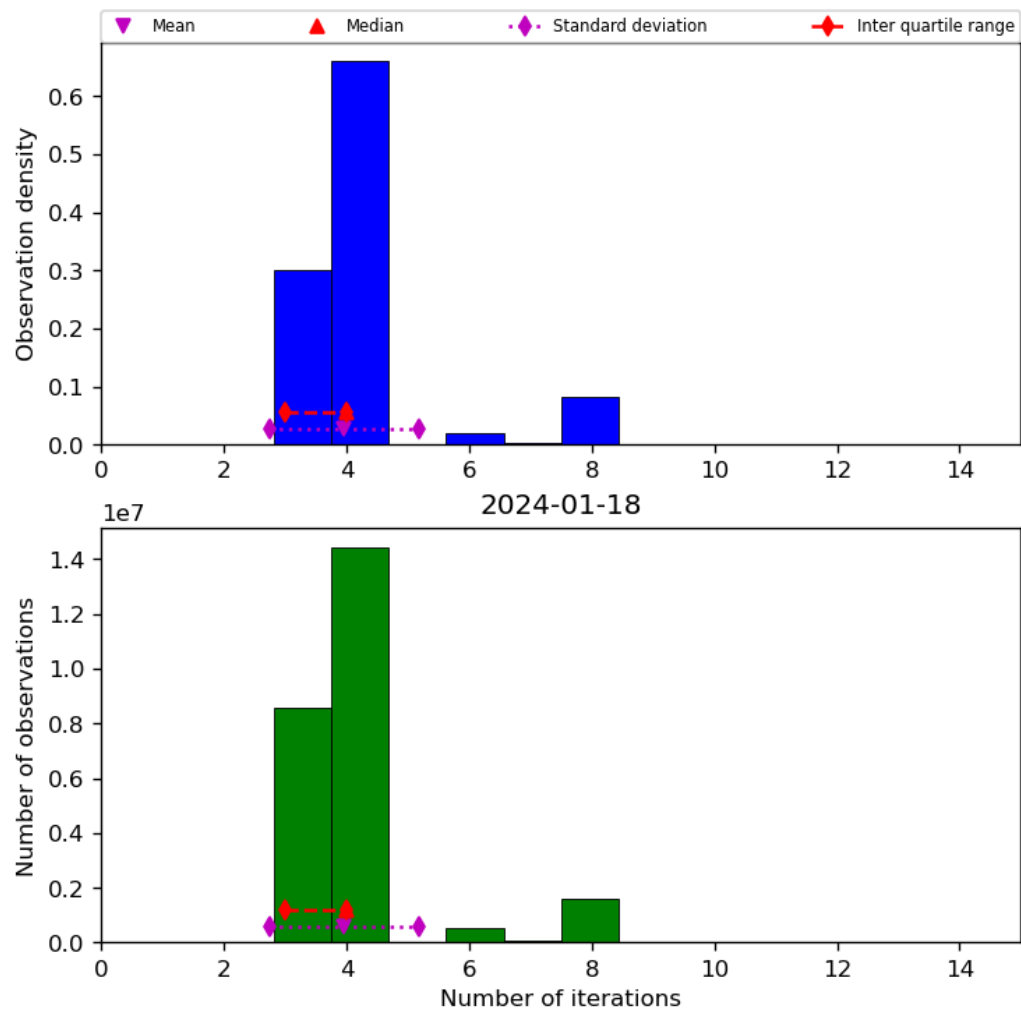
Figure 34: Histogram of “Number of iterations” for 2024-01-17 to 2024-01-19
