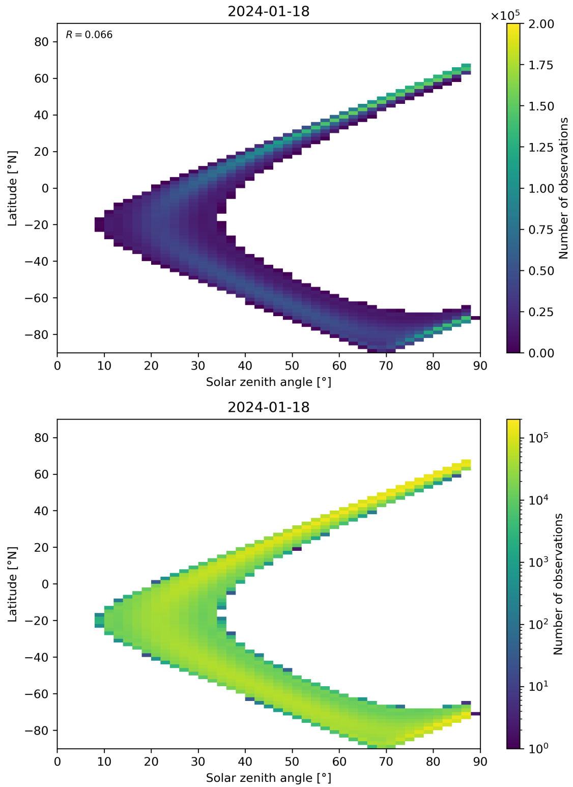
Figure 149: Scatter density plot of “Solar zenith angle” against “Latitude” for 2024-01-17 to 2024-01-19.
