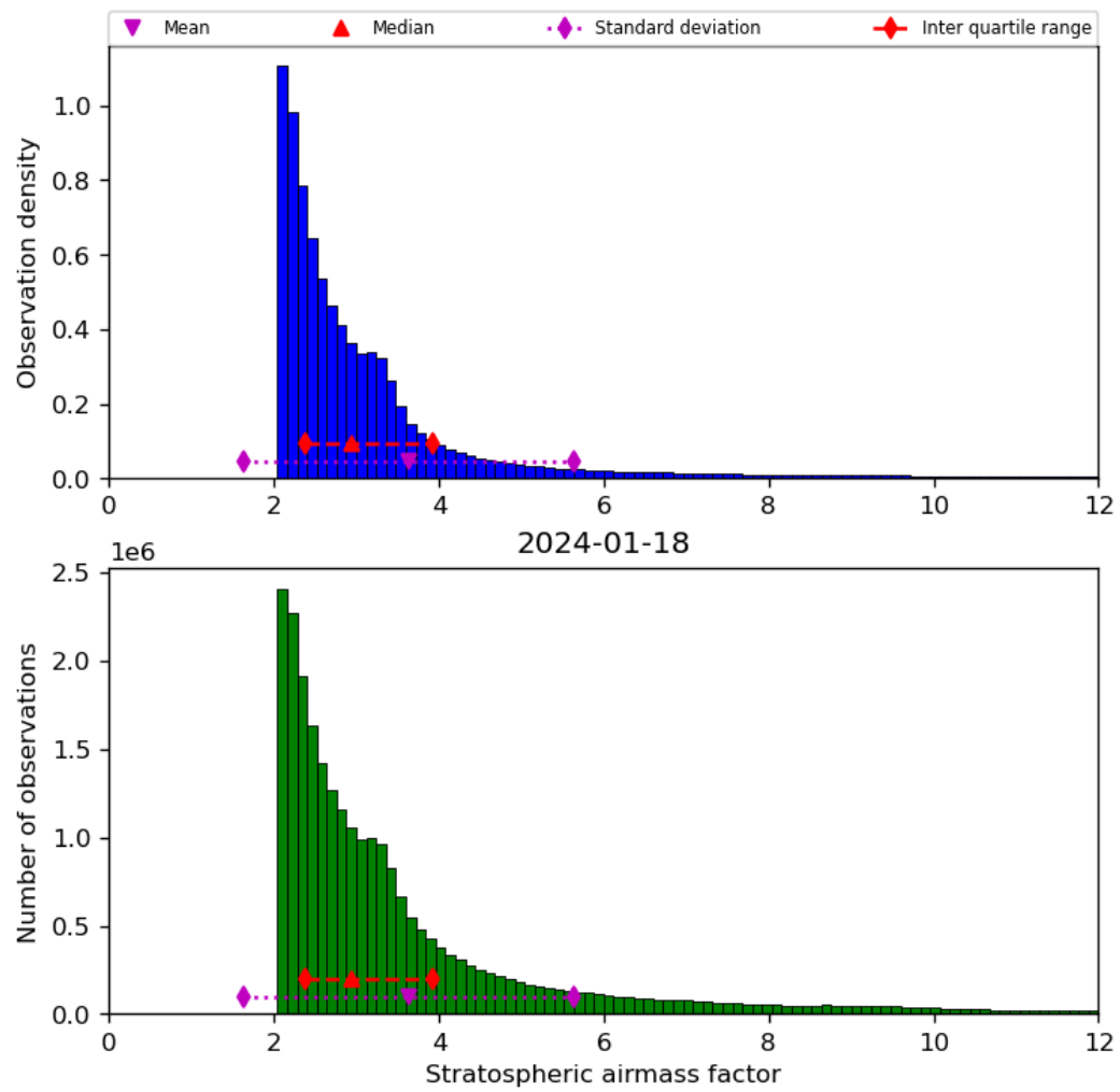
Figure 44: Histogram of “Stratospheric airmass factor” for 2024-01-17 to 2024-01-19
