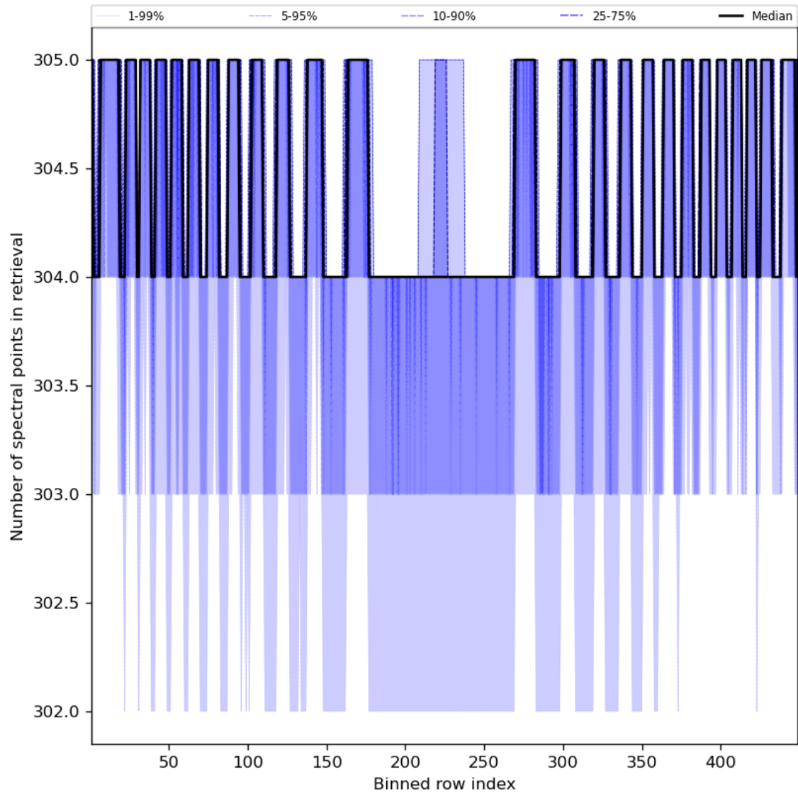
Figure 50: Along track statistics of “Number of spectral points in retrieval” for 2024-01-17 to 2024-01-19
