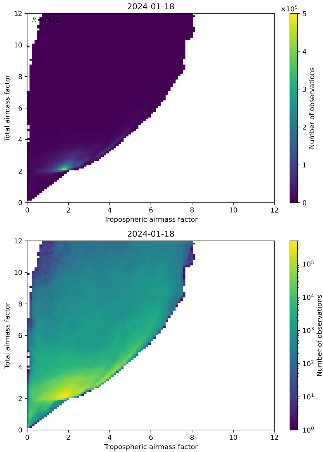
Figure 72: Scatter density plot of “Tropospheric airmass factor” against “Total airmass factor” for 2024-01-17 to 2024-01-19.
