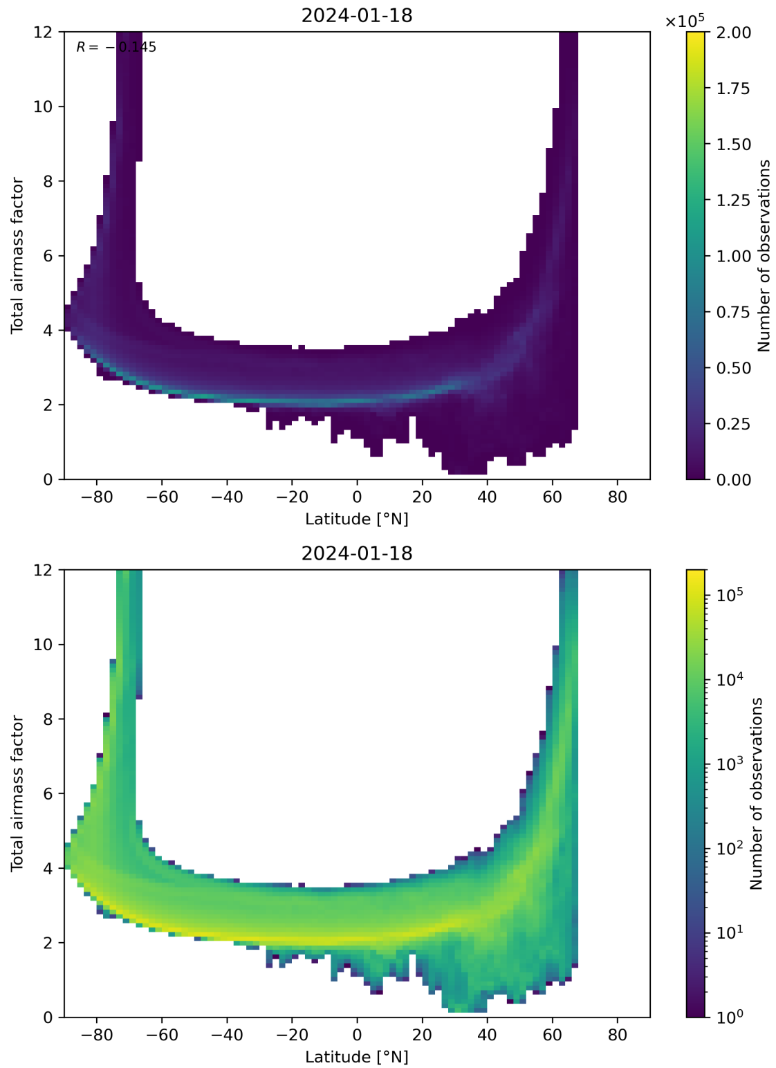
Figure 84: Scatter density plot of “Latitude” against “Total airmass factor” for 2024-01-17 to 2024-01-19.
