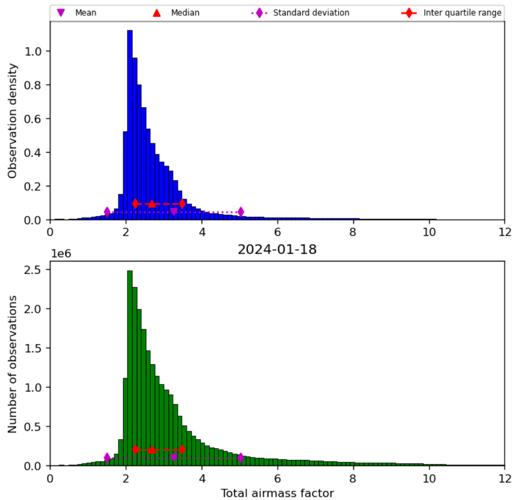
Figure 32: Histogram of “Total airmass factor” for 2024-01-17 to 2024-01-19
