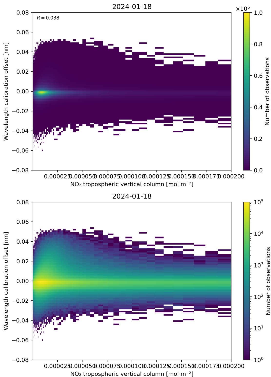
Figure 143: Scatter density plot of “NO 2 tropospheric vertical column” against “Wavelength calibration offset” for 2024-01-17 to 2024-01-19.
