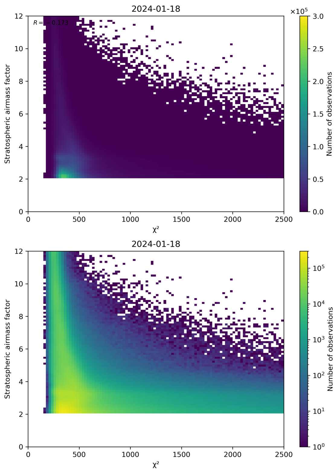
Figure 81: Scatter density plot of “ \chi^2 ” against “Stratospheric airmass factor” for 2024-01-17 to 2024-01-19.
