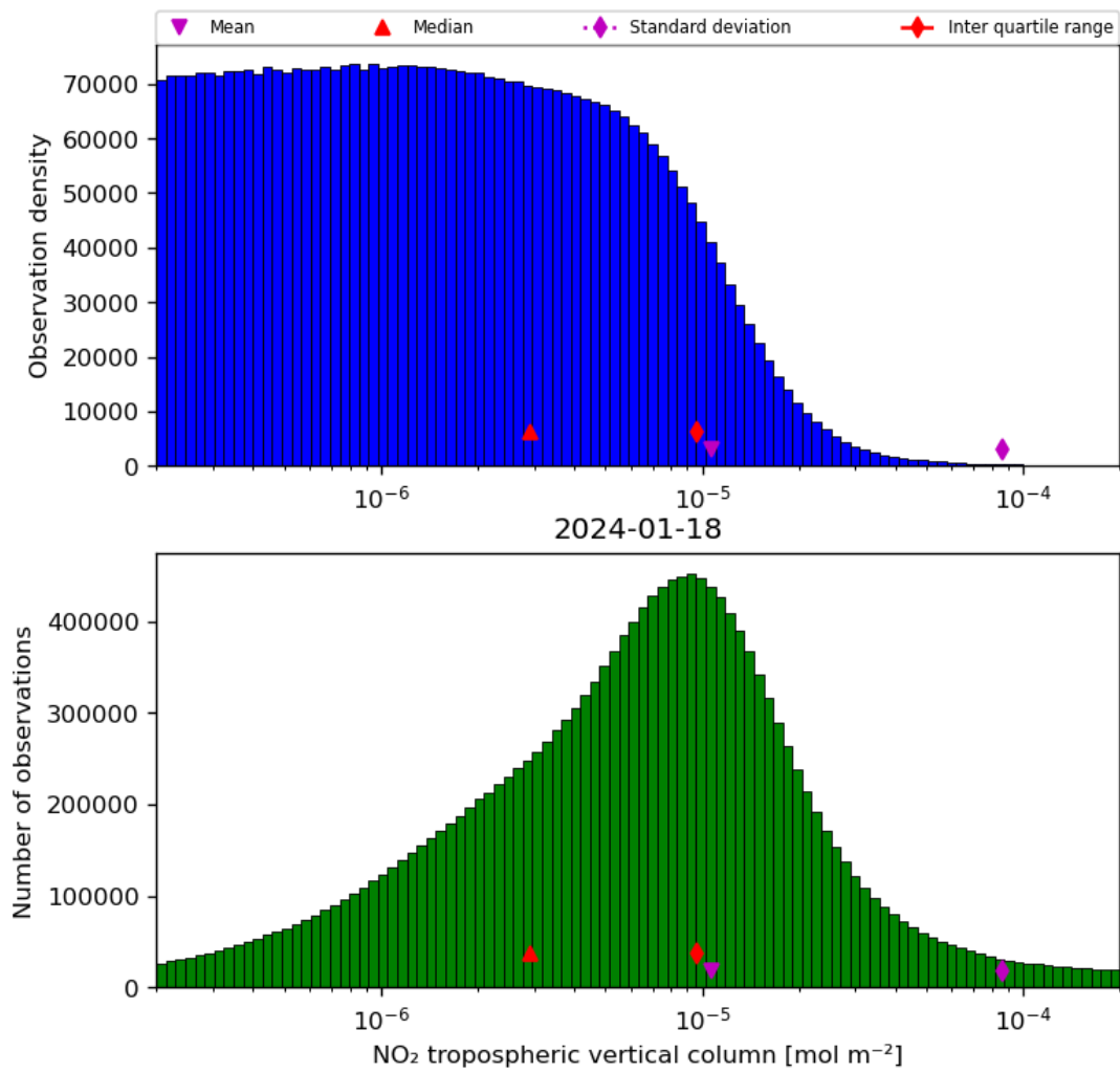
Figure 29: Histogram of “NO 2 tropospheric vertical column” for 2024-01-17 to 2024-01-19
