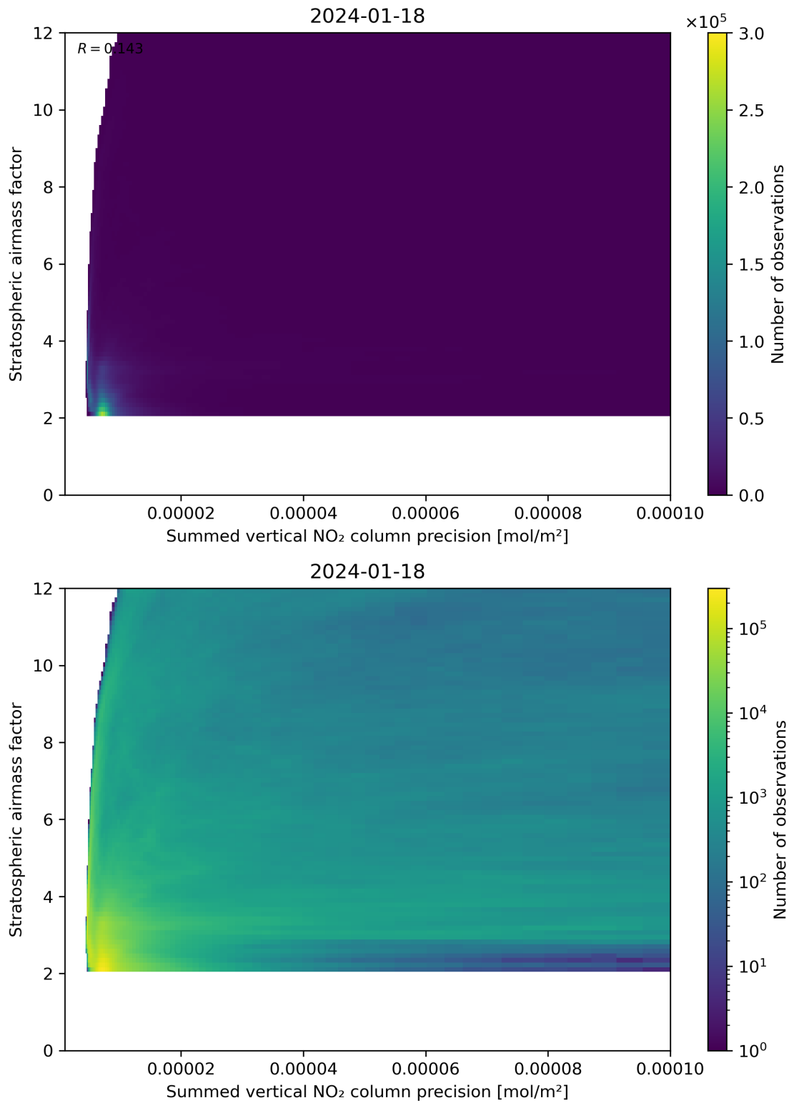
Figure 106: Scatter density plot of “Summed vertical NO 2 column precision” against “Stratospheric airmass factor” for 2024-01-17 to 2024-01-19.
