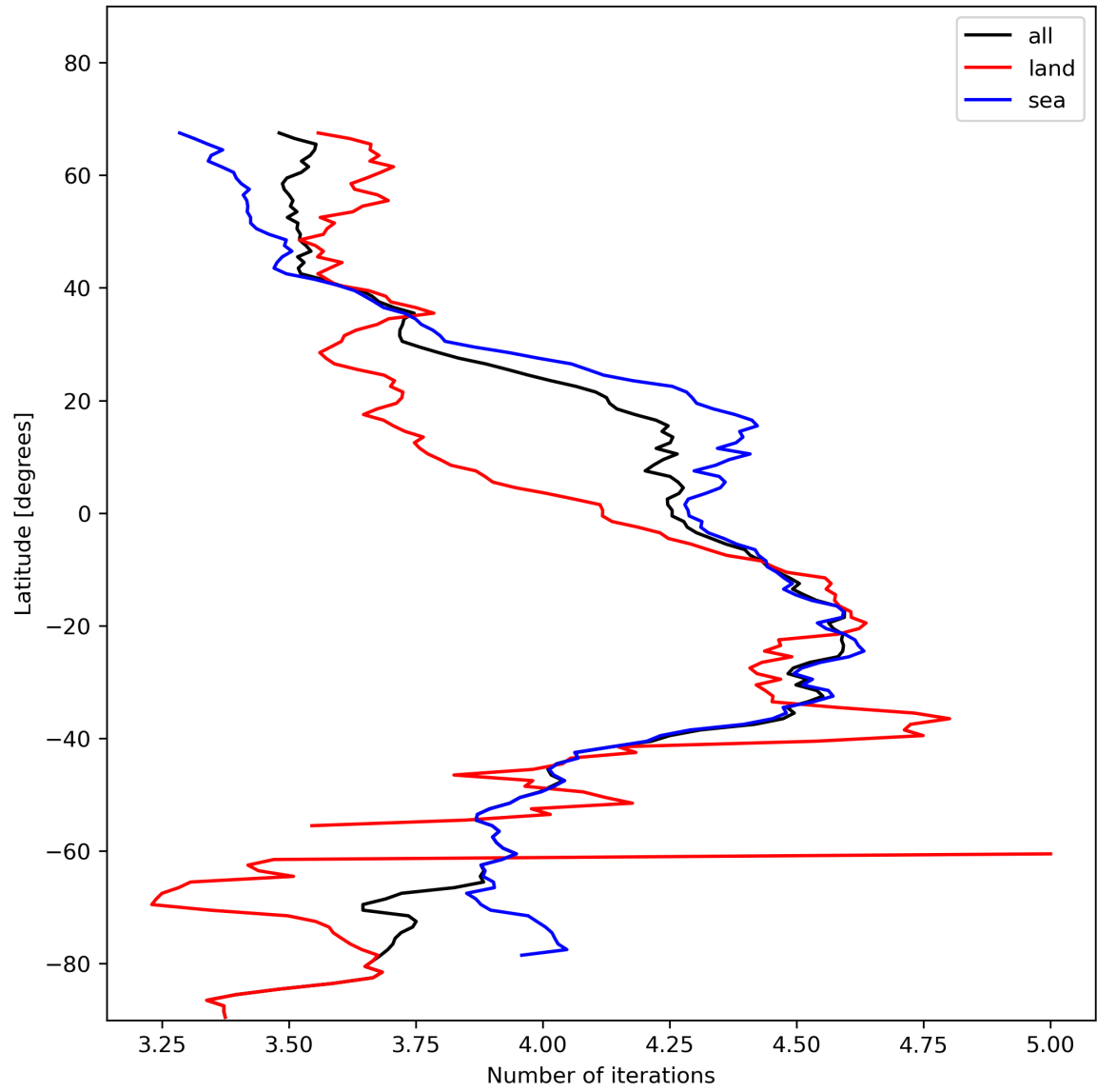
Figure 17: Zonal average of “Number of iterations” for 2024-01-17 to 2024-01-19.
