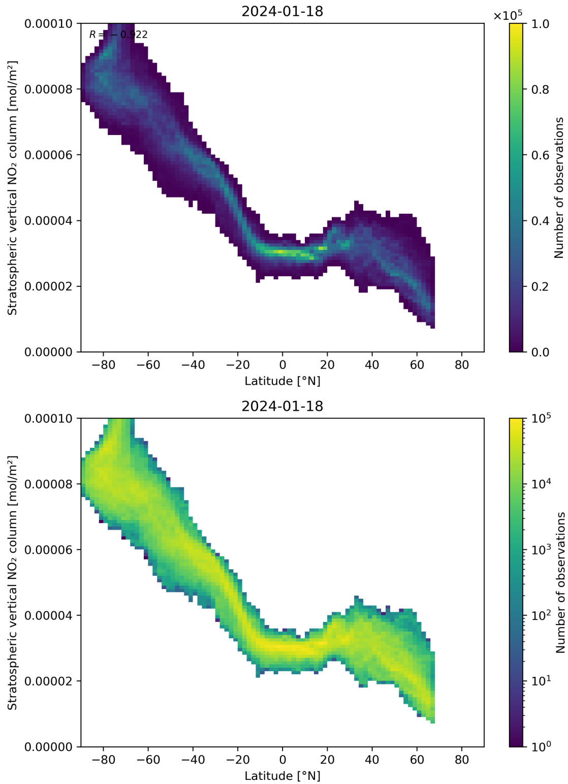
Figure 87: Scatter density plot of “Latitude” against “Stratospheric vertical NO 2 column” for 2024-01-17 to 2024-01-19.
