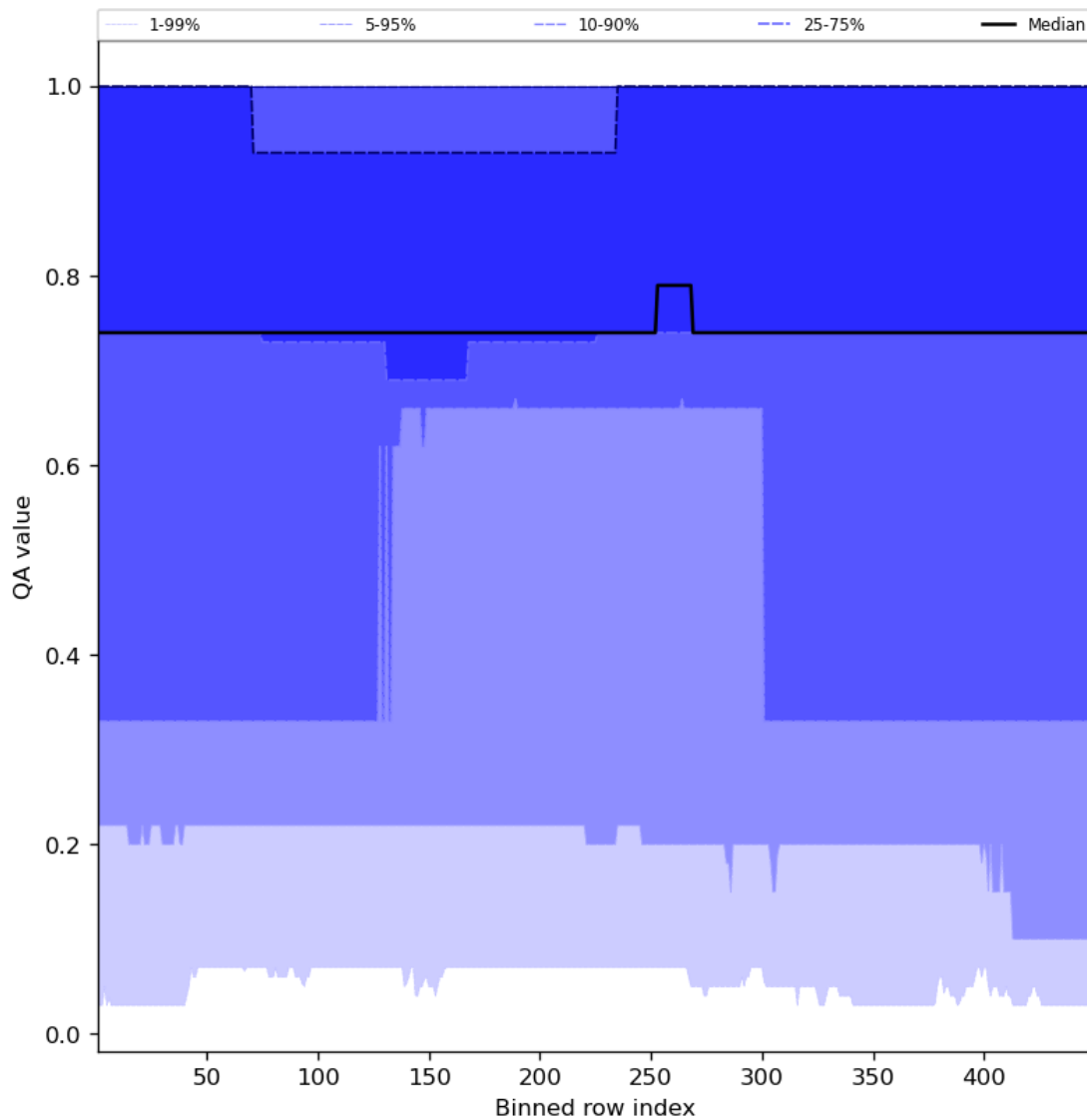
Figure 45: Along track statistics of “QA value” for 2024-01-17 to 2024-01-19
