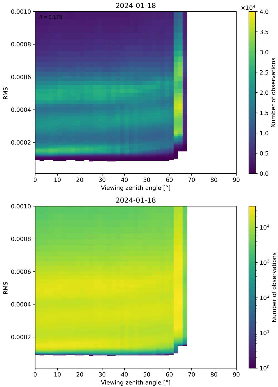
Figure 171: Scatter density plot of “Viewing zenith angle” against “RMS” for 2024-01-17 to 2024-01-19.
