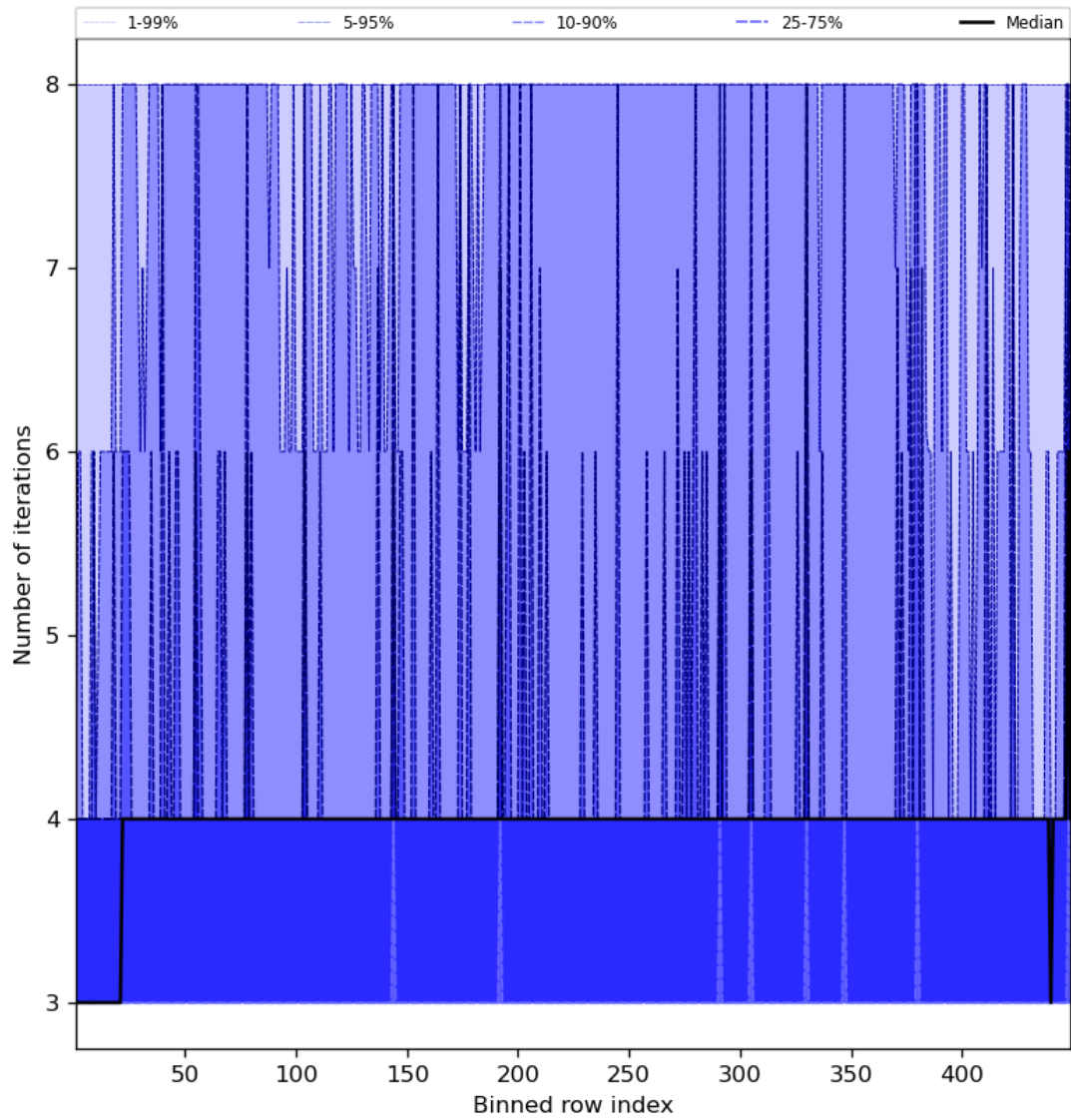
Figure 51: Along track statistics of “Number of iterations” for 2024-01-17 to 2024-01-19
