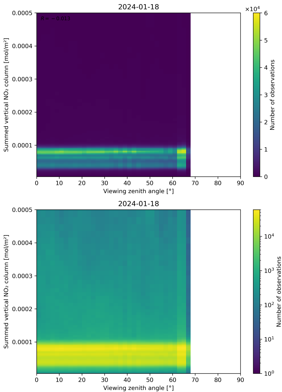
Figure 165: Scatter density plot of “Viewing zenith angle” against “Summed vertical NO 2 column” for 2024-01-17 to 2024-01-19.
