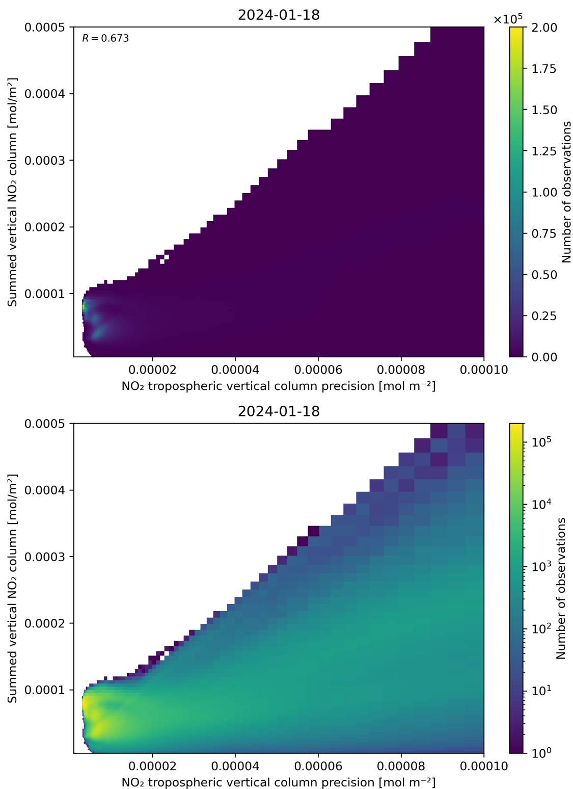
Figure 136: Scatter density plot of “NO 2 tropospheric vertical column precision” against “Summed vertical NO 2 column” for 2024-01-17 to 2024-01-19.
