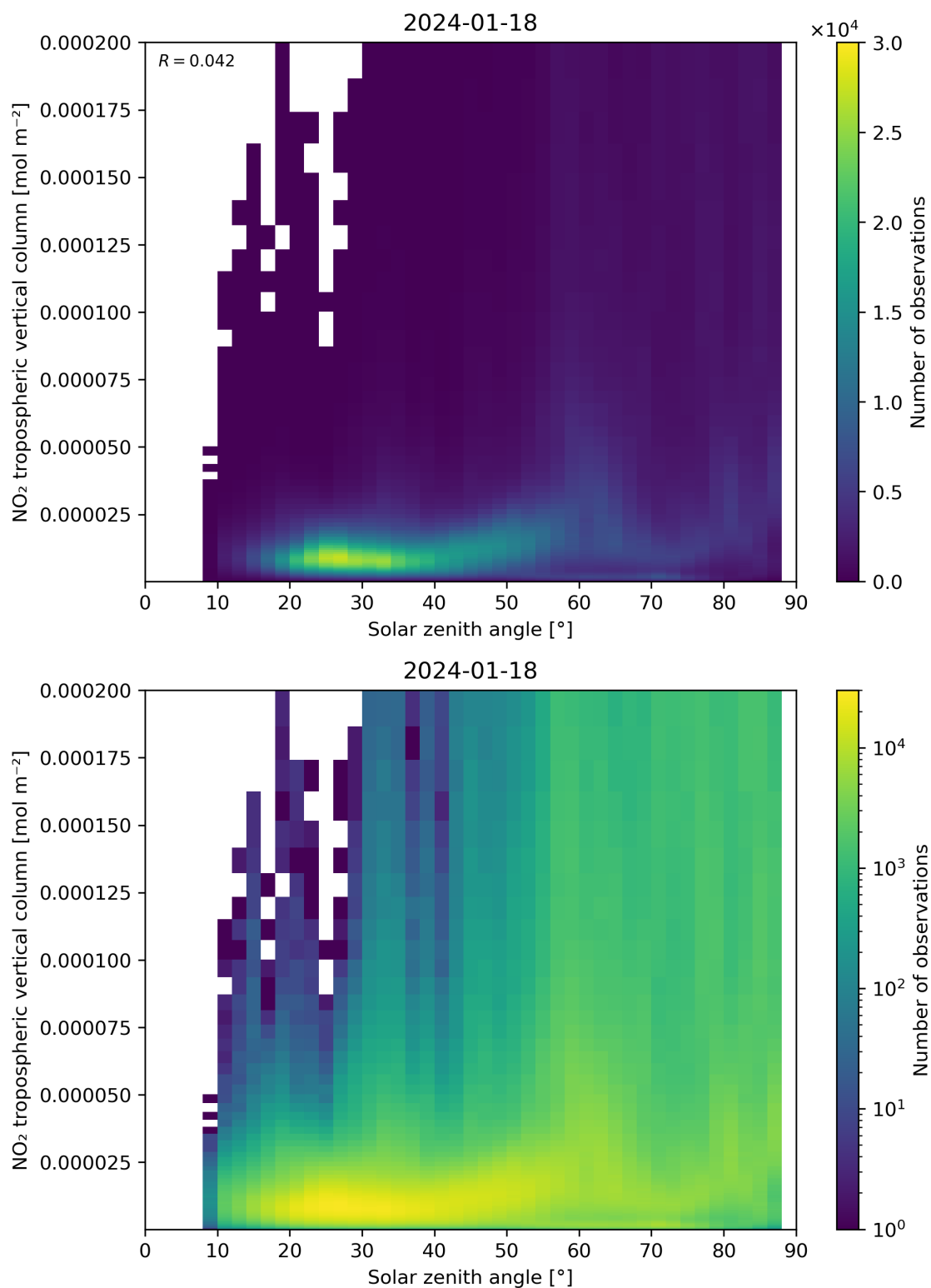
Figure 155: Scatter density plot of “Solar zenith angle” against “NO 2 tropospheric vertical column” for 2024-01-17 to 2024-01-19.
