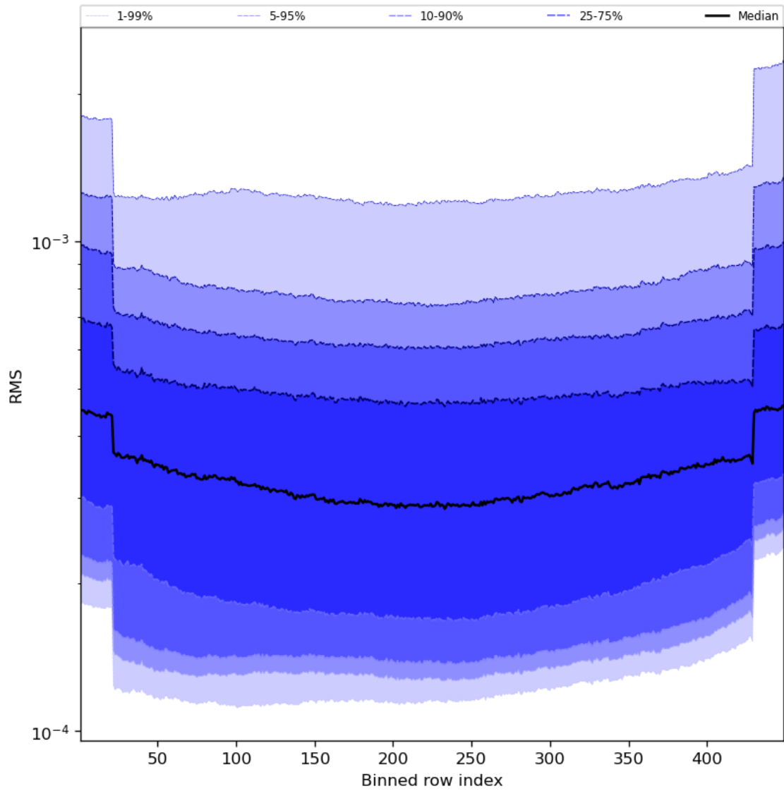
Figure 60: Along track statistics of “RMS” for 2024-01-17 to 2024-01-19
