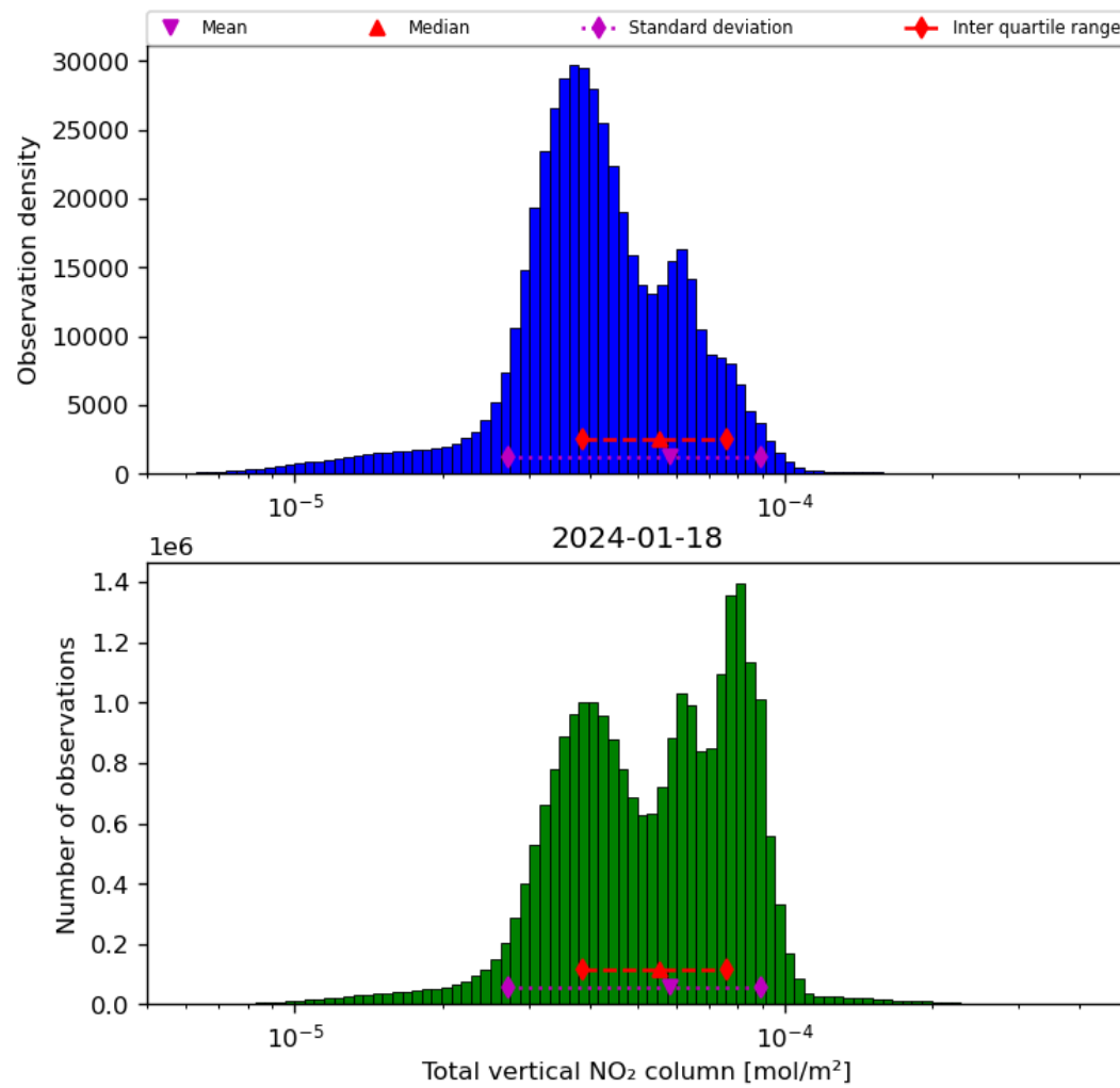
Figure 38: Histogram of “Total vertical NO 2 column” for 2024-01-17 to 2024-01-19
