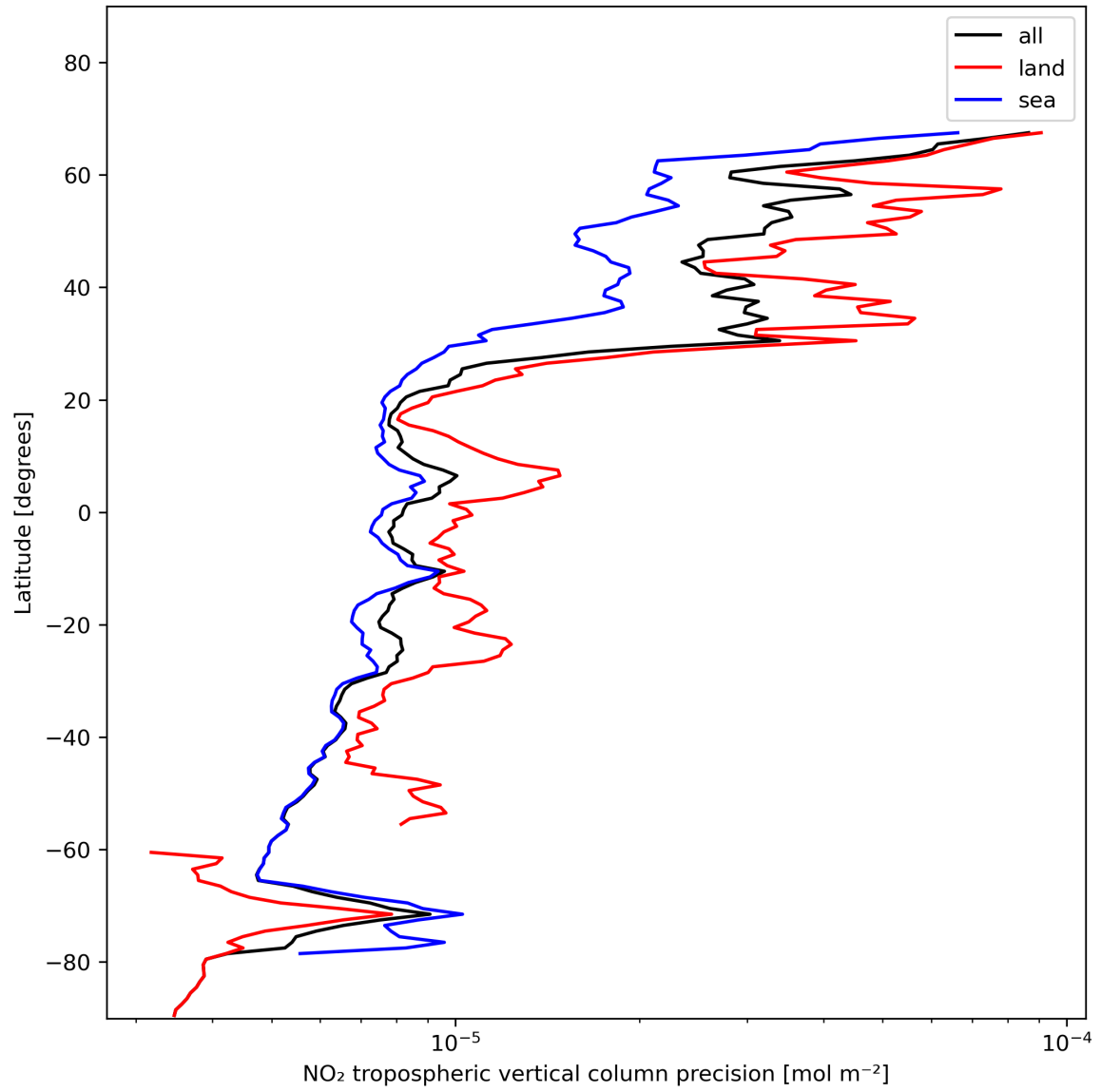
Figure 13: Zonal average of "NO 2 tropospheric vertical column precision" for 2024-01-17 to 2024-01-19.
