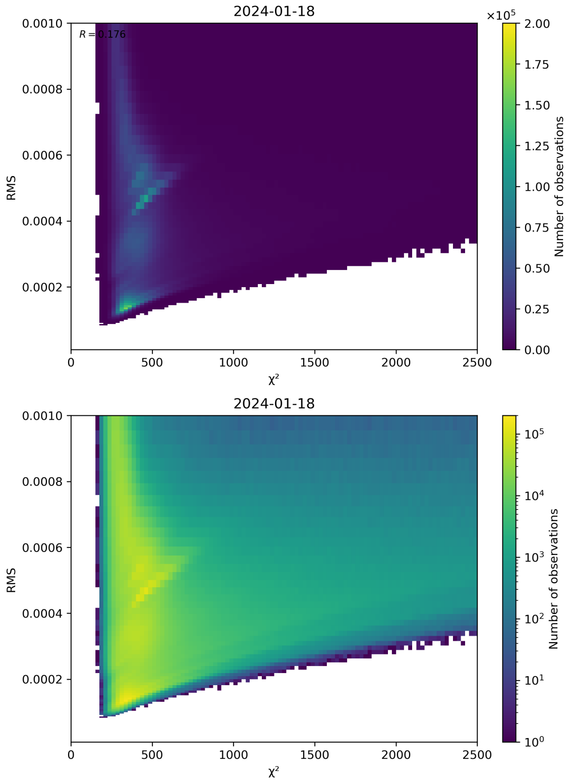
Figure 82: Scatter density plot of “ \chi^2 ” against “RMS” for 2024-01-17 to 2024-01-19.
