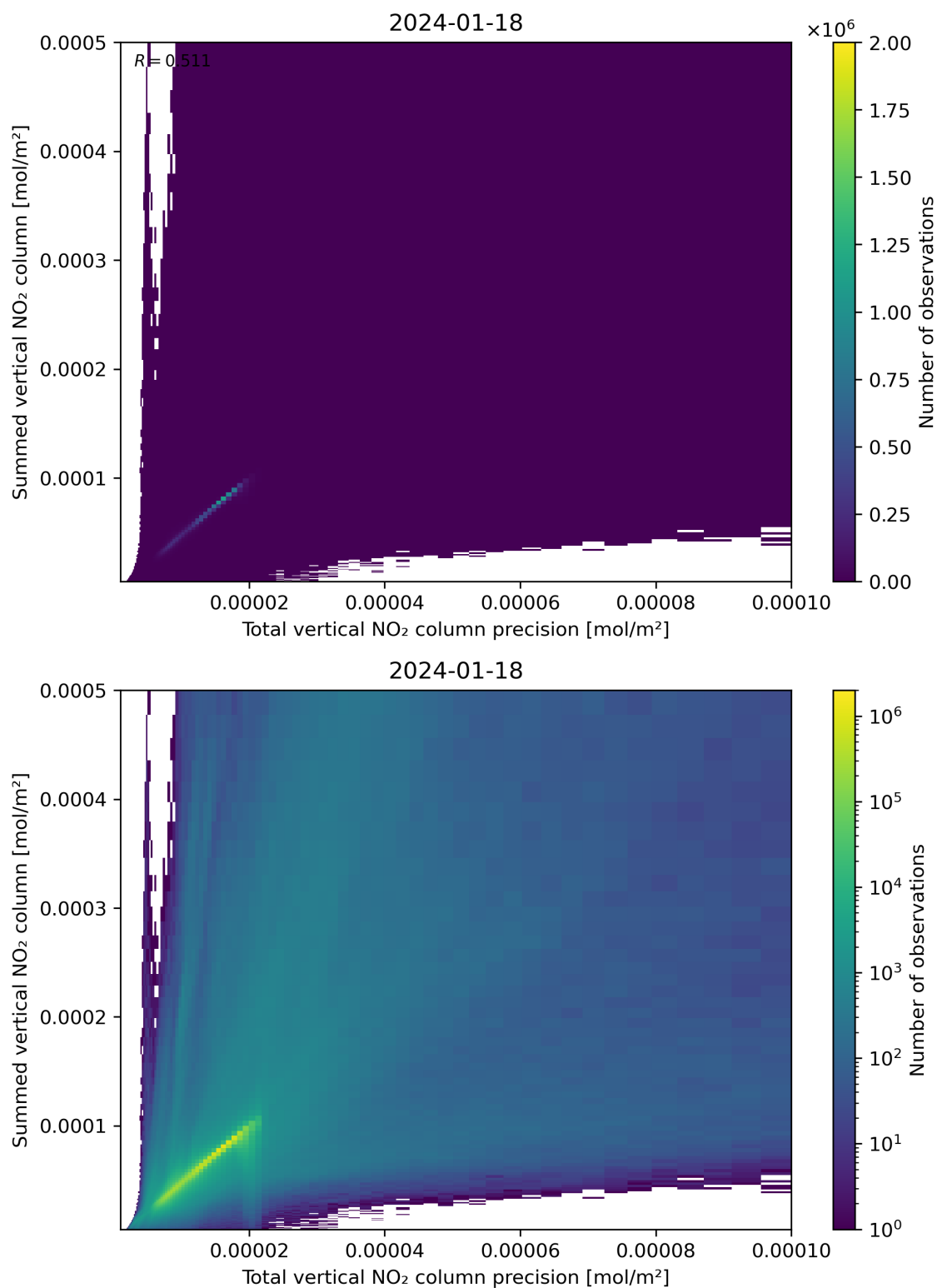
Figure 117: Scatter density plot of “Total vertical NO 2 column precision” against “Summed vertical NO 2 column” for 2024-01-17 to 2024-01-19.
