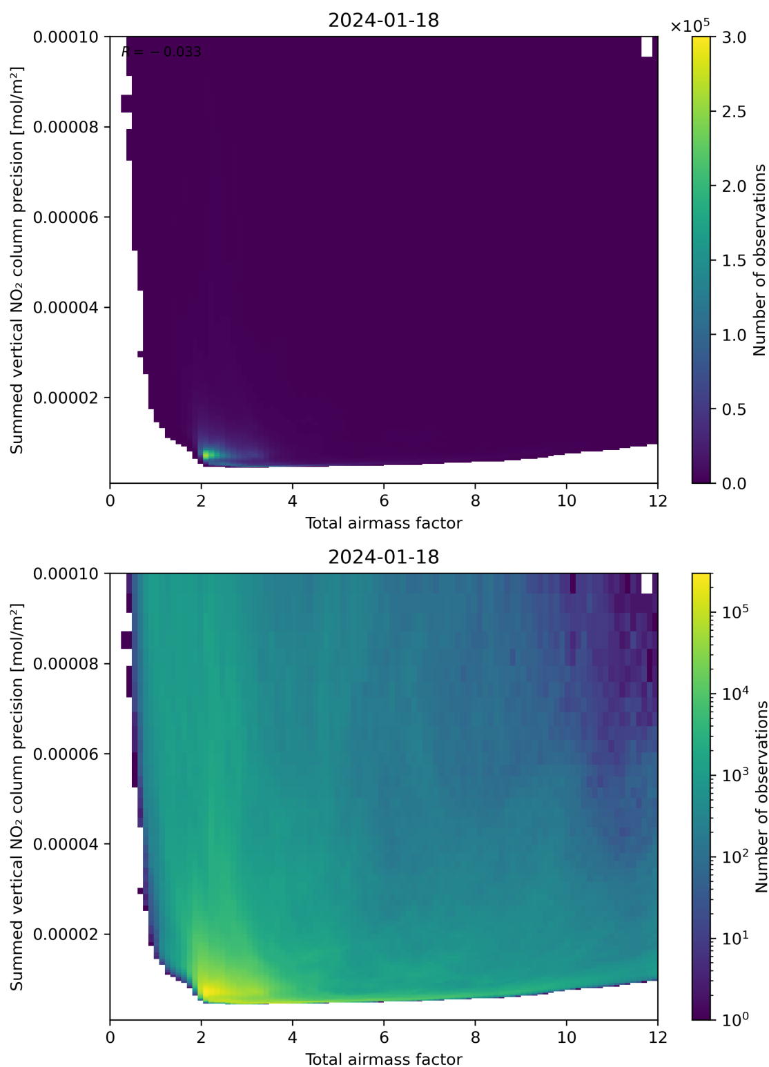
Figure 66: Scatter density plot of “Total airmass factor” against “Summed vertical NO 2 column precision” for 2024-01-17 to 2024-01-19.
