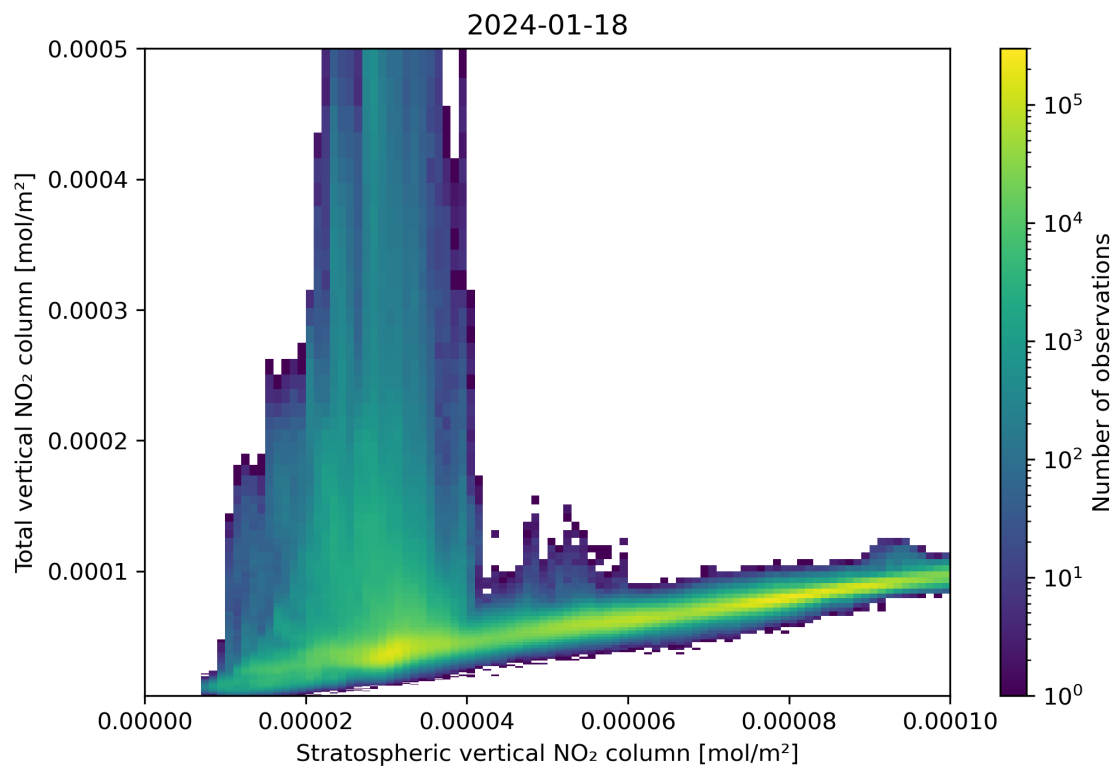
Figure 100: Scatter density plot of “Stratospheric vertical NO 2 column” against “Total vertical NO 2 column” for 2024-01-17 to 2024-01-19.
