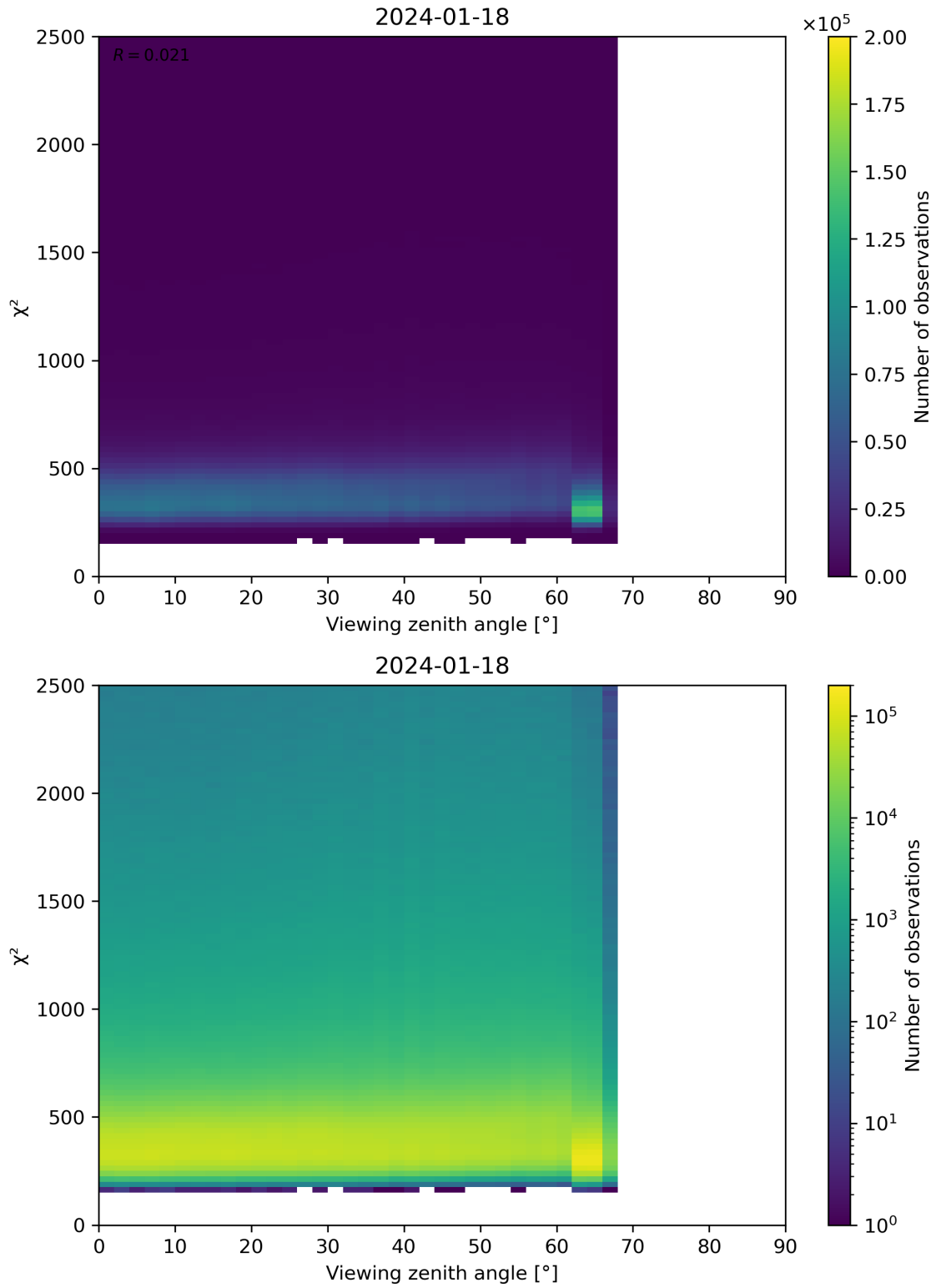
Figure 162: Scatter density plot of “Viewing zenith angle” against “ \chi^2 ” for 2024-01-17 to 2024-01-19.
