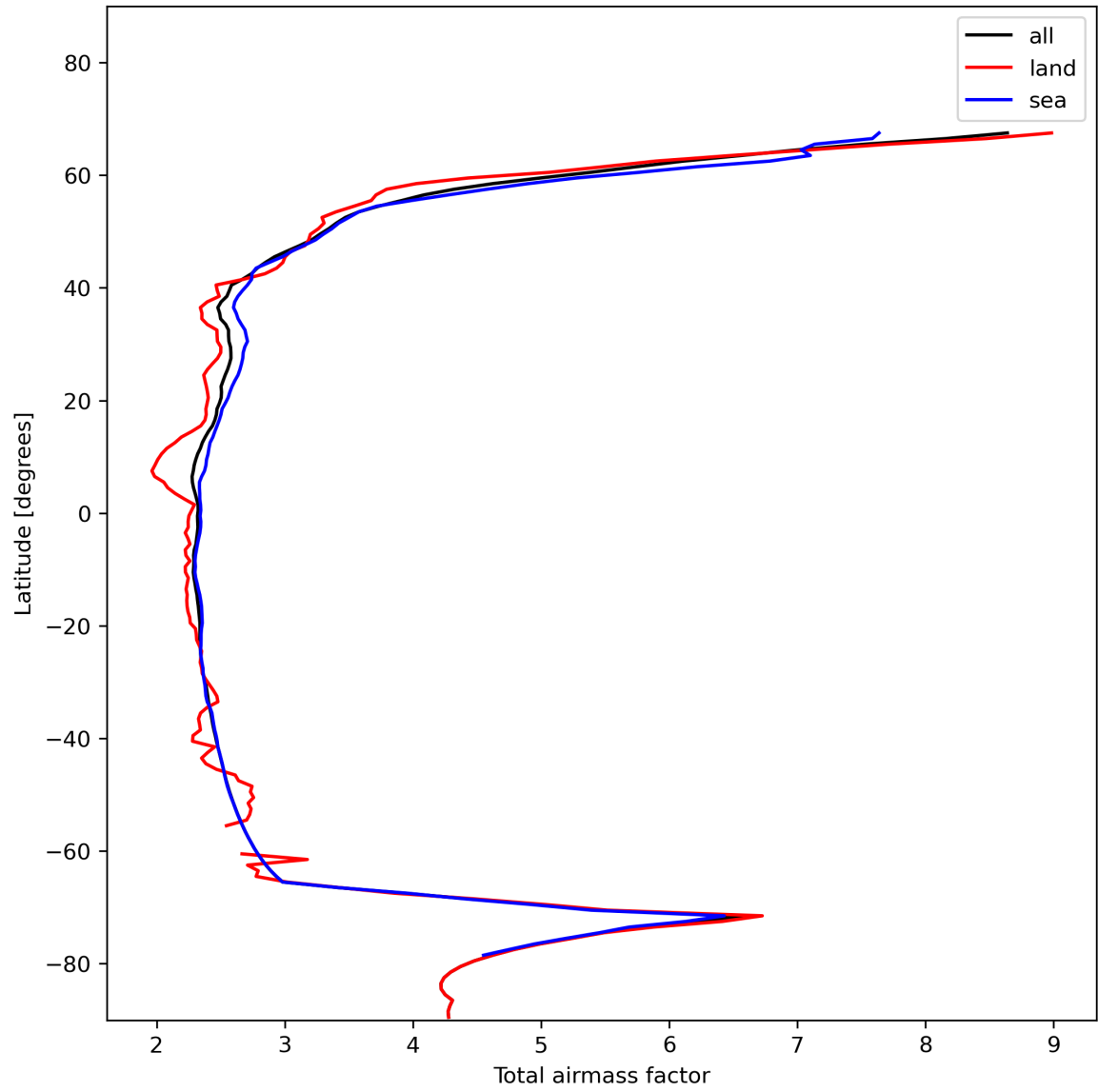
Figure 15: Zonal average of “Total airmass factor” for 2024-01-17 to 2024-01-19.
