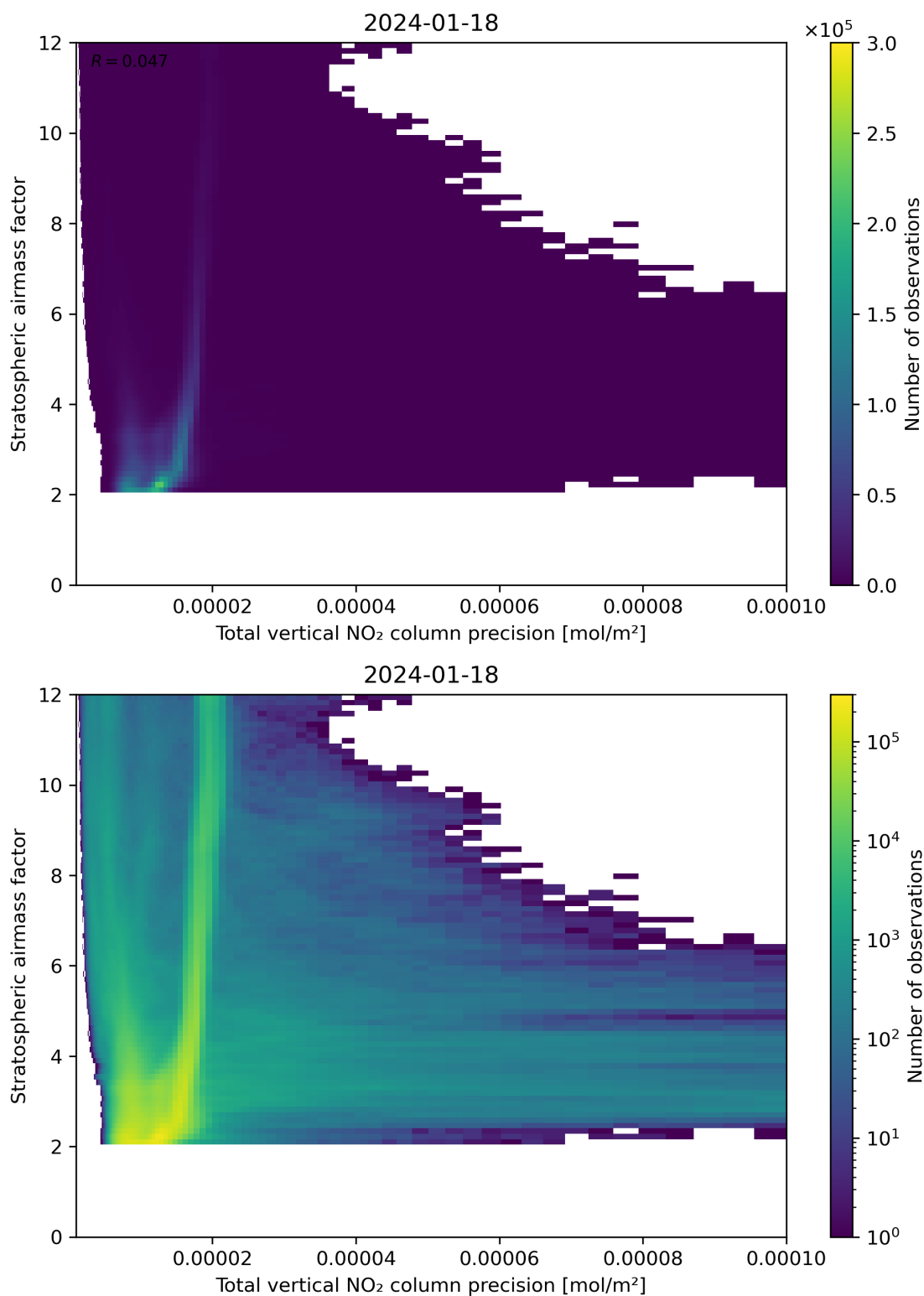
Figure 115: Scatter density plot of “Total vertical NO 2 column precision” against “Stratospheric air mass factor” for 2024-01-17 to 2024-01-19.
