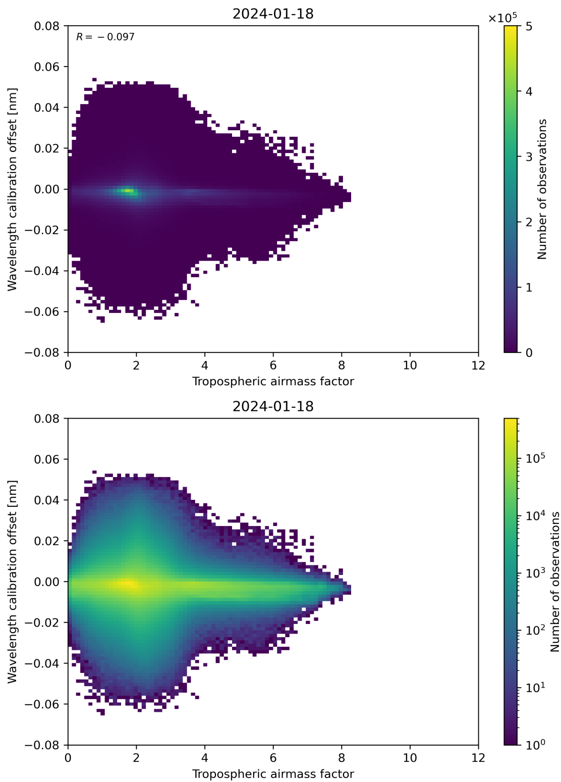
Figure 80: Scatter density plot of “Tropospheric airmass factor” against “Wavelength calibration offset” for 2024-01-17 to 2024-01-19.
