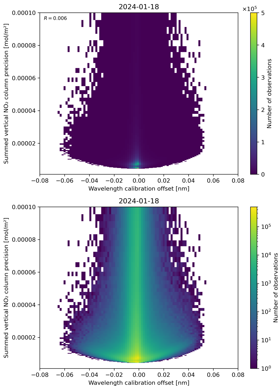
Figure 178: Scatter density plot of “Wavelength calibration offset” against “Summed vertical NO 2 column precision” for 2024-01-17 to 2024-01-19.
