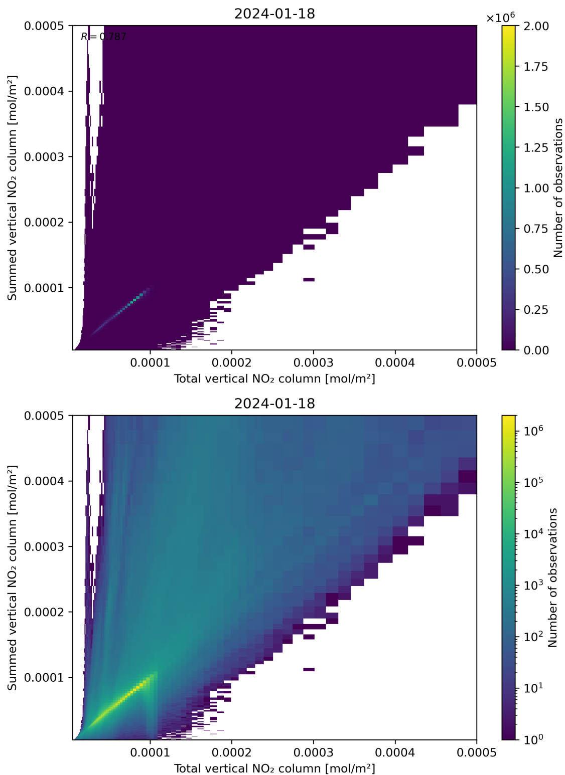
Figure 112: Scatter density plot of “Total vertical NO 2 column” against “Summed vertical NO 2 column” for 2024-01-17 to 2024-01-19.
