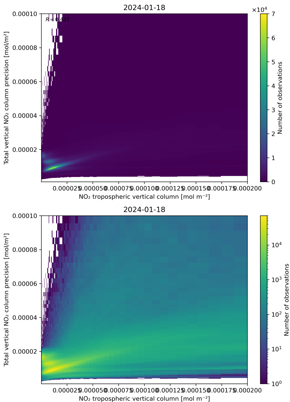
Figure 129: Scatter density plot of “NO 2 tropospheric vertical column” against “Total vertical NO 2 column precision” for 2024-01-17 to 2024-01-19.
