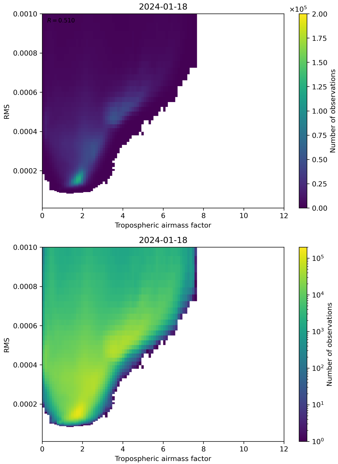
Figure 79: Scatter density plot of “Tropospheric airmass factor” against “RMS” for 2024-01-17 to 2024-01-19.
