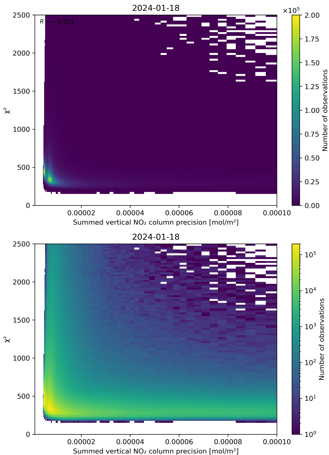
Figure 107: Scatter density plot of “Summed vertical NO 2 column precision” against “ \chi^2 ” for 2024-01-17 to 2024-01-19.
