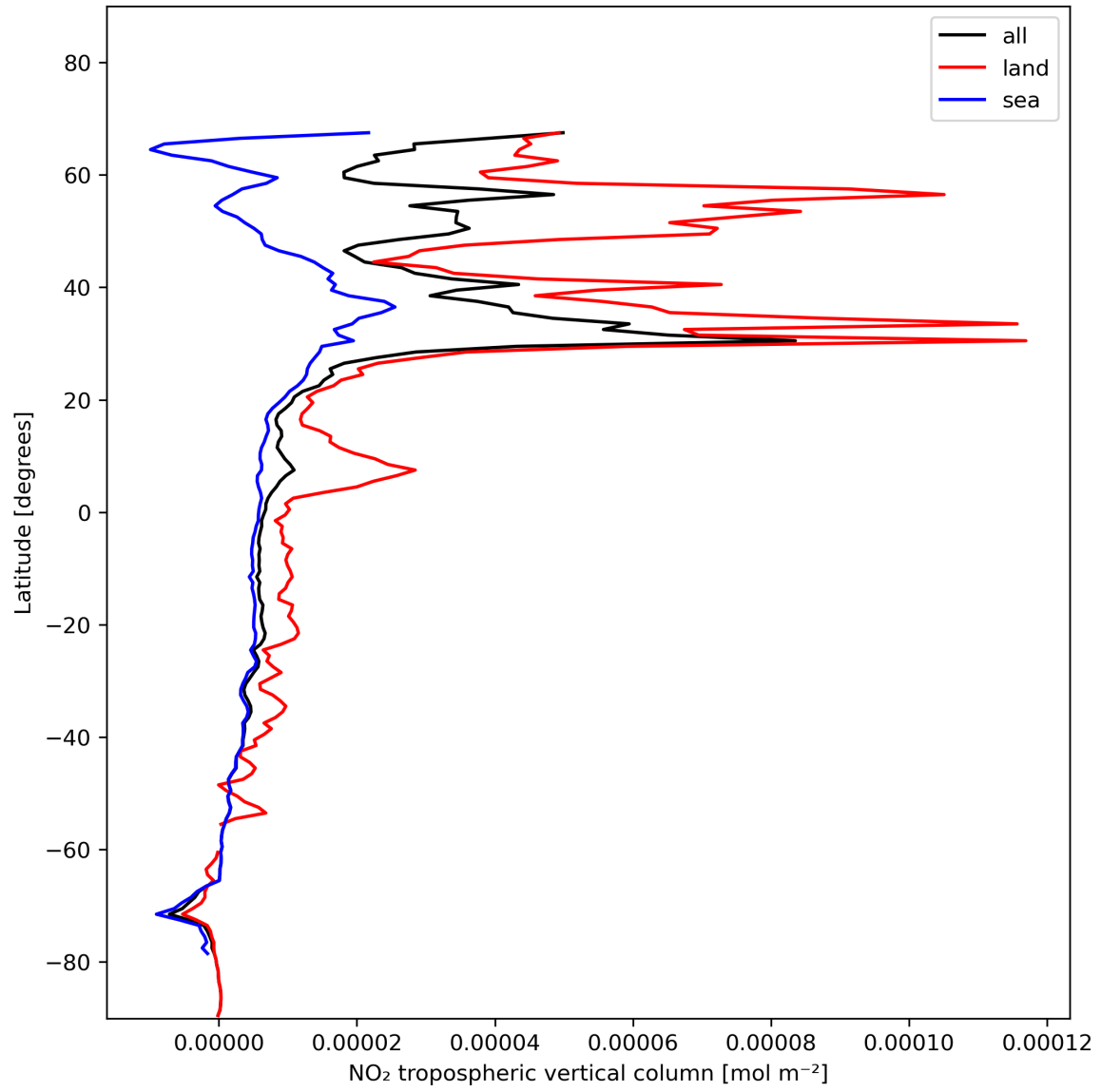
Figure 12: Zonal average of “NO 2 tropospheric vertical column” for 2024-01-17 to 2024-01-19.
