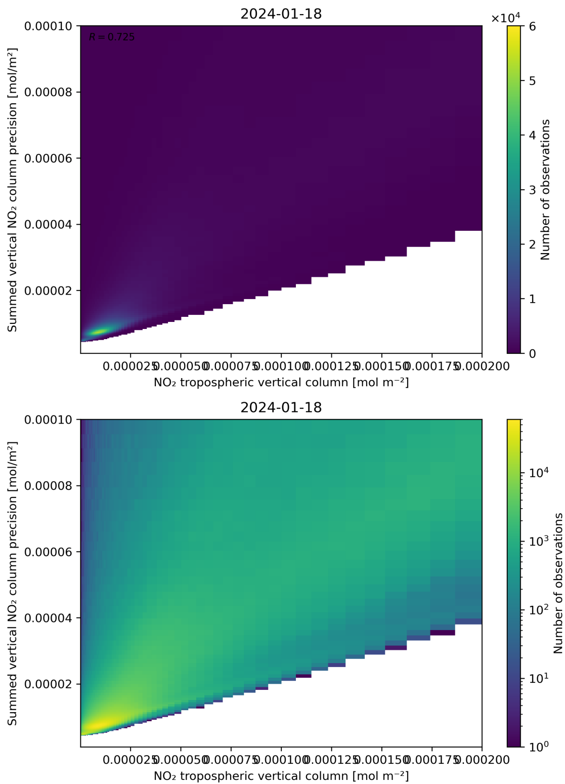
Figure 127: Scatter density plot of “NO 2 tropospheric vertical column” against “Summed vertical NO 2 column precision” for 2024-01-17 to 2024-01-19.
