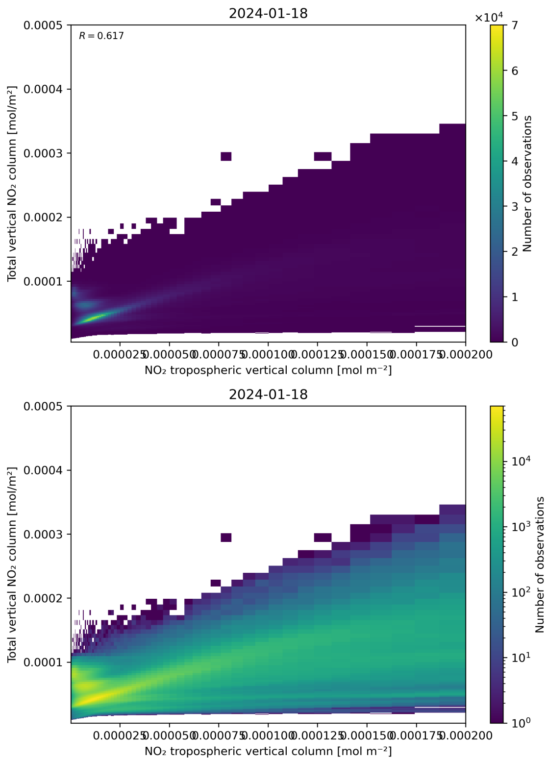
Figure 128: Scatter density plot of “NO 2 tropospheric vertical column” against “Total vertical NO 2 column” for 2024-01-17 to 2024-01-19.
