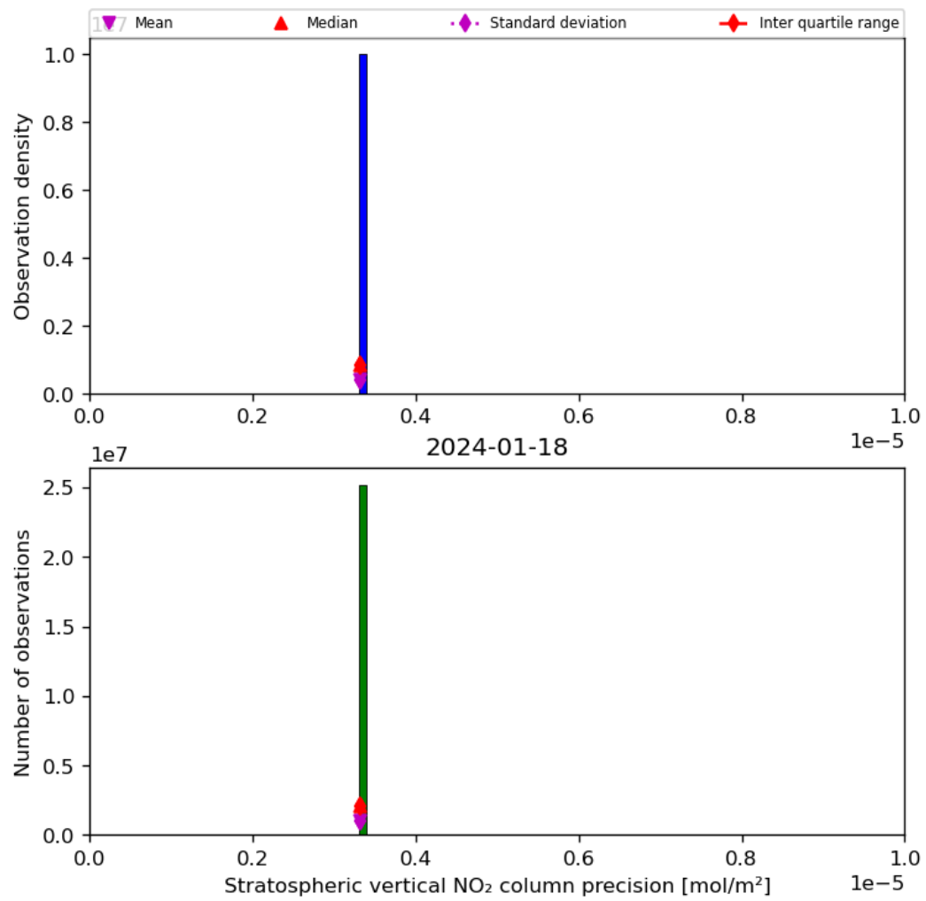
Figure 37: Histogram of “Stratospheric vertical NO 2 column precision” for 2024-01-17 to 2024-01-19
