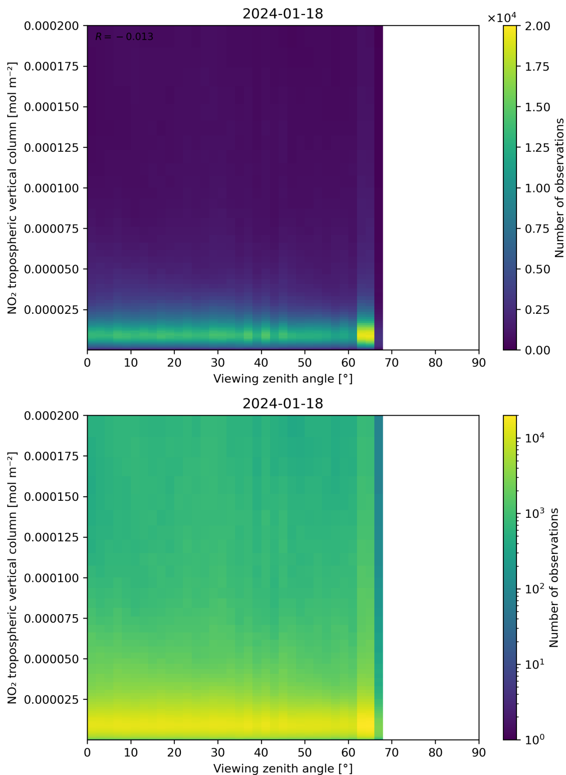
Figure 169: Scatter density plot of “Viewing zenith angle” against “NO 2 tropospheric vertical column” for 2024-01-17 to 2024-01-19.
