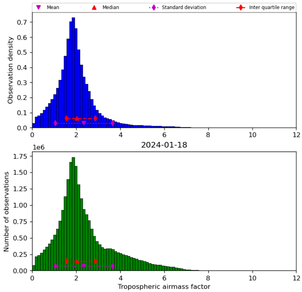
Figure 31: Histogram of “Tropospheric airmass factor” for 2024-01-17 to 2024-01-19
