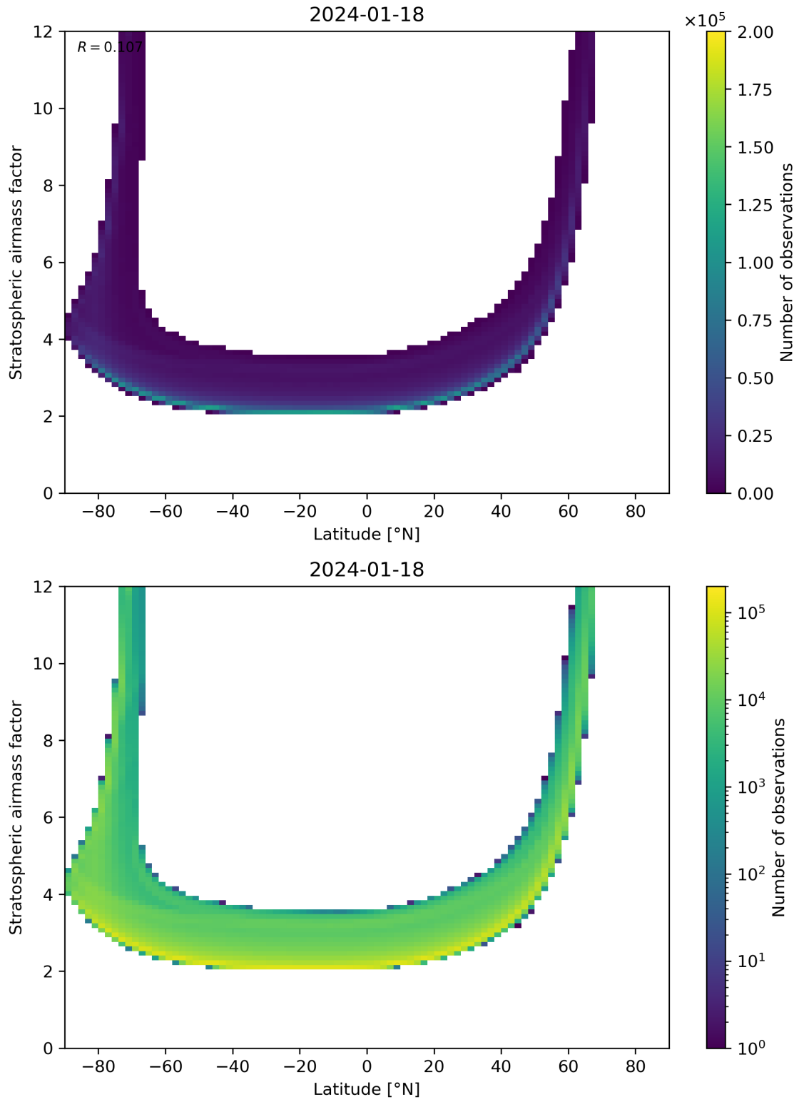
Figure 83: Scatter density plot of “Latitude” against “Stratospheric air mass factor” for 2024-01-17 to 2024-01-19.
