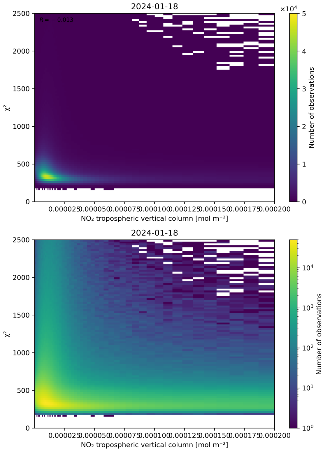
Figure 124: Scatter density plot of “NO 2 tropospheric vertical column” against “ \chi^2 ” for 2024-01-17 to 2024-01-19.
