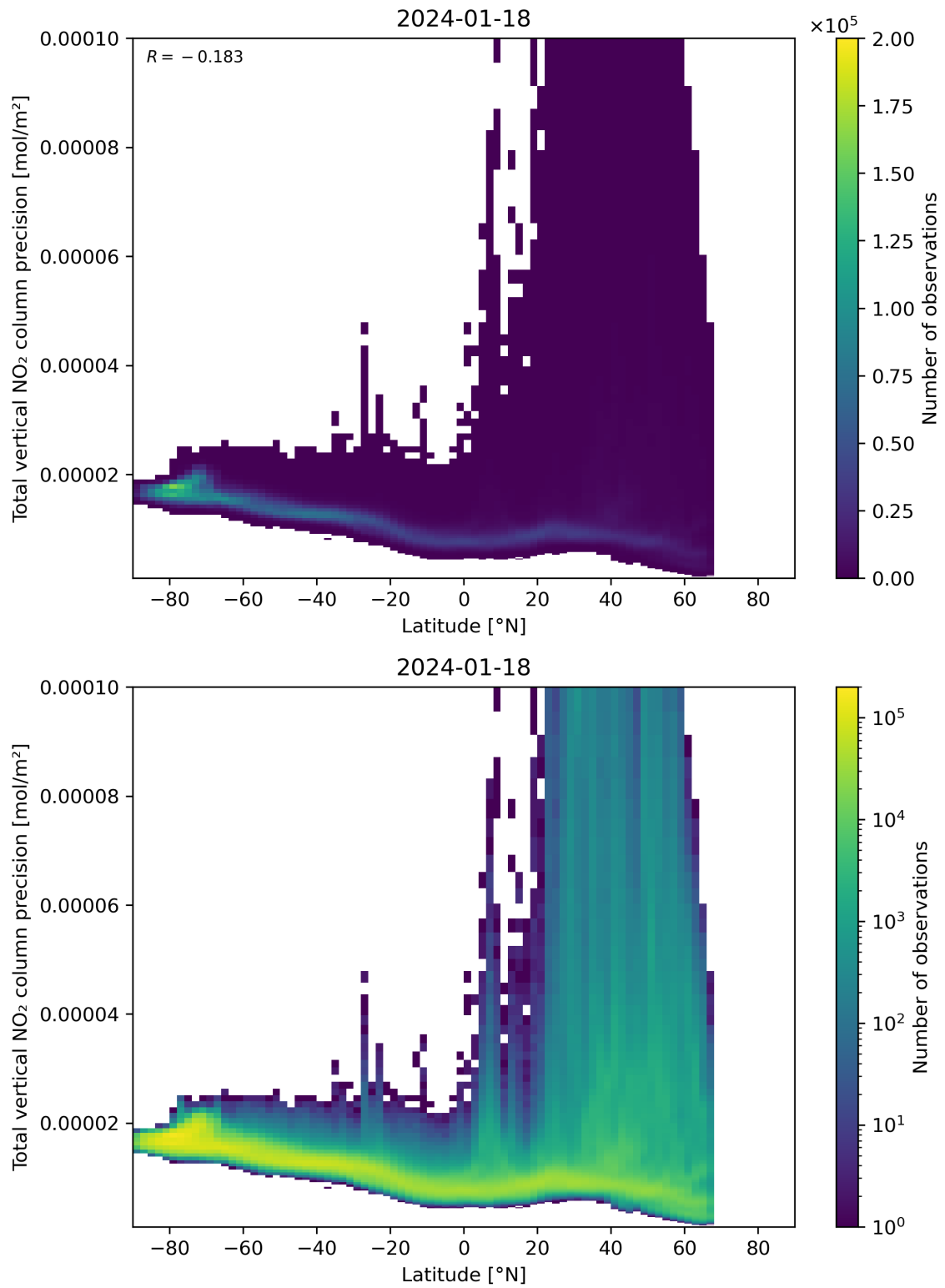
Figure 91: Scatter density plot of “Latitude” against “Total vertical NO 2 column precision” for 2024-01-17 to 2024-01-19.
