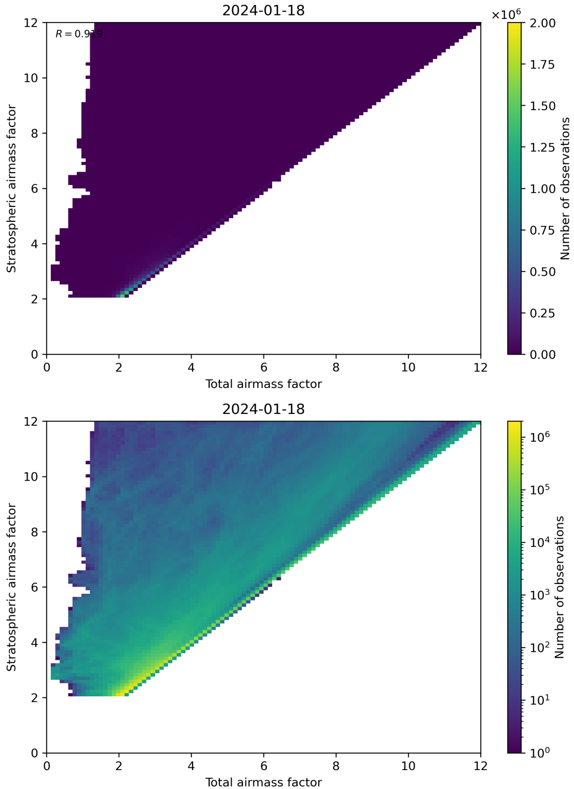
Figure 62: Scatter density plot of “Total airmass factor” against “Stratospheric airmass factor” for 2024-01-17 to 2024-01-19.
