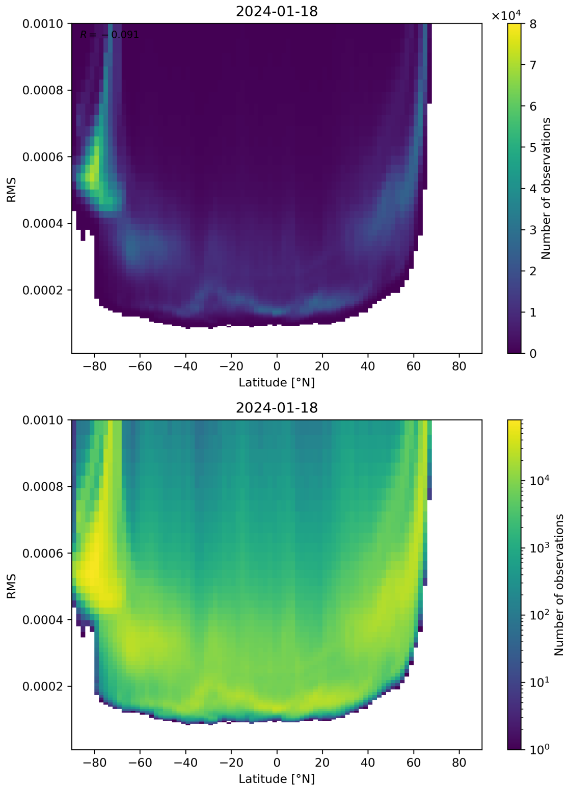
Figure 94: Scatter density plot of “Latitude” against “RMS” for 2024-01-17 to 2024-01-19.
