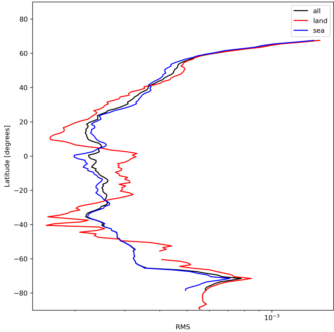
Figure 26: Zonal average of “RMS” for 2024-01-17 to 2024-01-19.
