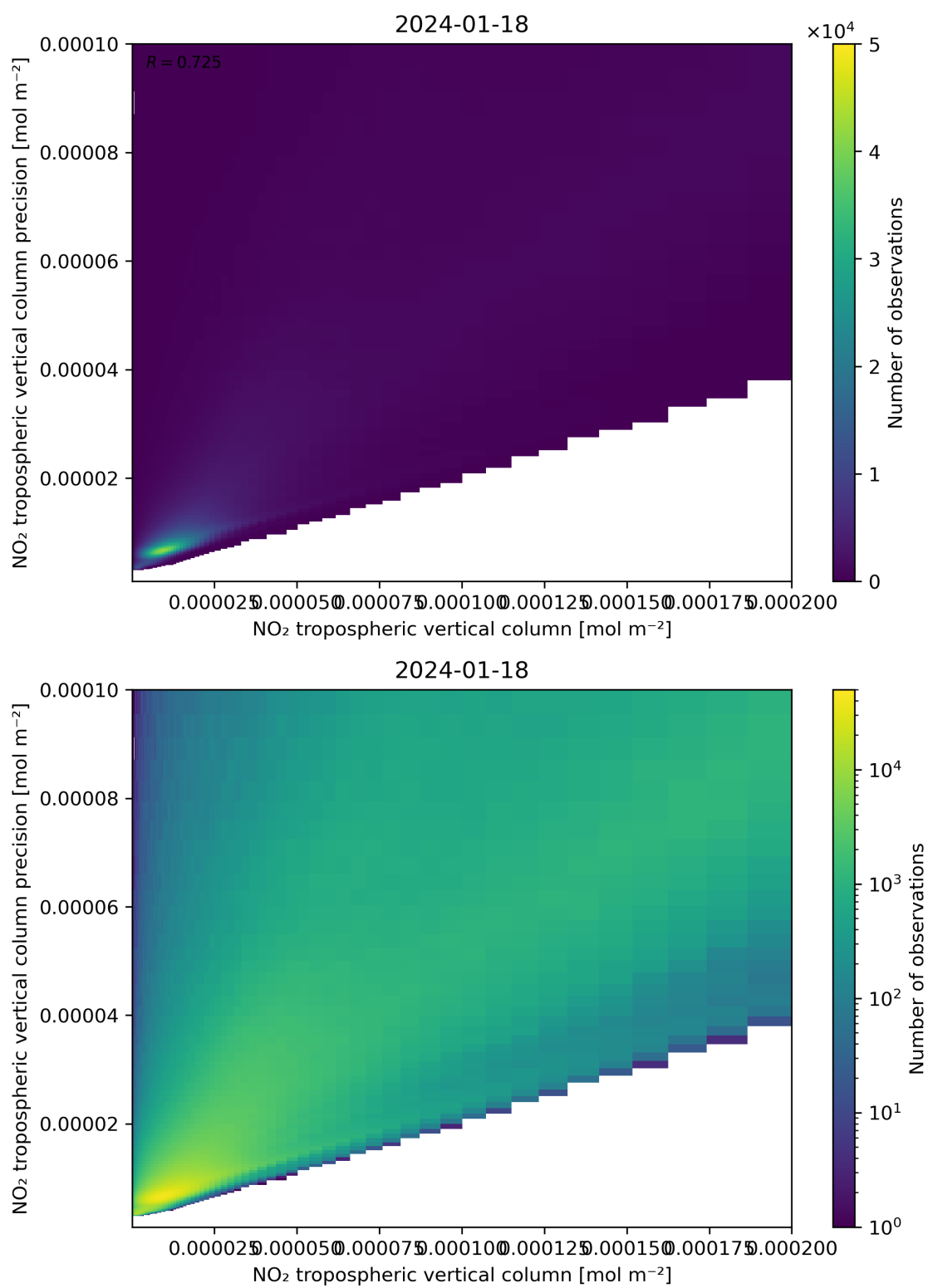
Figure 130: Scatter density plot of “NO 2 tropospheric vertical column” against “NO 2 tropospheric vertical column precision” for 2024-01-17 to 2024-01-19.
