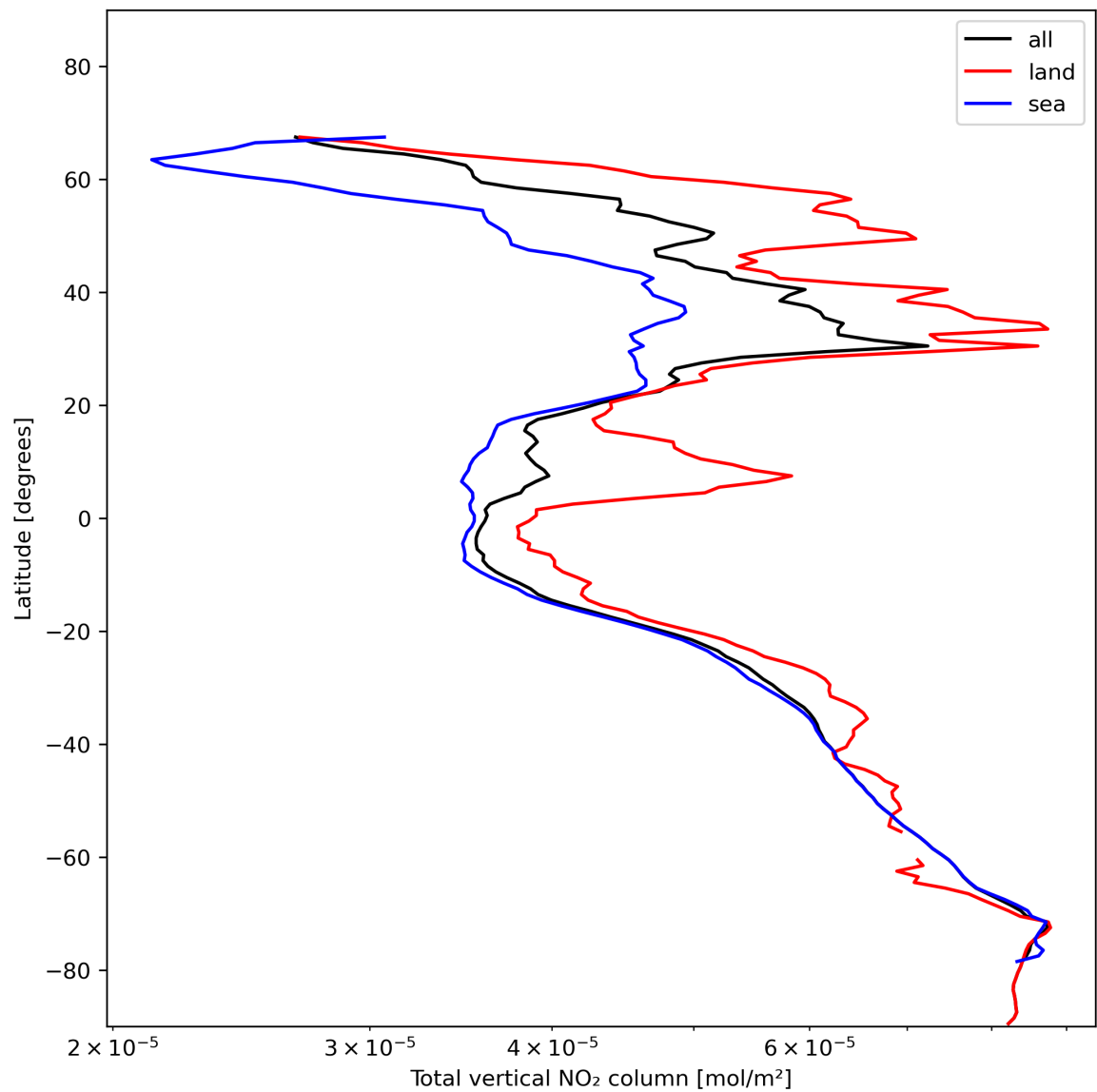
Figure 21: Zonal average of “Total vertical NO 2 column” for 2024-01-17 to 2024-01-19.
