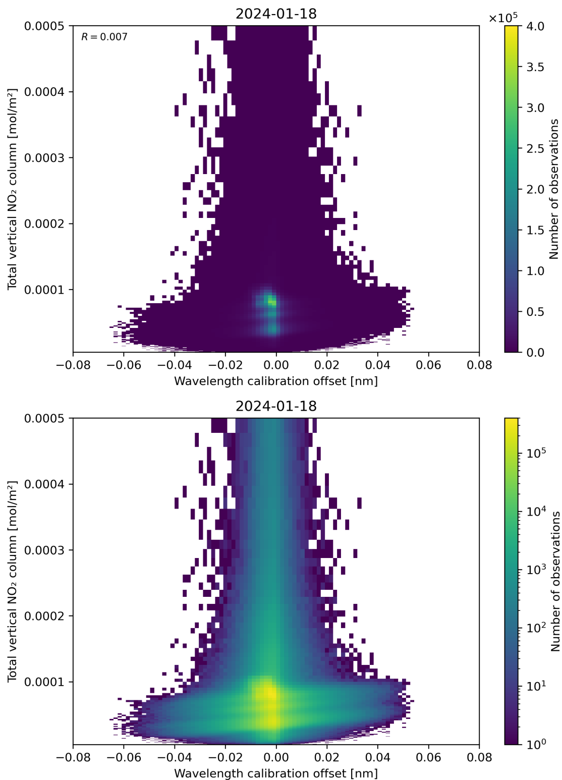
Figure 179: Scatter density plot of “Wavelength calibration offset” against “Total vertical NO 2 column” for 2024-01-17 to 2024-01-19.
