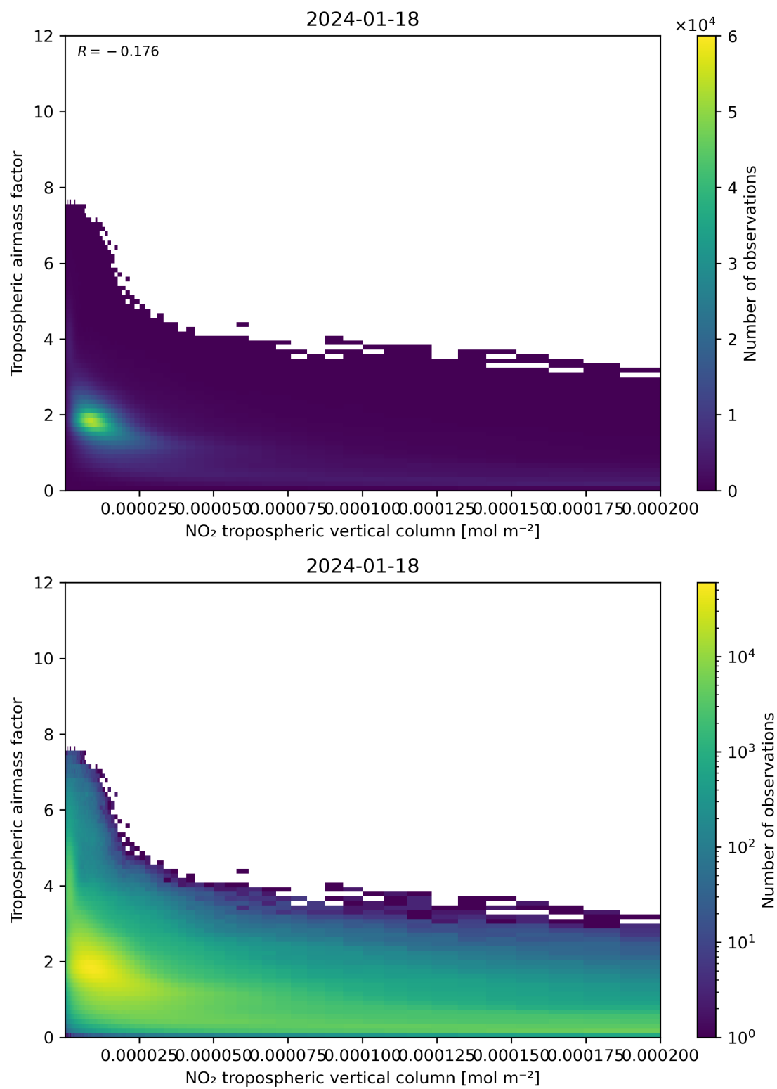
Figure 123: Scatter density plot of “NO 2 tropospheric vertical column” against “Tropospheric air mass factor” for 2024-01-17 to 2024-01-19.
