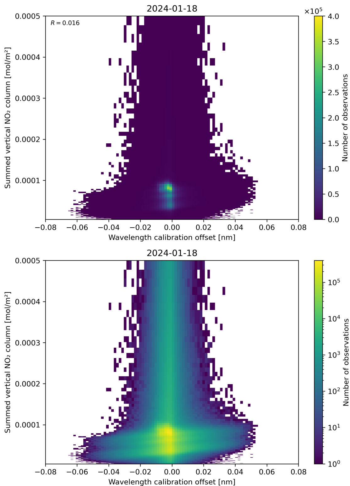
Figure 177: Scatter density plot of “Wavelength calibration offset” against “Summed vertical NO 2 column” for 2024-01-17 to 2024-01-19.
