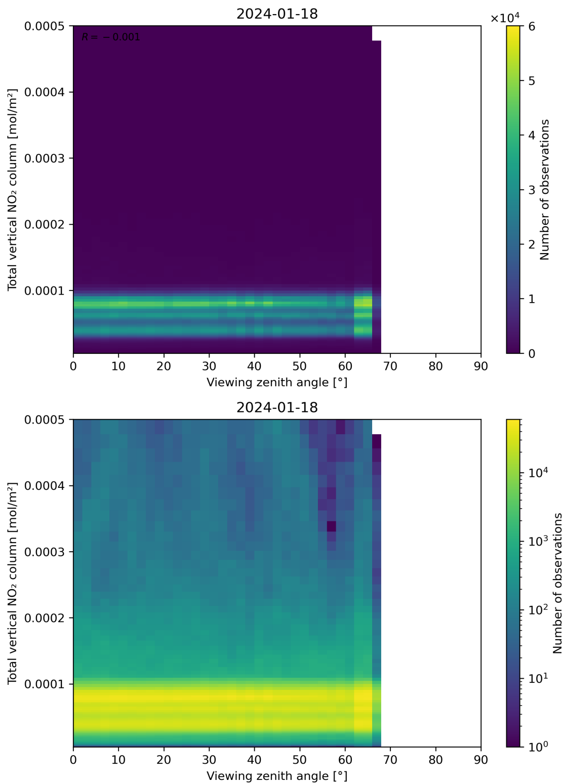
Figure 167: Scatter density plot of “Viewing zenith angle” against “Total vertical NO 2 column” for 2024-01-17 to 2024-01-19.
