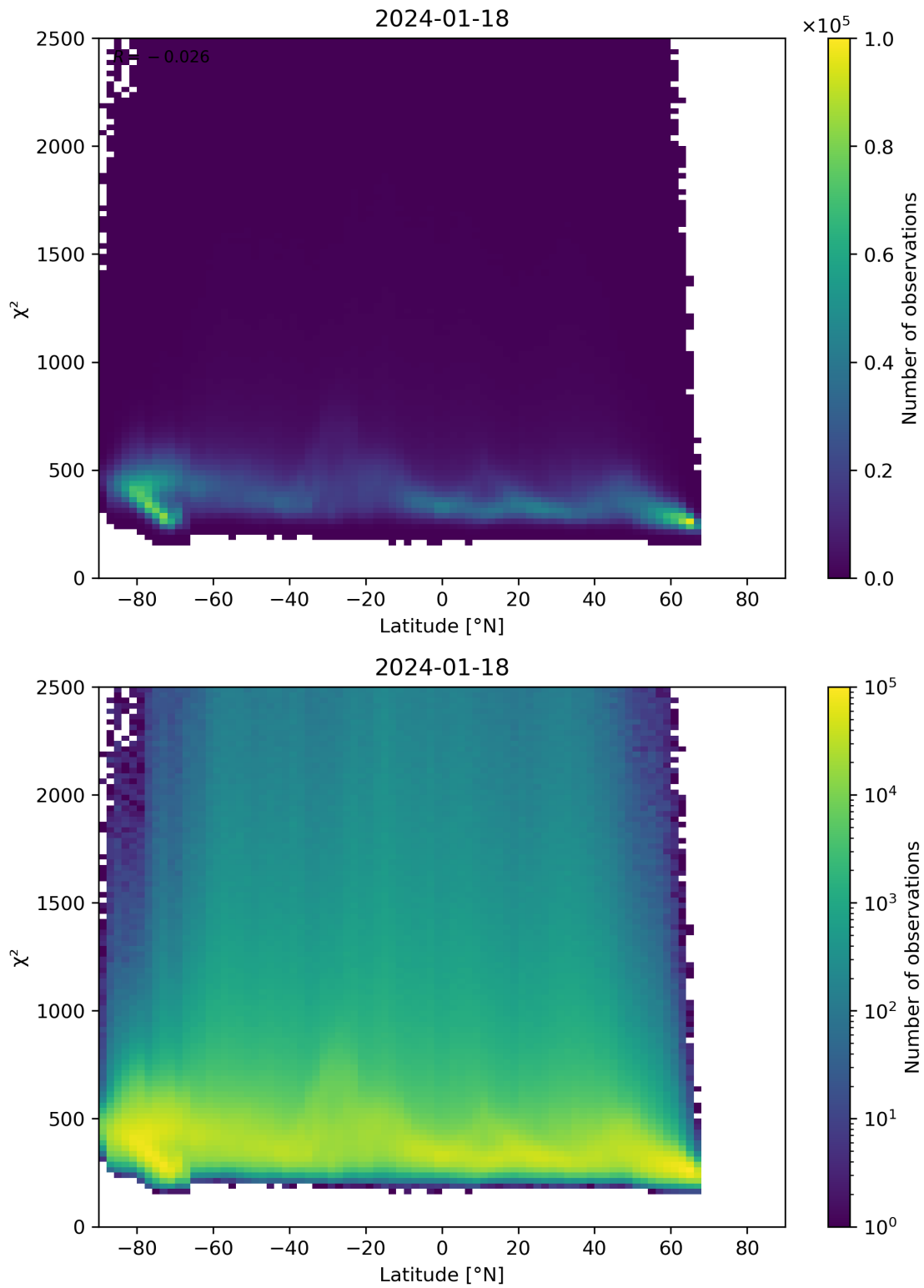
Figure 86: Scatter density plot of “Latitude” against “ \chi^2 ” for 2024-01-17 to 2024-01-19.
