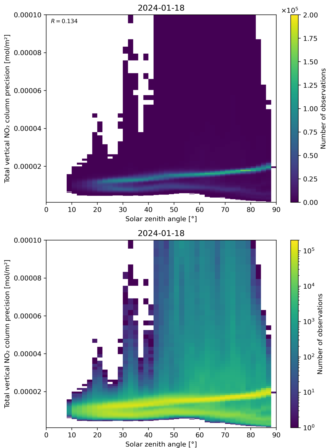
Figure 154: Scatter density plot of “Solar zenith angle” against “Total vertical NO 2 column precision” for 2024-01-17 to 2024-01-19.
