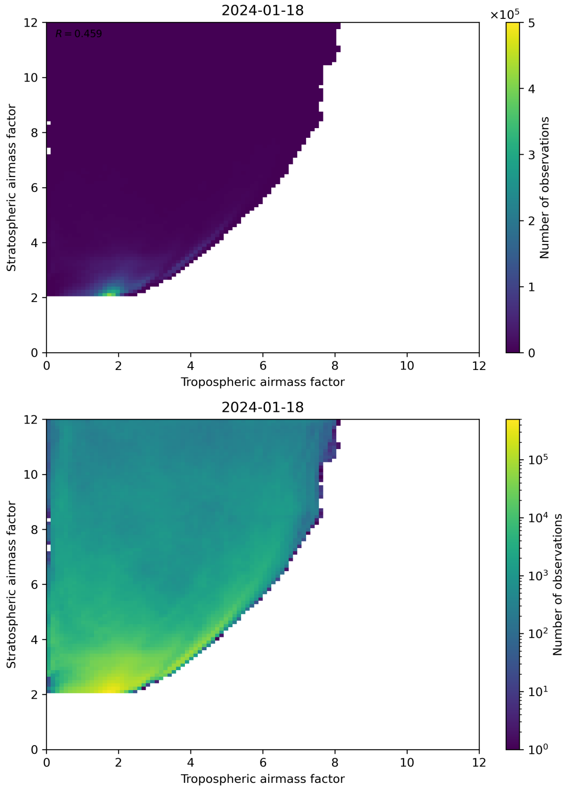
Figure 71: Scatter density plot of “Tropospheric airmass factor” against “Stratospheric airmass factor” for 2024-01-17 to 2024-01-19.
