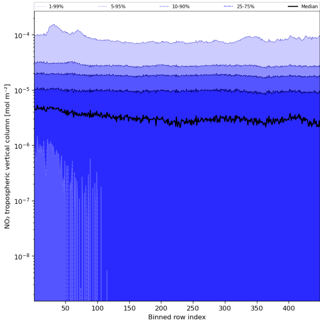
Figure 46: Along track statistics of “NO 2 tropospheric vertical column” for 2024-02-09 to 2024-02-11
