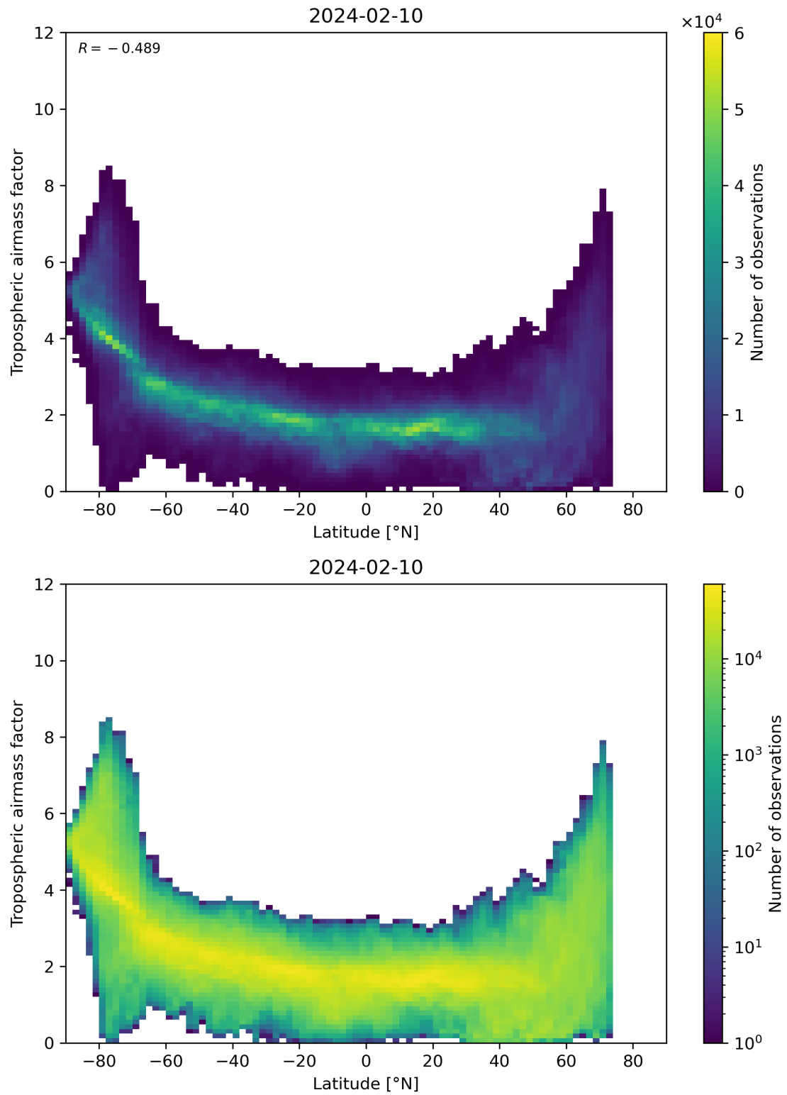
Figure 85: Scatter density plot of “Latitude” against “Tropospheric airmass factor” for 2024-02-09 to 2024-02-11.
