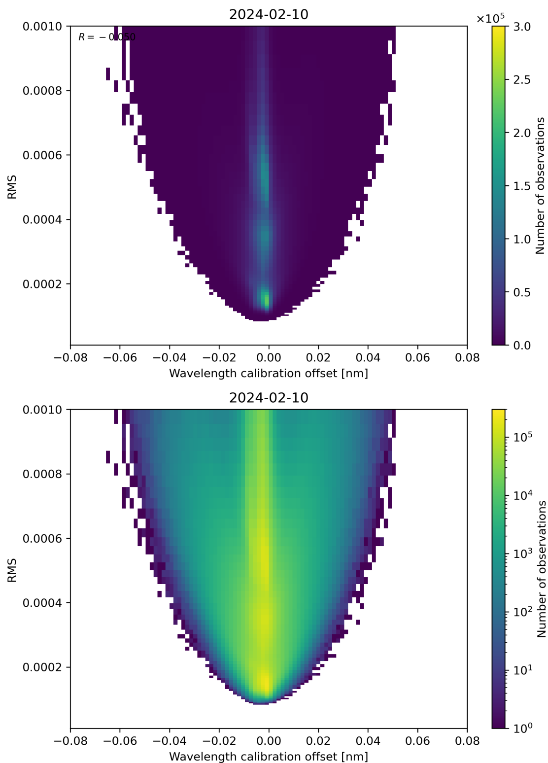
Figure 181: Scatter density plot of “Wavelength calibration offset” against “RMS” for 2024-02-09 to 2024-02-11.
