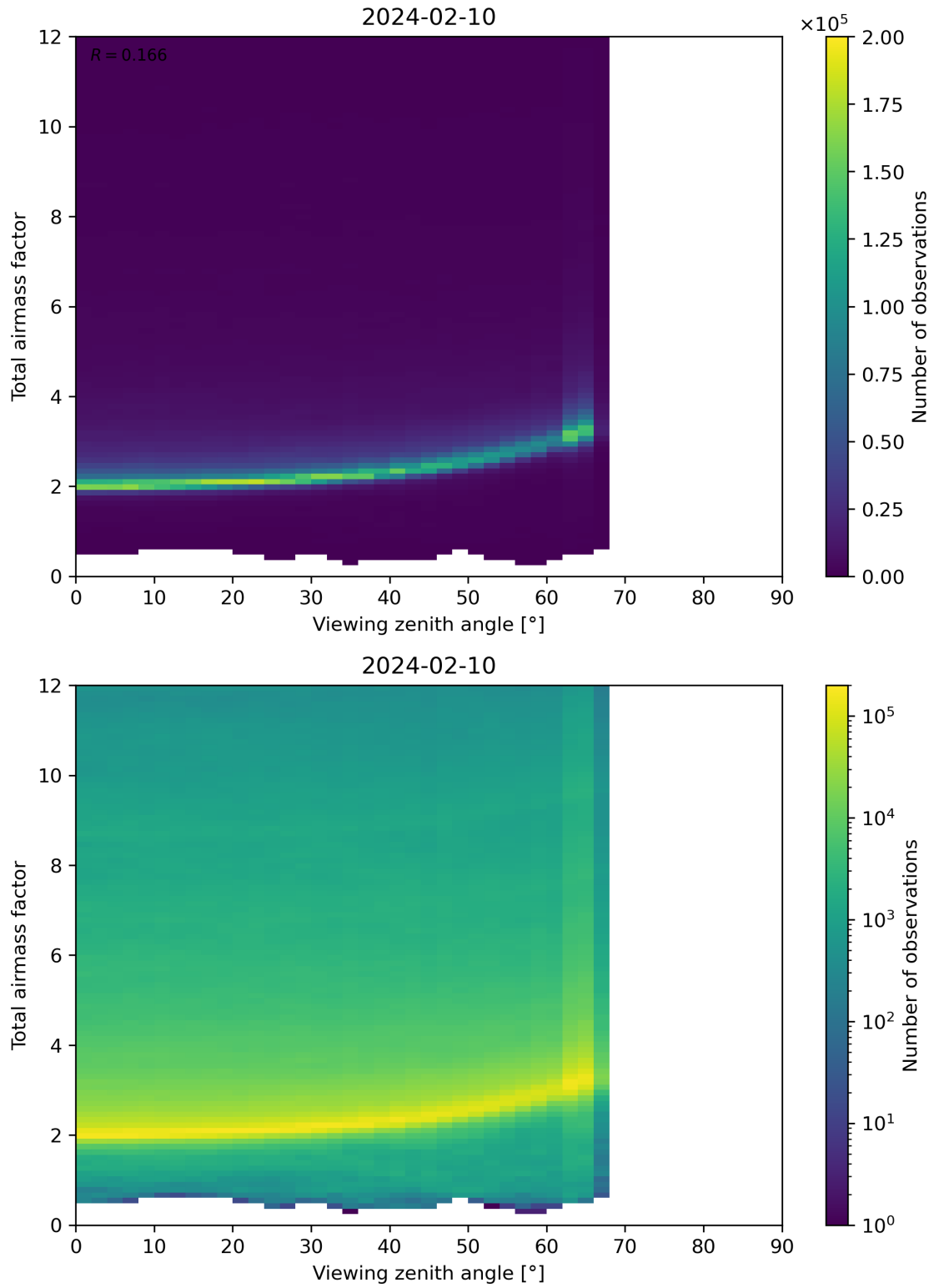
Figure 160: Scatter density plot of “Viewing zenith angle” against “Total airmass factor” for 2024-02-09 to 2024-02-11.
