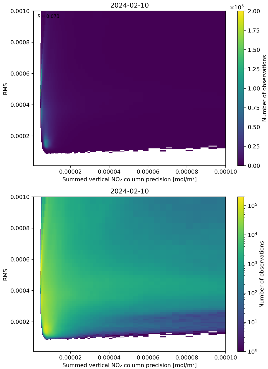
Figure 108: Scatter density plot of “Summed vertical NO 2 column precision” against “RMS” for 2024-02-09 to 2024-02-11.
