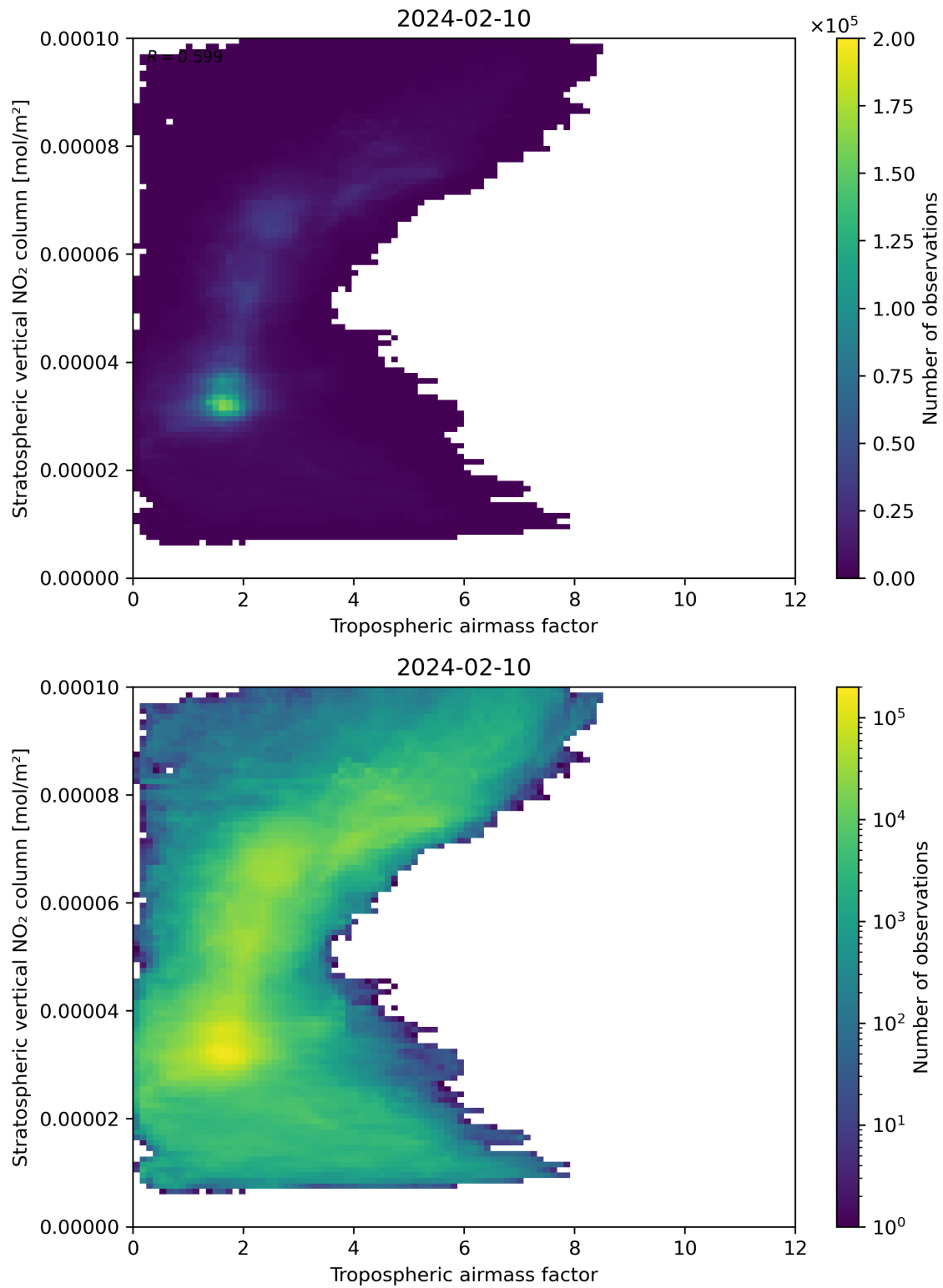
Figure 74: Scatter density plot of “Tropospheric air mass factor” against “Stratospheric vertical NO 2 column” for 2024-02-09 to 2024-02-11.
