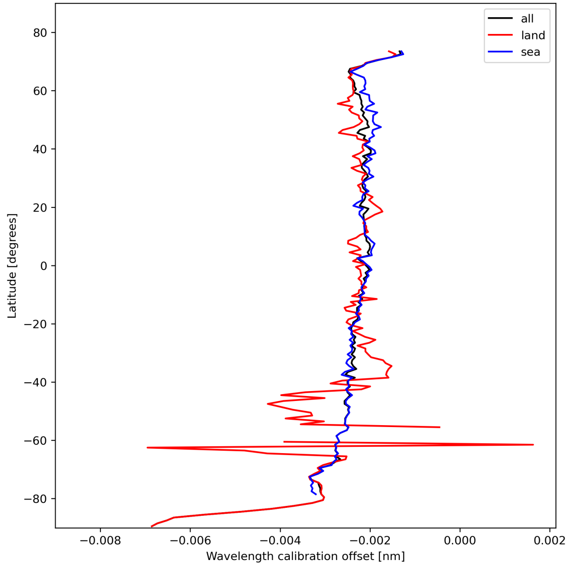
Figure 18: Zonal average of “Wavelength calibration offset” for 2024-02-09 to 2024-02-11.
