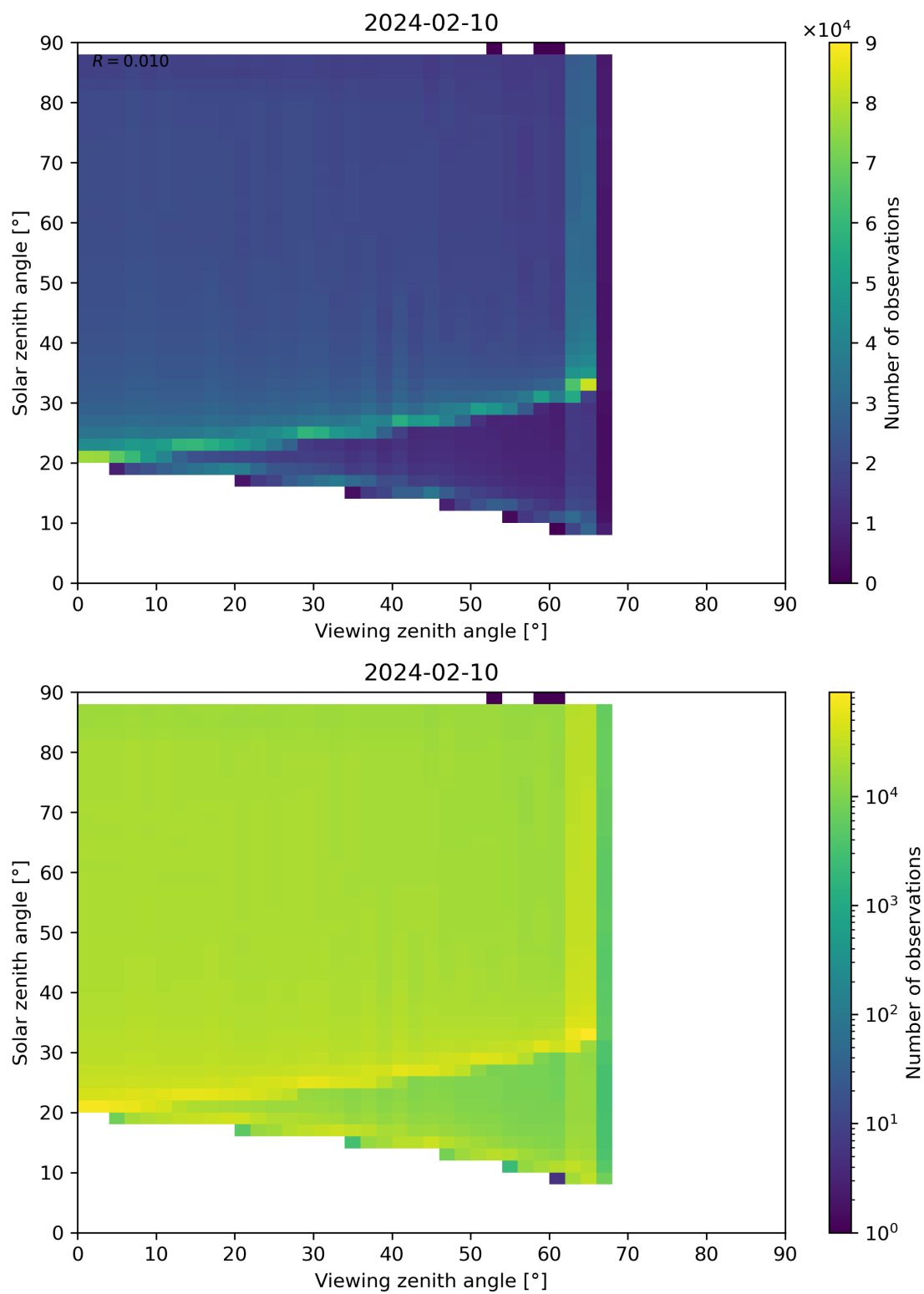
Figure 172: Scatter density plot of “Viewing zenith angle” against “Solar zenith angle” for 2024-02-09 to 2024-02-11.
