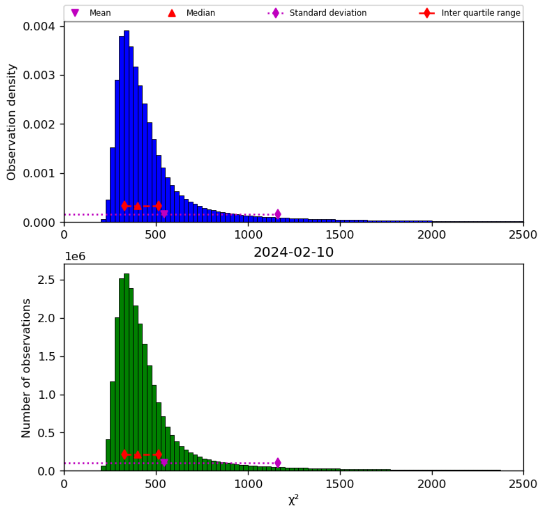
Figure 42: Histogram of “ \chi^2 ” for 2024-02-09 to 2024-02-11
