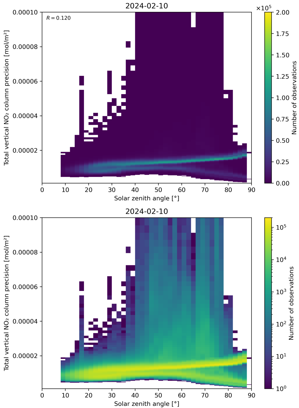
Figure 154: Scatter density plot of “Solar zenith angle” against “Total vertical NO 2 column precision” for 2024-02-09 to 2024-02-11.
