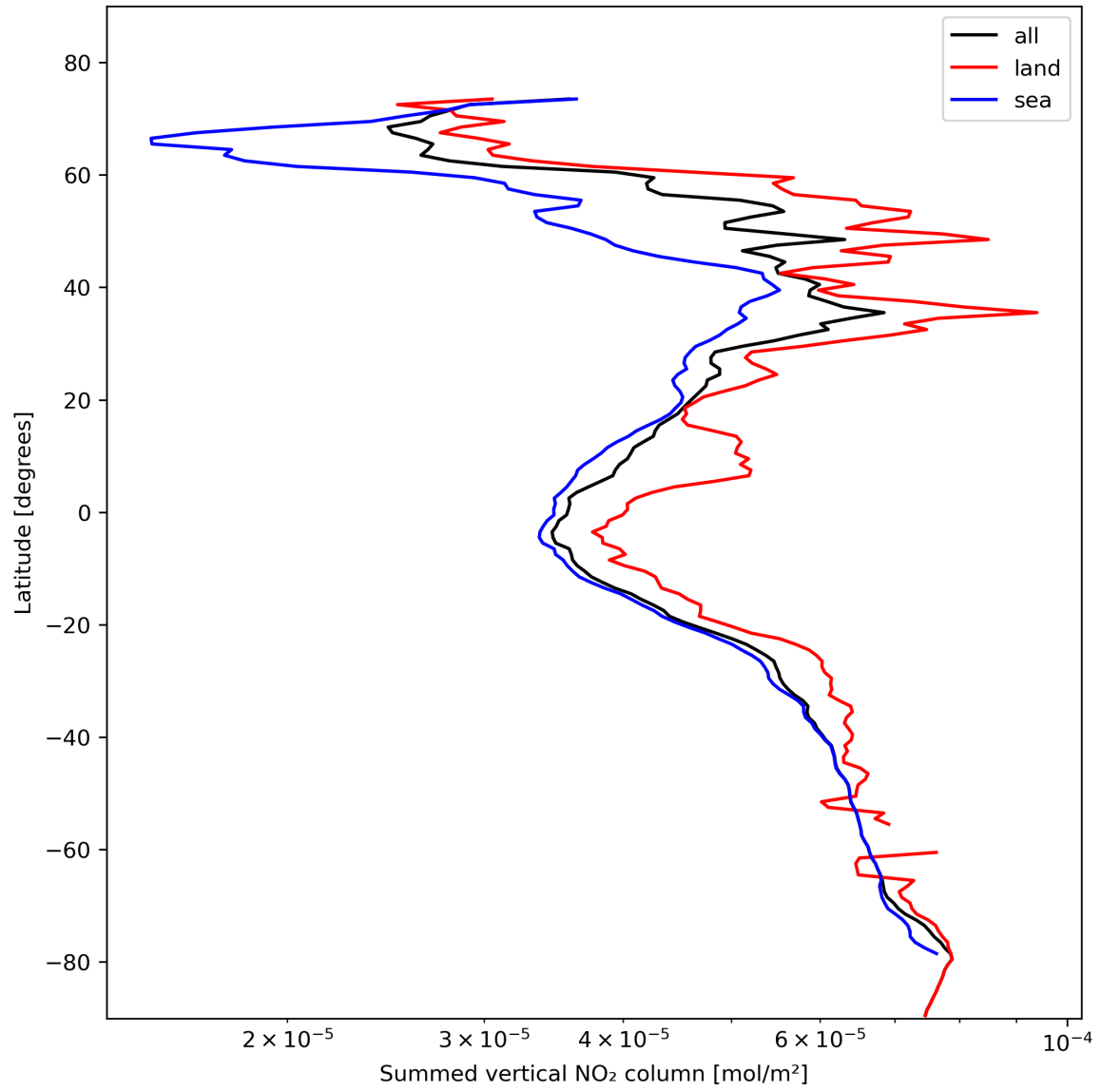
Figure 23: Zonal average of “Summed vertical NO 2 column” for 2024-02-09 to 2024-02-11.
