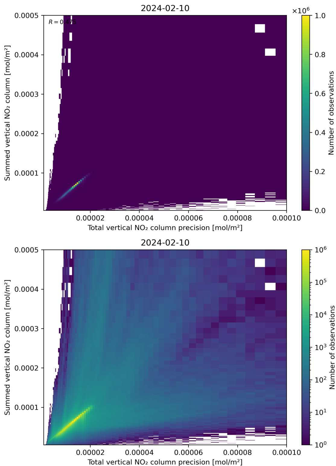
Figure 117: Scatter density plot of “Total vertical NO 2 column precision” against “Summed vertical NO 2 column” for 2024-02-09 to 2024-02-11.
