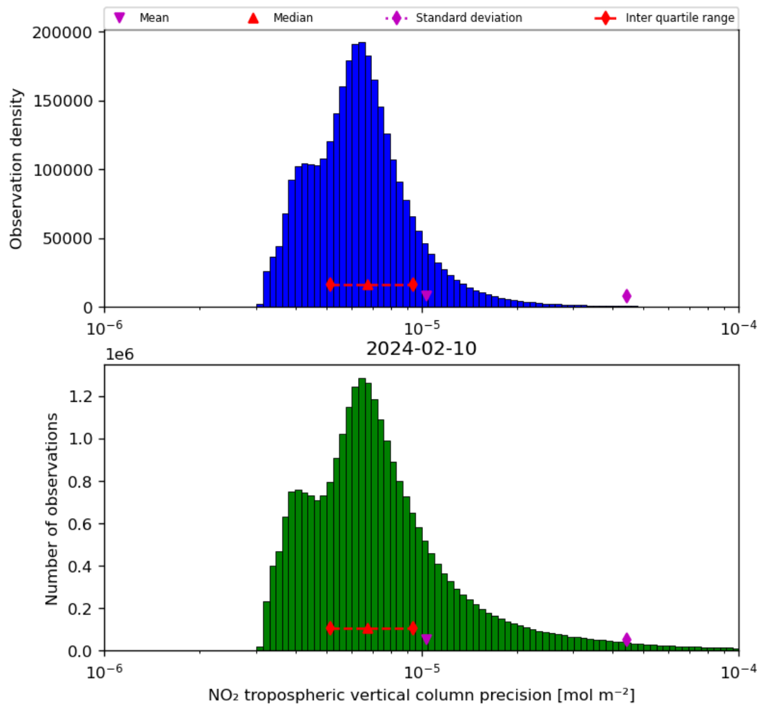
Figure 30: Histogram of “NO 2 tropospheric vertical column precision” for 2024-02-09 to 2024-02-11
