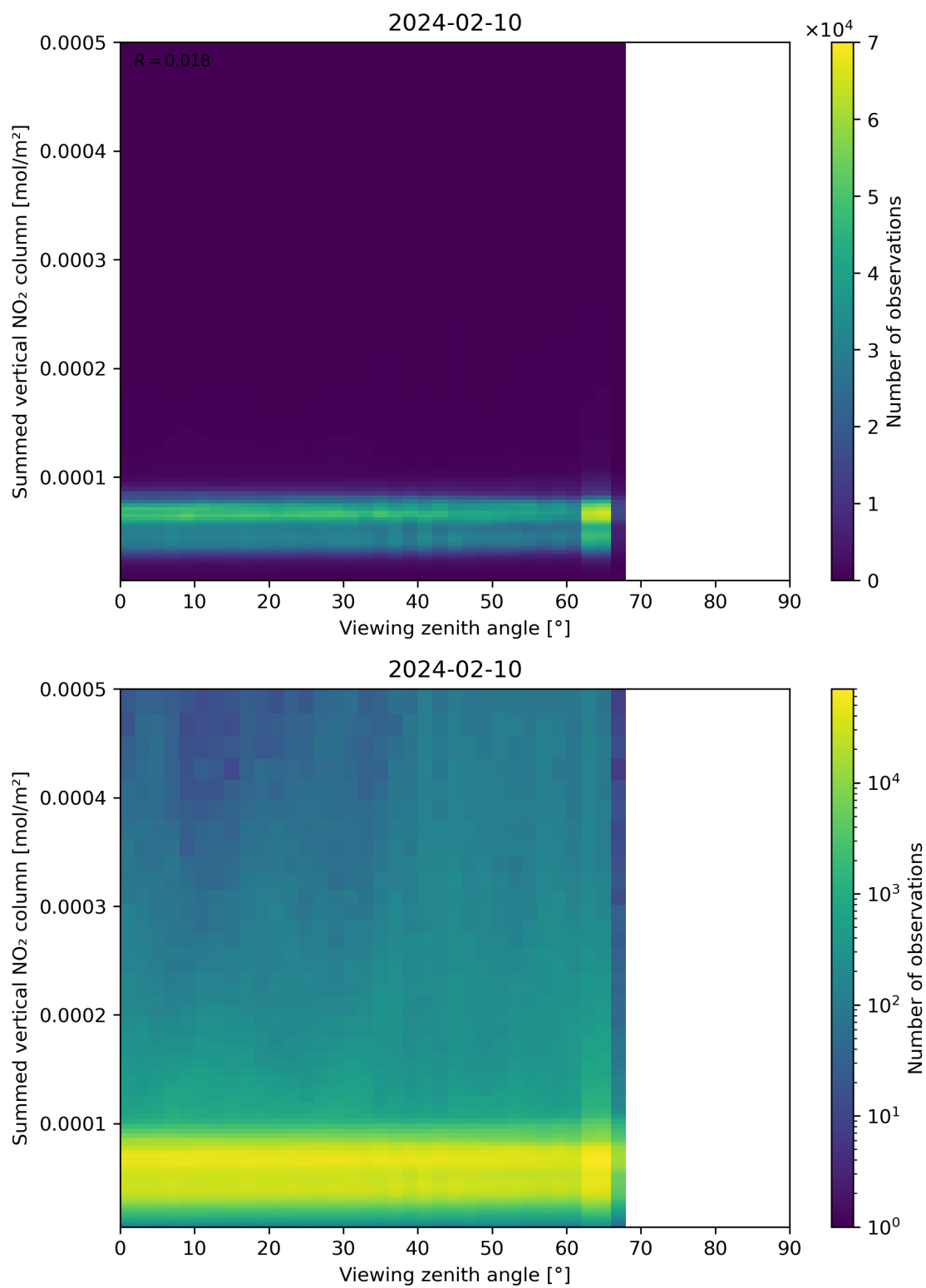
Figure 165: Scatter density plot of “Viewing zenith angle” against “Summed vertical NO 2 column” for 2024-02-09 to 2024-02-11.
