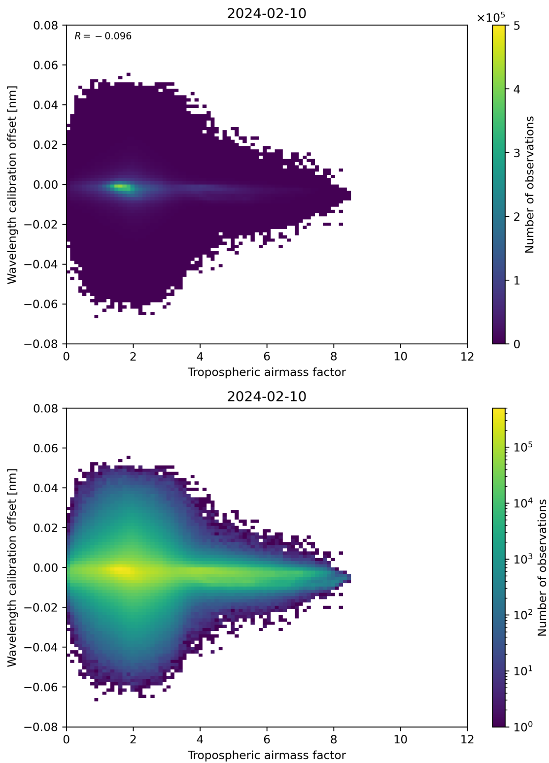
Figure 80: Scatter density plot of “Tropospheric air mass factor” against “Wavelength calibration offset” for 2024-02-09 to 2024-02-11.
