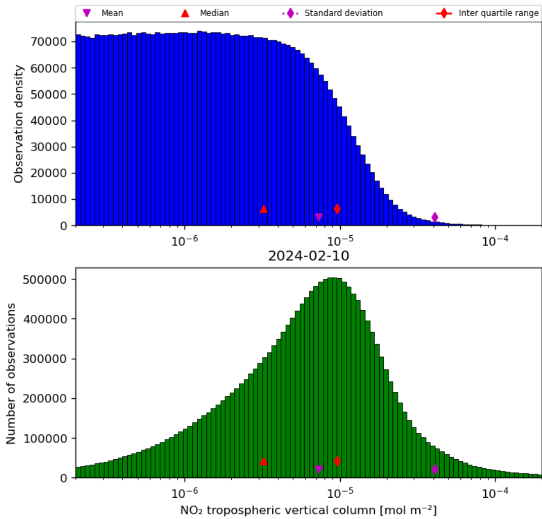
Figure 29: Histogram of “NO 2 tropospheric vertical column” for 2024-02-09 to 2024-02-11
