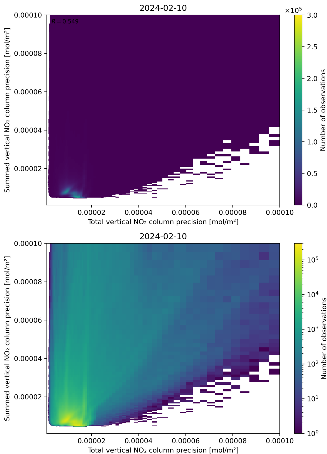
Figure 118: Scatter density plot of “Total vertical NO 2 column precision” against “Summed vertical NO 2 column precision” for 2024-02-09 to 2024-02-11.
