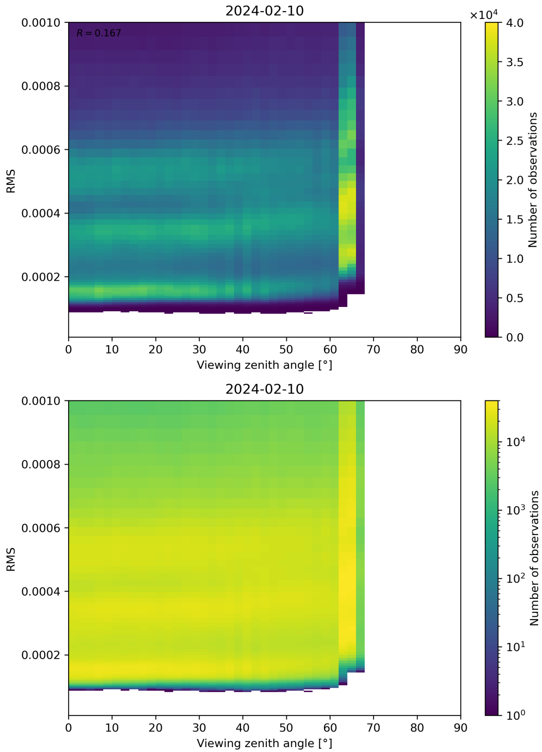
Figure 171: Scatter density plot of “Viewing zenith angle” against “RMS” for 2024-02-09 to 2024-02-11.
