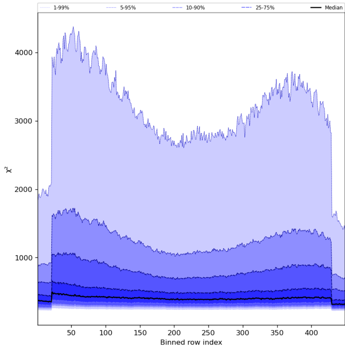
Figure 59: Along track statistics of “ \chi^2 ” for 2024-02-09 to 2024-02-11
