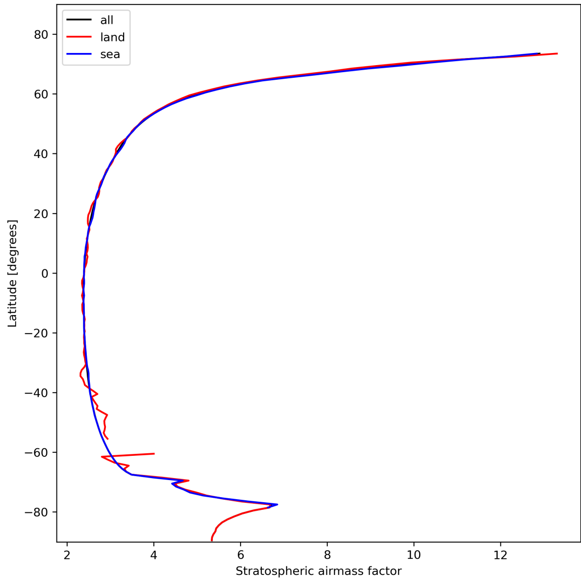
Figure 27: Zonal average of “Stratospheric air mass factor” for 2024-02-09 to 2024-02-11.
