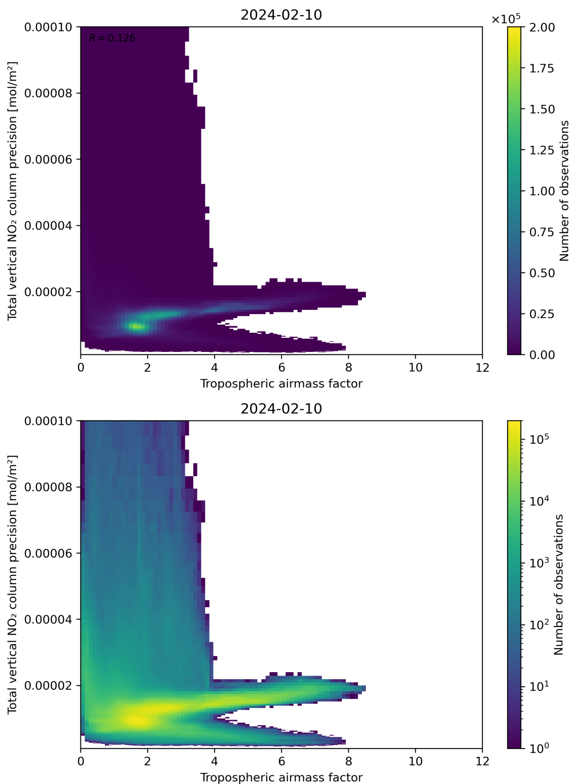
Figure 78: Scatter density plot of “Tropospheric air mass factor” against “Total vertical NO 2 column precision” for 2024-02-09 to 2024-02-11.
