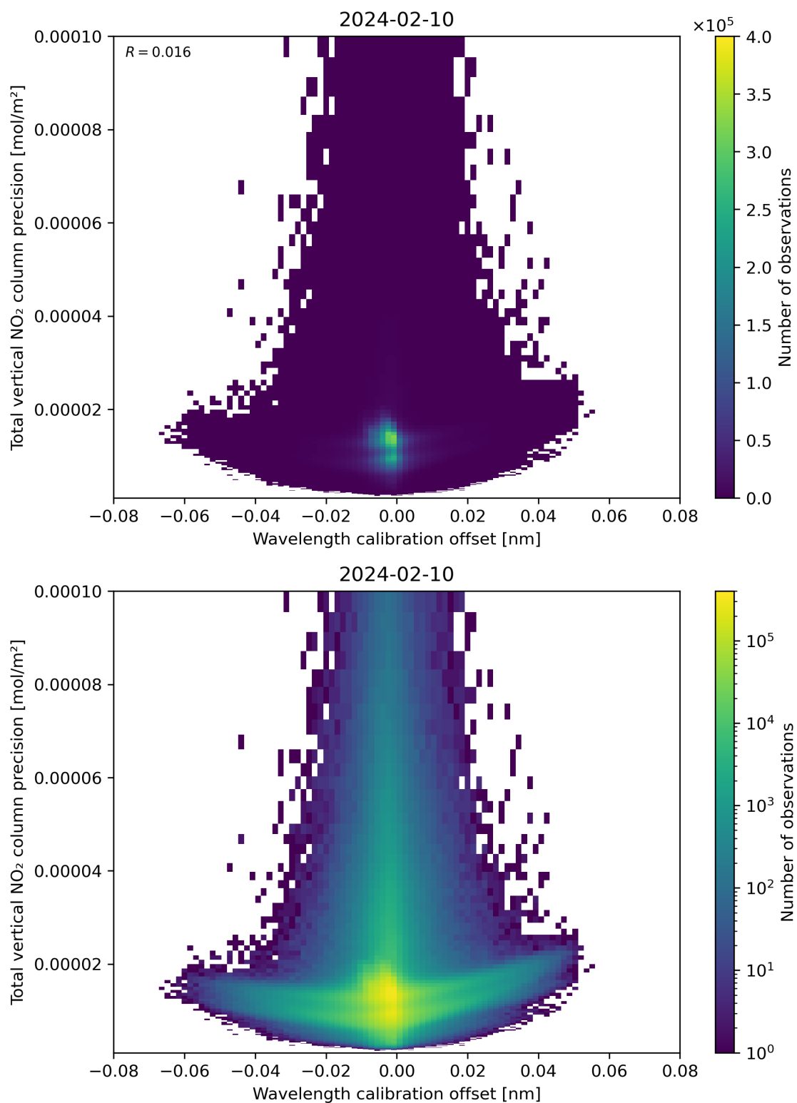
Figure 180: Scatter density plot of “Wavelength calibration offset” against “Total vertical NO 2 column precision” for 2024-02-09 to 2024-02-11.
