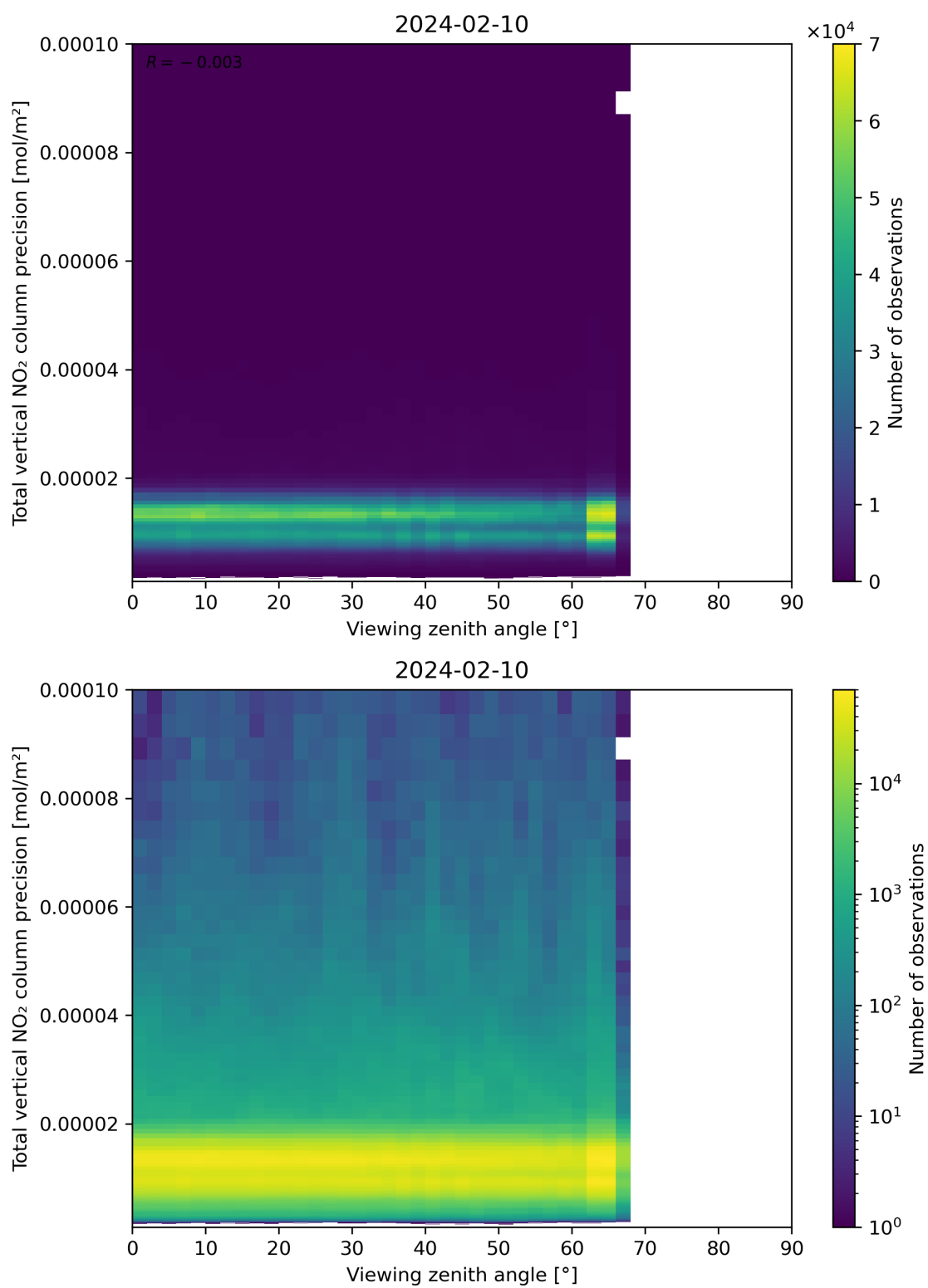
Figure 168: Scatter density plot of “Viewing zenith angle” against “Total vertical NO 2 column precision” for 2024-02-09 to 2024-02-11.
