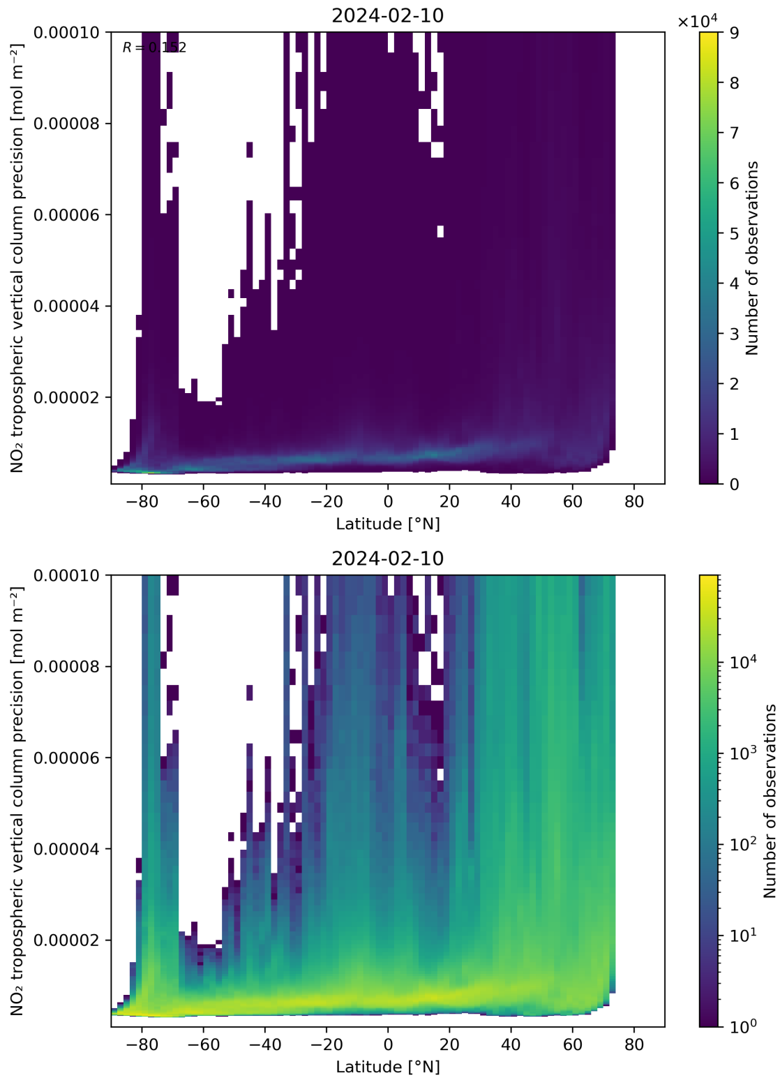
Figure 93: Scatter density plot of “Latitude” against “NO 2 tropospheric vertical column precision” for 2024-02-09 to 2024-02-11.
