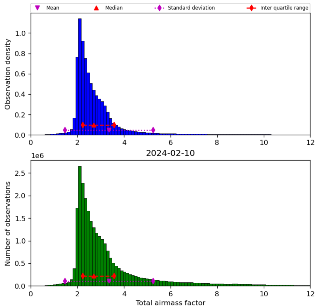
Figure 32: Histogram of “Total airmass factor” for 2024-02-09 to 2024-02-11
