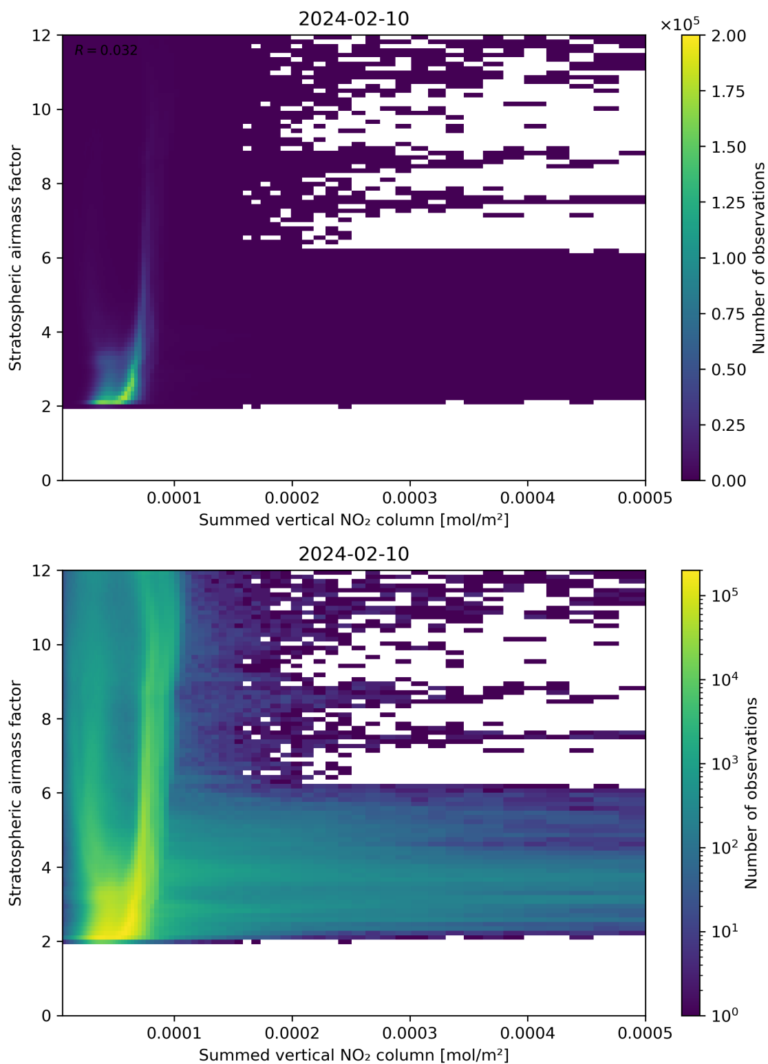
Figure 103: Scatter density plot of “Summed vertical NO 2 column” against “Stratospheric airmass factor” for 2024-02-09 to 2024-02-11.
