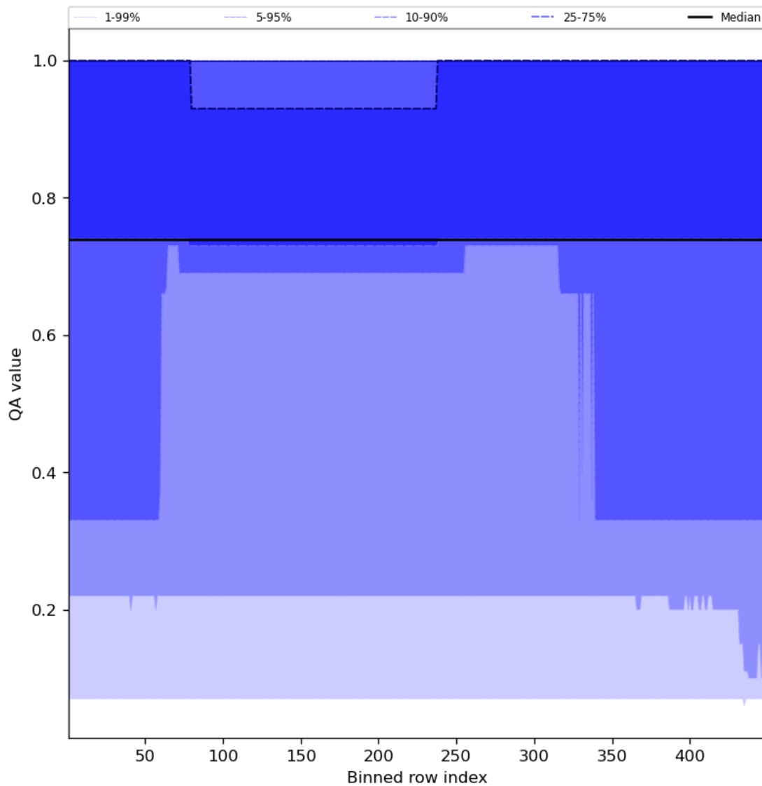
Figure 45: Along track statistics of “QA value” for 2024-02-09 to 2024-02-11
