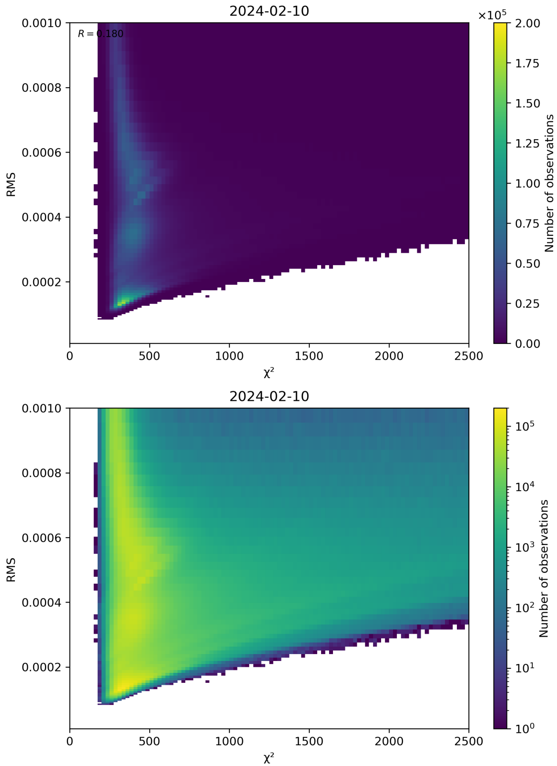
Figure 82: Scatter density plot of “ \chi^2 ” against “RMS” for 2024-02-09 to 2024-02-11.
