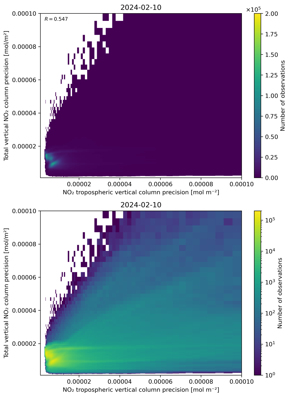
Figure 139: Scatter density plot of “NO 2 tropospheric vertical column precision” against “Total vertical NO 2 column precision” for 2024-02-09 to 2024-02-11.
