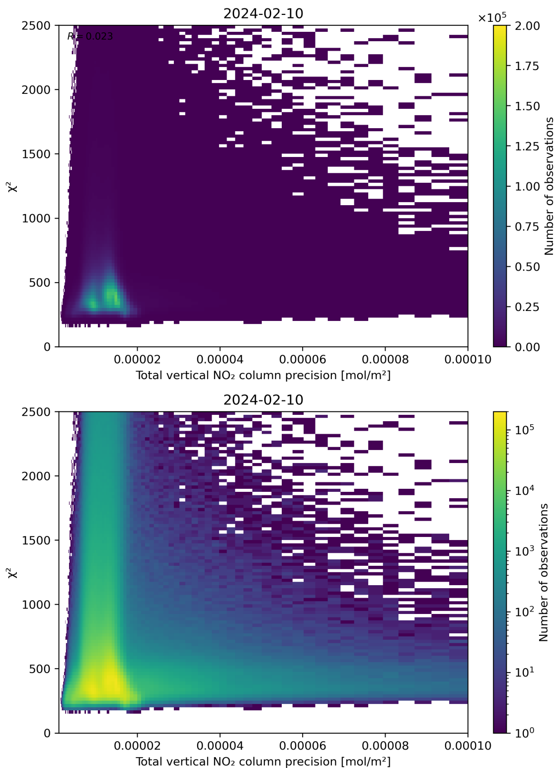
Figure 116: Scatter density plot of “Total vertical NO 2 column precision” against “ \chi^2 ” for 2024-02-09 to 2024-02-11.
