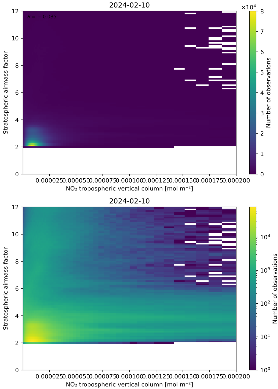
Figure 121: Scatter density plot of “NO 2 tropospheric vertical column” against “Stratospheric air mass factor” for 2024-02-09 to 2024-02-11.
