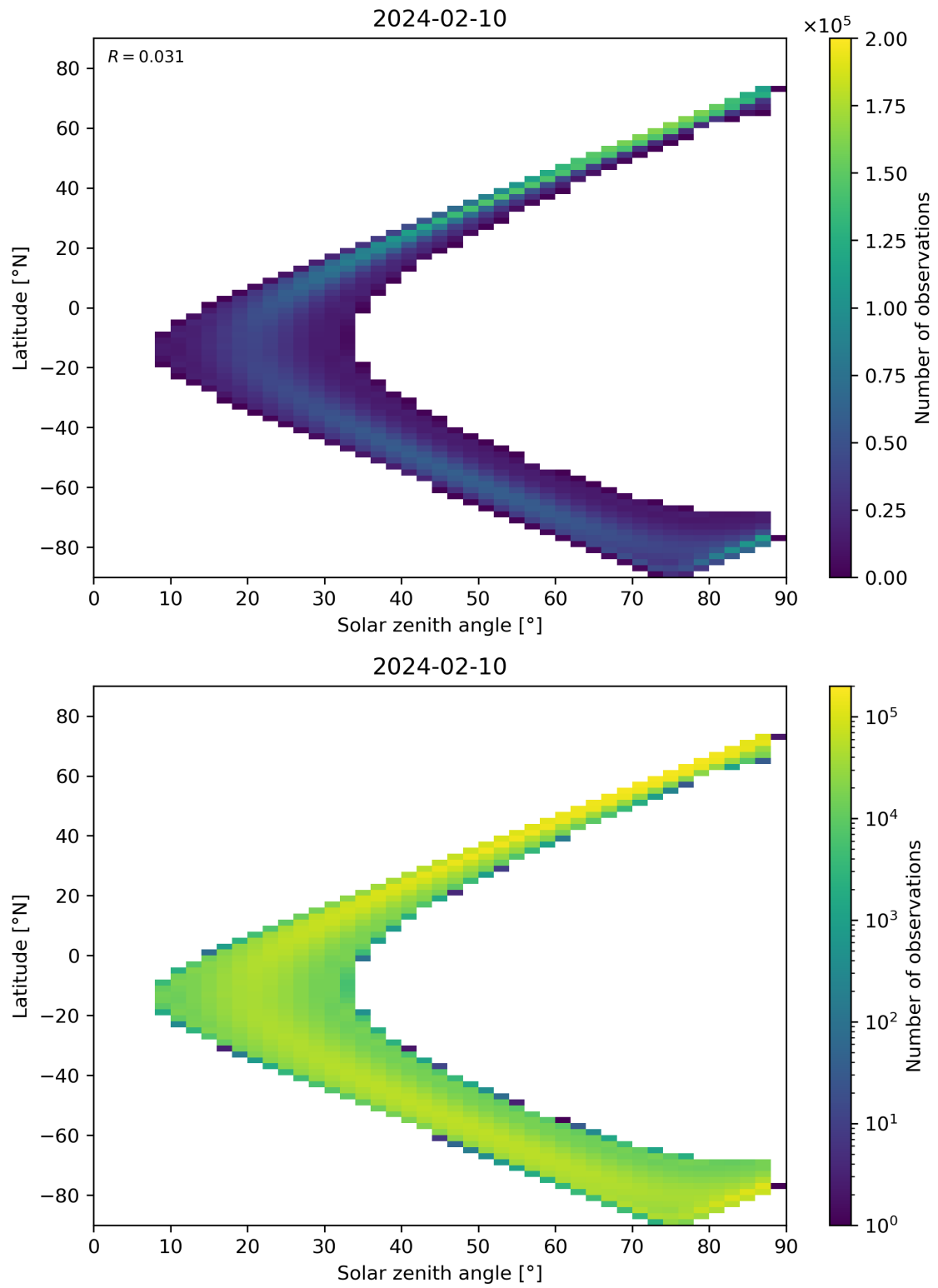
Figure 149: Scatter density plot of “Solar zenith angle” against “Latitude” for 2024-02-09 to 2024-02-11.
