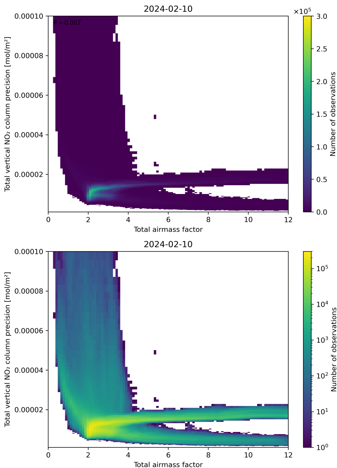
Figure 68: Scatter density plot of “Total airmass factor” against “Total vertical NO 2 column precision” for 2024-02-09 to 2024-02-11.
