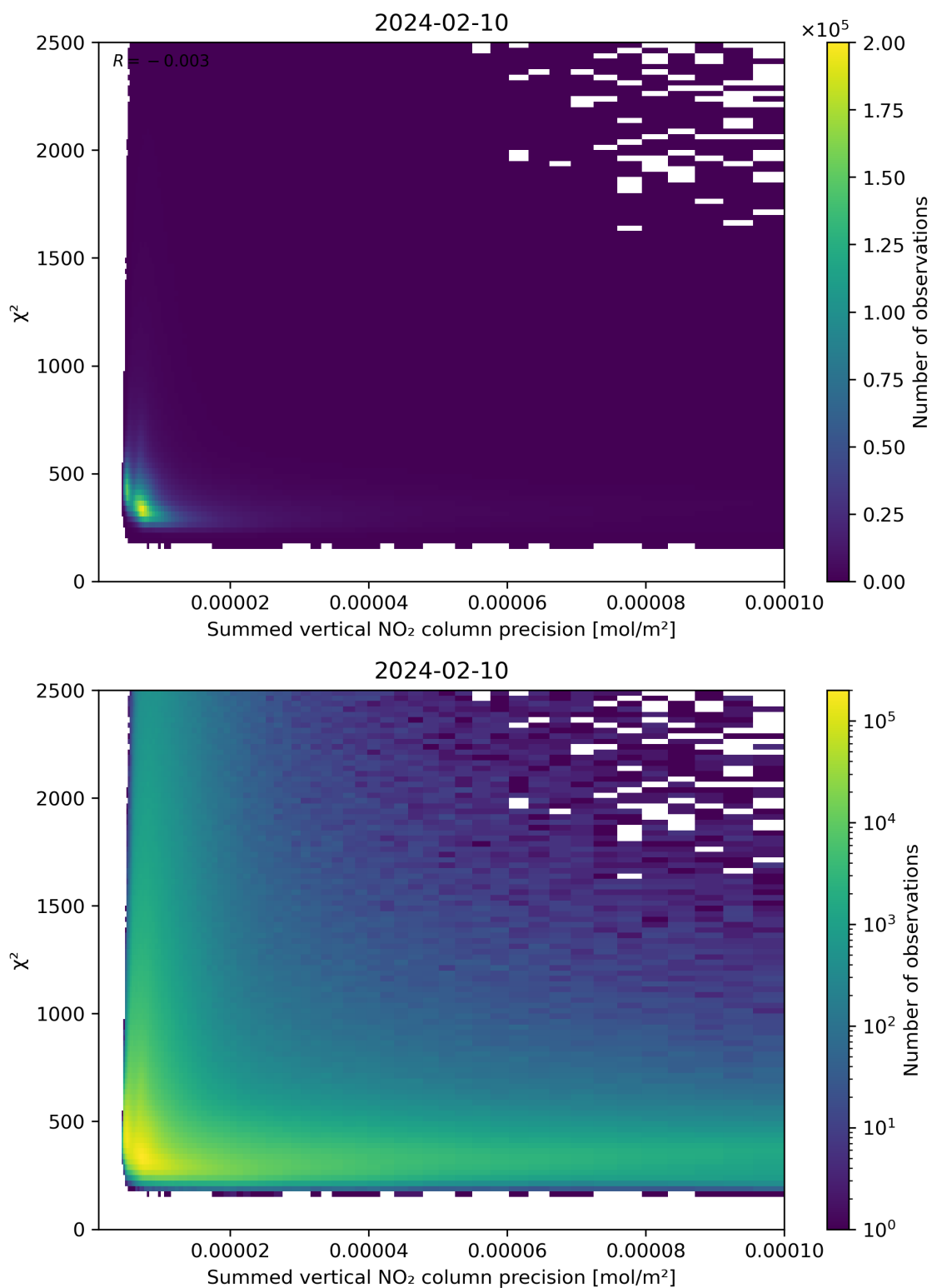
Figure 107: Scatter density plot of “Summed vertical NO 2 column precision” against “ \chi^2 ” for 2024-02-09 to 2024-02-11.
