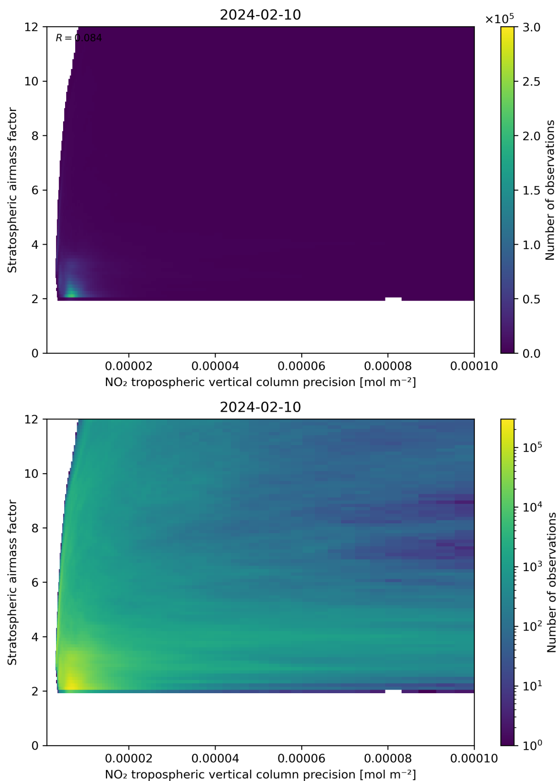
Figure 131: Scatter density plot of “NO 2 tropospheric vertical column precision” against “Stratospheric airmass factor” for 2024-02-09 to 2024-02-11.
