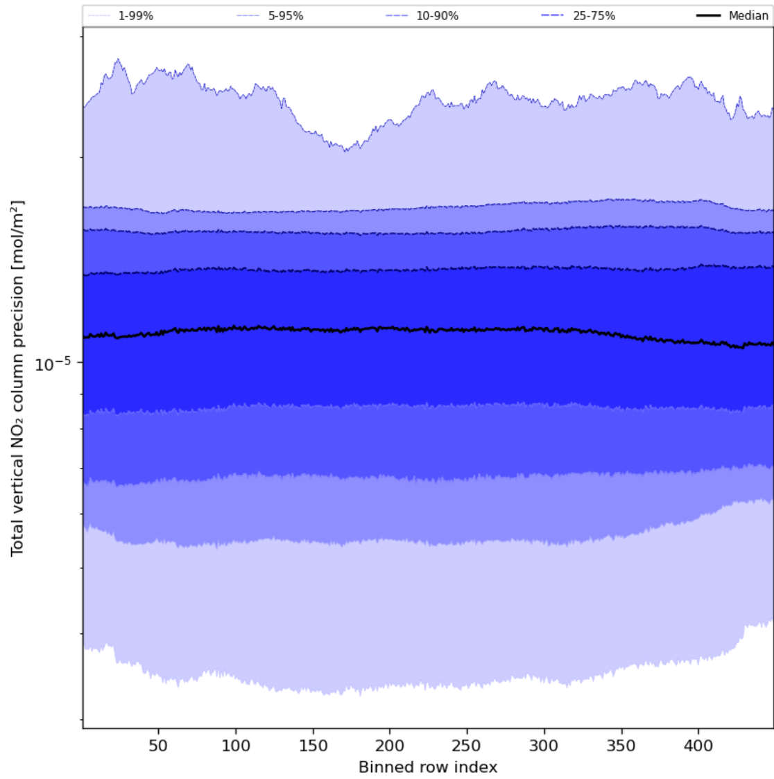
Figure 56: Along track statistics of “Total vertical NO 2 column precision” for 2024-02-09 to 2024-02-11
