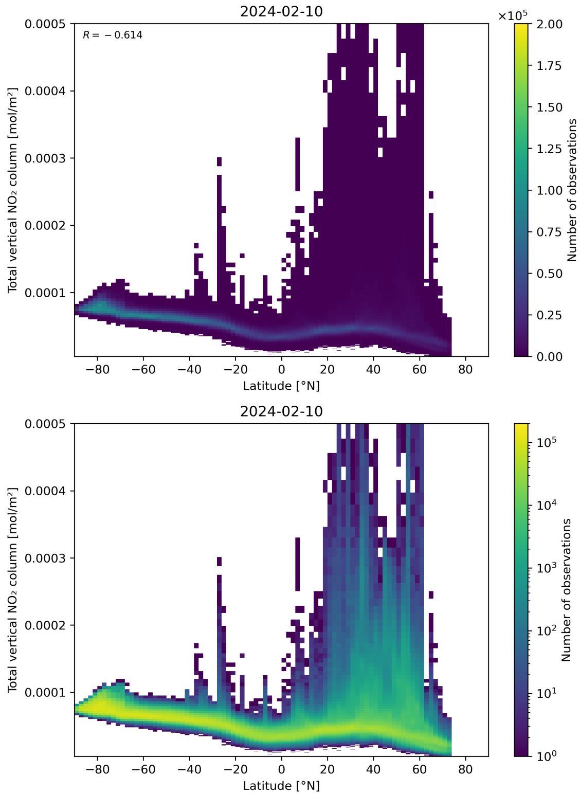
Figure 90: Scatter density plot of “Latitude” against “Total vertical NO 2 column” for 2024-02-09 to 2024-02-11.
