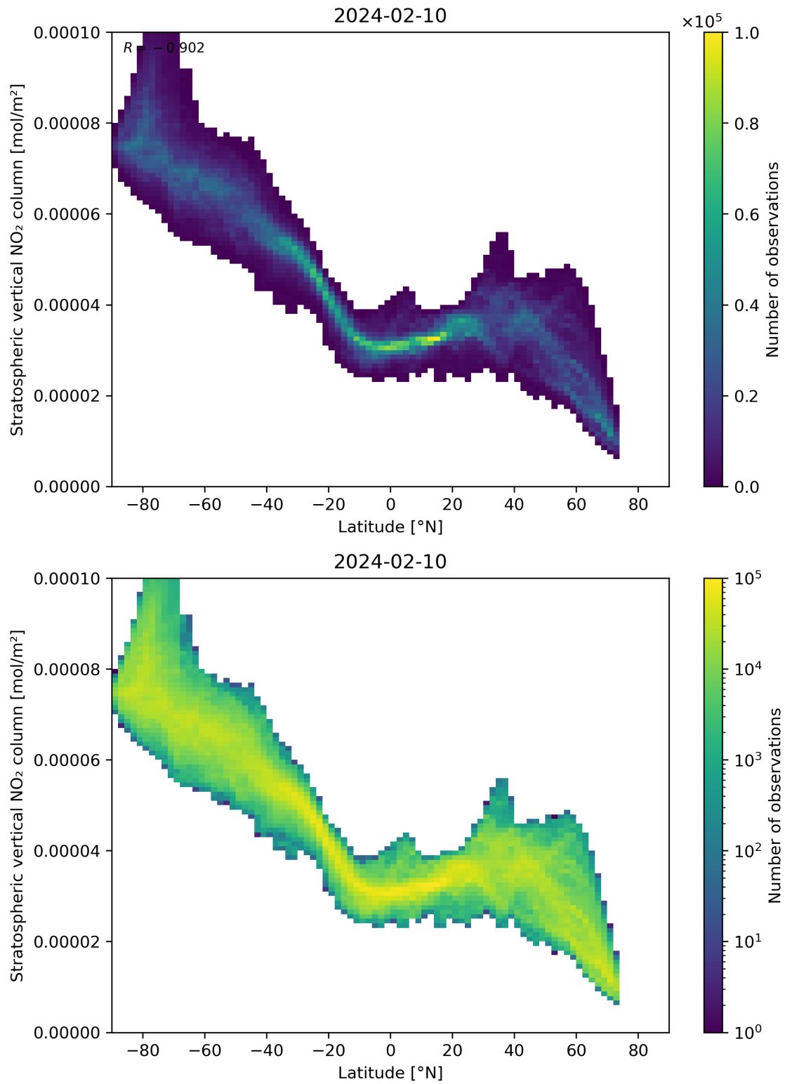
Figure 87: Scatter density plot of “Latitude” against “Stratospheric vertical NO 2 column” for 2024-02-09 to 2024-02-11.
