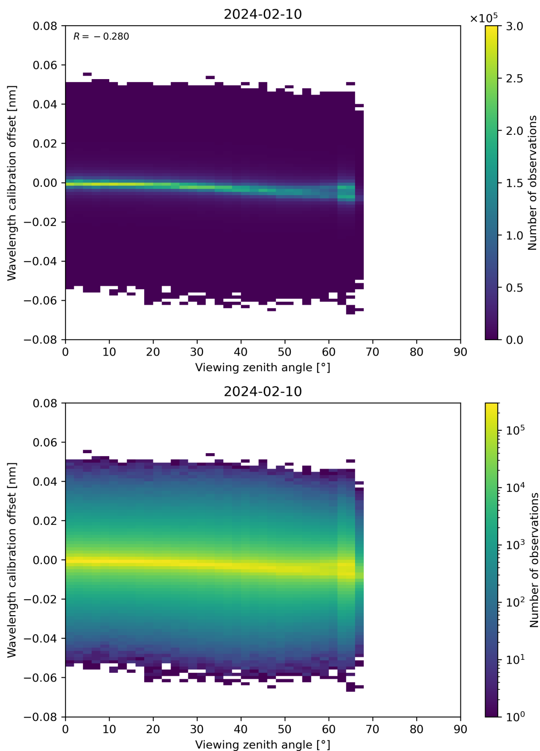
Figure 173: Scatter density plot of “Viewing zenith angle” against “Wavelength calibration offset” for 2024-02-09 to 2024-02-11.
