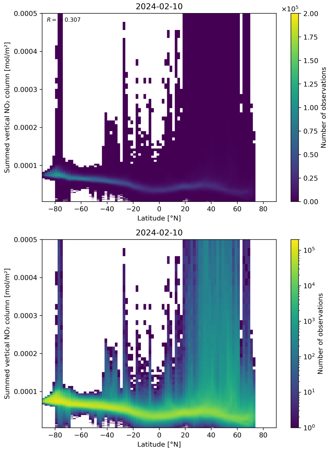
Figure 88: Scatter density plot of “Latitude” against “Summed vertical NO 2 column” for 2024-02-09 to 2024-02-11.
