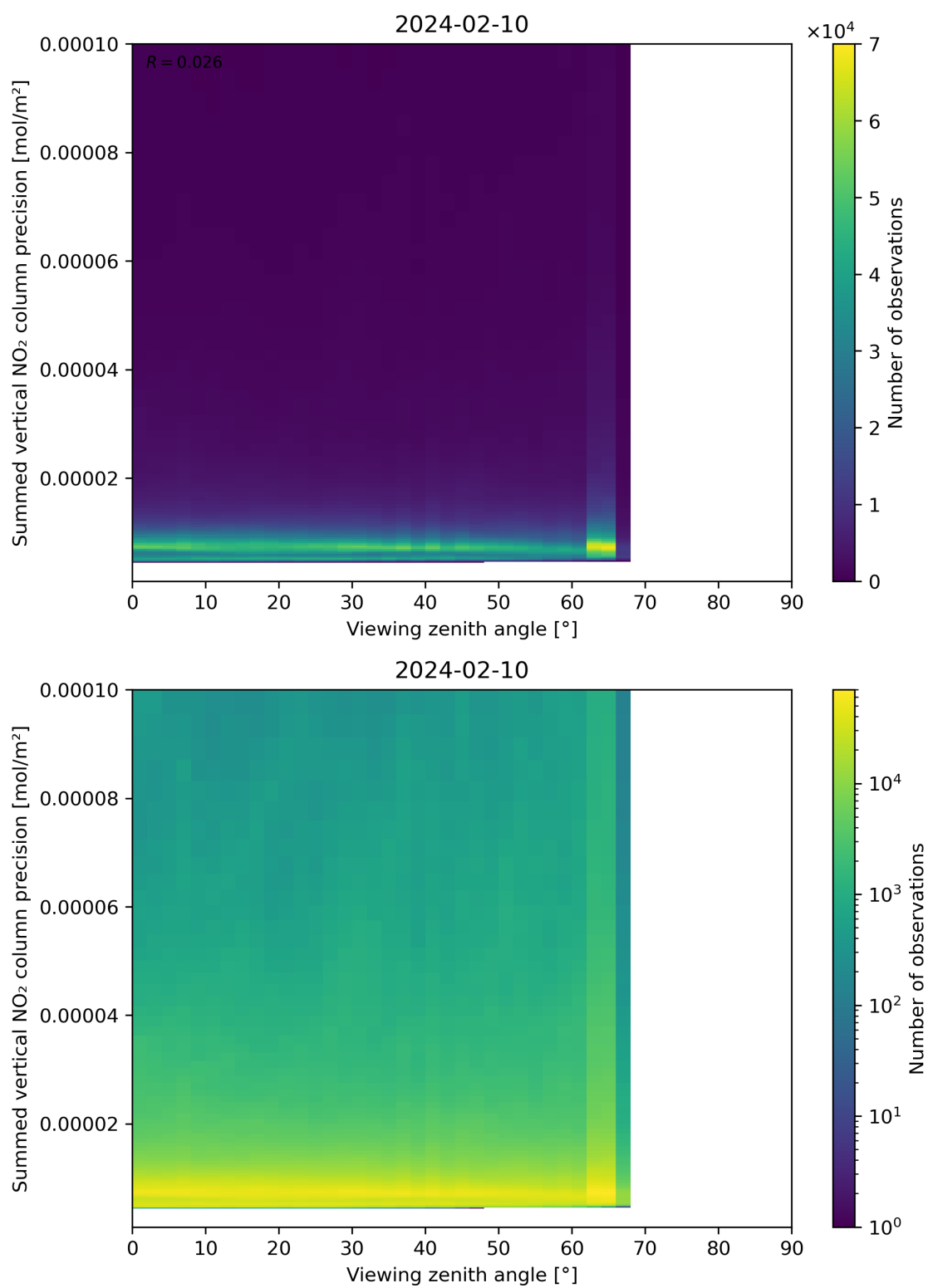
Figure 166: Scatter density plot of “Viewing zenith angle” against “Summed vertical NO 2 column precision” for 2024-02-09 to 2024-02-11.
