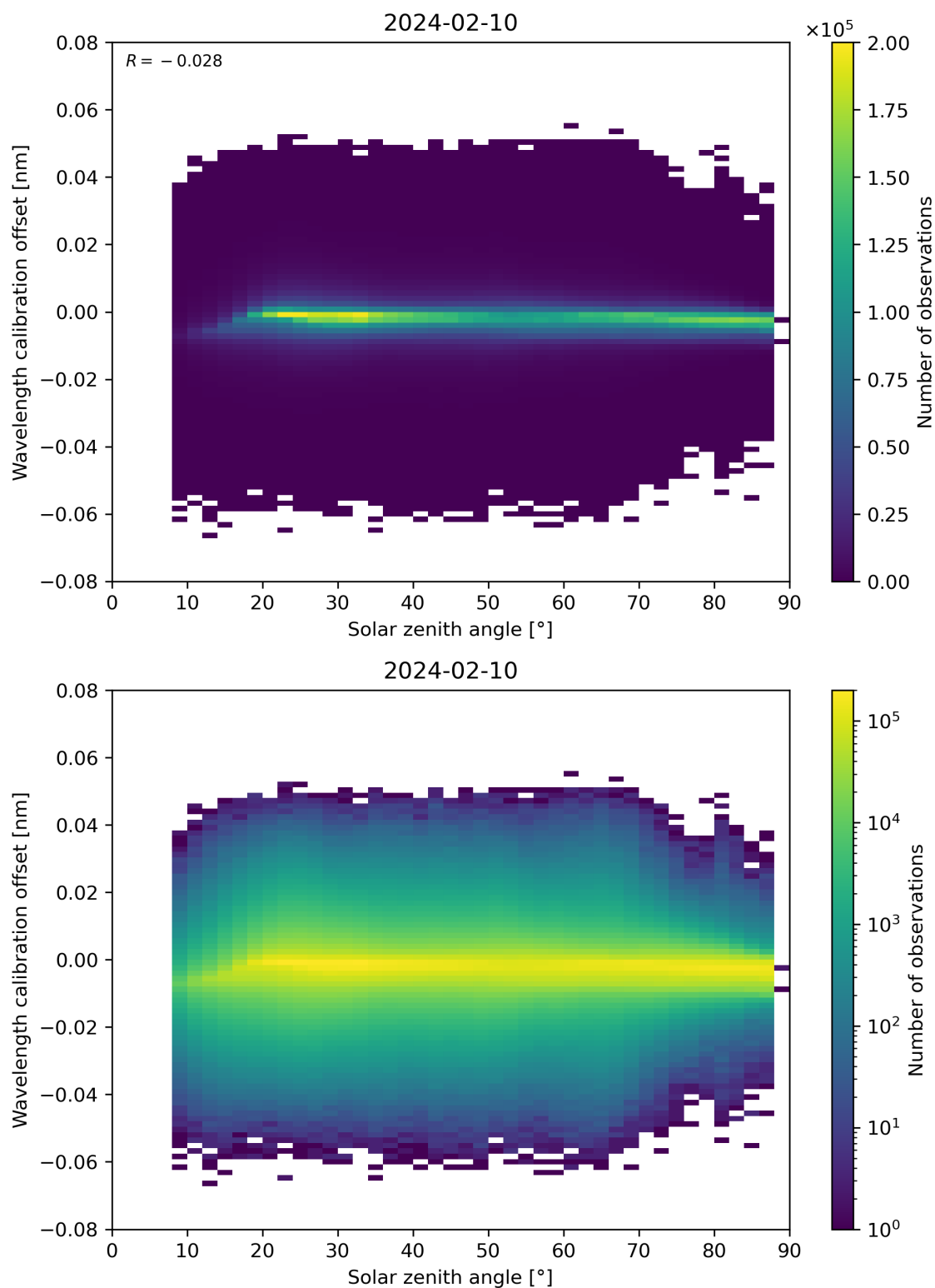
Figure 158: Scatter density plot of “Solar zenith angle” against “Wavelength calibration offset” for 2024-02-09 to 2024-02-11.
