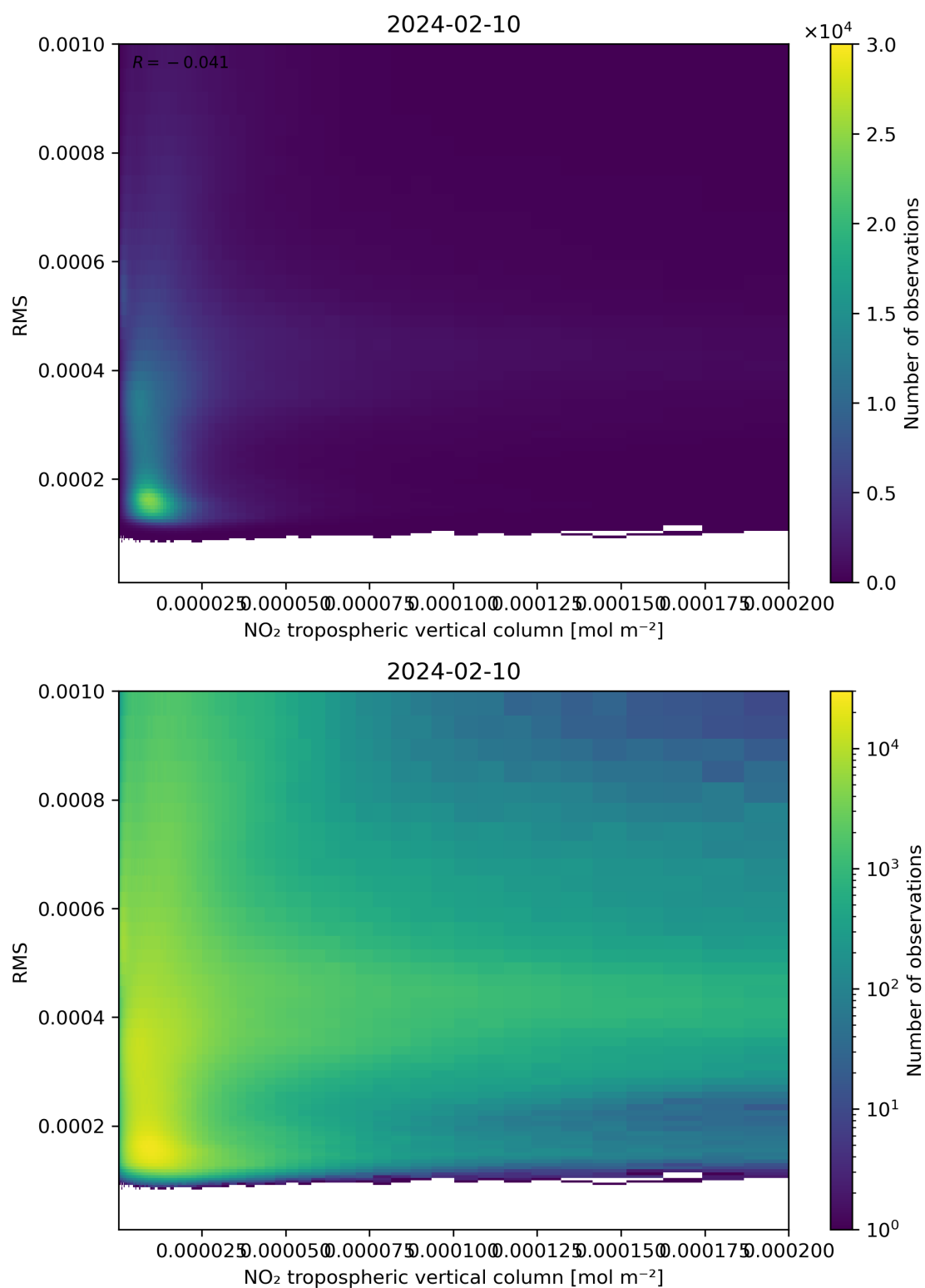
Figure 142: Scatter density plot of “NO 2 tropospheric vertical column” against “RMS” for 2024-02-09 to 2024-02-11.
