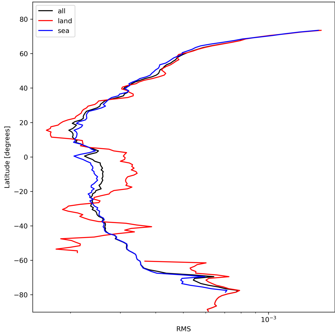
Figure 26: Zonal average of “RMS” for 2024-02-09 to 2024-02-11.
