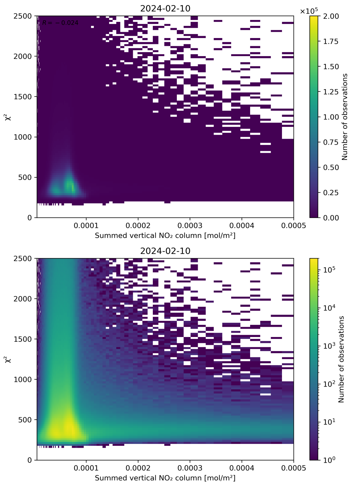
Figure 104: Scatter density plot of “Summed vertical NO 2 column” against “ \chi^2 ” for 2024-02-09 to 2024-02-11.
