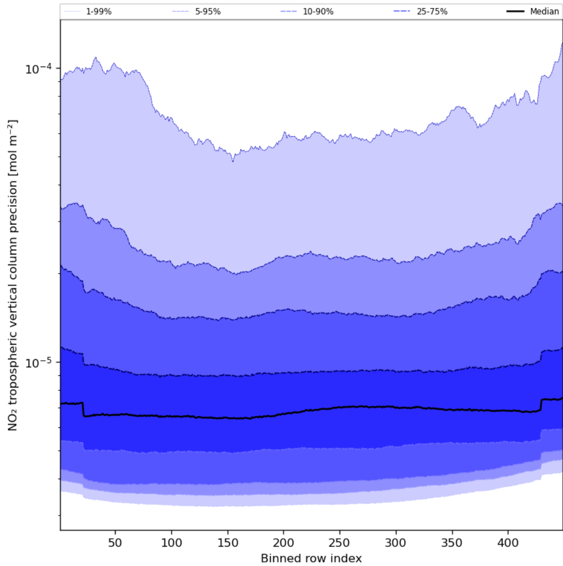
Figure 47: Along track statistics of “NO 2 tropospheric vertical column precision” for 2024-02-09 to 2024-02-11
