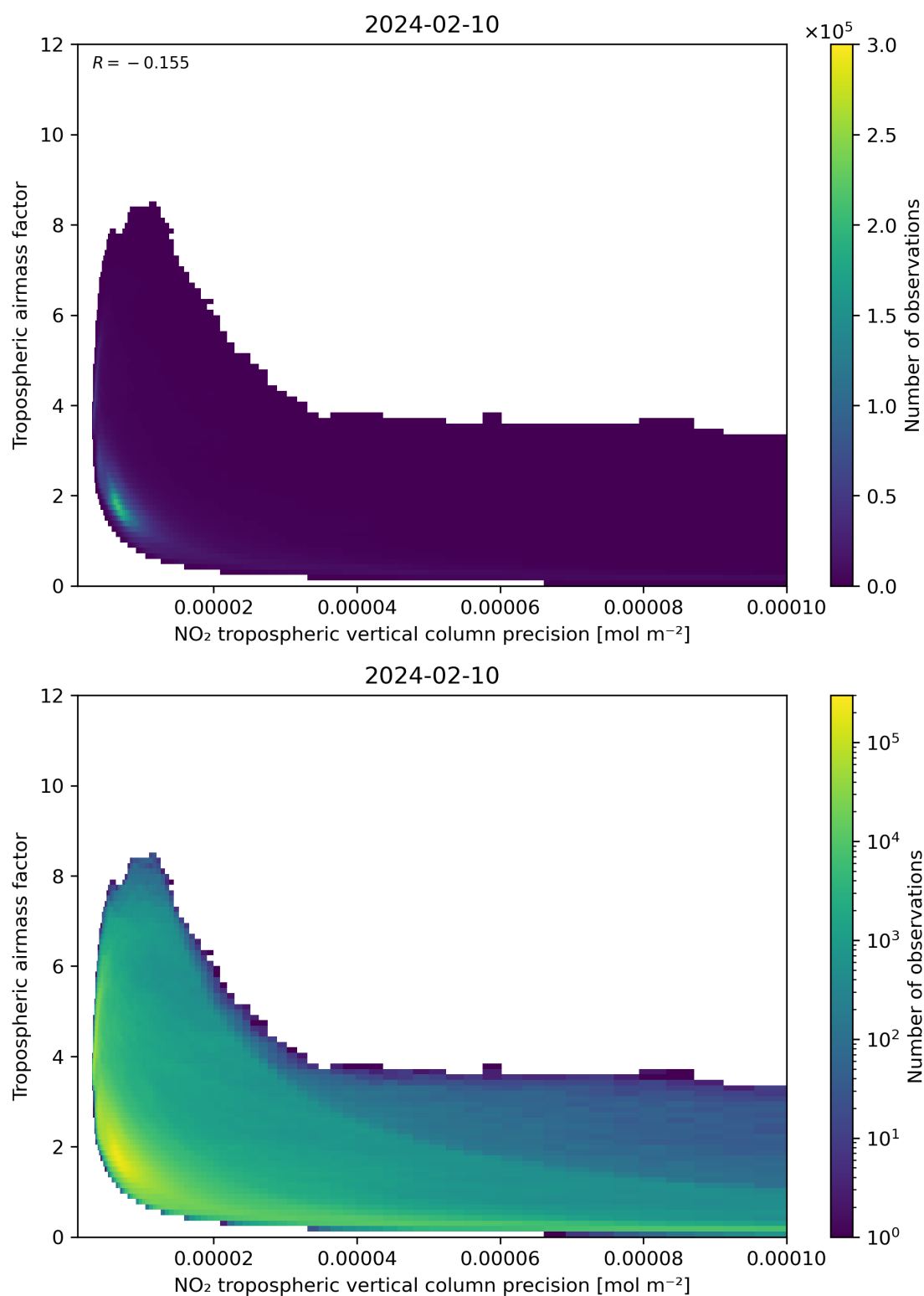
Figure 133: Scatter density plot of “NO 2 tropospheric vertical column precision” against “Tropospheric airmass factor” for 2024-02-09 to 2024-02-11.
