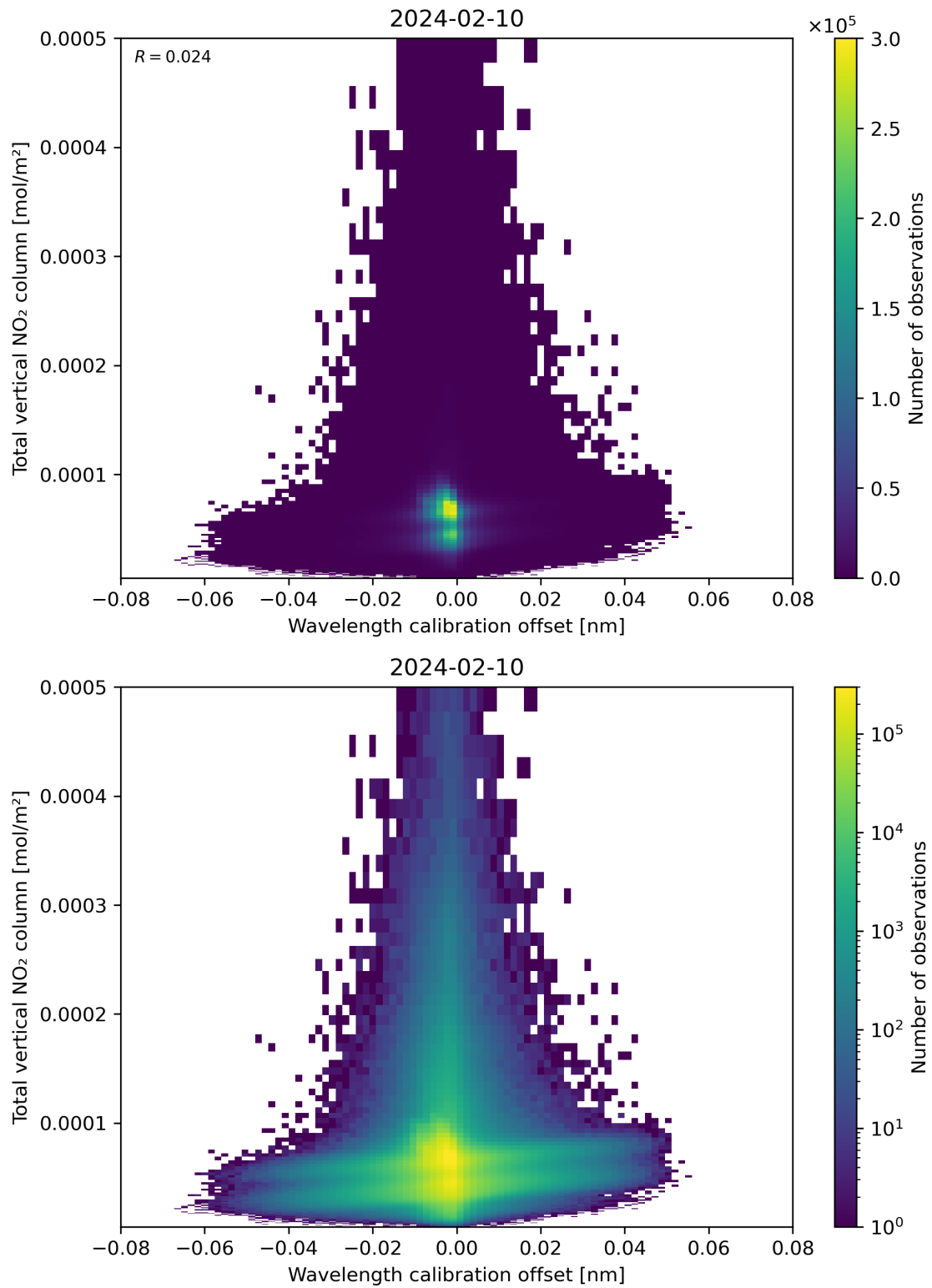
Figure 179: Scatter density plot of “Wavelength calibration offset” against “Total vertical NO 2 column” for 2024-02-09 to 2024-02-11.
