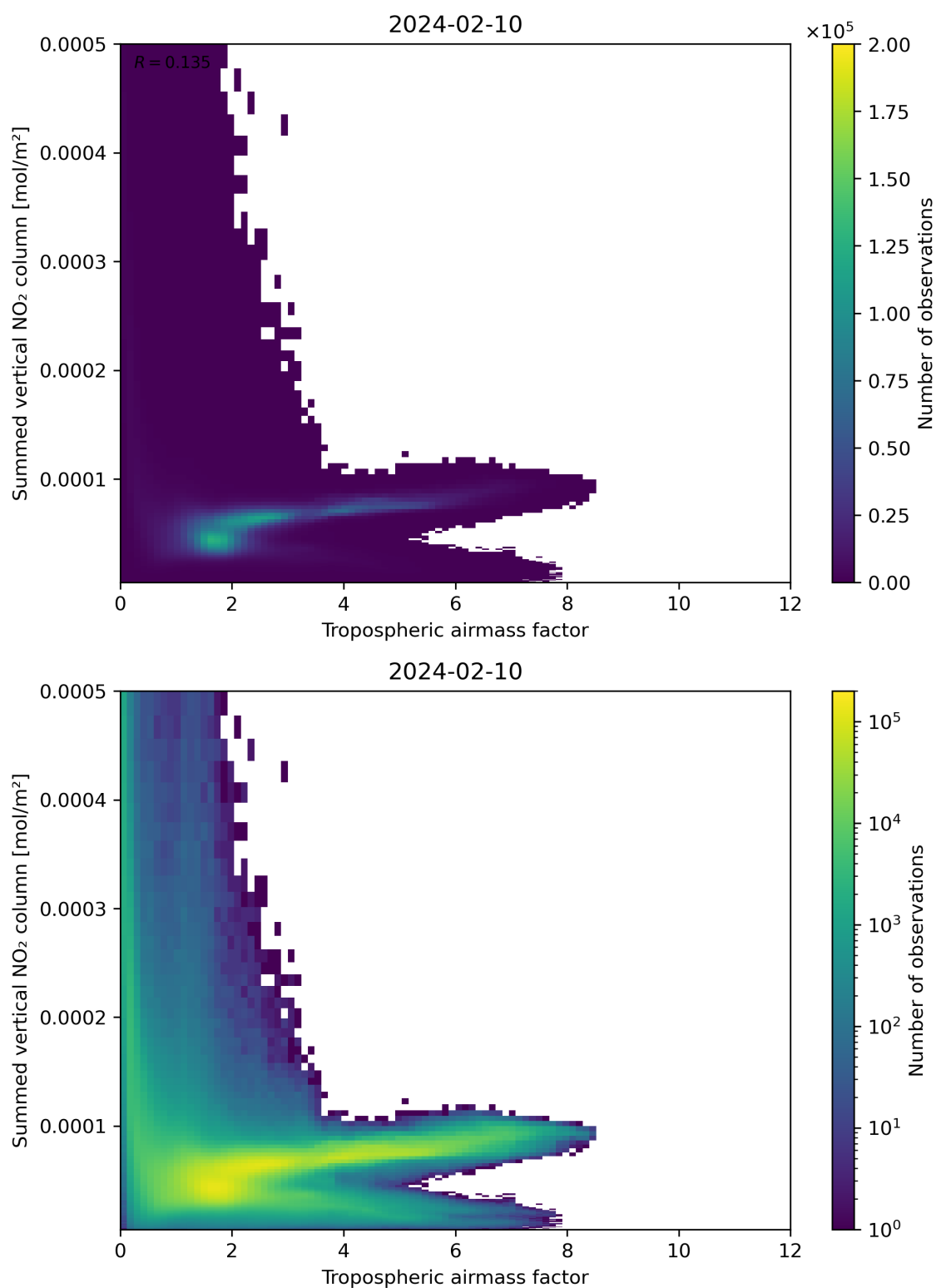
Figure 75: Scatter density plot of “Tropospheric airmass factor” against “Summed vertical NO 2 column” for 2024-02-09 to 2024-02-11.
