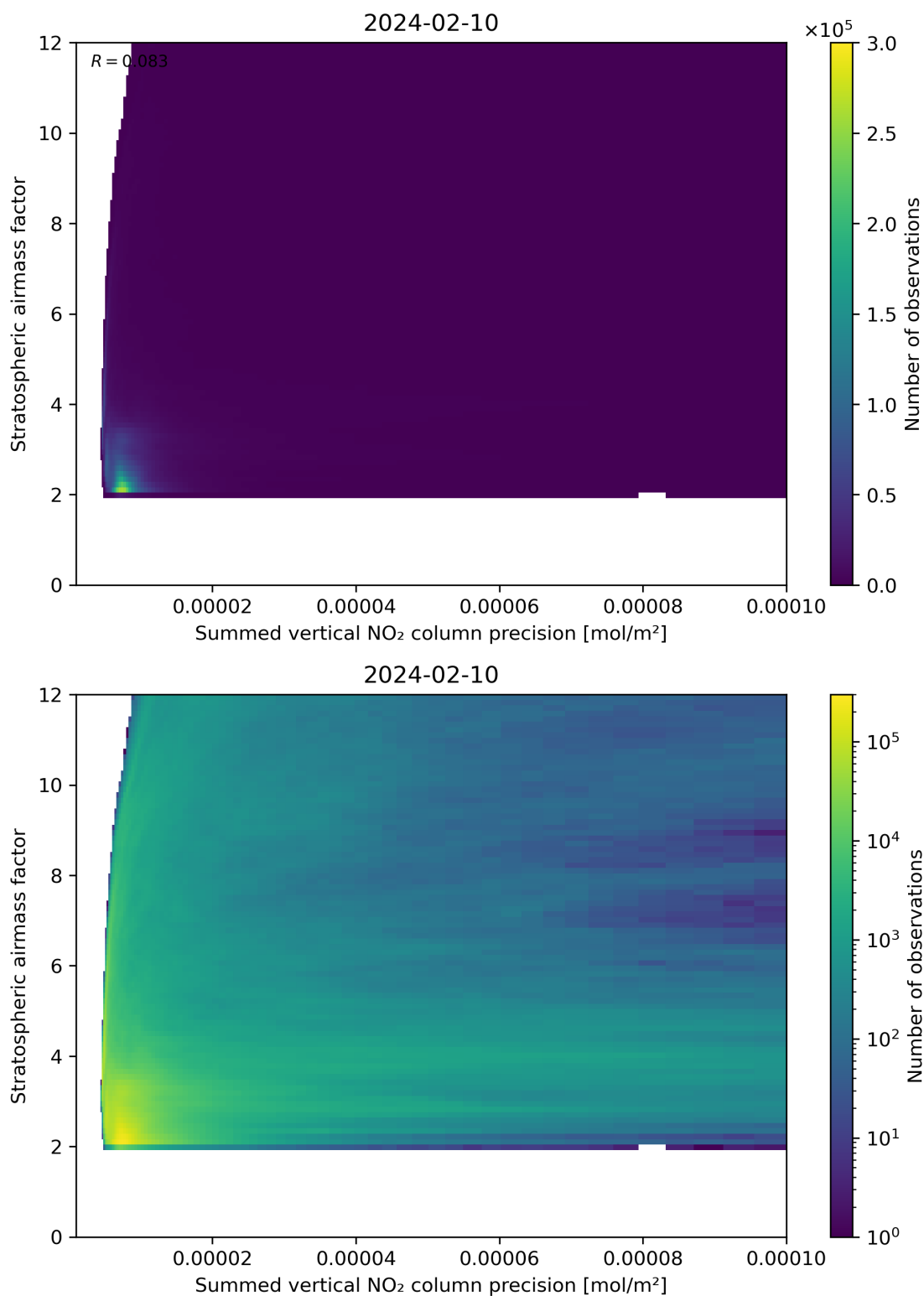
Figure 106: Scatter density plot of “Summed vertical NO 2 column precision” against “Stratospheric airmass factor” for 2024-02-09 to 2024-02-11.
