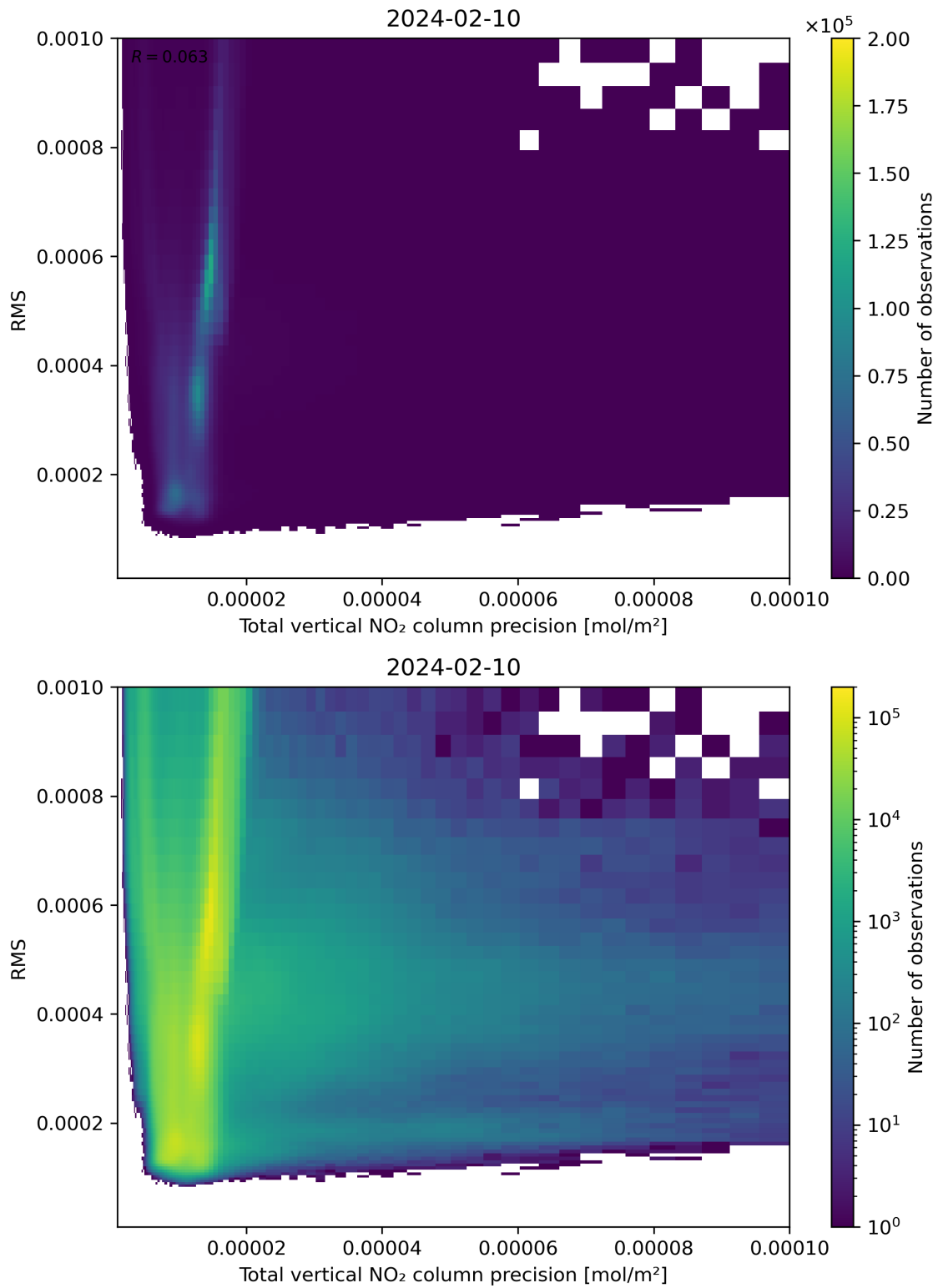
Figure 119: Scatter density plot of “Total vertical NO 2 column precision” against “RMS” for 2024-02-09 to 2024-02-11.
