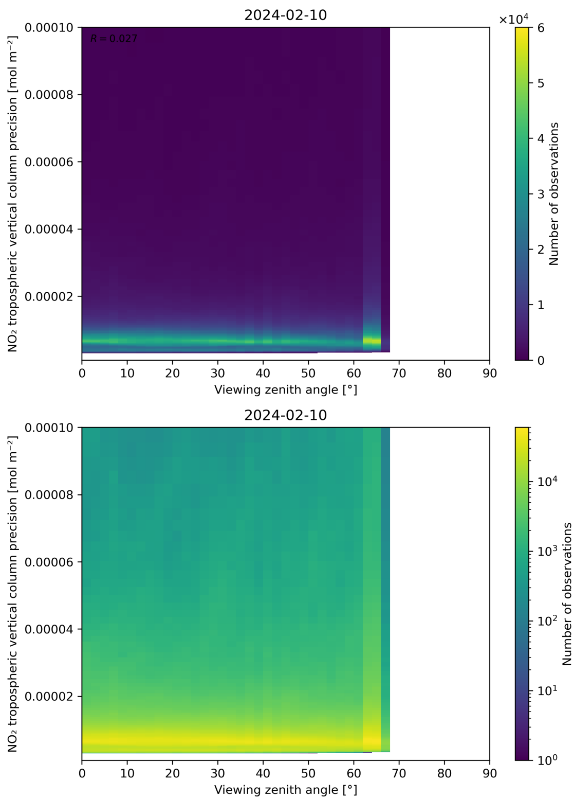
Figure 170: Scatter density plot of “Viewing zenith angle” against “NO 2 tropospheric vertical column precision” for 2024-02-09 to 2024-02-11.
