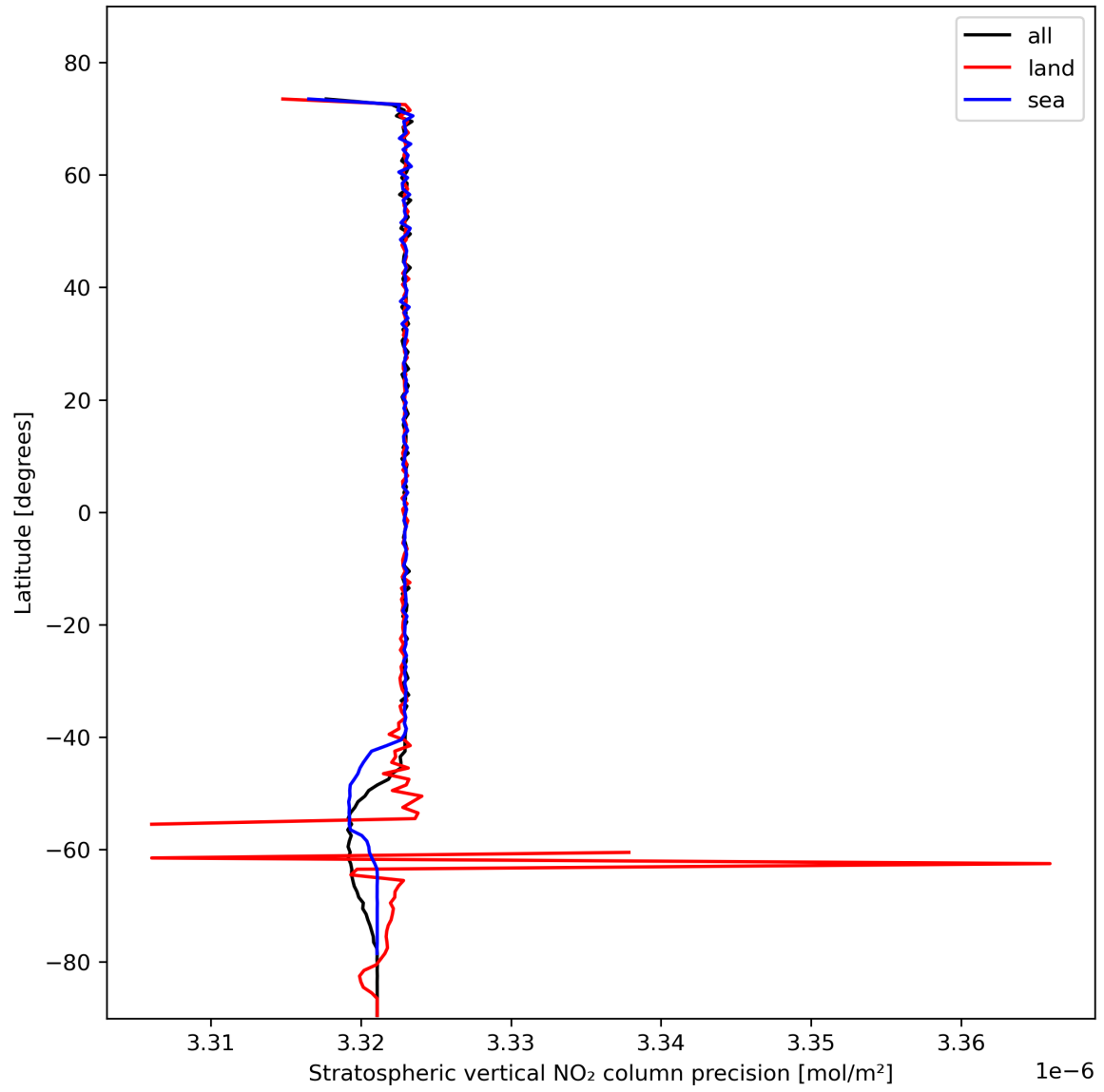
Figure 20: Zonal average of "Stratospheric vertical NO 2 column precision" for 2024-02-09 to 2024-02-11.
