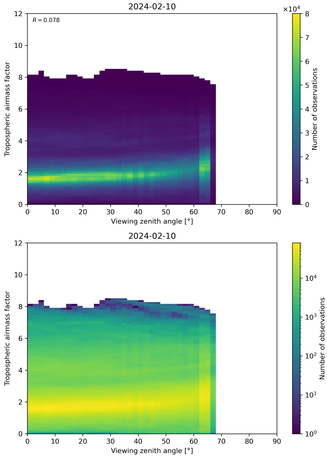
Figure 161: Scatter density plot of “Viewing zenith angle” against “Tropospheric airmass factor” for 2024-02-09 to 2024-02-11.
