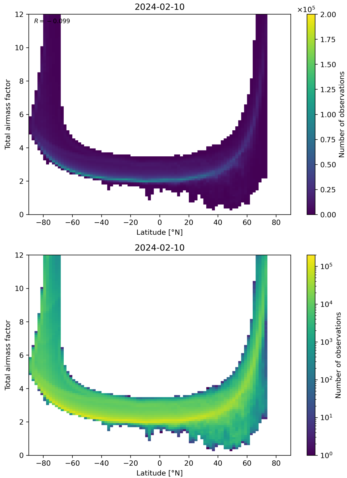
Figure 84: Scatter density plot of “Latitude” against “Total airmass factor” for 2024-02-09 to 2024-02-11.
