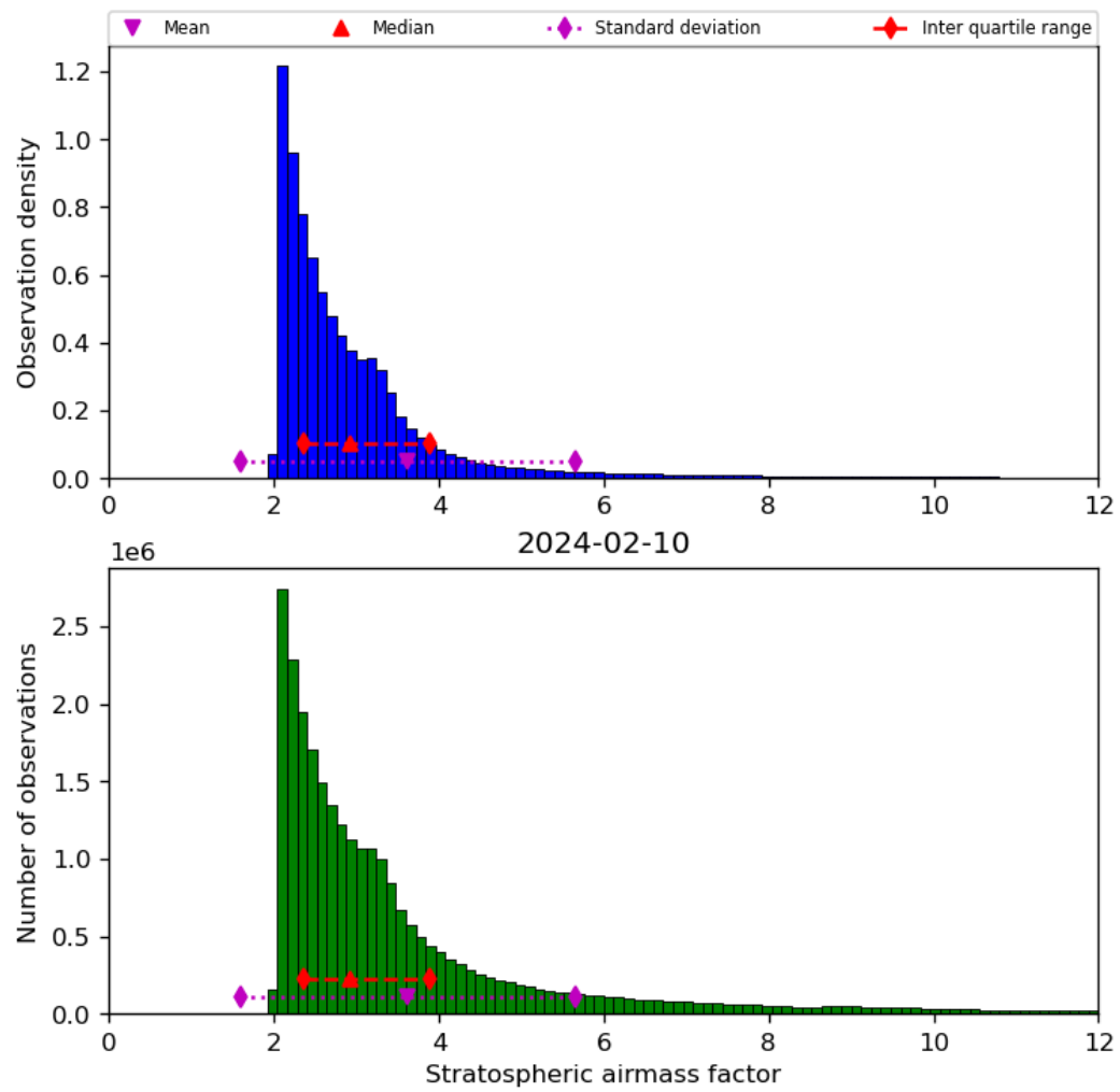
Figure 44: Histogram of “Stratospheric airmass factor” for 2024-02-09 to 2024-02-11
