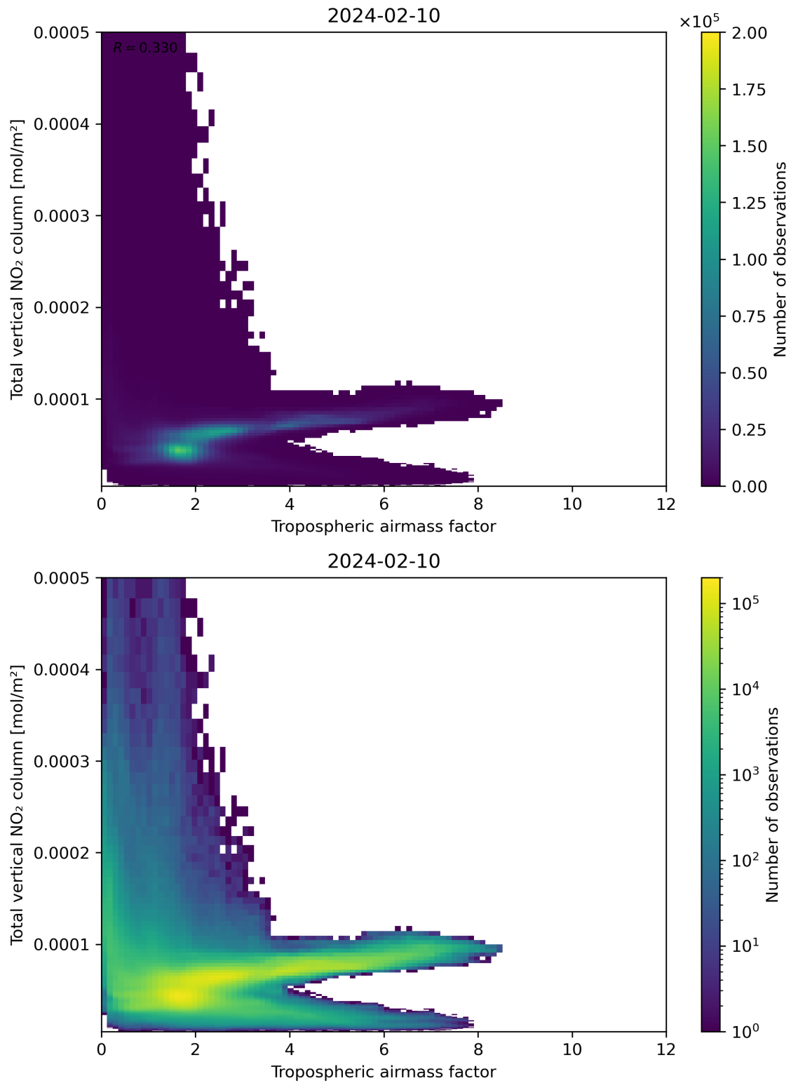
Figure 77: Scatter density plot of “Tropospheric airmass factor” against “Total vertical NO 2 column” for 2024-02-09 to 2024-02-11.
