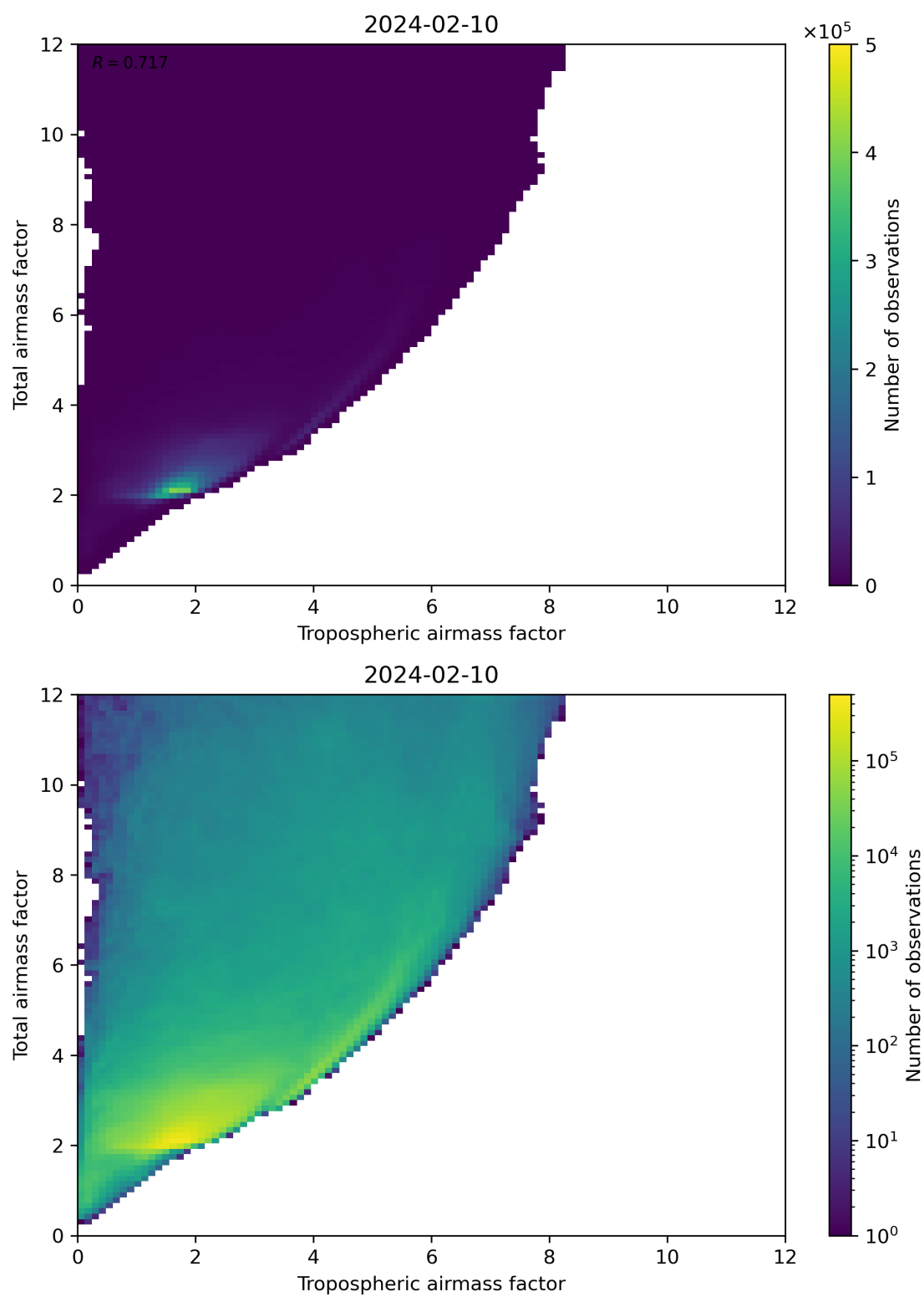
Figure 72: Scatter density plot of “Tropospheric airmass factor” against “Total airmass factor” for 2024-02-09 to 2024-02-11.
