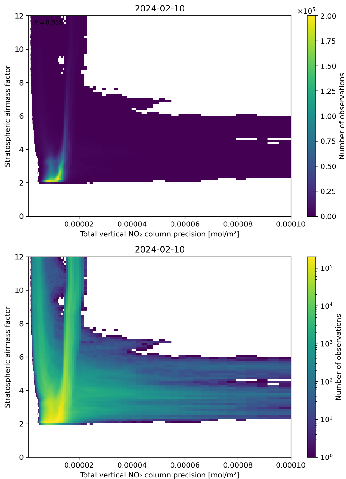
Figure 115: Scatter density plot of “Total vertical NO 2 column precision” against “Stratospheric air mass factor” for 2024-02-09 to 2024-02-11.
