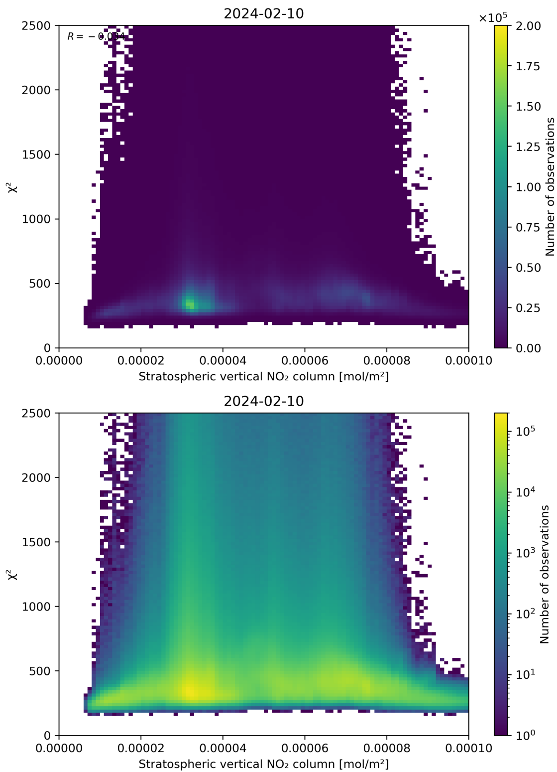
Figure 97: Scatter density plot of “Stratospheric vertical NO 2 column” against “ \chi^2 ” for 2024-02-09 to 2024-02-11.
