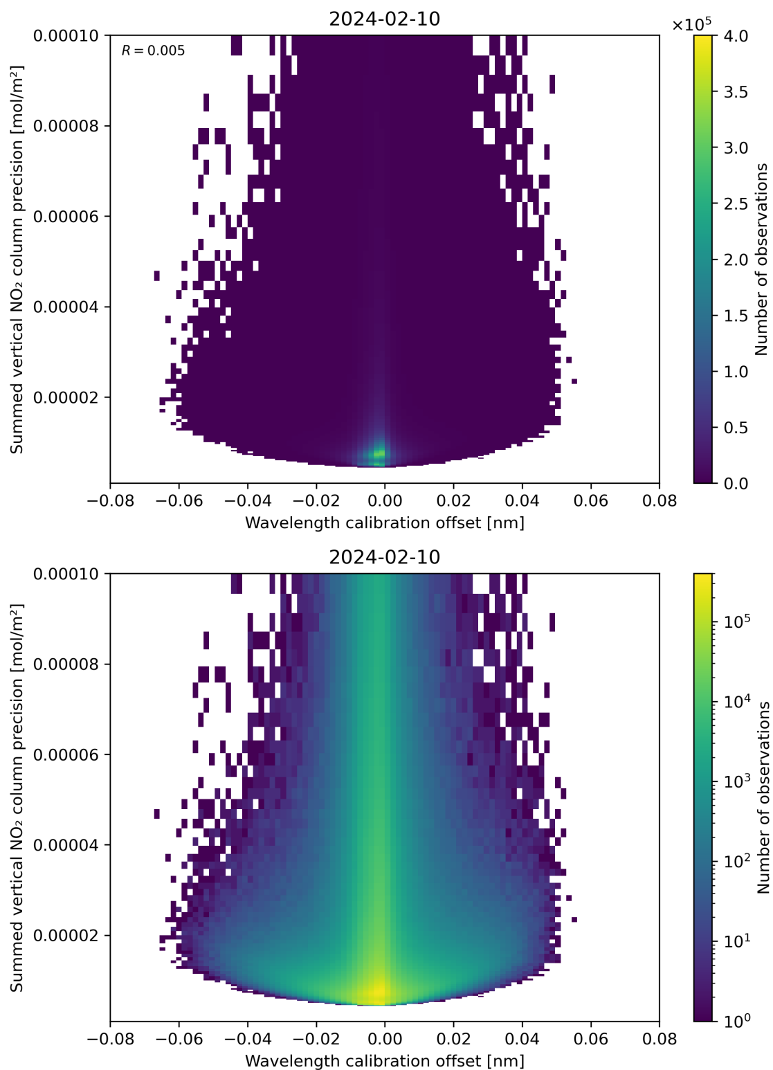
Figure 178: Scatter density plot of “Wavelength calibration offset” against “Summed vertical NO 2 column precision” for 2024-02-09 to 2024-02-11.
