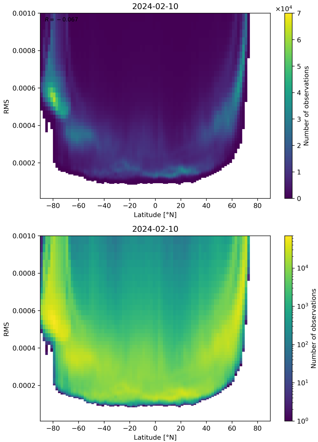
Figure 94: Scatter density plot of “Latitude” against “RMS” for 2024-02-09 to 2024-02-11.
