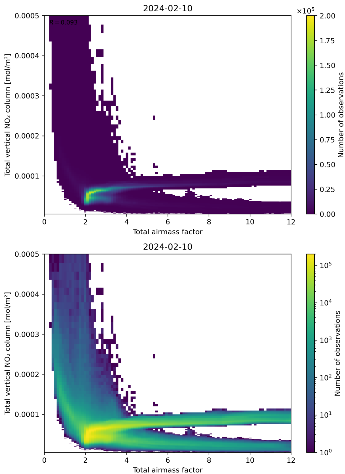
Figure 67: Scatter density plot of “Total airmass factor” against “Total vertical \text{NO}_2 column” for 2024-02-09 to 2024-02-11.
