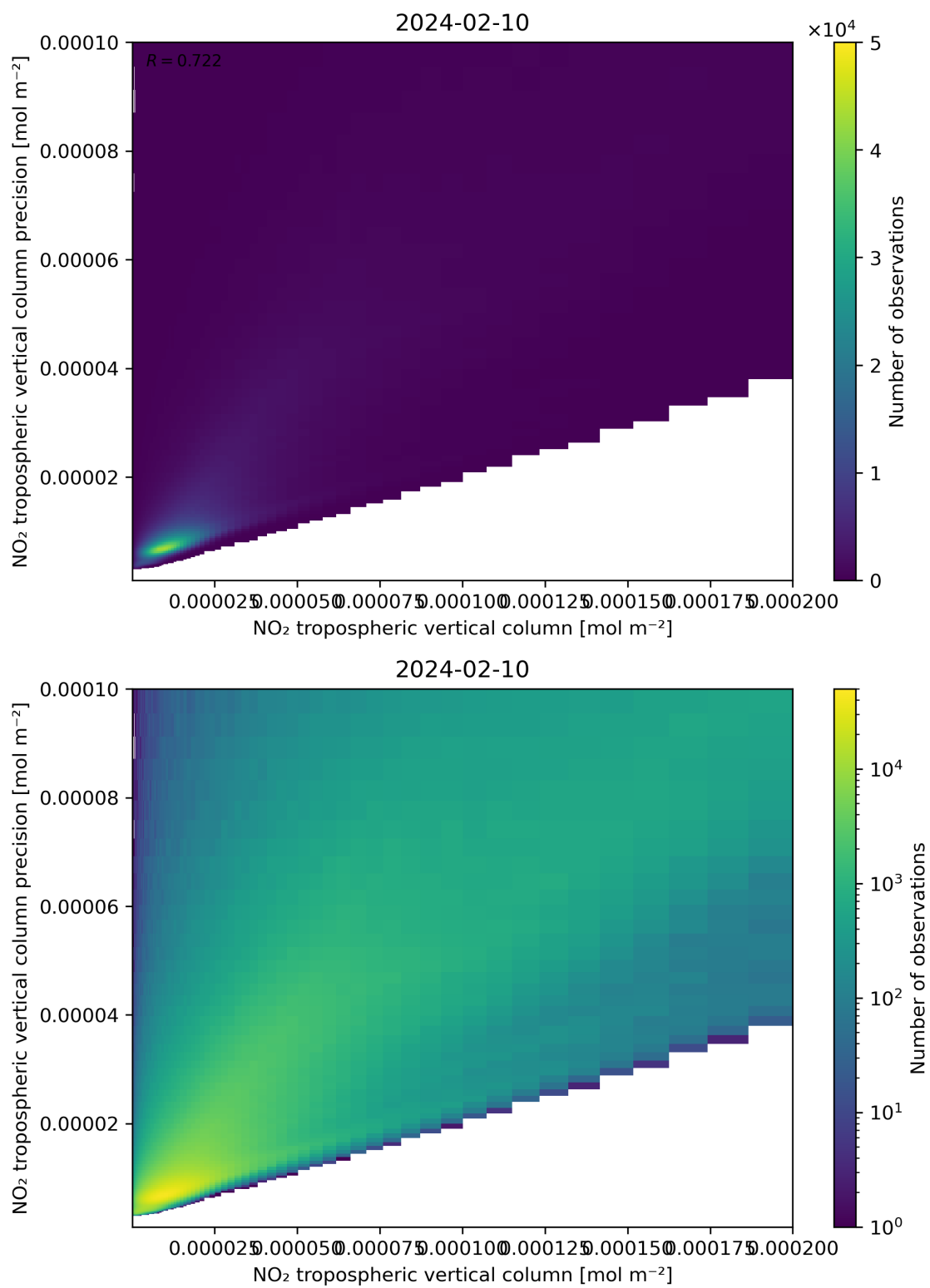
Figure 130: Scatter density plot of “NO 2 tropospheric vertical column” against “NO 2 tropospheric vertical column precision” for 2024-02-09 to 2024-02-11.
