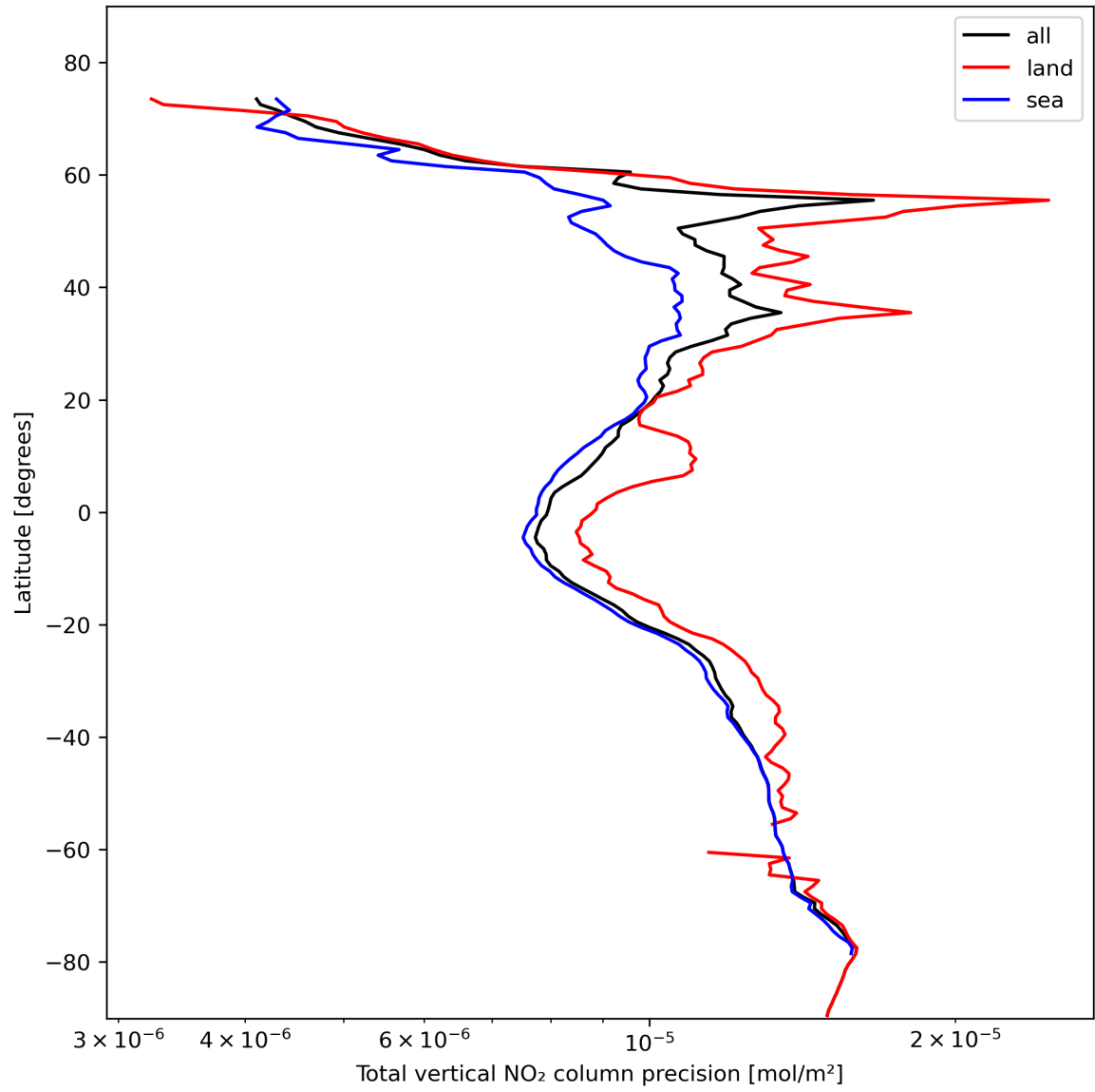
Figure 22: Zonal average of “Total vertical NO 2 column precision” for 2024-02-09 to 2024-02-11.
