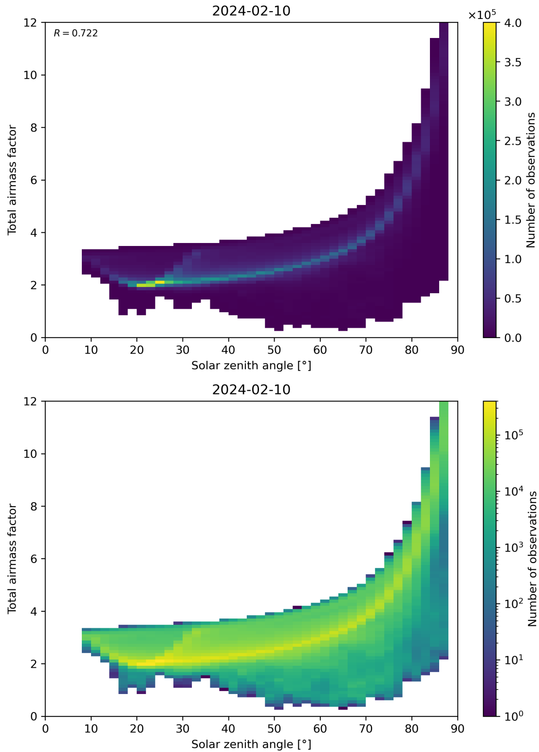
Figure 146: Scatter density plot of “Solar zenith angle” against “Total air mass factor” for 2024-02-09 to 2024-02-11.
