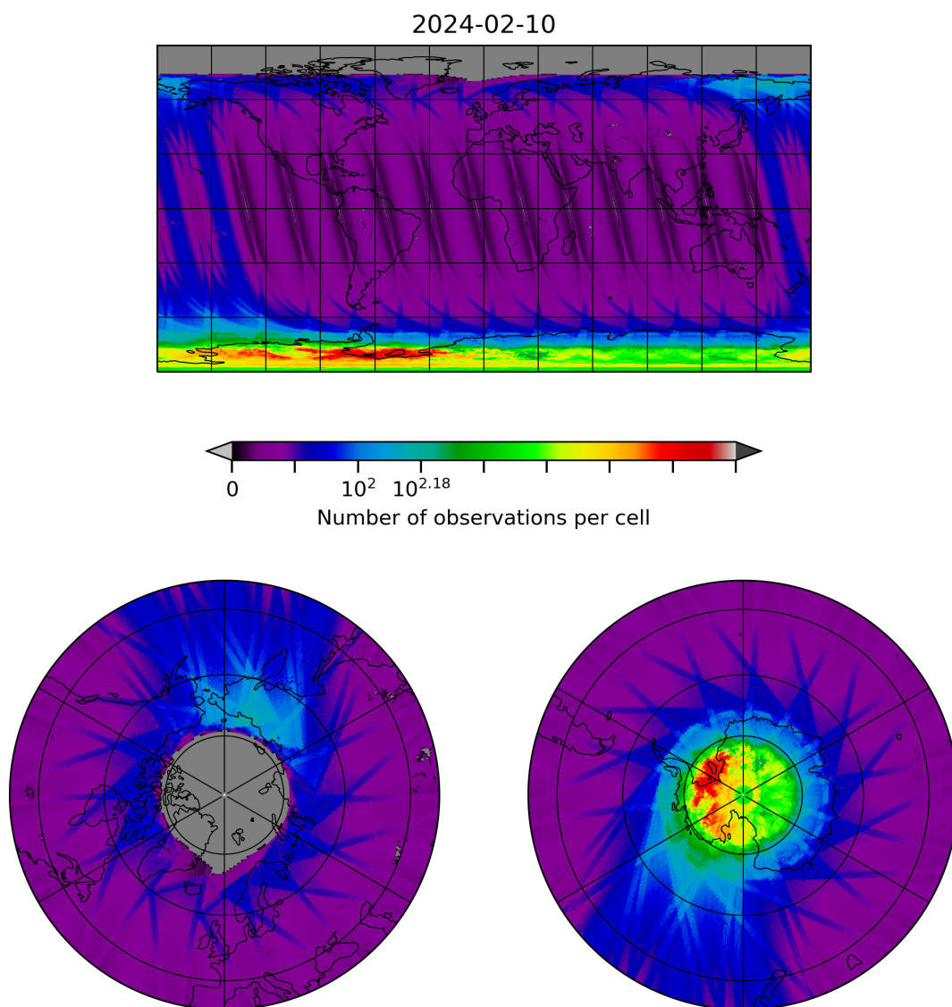
Figure 10: Map of the number of observations for 2024-02-09 to 2024-02-11
