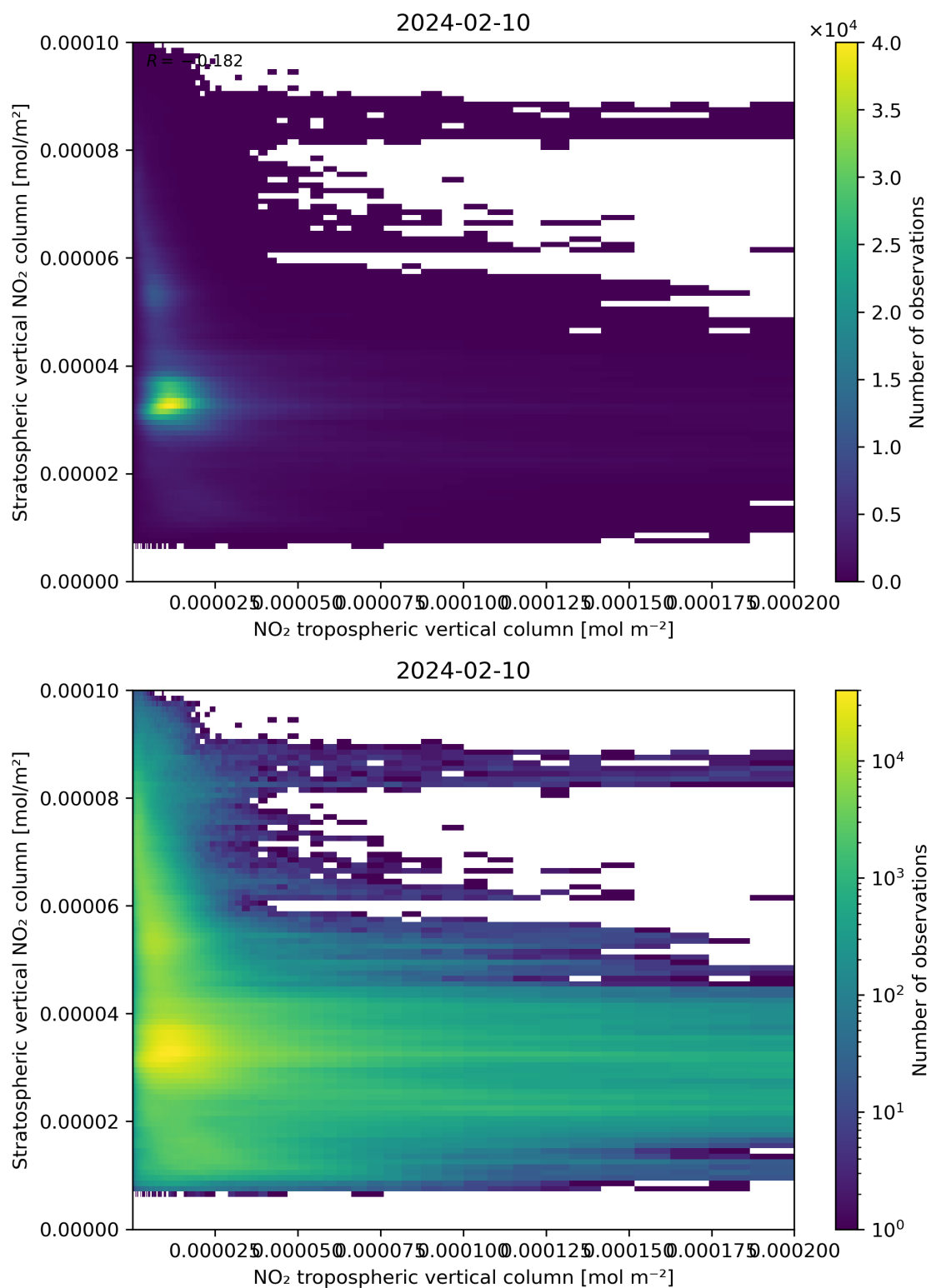
Figure 125: Scatter density plot of “NO 2 tropospheric vertical column” against “Stratospheric vertical NO 2 column” for 2024-02-09 to 2024-02-11.
