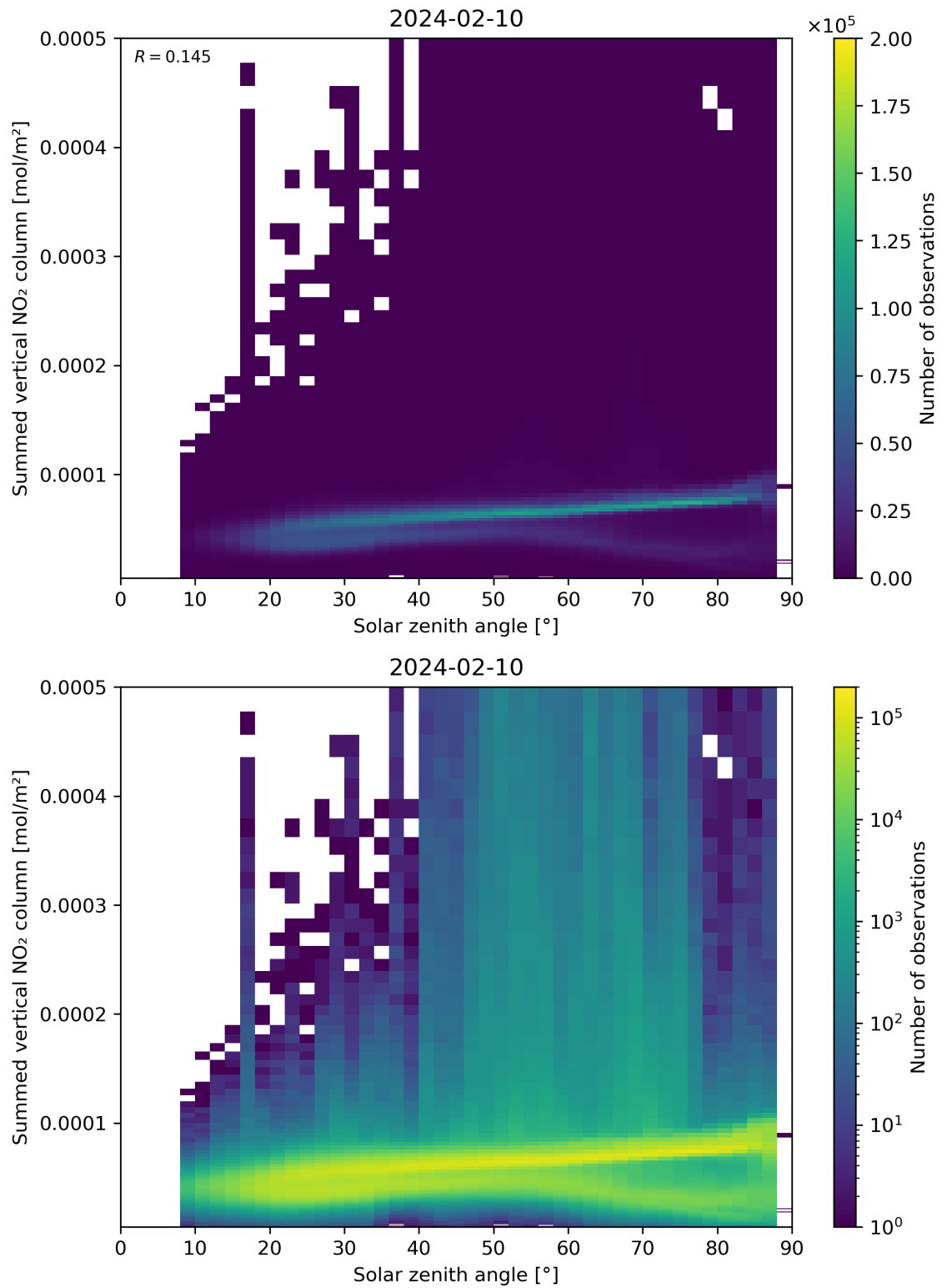
Figure 151: Scatter density plot of “Solar zenith angle” against “Summed vertical NO 2 column” for 2024-02-09 to 2024-02-11.
