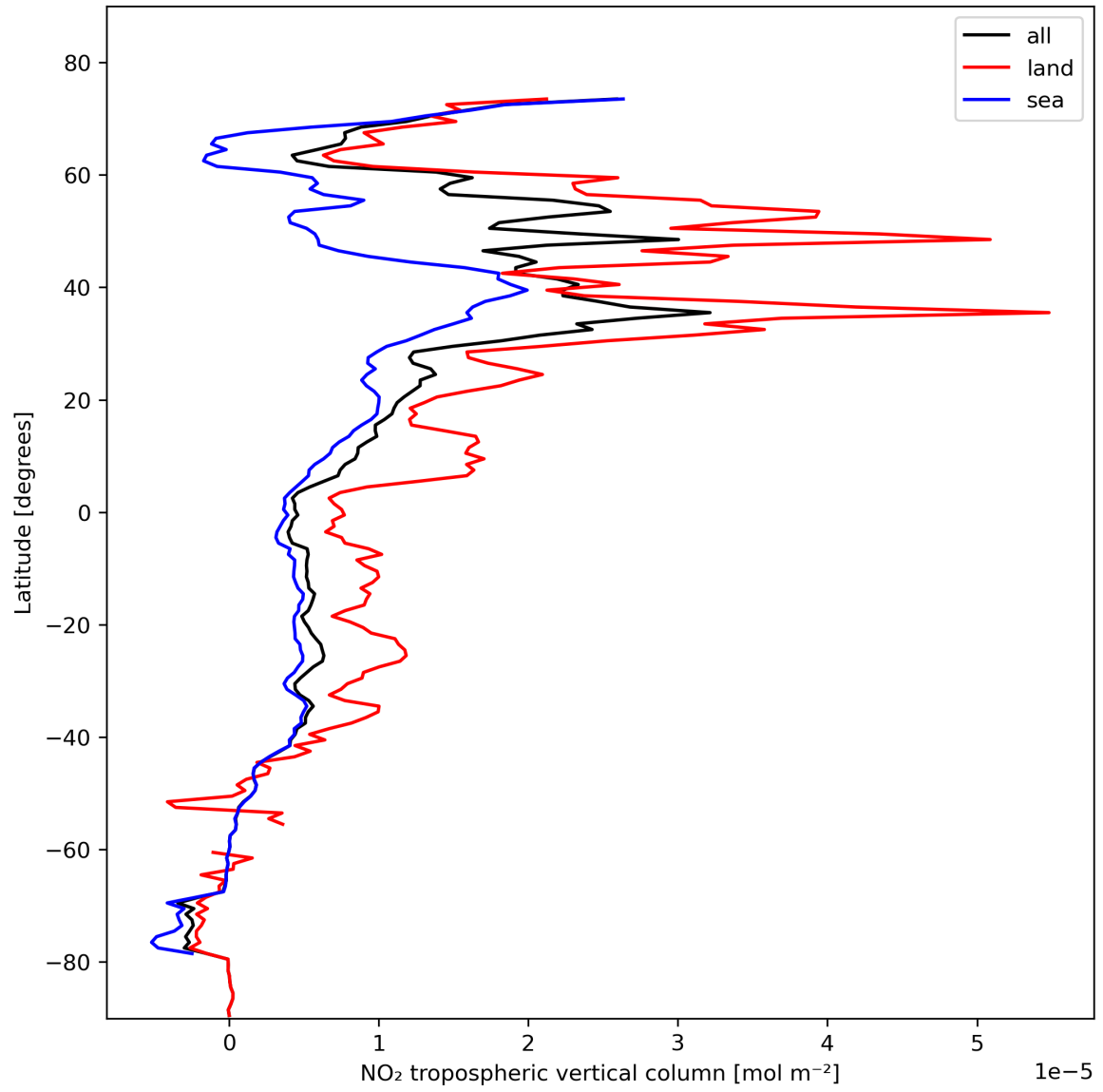
Figure 12: Zonal average of “NO 2 tropospheric vertical column” for 2024-02-09 to 2024-02-11.
