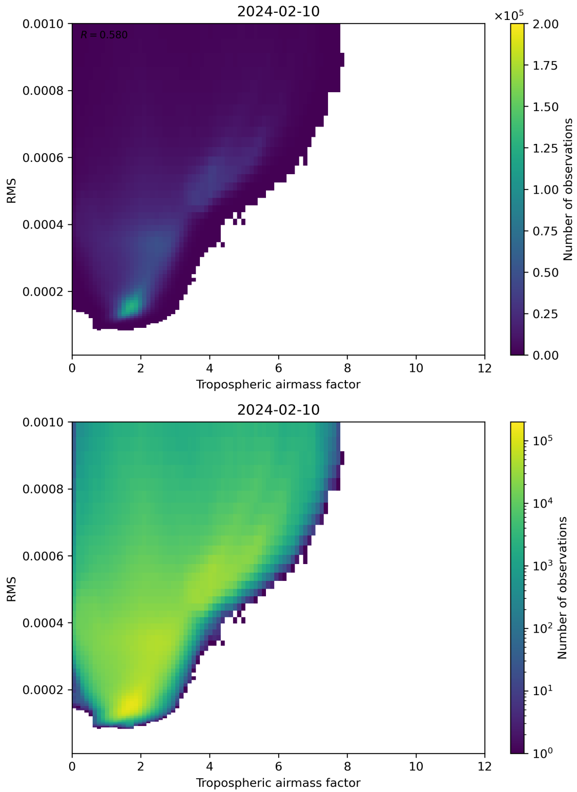
Figure 79: Scatter density plot of “Tropospheric airmass factor” against “RMS” for 2024-02-09 to 2024-02-11.
