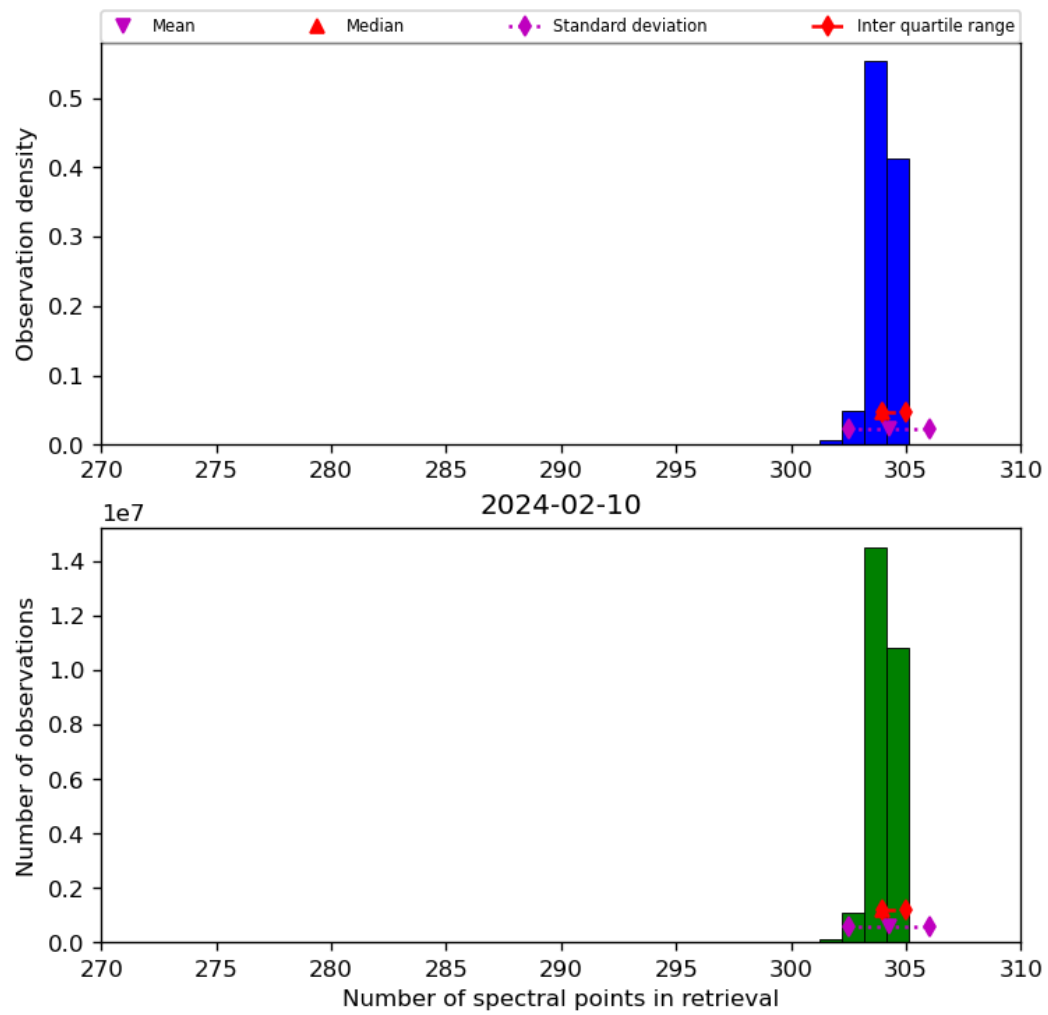
Figure 33: Histogram of “Number of spectral points in retrieval” for 2024-02-09 to 2024-02-11
