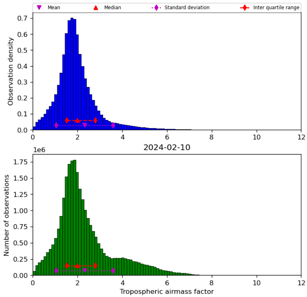
Figure 31: Histogram of “Tropospheric airmass factor” for 2024-02-09 to 2024-02-11
