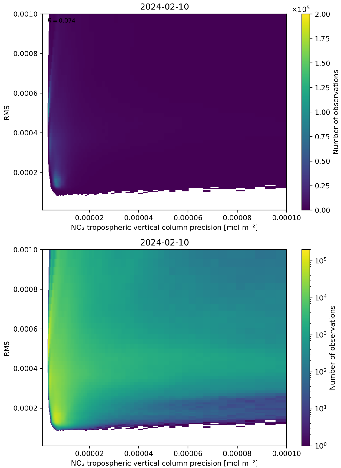
Figure 140: Scatter density plot of “NO 2 tropospheric vertical column precision” against “RMS” for 2024-02-09 to 2024-02-11.
