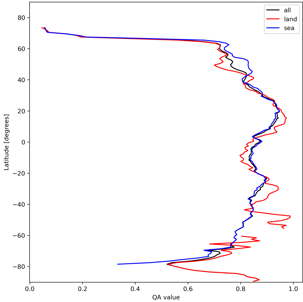
Figure 11: Zonal average of “QA value” for 2024-02-09 to 2024-02-11.
