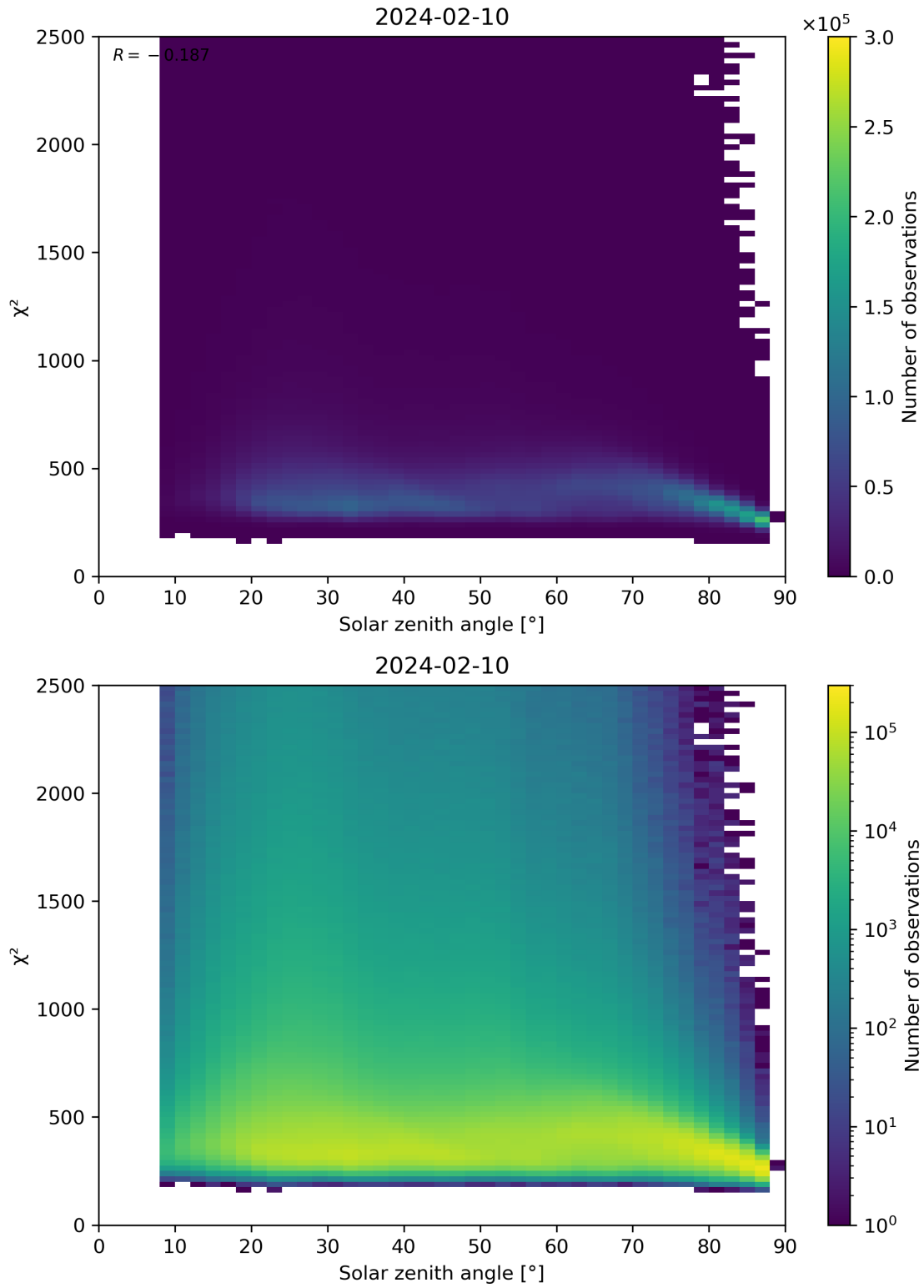
Figure 148: Scatter density plot of “Solar zenith angle” against “ \chi^2 ” for 2024-02-09 to 2024-02-11.
