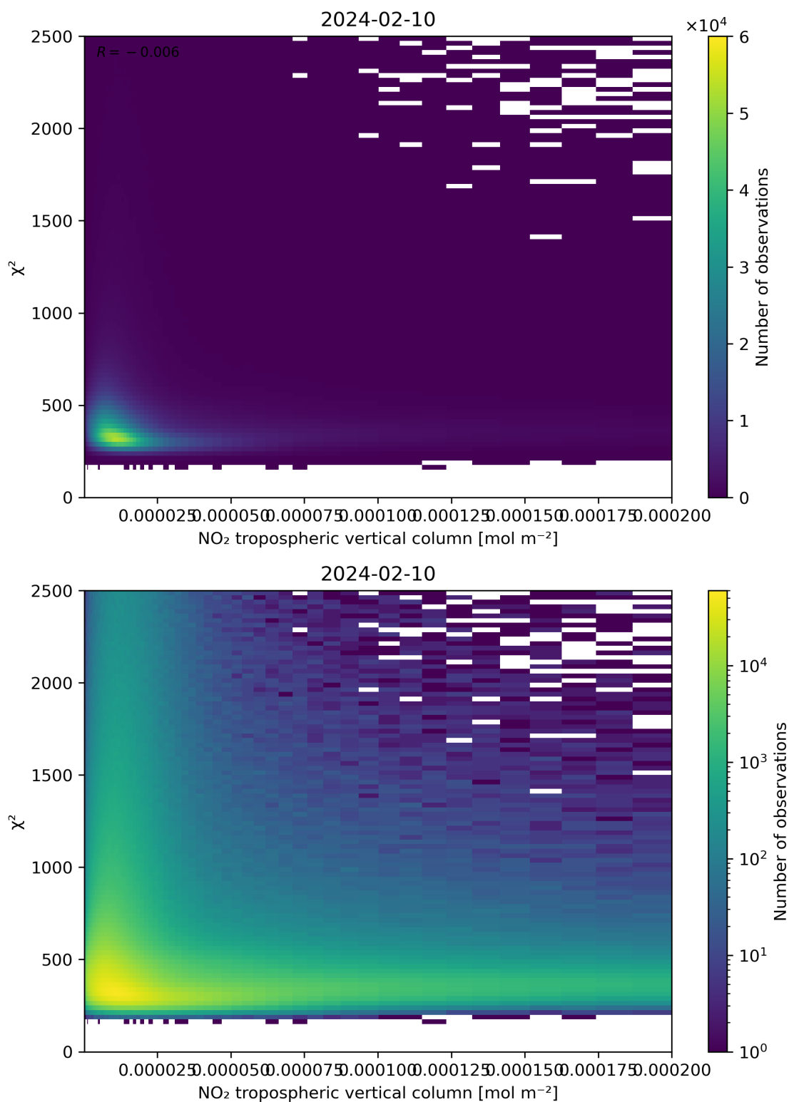
Figure 124: Scatter density plot of “NO 2 tropospheric vertical column” against “ \chi^2 ” for 2024-02-09 to 2024-02-11.
