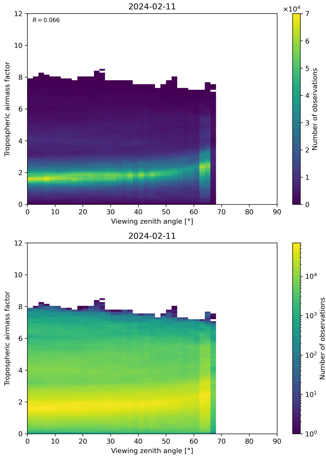
Figure 161: Scatter density plot of “Viewing zenith angle” against “Tropospheric airmass factor” for 2024-02-11 to 2024-02-12.
