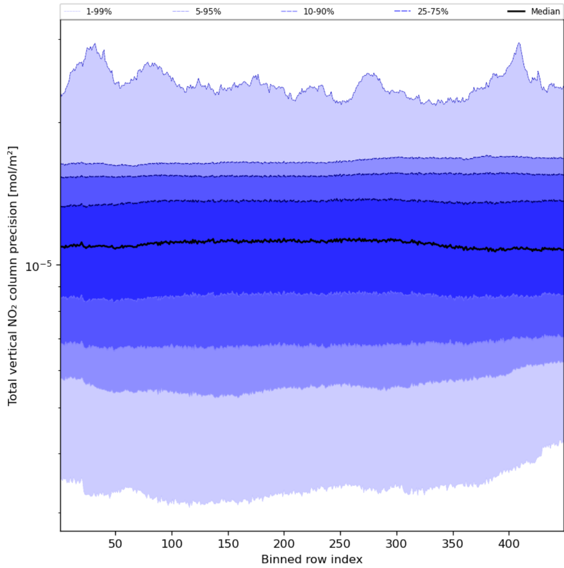
Figure 56: Along track statistics of “Total vertical NO 2 column precision” for 2024-02-11 to 2024-02-12
