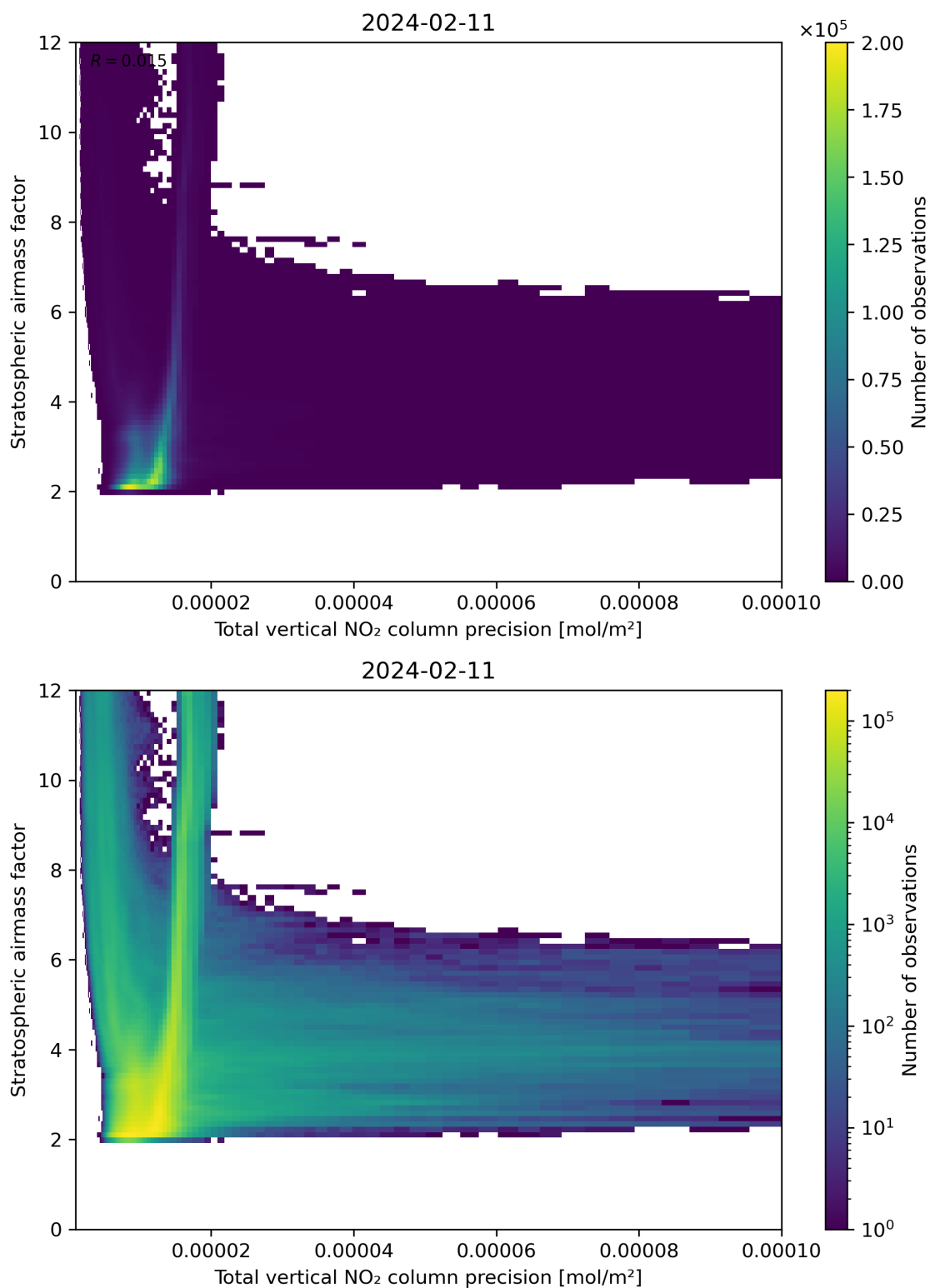
Figure 115: Scatter density plot of “Total vertical NO 2 column precision” against “Stratospheric air mass factor” for 2024-02-11 to 2024-02-12.
