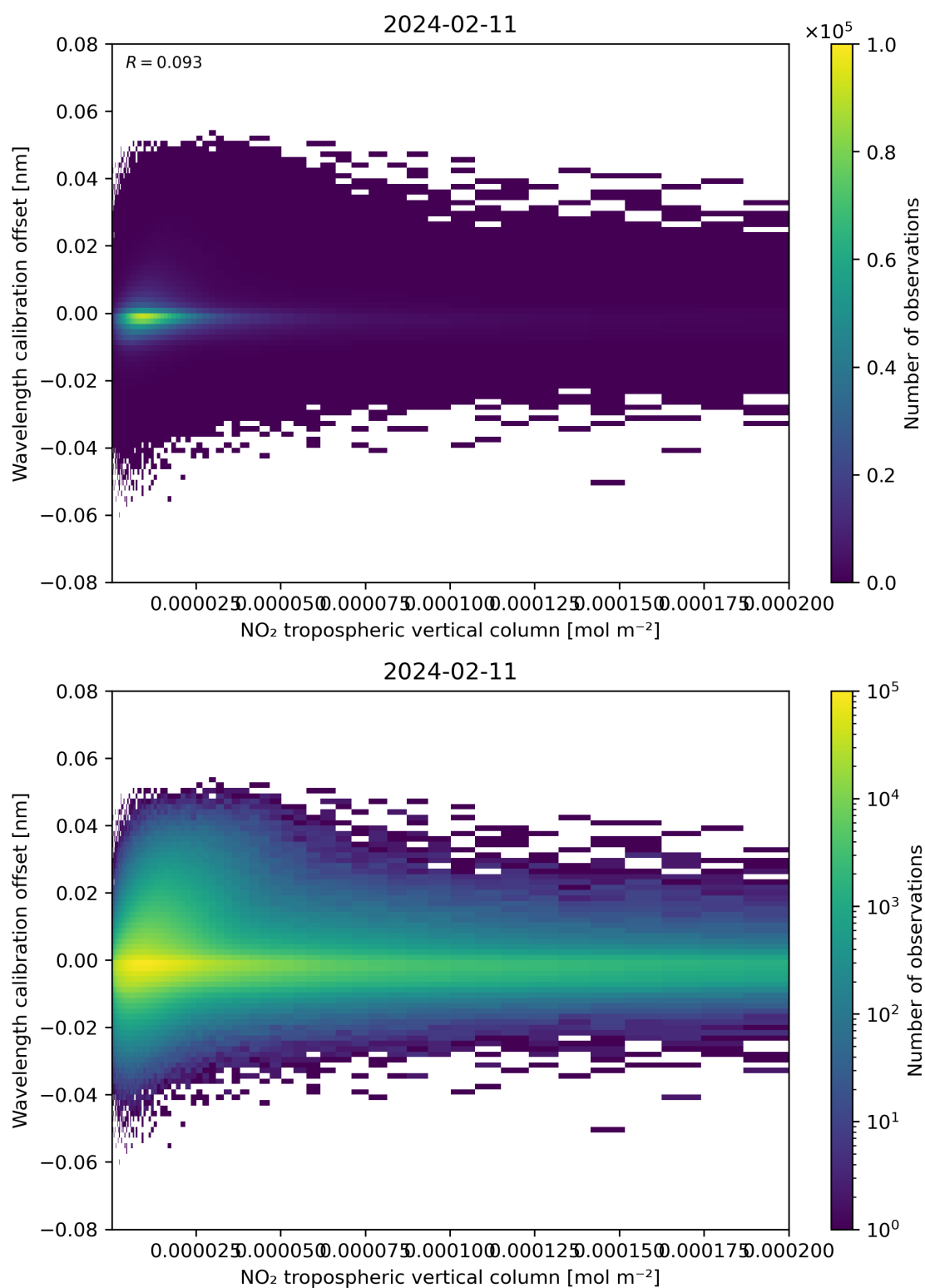
Figure 143: Scatter density plot of “NO 2 tropospheric vertical column” against “Wavelength calibration offset” for 2024-02-11 to 2024-02-12.
