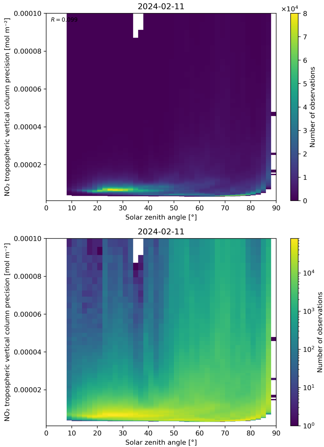
Figure 156: Scatter density plot of “Solar zenith angle” against “NO 2 tropospheric vertical column precision” for 2024-02-11 to 2024-02-12.
