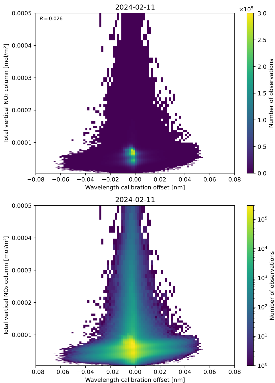
Figure 179: Scatter density plot of “Wavelength calibration offset” against “Total vertical NO 2 column” for 2024-02-11 to 2024-02-12.
