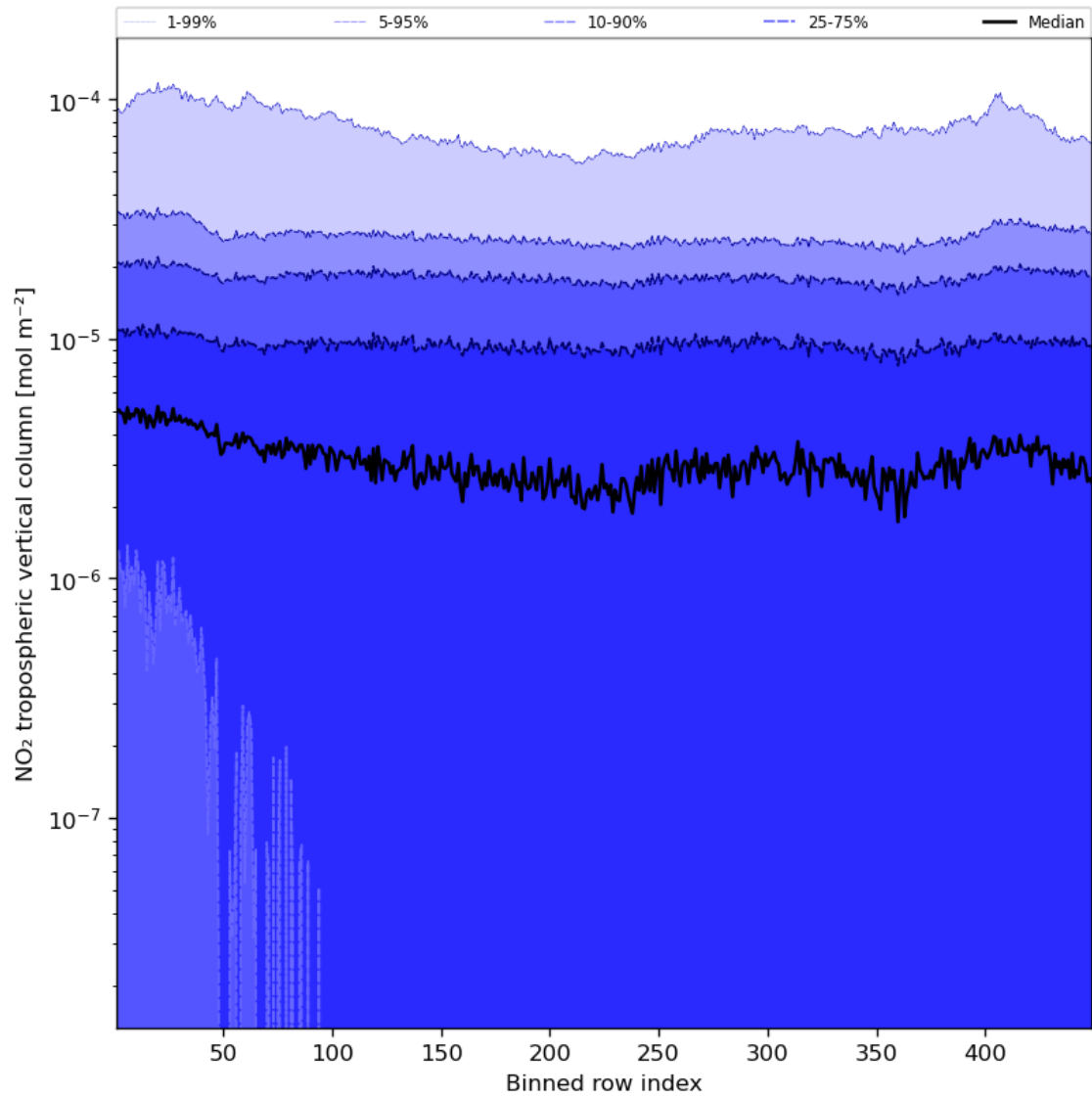
Figure 46: Along track statistics of “NO 2 tropospheric vertical column” for 2024-02-11 to 2024-02-12
