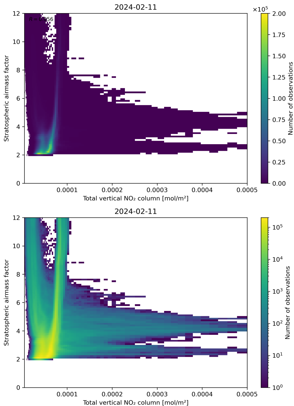
Figure 110: Scatter density plot of “Total vertical NO 2 column” against “Stratospheric airmass factor” for 2024-02-11 to 2024-02-12.
