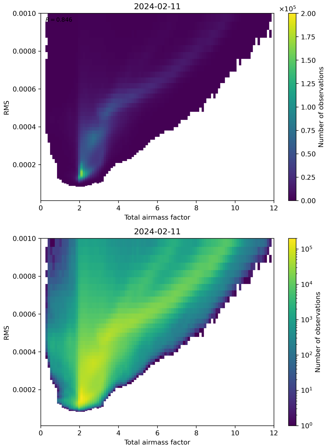
Figure 69: Scatter density plot of “Total airmass factor” against “RMS” for 2024-02-11 to 2024-02-12.
