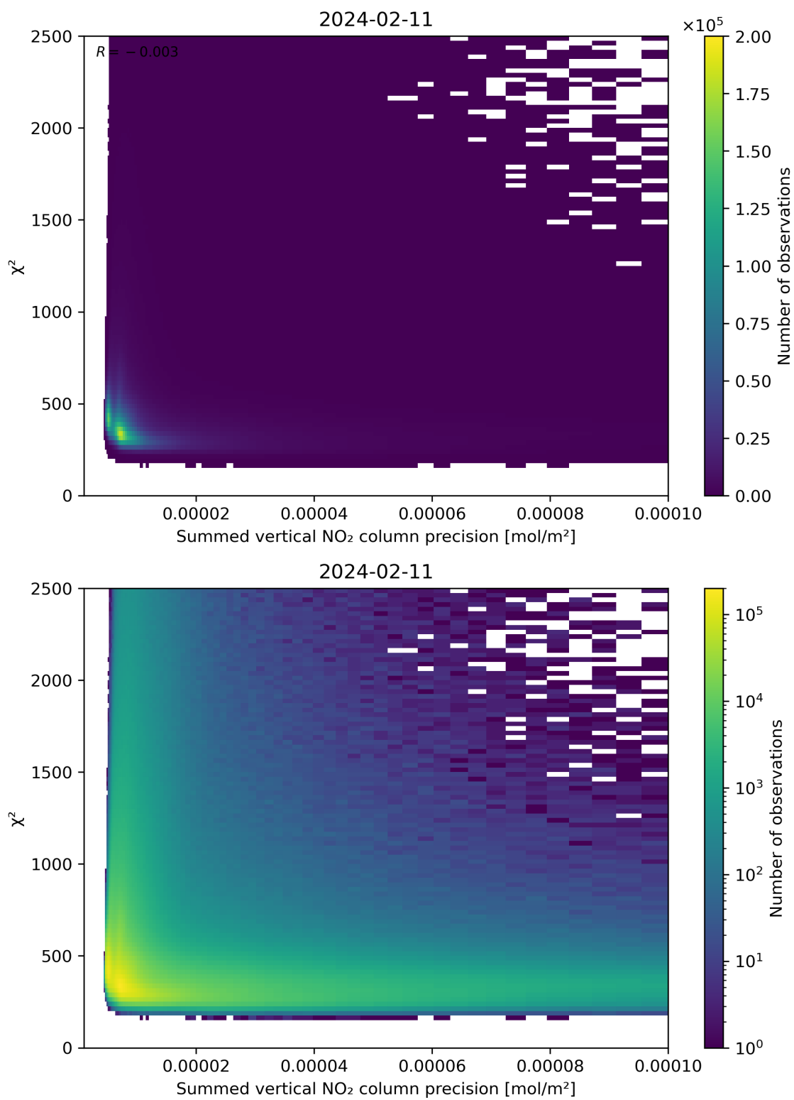
Figure 107: Scatter density plot of “Summed vertical NO 2 column precision” against “ \chi^2 ” for 2024-02-11 to 2024-02-12.
