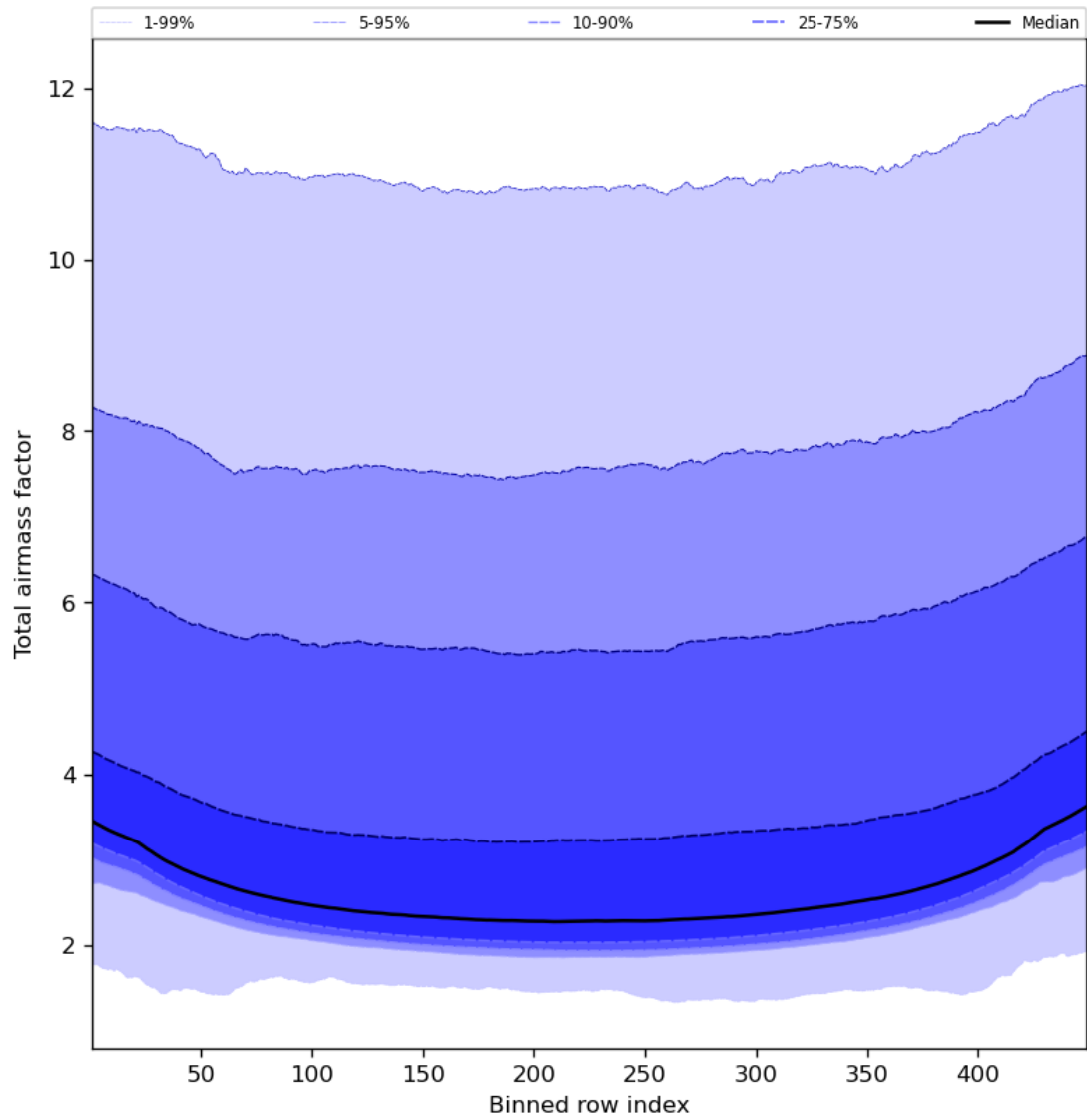
Figure 49: Along track statistics of “Total airmass factor” for 2024-02-11 to 2024-02-12
