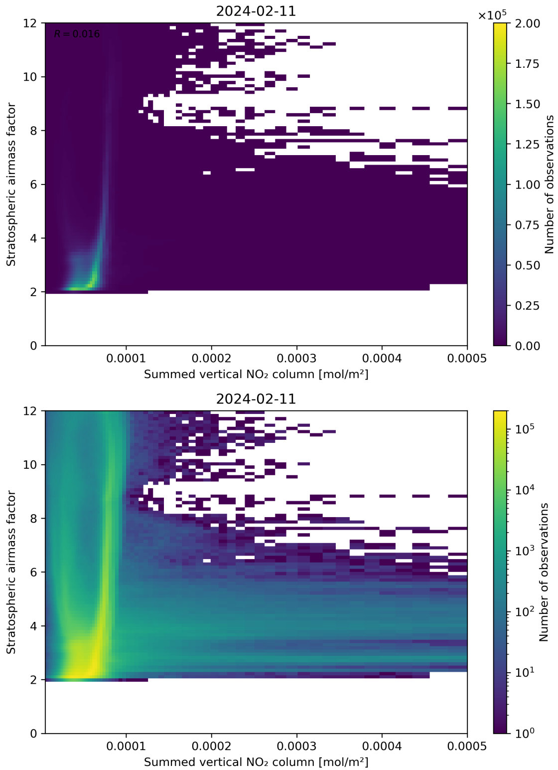
Figure 103: Scatter density plot of “Summed vertical NO 2 column” against “Stratospheric air mass factor” for 2024-02-11 to 2024-02-12.
