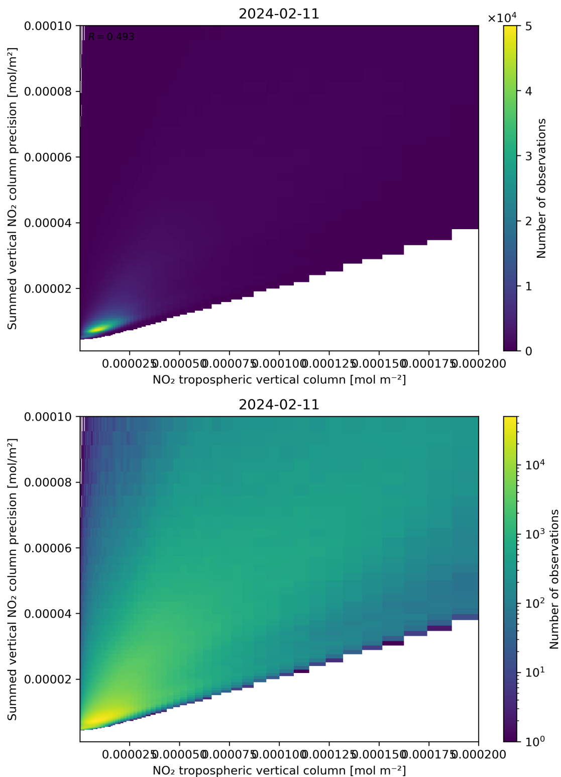
Figure 127: Scatter density plot of “NO 2 tropospheric vertical column” against “Summed vertical NO 2 column precision” for 2024-02-11 to 2024-02-12.
