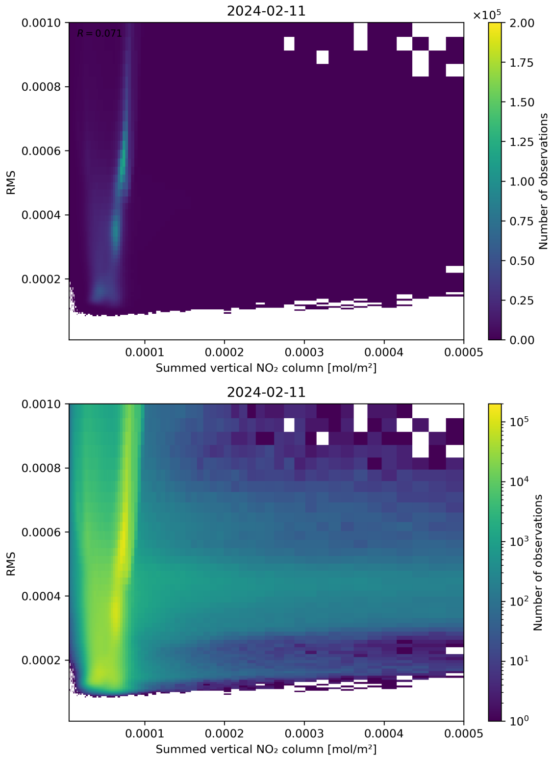
Figure 109: Scatter density plot of “Summed vertical NO 2 column” against “RMS” for 2024-02-11 to 2024-02-12.
