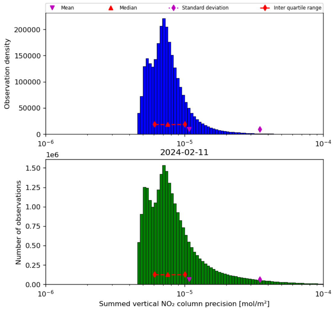
Figure 41: Histogram of "Summed vertical NO 2 column precision" for 2024-02-11 to 2024-02-12
