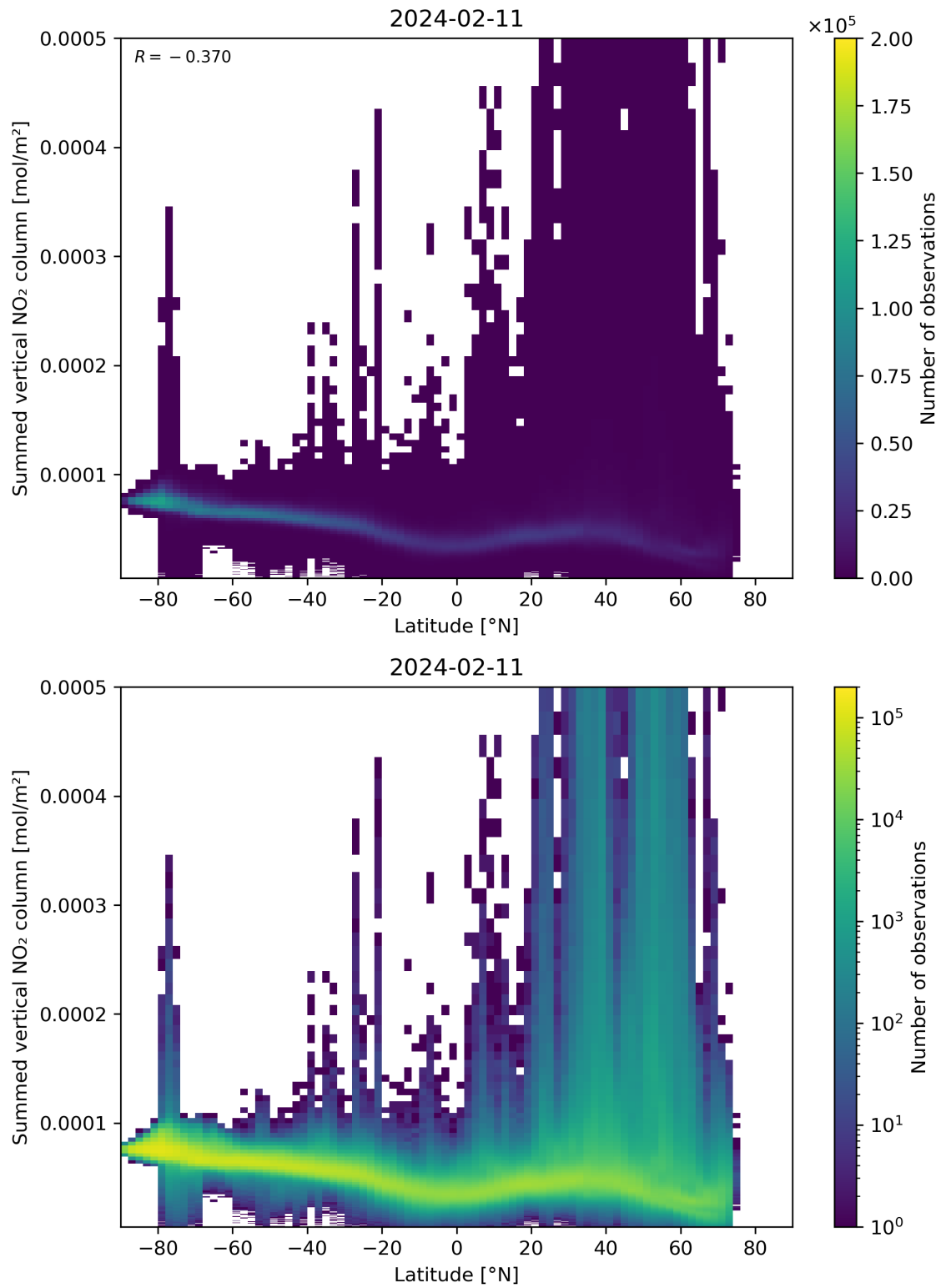
Figure 88: Scatter density plot of “Latitude” against “Summed vertical NO 2 column” for 2024-02-11 to 2024-02-12.
