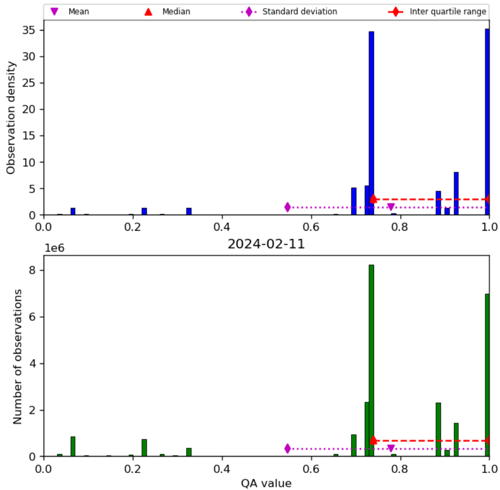
Figure 28: Histogram of “QA value” for 2024-02-11 to 2024-02-12
