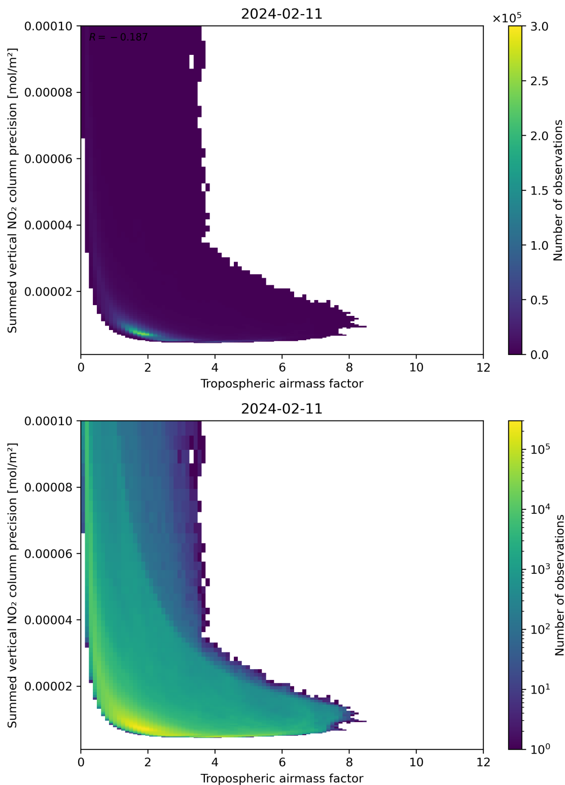
Figure 76: Scatter density plot of “Tropospheric air mass factor” against “Summed vertical NO 2 column precision” for 2024-02-11 to 2024-02-12.
