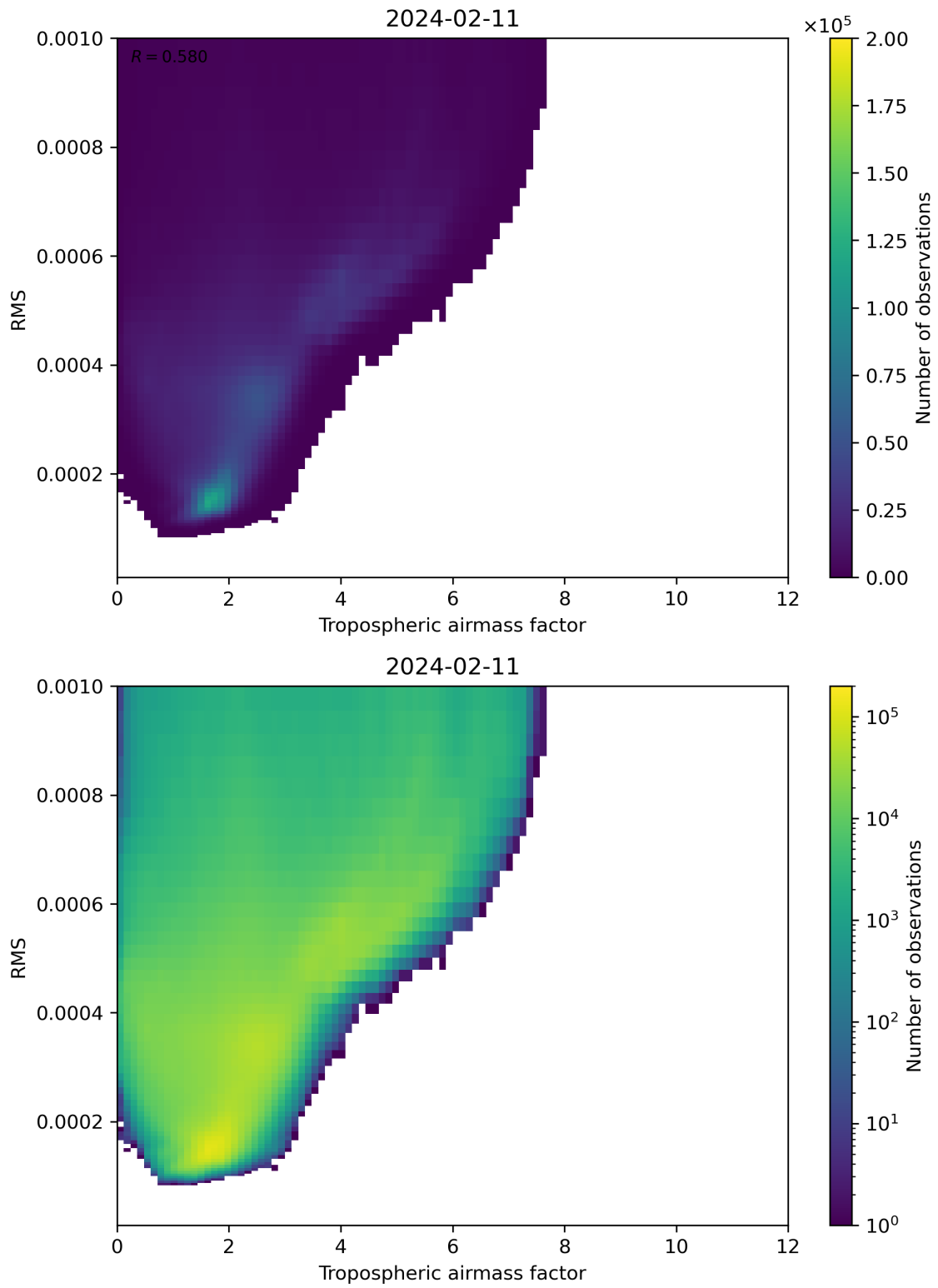
Figure 79: Scatter density plot of “Tropospheric airmass factor” against “RMS” for 2024-02-11 to 2024-02-12.
