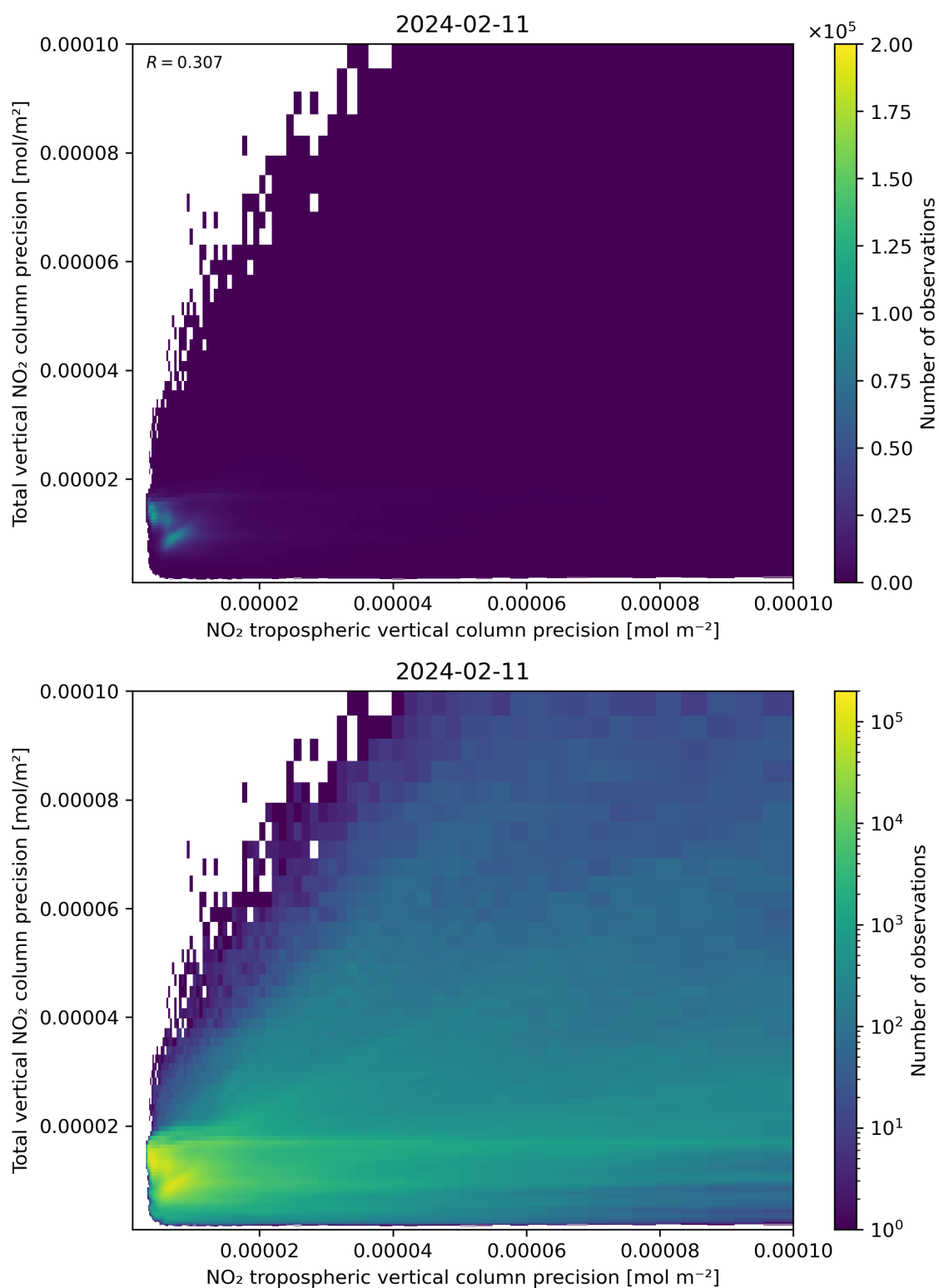
Figure 139: Scatter density plot of “NO 2 tropospheric vertical column precision” against “Total vertical NO 2 column precision” for 2024-02-11 to 2024-02-12.
