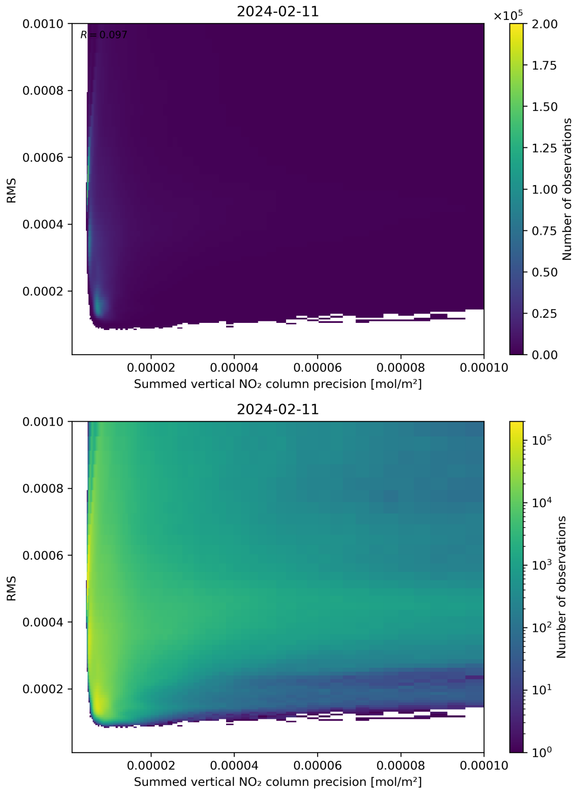
Figure 108: Scatter density plot of “Summed vertical NO 2 column precision” against “RMS” for 2024-02-11 to 2024-02-12.
