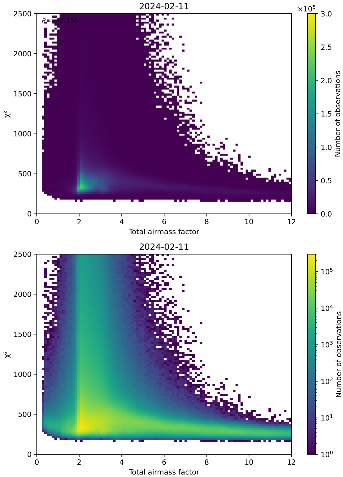
Figure 63: Scatter density plot of “Total airmass factor” against “ \chi^2 ” for 2024-02-11 to 2024-02-12.
