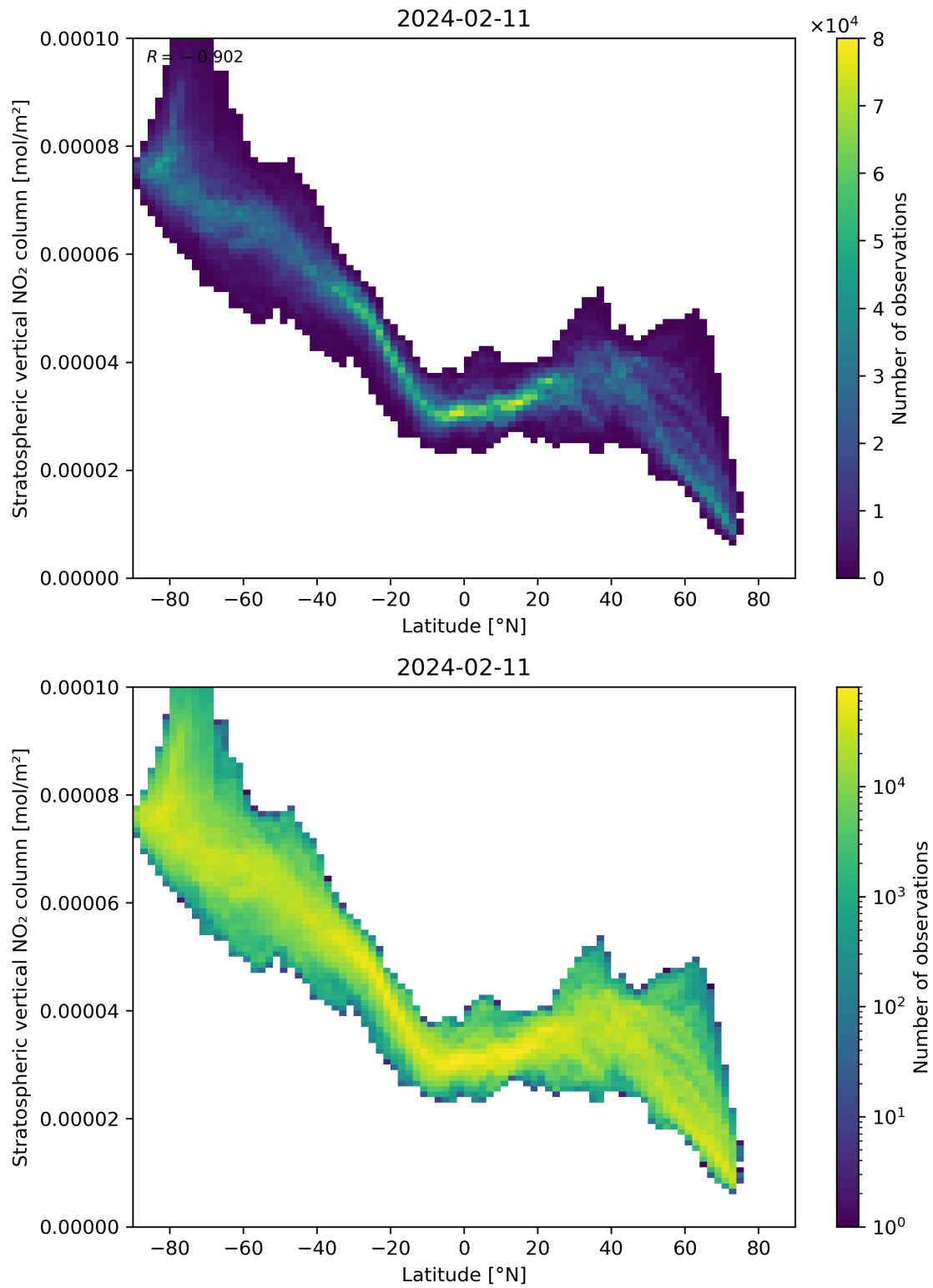
Figure 87: Scatter density plot of “Latitude” against “Stratospheric vertical NO 2 column” for 2024-02-11 to 2024-02-12.
