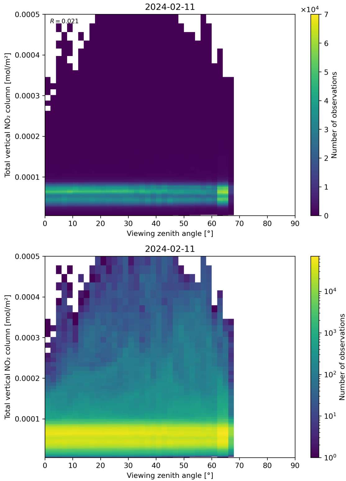
Figure 167: Scatter density plot of “Viewing zenith angle” against “Total vertical NO 2 column” for 2024-02-11 to 2024-02-12.
