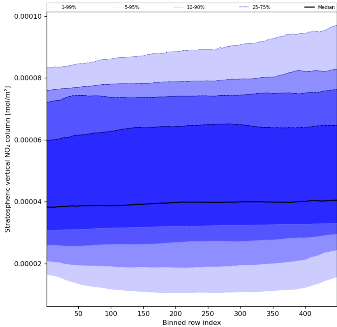
Figure 53: Along track statistics of “Stratospheric vertical NO 2 column” for 2024-02-11 to 2024-02-12
