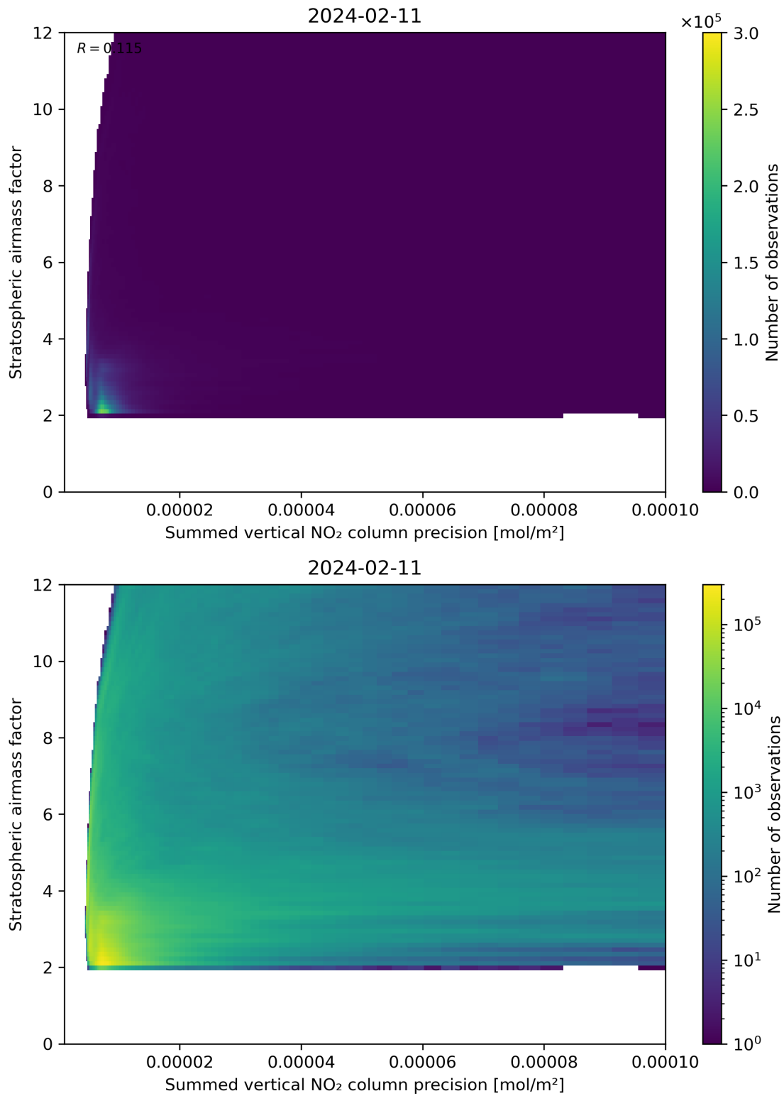
Figure 106: Scatter density plot of “Summed vertical NO 2 column precision” against “Stratospheric airmass factor” for 2024-02-11 to 2024-02-12.
