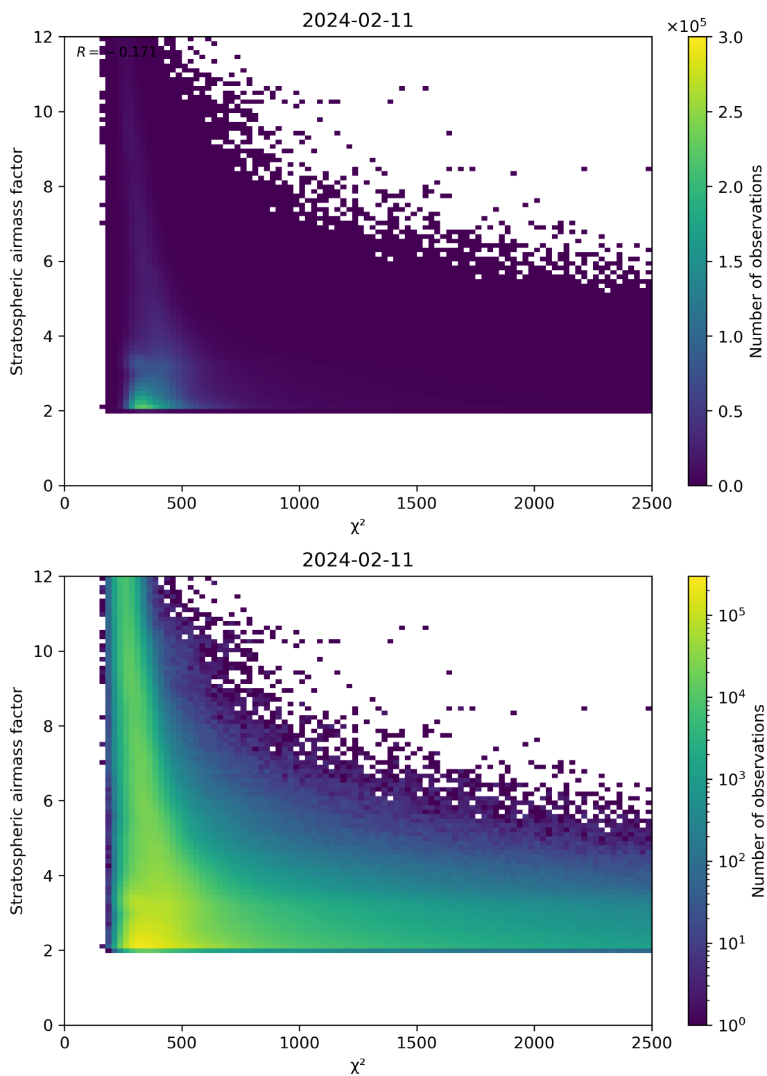
Figure 81: Scatter density plot of " \chi^2 " against "Stratospheric airmass factor" for 2024-02-11 to 2024-02-12.
