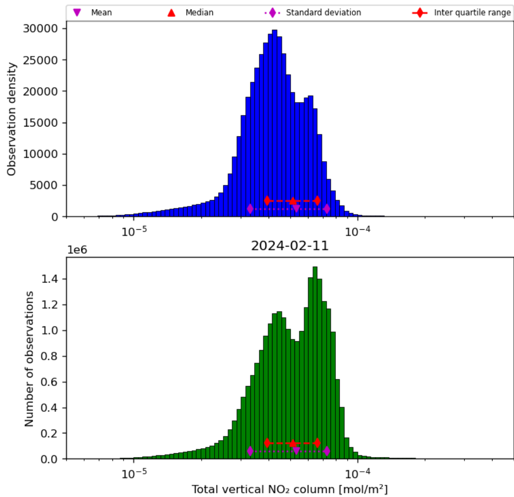
Figure 38: Histogram of “Total vertical NO 2 column” for 2024-02-11 to 2024-02-12
