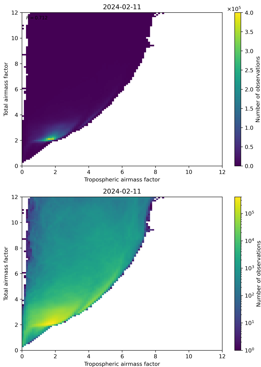
Figure 72: Scatter density plot of “Tropospheric airmass factor” against “Total airmass factor” for 2024-02-11 to 2024-02-12.
