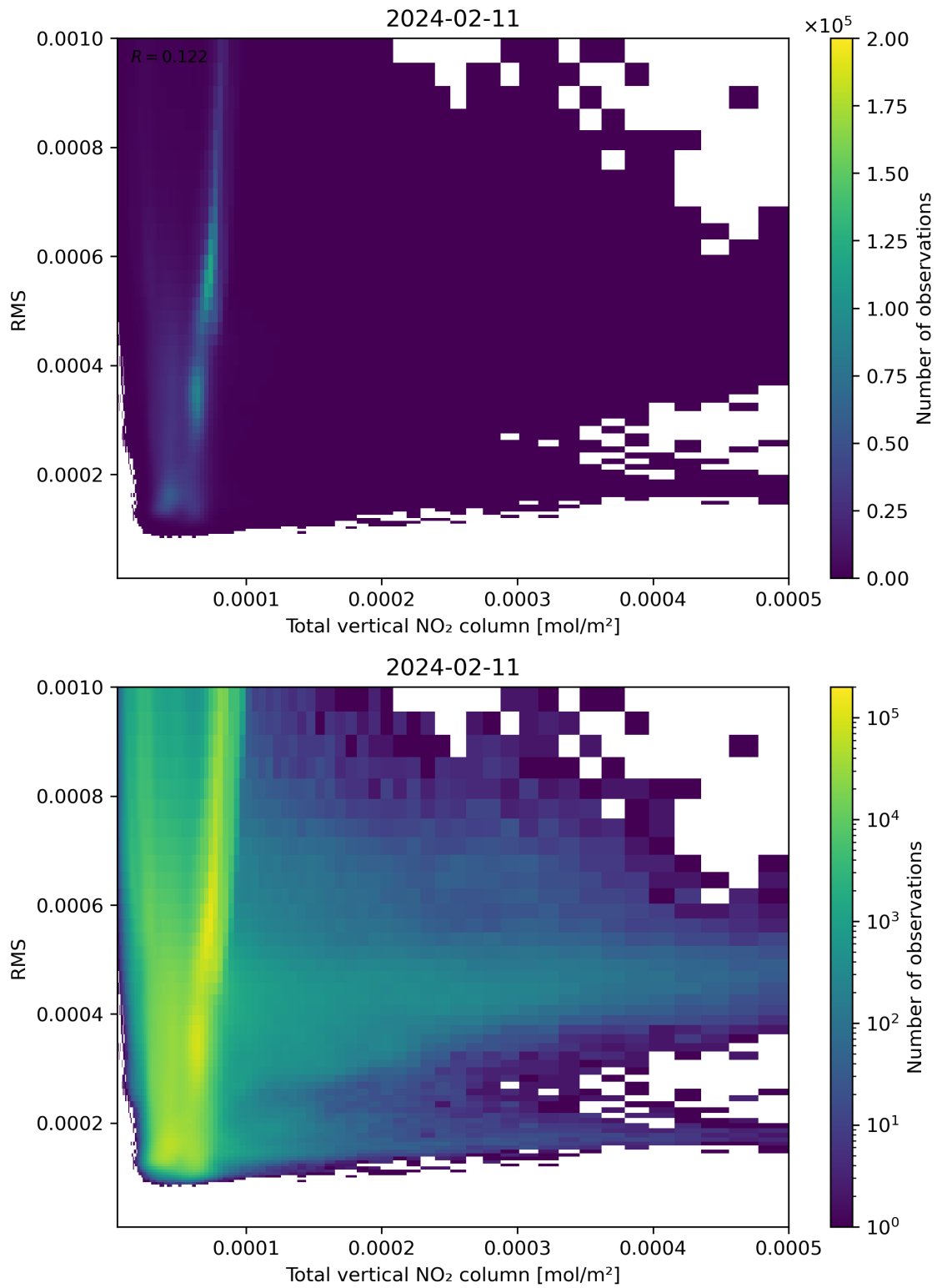
Figure 120: Scatter density plot of “Total vertical NO 2 column” against “RMS” for 2024-02-11 to 2024-02-12.
