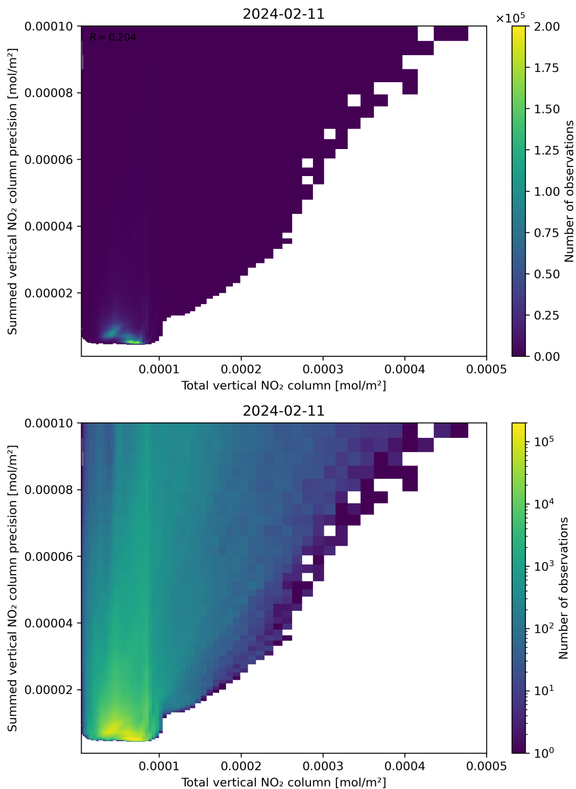
Figure 113: Scatter density plot of “Total vertical NO 2 column” against “Summed vertical NO 2 column precision” for 2024-02-11 to 2024-02-12.
