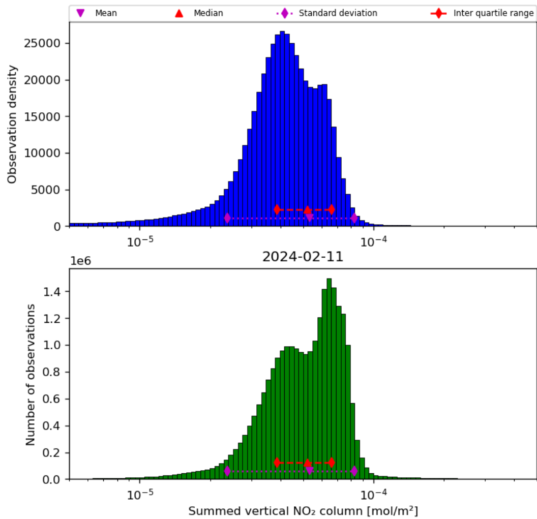
Figure 40: Histogram of “Summed vertical NO 2 column” for 2024-02-11 to 2024-02-12
