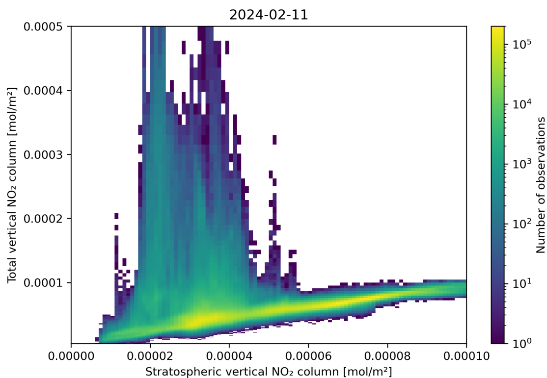
Figure 100: Scatter density plot of “Stratospheric vertical NO 2 column” against “Total vertical NO 2 column” for 2024-02-11 to 2024-02-12.
