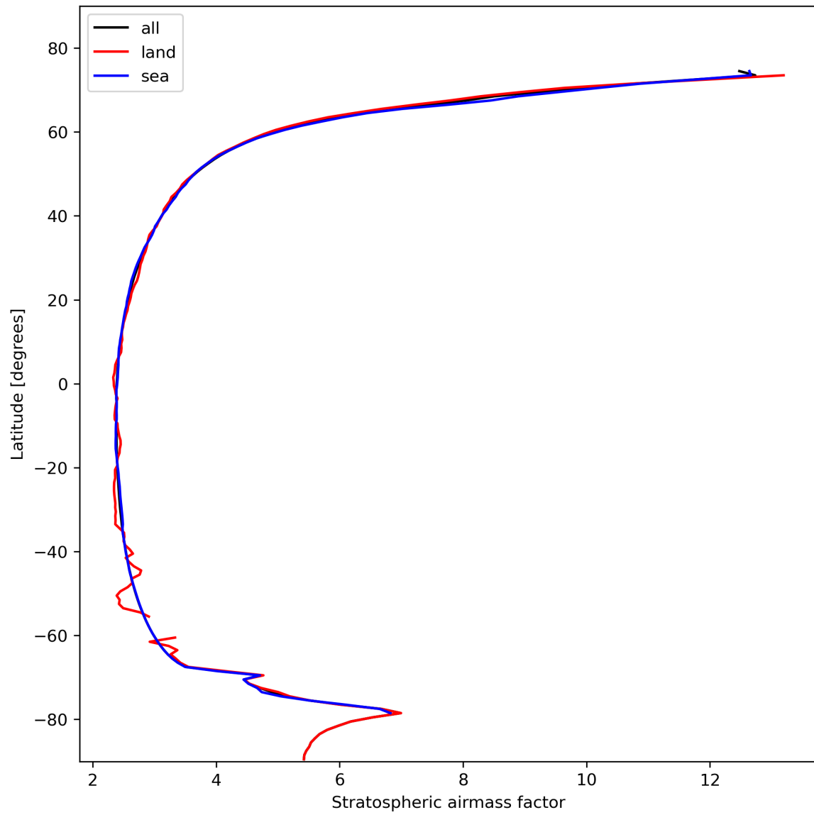
Figure 27: Zonal average of “Stratospheric air mass factor” for 2024-02-11 to 2024-02-12.
