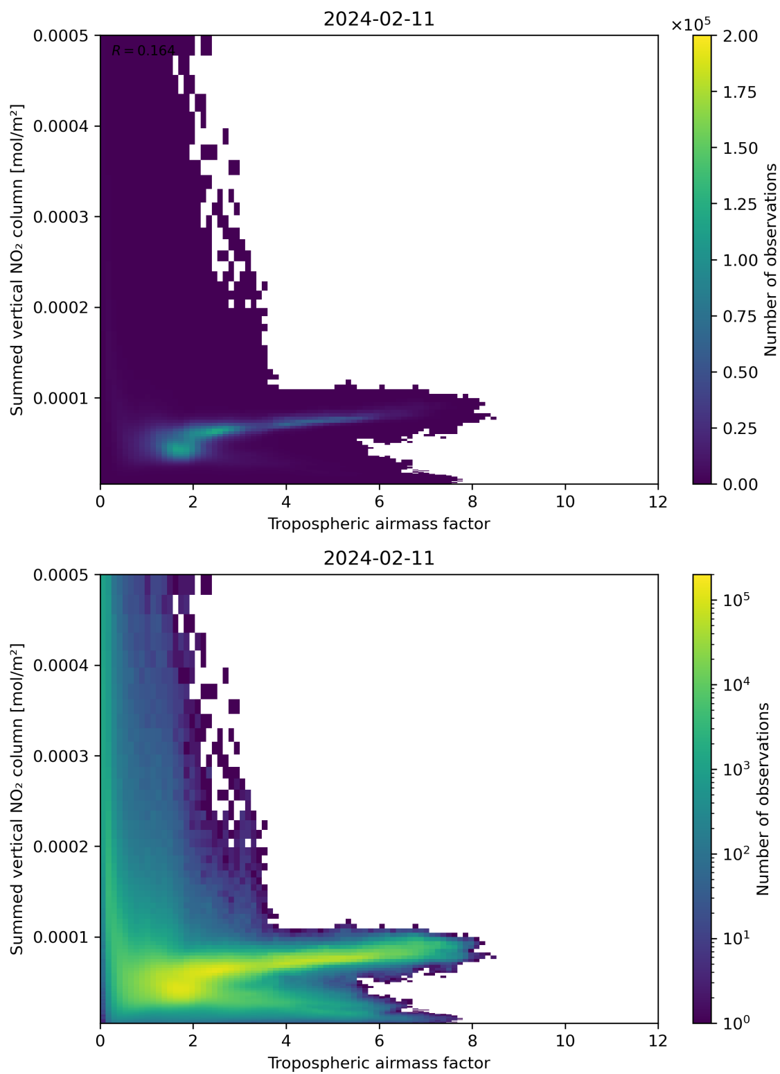
Figure 75: Scatter density plot of “Tropospheric air mass factor” against “Summed vertical NO 2 column” for 2024-02-11 to 2024-02-12.
