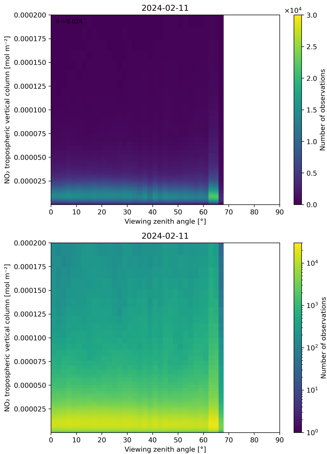
Figure 169: Scatter density plot of “Viewing zenith angle” against “NO 2 tropospheric vertical column” for 2024-02-11 to 2024-02-12.
