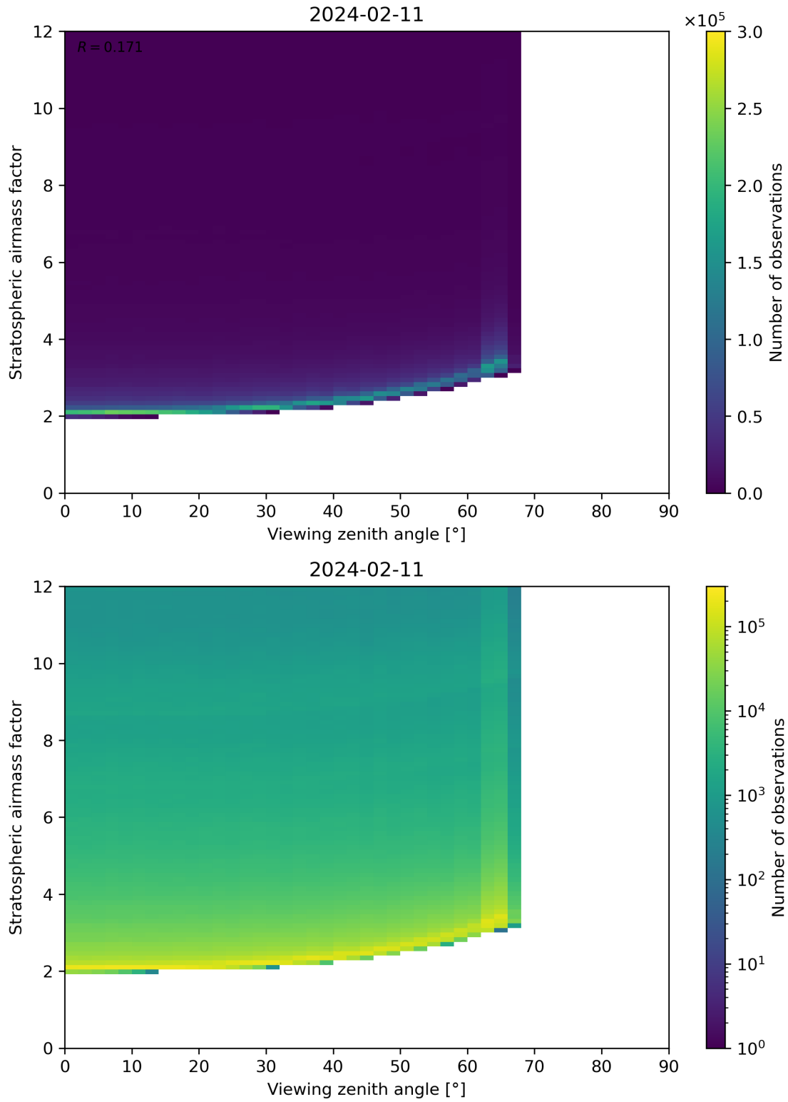
Figure 159: Scatter density plot of “Viewing zenith angle” against “Stratospheric airmass factor” for 2024-02-11 to 2024-02-12.
