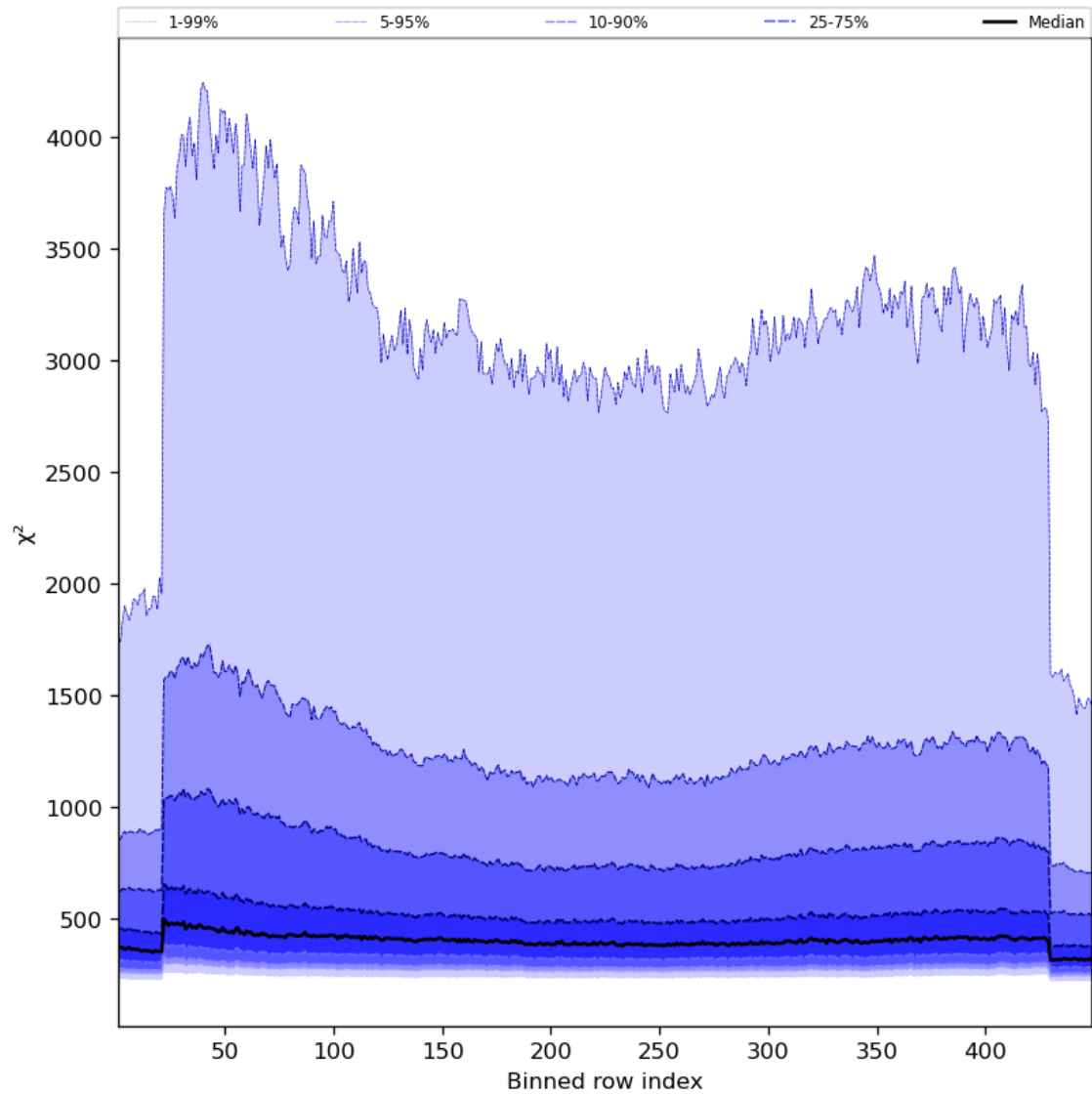
Figure 59: Along track statistics of “ \chi^2 ” for 2024-02-11 to 2024-02-12
