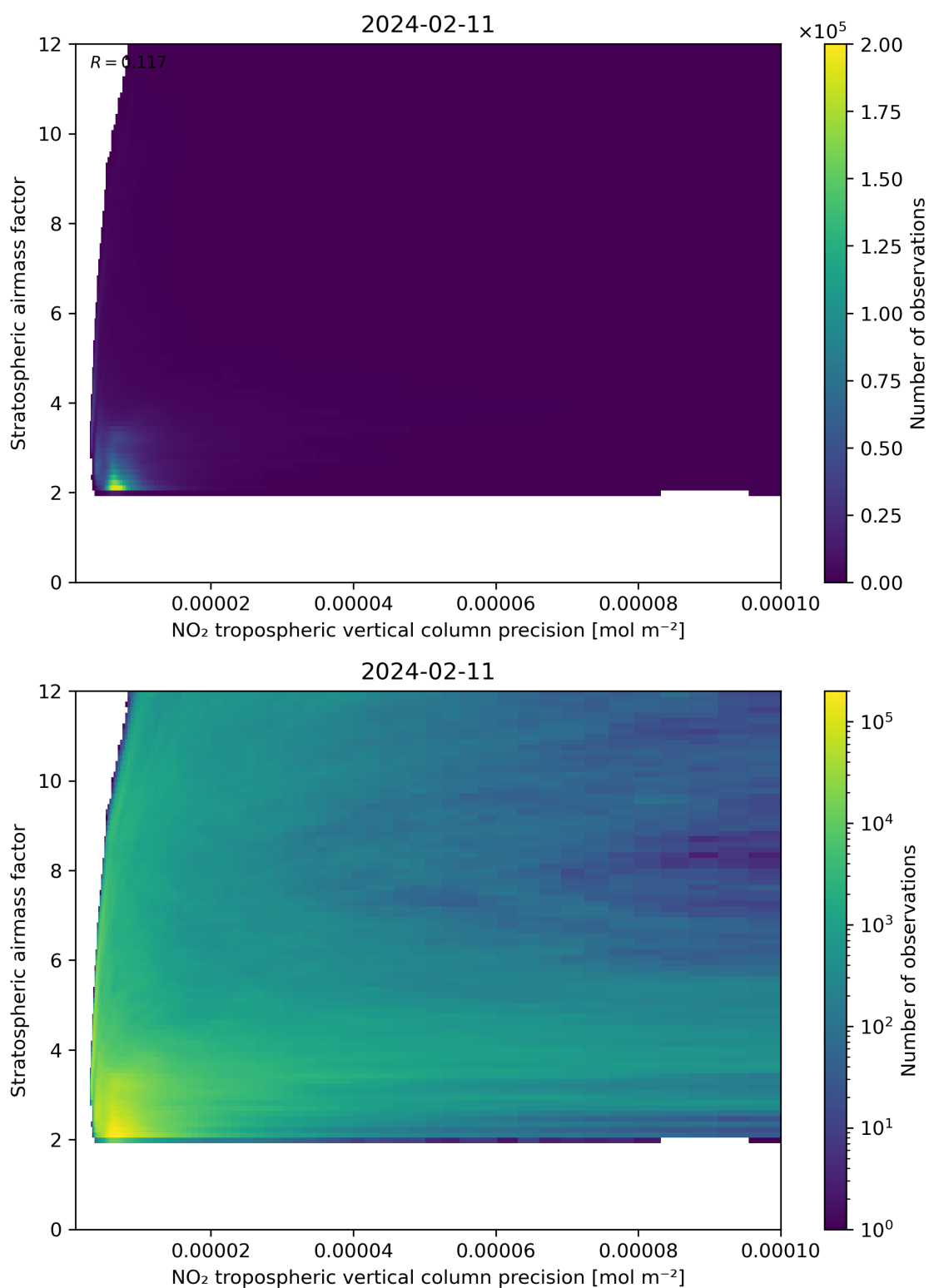
Figure 131: Scatter density plot of “NO 2 tropospheric vertical column precision” against “Stratospheric airmass factor” for 2024-02-11 to 2024-02-12.
