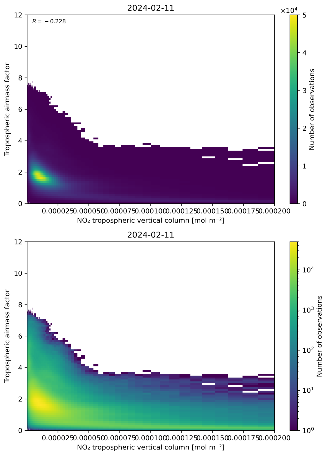
Figure 123: Scatter density plot of “NO 2 tropospheric vertical column” against “Tropospheric airmass factor” for 2024-02-11 to 2024-02-12.
