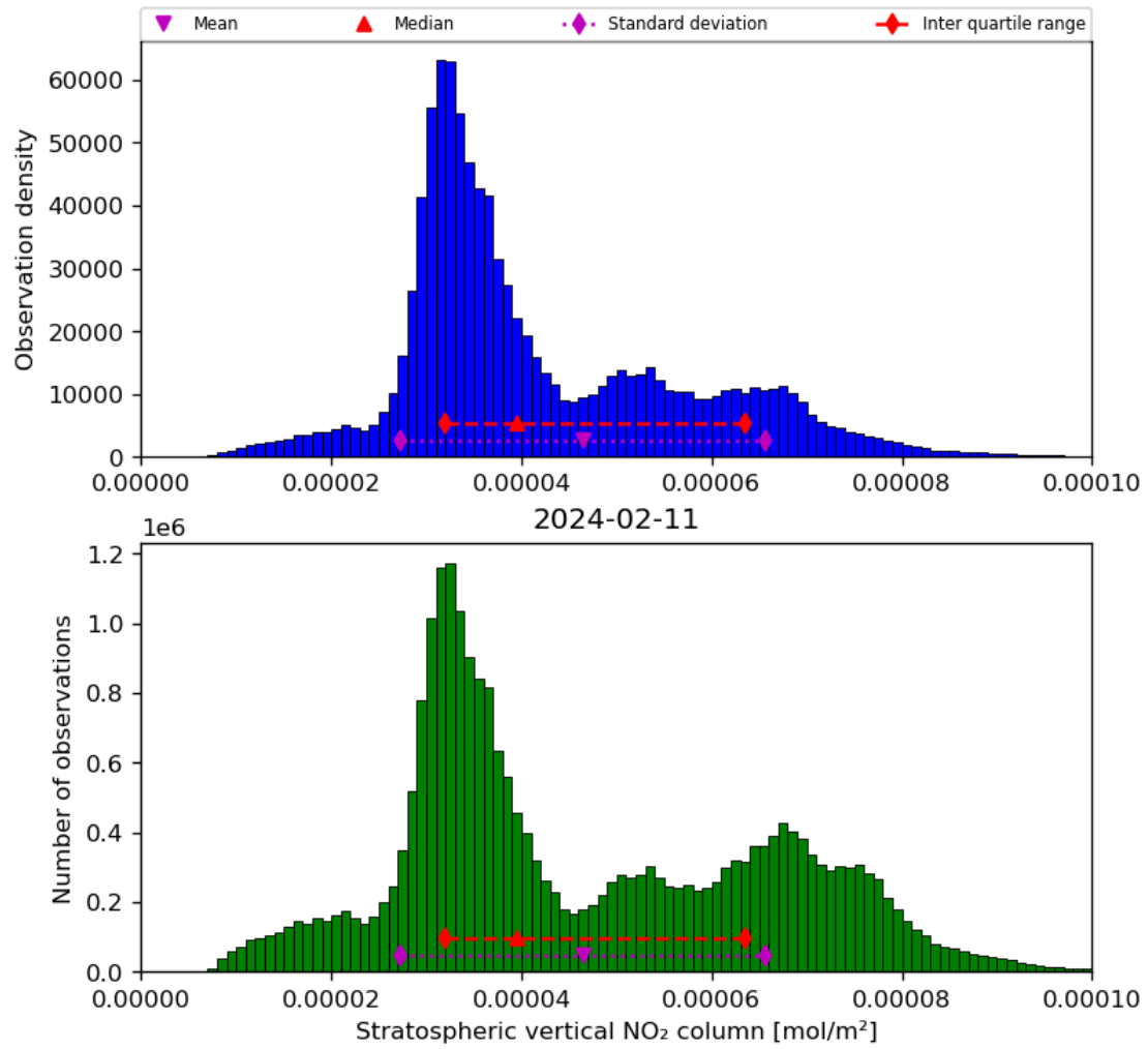
Figure 36: Histogram of “Stratospheric vertical NO 2 column” for 2024-02-11 to 2024-02-12
