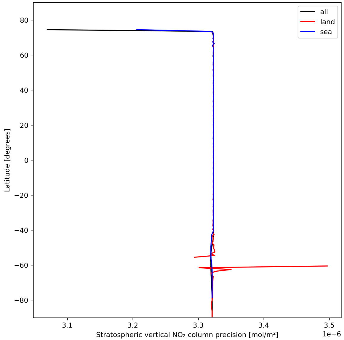
Figure 20: Zonal average of “Stratospheric vertical NO 2 column precision” for 2024-02-11 to 2024-02-12.
