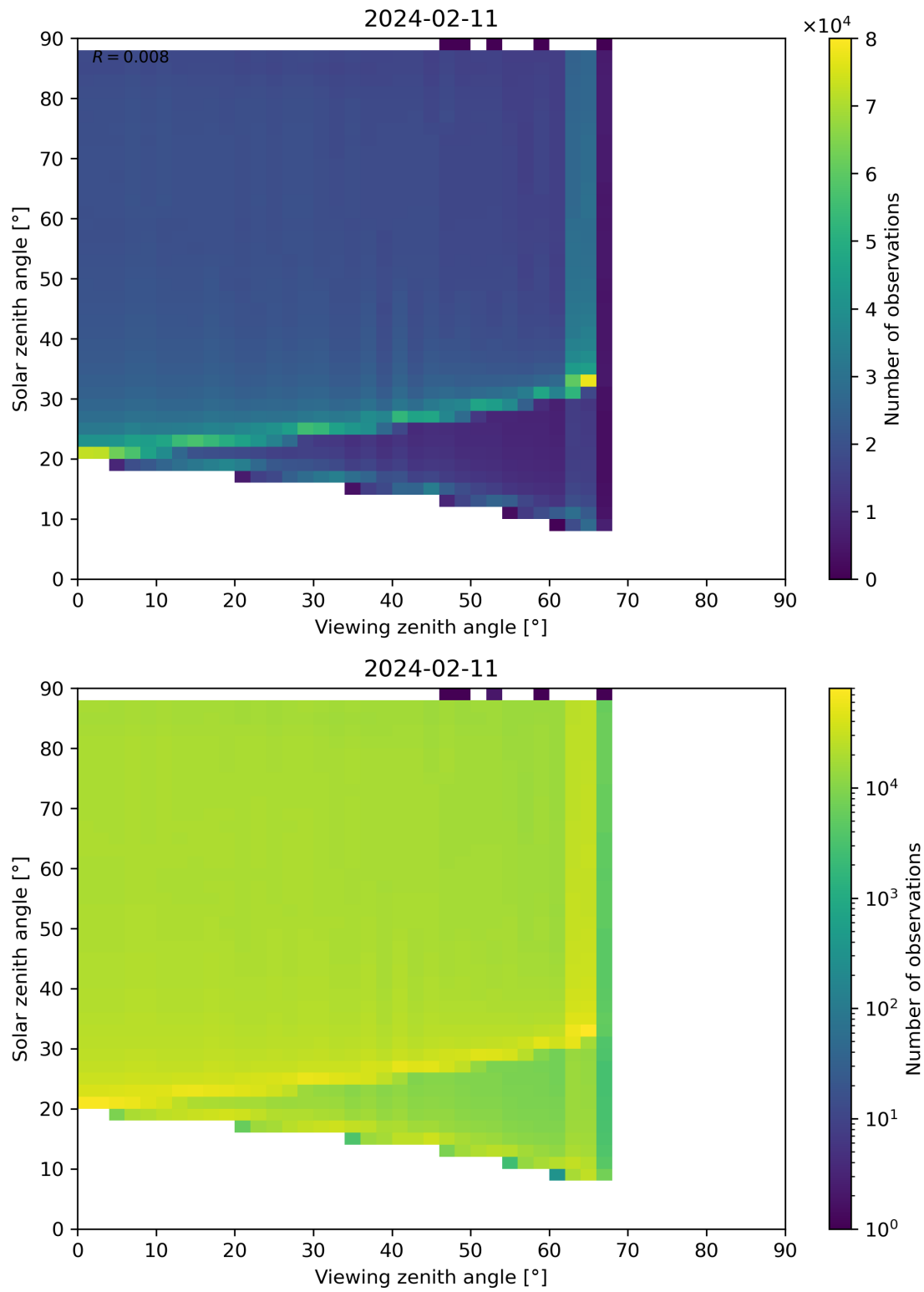
Figure 172: Scatter density plot of “Viewing zenith angle” against “Solar zenith angle” for 2024-02-11 to 2024-02-12.
