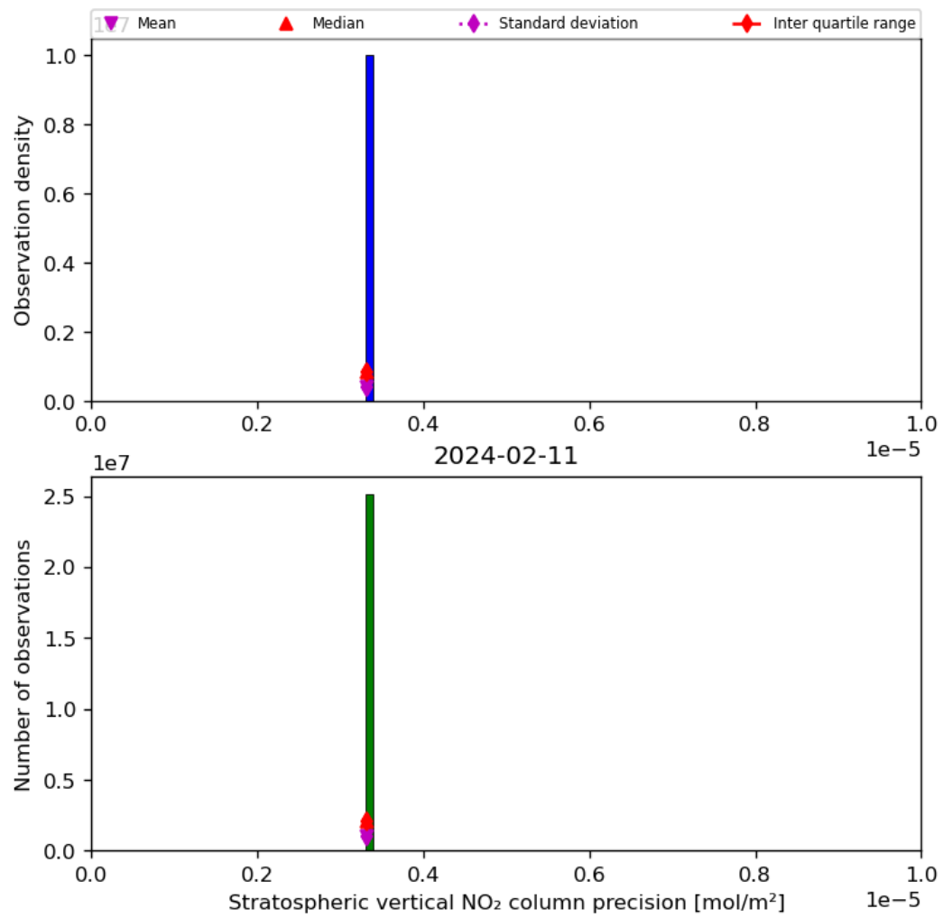
Figure 37: Histogram of “Stratospheric vertical NO 2 column precision” for 2024-02-11 to 2024-02-12
