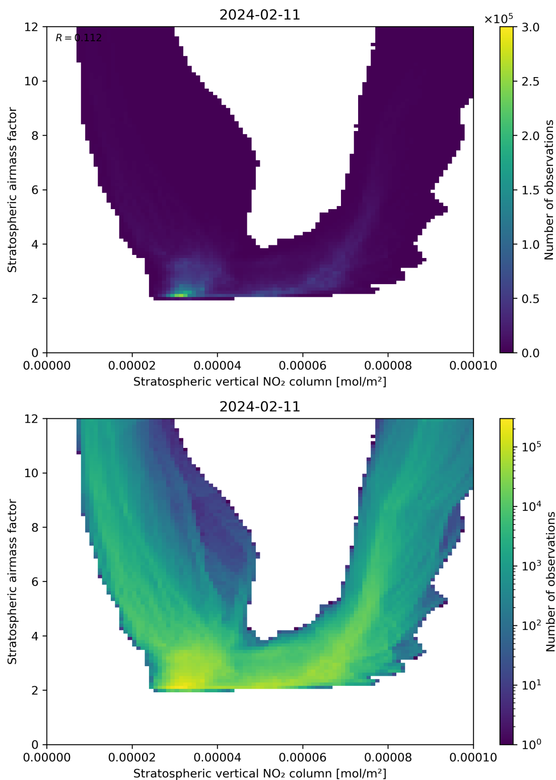
Figure 96: Scatter density plot of “Stratospheric vertical NO 2 column” against “Stratospheric airmass factor” for 2024-02-11 to 2024-02-12.
