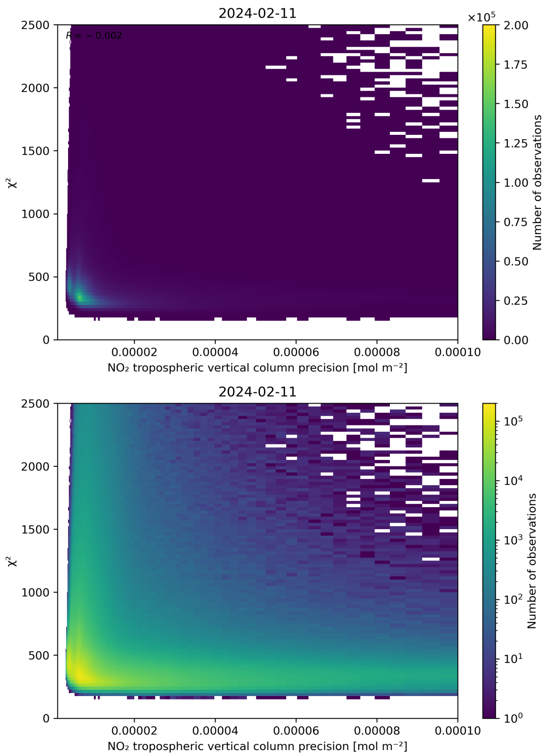
Figure 134: Scatter density plot of “NO 2 tropospheric vertical column precision” against “ \chi^2 ” for 2024-02-11 to 2024-02-12.
