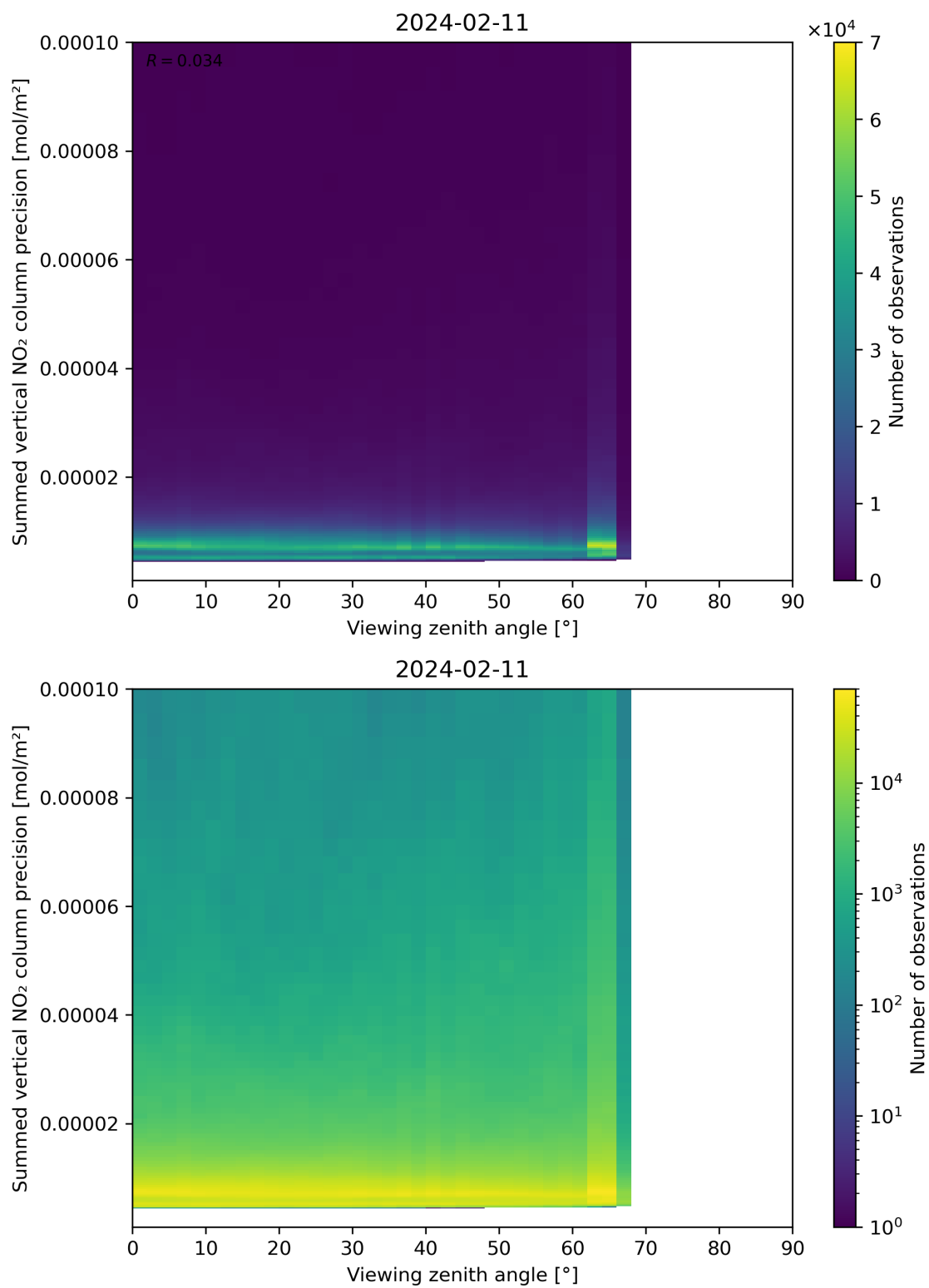
Figure 166: Scatter density plot of “Viewing zenith angle” against “Summed vertical NO 2 column precision” for 2024-02-11 to 2024-02-12.
