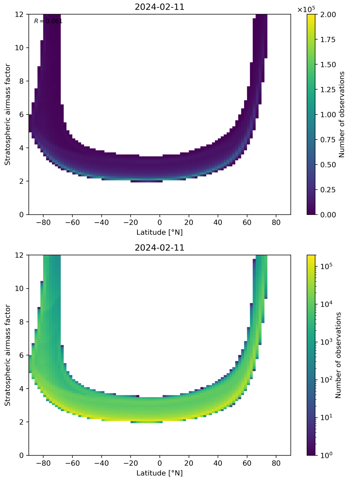
Figure 83: Scatter density plot of “Latitude” against “Stratospheric air mass factor” for 2024-02-11 to 2024-02-12.
