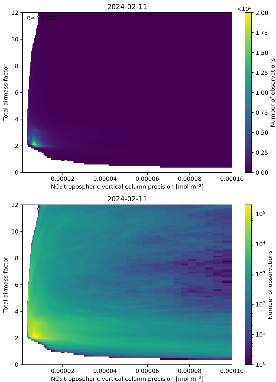
Figure 132: Scatter density plot of “NO 2 tropospheric vertical column precision” against “Total air mass factor” for 2024-02-11 to 2024-02-12.
