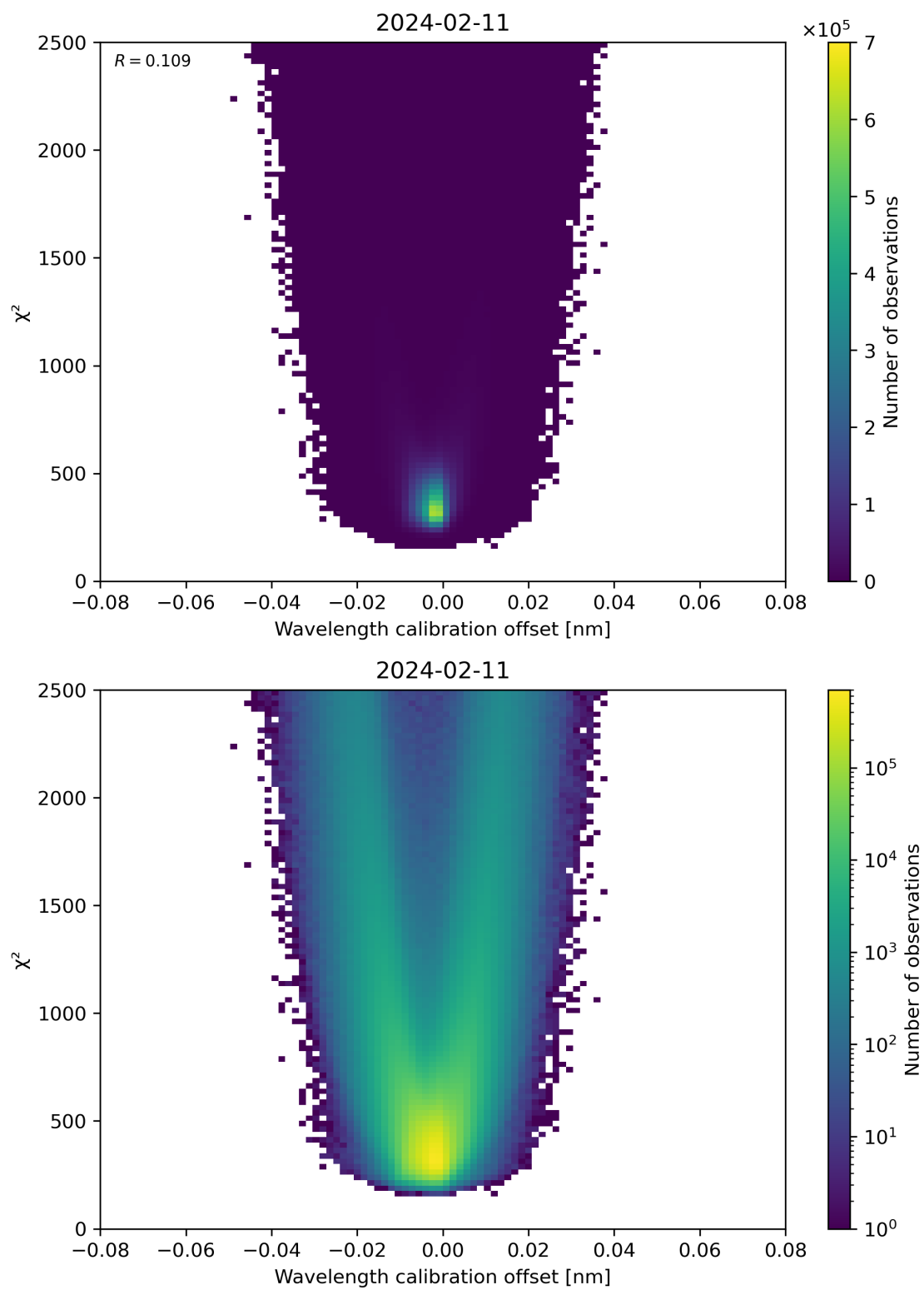
Figure 175: Scatter density plot of “Wavelength calibration offset” against “ \chi^2 ” for 2024-02-11 to 2024-02-12.
