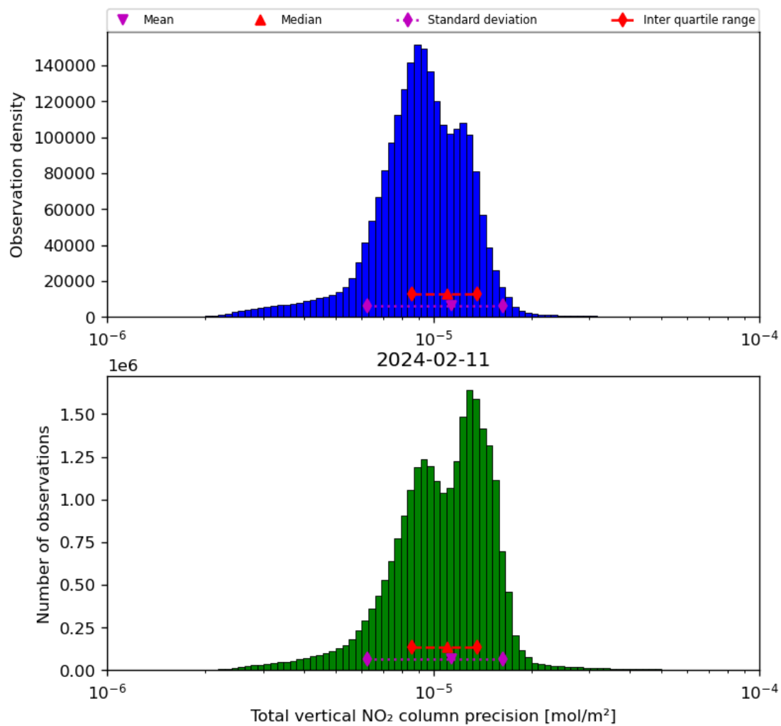
Figure 39: Histogram of “Total vertical NO 2 column precision” for 2024-02-11 to 2024-02-12
