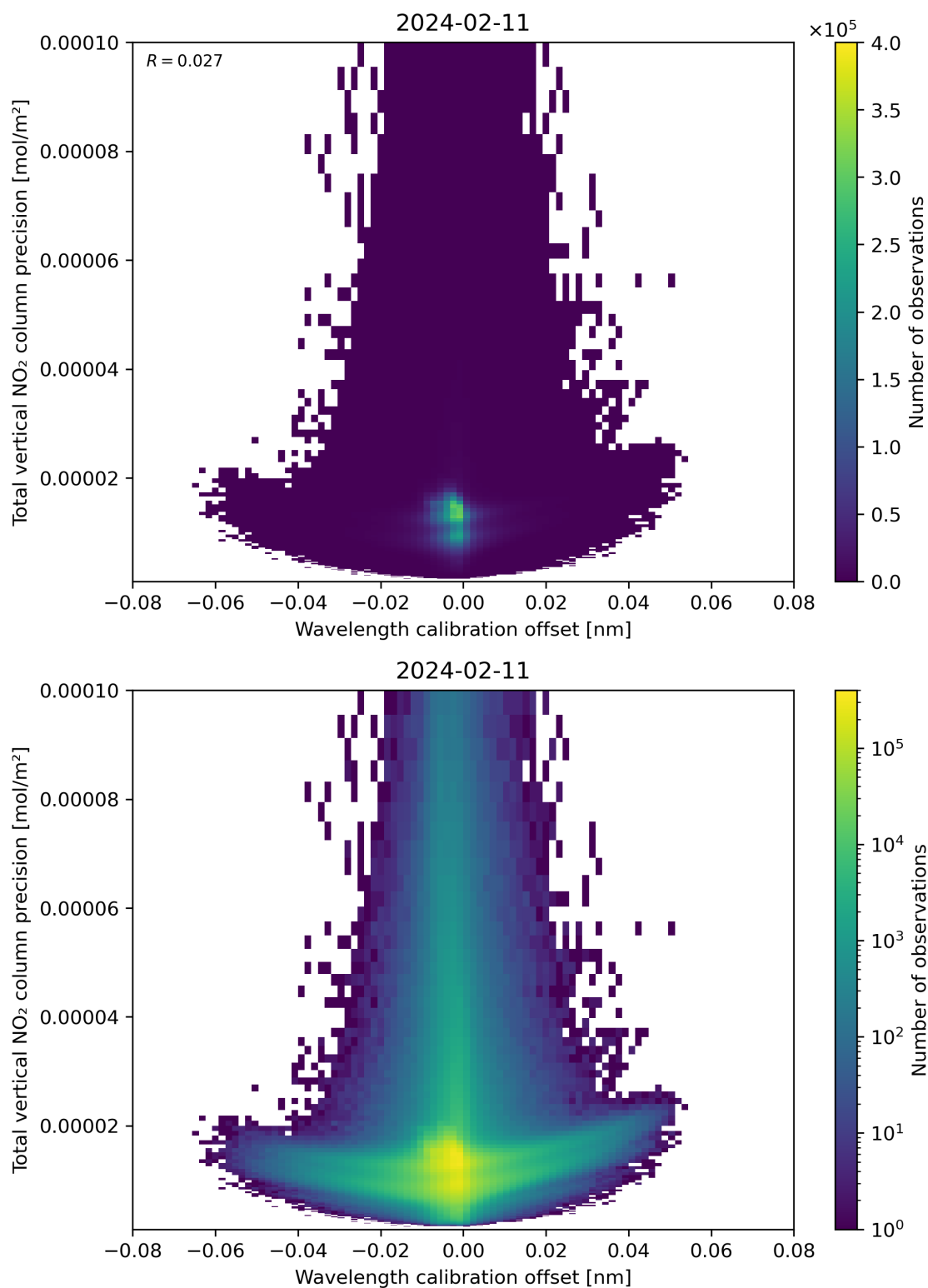
Figure 180: Scatter density plot of “Wavelength calibration offset” against “Total vertical NO 2 column precision” for 2024-02-11 to 2024-02-12.
