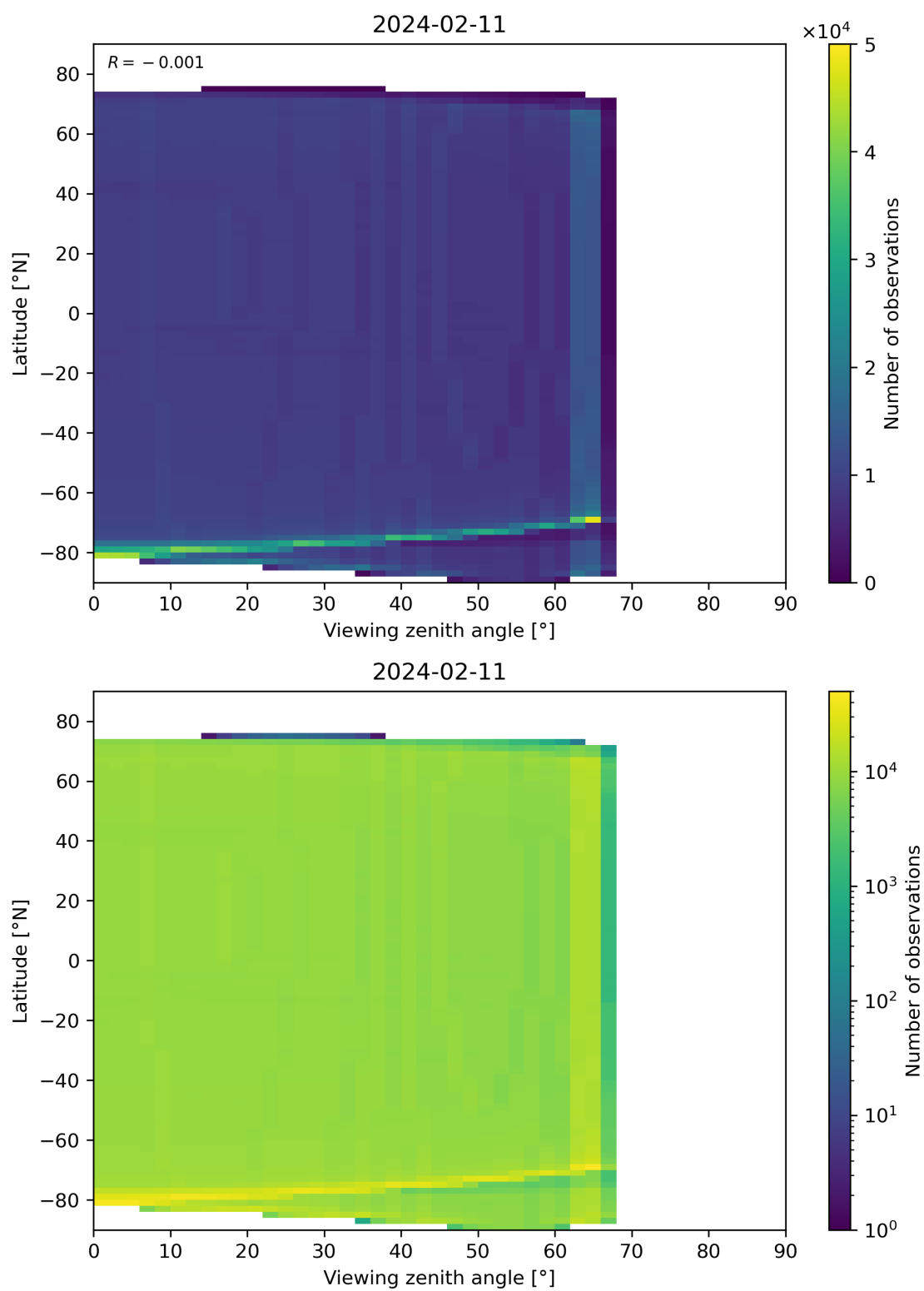
Figure 163: Scatter density plot of “Viewing zenith angle” against “Latitude” for 2024-02-11 to 2024-02-12.
