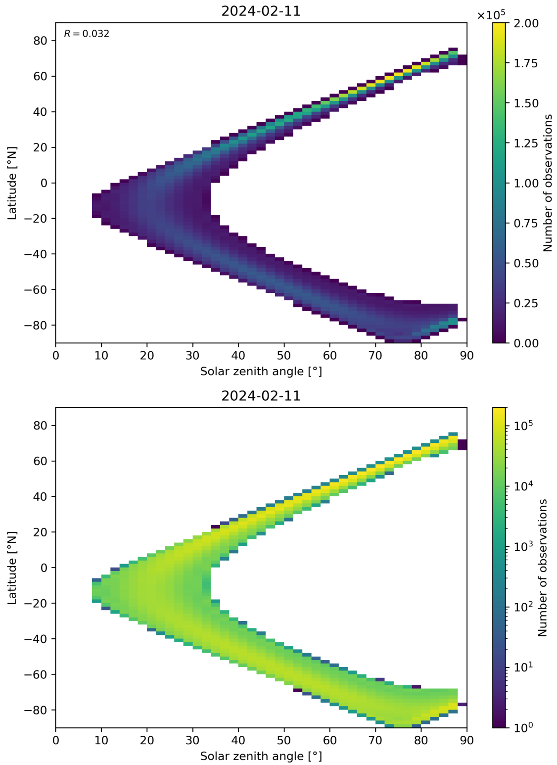
Figure 149: Scatter density plot of “Solar zenith angle” against “Latitude” for 2024-02-11 to 2024-02-12.
