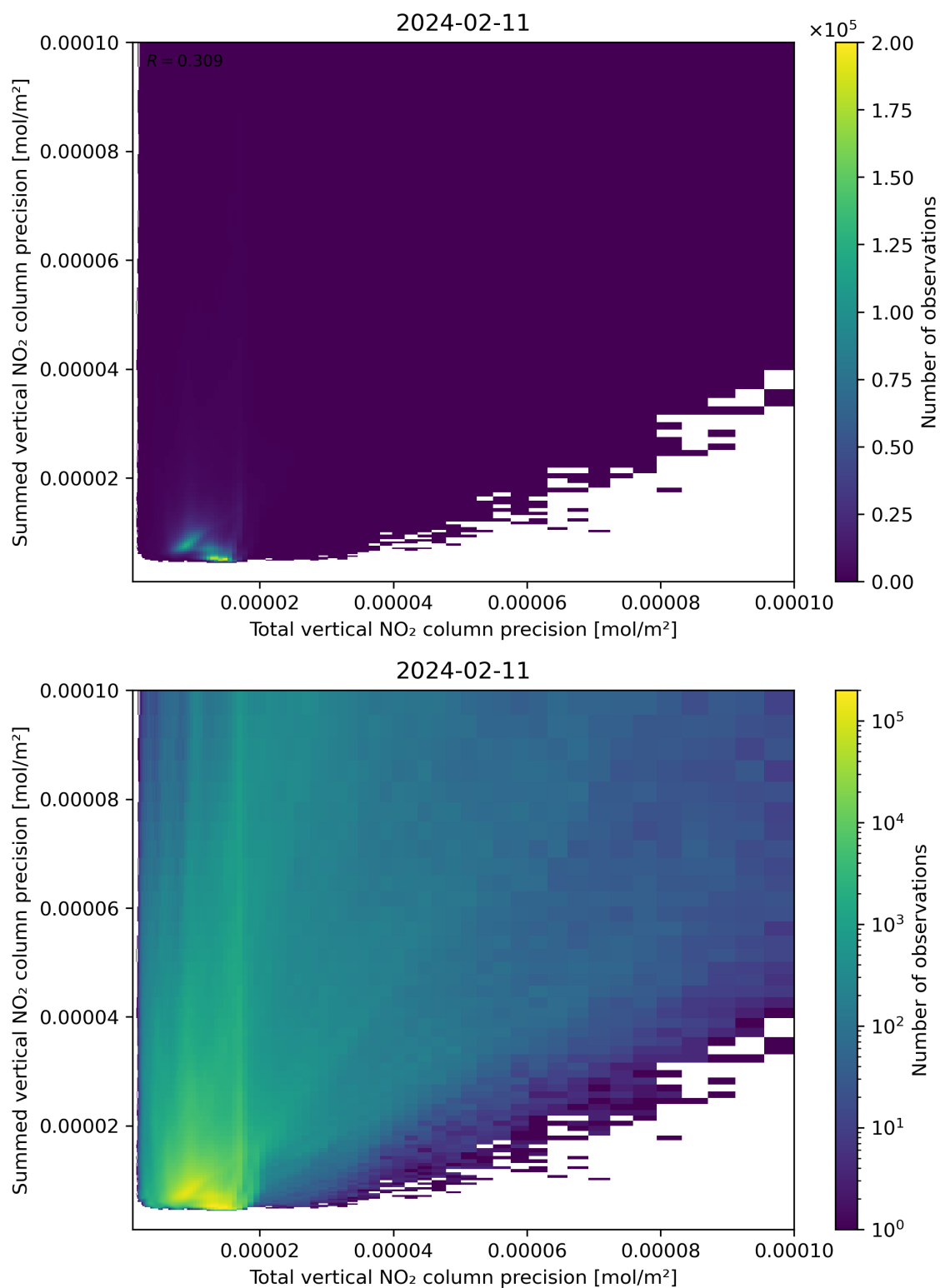
Figure 118: Scatter density plot of “Total vertical NO 2 column precision” against “Summed vertical NO 2 column precision” for 2024-02-11 to 2024-02-12.
