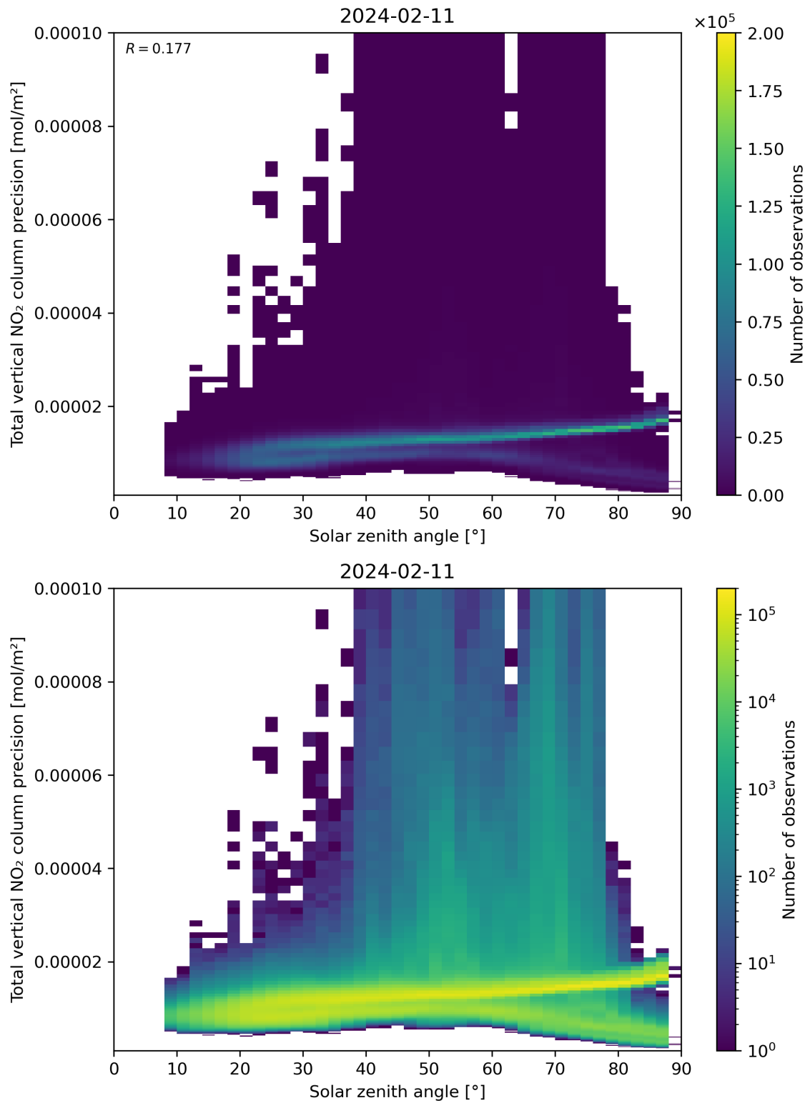
Figure 154: Scatter density plot of “Solar zenith angle” against “Total vertical NO 2 column precision” for 2024-02-11 to 2024-02-12.
