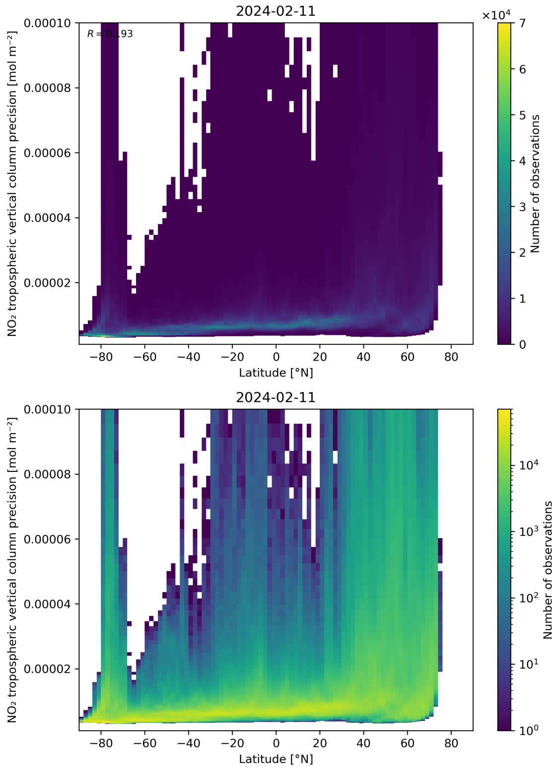
Figure 93: Scatter density plot of “Latitude” against “NO 2 tropospheric vertical column precision” for 2024-02-11 to 2024-02-12.
