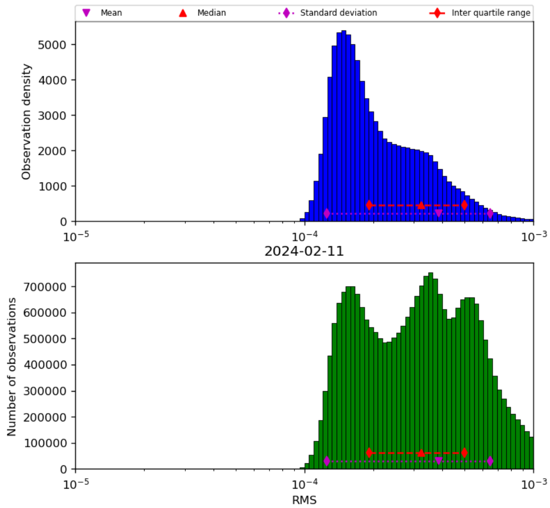
Figure 43: Histogram of “RMS” for 2024-02-11 to 2024-02-12
