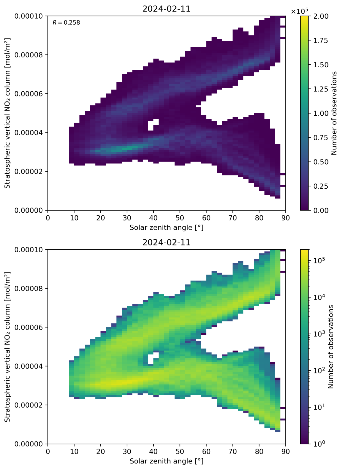
Figure 150: Scatter density plot of “Solar zenith angle” against “Stratospheric vertical NO 2 column” for 2024-02-11 to 2024-02-12.
