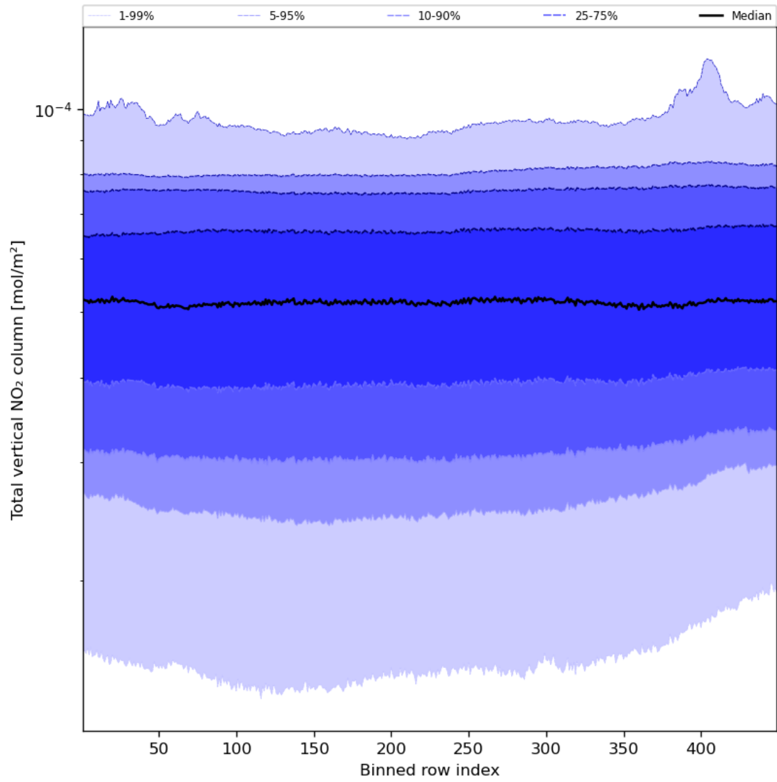
Figure 55: Along track statistics of “Total vertical NO 2 column” for 2024-02-11 to 2024-02-12
