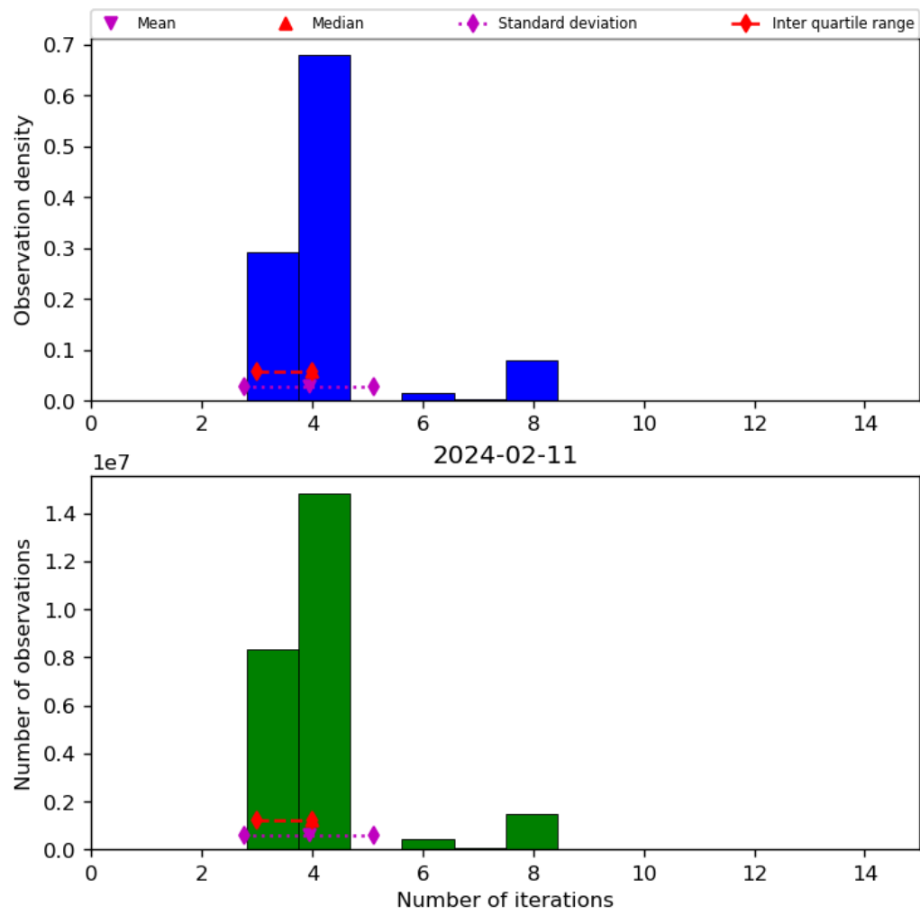
Figure 34: Histogram of “Number of iterations” for 2024-02-11 to 2024-02-12
