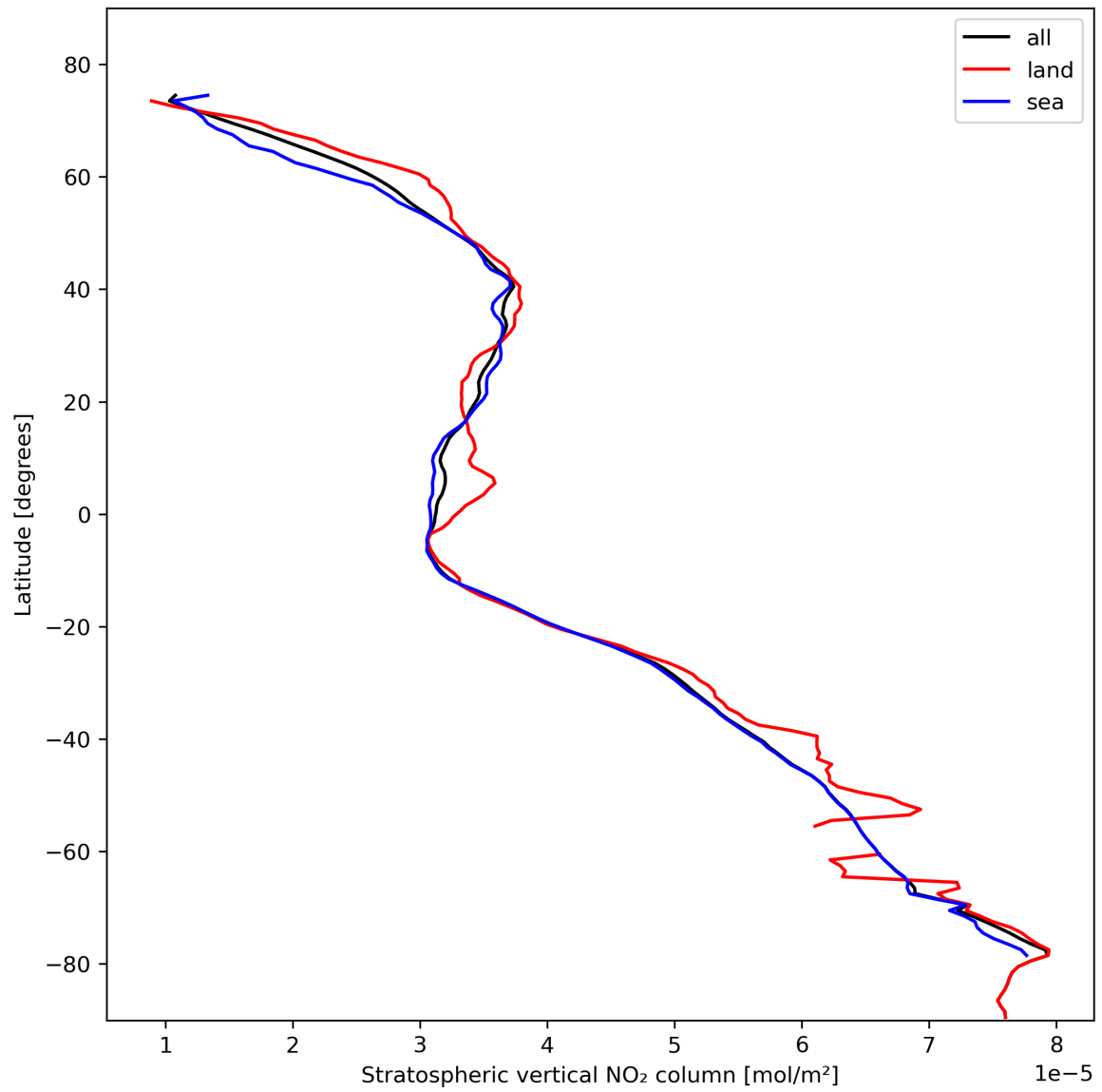
Figure 19: Zonal average of “Stratospheric vertical NO 2 column” for 2024-02-11 to 2024-02-12.
