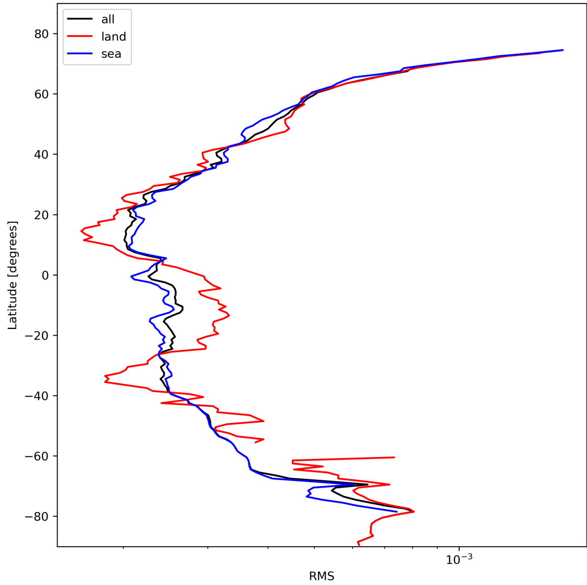
Figure 26: Zonal average of “RMS” for 2024-02-11 to 2024-02-12.
