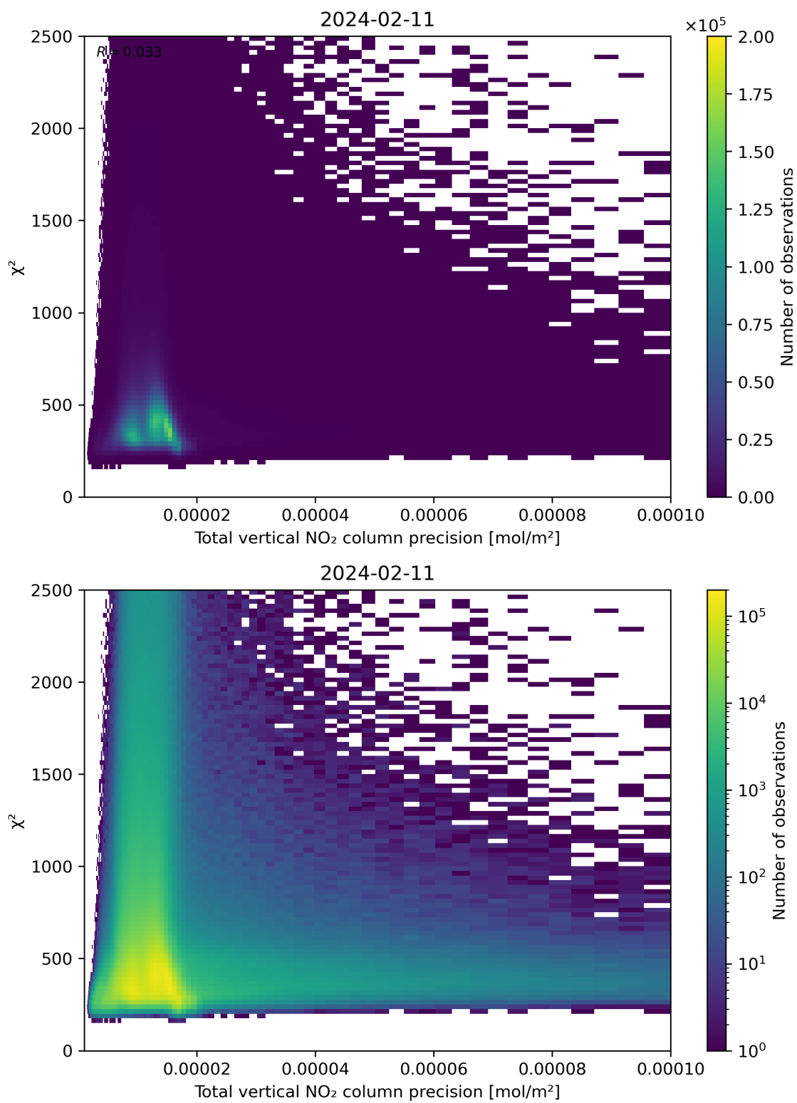
Figure 116: Scatter density plot of “Total vertical NO 2 column precision” against “ \chi^2 ” for 2024-02-11 to 2024-02-12.
