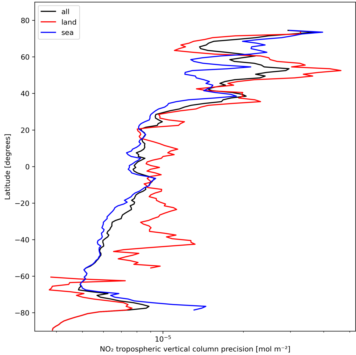
Figure 13: Zonal average of “NO 2 tropospheric vertical column precision” for 2024-02-11 to 2024-02-12.
