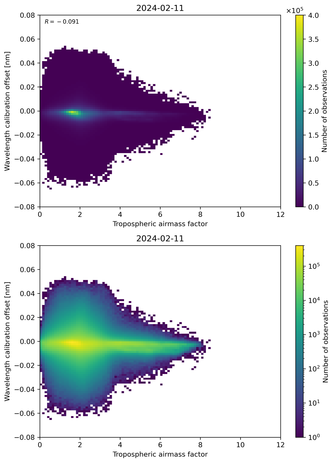
Figure 80: Scatter density plot of “Tropospheric airmass factor” against “Wavelength calibration offset” for 2024-02-11 to 2024-02-12.
