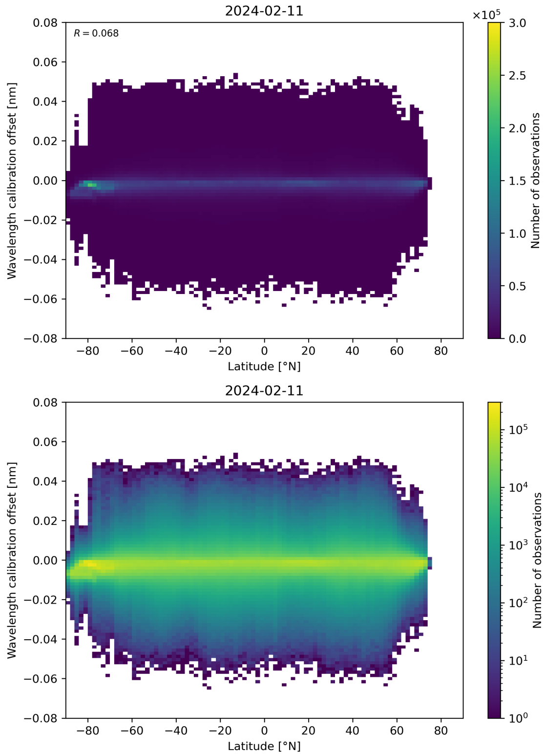
Figure 95: Scatter density plot of “Latitude” against “Wavelength calibration offset” for 2024-02-11 to 2024-02-12.
