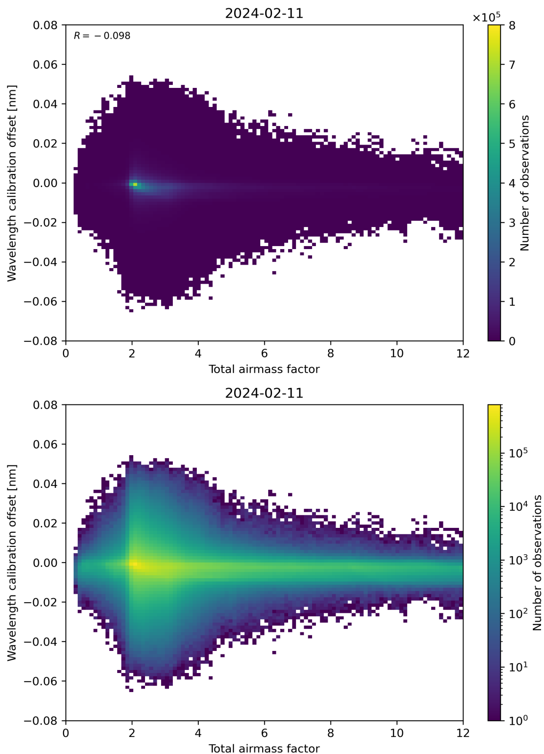
Figure 70: Scatter density plot of “Total airmass factor” against “Wavelength calibration offset” for 2024-02-11 to 2024-02-12.
