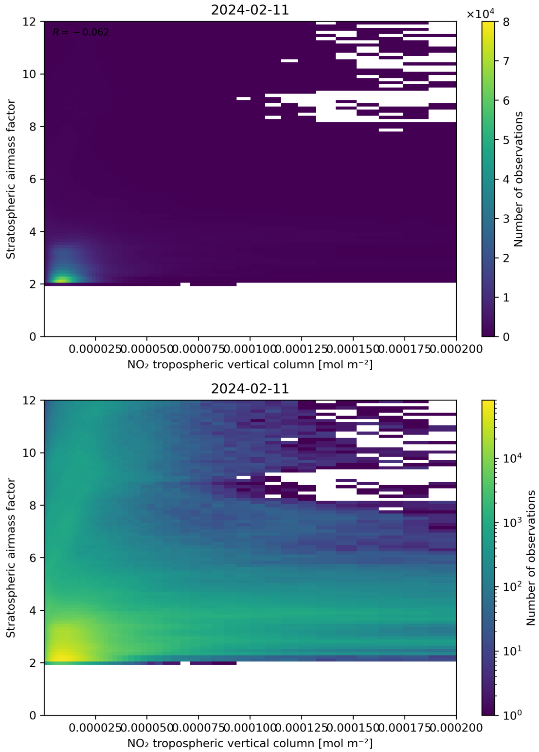
Figure 121: Scatter density plot of “NO 2 tropospheric vertical column” against “Stratospheric air mass factor” for 2024-02-11 to 2024-02-12.
