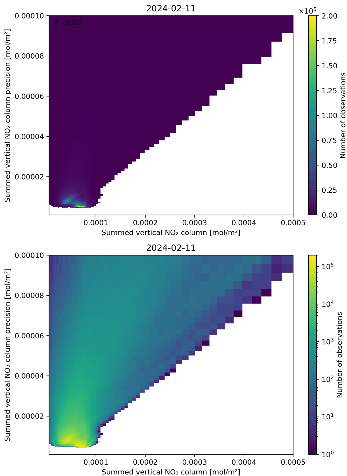
Figure 105: Scatter density plot of “Summed vertical NO 2 column” against “Summed vertical NO 2 column precision” for 2024-02-11 to 2024-02-12.
