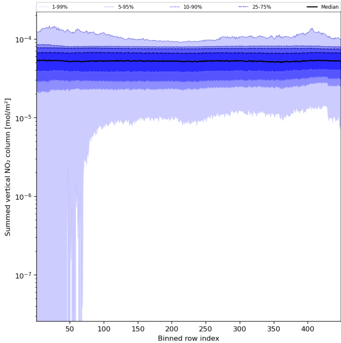
Figure 57: Along track statistics of “Summed vertical NO 2 column” for 2024-02-11 to 2024-02-12
