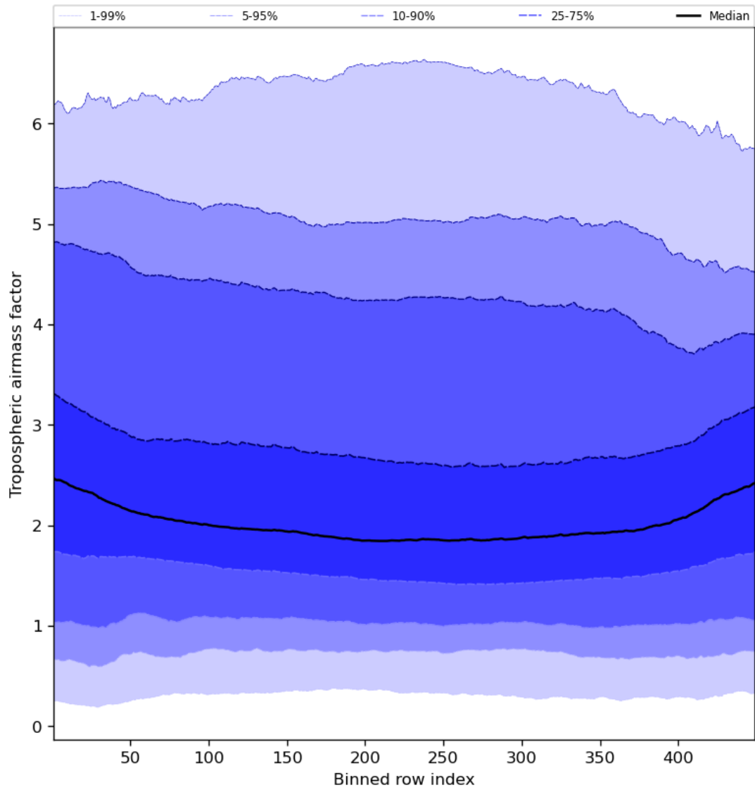
Figure 48: Along track statistics of “Tropospheric airmass factor” for 2024-02-11 to 2024-02-12
