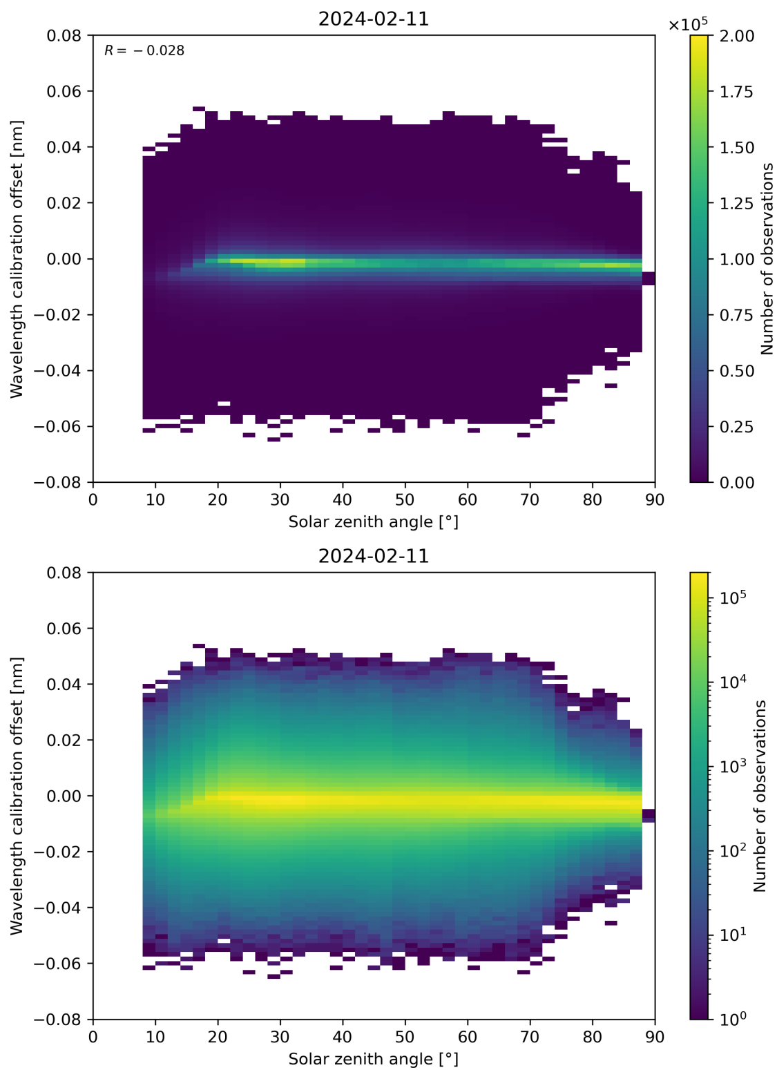
Figure 158: Scatter density plot of “Solar zenith angle” against “Wavelength calibration offset” for 2024-02-11 to 2024-02-12.
