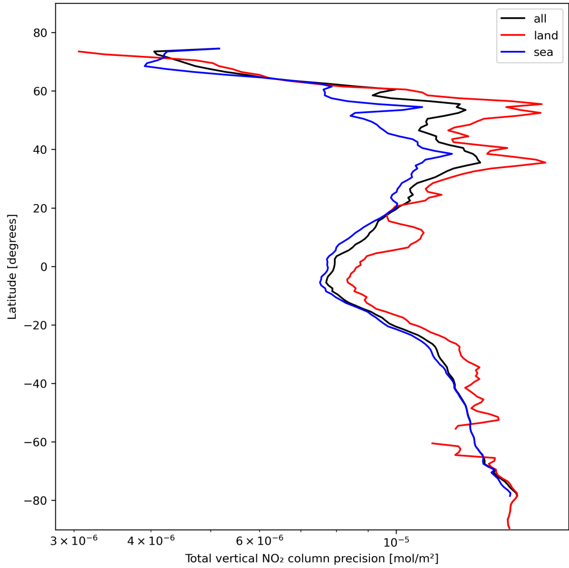
Figure 22: Zonal average of “Total vertical NO 2 column precision” for 2024-02-11 to 2024-02-12.
