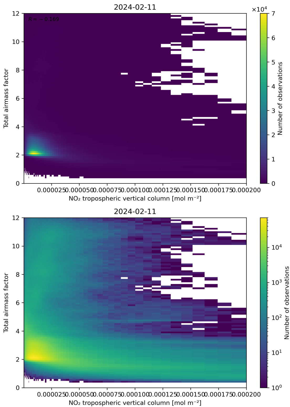
Figure 122: Scatter density plot of “NO 2 tropospheric vertical column” against “Total air mass factor” for 2024-02-11 to 2024-02-12.
