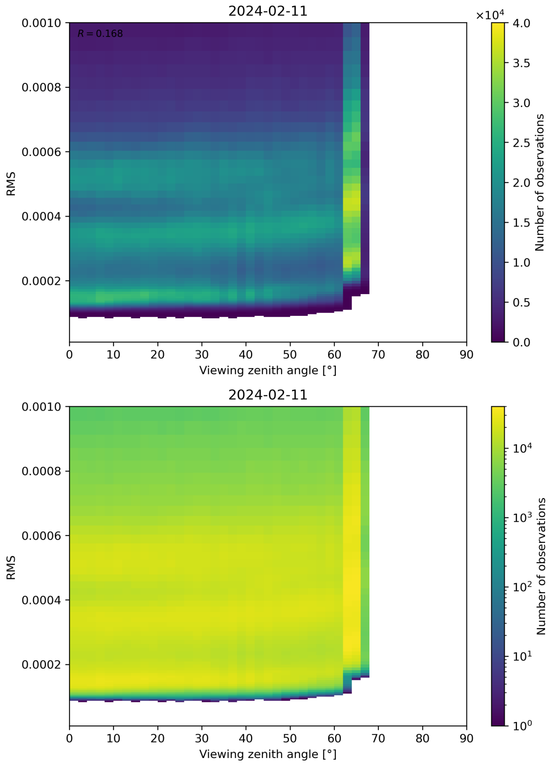
Figure 171: Scatter density plot of “Viewing zenith angle” against “RMS” for 2024-02-11 to 2024-02-12.
