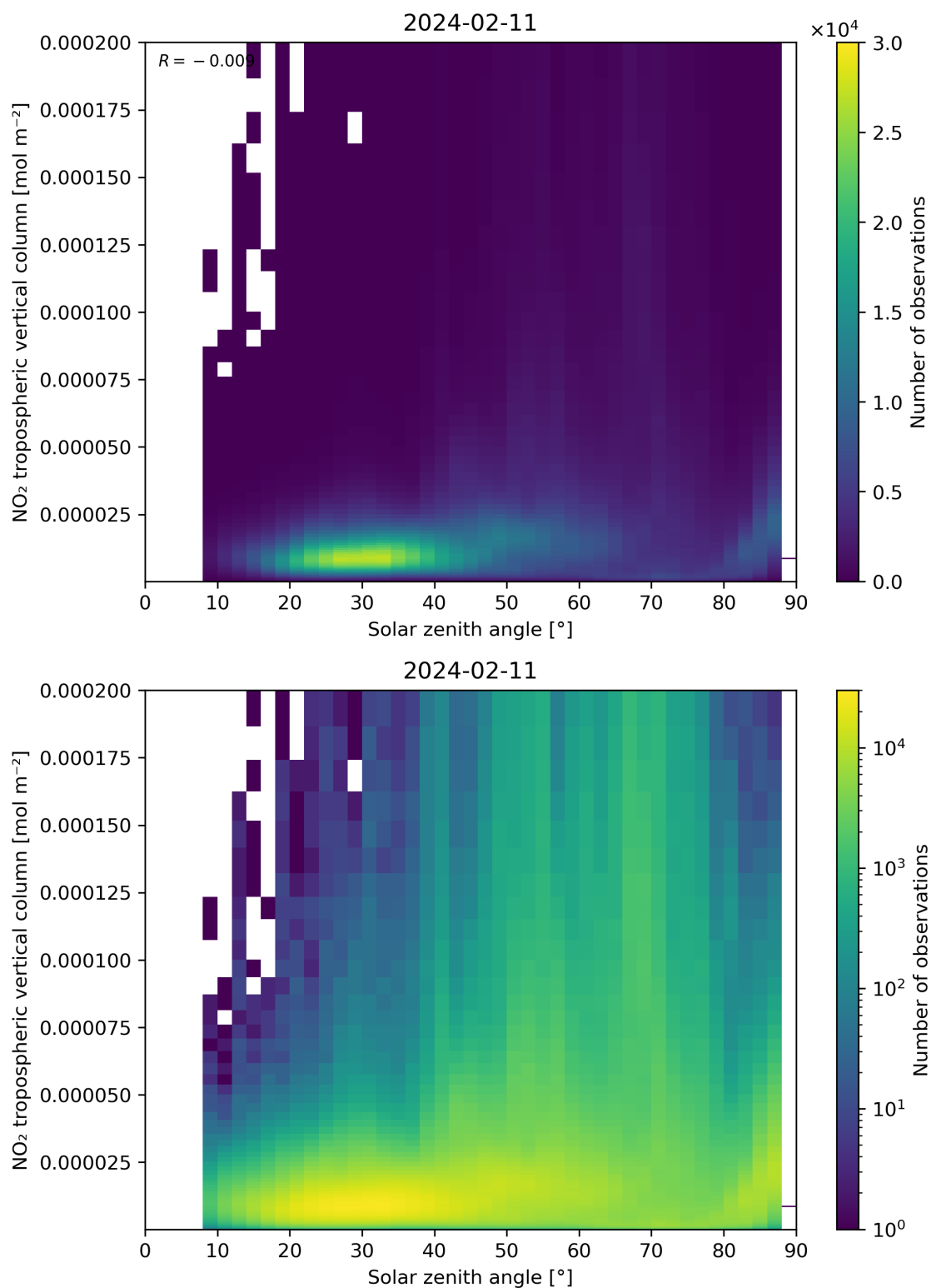
Figure 155: Scatter density plot of “Solar zenith angle” against “NO 2 tropospheric vertical column” for 2024-02-11 to 2024-02-12.
