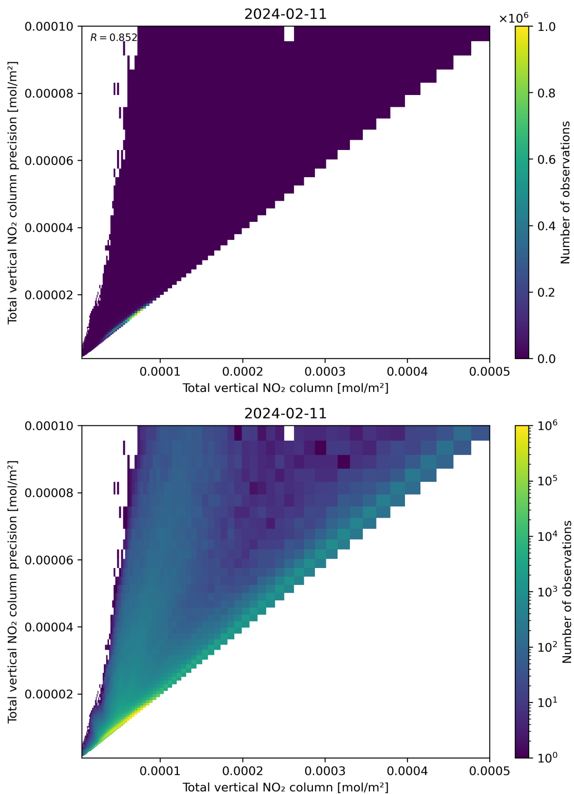
Figure 114: Scatter density plot of “Total vertical NO 2 column” against “Total vertical NO 2 column precision” for 2024-02-11 to 2024-02-12.
