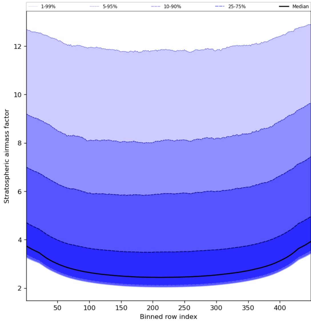
Figure 61: Along track statistics of “Stratospheric airmass factor” for 2024-02-11 to 2024-02-12
