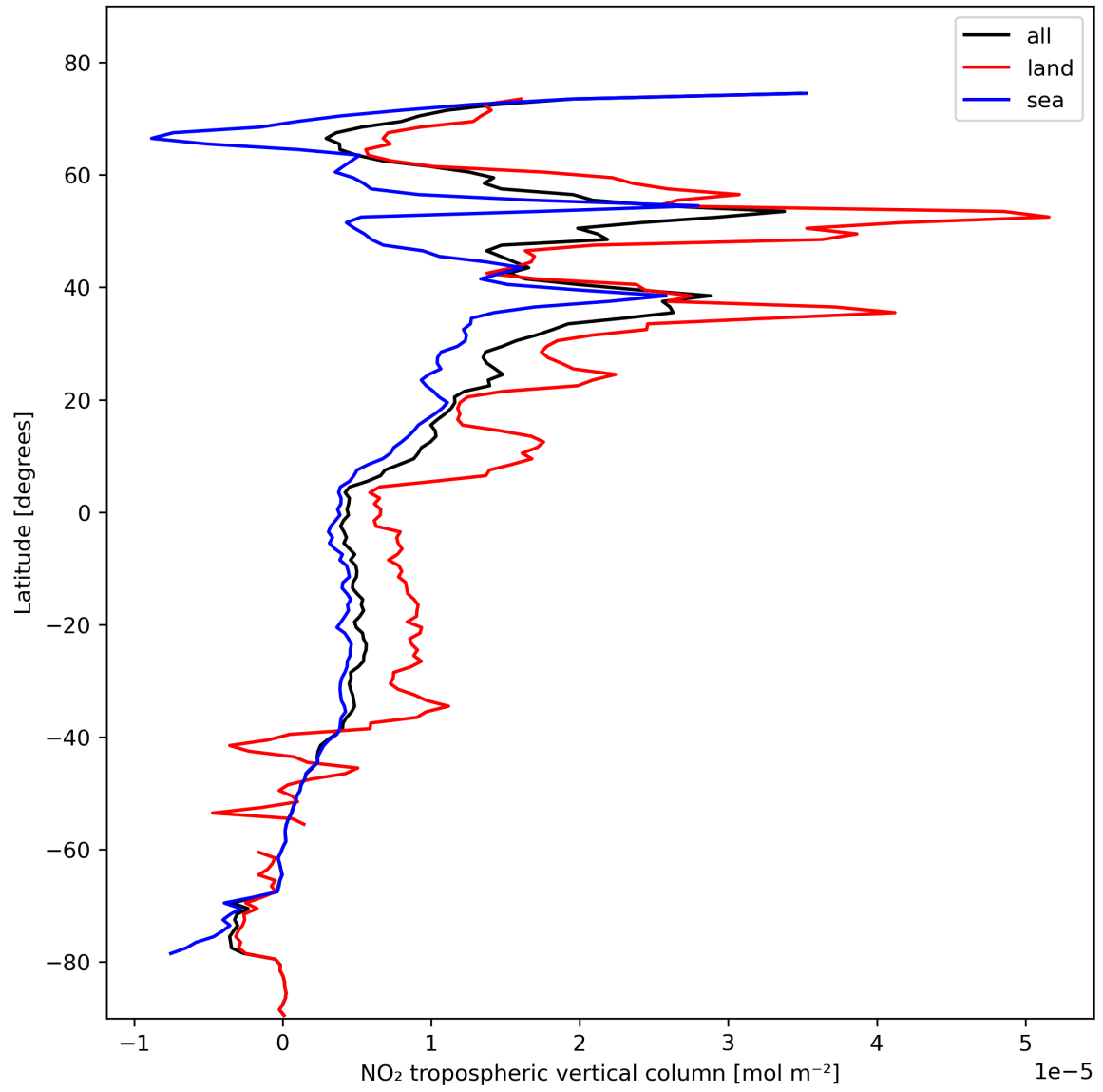
Figure 12: Zonal average of “NO 2 tropospheric vertical column” for 2024-02-11 to 2024-02-12.
