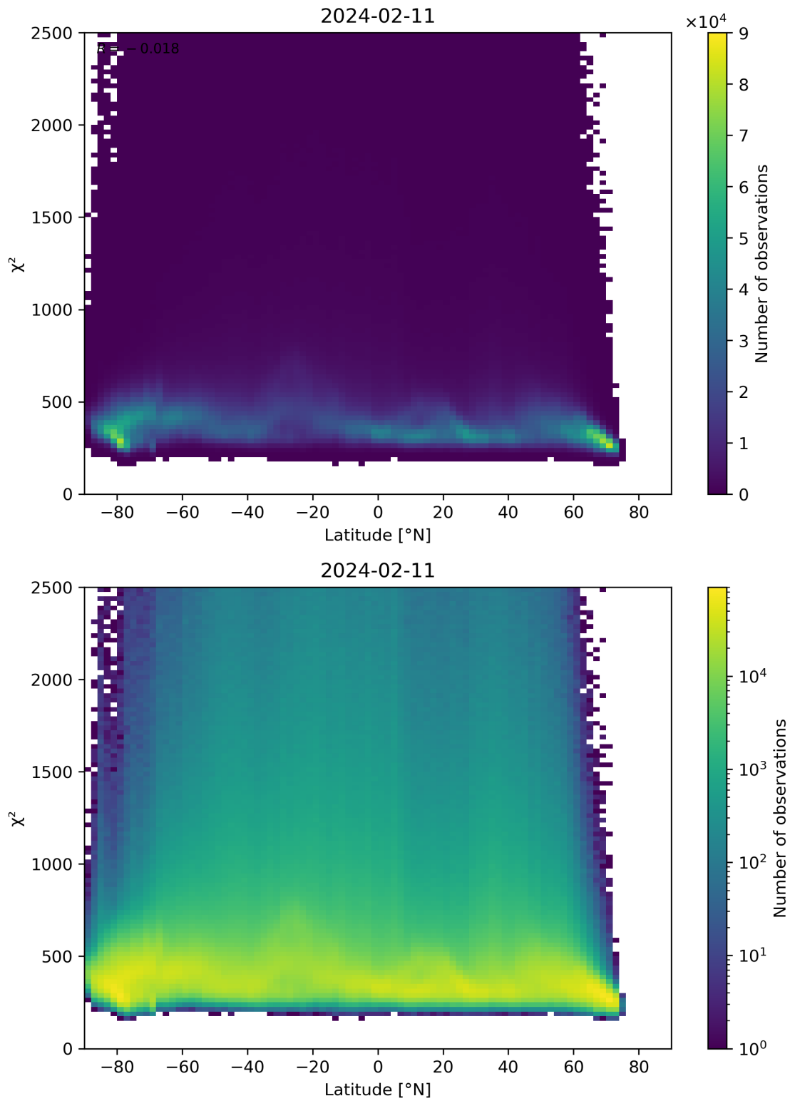
Figure 86: Scatter density plot of “Latitude” against “ \chi^2 ” for 2024-02-11 to 2024-02-12.
