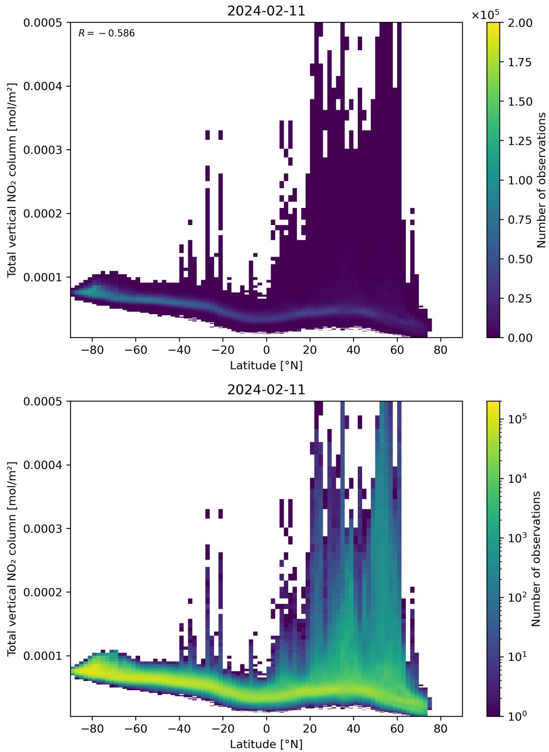
Figure 90: Scatter density plot of “Latitude” against “Total vertical NO 2 column” for 2024-02-11 to 2024-02-12.
