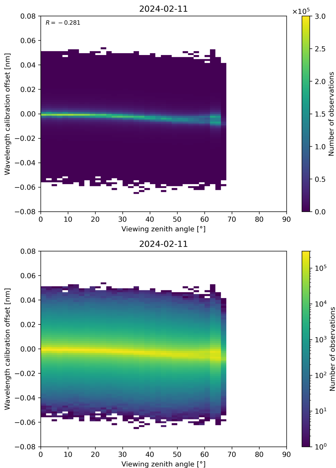
Figure 173: Scatter density plot of “Viewing zenith angle” against “Wavelength calibration offset” for 2024-02-11 to 2024-02-12.
