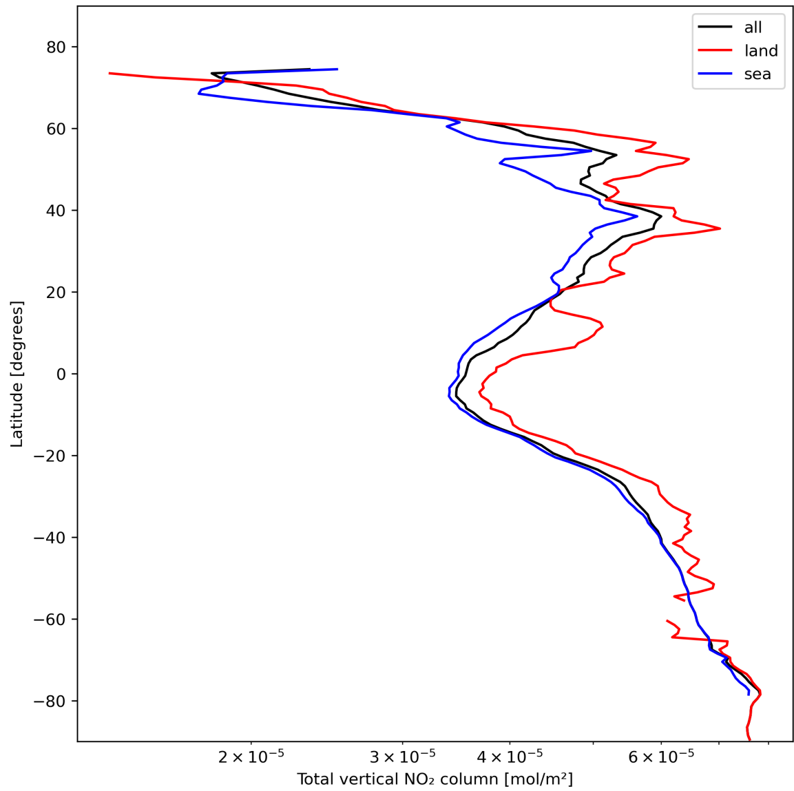
Figure 21: Zonal average of “Total vertical NO 2 column” for 2024-02-11 to 2024-02-12.
