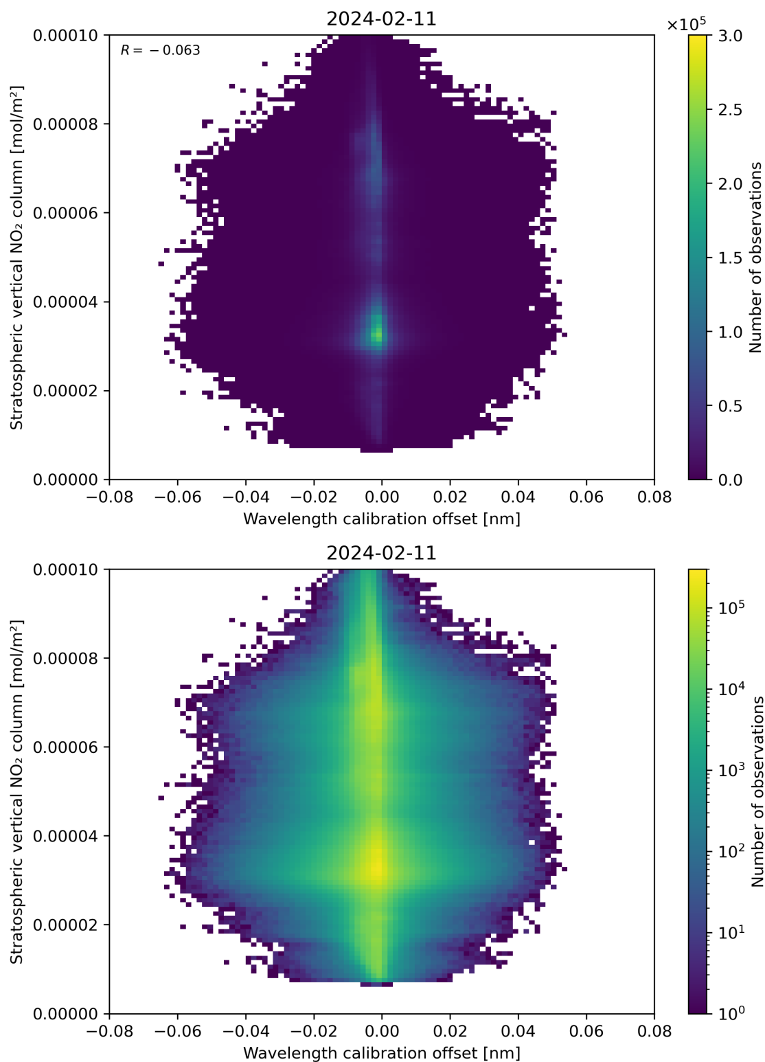
Figure 176: Scatter density plot of “Wavelength calibration offset” against “Stratospheric vertical NO 2 column” for 2024-02-11 to 2024-02-12.
