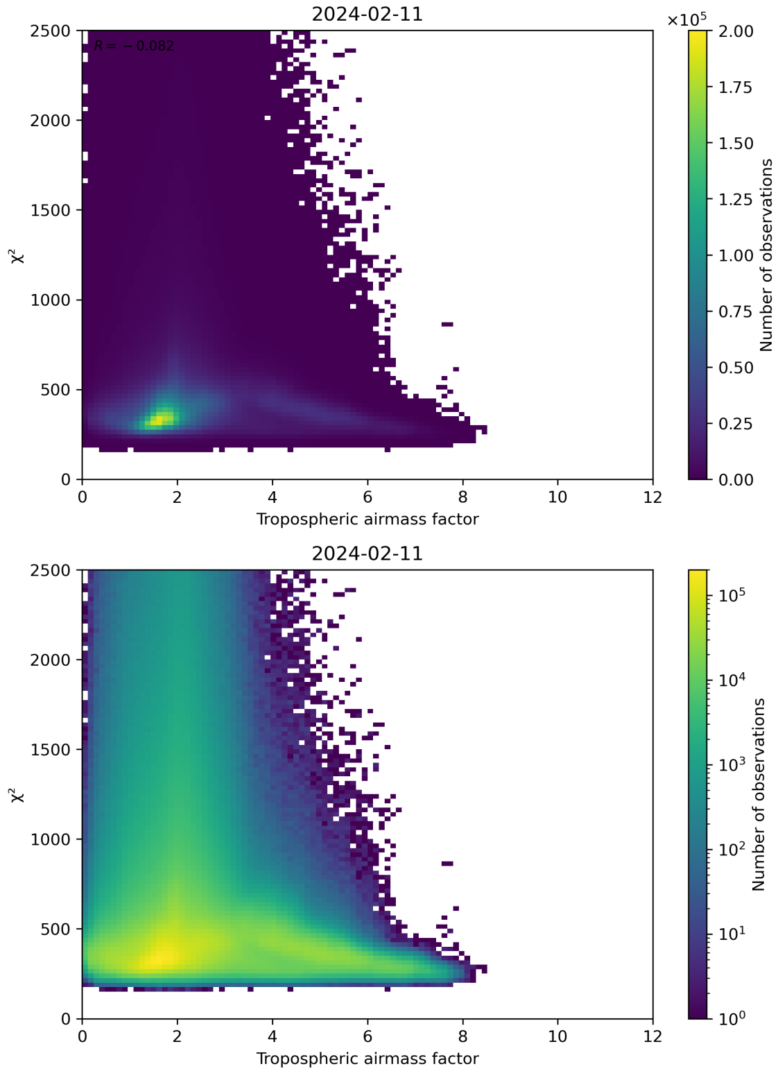
Figure 73: Scatter density plot of “Tropospheric airmass factor” against “ \chi^2 ” for 2024-02-11 to 2024-02-12.
