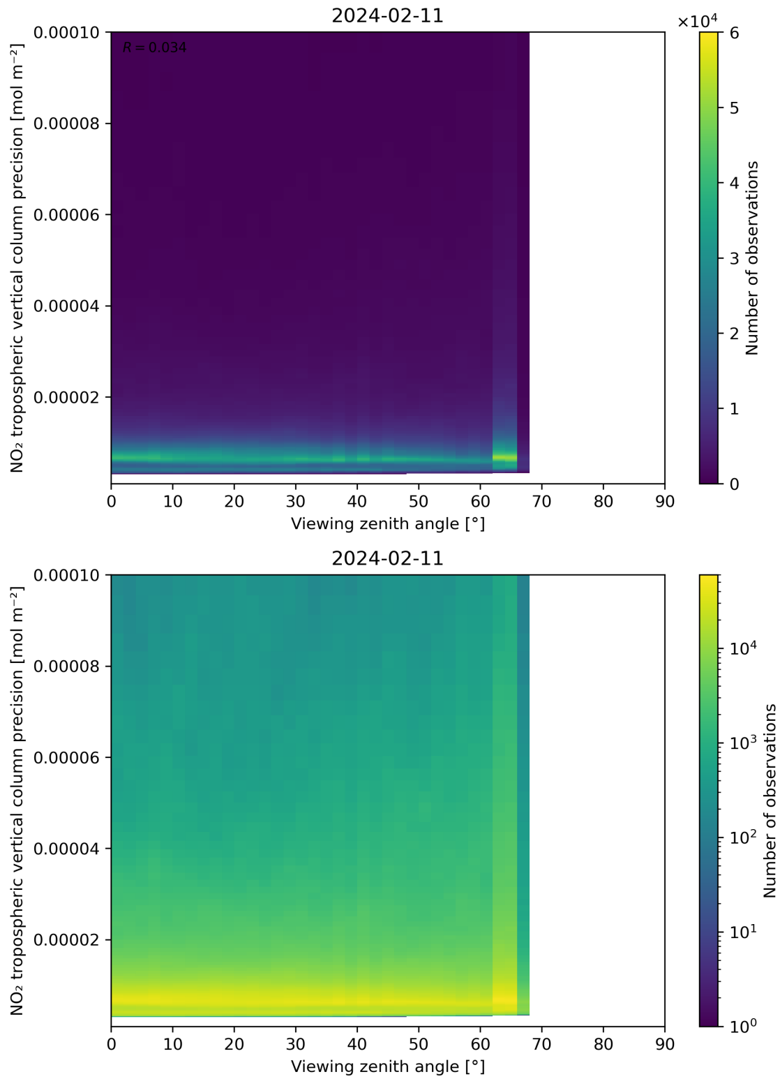
Figure 170: Scatter density plot of “Viewing zenith angle” against “NO 2 tropospheric vertical column precision” for 2024-02-11 to 2024-02-12.
