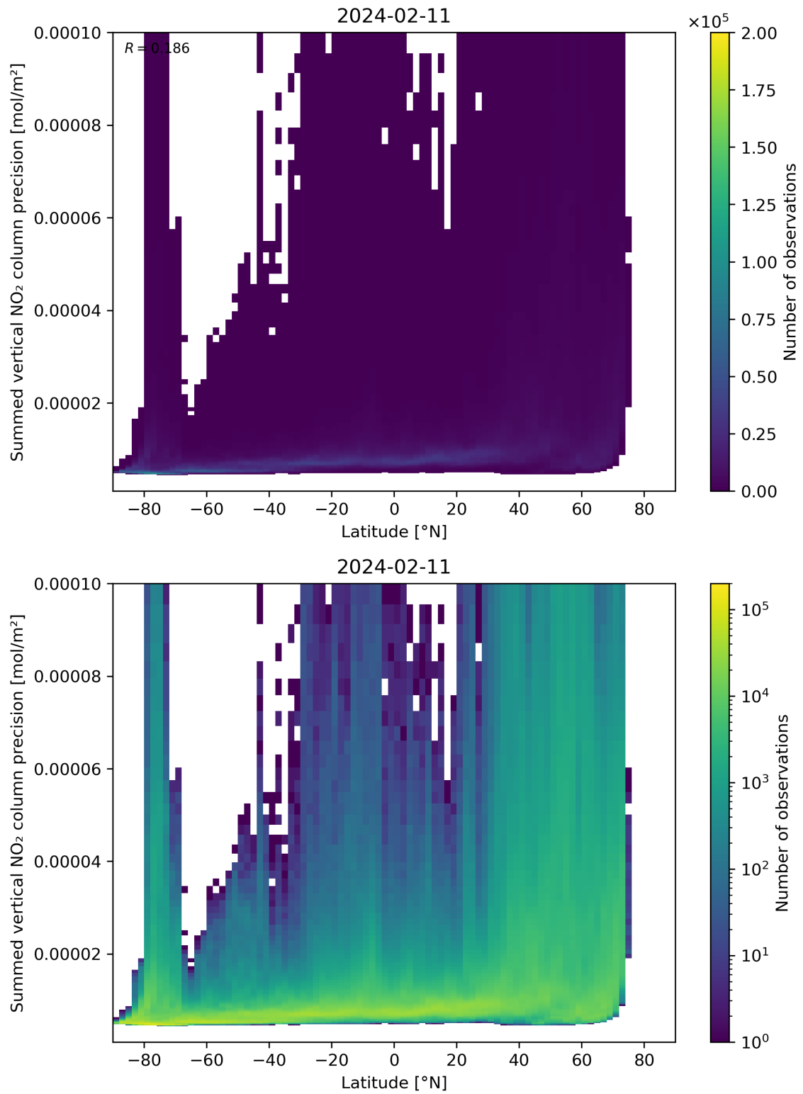
Figure 89: Scatter density plot of “Latitude” against “Summed vertical NO 2 column precision” for 2024-02-11 to 2024-02-12.
