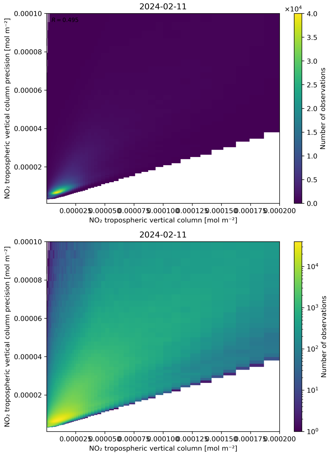
Figure 130: Scatter density plot of “NO 2 tropospheric vertical column” against “NO 2 tropospheric vertical column precision” for 2024-02-11 to 2024-02-12.
