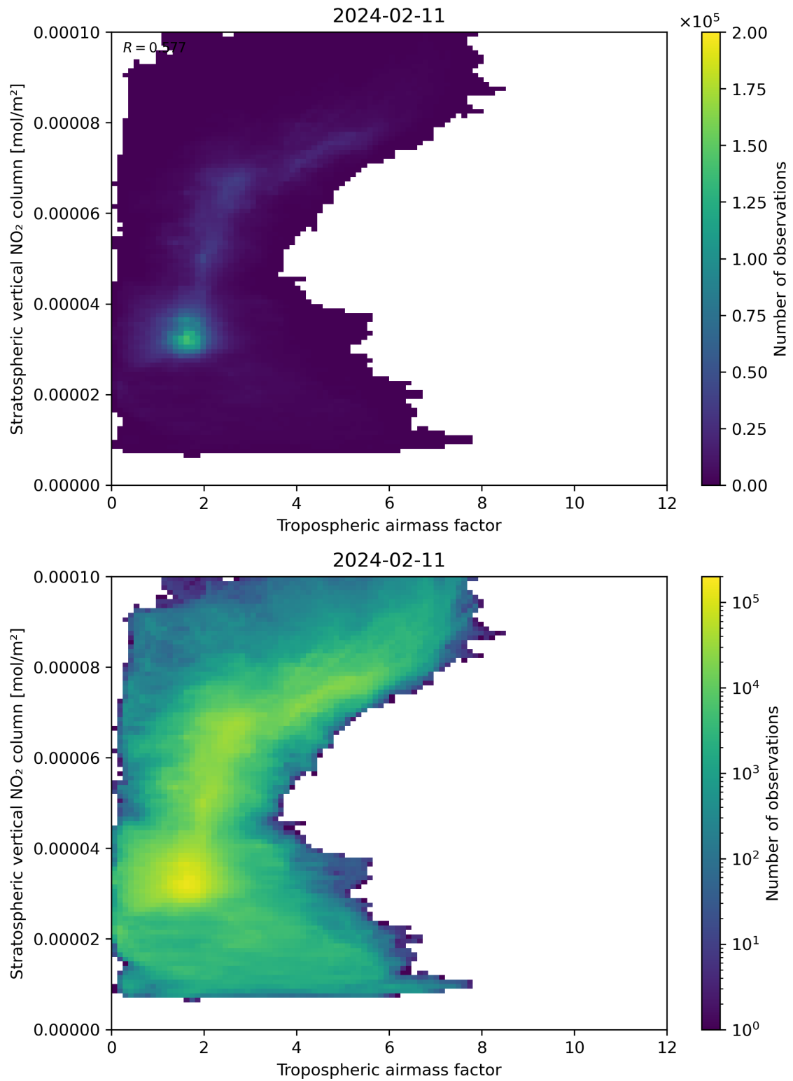
Figure 74: Scatter density plot of “Tropospheric air mass factor” against “Stratospheric vertical NO 2 column” for 2024-02-11 to 2024-02-12.
