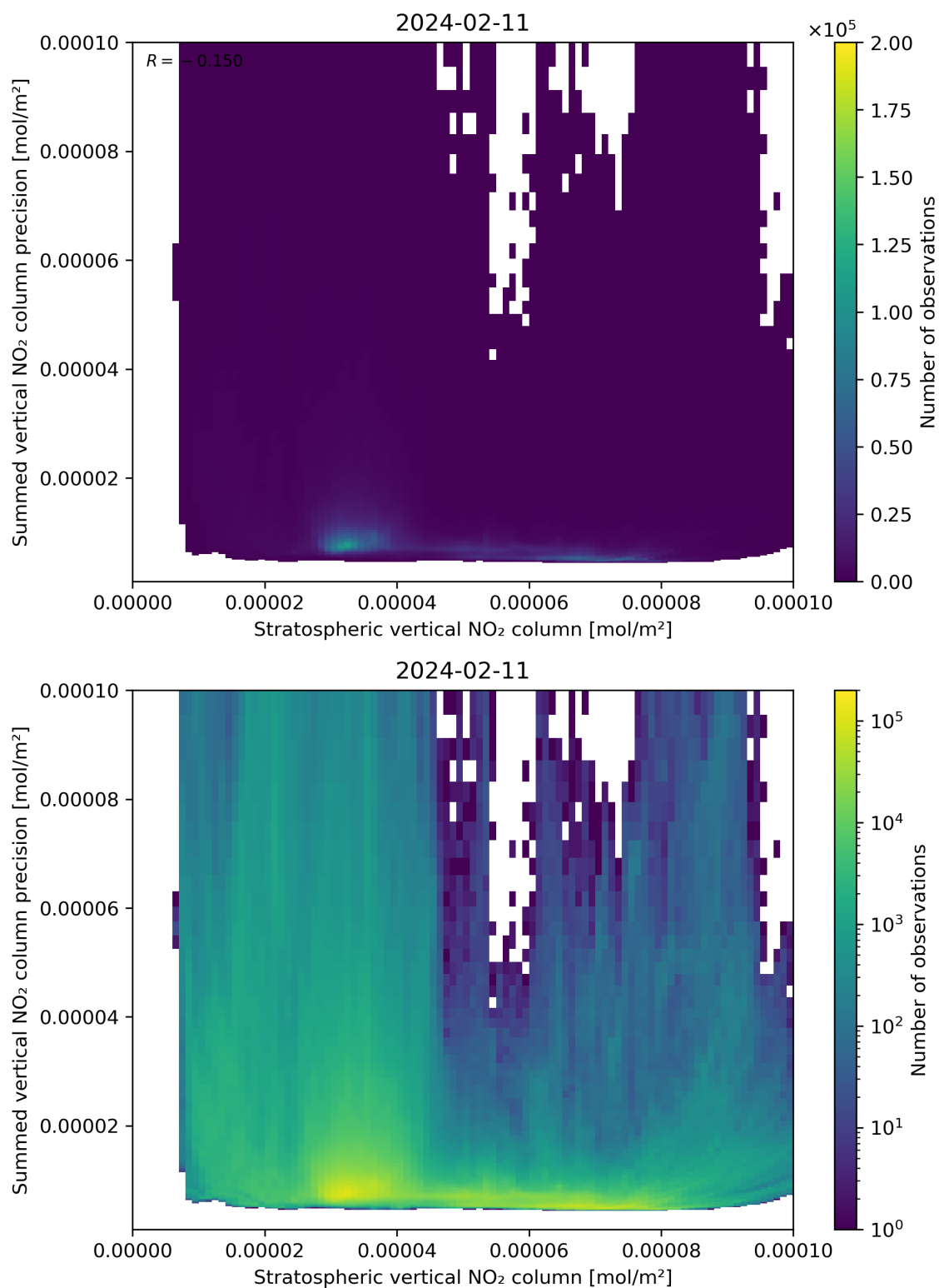
Figure 99: Scatter density plot of “Stratospheric vertical NO 2 column” against “Summed vertical NO 2 column precision” for 2024-02-11 to 2024-02-12.
