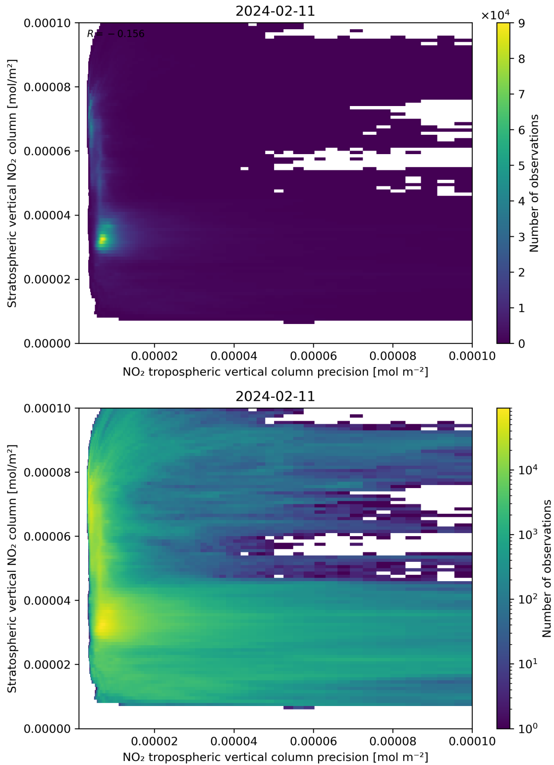
Figure 135: Scatter density plot of “NO 2 tropospheric vertical column precision” against “Stratospheric vertical NO 2 column” for 2024-02-11 to 2024-02-12.
