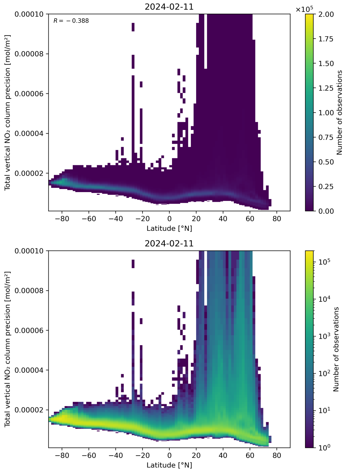
Figure 91: Scatter density plot of “Latitude” against “Total vertical NO 2 column precision” for 2024-02-11 to 2024-02-12.
