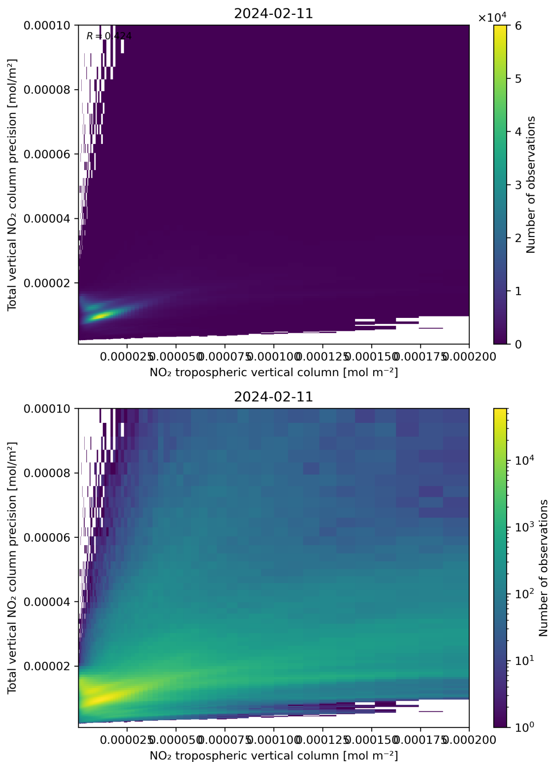
Figure 129: Scatter density plot of “NO 2 tropospheric vertical column” against “Total vertical NO 2 column precision” for 2024-02-11 to 2024-02-12.
