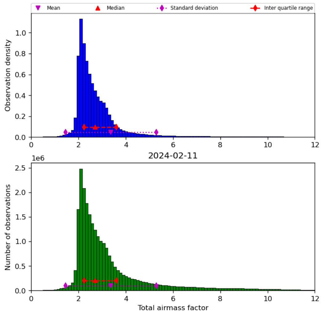
Figure 32: Histogram of “Total airmass factor” for 2024-02-11 to 2024-02-12
