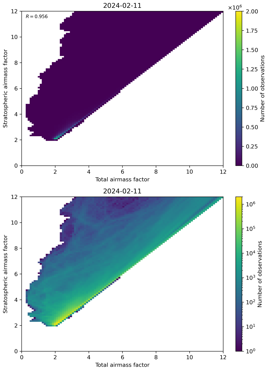
Figure 62: Scatter density plot of “Total airmass factor” against “Stratospheric airmass factor” for 2024-02-11 to 2024-02-12.
