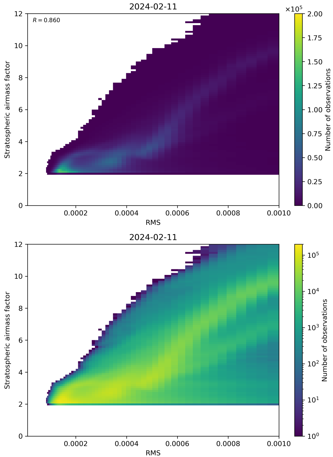
Figure 144: Scatter density plot of “RMS” against “Stratospheric airmass factor” for 2024-02-11 to 2024-02-12.
