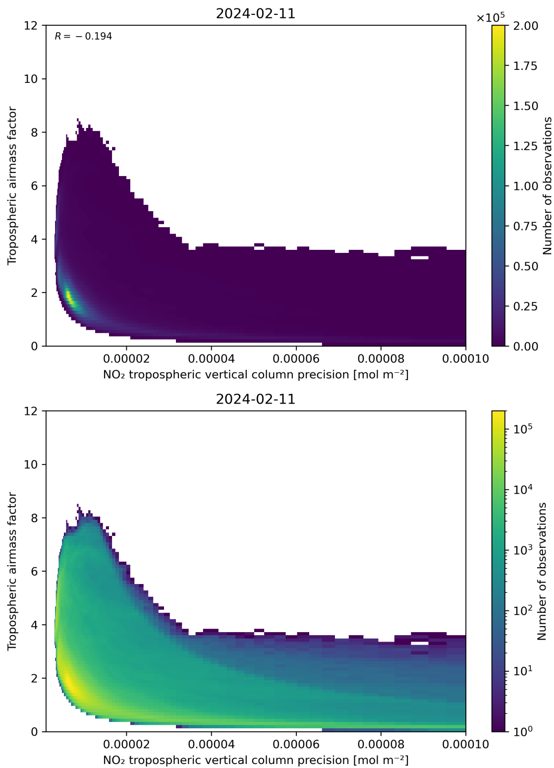
Figure 133: Scatter density plot of “NO 2 tropospheric vertical column precision” against “Tropospheric air mass factor” for 2024-02-11 to 2024-02-12.
