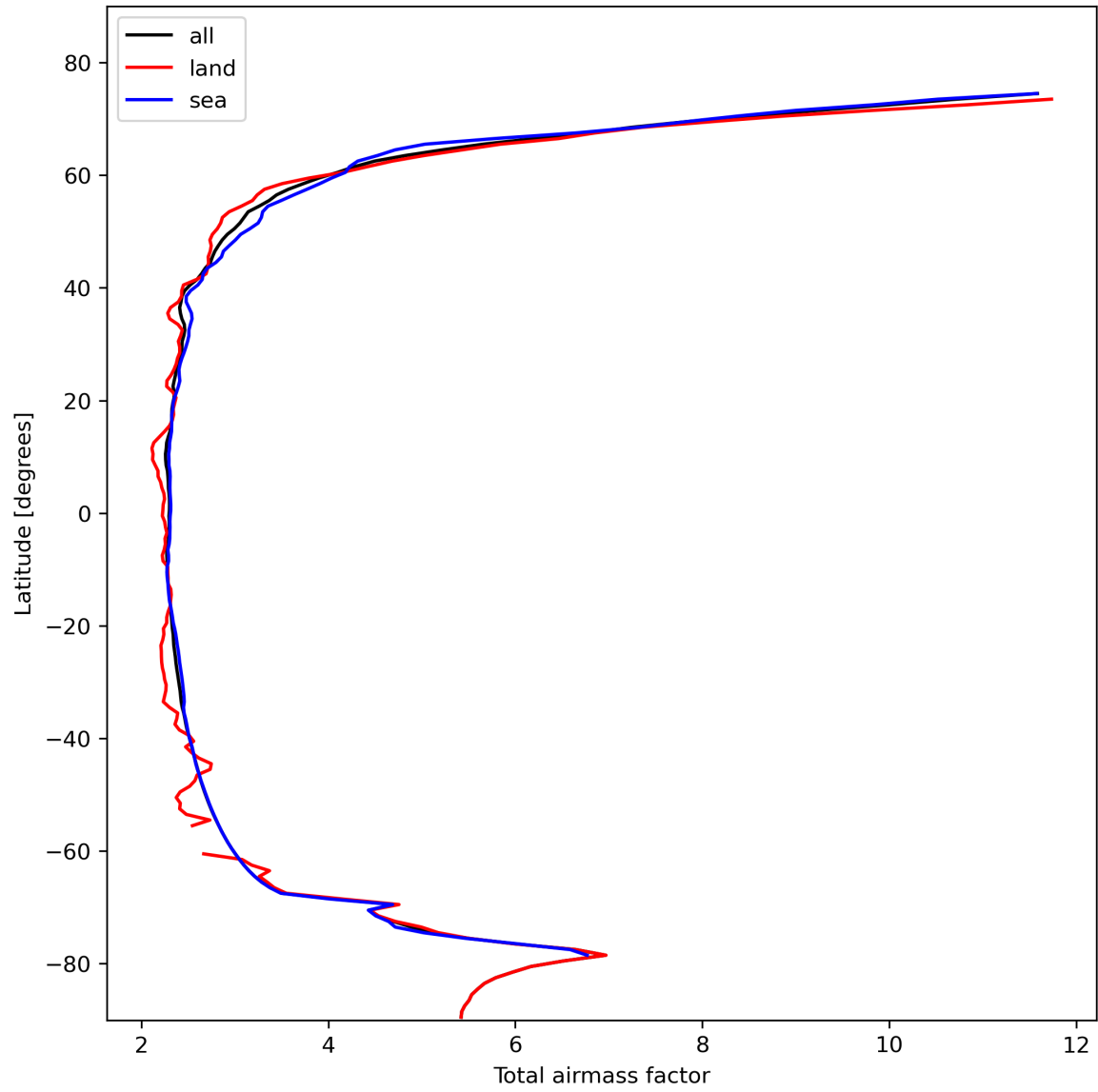
Figure 15: Zonal average of “Total airmass factor” for 2024-02-11 to 2024-02-12.
