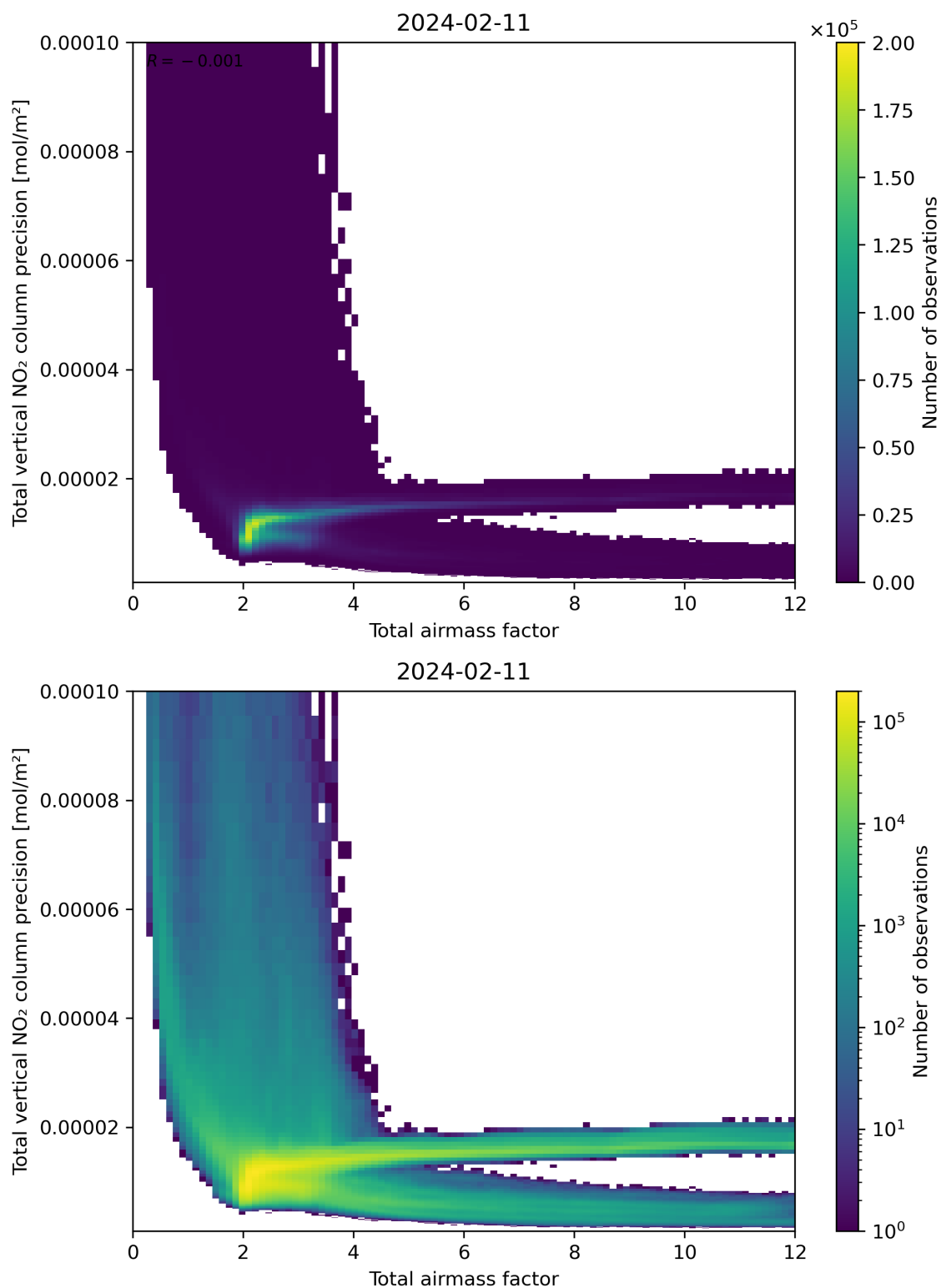
Figure 68: Scatter density plot of “Total airmass factor” against “Total vertical NO 2 column precision” for 2024-02-11 to 2024-02-12.
