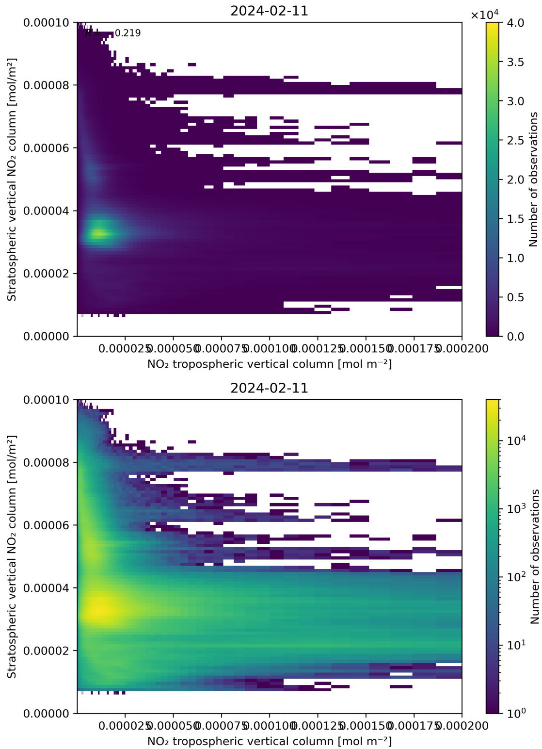
Figure 125: Scatter density plot of “NO 2 tropospheric vertical column” against “Stratospheric vertical NO 2 column” for 2024-02-11 to 2024-02-12.
