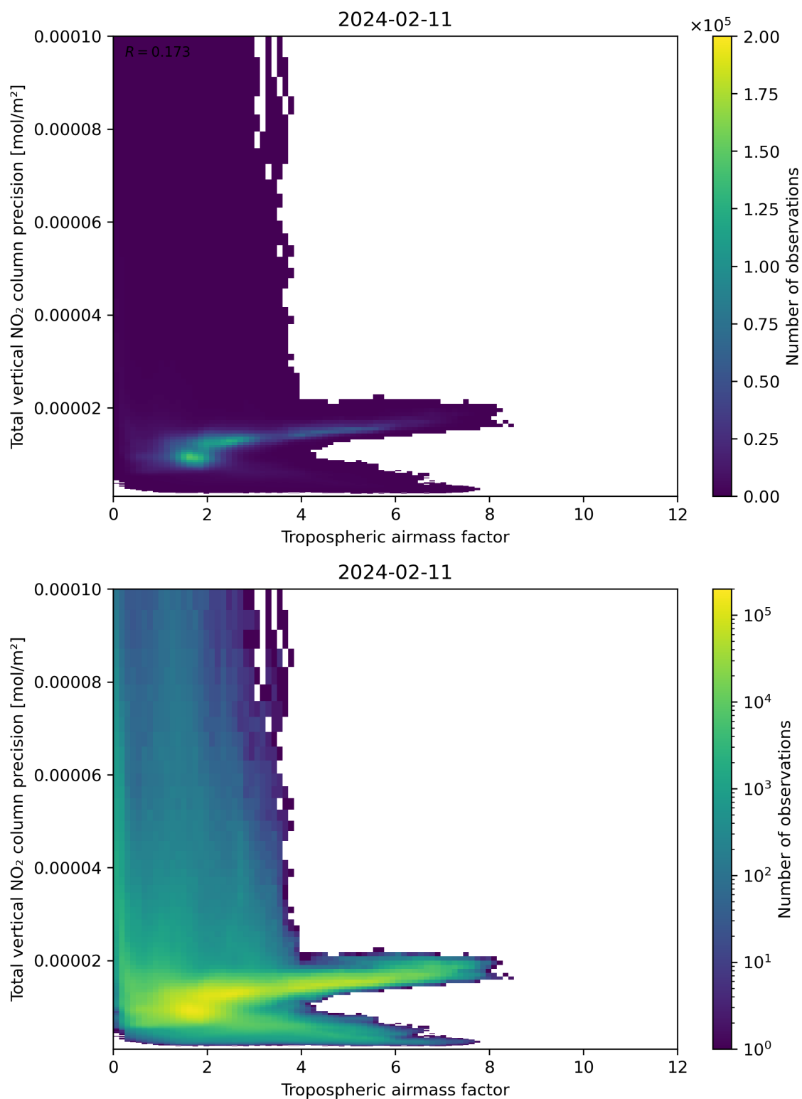
Figure 78: Scatter density plot of “Tropospheric air mass factor” against “Total vertical NO 2 column precision” for 2024-02-11 to 2024-02-12.
