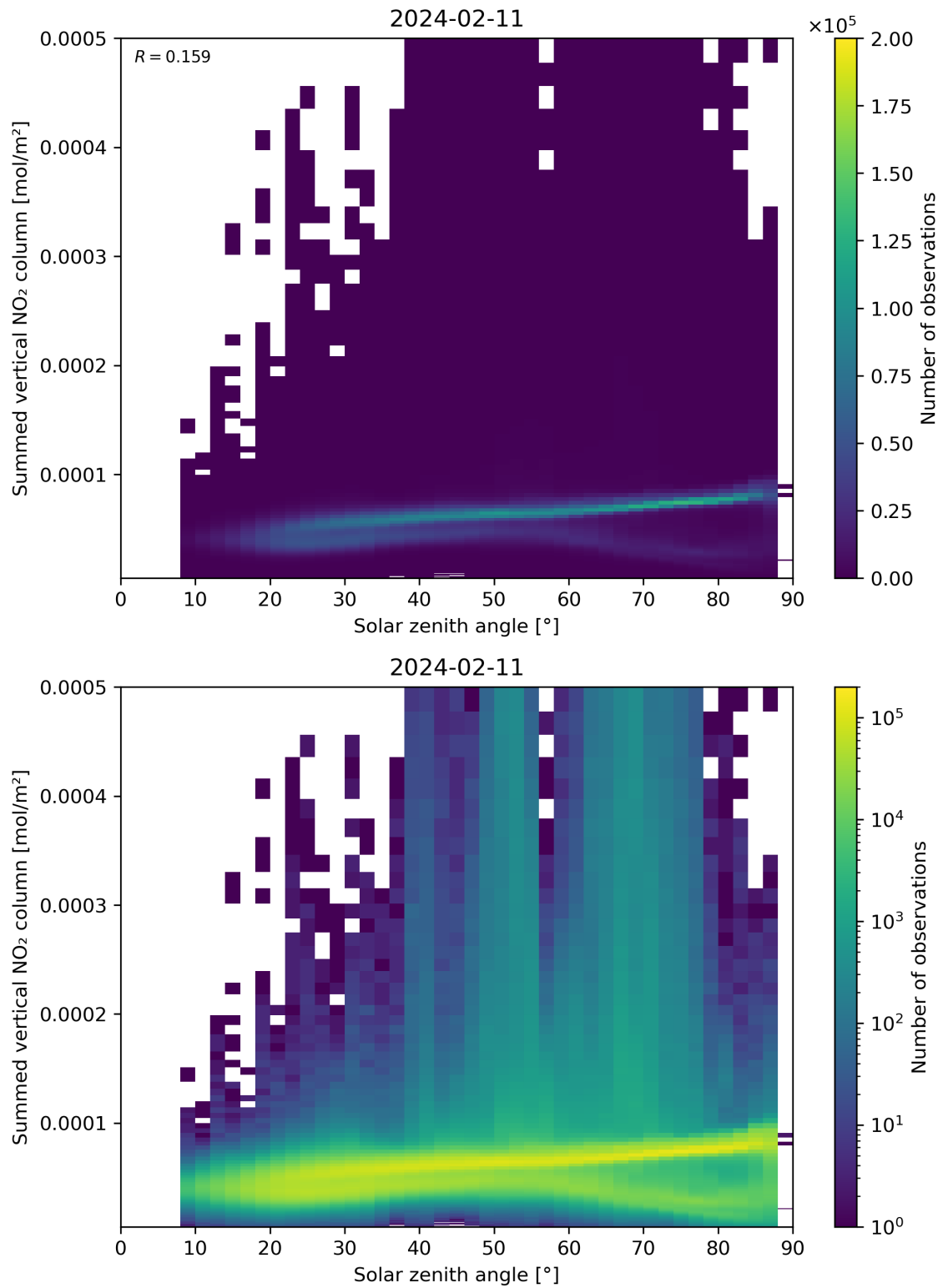
Figure 151: Scatter density plot of “Solar zenith angle” against “Summed vertical NO 2 column” for 2024-02-11 to 2024-02-12.
