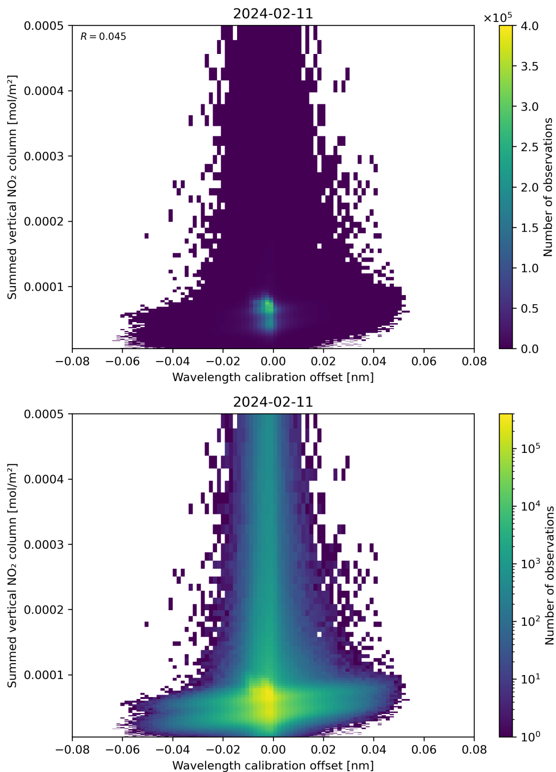
Figure 177: Scatter density plot of “Wavelength calibration offset” against “Summed vertical NO 2 column” for 2024-02-11 to 2024-02-12.
