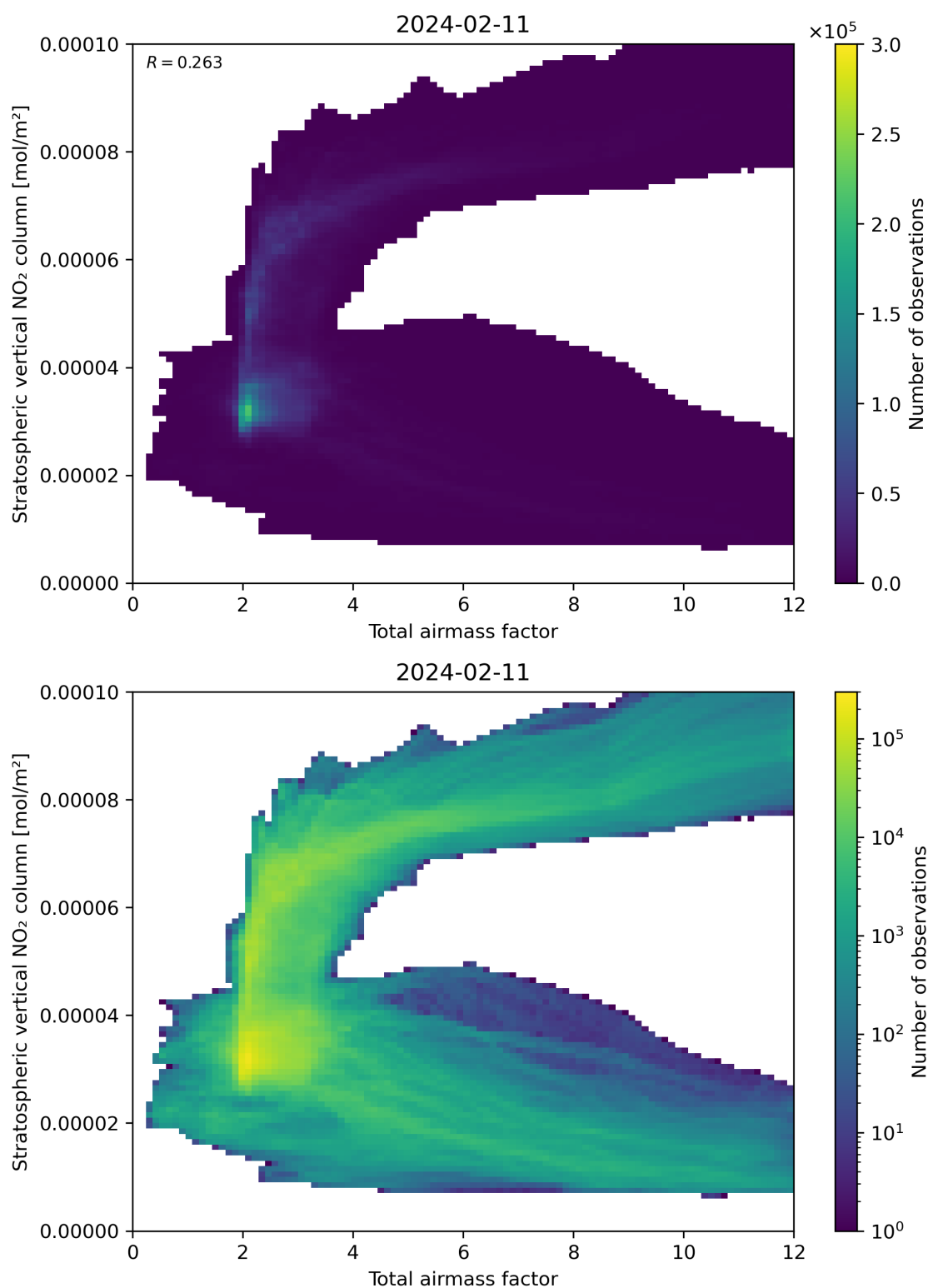
Figure 64: Scatter density plot of “Total airmass factor” against “Stratospheric vertical \text{NO}_2 column” for 2024-02-11 to 2024-02-12.
