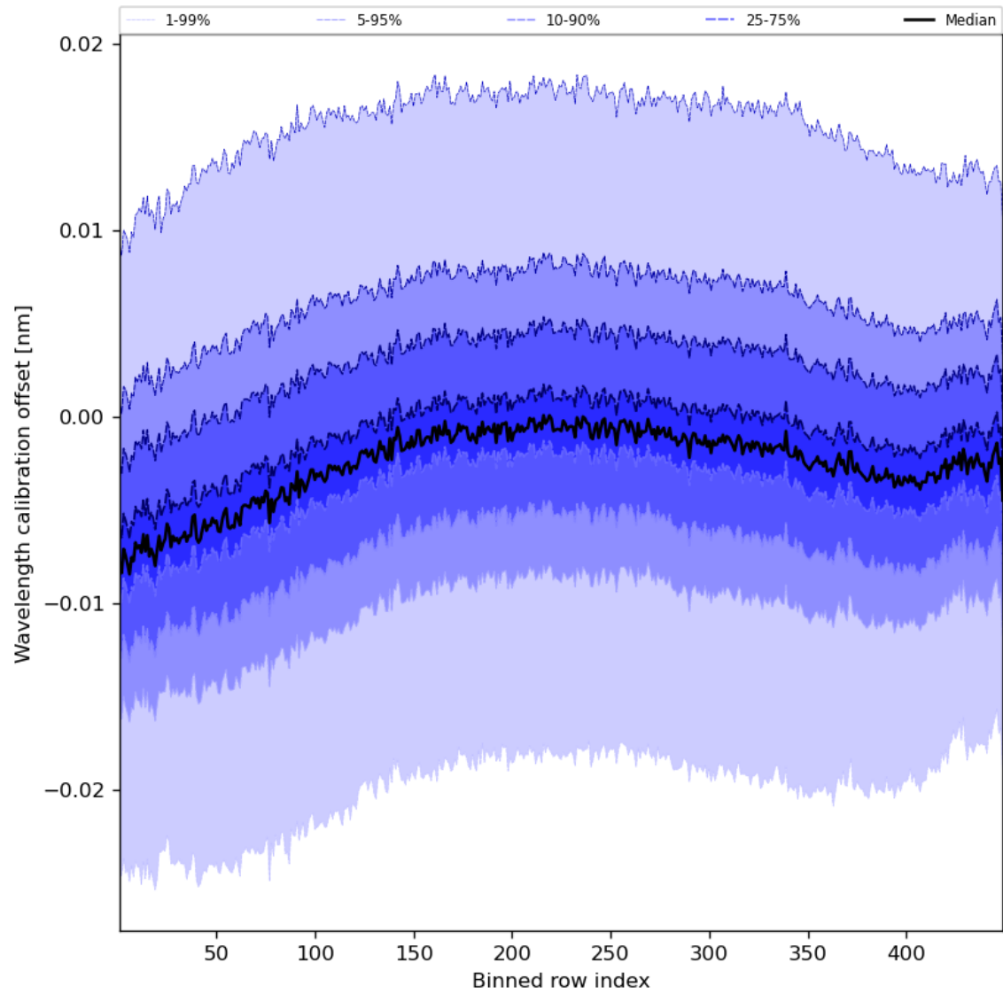
Figure 52: Along track statistics of “Wavelength calibration offset” for 2024-02-11 to 2024-02-12
