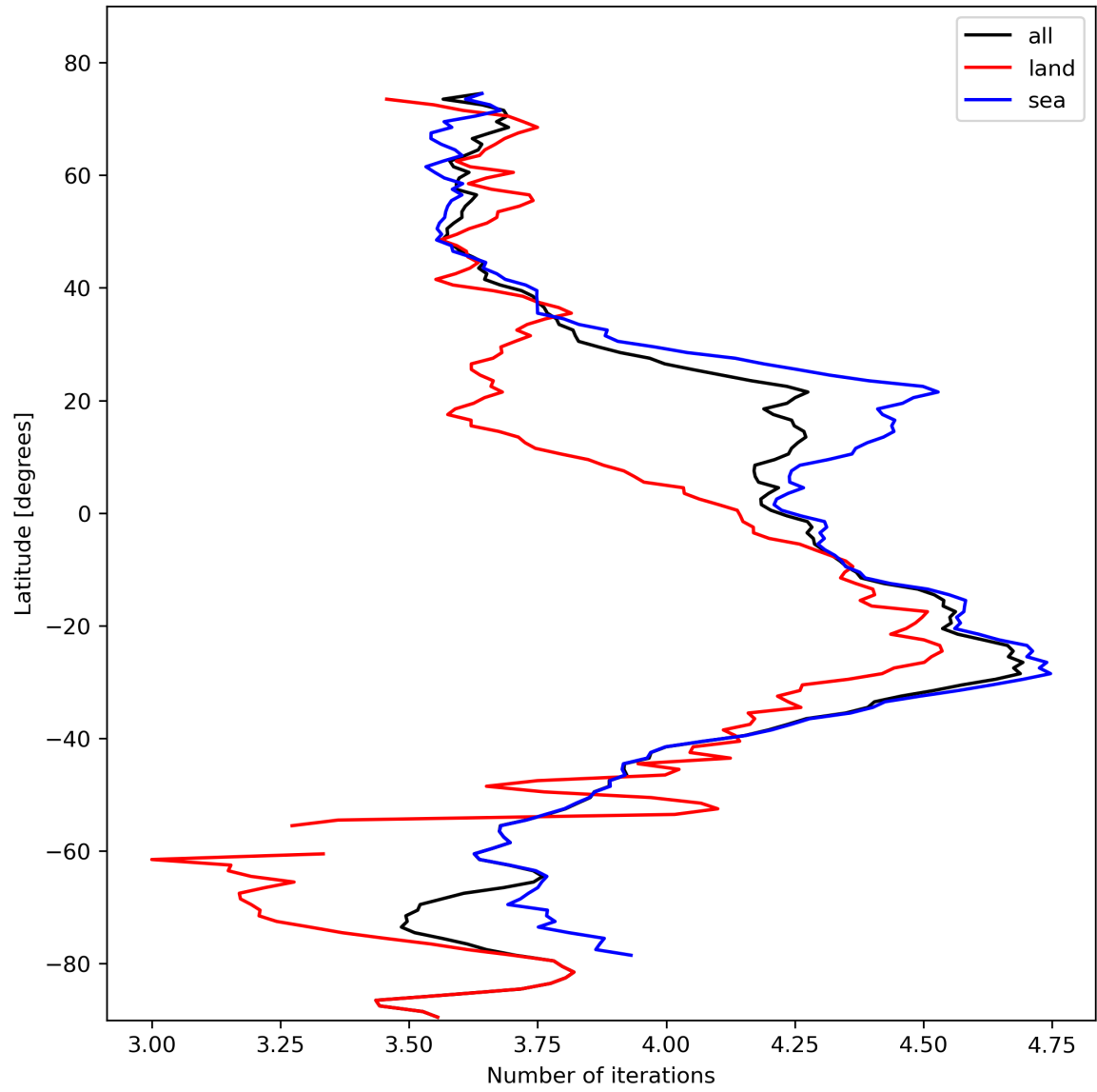
Figure 17: Zonal average of “Number of iterations” for 2024-02-11 to 2024-02-12.
