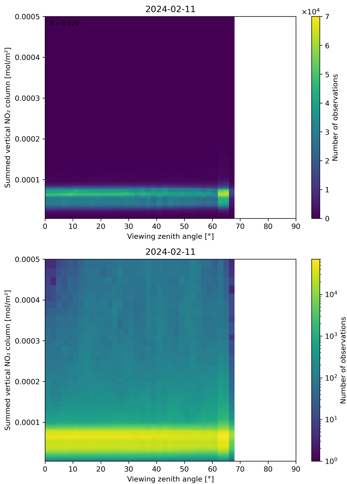
Figure 165: Scatter density plot of “Viewing zenith angle” against “Summed vertical NO 2 column” for 2024-02-11 to 2024-02-12.
