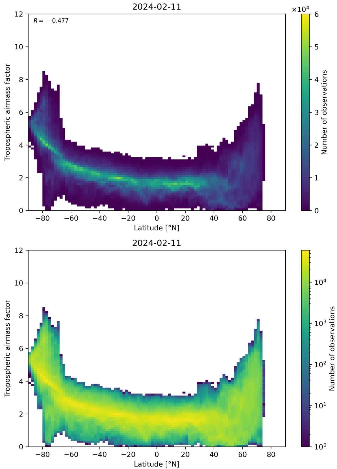
Figure 85: Scatter density plot of “Latitude” against “Tropospheric airmass factor” for 2024-02-11 to 2024-02-12.
