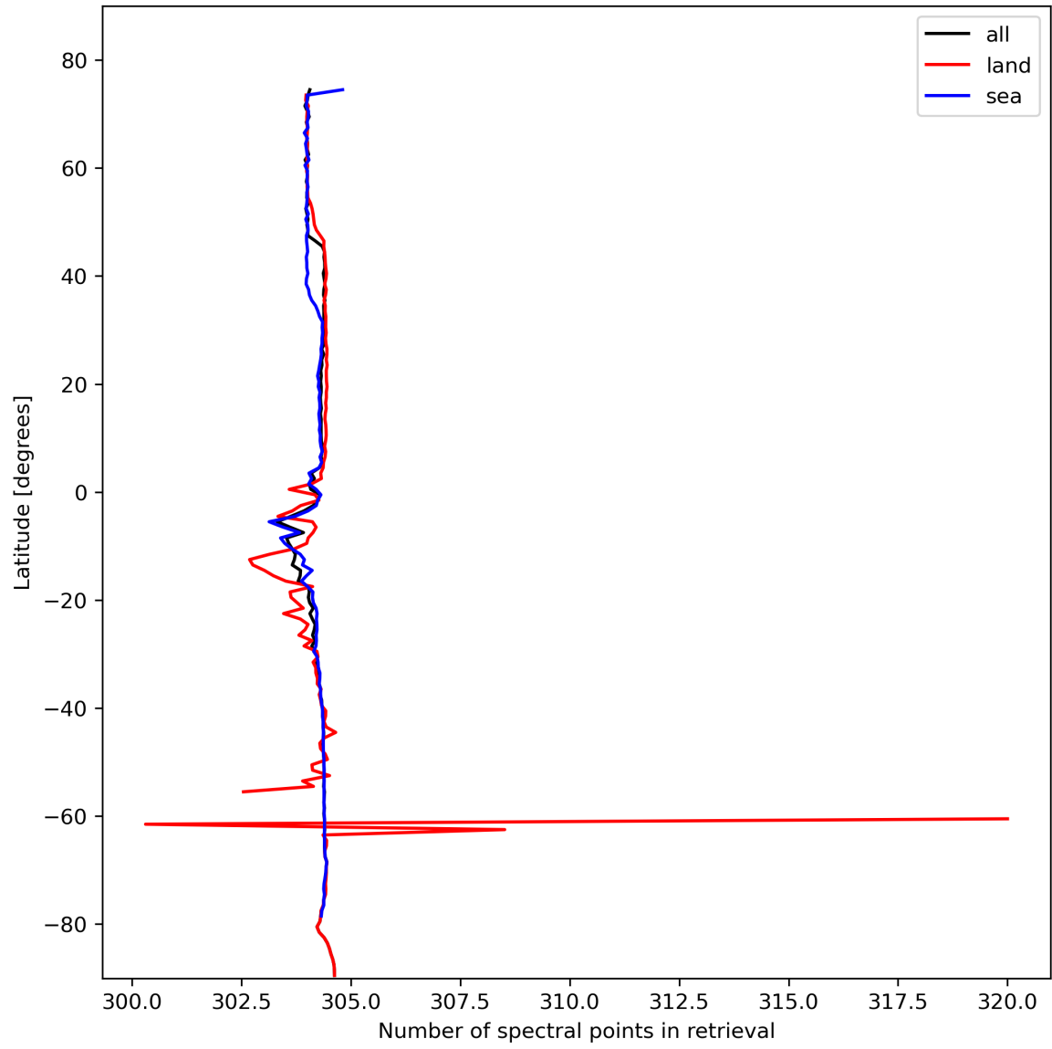
Figure 16: Zonal average of “Number of spectral points in retrieval” for 2024-02-11 to 2024-02-12.
