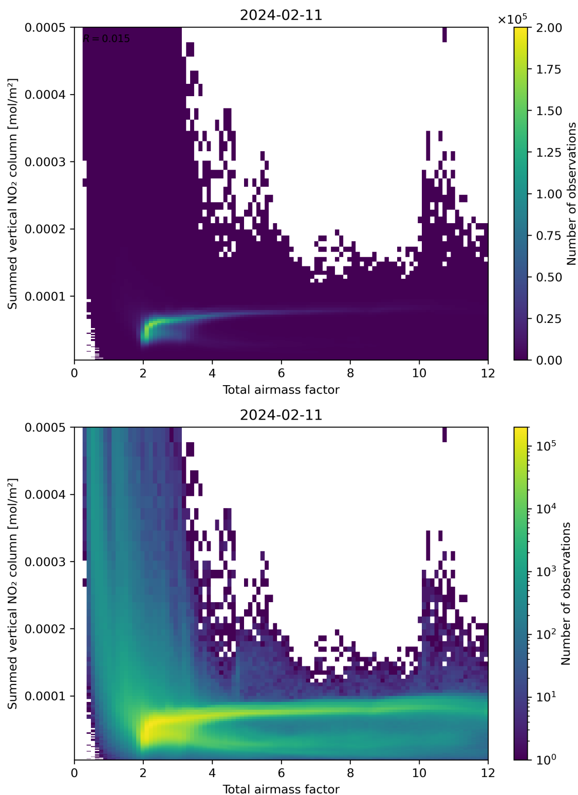
Figure 65: Scatter density plot of “Total airmass factor” against “Summed vertical NO 2 column” for 2024-02-11 to 2024-02-12.
