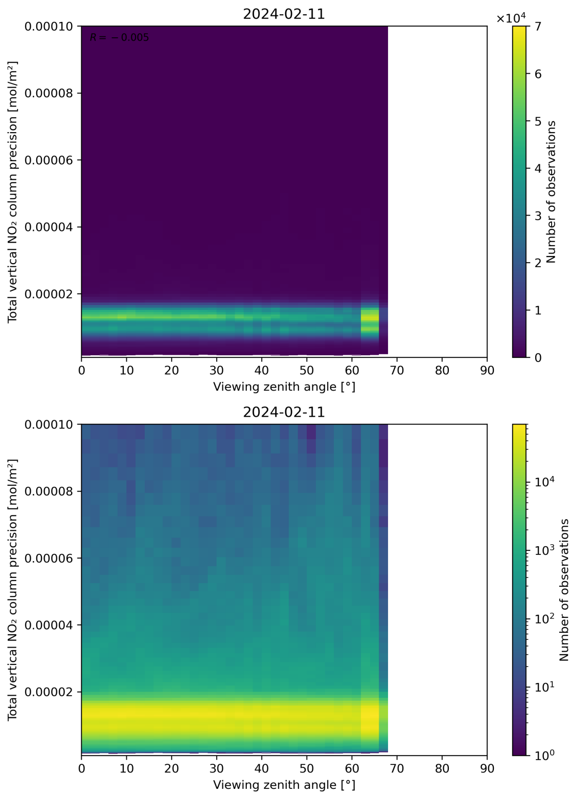
Figure 168: Scatter density plot of “Viewing zenith angle” against “Total vertical NO 2 column precision” for 2024-02-11 to 2024-02-12.
