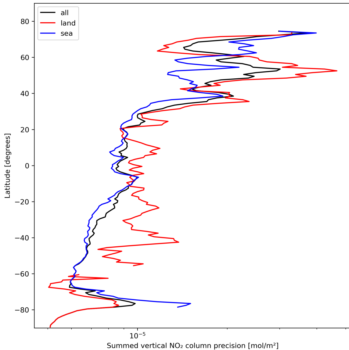
Figure 24: Zonal average of “Summed vertical NO 2 column precision” for 2024-02-11 to 2024-02-12.
