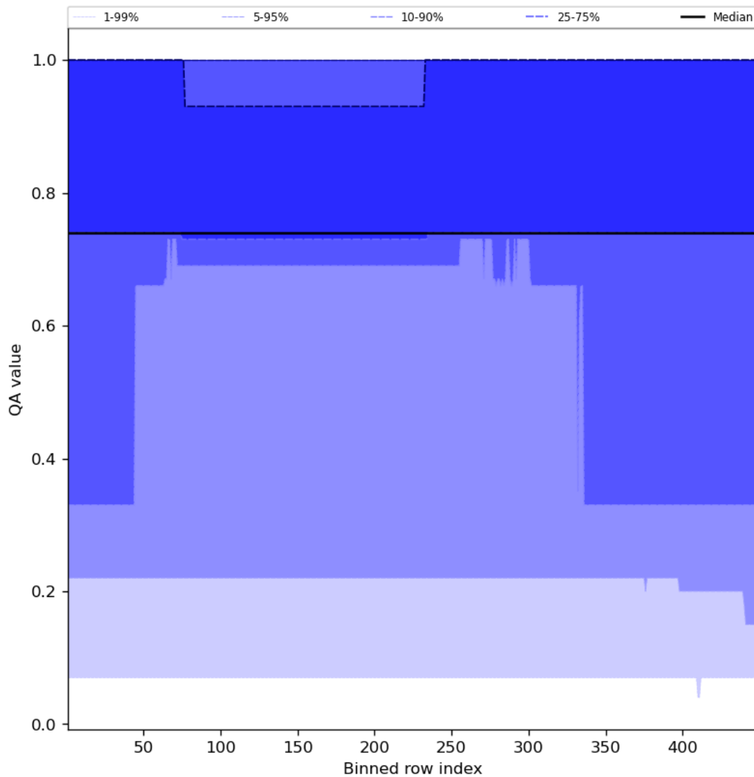
Figure 45: Along track statistics of “QA value” for 2024-02-11 to 2024-02-12
