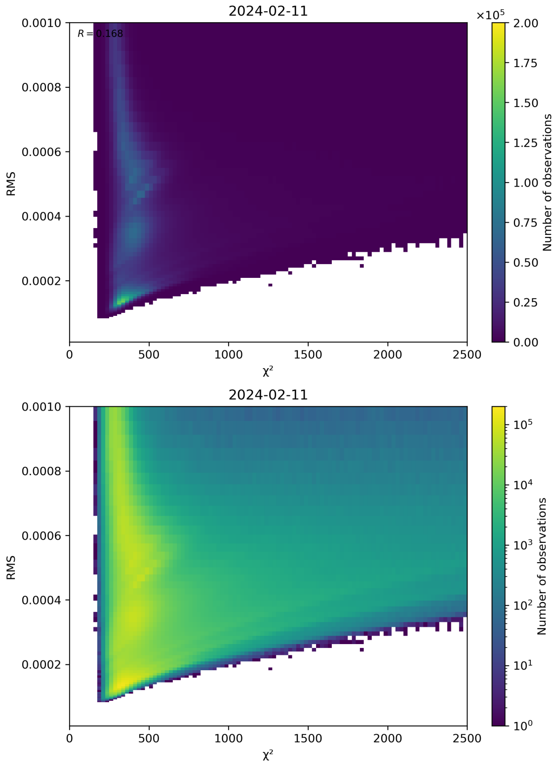
Figure 82: Scatter density plot of “ \chi^2 ” against “RMS” for 2024-02-11 to 2024-02-12.
