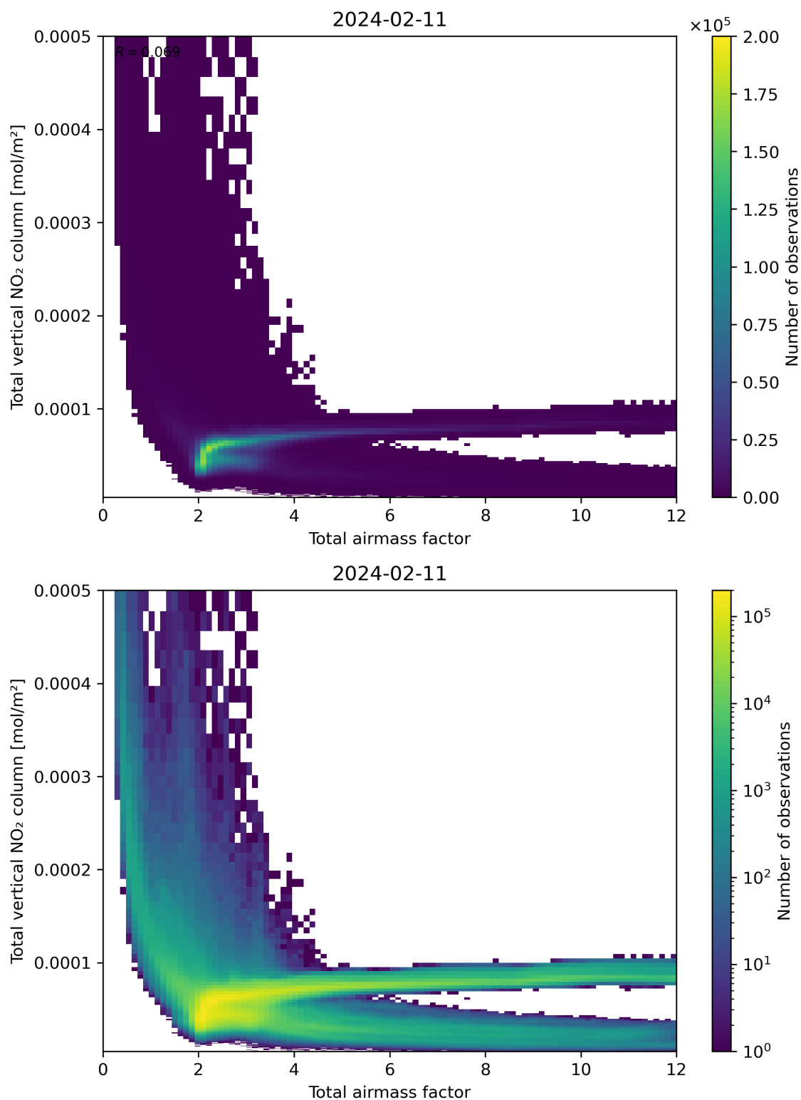
Figure 67: Scatter density plot of “Total airmass factor” against “Total vertical NO 2 column” for 2024-02-11 to 2024-02-12.
