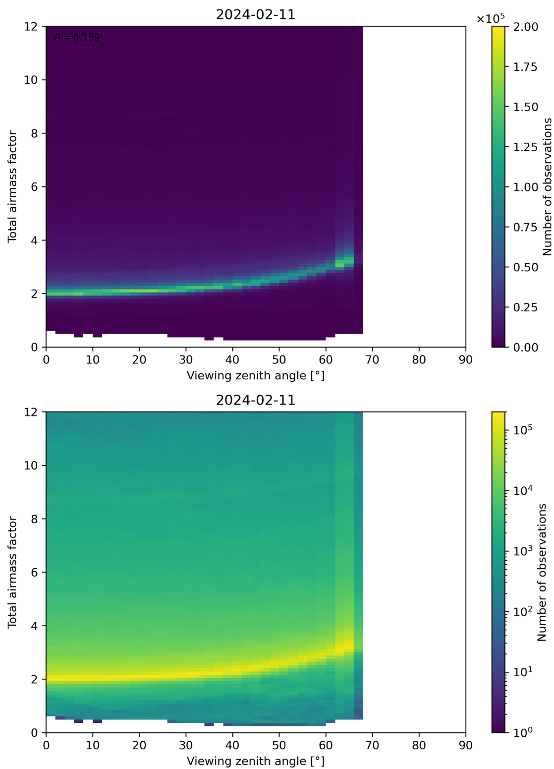
Figure 160: Scatter density plot of “Viewing zenith angle” against “Total airmass factor” for 2024-02-11 to 2024-02-12.
