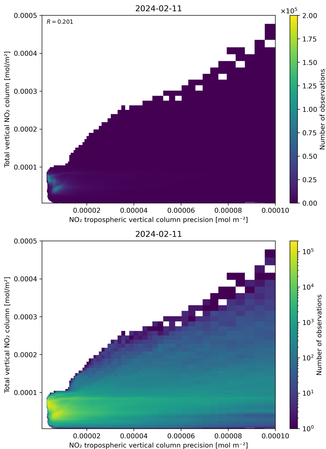
Figure 138: Scatter density plot of “NO 2 tropospheric vertical column precision” against “Total vertical NO 2 column” for 2024-02-11 to 2024-02-12.
