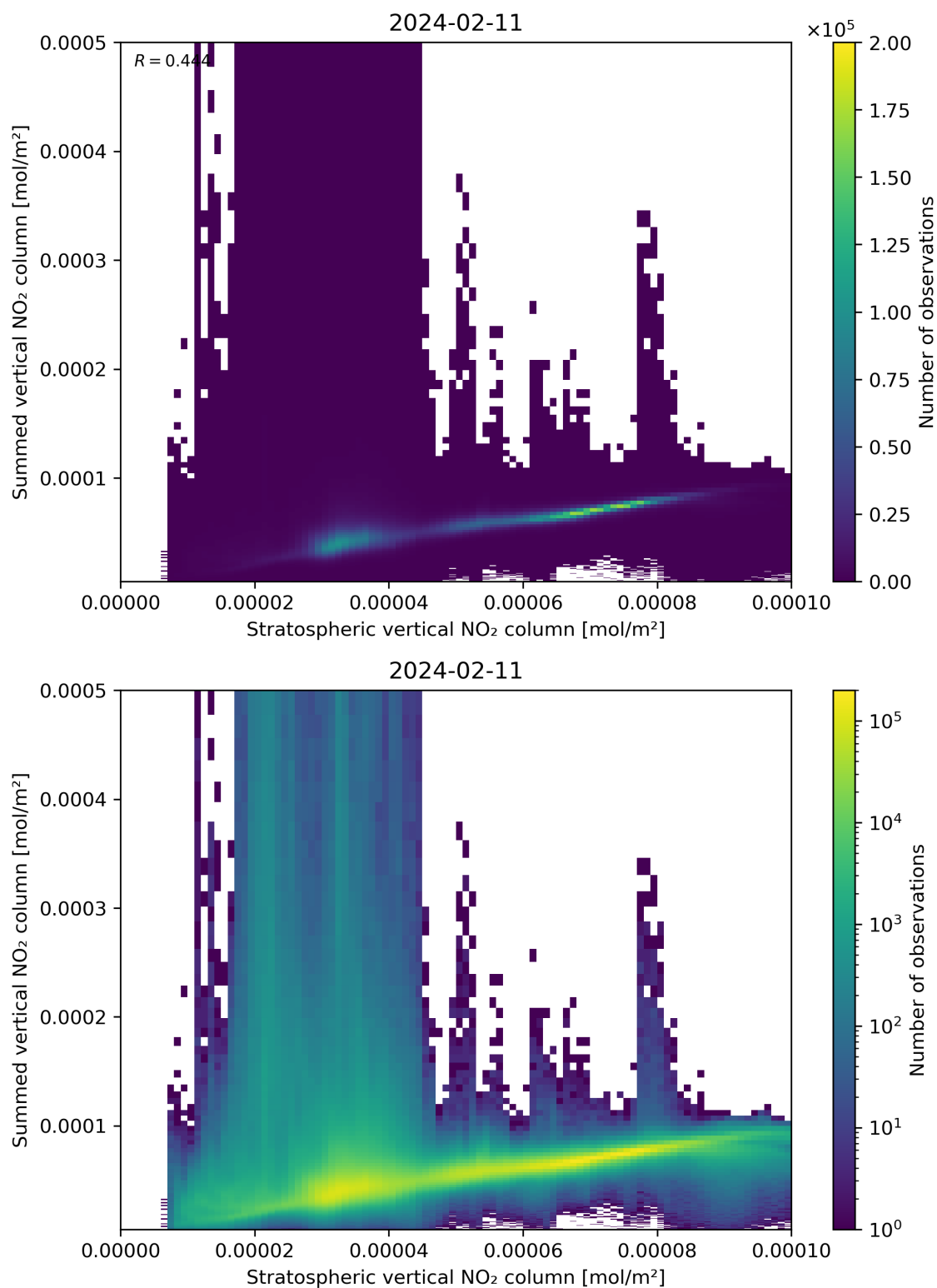
Figure 98: Scatter density plot of “Stratospheric vertical NO 2 column” against “Summed vertical NO 2 column” for 2024-02-11 to 2024-02-12.
