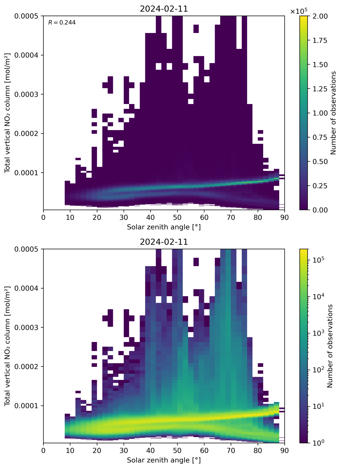
Figure 153: Scatter density plot of “Solar zenith angle” against “Total vertical NO 2 column” for 2024-02-11 to 2024-02-12.
