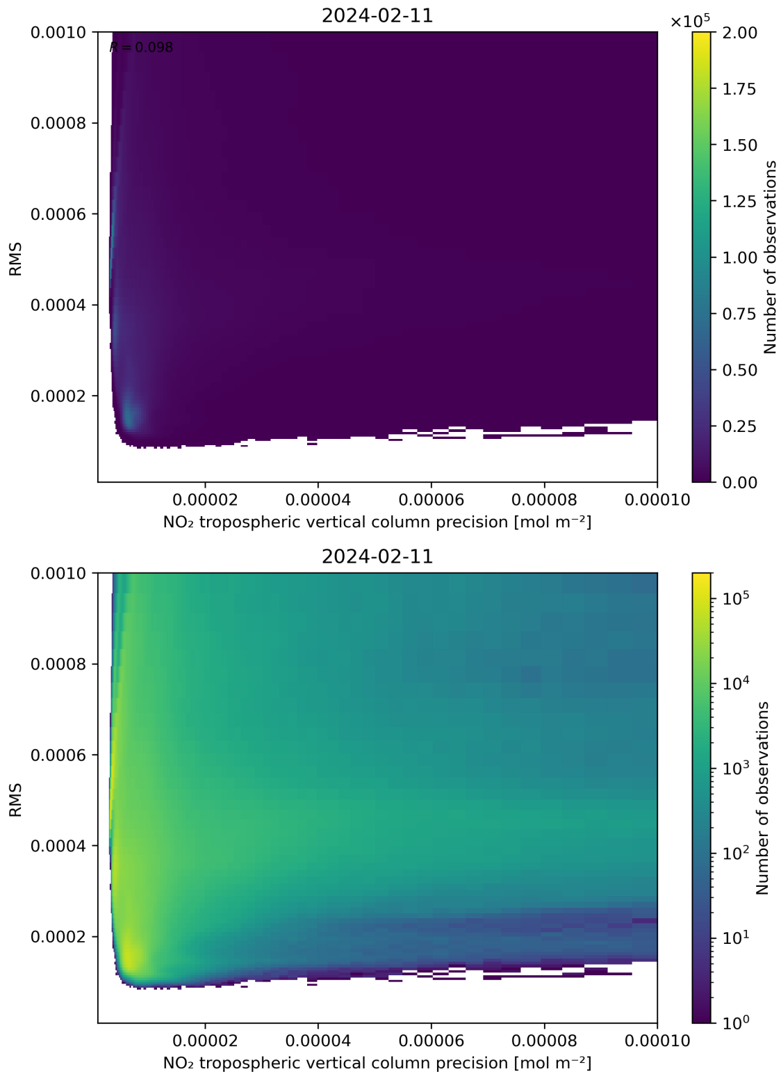
Figure 140: Scatter density plot of “NO 2 tropospheric vertical column precision” against “RMS” for 2024-02-11 to 2024-02-12.
