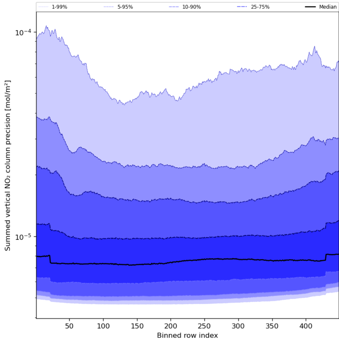
Figure 58: Along track statistics of “Summed vertical NO 2 column precision” for 2024-02-11 to 2024-02-12
