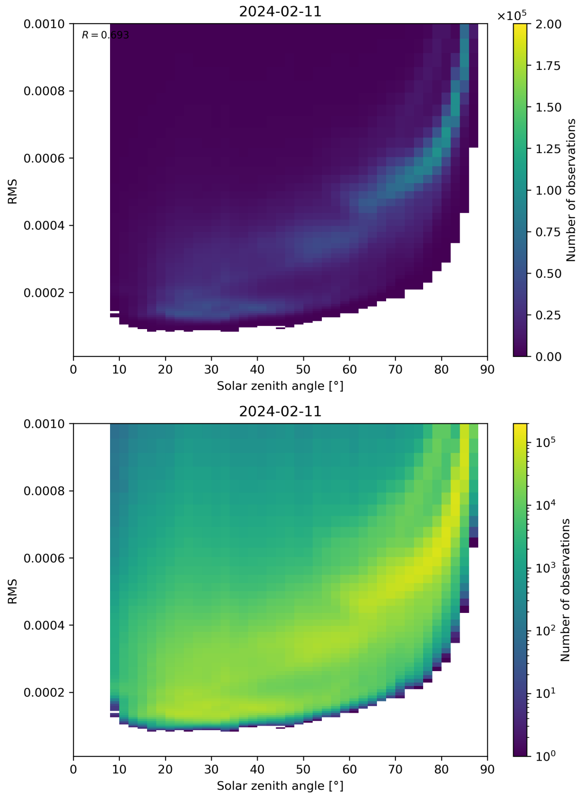
Figure 157: Scatter density plot of “Solar zenith angle” against “RMS” for 2024-02-11 to 2024-02-12.
