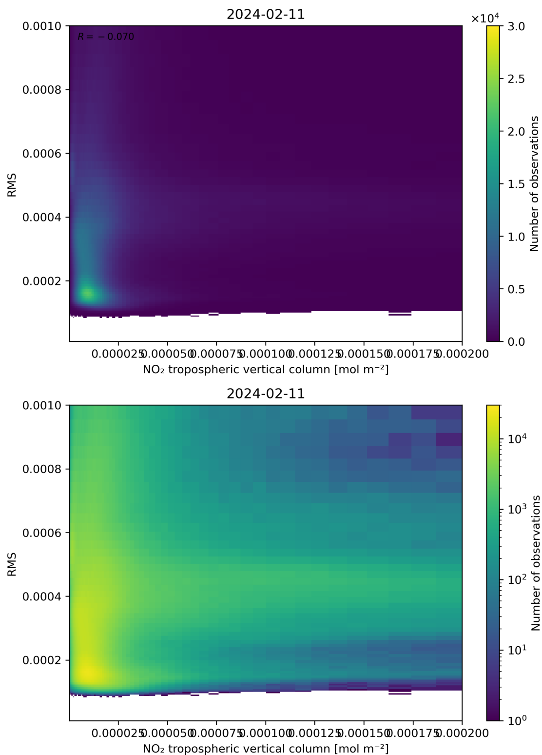
Figure 142: Scatter density plot of “NO 2 tropospheric vertical column” against “RMS” for 2024-02-11 to 2024-02-12.
