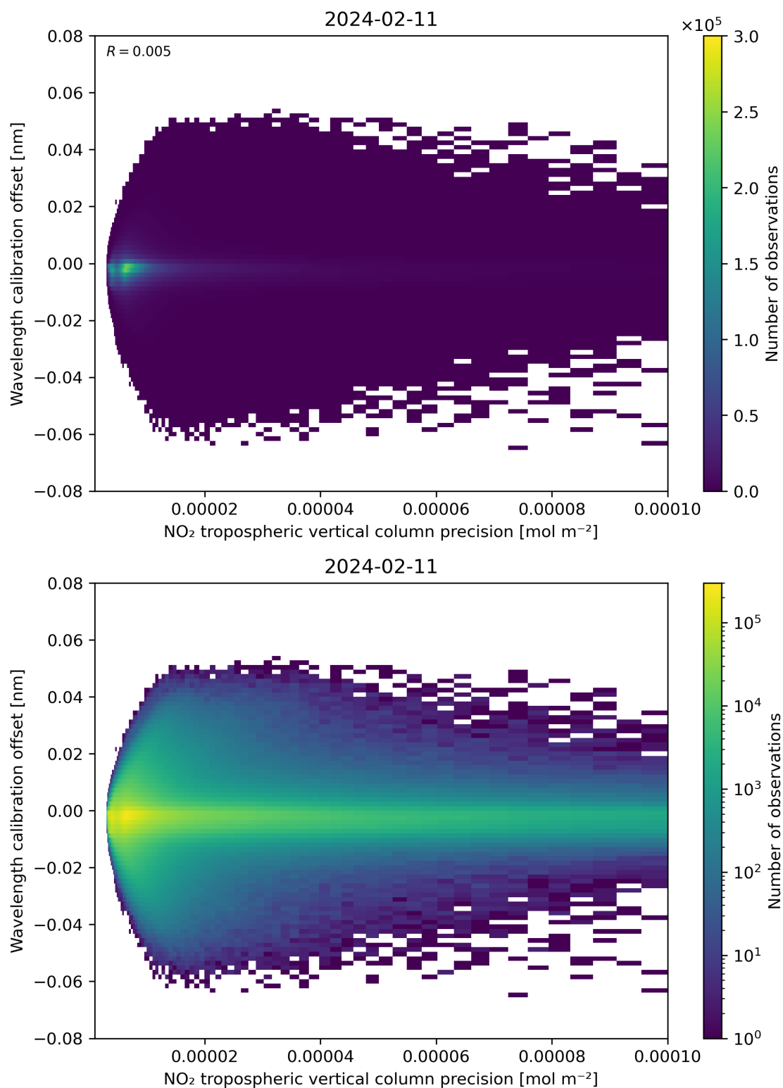
Figure 141: Scatter density plot of “NO 2 tropospheric vertical column precision” against “Wavelength calibration offset” for 2024-02-11 to 2024-02-12.
