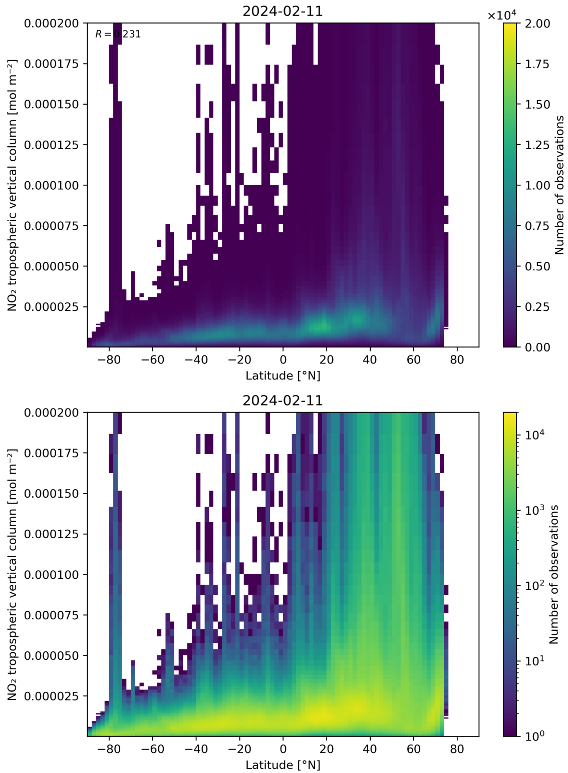
Figure 92: Scatter density plot of “Latitude” against “NO 2 tropospheric vertical column” for 2024-02-11 to 2024-02-12.
