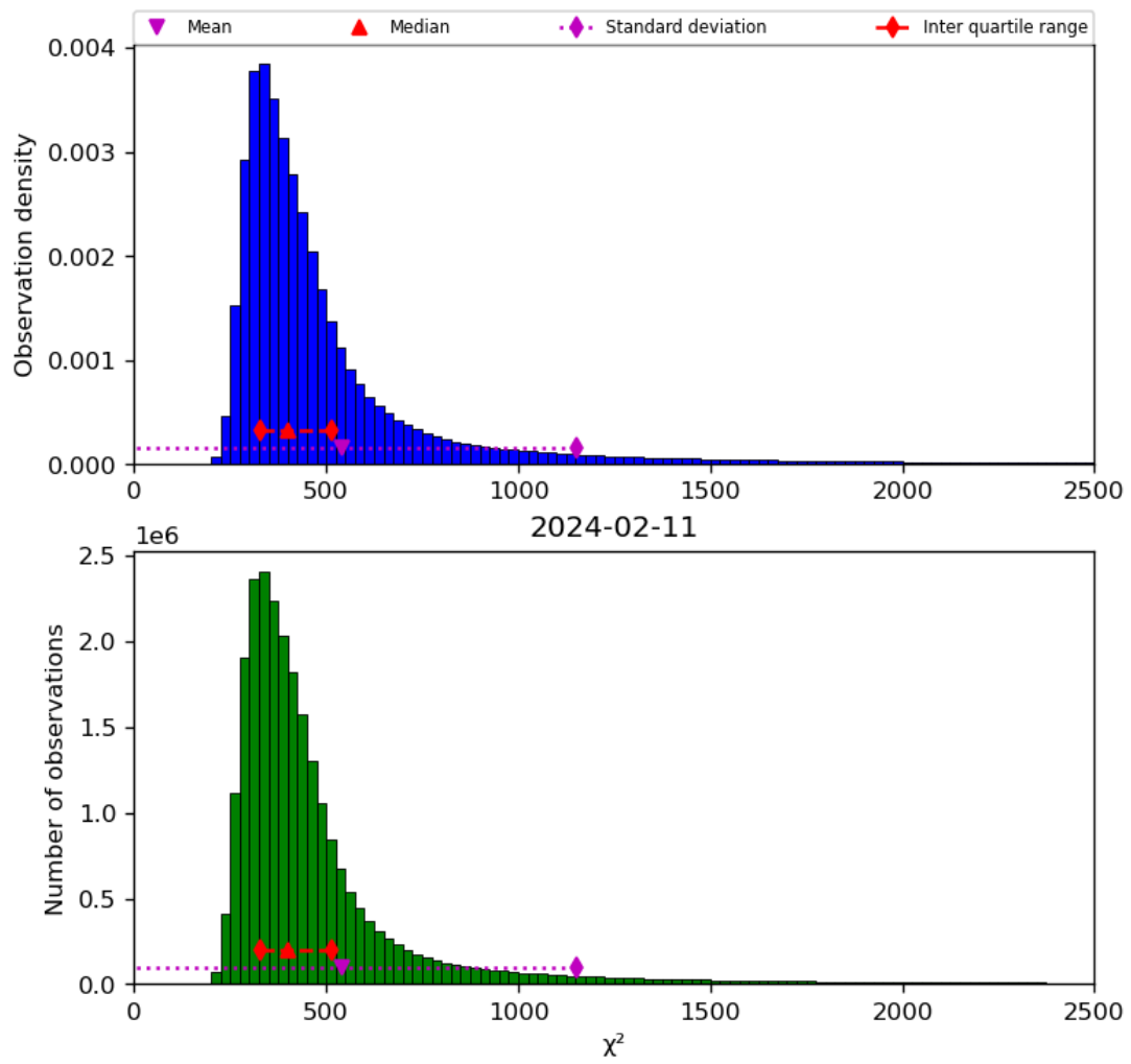
Figure 42: Histogram of “ \chi^2 ” for 2024-02-11 to 2024-02-12
