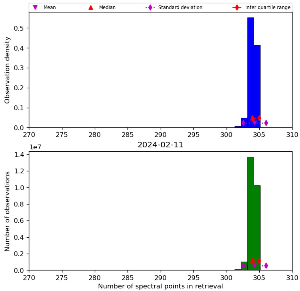
Figure 33: Histogram of “Number of spectral points in retrieval” for 2024-02-11 to 2024-02-12
