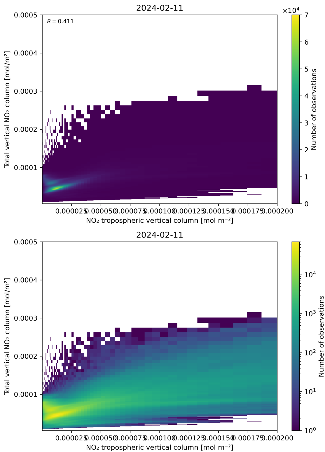
Figure 128: Scatter density plot of “NO 2 tropospheric vertical column” against “Total vertical NO 2 column” for 2024-02-11 to 2024-02-12.
