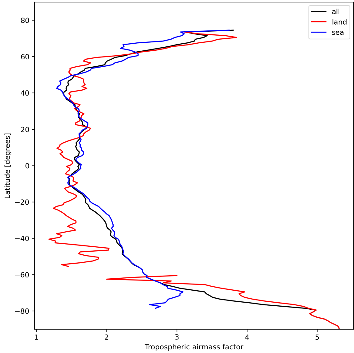
Figure 14: Zonal average of “Tropospheric airmass factor” for 2024-02-11 to 2024-02-12.
