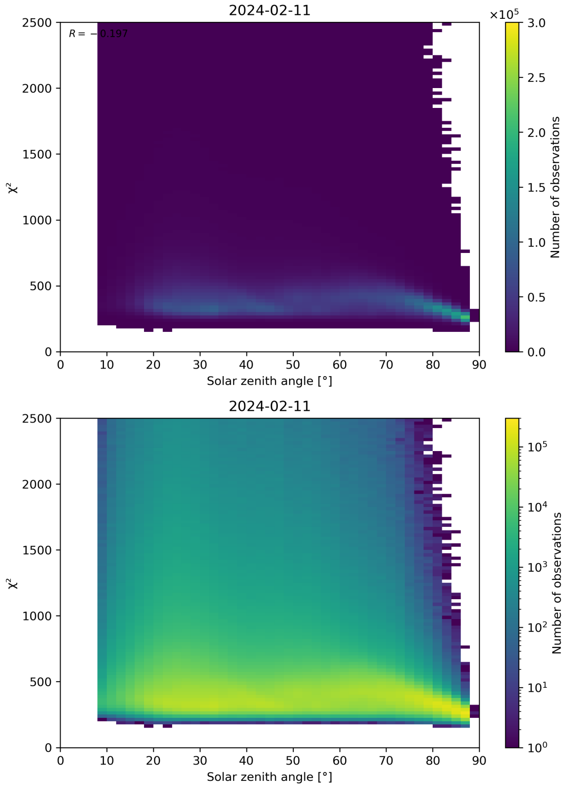
Figure 148: Scatter density plot of “Solar zenith angle” against “ \chi^2 ” for 2024-02-11 to 2024-02-12.
