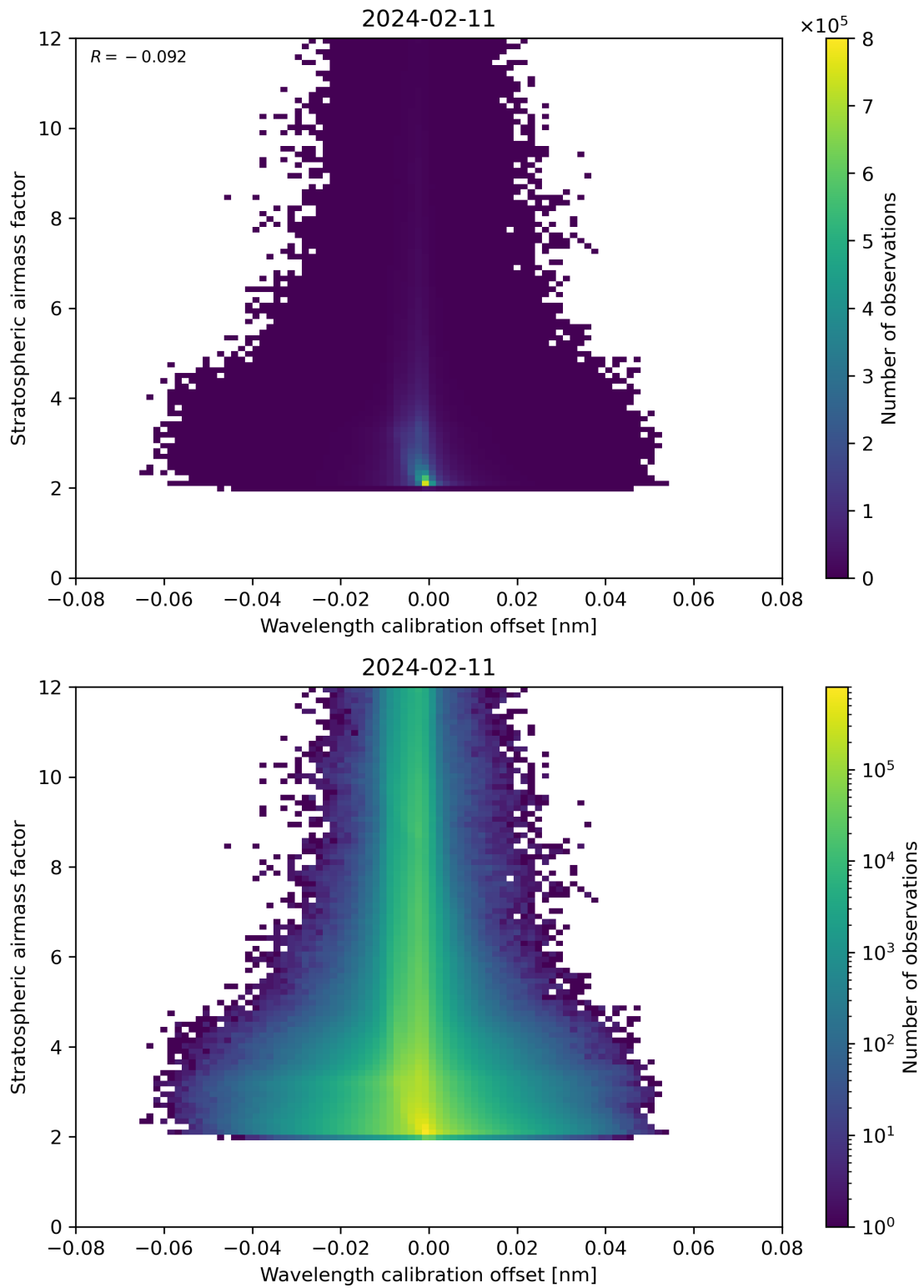
Figure 174: Scatter density plot of “Wavelength calibration offset” against “Stratospheric airmass factor” for 2024-02-11 to 2024-02-12.
