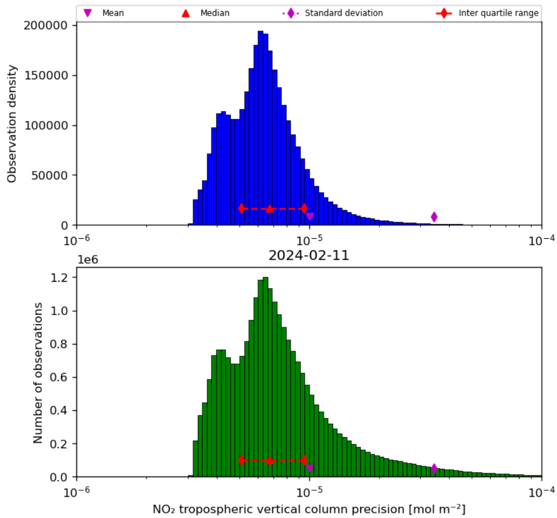
Figure 30: Histogram of “NO 2 tropospheric vertical column precision” for 2024-02-11 to 2024-02-12
