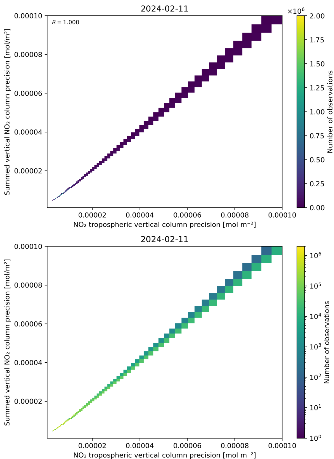
Figure 137: Scatter density plot of “NO 2 tropospheric vertical column precision” against “Summed vertical NO 2 column precision” for 2024-02-11 to 2024-02-12.
