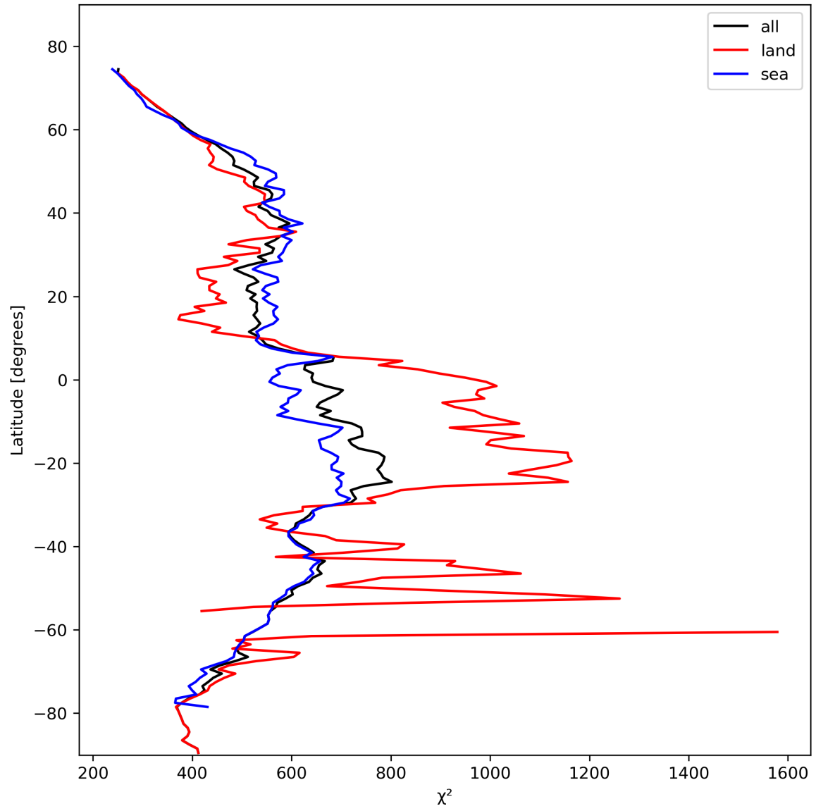
Figure 25: Zonal average of “ \chi^2 ” for 2024-02-11 to 2024-02-12.
