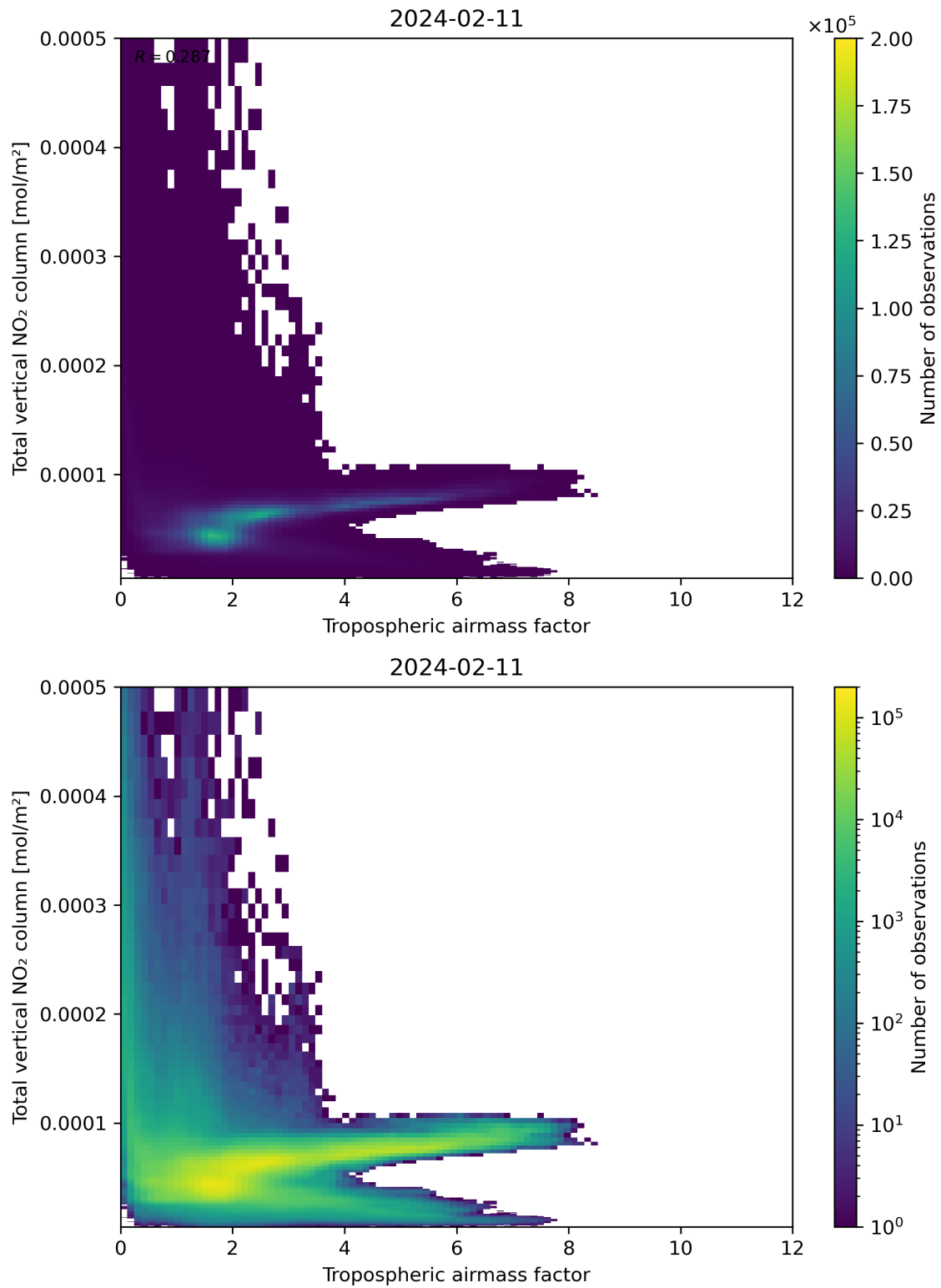
Figure 77: Scatter density plot of “Tropospheric airmass factor” against “Total vertical NO 2 column” for 2024-02-11 to 2024-02-12.
