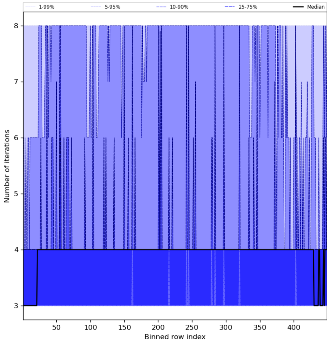
Figure 51: Along track statistics of “Number of iterations” for 2024-02-11 to 2024-02-12
