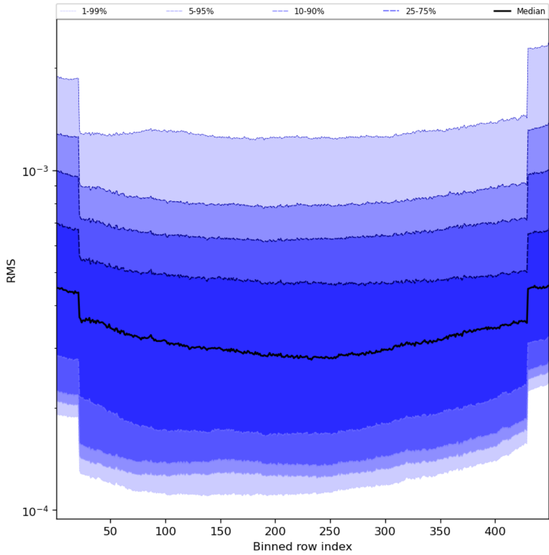
Figure 60: Along track statistics of “RMS” for 2024-02-11 to 2024-02-12
