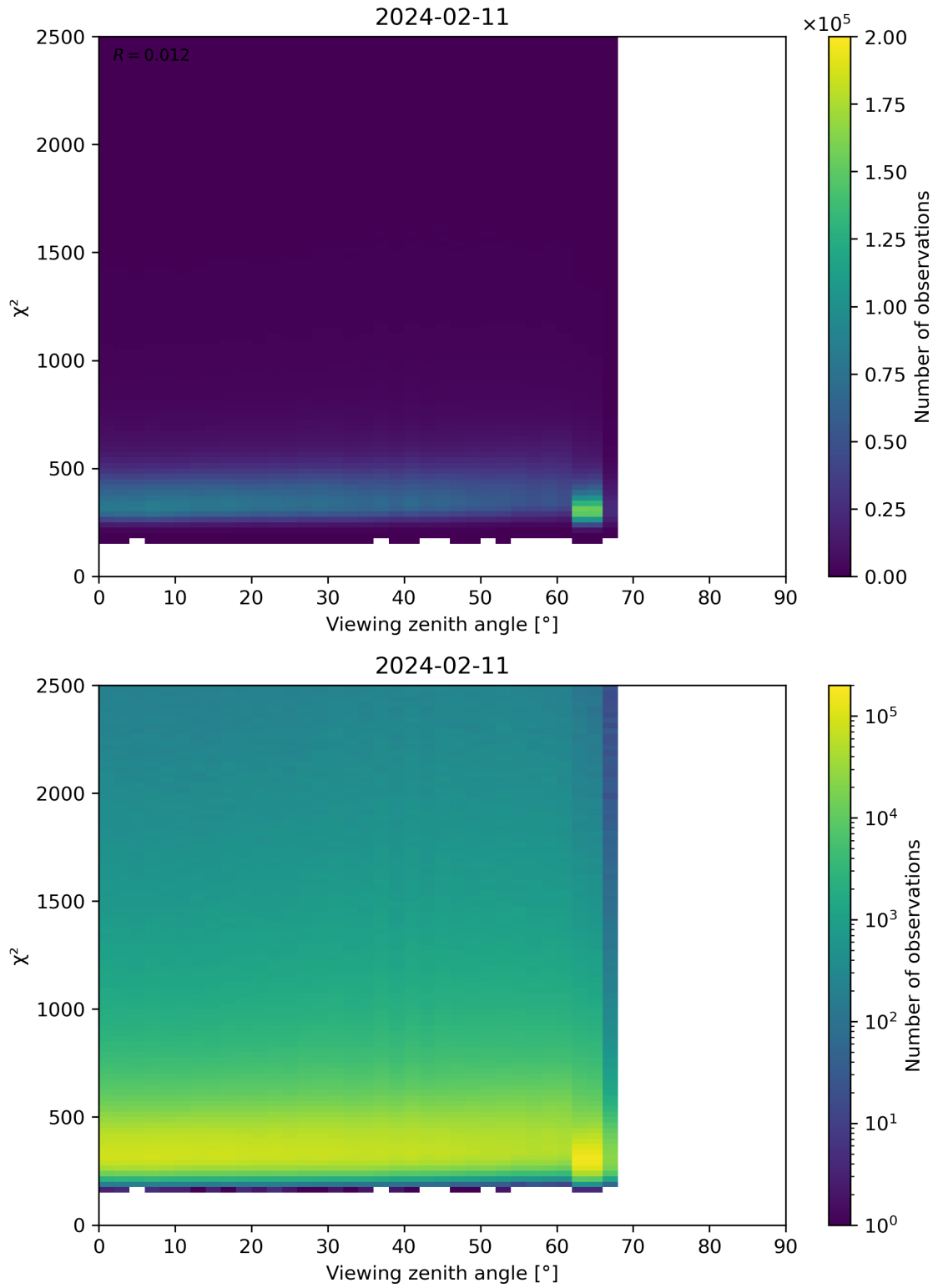
Figure 162: Scatter density plot of “Viewing zenith angle” against “ \chi^2 ” for 2024-02-11 to 2024-02-12.
