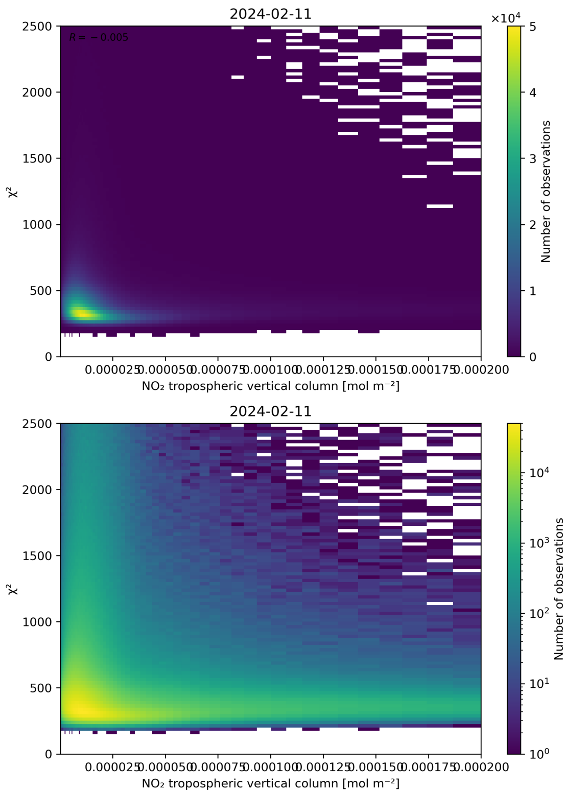
Figure 124: Scatter density plot of “NO 2 tropospheric vertical column” against “ \chi^2 ” for 2024-02-11 to 2024-02-12.
