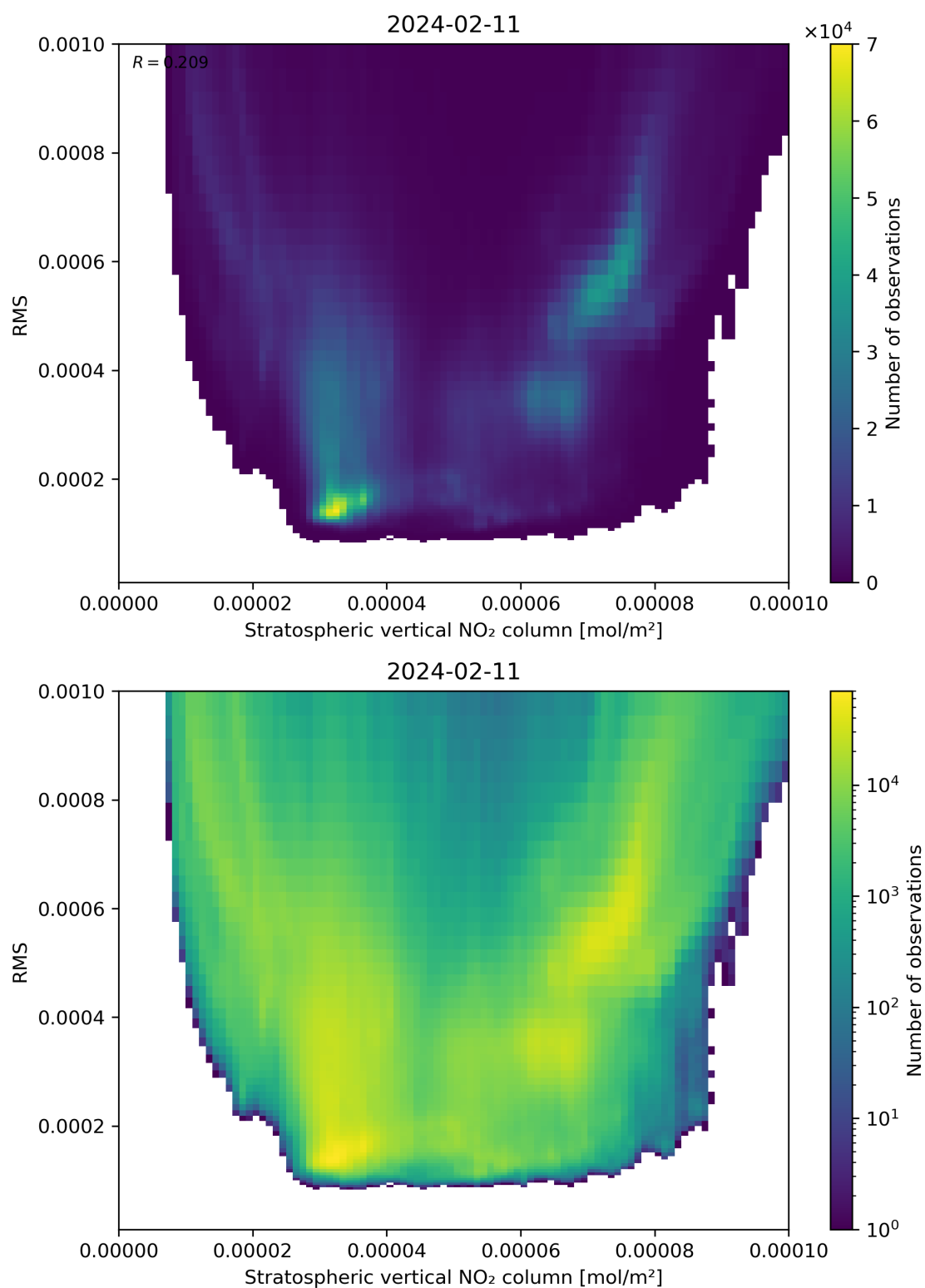
Figure 102: Scatter density plot of “Stratospheric vertical NO 2 column” against “RMS” for 2024-02-11 to 2024-02-12.
