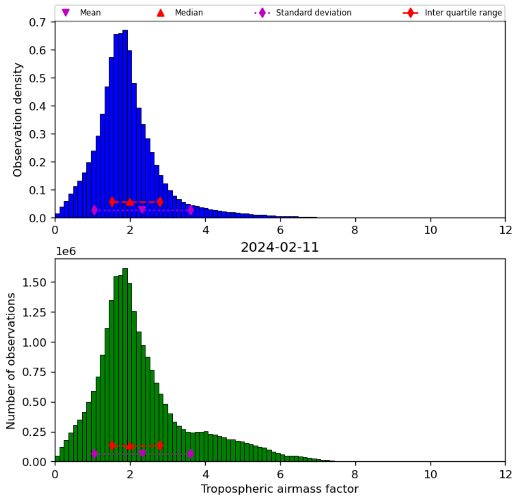
Figure 31: Histogram of “Tropospheric airmass factor” for 2024-02-11 to 2024-02-12
