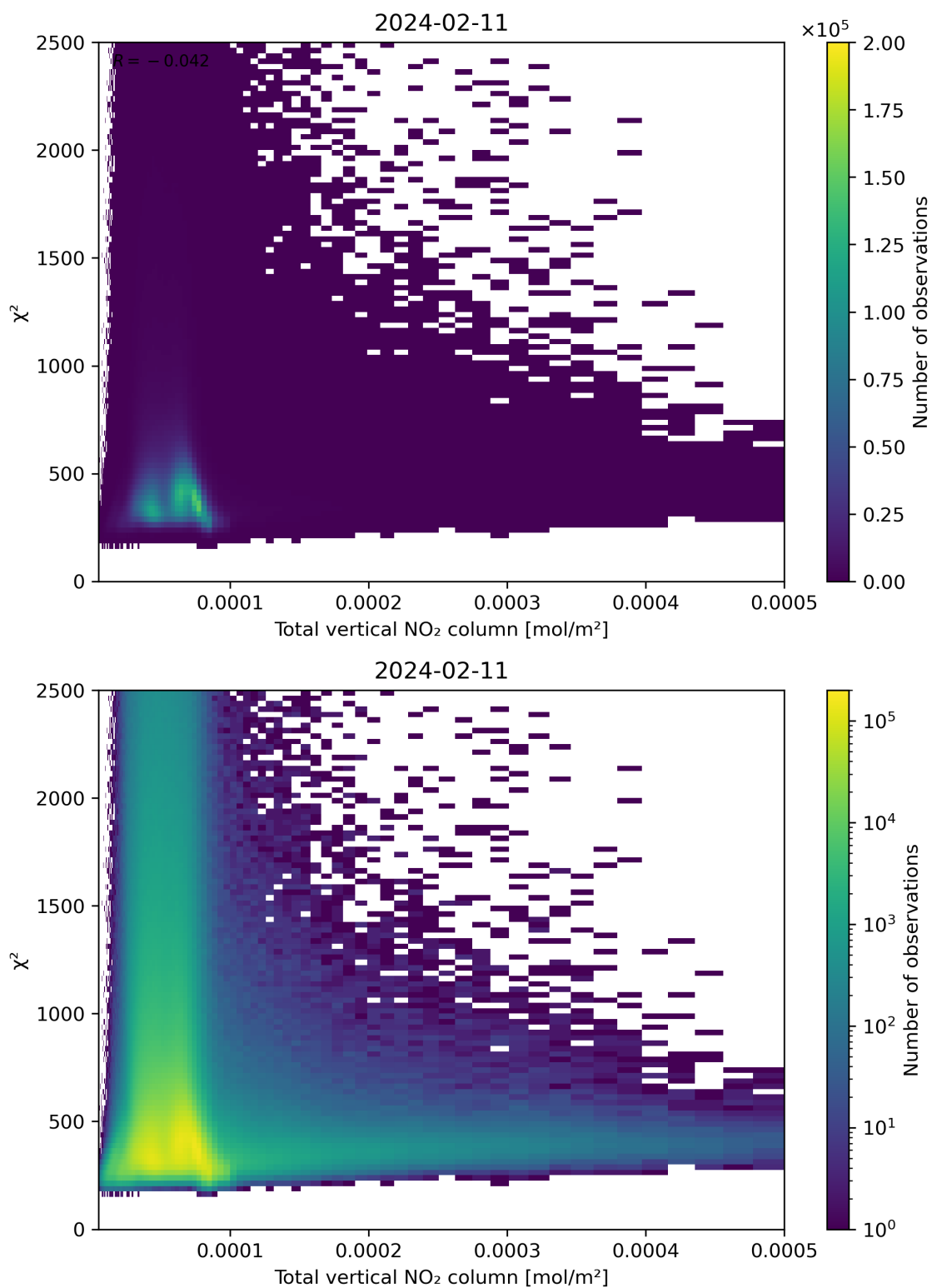
Figure 111: Scatter density plot of “Total vertical NO 2 column” against “ \chi^2 ” for 2024-02-11 to 2024-02-12.
