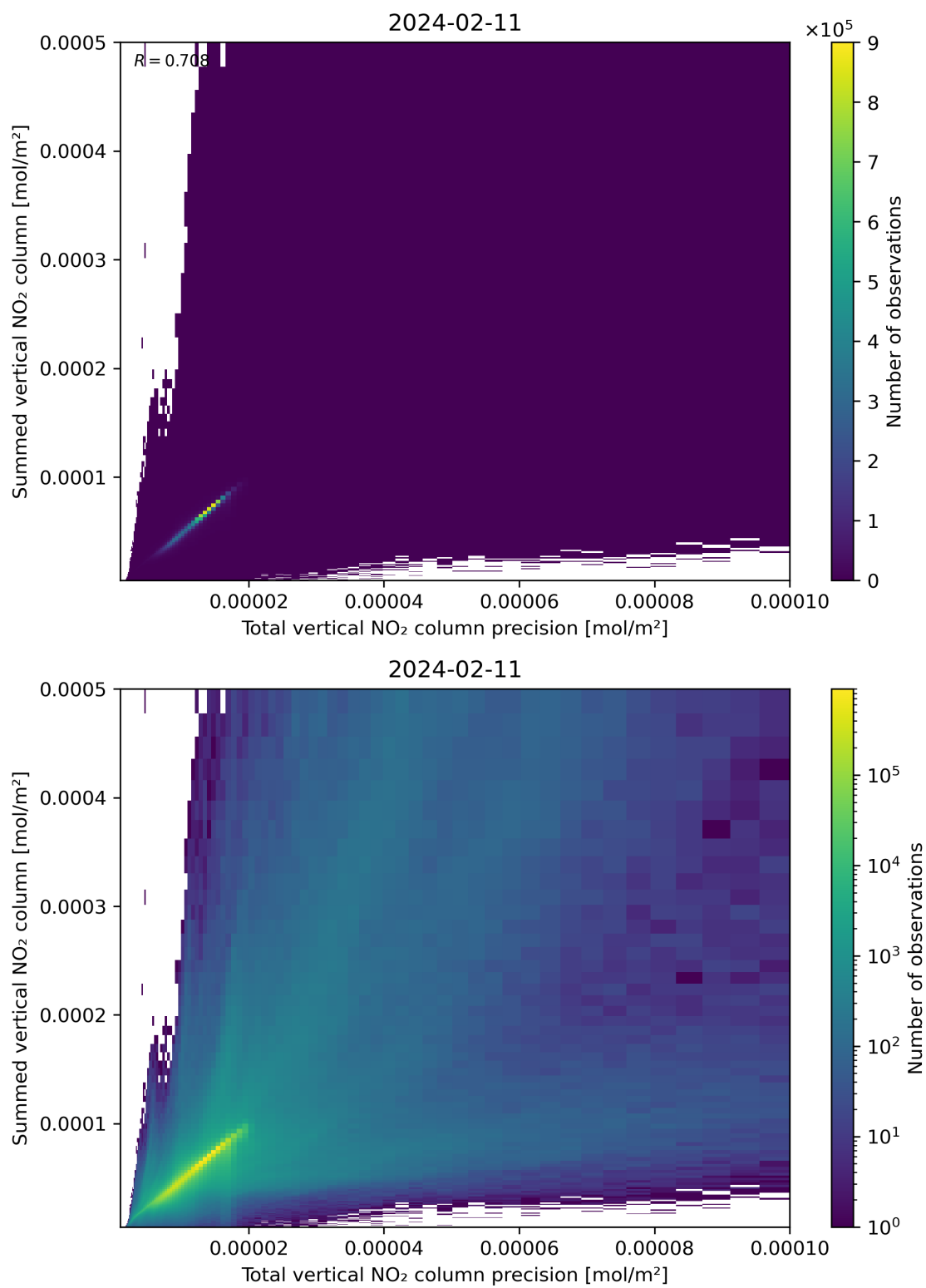
Figure 117: Scatter density plot of “Total vertical NO 2 column precision” against “Summed vertical NO 2 column” for 2024-02-11 to 2024-02-12.
