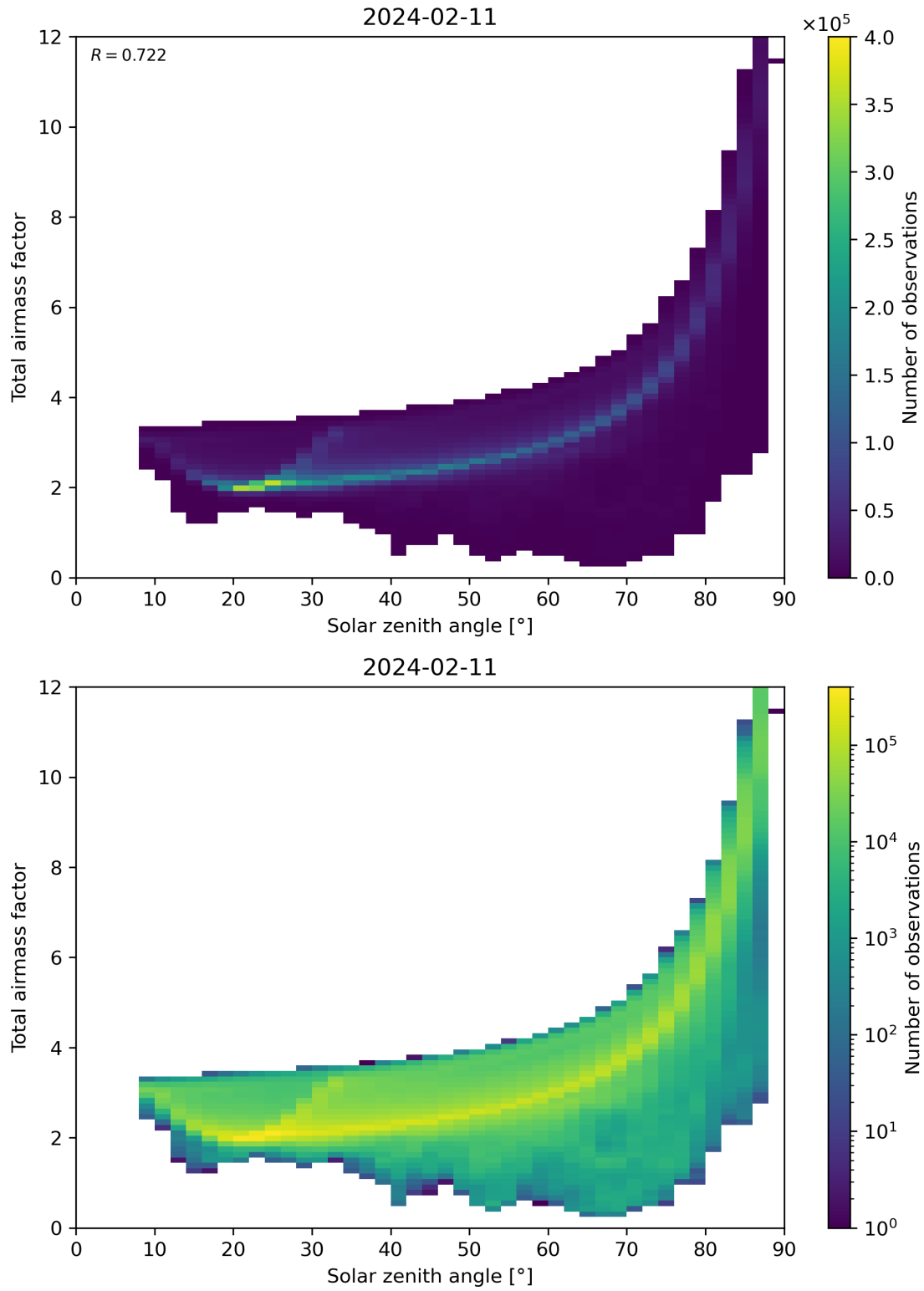
Figure 146: Scatter density plot of “Solar zenith angle” against “Total air mass factor” for 2024-02-11 to 2024-02-12.
