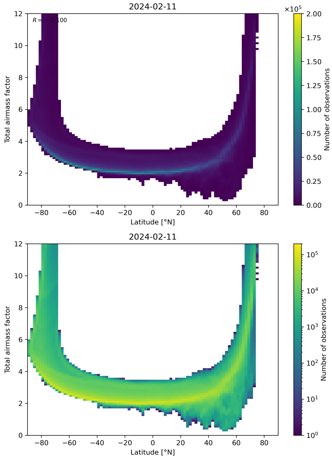
Figure 84: Scatter density plot of “Latitude” against “Total airmass factor” for 2024-02-11 to 2024-02-12.
