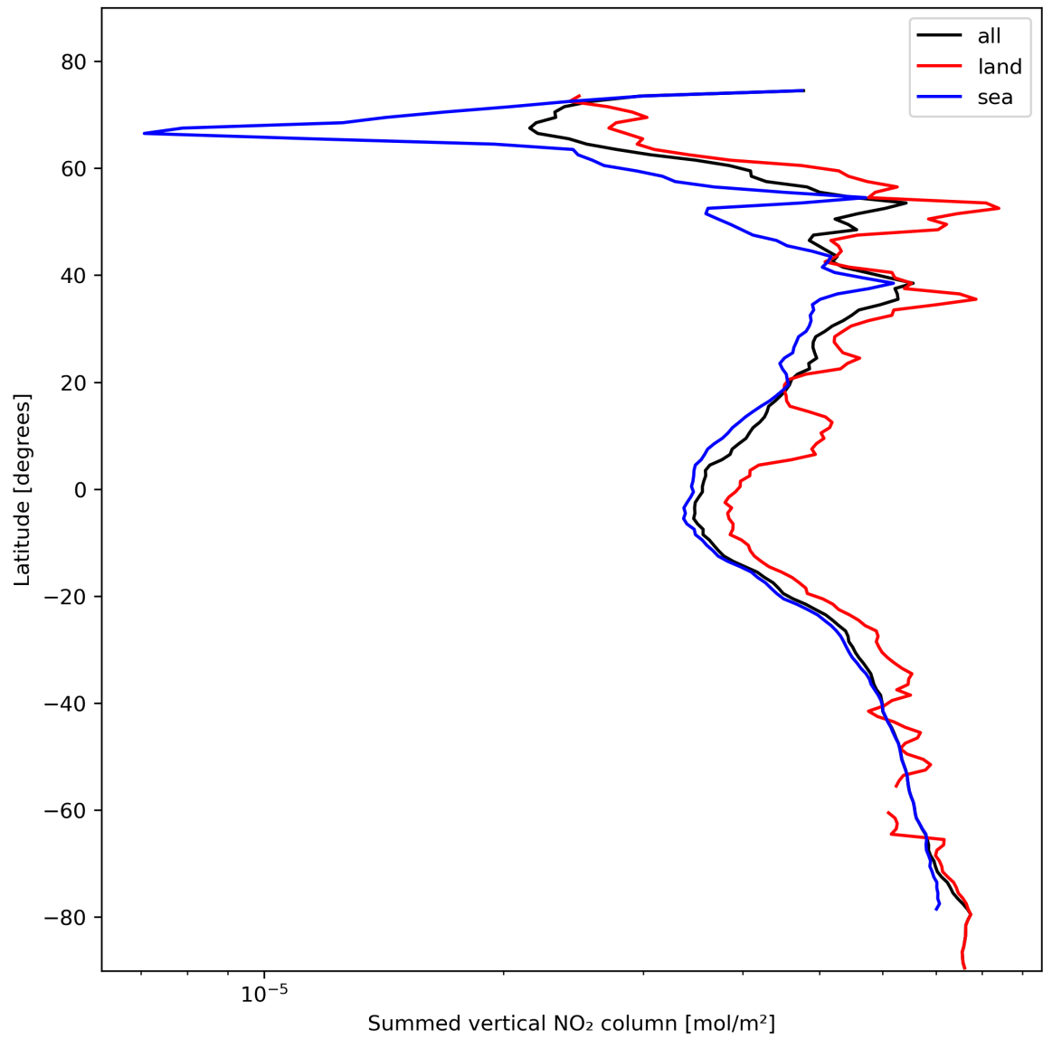
Figure 23: Zonal average of “Summed vertical NO 2 column” for 2024-02-11 to 2024-02-12.
