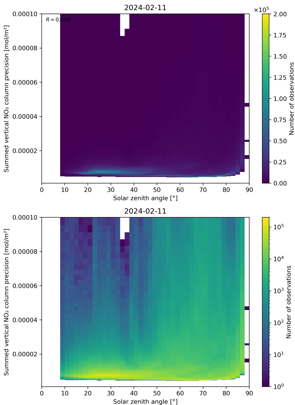
Figure 152: Scatter density plot of “Solar zenith angle” against “Summed vertical NO 2 column precision” for 2024-02-11 to 2024-02-12.
