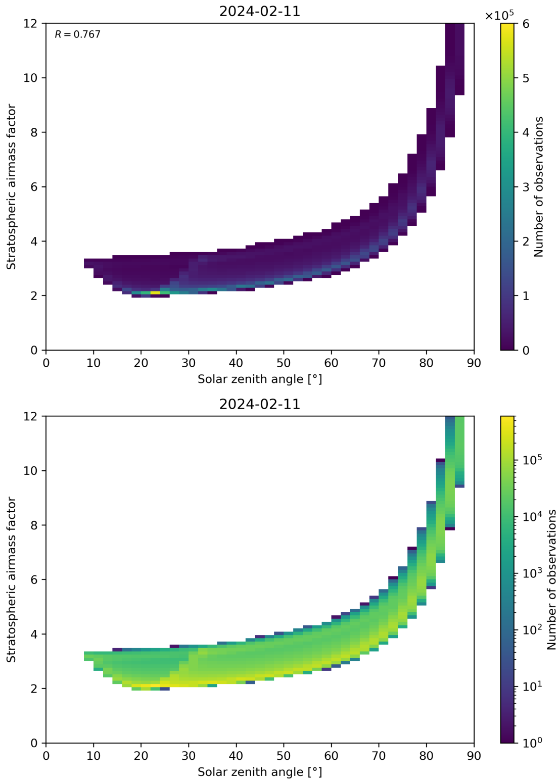
Figure 145: Scatter density plot of “Solar zenith angle” against “Stratospheric airmass factor” for 2024-02-11 to 2024-02-12.
