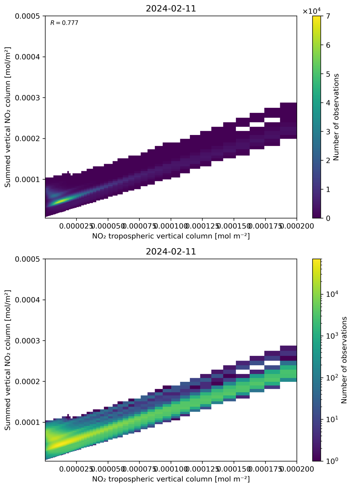
Figure 126: Scatter density plot of “NO 2 tropospheric vertical column” against “Summed vertical NO 2 column” for 2024-02-11 to 2024-02-12.
