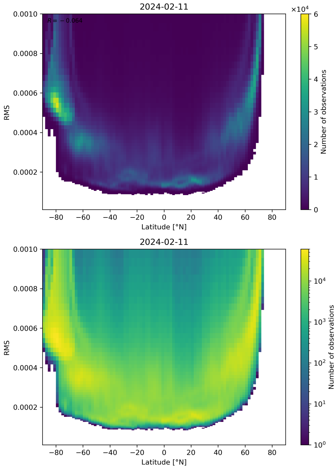
Figure 94: Scatter density plot of “Latitude” against “RMS” for 2024-02-11 to 2024-02-12.
