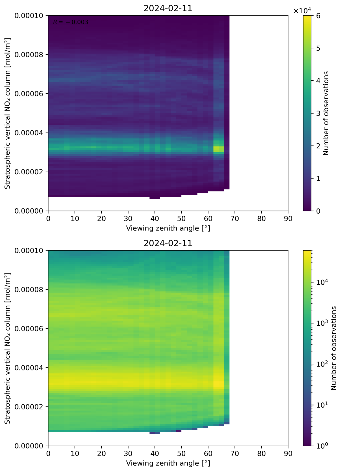
Figure 164: Scatter density plot of “Viewing zenith angle” against “Stratospheric vertical NO 2 column” for 2024-02-11 to 2024-02-12.
