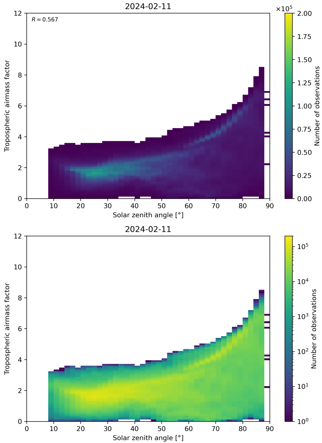
Figure 147: Scatter density plot of “Solar zenith angle” against “Tropospheric airmass factor” for 2024-02-11 to 2024-02-12.
