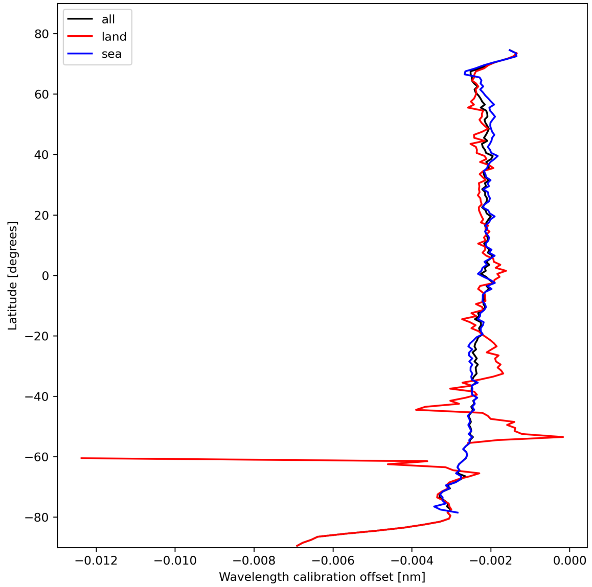
Figure 18: Zonal average of “Wavelength calibration offset” for 2024-02-11 to 2024-02-12.
