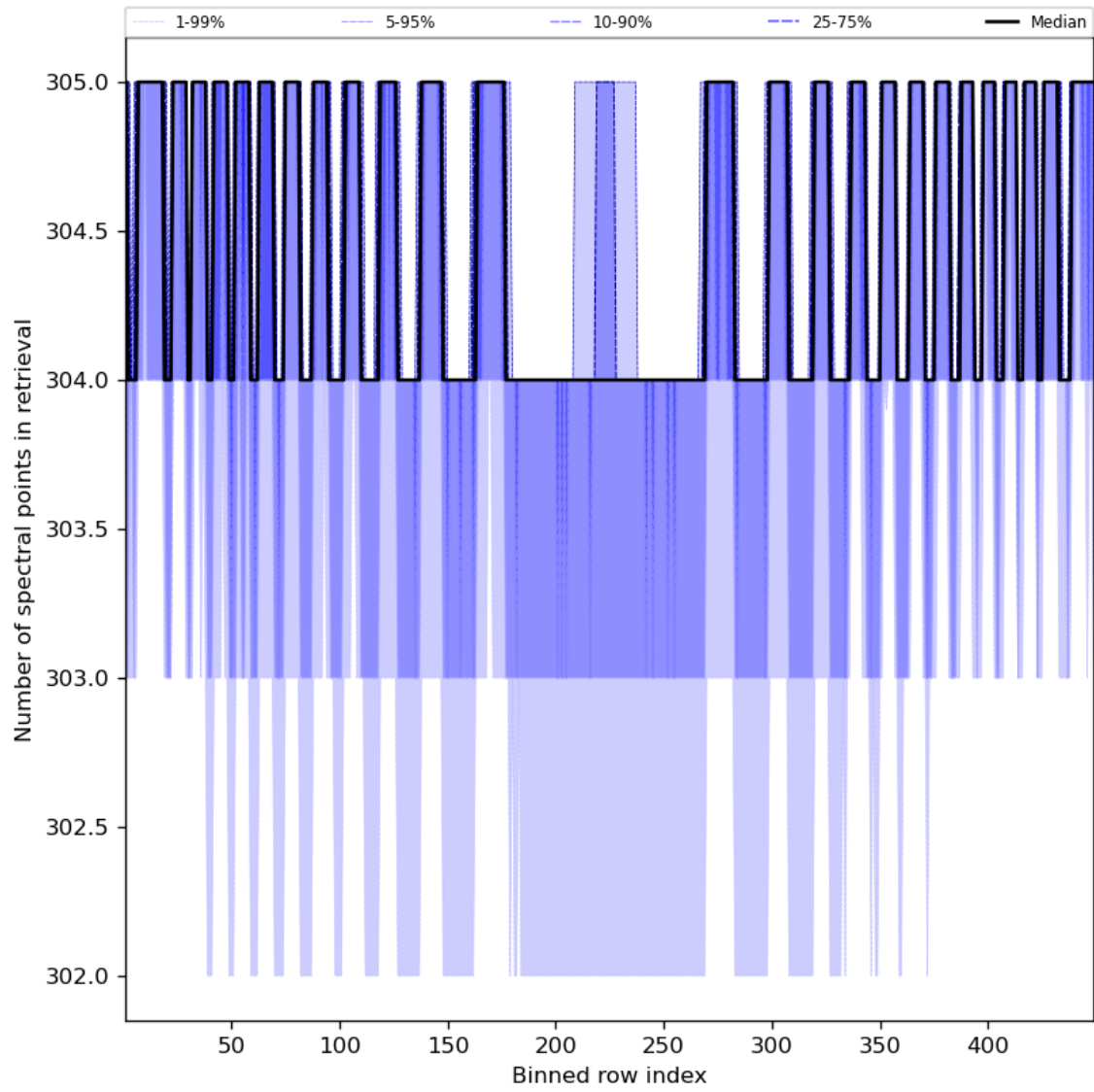
Figure 50: Along track statistics of “Number of spectral points in retrieval” for 2024-02-11 to 2024-02-12
