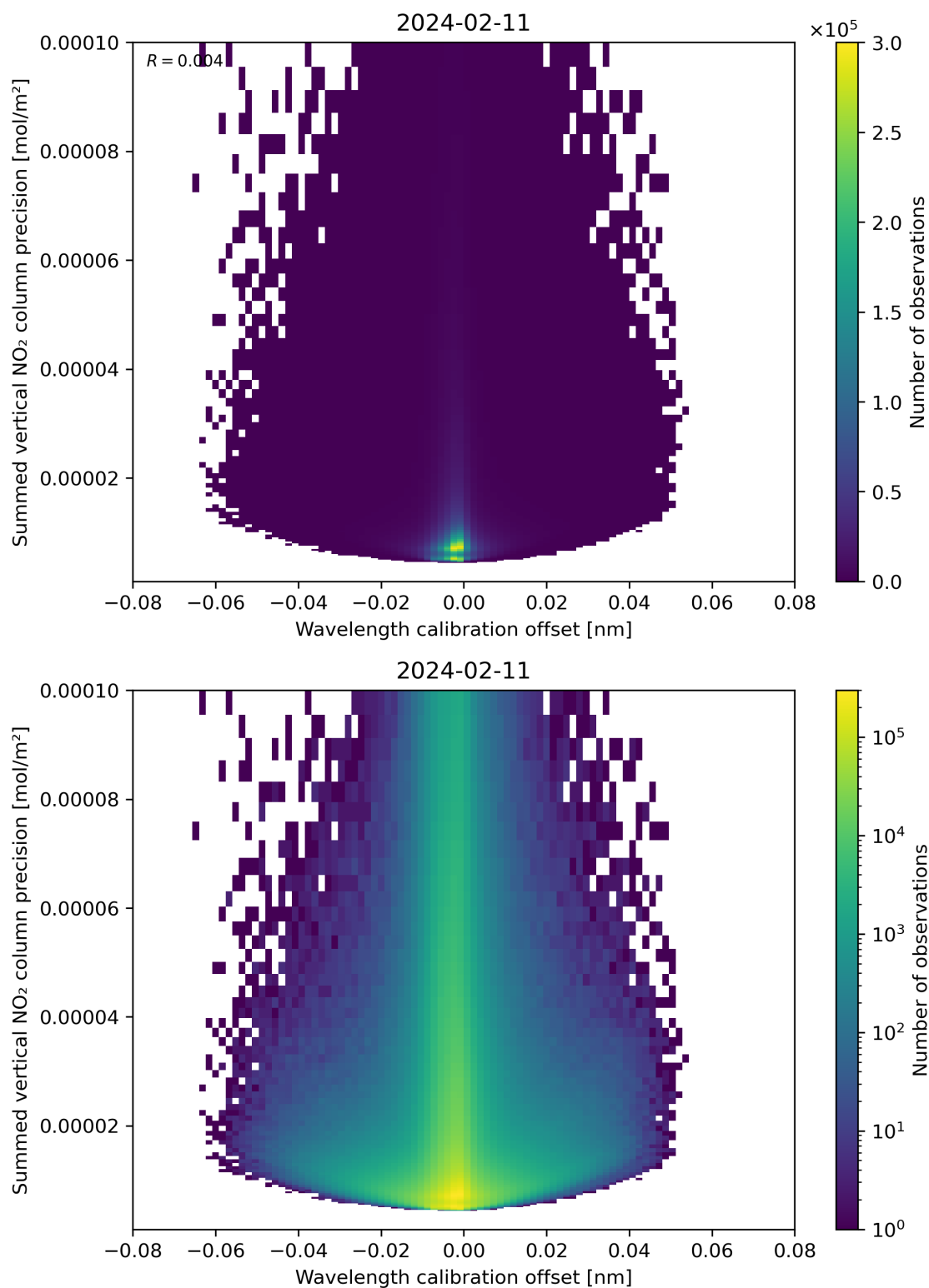
Figure 178: Scatter density plot of “Wavelength calibration offset” against “Summed vertical NO 2 column precision” for 2024-02-11 to 2024-02-12.
