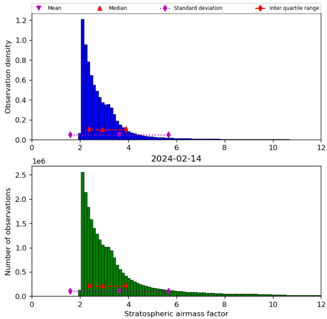
Figure 44: Histogram of “Stratospheric airmass factor” for 2024-02-13 to 2024-02-15
