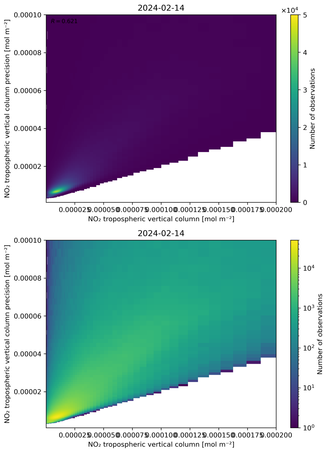
Figure 130: Scatter density plot of “NO 2 tropospheric vertical column” against “NO 2 tropospheric vertical column precision” for 2024-02-13 to 2024-02-15.
