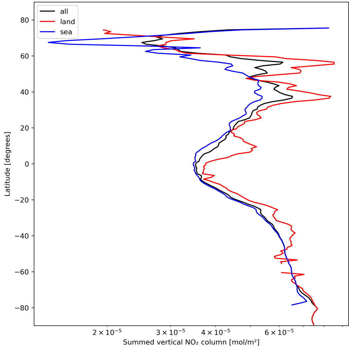
Figure 23: Zonal average of “Summed vertical NO 2 column” for 2024-02-13 to 2024-02-15.
