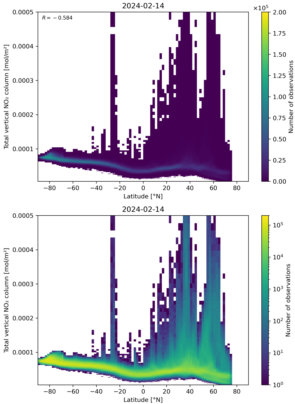
Figure 90: Scatter density plot of “Latitude” against “Total vertical NO 2 column” for 2024-02-13 to 2024-02-15.
