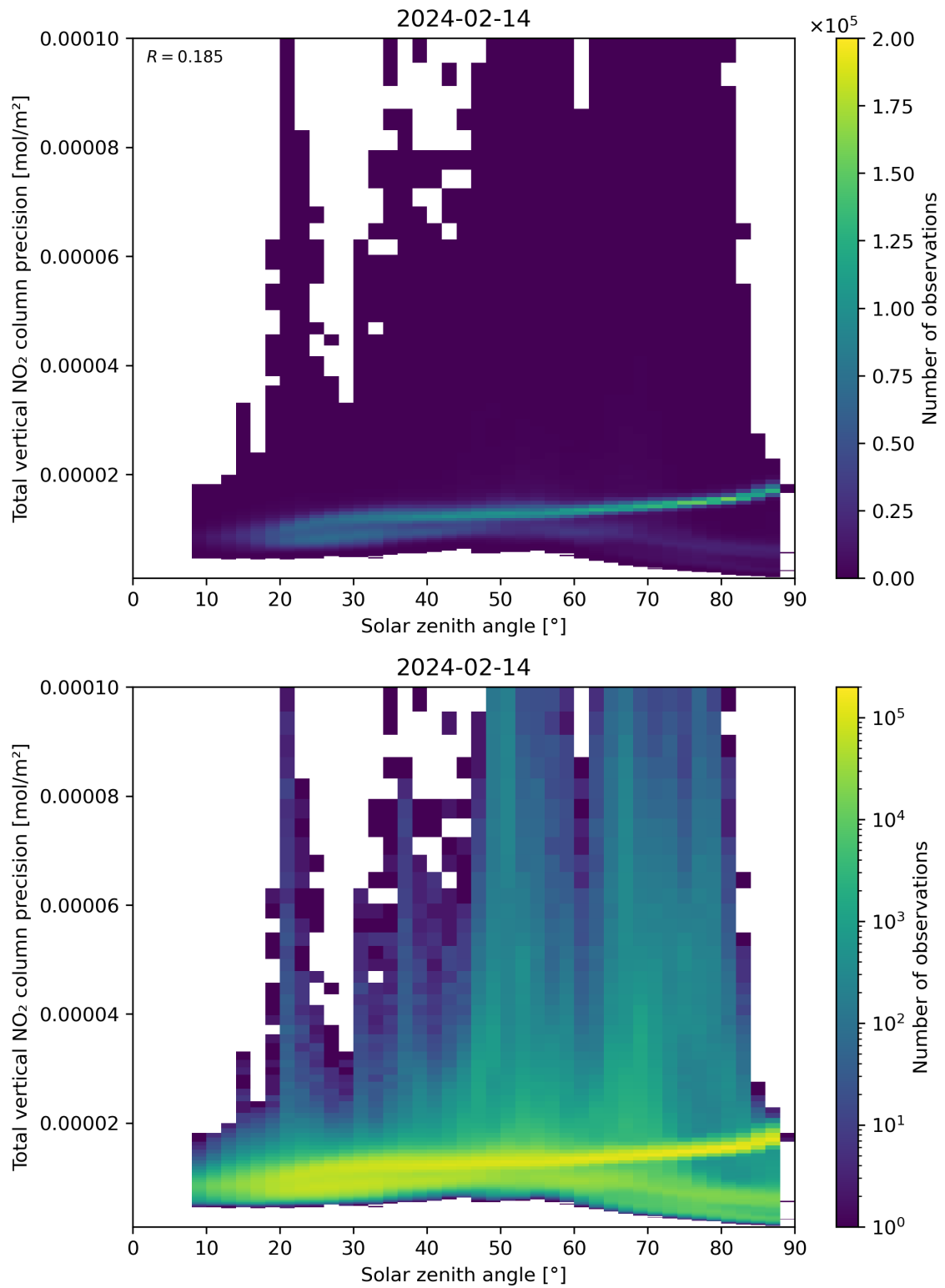
Figure 154: Scatter density plot of “Solar zenith angle” against “Total vertical NO 2 column precision” for 2024-02-13 to 2024-02-15.
