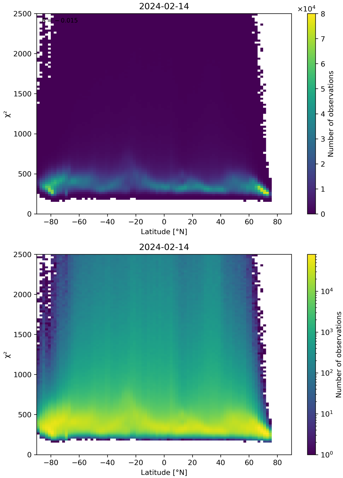
Figure 86: Scatter density plot of “Latitude” against “ \chi^2 ” for 2024-02-13 to 2024-02-15.
