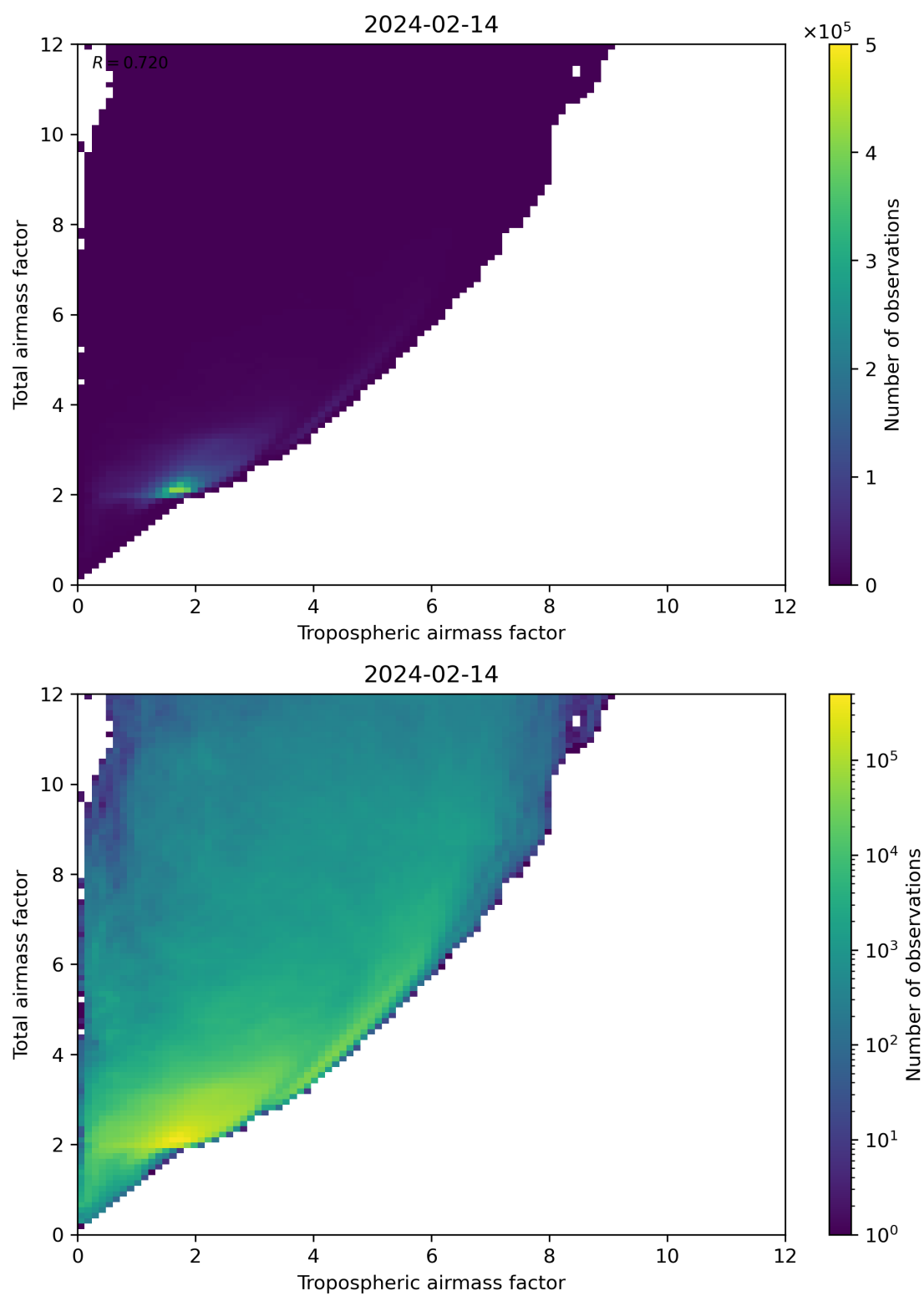
Figure 72: Scatter density plot of “Tropospheric airmass factor” against “Total airmass factor” for 2024-02-13 to 2024-02-15.
