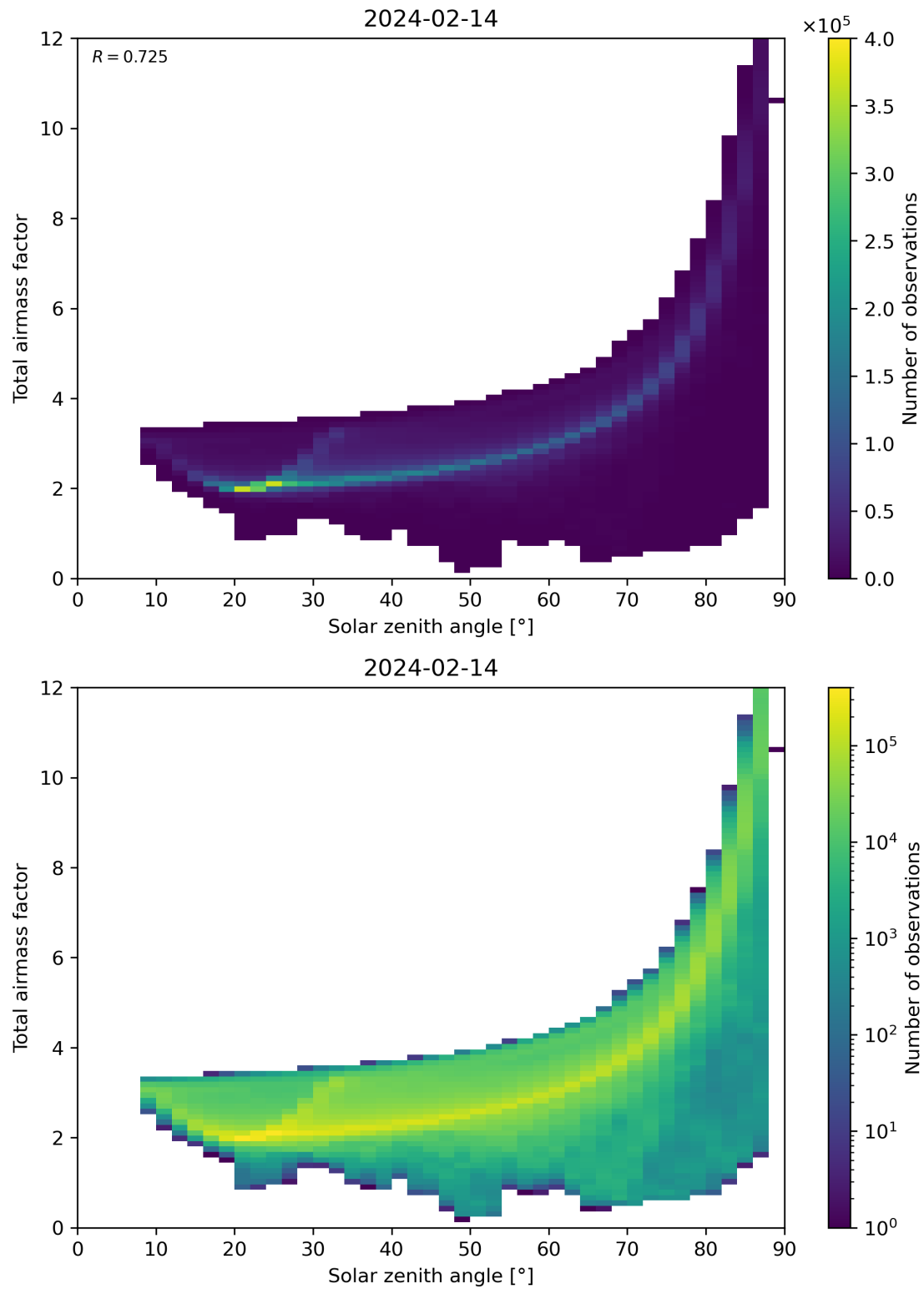
Figure 146: Scatter density plot of “Solar zenith angle” against “Total air mass factor” for 2024-02-13 to 2024-02-15.
