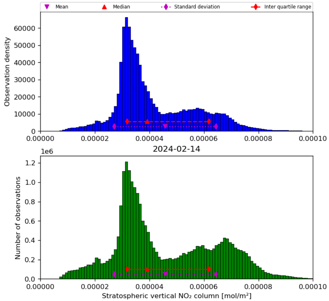
Figure 36: Histogram of “Stratospheric vertical NO 2 column” for 2024-02-13 to 2024-02-15
