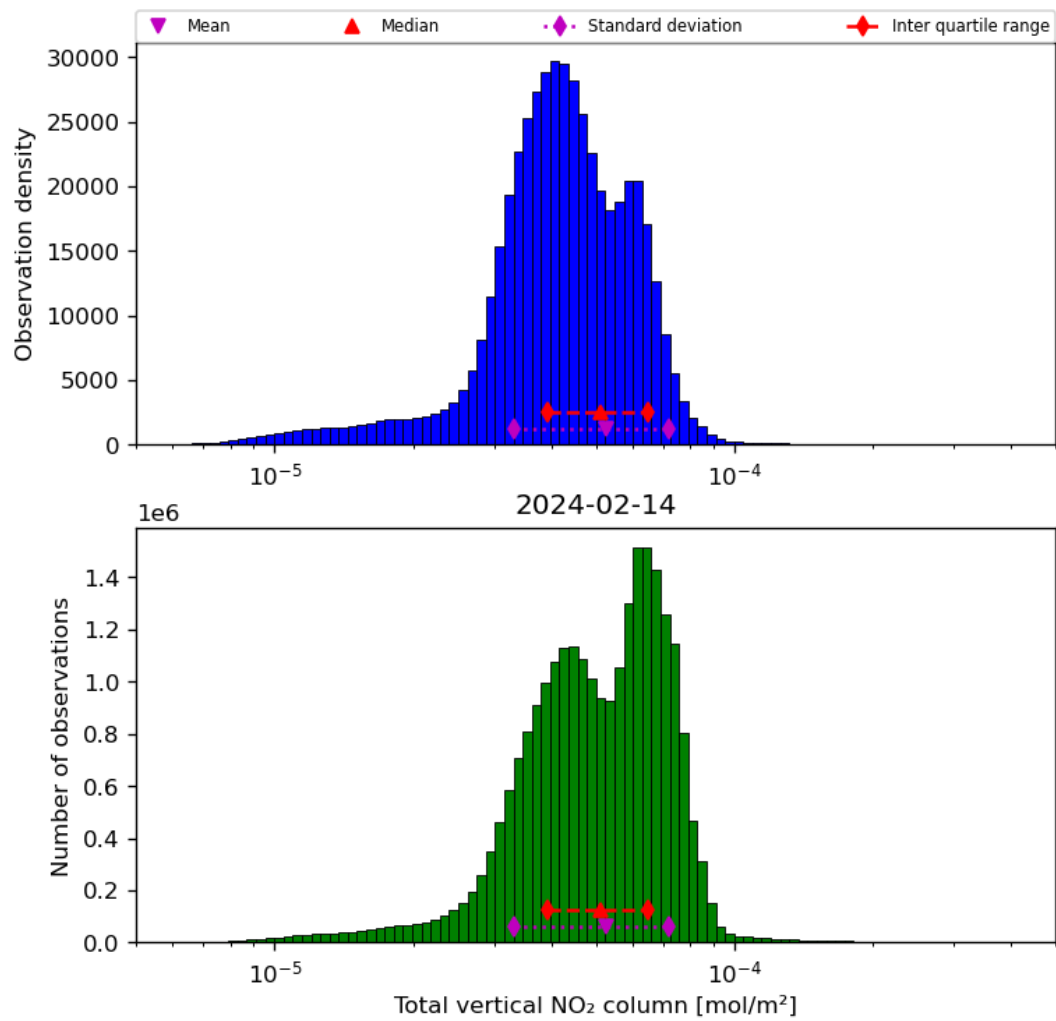
Figure 38: Histogram of “Total vertical NO 2 column” for 2024-02-13 to 2024-02-15
