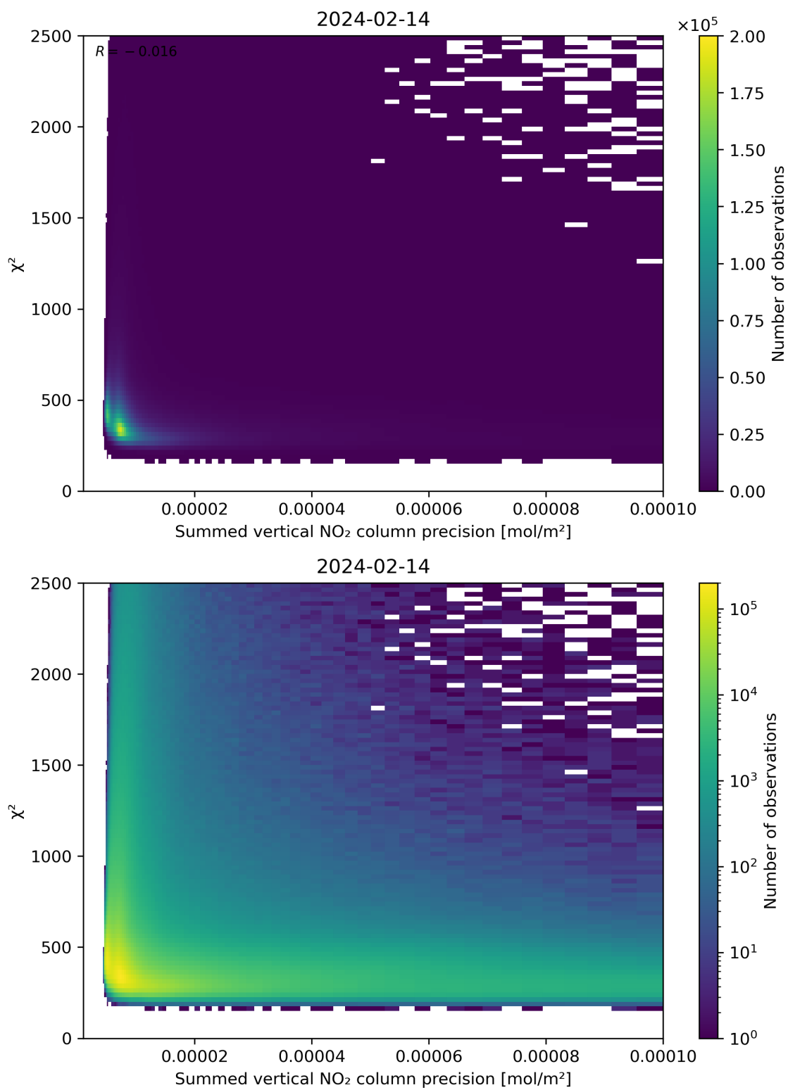
Figure 107: Scatter density plot of “Summed vertical NO 2 column precision” against “ \chi^2 ” for 2024-02-13 to 2024-02-15.
