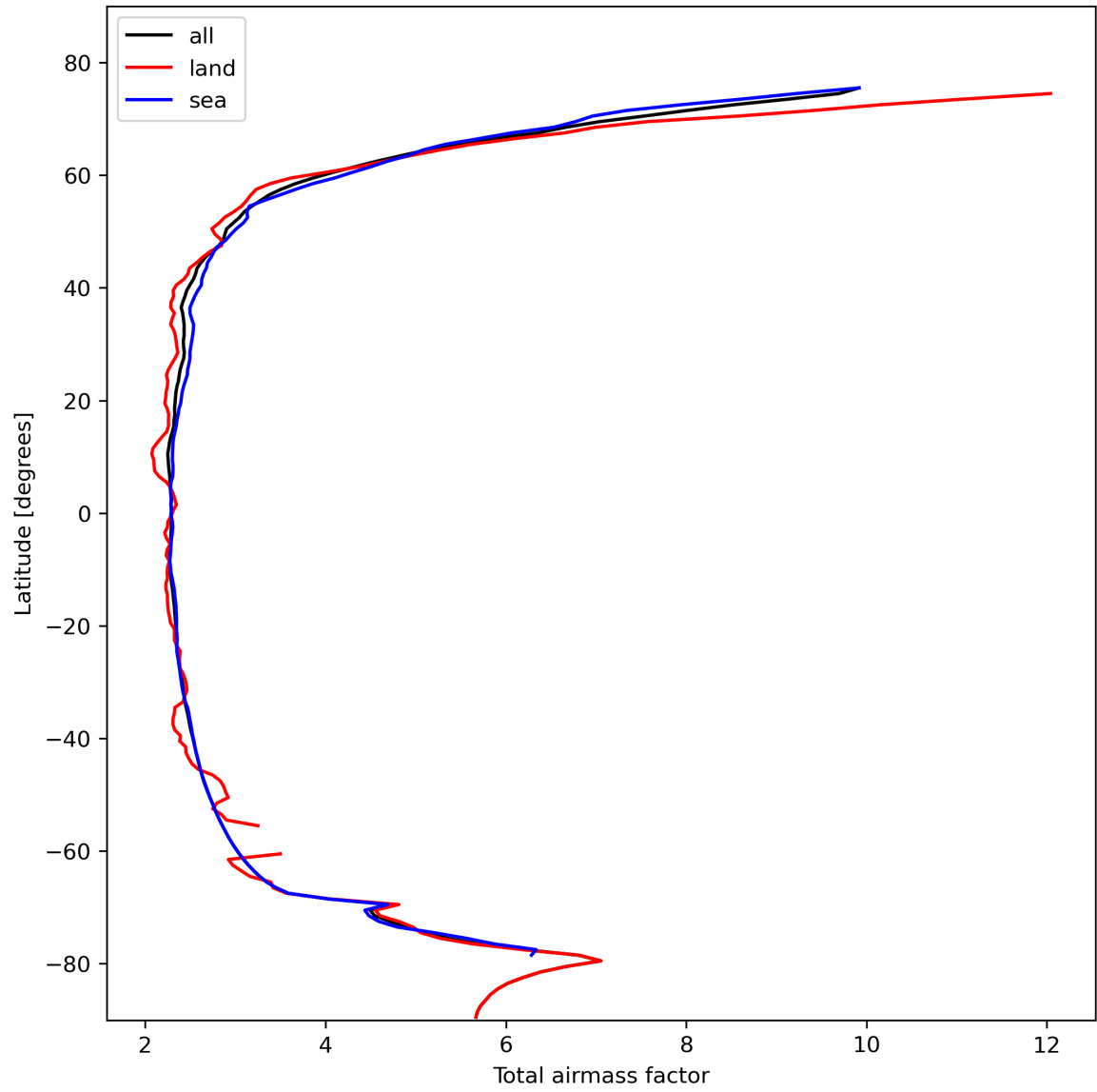
Figure 15: Zonal average of “Total airmass factor” for 2024-02-13 to 2024-02-15.
