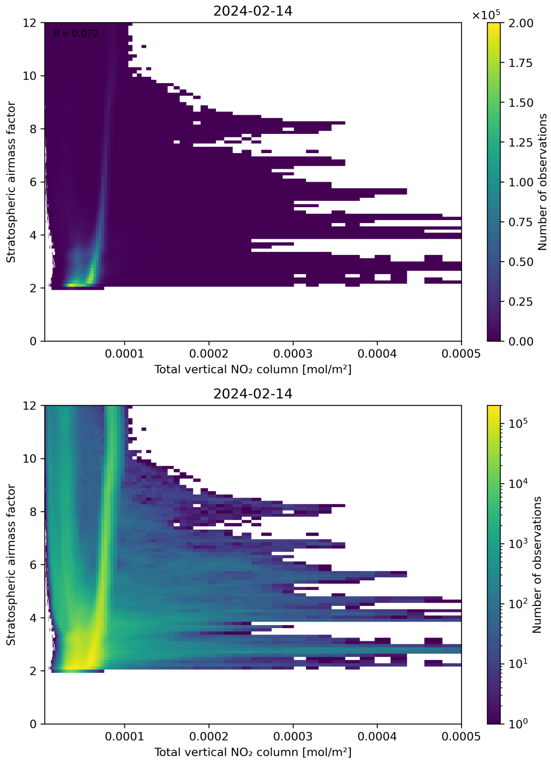
Figure 110: Scatter density plot of “Total vertical NO 2 column” against “Stratospheric airmass factor” for 2024-02-13 to 2024-02-15.
