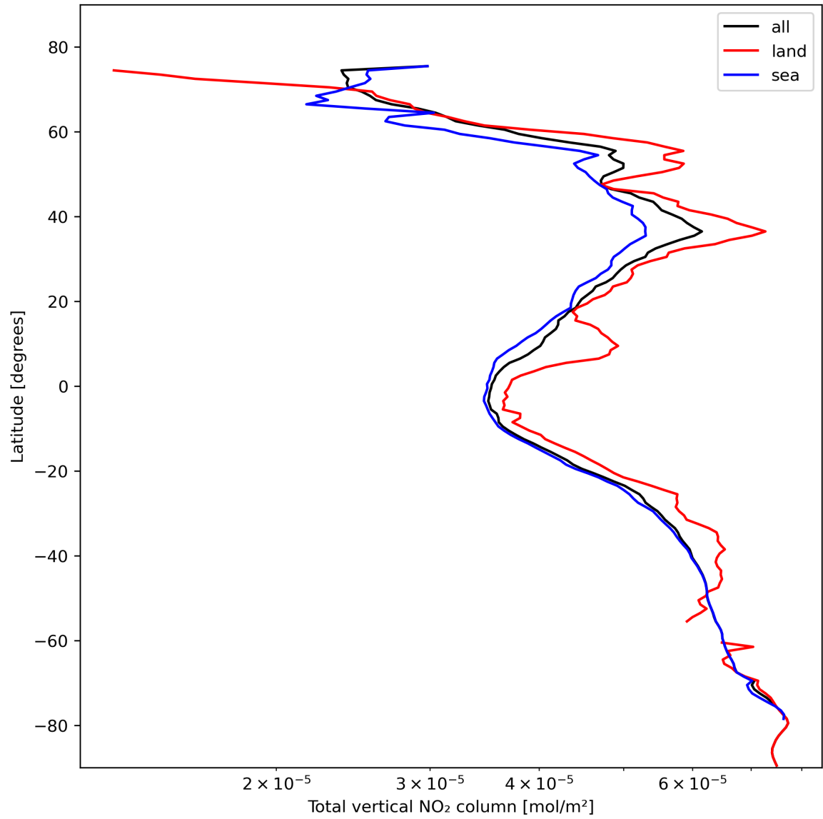
Figure 21: Zonal average of “Total vertical NO 2 column” for 2024-02-13 to 2024-02-15.
