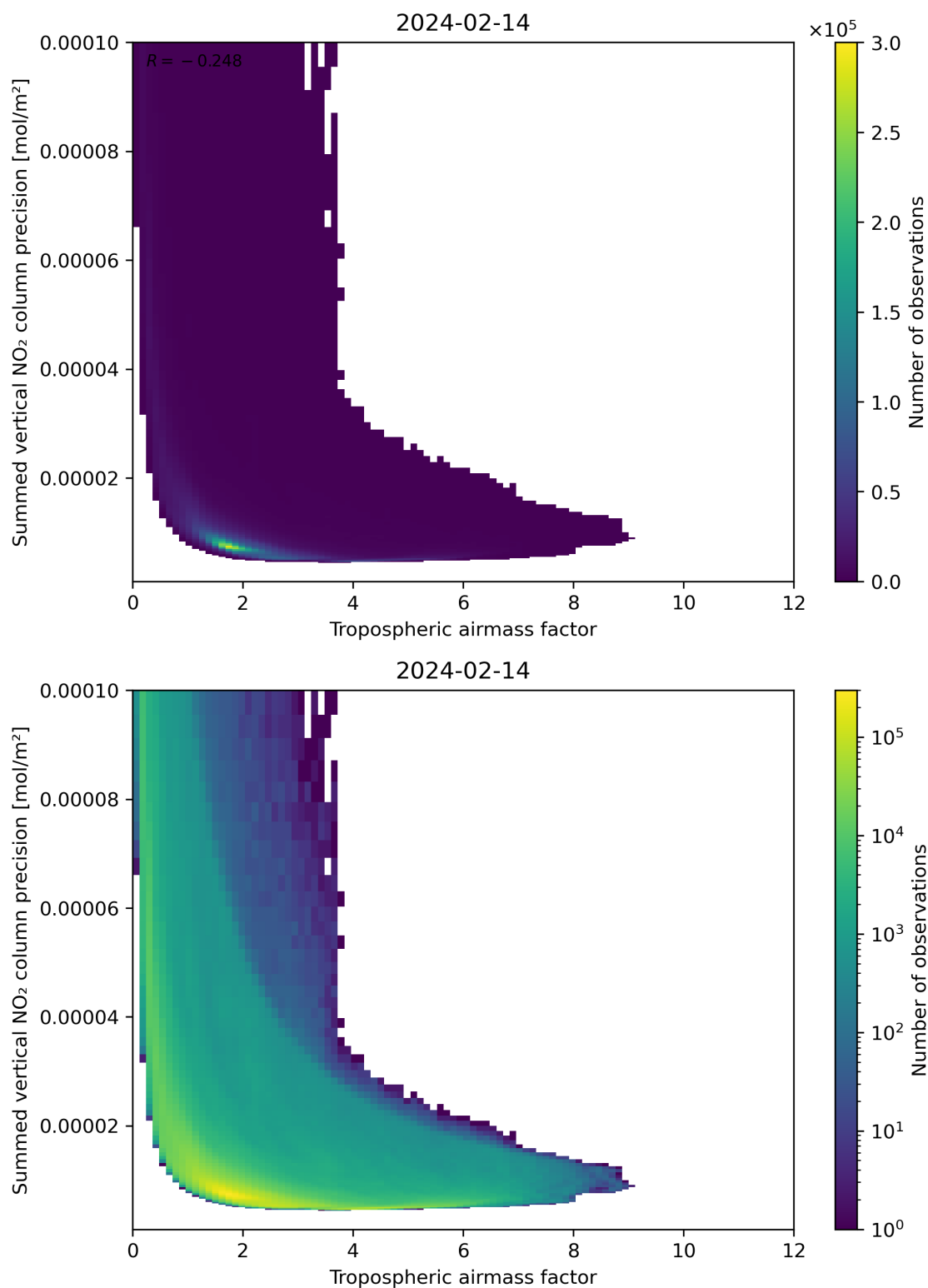
Figure 76: Scatter density plot of “Tropospheric air mass factor” against “Summed vertical NO 2 column precision” for 2024-02-13 to 2024-02-15.
