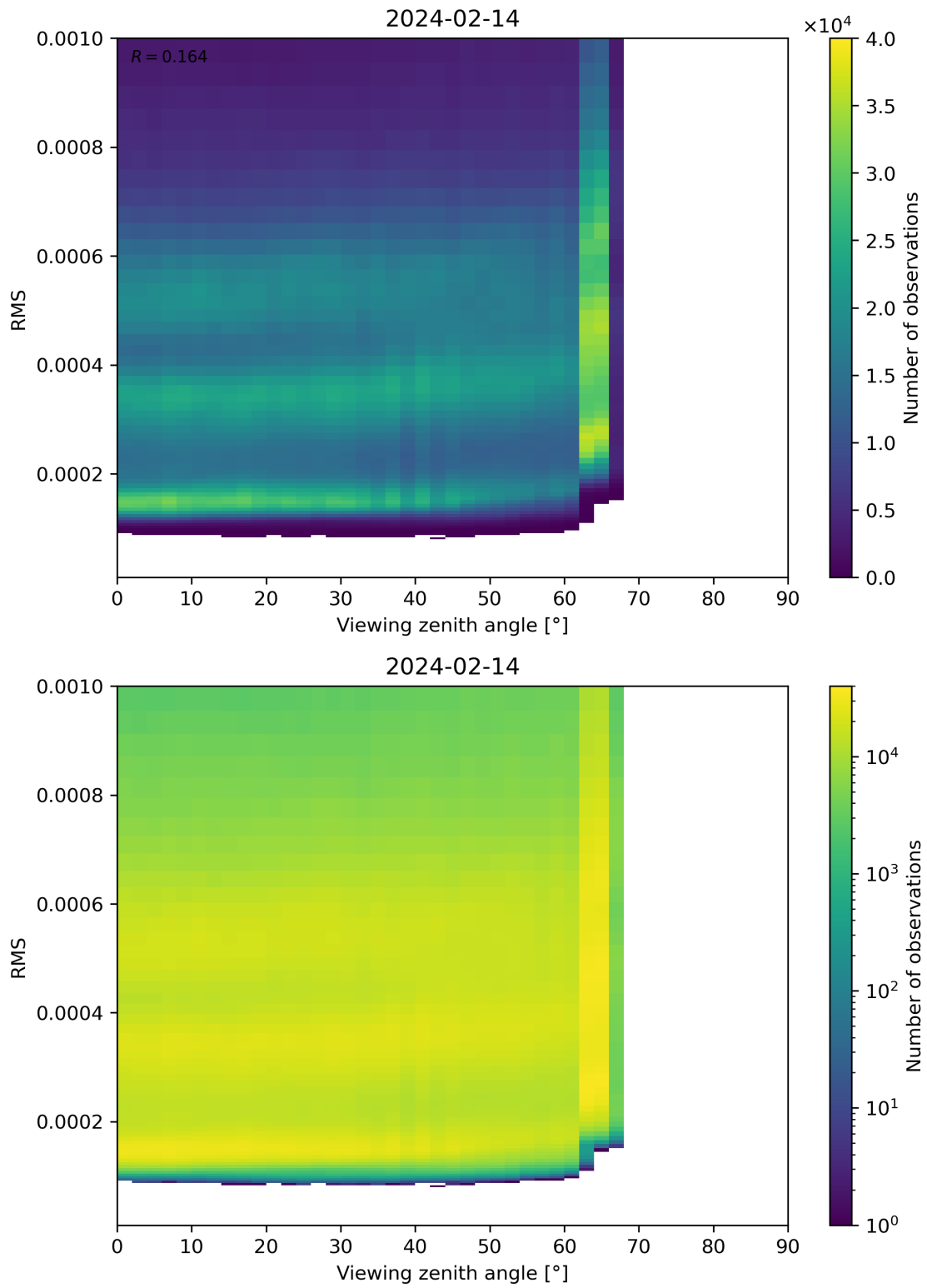
Figure 171: Scatter density plot of “Viewing zenith angle” against “RMS” for 2024-02-13 to 2024-02-15.
