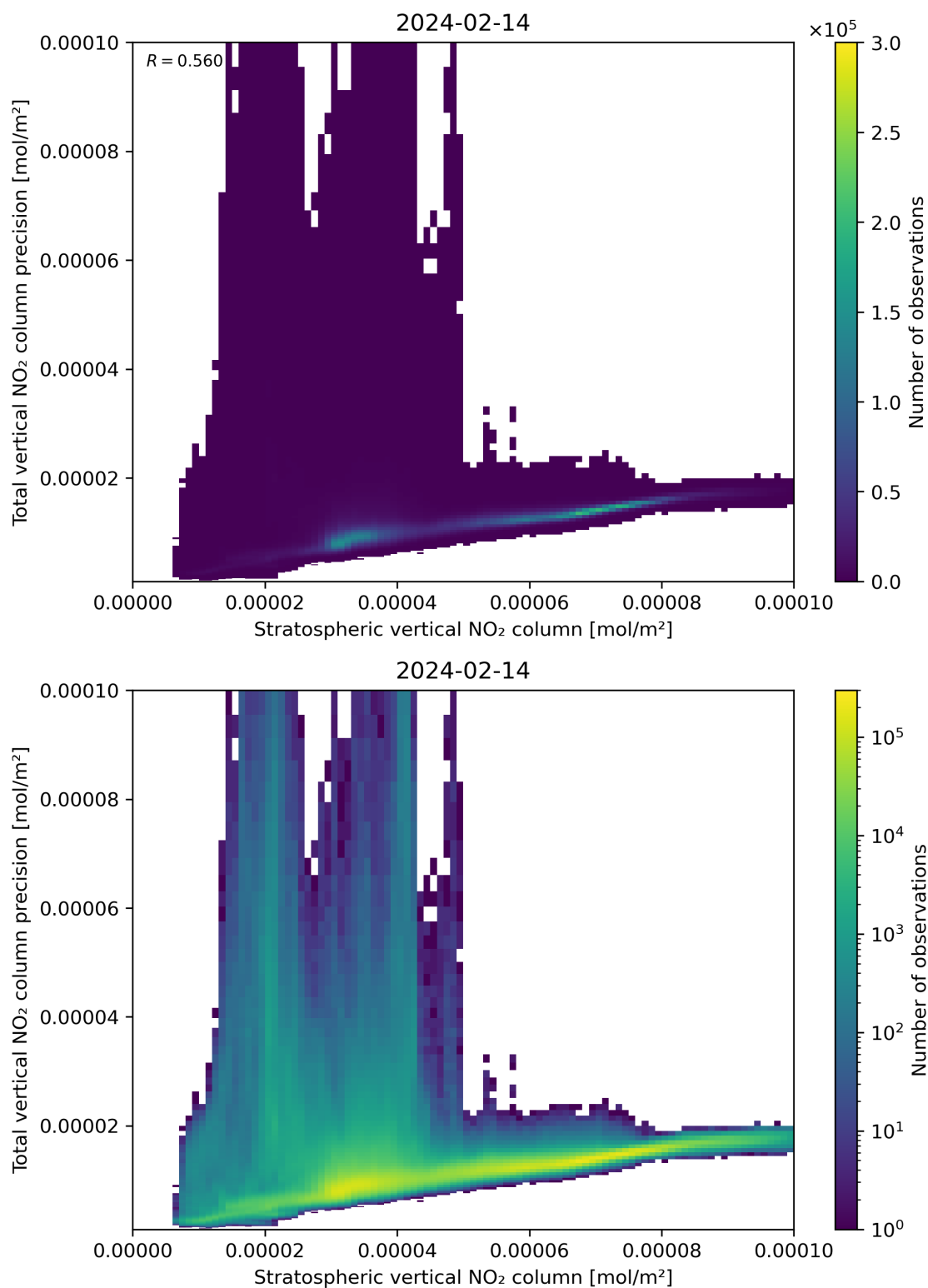
Figure 101: Scatter density plot of “Stratospheric vertical NO 2 column” against “Total vertical NO 2 column precision” for 2024-02-13 to 2024-02-15.
