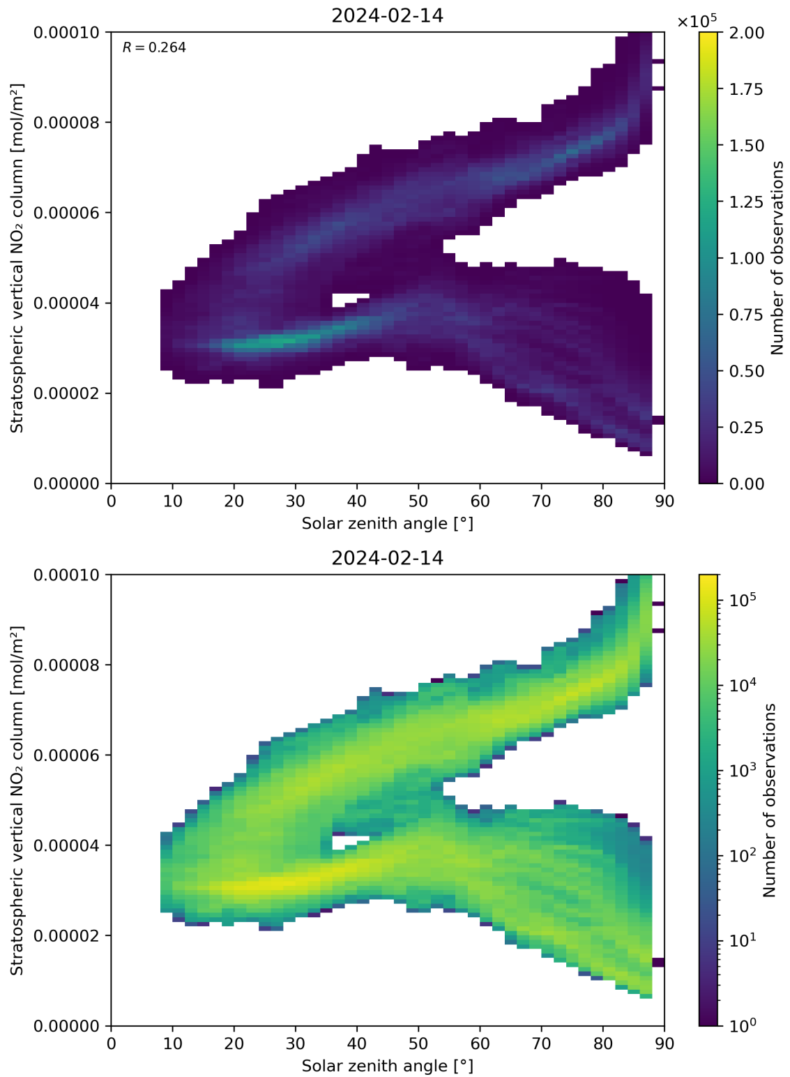
Figure 150: Scatter density plot of “Solar zenith angle” against “Stratospheric vertical NO 2 column” for 2024-02-13 to 2024-02-15.
