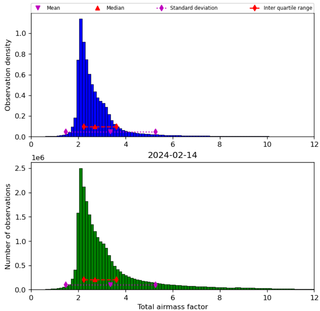
Figure 32: Histogram of “Total airmass factor” for 2024-02-13 to 2024-02-15
