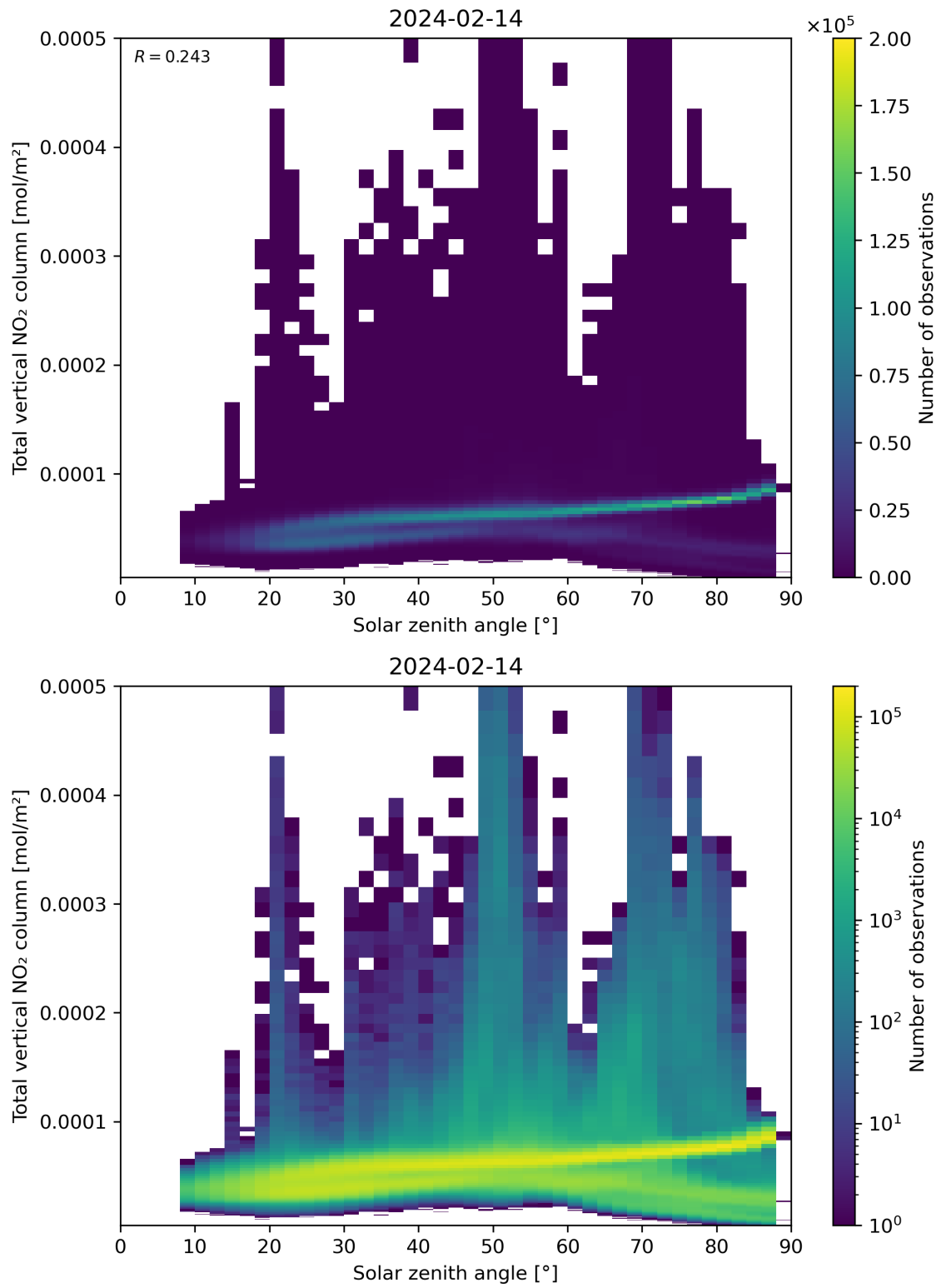
Figure 153: Scatter density plot of “Solar zenith angle” against “Total vertical NO 2 column” for 2024-02-13 to 2024-02-15.
