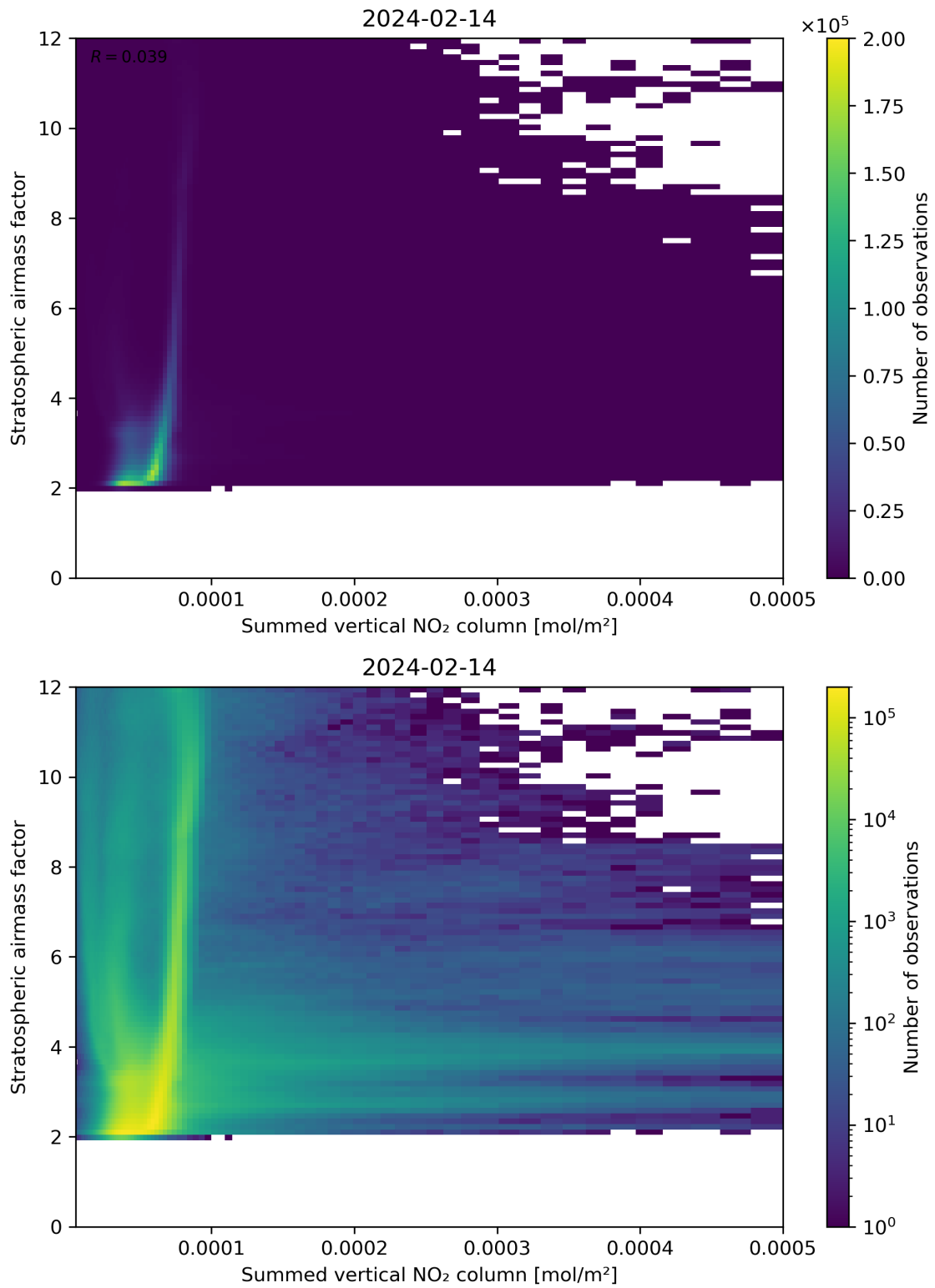
Figure 103: Scatter density plot of “Summed vertical NO 2 column” against “Stratospheric airmass factor” for 2024-02-13 to 2024-02-15.
