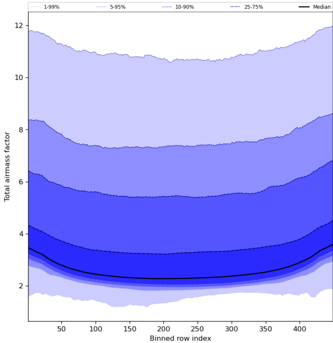
Figure 49: Along track statistics of “Total airmass factor” for 2024-02-13 to 2024-02-15
