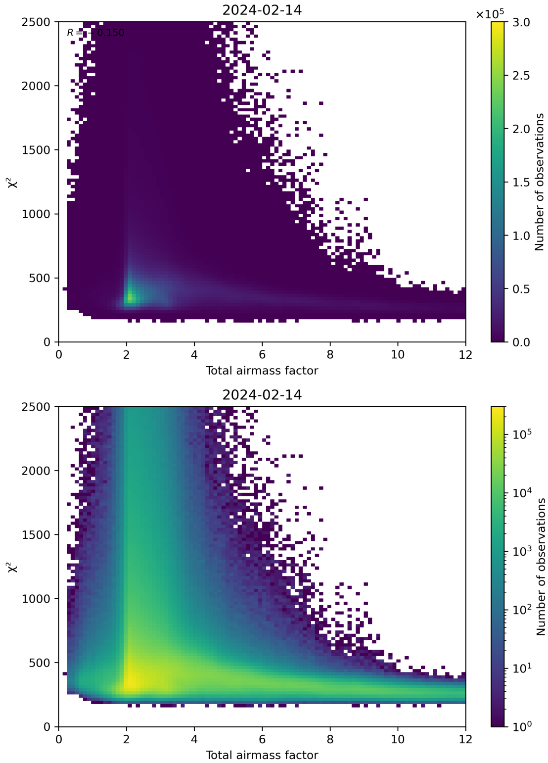
Figure 63: Scatter density plot of “Total airmass factor” against “ \chi^2 ” for 2024-02-13 to 2024-02-15.
