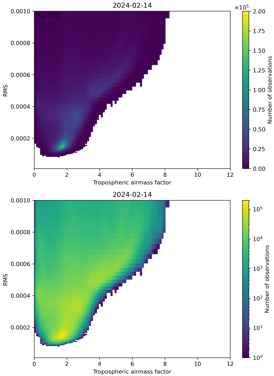
Figure 79: Scatter density plot of “Tropospheric airmass factor” against “RMS” for 2024-02-13 to 2024-02-15.
