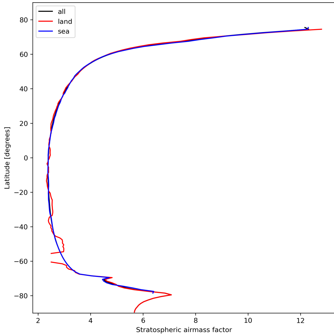
Figure 27: Zonal average of “Stratospheric air mass factor” for 2024-02-13 to 2024-02-15.
