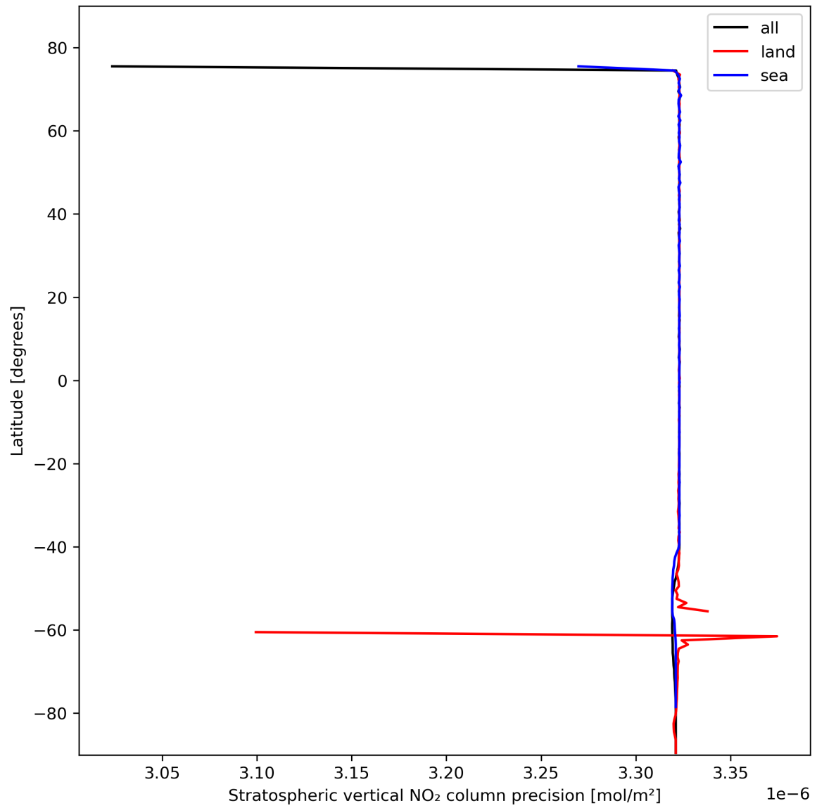
Figure 20: Zonal average of "Stratospheric vertical NO 2 column precision" for 2024-02-13 to 2024-02-15.
