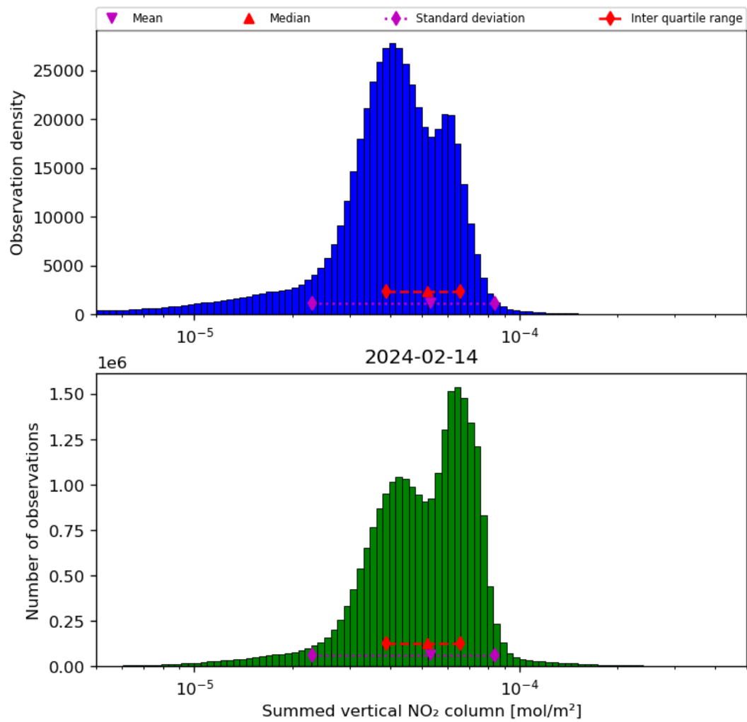
Figure 40: Histogram of “Summed vertical NO 2 column” for 2024-02-13 to 2024-02-15
