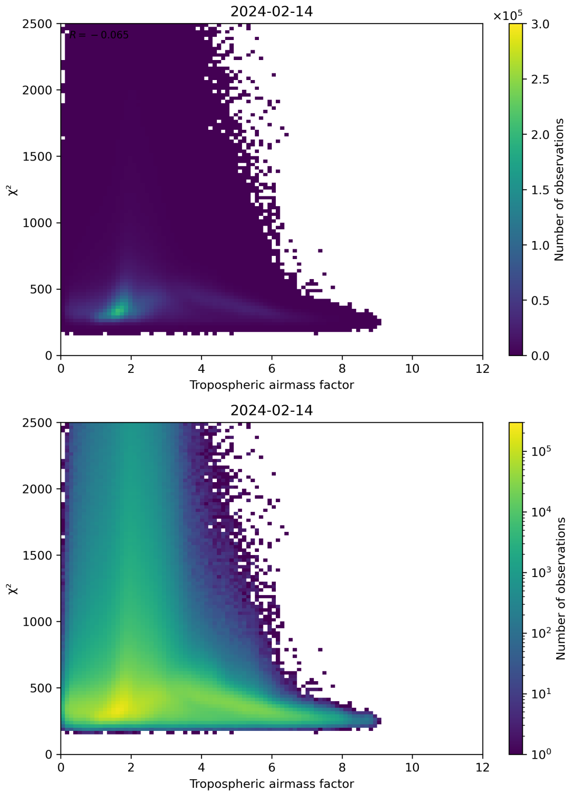
Figure 73: Scatter density plot of “Tropospheric airmass factor” against “ \chi^2 ” for 2024-02-13 to 2024-02-15.
