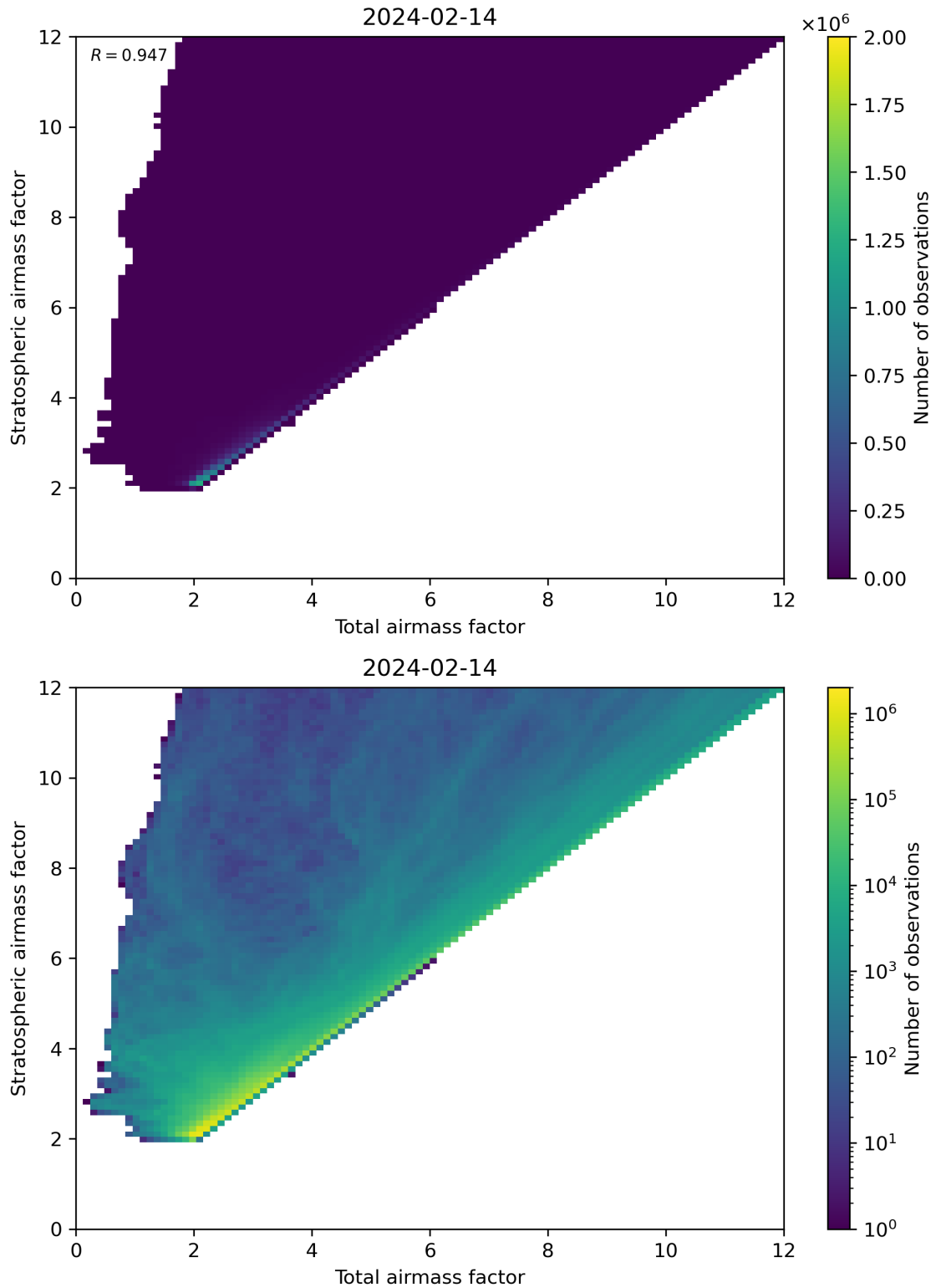
Figure 62: Scatter density plot of “Total airmass factor” against “Stratospheric airmass factor” for 2024-02-13 to 2024-02-15.
