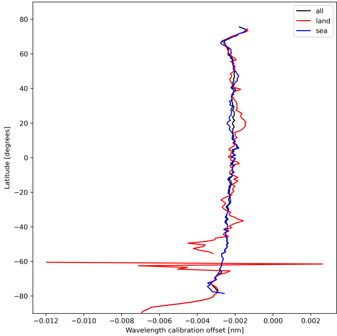
Figure 18: Zonal average of “Wavelength calibration offset” for 2024-02-13 to 2024-02-15.
