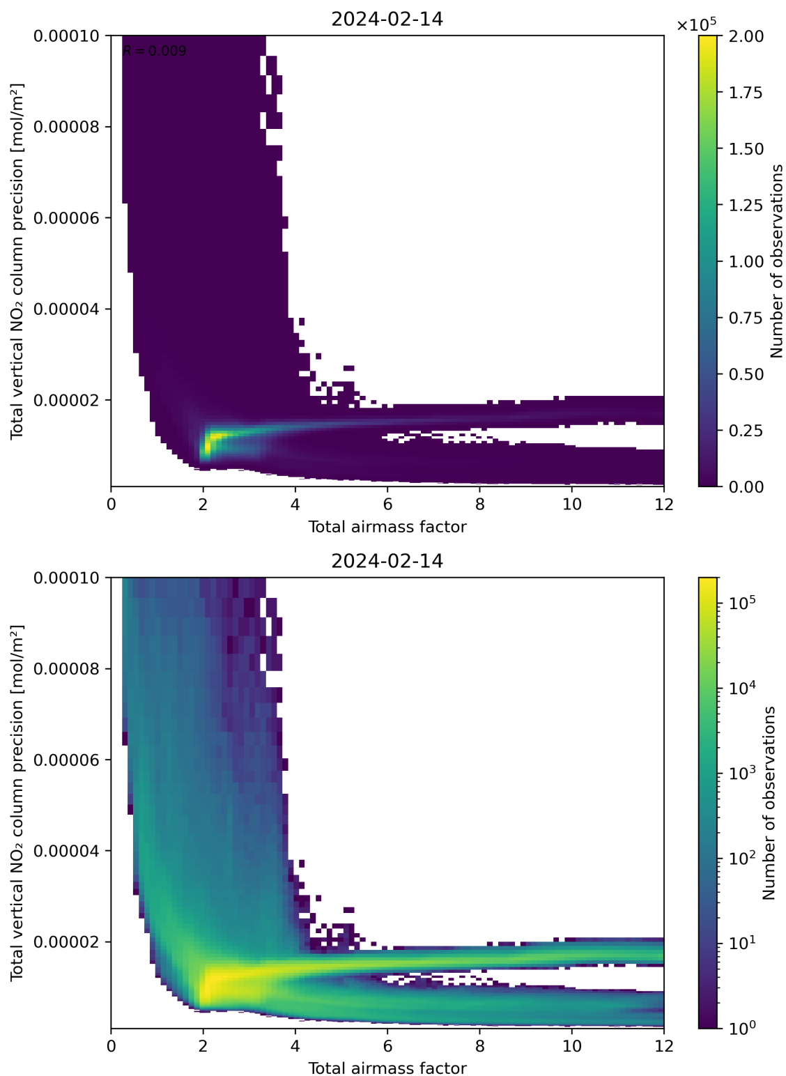
Figure 68: Scatter density plot of “Total airmass factor” against “Total vertical NO 2 column precision” for 2024-02-13 to 2024-02-15.
