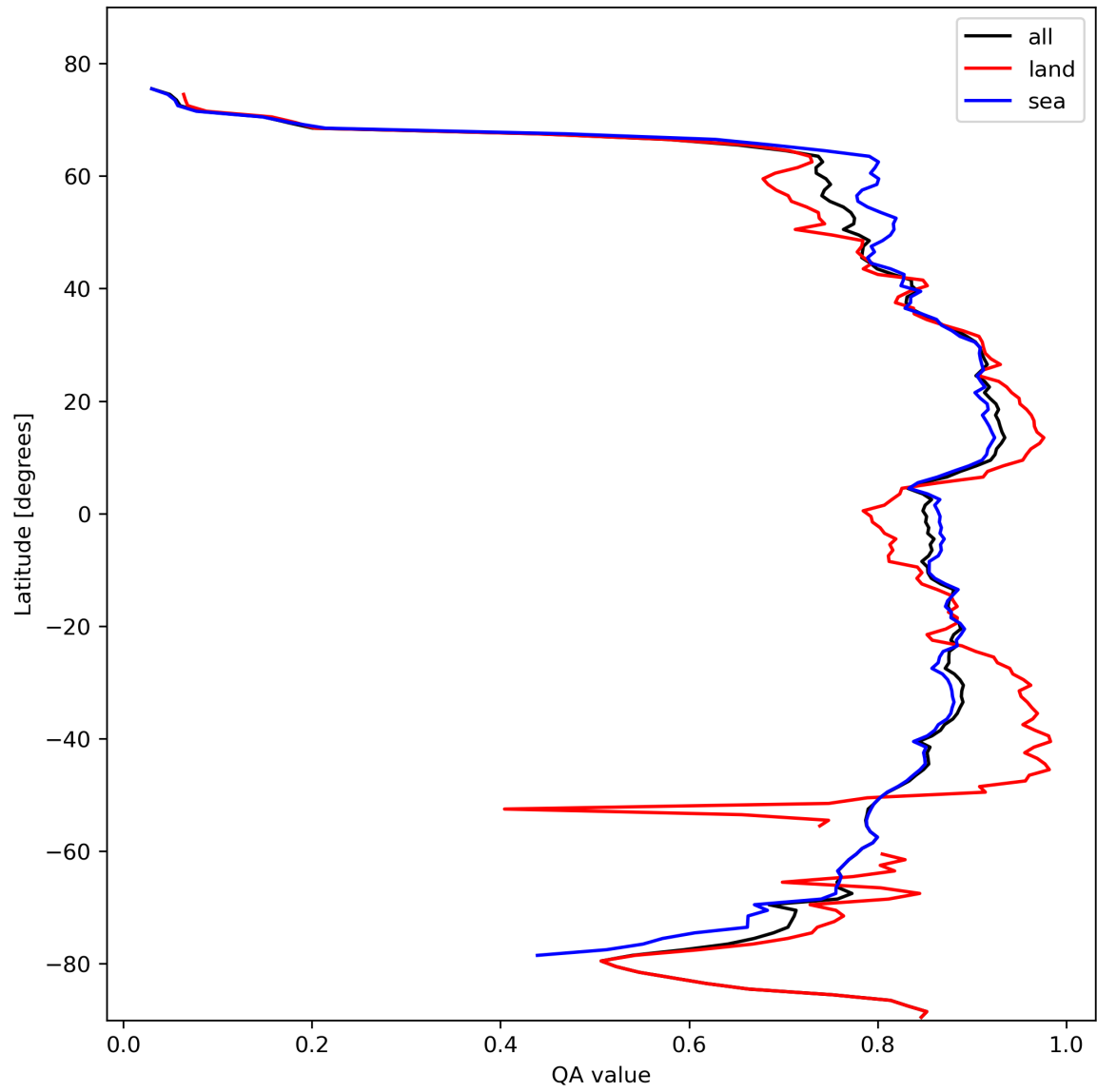
Figure 11: Zonal average of “QA value” for 2024-02-13 to 2024-02-15.
