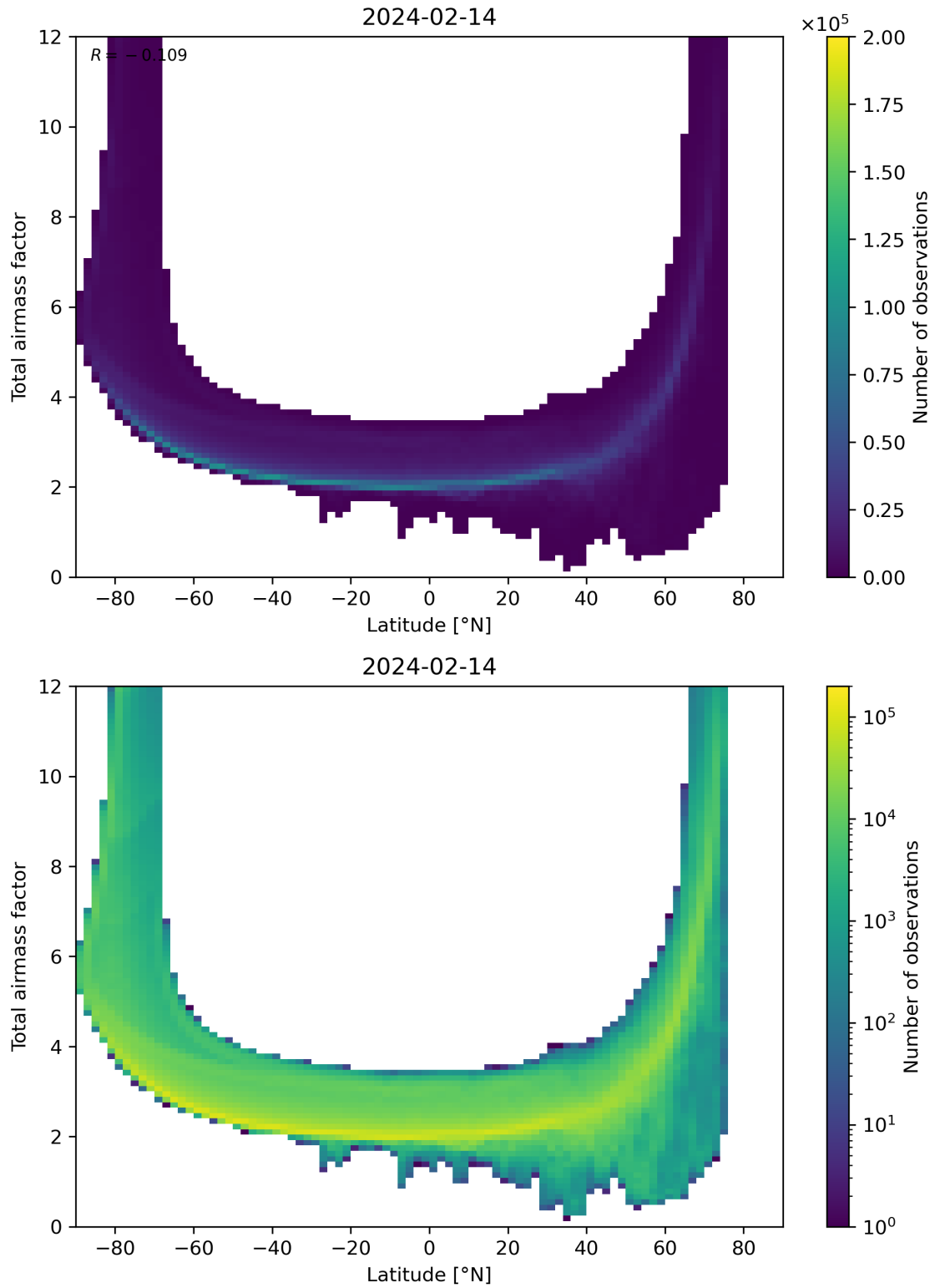
Figure 84: Scatter density plot of “Latitude” against “Total airmass factor” for 2024-02-13 to 2024-02-15.
