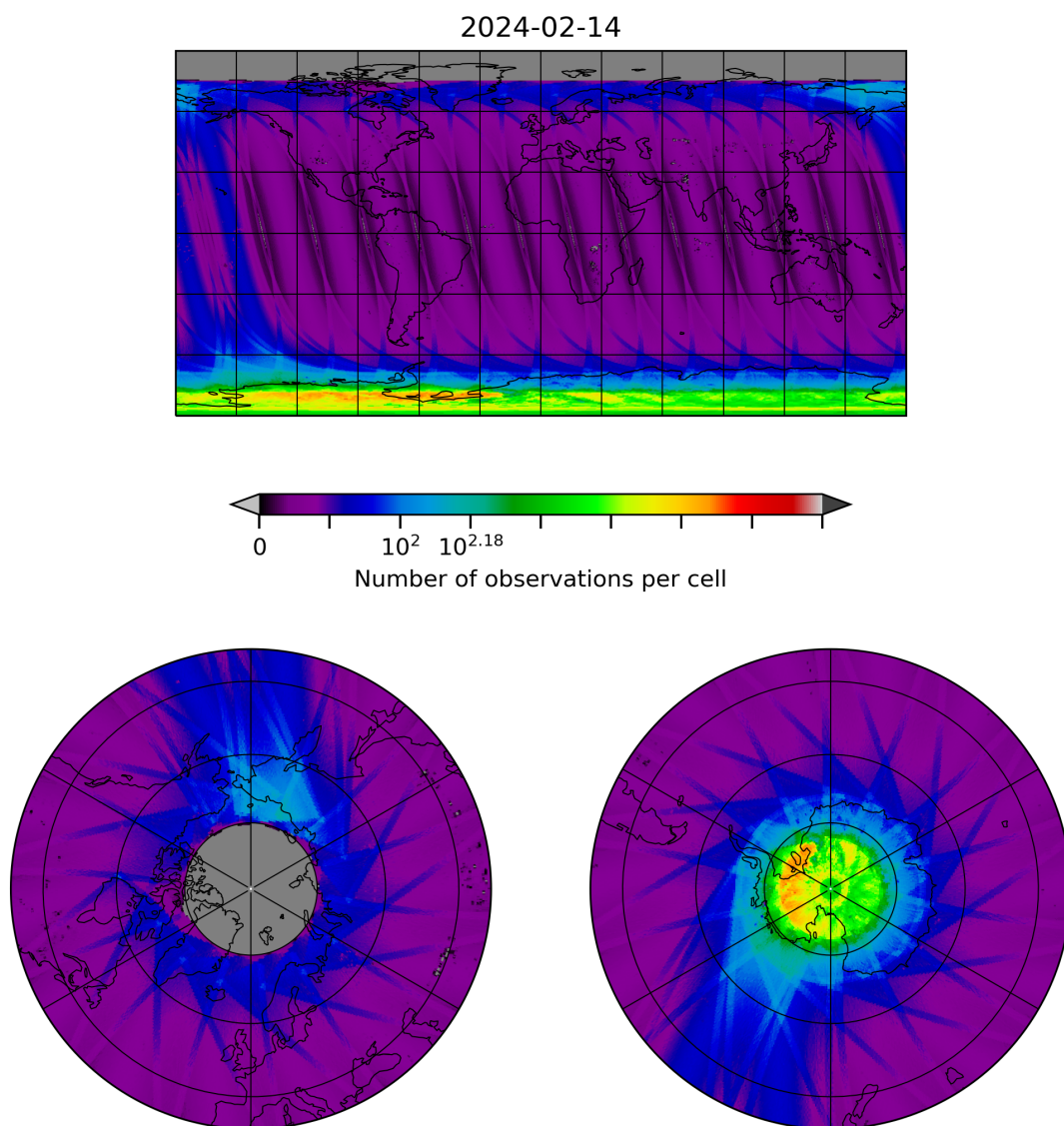
Figure 10: Map of the number of observations for 2024-02-13 to 2024-02-15
