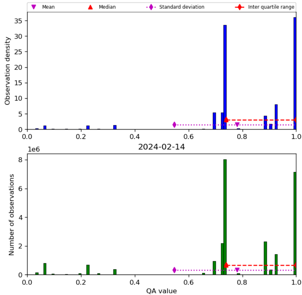
Figure 28: Histogram of “QA value” for 2024-02-13 to 2024-02-15
