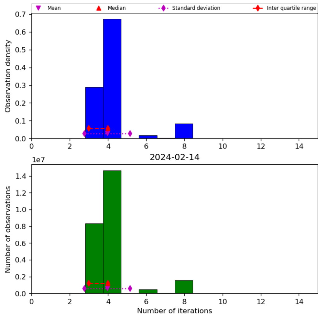
Figure 34: Histogram of “Number of iterations” for 2024-02-13 to 2024-02-15
