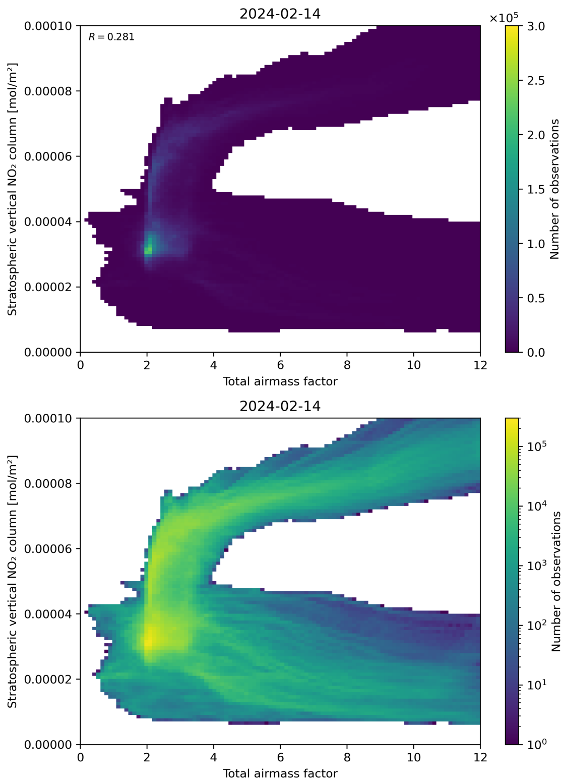
Figure 64: Scatter density plot of “Total airmass factor” against “Stratospheric vertical NO 2 column” for 2024-02-13 to 2024-02-15.
