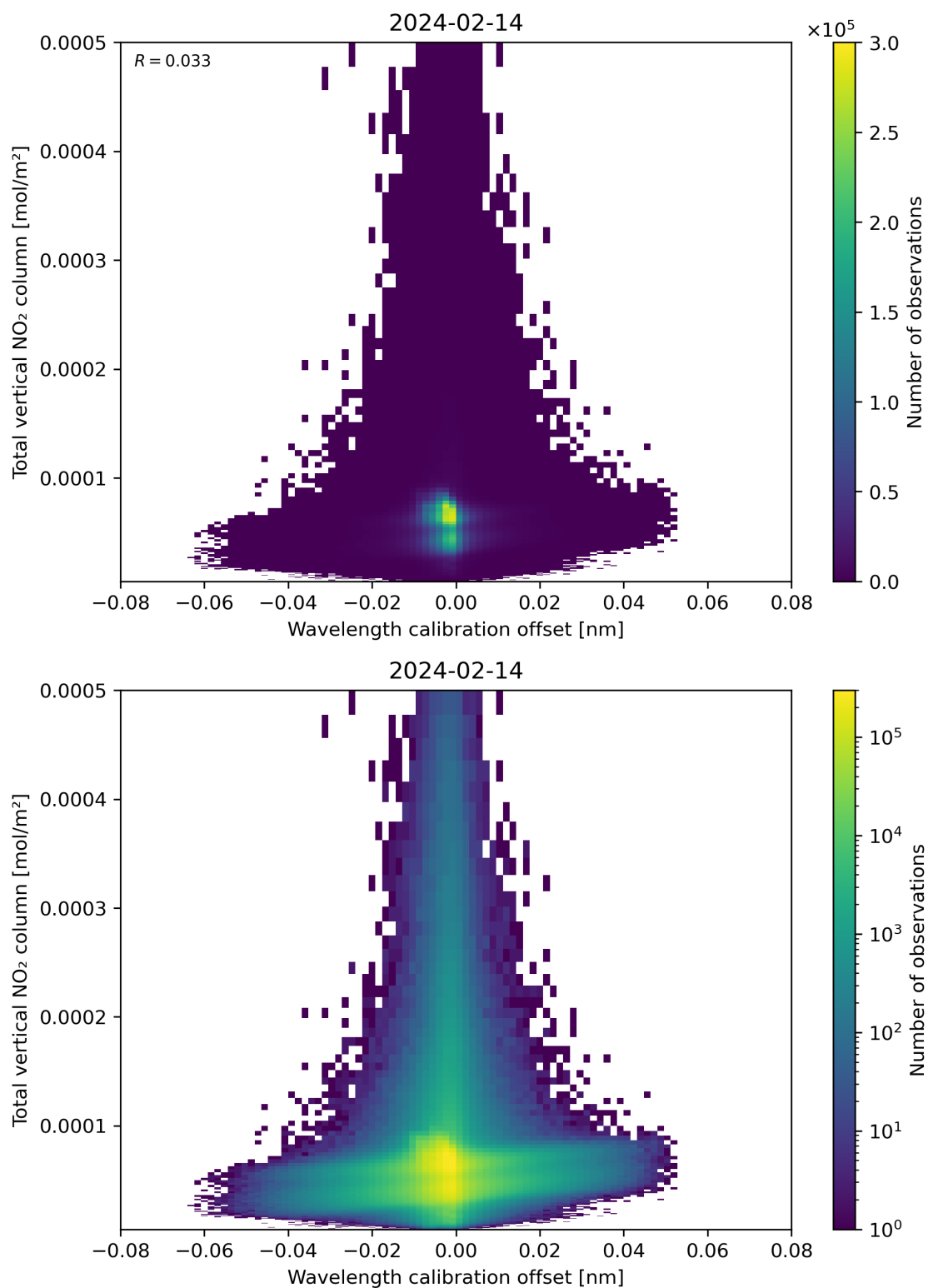
Figure 179: Scatter density plot of “Wavelength calibration offset” against “Total vertical NO 2 column” for 2024-02-13 to 2024-02-15.
