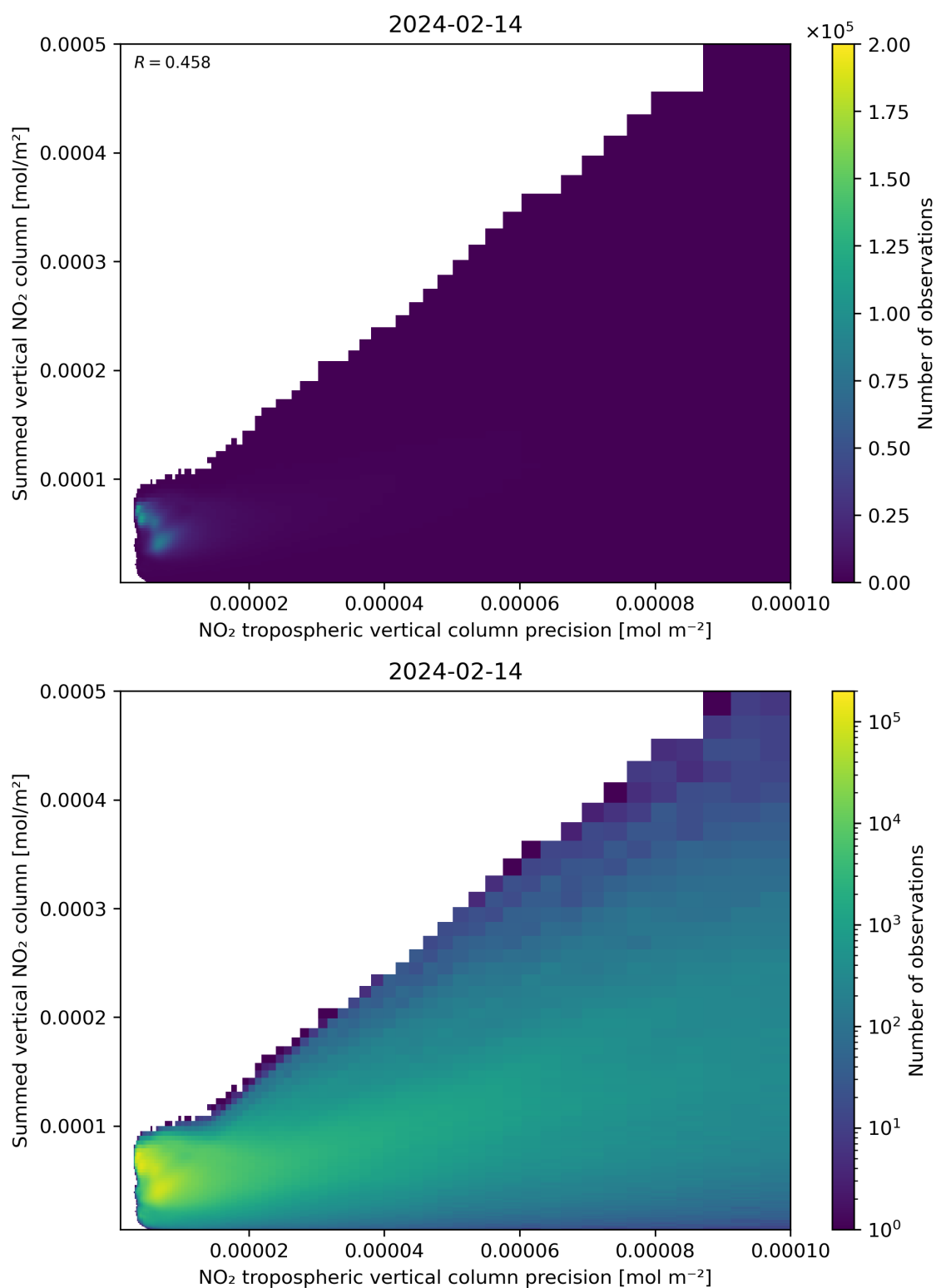
Figure 136: Scatter density plot of “NO 2 tropospheric vertical column precision” against “Summed vertical NO 2 column” for 2024-02-13 to 2024-02-15.
