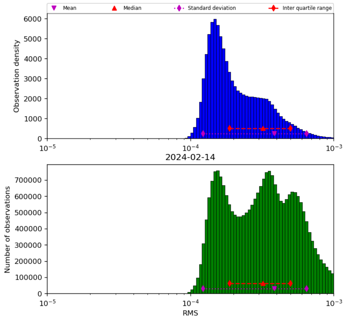
Figure 43: Histogram of “RMS” for 2024-02-13 to 2024-02-15
