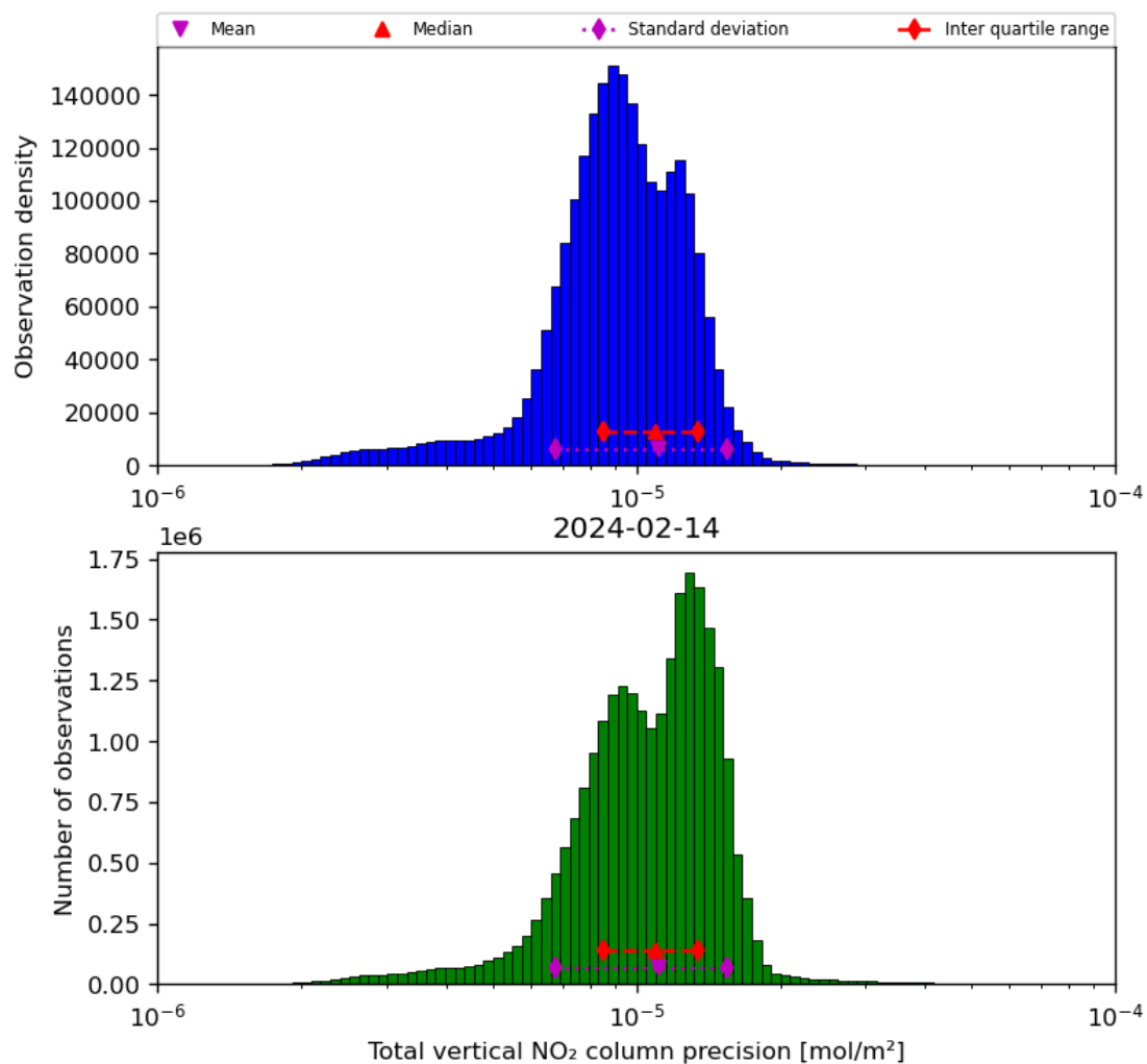
Figure 39: Histogram of “Total vertical NO 2 column precision” for 2024-02-13 to 2024-02-15
