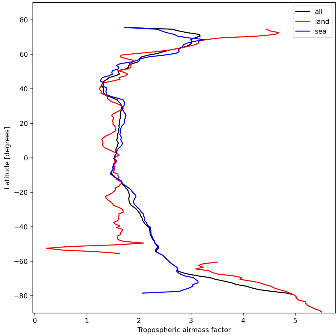
Figure 14: Zonal average of “Tropospheric airmass factor” for 2024-02-13 to 2024-02-15.
