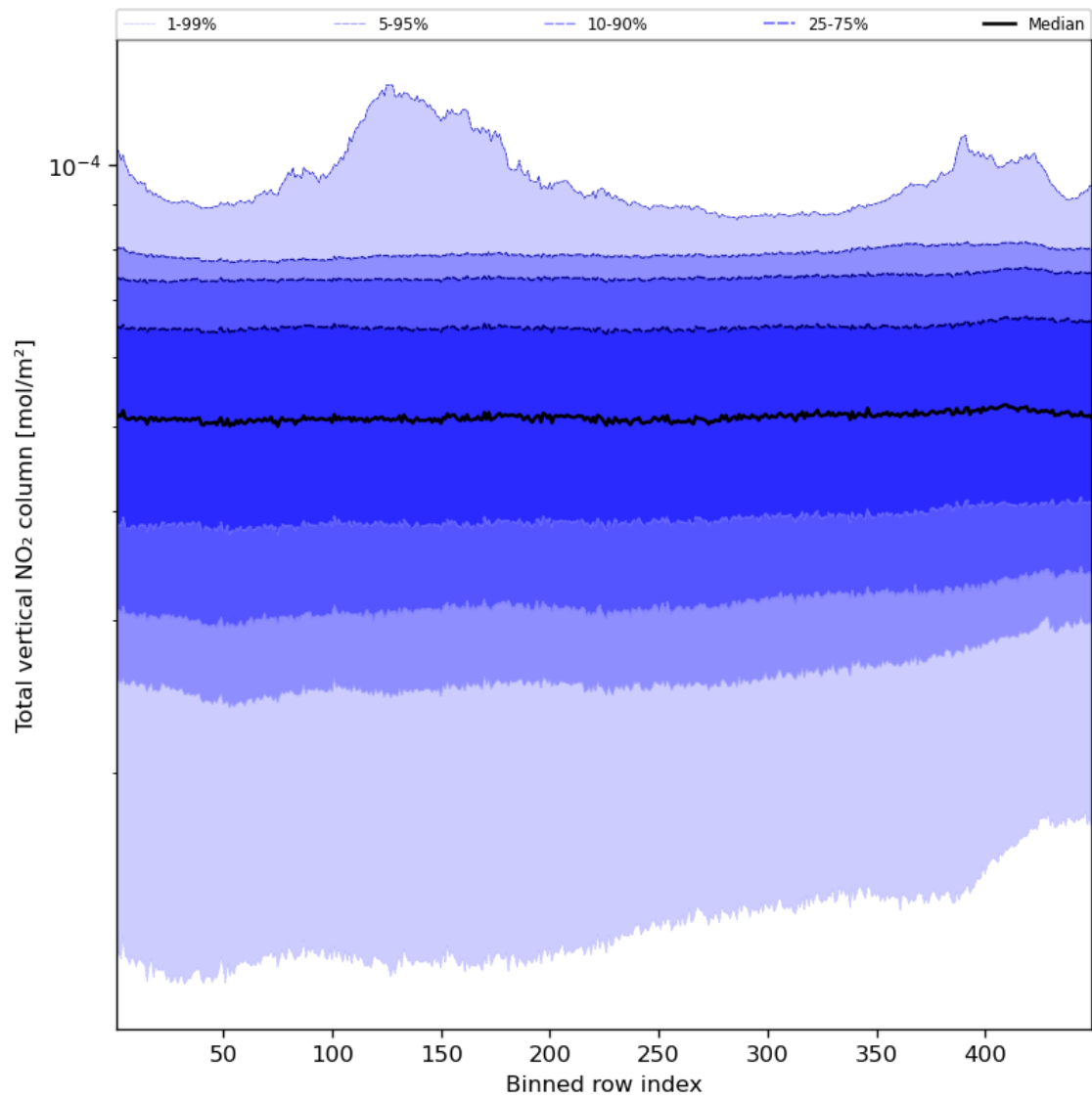
Figure 55: Along track statistics of “Total vertical NO 2 column” for 2024-02-13 to 2024-02-15
