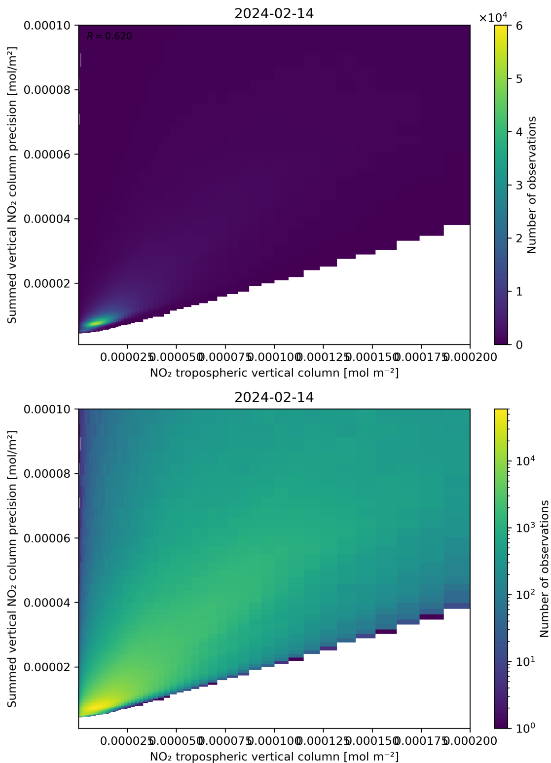
Figure 127: Scatter density plot of “NO 2 tropospheric vertical column” against “Summed vertical NO 2 column precision” for 2024-02-13 to 2024-02-15.
