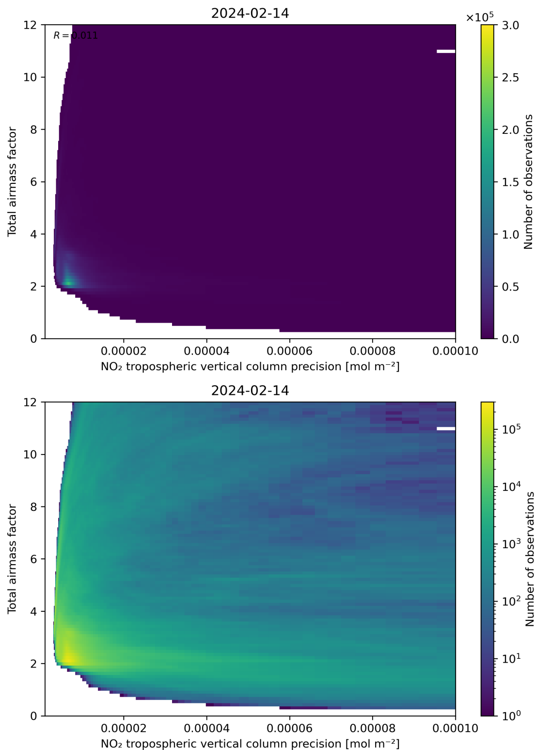
Figure 132: Scatter density plot of “NO 2 tropospheric vertical column precision” against “Total airmass factor” for 2024-02-13 to 2024-02-15.
