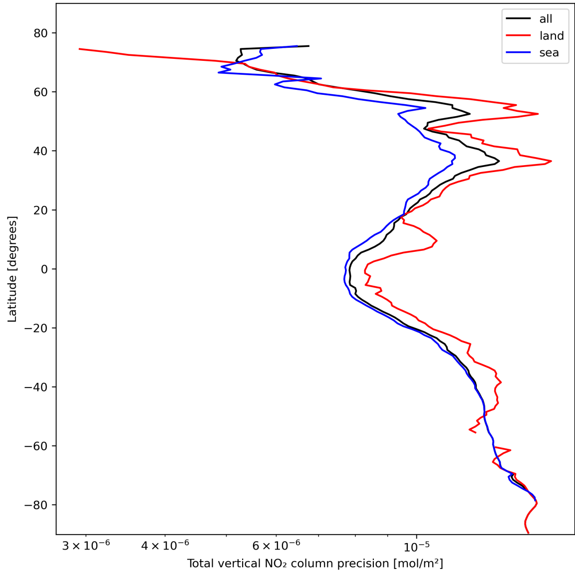
Figure 22: Zonal average of “Total vertical NO 2 column precision” for 2024-02-13 to 2024-02-15.
