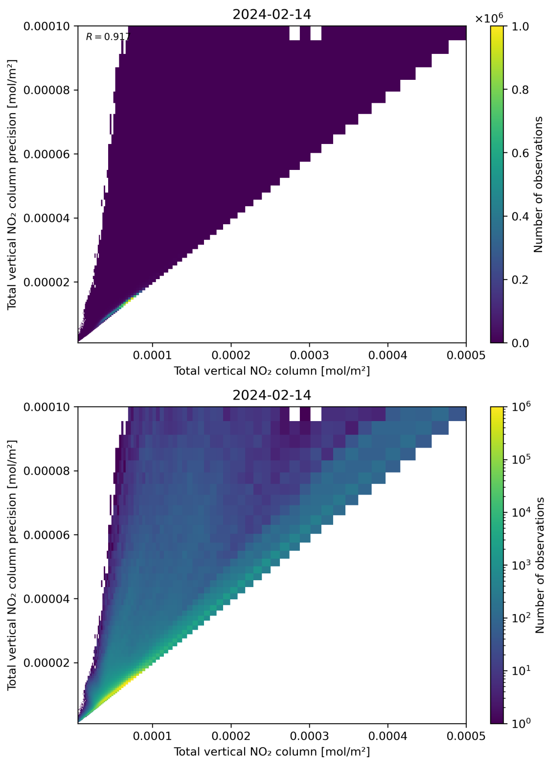
Figure 114: Scatter density plot of “Total vertical NO 2 column” against “Total vertical NO 2 column precision” for 2024-02-13 to 2024-02-15.
