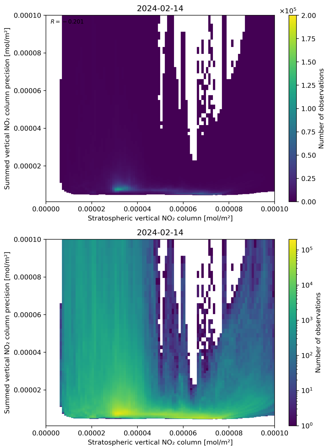
Figure 99: Scatter density plot of “Stratospheric vertical NO 2 column” against “Summed vertical NO 2 column precision” for 2024-02-13 to 2024-02-15.
