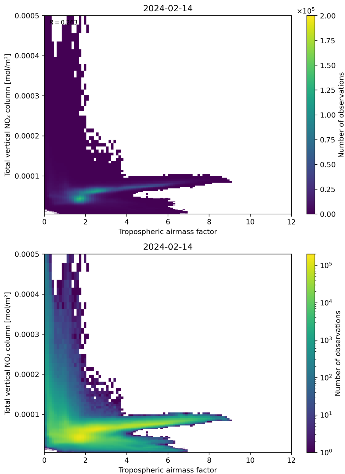
Figure 77: Scatter density plot of “Tropospheric airmass factor” against “Total vertical NO 2 column” for 2024-02-13 to 2024-02-15.
