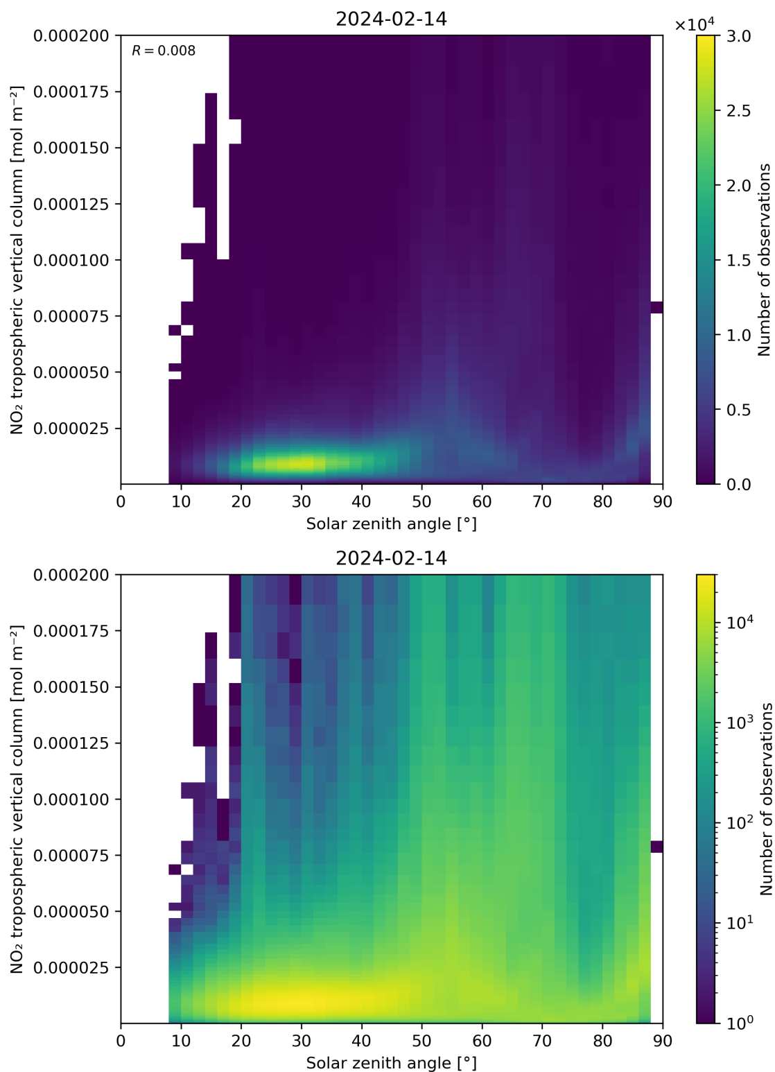
Figure 155: Scatter density plot of “Solar zenith angle” against “NO 2 tropospheric vertical column” for 2024-02-13 to 2024-02-15.
