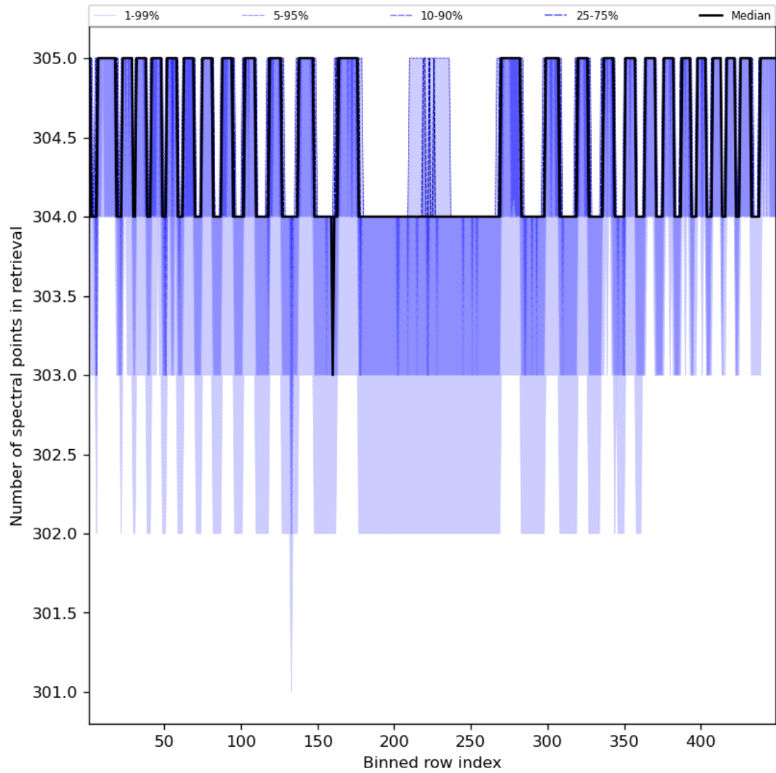
Figure 50: Along track statistics of “Number of spectral points in retrieval” for 2024-02-13 to 2024-02-15
