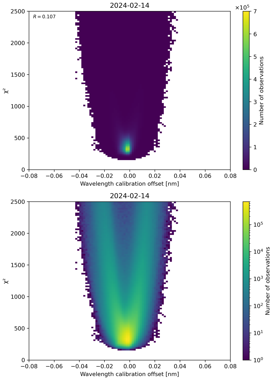
Figure 175: Scatter density plot of “Wavelength calibration offset” against “ \chi^2 ” for 2024-02-13 to 2024-02-15.
