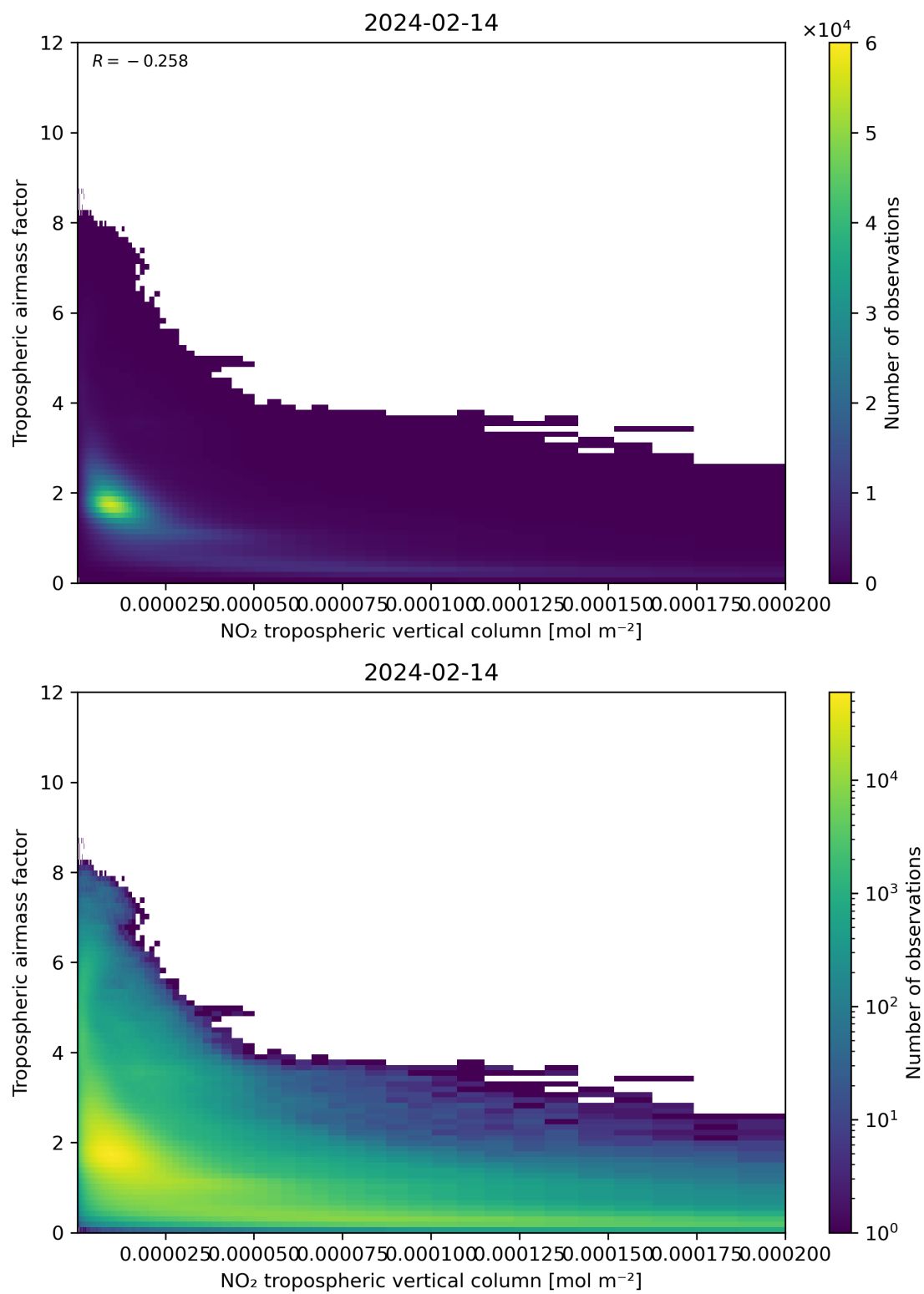
Figure 123: Scatter density plot of “NO 2 tropospheric vertical column” against “Tropospheric air mass factor” for 2024-02-13 to 2024-02-15.
