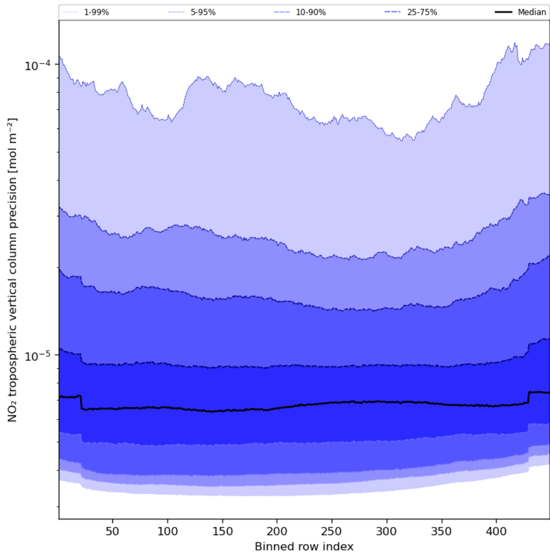
Figure 47: Along track statistics of “NO 2 tropospheric vertical column precision” for 2024-02-13 to 2024-02-15
