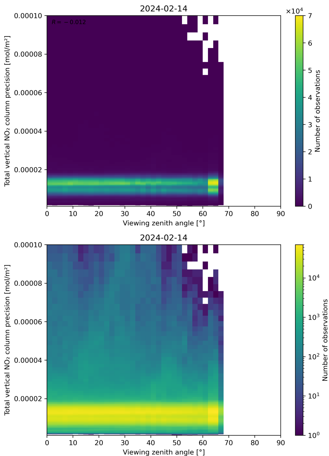
Figure 168: Scatter density plot of “Viewing zenith angle” against “Total vertical NO 2 column precision” for 2024-02-13 to 2024-02-15.
