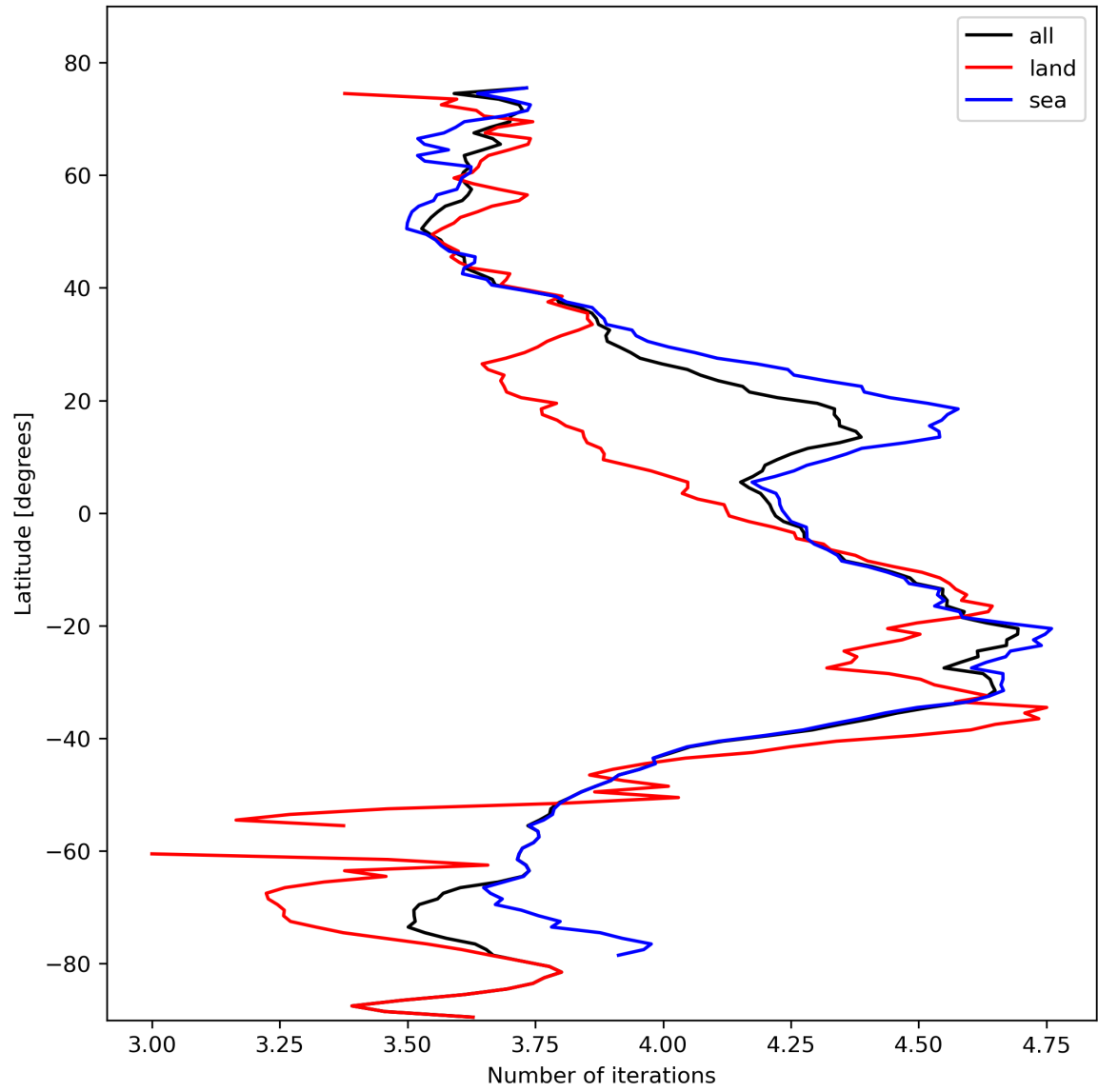
Figure 17: Zonal average of “Number of iterations” for 2024-02-13 to 2024-02-15.
