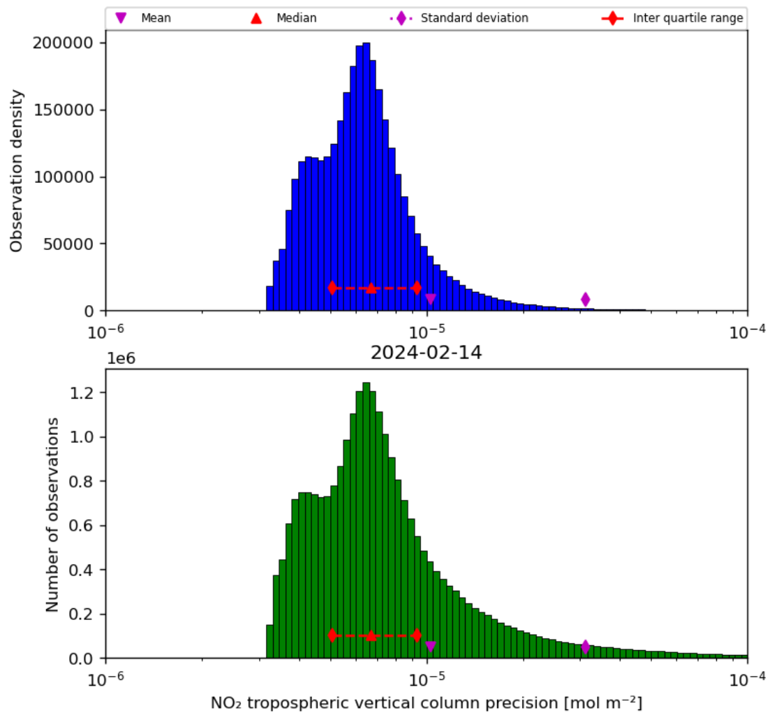
Figure 30: Histogram of “NO 2 tropospheric vertical column precision” for 2024-02-13 to 2024-02-15
