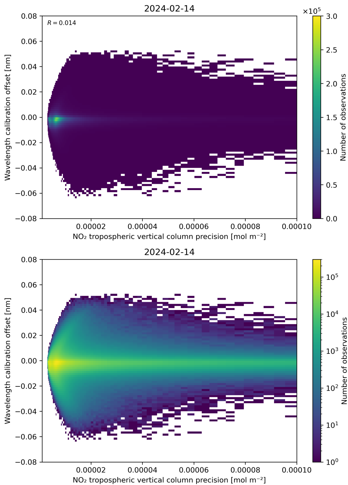
Figure 141: Scatter density plot of “NO 2 tropospheric vertical column precision” against “Wavelength calibration offset” for 2024-02-13 to 2024-02-15.
