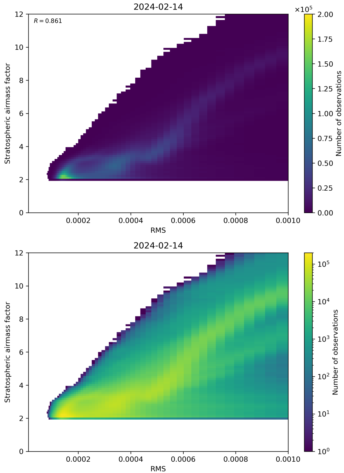
Figure 144: Scatter density plot of “RMS” against “Stratospheric airmass factor” for 2024-02-13 to 2024-02-15.
