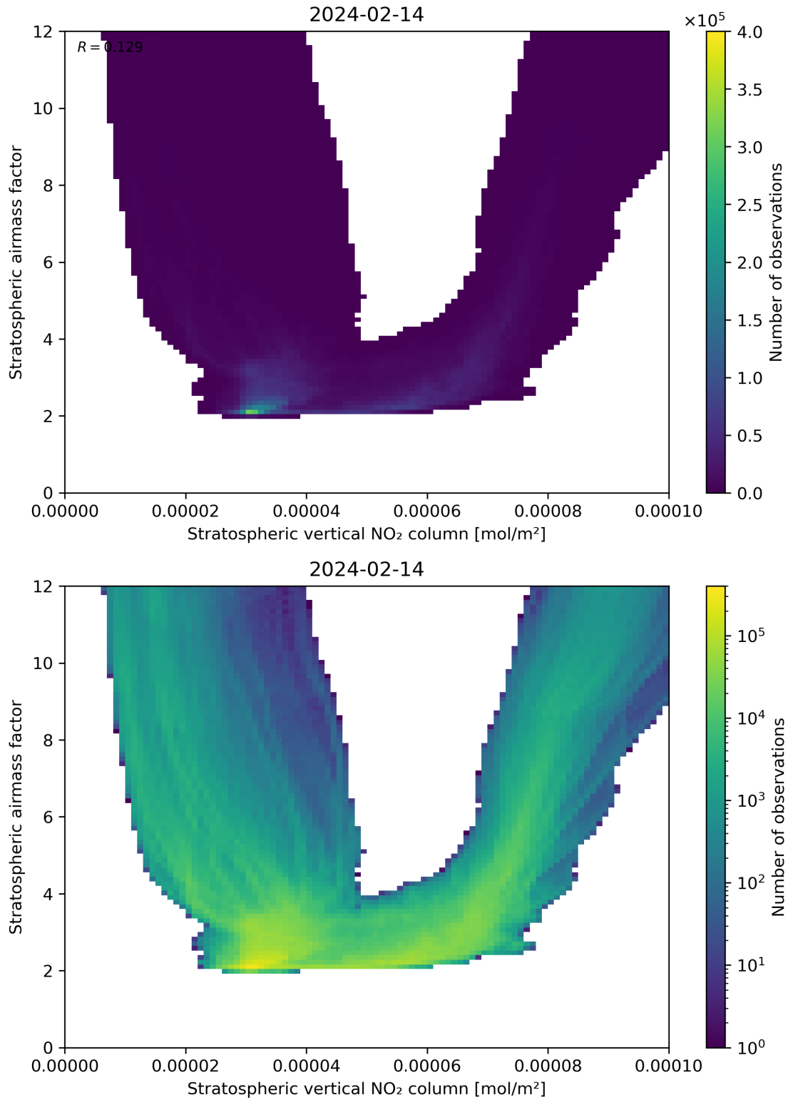
Figure 96: Scatter density plot of “Stratospheric vertical NO 2 column” against “Stratospheric airmass factor” for 2024-02-13 to 2024-02-15.
