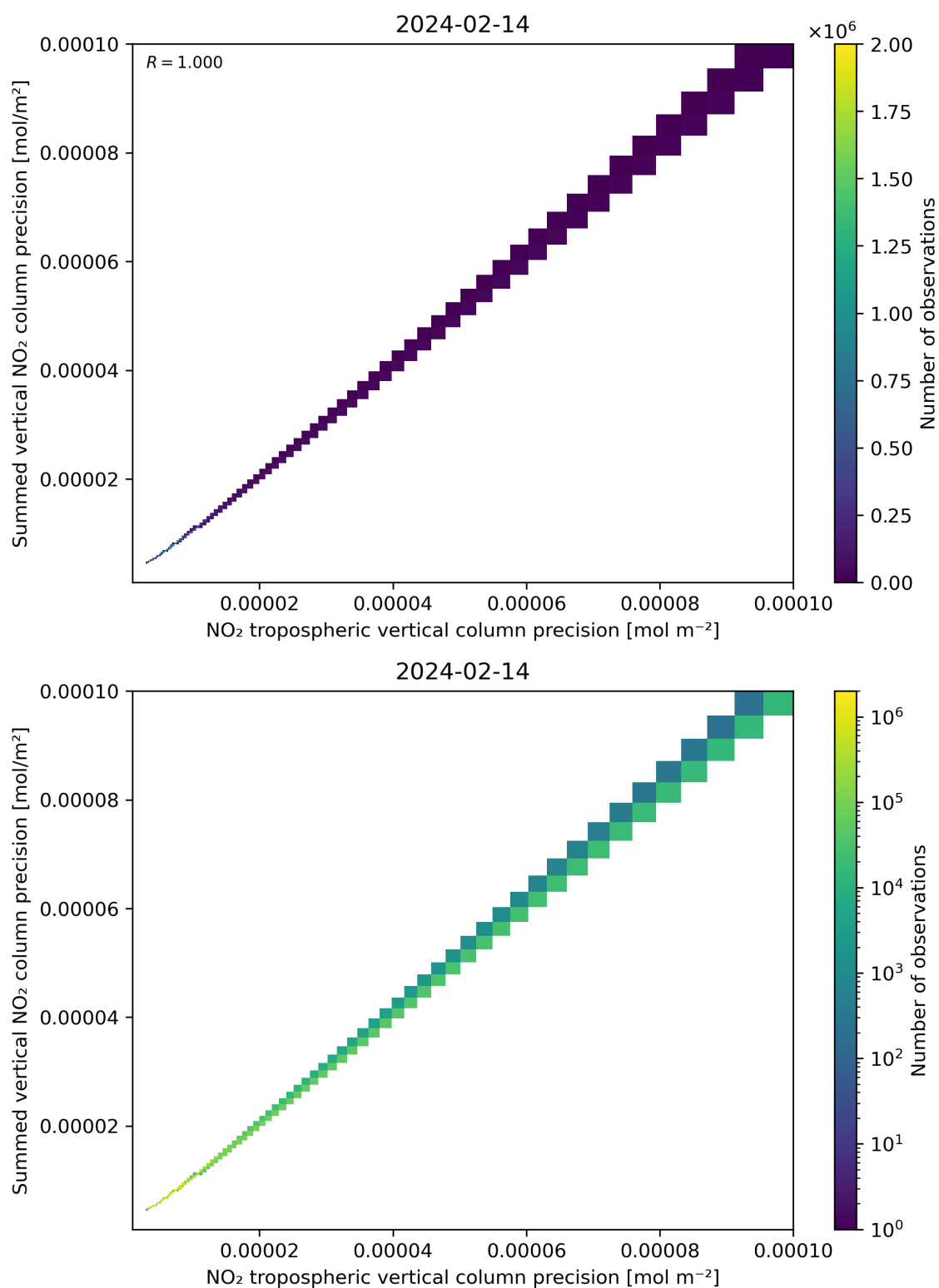
Figure 137: Scatter density plot of “NO 2 tropospheric vertical column precision” against “Summed vertical NO 2 column precision” for 2024-02-13 to 2024-02-15.
