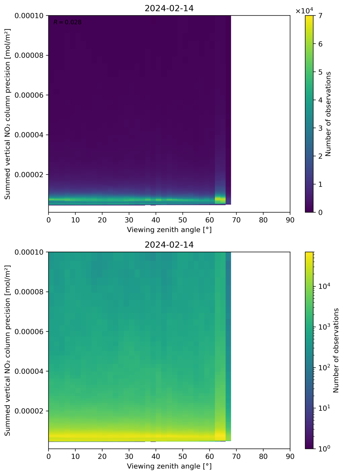
Figure 166: Scatter density plot of “Viewing zenith angle” against “Summed vertical NO 2 column precision” for 2024-02-13 to 2024-02-15.
