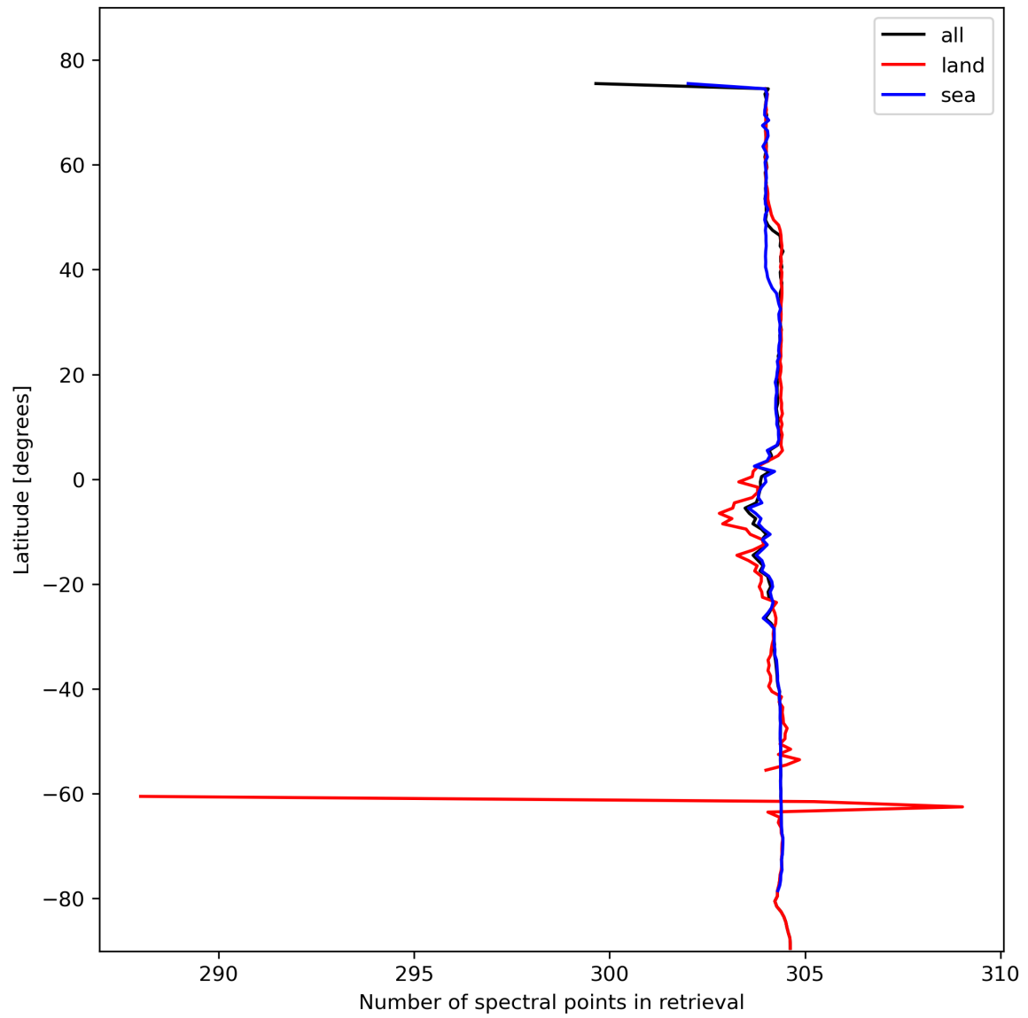
Figure 16: Zonal average of “Number of spectral points in retrieval” for 2024-02-13 to 2024-02-15.
