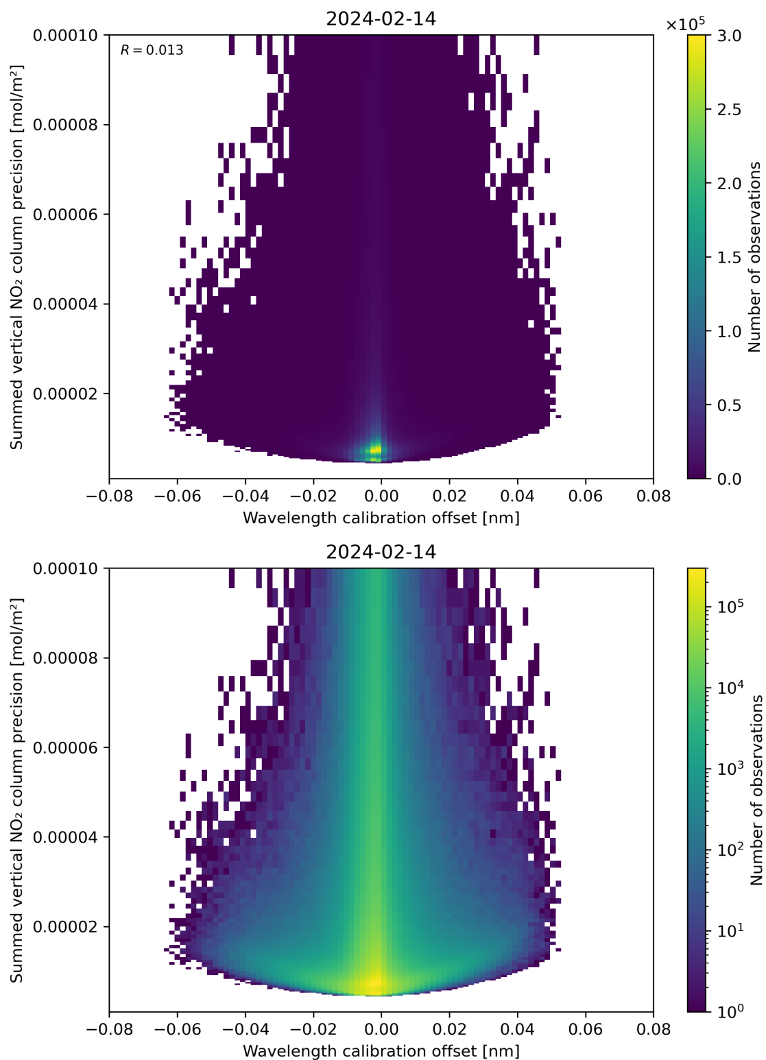
Figure 178: Scatter density plot of “Wavelength calibration offset” against “Summed vertical NO 2 column precision” for 2024-02-13 to 2024-02-15.
