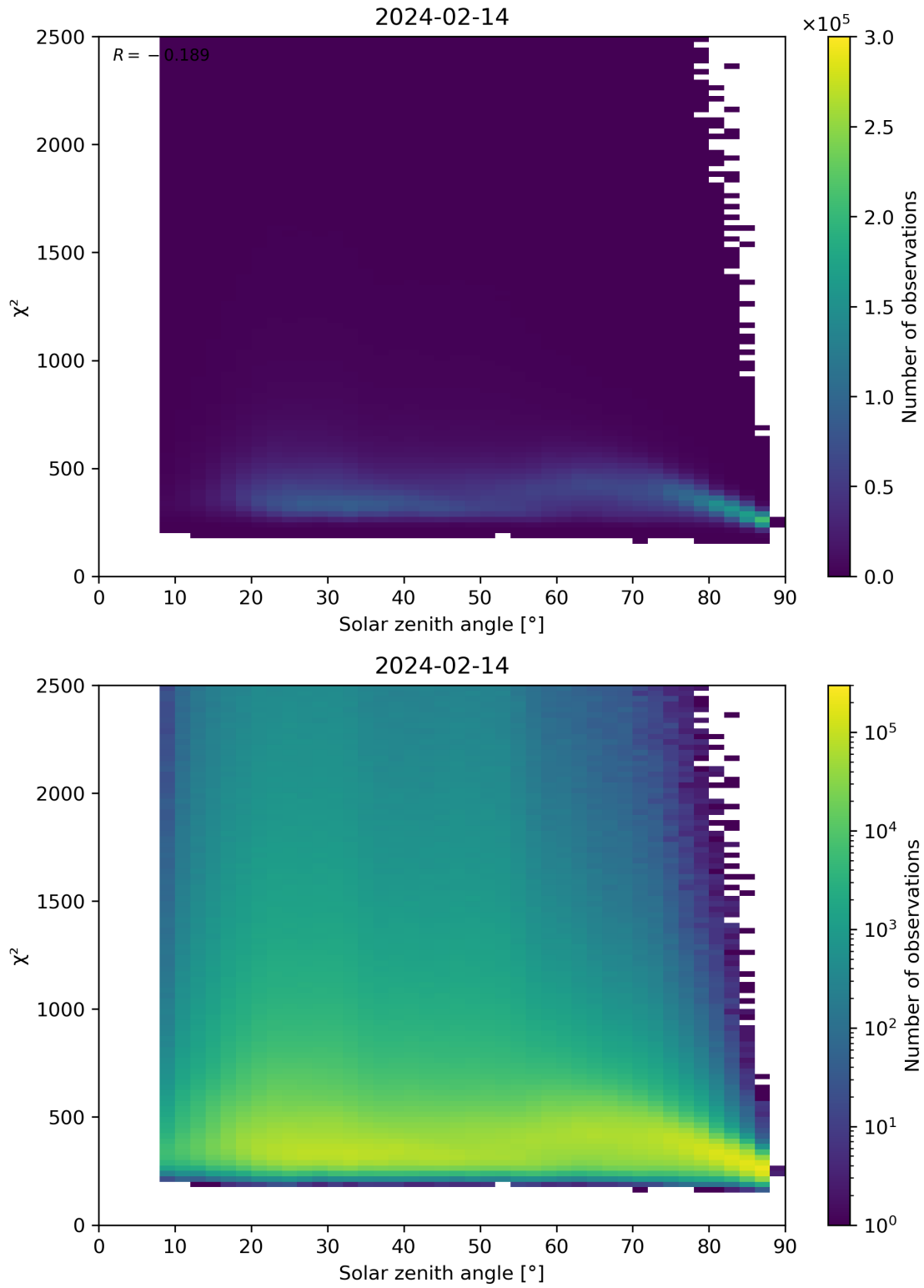
Figure 148: Scatter density plot of “Solar zenith angle” against “ \chi^2 ” for 2024-02-13 to 2024-02-15.
