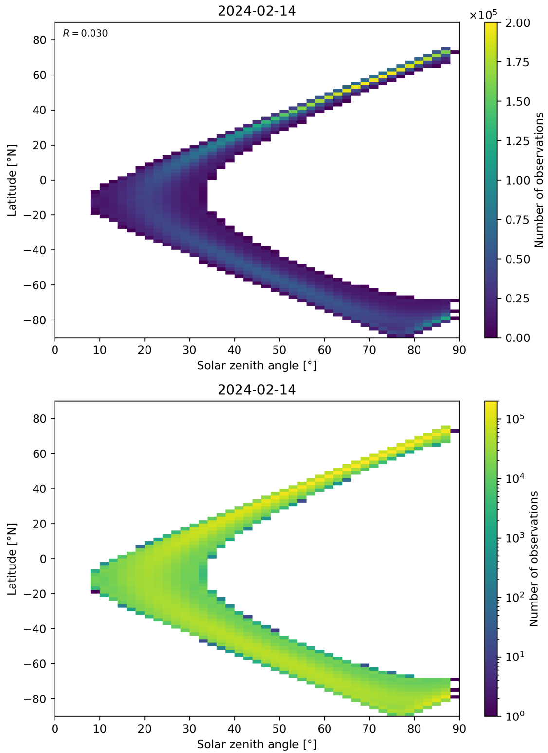
Figure 149: Scatter density plot of “Solar zenith angle” against “Latitude” for 2024-02-13 to 2024-02-15.
