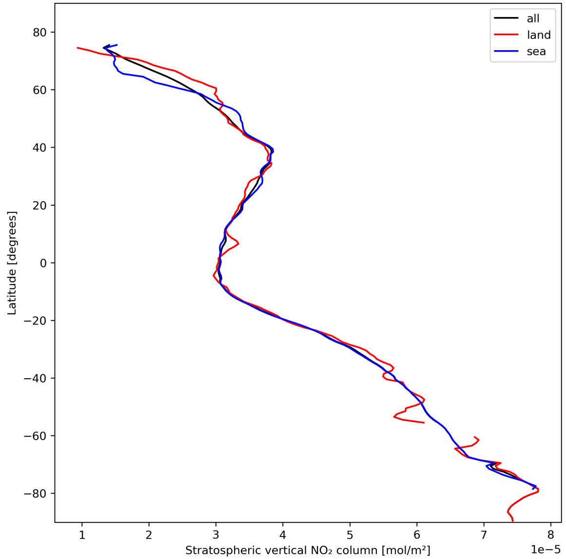
Figure 19: Zonal average of “Stratospheric vertical NO 2 column” for 2024-02-13 to 2024-02-15.
