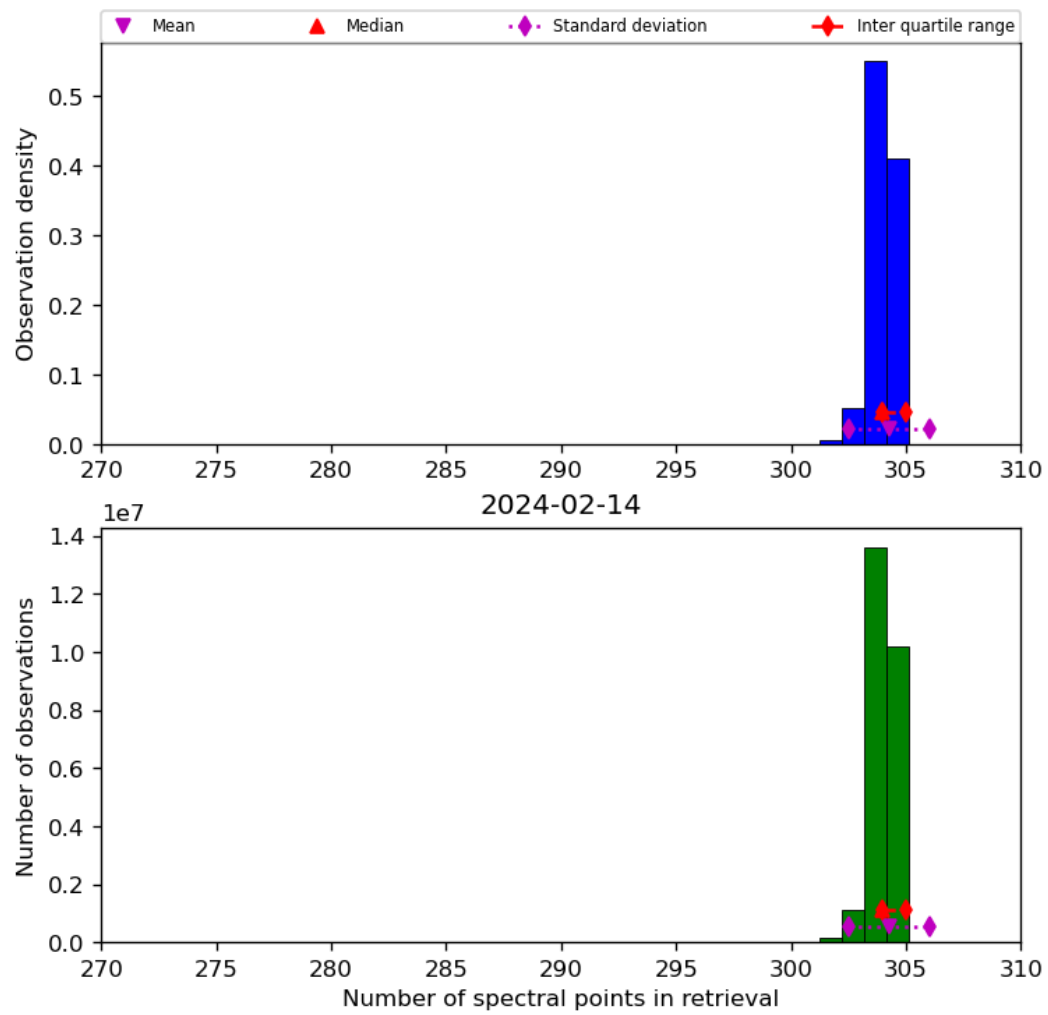
Figure 33: Histogram of “Number of spectral points in retrieval” for 2024-02-13 to 2024-02-15
