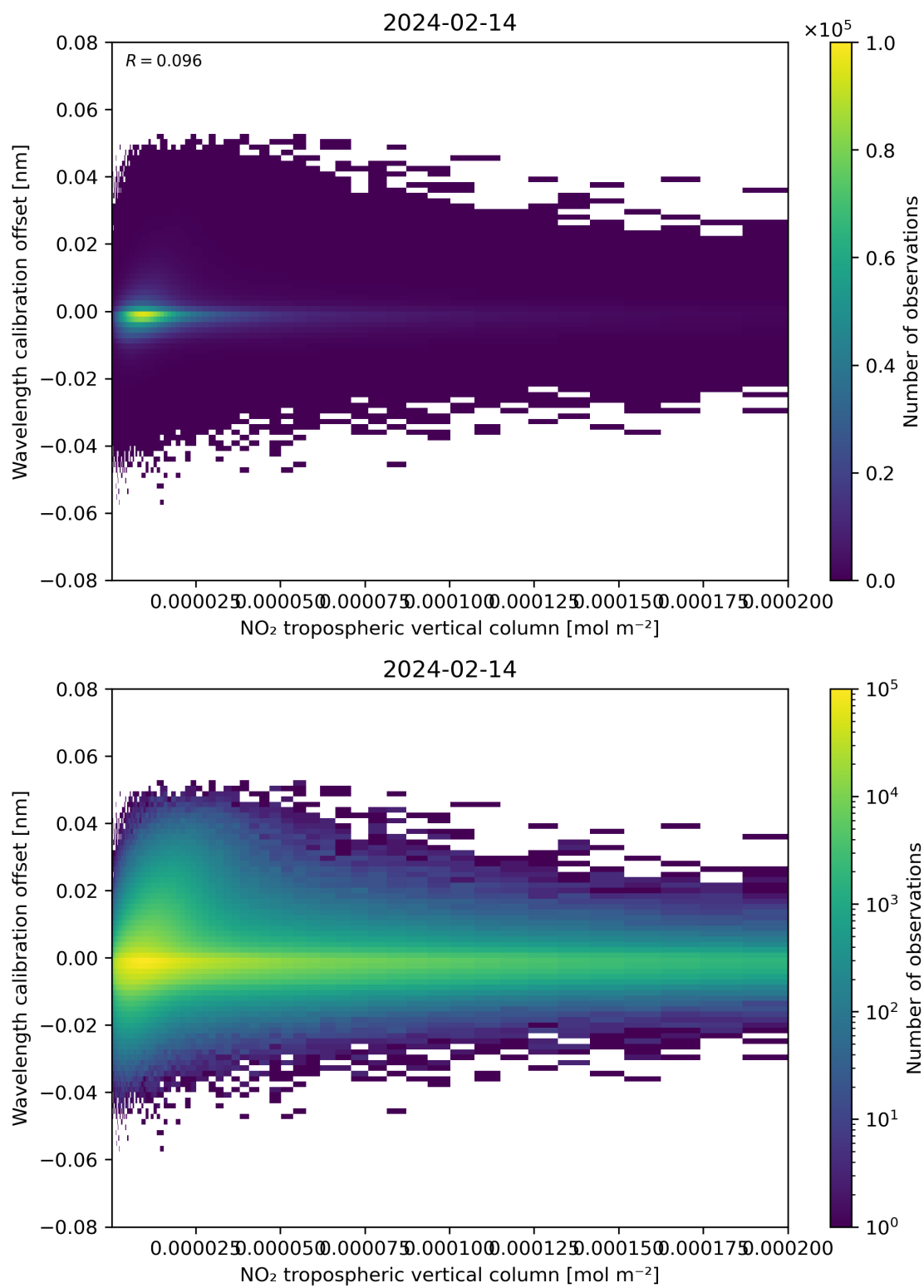
Figure 143: Scatter density plot of “NO 2 tropospheric vertical column” against “Wavelength calibration offset” for 2024-02-13 to 2024-02-15.
