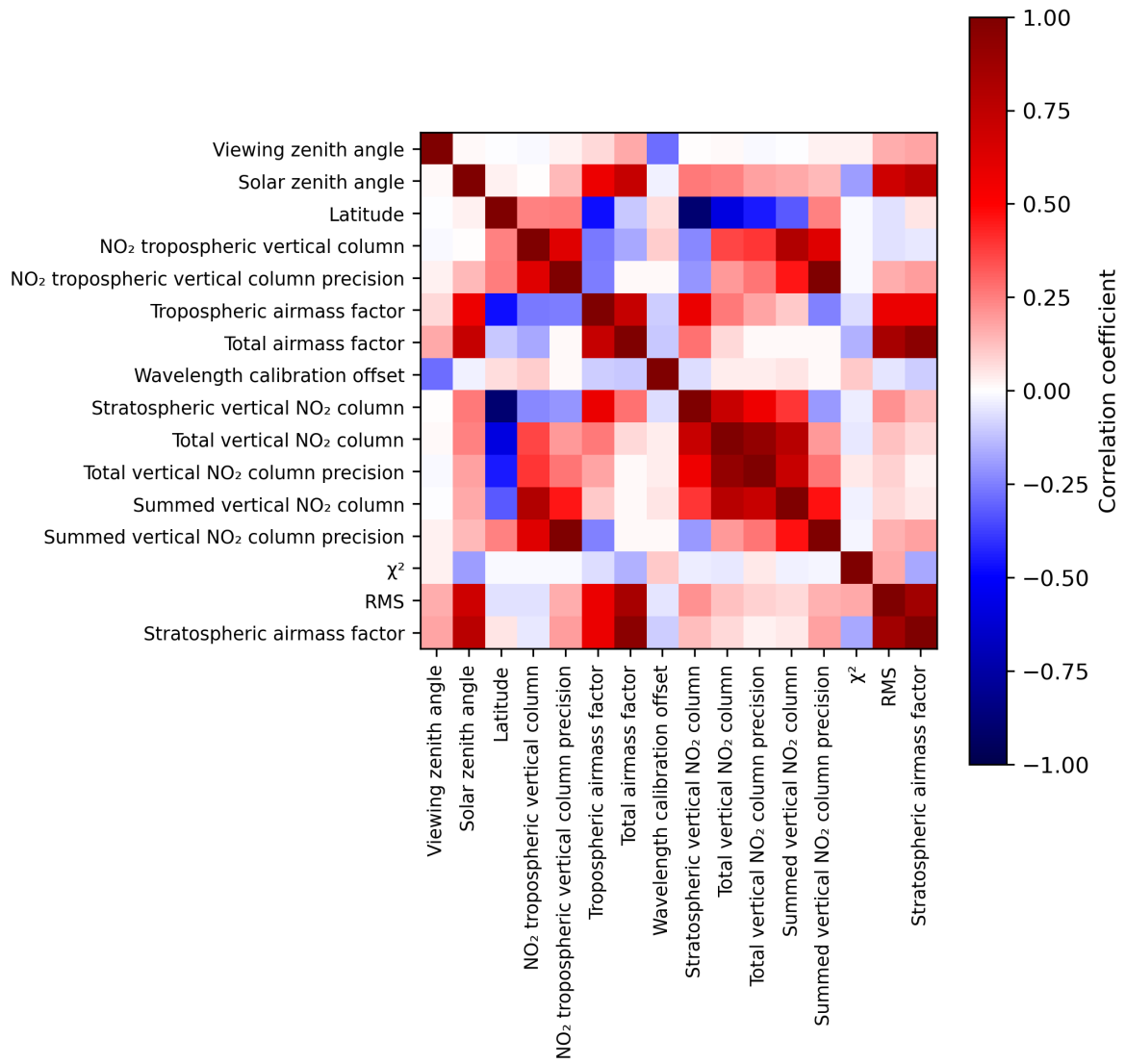
Figure 2: Map of correlation matrix for 2024-02-13 to 2024-02-15.
