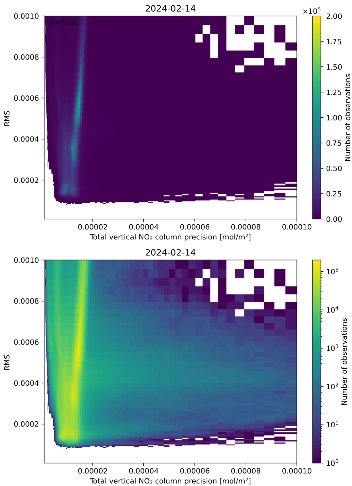
Figure 119: Scatter density plot of “Total vertical NO 2 column precision” against “RMS” for 2024-02-13 to 2024-02-15.
