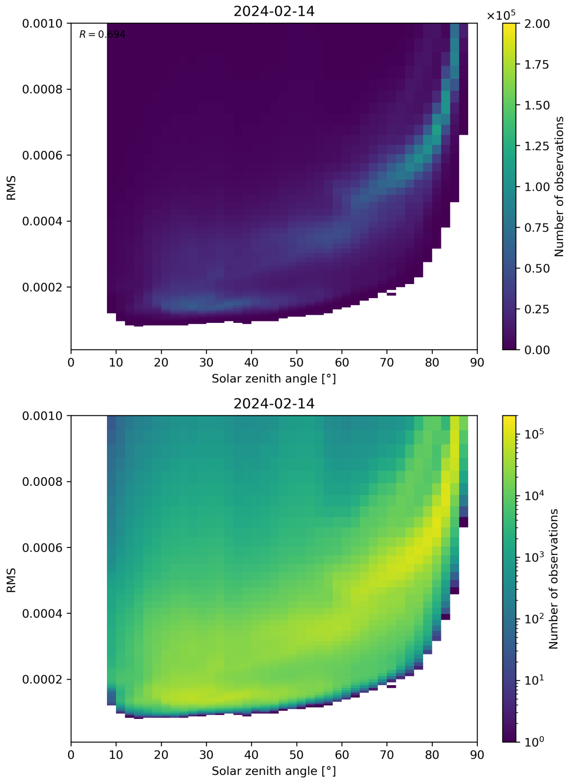
Figure 157: Scatter density plot of “Solar zenith angle” against “RMS” for 2024-02-13 to 2024-02-15.
