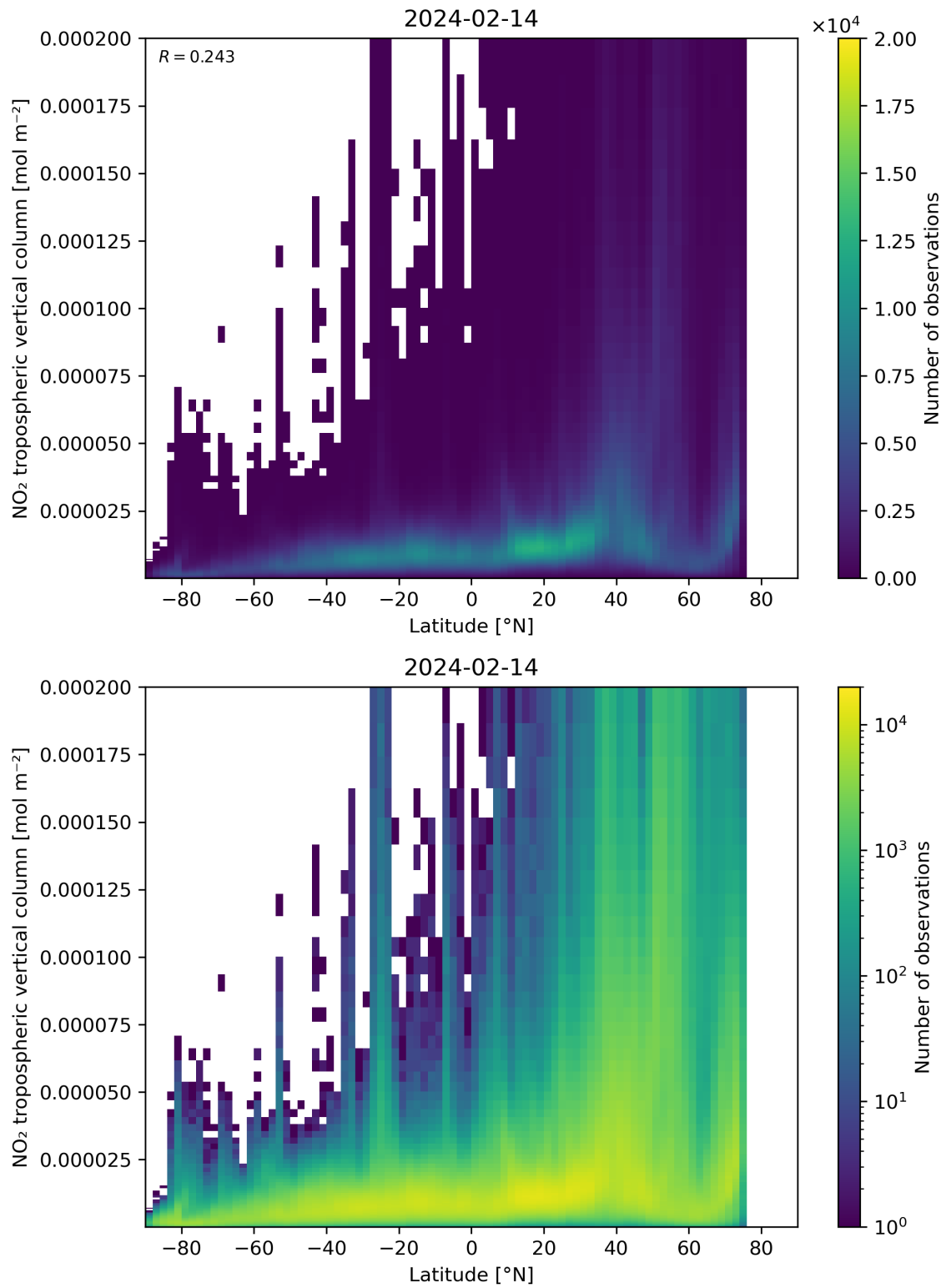
Figure 92: Scatter density plot of “Latitude” against “NO 2 tropospheric vertical column” for 2024-02-13 to 2024-02-15.
