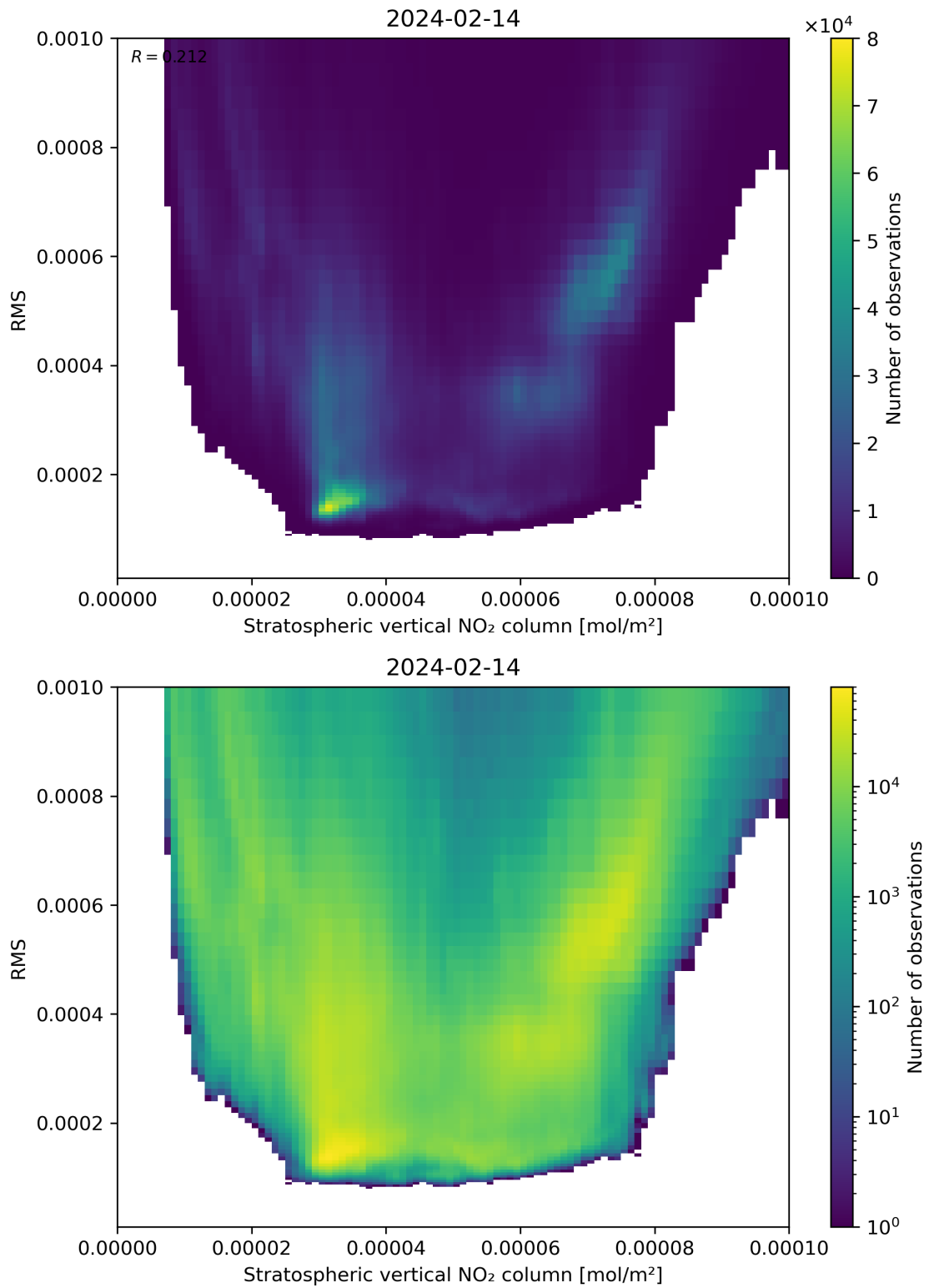
Figure 102: Scatter density plot of “Stratospheric vertical NO 2 column” against “RMS” for 2024-02-13 to 2024-02-15.
