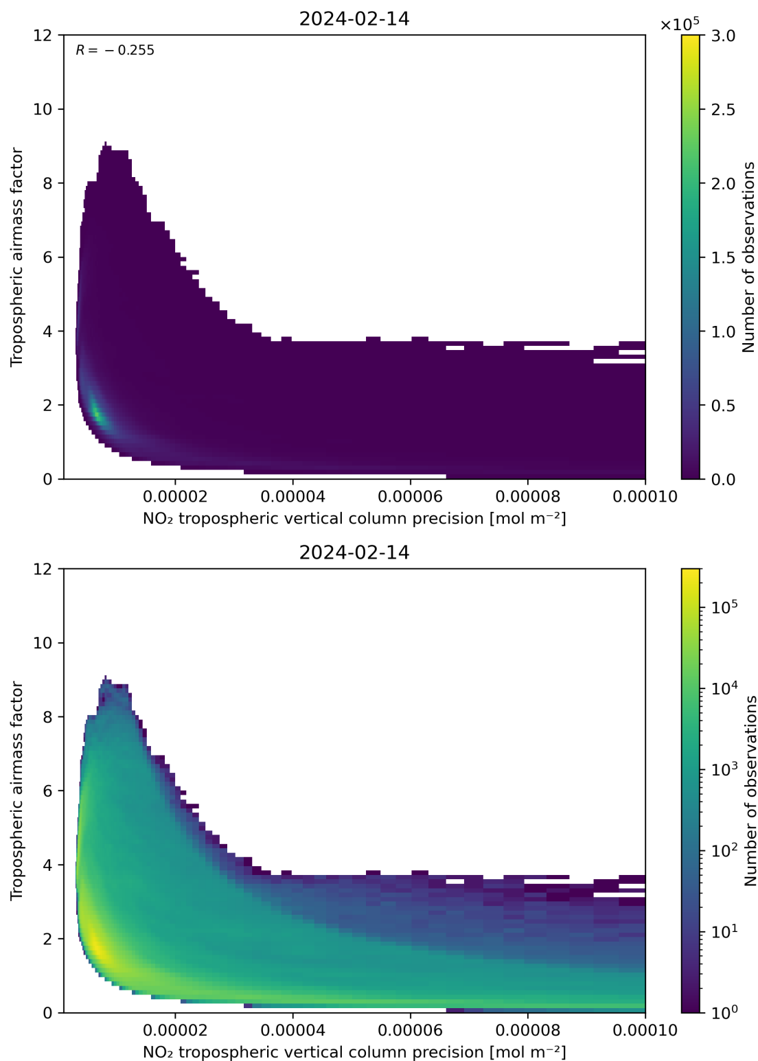
Figure 133: Scatter density plot of “NO 2 tropospheric vertical column precision” against “Tropospheric airmass factor” for 2024-02-13 to 2024-02-15.
