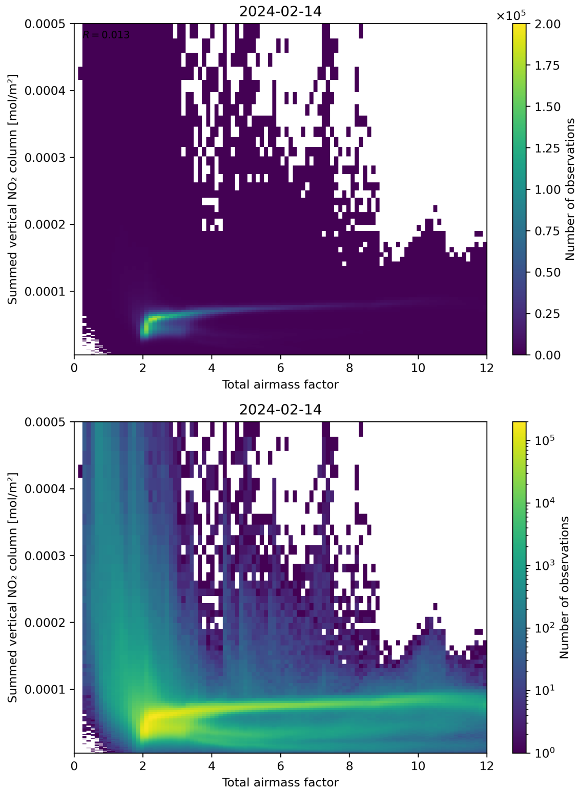
Figure 65: Scatter density plot of “Total airmass factor” against “Summed vertical NO 2 column” for 2024-02-13 to 2024-02-15.
