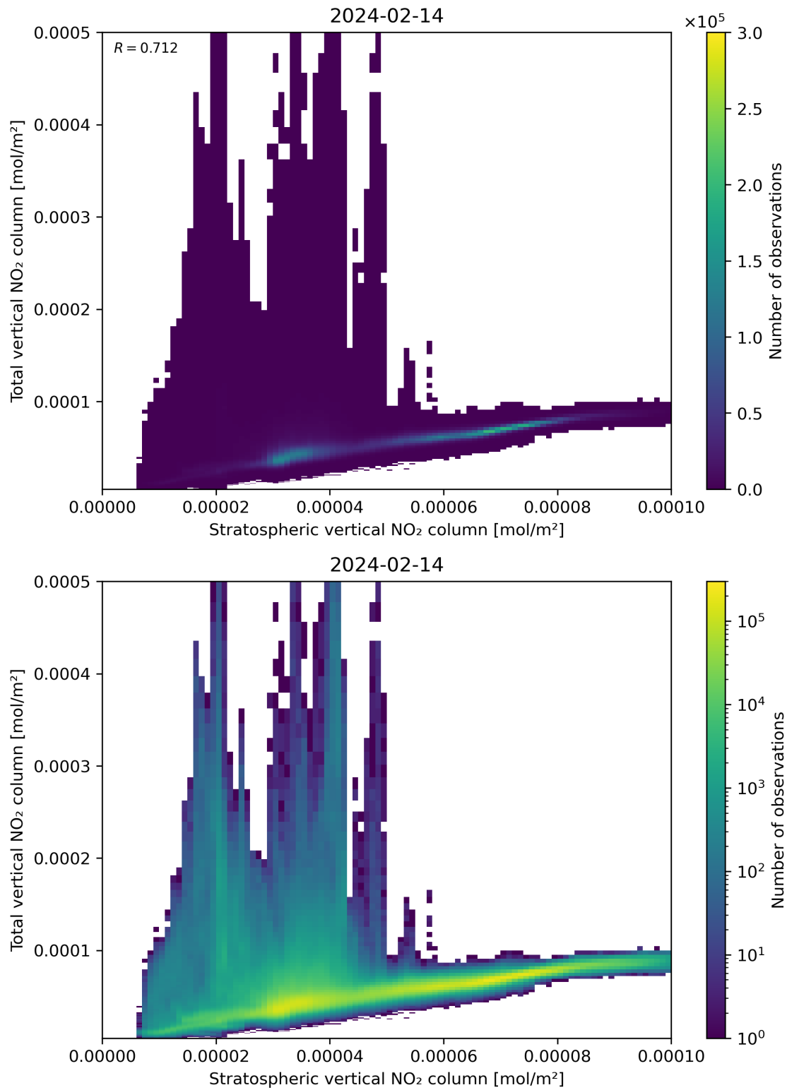
Figure 100: Scatter density plot of “Stratospheric vertical NO 2 column” against “Total vertical NO 2 column” for 2024-02-13 to 2024-02-15.
