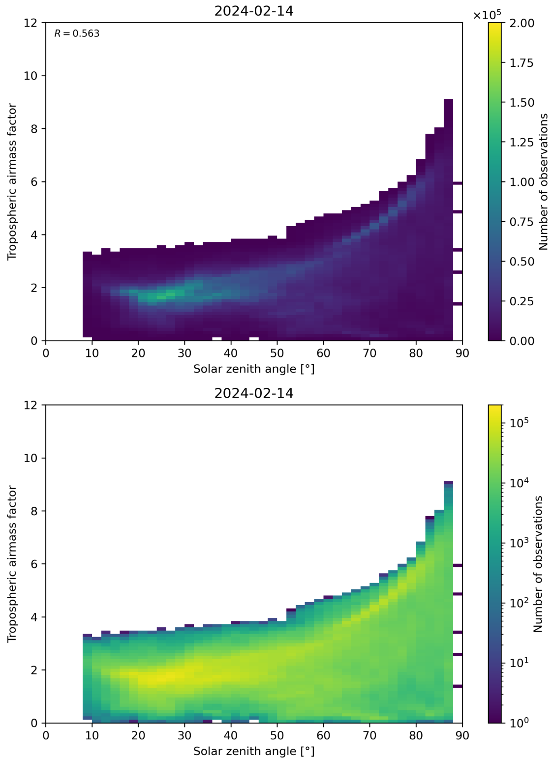
Figure 147: Scatter density plot of “Solar zenith angle” against “Tropospheric airmass factor” for 2024-02-13 to 2024-02-15.
