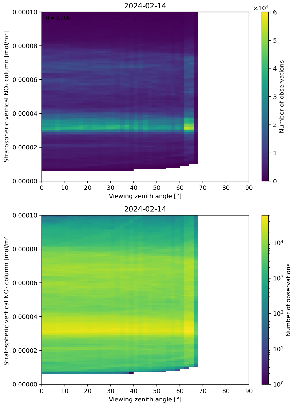
Figure 164: Scatter density plot of “Viewing zenith angle” against “Stratospheric vertical NO 2 column” for 2024-02-13 to 2024-02-15.
