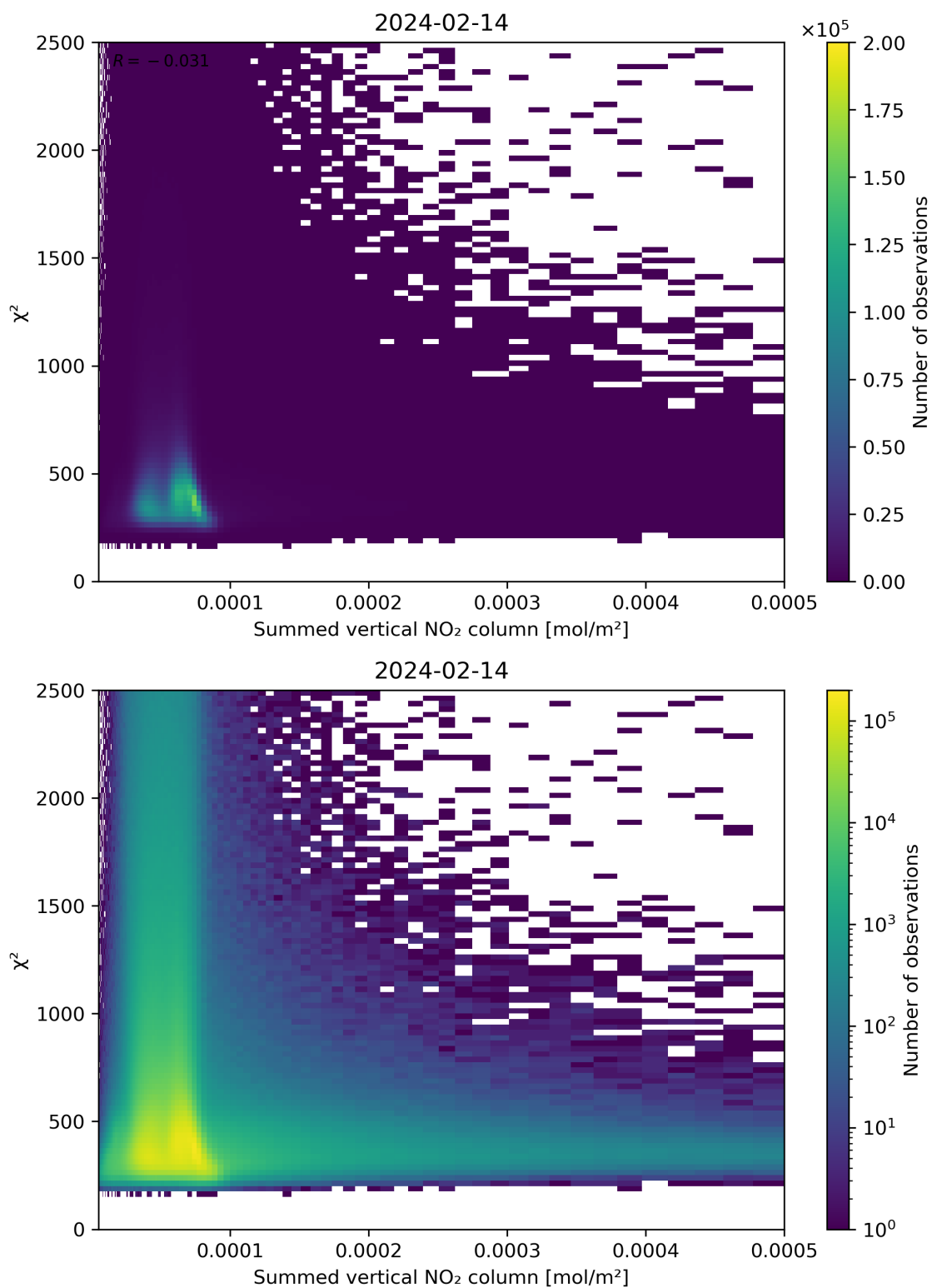
Figure 104: Scatter density plot of “Summed vertical NO 2 column” against “ \chi^2 ” for 2024-02-13 to 2024-02-15.
