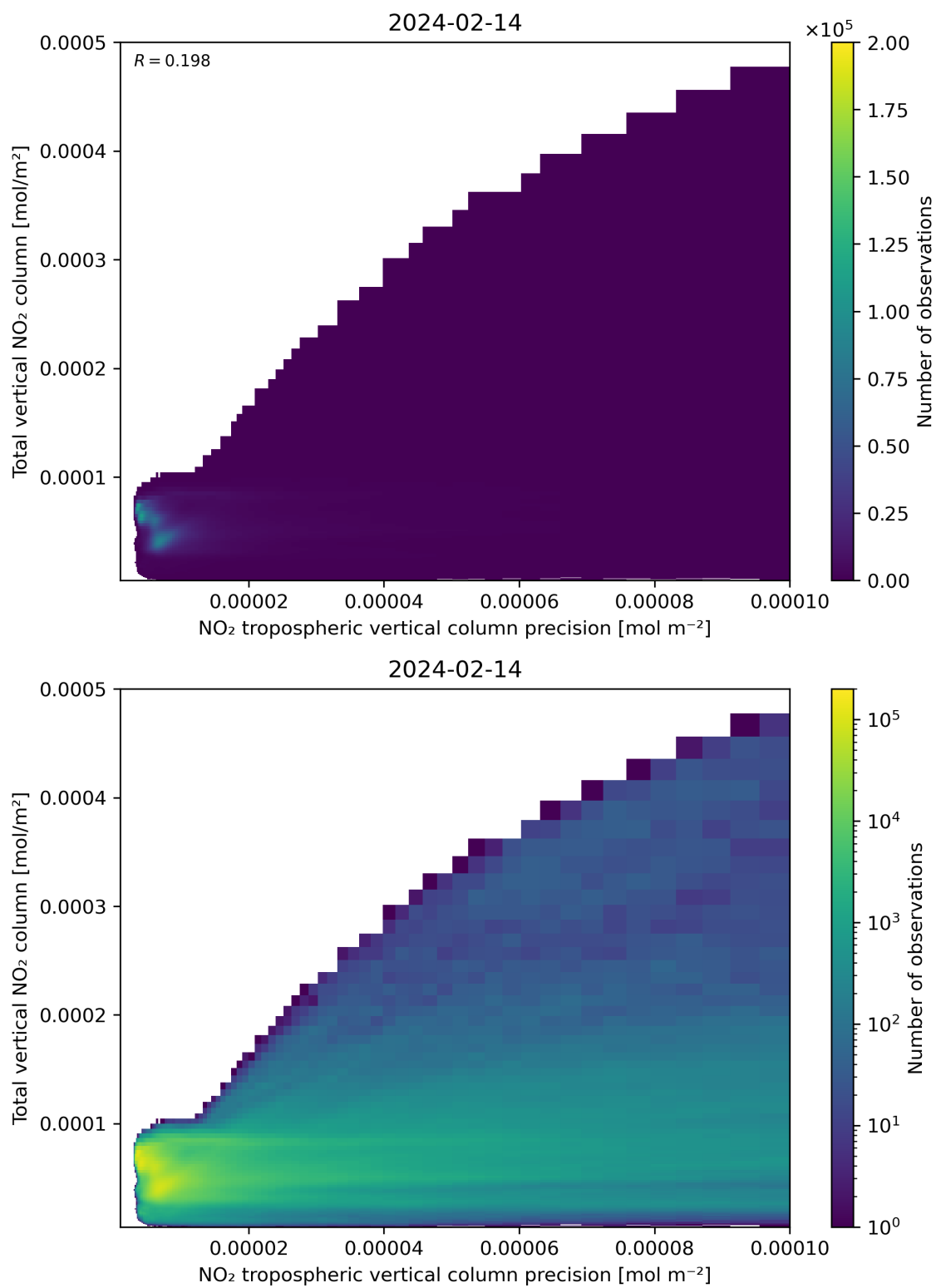
Figure 138: Scatter density plot of “NO 2 tropospheric vertical column precision” against “Total vertical NO 2 column” for 2024-02-13 to 2024-02-15.
