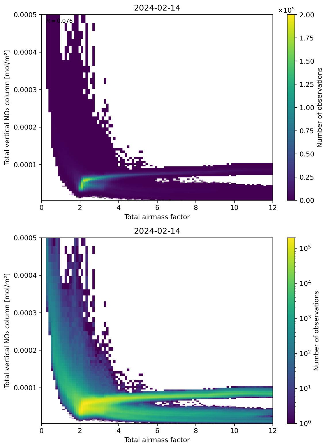
Figure 67: Scatter density plot of “Total airmass factor” against “Total vertical NO 2 column” for 2024-02-13 to 2024-02-15.
