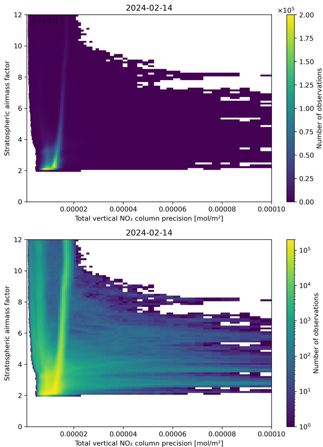
Figure 115: Scatter density plot of “Total vertical NO 2 column precision” against “Stratospheric air mass factor” for 2024-02-13 to 2024-02-15.
