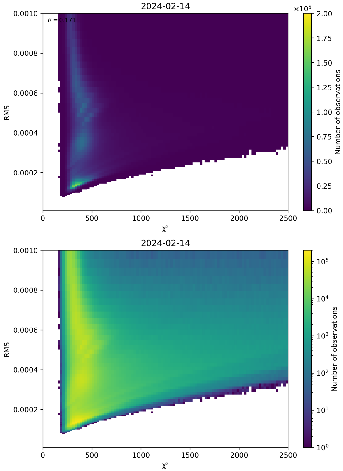
Figure 82: Scatter density plot of “ \chi^2 ” against “RMS” for 2024-02-13 to 2024-02-15.
