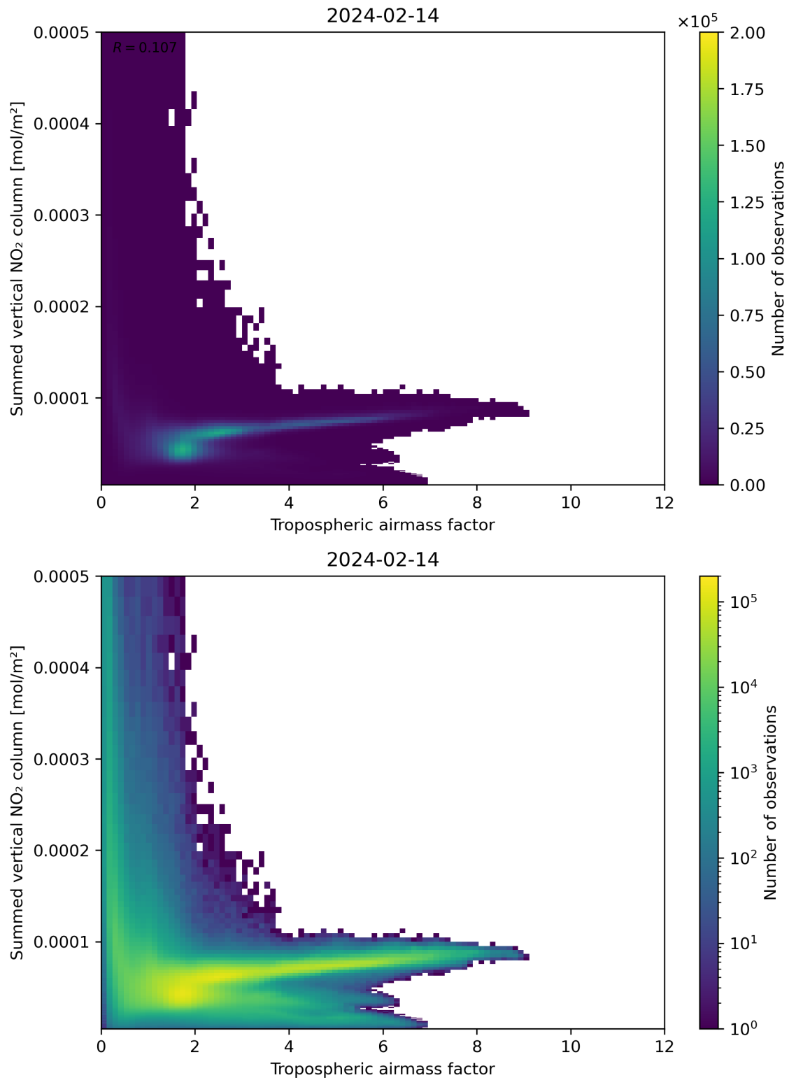
Figure 75: Scatter density plot of “Tropospheric airmass factor” against “Summed vertical NO 2 column” for 2024-02-13 to 2024-02-15.
