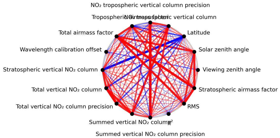
Figure 1: Map of correlation graph for 2024-02-13 to 2024-02-15.
