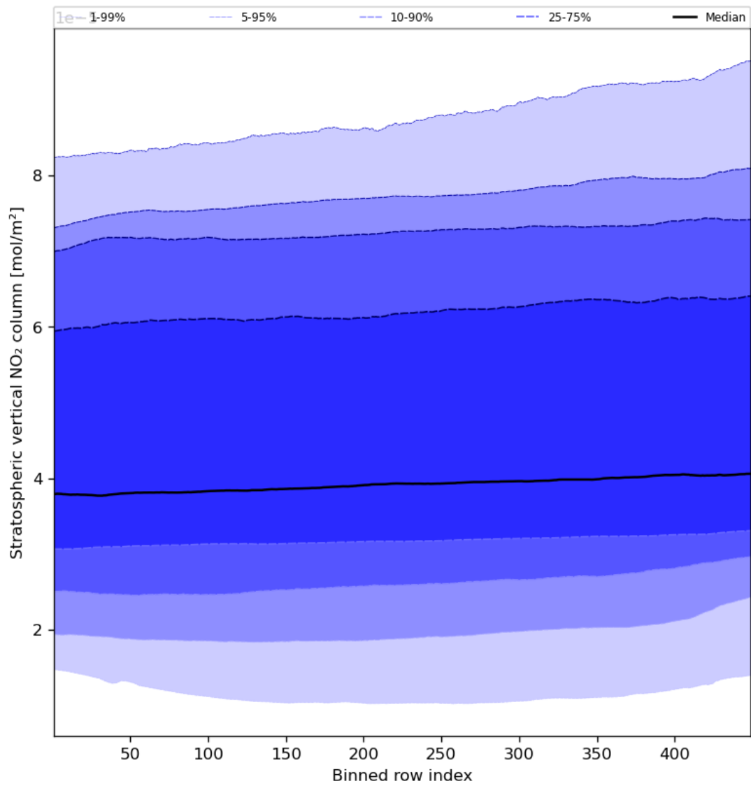
Figure 53: Along track statistics of “Stratospheric vertical NO 2 column” for 2024-02-13 to 2024-02-15
