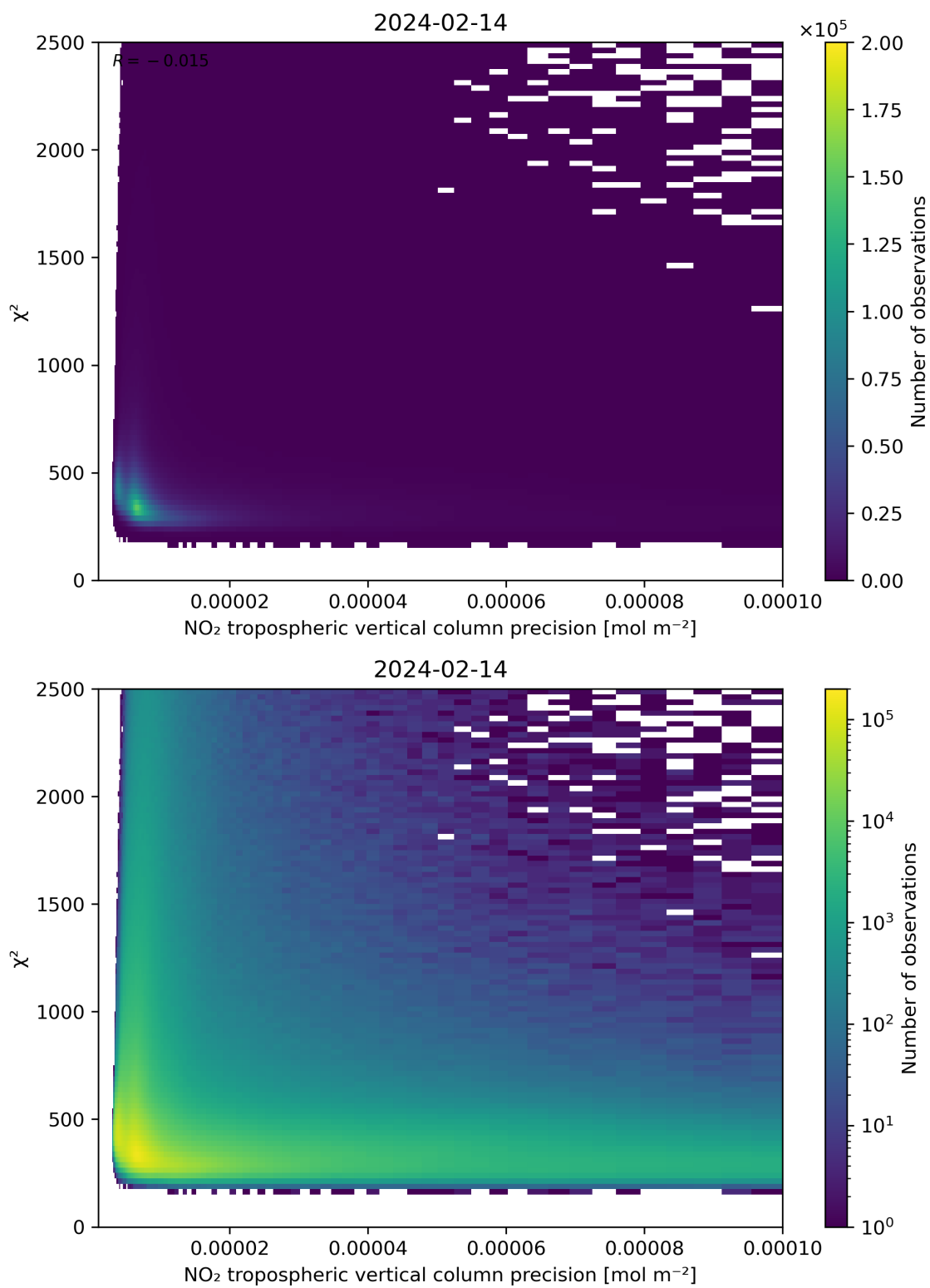
Figure 134: Scatter density plot of “NO 2 tropospheric vertical column precision” against “ \chi^2 ” for 2024-02-13 to 2024-02-15.
