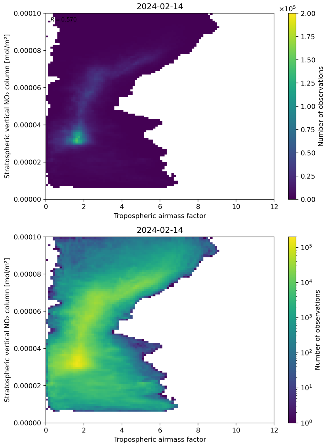
Figure 74: Scatter density plot of “Tropospheric air mass factor” against “Stratospheric vertical NO 2 column” for 2024-02-13 to 2024-02-15.
