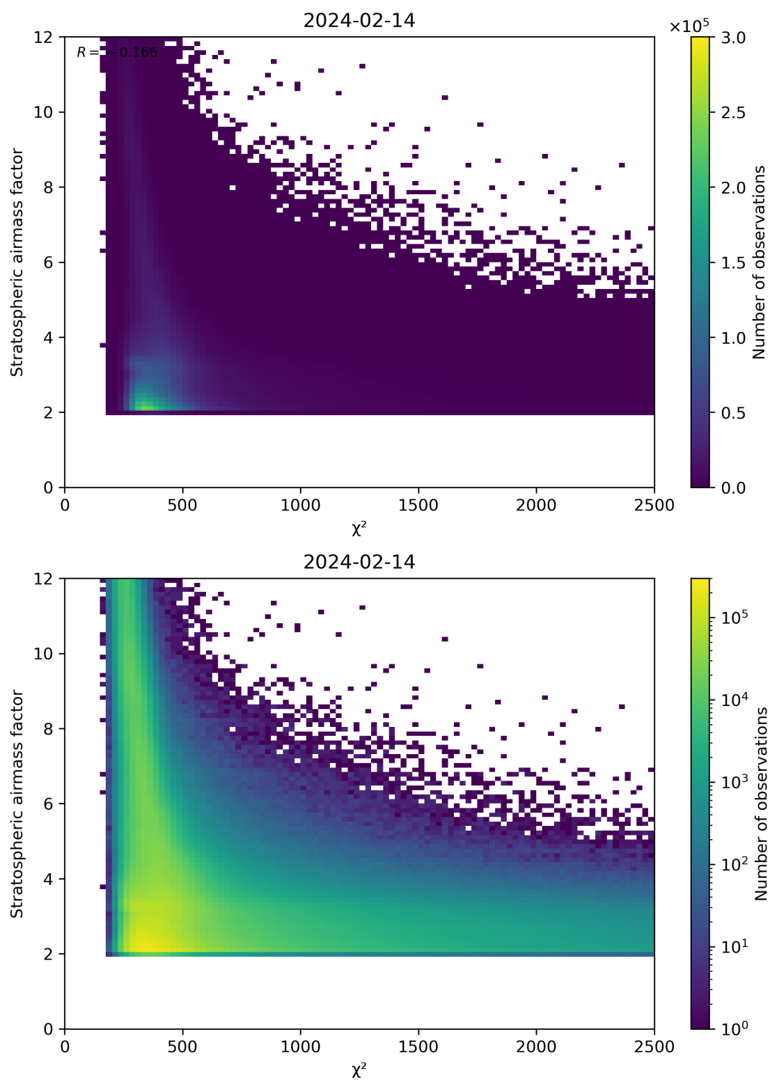
Figure 81: Scatter density plot of “ \chi^2 ” against “Stratospheric airmass factor” for 2024-02-13 to 2024-02-15.
