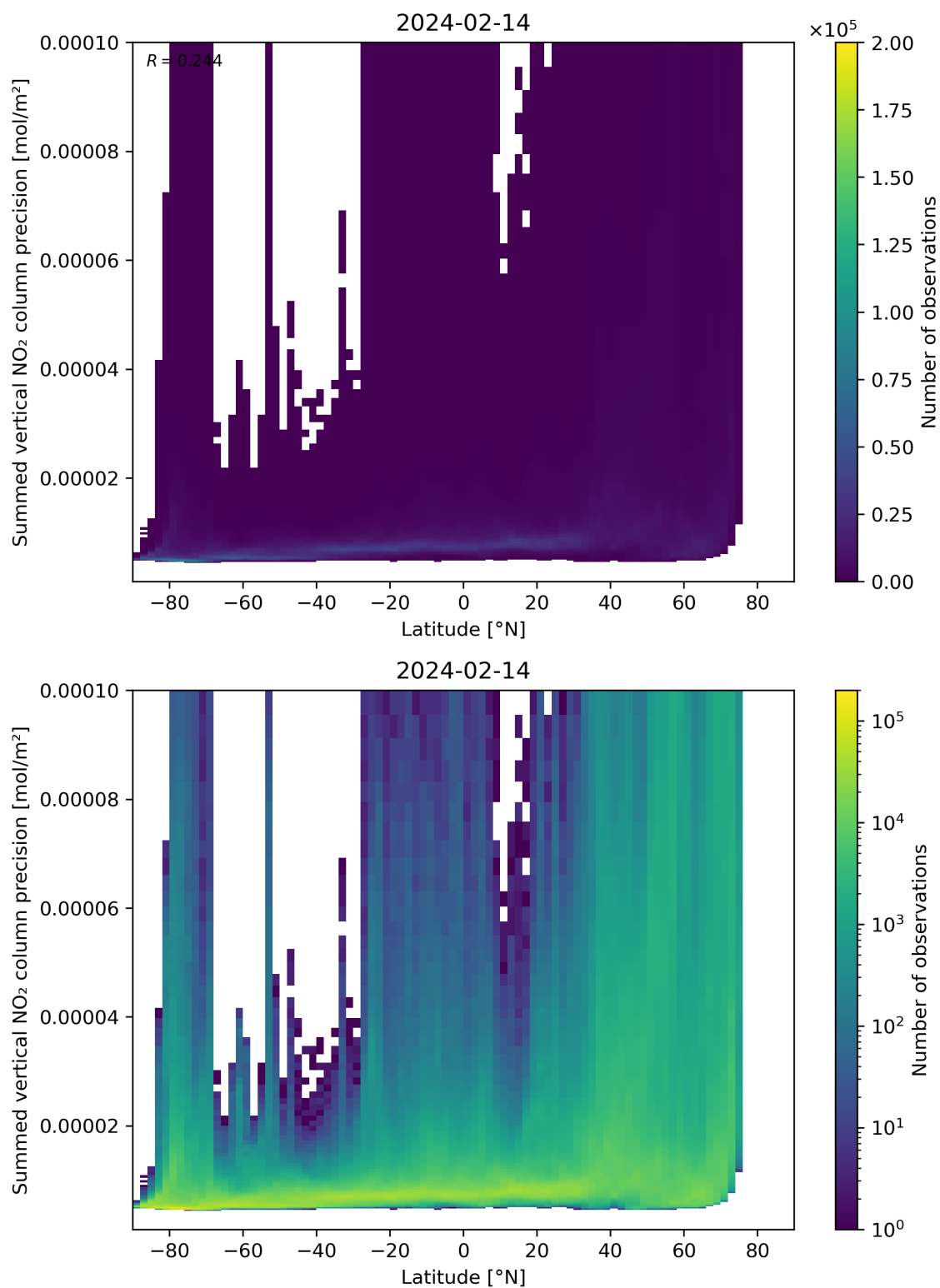
Figure 89: Scatter density plot of “Latitude” against “Summed vertical NO 2 column precision” for 2024-02-13 to 2024-02-15.
