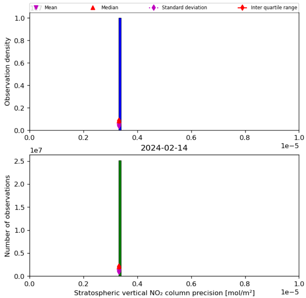
Figure 37: Histogram of “Stratospheric vertical NO 2 column precision” for 2024-02-13 to 2024-02-15
