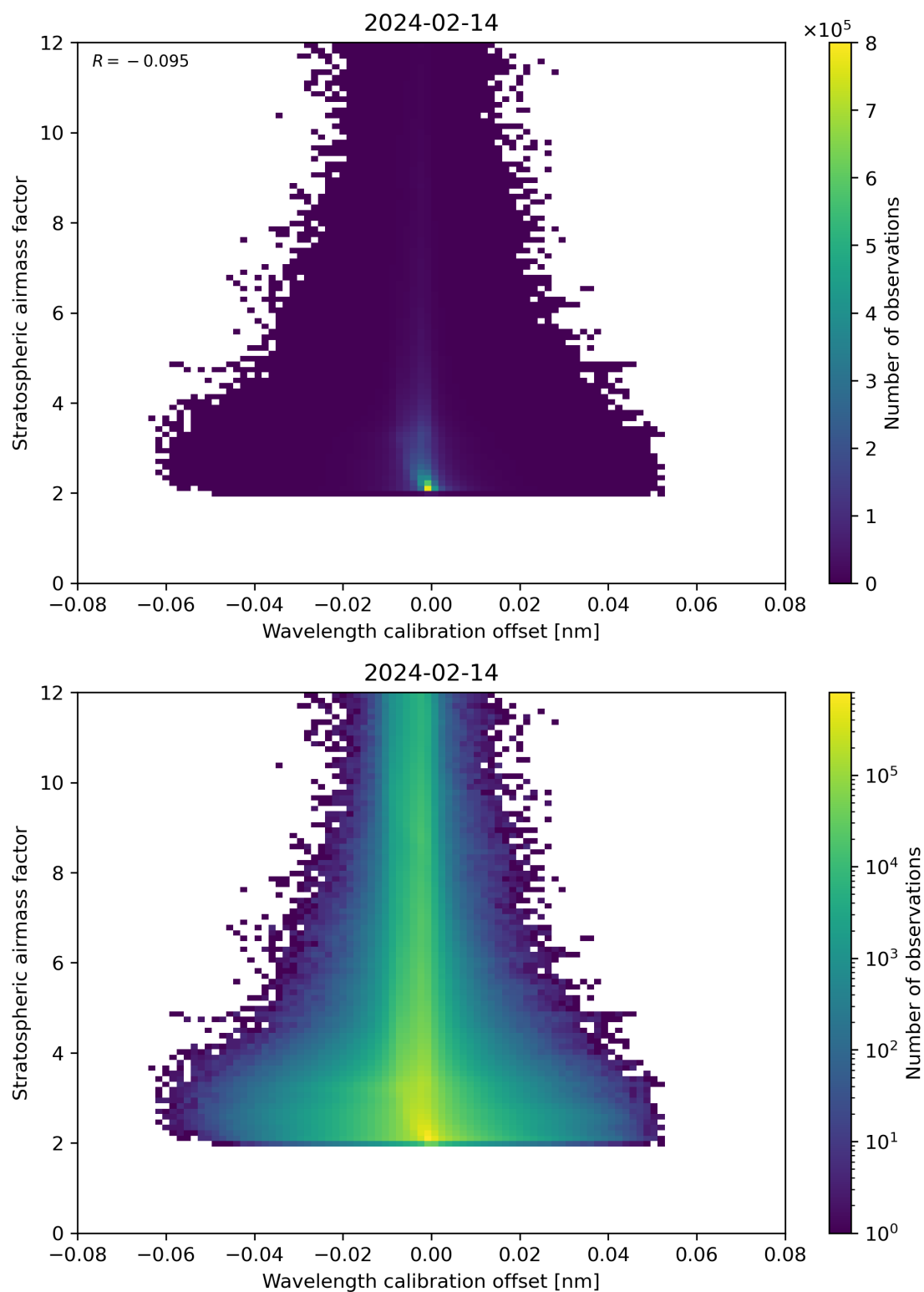
Figure 174: Scatter density plot of “Wavelength calibration offset” against “Stratospheric airmass factor” for 2024-02-13 to 2024-02-15.
