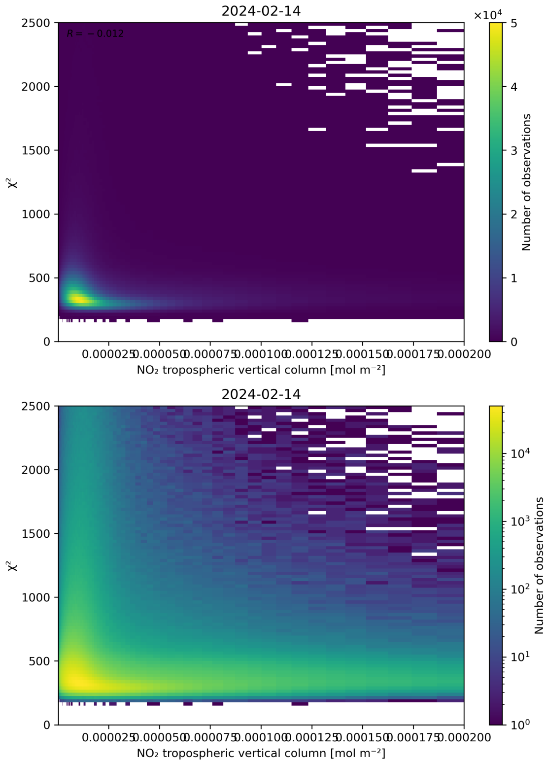
Figure 124: Scatter density plot of “NO 2 tropospheric vertical column” against “ \chi^2 ” for 2024-02-13 to 2024-02-15.
