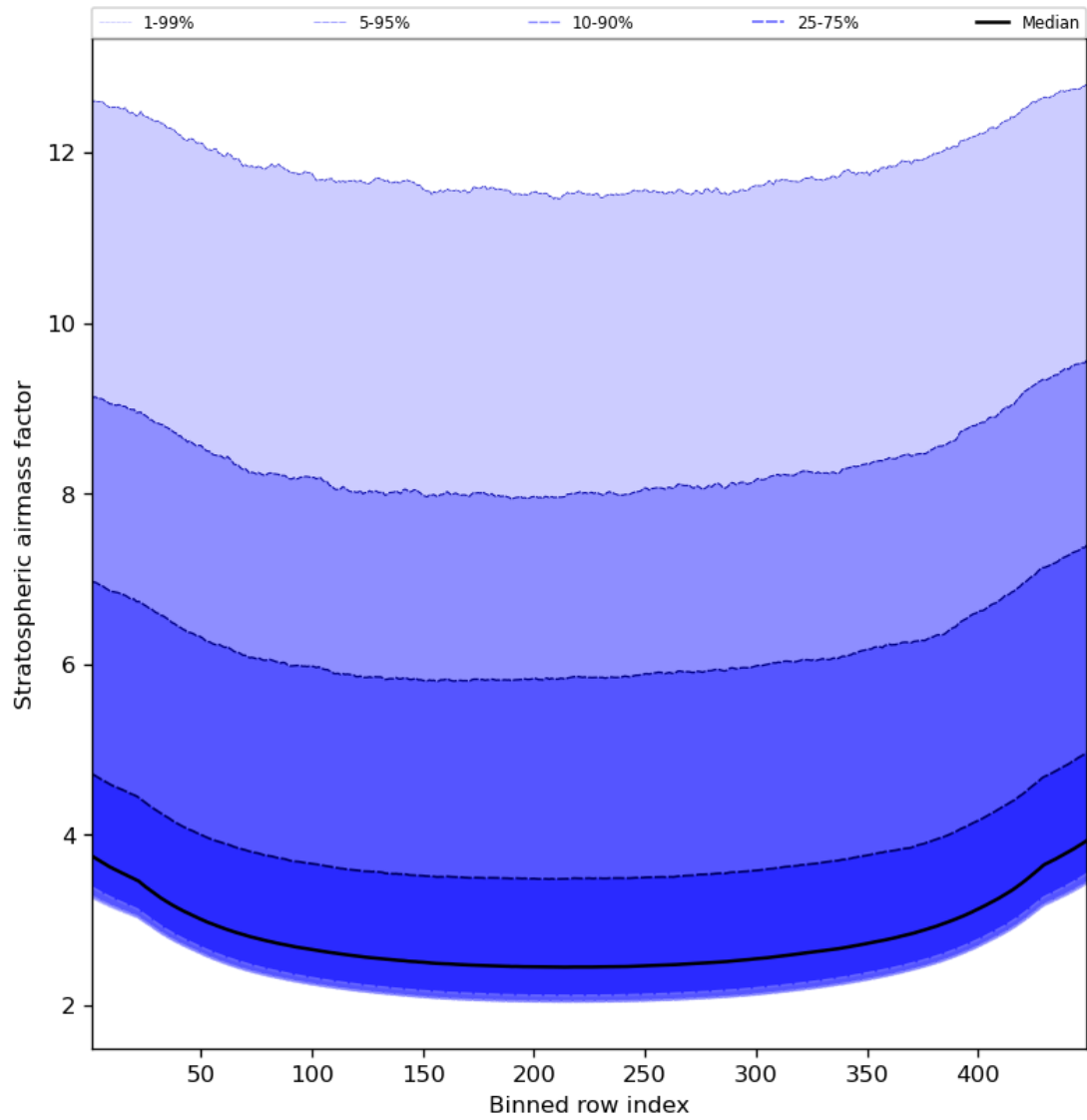
Figure 61: Along track statistics of “Stratospheric airmass factor” for 2024-02-13 to 2024-02-15
