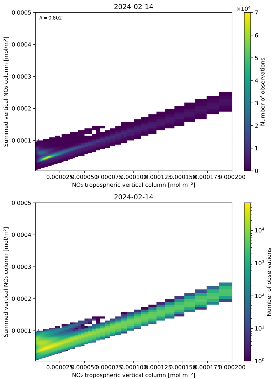
Figure 126: Scatter density plot of “NO 2 tropospheric vertical column” against “Summed vertical NO 2 column” for 2024-02-13 to 2024-02-15.
