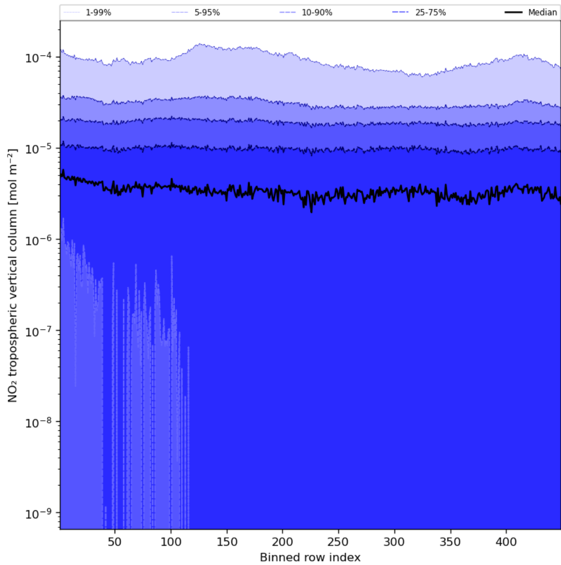
Figure 46: Along track statistics of "NO 2 tropospheric vertical column" for 2024-02-13 to 2024-02-15
