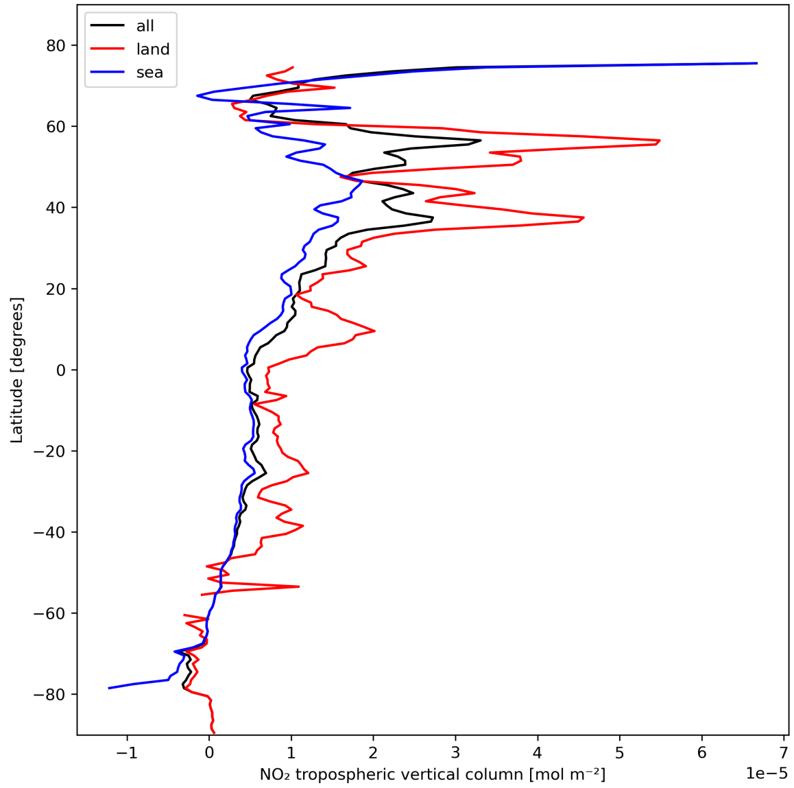
Figure 12: Zonal average of “NO 2 tropospheric vertical column” for 2024-02-13 to 2024-02-15.
