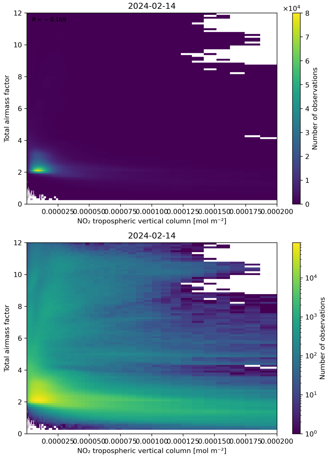
Figure 122: Scatter density plot of “NO 2 tropospheric vertical column” against “Total air mass factor” for 2024-02-13 to 2024-02-15.
