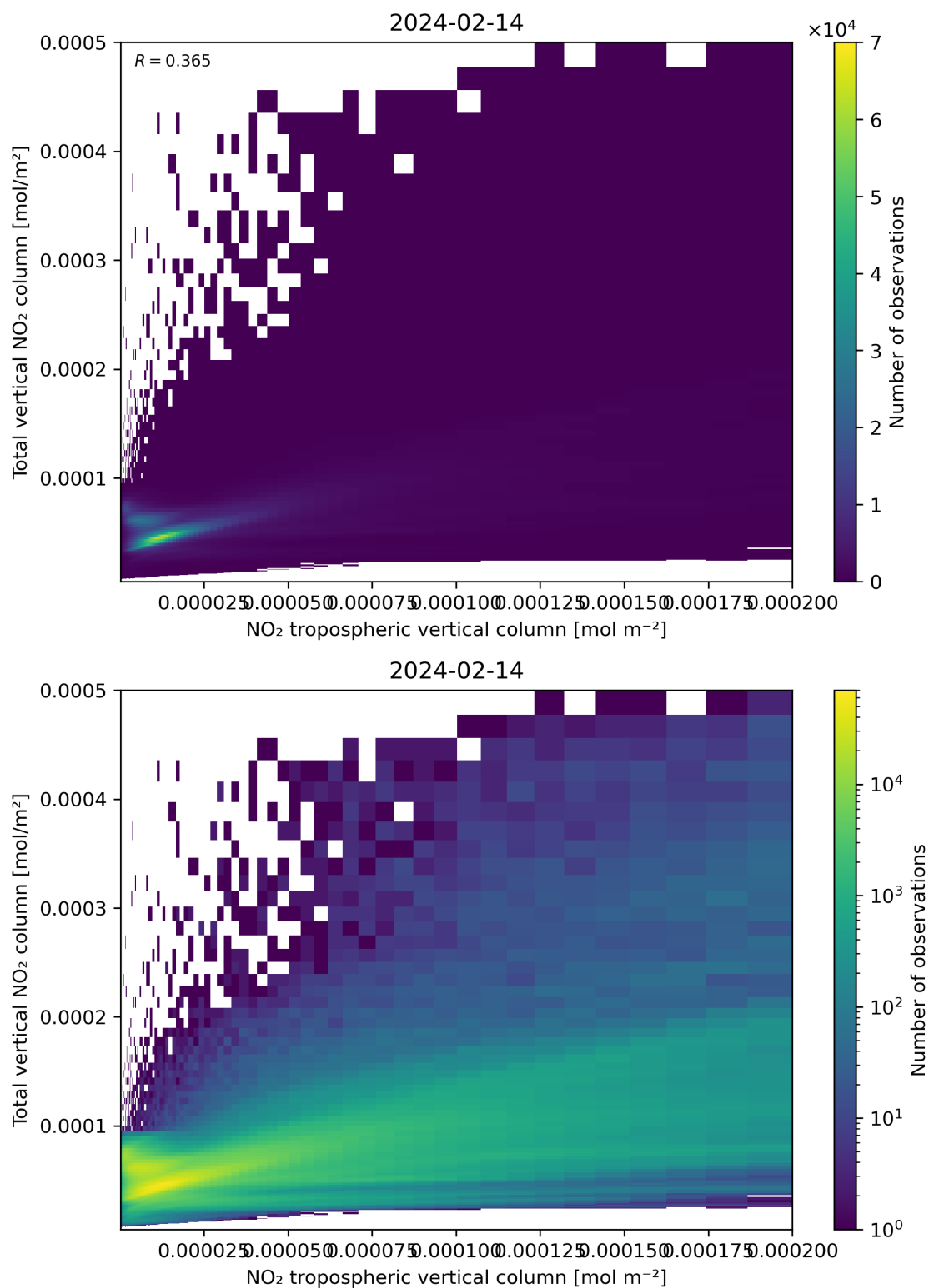
Figure 128: Scatter density plot of “NO 2 tropospheric vertical column” against “Total vertical NO 2 column” for 2024-02-13 to 2024-02-15.
