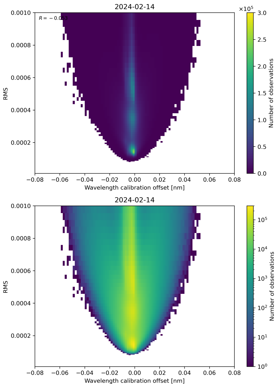
Figure 181: Scatter density plot of “Wavelength calibration offset” against “RMS” for 2024-02-13 to 2024-02-15.
