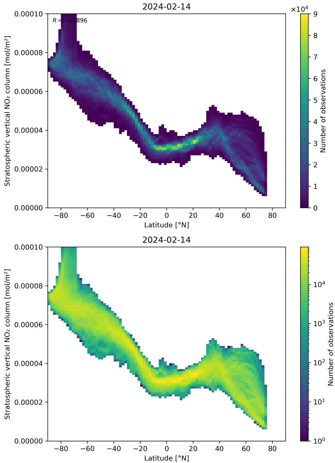
Figure 87: Scatter density plot of “Latitude” against “Stratospheric vertical NO 2 column” for 2024-02-13 to 2024-02-15.
