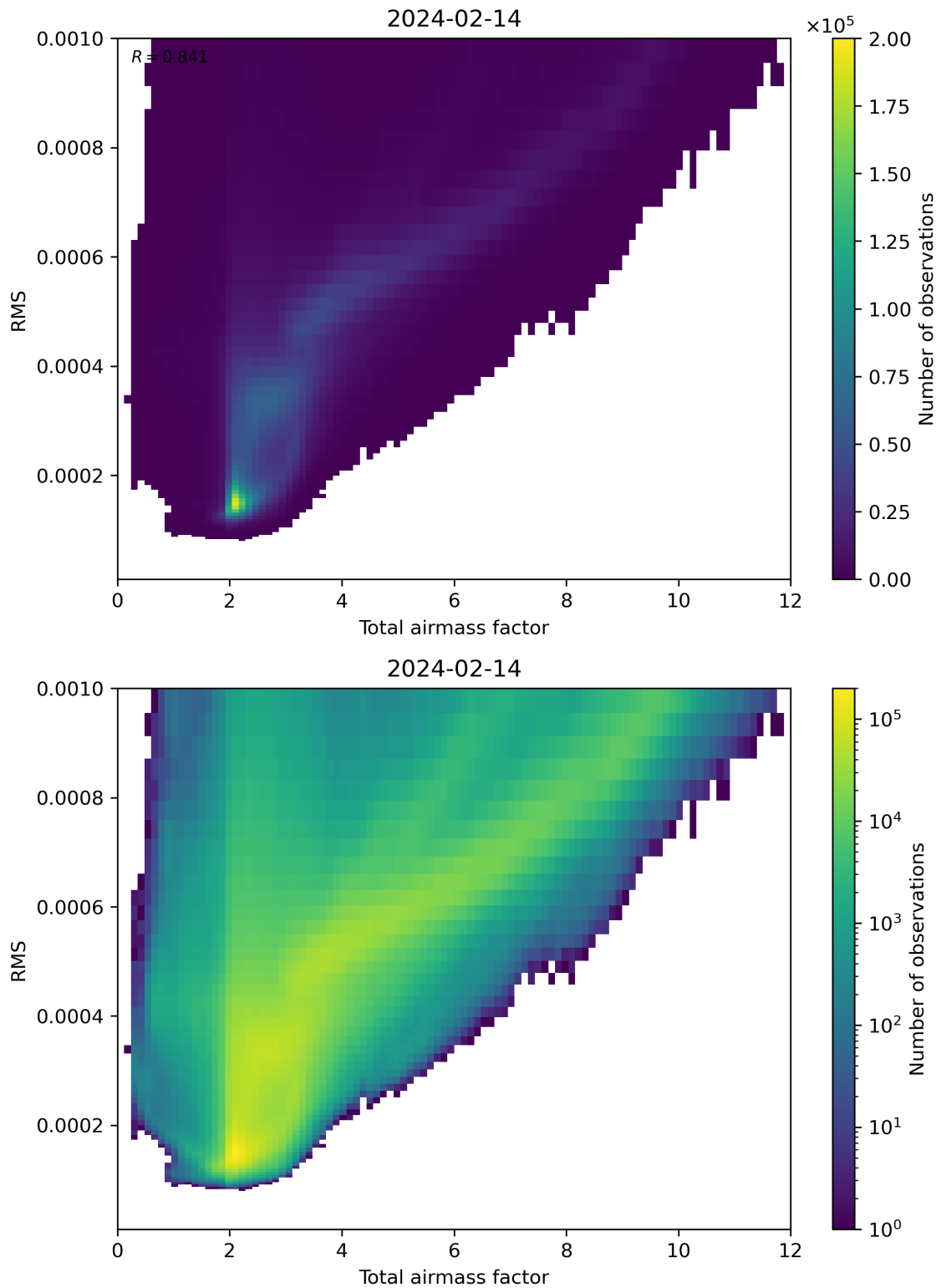
Figure 69: Scatter density plot of “Total airmass factor” against “RMS” for 2024-02-13 to 2024-02-15.
