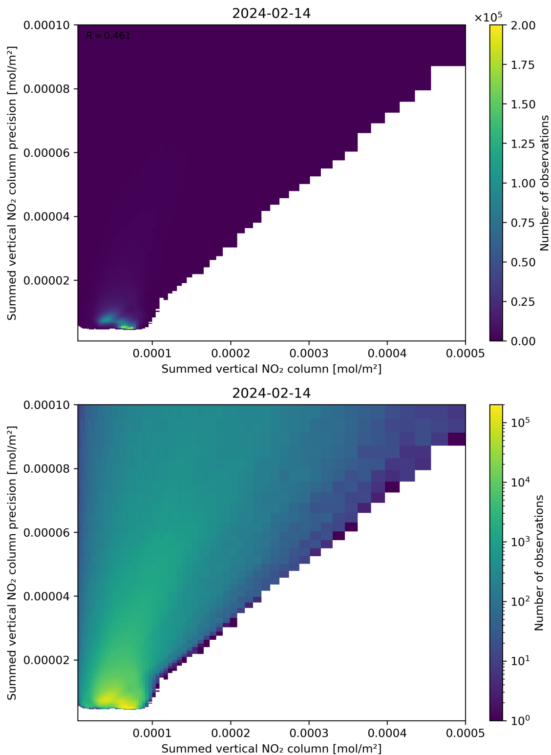
Figure 105: Scatter density plot of “Summed vertical NO 2 column” against “Summed vertical NO 2 column precision” for 2024-02-13 to 2024-02-15.
