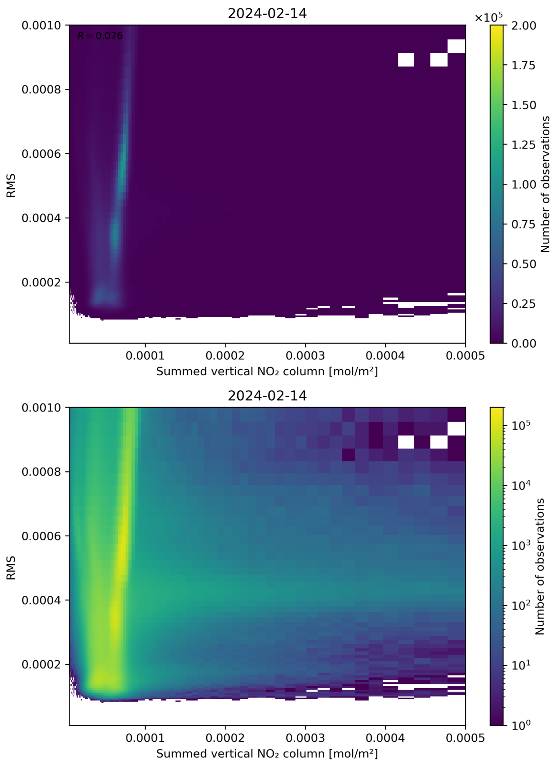
Figure 109: Scatter density plot of “Summed vertical NO 2 column” against “RMS” for 2024-02-13 to 2024-02-15.
