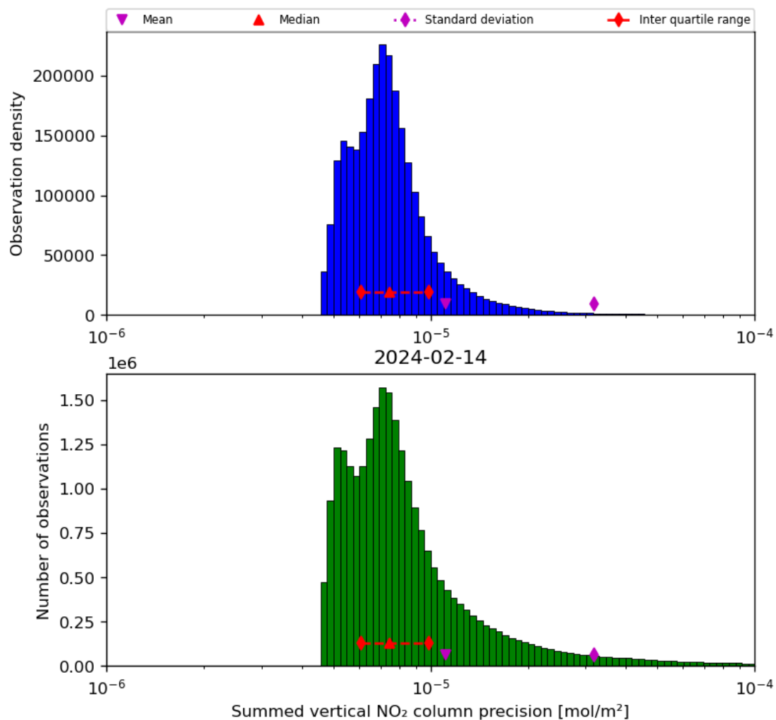
Figure 41: Histogram of "Summed vertical NO 2 column precision" for 2024-02-13 to 2024-02-15
