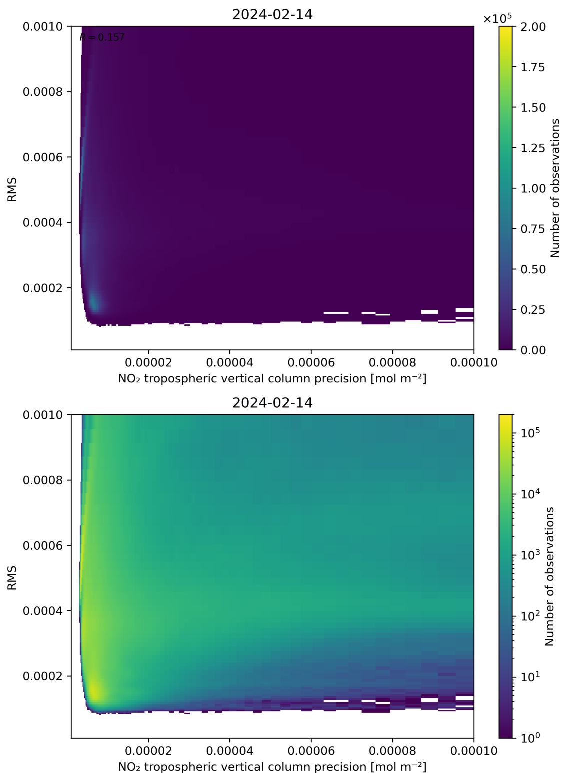
Figure 140: Scatter density plot of “NO 2 tropospheric vertical column precision” against “RMS” for 2024-02-13 to 2024-02-15.
