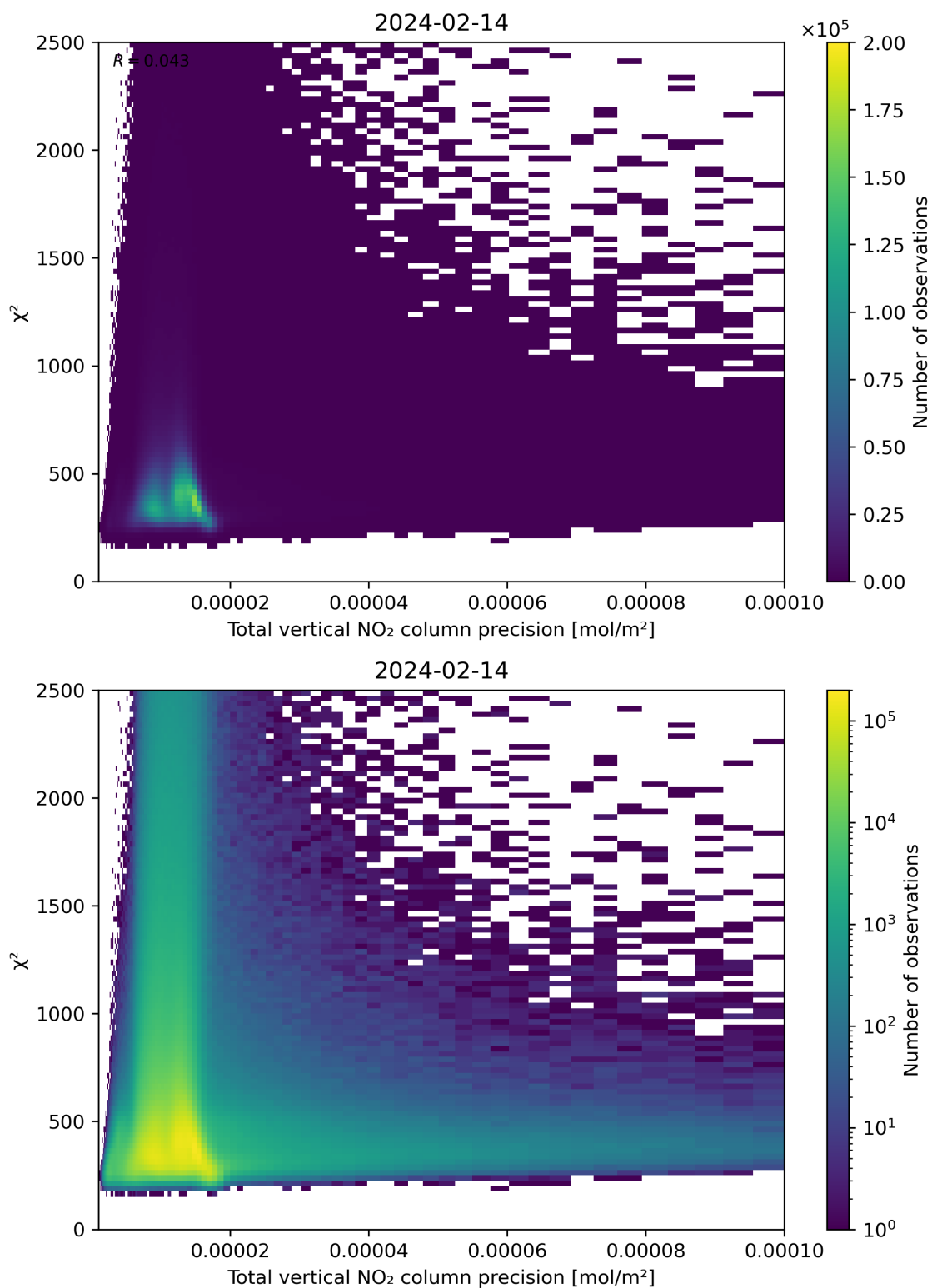
Figure 116: Scatter density plot of “Total vertical NO 2 column precision” against “ \chi^2 ” for 2024-02-13 to 2024-02-15.
