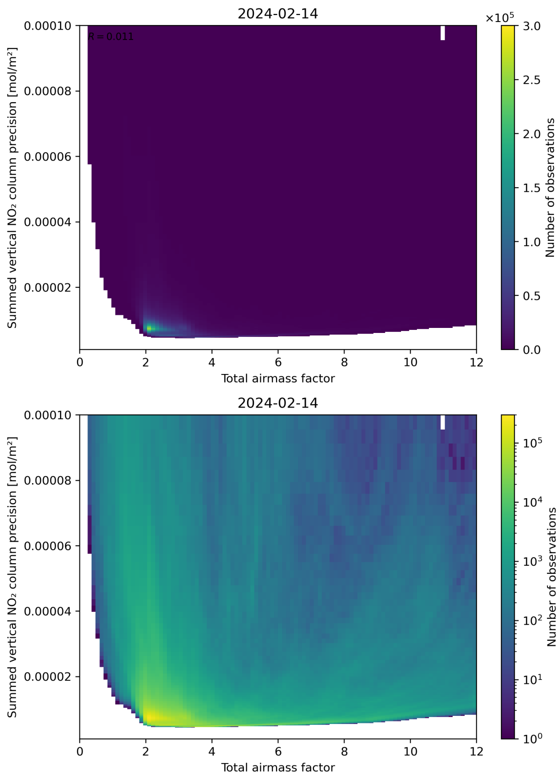
Figure 66: Scatter density plot of “Total airmass factor” against “Summed vertical NO 2 column precision” for 2024-02-13 to 2024-02-15.
