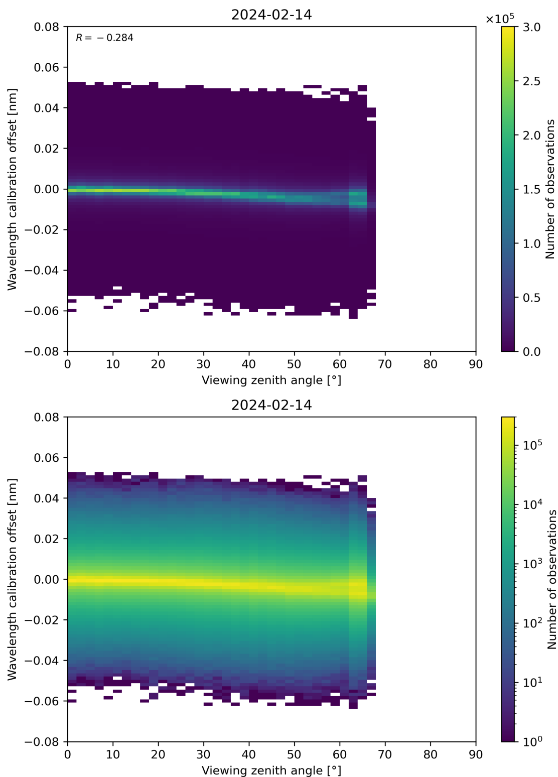
Figure 173: Scatter density plot of “Viewing zenith angle” against “Wavelength calibration offset” for 2024-02-13 to 2024-02-15.
