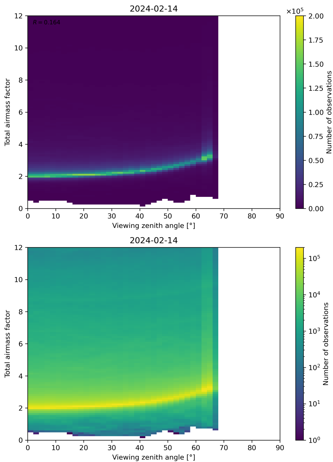
Figure 160: Scatter density plot of “Viewing zenith angle” against “Total airmass factor” for 2024-02-13 to 2024-02-15.
