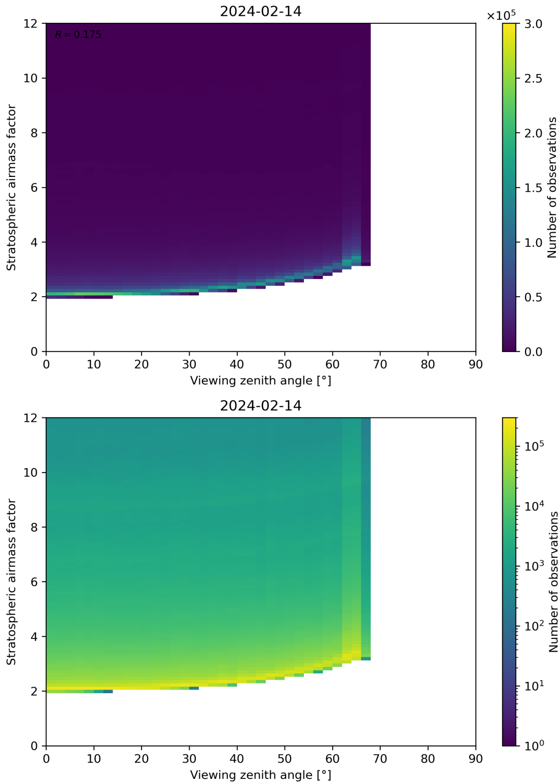
Figure 159: Scatter density plot of “Viewing zenith angle” against “Stratospheric airmass factor” for 2024-02-13 to 2024-02-15.
