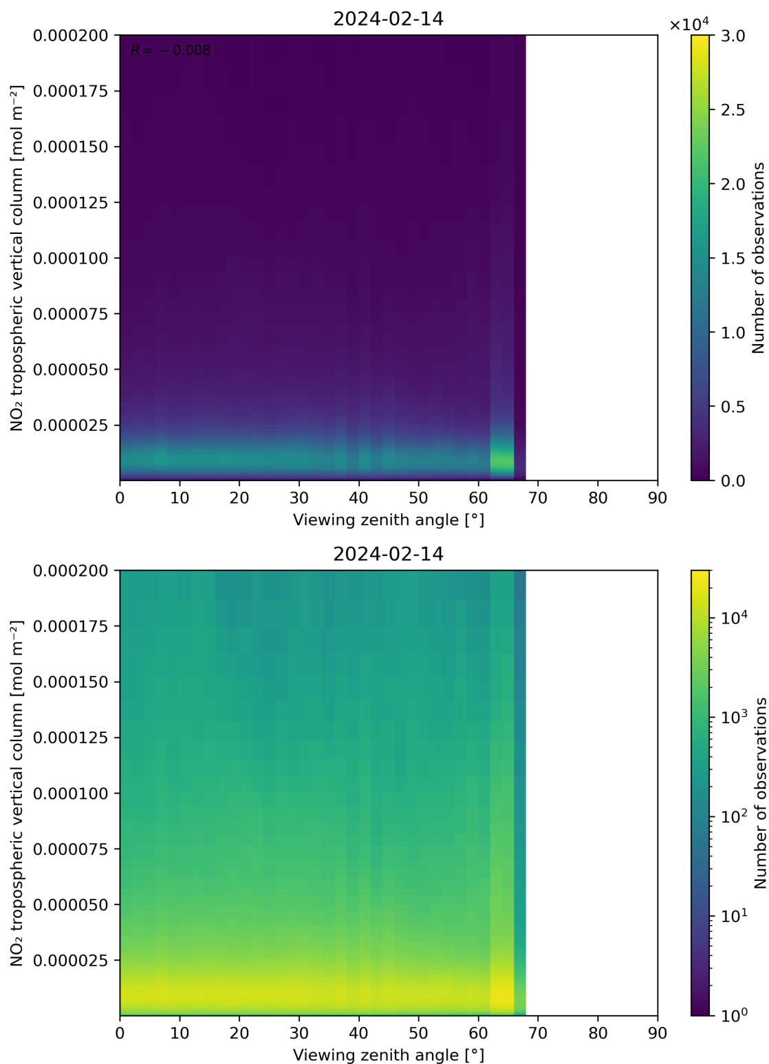
Figure 169: Scatter density plot of “Viewing zenith angle” against “NO 2 tropospheric vertical column” for 2024-02-13 to 2024-02-15.
