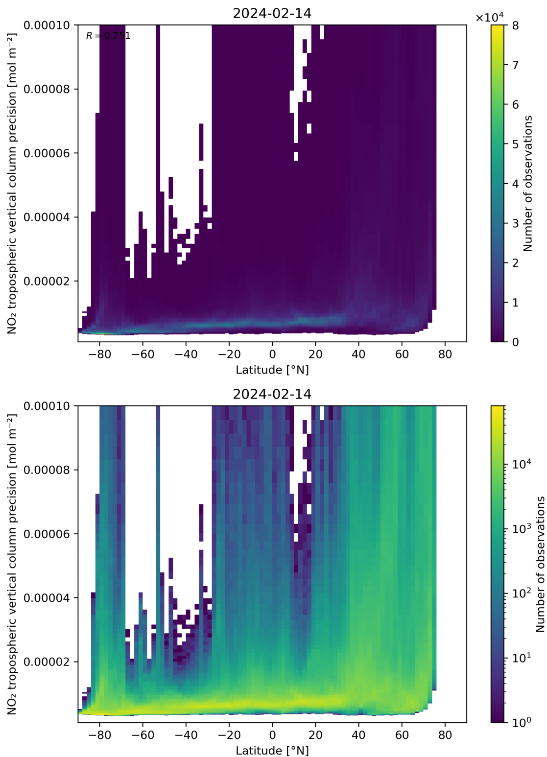
Figure 93: Scatter density plot of “Latitude” against “NO 2 tropospheric vertical column precision” for 2024-02-13 to 2024-02-15.
