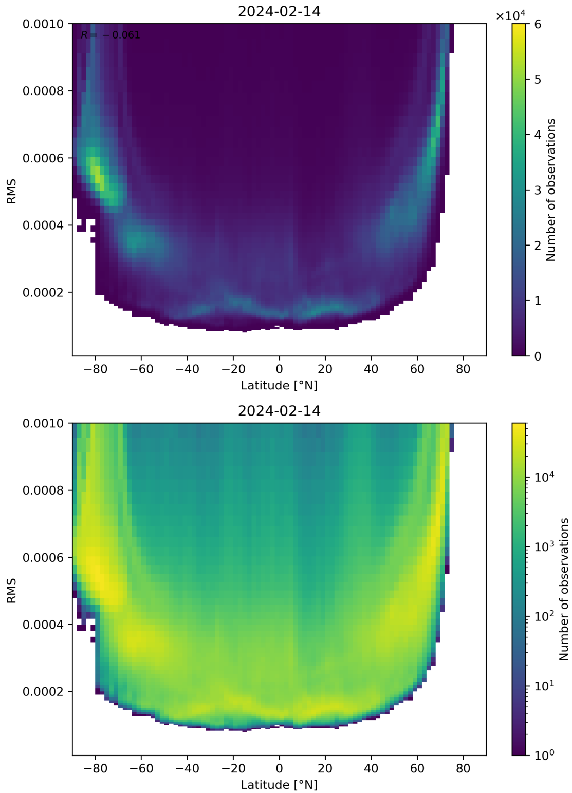
Figure 94: Scatter density plot of “Latitude” against “RMS” for 2024-02-13 to 2024-02-15.
