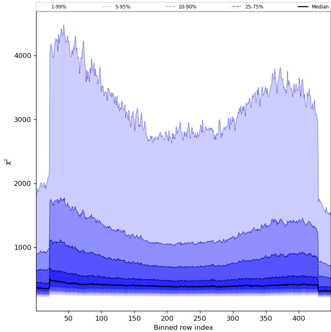
Figure 59: Along track statistics of “ \chi^2 ” for 2024-02-13 to 2024-02-15
