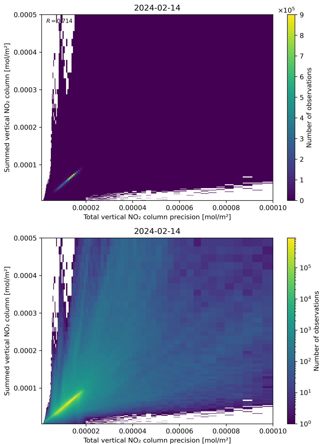
Figure 117: Scatter density plot of “Total vertical NO 2 column precision” against “Summed vertical NO 2 column” for 2024-02-13 to 2024-02-15.
