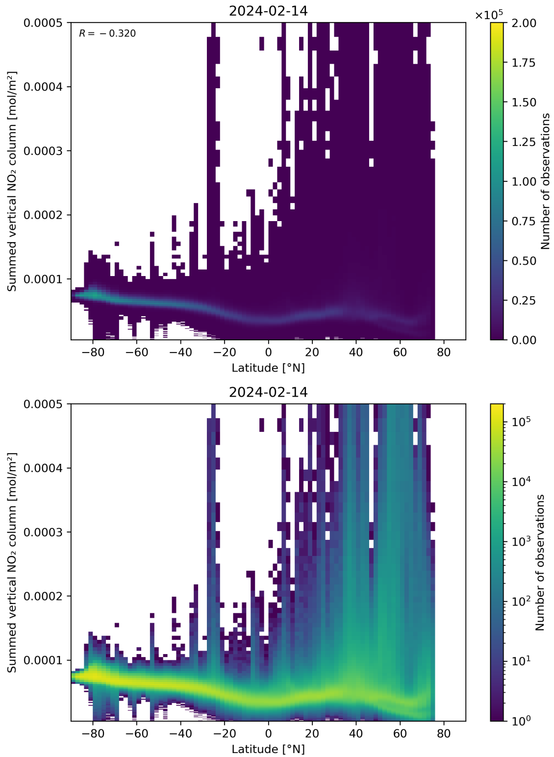
Figure 88: Scatter density plot of “Latitude” against “Summed vertical NO 2 column” for 2024-02-13 to 2024-02-15.
