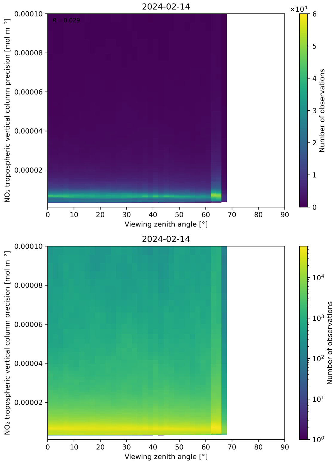
Figure 170: Scatter density plot of “Viewing zenith angle” against “NO 2 tropospheric vertical column precision” for 2024-02-13 to 2024-02-15.
