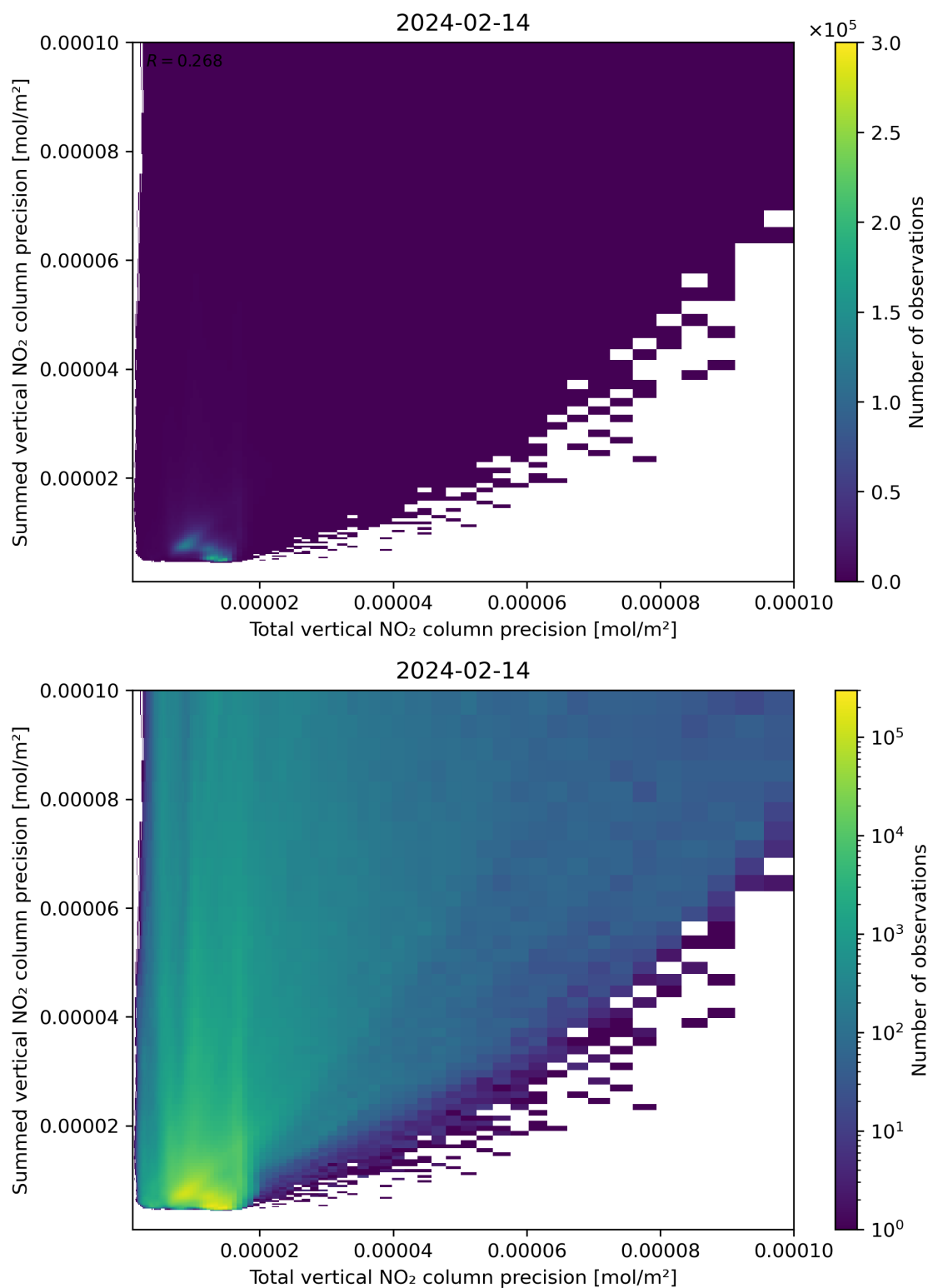
Figure 118: Scatter density plot of “Total vertical NO 2 column precision” against “Summed vertical NO 2 column precision” for 2024-02-13 to 2024-02-15.
