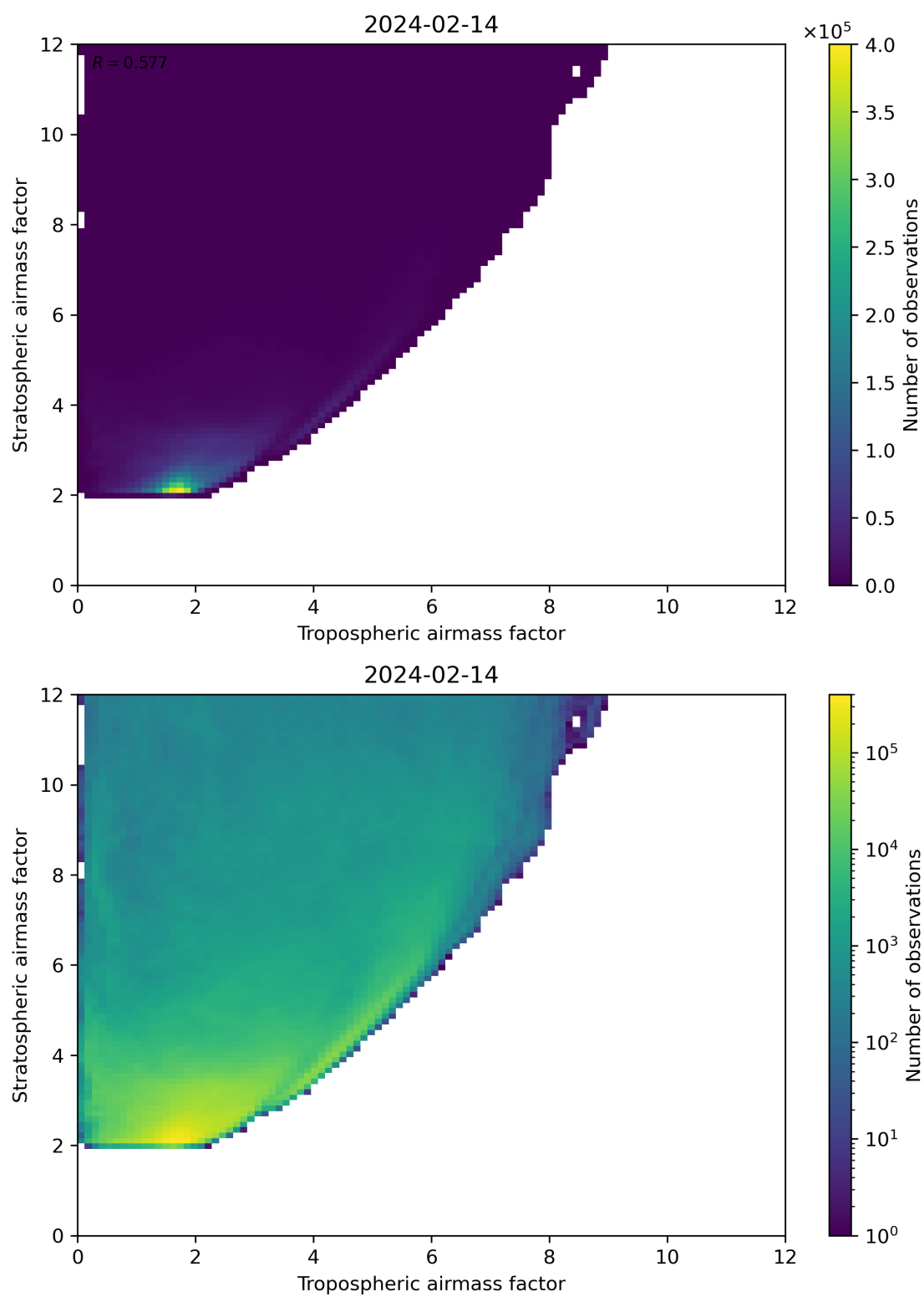
Figure 71: Scatter density plot of “Tropospheric airmass factor” against “Stratospheric airmass factor” for 2024-02-13 to 2024-02-15.
