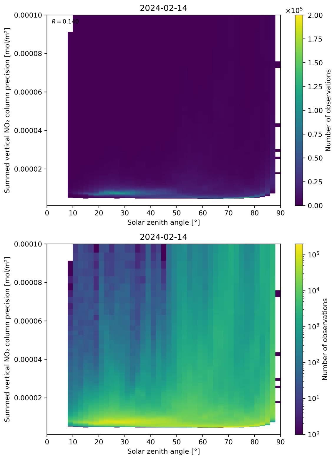
Figure 152: Scatter density plot of “Solar zenith angle” against “Summed vertical NO 2 column precision” for 2024-02-13 to 2024-02-15.
