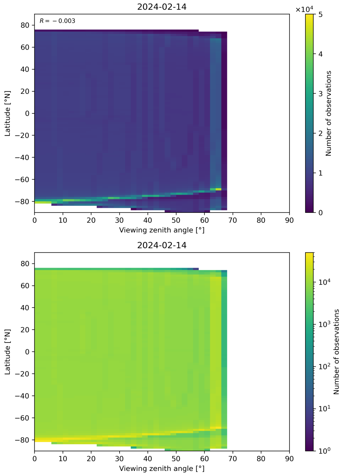
Figure 163: Scatter density plot of “Viewing zenith angle” against “Latitude” for 2024-02-13 to 2024-02-15.
