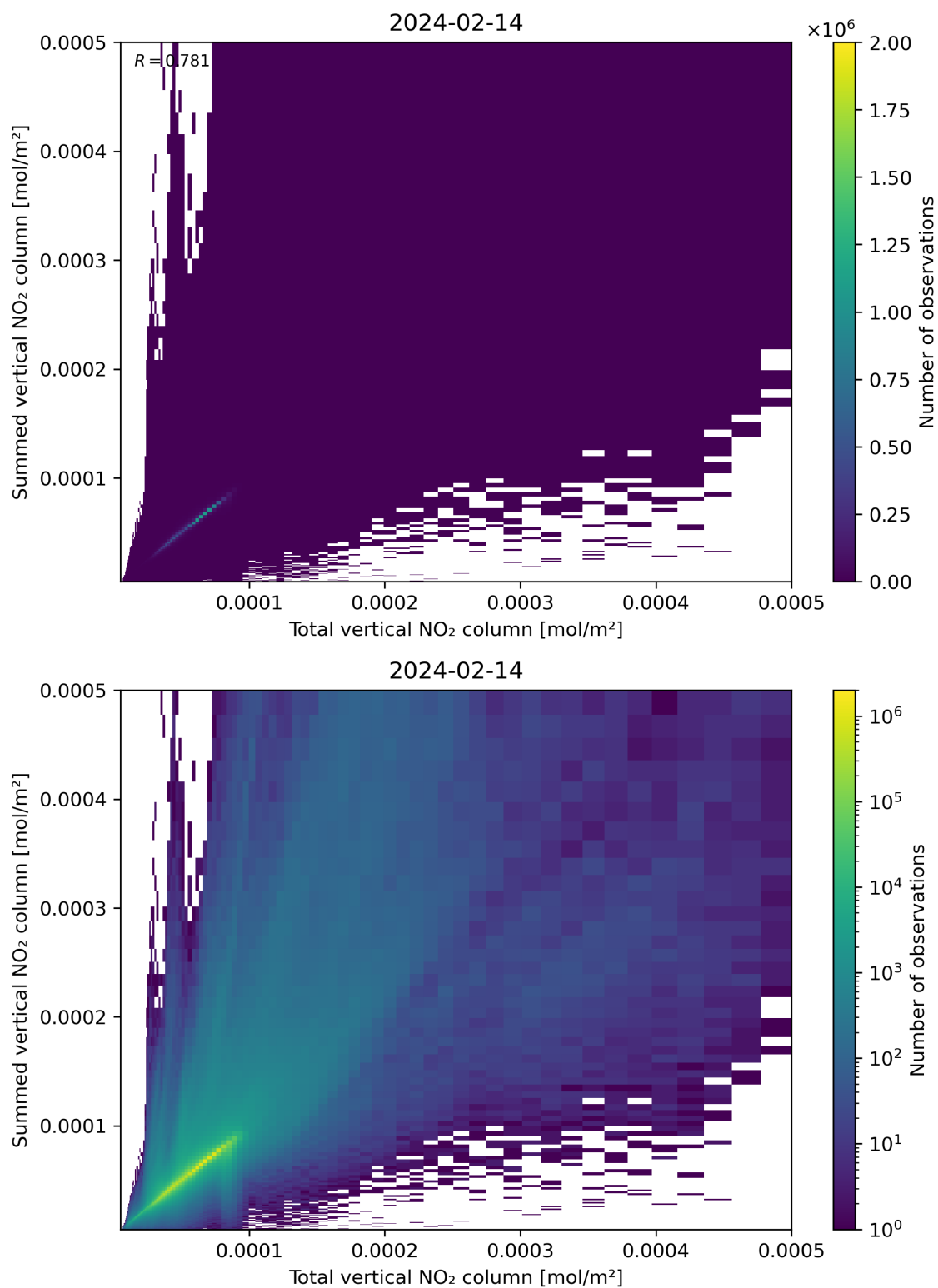
Figure 112: Scatter density plot of “Total vertical NO 2 column” against “Summed vertical NO 2 column” for 2024-02-13 to 2024-02-15.
