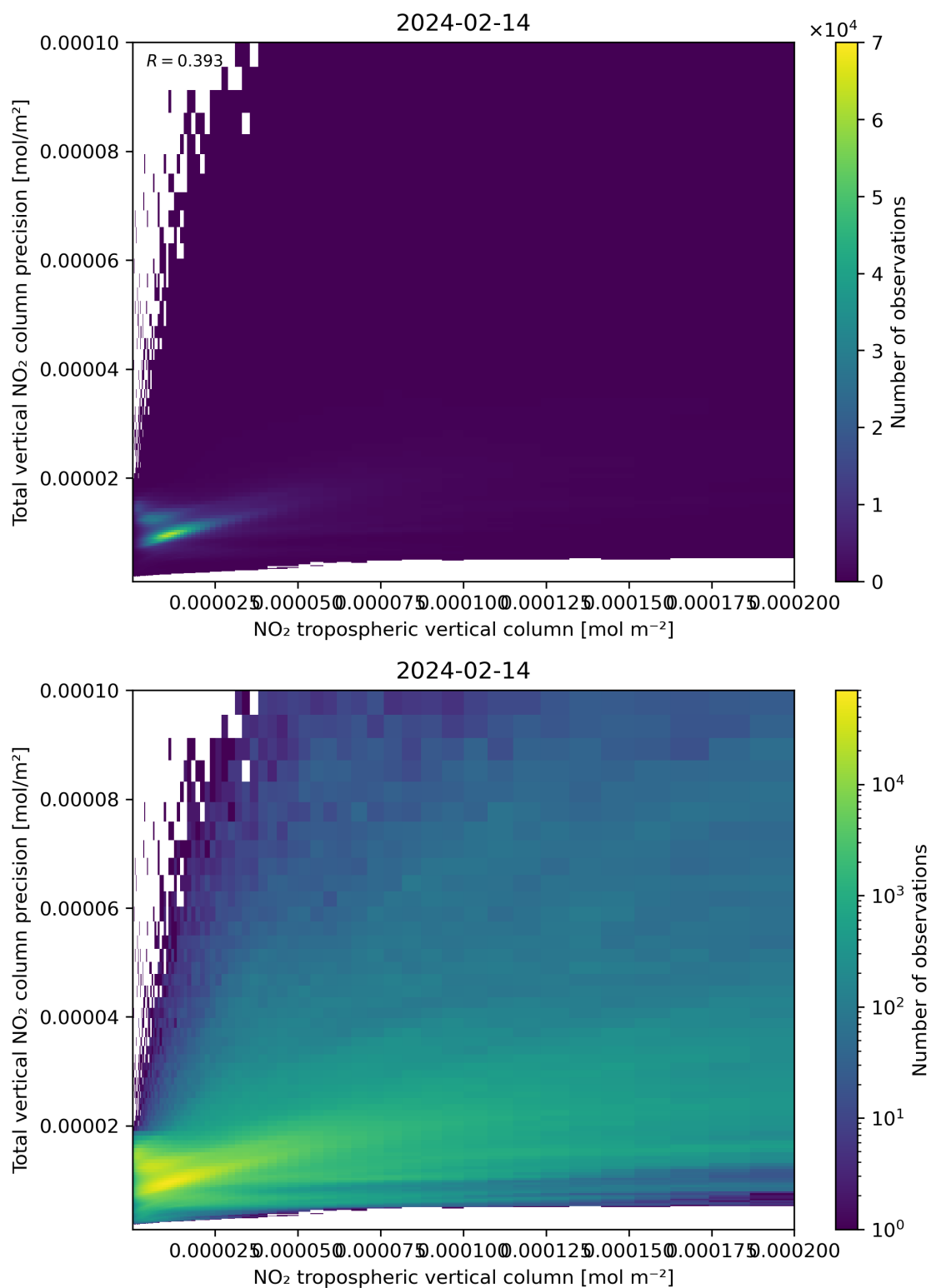
Figure 129: Scatter density plot of “NO 2 tropospheric vertical column” against “Total vertical NO 2 column precision” for 2024-02-13 to 2024-02-15.
