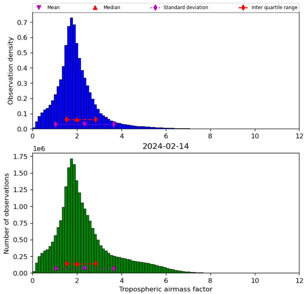
Figure 31: Histogram of “Tropospheric airmass factor” for 2024-02-13 to 2024-02-15
