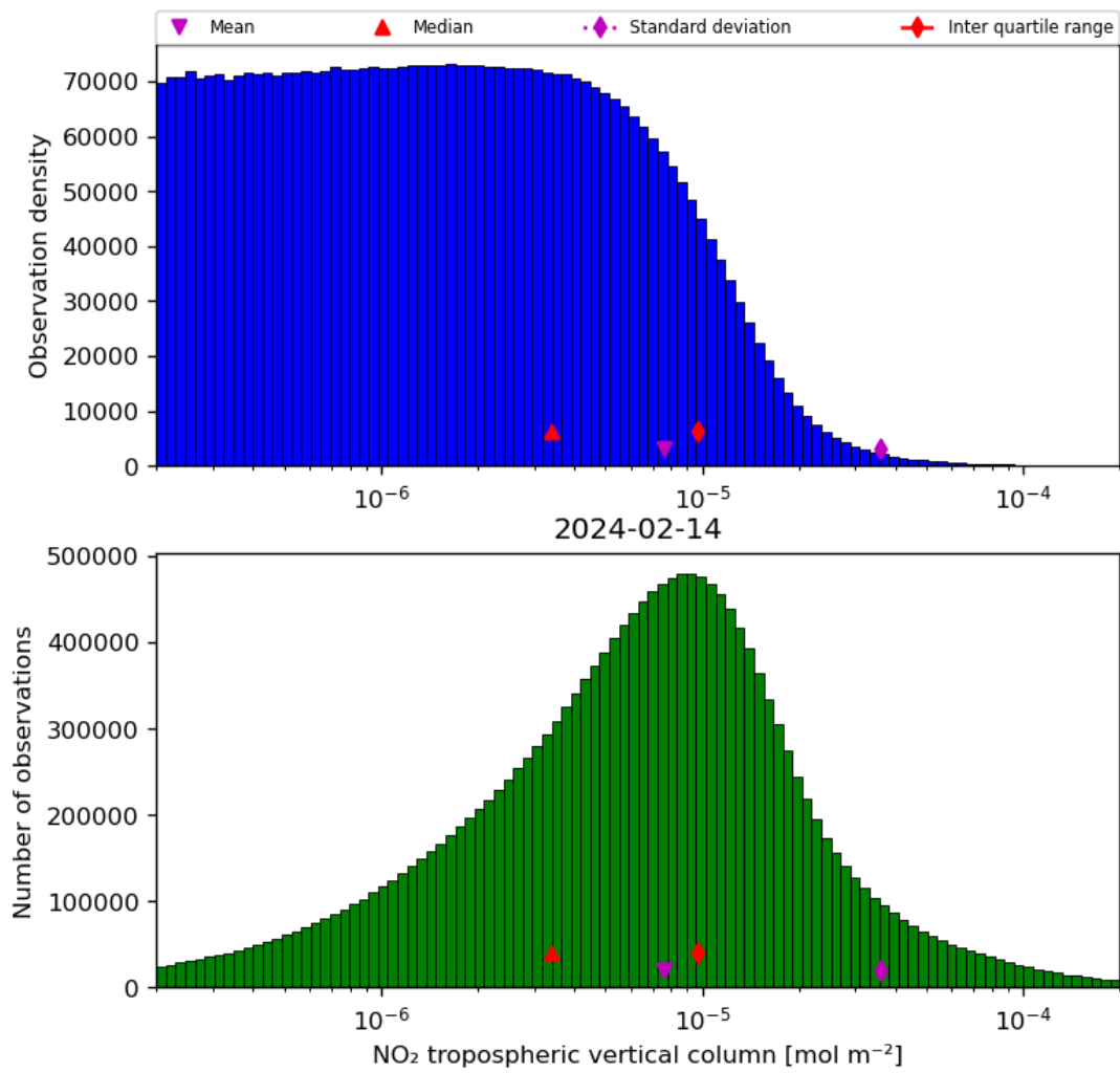
Figure 29: Histogram of “NO 2 tropospheric vertical column” for 2024-02-13 to 2024-02-15
