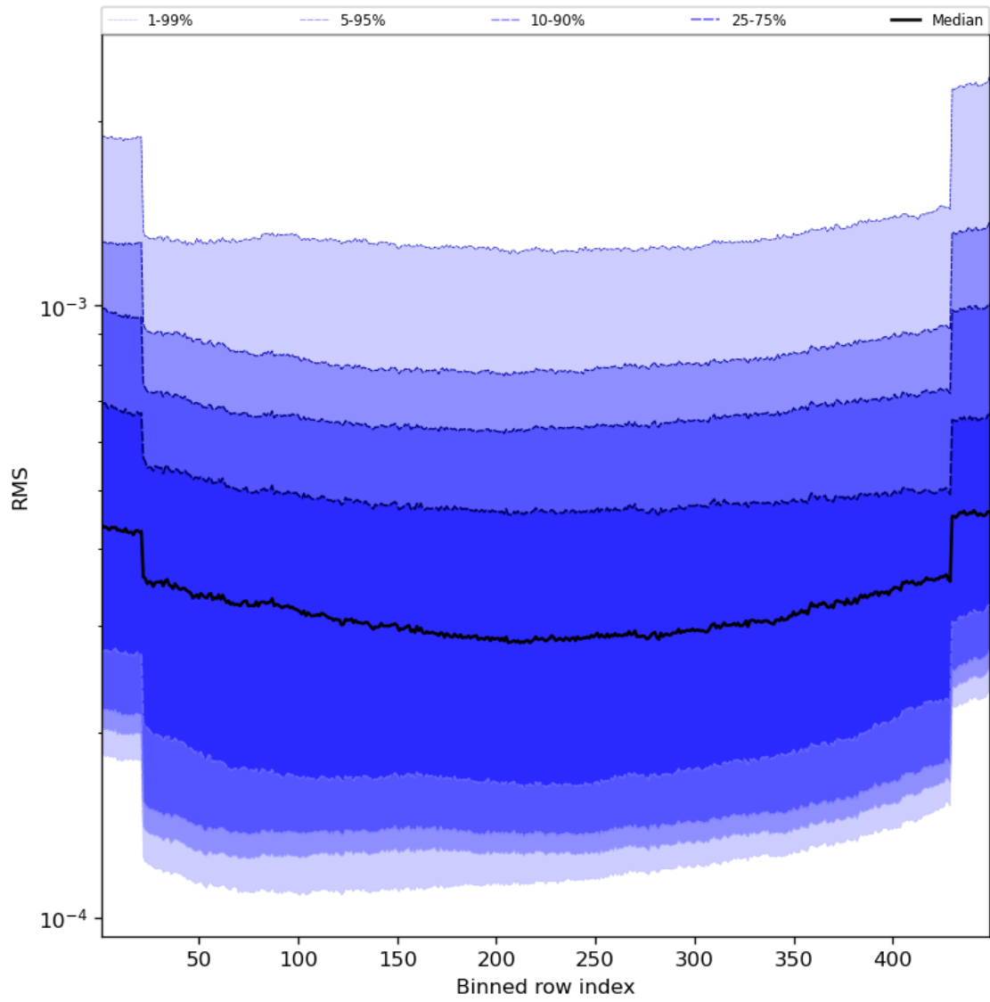
Figure 60: Along track statistics of “RMS” for 2024-02-13 to 2024-02-15
