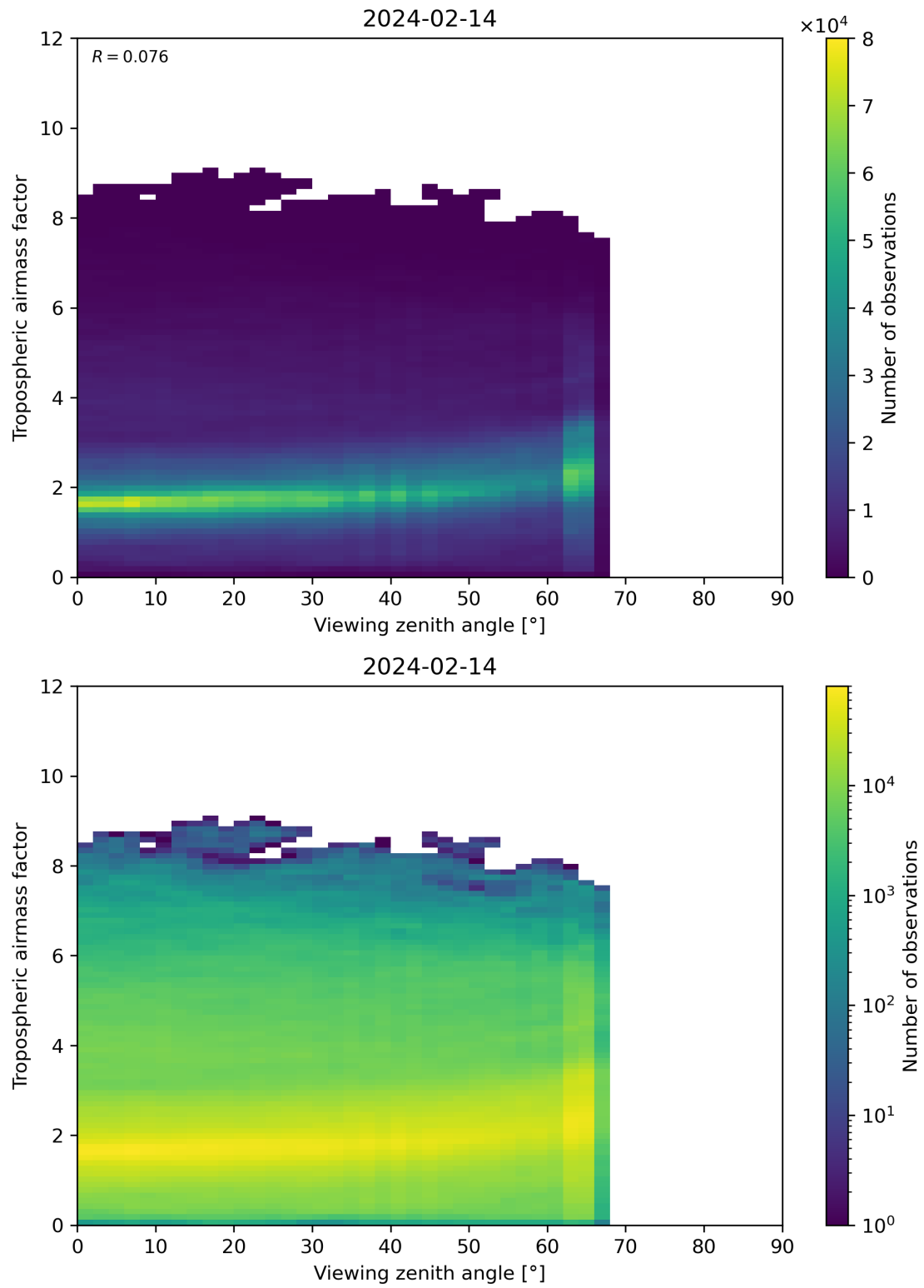
Figure 161: Scatter density plot of “Viewing zenith angle” against “Tropospheric airmass factor” for 2024-02-13 to 2024-02-15.
