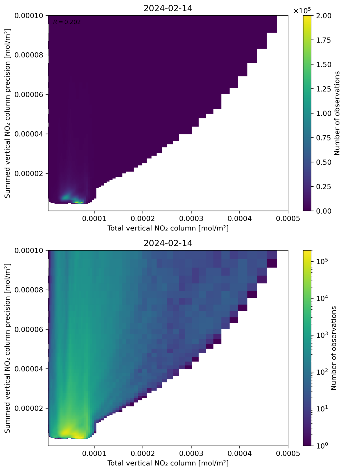
Figure 113: Scatter density plot of “Total vertical NO 2 column” against “Summed vertical NO 2 column precision” for 2024-02-13 to 2024-02-15.
