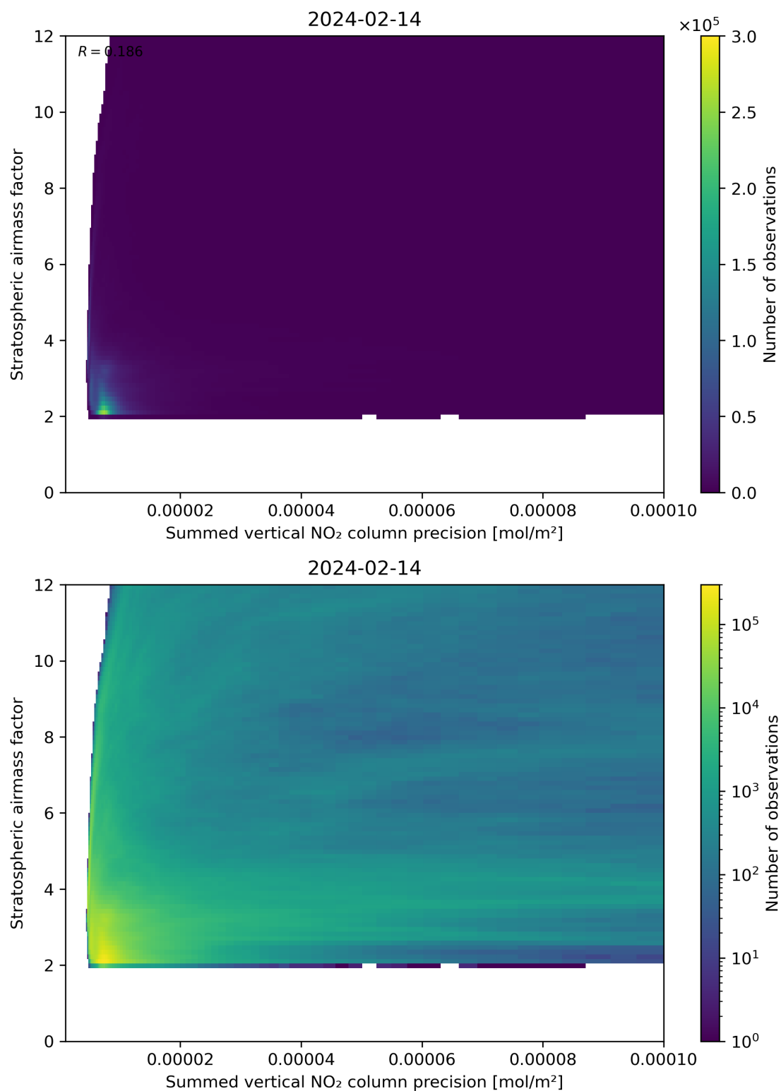
Figure 106: Scatter density plot of “Summed vertical NO 2 column precision” against “Stratospheric airmass factor” for 2024-02-13 to 2024-02-15.
