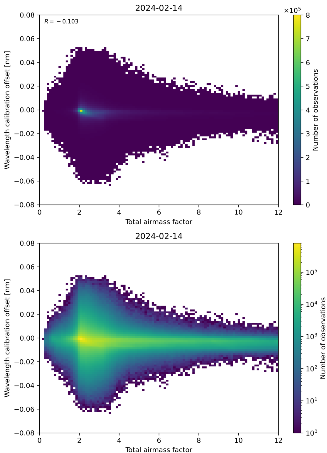
Figure 70: Scatter density plot of “Total airmass factor” against “Wavelength calibration offset” for 2024-02-13 to 2024-02-15.
