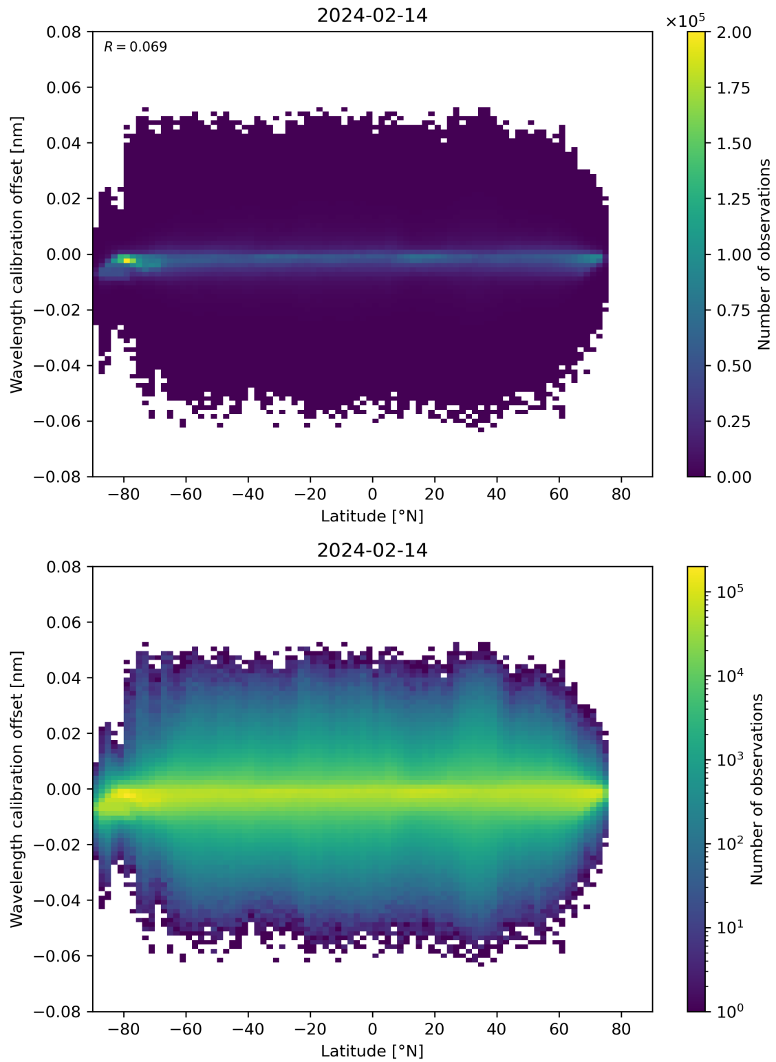
Figure 95: Scatter density plot of “Latitude” against “Wavelength calibration offset” for 2024-02-13 to 2024-02-15.
