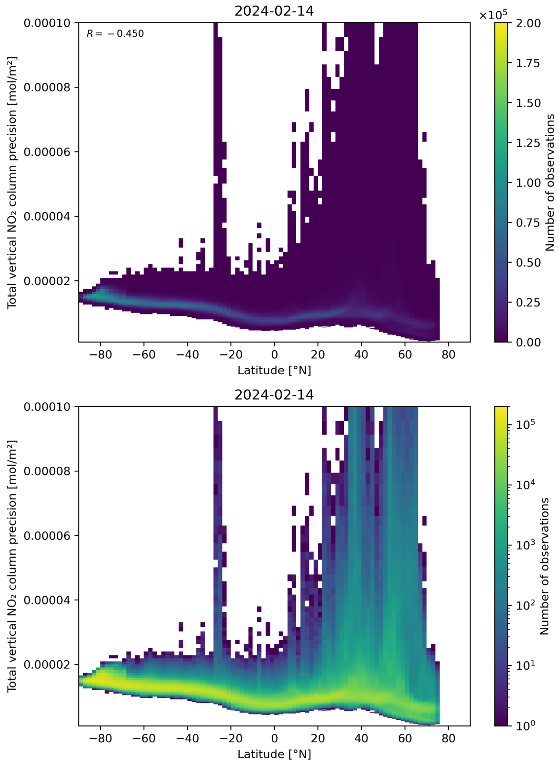
Figure 91: Scatter density plot of “Latitude” against “Total vertical NO 2 column precision” for 2024-02-13 to 2024-02-15.
