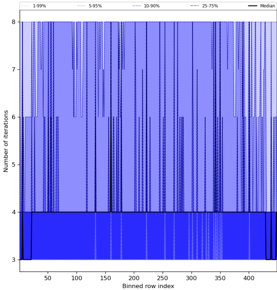
Figure 51: Along track statistics of “Number of iterations” for 2024-02-13 to 2024-02-15
