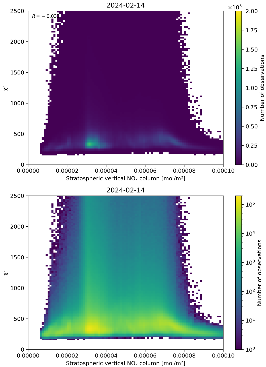
Figure 97: Scatter density plot of “Stratospheric vertical NO 2 column” against “ \chi^2 ” for 2024-02-13 to 2024-02-15.
