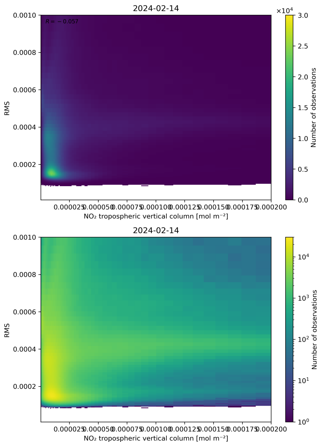
Figure 142: Scatter density plot of “NO 2 tropospheric vertical column” against “RMS” for 2024-02-13 to 2024-02-15.
