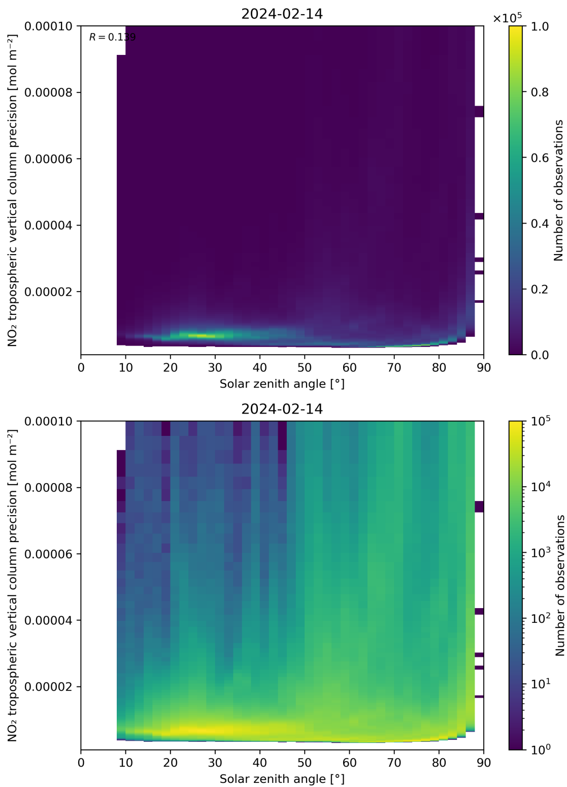
Figure 156: Scatter density plot of “Solar zenith angle” against “NO 2 tropospheric vertical column precision” for 2024-02-13 to 2024-02-15.
