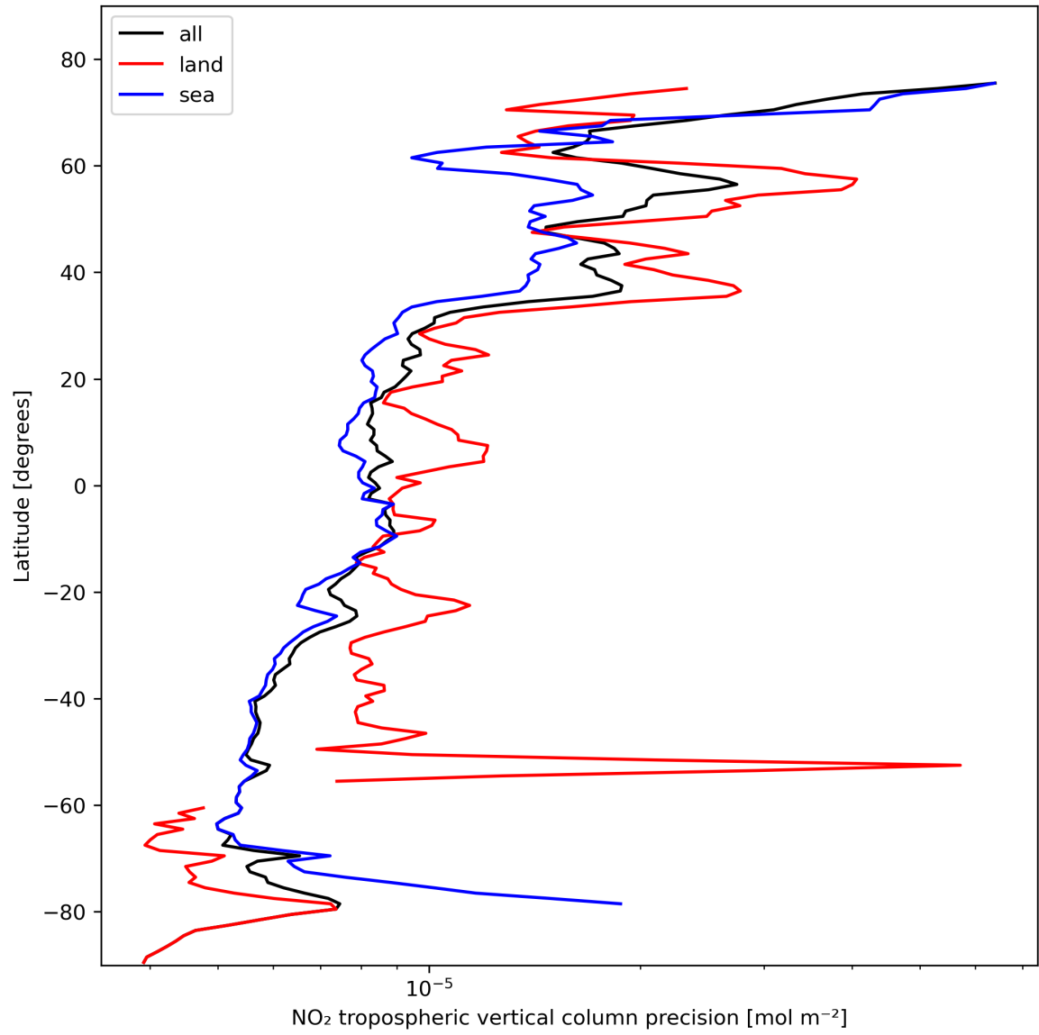
Figure 13: Zonal average of “NO 2 tropospheric vertical column precision” for 2024-02-13 to 2024-02-15.
