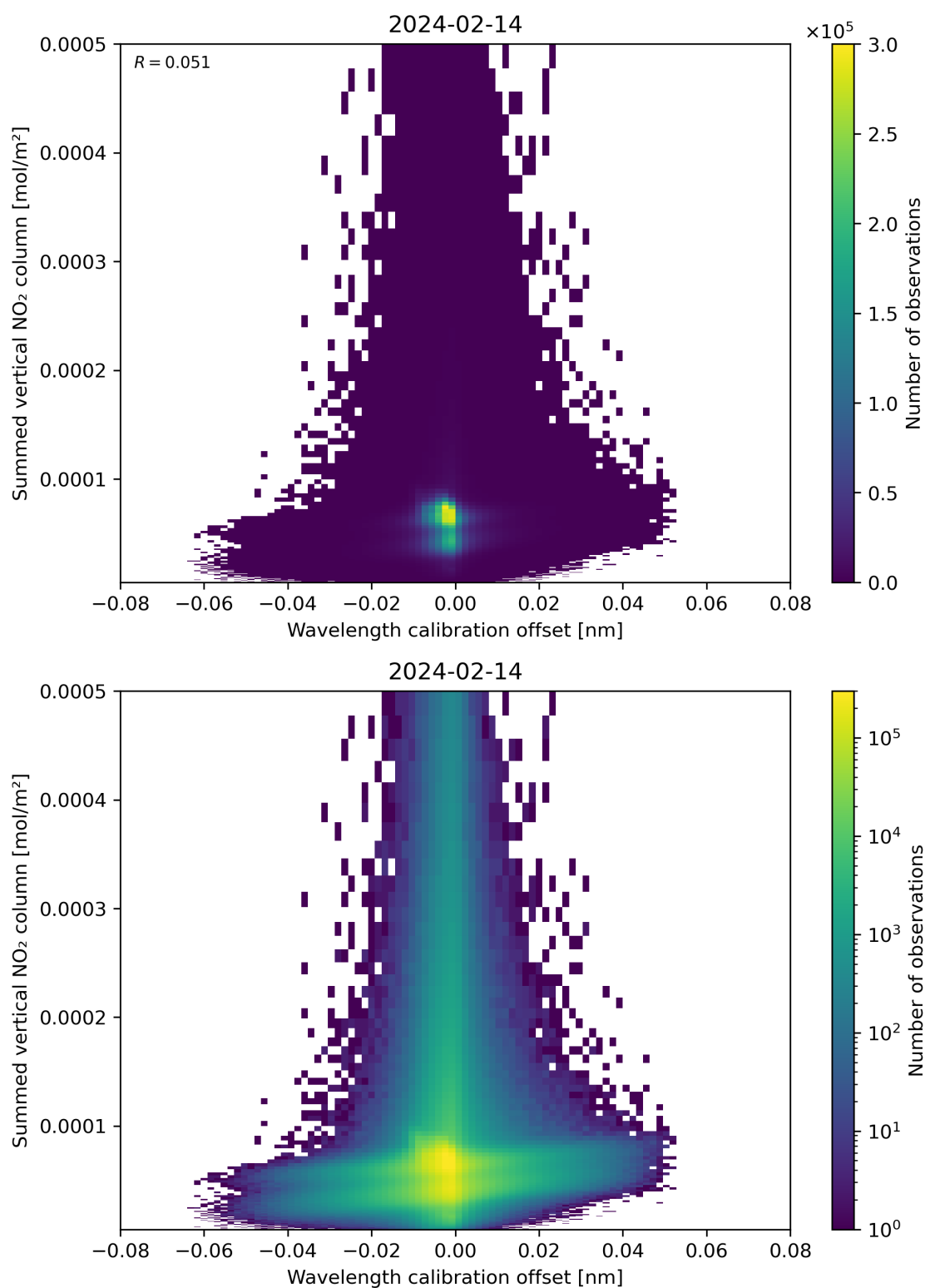
Figure 177: Scatter density plot of “Wavelength calibration offset” against “Summed vertical NO 2 column” for 2024-02-13 to 2024-02-15.
