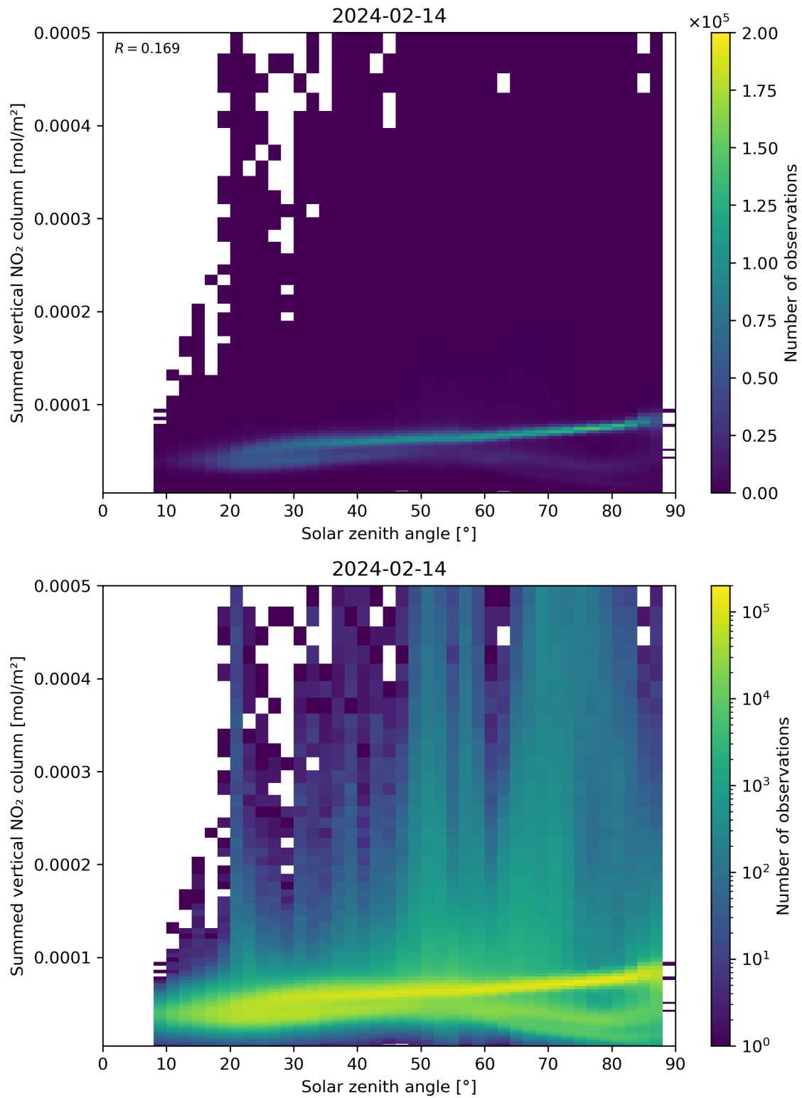
Figure 151: Scatter density plot of “Solar zenith angle” against “Summed vertical NO 2 column” for 2024-02-13 to 2024-02-15.
