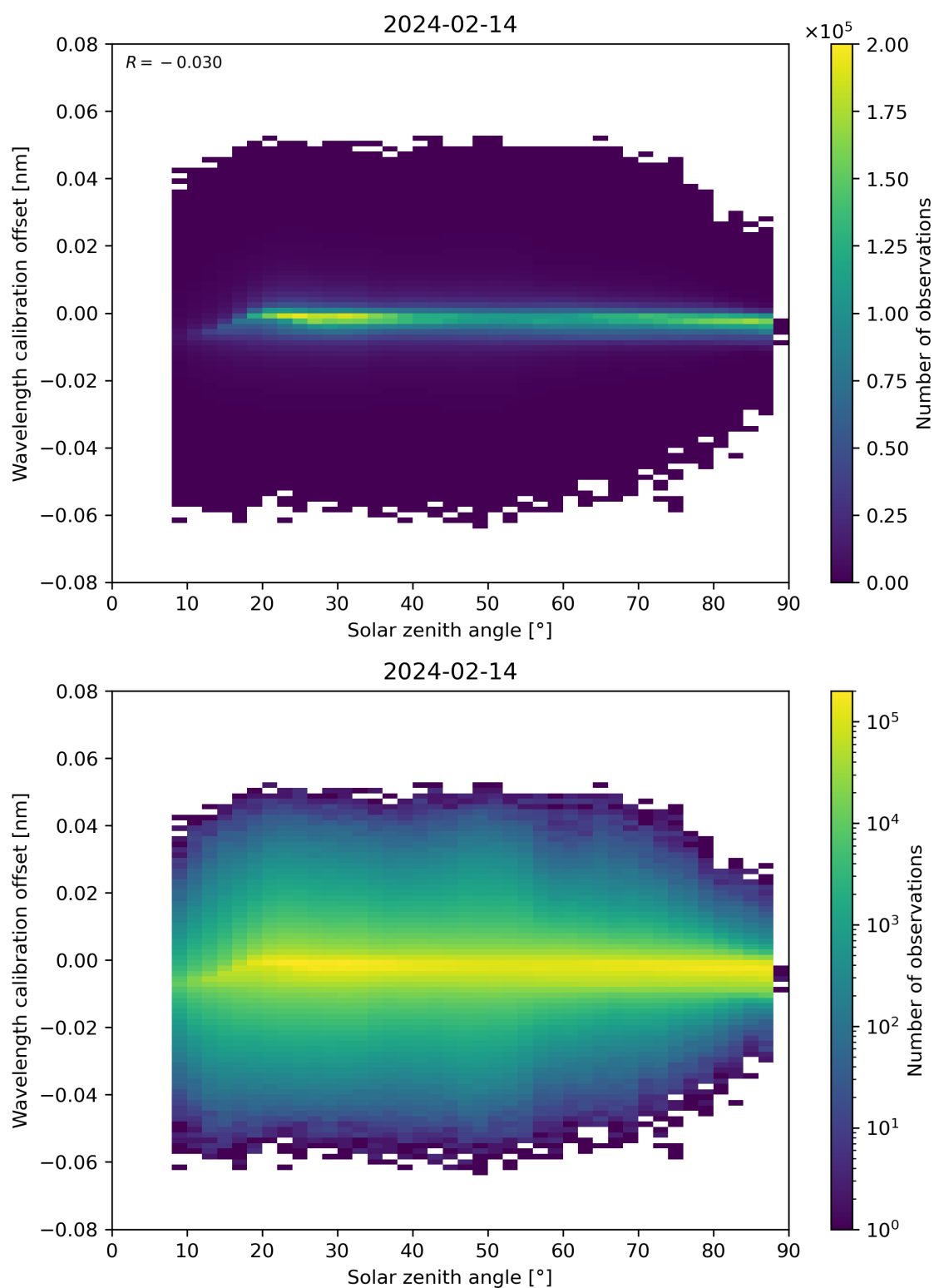
Figure 158: Scatter density plot of “Solar zenith angle” against “Wavelength calibration offset” for 2024-02-13 to 2024-02-15.
