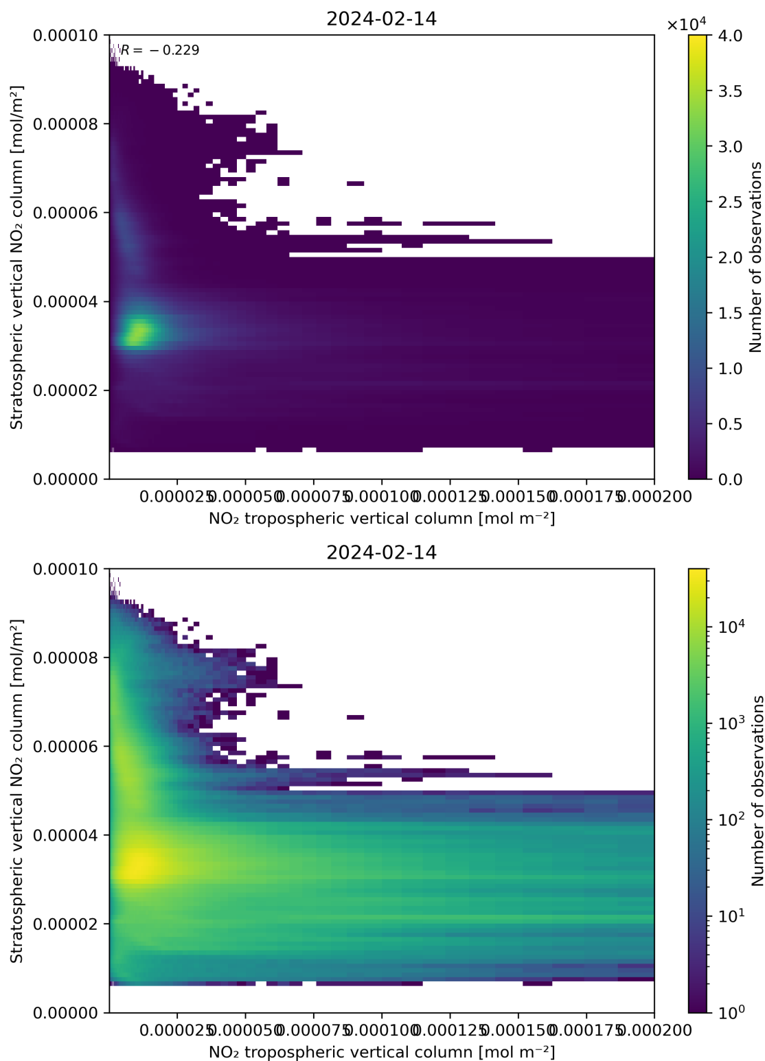
Figure 125: Scatter density plot of “NO 2 tropospheric vertical column” against “Stratospheric vertical NO 2 column” for 2024-02-13 to 2024-02-15.
