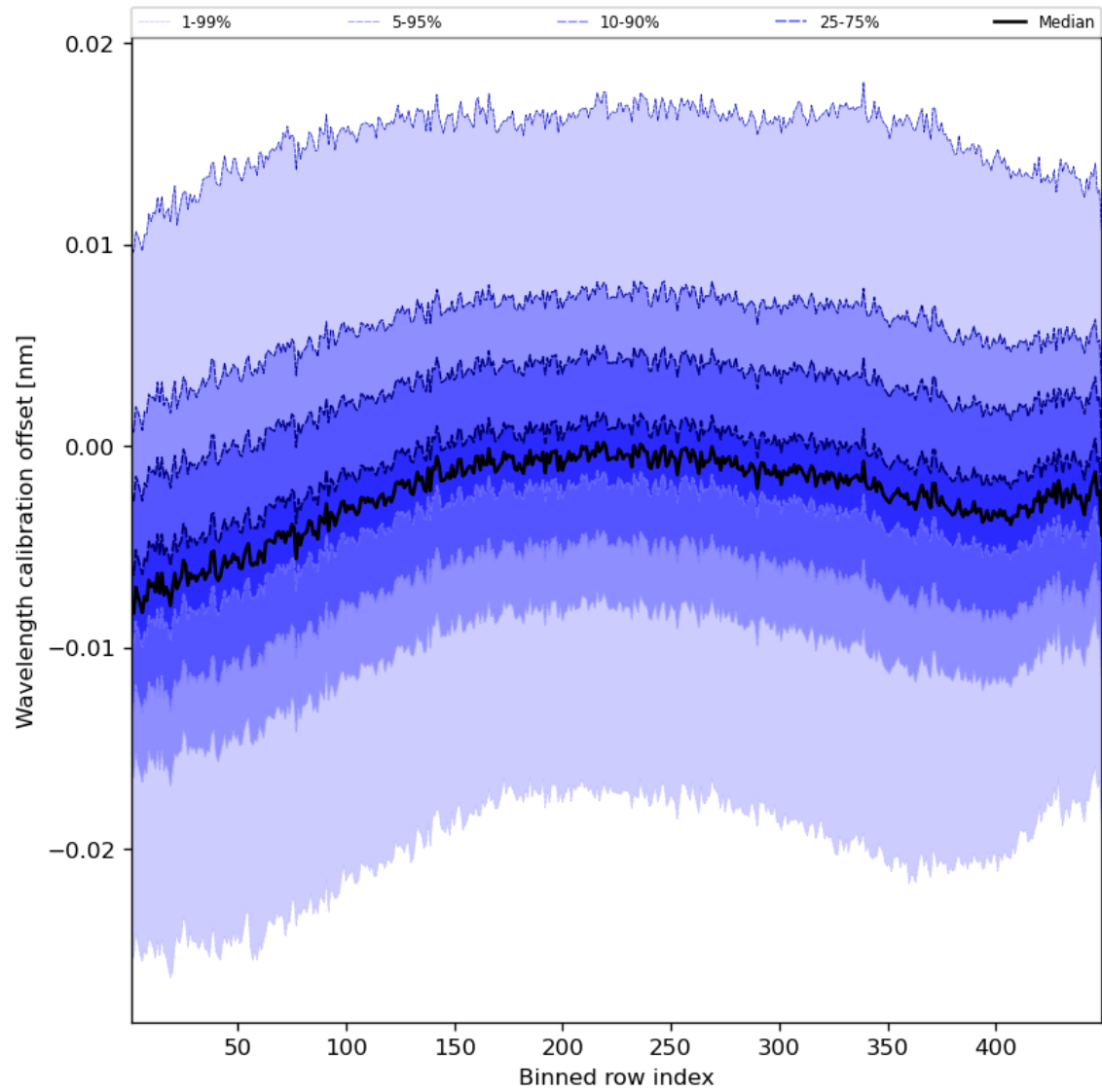
Figure 52: Along track statistics of “Wavelength calibration offset” for 2024-02-13 to 2024-02-15
