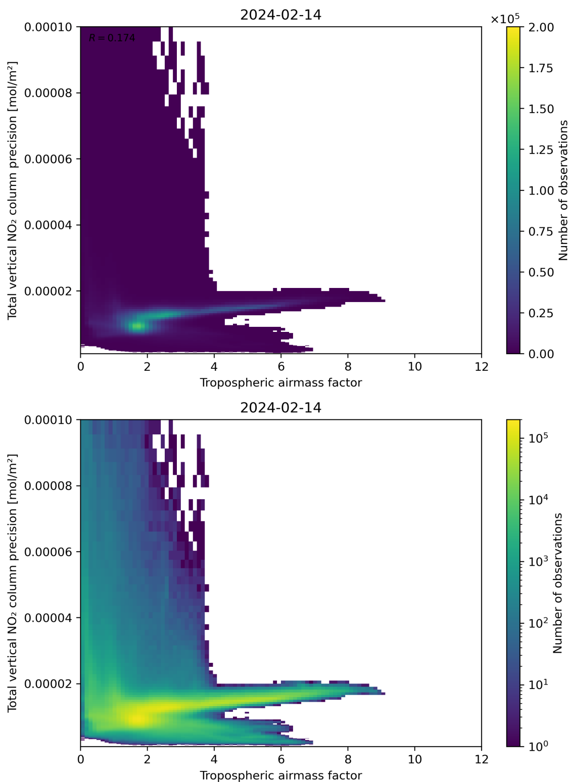
Figure 78: Scatter density plot of “Tropospheric air mass factor” against “Total vertical NO 2 column precision” for 2024-02-13 to 2024-02-15.
