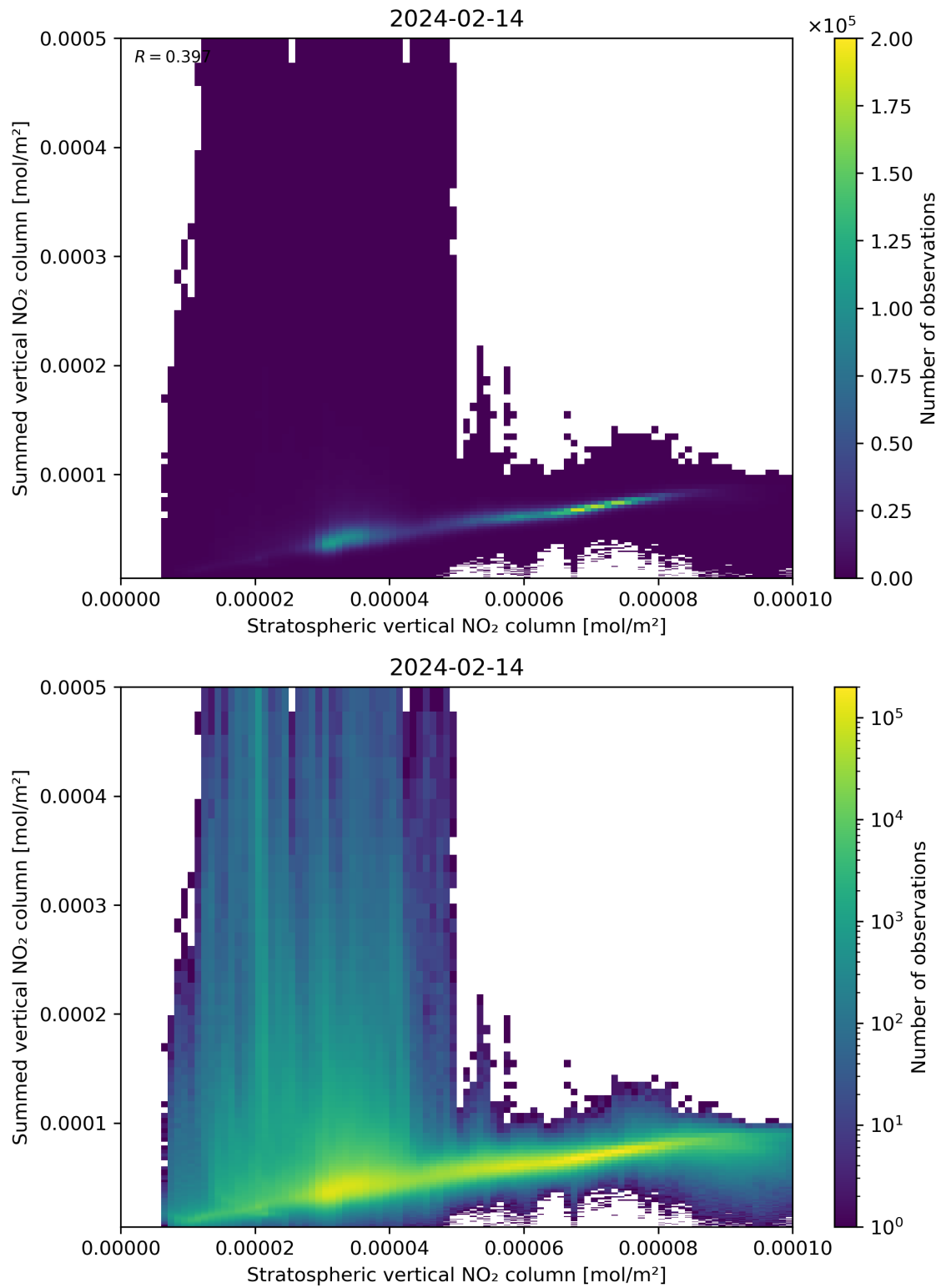
Figure 98: Scatter density plot of “Stratospheric vertical NO 2 column” against “Summed vertical NO 2 column” for 2024-02-13 to 2024-02-15.
