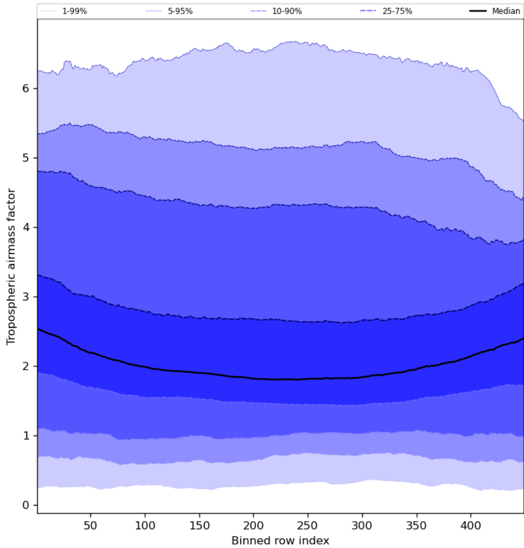
Figure 48: Along track statistics of “Tropospheric air mass factor” for 2024-02-13 to 2024-02-15
