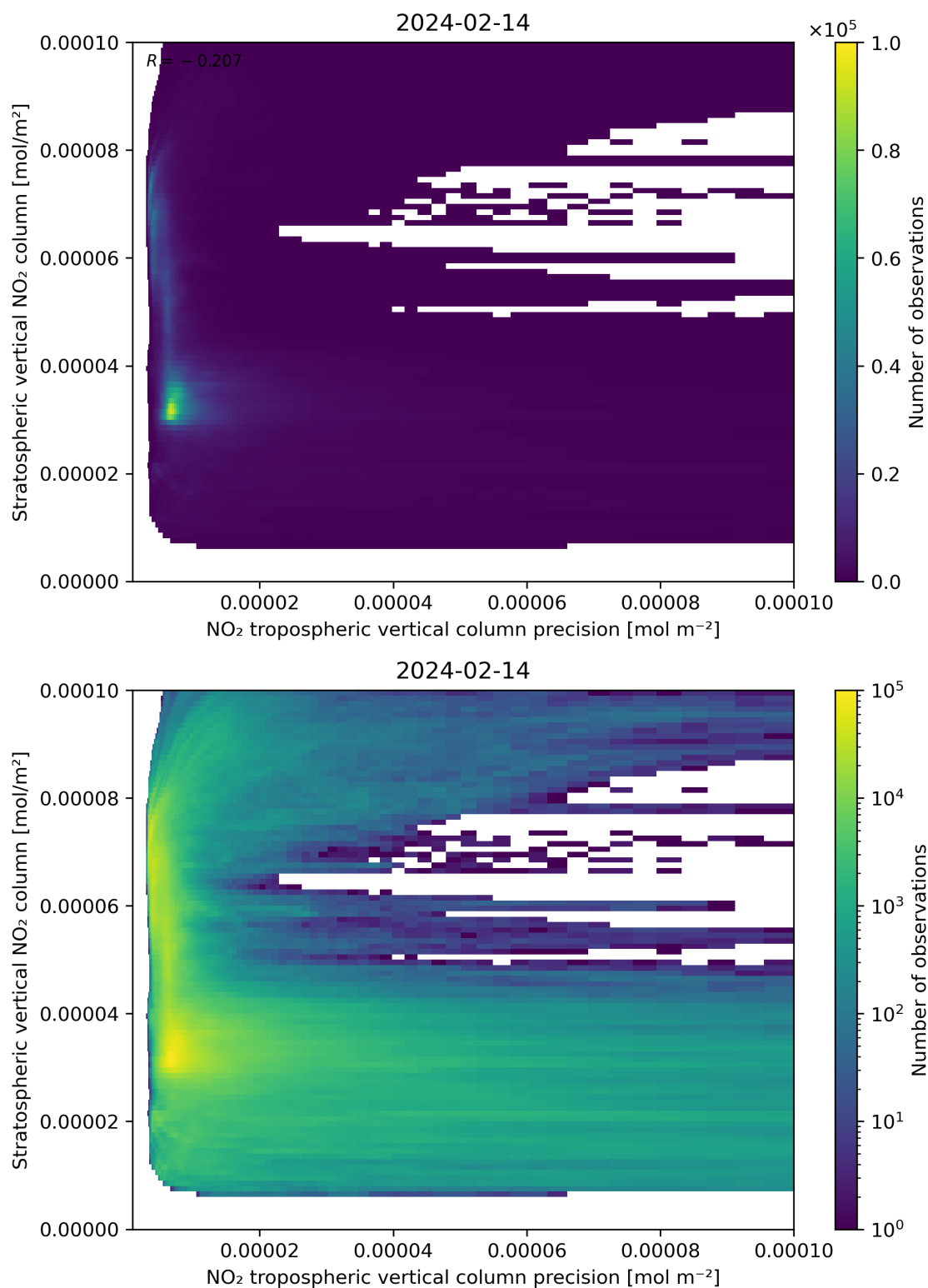
Figure 135: Scatter density plot of “NO 2 tropospheric vertical column precision” against “Stratospheric vertical NO 2 column” for 2024-02-13 to 2024-02-15.
