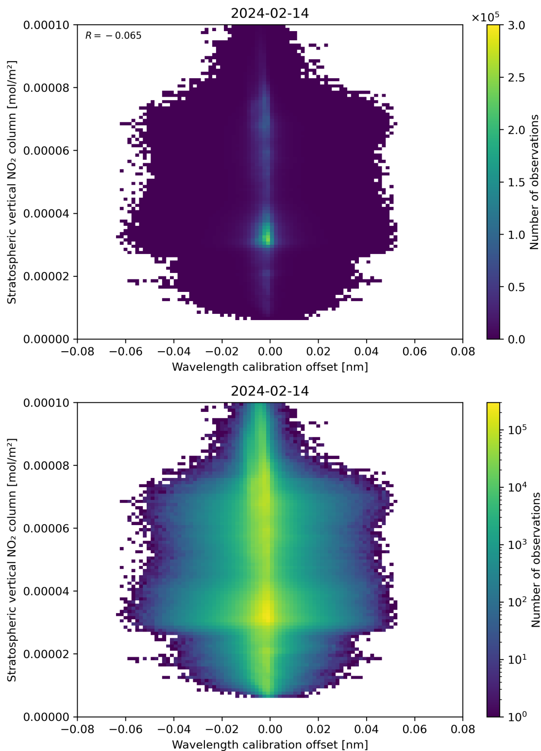
Figure 176: Scatter density plot of “Wavelength calibration offset” against “Stratospheric vertical NO 2 column” for 2024-02-13 to 2024-02-15.
