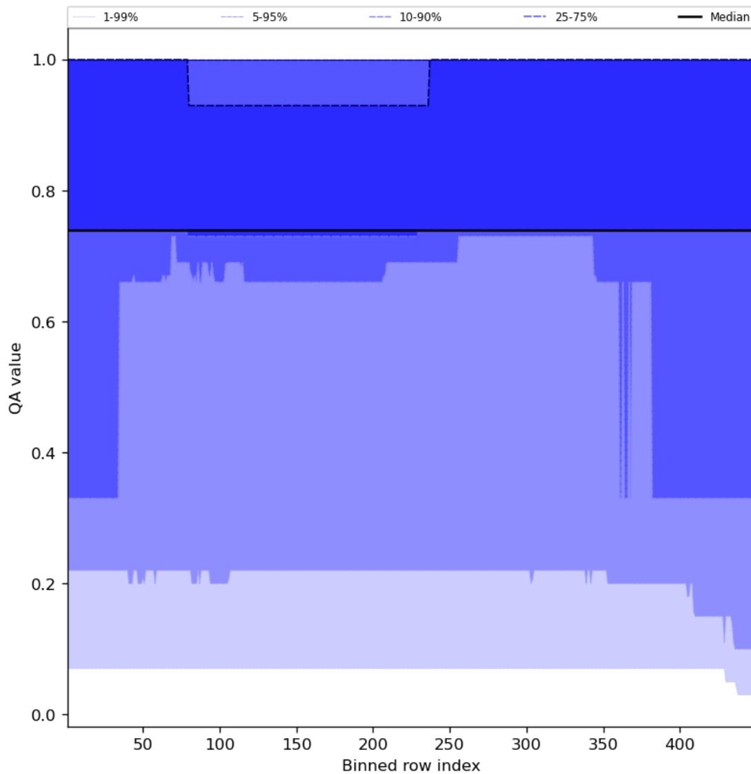
Figure 45: Along track statistics of “QA value” for 2024-02-13 to 2024-02-15
