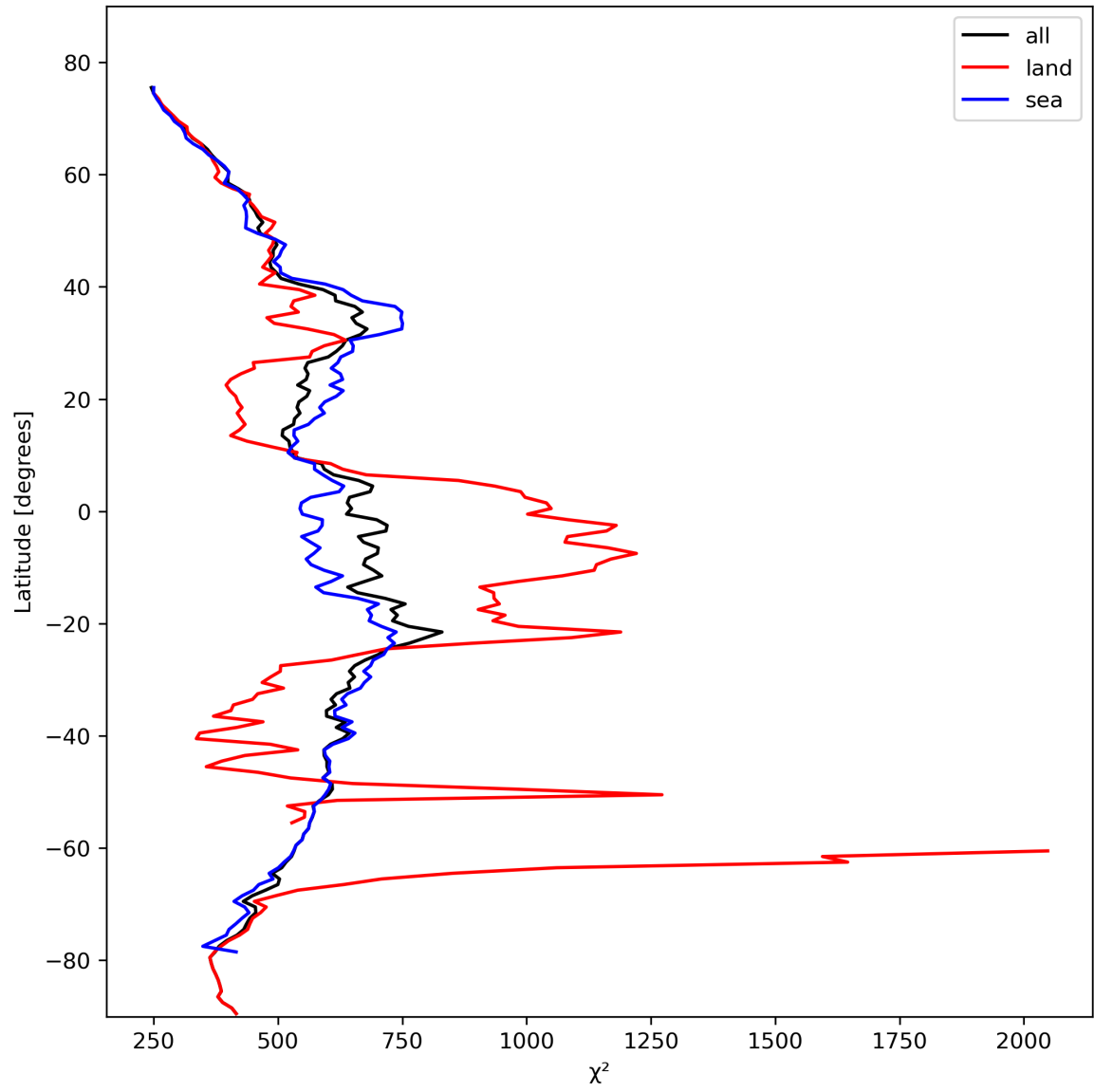
Figure 25: Zonal average of “ \chi^2 ” for 2024-02-13 to 2024-02-15.
