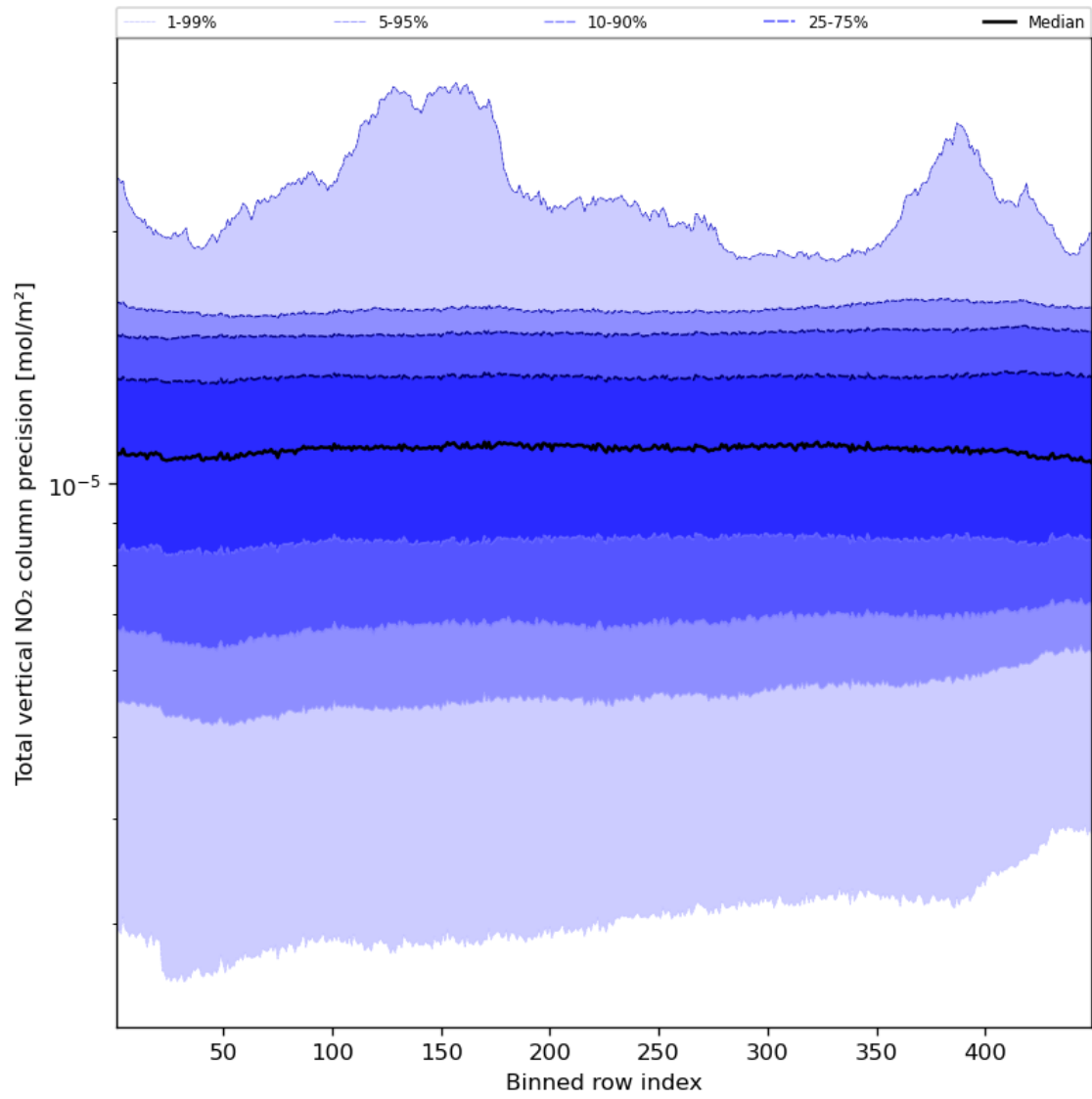
Figure 56: Along track statistics of “Total vertical NO 2 column precision” for 2024-02-13 to 2024-02-15
