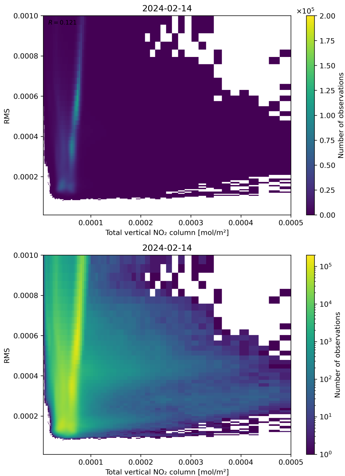
Figure 120: Scatter density plot of “Total vertical NO 2 column” against “RMS” for 2024-02-13 to 2024-02-15.
