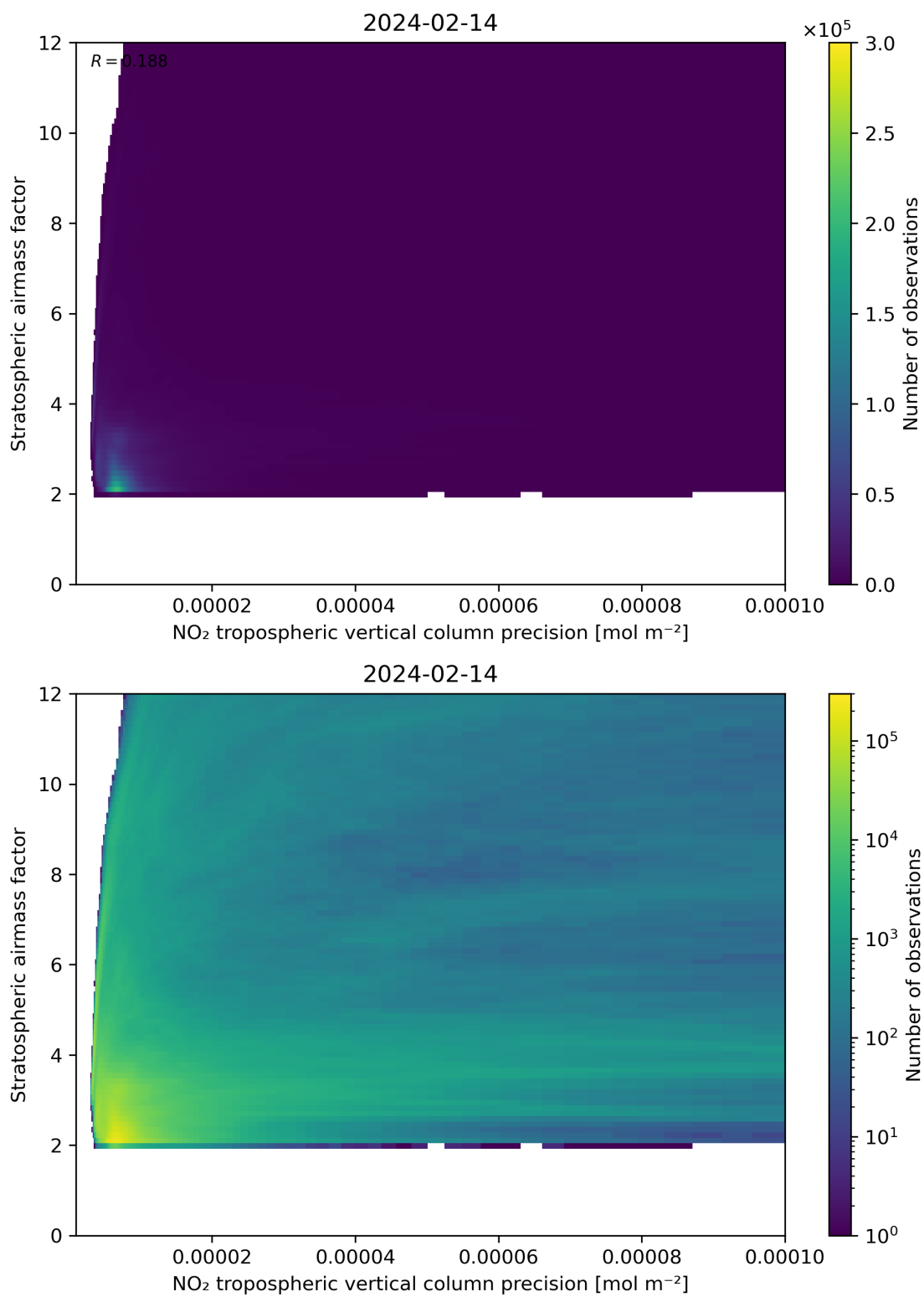
Figure 131: Scatter density plot of “NO 2 tropospheric vertical column precision” against “Stratospheric airmass factor” for 2024-02-13 to 2024-02-15.
