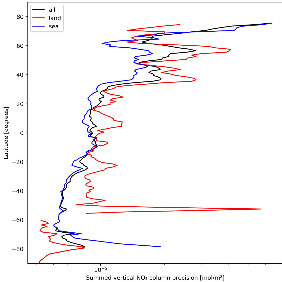
Figure 24: Zonal average of “Summed vertical NO 2 column precision” for 2024-02-13 to 2024-02-15.
