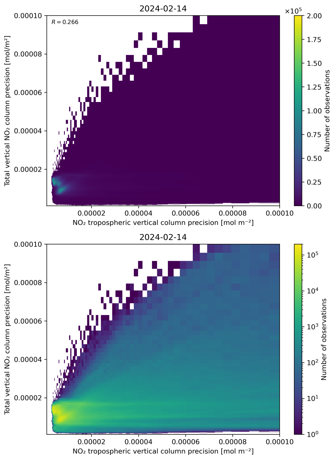
Figure 139: Scatter density plot of “NO 2 tropospheric vertical column precision” against “Total vertical NO 2 column precision” for 2024-02-13 to 2024-02-15.
