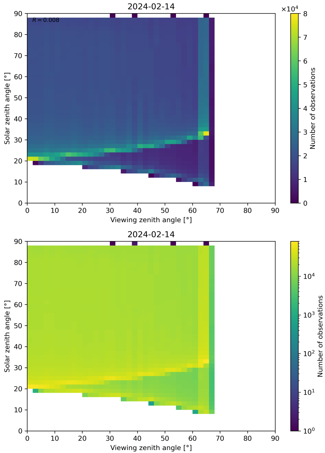
Figure 172: Scatter density plot of “Viewing zenith angle” against “Solar zenith angle” for 2024-02-13 to 2024-02-15.
