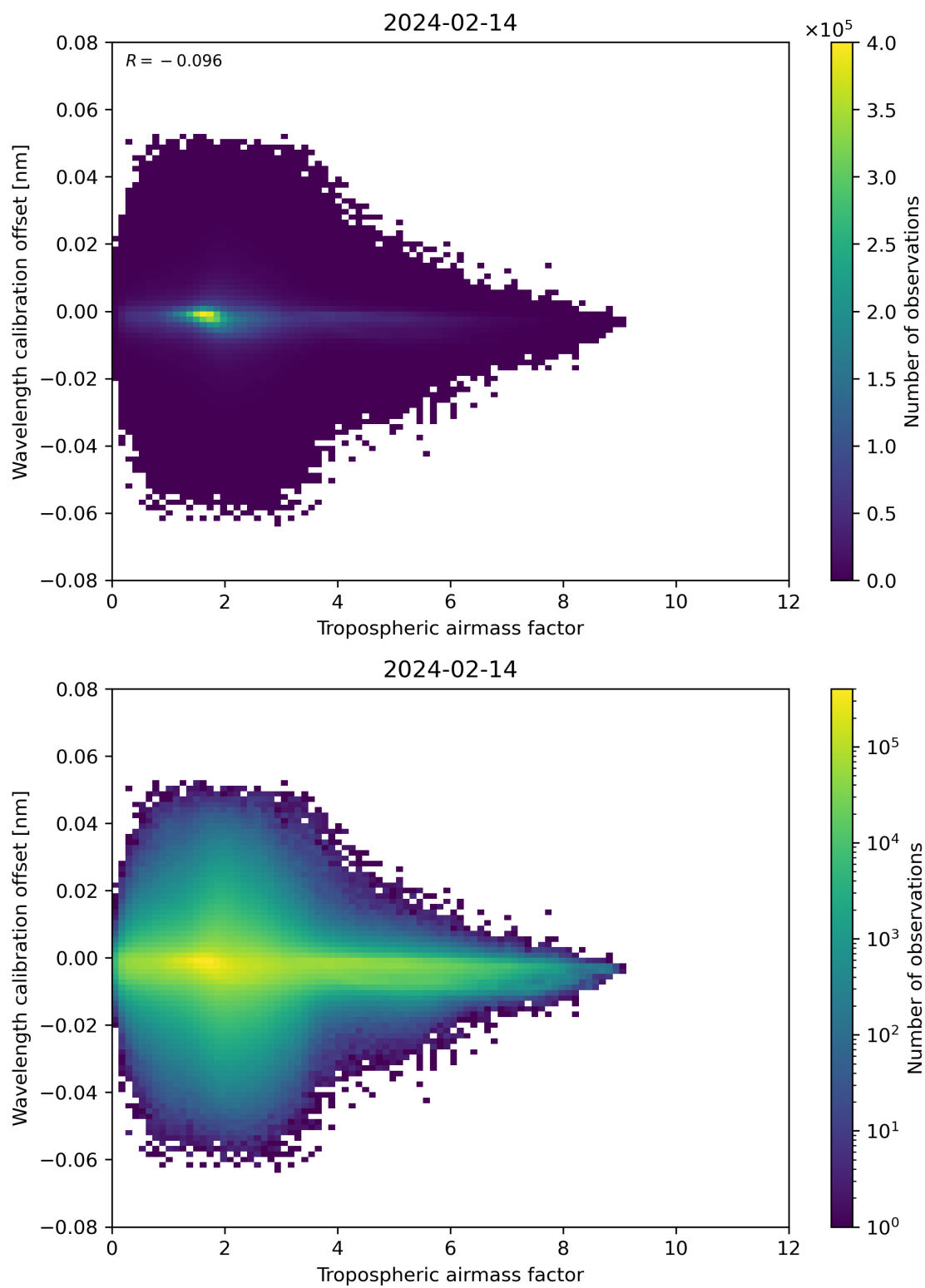
Figure 80: Scatter density plot of “Tropospheric airmass factor” against “Wavelength calibration offset” for 2024-02-13 to 2024-02-15.
