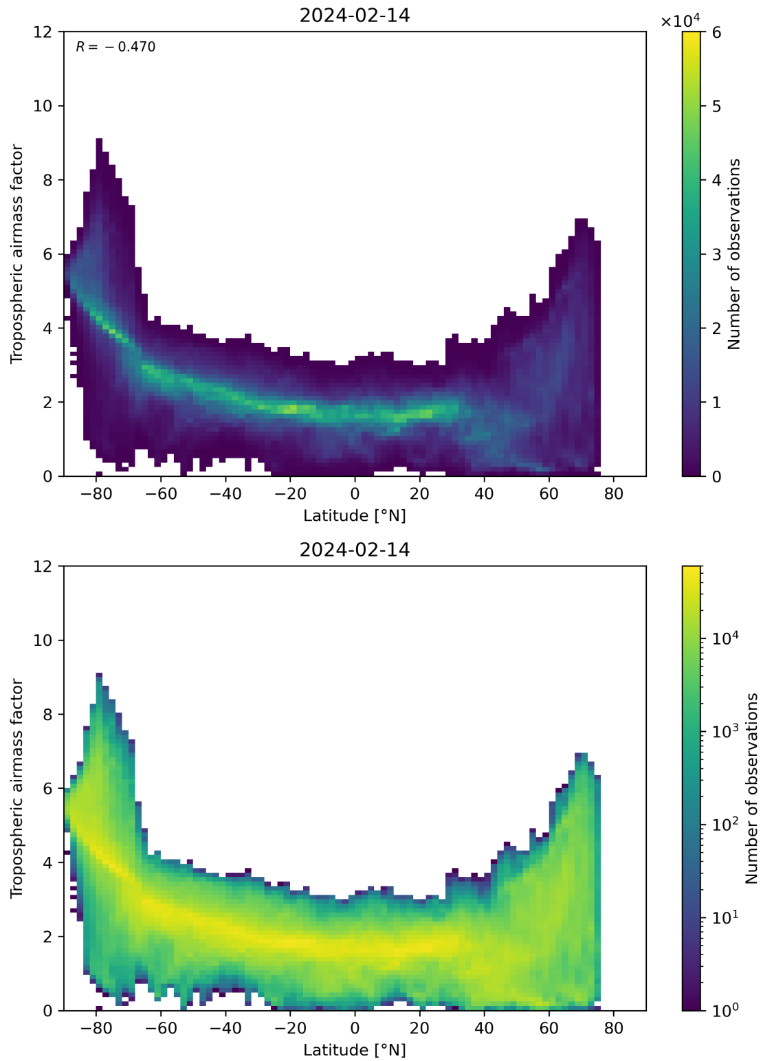
Figure 85: Scatter density plot of “Latitude” against “Tropospheric airmass factor” for 2024-02-13 to 2024-02-15.
