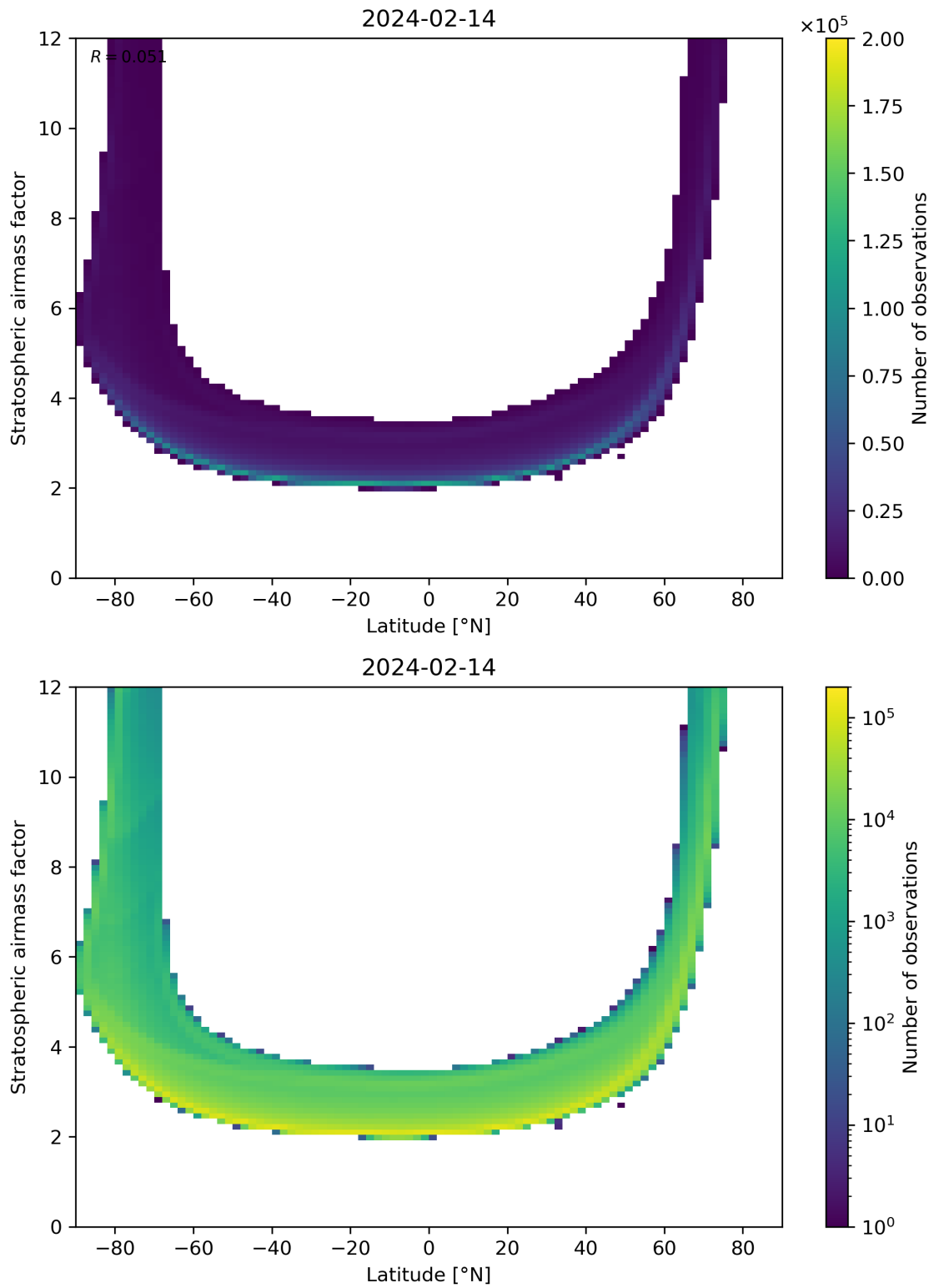
Figure 83: Scatter density plot of “Latitude” against “Stratospheric airmass factor” for 2024-02-13 to 2024-02-15.
