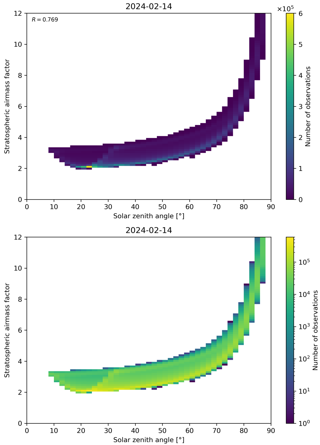
Figure 145: Scatter density plot of “Solar zenith angle” against “Stratospheric airmass factor” for 2024-02-13 to 2024-02-15.
