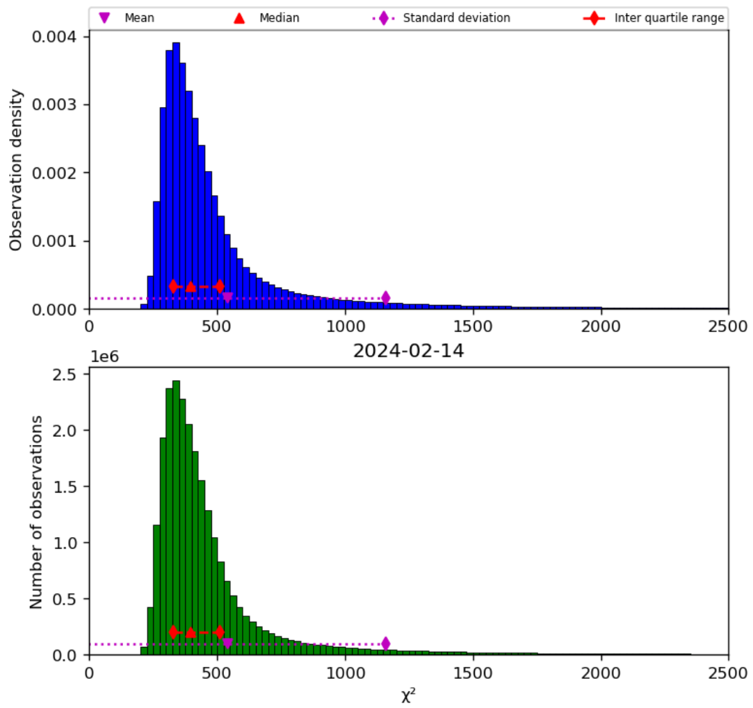
Figure 42: Histogram of “ \chi^2 ” for 2024-02-13 to 2024-02-15
