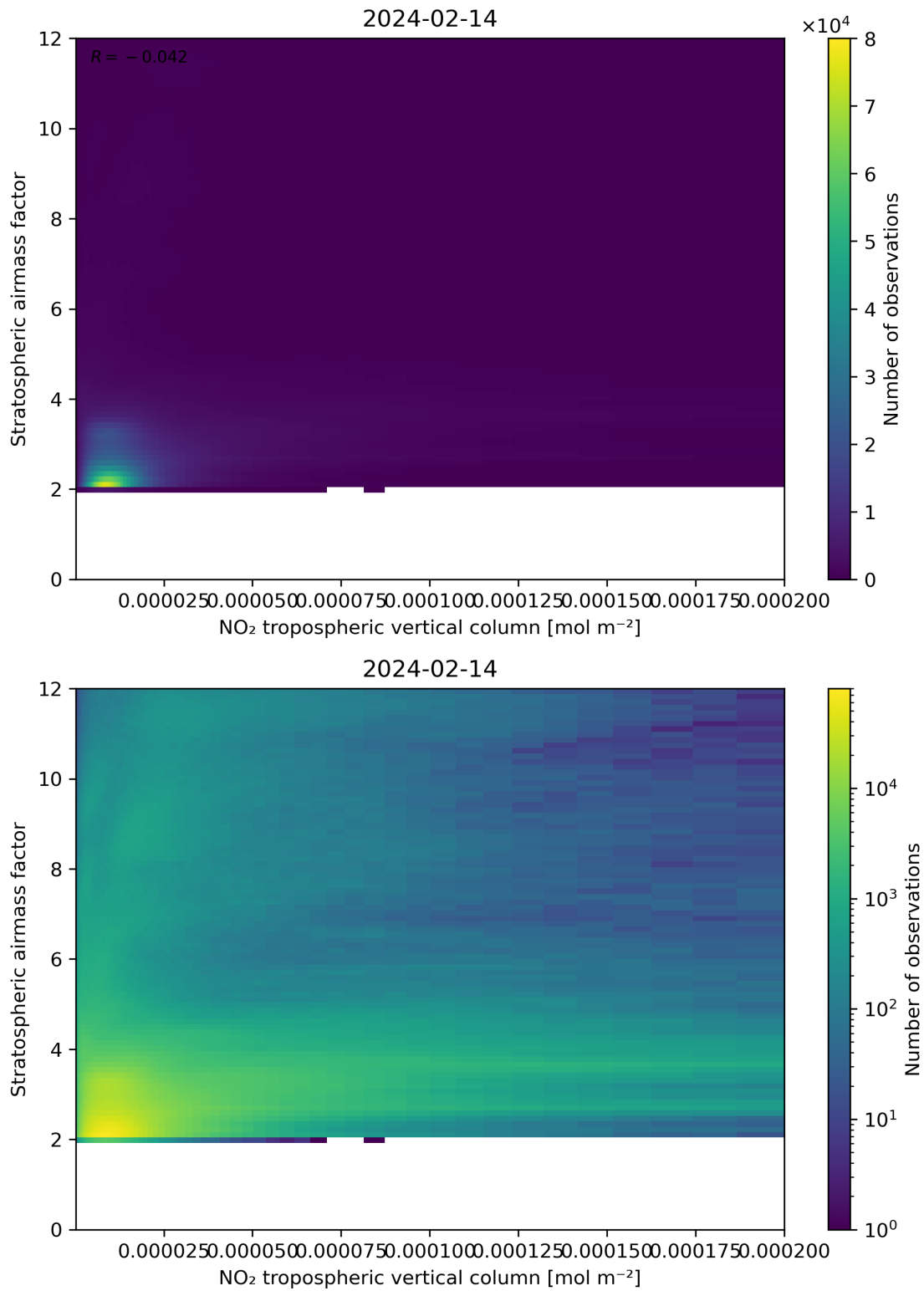
Figure 121: Scatter density plot of “NO 2 tropospheric vertical column” against “Stratospheric airmass factor” for 2024-02-13 to 2024-02-15.
