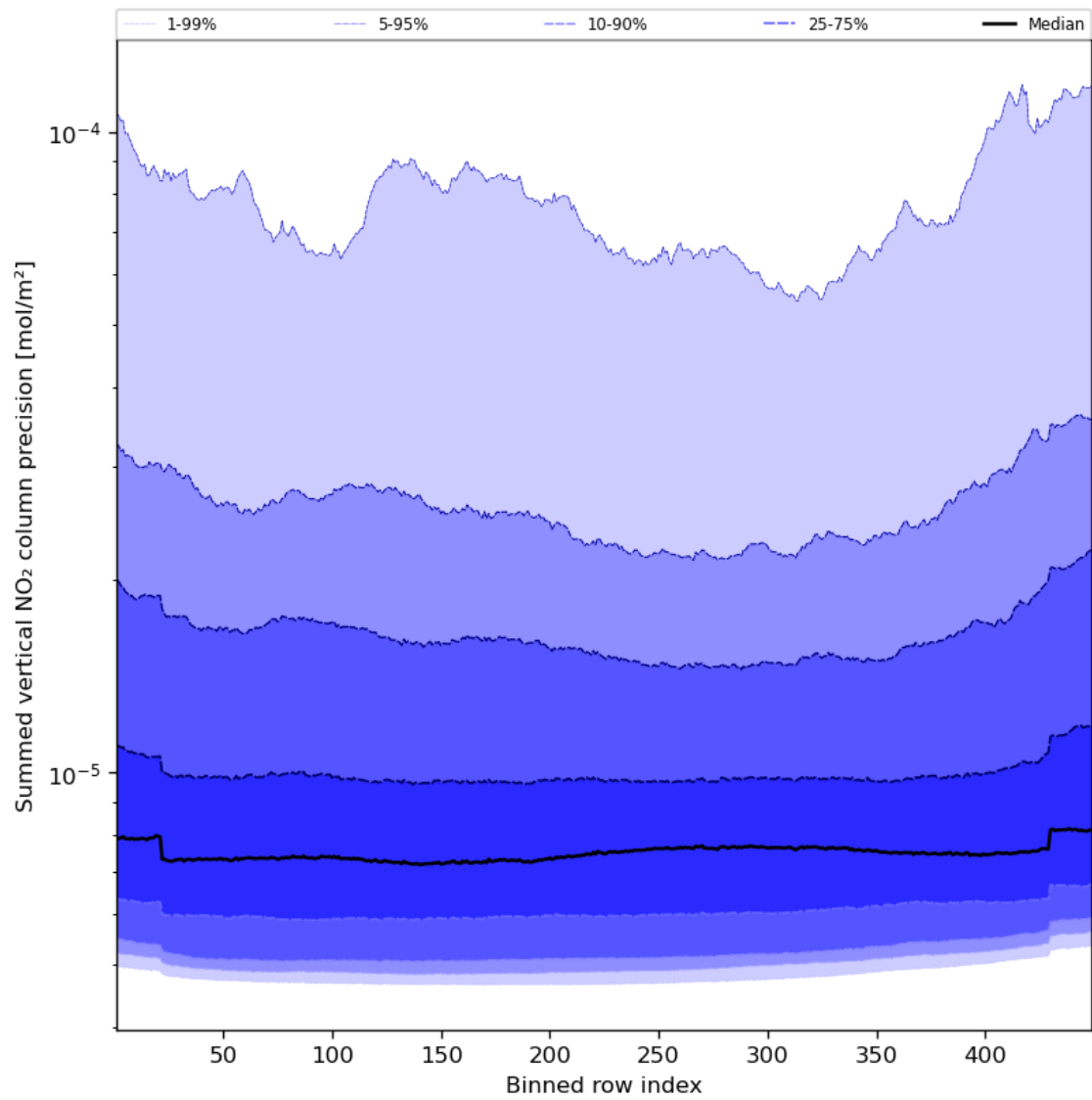
Figure 58: Along track statistics of “Summed vertical NO 2 column precision” for 2024-02-13 to 2024-02-15
