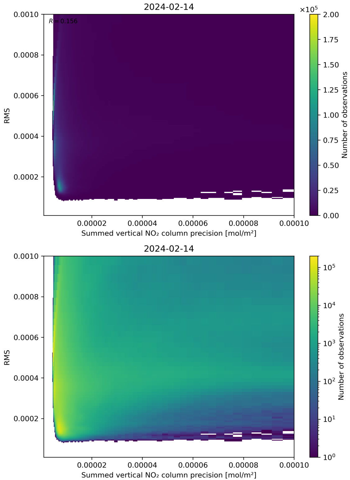
Figure 108: Scatter density plot of “Summed vertical NO 2 column precision” against “RMS” for 2024-02-13 to 2024-02-15.
