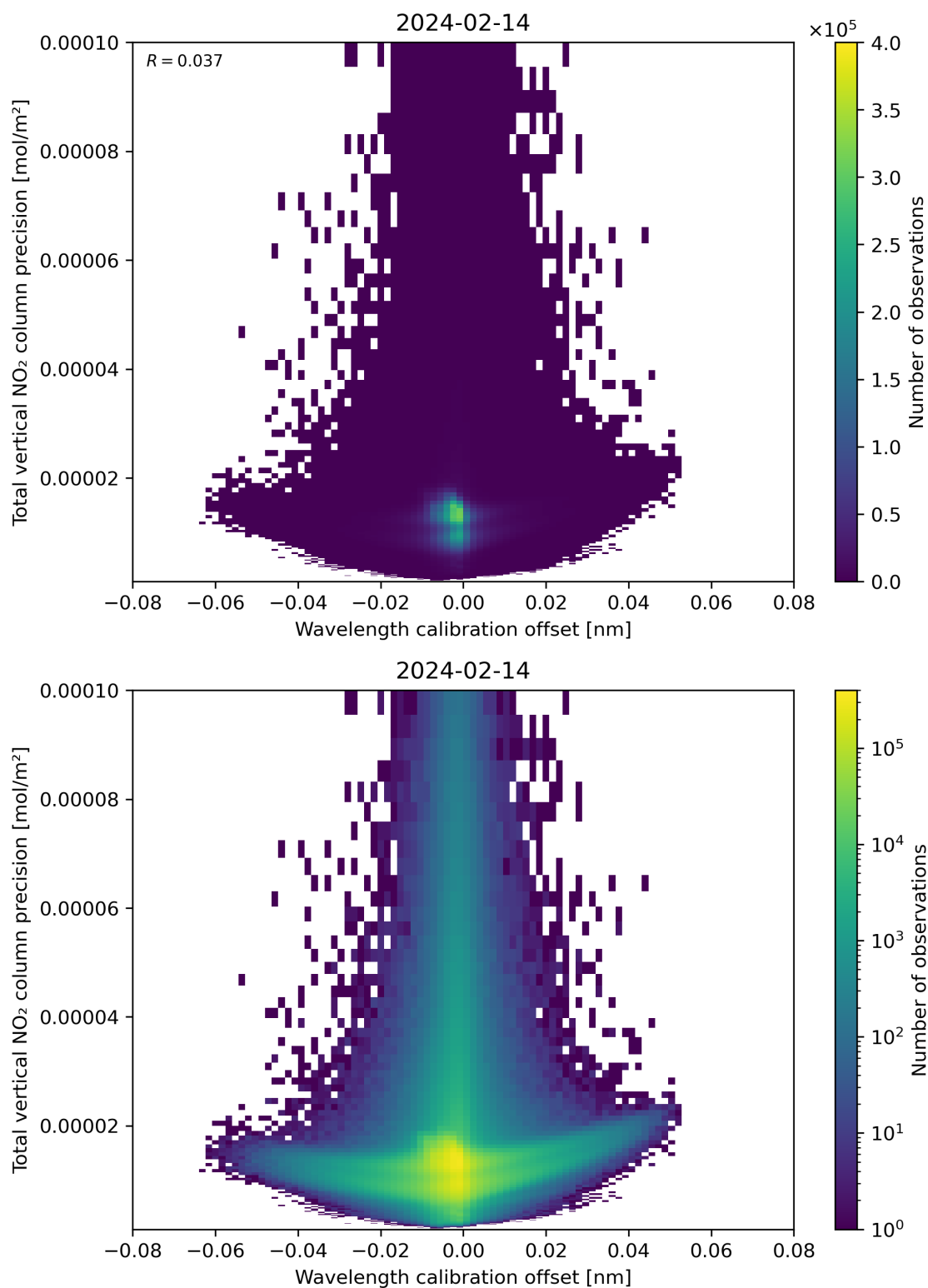
Figure 180: Scatter density plot of “Wavelength calibration offset” against “Total vertical NO 2 column precision” for 2024-02-13 to 2024-02-15.
