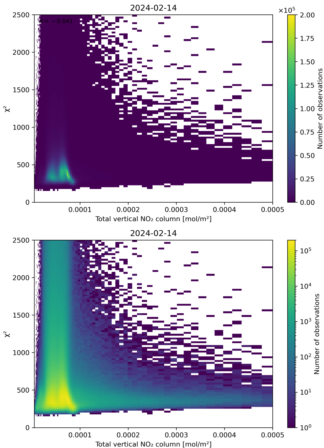
Figure 111: Scatter density plot of “Total vertical NO 2 column” against “ \chi^2 ” for 2024-02-13 to 2024-02-15.
