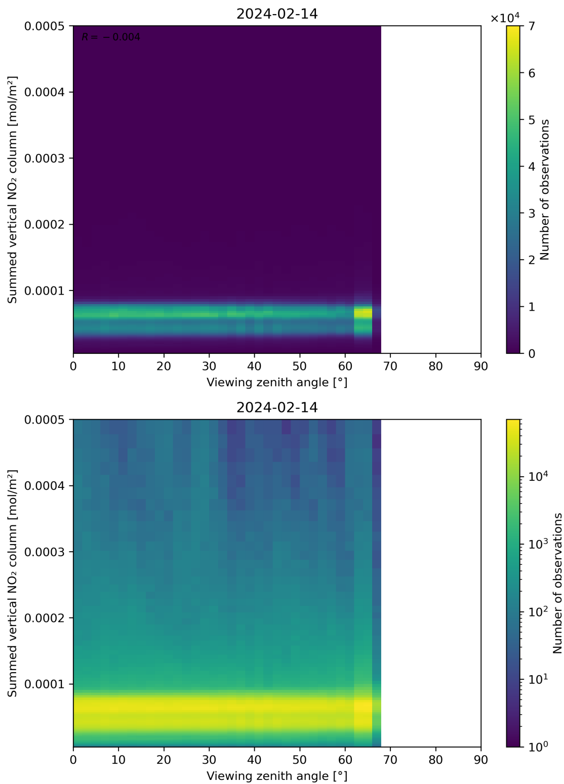
Figure 165: Scatter density plot of “Viewing zenith angle” against “Summed vertical NO 2 column” for 2024-02-13 to 2024-02-15.
