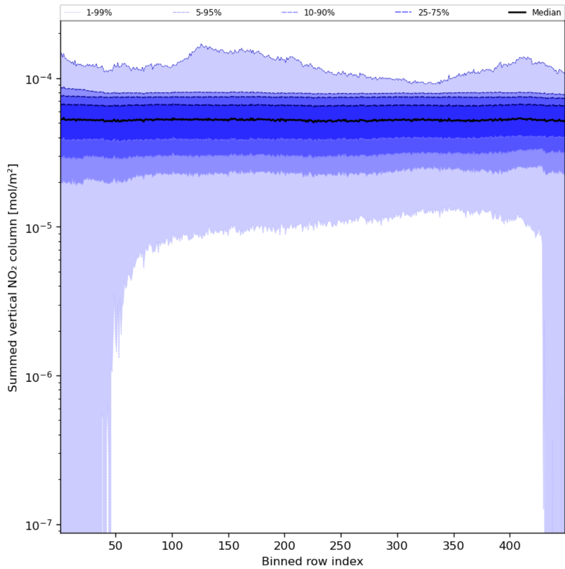
Figure 57: Along track statistics of “Summed vertical NO 2 column” for 2024-02-13 to 2024-02-15
