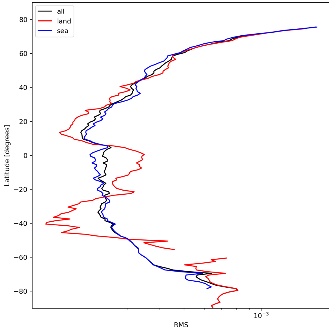
Figure 26: Zonal average of “RMS” for 2024-02-13 to 2024-02-15.
