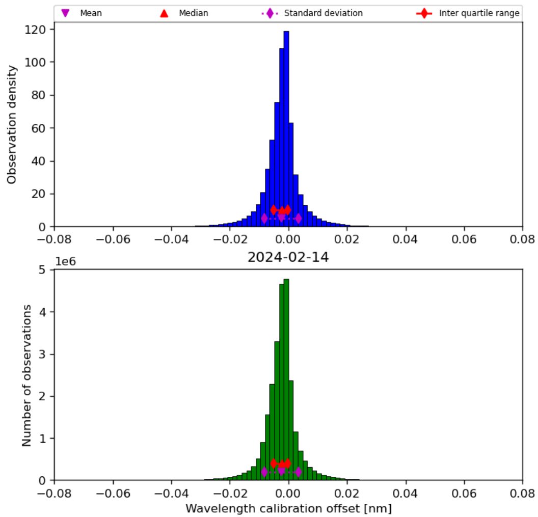
Figure 35: Histogram of “Wavelength calibration offset” for 2024-02-13 to 2024-02-15
