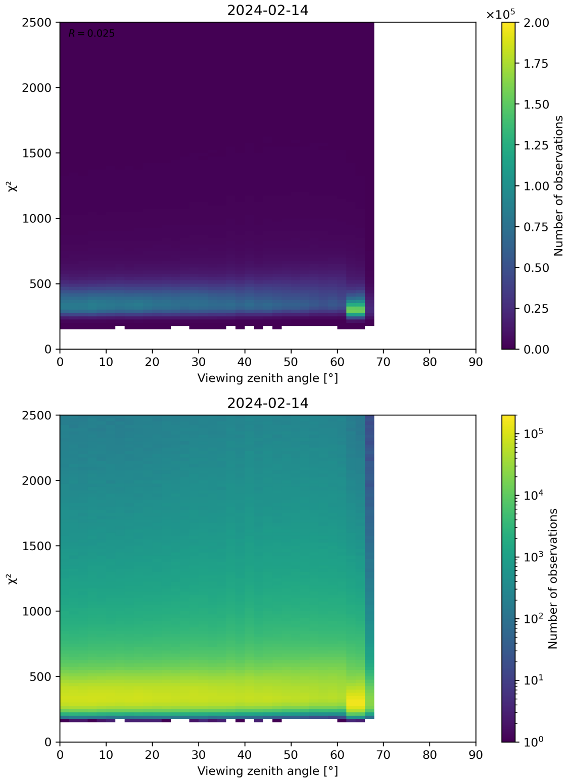
Figure 162: Scatter density plot of “Viewing zenith angle” against “ \chi^2 ” for 2024-02-13 to 2024-02-15.
