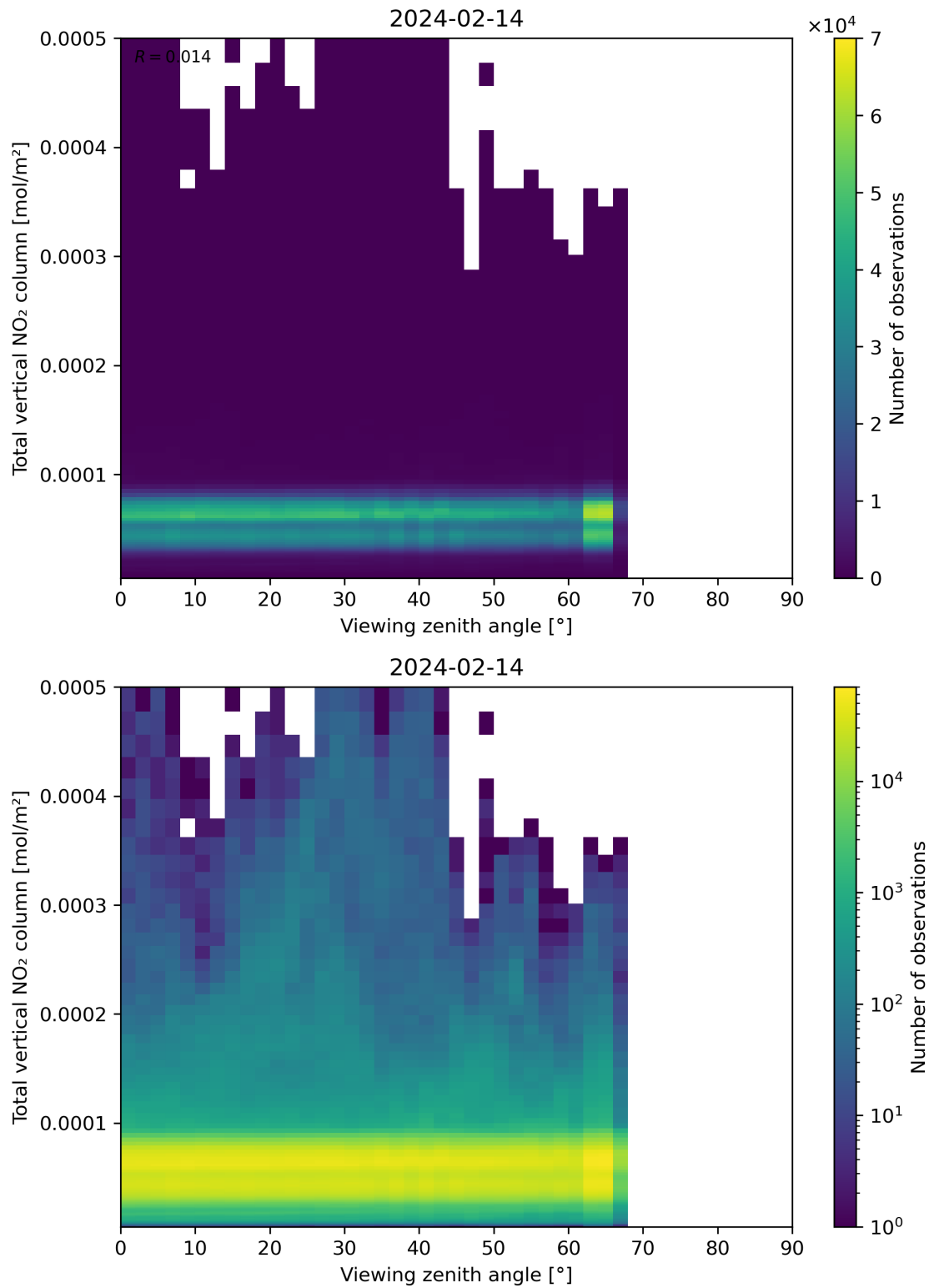
Figure 167: Scatter density plot of “Viewing zenith angle” against “Total vertical NO 2 column” for 2024-02-13 to 2024-02-15.
