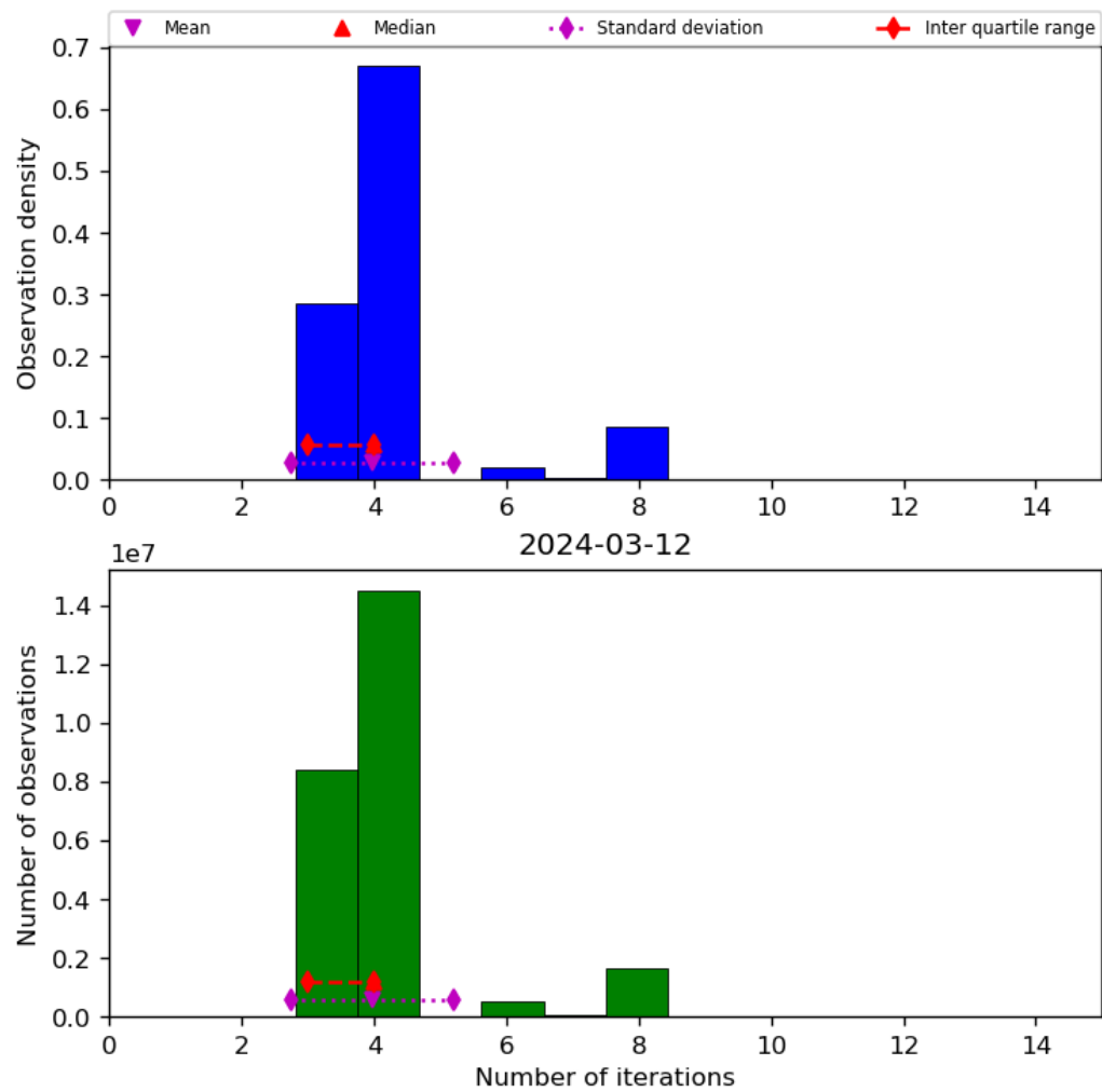
Figure 34: Histogram of “Number of iterations” for 2024-03-11 to 2024-03-13
