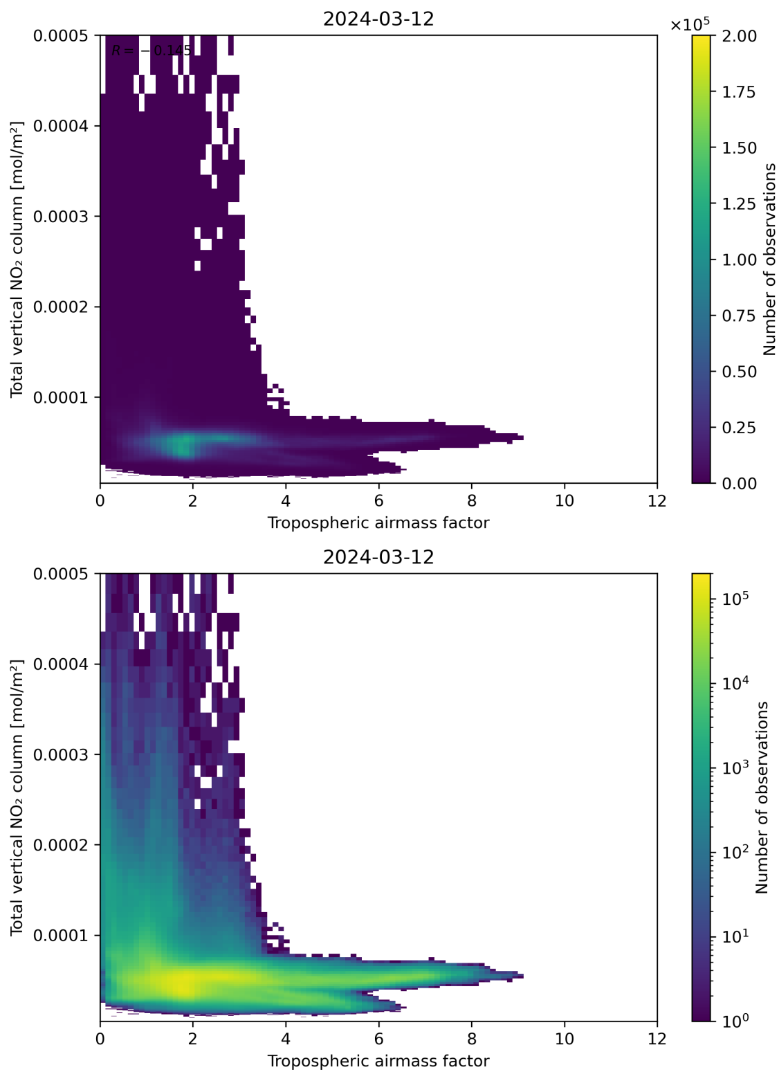
Figure 77: Scatter density plot of “Tropospheric airmass factor” against “Total vertical NO 2 column” for 2024-03-11 to 2024-03-13.
