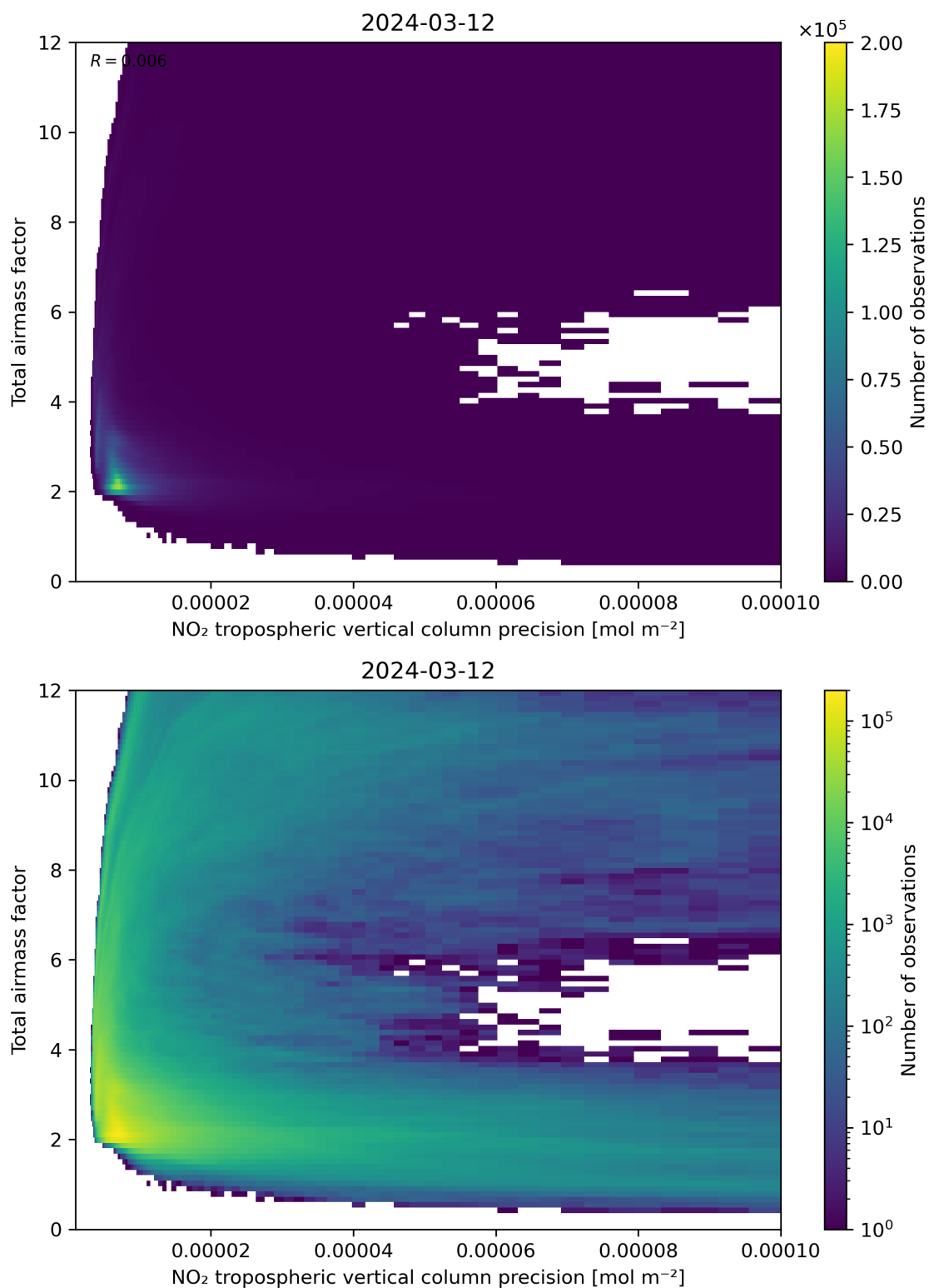
Figure 132: Scatter density plot of “NO 2 tropospheric vertical column precision” against “Total air mass factor” for 2024-03-11 to 2024-03-13.
