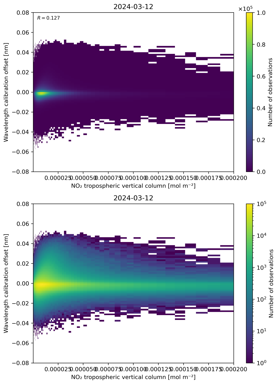
Figure 143: Scatter density plot of “NO 2 tropospheric vertical column” against “Wavelength calibration offset” for 2024-03-11 to 2024-03-13.
