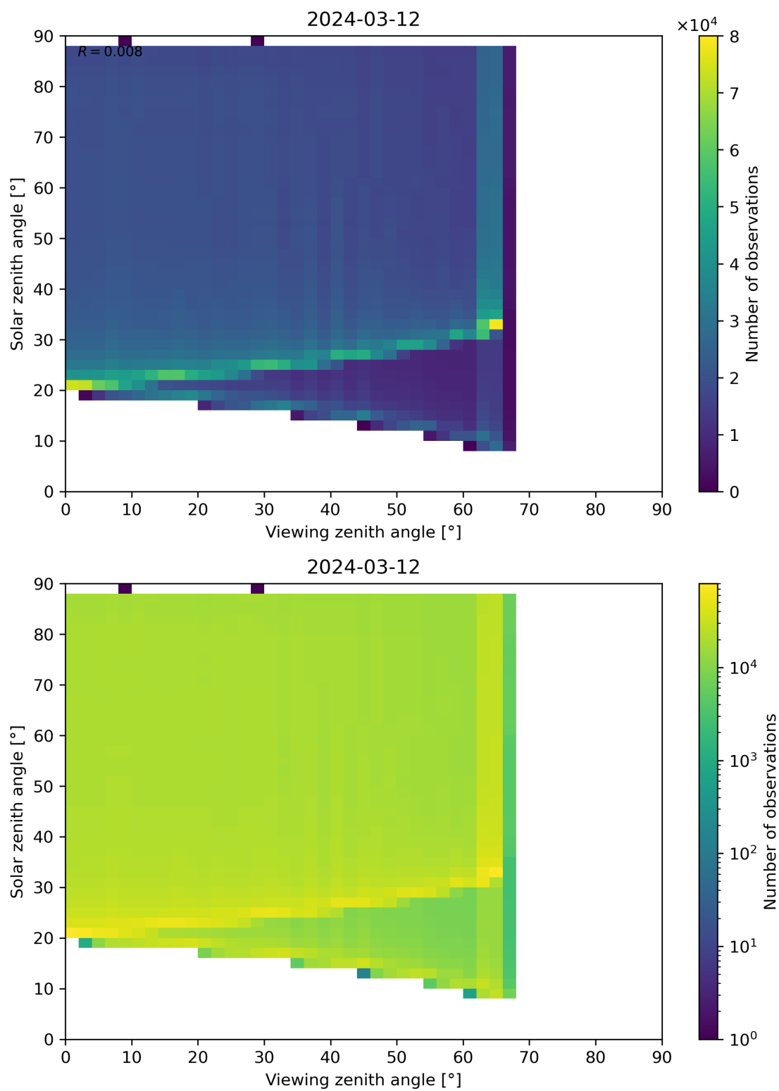
Figure 172: Scatter density plot of “Viewing zenith angle” against “Solar zenith angle” for 2024-03-11 to 2024-03-13.
