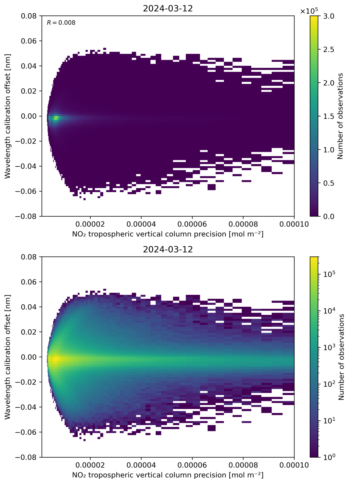
Figure 141: Scatter density plot of “NO 2 tropospheric vertical column precision” against “Wavelength calibration offset” for 2024-03-11 to 2024-03-13.
