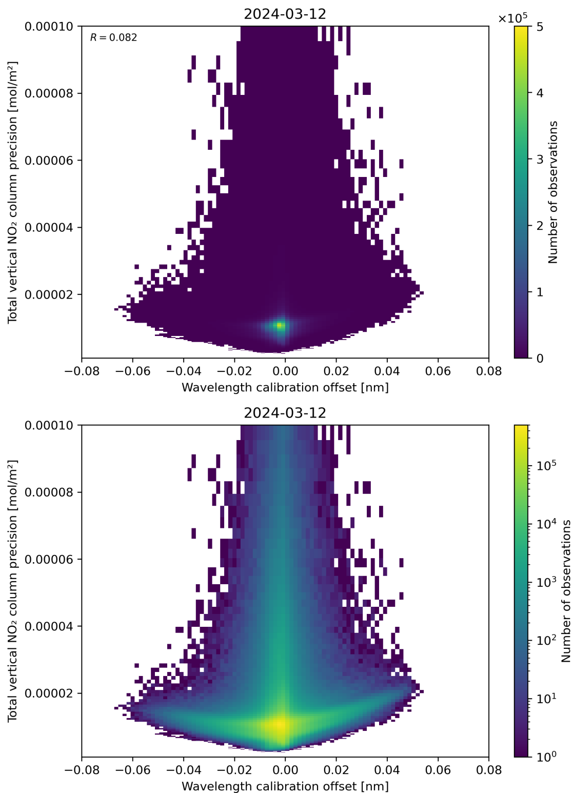
Figure 180: Scatter density plot of “Wavelength calibration offset” against “Total vertical NO 2 column precision” for 2024-03-11 to 2024-03-13.
