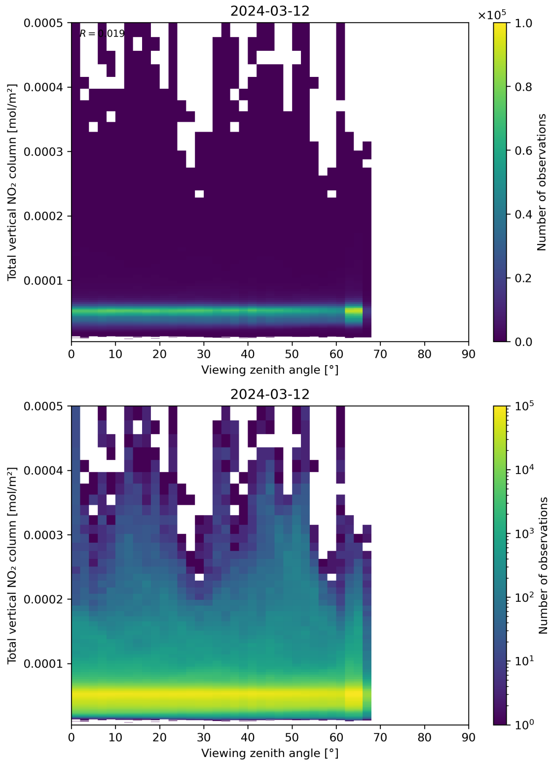
Figure 167: Scatter density plot of “Viewing zenith angle” against “Total vertical NO 2 column” for 2024-03-11 to 2024-03-13.
