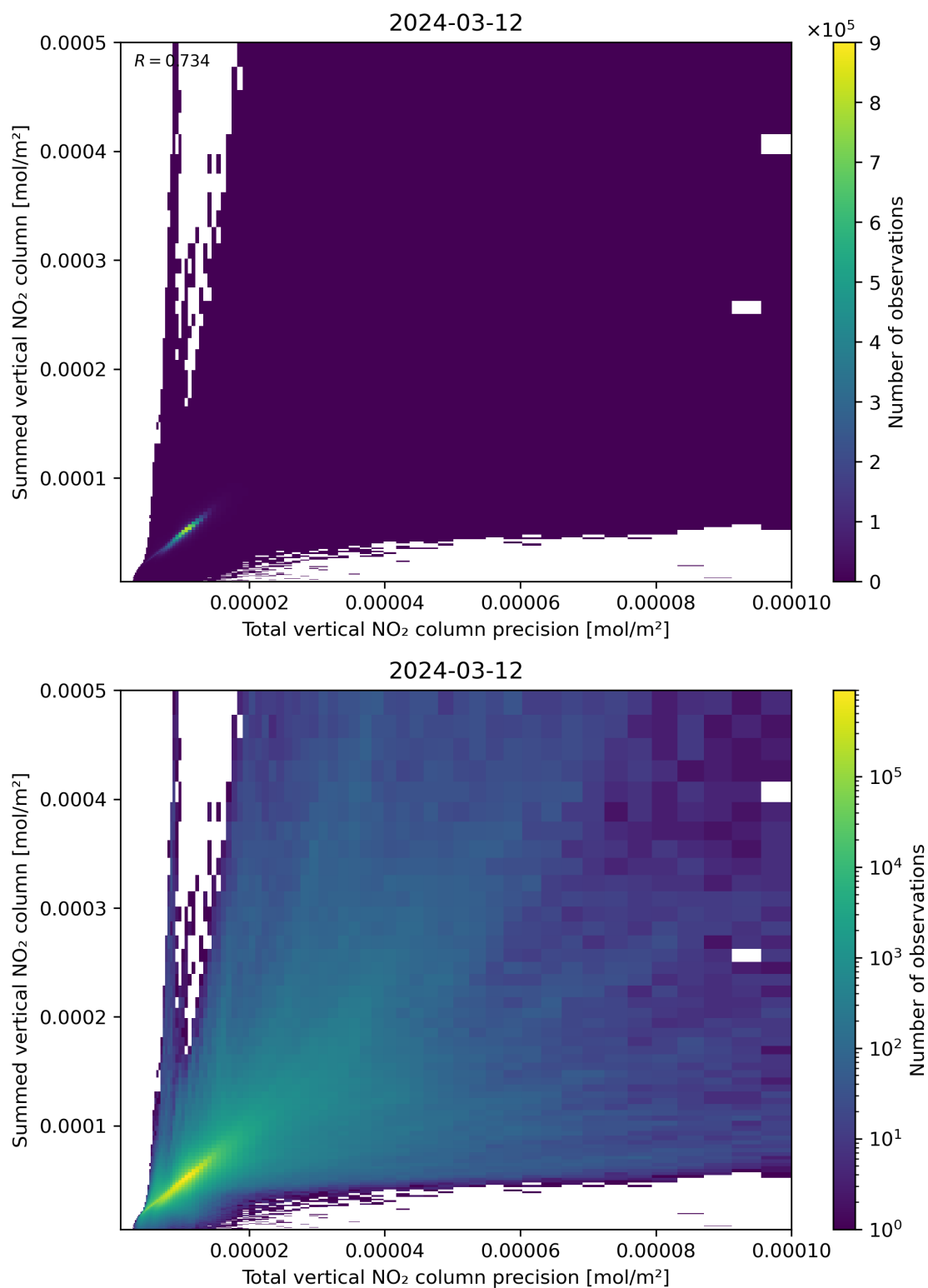
Figure 117: Scatter density plot of “Total vertical NO 2 column precision” against “Summed vertical NO 2 column” for 2024-03-11 to 2024-03-13.
