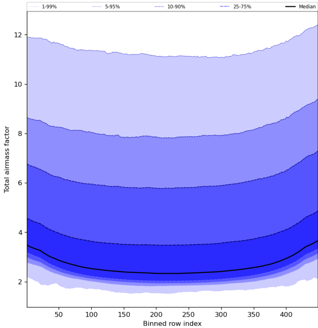
Figure 49: Along track statistics of “Total airmass factor” for 2024-03-11 to 2024-03-13
