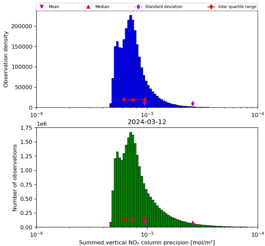
Figure 41: Histogram of “Summed vertical NO 2 column precision” for 2024-03-11 to 2024-03-13
