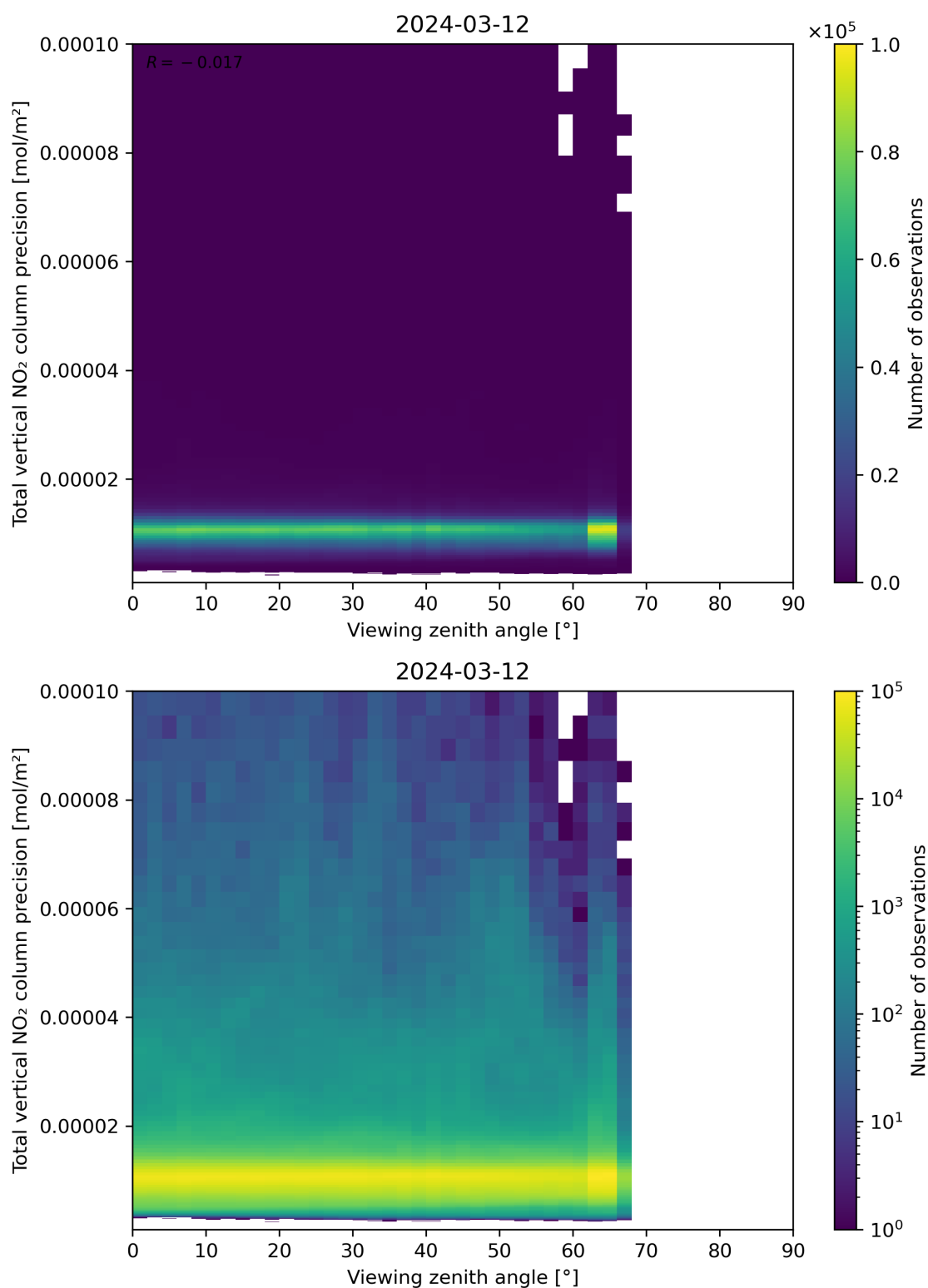
Figure 168: Scatter density plot of “Viewing zenith angle” against “Total vertical NO 2 column precision” for 2024-03-11 to 2024-03-13.
