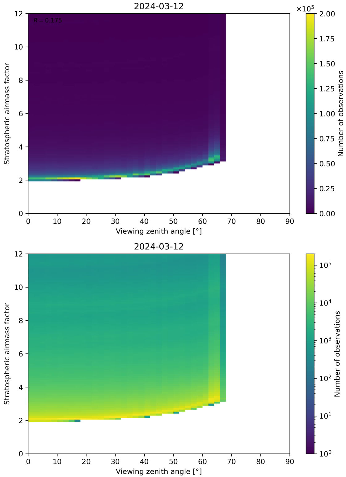
Figure 159: Scatter density plot of “Viewing zenith angle” against “Stratospheric airmass factor” for 2024-03-11 to 2024-03-13.
