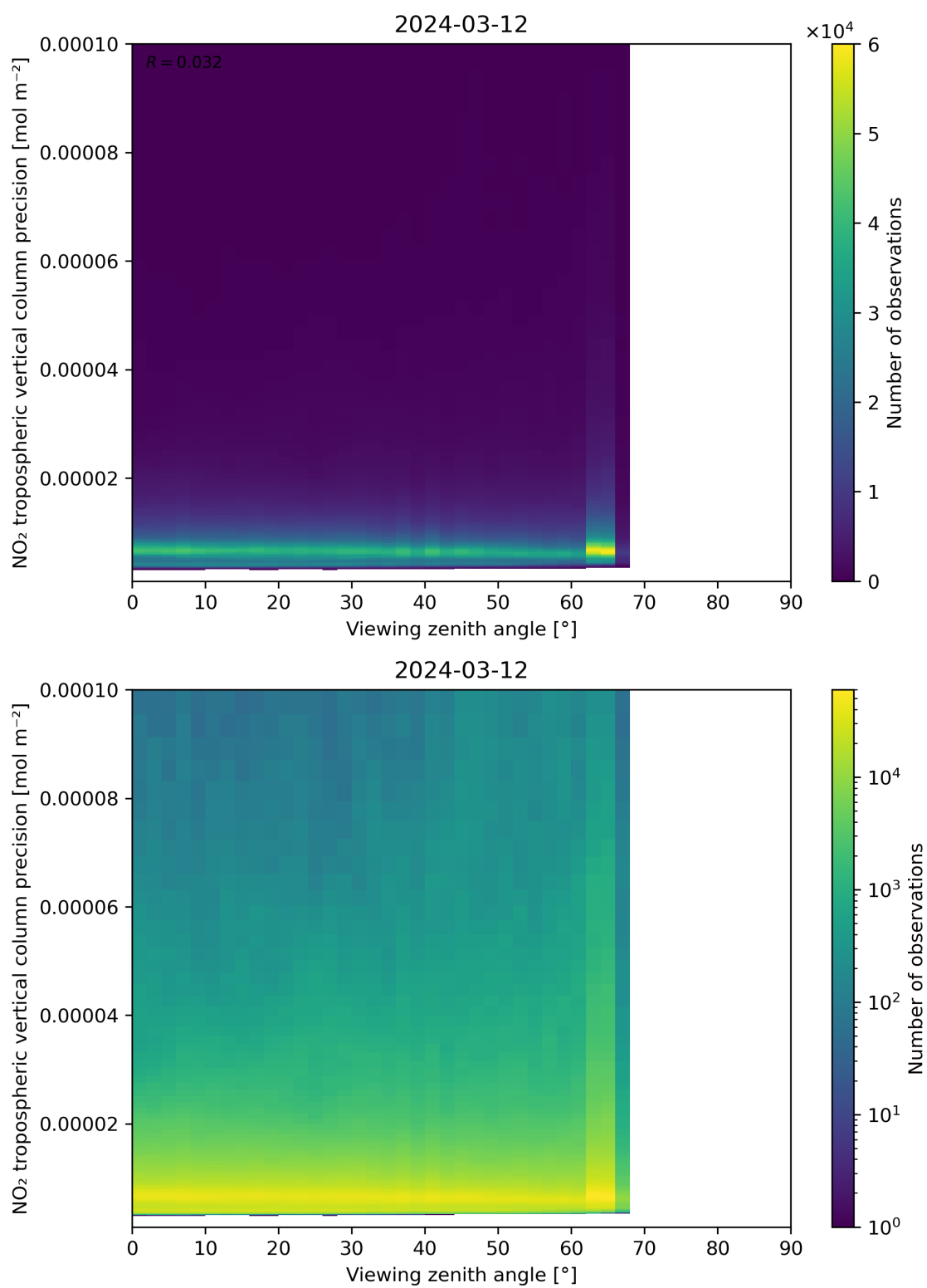
Figure 170: Scatter density plot of “Viewing zenith angle” against “NO 2 tropospheric vertical column precision” for 2024-03-11 to 2024-03-13.
