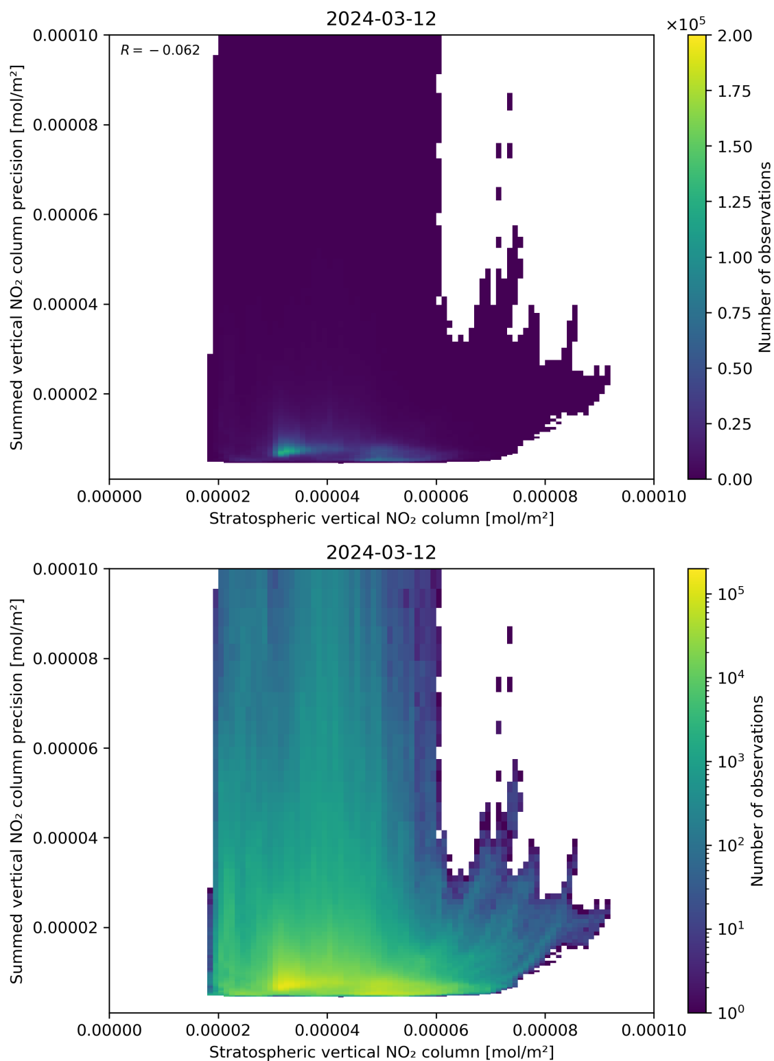
Figure 99: Scatter density plot of “Stratospheric vertical NO 2 column” against “Summed vertical NO 2 column precision” for 2024-03-11 to 2024-03-13.
