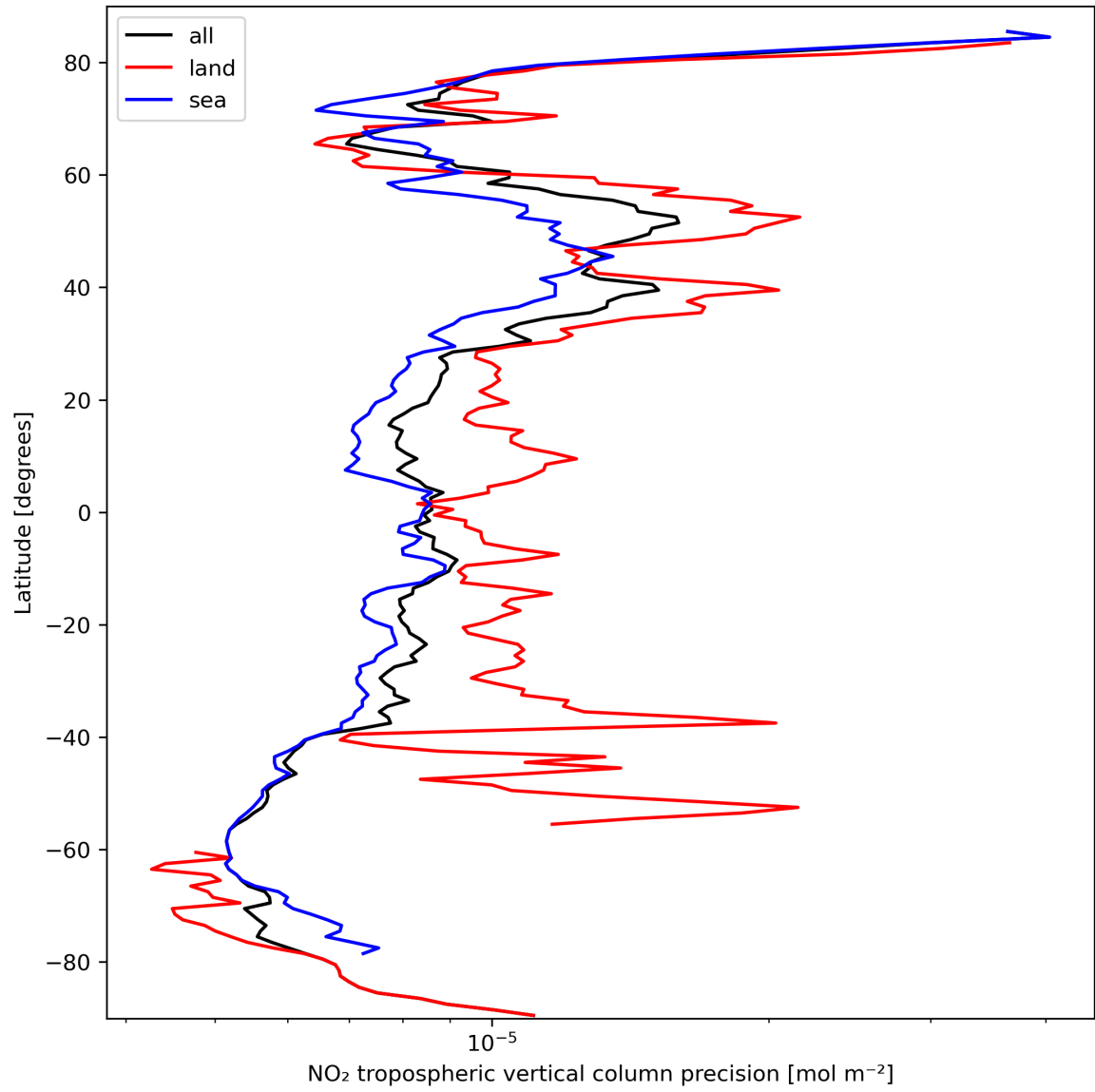
Figure 13: Zonal average of “NO 2 tropospheric vertical column precision” for 2024-03-11 to 2024-03-13.
