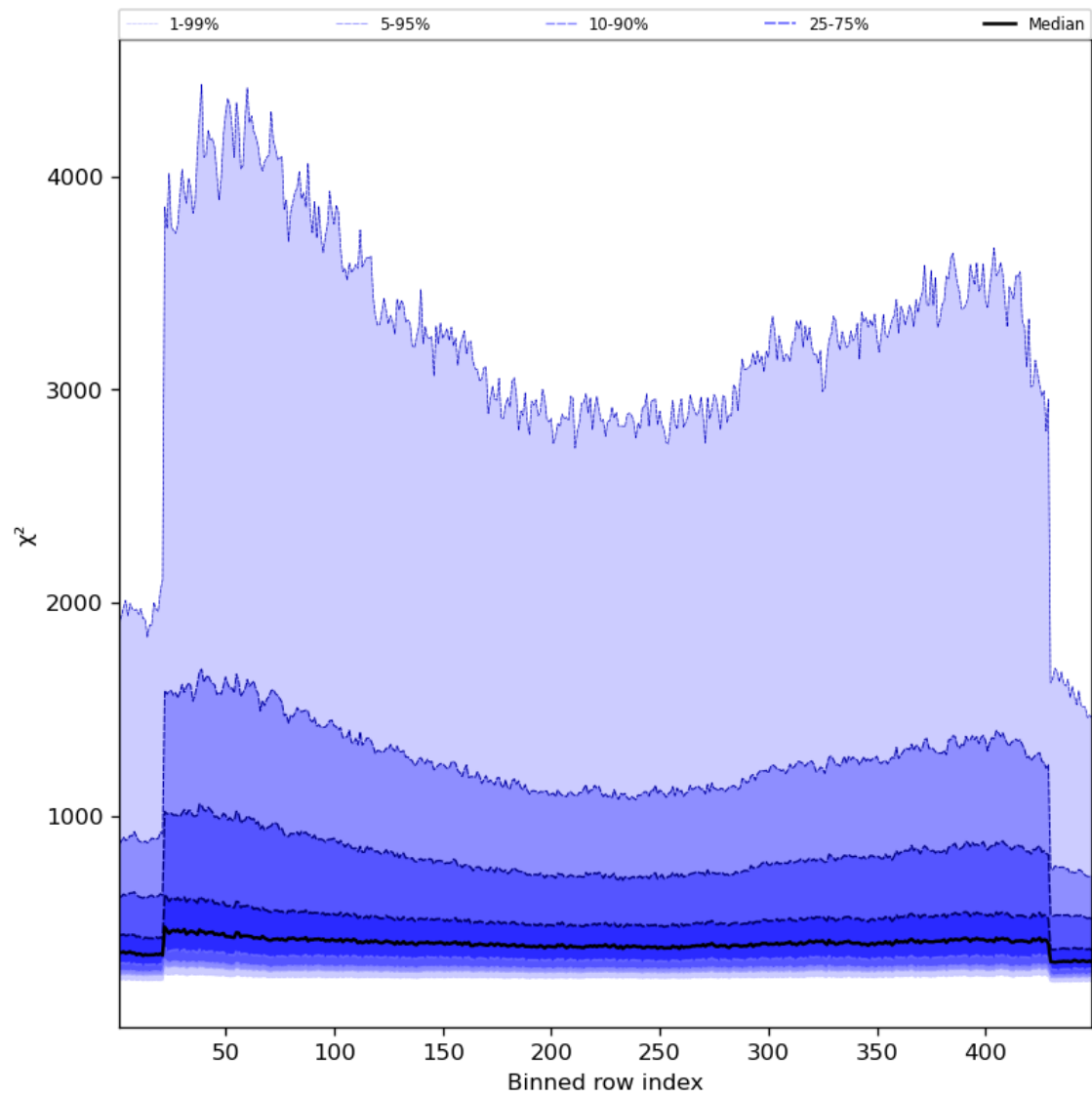
Figure 59: Along track statistics of “ \chi^2 ” for 2024-03-11 to 2024-03-13
