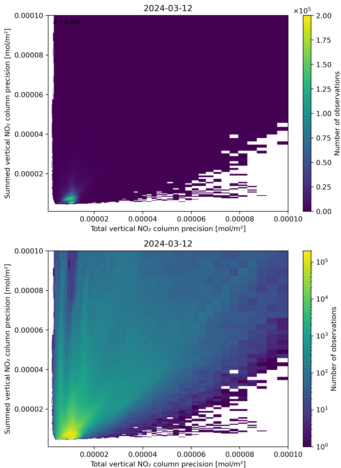
Figure 118: Scatter density plot of “Total vertical NO 2 column precision” against “Summed vertical NO 2 column precision” for 2024-03-11 to 2024-03-13.
