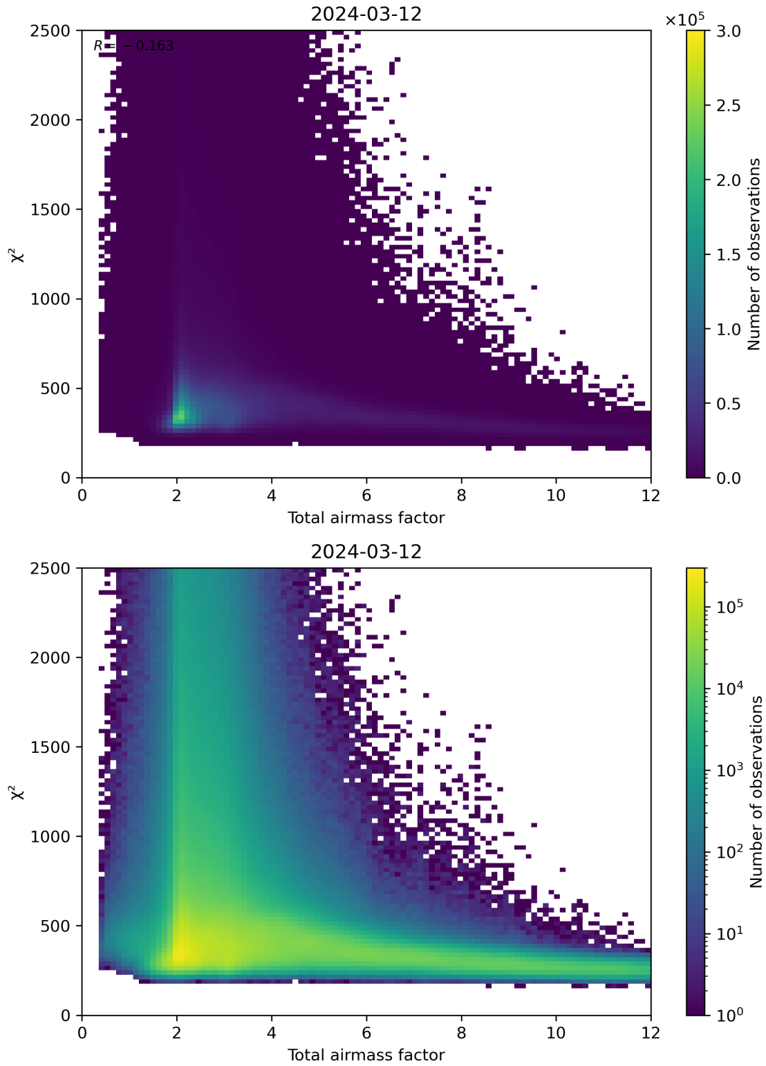
Figure 63: Scatter density plot of “Total airmass factor” against “ \chi^2 ” for 2024-03-11 to 2024-03-13.
