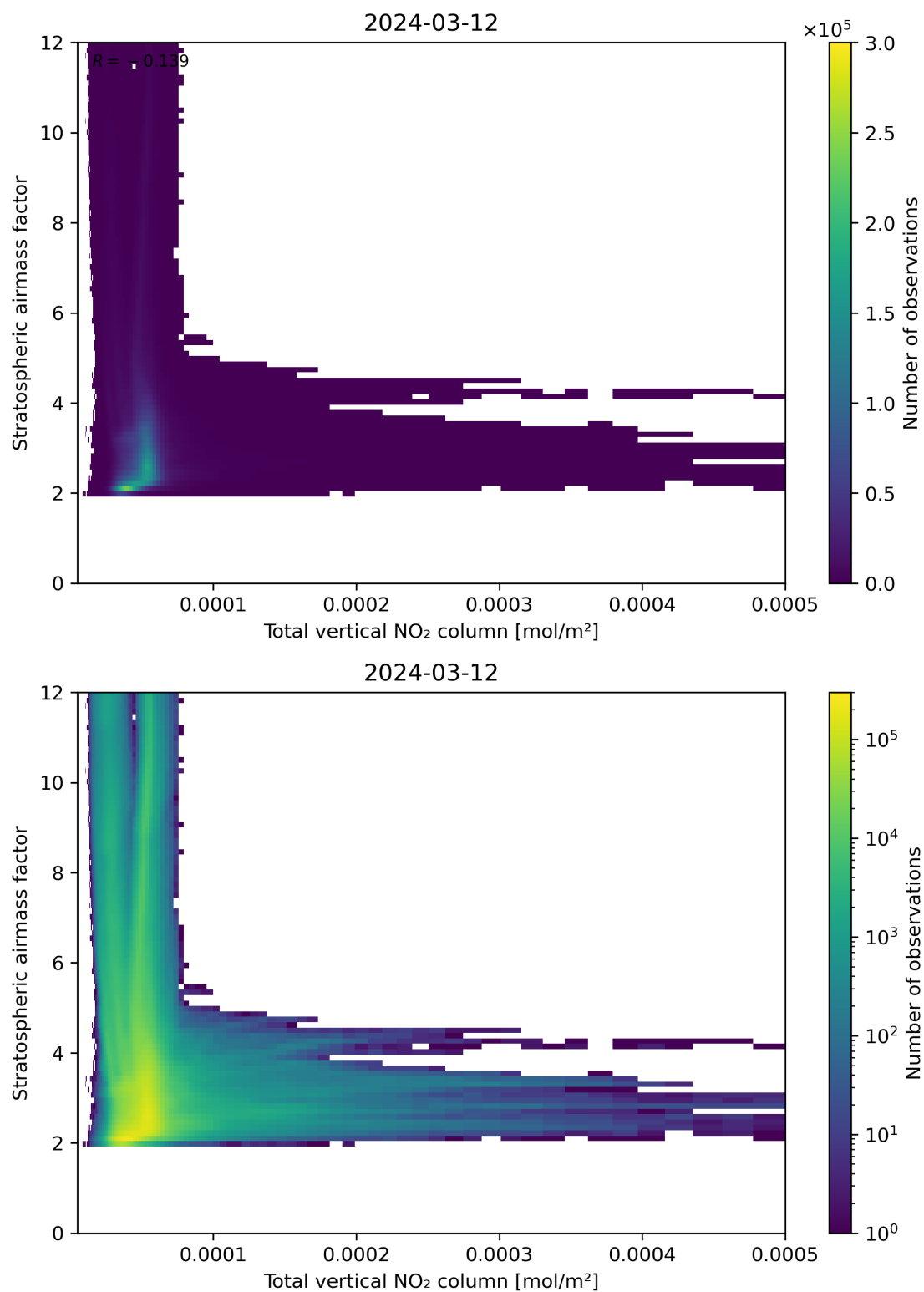
Figure 110: Scatter density plot of “Total vertical NO 2 column” against “Stratospheric airmass factor” for 2024-03-11 to 2024-03-13.
