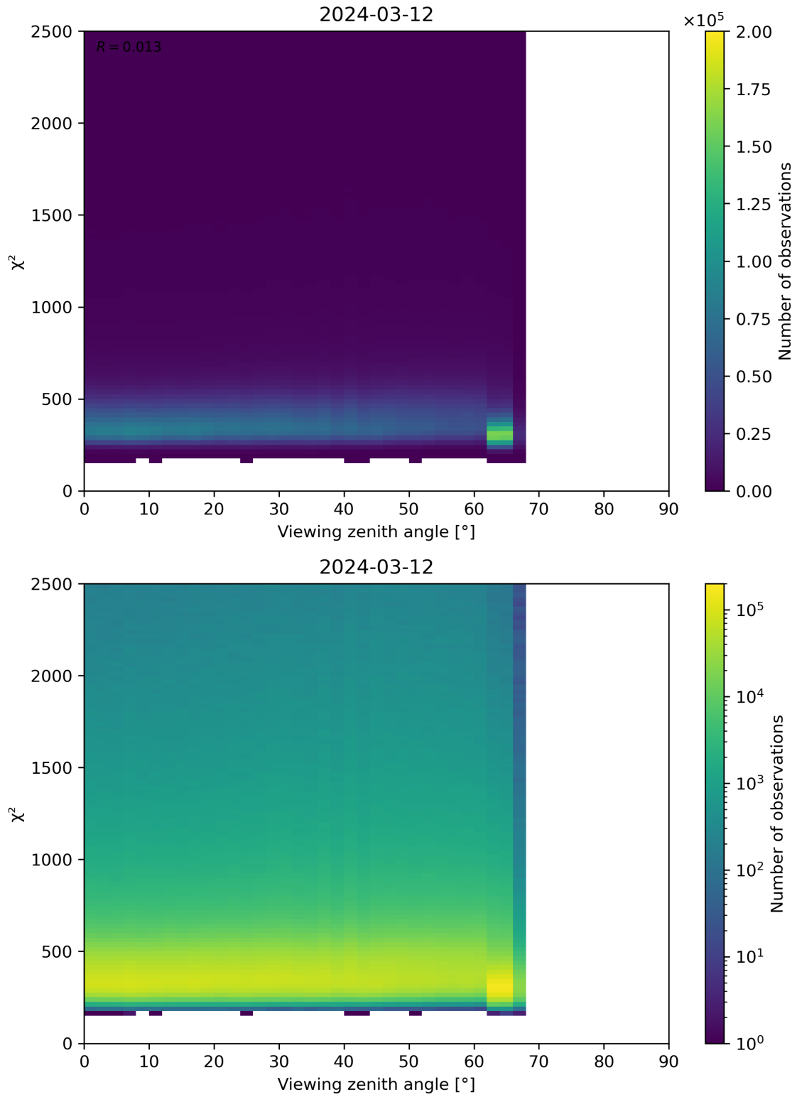
Figure 162: Scatter density plot of “Viewing zenith angle” against “ \chi^2 ” for 2024-03-11 to 2024-03-13.
