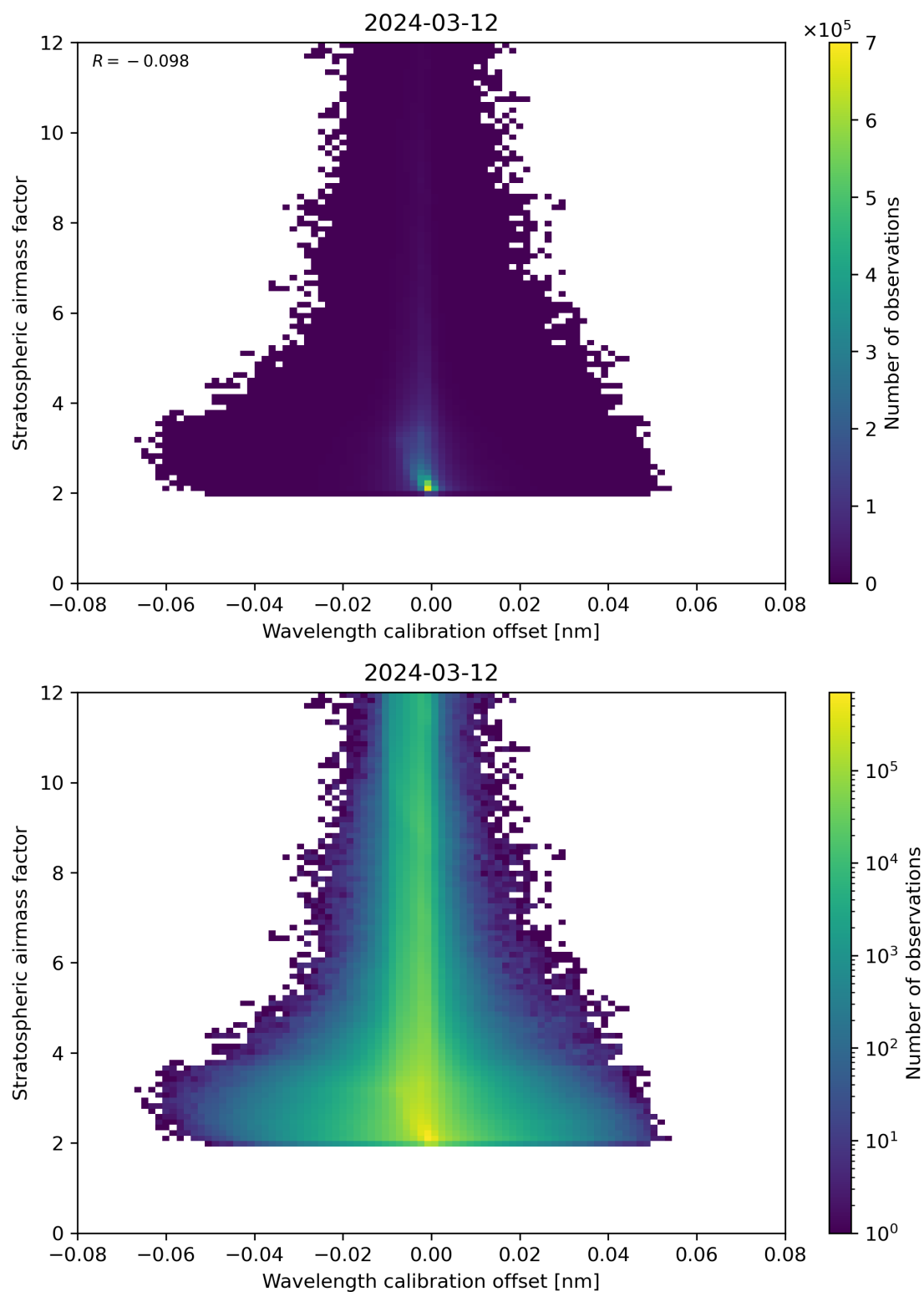
Figure 174: Scatter density plot of “Wavelength calibration offset” against “Stratospheric air mass factor” for 2024-03-11 to 2024-03-13.
