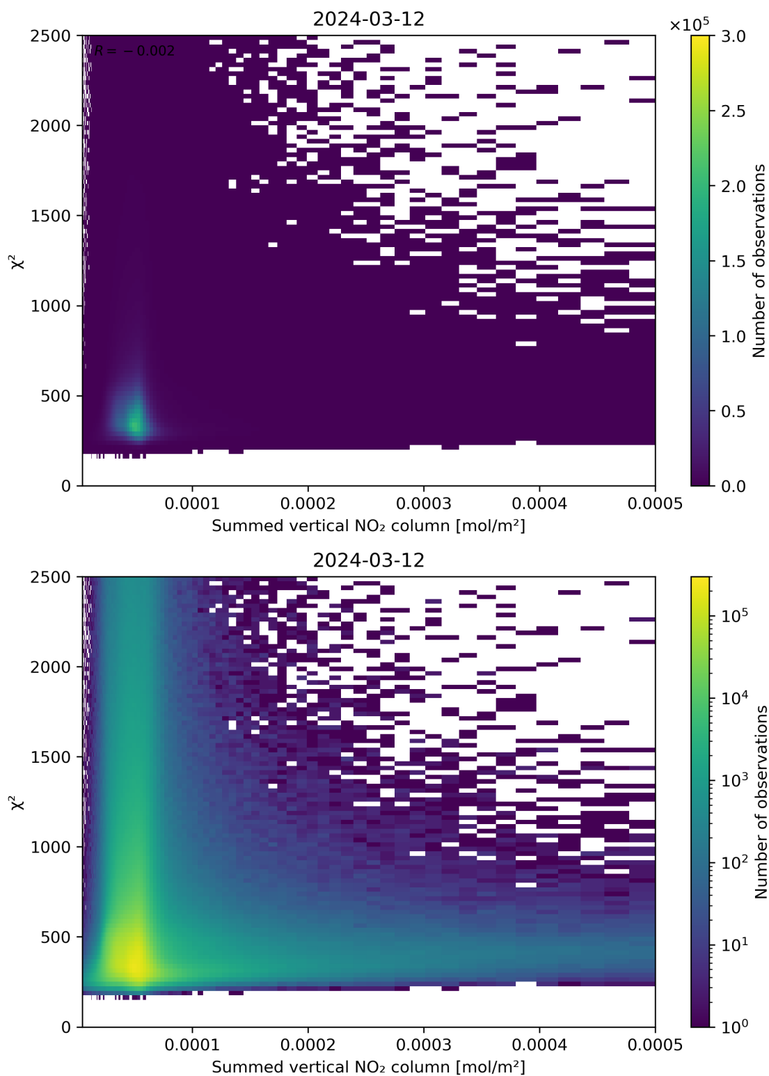
Figure 104: Scatter density plot of “Summed vertical NO 2 column” against “ \chi^2 ” for 2024-03-11 to 2024-03-13.
