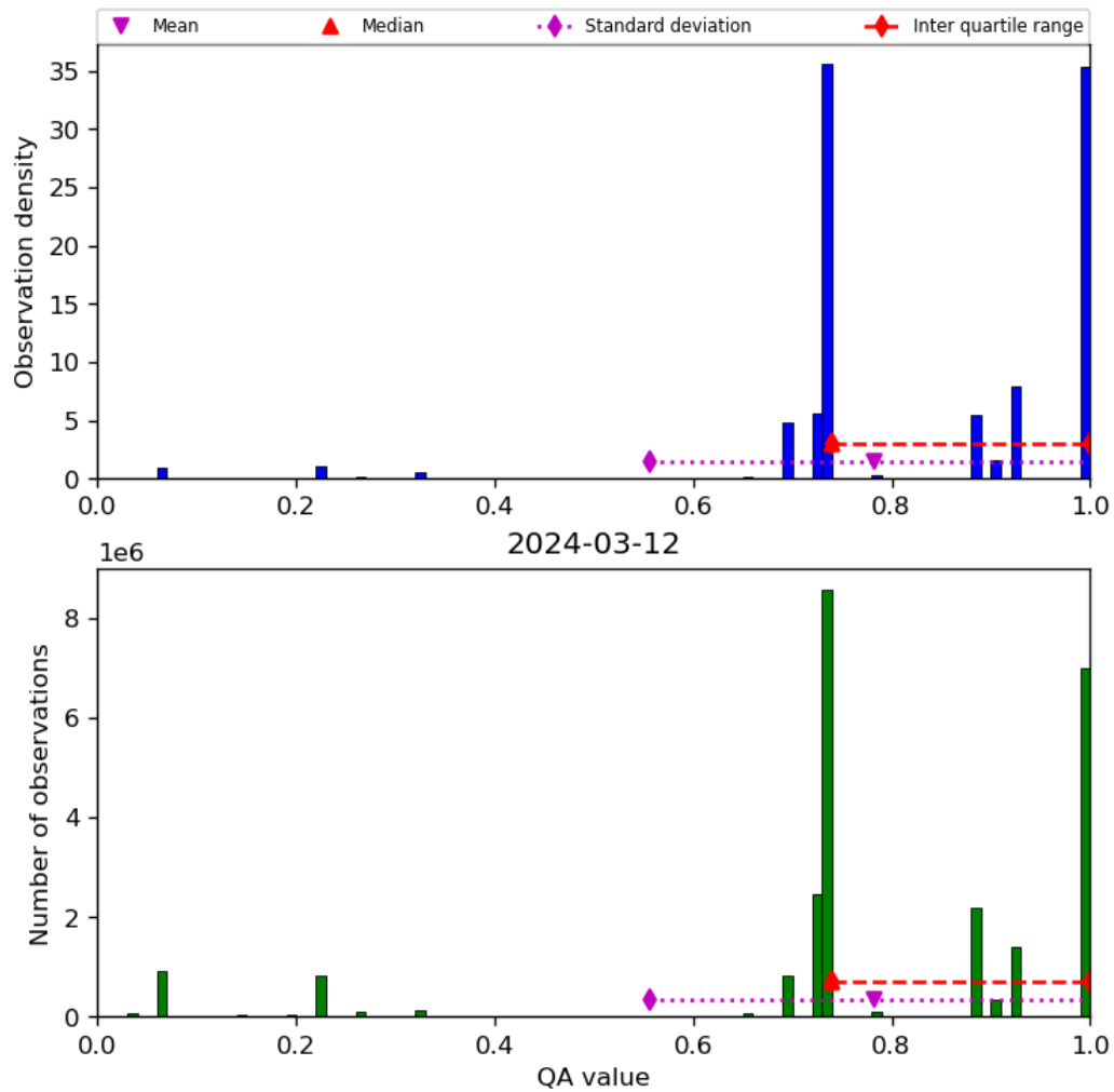
Figure 28: Histogram of “QA value” for 2024-03-11 to 2024-03-13
