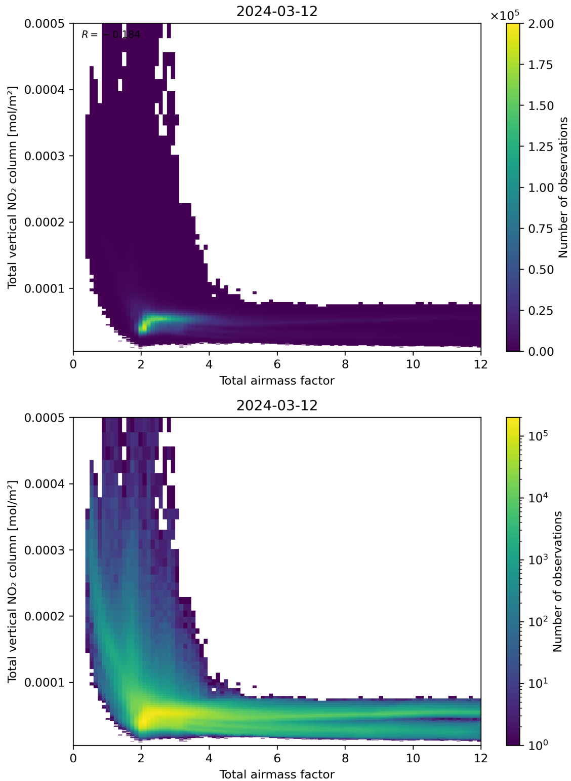
Figure 67: Scatter density plot of “Total air mass factor” against “Total vertical NO 2 column” for 2024-03-11 to 2024-03-13.
