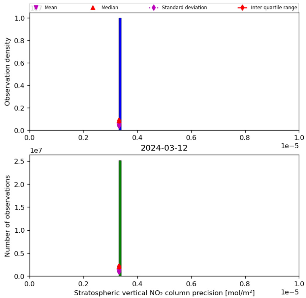
Figure 37: Histogram of “Stratospheric vertical NO 2 column precision” for 2024-03-11 to 2024-03-13
