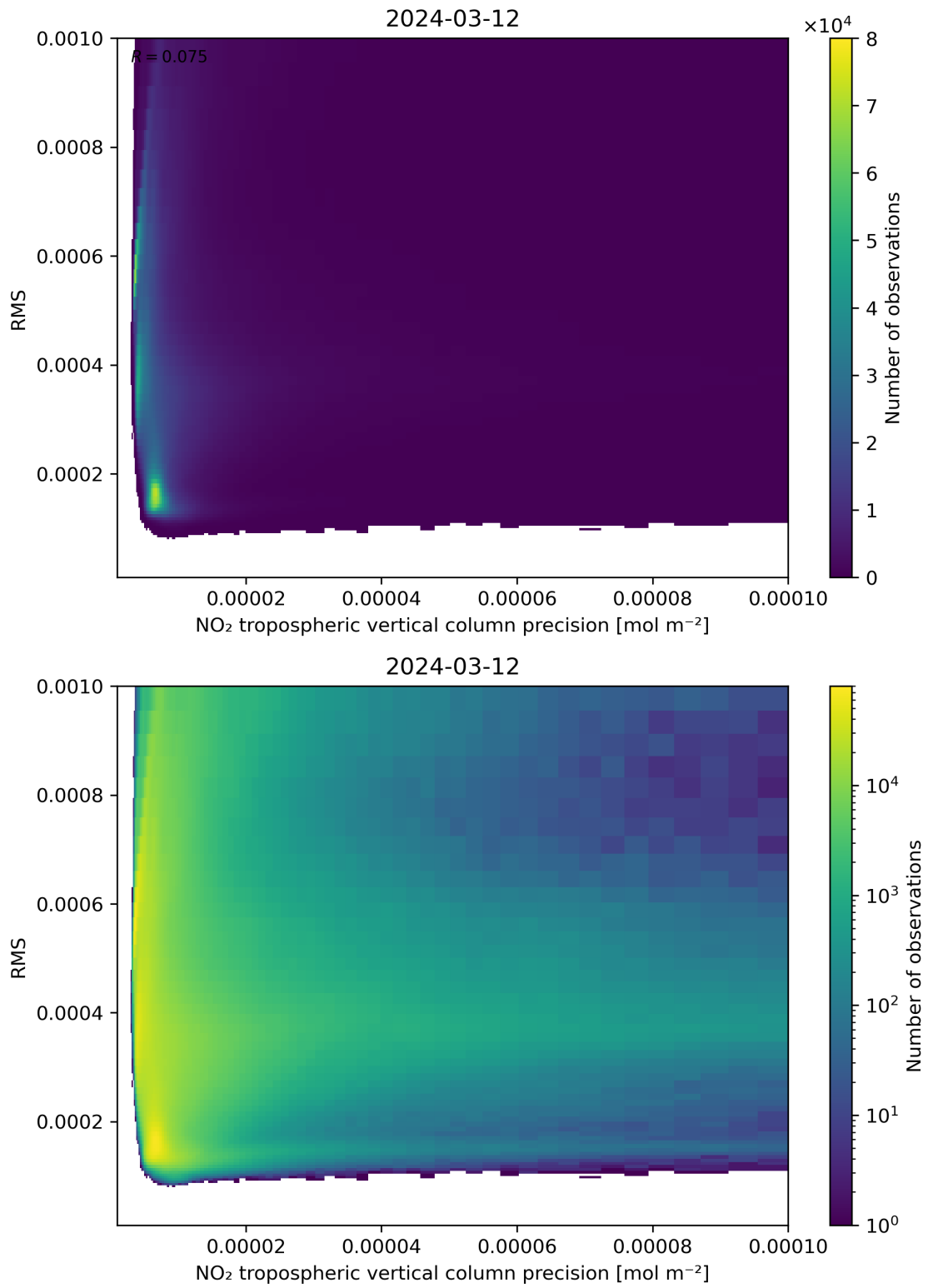
Figure 140: Scatter density plot of “NO 2 tropospheric vertical column precision” against “RMS” for 2024-03-11 to 2024-03-13.
