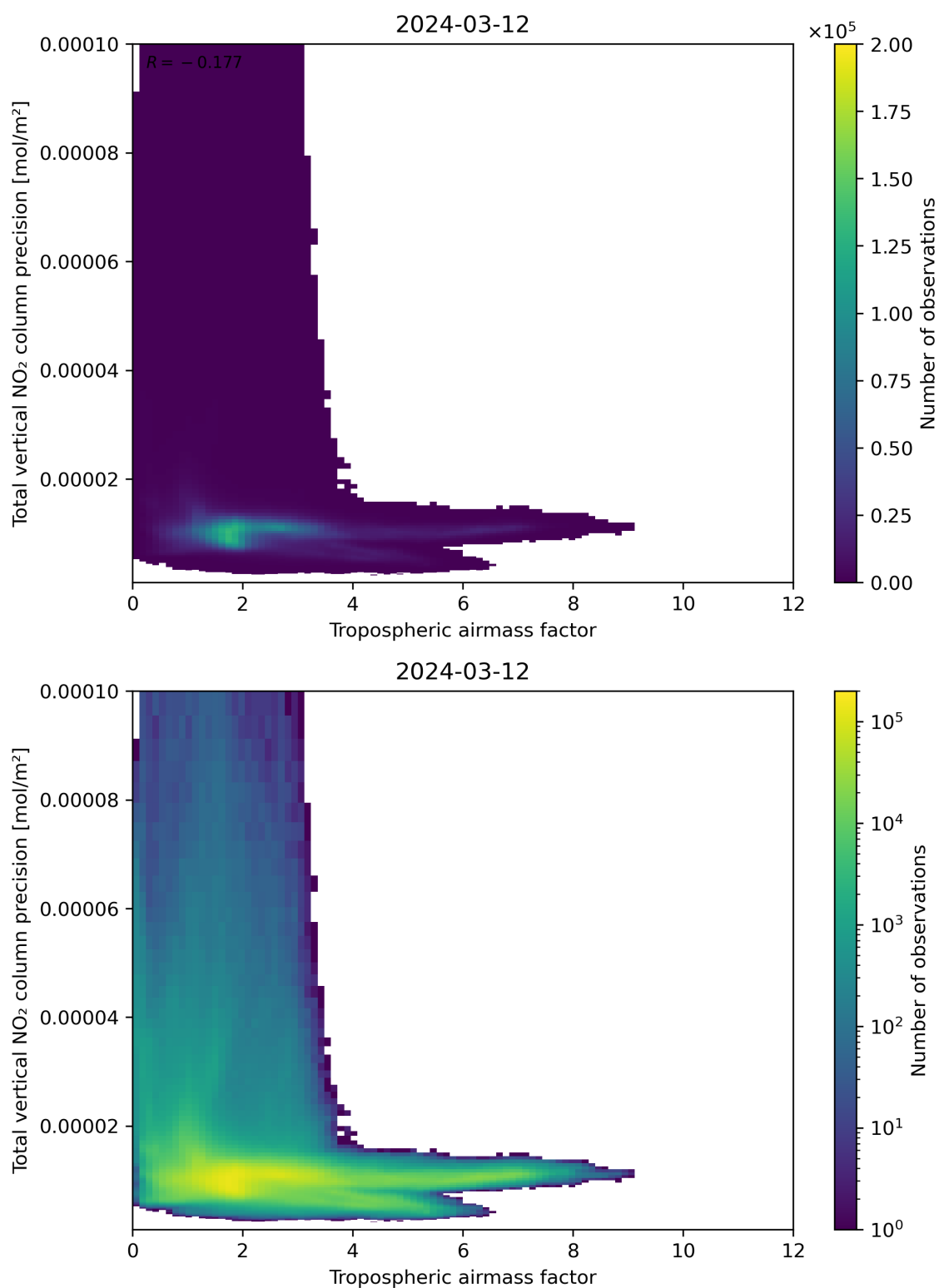
Figure 78: Scatter density plot of “Tropospheric airmass factor” against “Total vertical NO 2 column precision” for 2024-03-11 to 2024-03-13.
