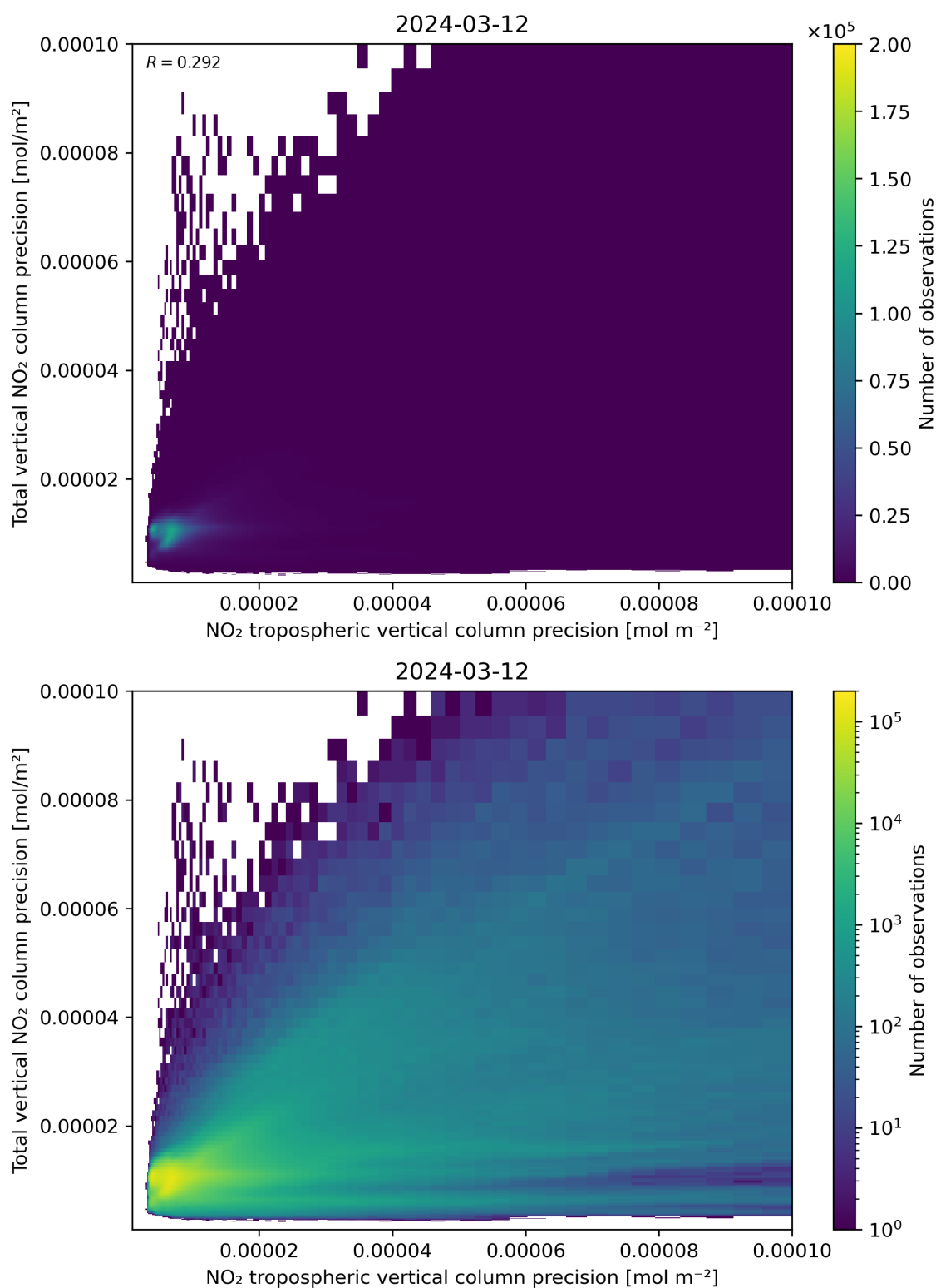
Figure 139: Scatter density plot of “NO 2 tropospheric vertical column precision” against “Total vertical NO 2 column precision” for 2024-03-11 to 2024-03-13.
