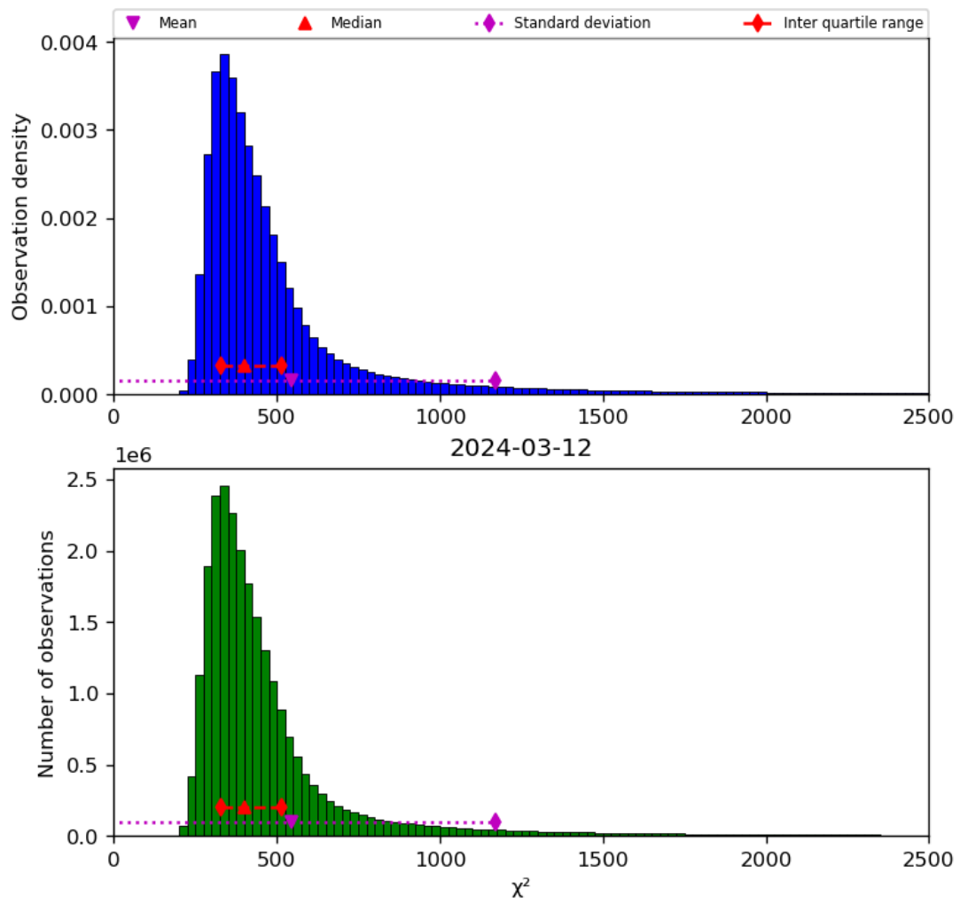
Figure 42: Histogram of “ \chi^2 ” for 2024-03-11 to 2024-03-13
