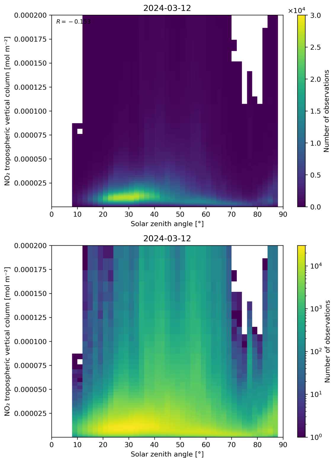
Figure 155: Scatter density plot of “Solar zenith angle” against “NO 2 tropospheric vertical column” for 2024-03-11 to 2024-03-13.
