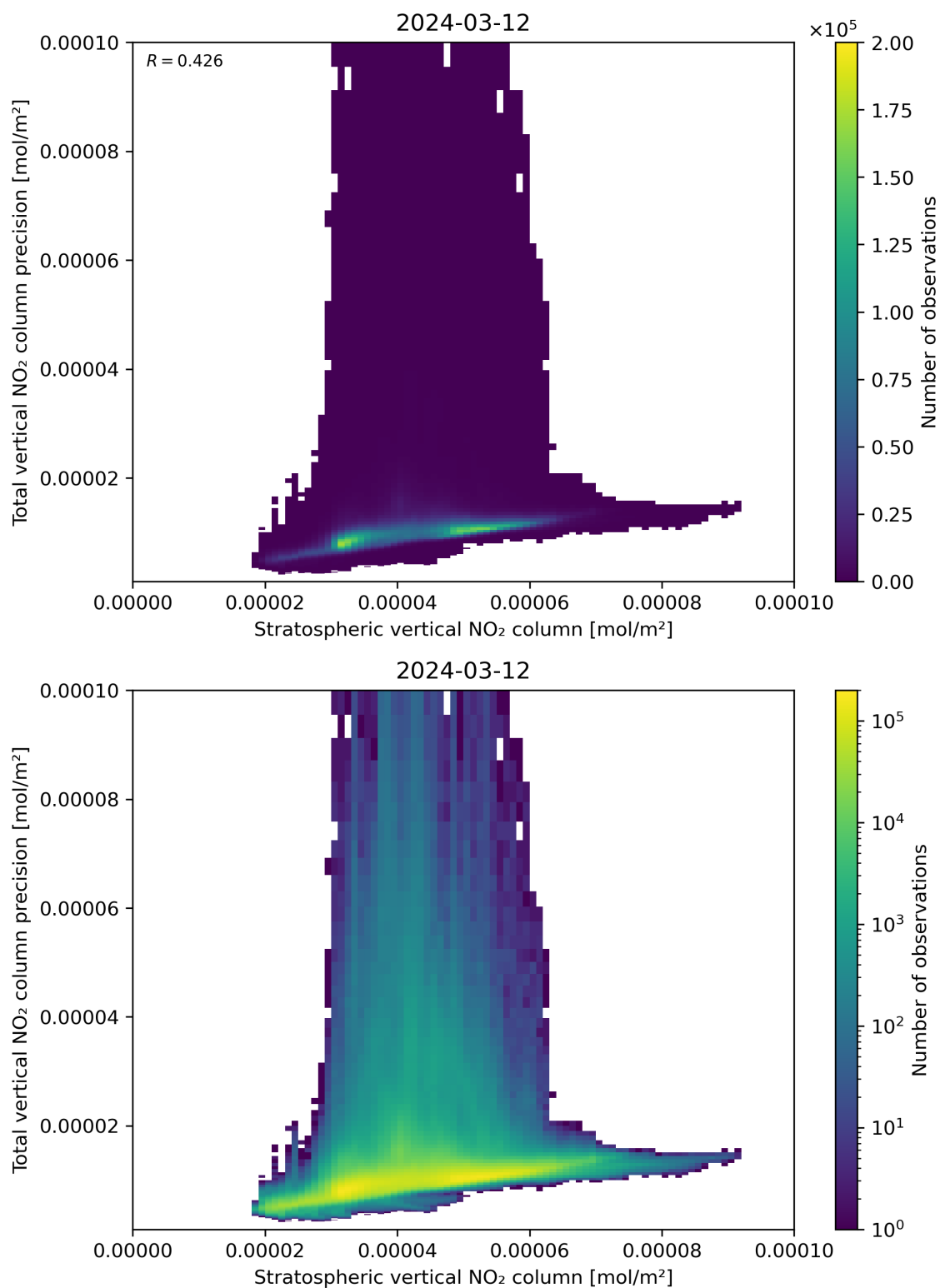
Figure 101: Scatter density plot of “Stratospheric vertical NO 2 column” against “Total vertical NO 2 column precision” for 2024-03-11 to 2024-03-13.
