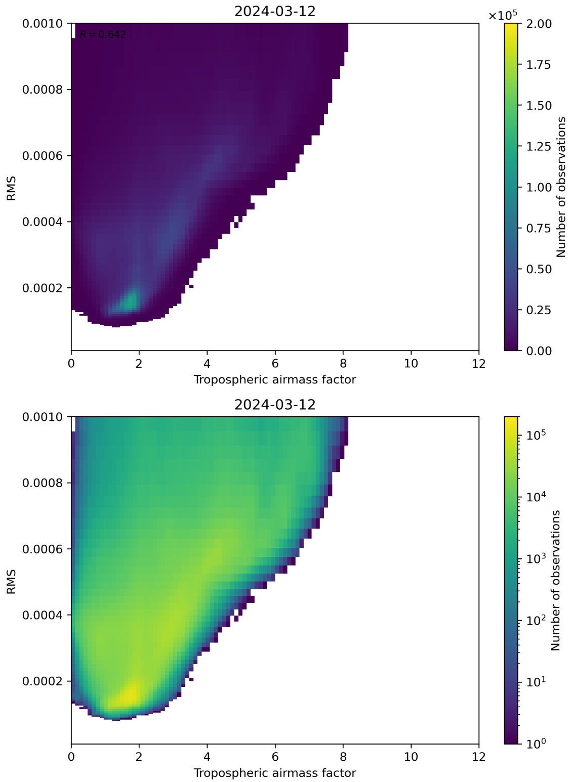
Figure 79: Scatter density plot of “Tropospheric airmass factor” against “RMS” for 2024-03-11 to 2024-03-13.
