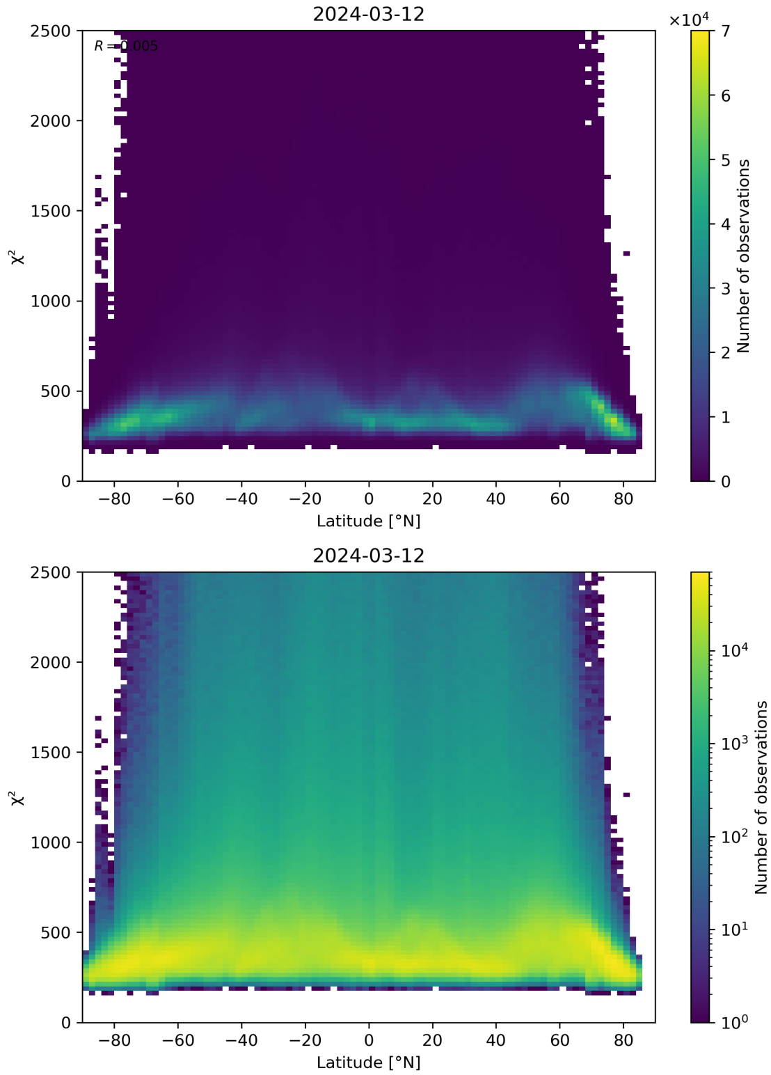
Figure 86: Scatter density plot of “Latitude” against “ \chi^2 ” for 2024-03-11 to 2024-03-13.
