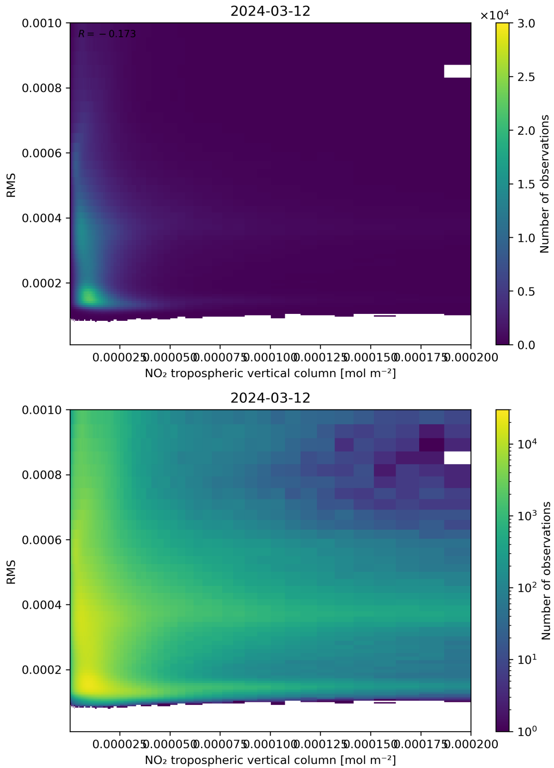
Figure 142: Scatter density plot of “NO 2 tropospheric vertical column” against “RMS” for 2024-03-11 to 2024-03-13.
