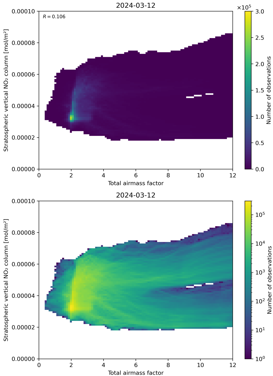
Figure 64: Scatter density plot of “Total airmass factor” against “Stratospheric vertical \text{NO}_2 column” for 2024-03-11 to 2024-03-13.
