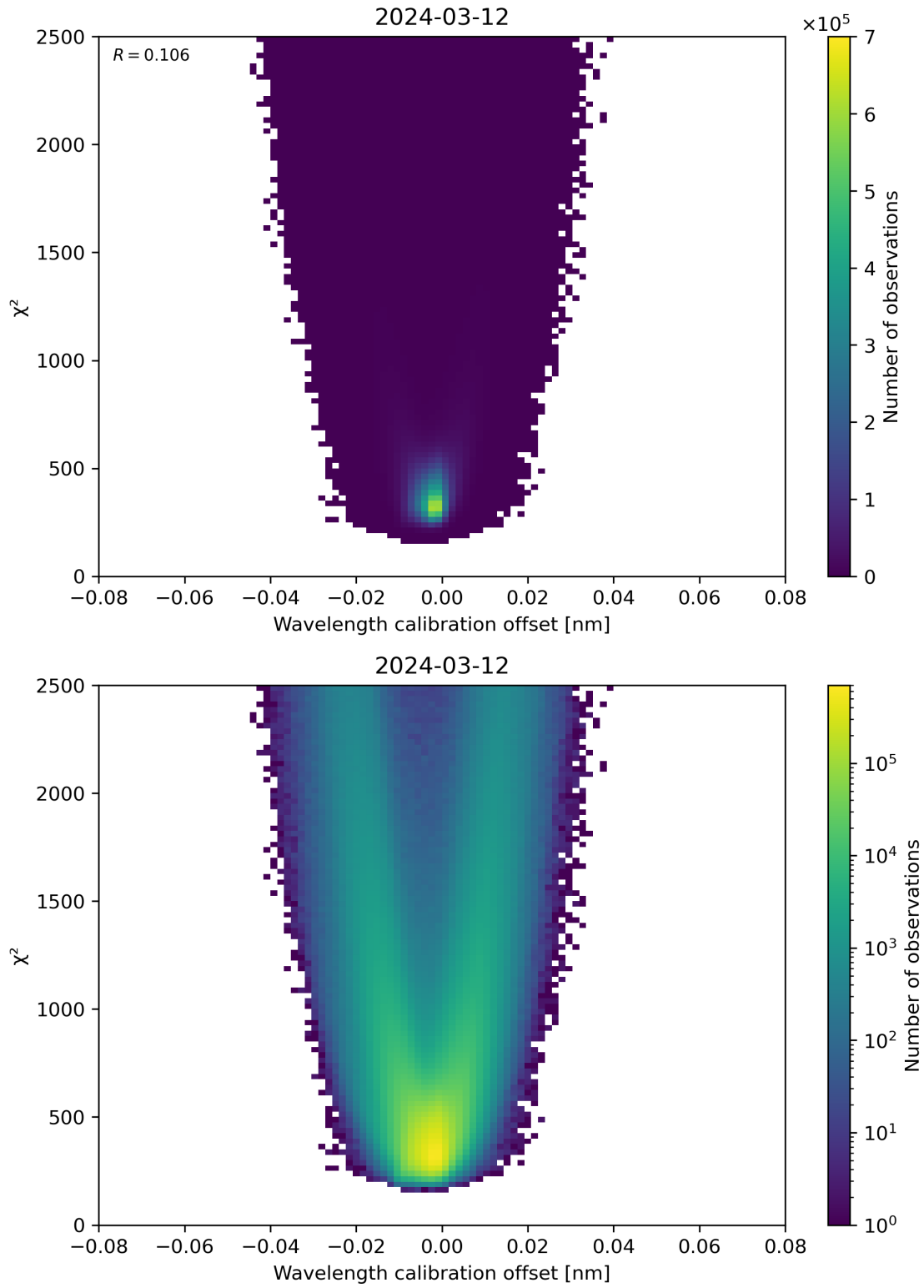
Figure 175: Scatter density plot of “Wavelength calibration offset” against “ \chi^2 ” for 2024-03-11 to 2024-03-13.
