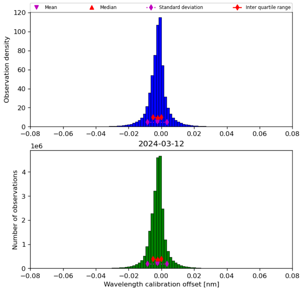
Figure 35: Histogram of “Wavelength calibration offset” for 2024-03-11 to 2024-03-13
