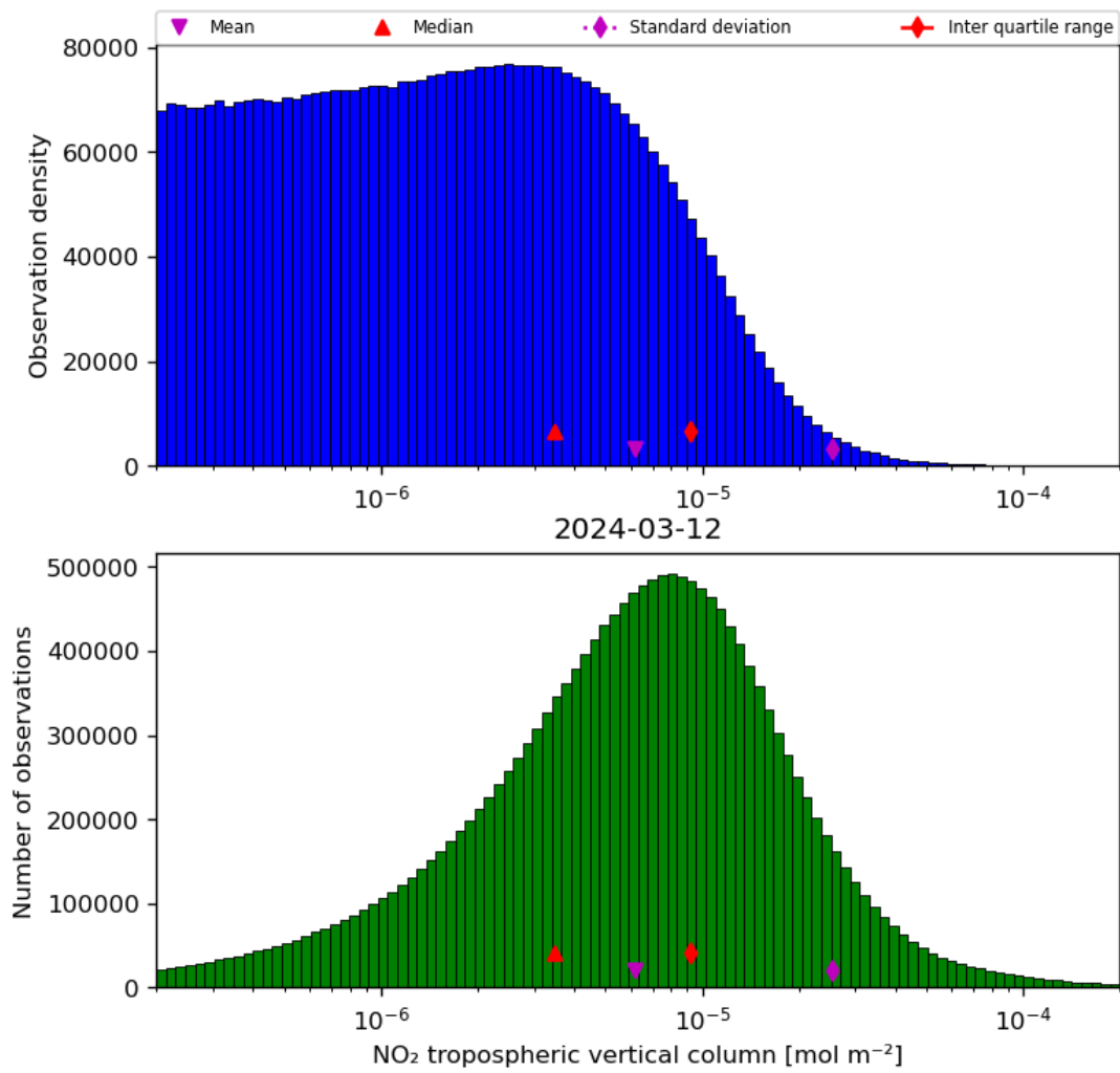
Figure 29: Histogram of “NO 2 tropospheric vertical column” for 2024-03-11 to 2024-03-13
