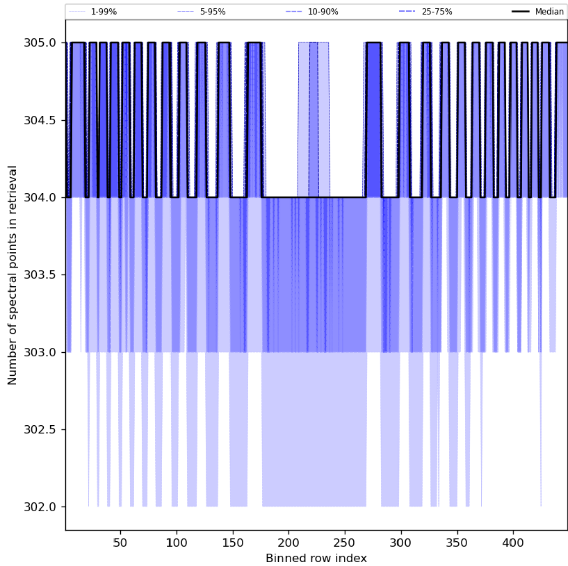
Figure 50: Along track statistics of “Number of spectral points in retrieval” for 2024-03-11 to 2024-03-13
