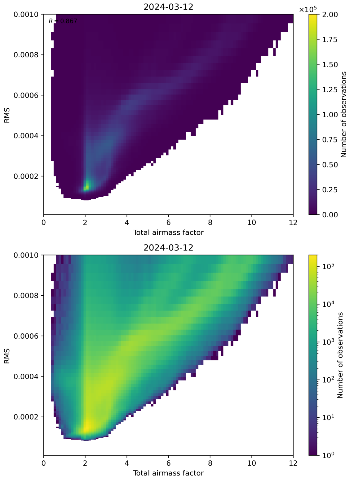
Figure 69: Scatter density plot of “Total airmass factor” against “RMS” for 2024-03-11 to 2024-03-13.
