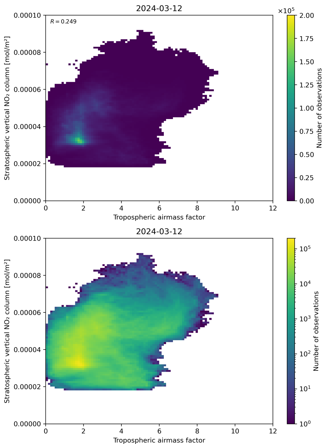
Figure 74: Scatter density plot of “Tropospheric air mass factor” against “Stratospheric vertical NO 2 column” for 2024-03-11 to 2024-03-13.
