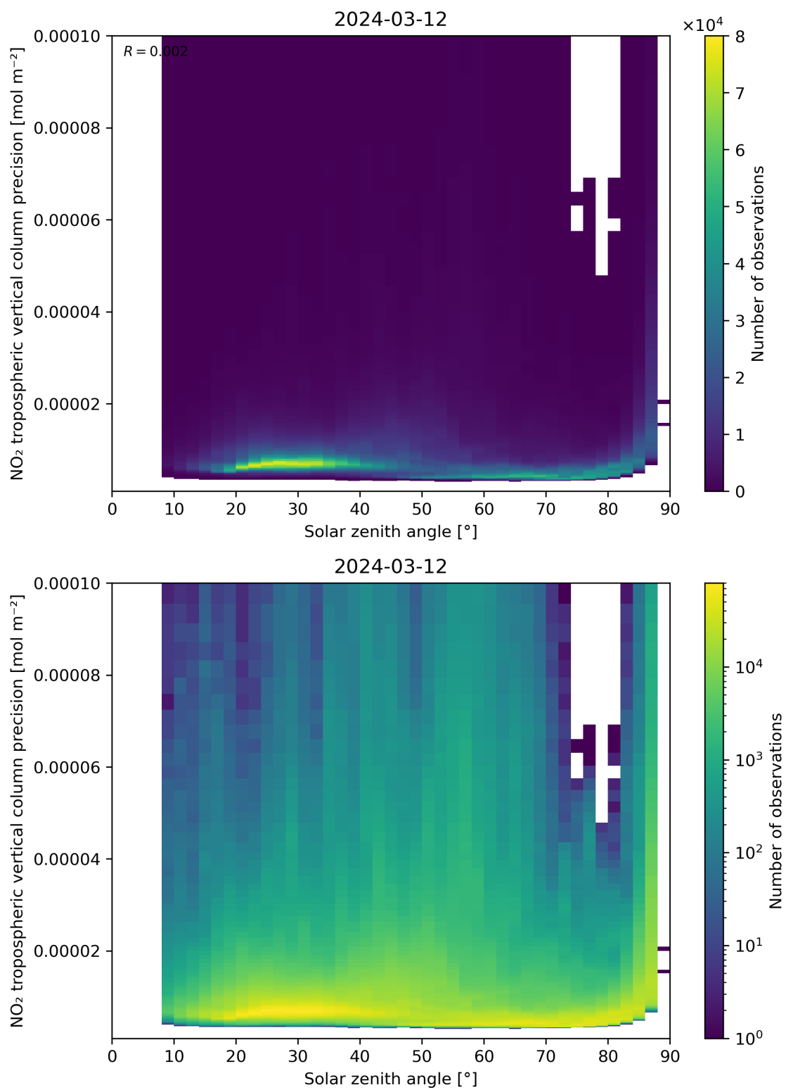
Figure 156: Scatter density plot of “Solar zenith angle” against “NO 2 tropospheric vertical column precision” for 2024-03-11 to 2024-03-13.
