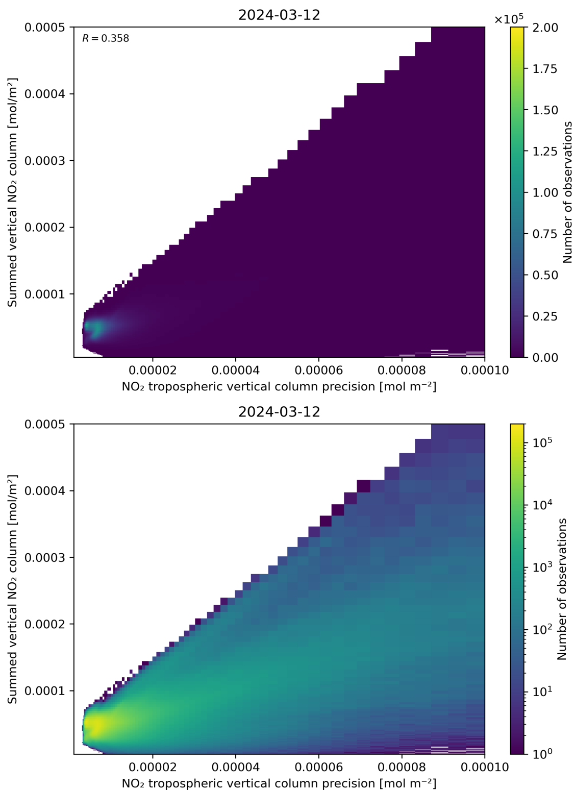
Figure 136: Scatter density plot of “NO 2 tropospheric vertical column precision” against “Summed vertical NO 2 column” for 2024-03-11 to 2024-03-13.
