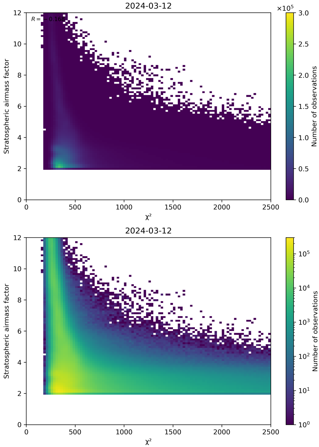
Figure 81: Scatter density plot of “ \chi^2 ” against “Stratospheric airmass factor” for 2024-03-11 to 2024-03-13.
