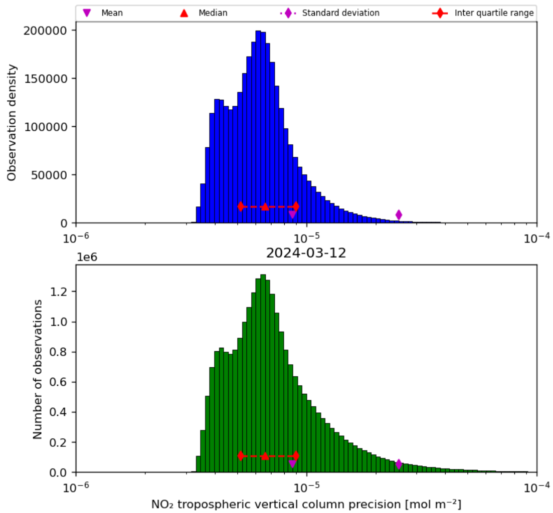
Figure 30: Histogram of “NO 2 tropospheric vertical column precision” for 2024-03-11 to 2024-03-13
