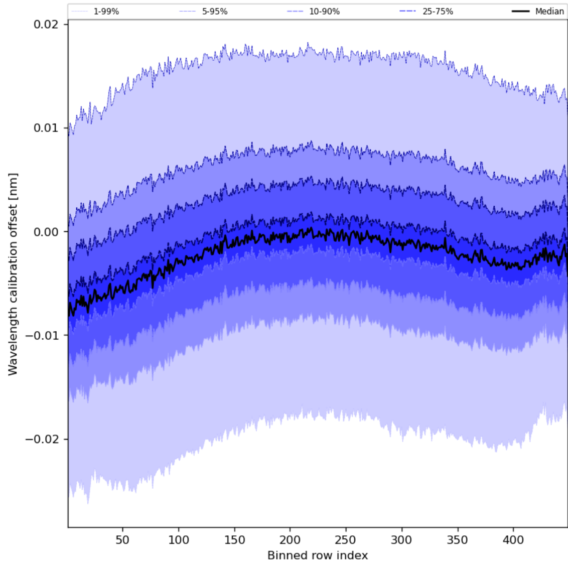
Figure 52: Along track statistics of “Wavelength calibration offset” for 2024-03-11 to 2024-03-13
