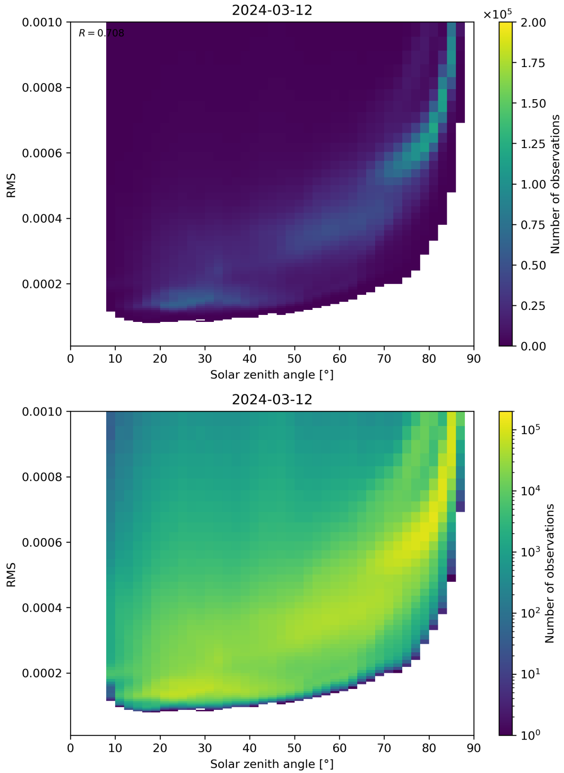
Figure 157: Scatter density plot of “Solar zenith angle” against “RMS” for 2024-03-11 to 2024-03-13.
