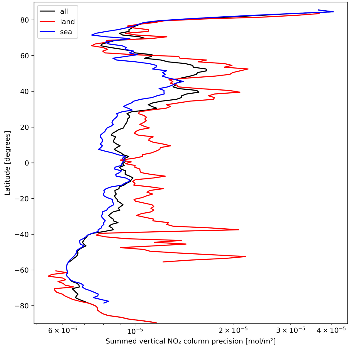
Figure 24: Zonal average of “Summed vertical NO 2 column precision” for 2024-03-11 to 2024-03-13.
