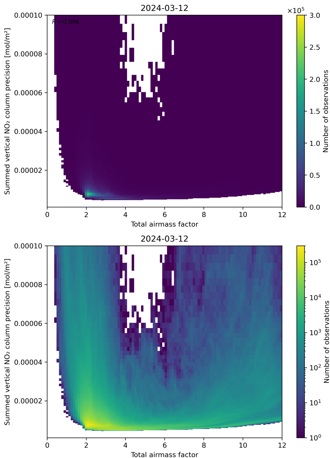
Figure 66: Scatter density plot of “Total airmass factor” against “Summed vertical NO 2 column precision” for 2024-03-11 to 2024-03-13.
