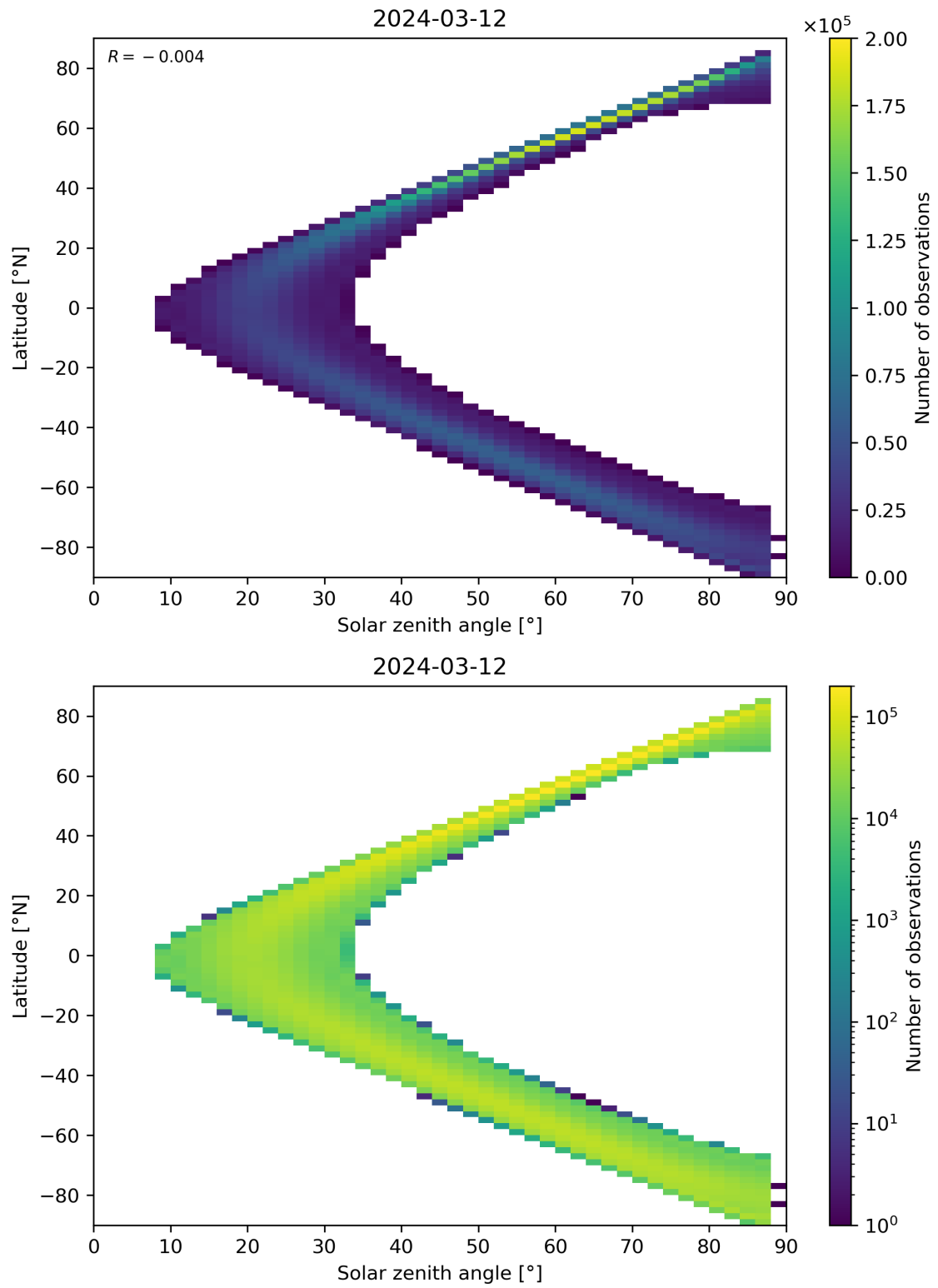
Figure 149: Scatter density plot of “Solar zenith angle” against “Latitude” for 2024-03-11 to 2024-03-13.
