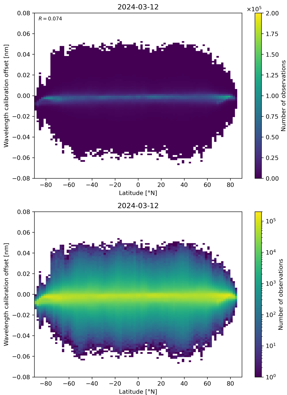
Figure 95: Scatter density plot of “Latitude” against “Wavelength calibration offset” for 2024-03-11 to 2024-03-13.
