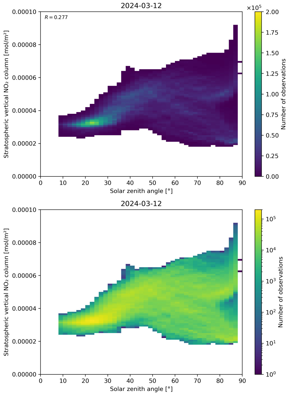
Figure 150: Scatter density plot of “Solar zenith angle” against “Stratospheric vertical NO 2 column” for 2024-03-11 to 2024-03-13.
