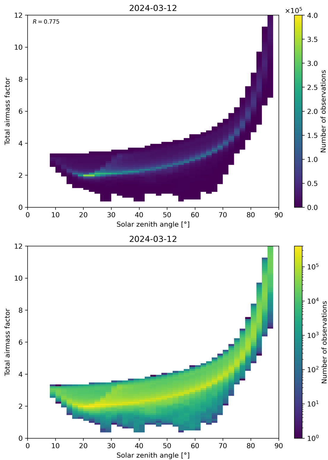
Figure 146: Scatter density plot of “Solar zenith angle” against “Total air mass factor” for 2024-03-11 to 2024-03-13.
