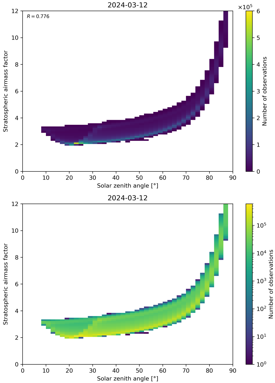
Figure 145: Scatter density plot of “Solar zenith angle” against “Stratospheric airmass factor” for 2024-03-11 to 2024-03-13.
