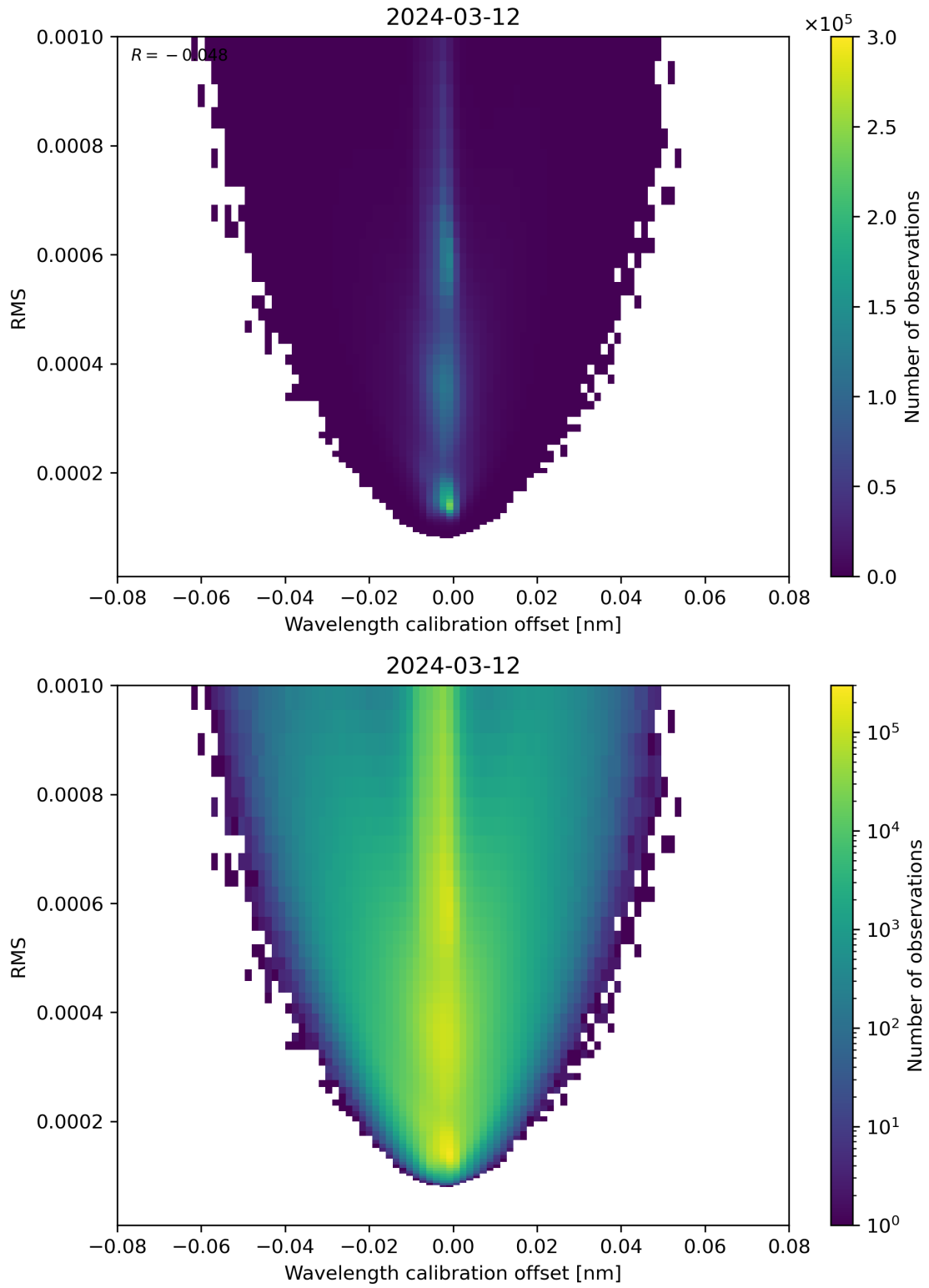
Figure 181: Scatter density plot of “Wavelength calibration offset” against “RMS” for 2024-03-11 to 2024-03-13.
