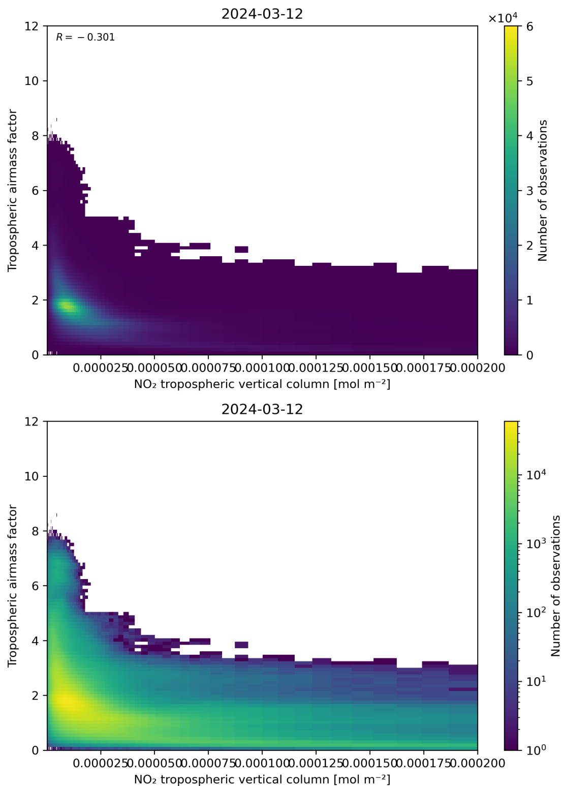
Figure 123: Scatter density plot of “NO 2 tropospheric vertical column” against “Tropospheric air mass factor” for 2024-03-11 to 2024-03-13.
