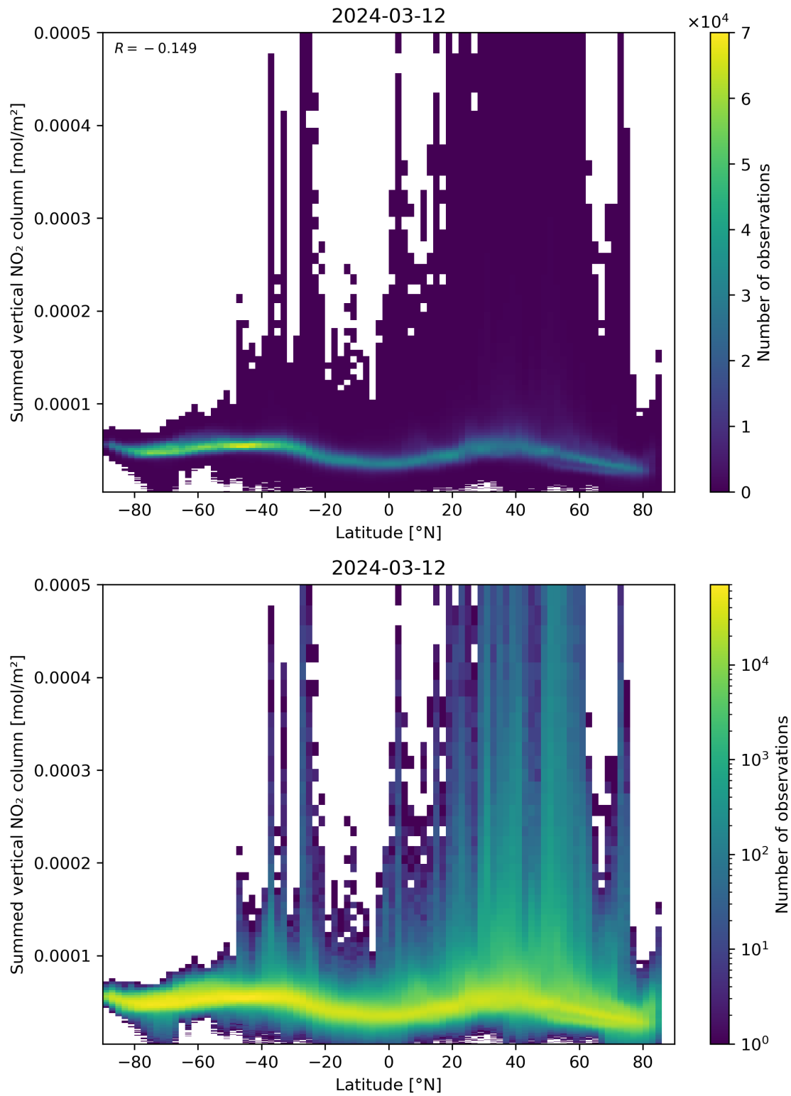
Figure 88: Scatter density plot of “Latitude” against “Summed vertical NO 2 column” for 2024-03-11 to 2024-03-13.
