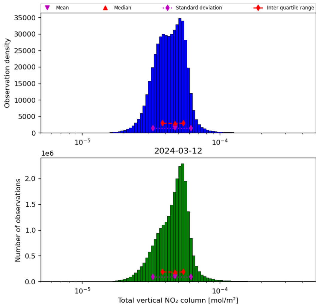
Figure 38: Histogram of “Total vertical NO 2 column” for 2024-03-11 to 2024-03-13
