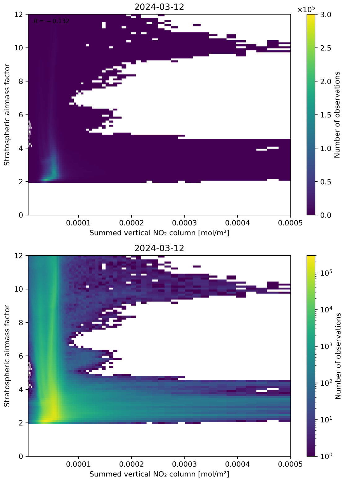
Figure 103: Scatter density plot of “Summed vertical NO 2 column” against “Stratospheric air mass factor” for 2024-03-11 to 2024-03-13.
