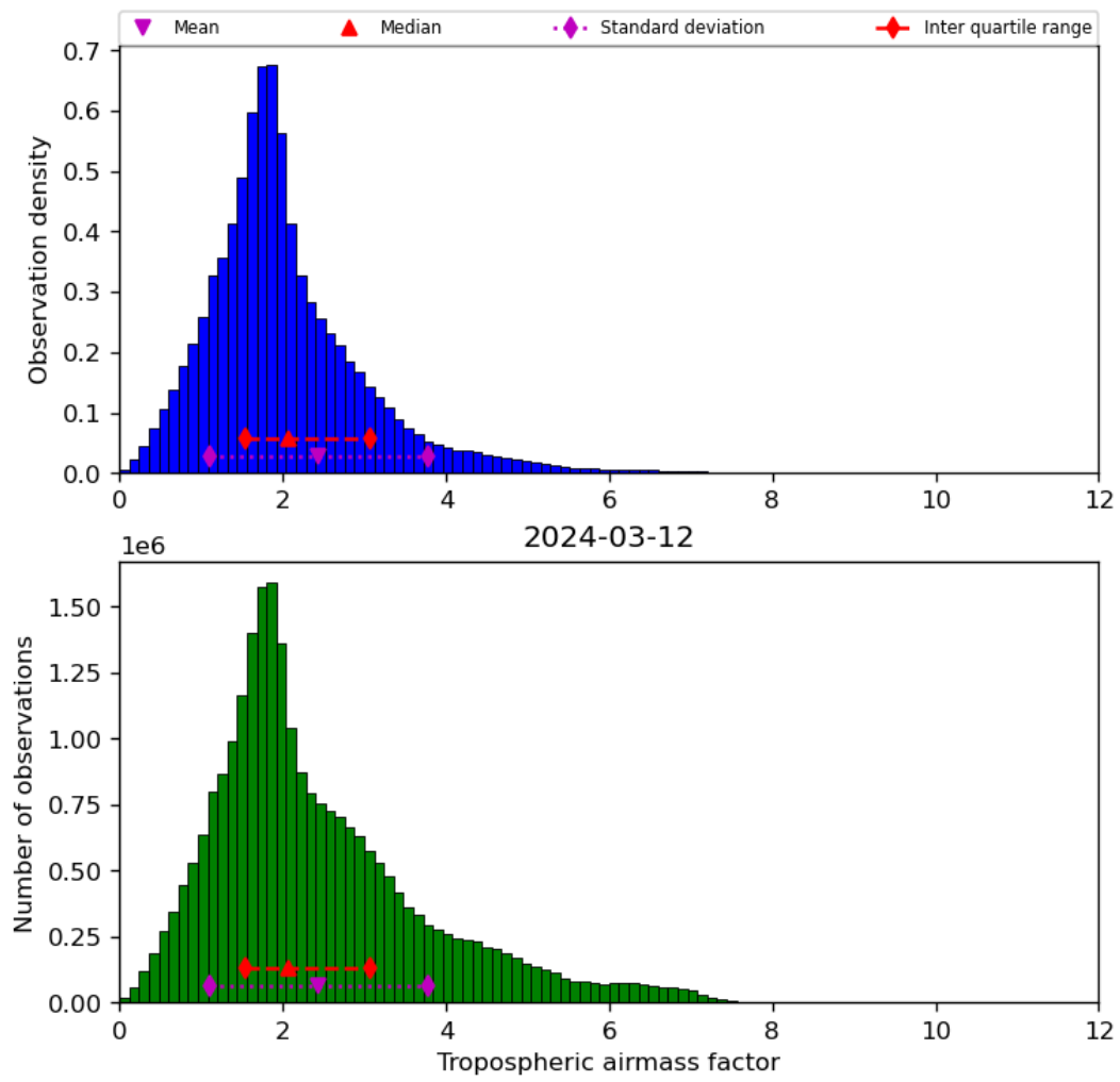
Figure 31: Histogram of “Tropospheric airmass factor” for 2024-03-11 to 2024-03-13
