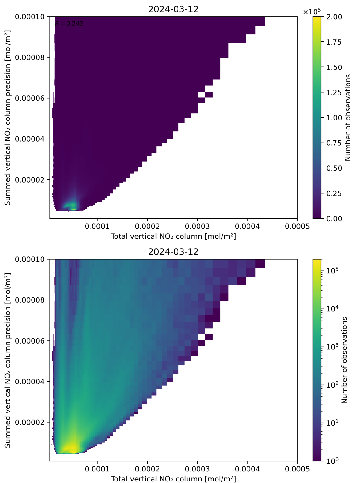
Figure 113: Scatter density plot of “Total vertical NO 2 column” against “Summed vertical NO 2 column precision” for 2024-03-11 to 2024-03-13.
