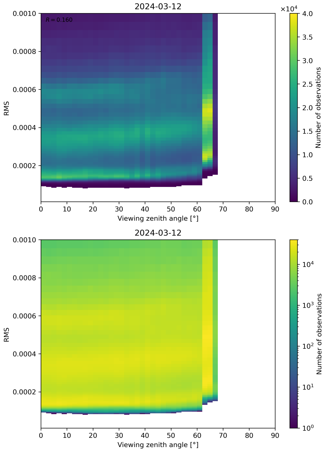
Figure 171: Scatter density plot of “Viewing zenith angle” against “RMS” for 2024-03-11 to 2024-03-13.
