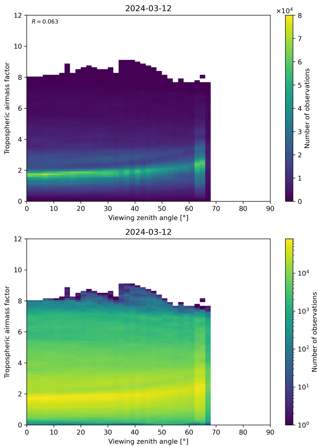
Figure 161: Scatter density plot of “Viewing zenith angle” against “Tropospheric airmass factor” for 2024-03-11 to 2024-03-13.
