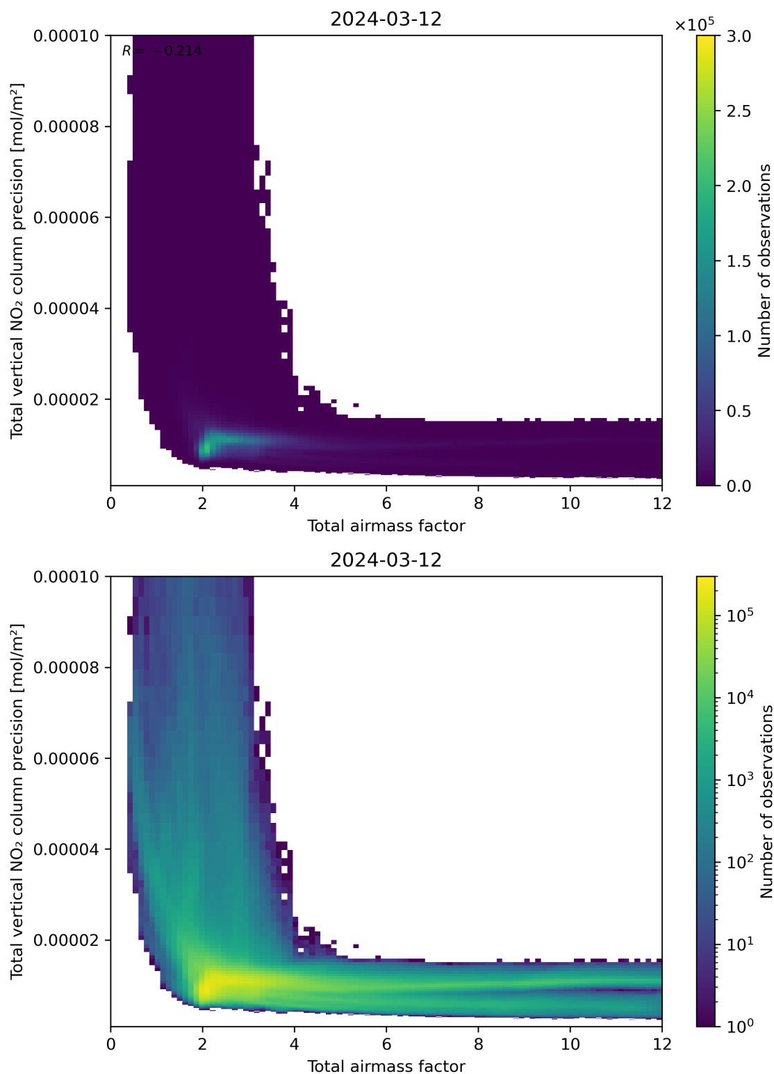
Figure 68: Scatter density plot of “Total airmass factor” against “Total vertical NO 2 column precision” for 2024-03-11 to 2024-03-13.
