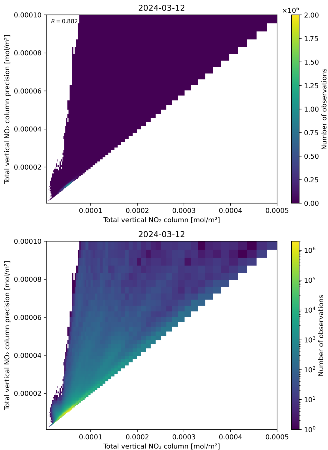
Figure 114: Scatter density plot of “Total vertical NO 2 column” against “Total vertical NO 2 column precision” for 2024-03-11 to 2024-03-13.
