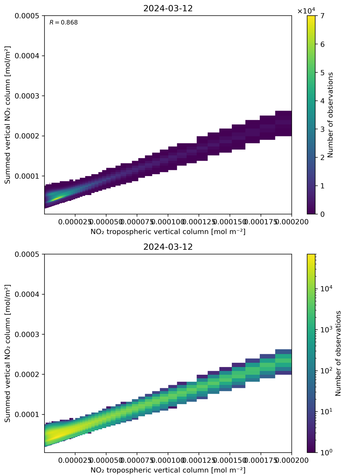
Figure 126: Scatter density plot of “NO 2 tropospheric vertical column” against “Summed vertical NO 2 column” for 2024-03-11 to 2024-03-13.
