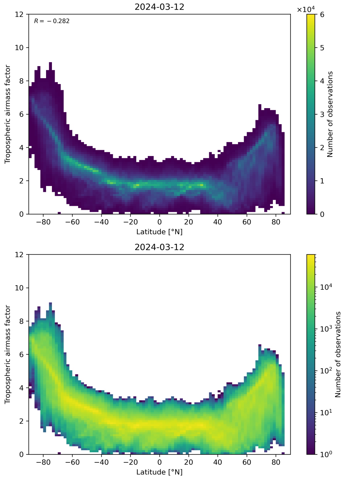
Figure 85: Scatter density plot of “Latitude” against “Tropospheric air mass factor” for 2024-03-11 to 2024-03-13.
