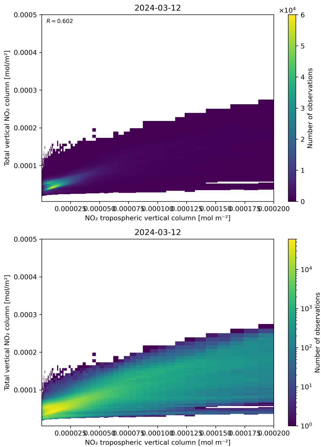
Figure 128: Scatter density plot of “NO 2 tropospheric vertical column” against “Total vertical NO 2 column” for 2024-03-11 to 2024-03-13.
