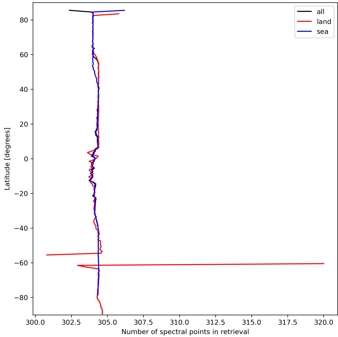
Figure 16: Zonal average of “Number of spectral points in retrieval” for 2024-03-11 to 2024-03-13.
