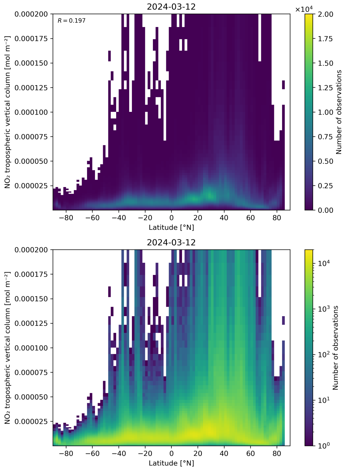
Figure 92: Scatter density plot of “Latitude” against “NO 2 tropospheric vertical column” for 2024-03-11 to 2024-03-13.
