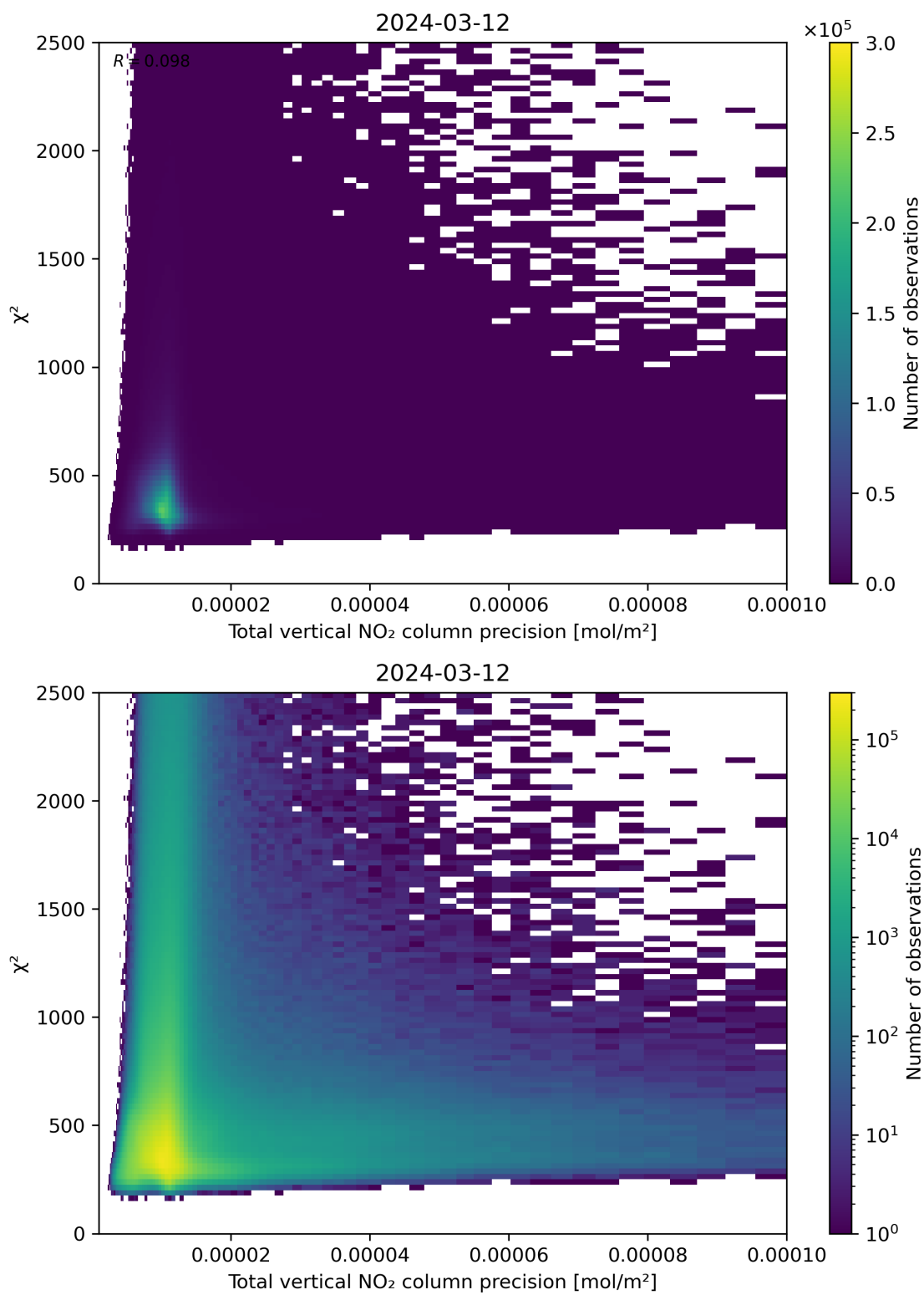
Figure 116: Scatter density plot of “Total vertical NO 2 column precision” against “ \chi^2 ” for 2024-03-11 to 2024-03-13.
