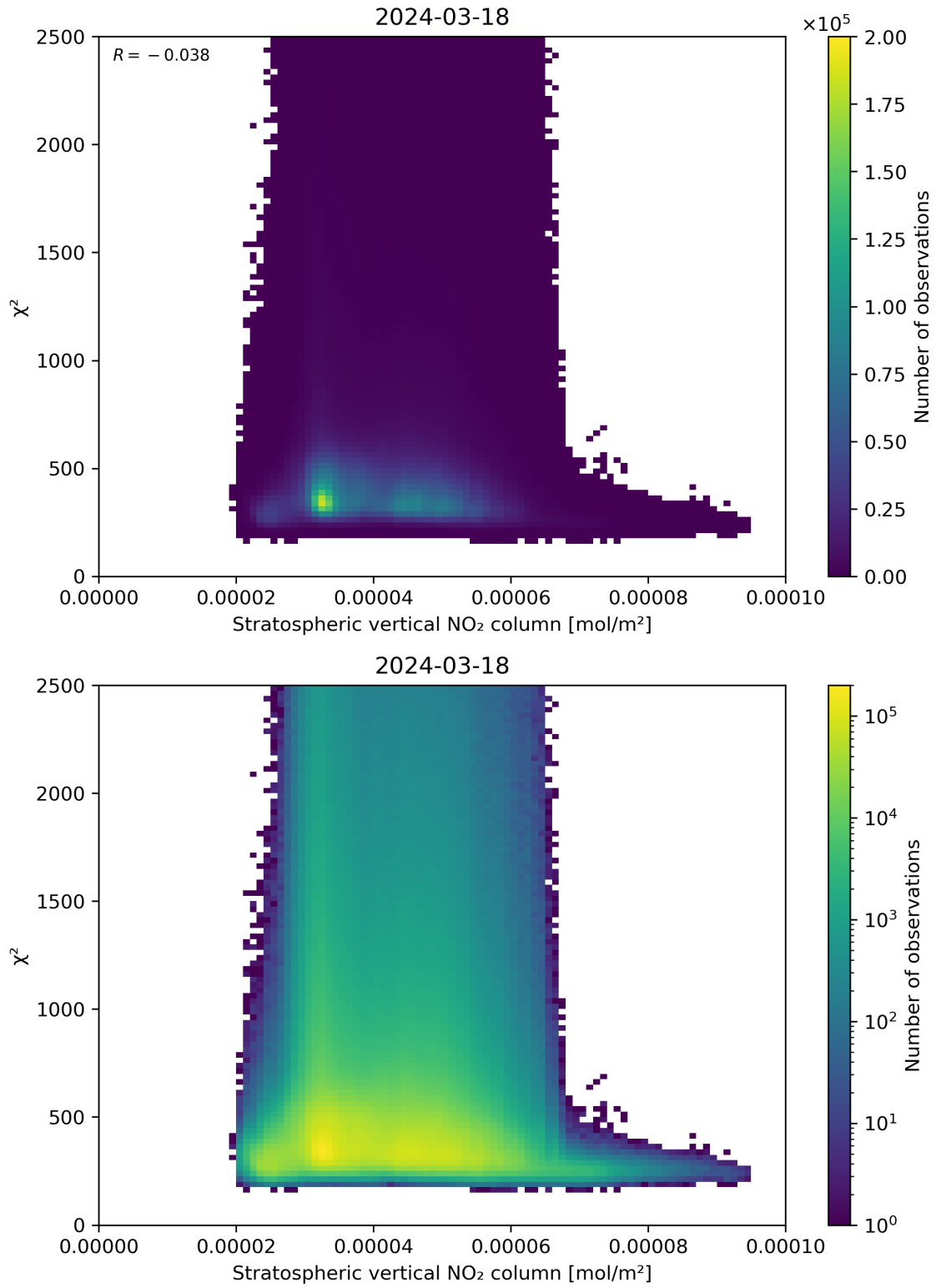
Figure 97: Scatter density plot of “Stratospheric vertical NO 2 column” against “ \chi^2 ” for 2024-03-17 to 2024-03-19.
