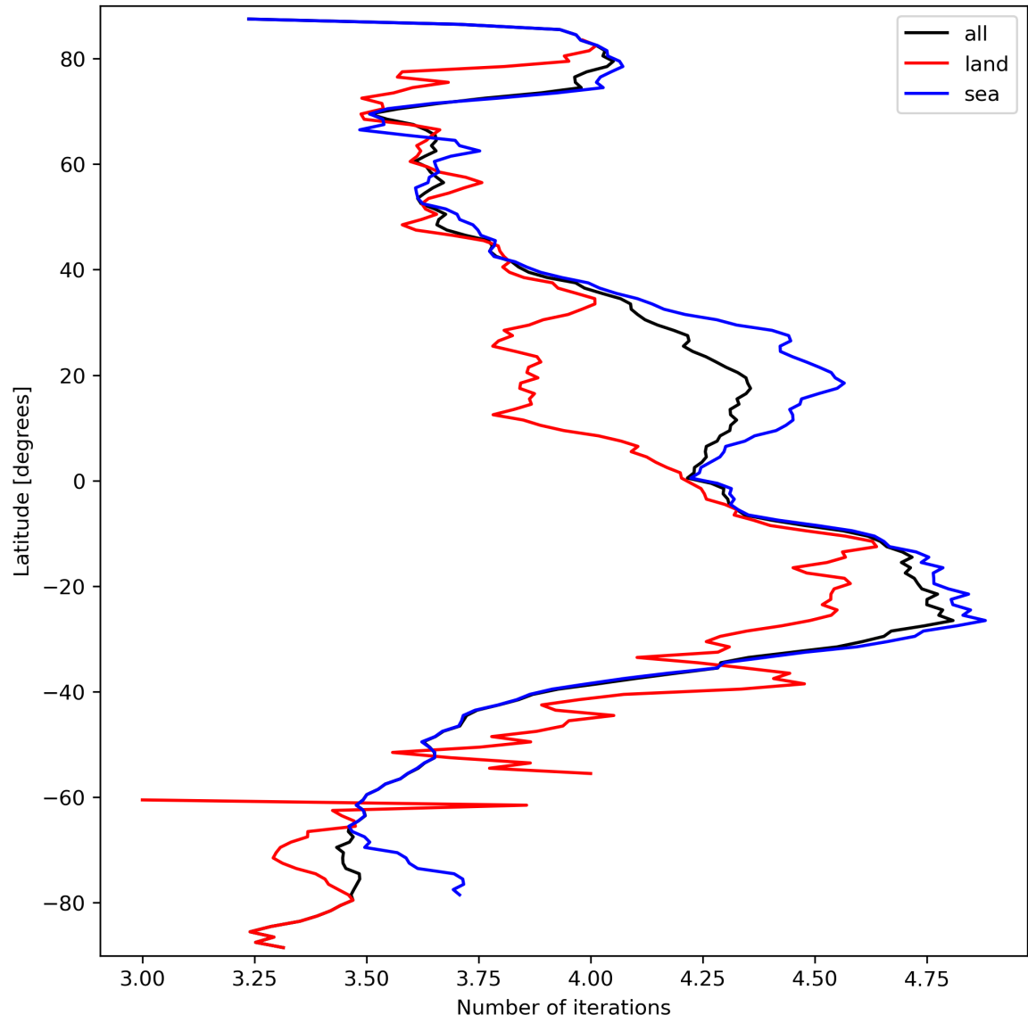
Figure 17: Zonal average of “Number of iterations” for 2024-03-17 to 2024-03-19.
