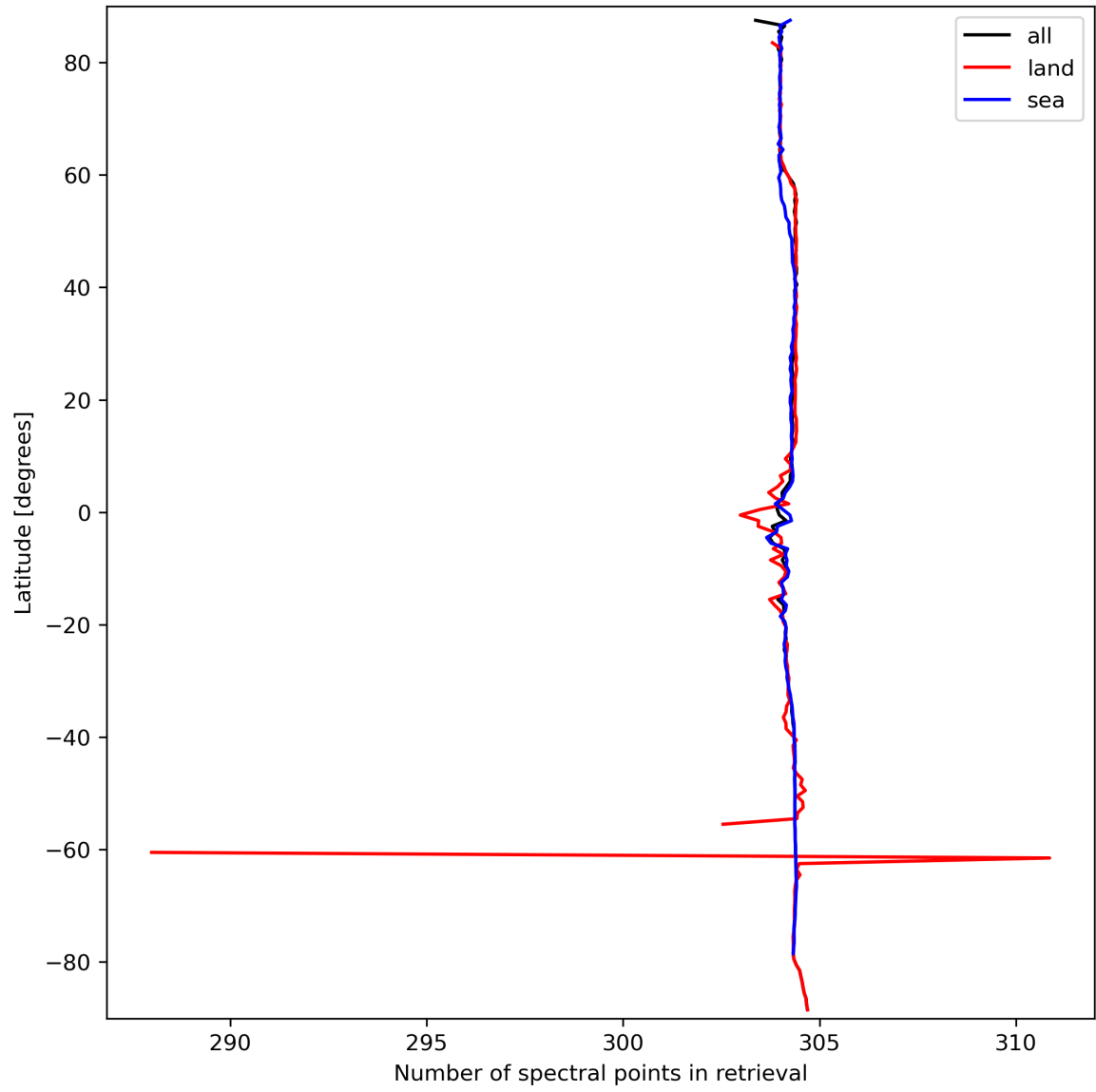
Figure 16: Zonal average of “Number of spectral points in retrieval” for 2024-03-17 to 2024-03-19.
