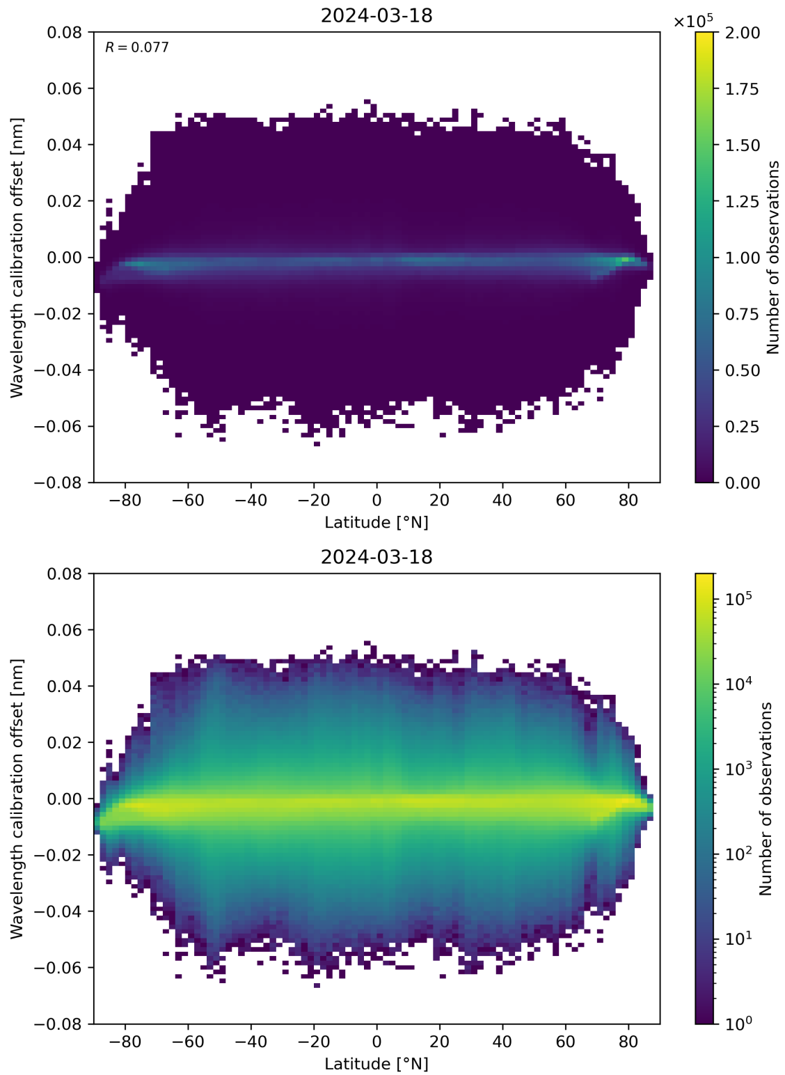
Figure 95: Scatter density plot of “Latitude” against “Wavelength calibration offset” for 2024-03-17 to 2024-03-19.
