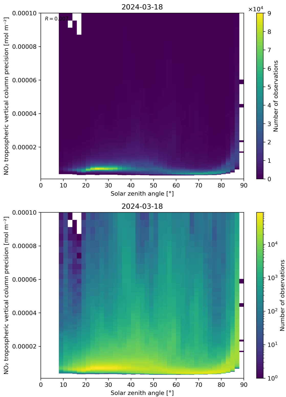
Figure 156: Scatter density plot of “Solar zenith angle” against “NO 2 tropospheric vertical column precision” for 2024-03-17 to 2024-03-19.
