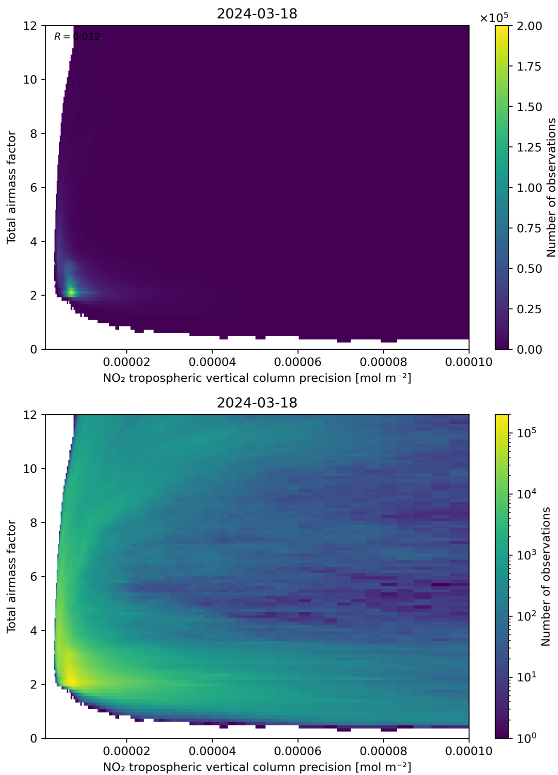
Figure 132: Scatter density plot of “NO 2 tropospheric vertical column precision” against “Total air mass factor” for 2024-03-17 to 2024-03-19.
