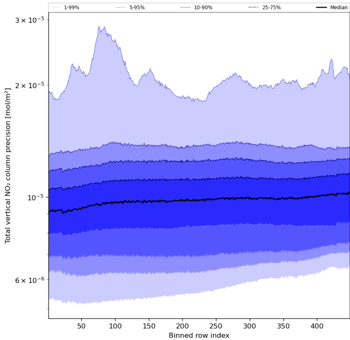
Figure 56: Along track statistics of “Total vertical NO 2 column precision” for 2024-03-17 to 2024-03-19
