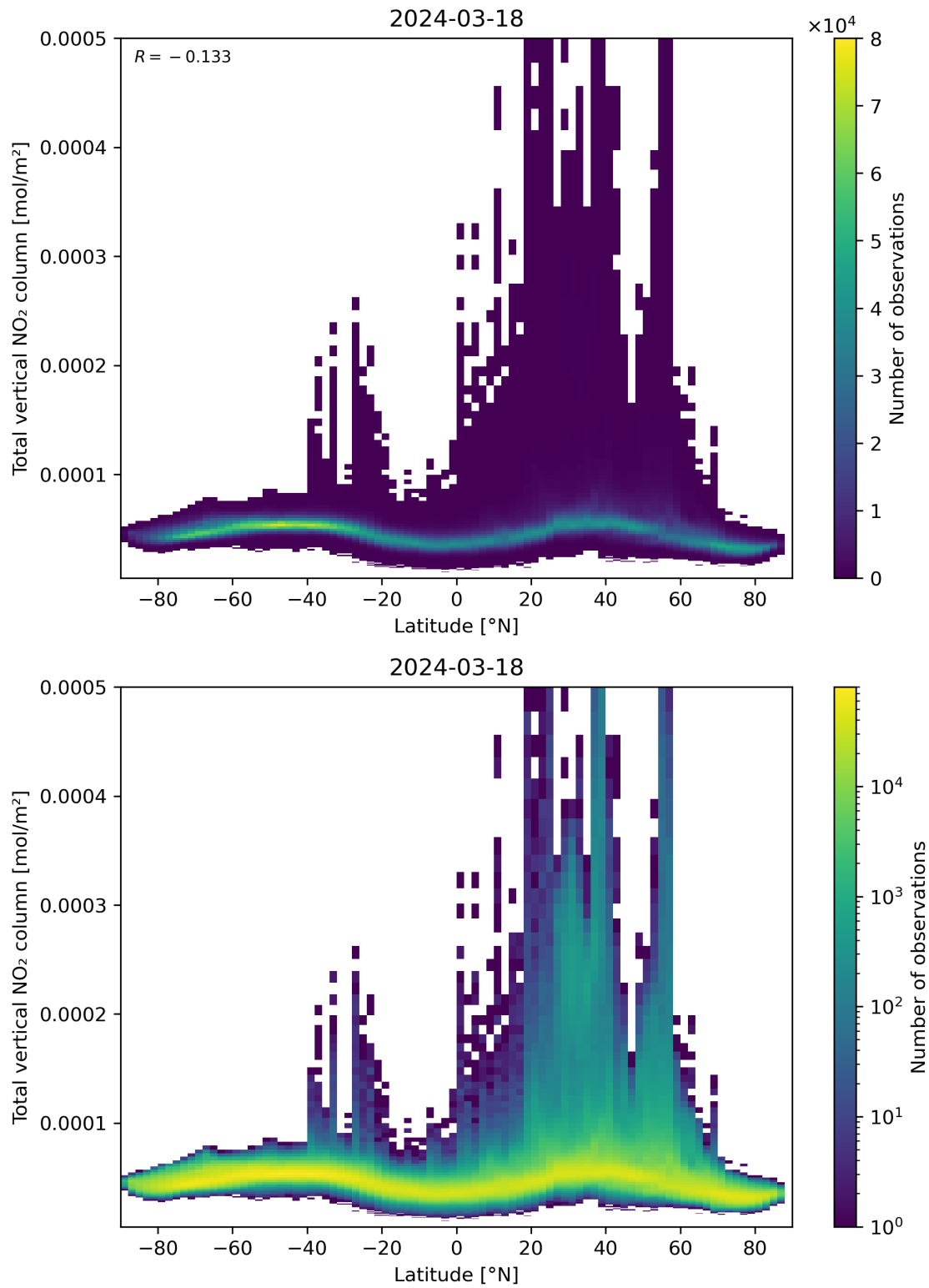
Figure 90: Scatter density plot of “Latitude” against “Total vertical NO 2 column” for 2024-03-17 to 2024-03-19.
