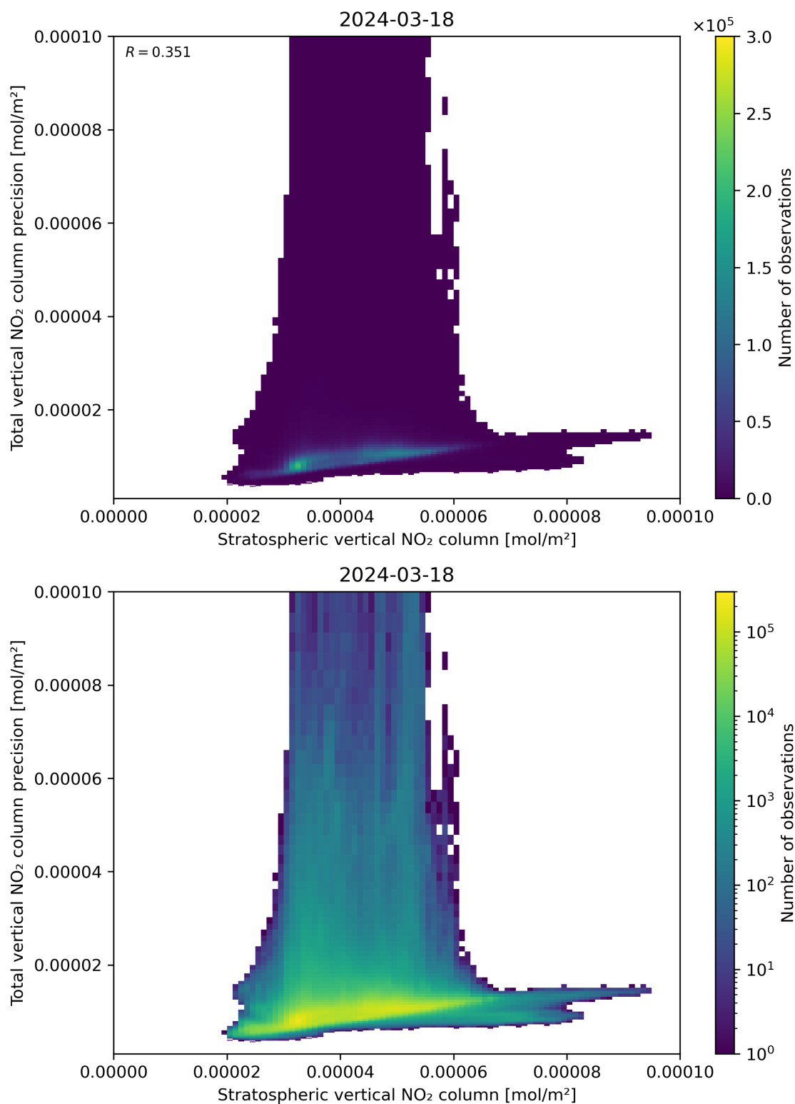
Figure 101: Scatter density plot of “Stratospheric vertical NO 2 column” against “Total vertical NO 2 column precision” for 2024-03-17 to 2024-03-19.
