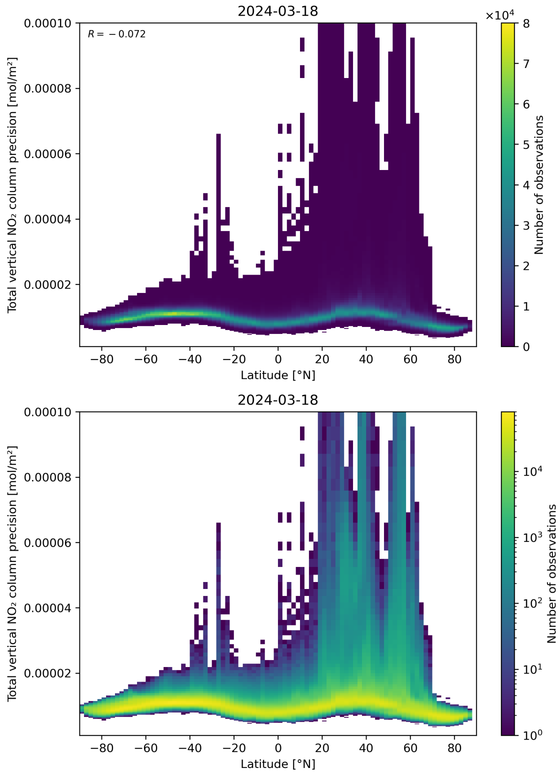
Figure 91: Scatter density plot of “Latitude” against “Total vertical NO 2 column precision” for 2024-03-17 to 2024-03-19.
