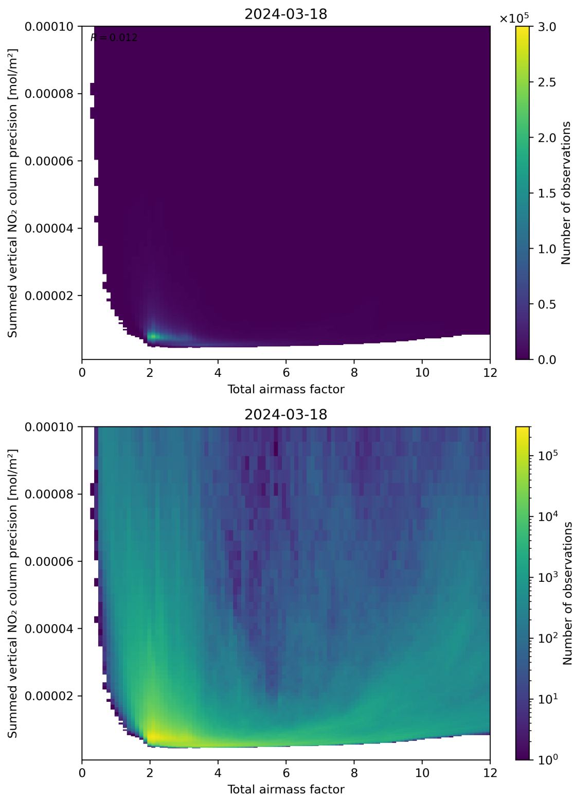
Figure 66: Scatter density plot of “Total airmass factor” against “Summed vertical NO 2 column precision” for 2024-03-17 to 2024-03-19.
