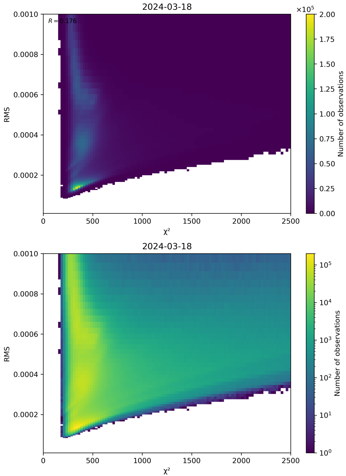
Figure 82: Scatter density plot of “ \chi^2 ” against “RMS” for 2024-03-17 to 2024-03-19.
