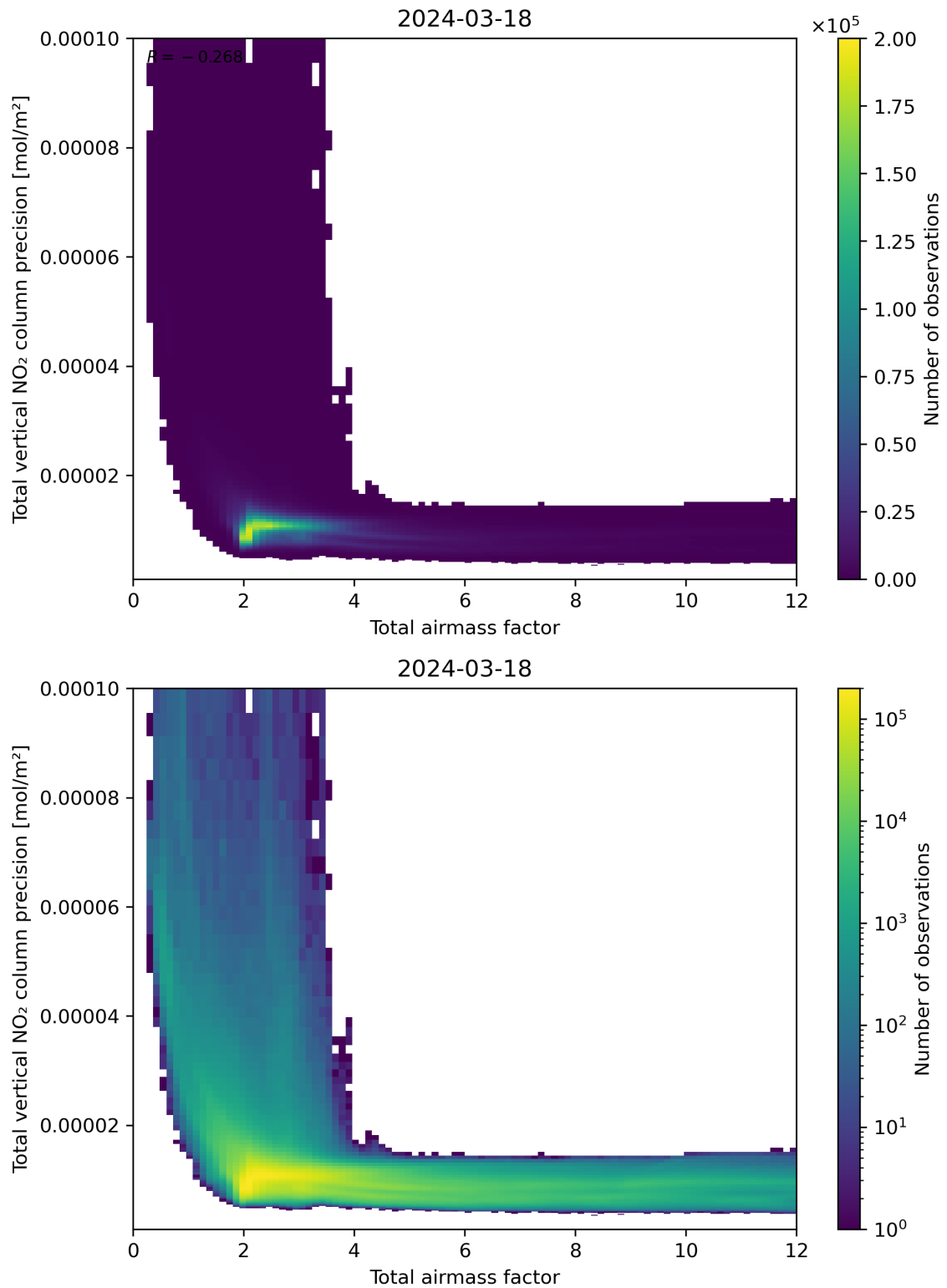
Figure 68: Scatter density plot of “Total airmass factor” against “Total vertical NO 2 column precision” for 2024-03-17 to 2024-03-19.
