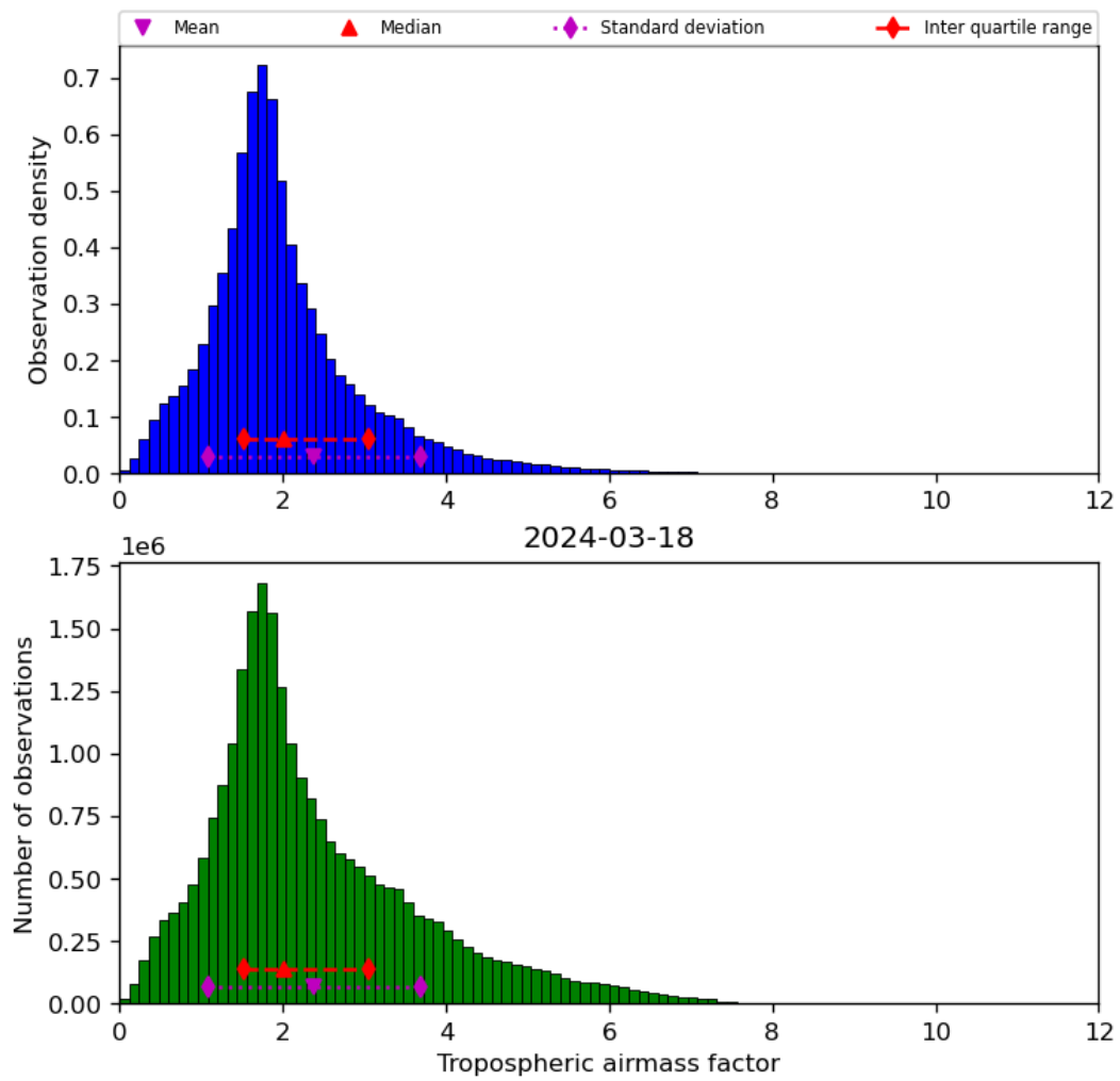
Figure 31: Histogram of “Tropospheric airmass factor” for 2024-03-17 to 2024-03-19
