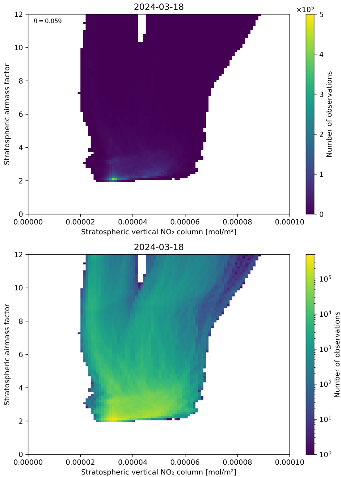
Figure 96: Scatter density plot of “Stratospheric vertical NO 2 column” against “Stratospheric airmass factor” for 2024-03-17 to 2024-03-19.
