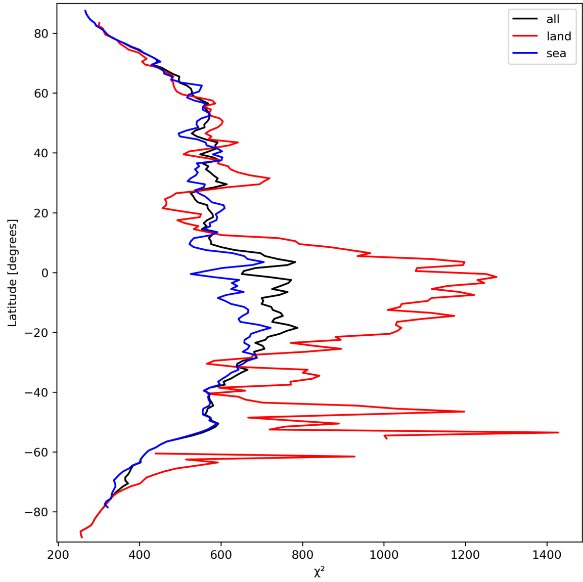
Figure 25: Zonal average of “ \chi^2 ” for 2024-03-17 to 2024-03-19.
