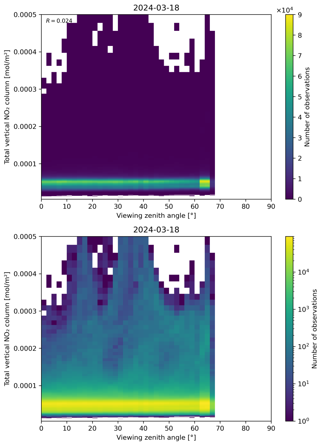
Figure 167: Scatter density plot of “Viewing zenith angle” against “Total vertical NO 2 column” for 2024-03-17 to 2024-03-19.
