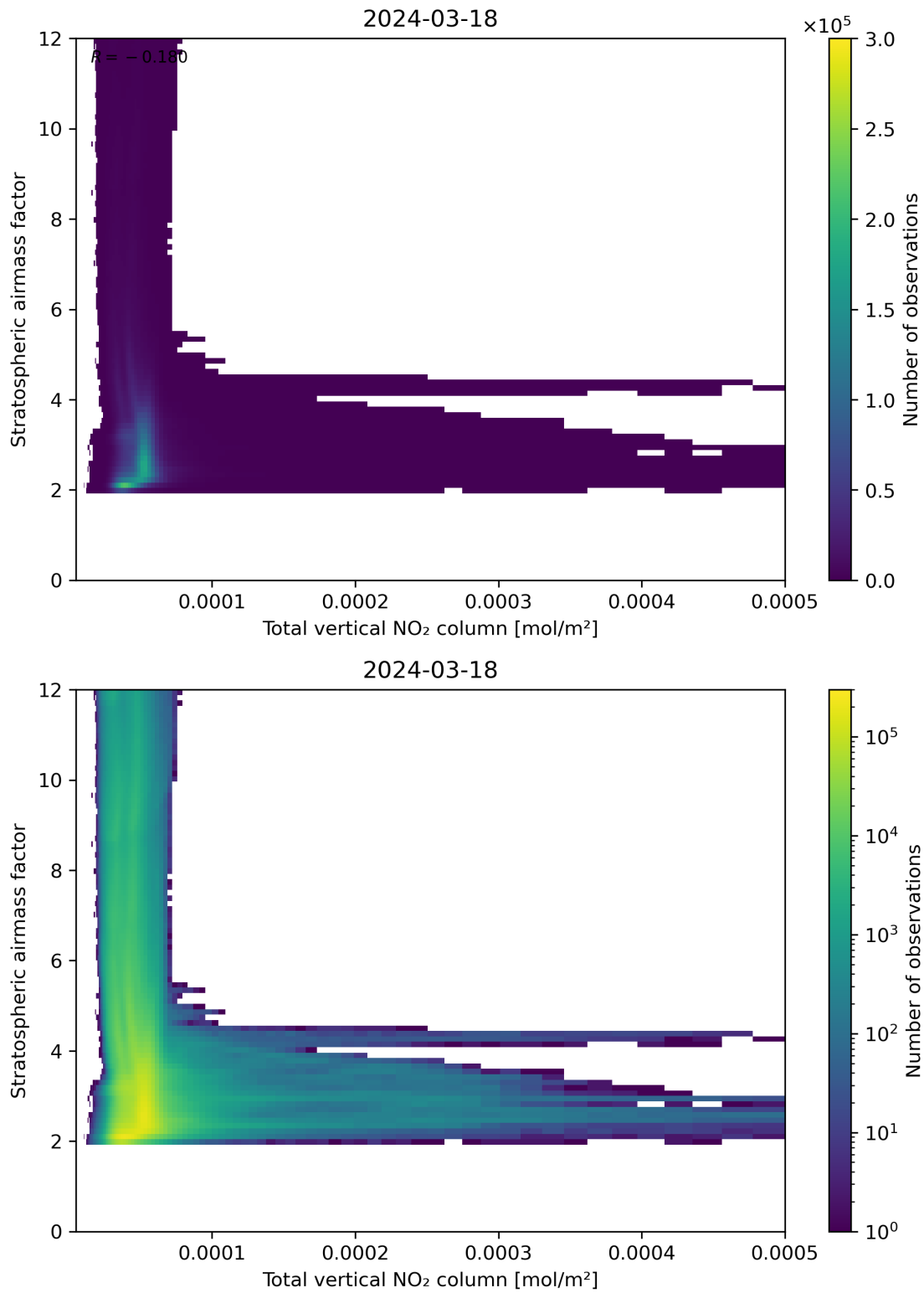
Figure 110: Scatter density plot of “Total vertical NO 2 column” against “Stratospheric airmass factor” for 2024-03-17 to 2024-03-19.
