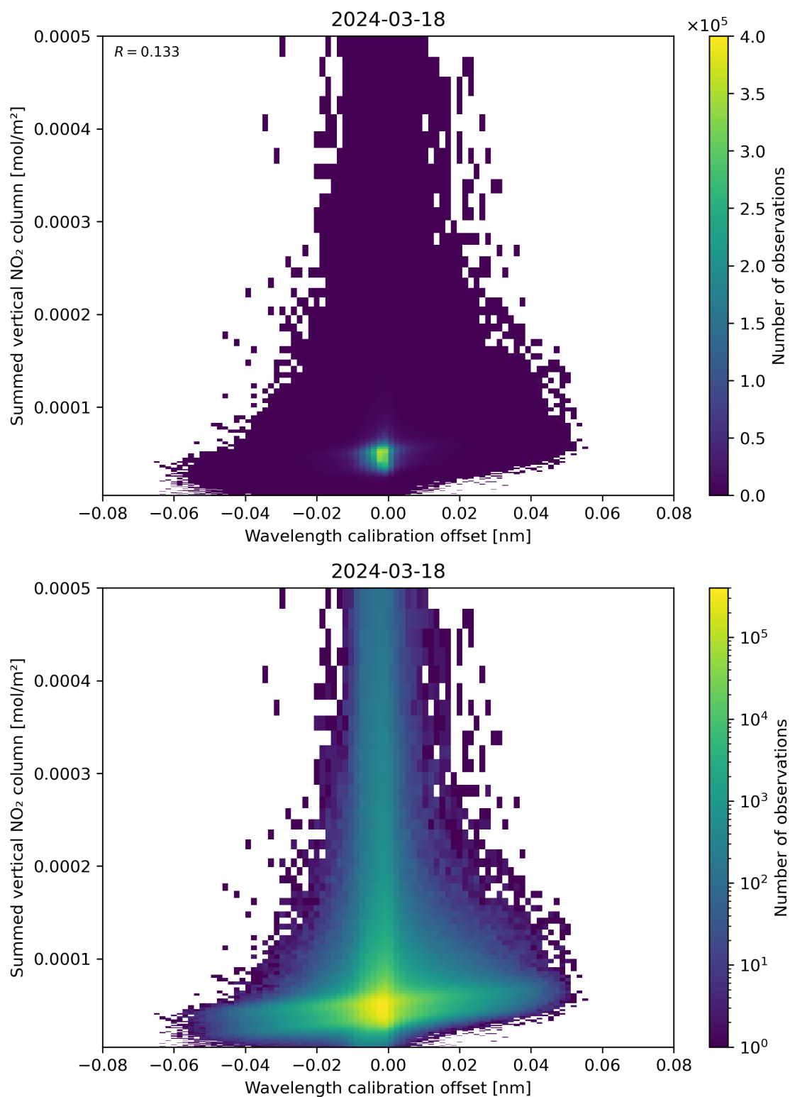
Figure 177: Scatter density plot of “Wavelength calibration offset” against “Summed vertical NO 2 column” for 2024-03-17 to 2024-03-19.
