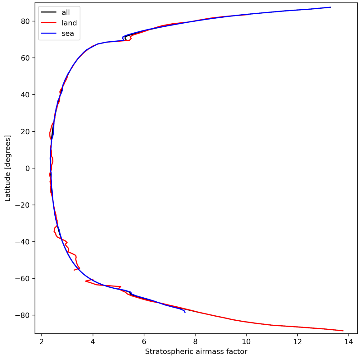
Figure 27: Zonal average of “Stratospheric air mass factor” for 2024-03-17 to 2024-03-19.
