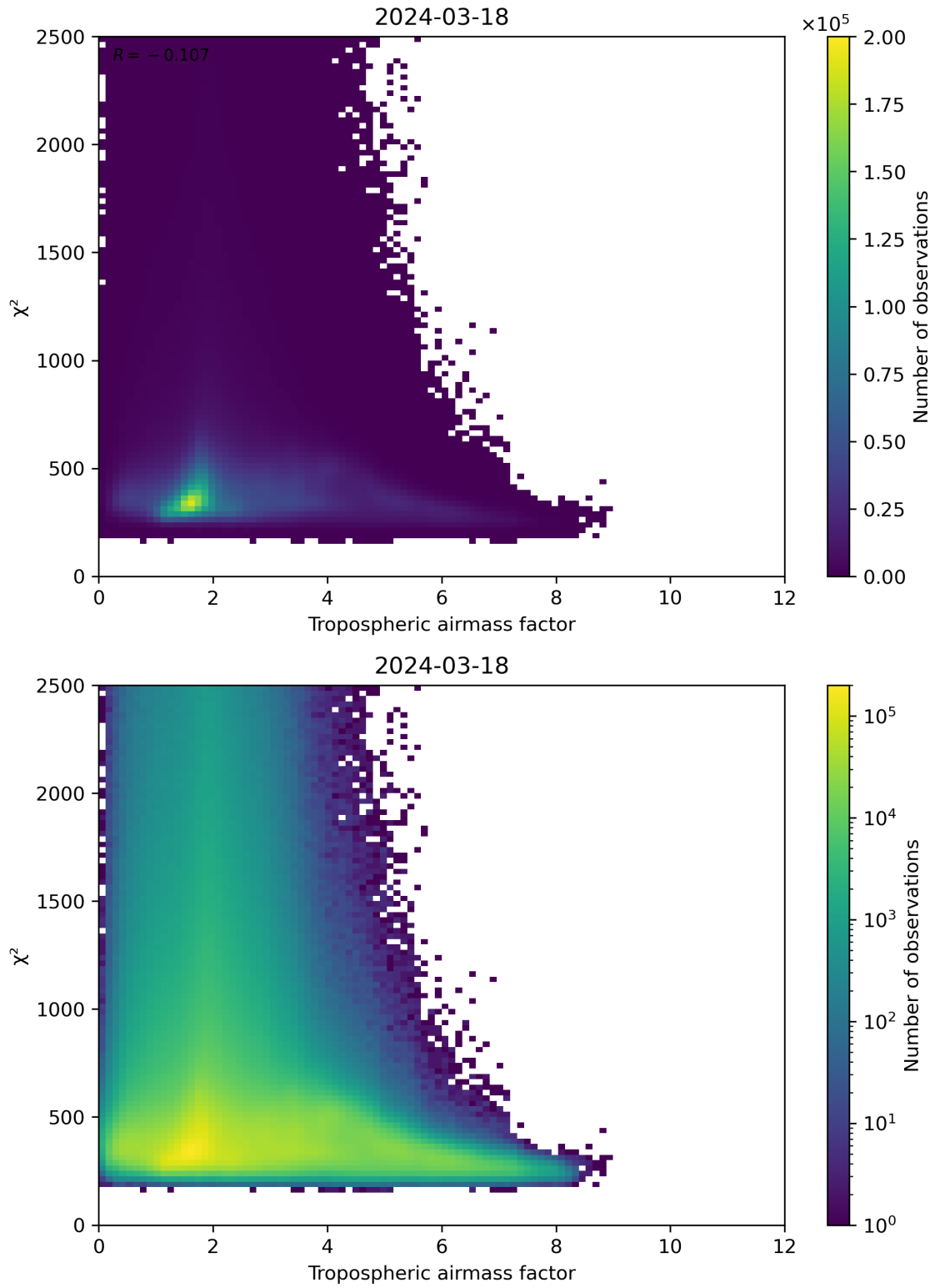
Figure 73: Scatter density plot of “Tropospheric airmass factor” against “ \chi^2 ” for 2024-03-17 to 2024-03-19.
