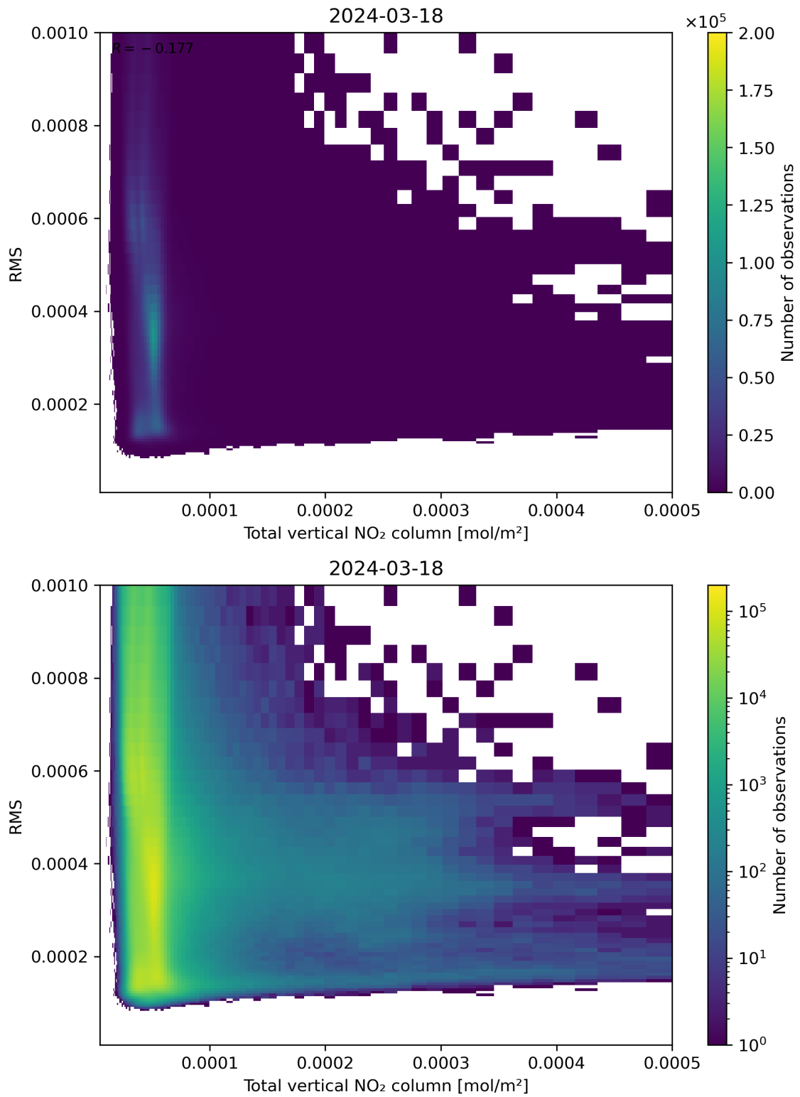
Figure 120: Scatter density plot of “Total vertical NO 2 column” against “RMS” for 2024-03-17 to 2024-03-19.
