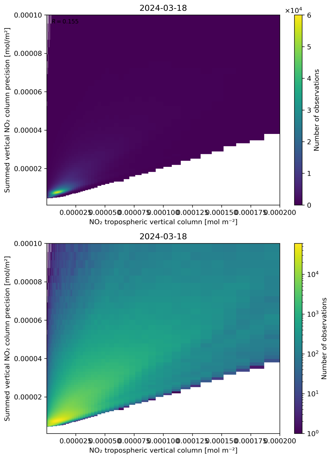
Figure 127: Scatter density plot of “NO 2 tropospheric vertical column” against “Summed vertical NO 2 column precision” for 2024-03-17 to 2024-03-19.
