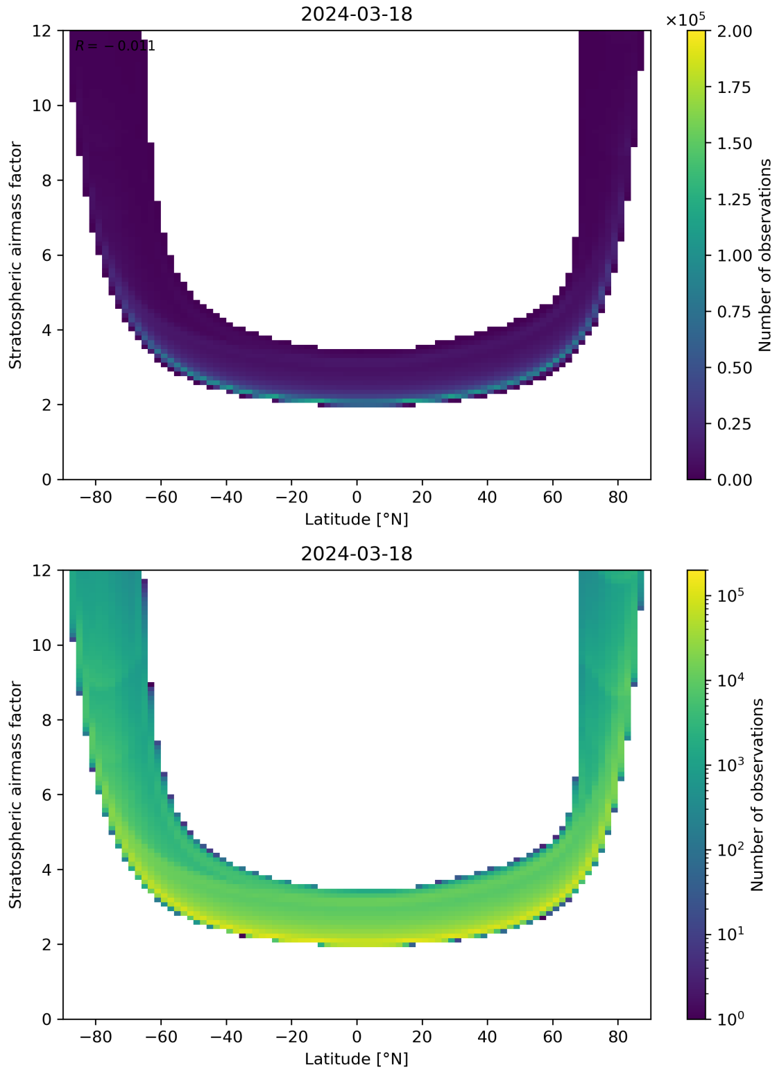
Figure 83: Scatter density plot of “Latitude” against “Stratospheric air mass factor” for 2024-03-17 to 2024-03-19.
