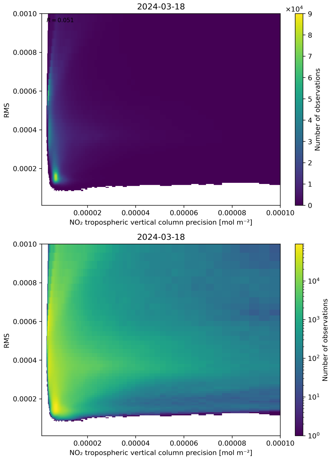
Figure 140: Scatter density plot of “NO 2 tropospheric vertical column precision” against “RMS” for 2024-03-17 to 2024-03-19.
