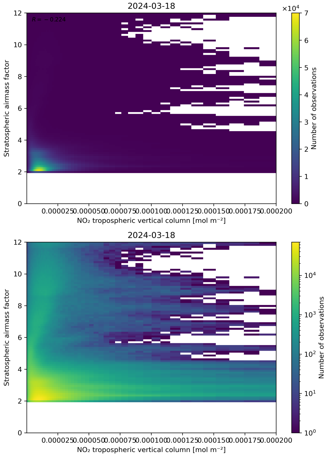
Figure 121: Scatter density plot of “NO 2 tropospheric vertical column” against “Stratospheric air mass factor” for 2024-03-17 to 2024-03-19.
