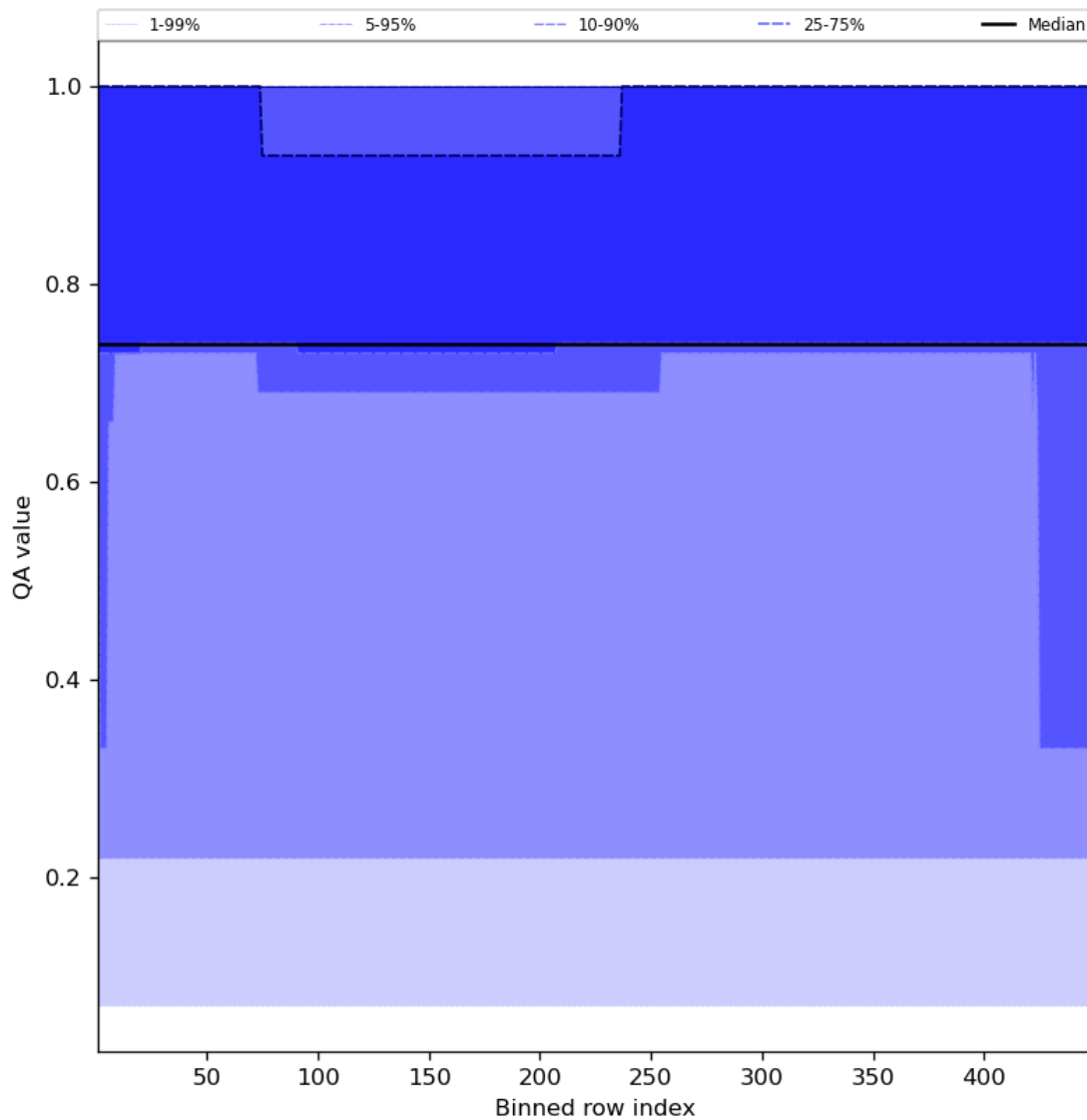
Figure 45: Along track statistics of “QA value” for 2024-03-17 to 2024-03-19
