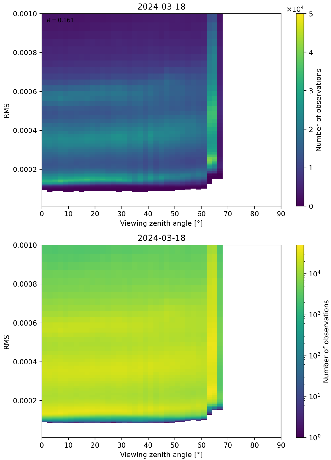
Figure 171: Scatter density plot of “Viewing zenith angle” against “RMS” for 2024-03-17 to 2024-03-19.
