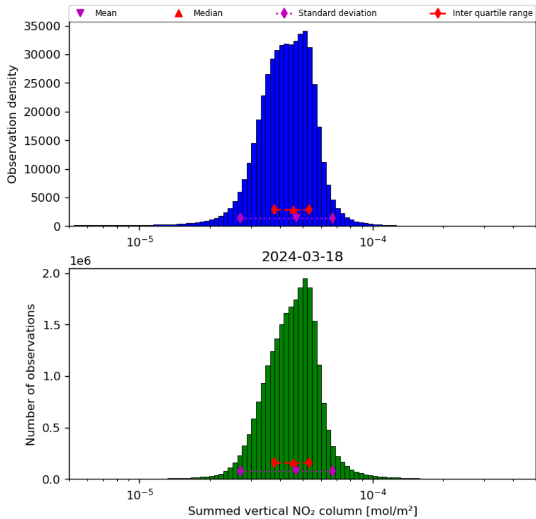
Figure 40: Histogram of “Summed vertical NO 2 column” for 2024-03-17 to 2024-03-19
