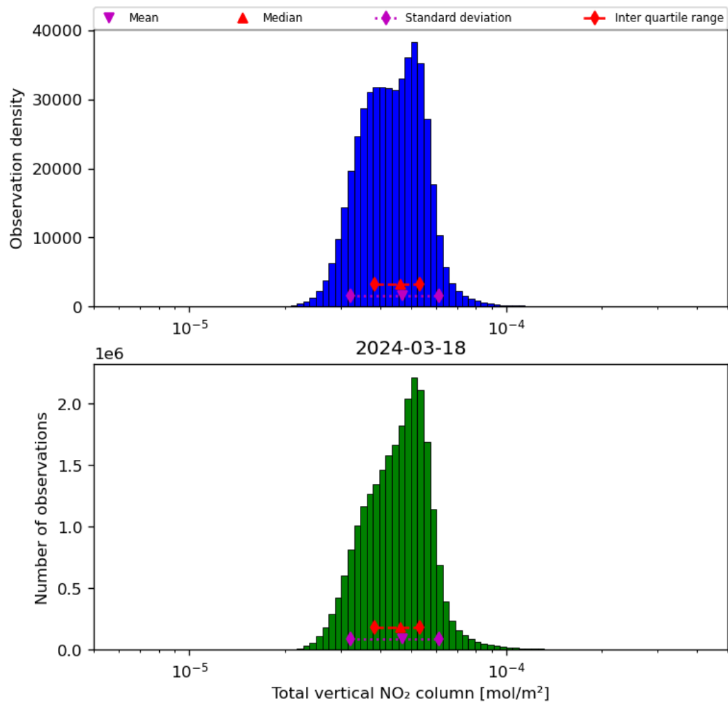
Figure 38: Histogram of "Total vertical NO 2 column" for 2024-03-17 to 2024-03-19
