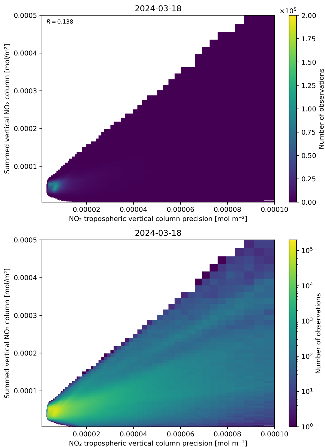
Figure 136: Scatter density plot of “NO 2 tropospheric vertical column precision” against “Summed vertical NO 2 column” for 2024-03-17 to 2024-03-19.
