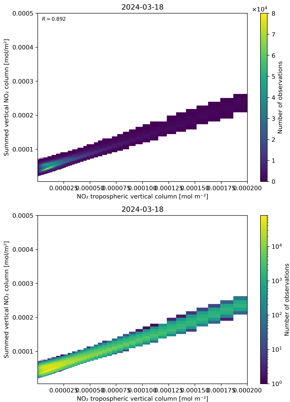
Figure 126: Scatter density plot of “NO 2 tropospheric vertical column” against “Summed vertical NO 2 column” for 2024-03-17 to 2024-03-19.
