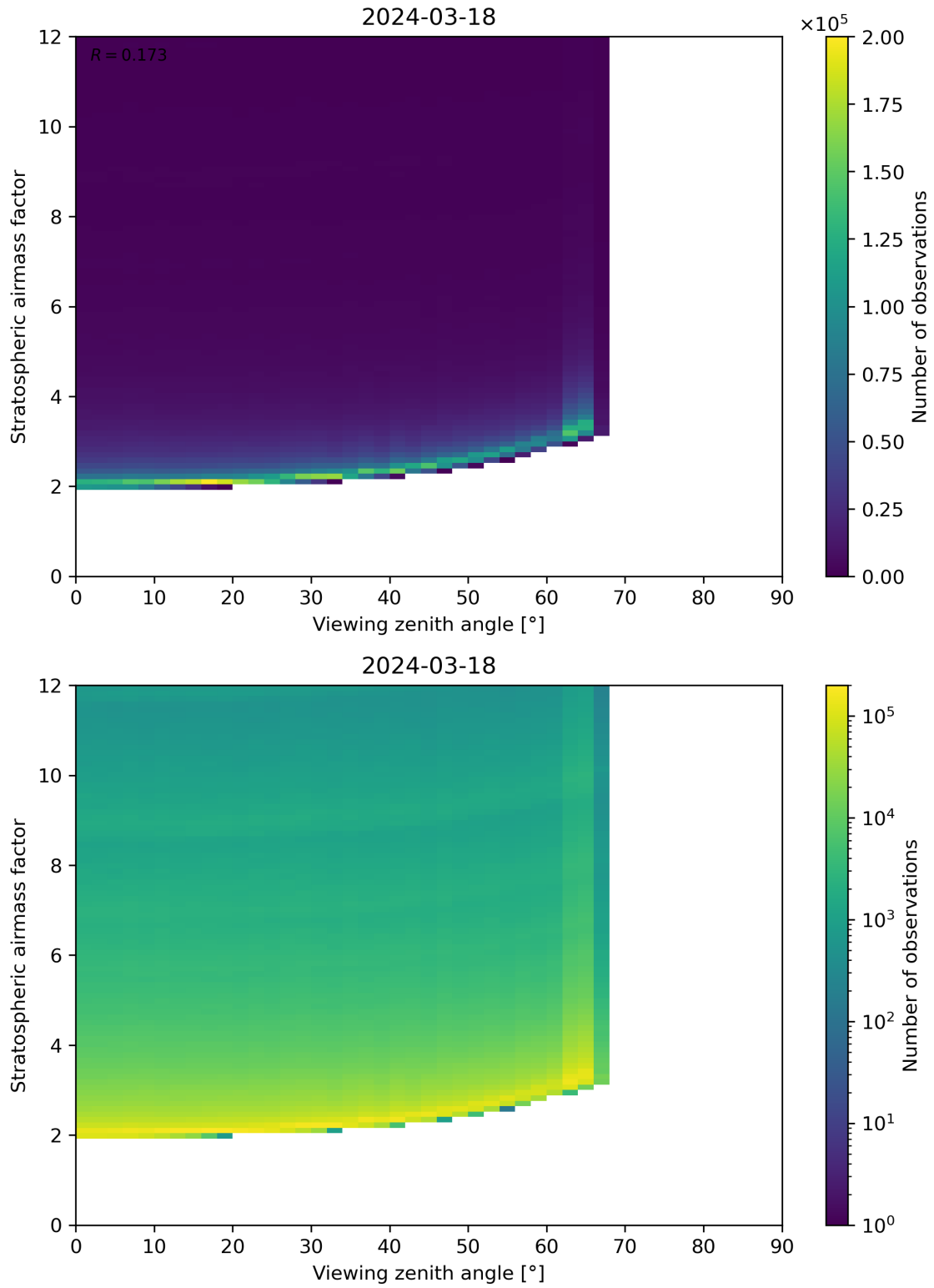
Figure 159: Scatter density plot of “Viewing zenith angle” against “Stratospheric airmass factor” for 2024-03-17 to 2024-03-19.
