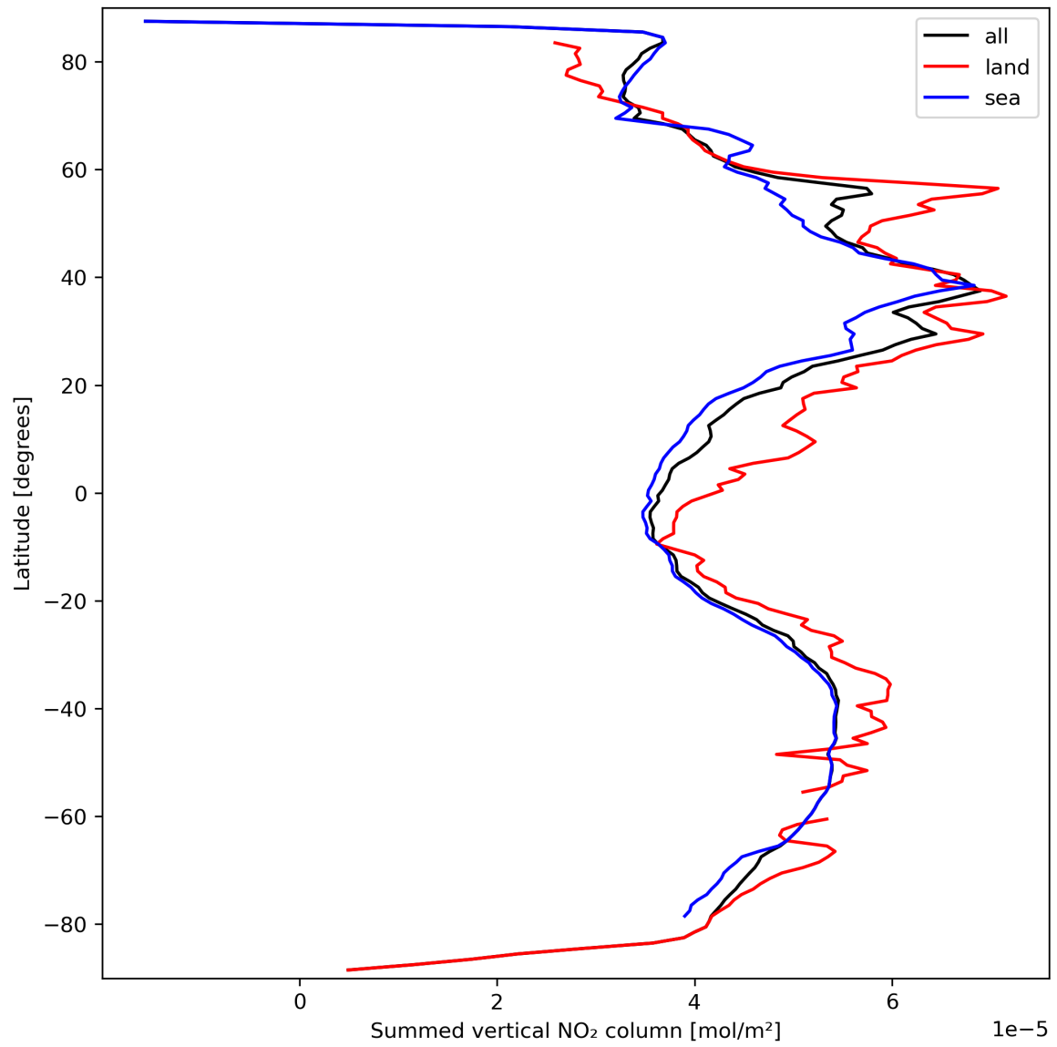
Figure 23: Zonal average of “Summed vertical NO 2 column” for 2024-03-17 to 2024-03-19.
