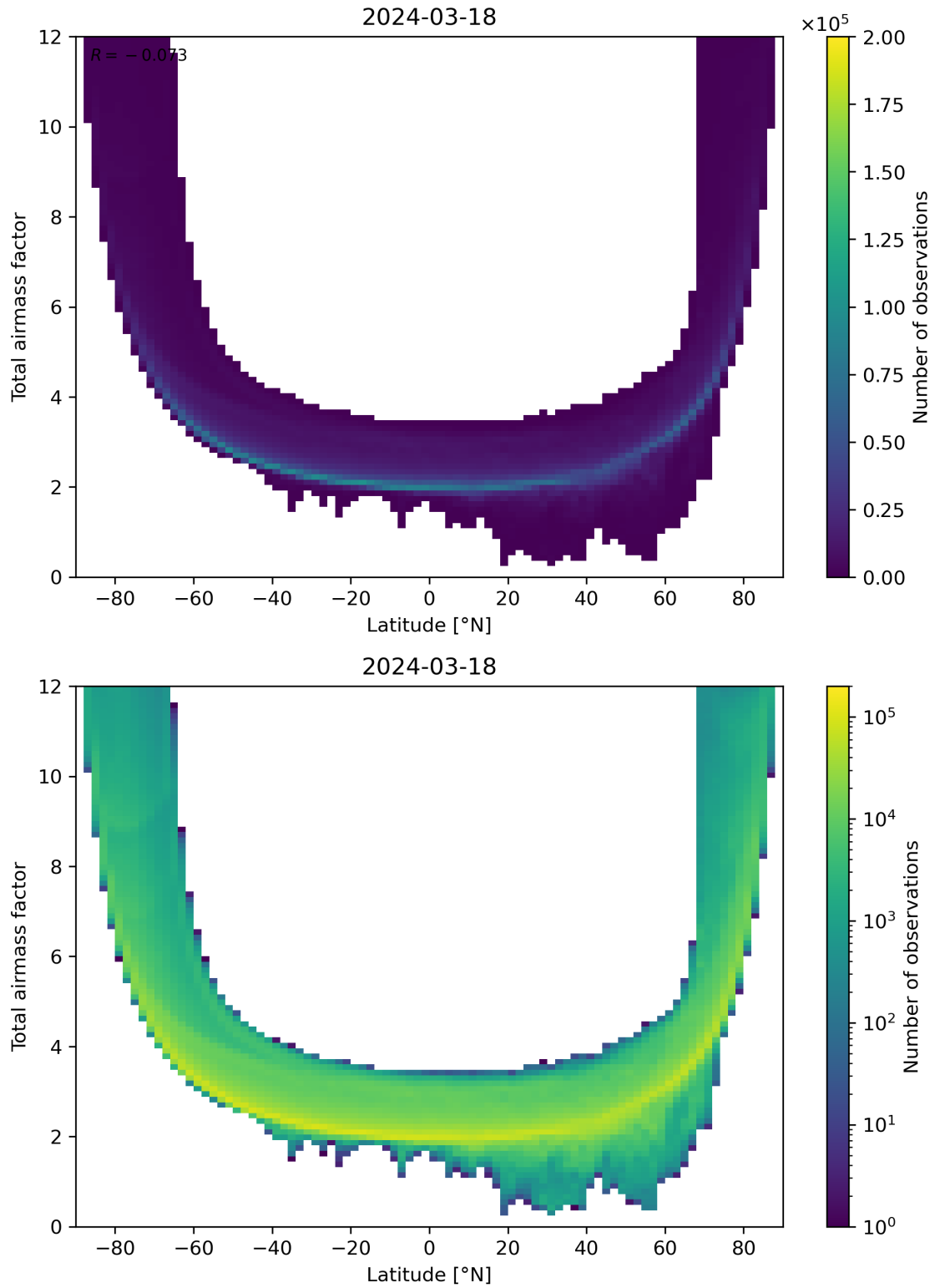
Figure 84: Scatter density plot of “Latitude” against “Total airmass factor” for 2024-03-17 to 2024-03-19.
