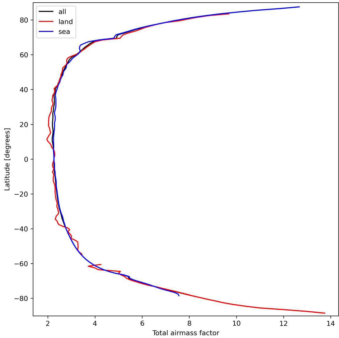
Figure 15: Zonal average of “Total airmass factor” for 2024-03-17 to 2024-03-19.
