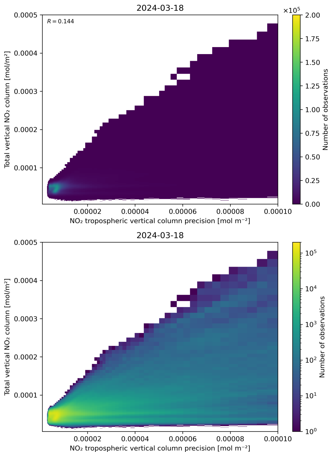
Figure 138: Scatter density plot of “NO 2 tropospheric vertical column precision” against “Total vertical NO 2 column” for 2024-03-17 to 2024-03-19.
