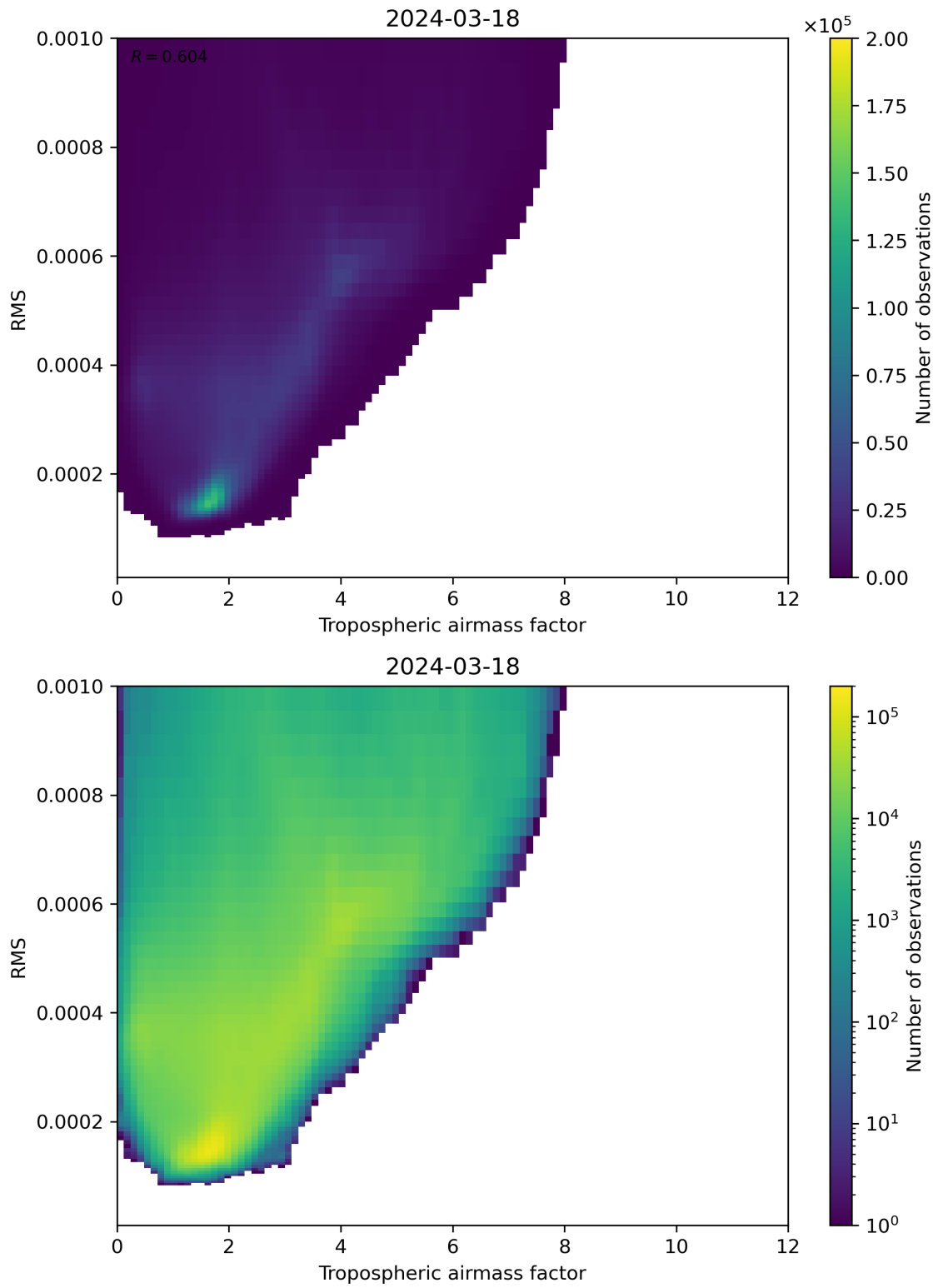
Figure 79: Scatter density plot of “Tropospheric airmass factor” against “RMS” for 2024-03-17 to 2024-03-19.
