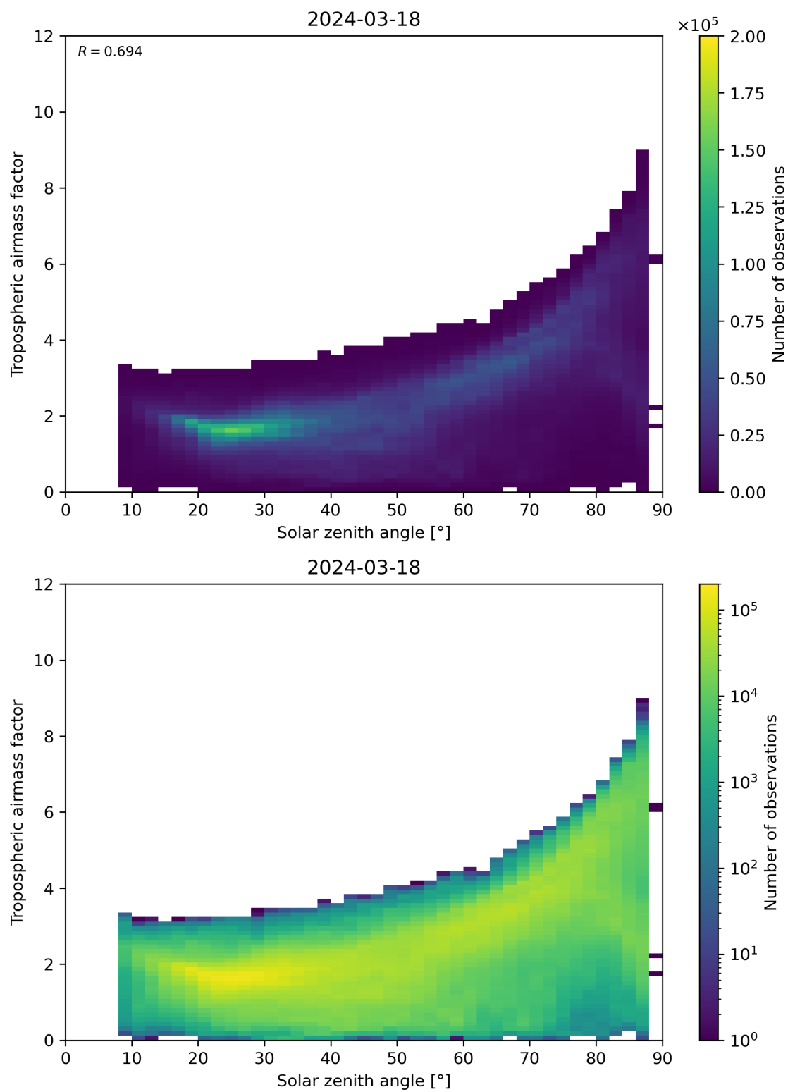
Figure 147: Scatter density plot of “Solar zenith angle” against “Tropospheric airmass factor” for 2024-03-17 to 2024-03-19.
