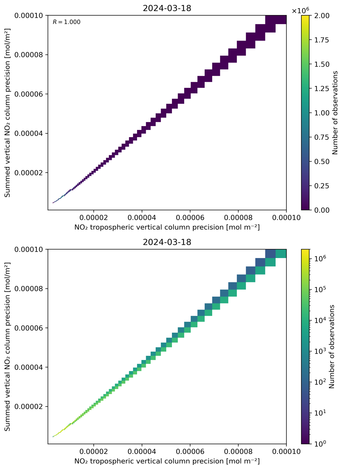
Figure 137: Scatter density plot of “NO 2 tropospheric vertical column precision” against “Summed vertical NO 2 column precision” for 2024-03-17 to 2024-03-19.
