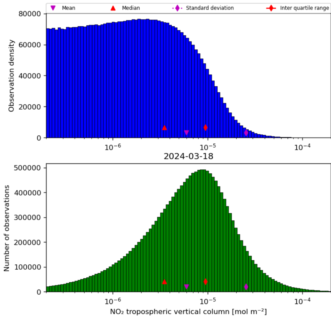
Figure 29: Histogram of “ \text{NO}_2 tropospheric vertical column” for 2024-03-17 to 2024-03-19
