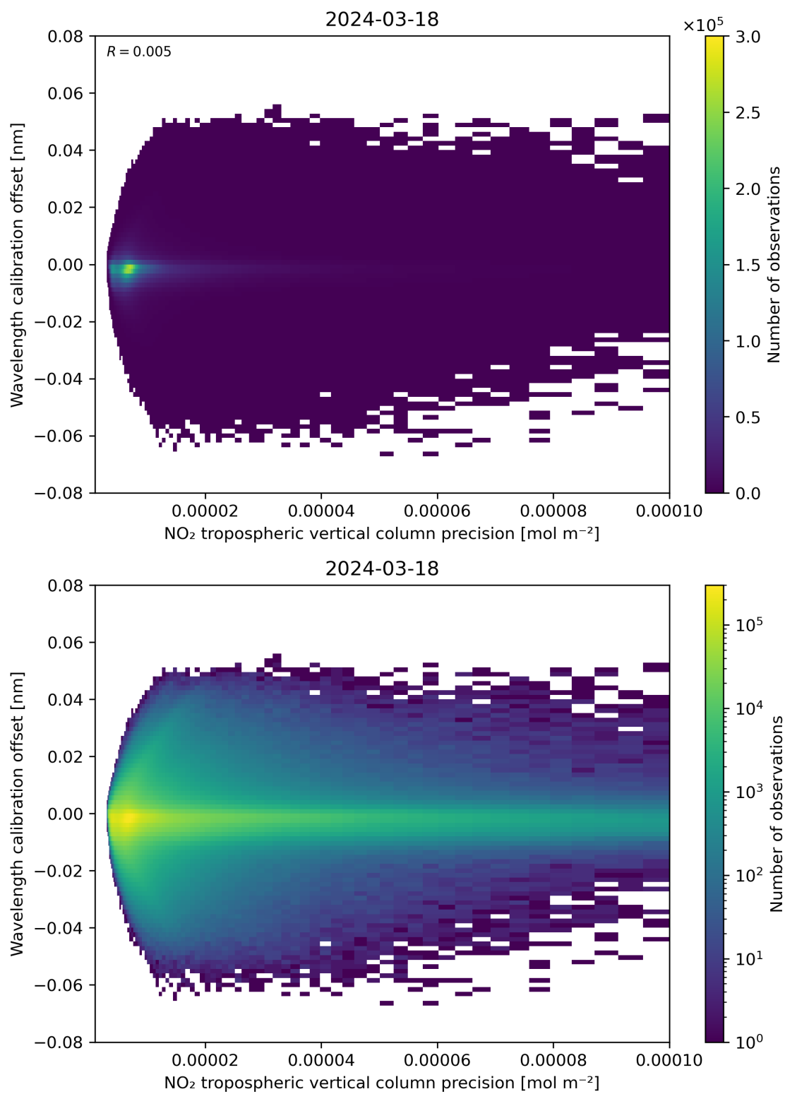
Figure 141: Scatter density plot of “NO 2 tropospheric vertical column precision” against “Wavelength calibration offset” for 2024-03-17 to 2024-03-19.
