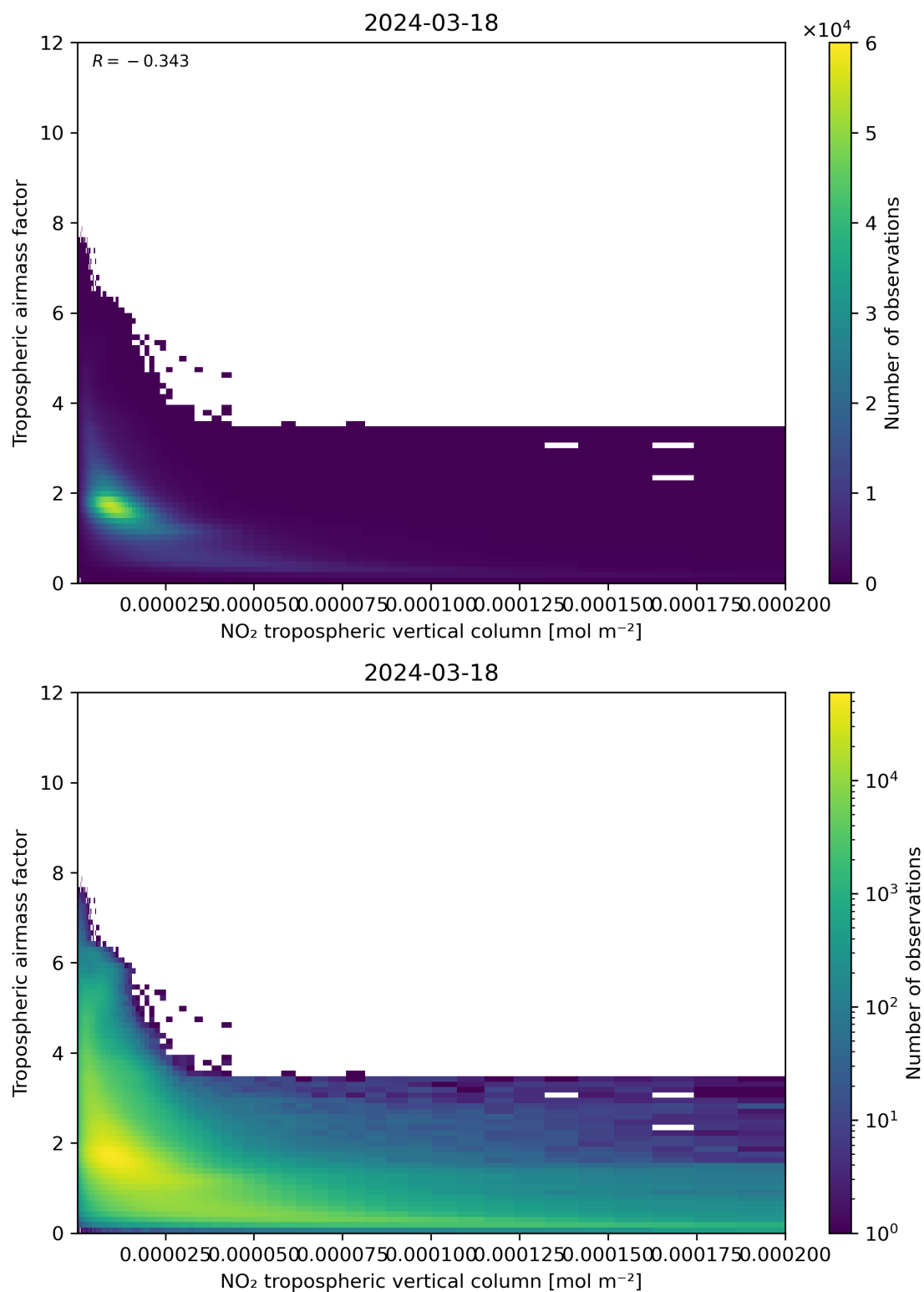
Figure 123: Scatter density plot of “NO 2 tropospheric vertical column” against “Tropospheric airmass factor” for 2024-03-17 to 2024-03-19.
