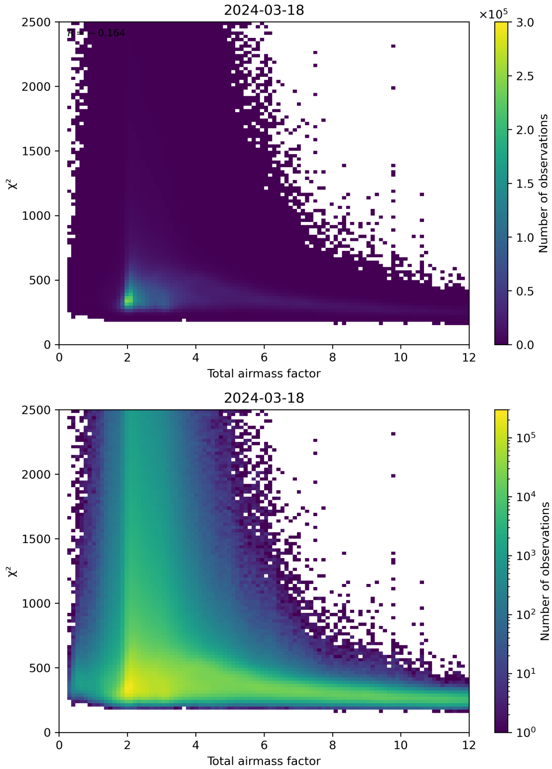
Figure 63: Scatter density plot of “Total airmass factor” against “ \chi^2 ” for 2024-03-17 to 2024-03-19.
