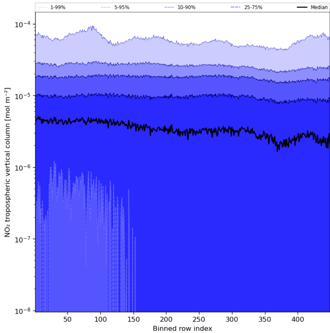
Figure 46: Along track statistics of “NO 2 tropospheric vertical column” for 2024-03-17 to 2024-03-19
