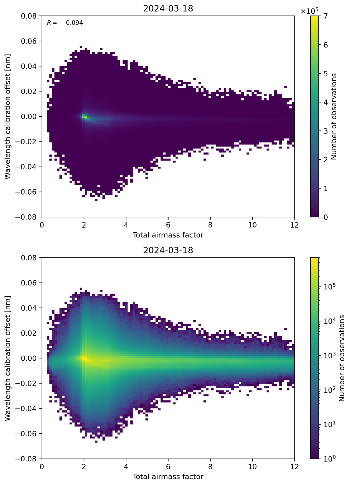
Figure 70: Scatter density plot of “Total airmass factor” against “Wavelength calibration offset” for 2024-03-17 to 2024-03-19.
