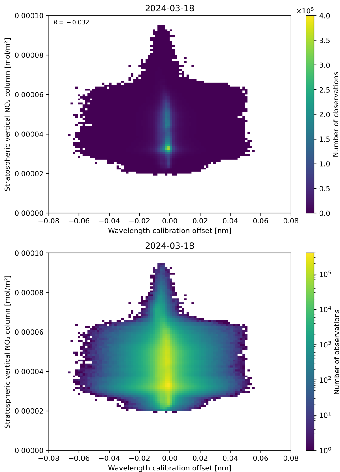
Figure 176: Scatter density plot of “Wavelength calibration offset” against “Stratospheric vertical NO 2 column” for 2024-03-17 to 2024-03-19.
