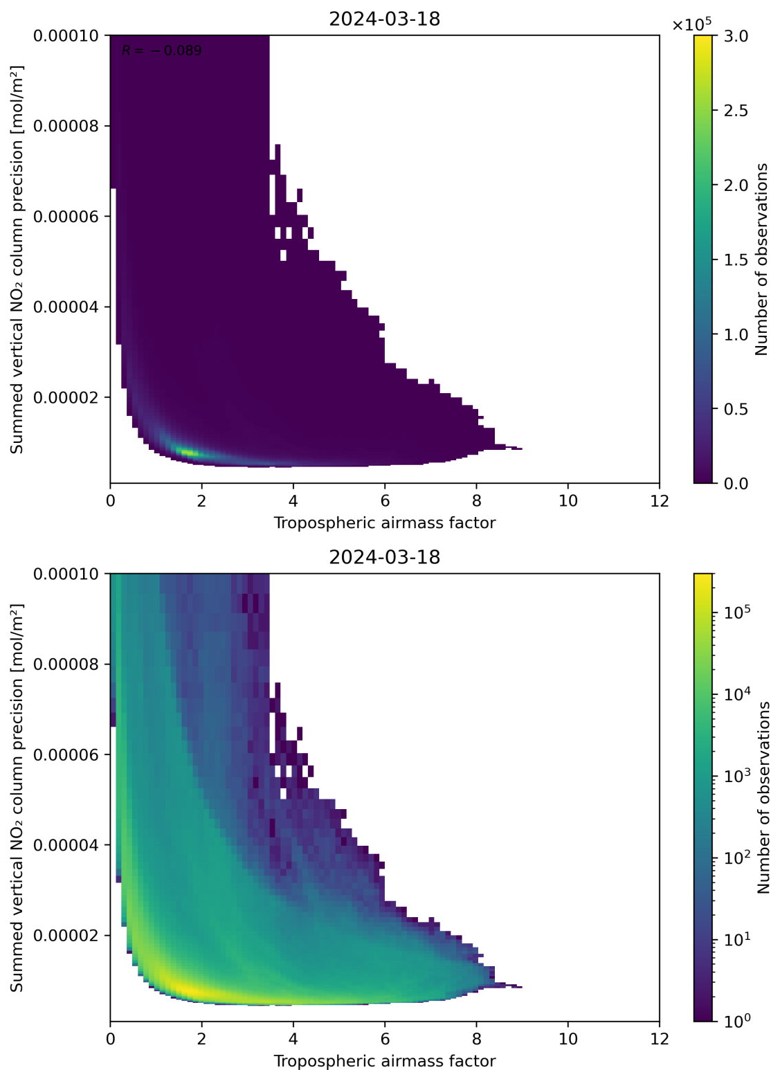
Figure 76: Scatter density plot of “Tropospheric air mass factor” against “Summed vertical NO 2 column precision” for 2024-03-17 to 2024-03-19.
