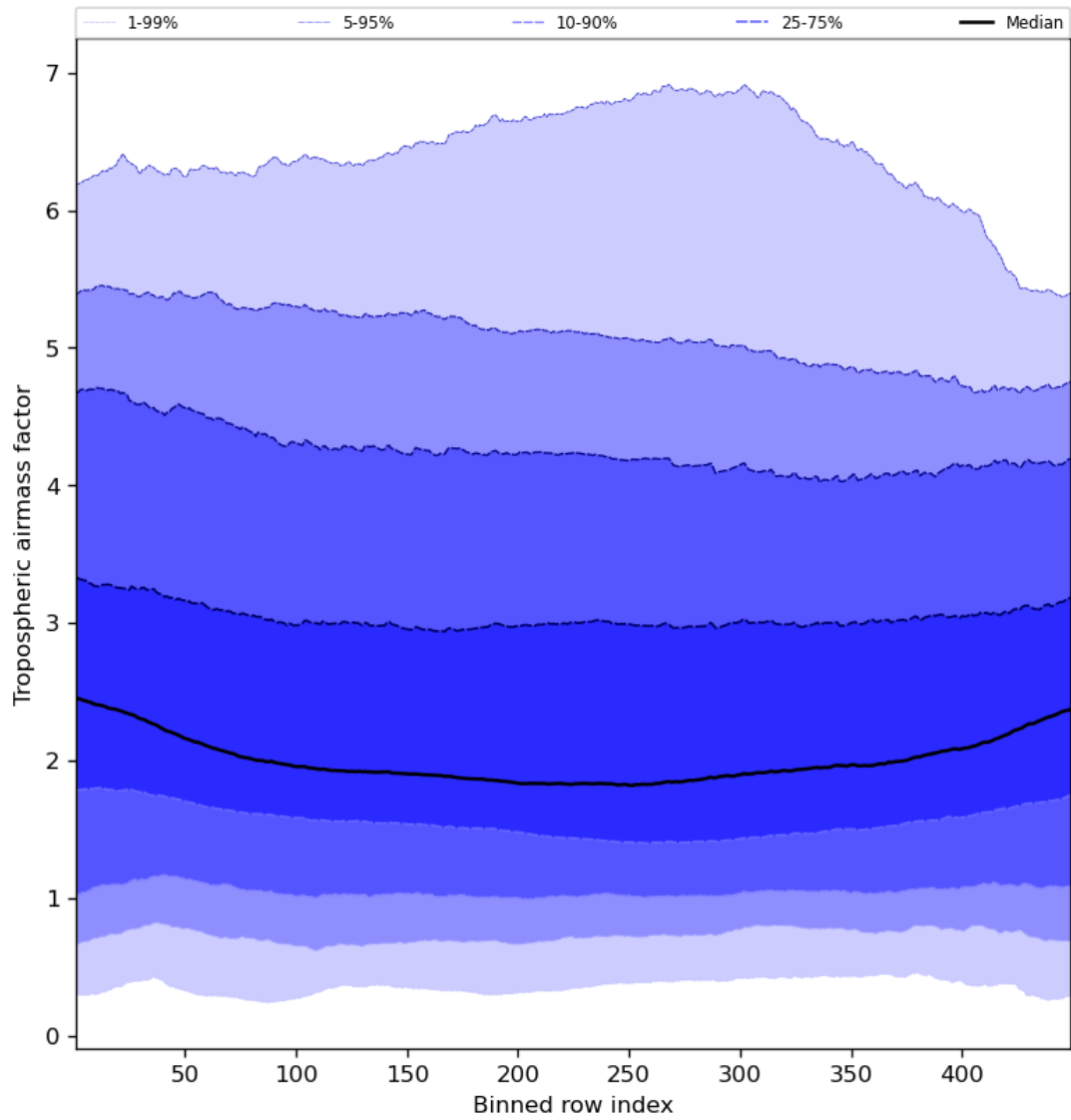
Figure 48: Along track statistics of “Tropospheric airmass factor” for 2024-03-17 to 2024-03-19
