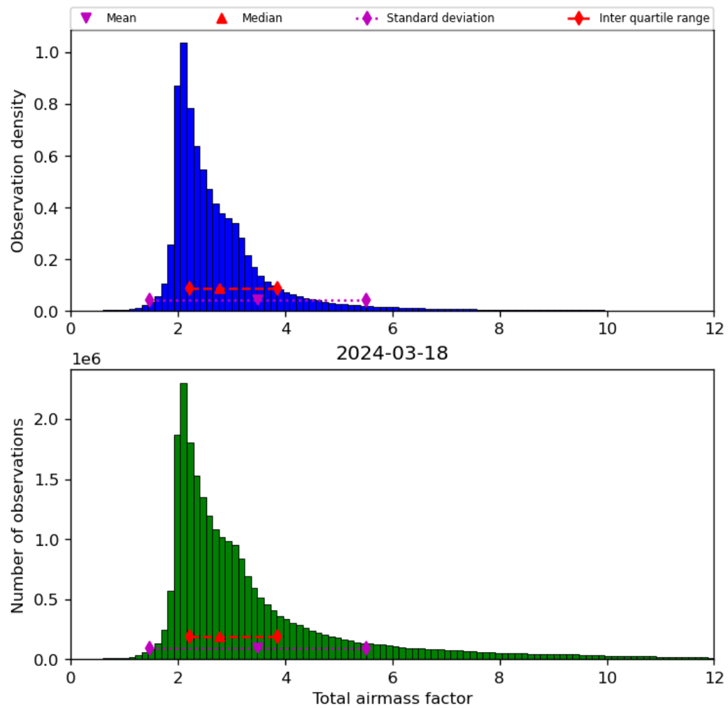
Figure 32: Histogram of “Total airmass factor” for 2024-03-17 to 2024-03-19
