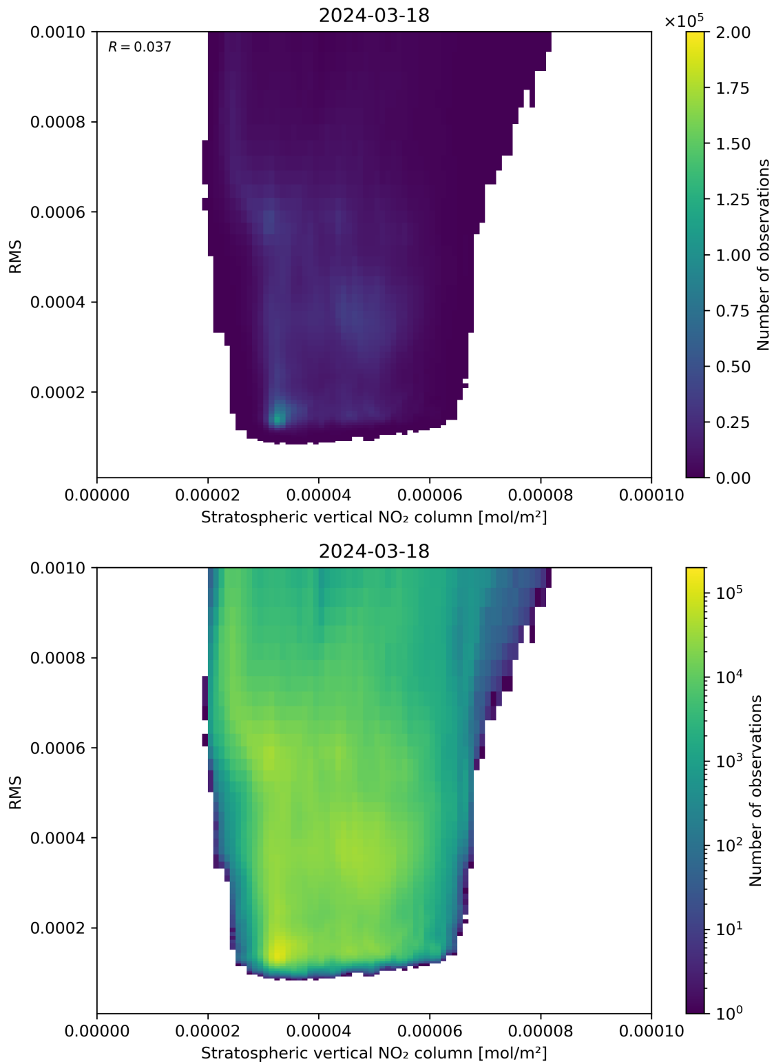
Figure 102: Scatter density plot of “Stratospheric vertical NO 2 column” against “RMS” for 2024-03-17 to 2024-03-19.
