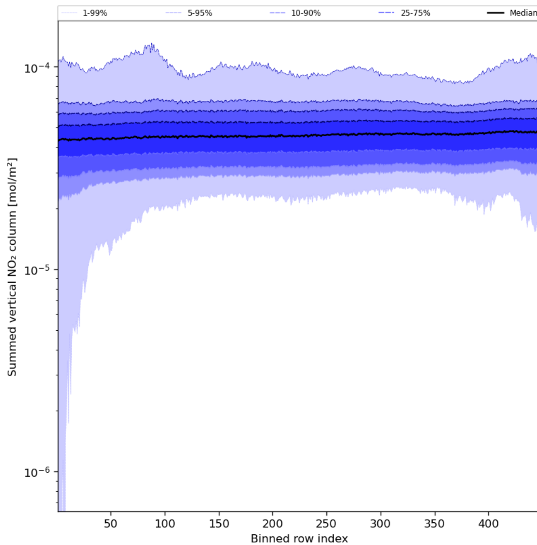
Figure 57: Along track statistics of “Summed vertical NO 2 column” for 2024-03-17 to 2024-03-19
