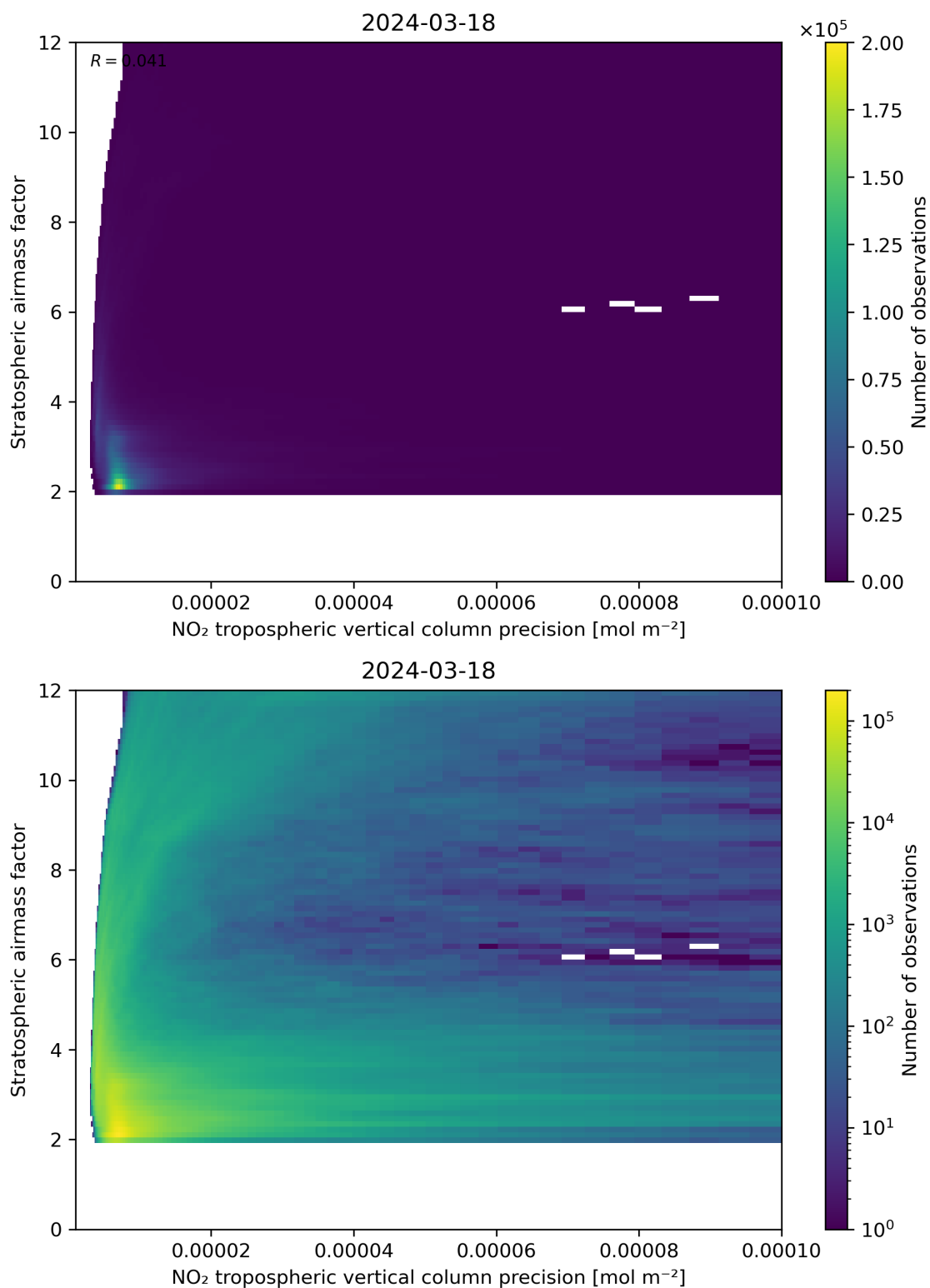
Figure 131: Scatter density plot of “NO 2 tropospheric vertical column precision” against “Stratospheric airmass factor” for 2024-03-17 to 2024-03-19.
