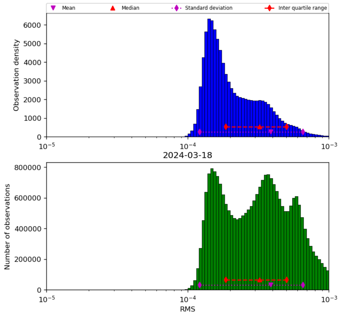
Figure 43: Histogram of “RMS” for 2024-03-17 to 2024-03-19
