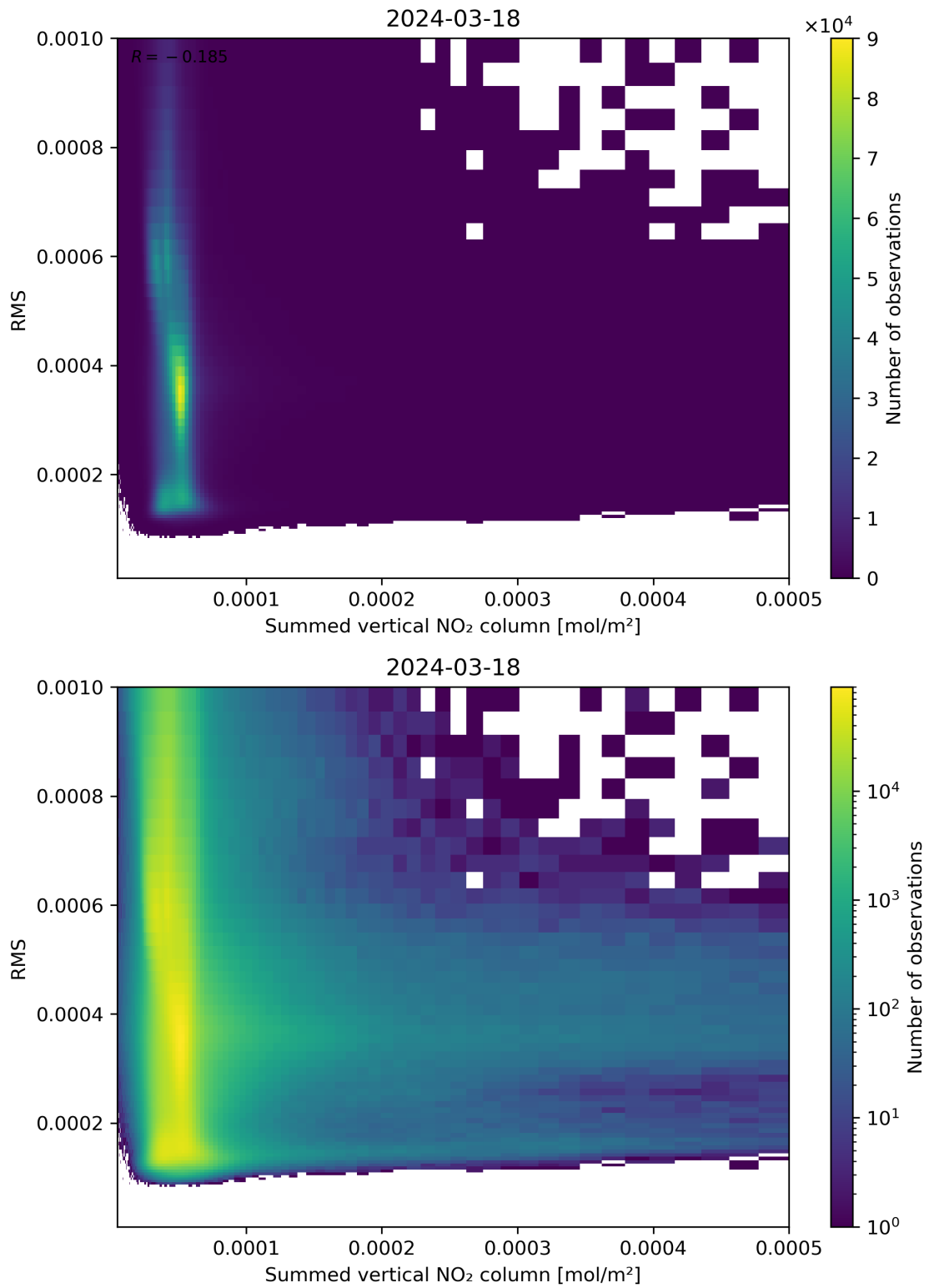
Figure 109: Scatter density plot of “Summed vertical NO 2 column” against “RMS” for 2024-03-17 to 2024-03-19.
