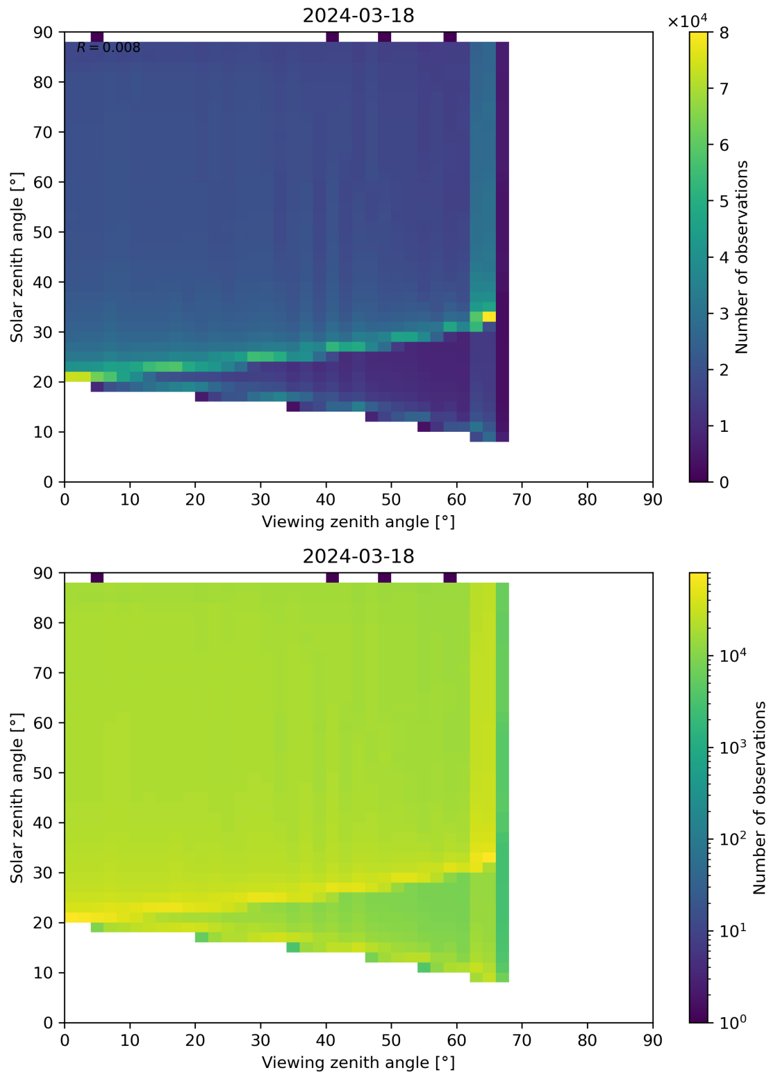
Figure 172: Scatter density plot of “Viewing zenith angle” against “Solar zenith angle” for 2024-03-17 to 2024-03-19.
