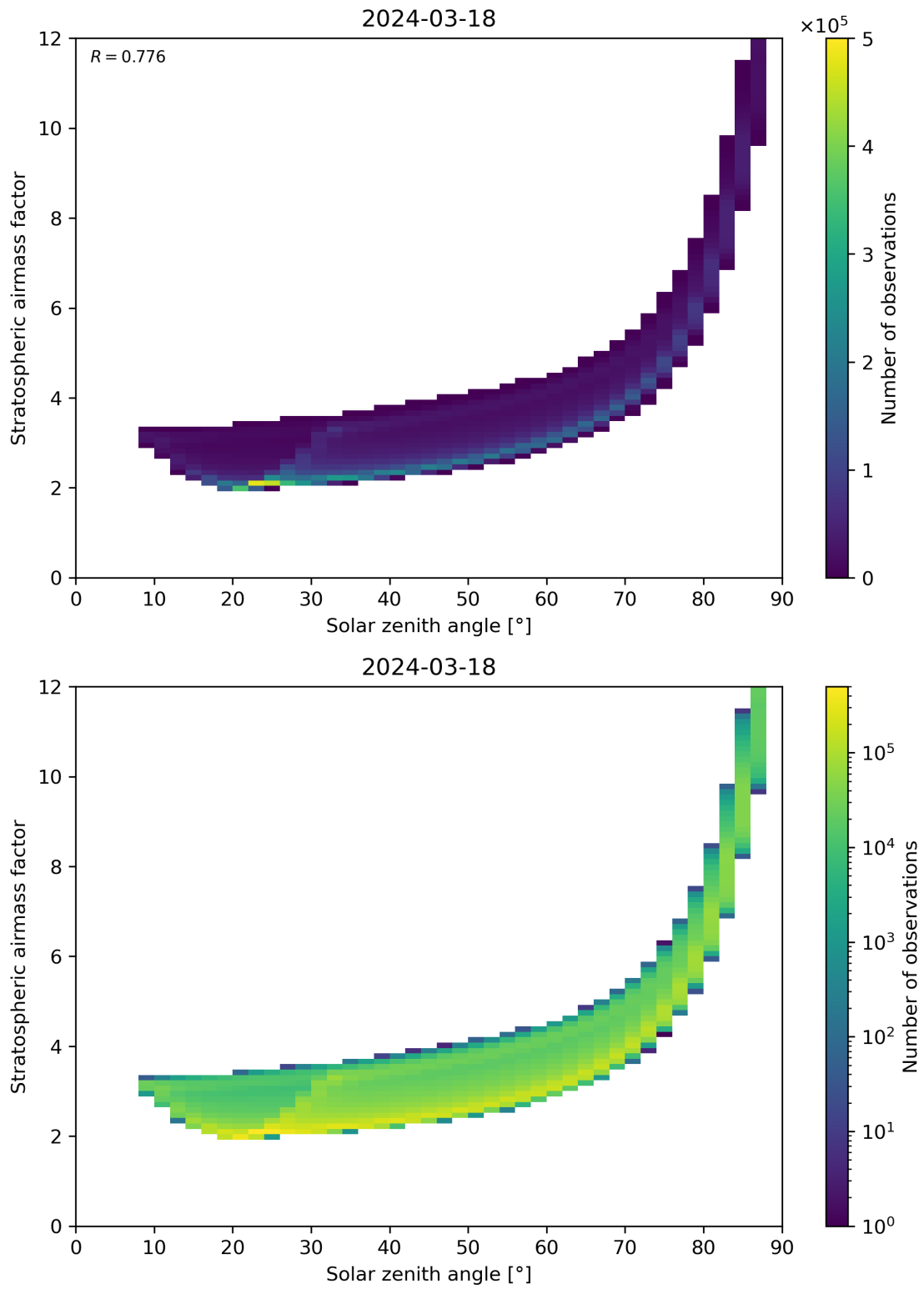
Figure 145: Scatter density plot of “Solar zenith angle” against “Stratospheric airmass factor” for 2024-03-17 to 2024-03-19.
