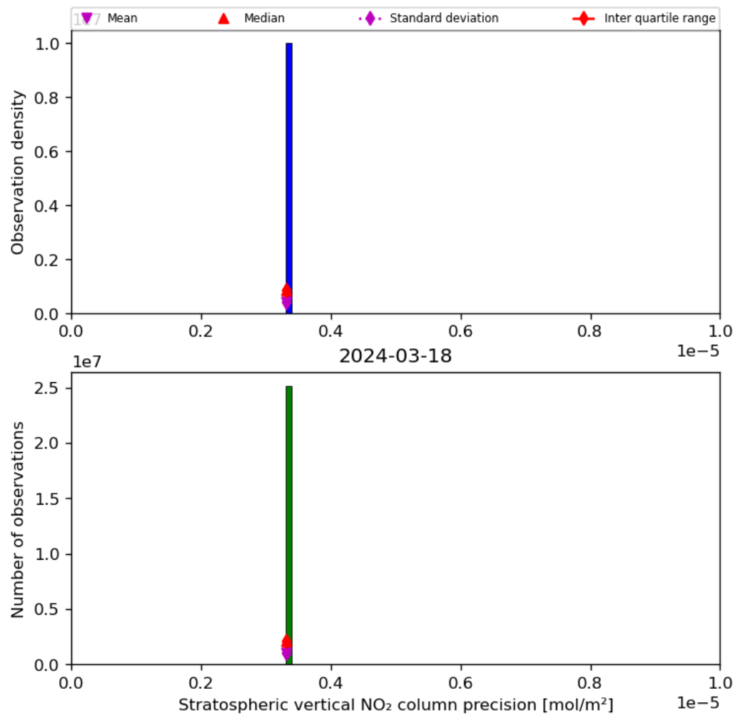
Figure 37: Histogram of “Stratospheric vertical NO 2 column precision” for 2024-03-17 to 2024-03-19
