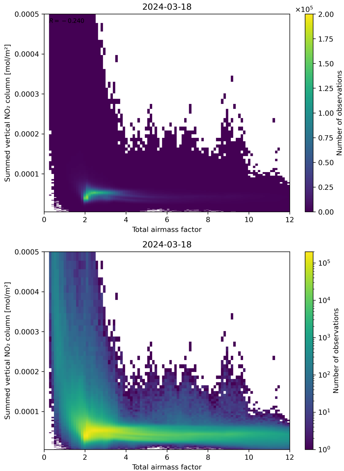
Figure 65: Scatter density plot of “Total airmass factor” against “Summed vertical NO 2 column” for 2024-03-17 to 2024-03-19.
