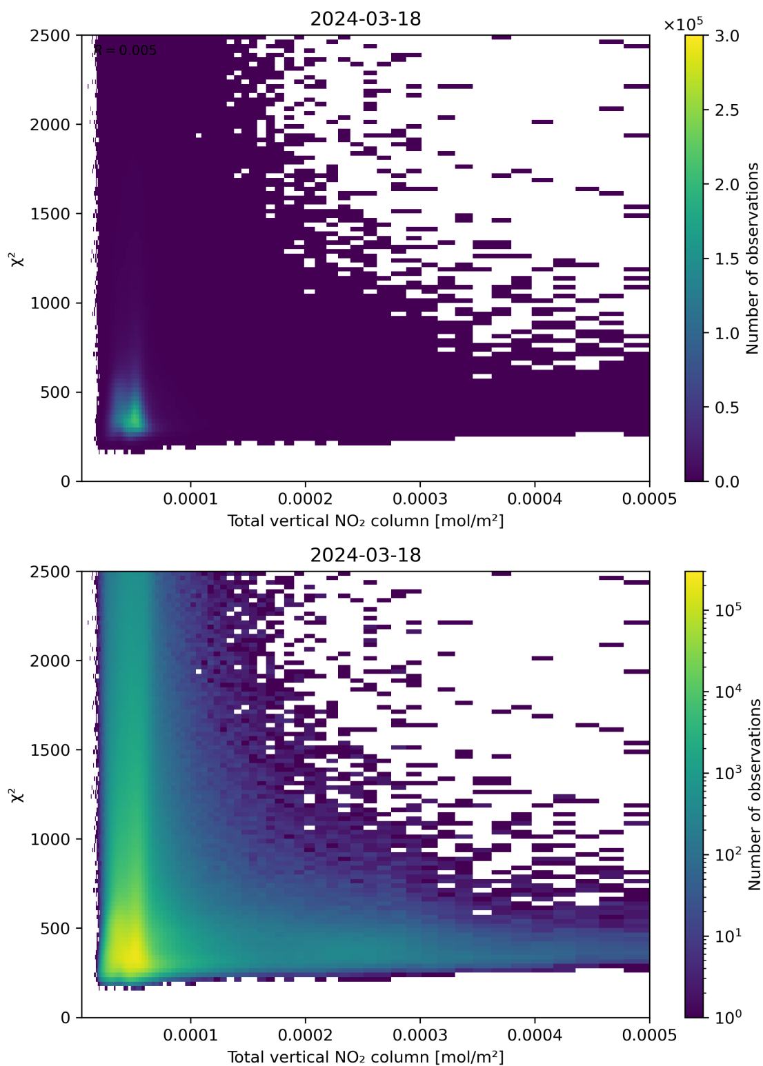
Figure 111: Scatter density plot of “Total vertical NO 2 column” against “ \chi^2 ” for 2024-03-17 to 2024-03-19.
