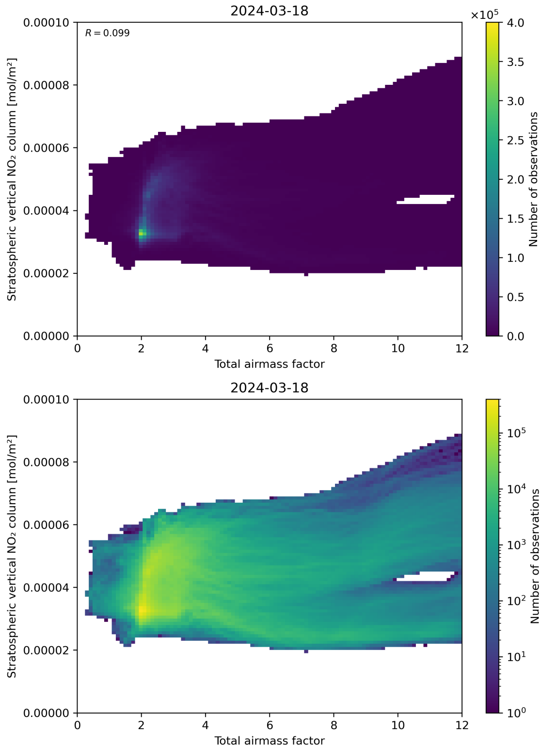
Figure 64: Scatter density plot of “Total airmass factor” against “Stratospheric vertical NO 2 column” for 2024-03-17 to 2024-03-19.
