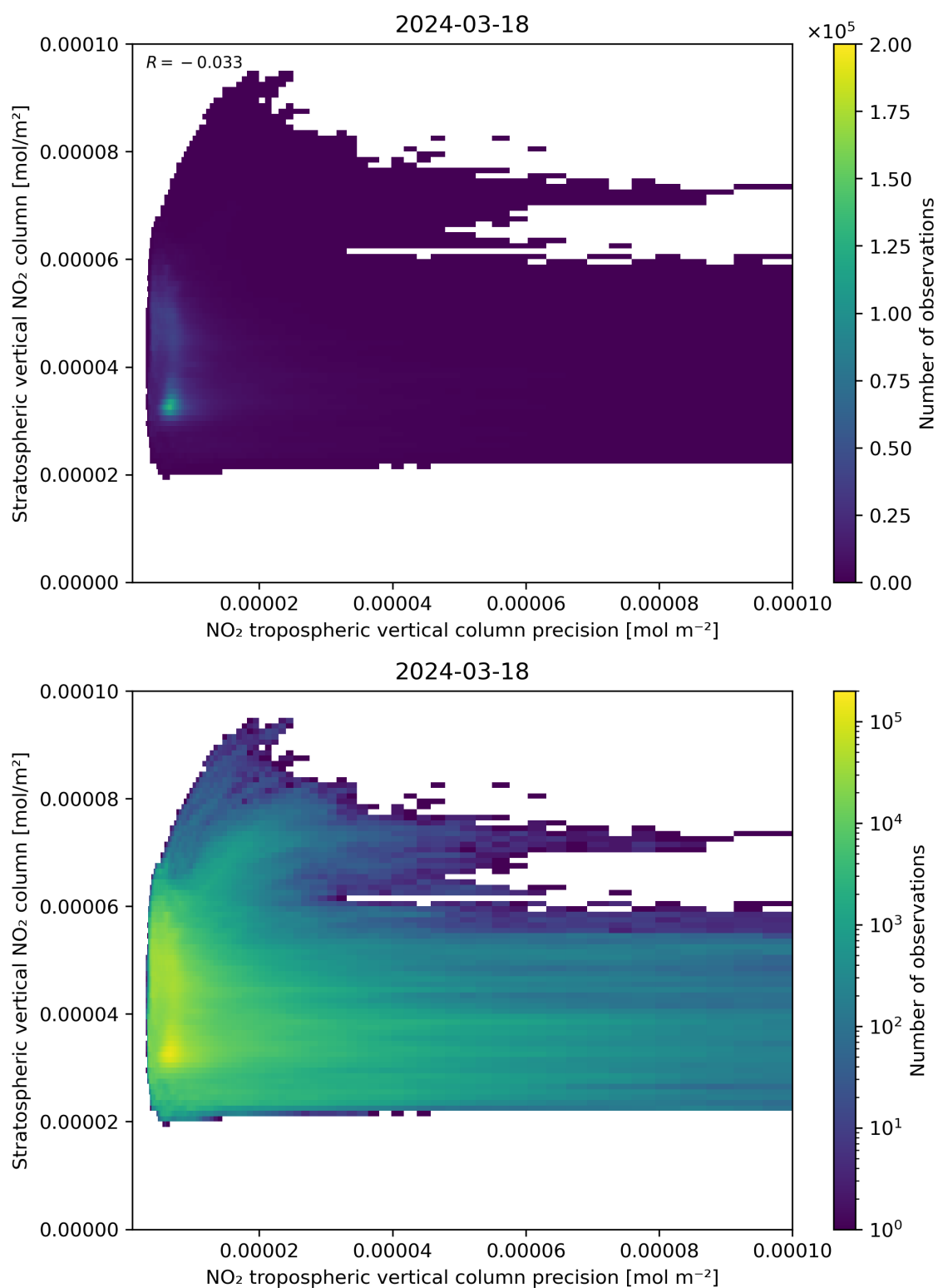
Figure 135: Scatter density plot of “NO 2 tropospheric vertical column precision” against “Stratospheric vertical NO 2 column” for 2024-03-17 to 2024-03-19.
