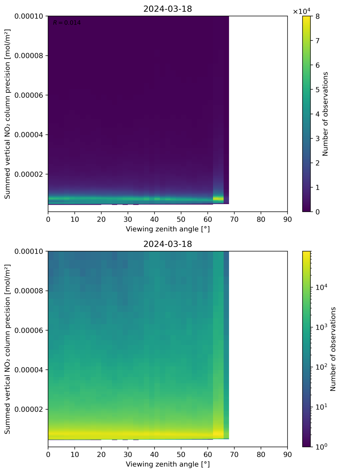
Figure 166: Scatter density plot of “Viewing zenith angle” against “Summed vertical NO 2 column precision” for 2024-03-17 to 2024-03-19.
