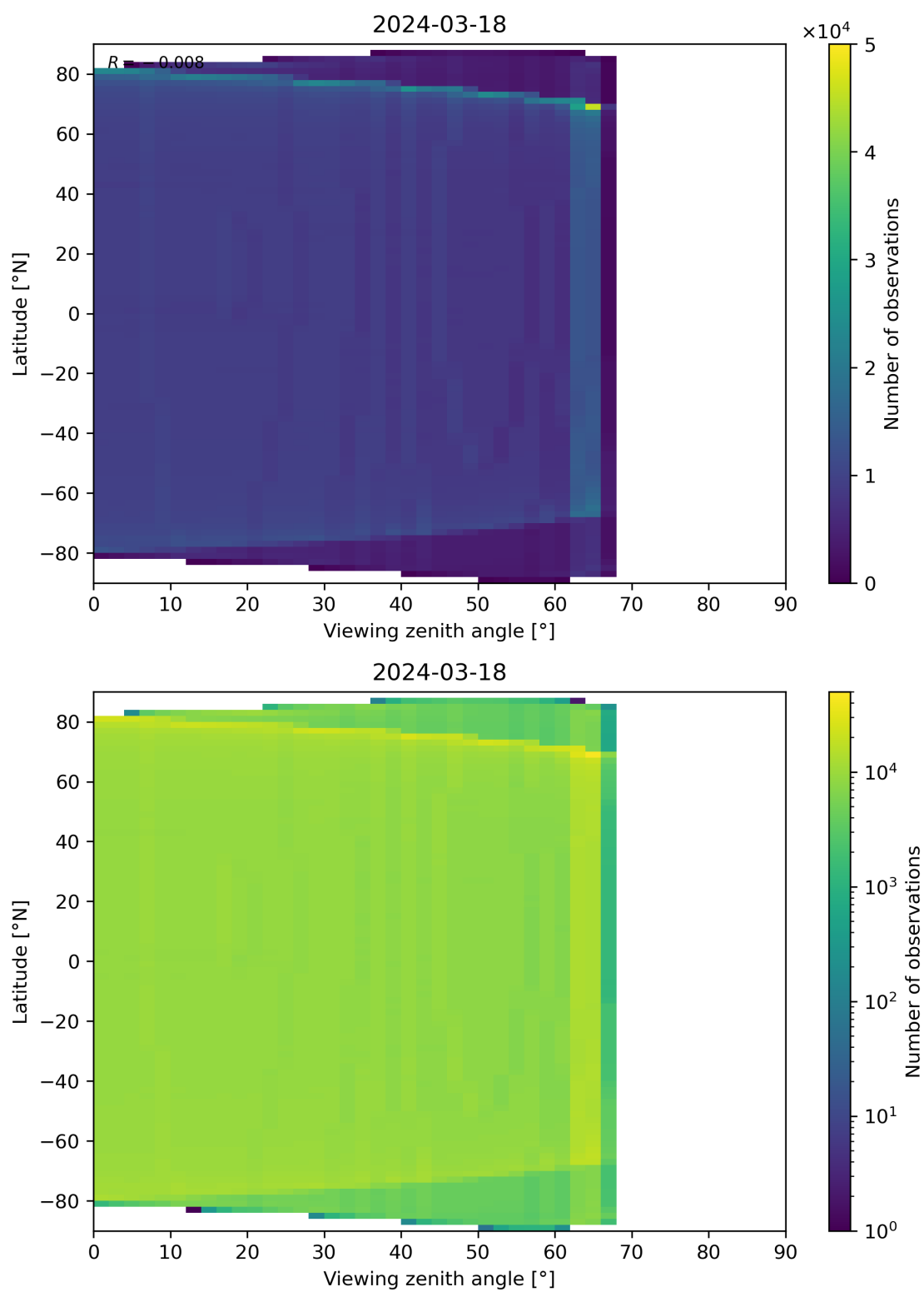
Figure 163: Scatter density plot of “Viewing zenith angle” against “Latitude” for 2024-03-17 to 2024-03-19.
