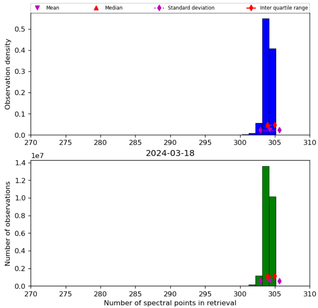
Figure 33: Histogram of “Number of spectral points in retrieval” for 2024-03-17 to 2024-03-19
