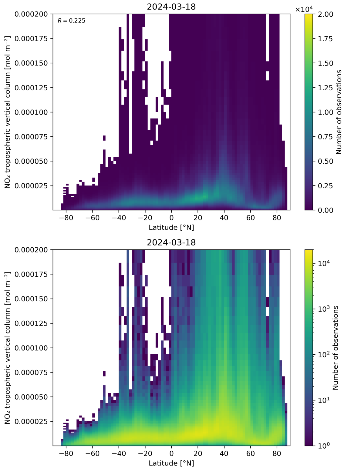
Figure 92: Scatter density plot of “Latitude” against “NO 2 tropospheric vertical column” for 2024-03-17 to 2024-03-19.
