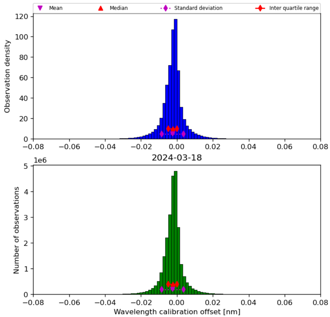
Figure 35: Histogram of “Wavelength calibration offset” for 2024-03-17 to 2024-03-19
