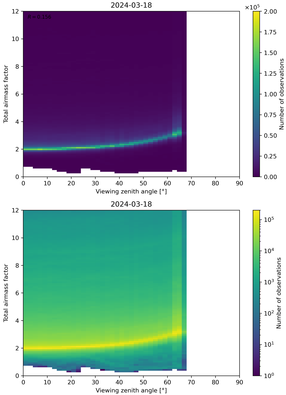
Figure 160: Scatter density plot of “Viewing zenith angle” against “Total airmass factor” for 2024-03-17 to 2024-03-19.
