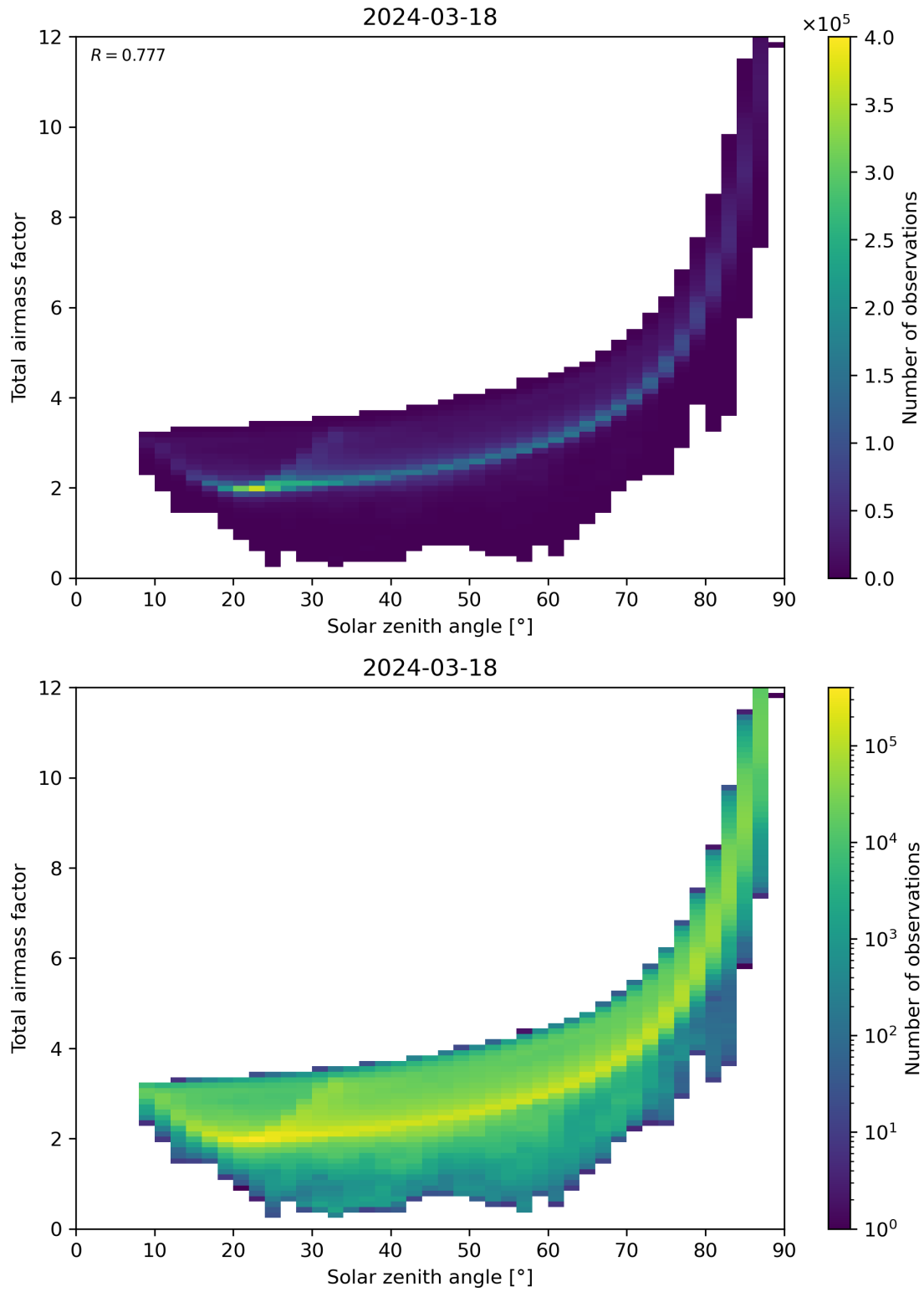
Figure 146: Scatter density plot of “Solar zenith angle” against “Total air mass factor” for 2024-03-17 to 2024-03-19.
