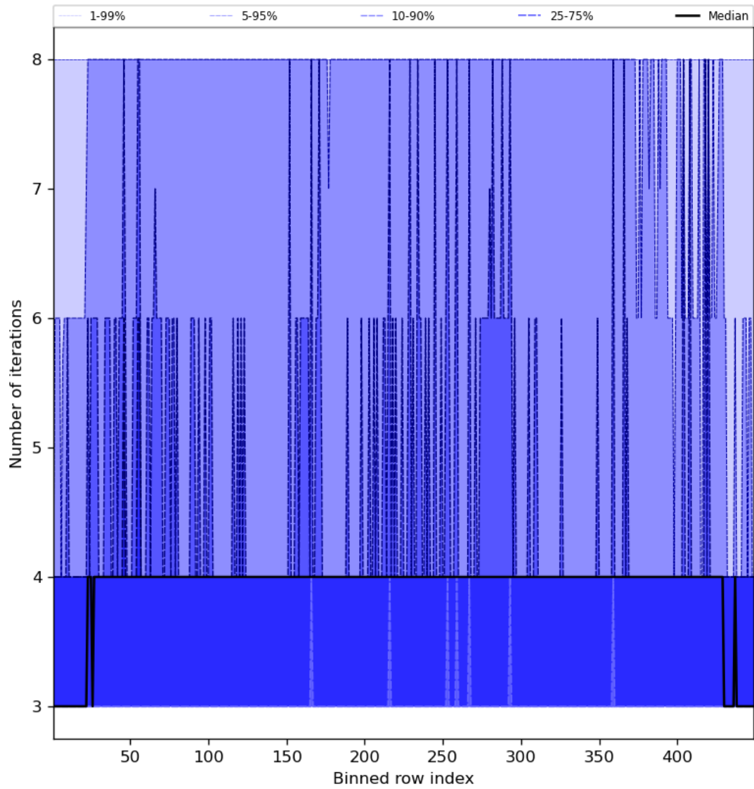
Figure 51: Along track statistics of “Number of iterations” for 2024-03-17 to 2024-03-19
