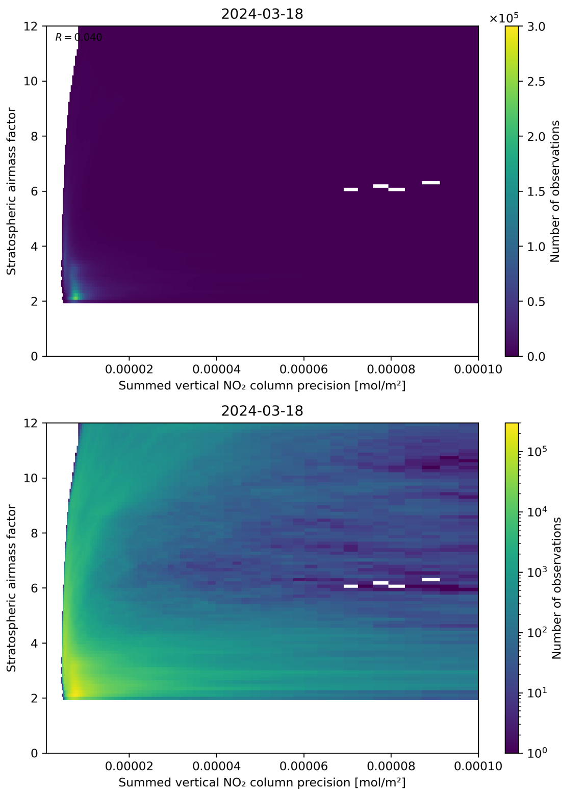
Figure 106: Scatter density plot of “Summed vertical NO 2 column precision” against “Stratospheric airmass factor” for 2024-03-17 to 2024-03-19.
