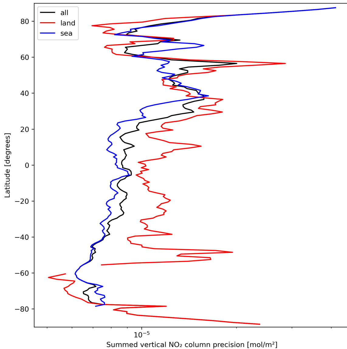
Figure 24: Zonal average of “Summed vertical NO 2 column precision” for 2024-03-17 to 2024-03-19.
