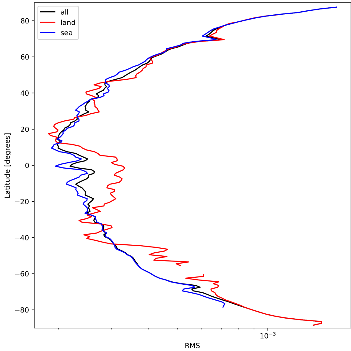
Figure 26: Zonal average of “RMS” for 2024-03-17 to 2024-03-19.
