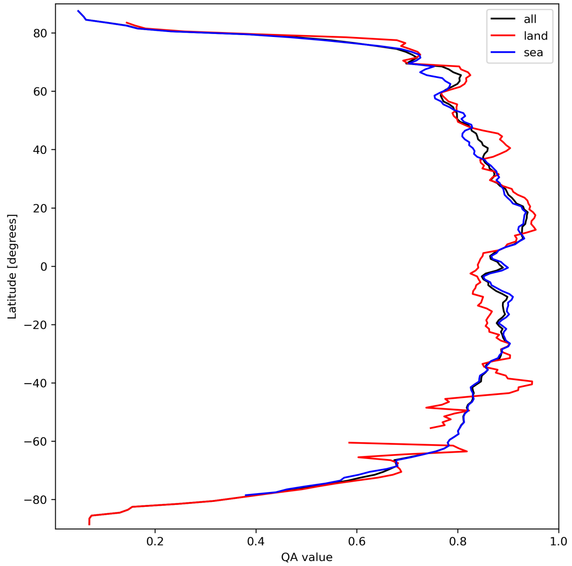
Figure 11: Zonal average of “QA value” for 2024-03-17 to 2024-03-19.
