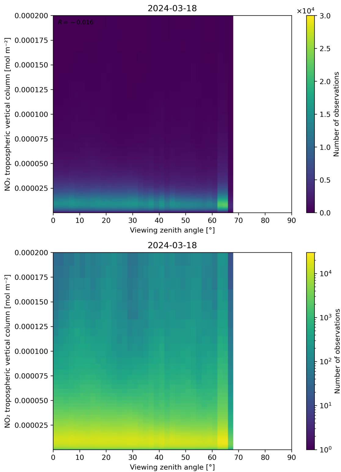
Figure 169: Scatter density plot of “Viewing zenith angle” against “NO 2 tropospheric vertical column” for 2024-03-17 to 2024-03-19.
