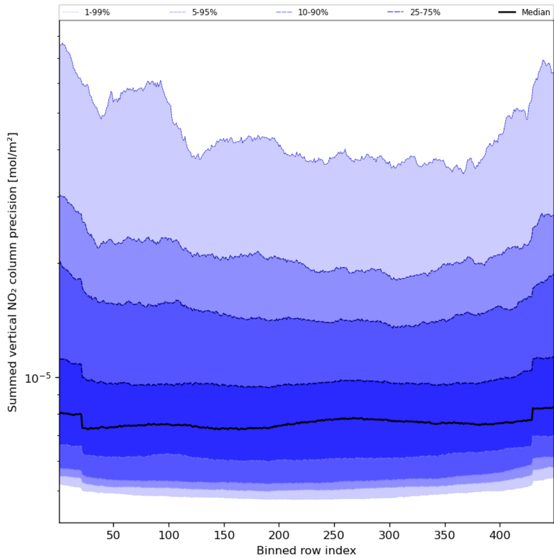
Figure 58: Along track statistics of “Summed vertical NO 2 column precision” for 2024-03-17 to 2024-03-19
