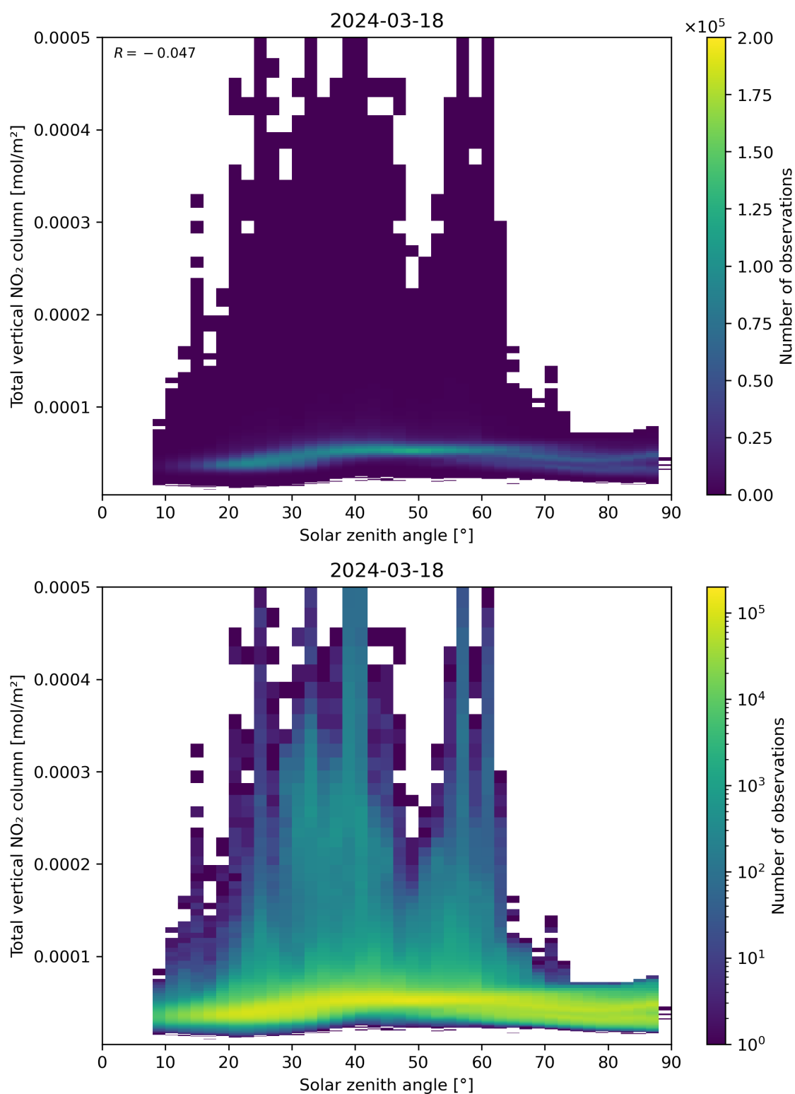
Figure 153: Scatter density plot of “Solar zenith angle” against “Total vertical NO 2 column” for 2024-03-17 to 2024-03-19.
