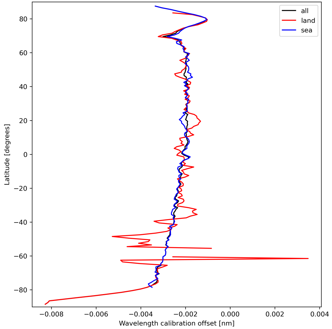
Figure 18: Zonal average of “Wavelength calibration offset” for 2024-03-17 to 2024-03-19.
