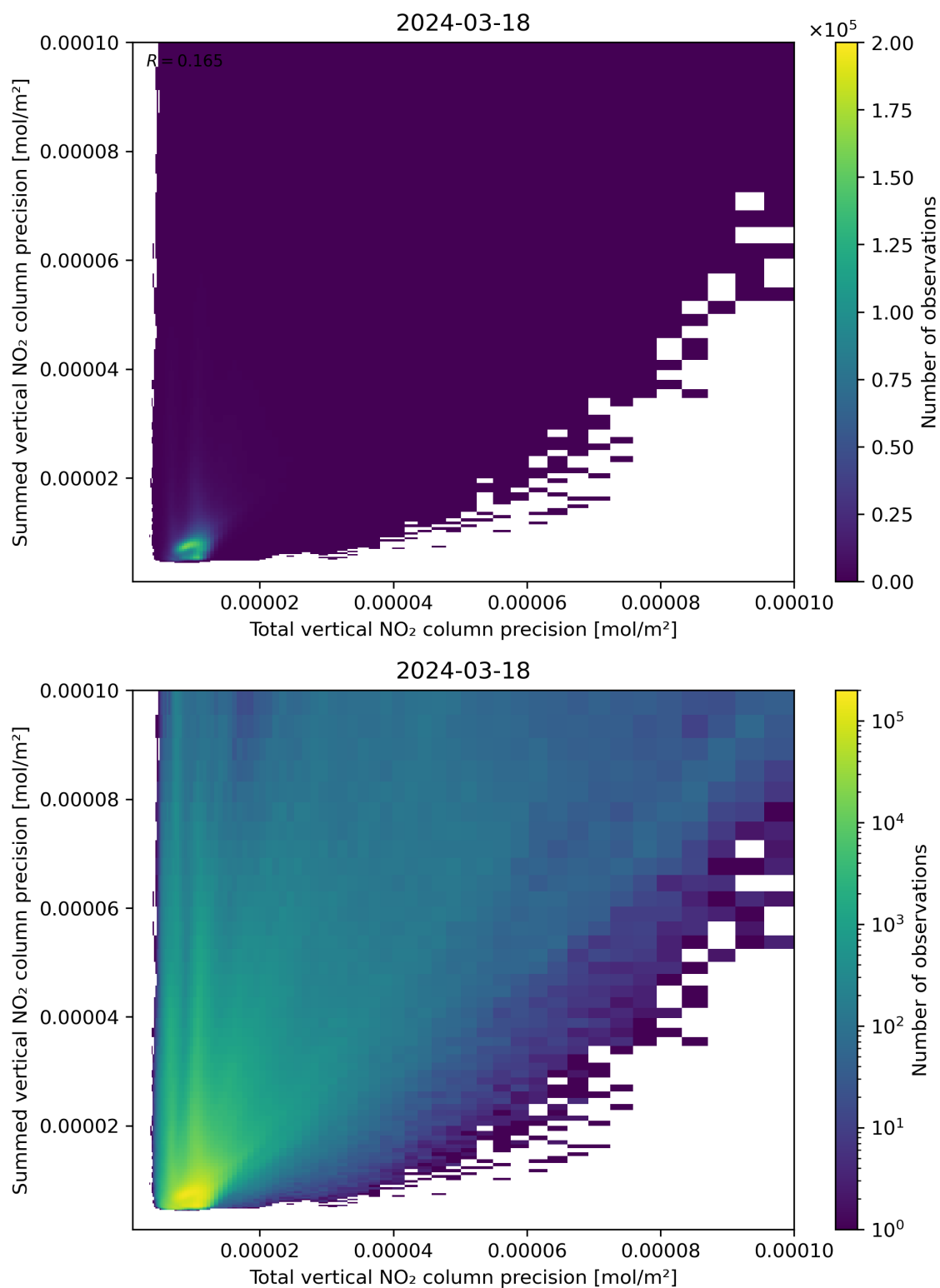
Figure 118: Scatter density plot of “Total vertical NO 2 column precision” against “Summed vertical NO 2 column precision” for 2024-03-17 to 2024-03-19.
