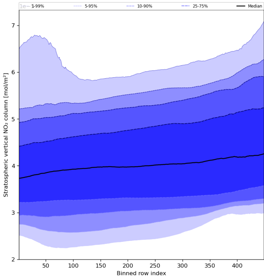
Figure 53: Along track statistics of “Stratospheric vertical NO 2 column” for 2024-03-17 to 2024-03-19
