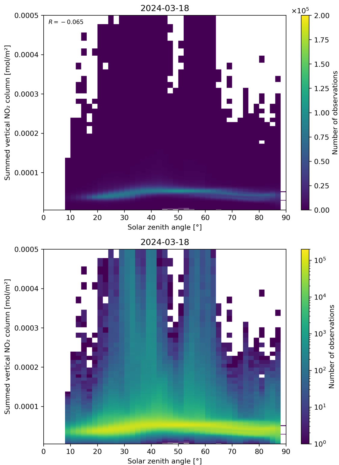
Figure 151: Scatter density plot of “Solar zenith angle” against “Summed vertical NO 2 column” for 2024-03-17 to 2024-03-19.
