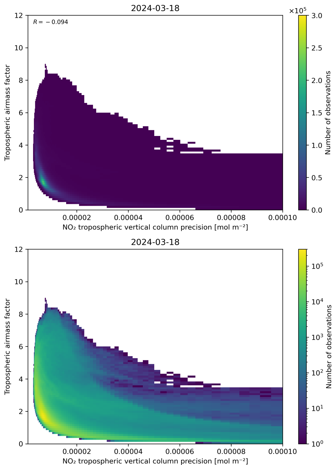
Figure 133: Scatter density plot of “NO 2 tropospheric vertical column precision” against “Tropospheric air mass factor” for 2024-03-17 to 2024-03-19.
