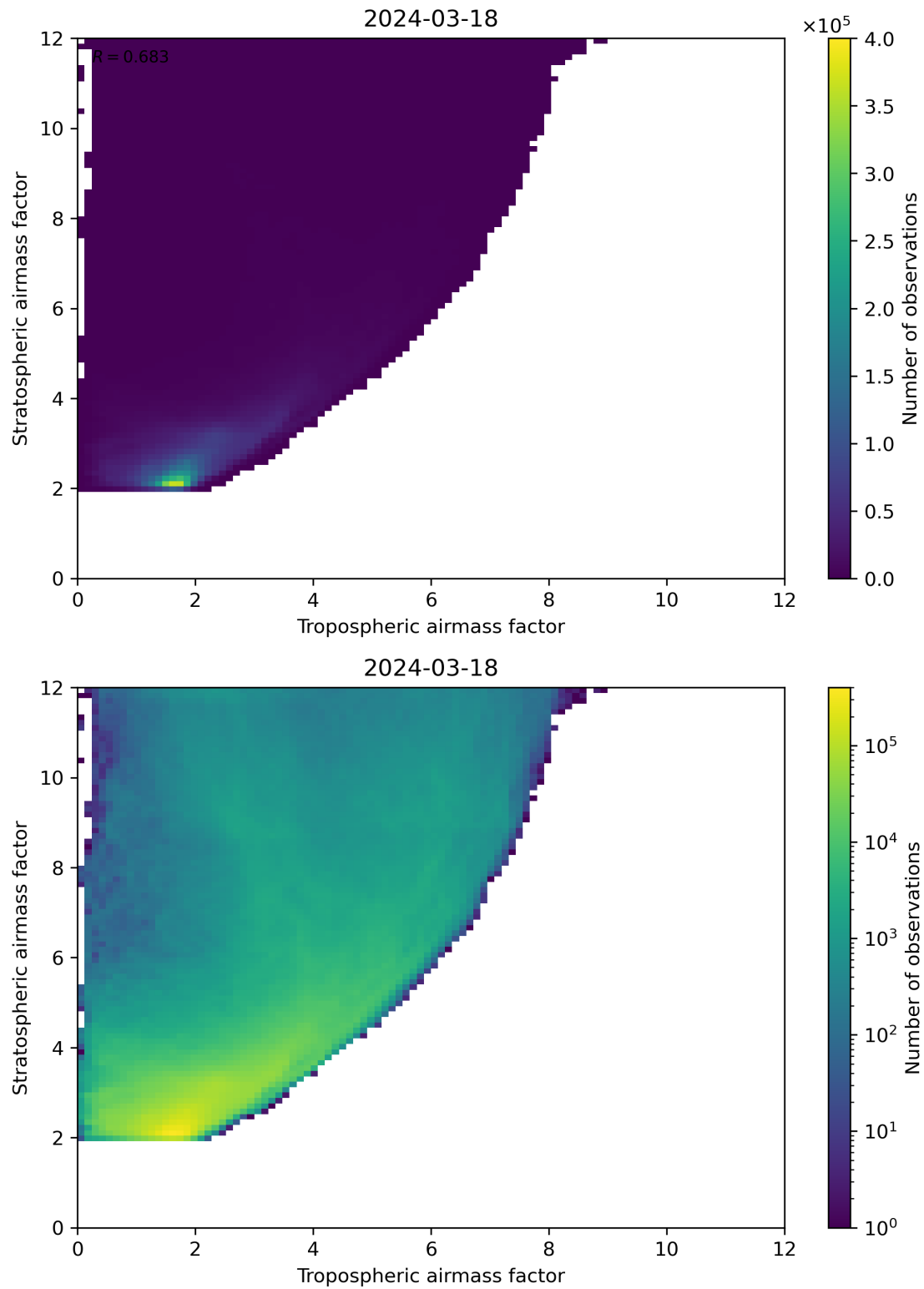
Figure 71: Scatter density plot of “Tropospheric airmass factor” against “Stratospheric airmass factor” for 2024-03-17 to 2024-03-19.
