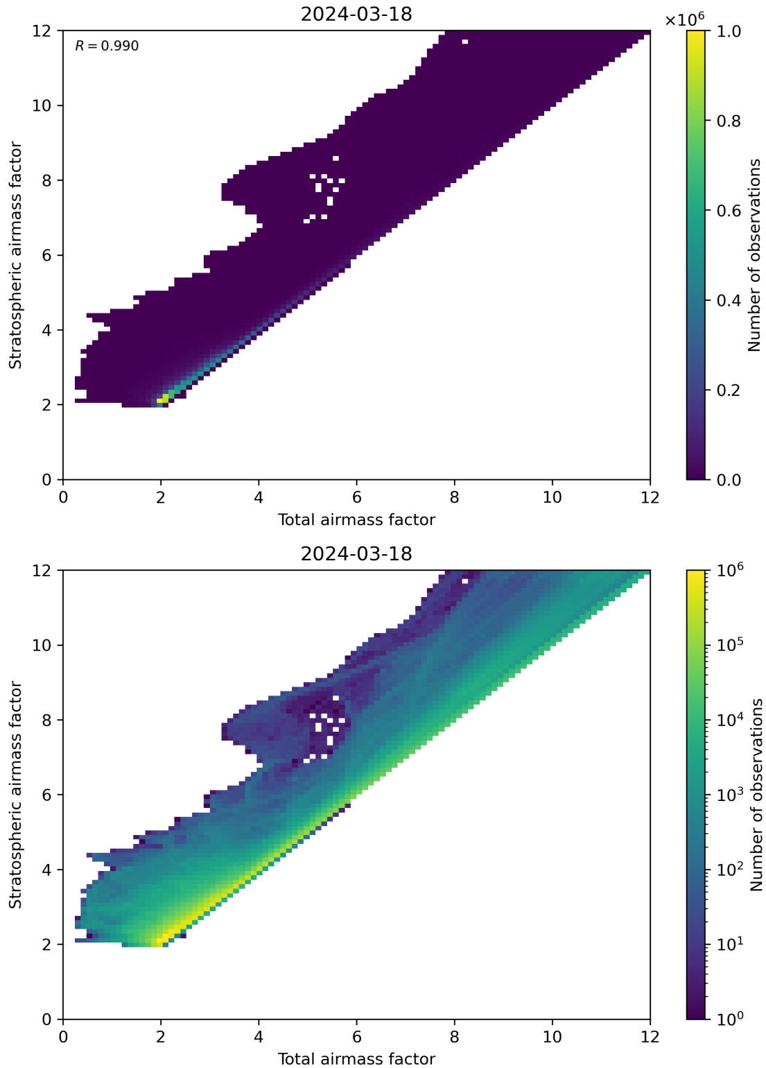
Figure 62: Scatter density plot of “Total airmass factor” against “Stratospheric airmass factor” for 2024-03-17 to 2024-03-19.
