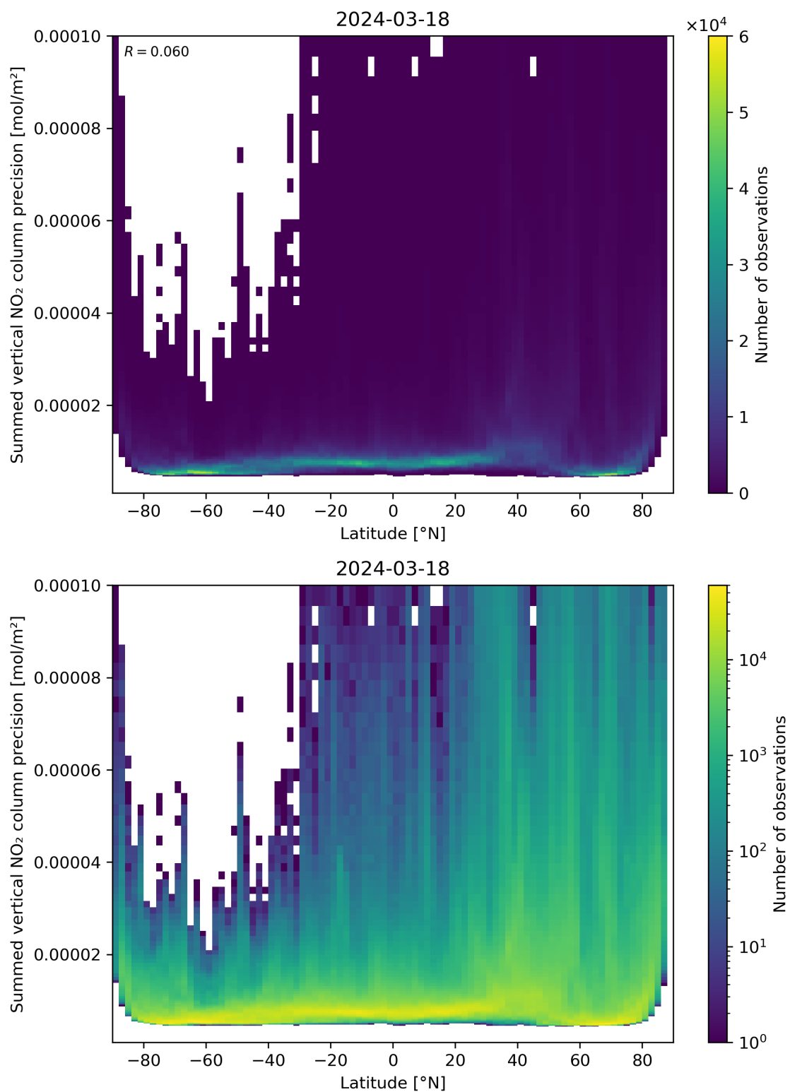
Figure 89: Scatter density plot of “Latitude” against “Summed vertical NO 2 column precision” for 2024-03-17 to 2024-03-19.
