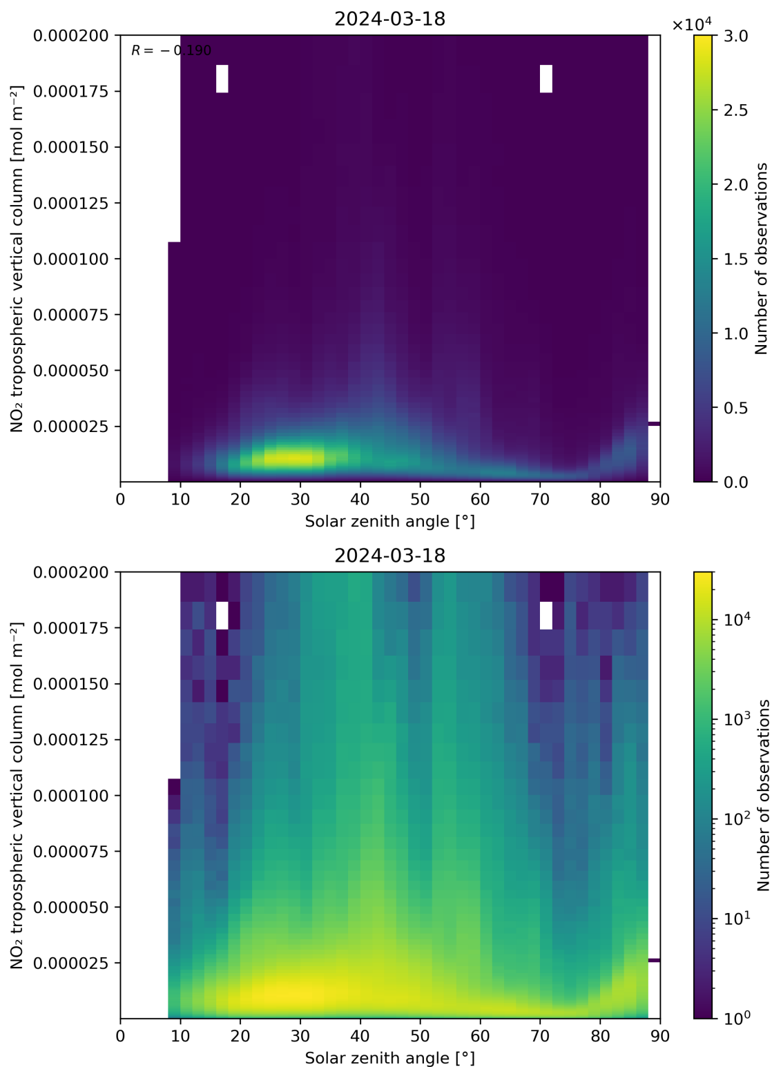
Figure 155: Scatter density plot of “Solar zenith angle” against “NO 2 tropospheric vertical column” for 2024-03-17 to 2024-03-19.
