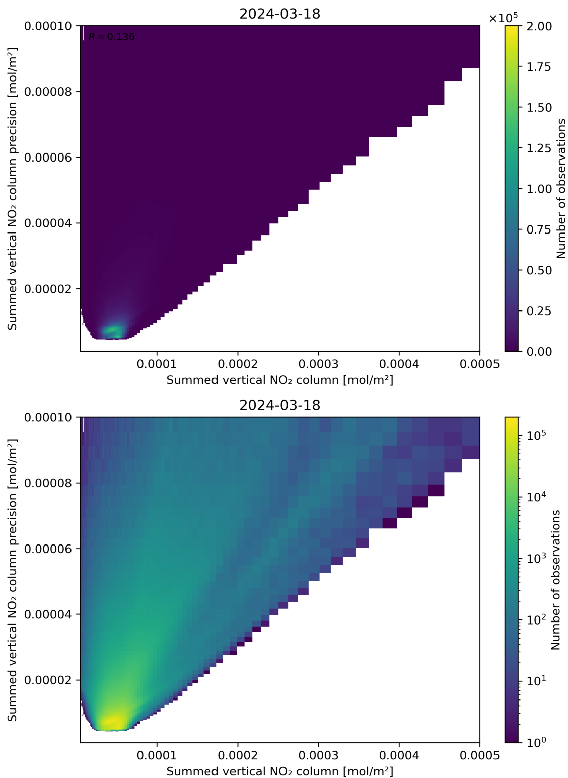
Figure 105: Scatter density plot of “Summed vertical NO 2 column” against “Summed vertical NO 2 column precision” for 2024-03-17 to 2024-03-19.
