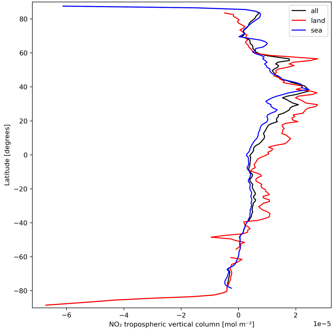
Figure 12: Zonal average of “NO 2 tropospheric vertical column” for 2024-03-17 to 2024-03-19.
