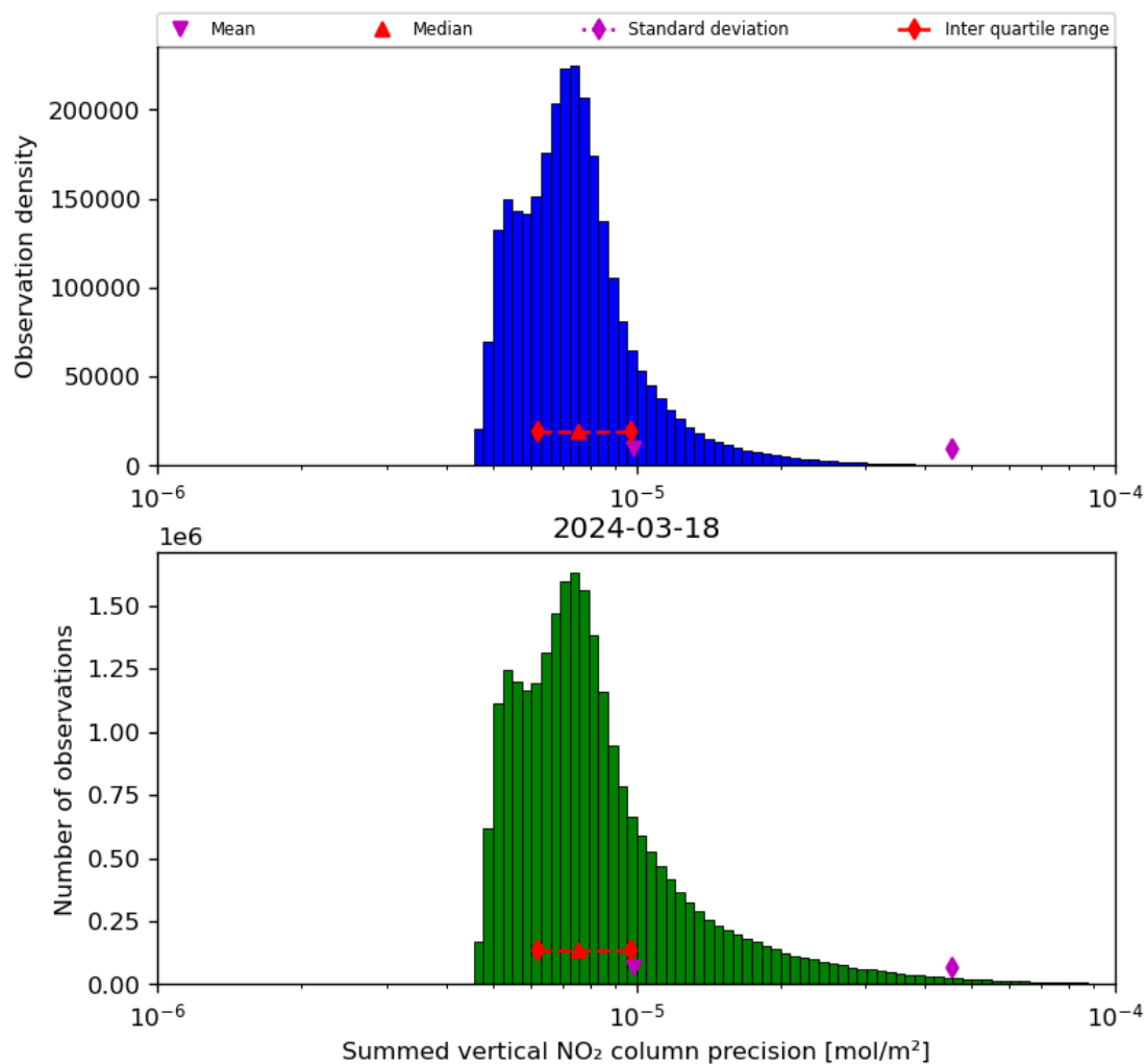
Figure 41: Histogram of "Summed vertical NO 2 column precision" for 2024-03-17 to 2024-03-19
