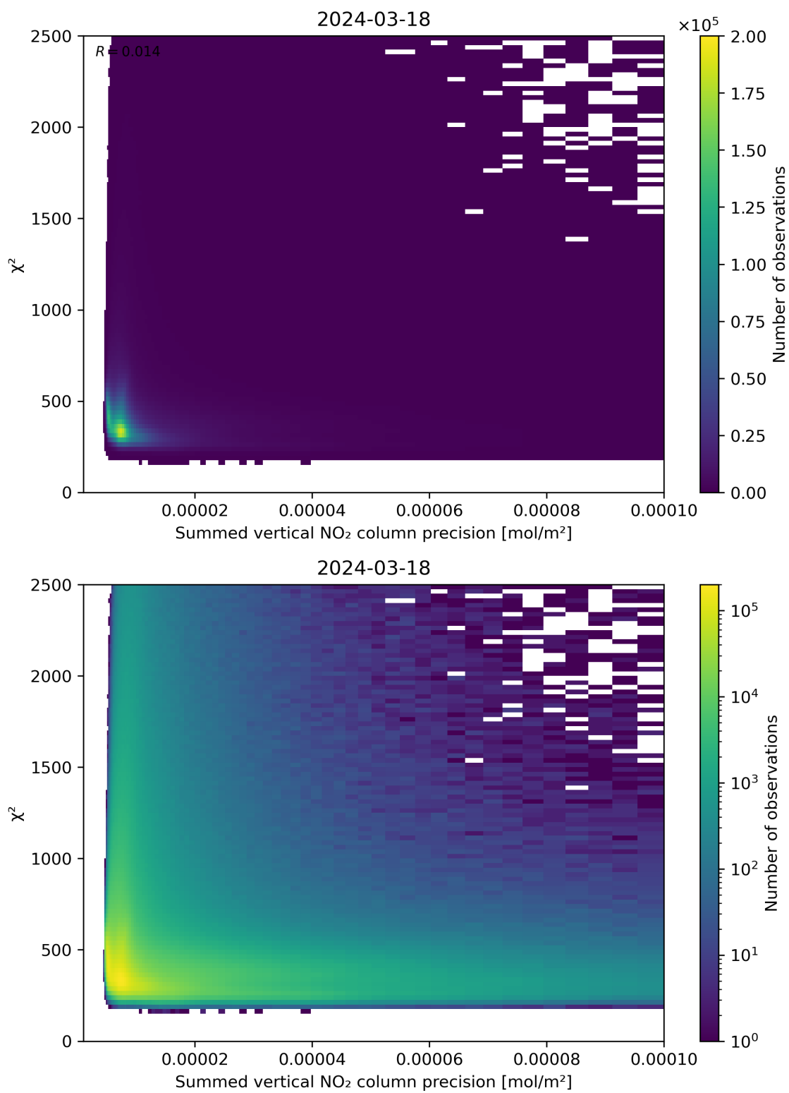
Figure 107: Scatter density plot of “Summed vertical NO 2 column precision” against “ \chi^2 ” for 2024-03-17 to 2024-03-19.
