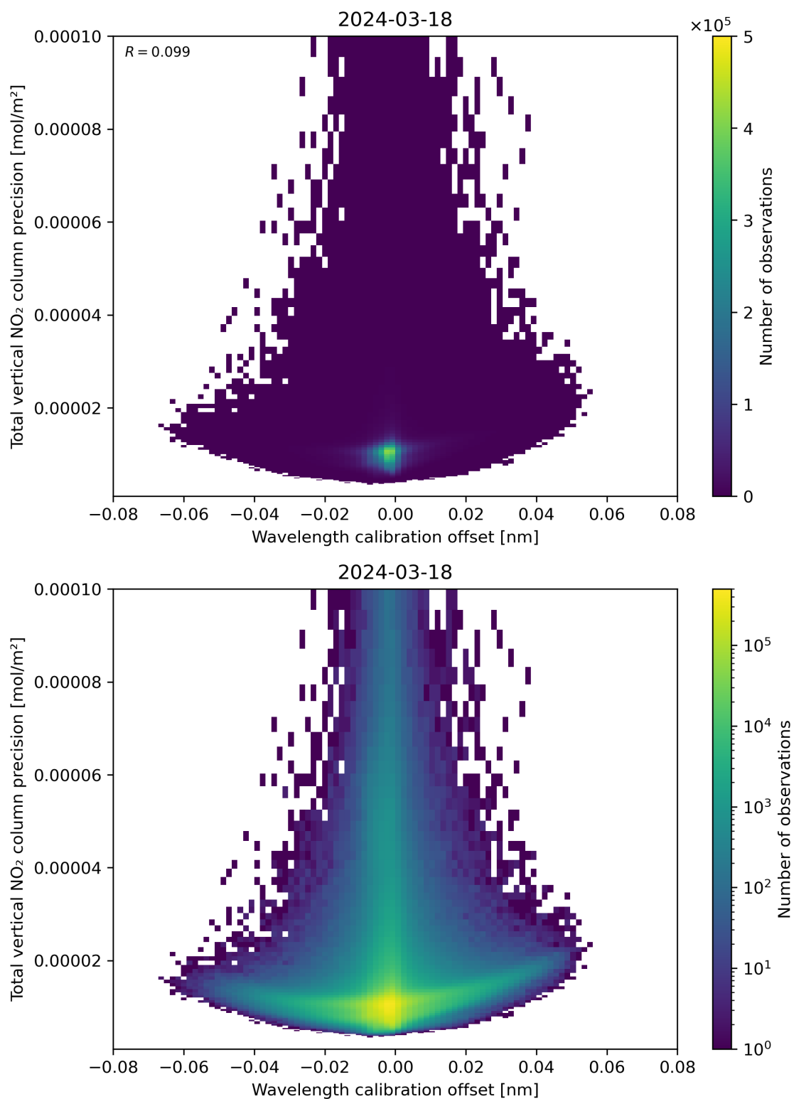
Figure 180: Scatter density plot of “Wavelength calibration offset” against “Total vertical NO 2 column precision” for 2024-03-17 to 2024-03-19.
