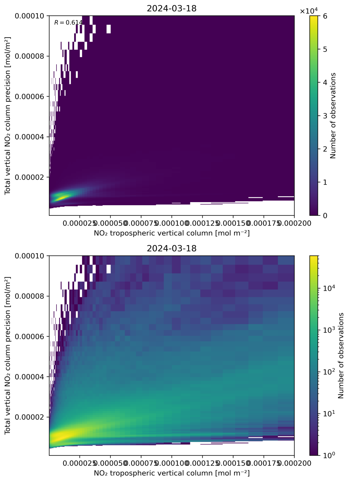
Figure 129: Scatter density plot of “NO 2 tropospheric vertical column” against “Total vertical NO 2 column precision” for 2024-03-17 to 2024-03-19.
