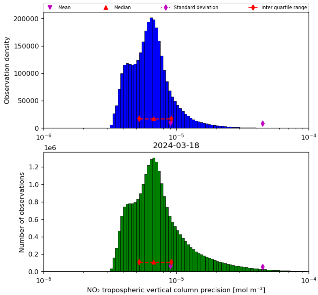
Figure 30: Histogram of “NO 2 tropospheric vertical column precision” for 2024-03-17 to 2024-03-19
