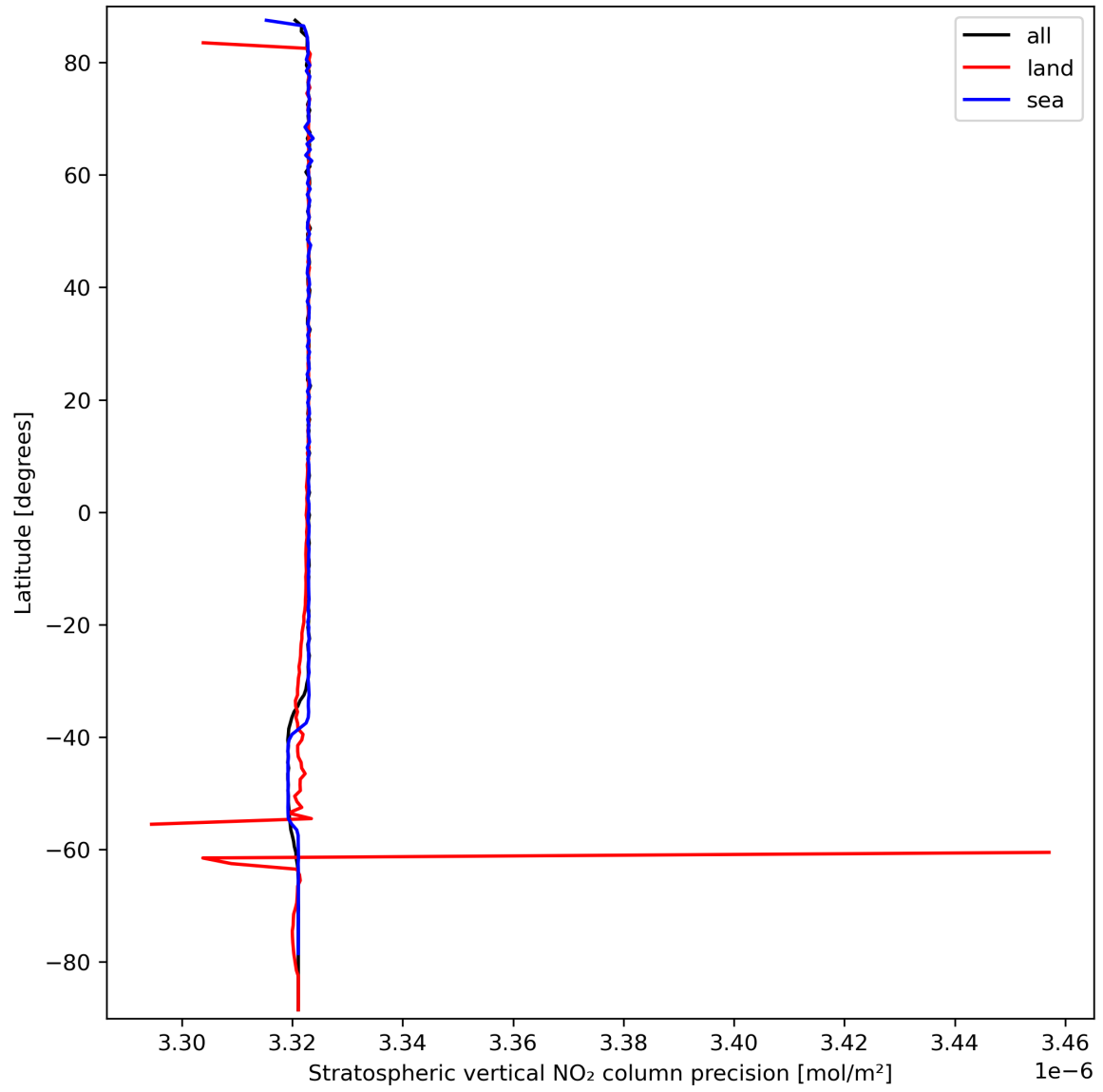
Figure 20: Zonal average of “Stratospheric vertical NO 2 column precision” for 2024-03-17 to 2024-03-19.
