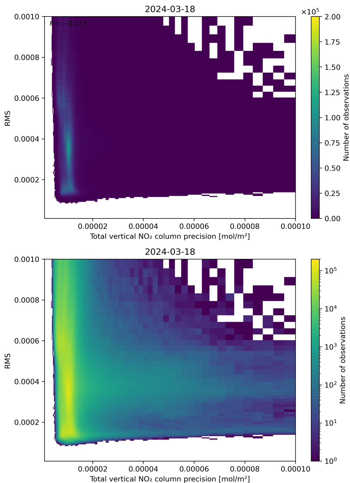
Figure 119: Scatter density plot of “Total vertical NO 2 column precision” against “RMS” for 2024-03-17 to 2024-03-19.
