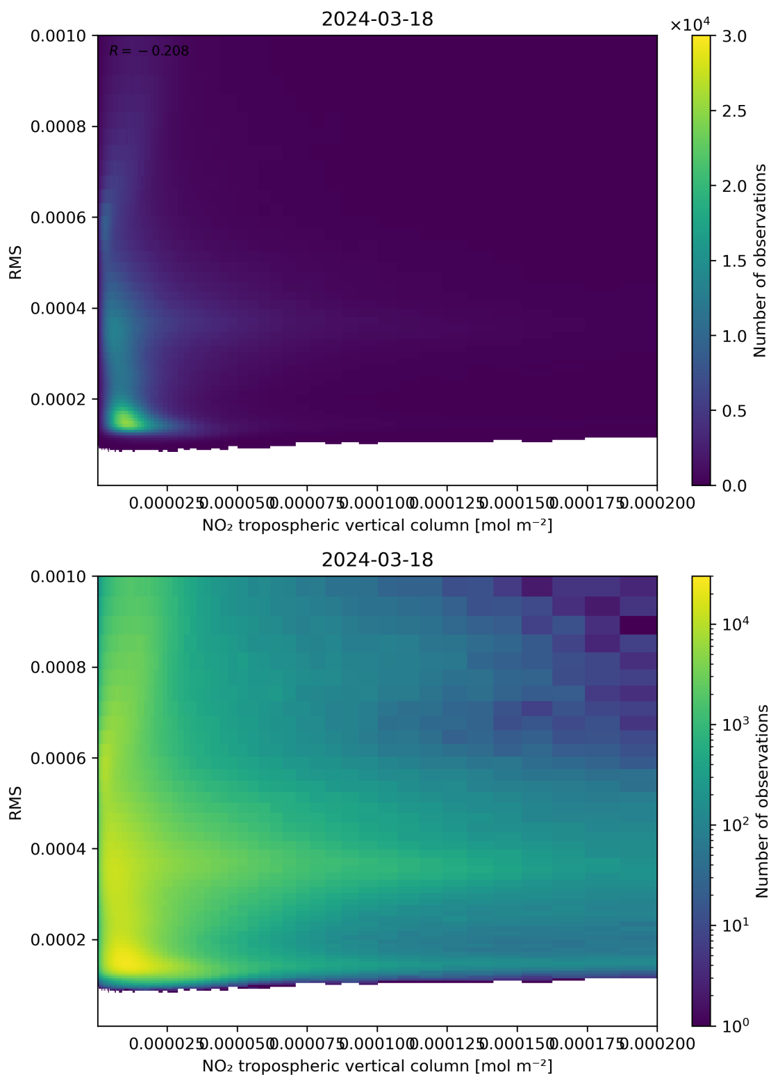
Figure 142: Scatter density plot of “NO 2 tropospheric vertical column” against “RMS” for 2024-03-17 to 2024-03-19.
