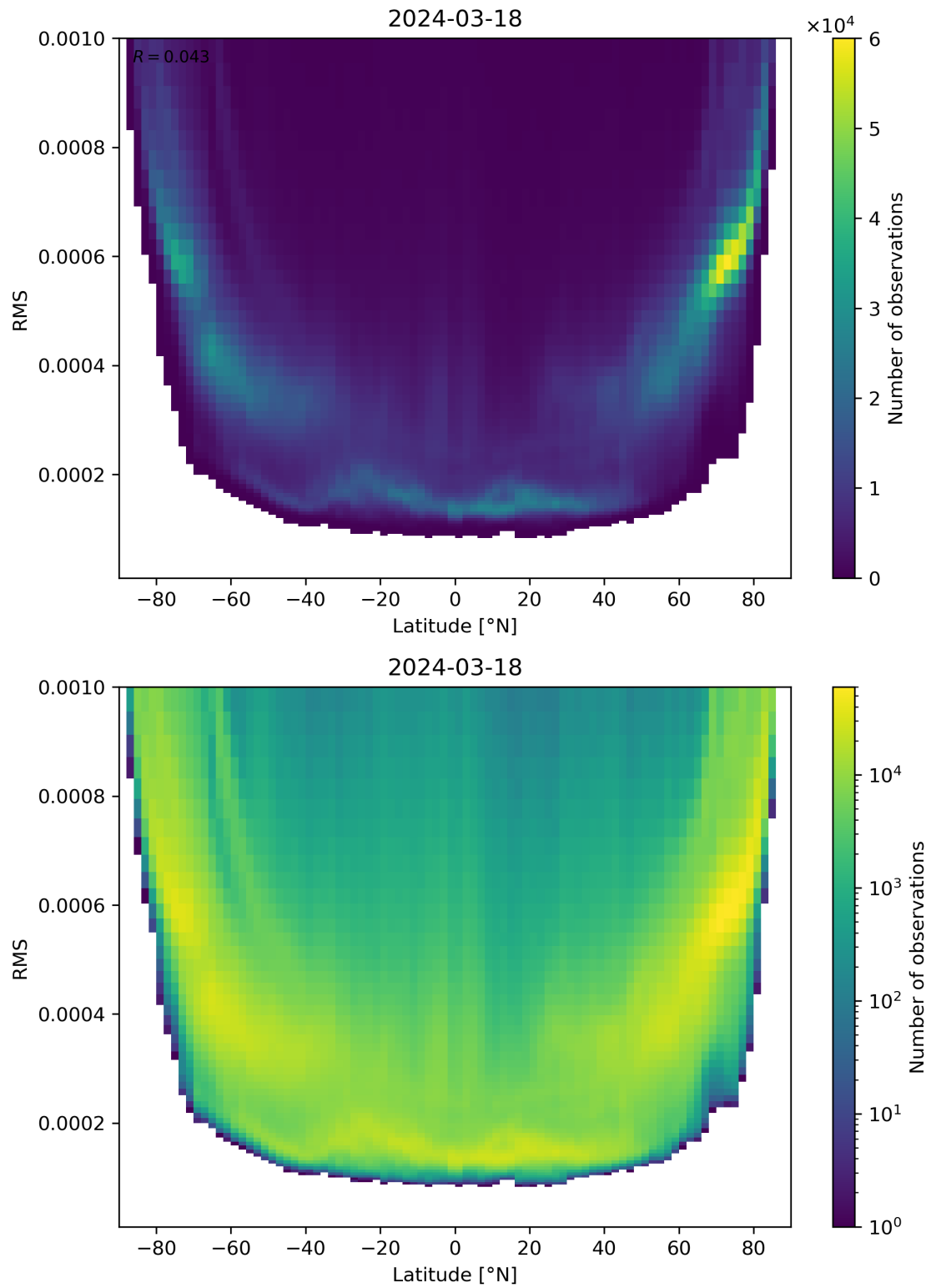
Figure 94: Scatter density plot of “Latitude” against “RMS” for 2024-03-17 to 2024-03-19.
