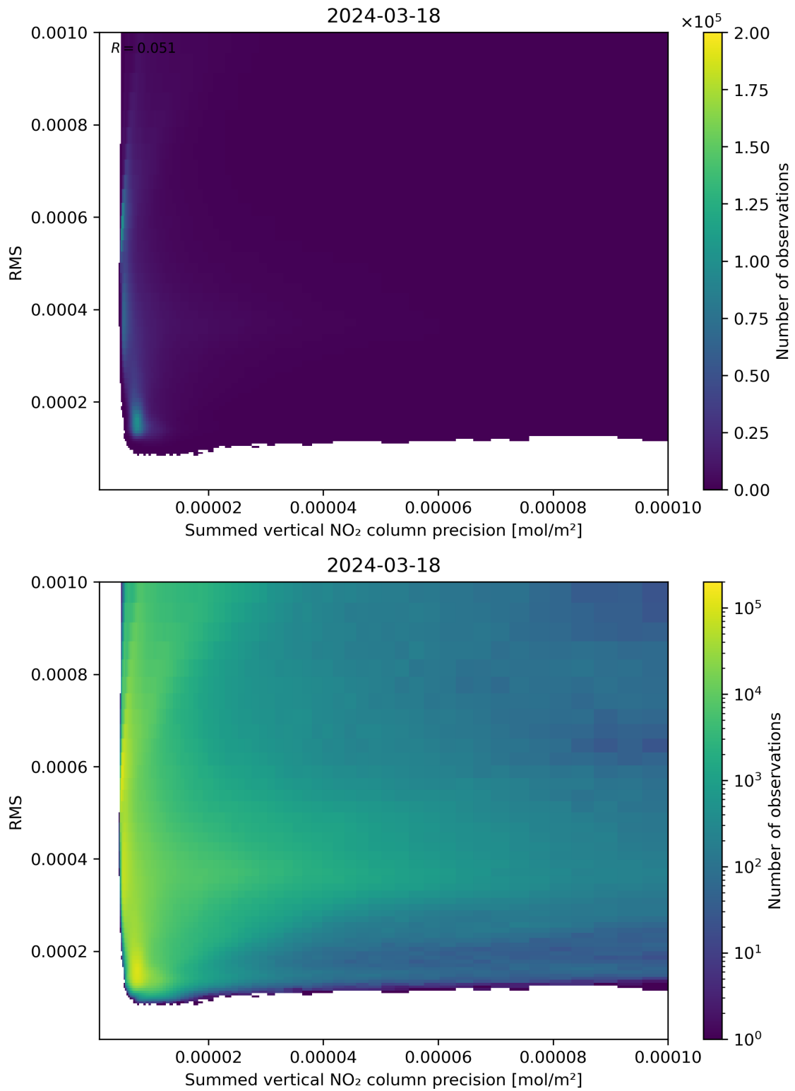
Figure 108: Scatter density plot of “Summed vertical NO 2 column precision” against “RMS” for 2024-03-17 to 2024-03-19.
