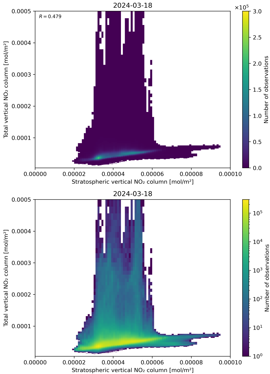
Figure 100: Scatter density plot of “Stratospheric vertical NO 2 column” against “Total vertical NO 2 column” for 2024-03-17 to 2024-03-19.
