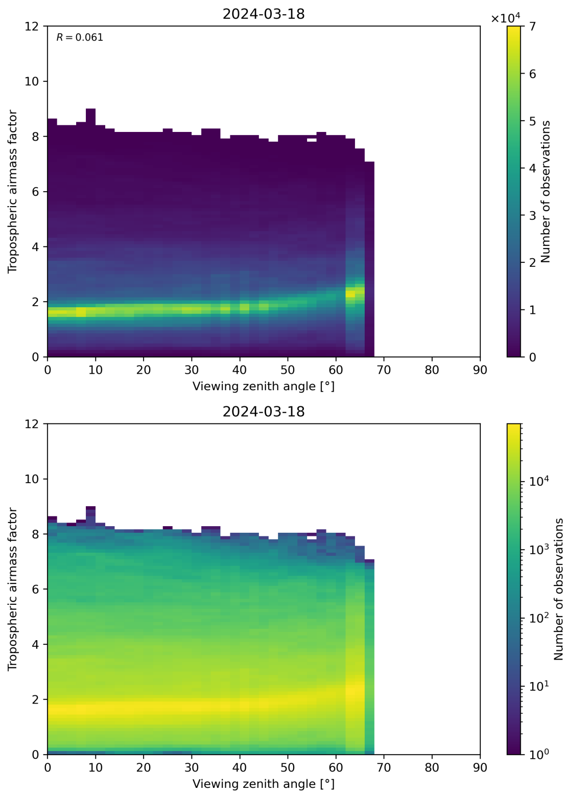
Figure 161: Scatter density plot of “Viewing zenith angle” against “Tropospheric airmass factor” for 2024-03-17 to 2024-03-19.
