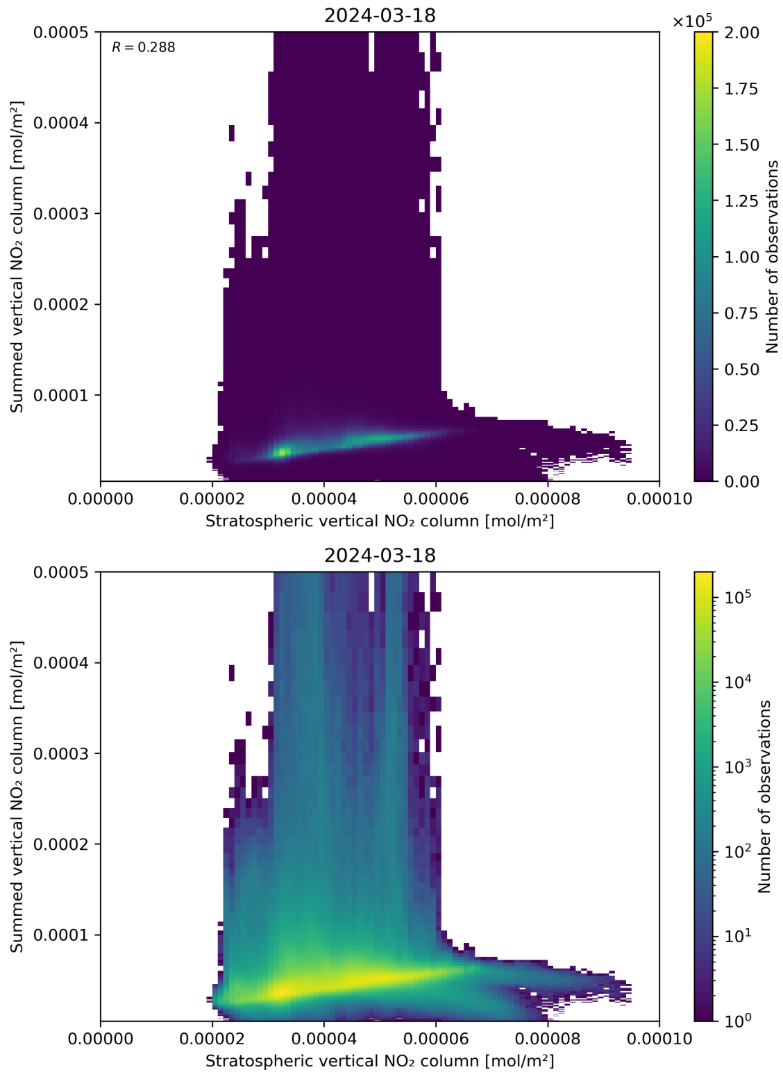
Figure 98: Scatter density plot of “Stratospheric vertical NO 2 column” against “Summed vertical NO 2 column” for 2024-03-17 to 2024-03-19.
