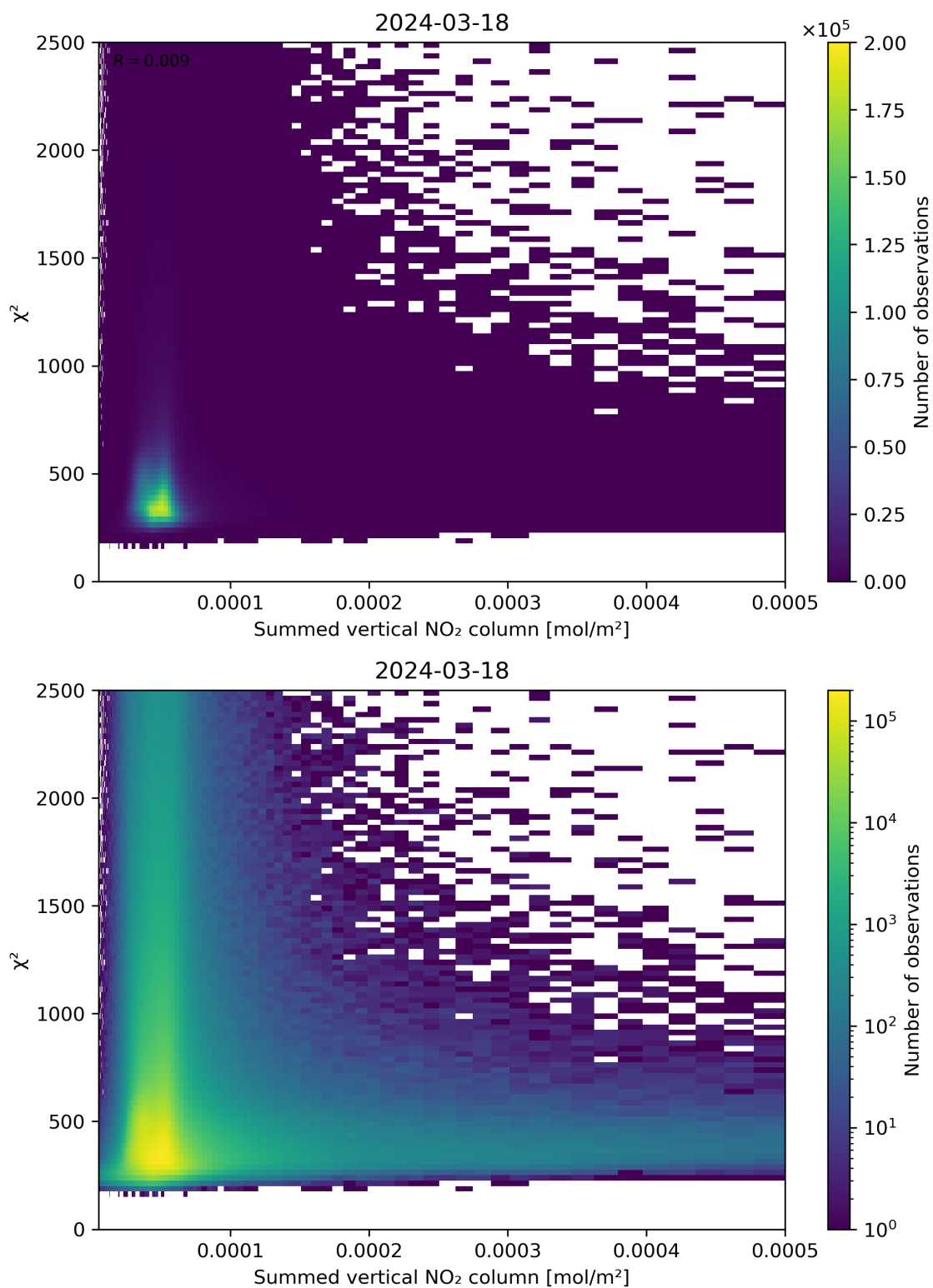
Figure 104: Scatter density plot of “Summed vertical NO 2 column” against “ \chi^2 ” for 2024-03-17 to 2024-03-19.
