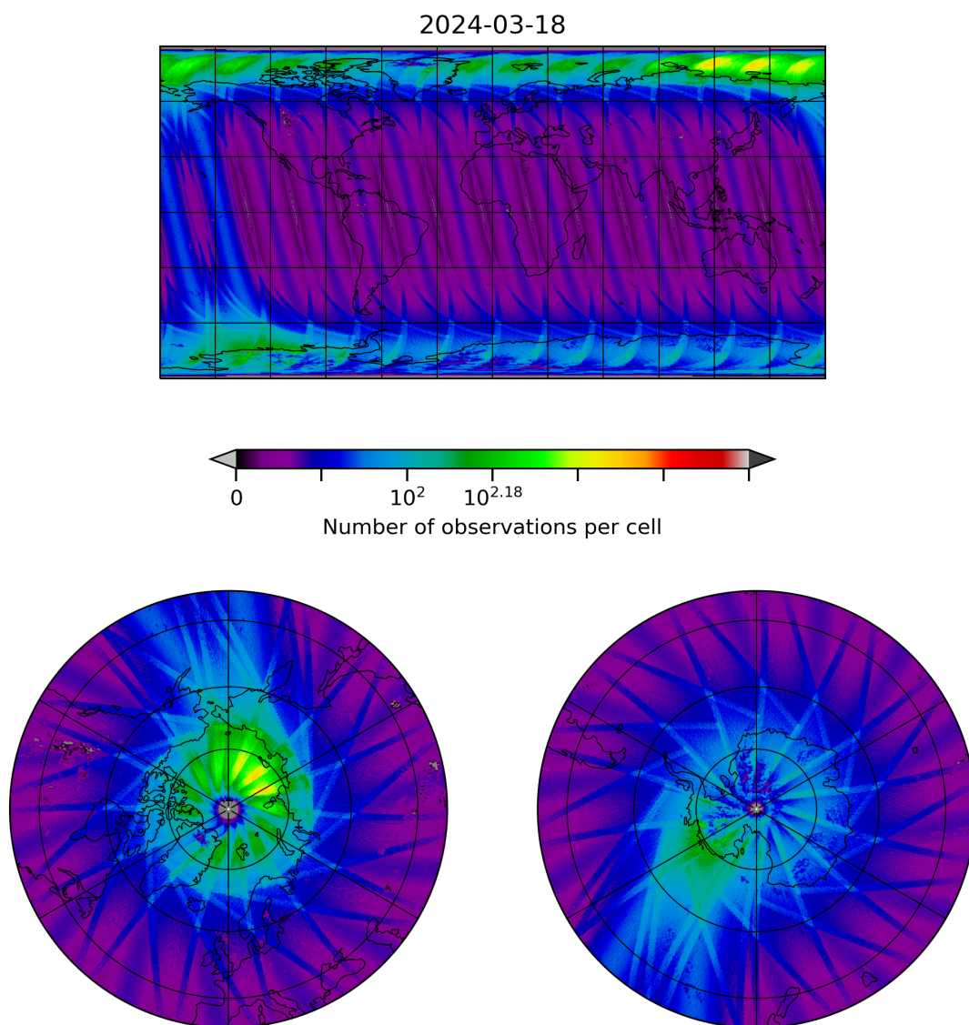
Figure 10: Map of the number of observations for 2024-03-17 to 2024-03-19
