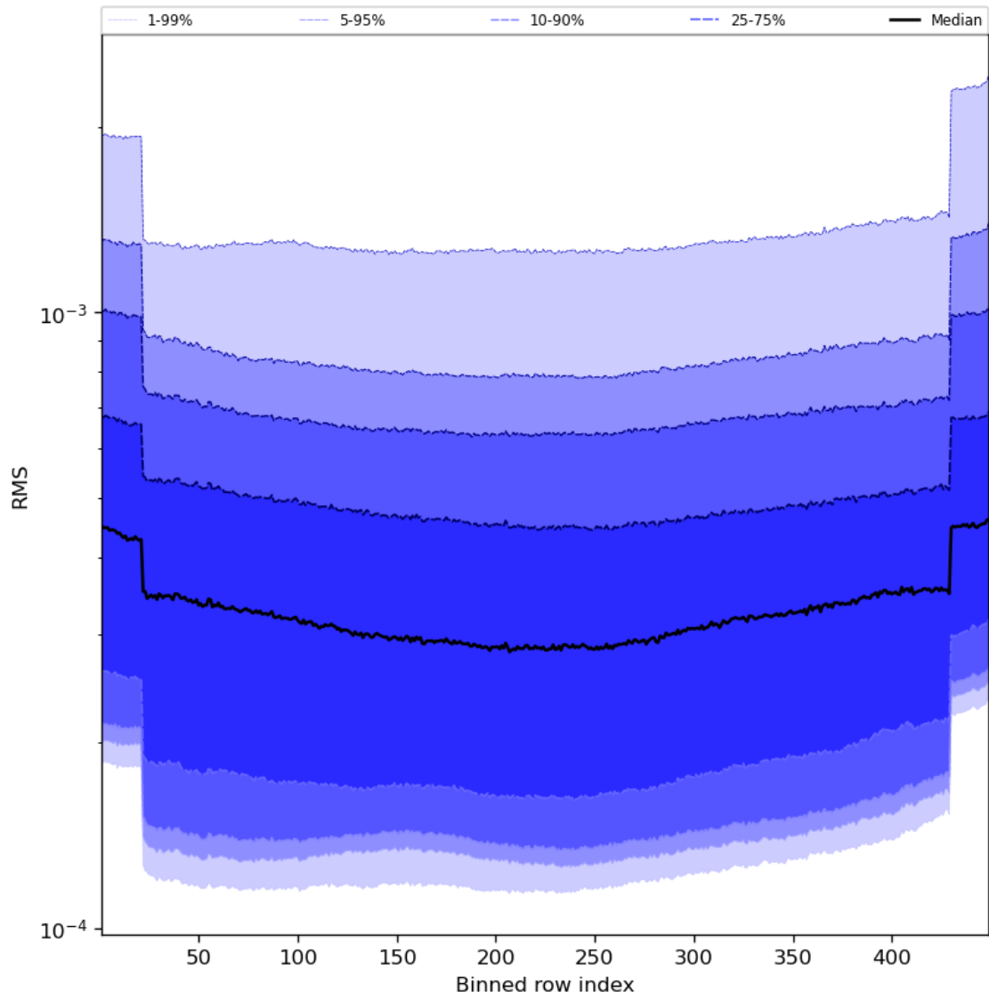
Figure 60: Along track statistics of “RMS” for 2024-03-17 to 2024-03-19
