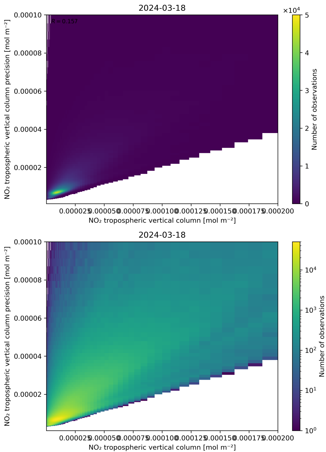
Figure 130: Scatter density plot of “NO 2 tropospheric vertical column” against “NO 2 tropospheric vertical column precision” for 2024-03-17 to 2024-03-19.
