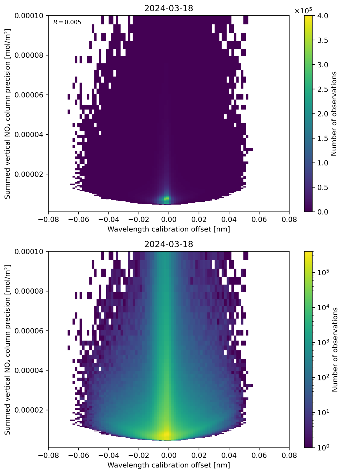
Figure 178: Scatter density plot of “Wavelength calibration offset” against “Summed vertical NO 2 column precision” for 2024-03-17 to 2024-03-19.
