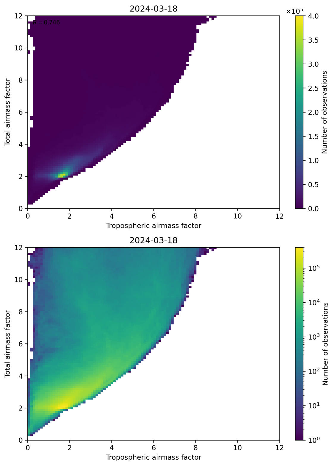
Figure 72: Scatter density plot of “Tropospheric airmass factor” against “Total airmass factor” for 2024-03-17 to 2024-03-19.
