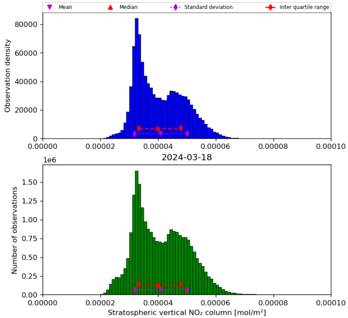
Figure 36: Histogram of “Stratospheric vertical NO 2 column” for 2024-03-17 to 2024-03-19
