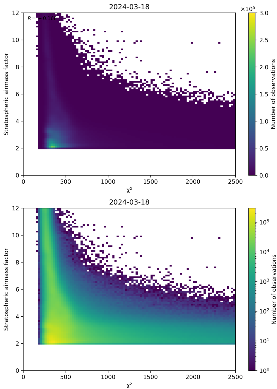
Figure 81: Scatter density plot of “ \chi^2 ” against “Stratospheric airmass factor” for 2024-03-17 to 2024-03-19.
