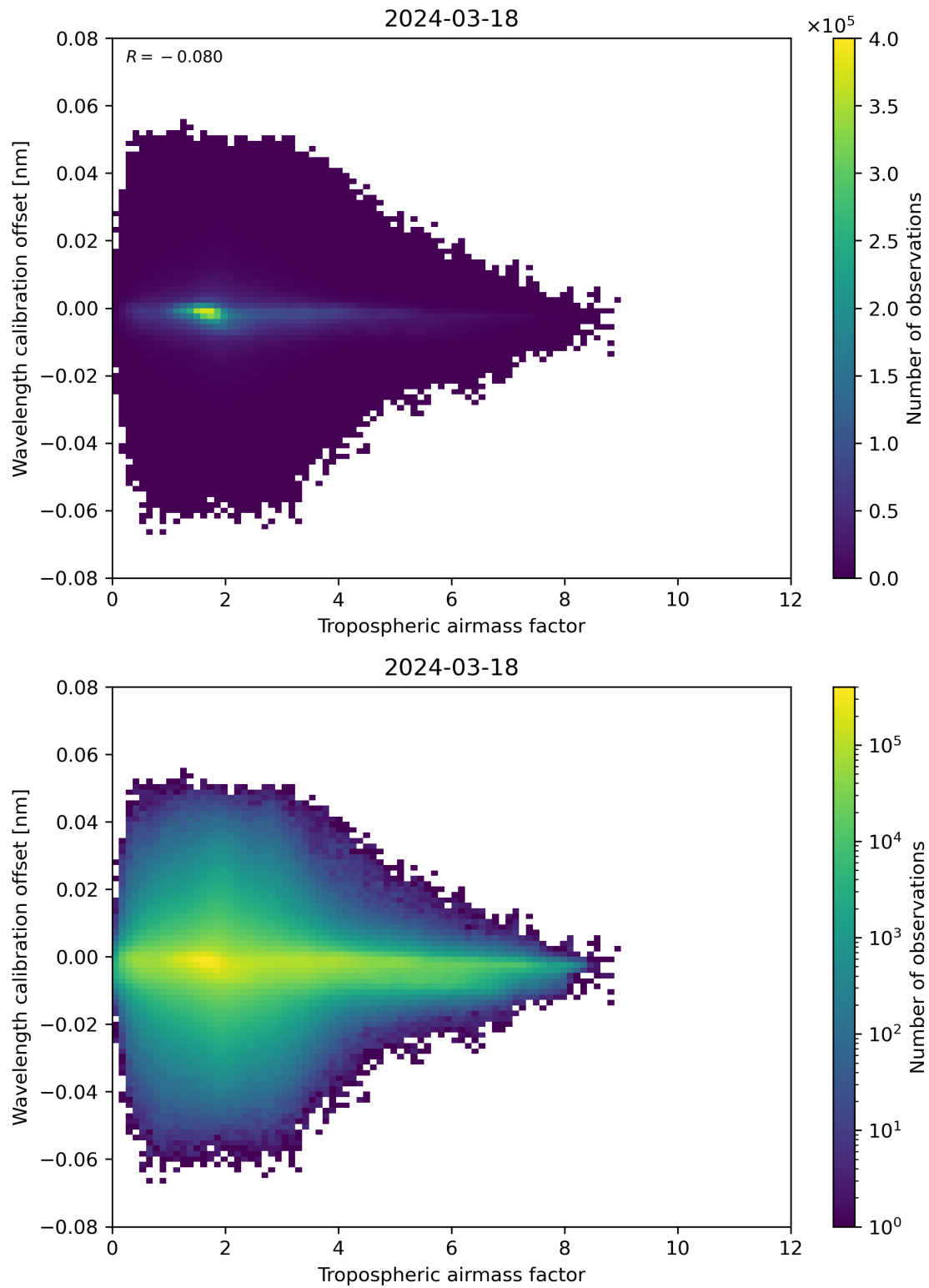
Figure 80: Scatter density plot of “Tropospheric airmass factor” against “Wavelength calibration offset” for 2024-03-17 to 2024-03-19.
