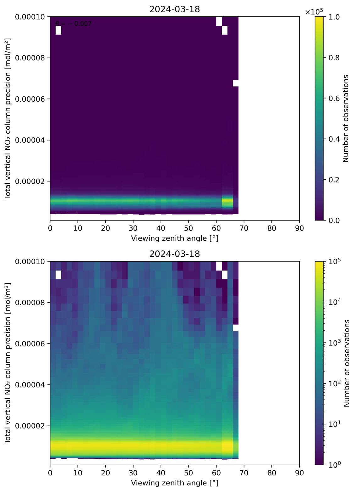
Figure 168: Scatter density plot of “Viewing zenith angle” against “Total vertical NO 2 column precision” for 2024-03-17 to 2024-03-19.
