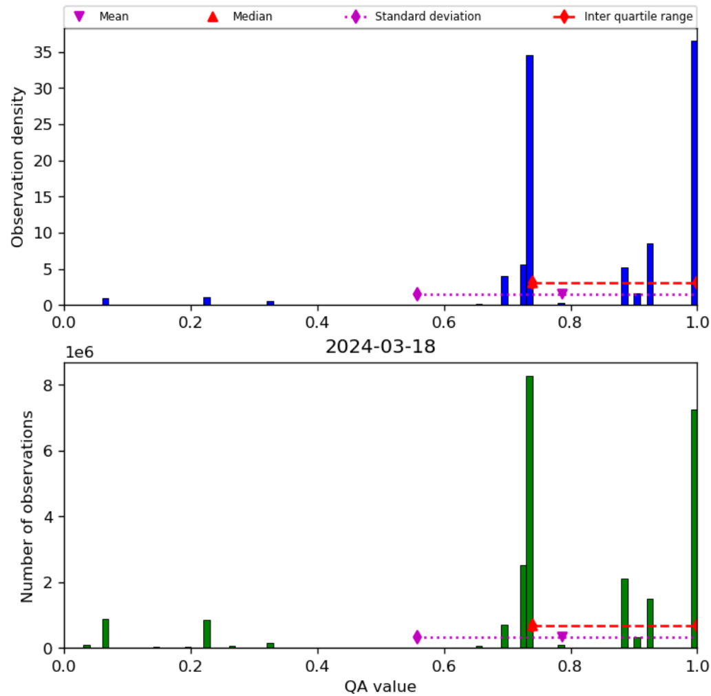
Figure 28: Histogram of “QA value” for 2024-03-17 to 2024-03-19
