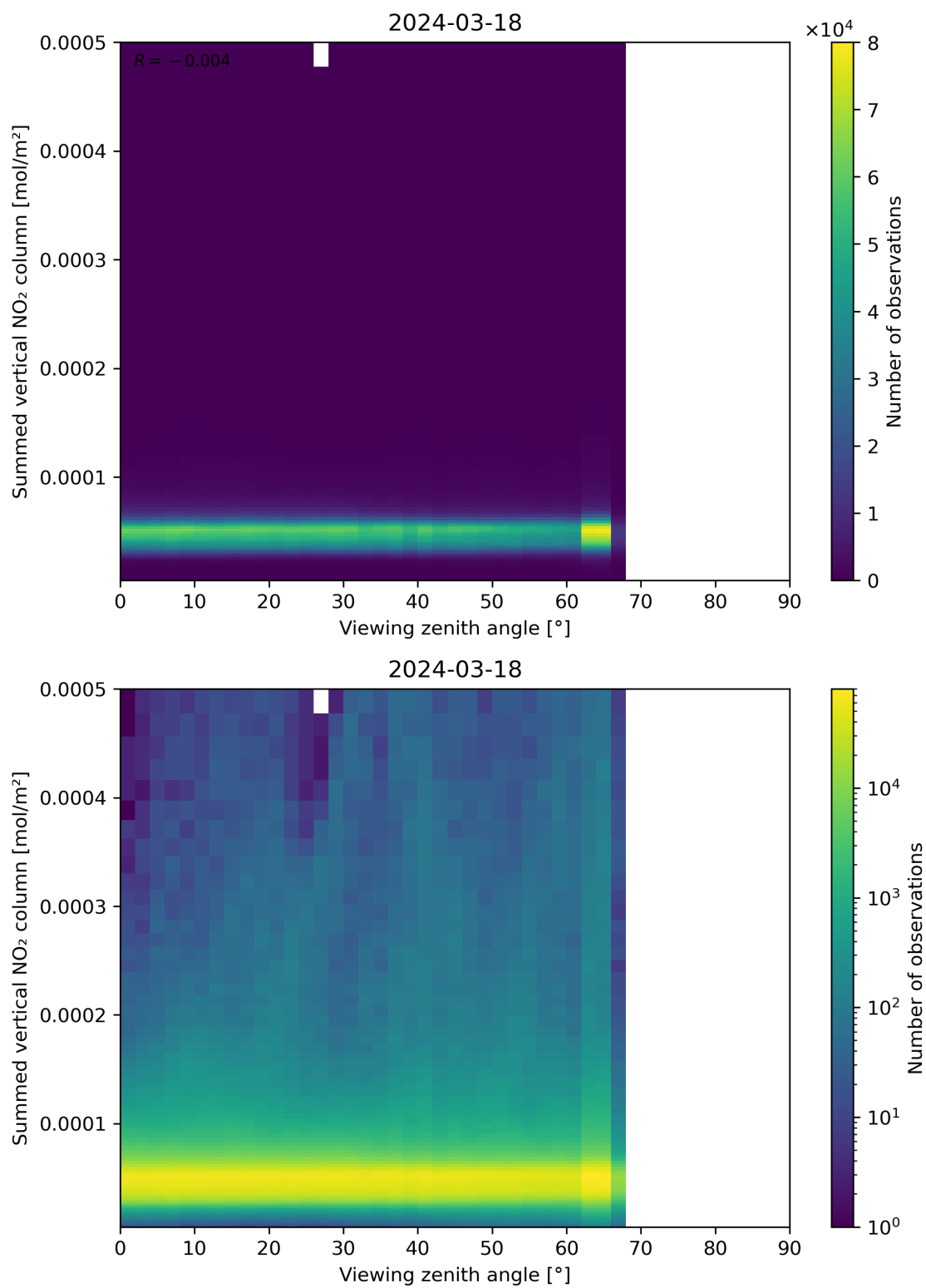
Figure 165: Scatter density plot of “Viewing zenith angle” against “Summed vertical NO 2 column” for 2024-03-17 to 2024-03-19.
