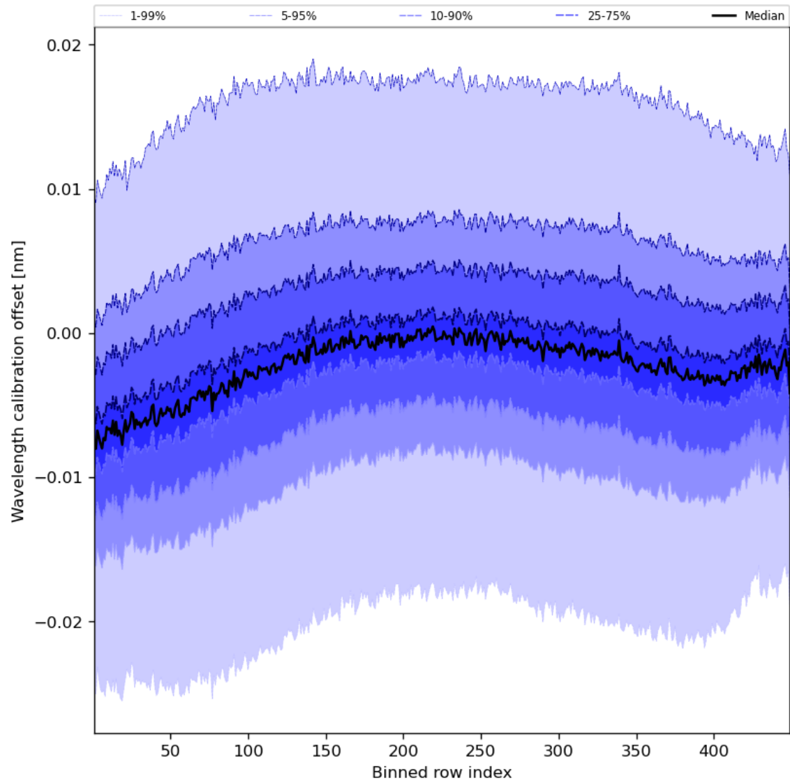
Figure 52: Along track statistics of “Wavelength calibration offset” for 2024-03-17 to 2024-03-19
