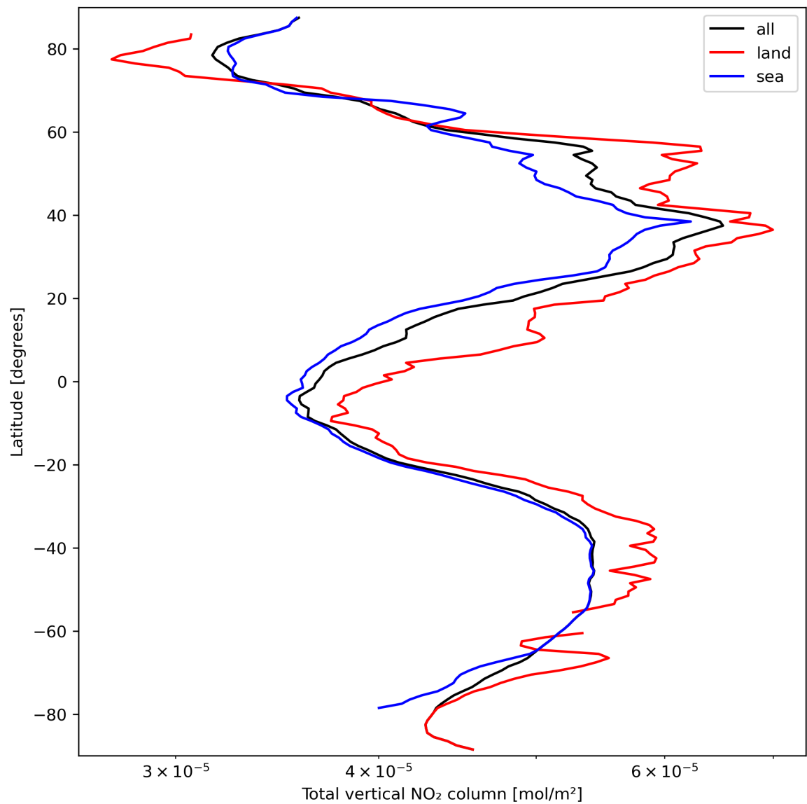
Figure 21: Zonal average of “Total vertical NO 2 column” for 2024-03-17 to 2024-03-19.
