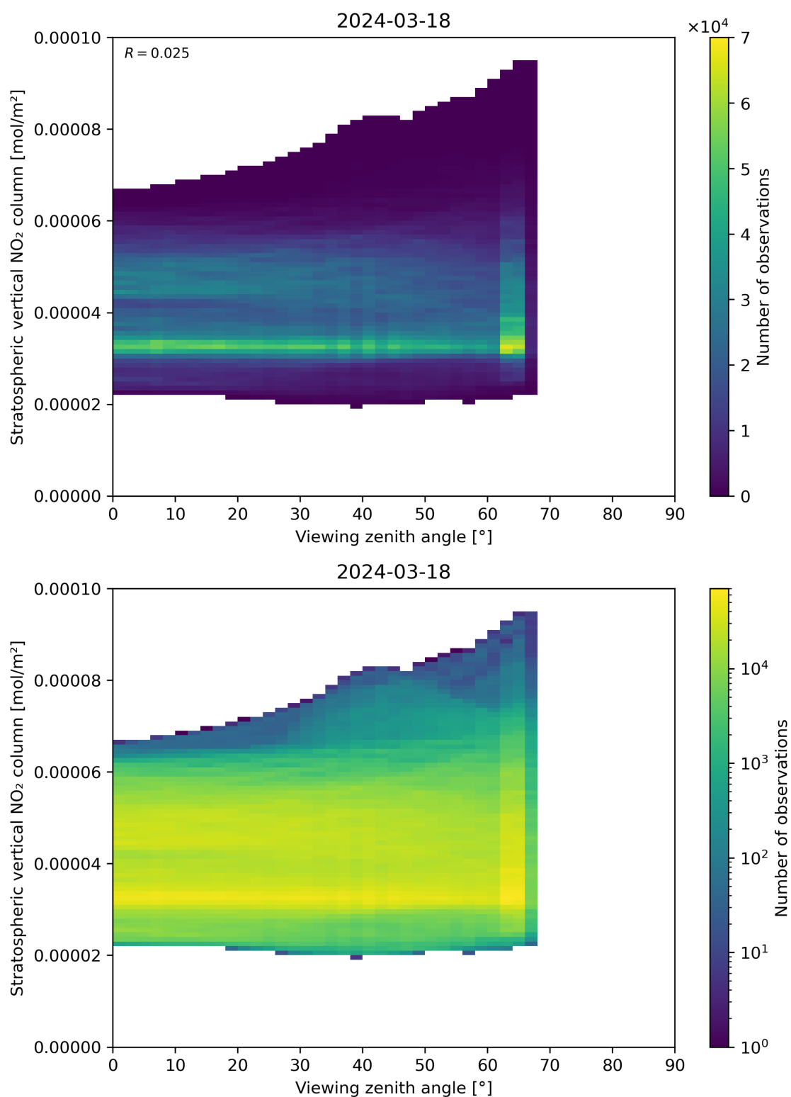
Figure 164: Scatter density plot of “Viewing zenith angle” against “Stratospheric vertical NO 2 column” for 2024-03-17 to 2024-03-19.
