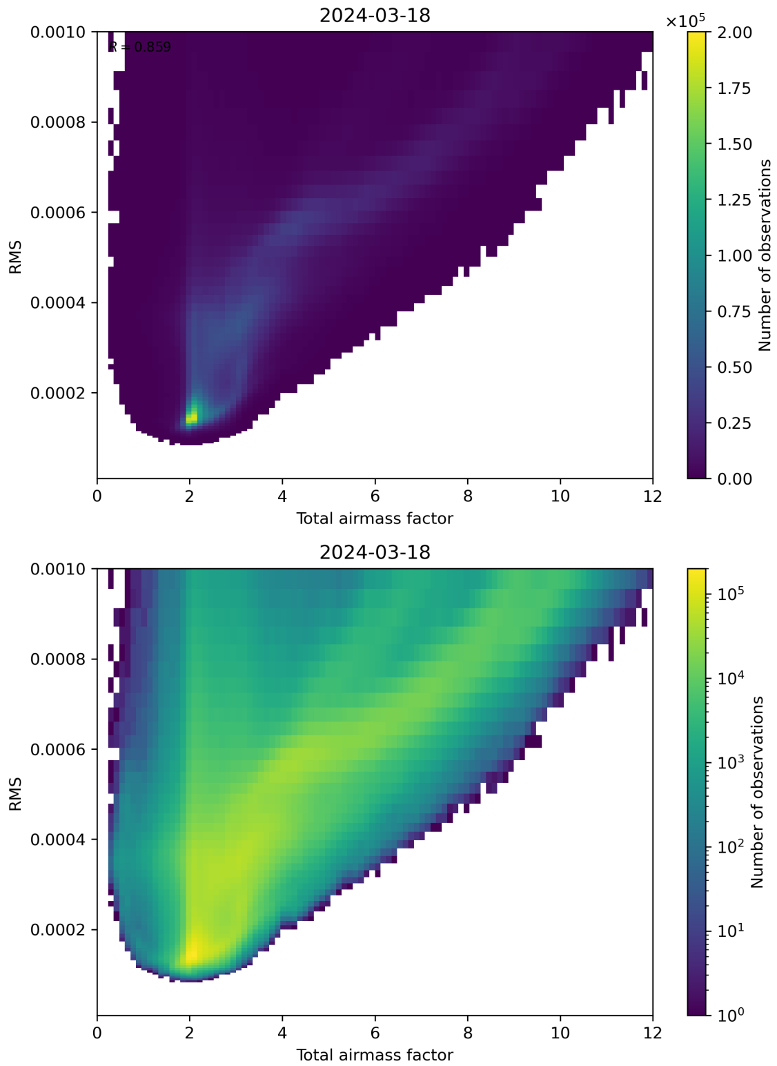
Figure 69: Scatter density plot of “Total airmass factor” against “RMS” for 2024-03-17 to 2024-03-19.
