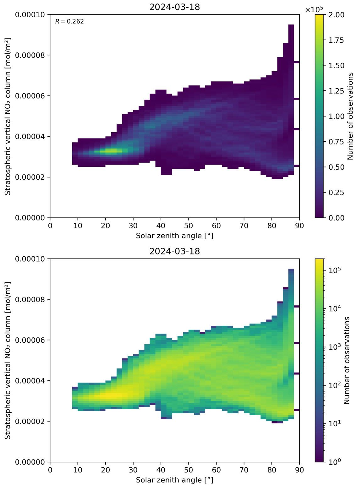
Figure 150: Scatter density plot of “Solar zenith angle” against “Stratospheric vertical \text{NO}_2 column” for 2024-03-17 to 2024-03-19.
