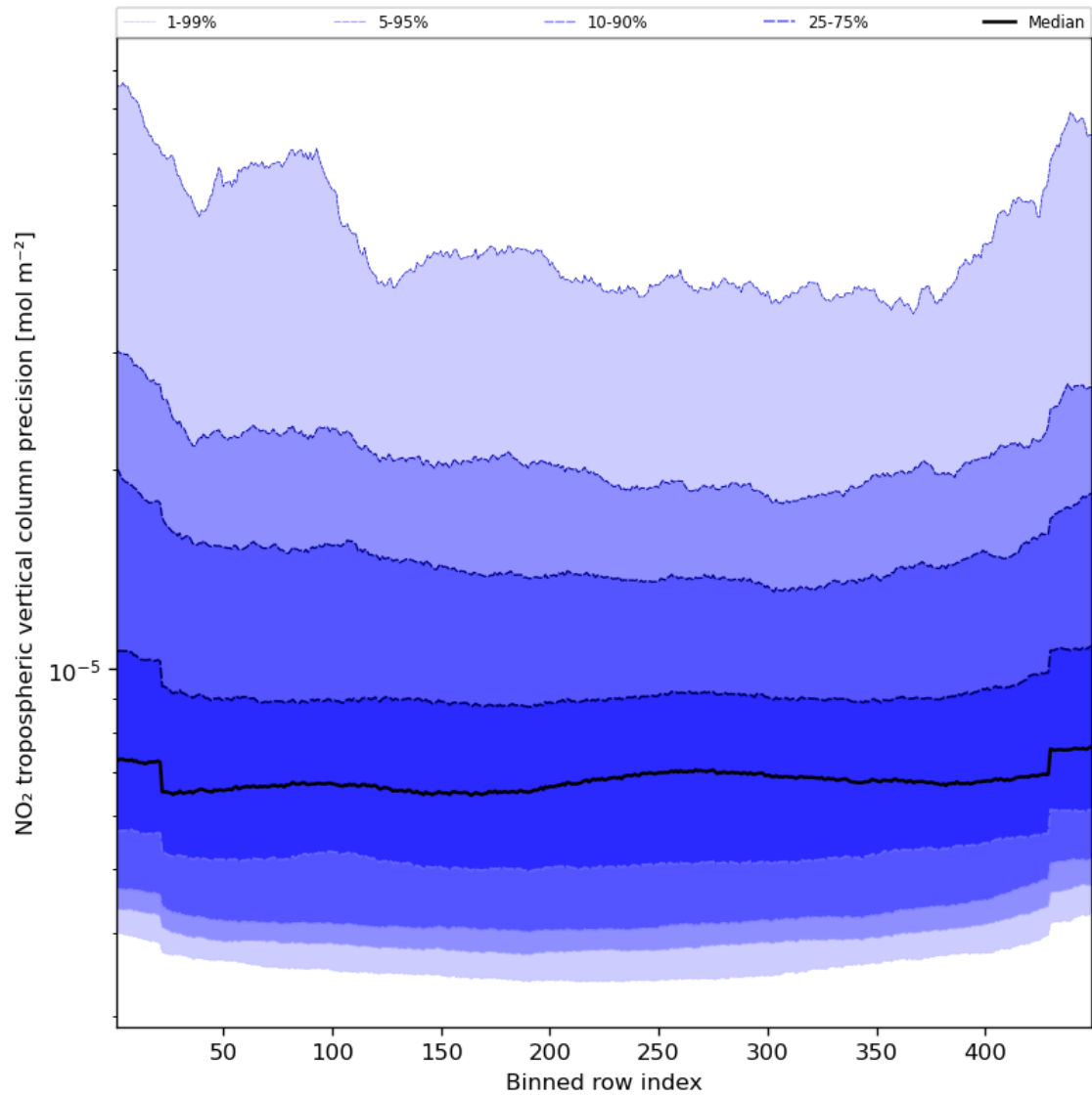
Figure 47: Along track statistics of “NO 2 tropospheric vertical column precision” for 2024-03-17 to 2024-03-19
