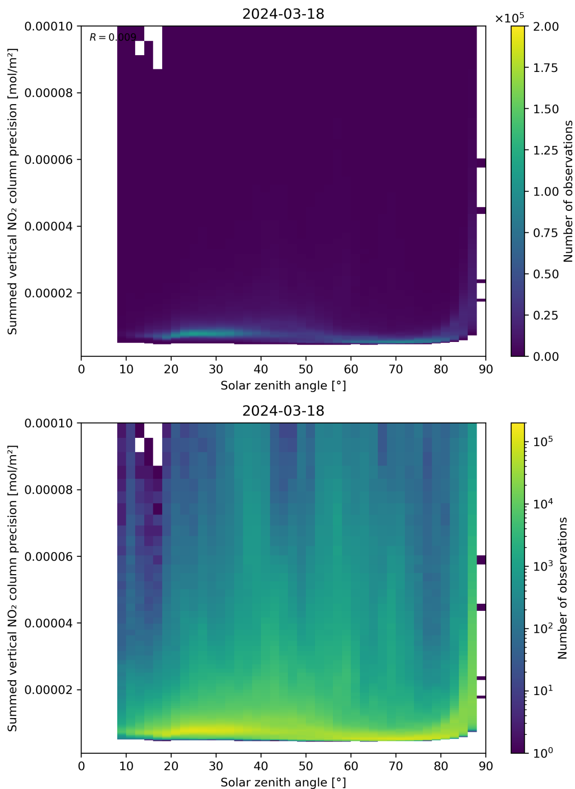
Figure 152: Scatter density plot of “Solar zenith angle” against “Summed vertical NO 2 column precision” for 2024-03-17 to 2024-03-19.
