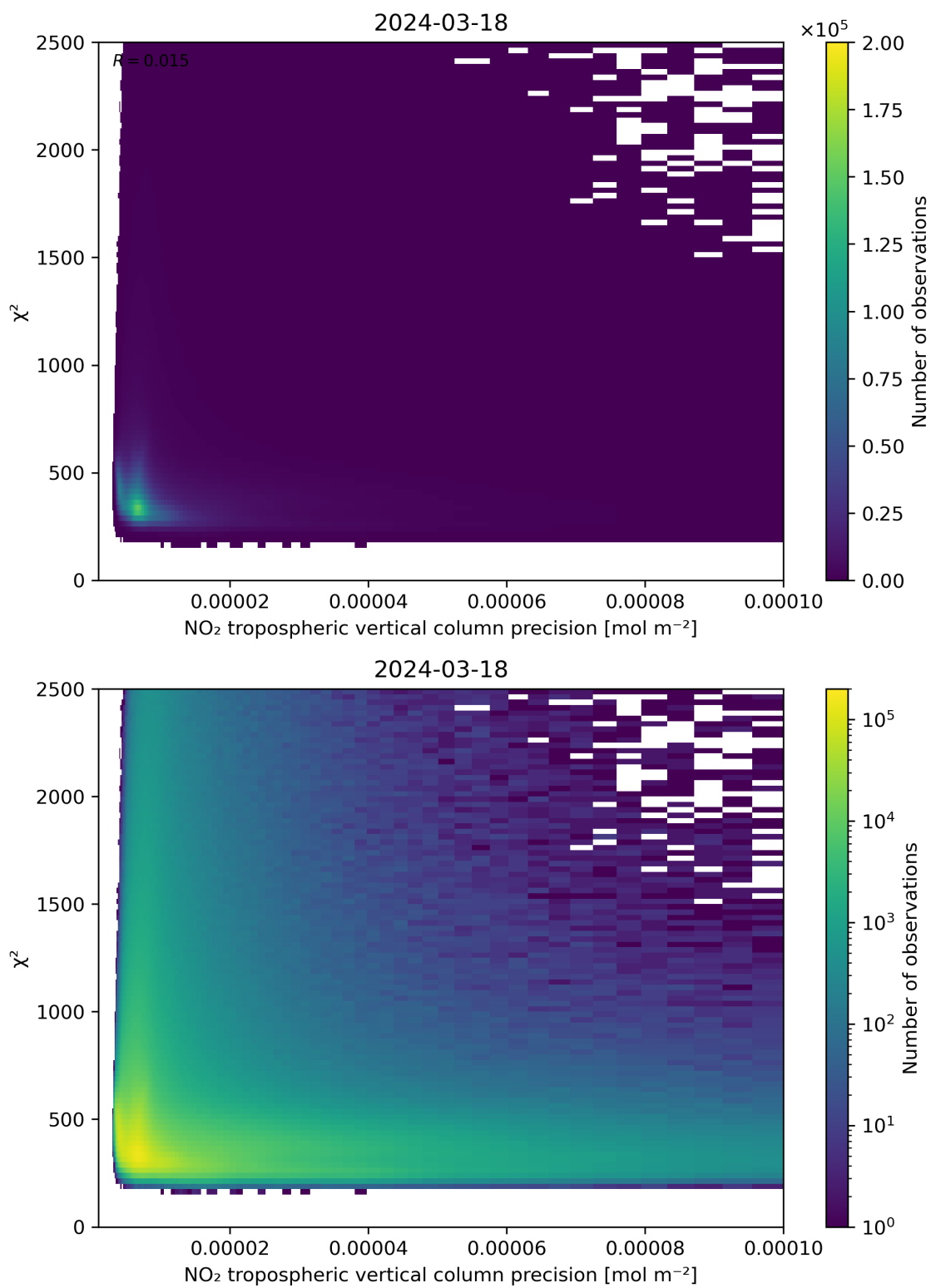
Figure 134: Scatter density plot of “NO 2 tropospheric vertical column precision” against “ \chi^2 ” for 2024-03-17 to 2024-03-19.
