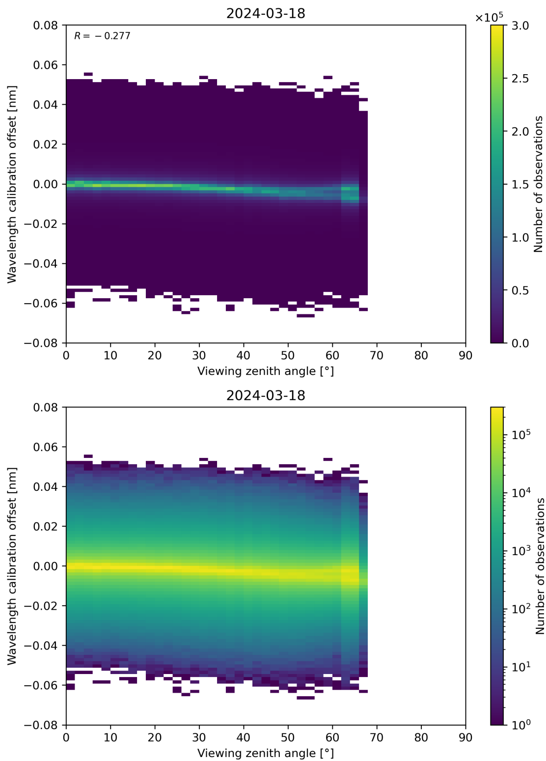
Figure 173: Scatter density plot of “Viewing zenith angle” against “Wavelength calibration offset” for 2024-03-17 to 2024-03-19.
