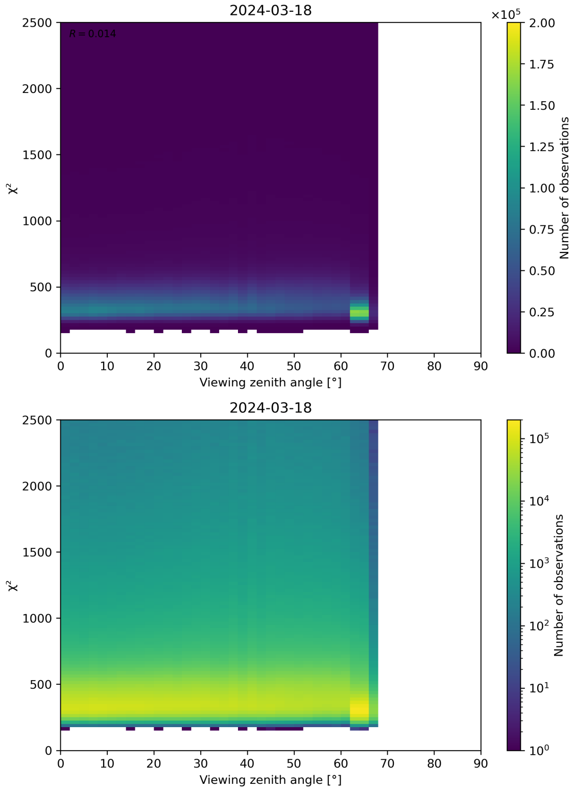
Figure 162: Scatter density plot of “Viewing zenith angle” against “ \chi^2 ” for 2024-03-17 to 2024-03-19.
