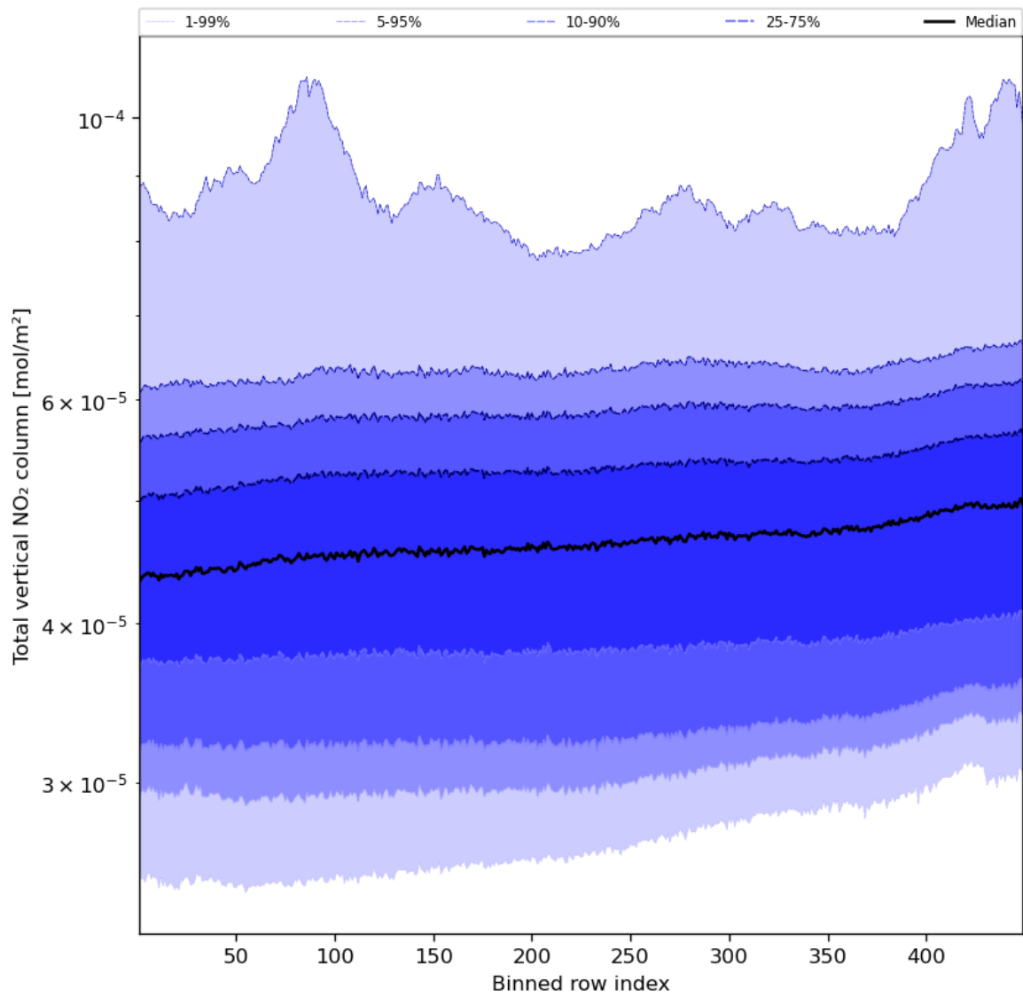
Figure 55: Along track statistics of “Total vertical NO 2 column” for 2024-03-17 to 2024-03-19
