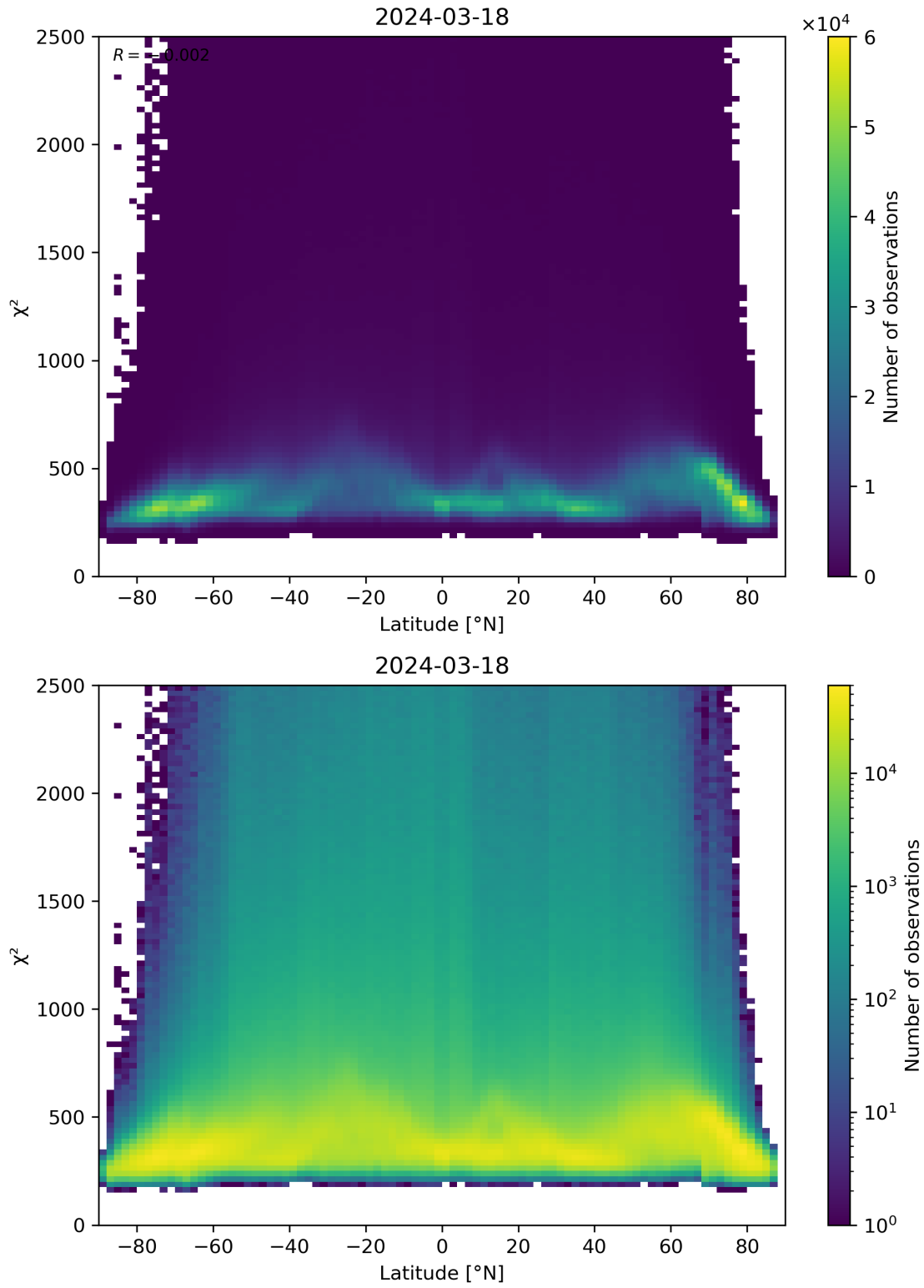
Figure 86: Scatter density plot of “Latitude” against “ \chi^2 ” for 2024-03-17 to 2024-03-19.
