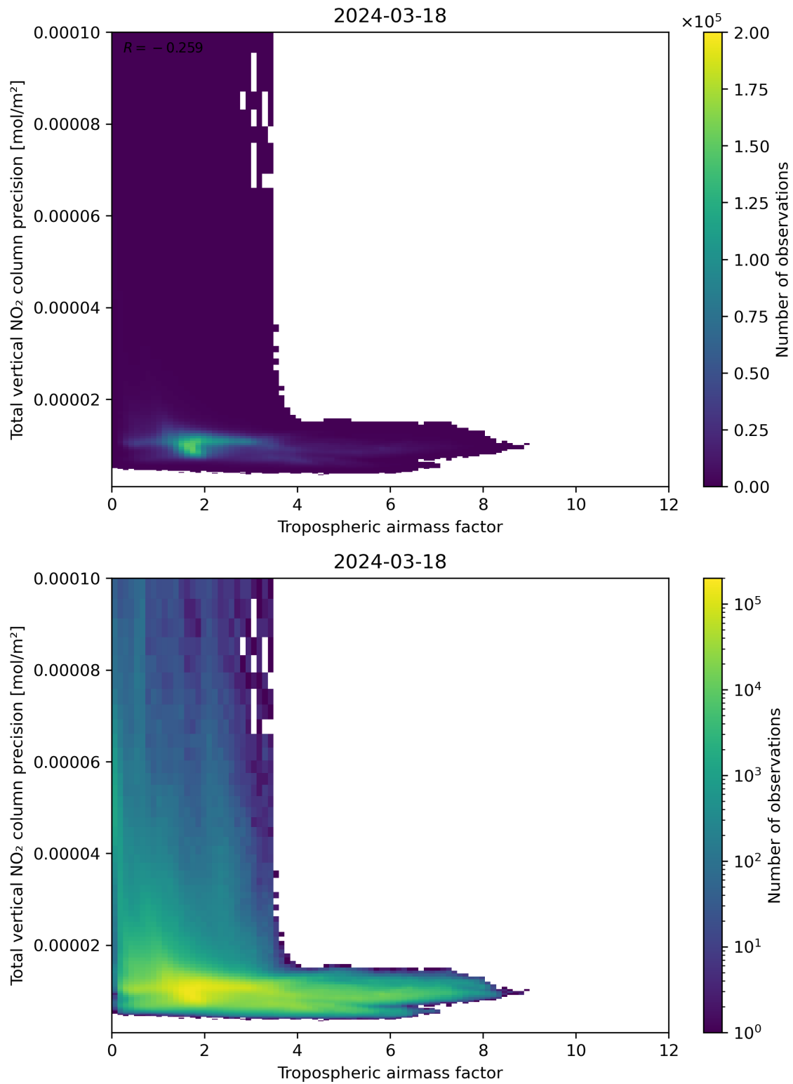
Figure 78: Scatter density plot of “Tropospheric air mass factor” against “Total vertical NO 2 column precision” for 2024-03-17 to 2024-03-19.
