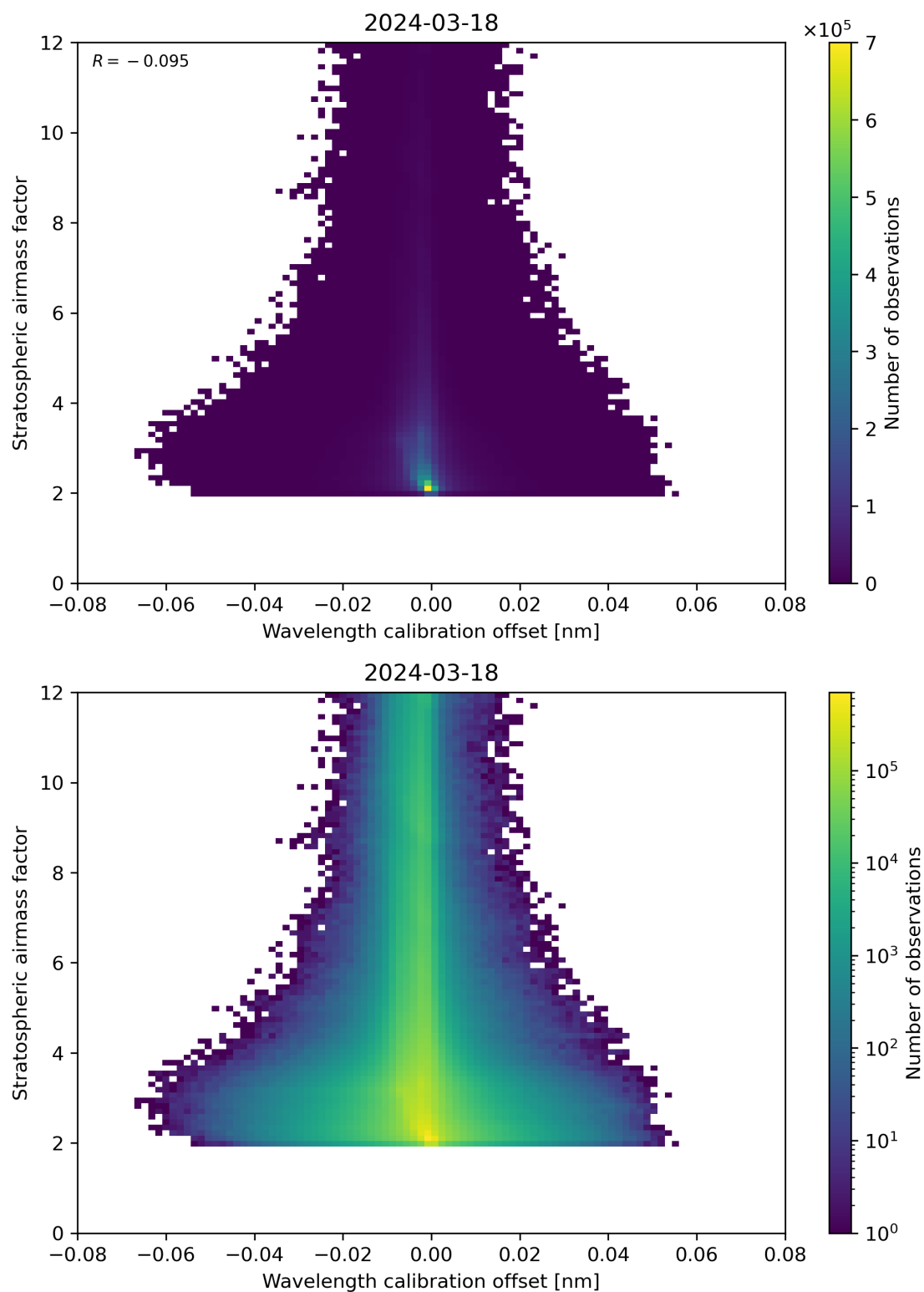
Figure 174: Scatter density plot of “Wavelength calibration offset” against “Stratospheric air mass factor” for 2024-03-17 to 2024-03-19.
