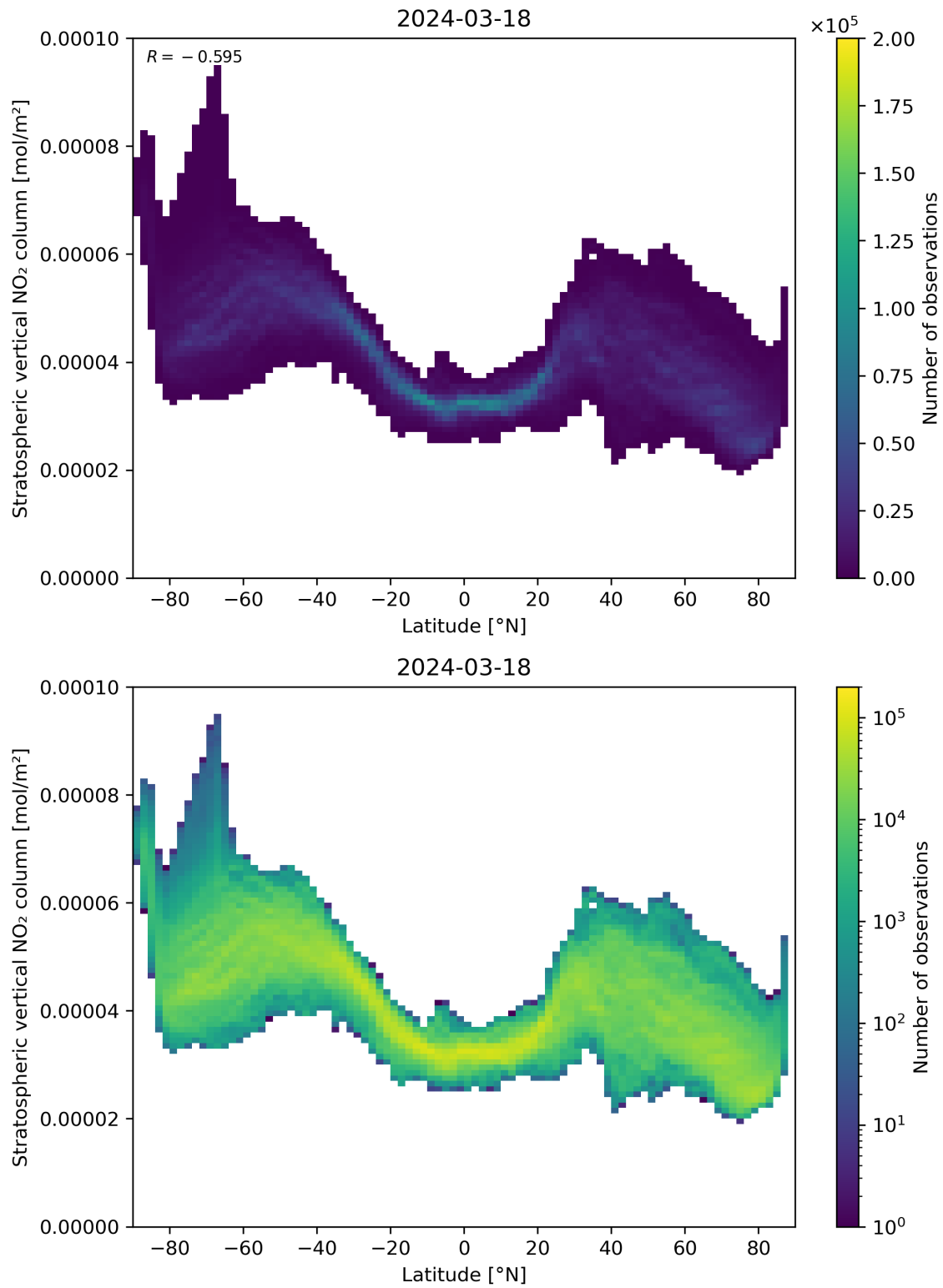
Figure 87: Scatter density plot of “Latitude” against “Stratospheric vertical NO 2 column” for 2024-03-17 to 2024-03-19.
