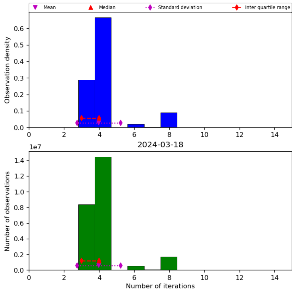
Figure 34: Histogram of “Number of iterations” for 2024-03-17 to 2024-03-19
