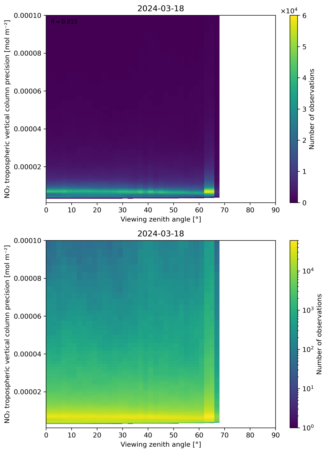
Figure 170: Scatter density plot of “Viewing zenith angle” against “NO 2 tropospheric vertical column precision” for 2024-03-17 to 2024-03-19.
