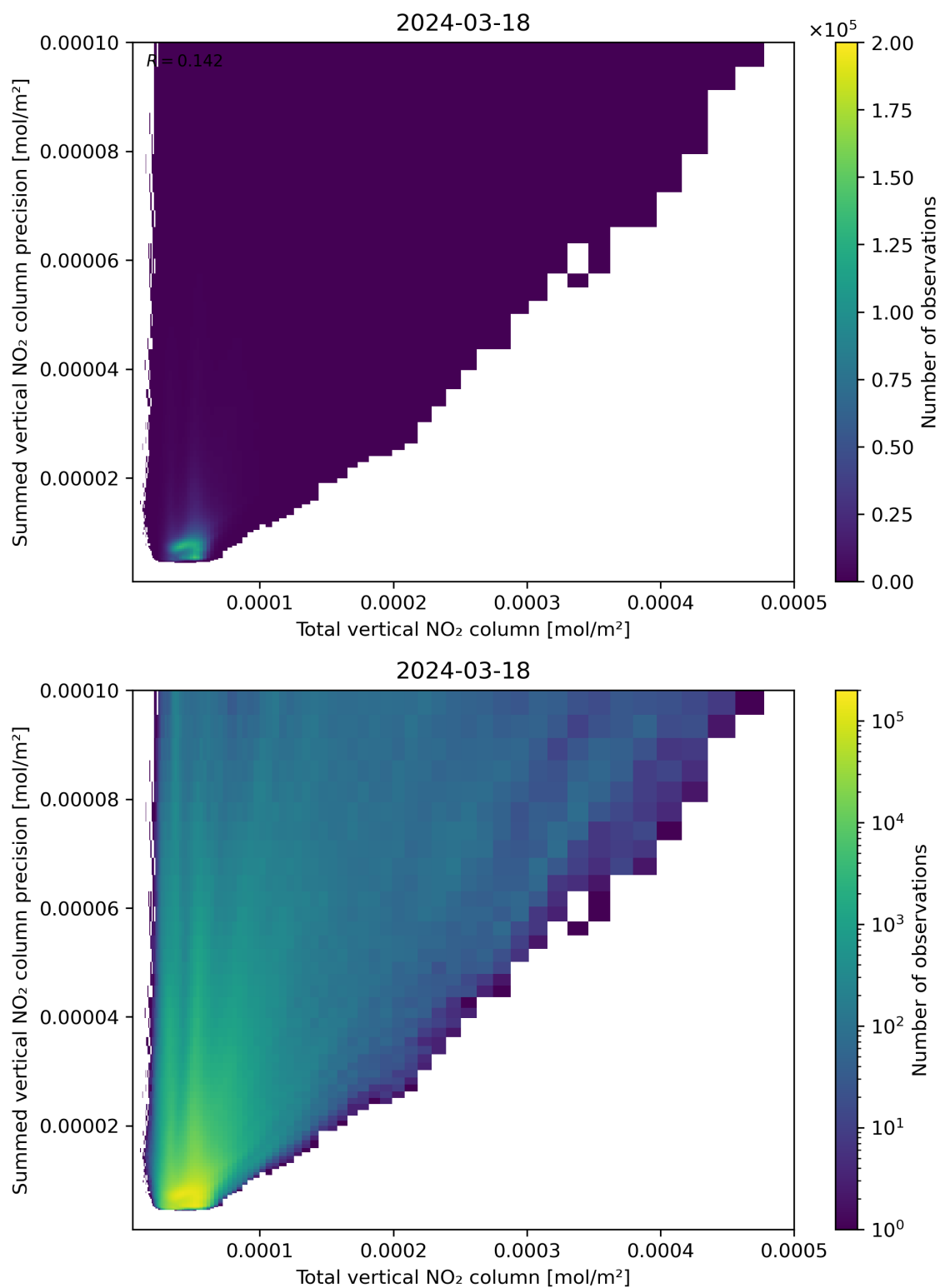
Figure 113: Scatter density plot of “Total vertical NO 2 column” against “Summed vertical NO 2 column precision” for 2024-03-17 to 2024-03-19.
