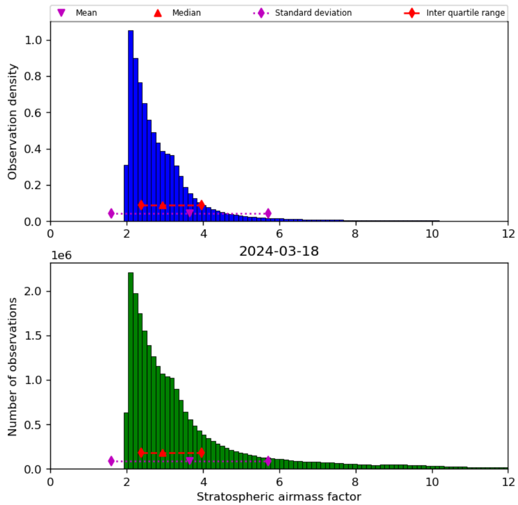
Figure 44: Histogram of “Stratospheric airmass factor” for 2024-03-17 to 2024-03-19
