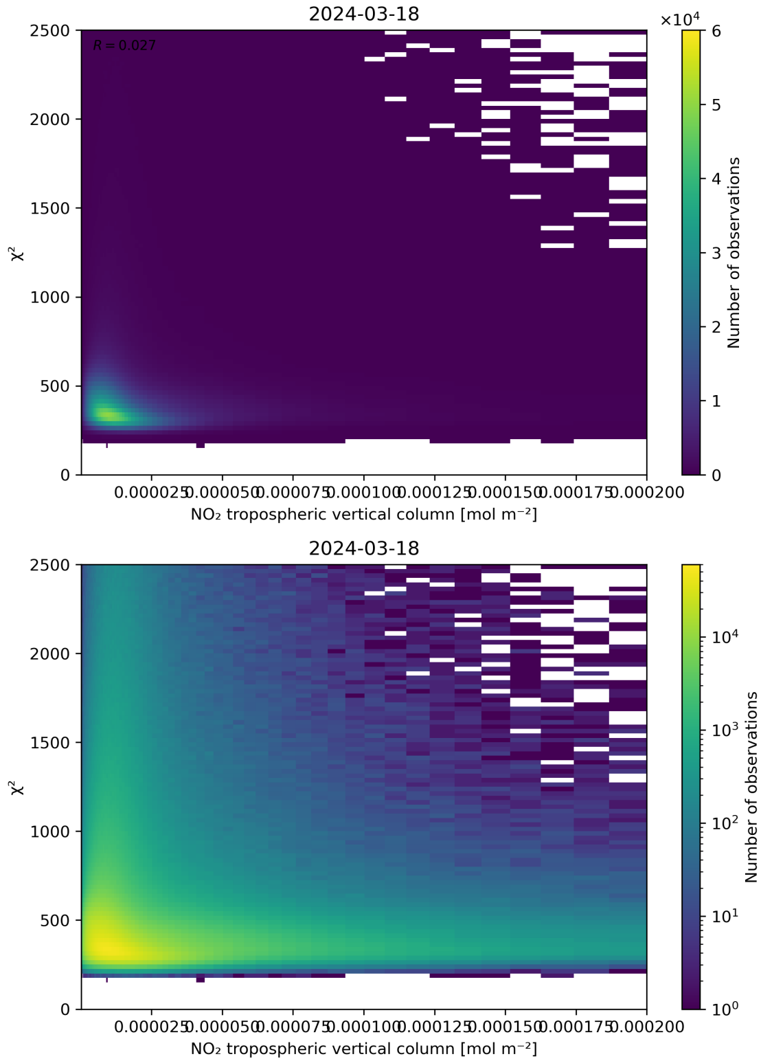
Figure 124: Scatter density plot of “NO 2 tropospheric vertical column” against “ \chi^2 ” for 2024-03-17 to 2024-03-19.
