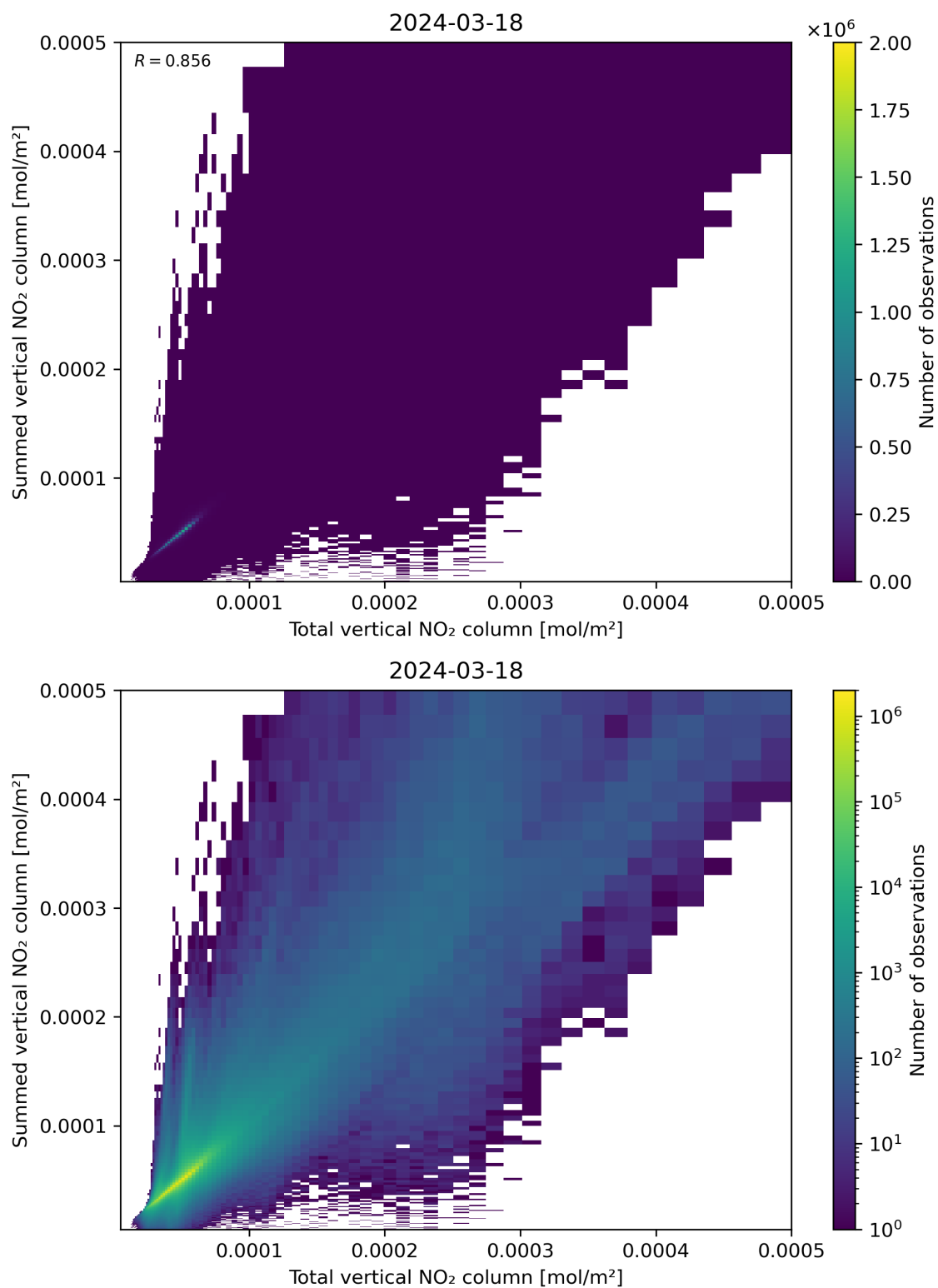
Figure 112: Scatter density plot of “Total vertical NO 2 column” against “Summed vertical NO 2 column” for 2024-03-17 to 2024-03-19.
