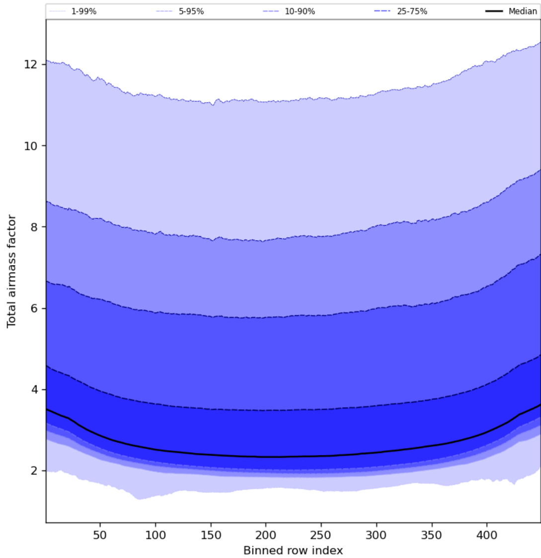
Figure 49: Along track statistics of “Total airmass factor” for 2024-03-17 to 2024-03-19
