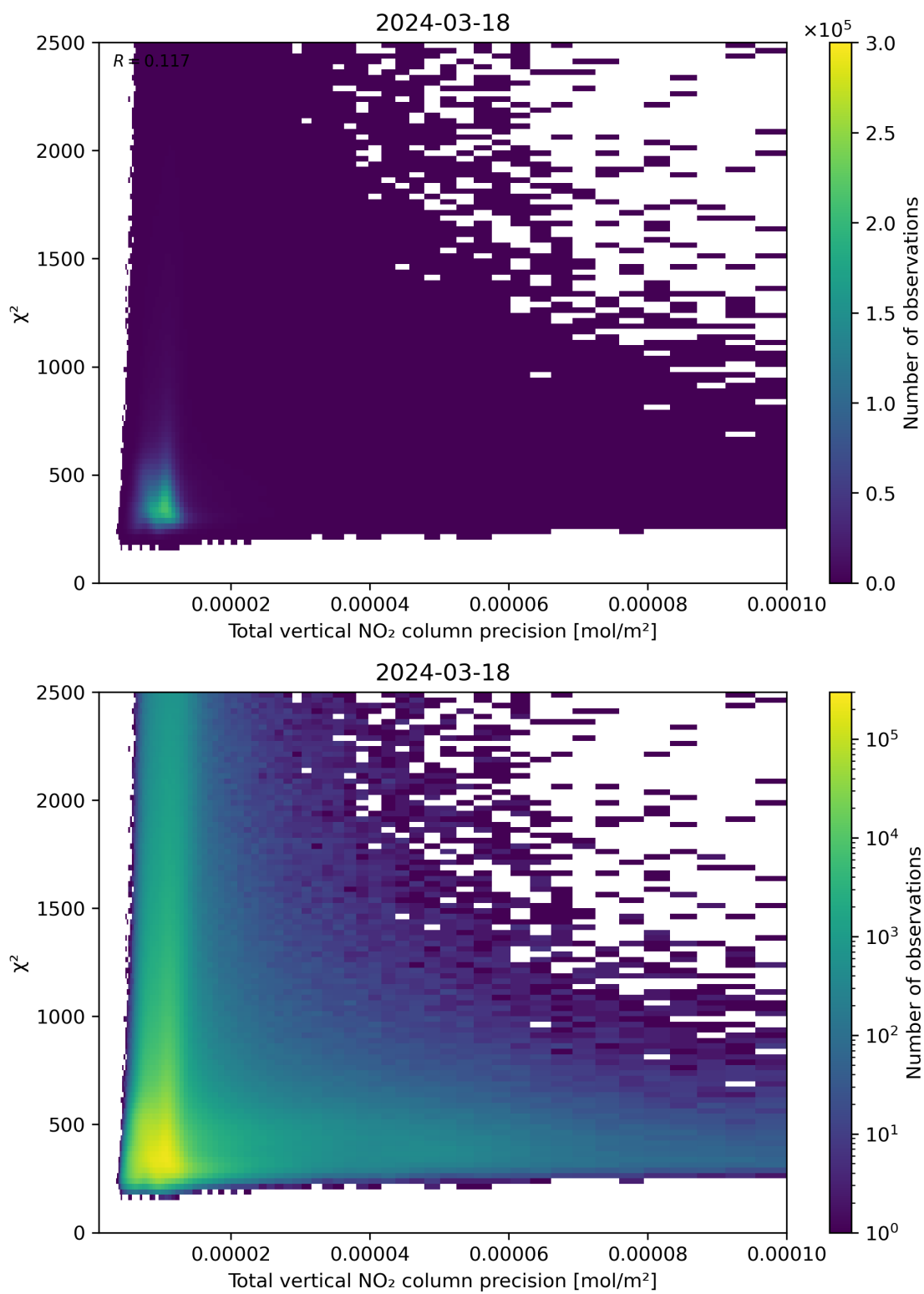
Figure 116: Scatter density plot of “Total vertical NO 2 column precision” against “ \chi^2 ” for 2024-03-17 to 2024-03-19.
