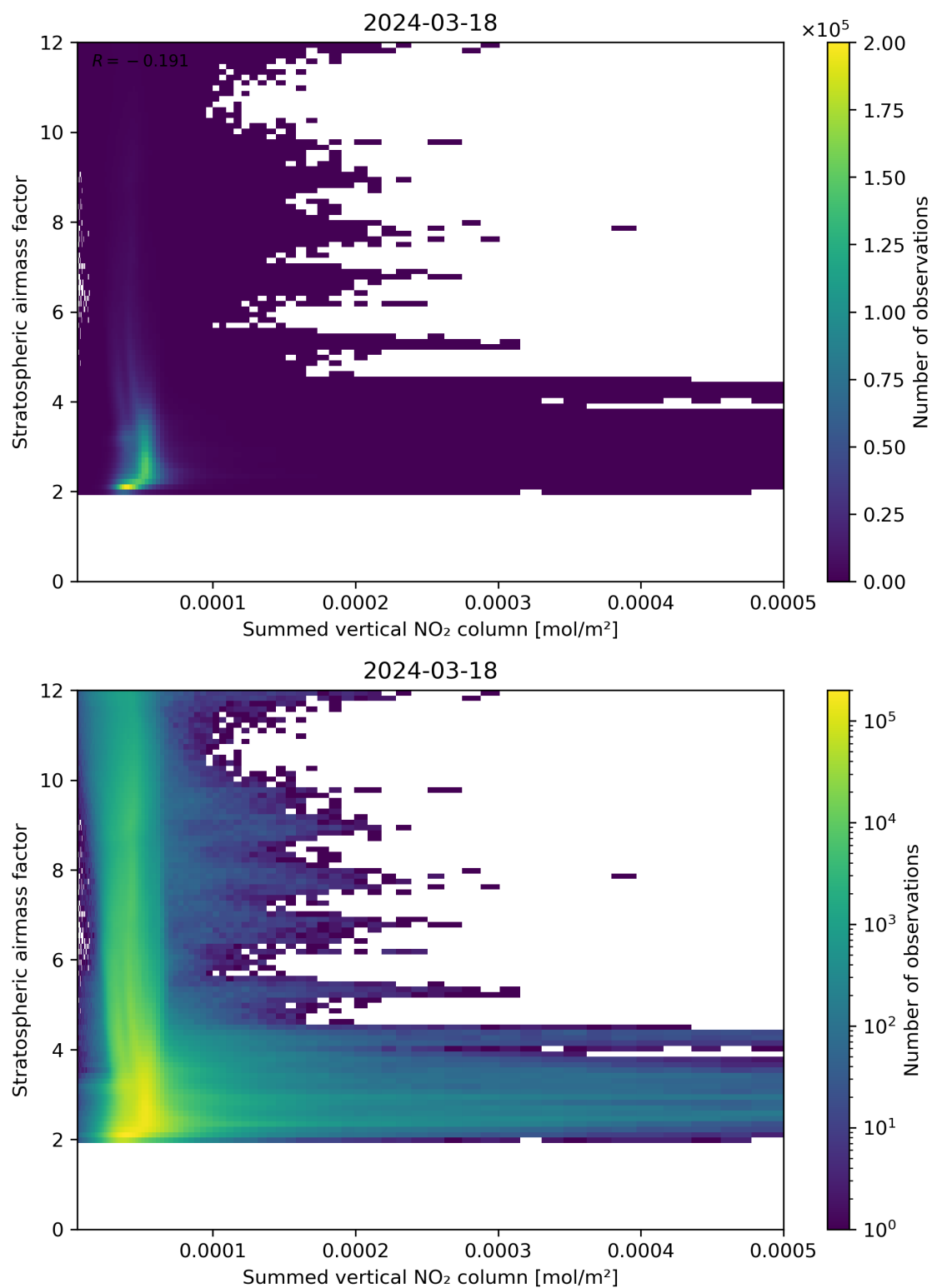
Figure 103: Scatter density plot of “Summed vertical NO 2 column” against “Stratospheric airmass factor” for 2024-03-17 to 2024-03-19.
