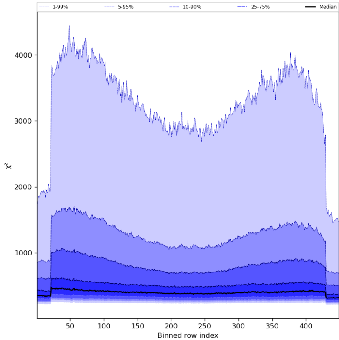
Figure 59: Along track statistics of “ \chi^2 ” for 2024-03-17 to 2024-03-19
