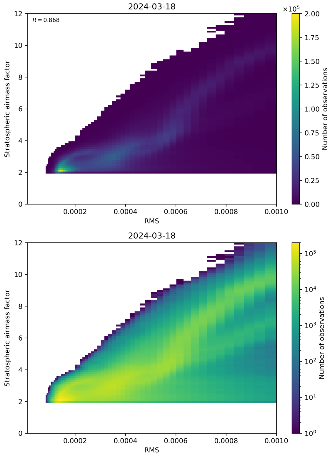
Figure 144: Scatter density plot of “RMS” against “Stratospheric airmass factor” for 2024-03-17 to 2024-03-19.
