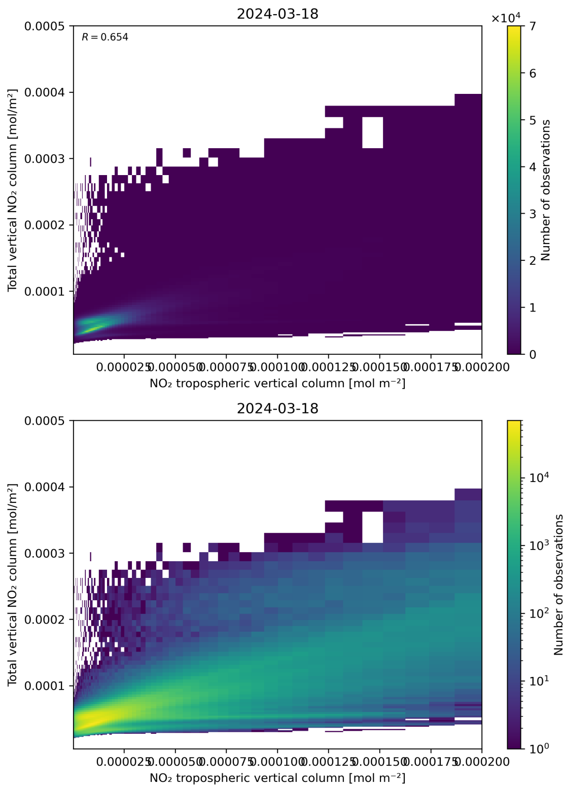
Figure 128: Scatter density plot of “NO 2 tropospheric vertical column” against “Total vertical NO 2 column” for 2024-03-17 to 2024-03-19.
