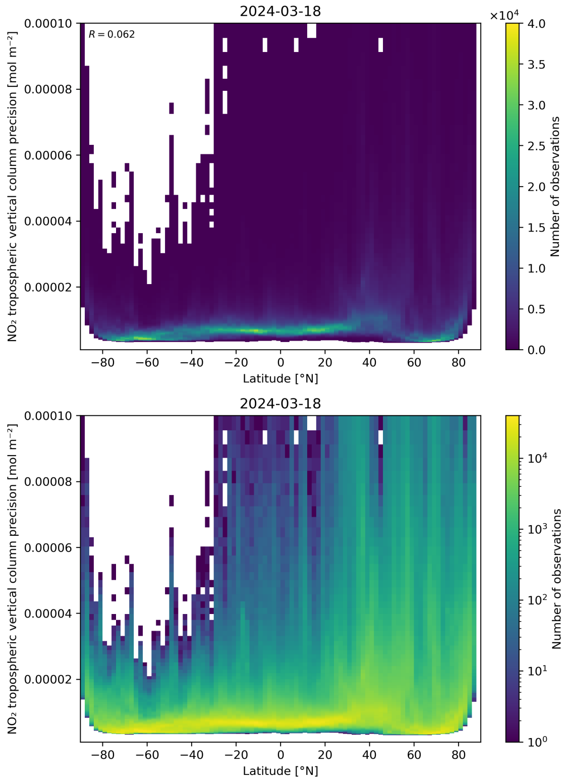
Figure 93: Scatter density plot of “Latitude” against “NO 2 tropospheric vertical column precision” for 2024-03-17 to 2024-03-19.
