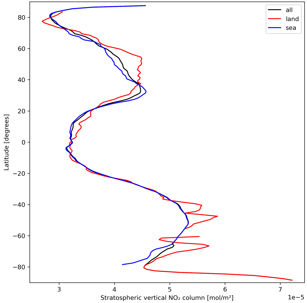
Figure 19: Zonal average of “Stratospheric vertical NO 2 column” for 2024-03-17 to 2024-03-19.
