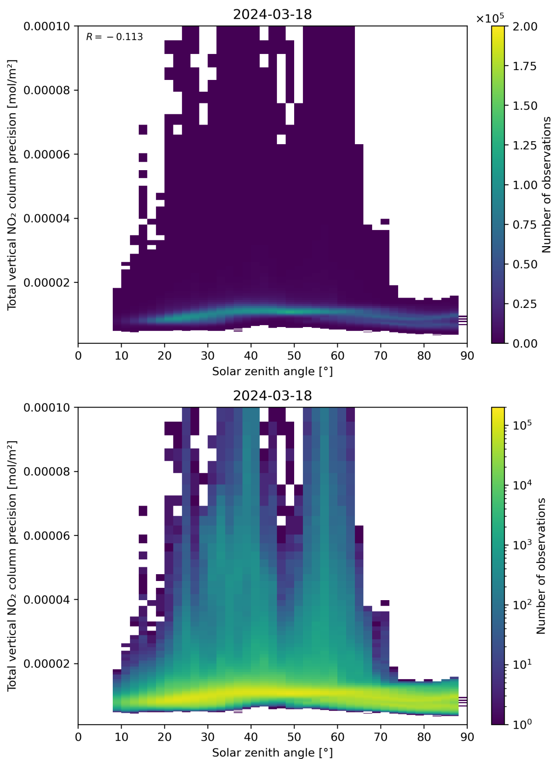
Figure 154: Scatter density plot of “Solar zenith angle” against “Total vertical NO 2 column precision” for 2024-03-17 to 2024-03-19.
