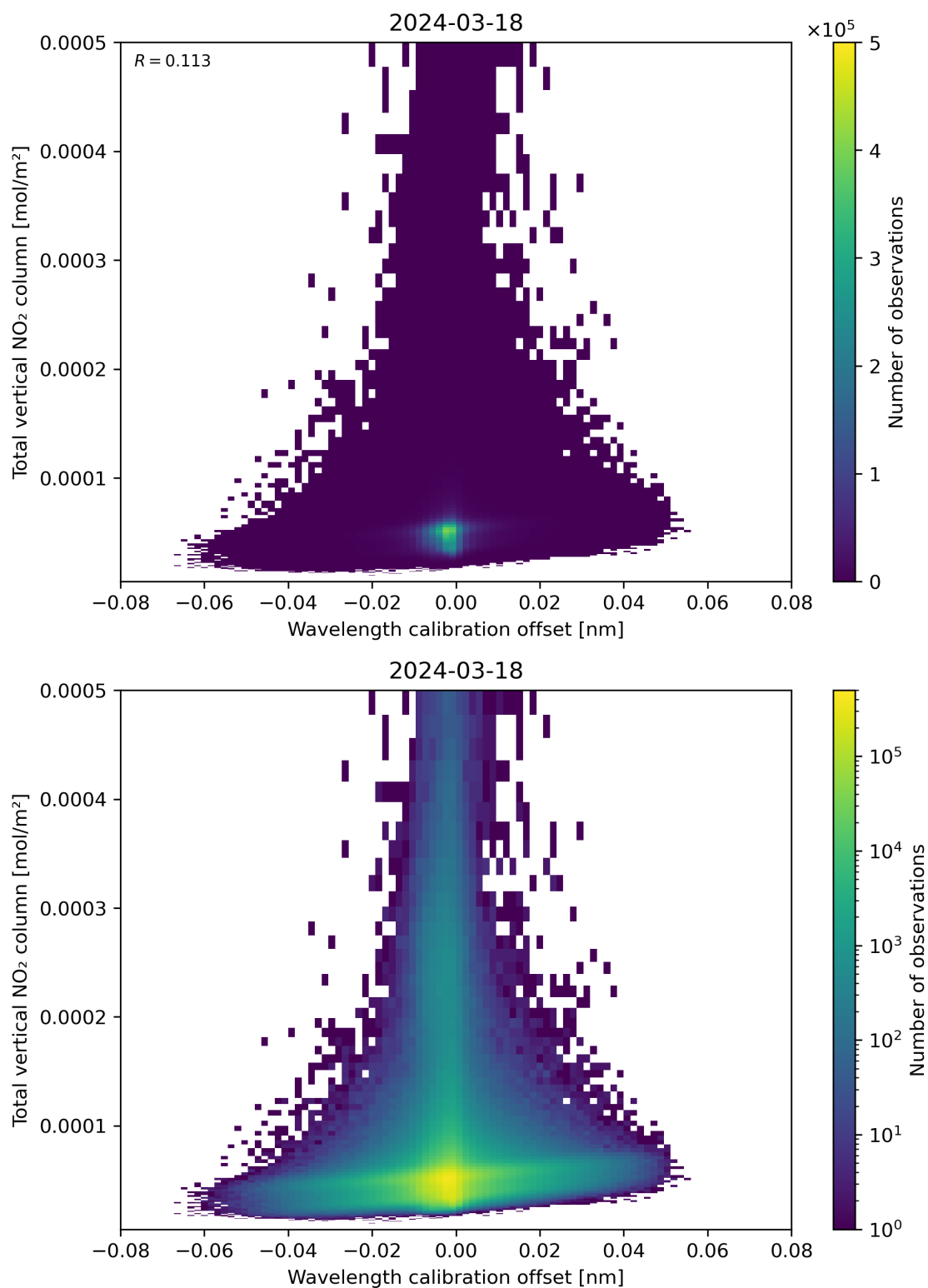
Figure 179: Scatter density plot of “Wavelength calibration offset” against “Total vertical NO 2 column” for 2024-03-17 to 2024-03-19.
