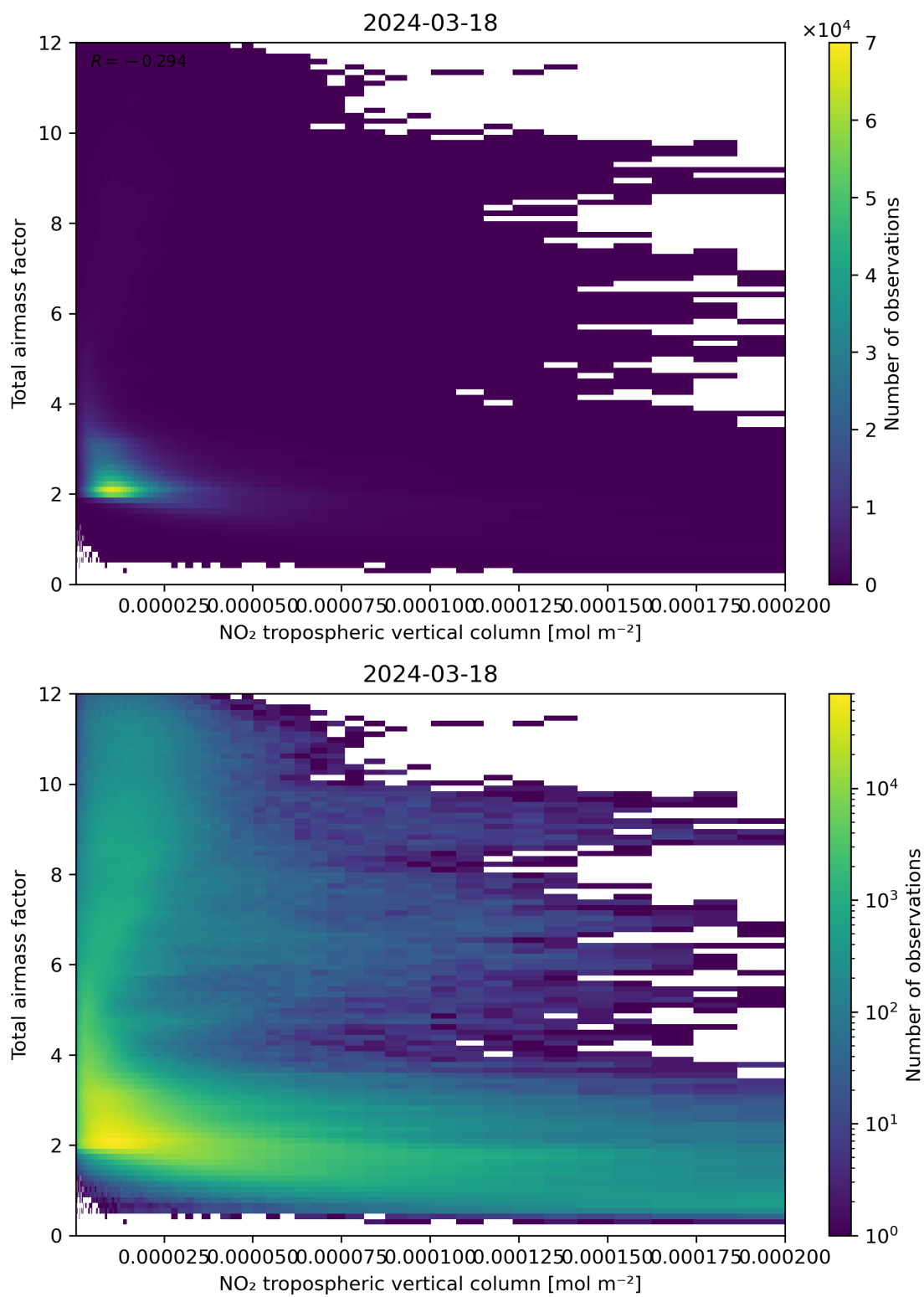
Figure 122: Scatter density plot of “NO 2 tropospheric vertical column” against “Total air mass factor” for 2024-03-17 to 2024-03-19.
