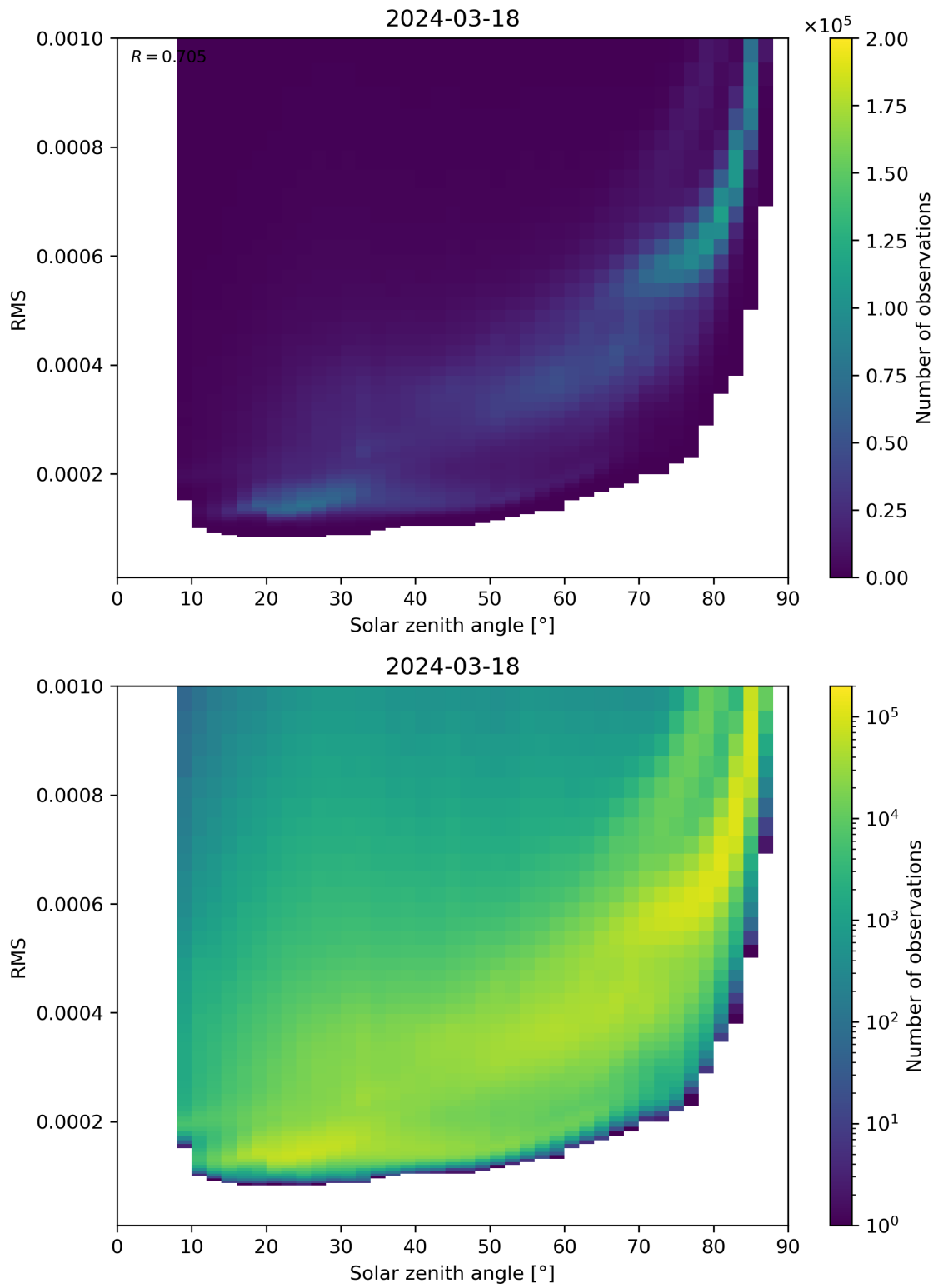
Figure 157: Scatter density plot of “Solar zenith angle” against “RMS” for 2024-03-17 to 2024-03-19.
