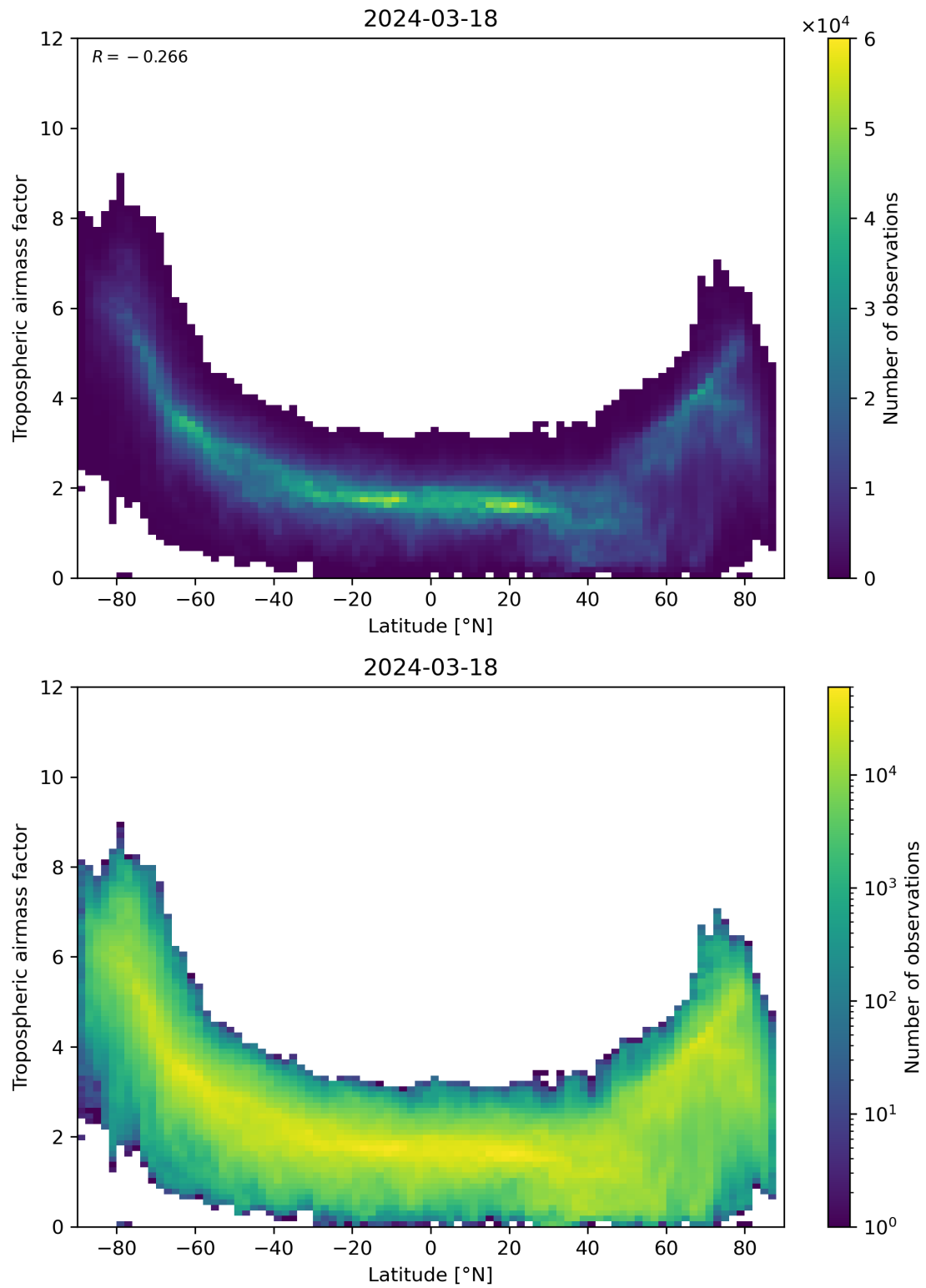
Figure 85: Scatter density plot of “Latitude” against “Tropospheric airmass factor” for 2024-03-17 to 2024-03-19.
