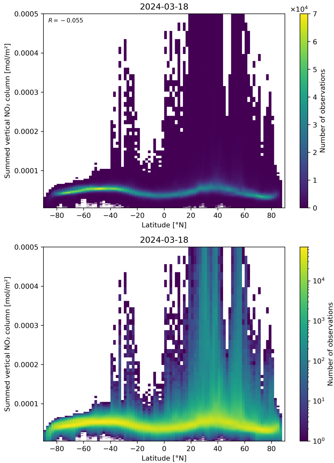
Figure 88: Scatter density plot of “Latitude” against “Summed vertical NO 2 column” for 2024-03-17 to 2024-03-19.
