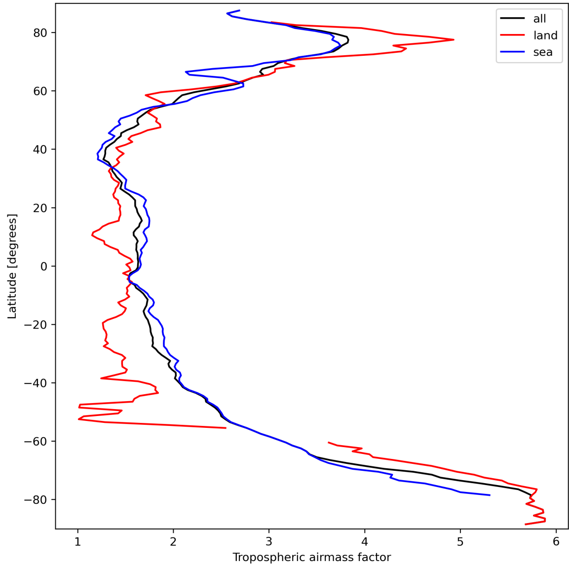
Figure 14: Zonal average of “Tropospheric airmass factor” for 2024-03-17 to 2024-03-19.
