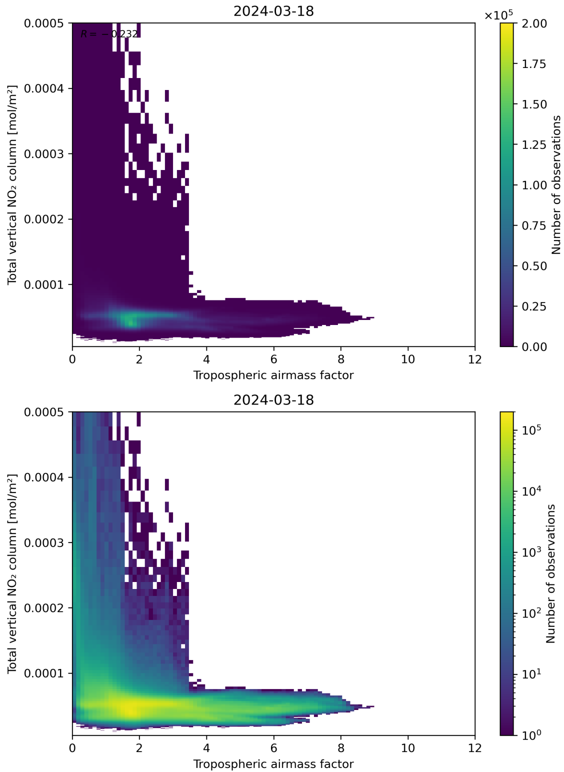
Figure 77: Scatter density plot of “Tropospheric airmass factor” against “Total vertical NO 2 column” for 2024-03-17 to 2024-03-19.
