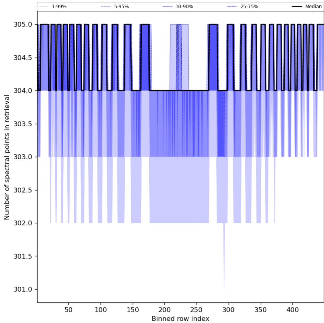
Figure 50: Along track statistics of “Number of spectral points in retrieval” for 2024-03-17 to 2024-03-19
