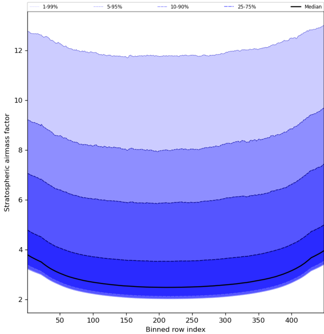
Figure 61: Along track statistics of “Stratospheric airmass factor” for 2024-03-17 to 2024-03-19
