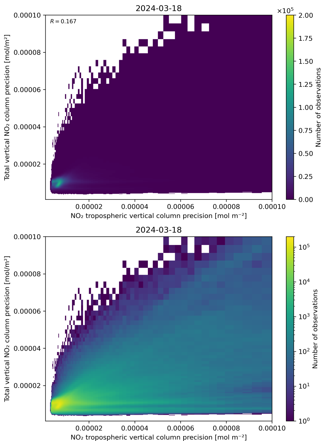
Figure 139: Scatter density plot of “NO 2 tropospheric vertical column precision” against “Total vertical NO 2 column precision” for 2024-03-17 to 2024-03-19.
