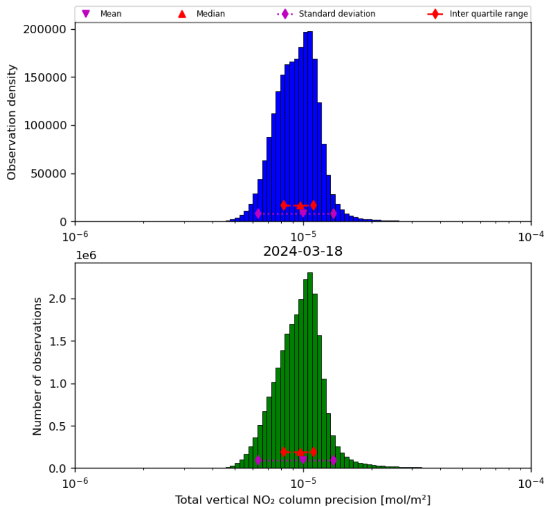
Figure 39: Histogram of “Total vertical NO 2 column precision” for 2024-03-17 to 2024-03-19
