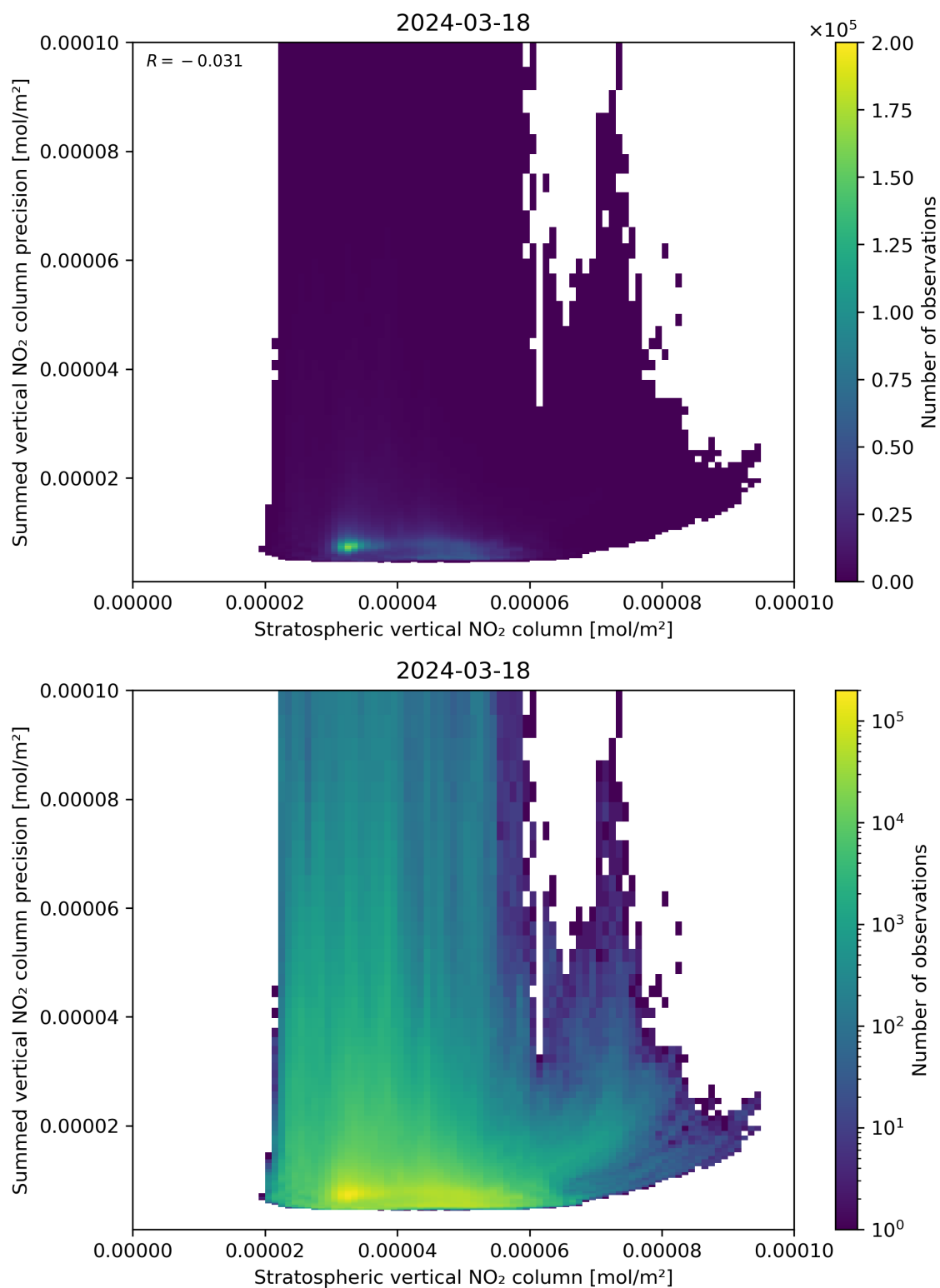
Figure 99: Scatter density plot of “Stratospheric vertical NO 2 column” against “Summed vertical NO 2 column precision” for 2024-03-17 to 2024-03-19.
