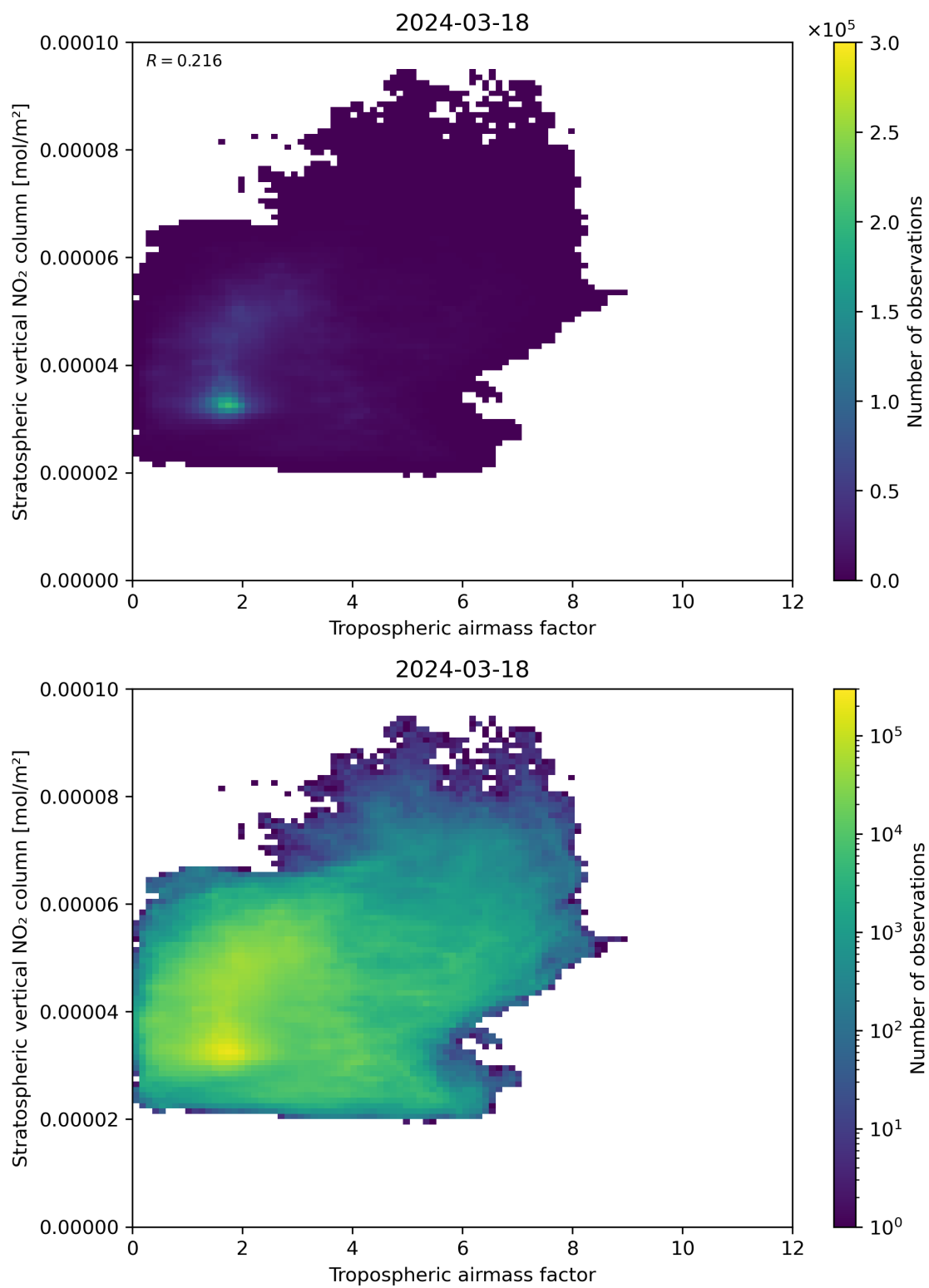
Figure 74: Scatter density plot of “Tropospheric air mass factor” against “Stratospheric vertical NO 2 column” for 2024-03-17 to 2024-03-19.
