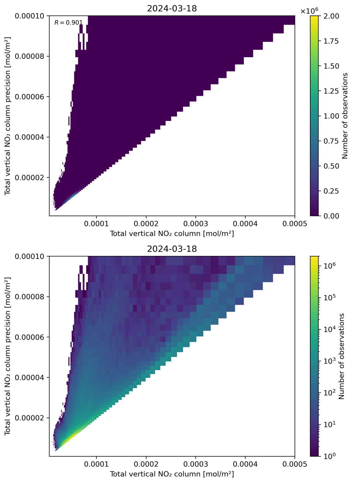
Figure 114: Scatter density plot of “Total vertical NO 2 column” against “Total vertical NO 2 column precision” for 2024-03-17 to 2024-03-19.
