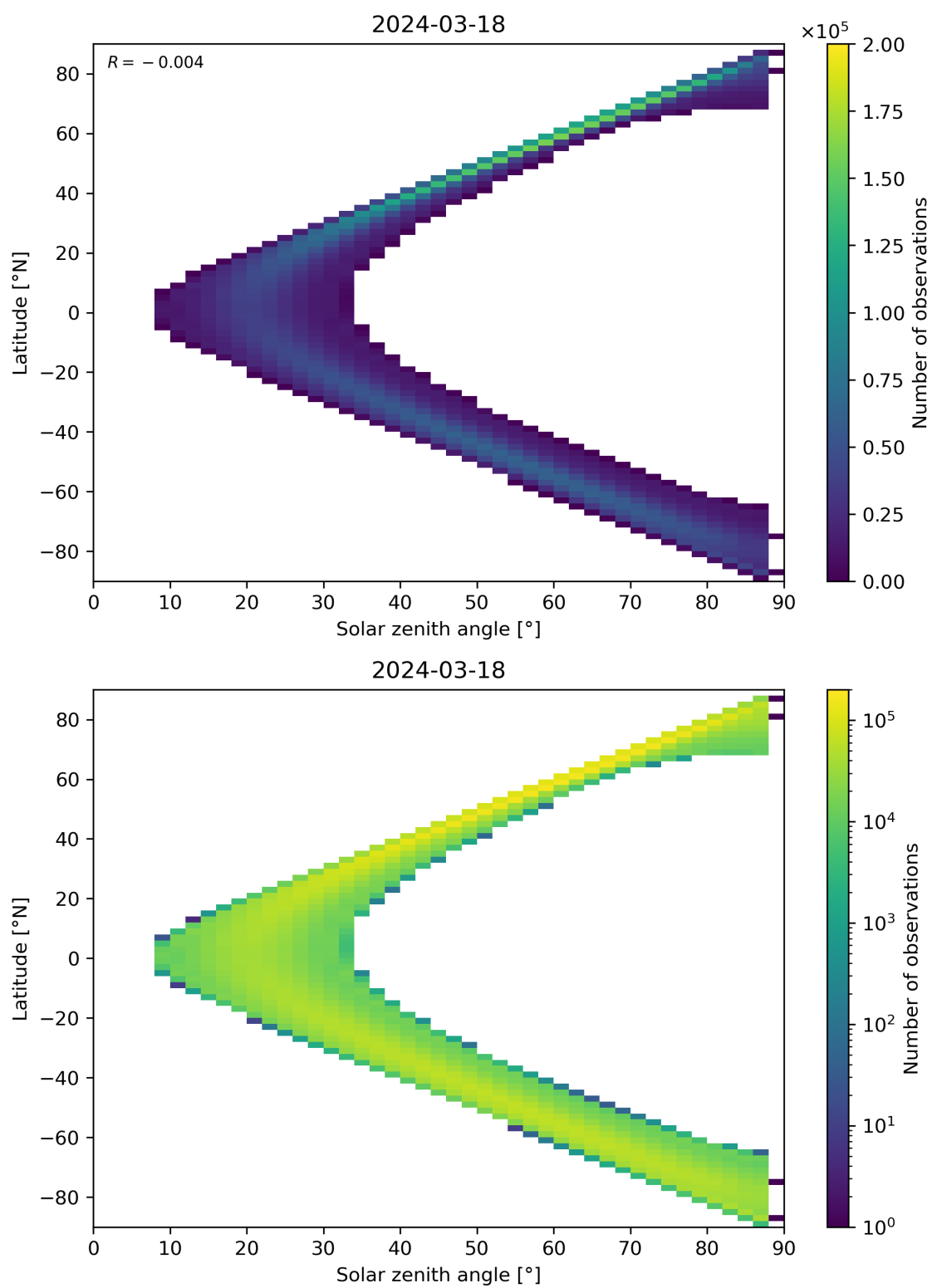
Figure 149: Scatter density plot of “Solar zenith angle” against “Latitude” for 2024-03-17 to 2024-03-19.
