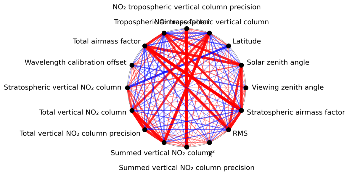
Figure 1: Map of correlation graph for 2024-03-17 to 2024-03-19.
