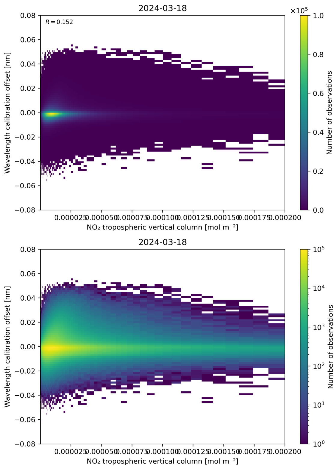
Figure 143: Scatter density plot of “NO 2 tropospheric vertical column” against “Wavelength calibration offset” for 2024-03-17 to 2024-03-19.
