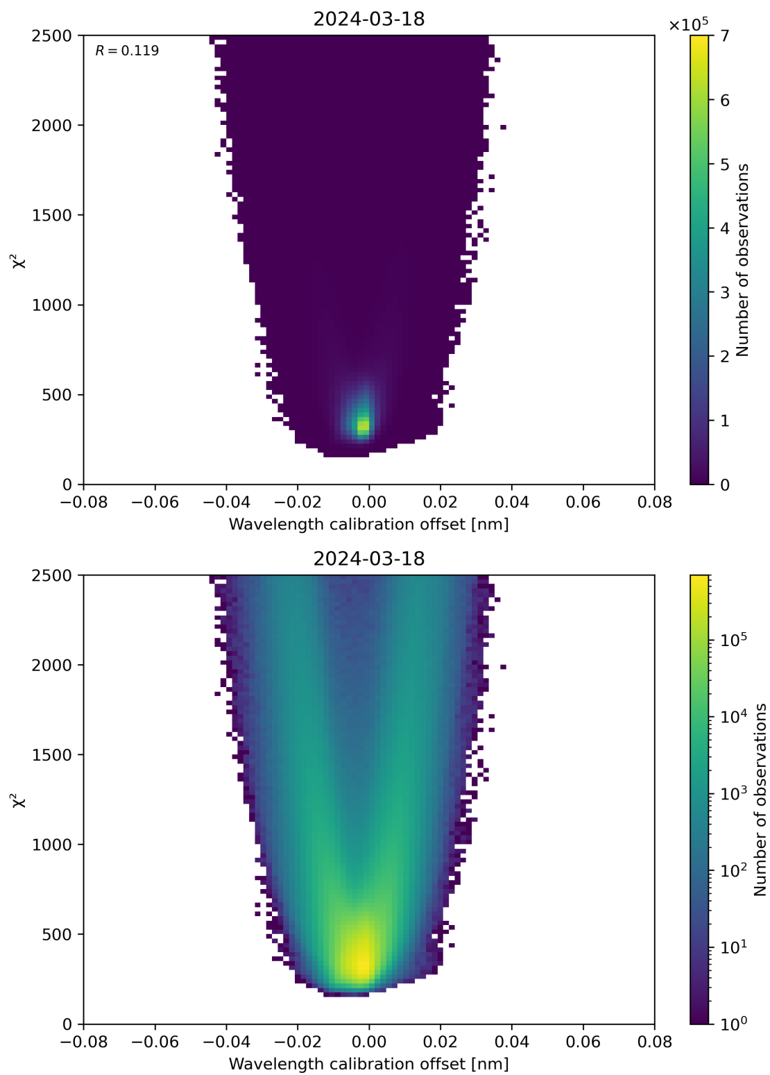
Figure 175: Scatter density plot of “Wavelength calibration offset” against “ \chi^2 ” for 2024-03-17 to 2024-03-19.
