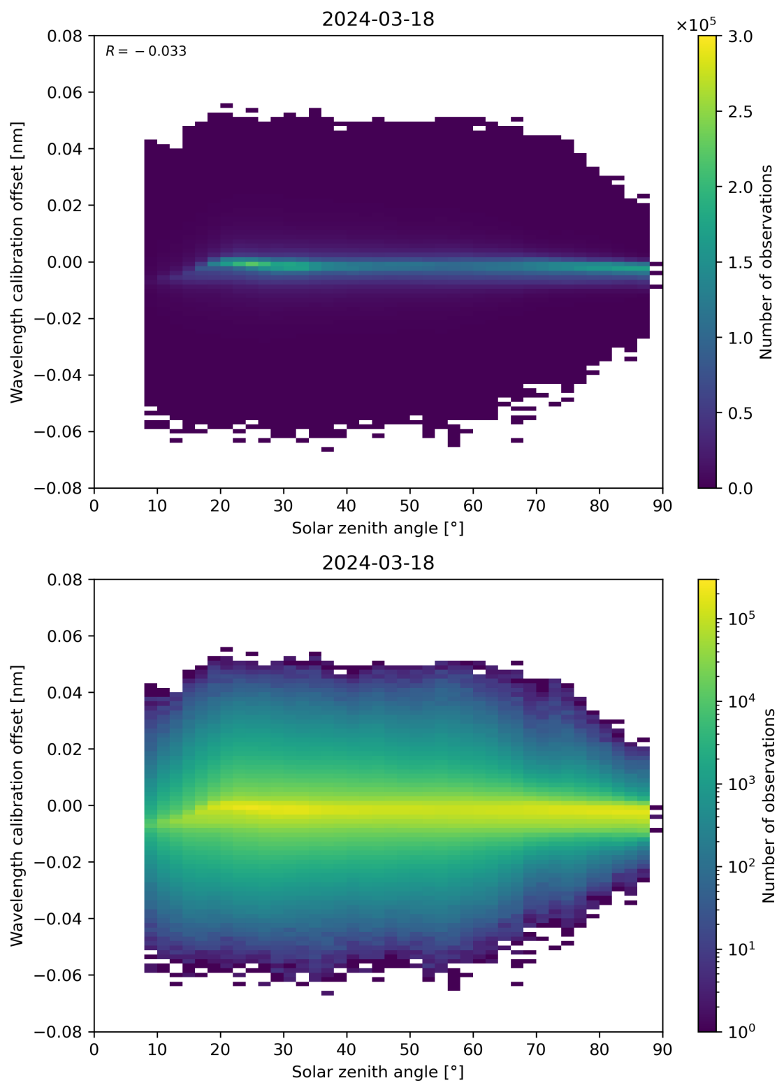
Figure 158: Scatter density plot of “Solar zenith angle” against “Wavelength calibration offset” for 2024-03-17 to 2024-03-19.
