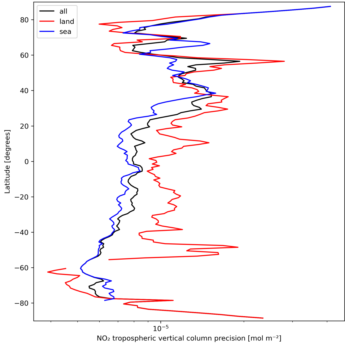
Figure 13: Zonal average of “NO 2 tropospheric vertical column precision” for 2024-03-17 to 2024-03-19.
