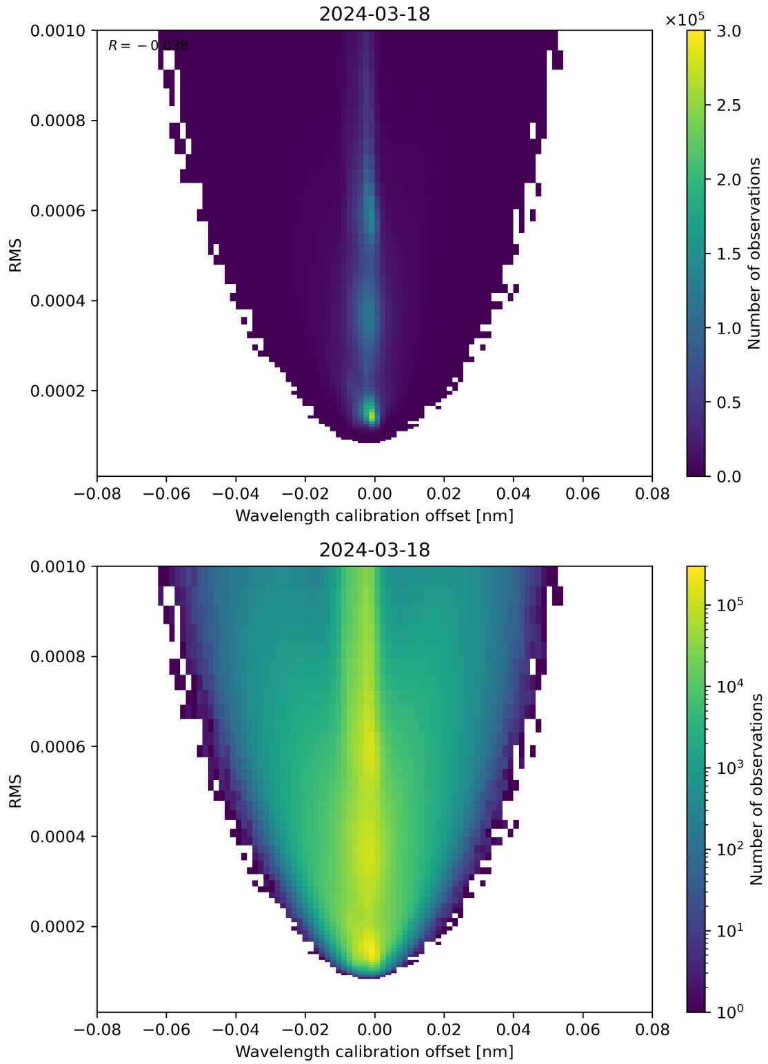
Figure 181: Scatter density plot of “Wavelength calibration offset” against “RMS” for 2024-03-17 to 2024-03-19.
