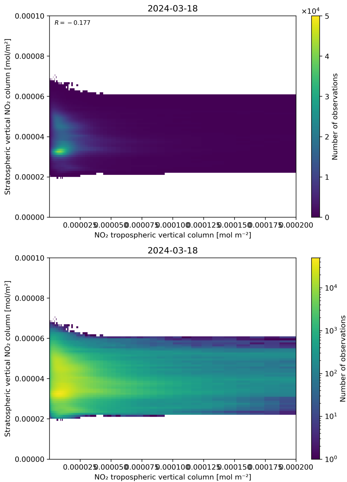
Figure 125: Scatter density plot of “NO 2 tropospheric vertical column” against “Stratospheric vertical NO 2 column” for 2024-03-17 to 2024-03-19.
