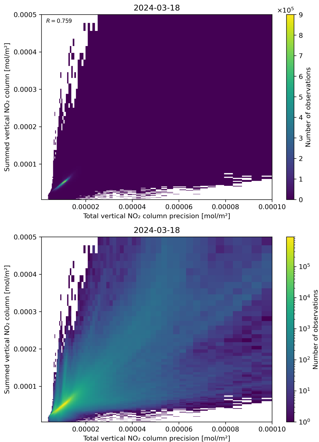
Figure 117: Scatter density plot of “Total vertical NO 2 column precision” against “Summed vertical NO 2 column” for 2024-03-17 to 2024-03-19.
