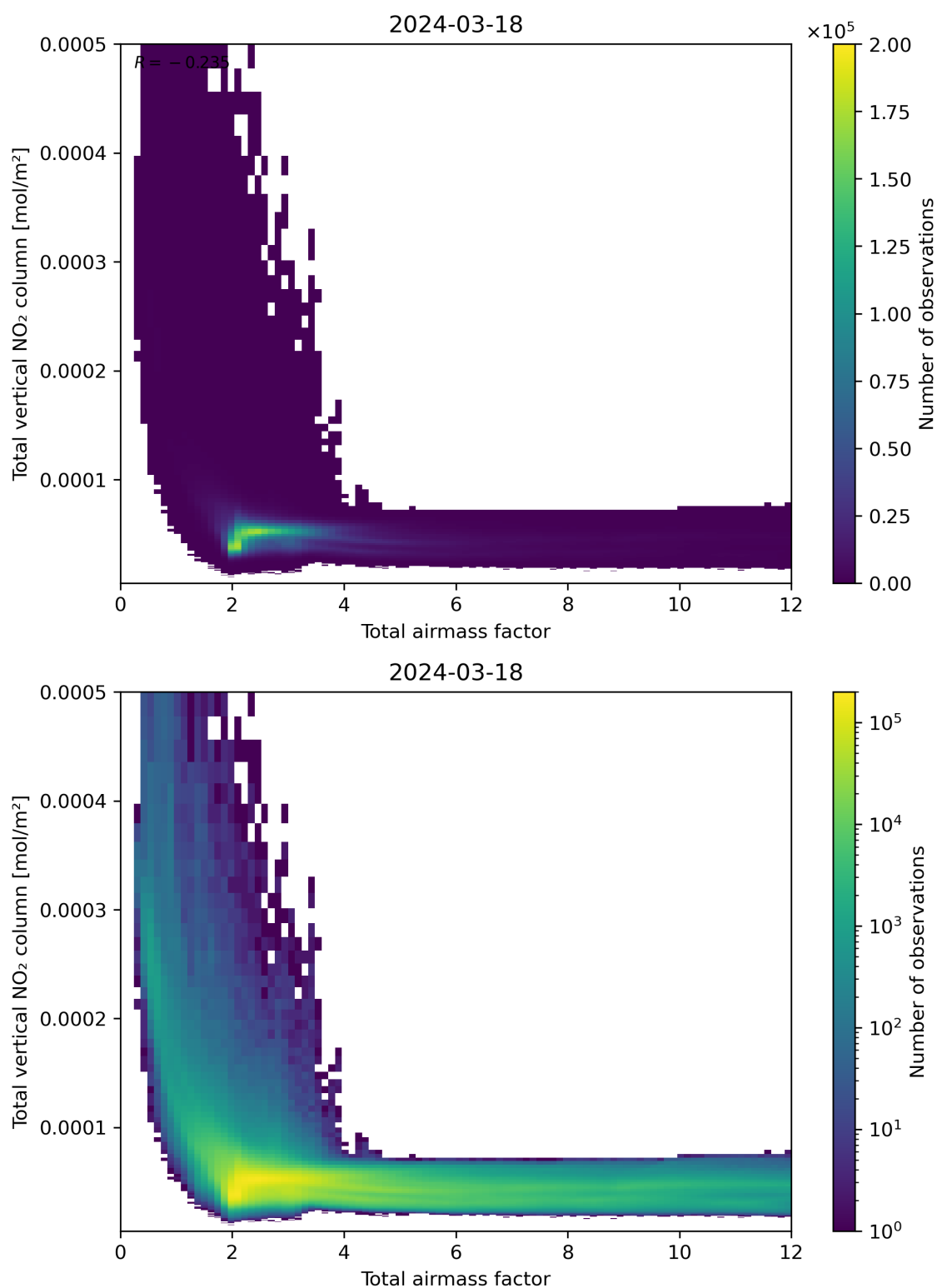
Figure 67: Scatter density plot of “Total airmass factor” against “Total vertical NO 2 column” for 2024-03-17 to 2024-03-19.
