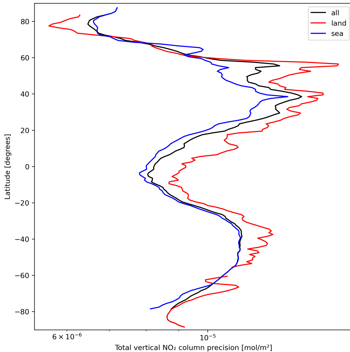
Figure 22: Zonal average of “Total vertical NO 2 column precision” for 2024-03-17 to 2024-03-19.
