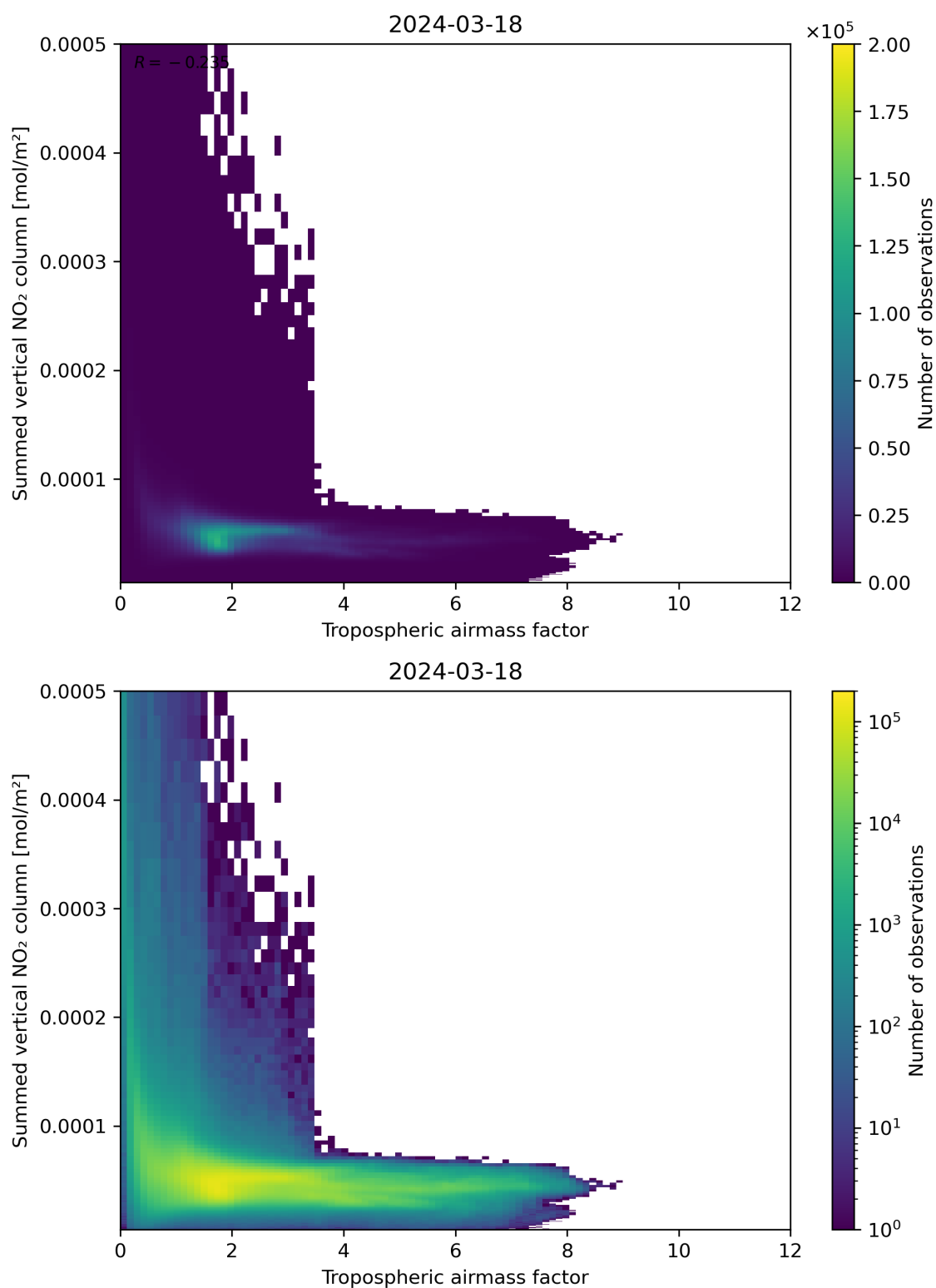
Figure 75: Scatter density plot of “Tropospheric airmass factor” against “Summed vertical NO 2 column” for 2024-03-17 to 2024-03-19.
