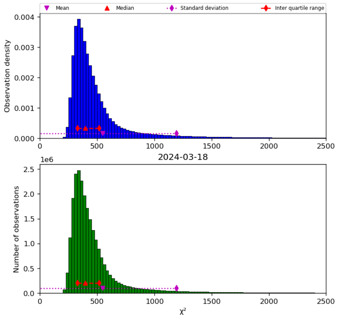
Figure 42: Histogram of “ \chi^2 ” for 2024-03-17 to 2024-03-19
