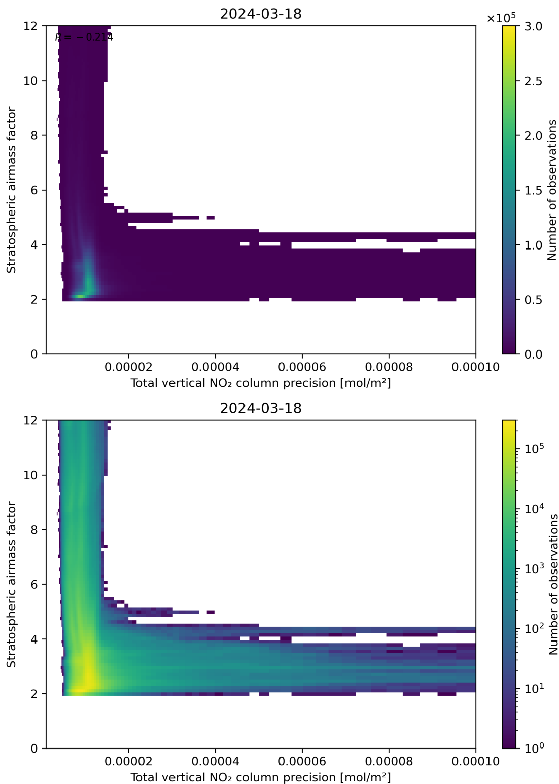
Figure 115: Scatter density plot of “Total vertical NO 2 column precision” against “Stratospheric air mass factor” for 2024-03-17 to 2024-03-19.
