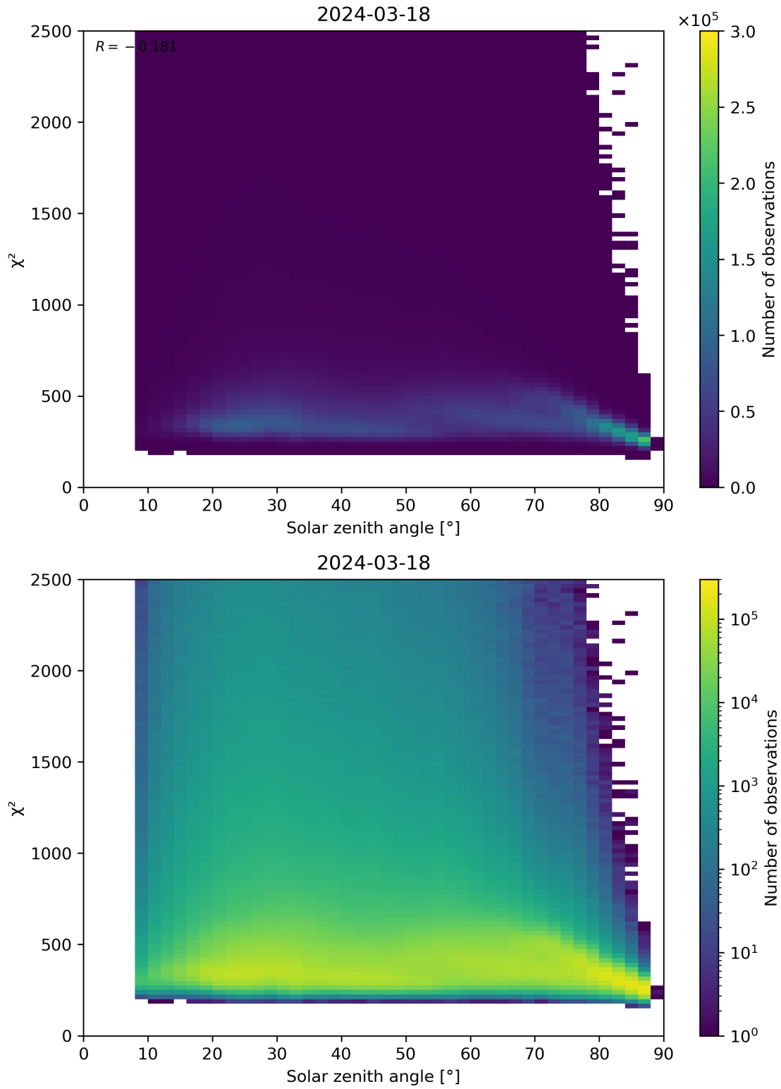
Figure 148: Scatter density plot of “Solar zenith angle” against “ \chi^2 ” for 2024-03-17 to 2024-03-19.
