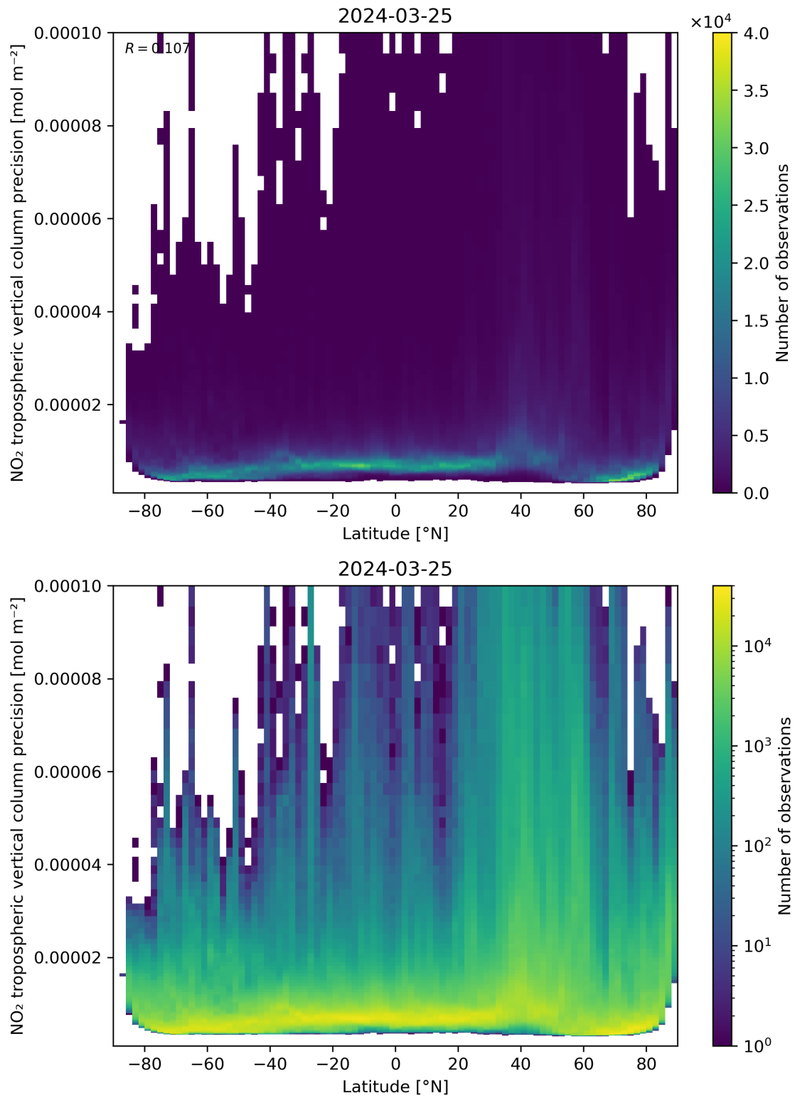
Figure 93: Scatter density plot of “Latitude” against “NO 2 tropospheric vertical column precision” for 2024-03-25 to 2024-03-26.
