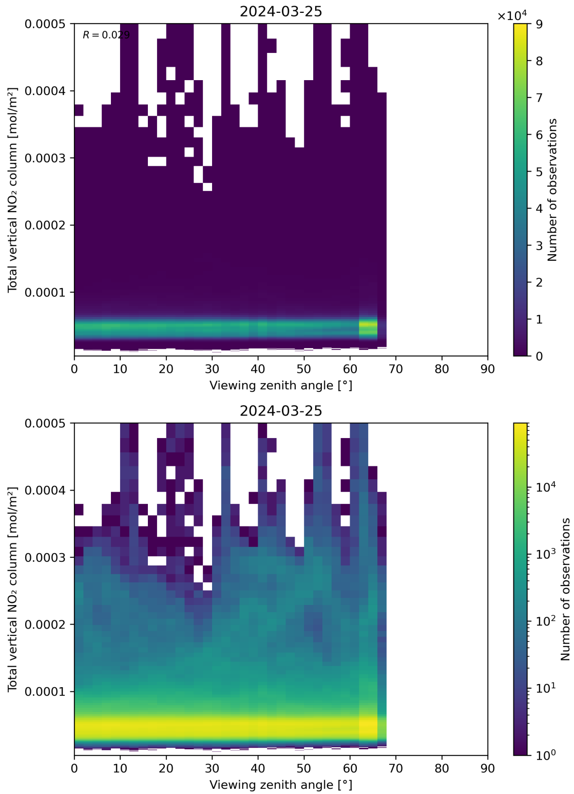
Figure 167: Scatter density plot of “Viewing zenith angle” against “Total vertical NO 2 column” for 2024-03-25 to 2024-03-26.
