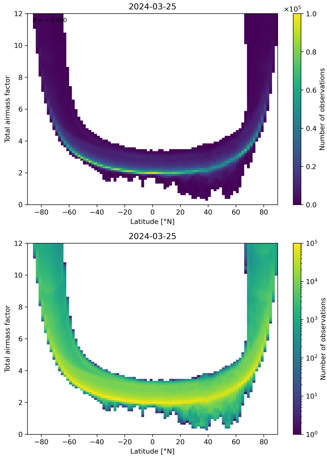
Figure 84: Scatter density plot of “Latitude” against “Total airmass factor” for 2024-03-25 to 2024-03-26.
