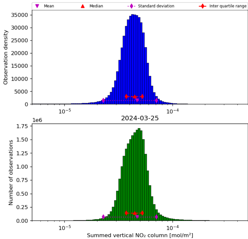
Figure 40: Histogram of “Summed vertical NO 2 column” for 2024-03-25 to 2024-03-26
