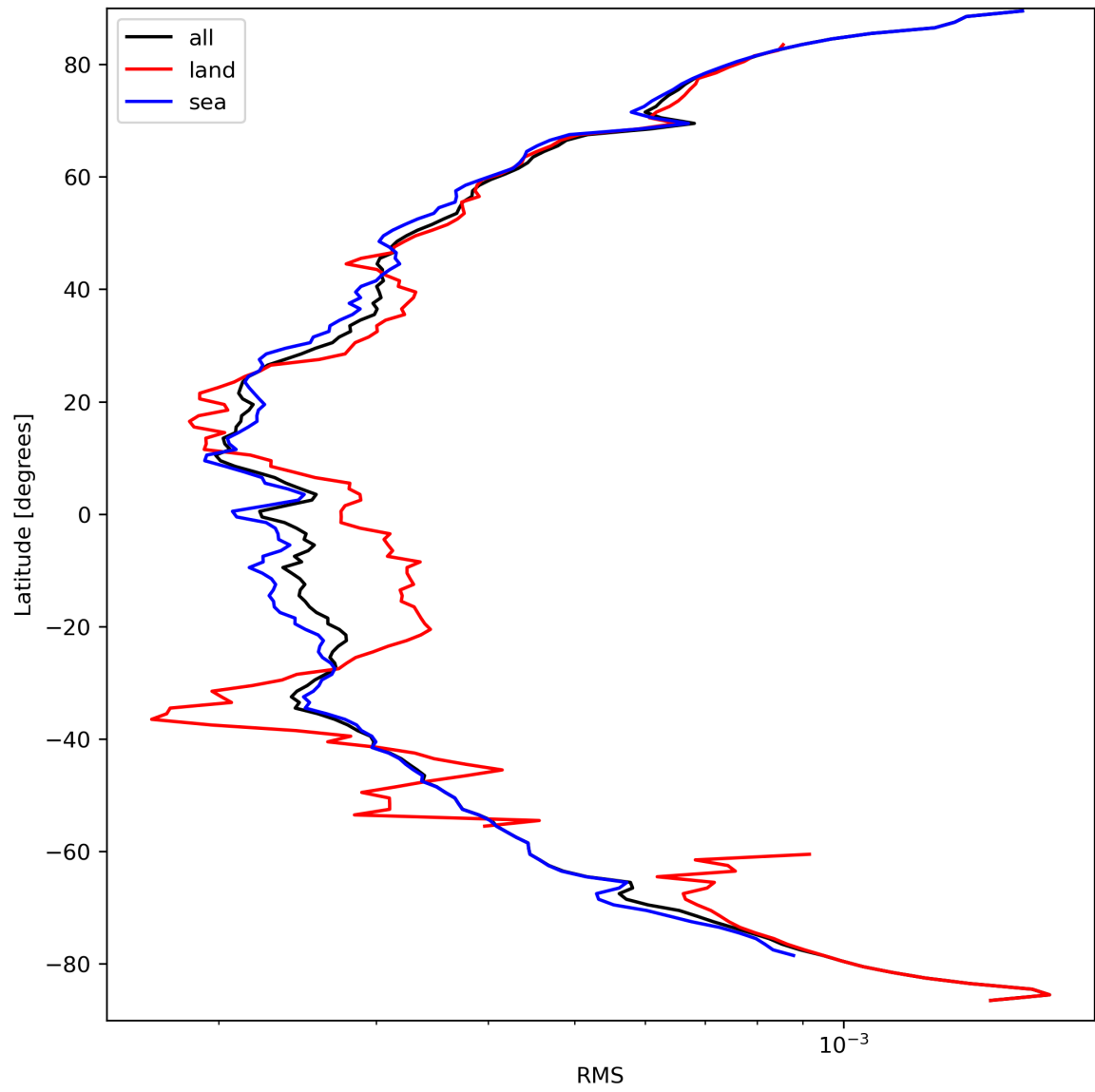
Figure 26: Zonal average of “RMS” for 2024-03-25 to 2024-03-26.
