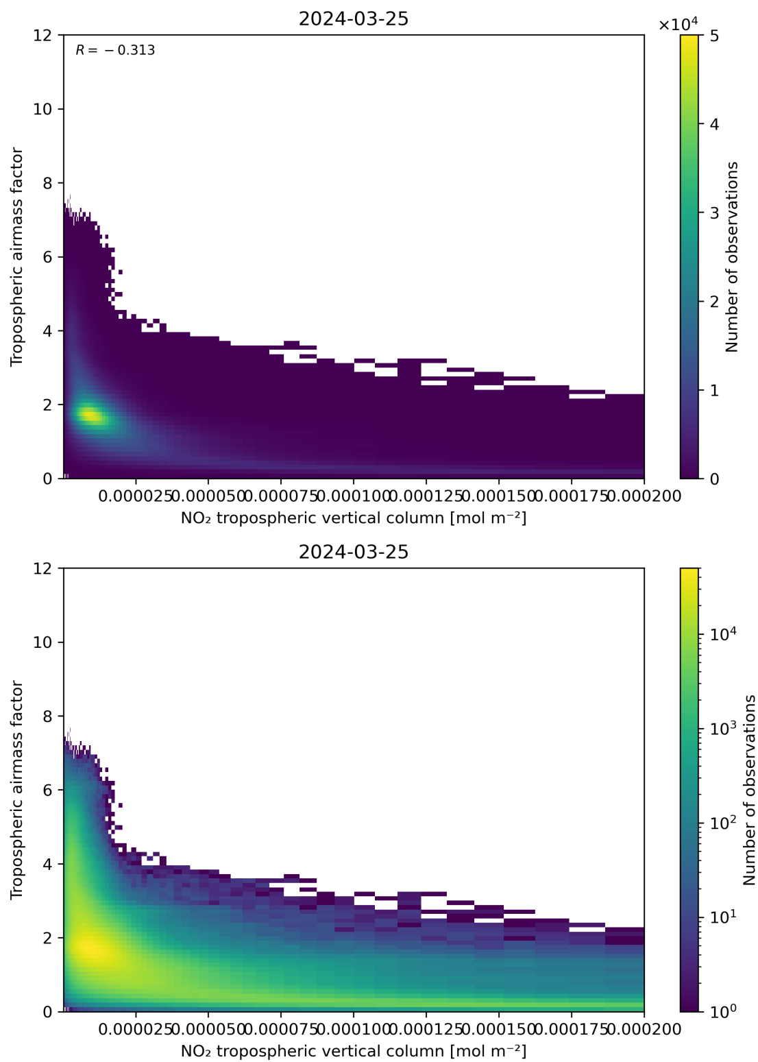
Figure 123: Scatter density plot of “NO 2 tropospheric vertical column” against “Tropospheric air mass factor” for 2024-03-25 to 2024-03-26.
