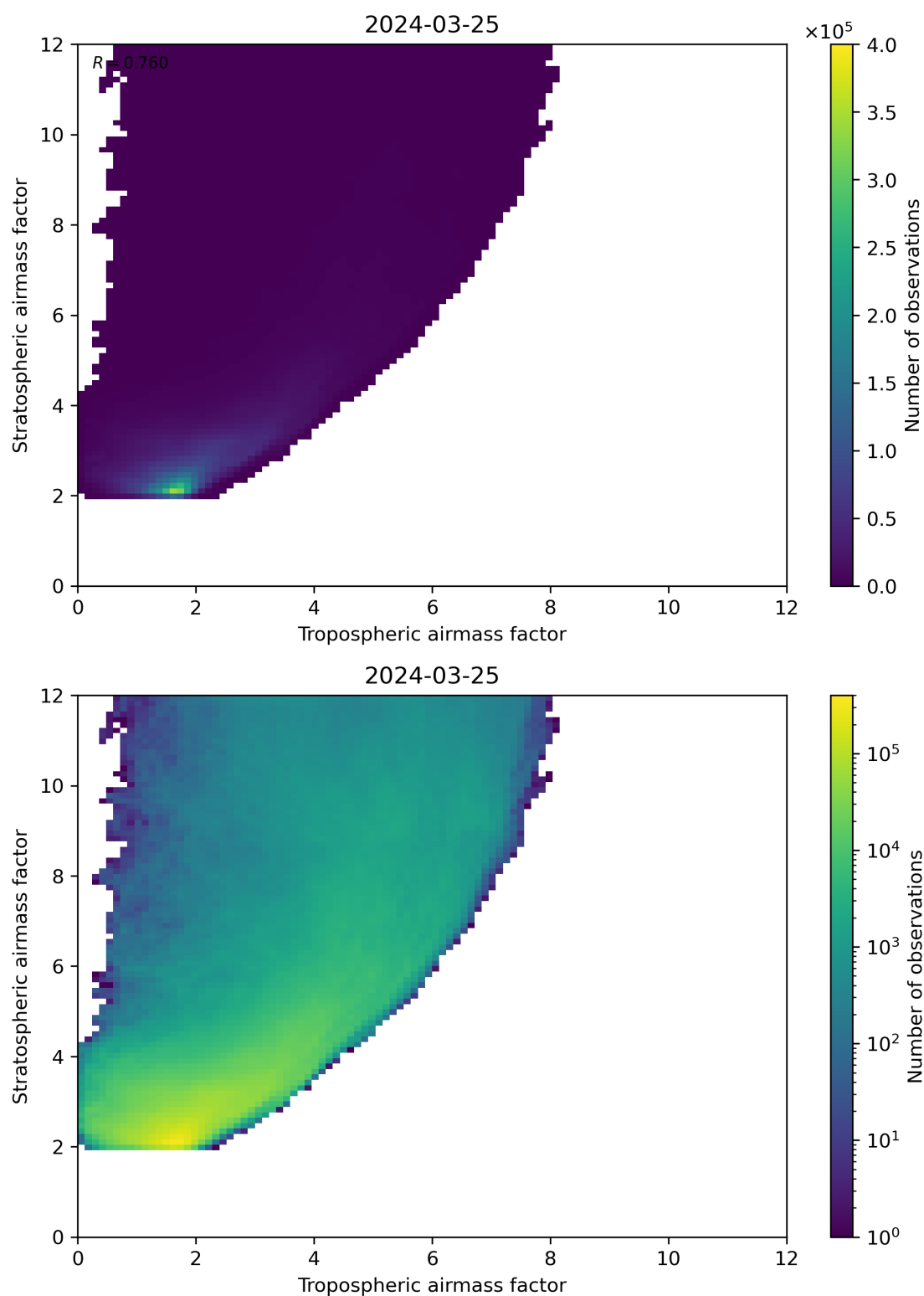
Figure 71: Scatter density plot of “Tropospheric airmass factor” against “Stratospheric airmass factor” for 2024-03-25 to 2024-03-26.
