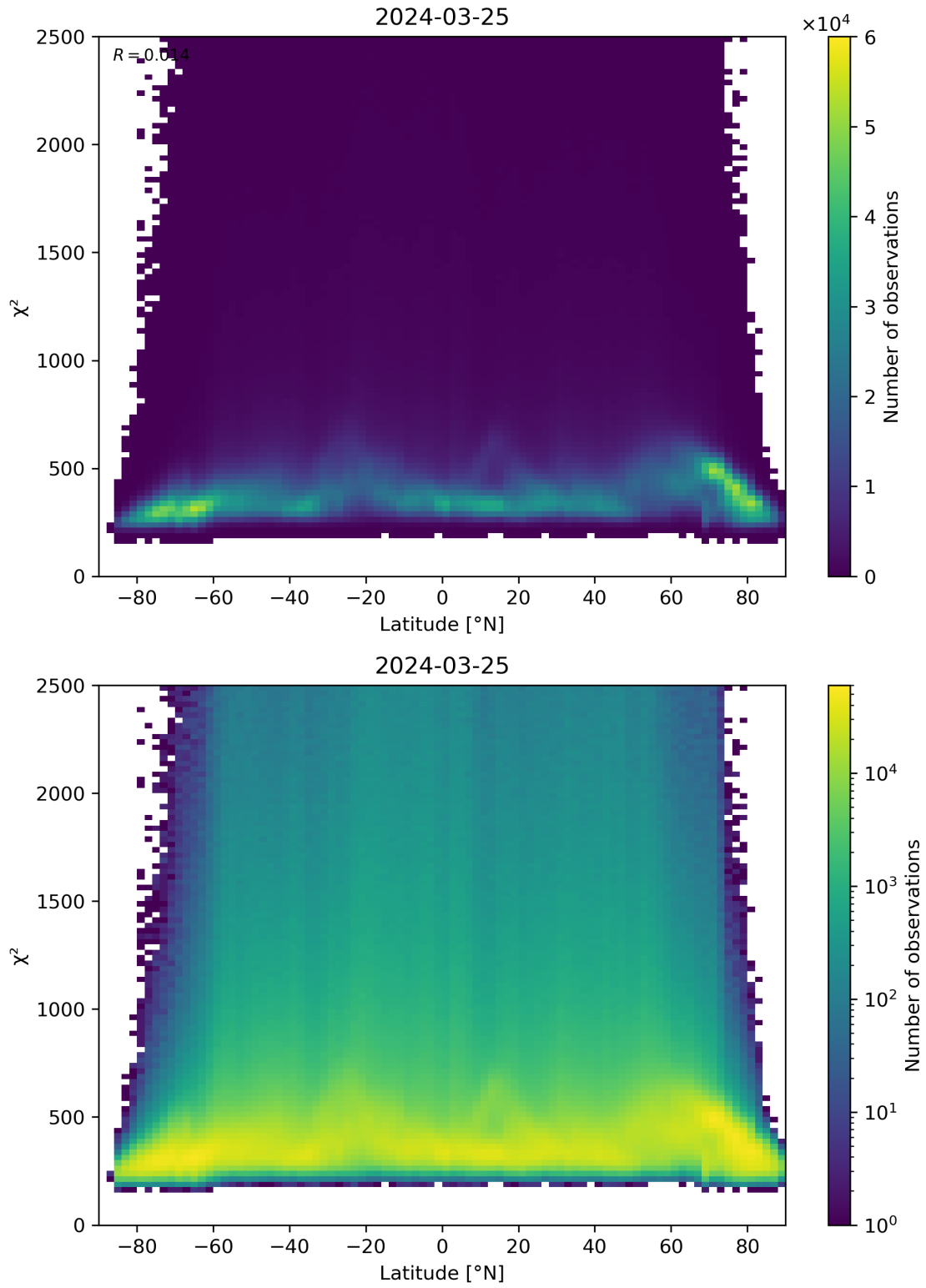
Figure 86: Scatter density plot of “Latitude” against “ \chi^2 ” for 2024-03-25 to 2024-03-26.
