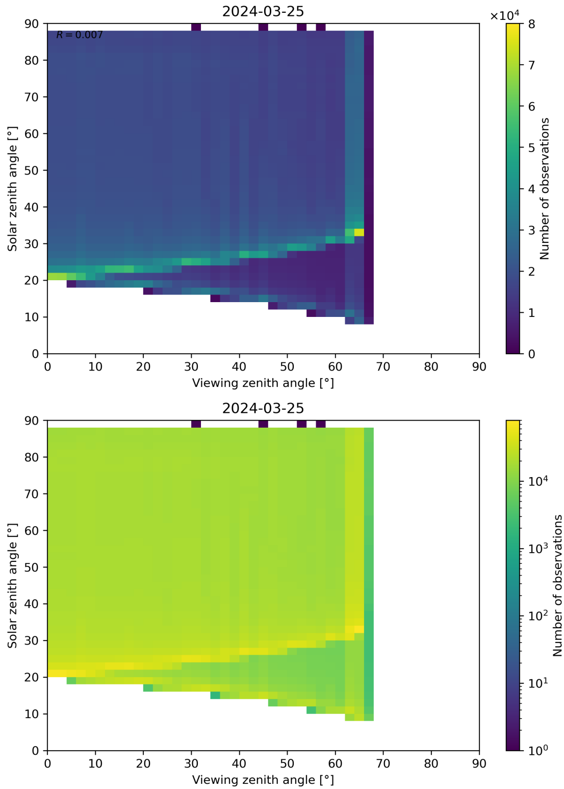
Figure 172: Scatter density plot of “Viewing zenith angle” against “Solar zenith angle” for 2024-03-25 to 2024-03-26.
