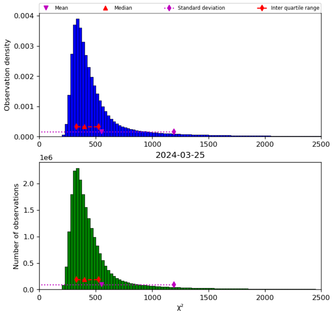
Figure 42: Histogram of " \chi^2 " for 2024-03-25 to 2024-03-26
