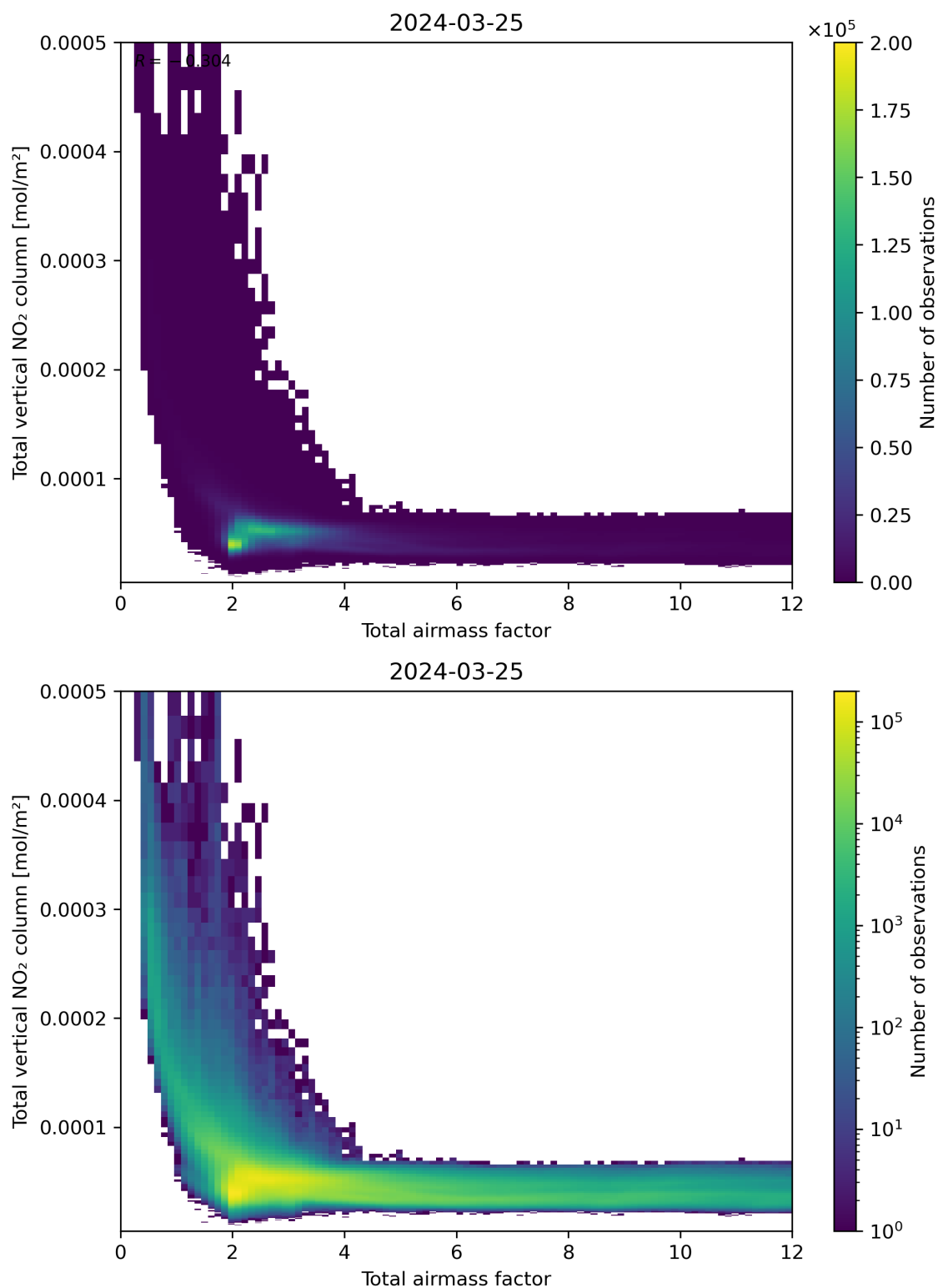
Figure 67: Scatter density plot of “Total airmass factor” against “Total vertical NO 2 column” for 2024-03-25 to 2024-03-26.
