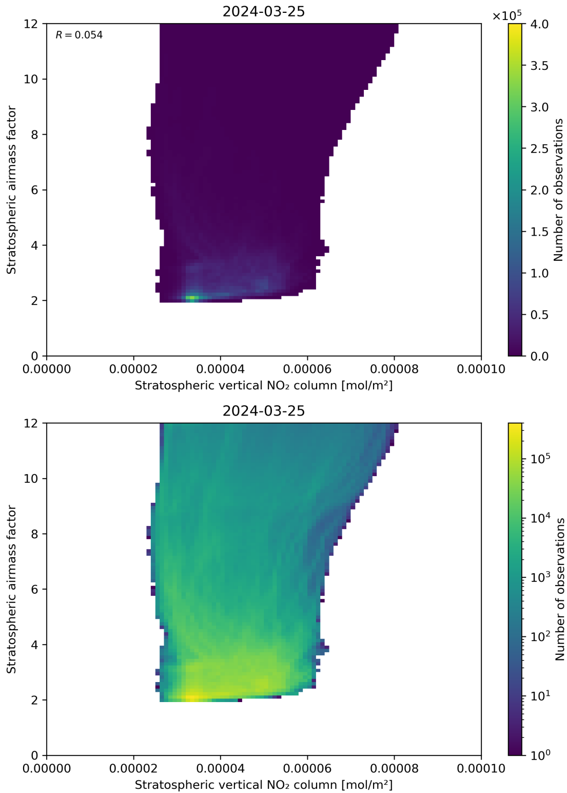
Figure 96: Scatter density plot of “Stratospheric vertical NO 2 column” against “Stratospheric airmass factor” for 2024-03-25 to 2024-03-26.
