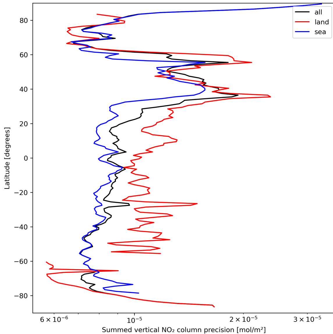
Figure 24: Zonal average of “Summed vertical NO 2 column precision” for 2024-03-25 to 2024-03-26.
