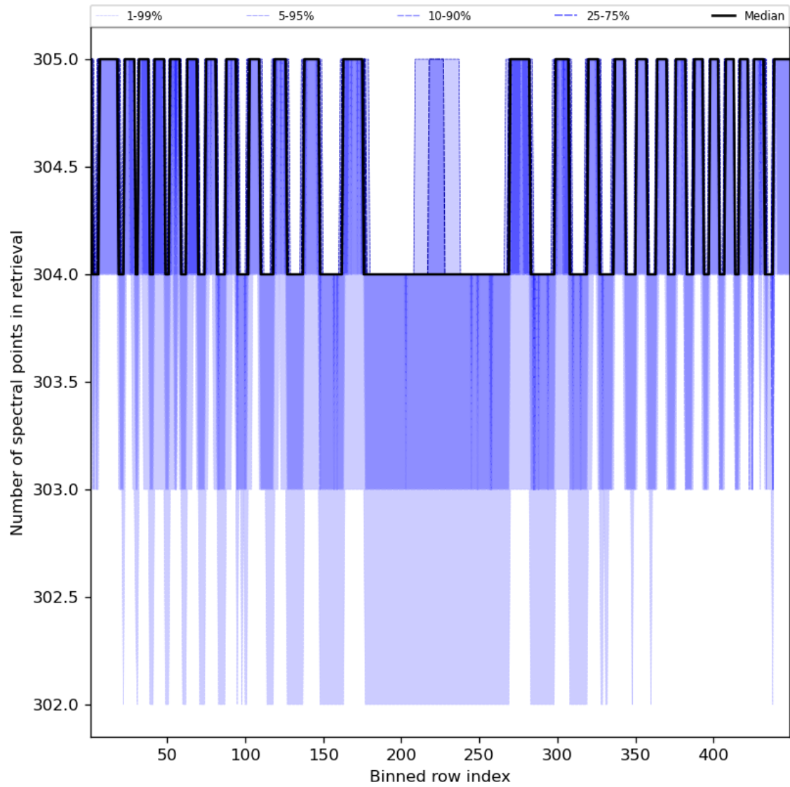
Figure 50: Along track statistics of “Number of spectral points in retrieval” for 2024-03-25 to 2024-03-26
