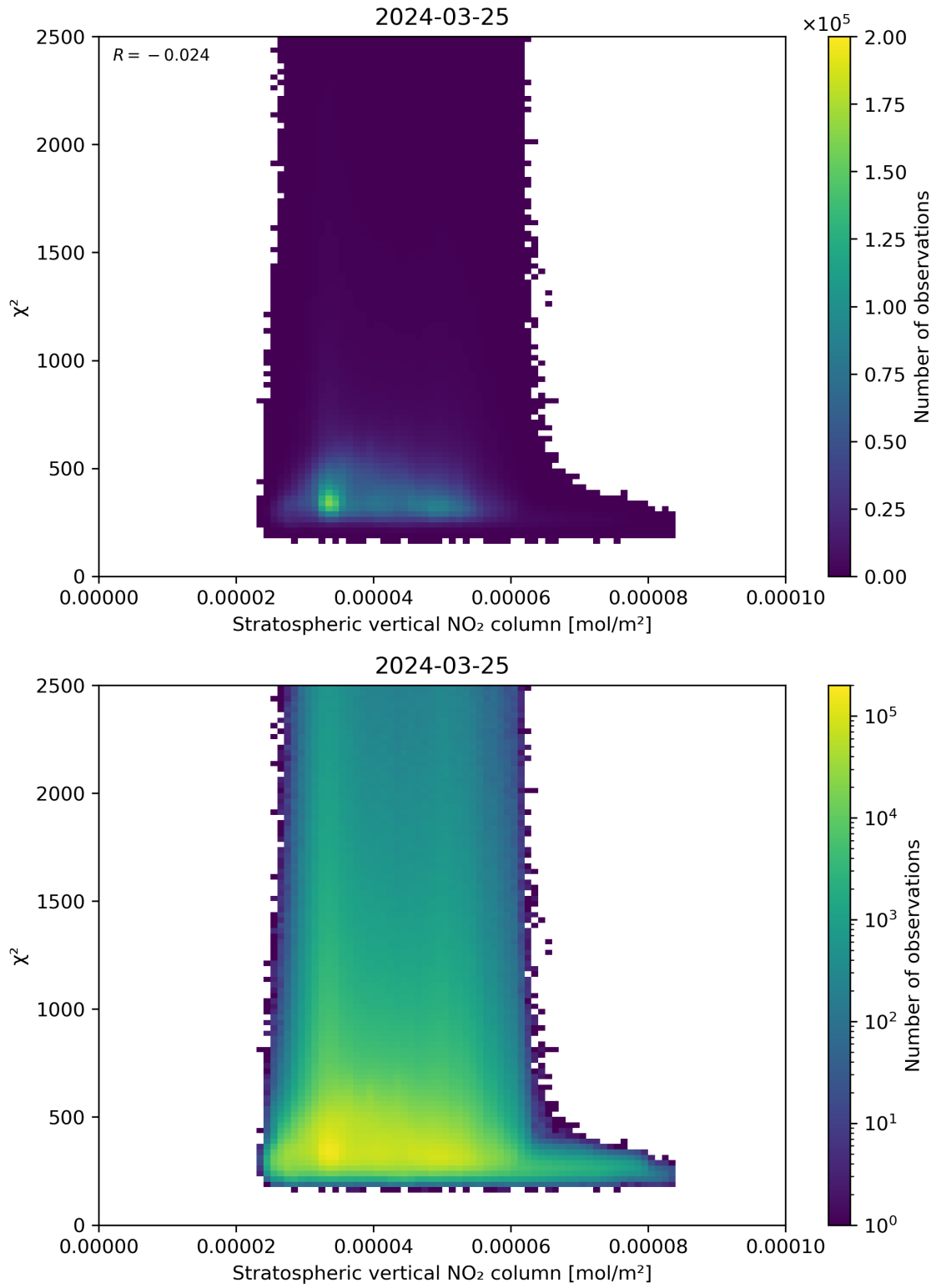
Figure 97: Scatter density plot of “Stratospheric vertical NO 2 column” against “ \chi^2 ” for 2024-03-25 to 2024-03-26.
