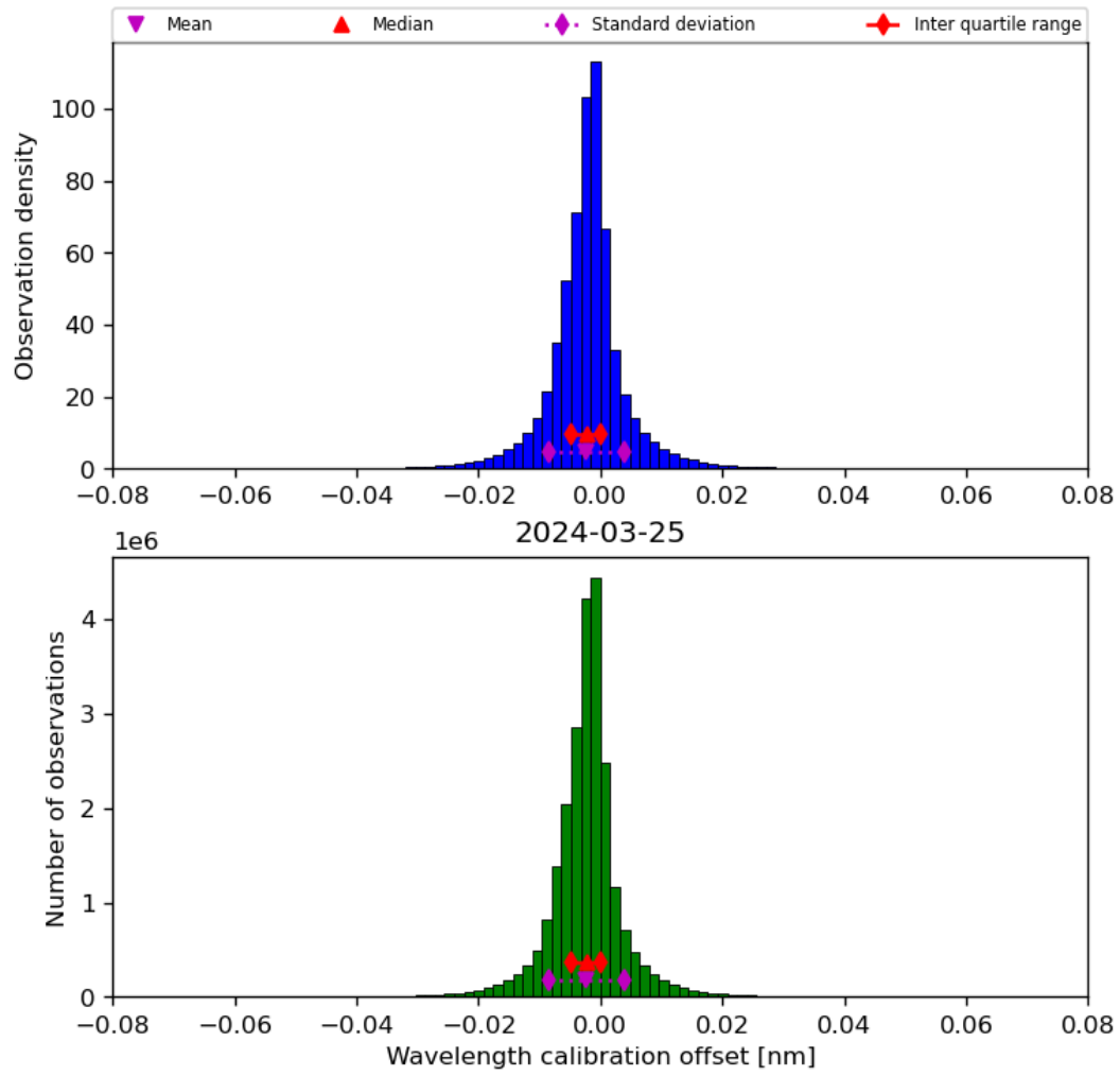
Figure 35: Histogram of “Wavelength calibration offset” for 2024-03-25 to 2024-03-26
