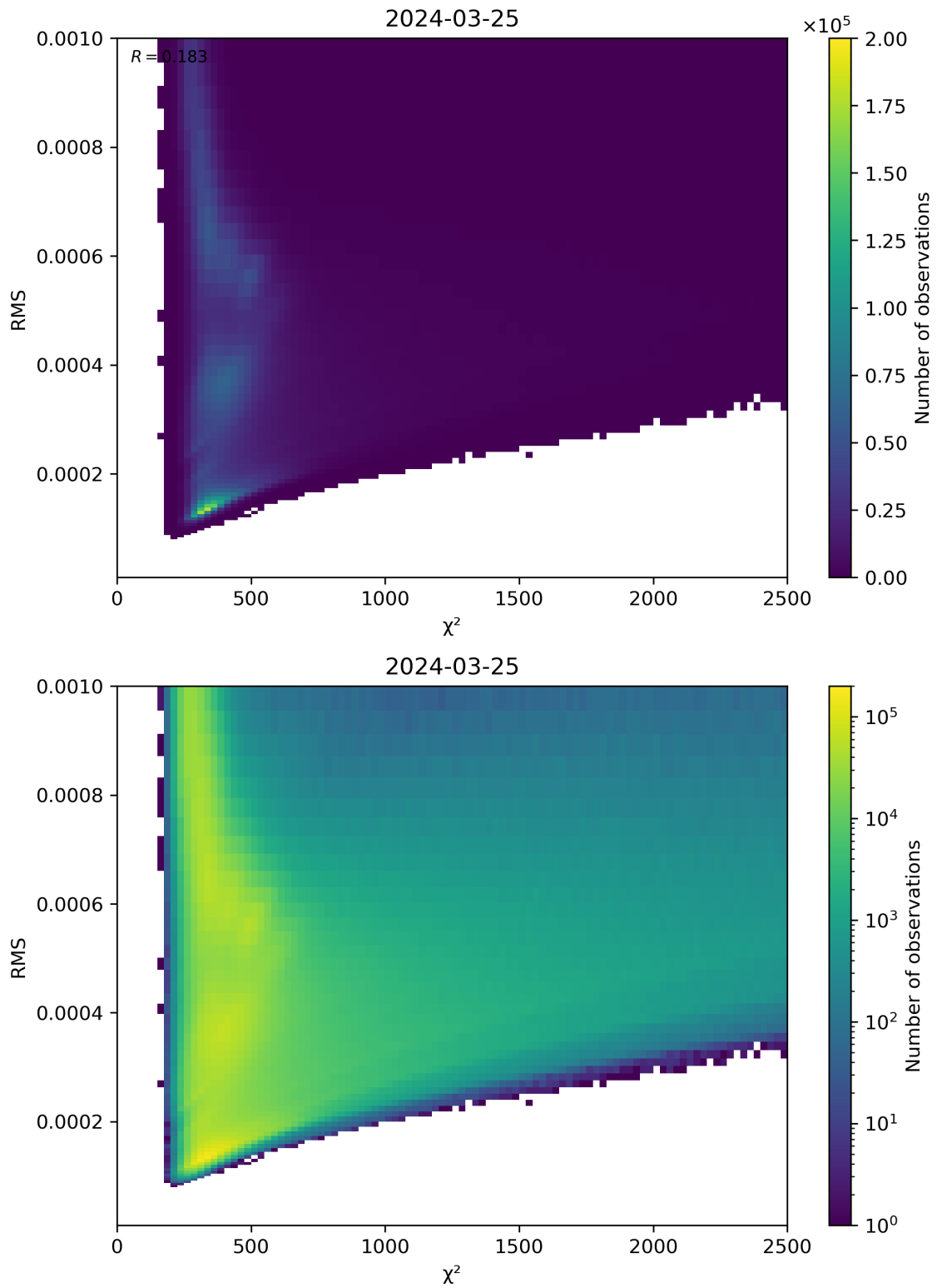
Figure 82: Scatter density plot of “ \chi^2 ” against “RMS” for 2024-03-25 to 2024-03-26.
