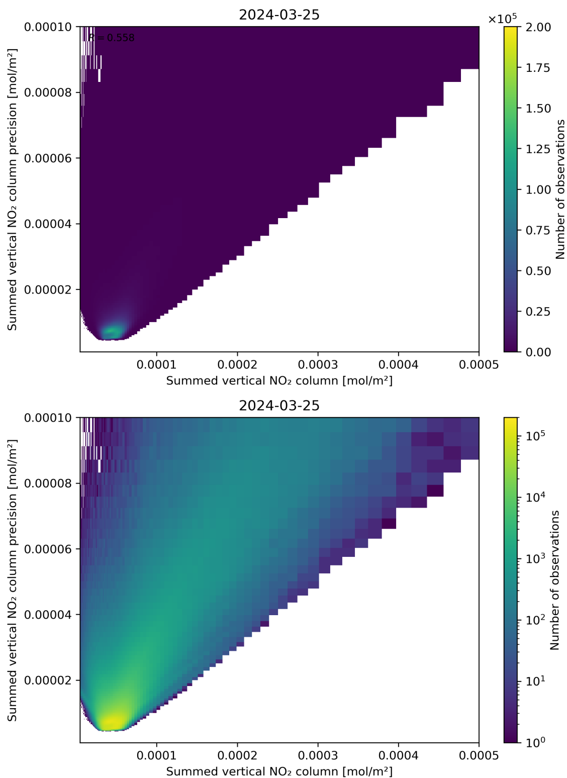
Figure 105: Scatter density plot of “Summed vertical NO 2 column” against “Summed vertical NO 2 column precision” for 2024-03-25 to 2024-03-26.
