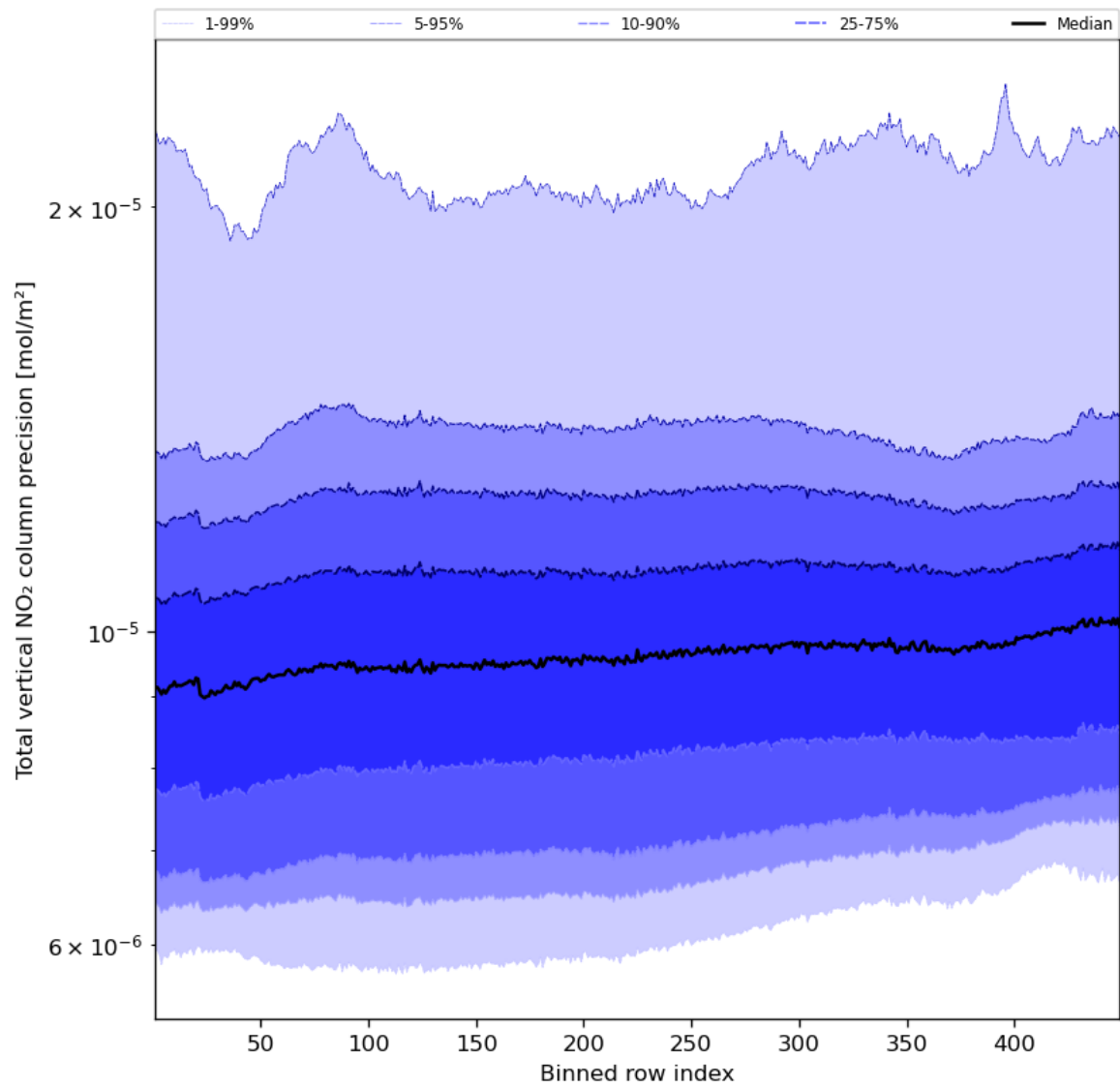
Figure 56: Along track statistics of “Total vertical NO 2 column precision” for 2024-03-25 to 2024-03-26
