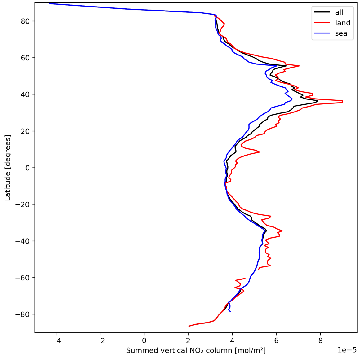
Figure 23: Zonal average of “Summed vertical NO 2 column” for 2024-03-25 to 2024-03-26.
