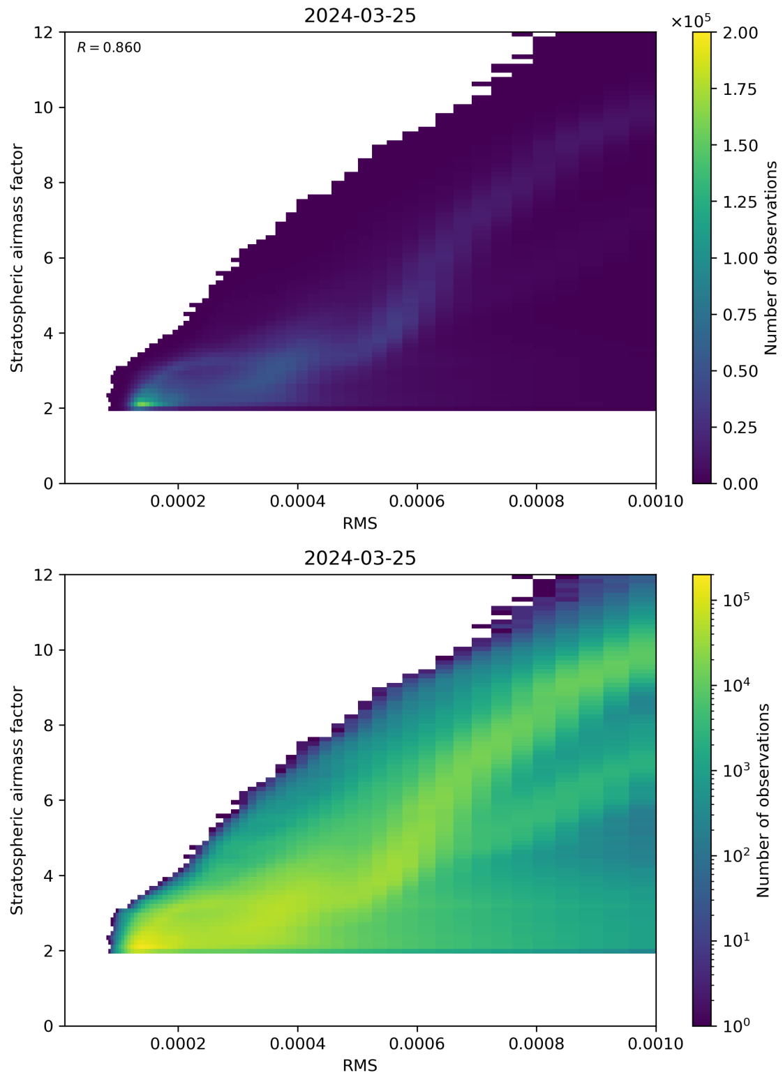
Figure 144: Scatter density plot of “RMS” against “Stratospheric airmass factor” for 2024-03-25 to 2024-03-26.
