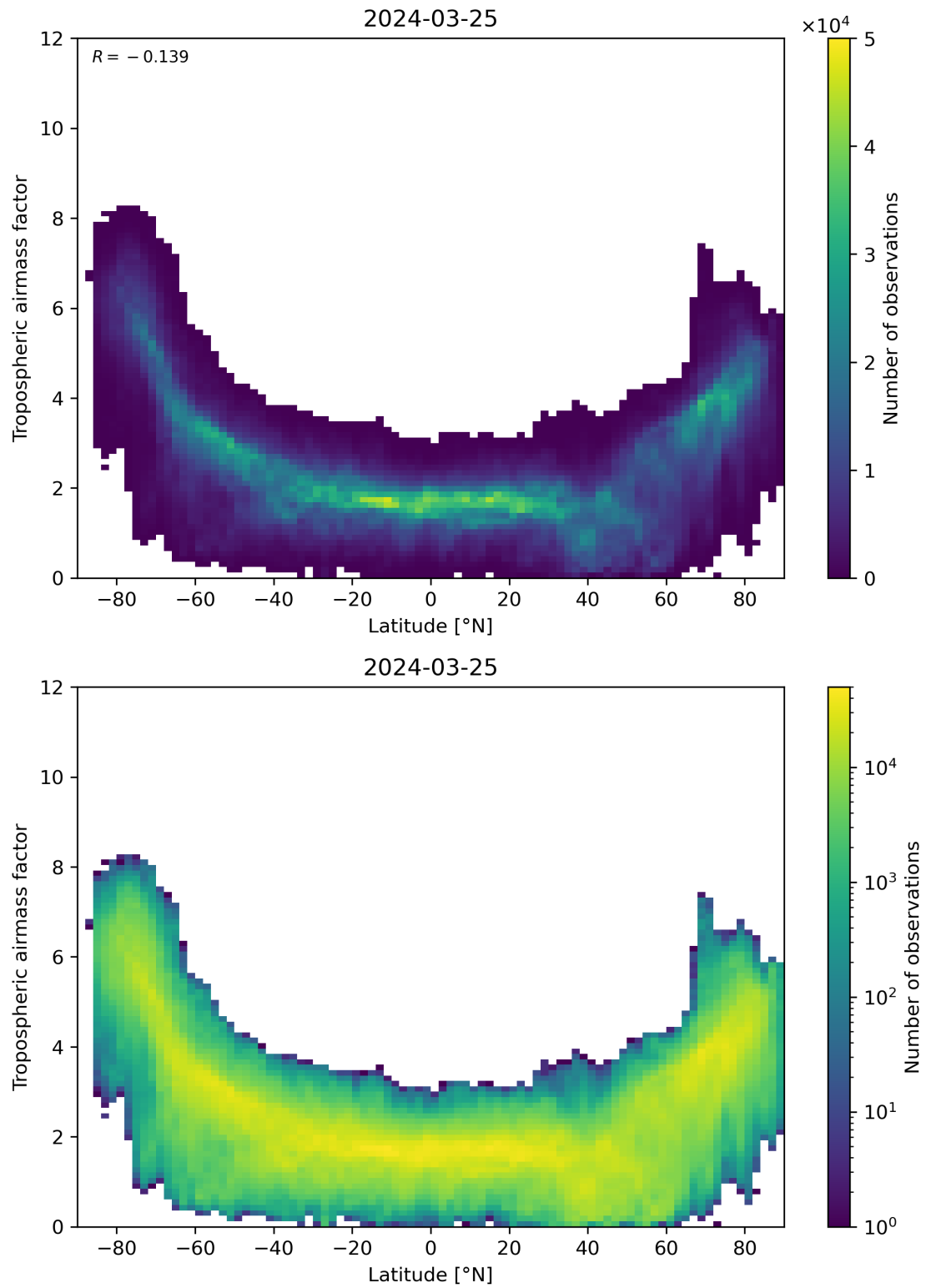
Figure 85: Scatter density plot of “Latitude” against “Tropospheric airmass factor” for 2024-03-25 to 2024-03-26.
