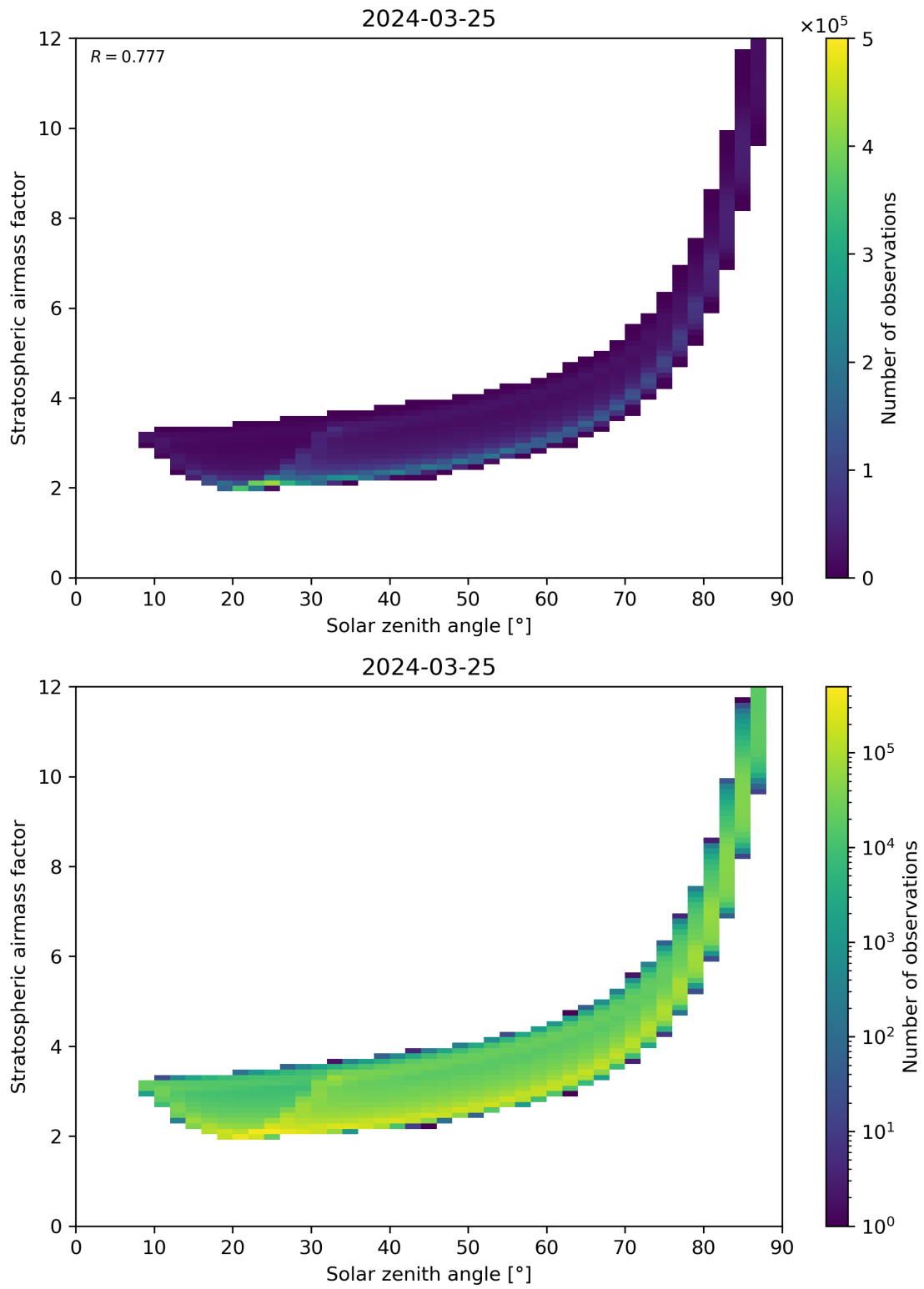
Figure 145: Scatter density plot of “Solar zenith angle” against “Stratospheric airmass factor” for 2024-03-25 to 2024-03-26.
