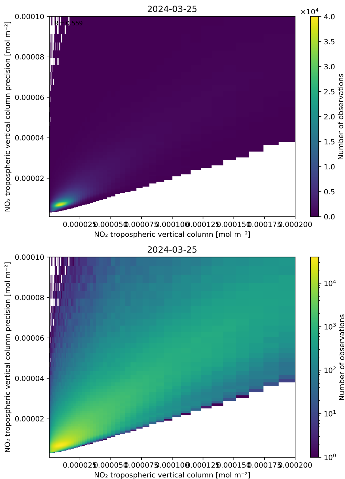
Figure 130: Scatter density plot of “NO 2 tropospheric vertical column” against “NO 2 tropospheric vertical column precision” for 2024-03-25 to 2024-03-26.
