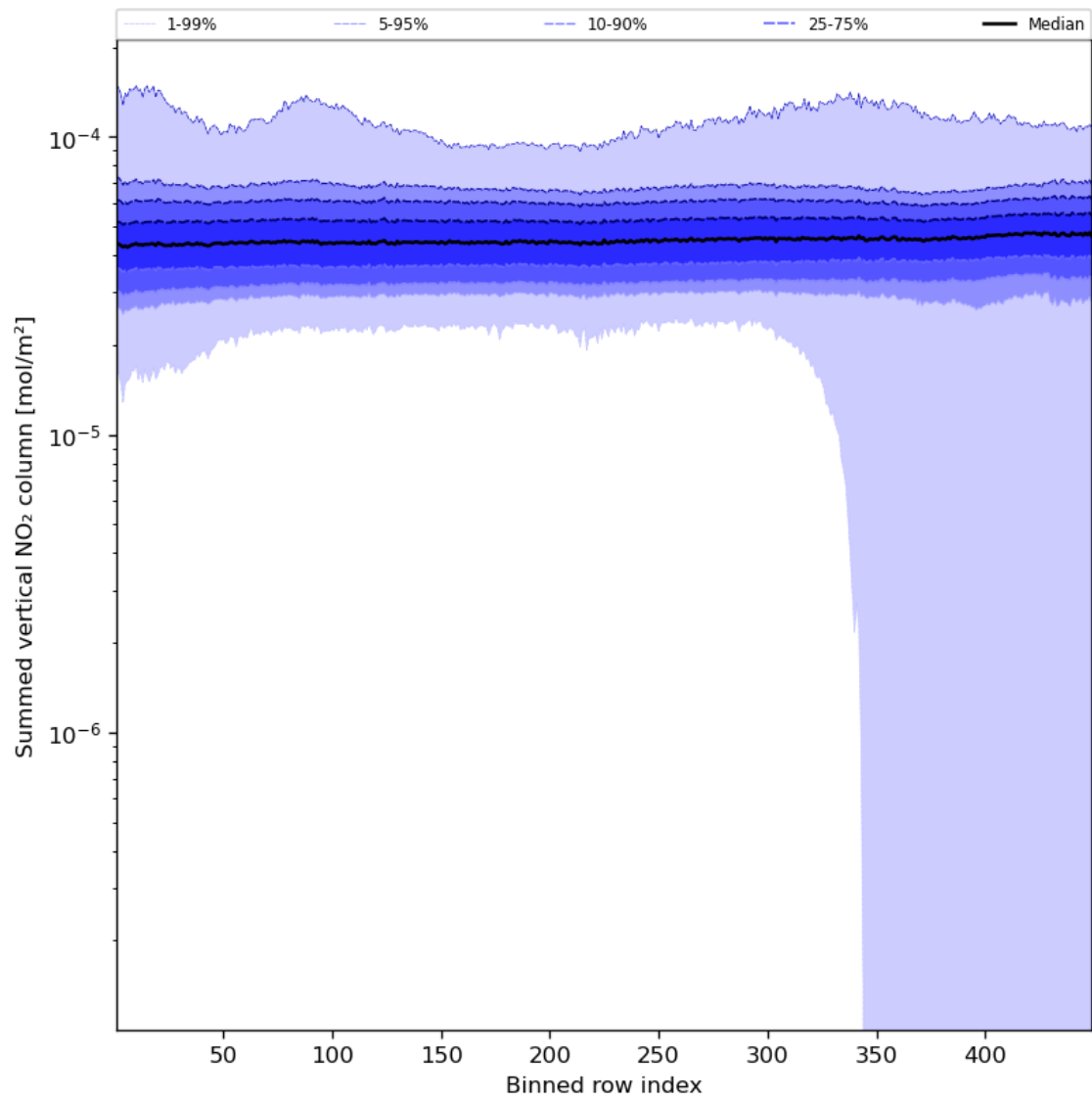
Figure 57: Along track statistics of “Summed vertical NO 2 column” for 2024-03-25 to 2024-03-26
