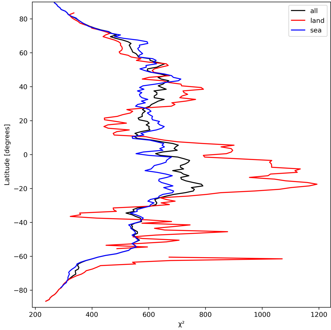
Figure 25: Zonal average of “ \chi^2 ” for 2024-03-25 to 2024-03-26.
