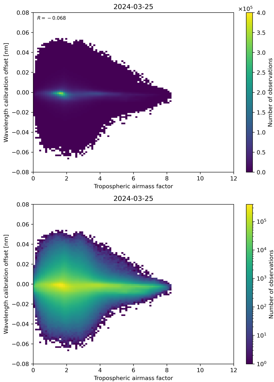
Figure 80: Scatter density plot of “Tropospheric airmass factor” against “Wavelength calibration offset” for 2024-03-25 to 2024-03-26.
