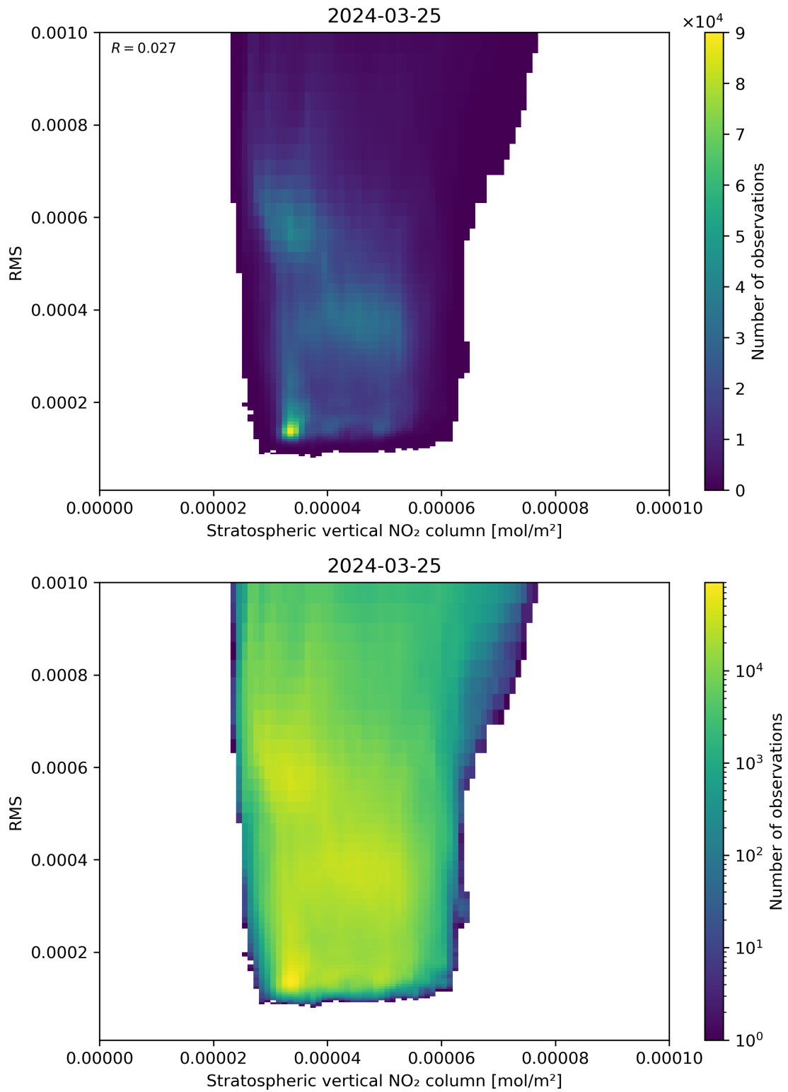
Figure 102: Scatter density plot of “Stratospheric vertical NO 2 column” against “RMS” for 2024-03-25 to 2024-03-26.
