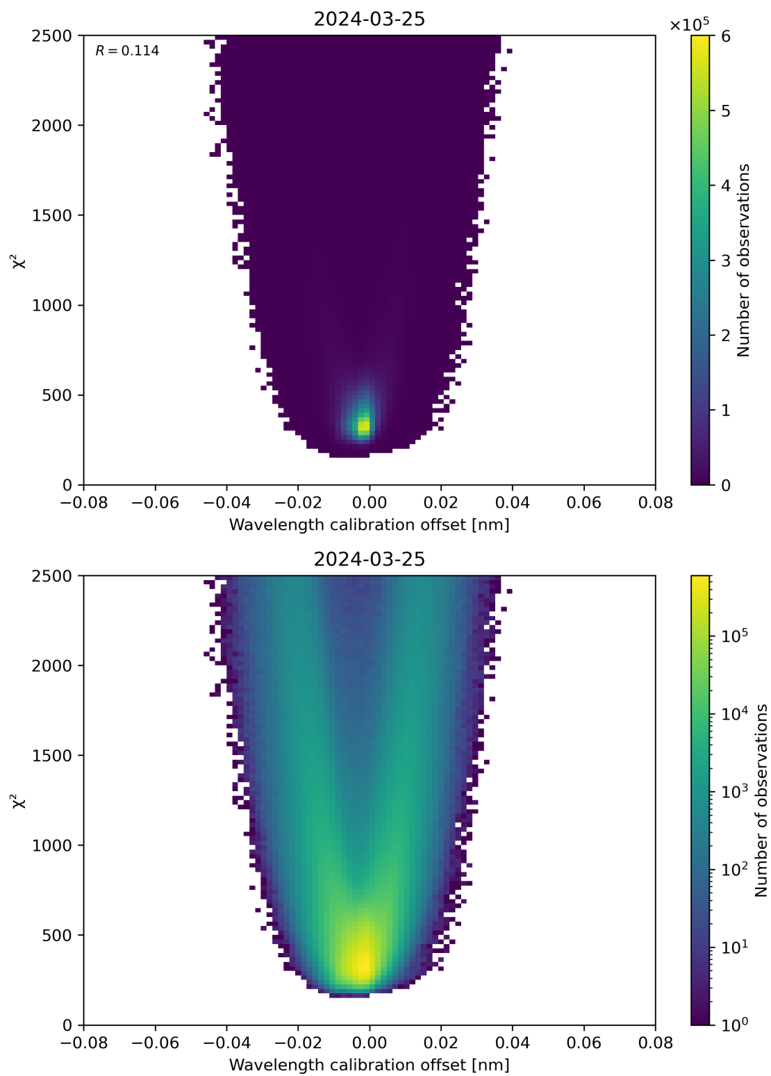
Figure 175: Scatter density plot of “Wavelength calibration offset” against “ \chi^2 ” for 2024-03-25 to 2024-03-26.
