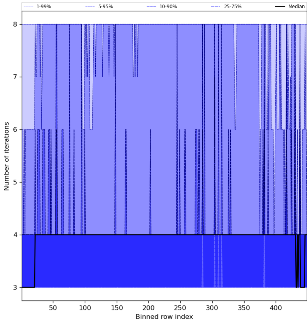
Figure 51: Along track statistics of “Number of iterations” for 2024-03-25 to 2024-03-26
