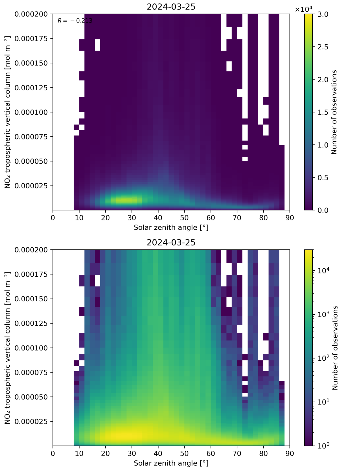
Figure 155: Scatter density plot of “Solar zenith angle” against “NO 2 tropospheric vertical column” for 2024-03-25 to 2024-03-26.
