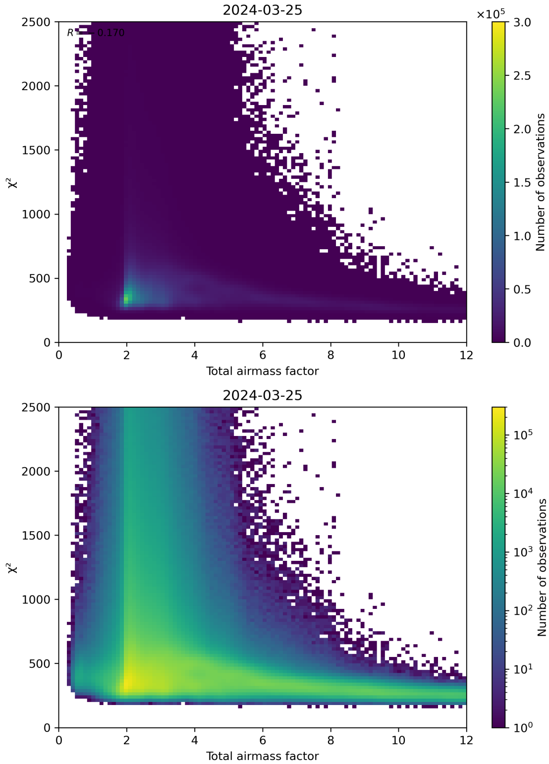
Figure 63: Scatter density plot of “Total airmass factor” against “ \chi^2 ” for 2024-03-25 to 2024-03-26.
