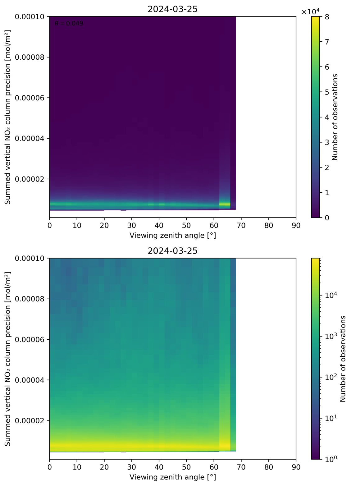
Figure 166: Scatter density plot of “Viewing zenith angle” against “Summed vertical NO 2 column precision” for 2024-03-25 to 2024-03-26.
