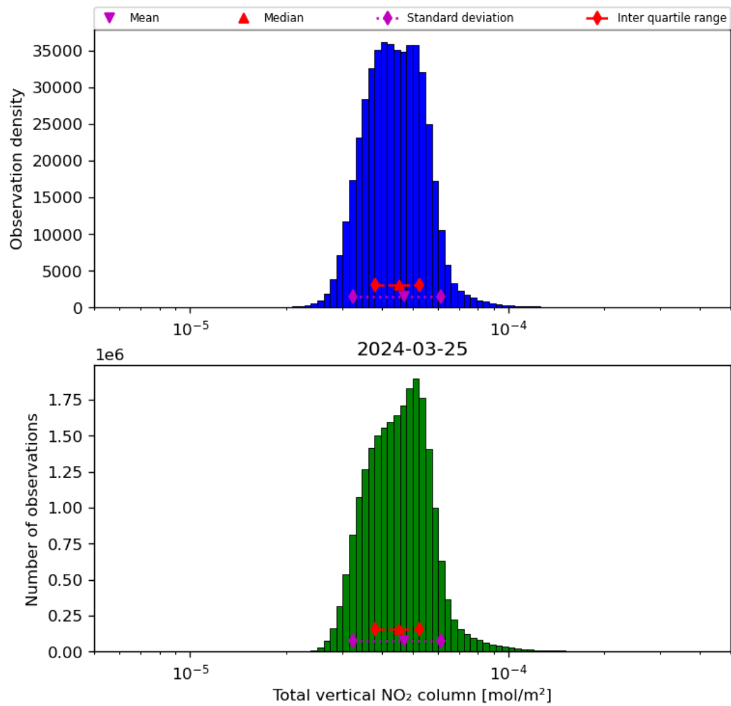
Figure 38: Histogram of "Total vertical NO 2 column" for 2024-03-25 to 2024-03-26
