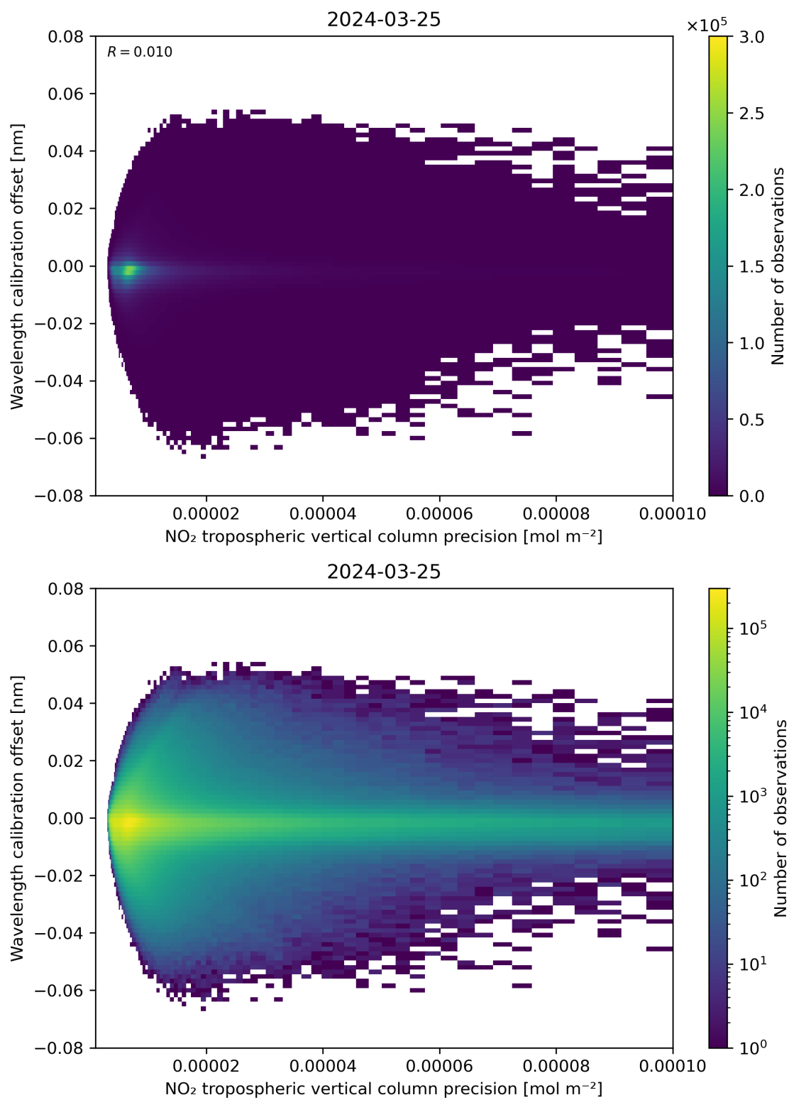
Figure 141: Scatter density plot of “NO 2 tropospheric vertical column precision” against “Wavelength calibration offset” for 2024-03-25 to 2024-03-26.
