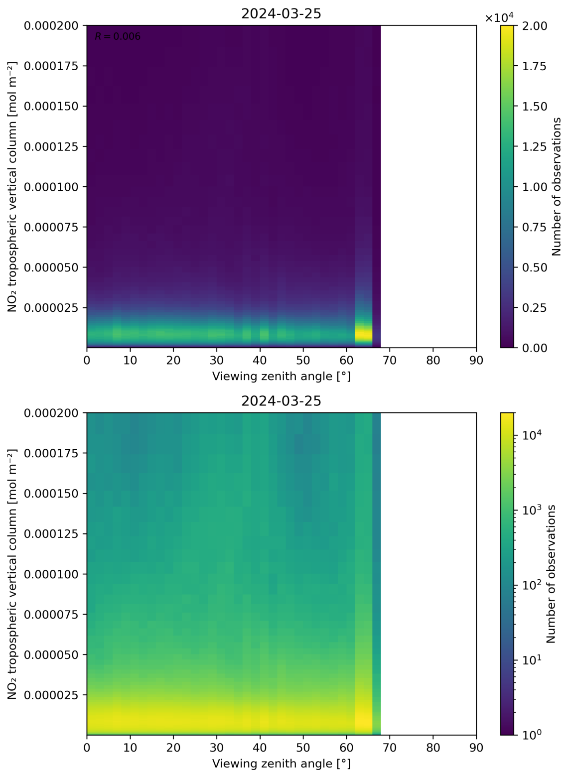
Figure 169: Scatter density plot of “Viewing zenith angle” against “NO 2 tropospheric vertical column” for 2024-03-25 to 2024-03-26.
