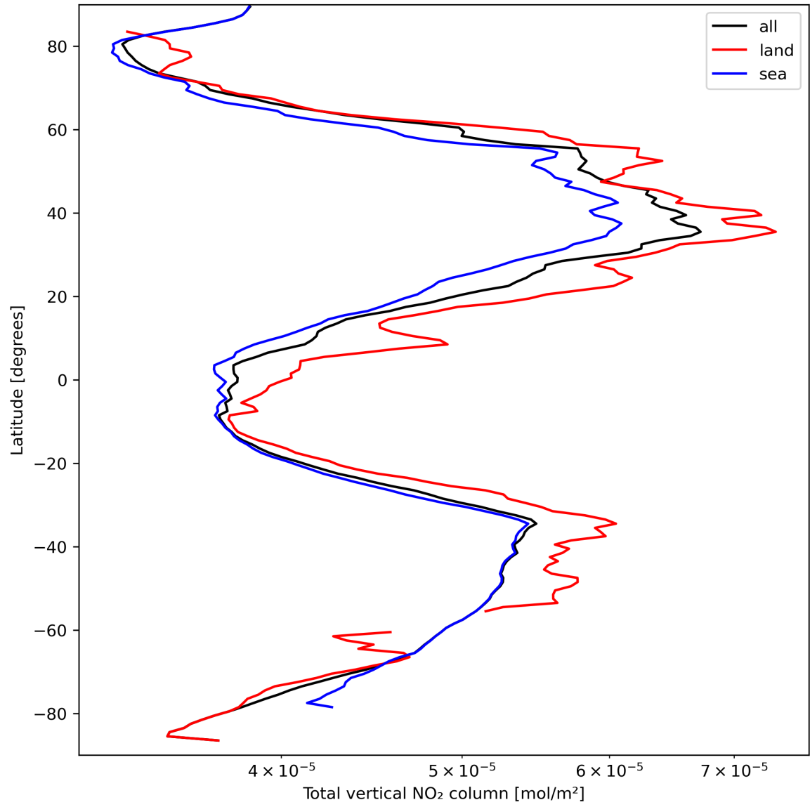
Figure 21: Zonal average of “Total vertical NO 2 column” for 2024-03-25 to 2024-03-26.
