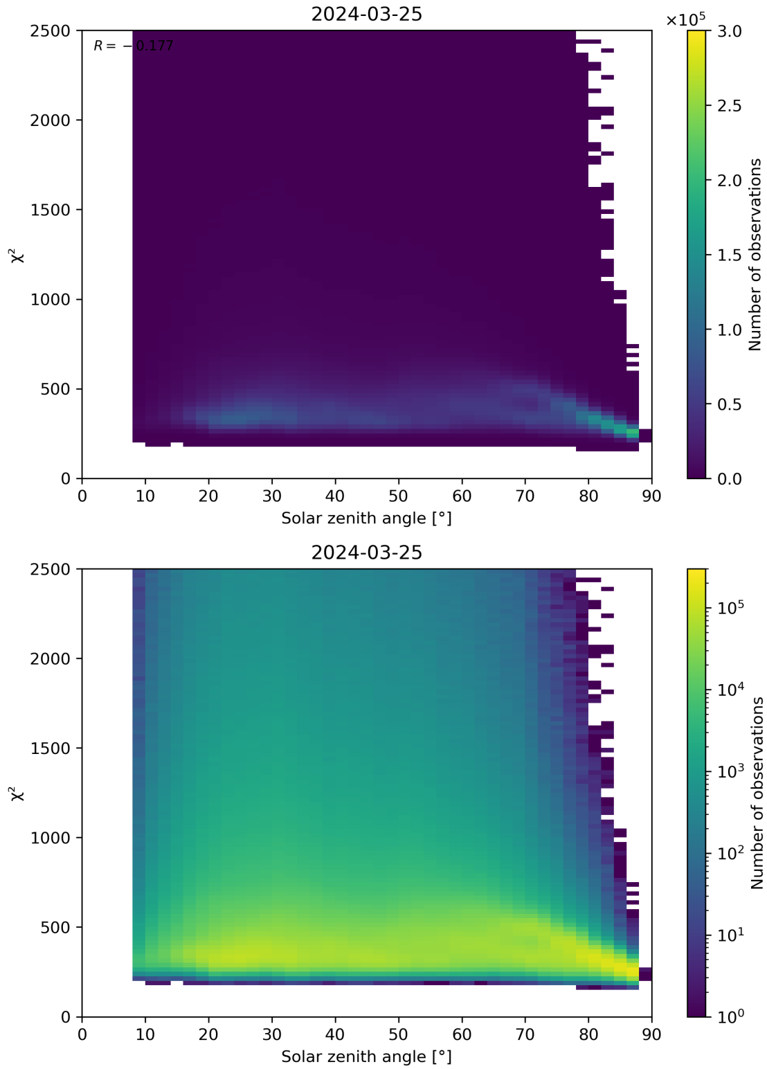
Figure 148: Scatter density plot of “Solar zenith angle” against “ \chi^2 ” for 2024-03-25 to 2024-03-26.
