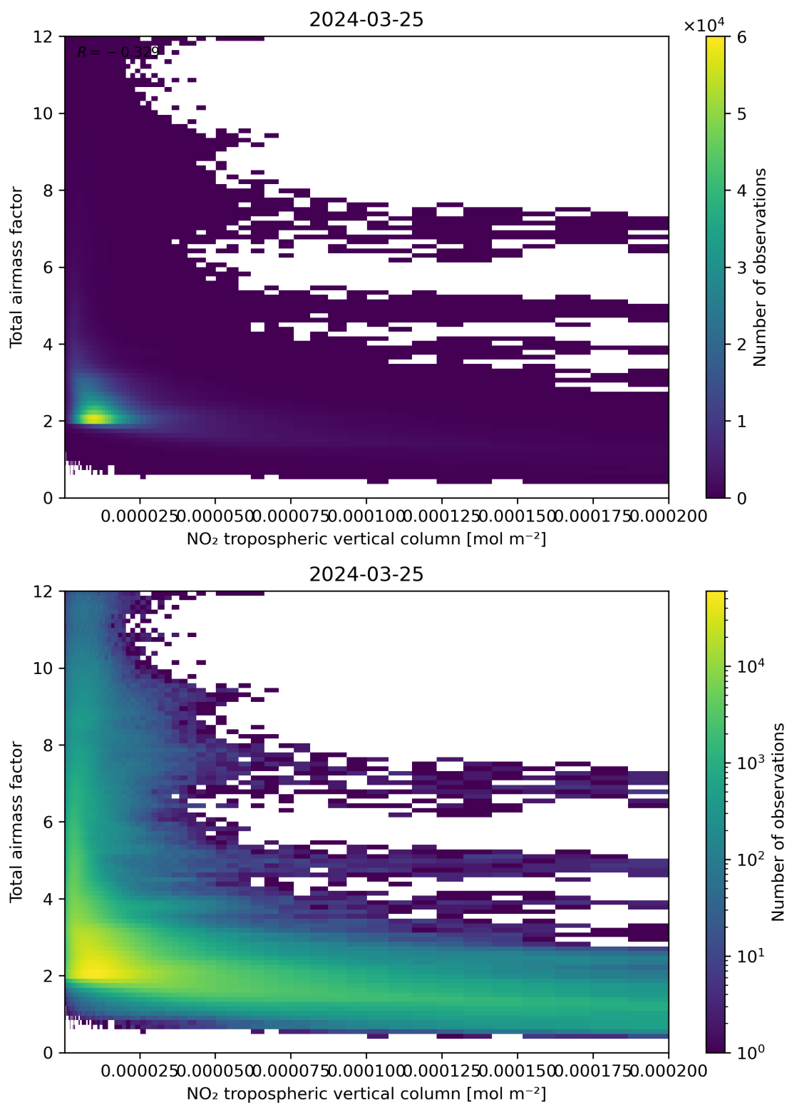
Figure 122: Scatter density plot of “NO 2 tropospheric vertical column” against “Total air mass factor” for 2024-03-25 to 2024-03-26.
