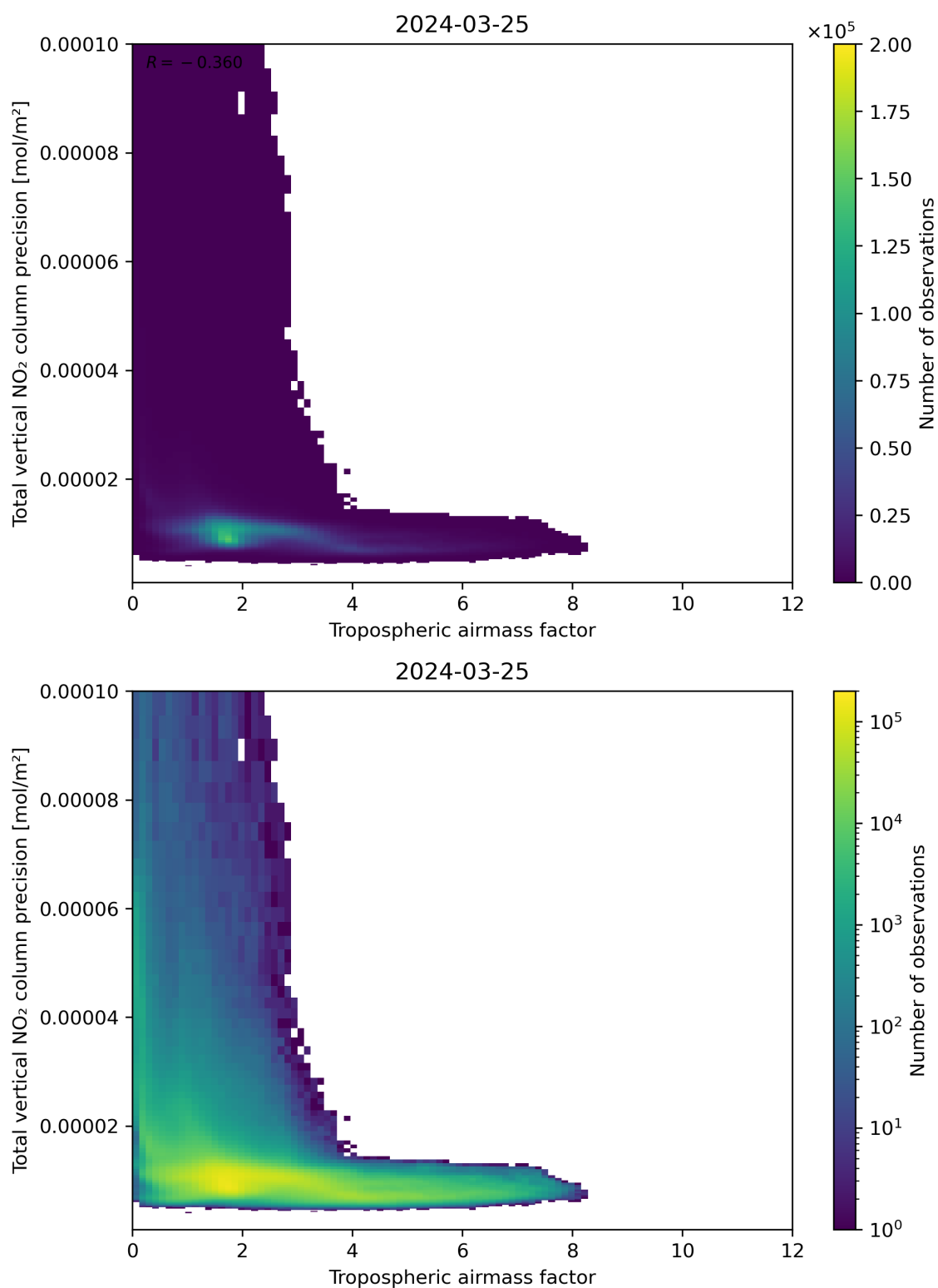
Figure 78: Scatter density plot of “Tropospheric air mass factor” against “Total vertical NO 2 column precision” for 2024-03-25 to 2024-03-26.
