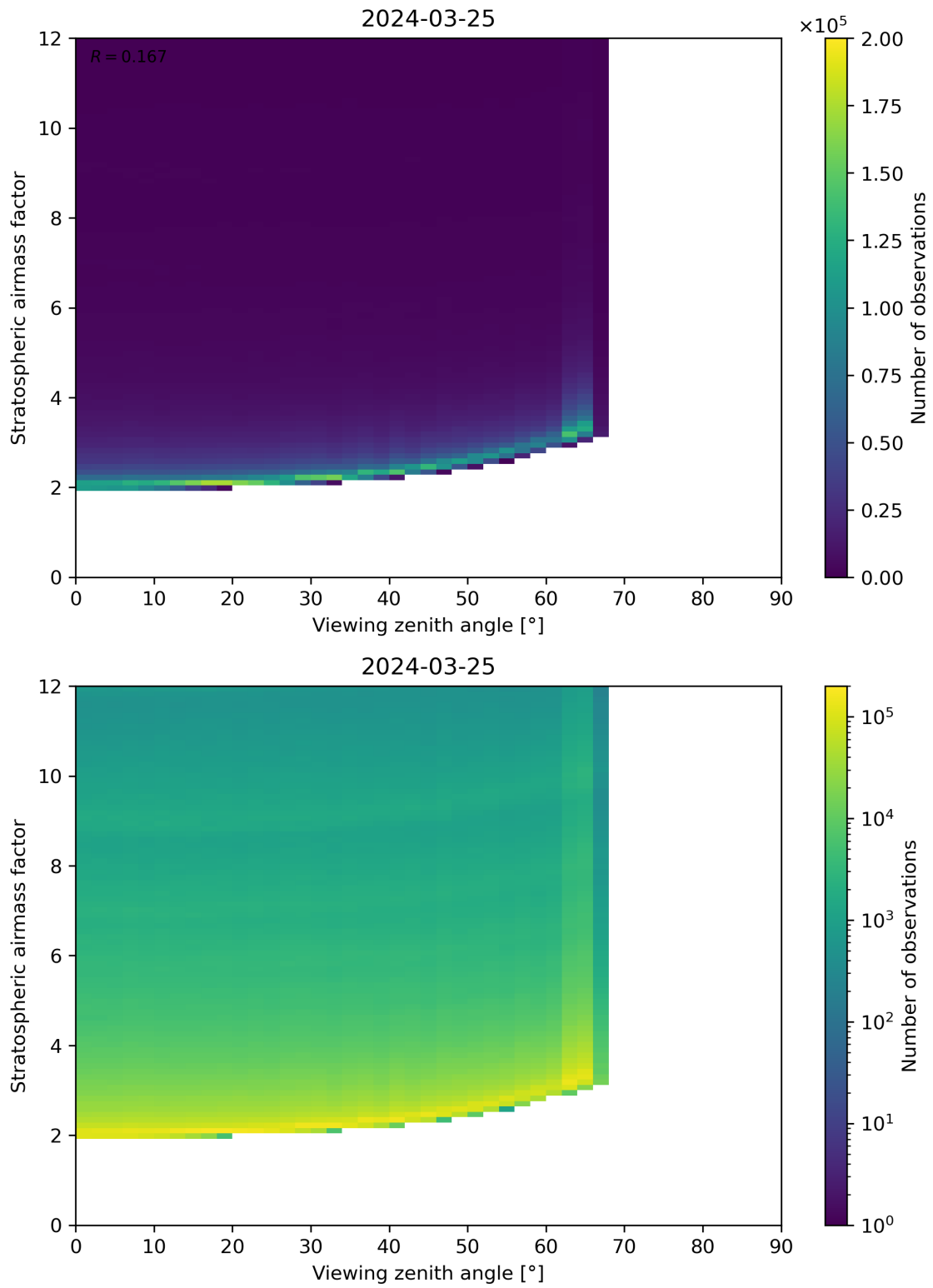
Figure 159: Scatter density plot of “Viewing zenith angle” against “Stratospheric airmass factor” for 2024-03-25 to 2024-03-26.
