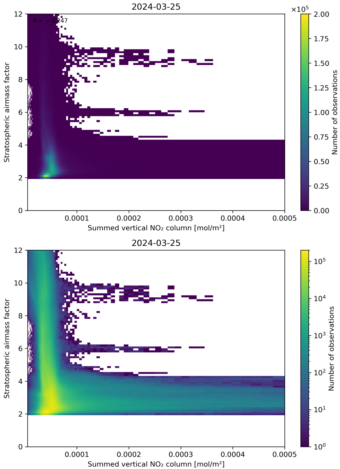
Figure 103: Scatter density plot of “Summed vertical NO 2 column” against “Stratospheric air mass factor” for 2024-03-25 to 2024-03-26.
