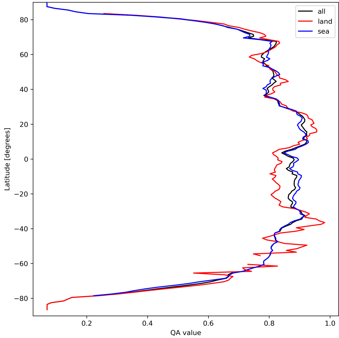
Figure 11: Zonal average of “QA value” for 2024-03-25 to 2024-03-26.
