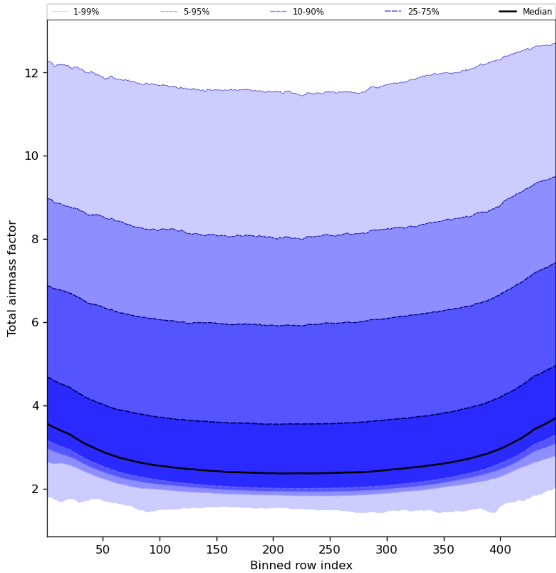
Figure 49: Along track statistics of “Total airmass factor” for 2024-03-25 to 2024-03-26
