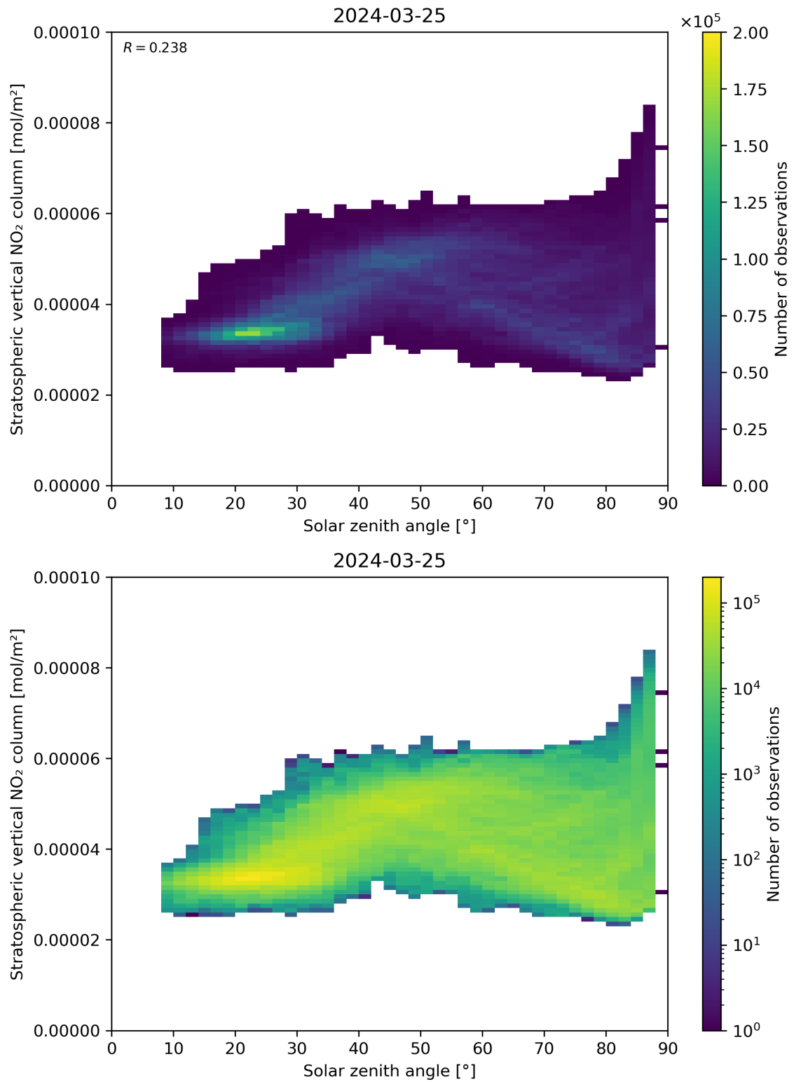
Figure 150: Scatter density plot of “Solar zenith angle” against “Stratospheric vertical NO 2 column” for 2024-03-25 to 2024-03-26.
