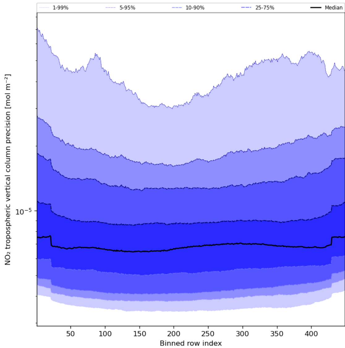
Figure 47: Along track statistics of “NO 2 tropospheric vertical column precision” for 2024-03-25 to 2024-03-26
