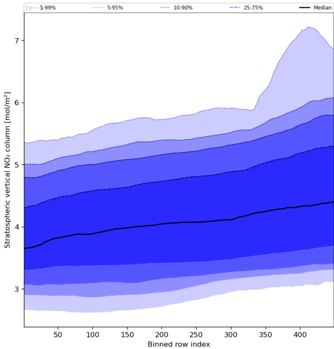
Figure 53: Along track statistics of “Stratospheric vertical NO 2 column” for 2024-03-25 to 2024-03-26
