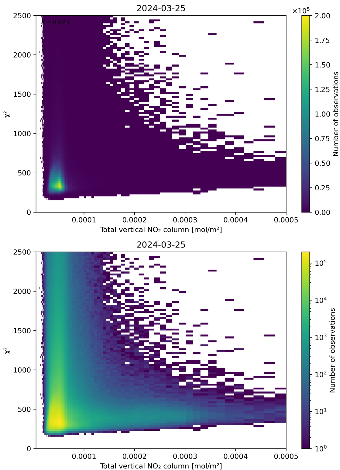
Figure 111: Scatter density plot of “Total vertical NO 2 column” against “ \chi^2 ” for 2024-03-25 to 2024-03-26.
