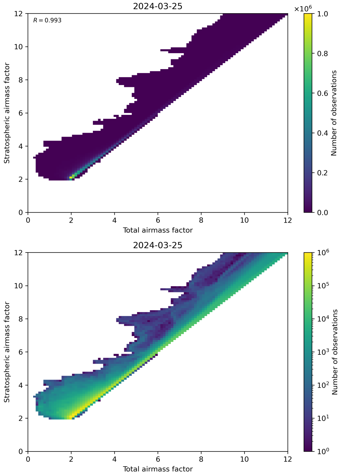
Figure 62: Scatter density plot of “Total airmass factor” against “Stratospheric airmass factor” for 2024-03-25 to 2024-03-26.
