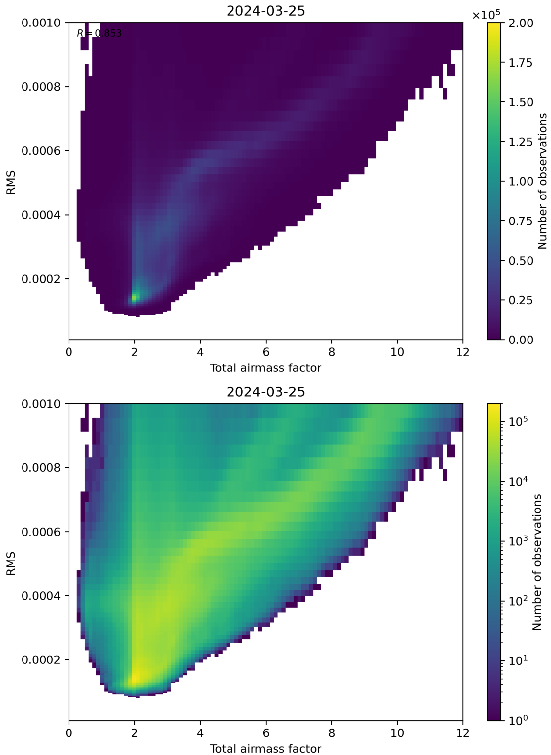
Figure 69: Scatter density plot of “Total airmass factor” against “RMS” for 2024-03-25 to 2024-03-26.
