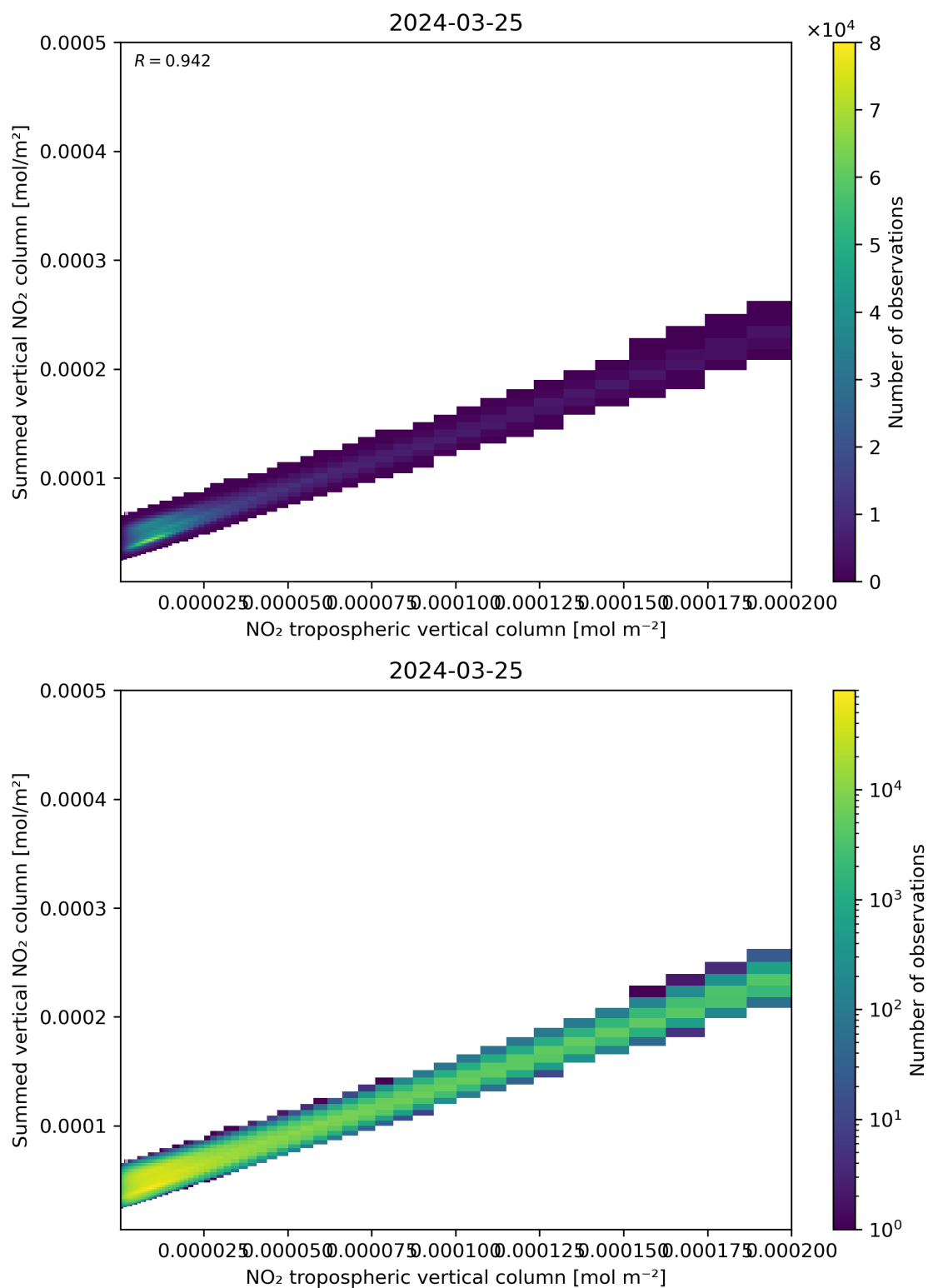
Figure 126: Scatter density plot of “NO 2 tropospheric vertical column” against “Summed vertical NO 2 column” for 2024-03-25 to 2024-03-26.
