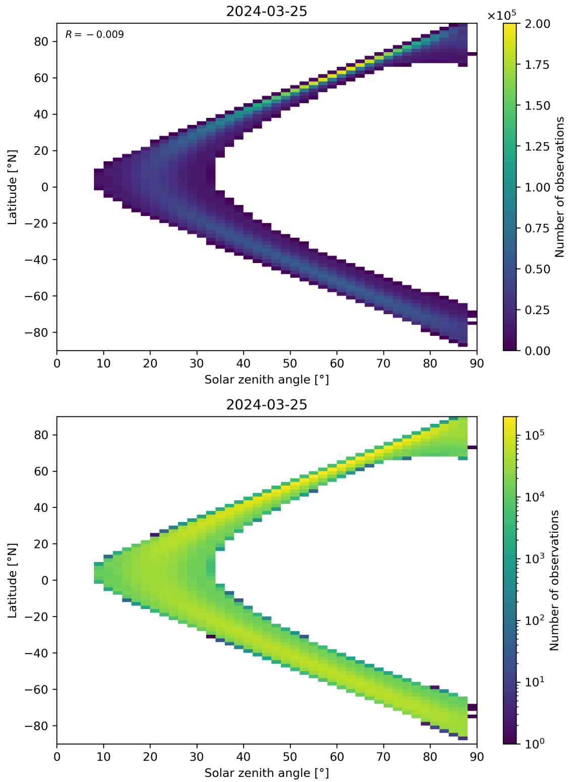
Figure 149: Scatter density plot of “Solar zenith angle” against “Latitude” for 2024-03-25 to 2024-03-26.
