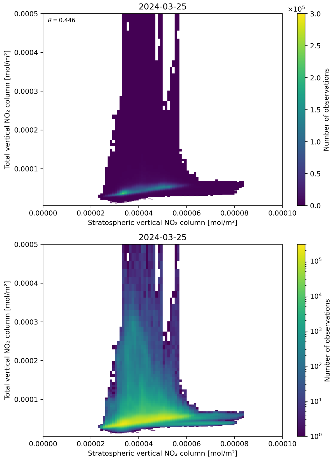
Figure 100: Scatter density plot of “Stratospheric vertical NO 2 column” against “Total vertical NO 2 column” for 2024-03-25 to 2024-03-26.
