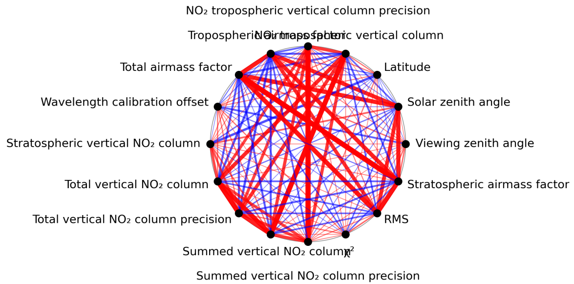
Figure 1: Map of correlation graph for 2024-03-25 to 2024-03-26.
