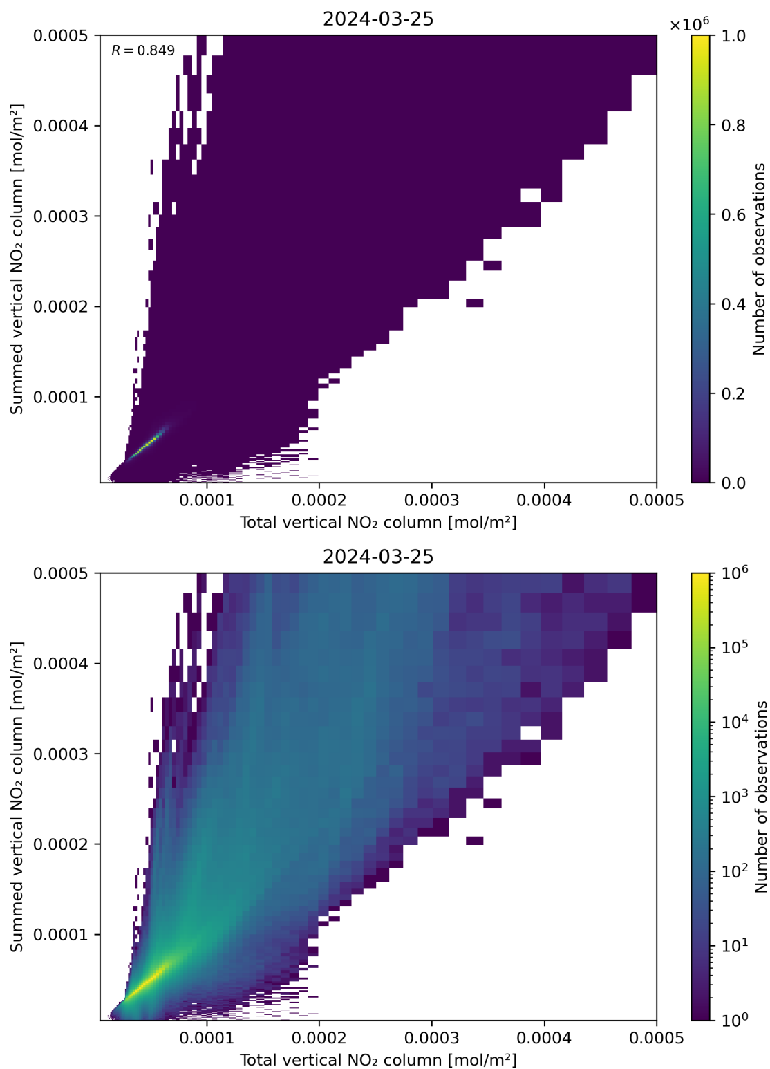
Figure 112: Scatter density plot of “Total vertical NO 2 column” against “Summed vertical NO 2 column” for 2024-03-25 to 2024-03-26.
