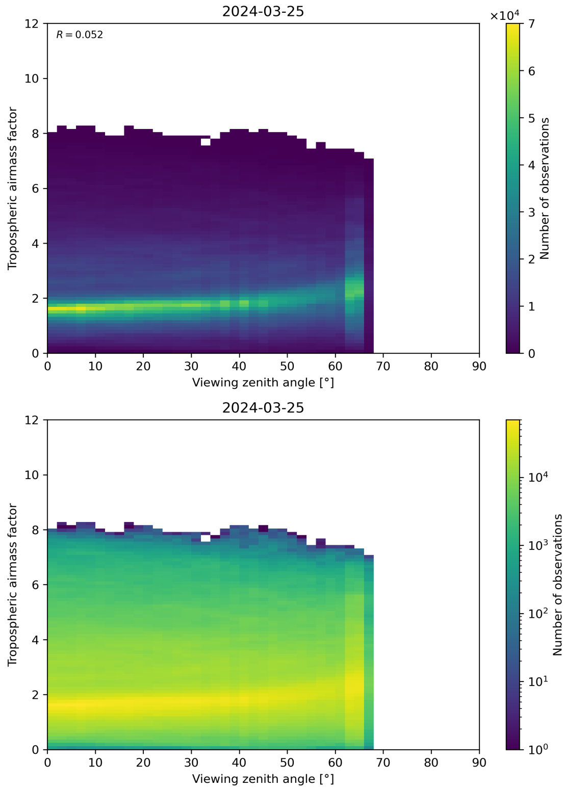
Figure 161: Scatter density plot of “Viewing zenith angle” against “Tropospheric airmass factor” for 2024-03-25 to 2024-03-26.
