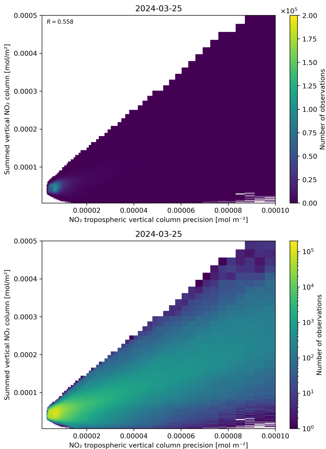
Figure 136: Scatter density plot of “NO 2 tropospheric vertical column precision” against “Summed vertical NO 2 column” for 2024-03-25 to 2024-03-26.
