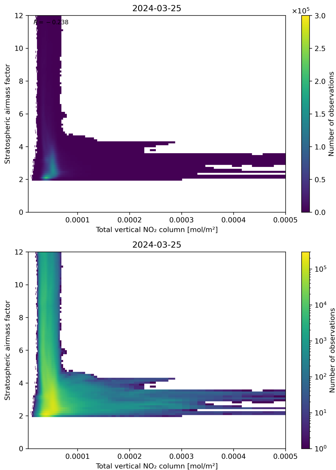
Figure 110: Scatter density plot of “Total vertical NO 2 column” against “Stratospheric airmass factor” for 2024-03-25 to 2024-03-26.
