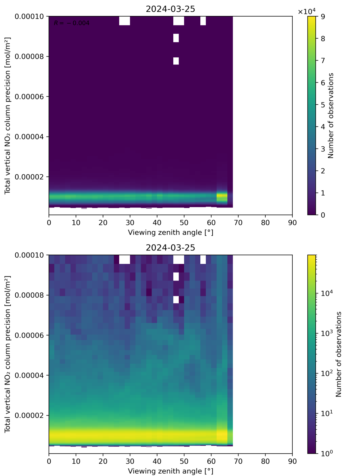
Figure 168: Scatter density plot of “Viewing zenith angle” against “Total vertical NO 2 column precision” for 2024-03-25 to 2024-03-26.
