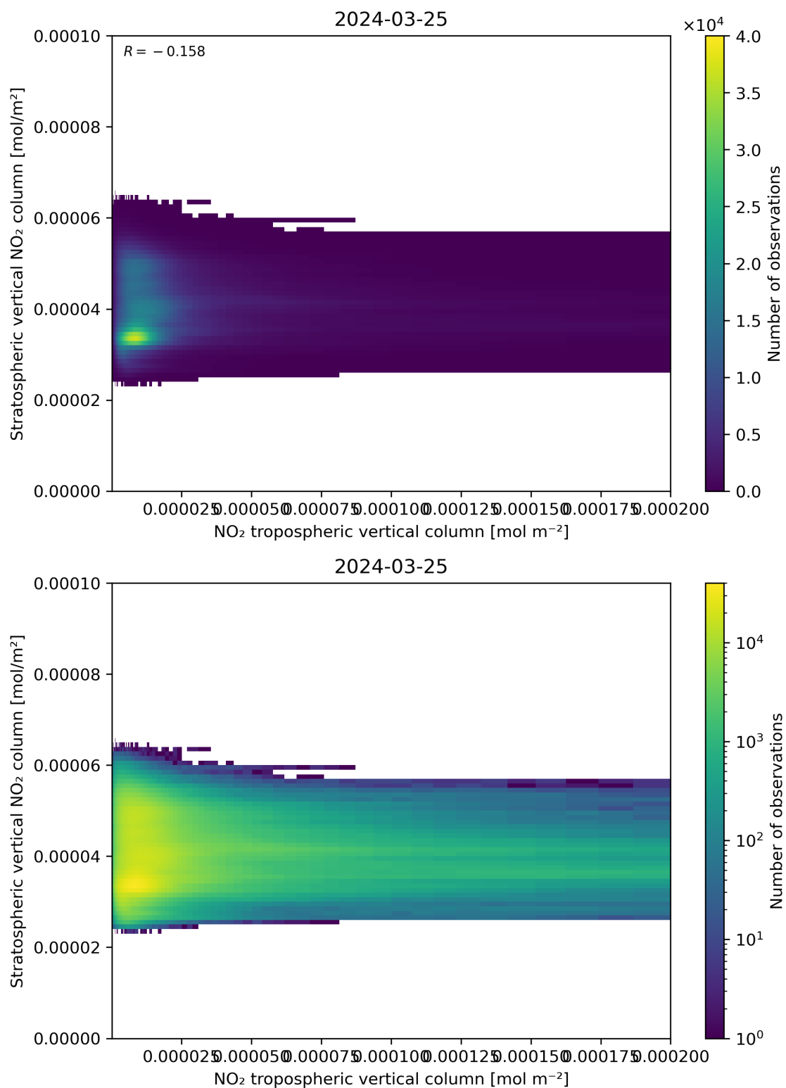
Figure 125: Scatter density plot of “NO 2 tropospheric vertical column” against “Stratospheric vertical NO 2 column” for 2024-03-25 to 2024-03-26.
