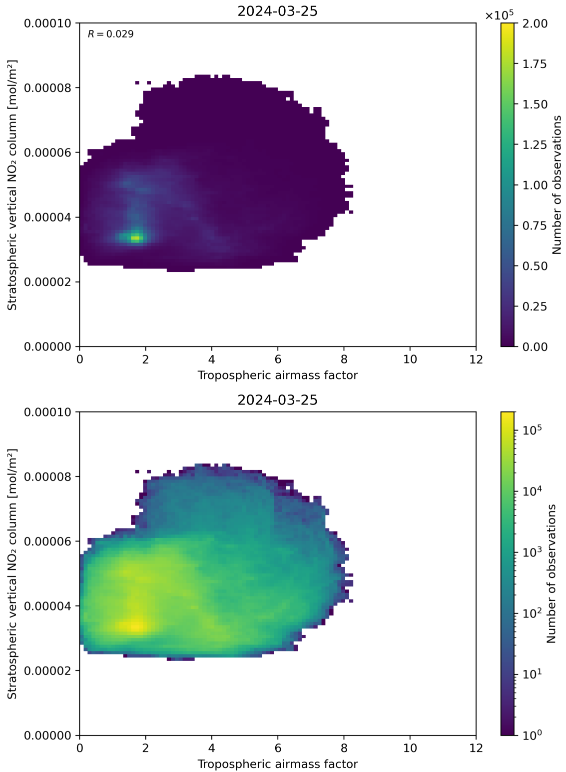
Figure 74: Scatter density plot of “Tropospheric air mass factor” against “Stratospheric vertical NO 2 column” for 2024-03-25 to 2024-03-26.
