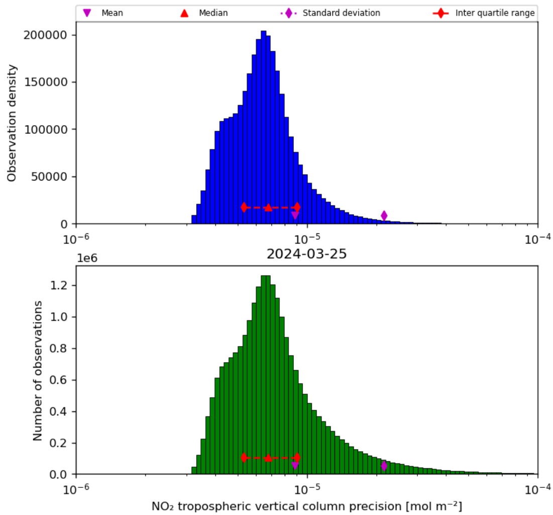
Figure 30: Histogram of “NO 2 tropospheric vertical column precision” for 2024-03-25 to 2024-03-26
