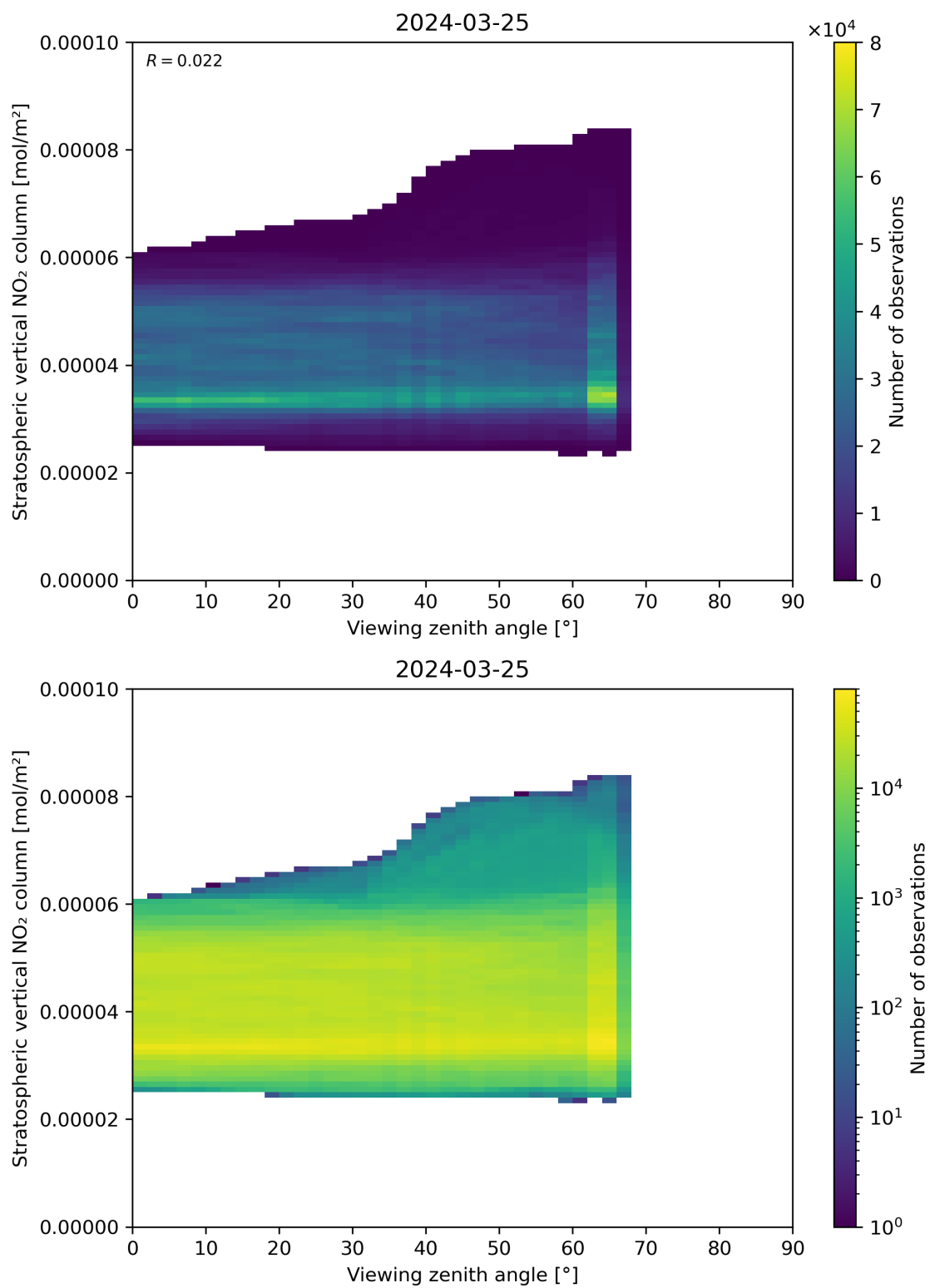
Figure 164: Scatter density plot of “Viewing zenith angle” against “Stratospheric vertical NO 2 column” for 2024-03-25 to 2024-03-26.
