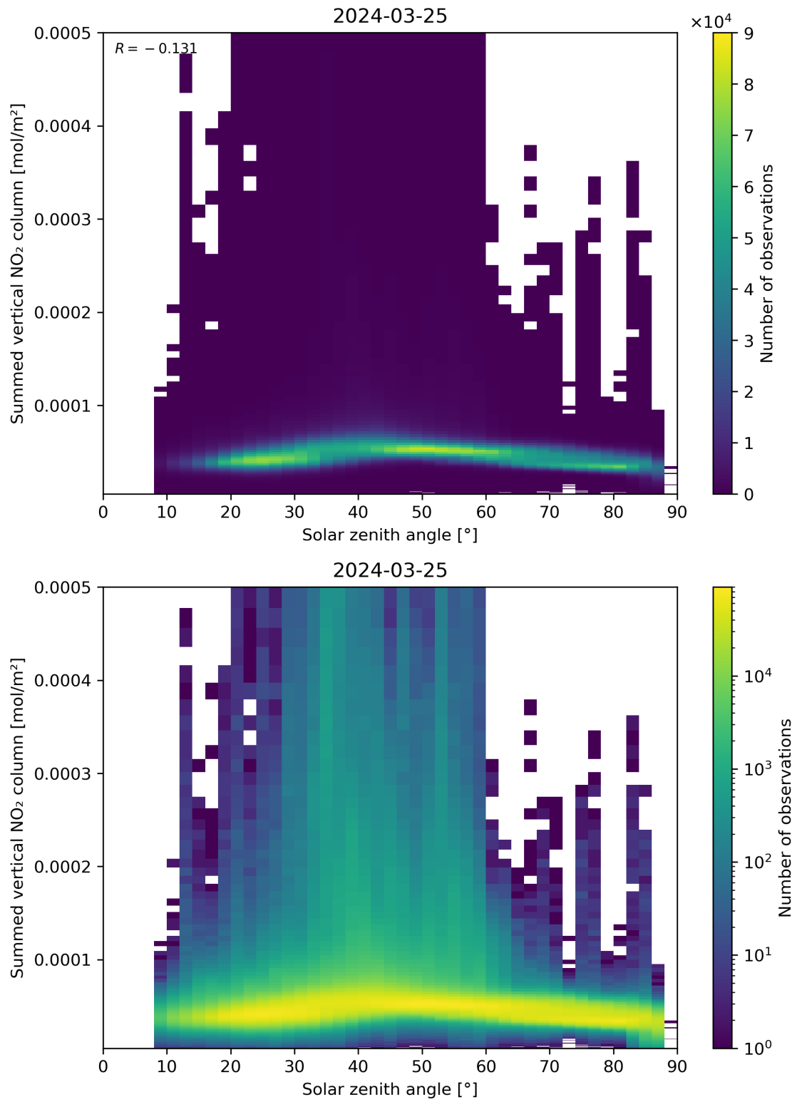
Figure 151: Scatter density plot of “Solar zenith angle” against “Summed vertical NO 2 column” for 2024-03-25 to 2024-03-26.
