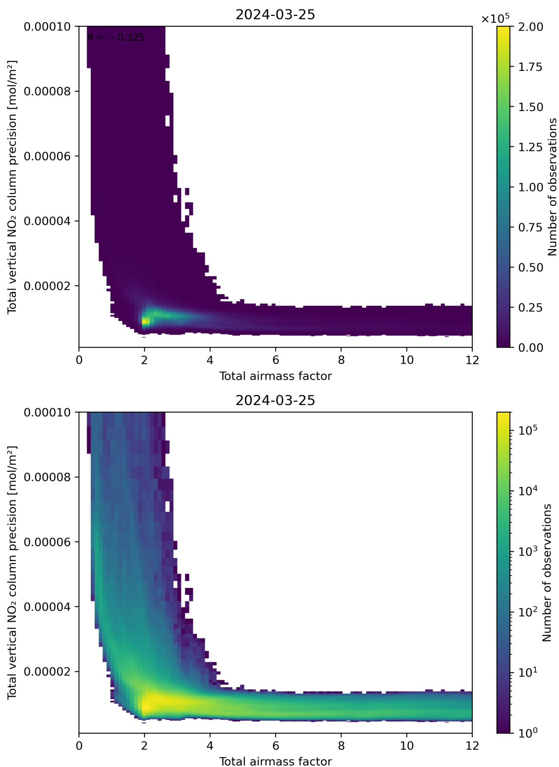
Figure 68: Scatter density plot of “Total airmass factor” against “Total vertical NO 2 column precision” for 2024-03-25 to 2024-03-26.
