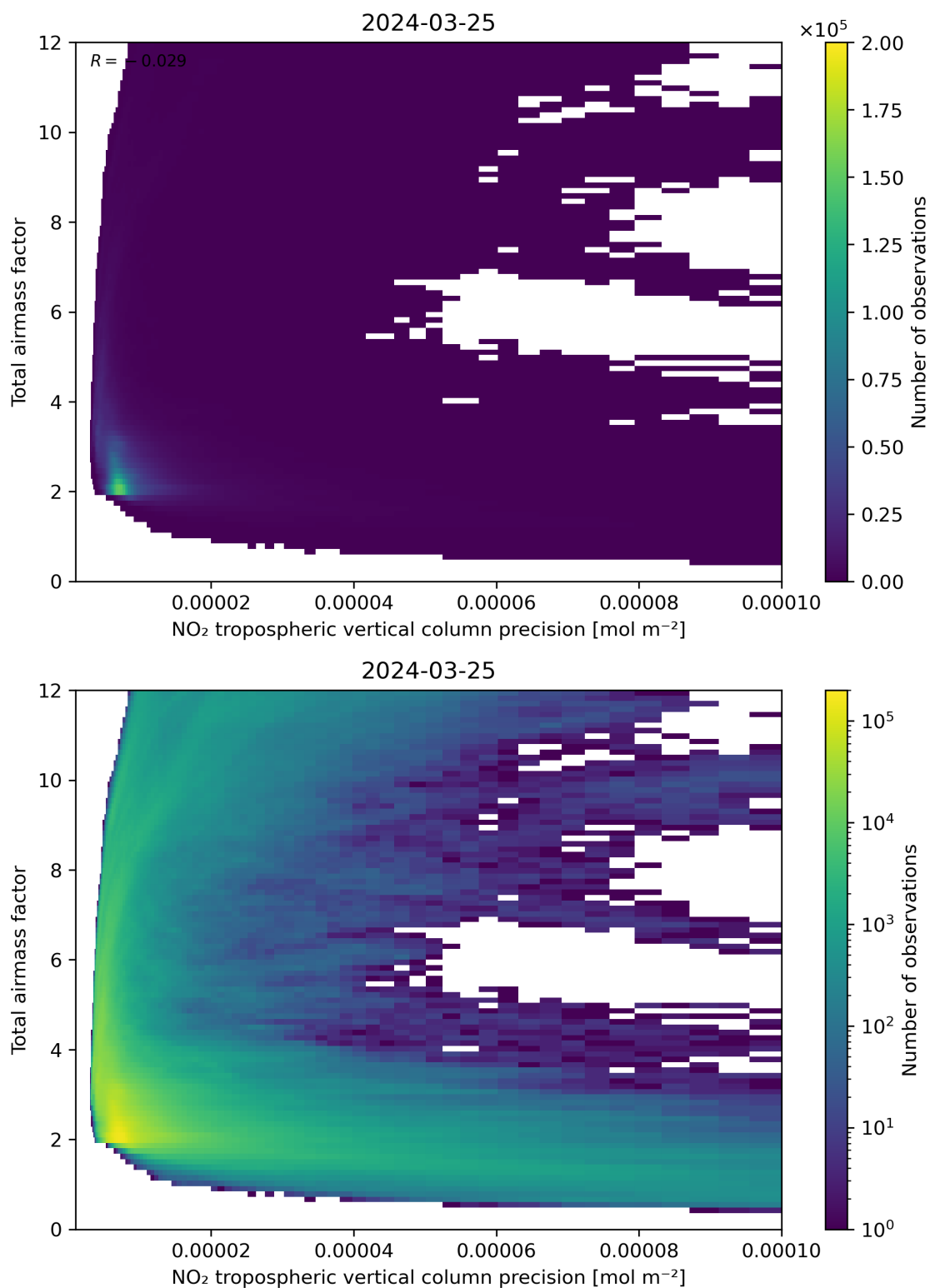
Figure 132: Scatter density plot of “NO 2 tropospheric vertical column precision” against “Total air mass factor” for 2024-03-25 to 2024-03-26.
