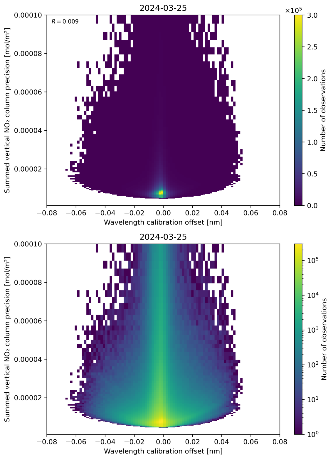
Figure 178: Scatter density plot of “Wavelength calibration offset” against “Summed vertical NO 2 column precision” for 2024-03-25 to 2024-03-26.
