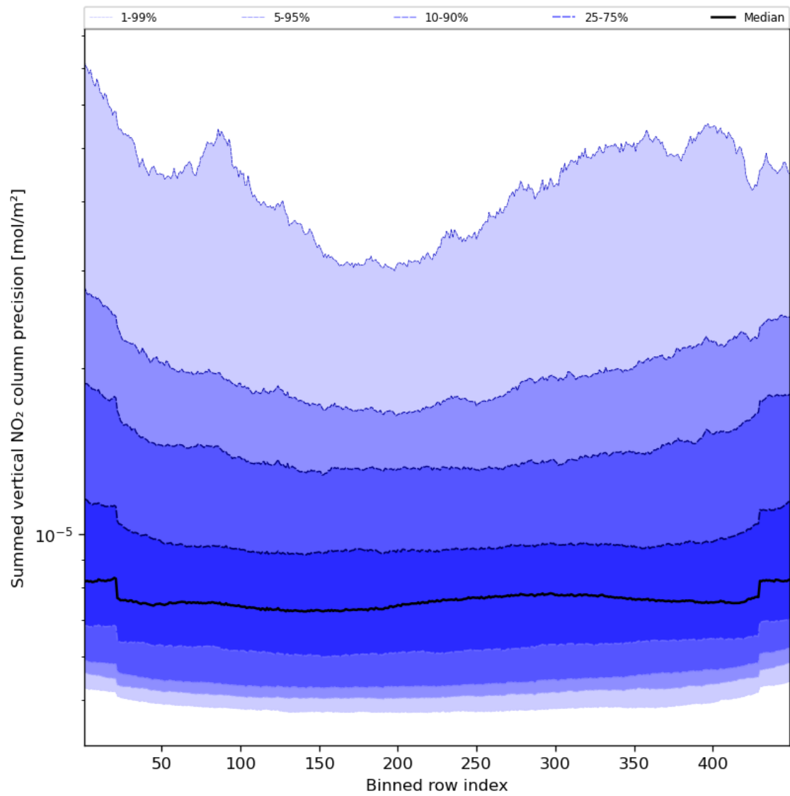
Figure 58: Along track statistics of “Summed vertical NO 2 column precision” for 2024-03-25 to 2024-03-26
