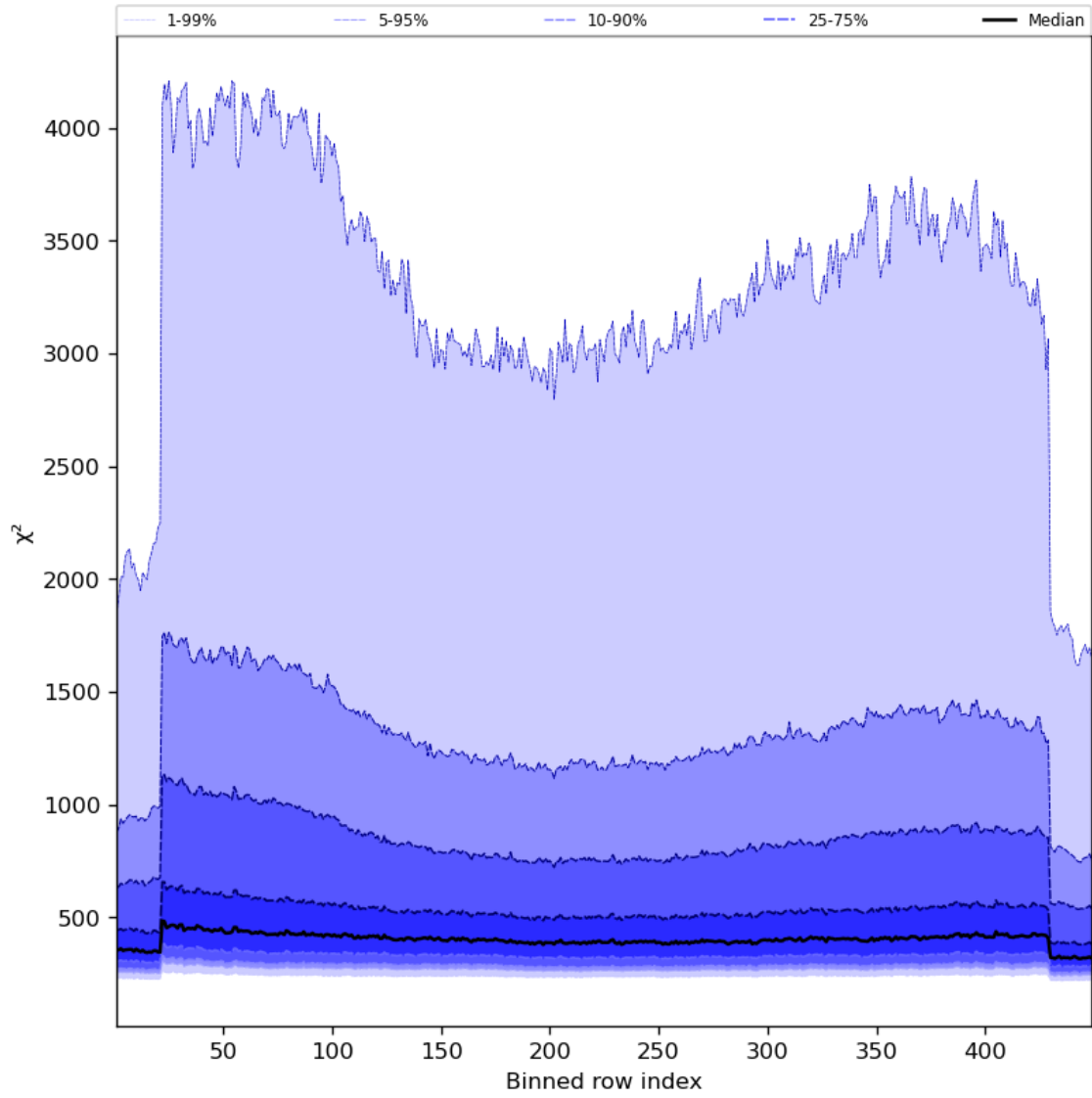
Figure 59: Along track statistics of “ \chi^2 ” for 2024-03-25 to 2024-03-26
