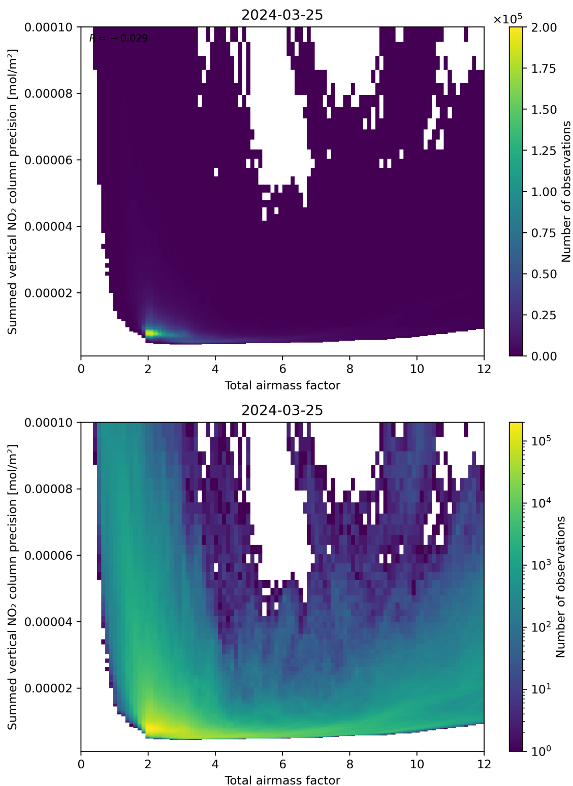
Figure 66: Scatter density plot of “Total airmass factor” against “Summed vertical NO 2 column precision” for 2024-03-25 to 2024-03-26.
