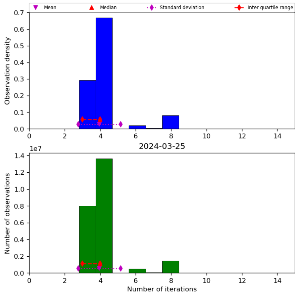
Figure 34: Histogram of “Number of iterations” for 2024-03-25 to 2024-03-26
