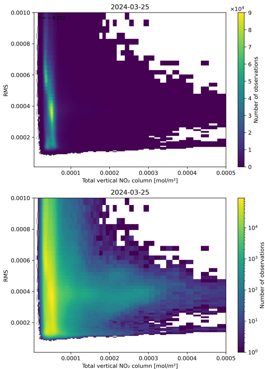
Figure 120: Scatter density plot of “Total vertical NO 2 column” against “RMS” for 2024-03-25 to 2024-03-26.
