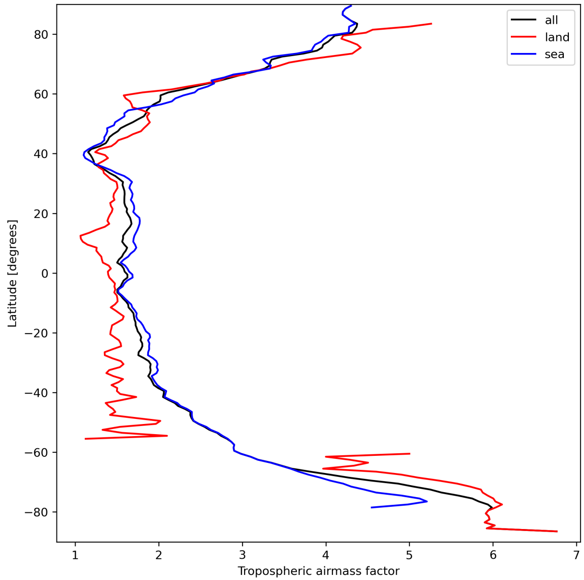
Figure 14: Zonal average of “Tropospheric airmass factor” for 2024-03-25 to 2024-03-26.
