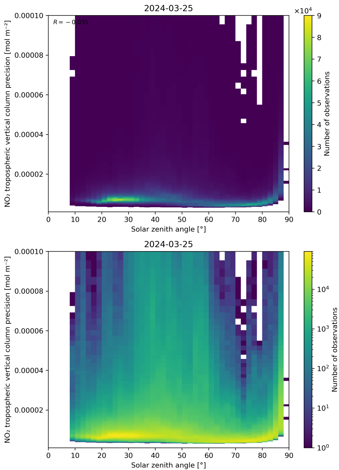
Figure 156: Scatter density plot of “Solar zenith angle” against “NO 2 tropospheric vertical column precision” for 2024-03-25 to 2024-03-26.
