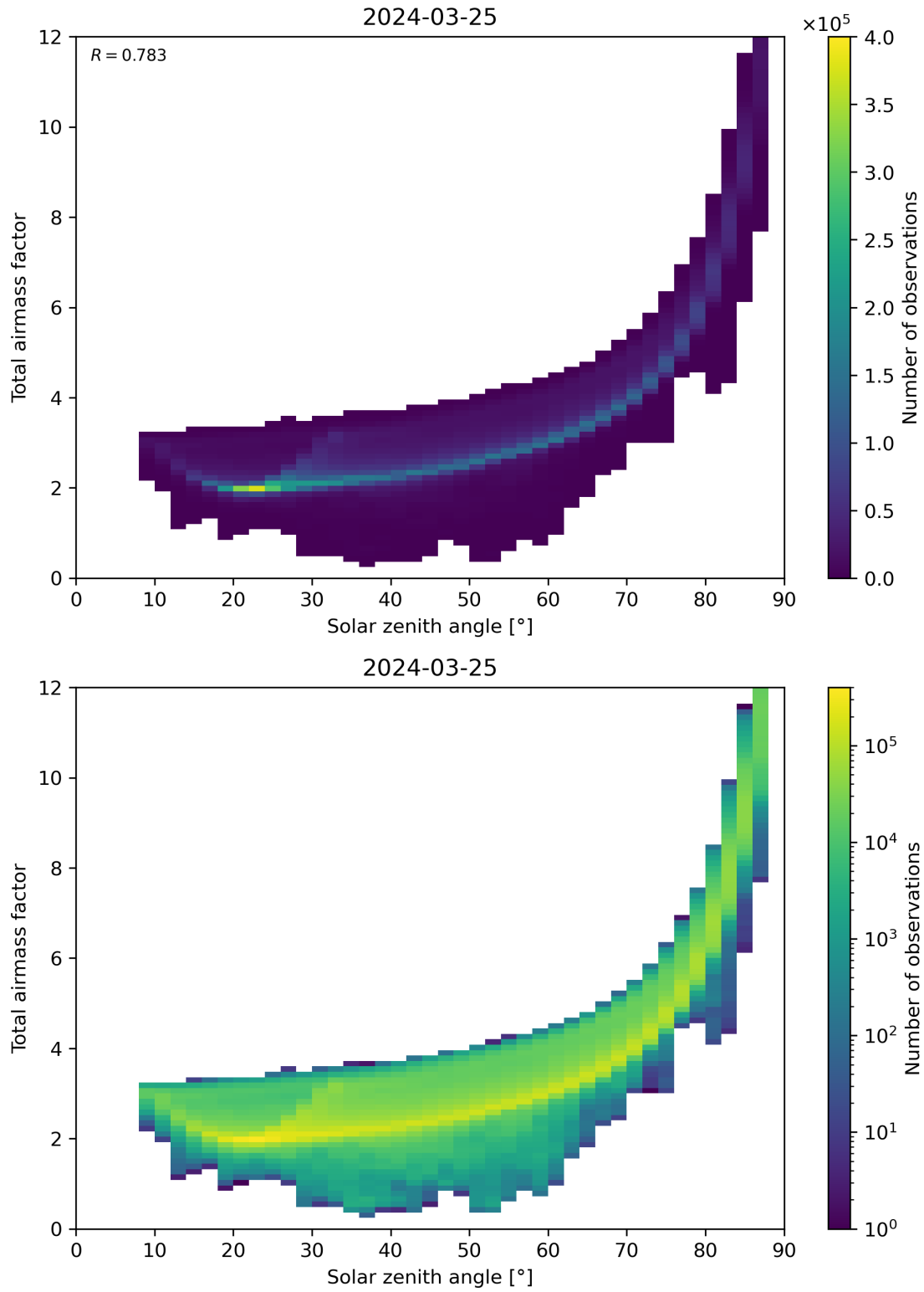
Figure 146: Scatter density plot of “Solar zenith angle” against “Total air mass factor” for 2024-03-25 to 2024-03-26.
