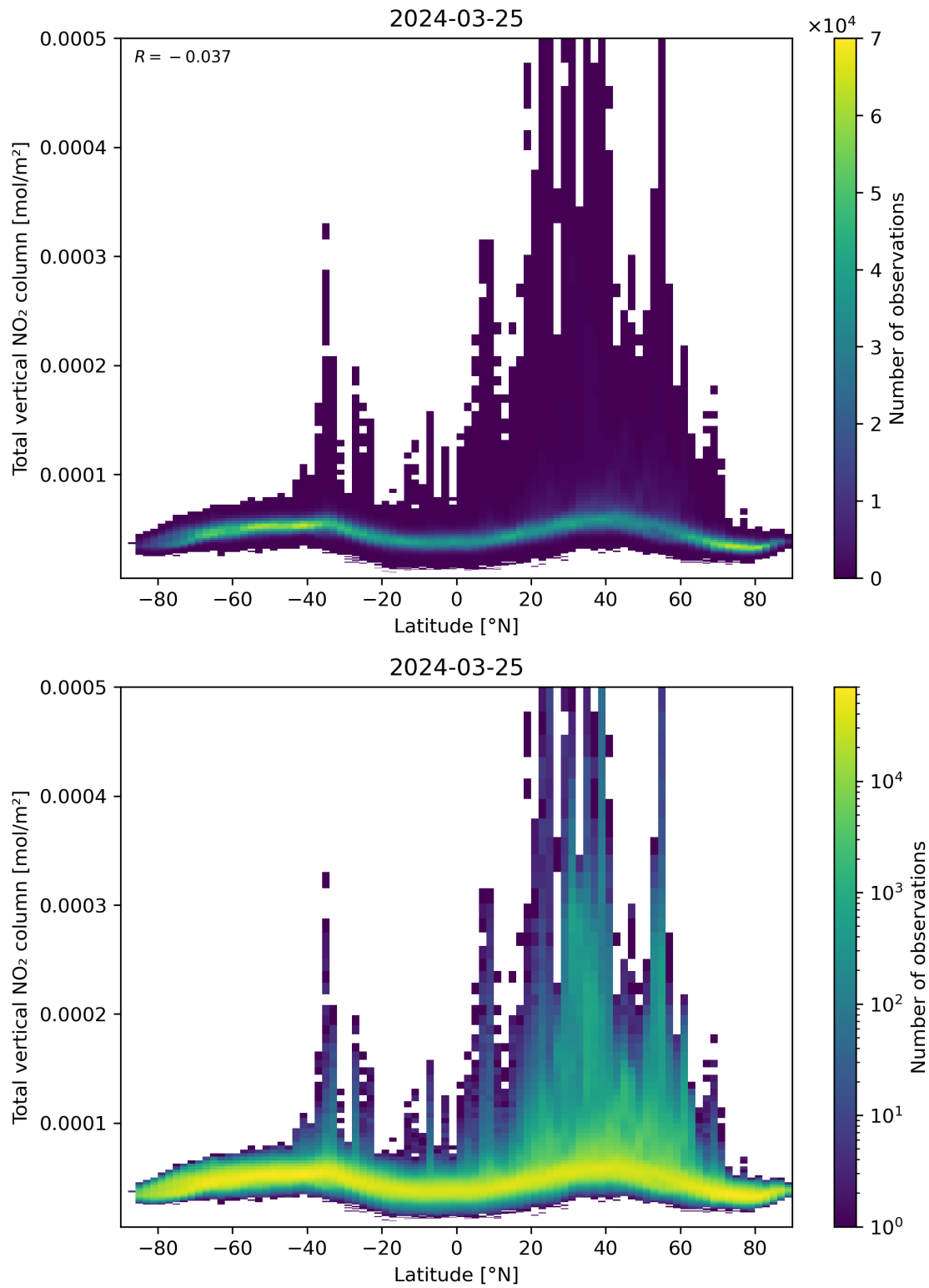
Figure 90: Scatter density plot of “Latitude” against “Total vertical NO 2 column” for 2024-03-25 to 2024-03-26.
