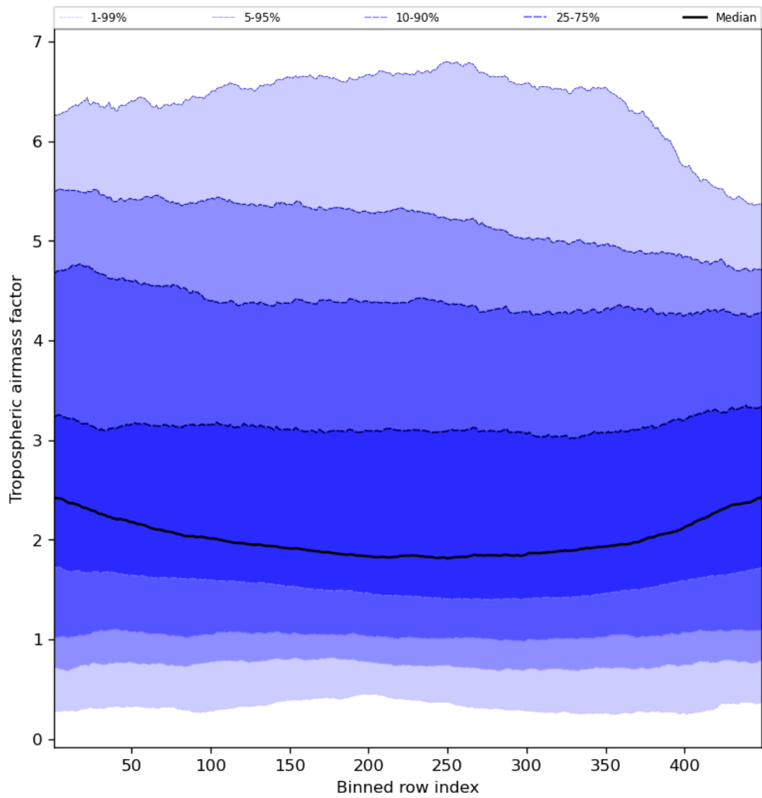
Figure 48: Along track statistics of “Tropospheric air mass factor” for 2024-03-25 to 2024-03-26
