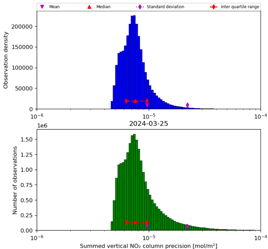
Figure 41: Histogram of “Summed vertical NO 2 column precision” for 2024-03-25 to 2024-03-26
