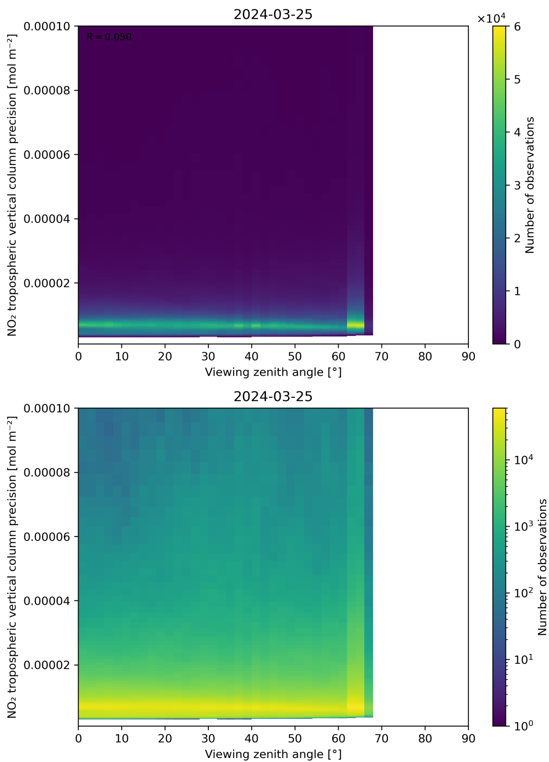
Figure 170: Scatter density plot of “Viewing zenith angle” against “NO 2 tropospheric vertical column precision” for 2024-03-25 to 2024-03-26.
