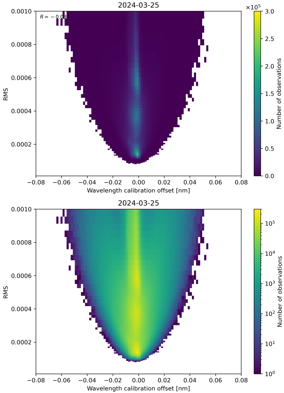
Figure 181: Scatter density plot of “Wavelength calibration offset” against “RMS” for 2024-03-25 to 2024-03-26.
