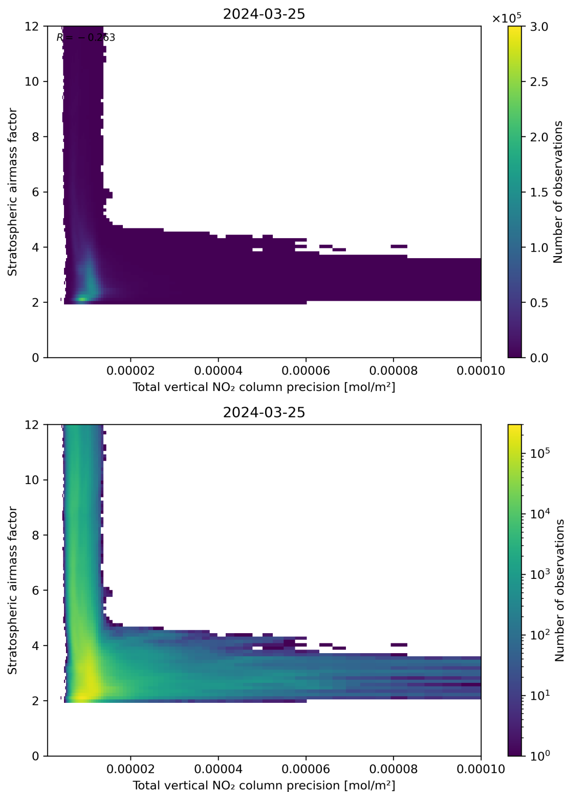
Figure 115: Scatter density plot of “Total vertical NO 2 column precision” against “Stratospheric air mass factor” for 2024-03-25 to 2024-03-26.
