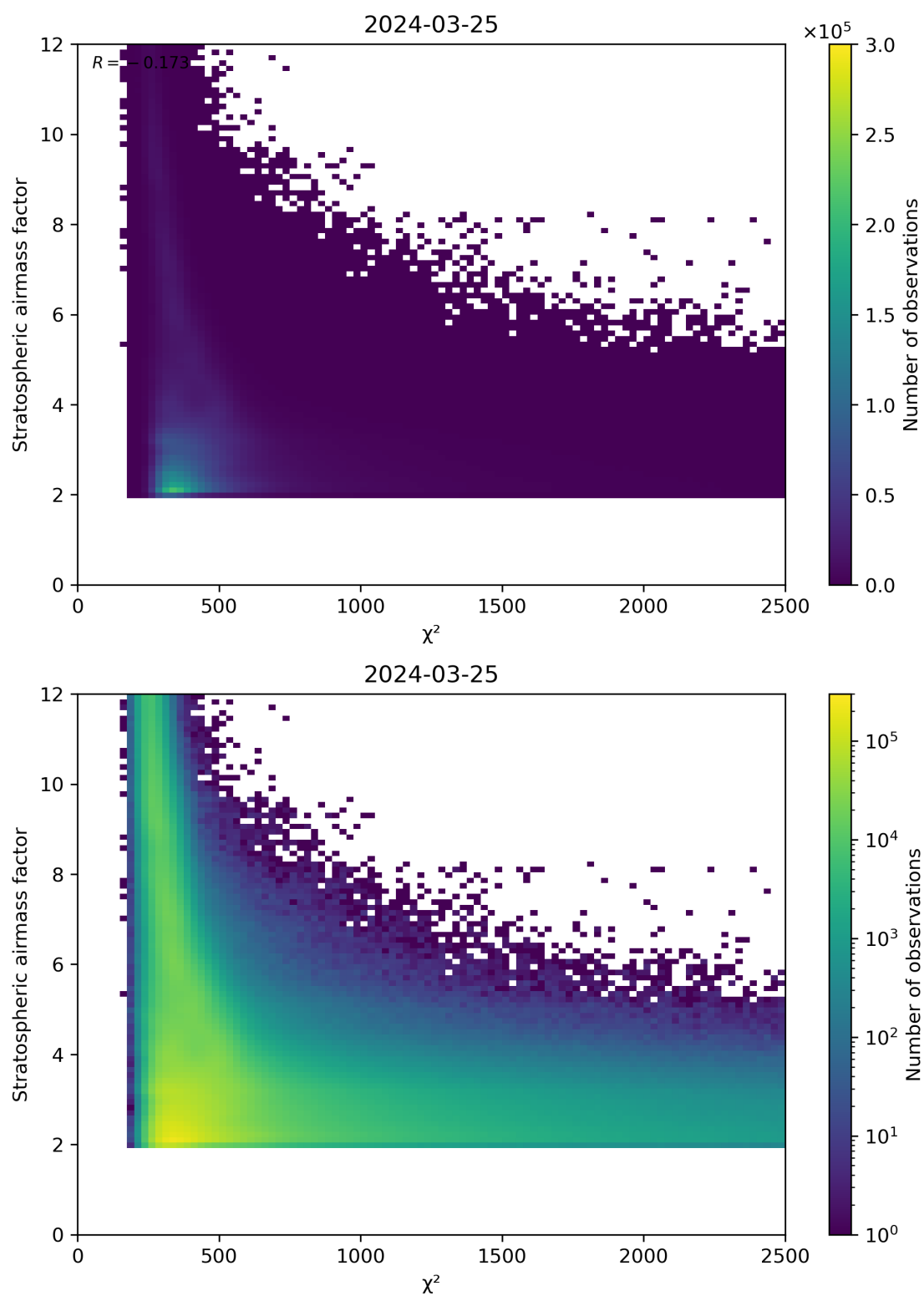
Figure 81: Scatter density plot of “ \chi^2 ” against “Stratospheric airmass factor” for 2024-03-25 to 2024-03-26.
