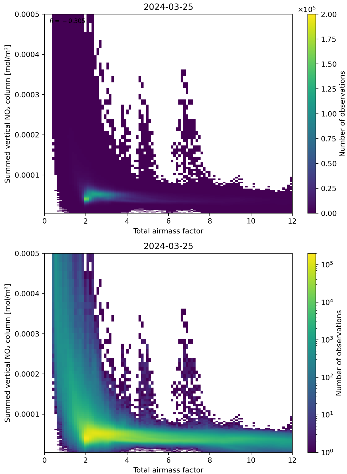
Figure 65: Scatter density plot of “Total airmass factor” against “Summed vertical NO 2 column” for 2024-03-25 to 2024-03-26.
