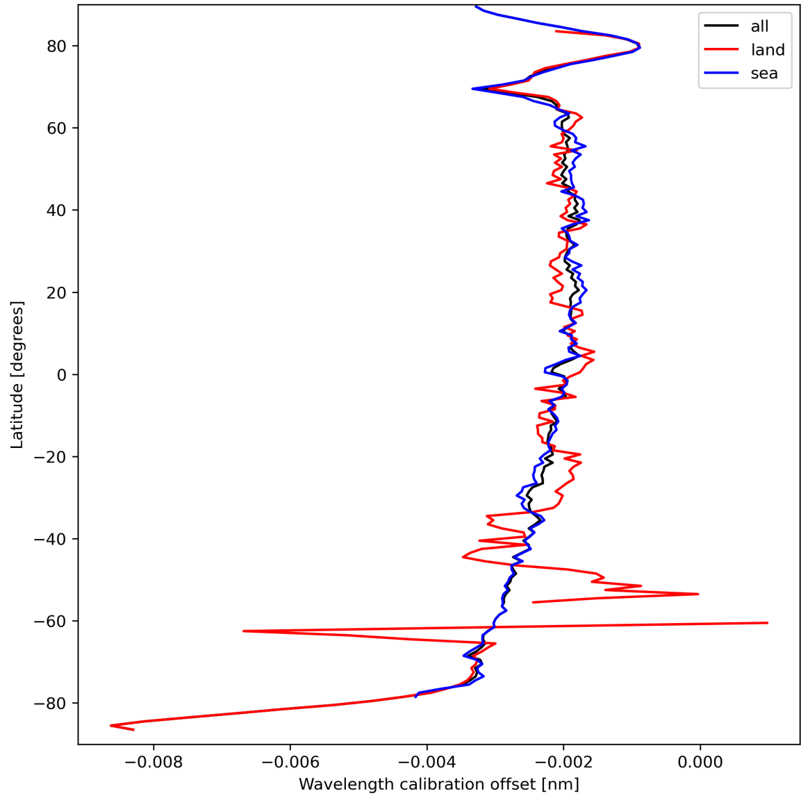
Figure 18: Zonal average of “Wavelength calibration offset” for 2024-03-25 to 2024-03-26.
