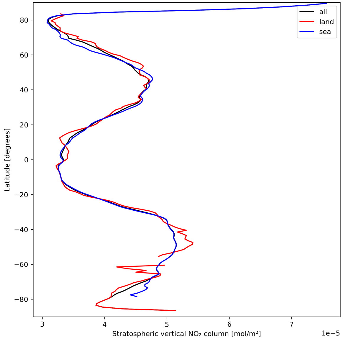
Figure 19: Zonal average of “Stratospheric vertical NO 2 column” for 2024-03-25 to 2024-03-26.
