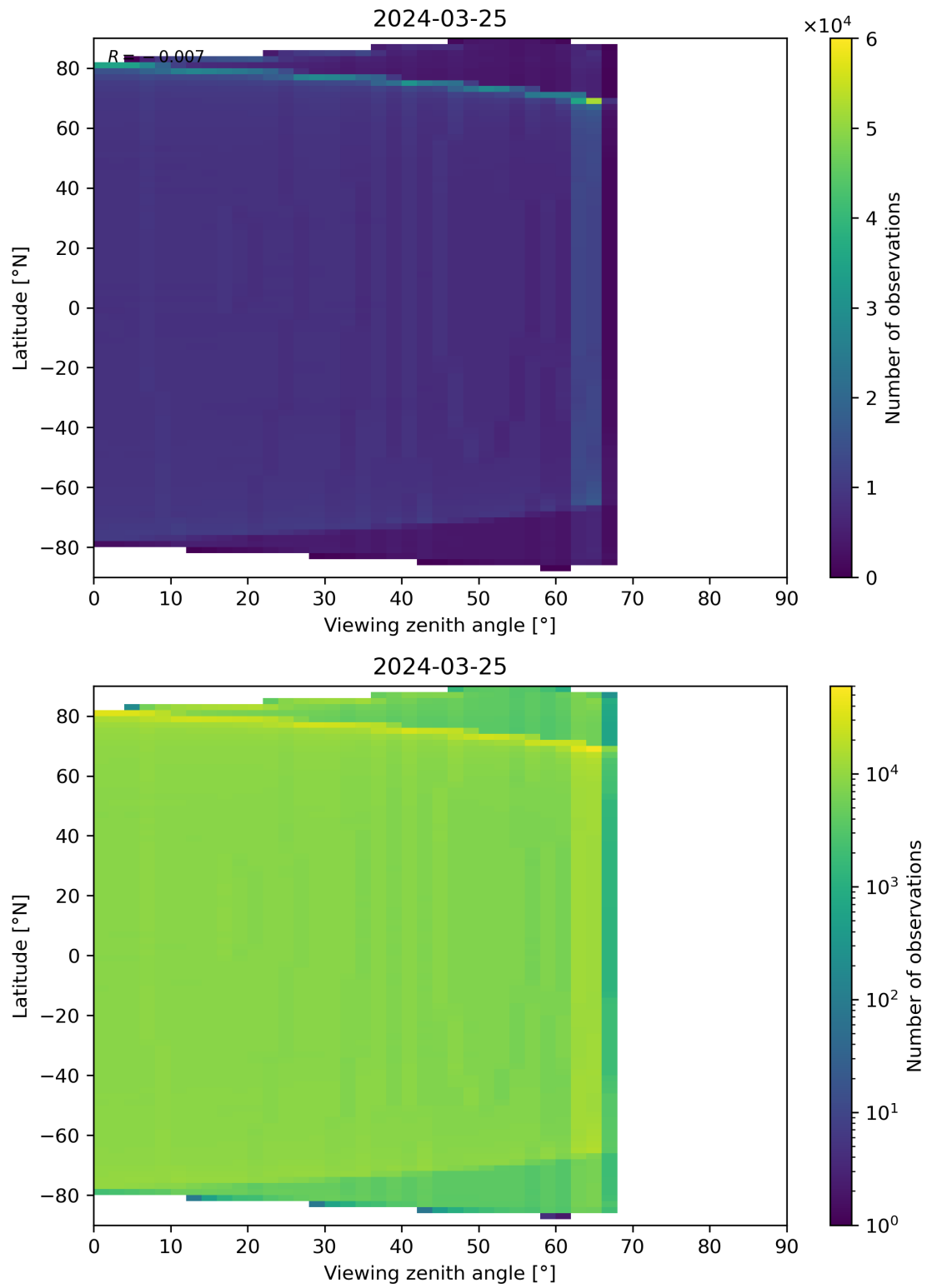
Figure 163: Scatter density plot of “Viewing zenith angle” against “Latitude” for 2024-03-25 to 2024-03-26.
