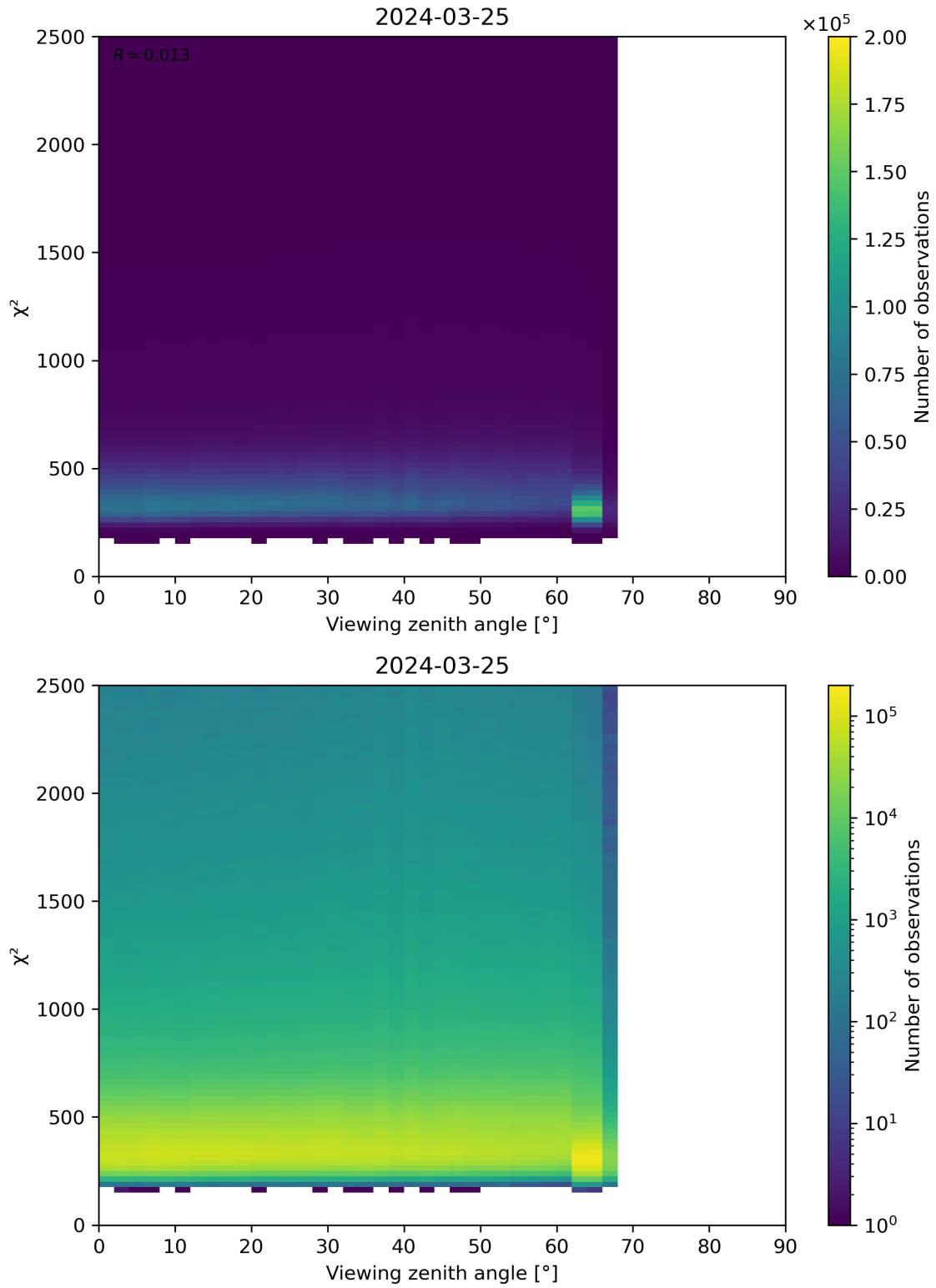
Figure 162: Scatter density plot of “Viewing zenith angle” against “ \chi^2 ” for 2024-03-25 to 2024-03-26.
