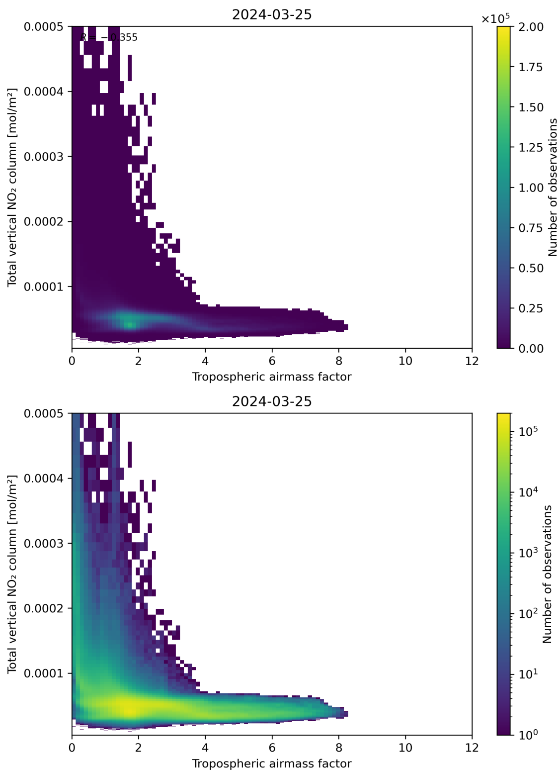
Figure 77: Scatter density plot of “Tropospheric airmass factor” against “Total vertical NO 2 column” for 2024-03-25 to 2024-03-26.
