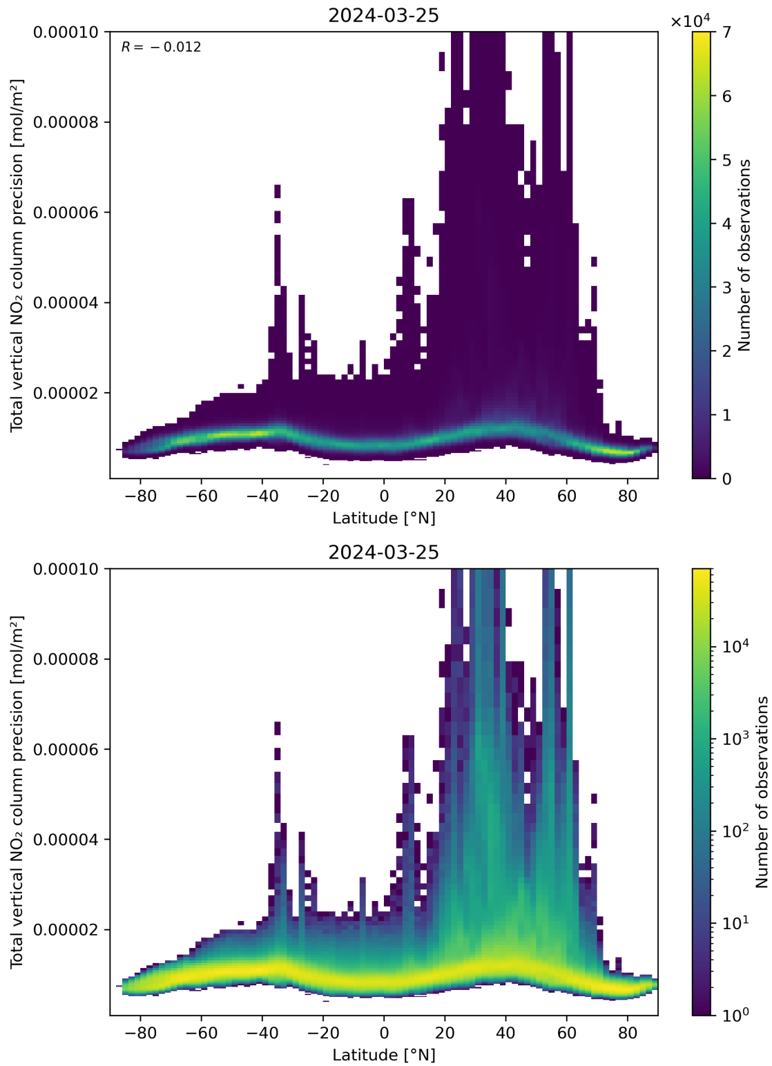
Figure 91: Scatter density plot of “Latitude” against “Total vertical NO 2 column precision” for 2024-03-25 to 2024-03-26.
