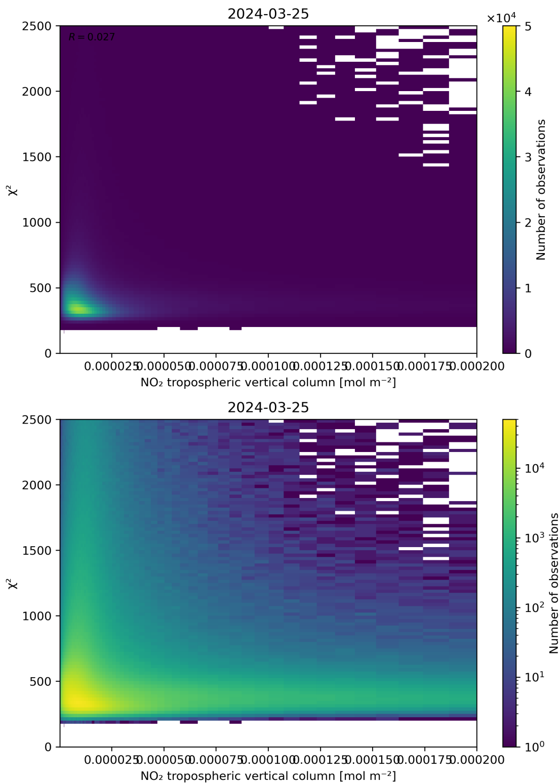
Figure 124: Scatter density plot of “NO 2 tropospheric vertical column” against “ \chi^2 ” for 2024-03-25 to 2024-03-26.
