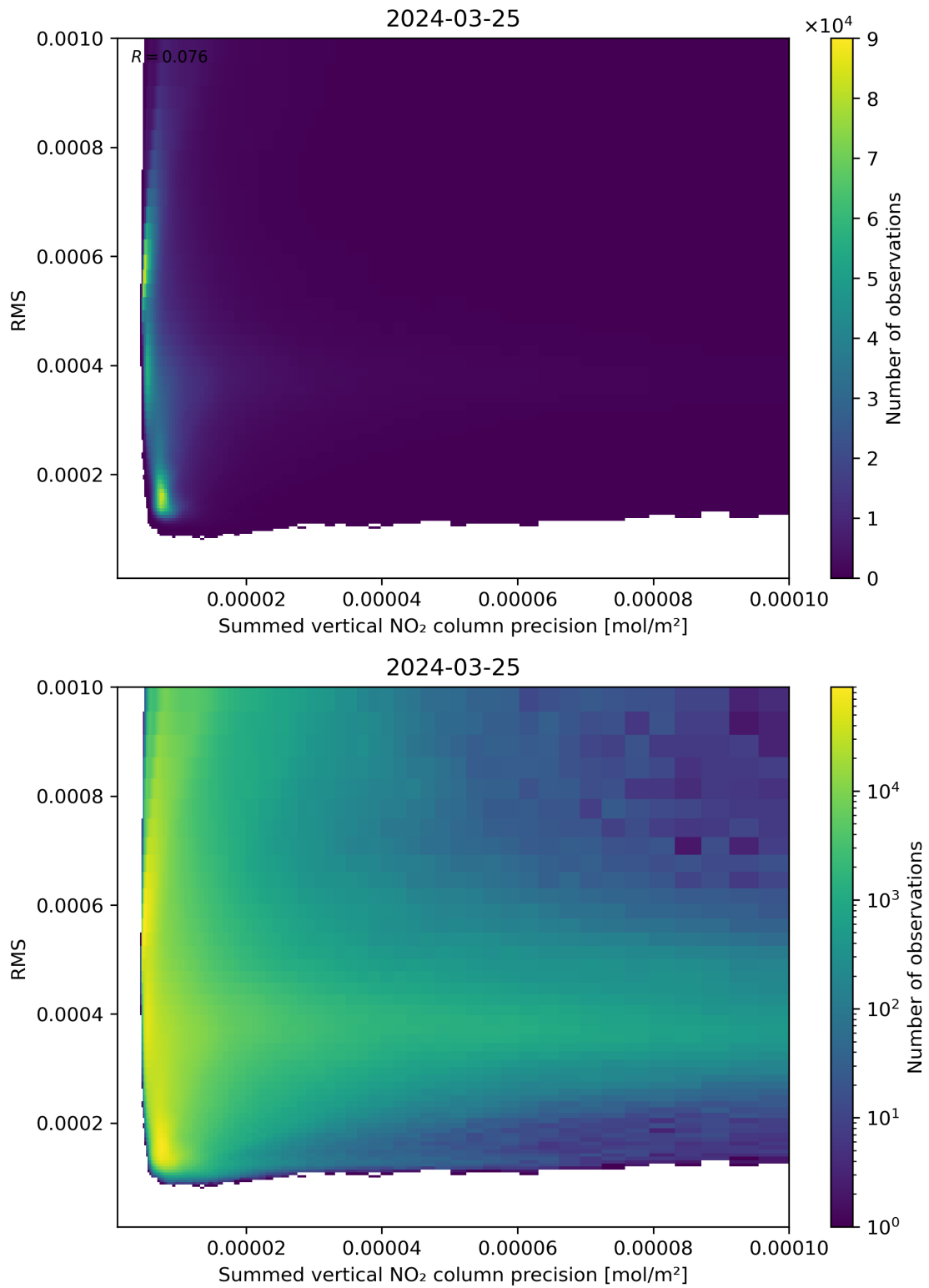
Figure 108: Scatter density plot of “Summed vertical NO 2 column precision” against “RMS” for 2024-03-25 to 2024-03-26.
