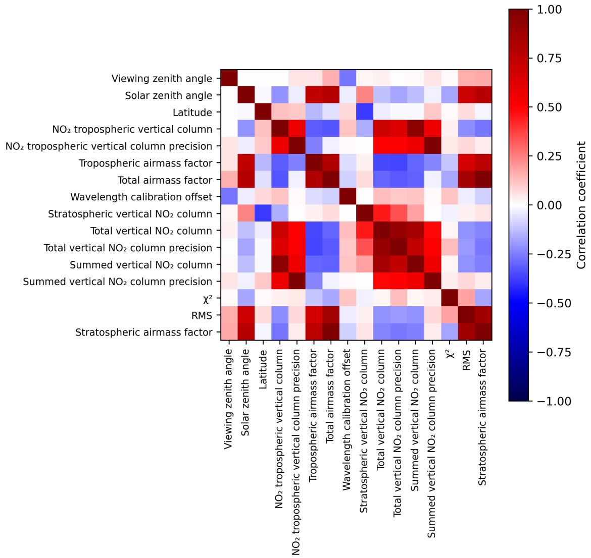
Figure 2: Map of correlation matrix for 2024-03-25 to 2024-03-26.
