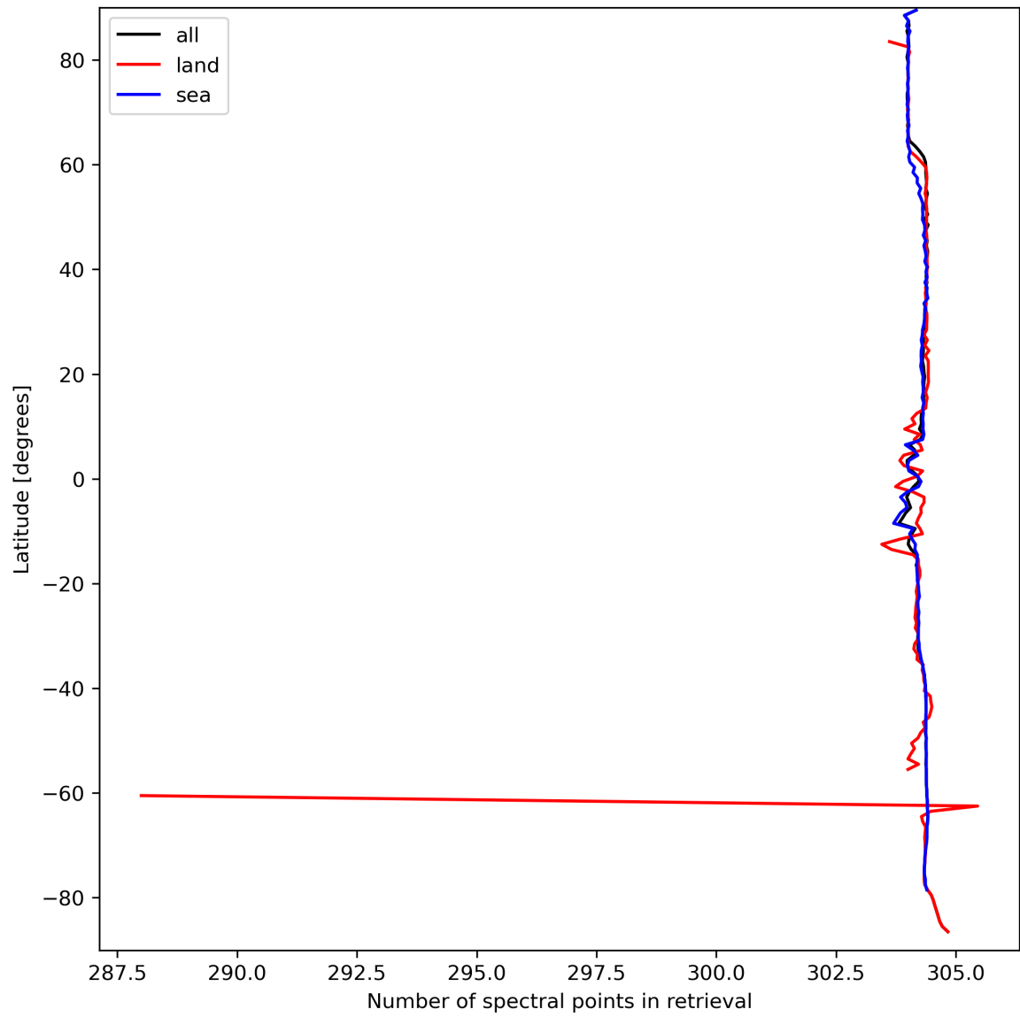
Figure 16: Zonal average of “Number of spectral points in retrieval” for 2024-03-25 to 2024-03-26.
