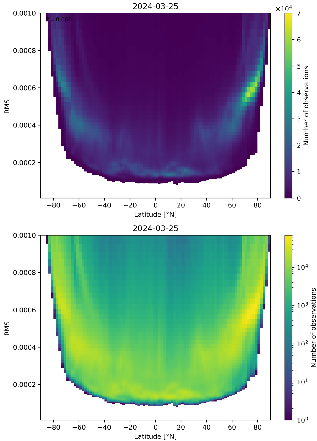
Figure 94: Scatter density plot of “Latitude” against “RMS” for 2024-03-25 to 2024-03-26.
