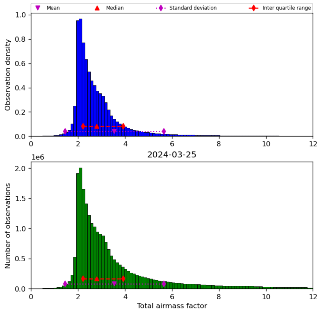
Figure 32: Histogram of “Total airmass factor” for 2024-03-25 to 2024-03-26
