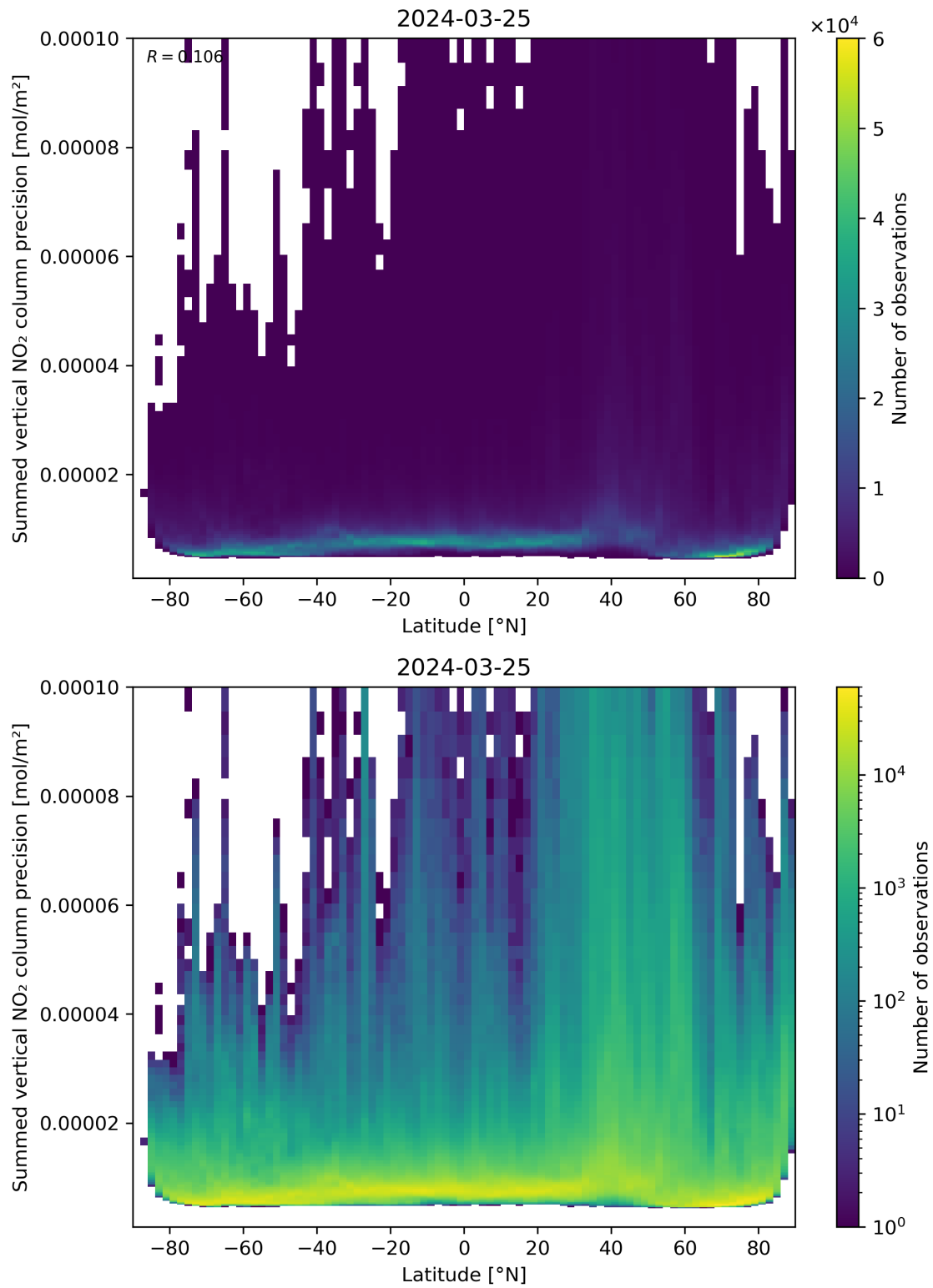
Figure 89: Scatter density plot of “Latitude” against “Summed vertical NO 2 column precision” for 2024-03-25 to 2024-03-26.
