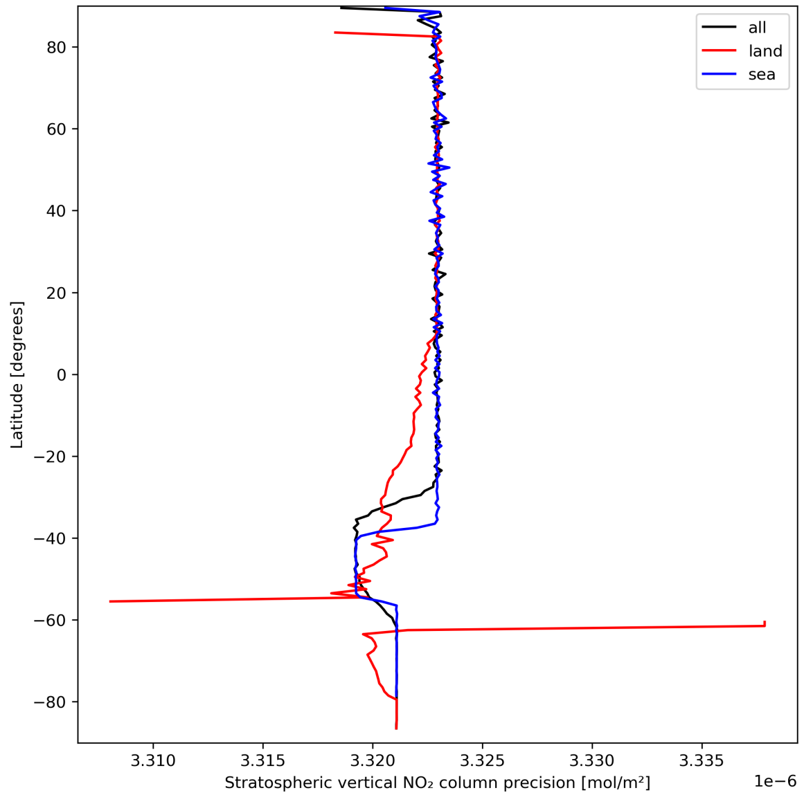
Figure 20: Zonal average of “Stratospheric vertical NO 2 column precision” for 2024-03-25 to 2024-03-26.
