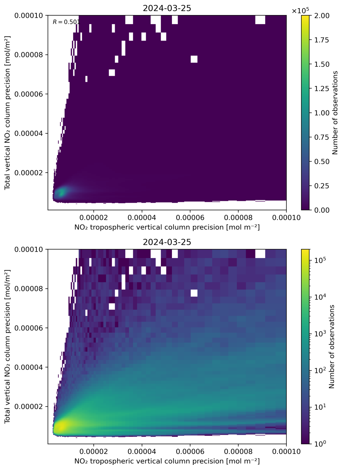
Figure 139: Scatter density plot of “NO 2 tropospheric vertical column precision” against “Total vertical NO 2 column precision” for 2024-03-25 to 2024-03-26.
