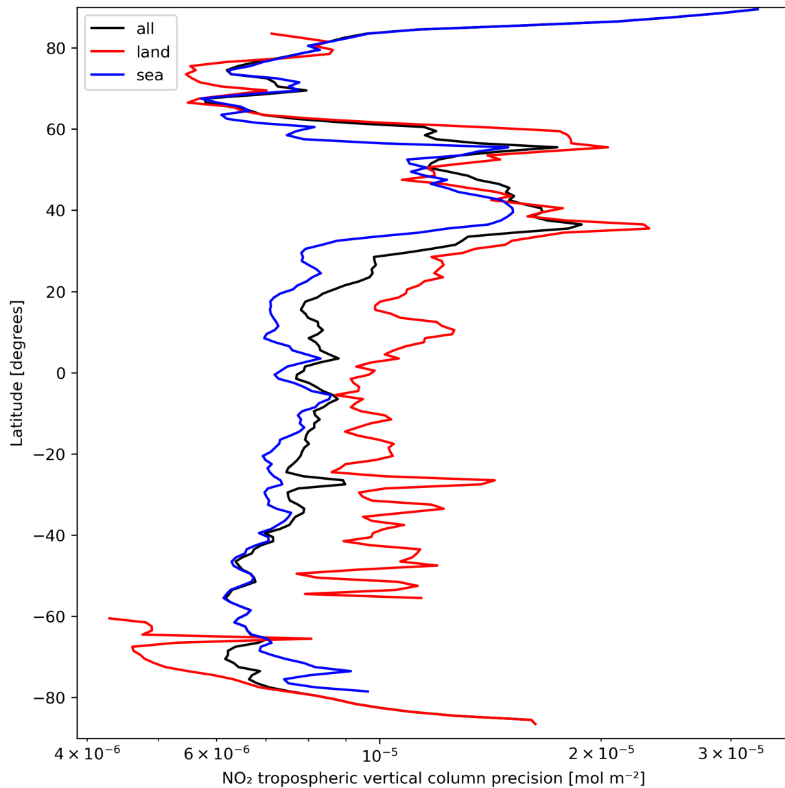
Figure 13: Zonal average of “NO 2 tropospheric vertical column precision” for 2024-03-25 to 2024-03-26.
