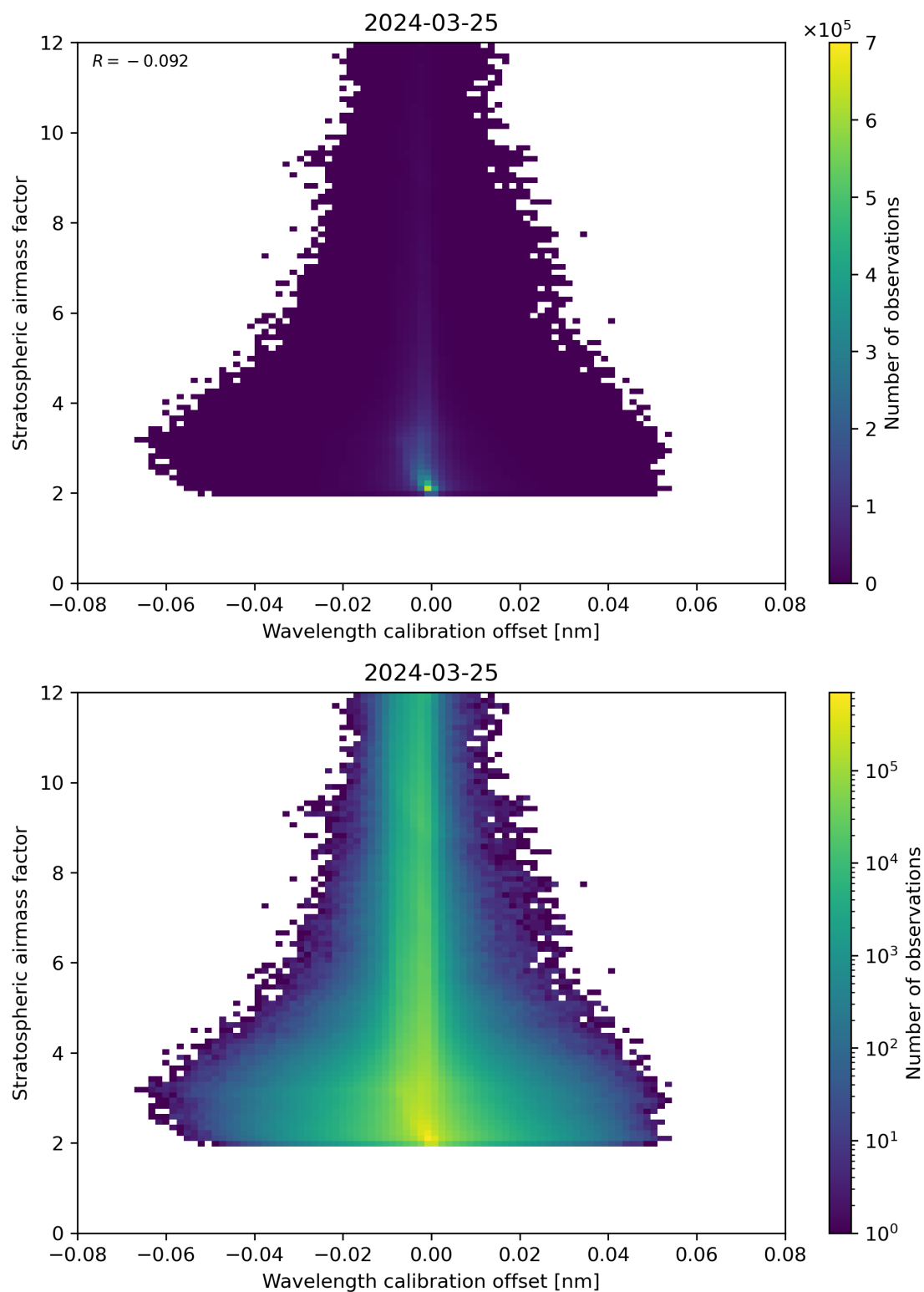
Figure 174: Scatter density plot of “Wavelength calibration offset” against “Stratospheric air mass factor” for 2024-03-25 to 2024-03-26.
