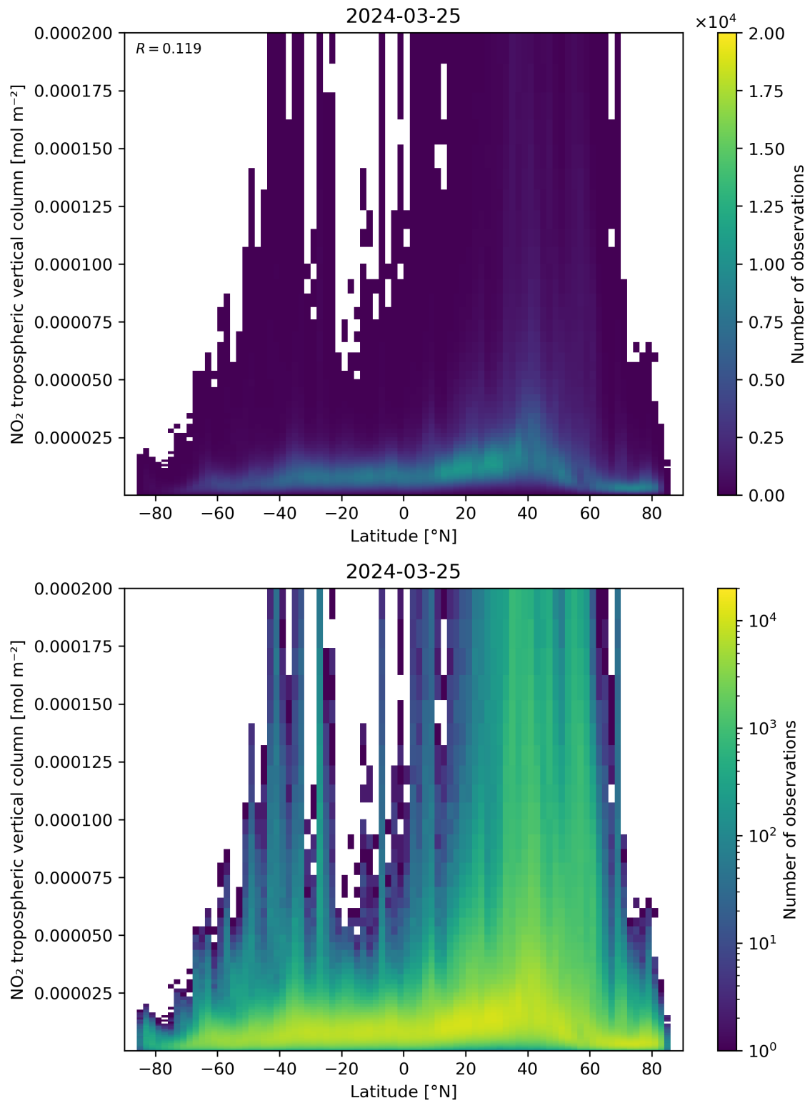
Figure 92: Scatter density plot of “Latitude” against “NO 2 tropospheric vertical column” for 2024-03-25 to 2024-03-26.
