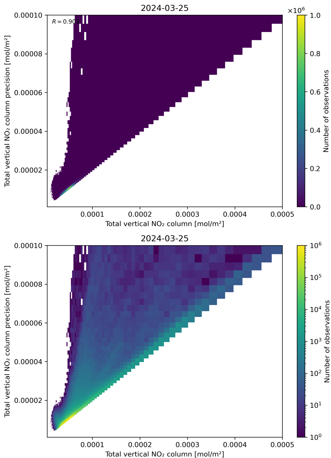
Figure 114: Scatter density plot of “Total vertical NO 2 column” against “Total vertical NO 2 column precision” for 2024-03-25 to 2024-03-26.
