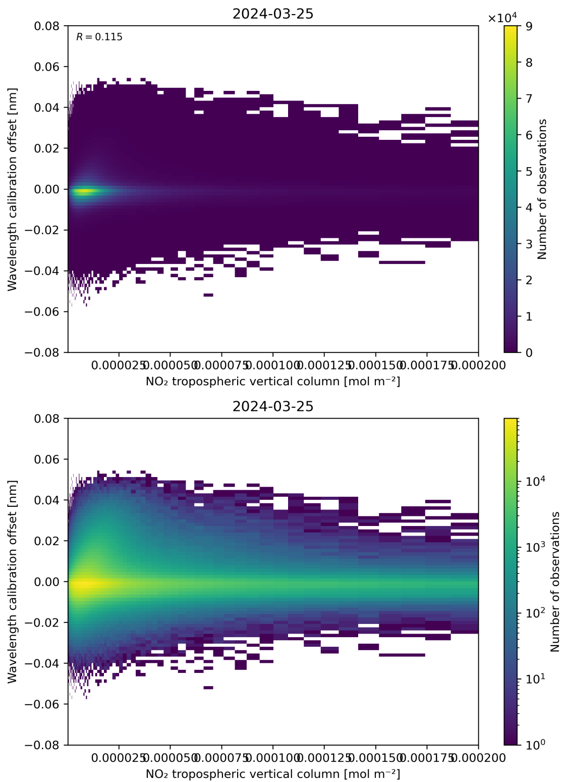
Figure 143: Scatter density plot of “NO 2 tropospheric vertical column” against “Wavelength calibration offset” for 2024-03-25 to 2024-03-26.
