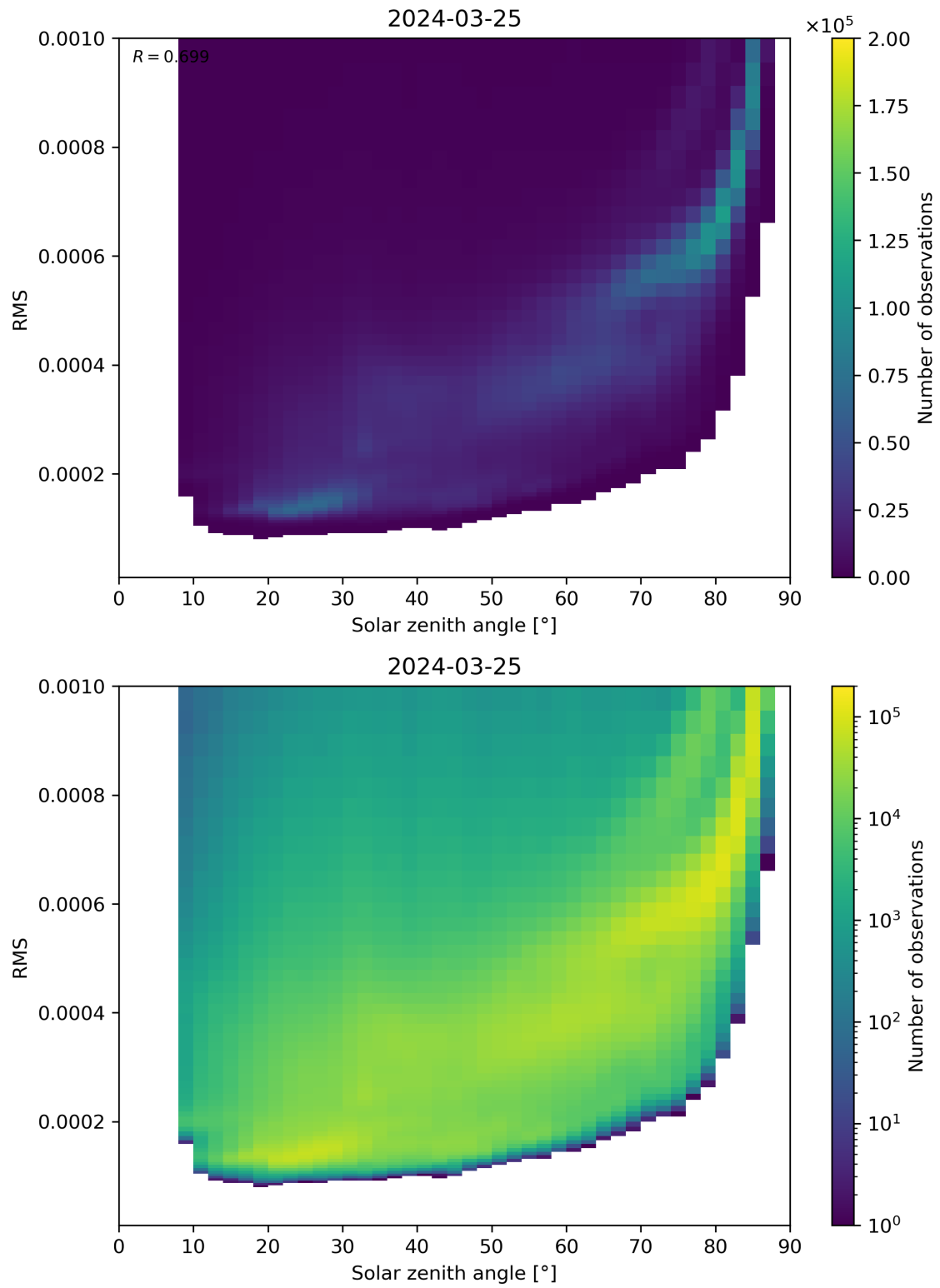
Figure 157: Scatter density plot of “Solar zenith angle” against “RMS” for 2024-03-25 to 2024-03-26.
