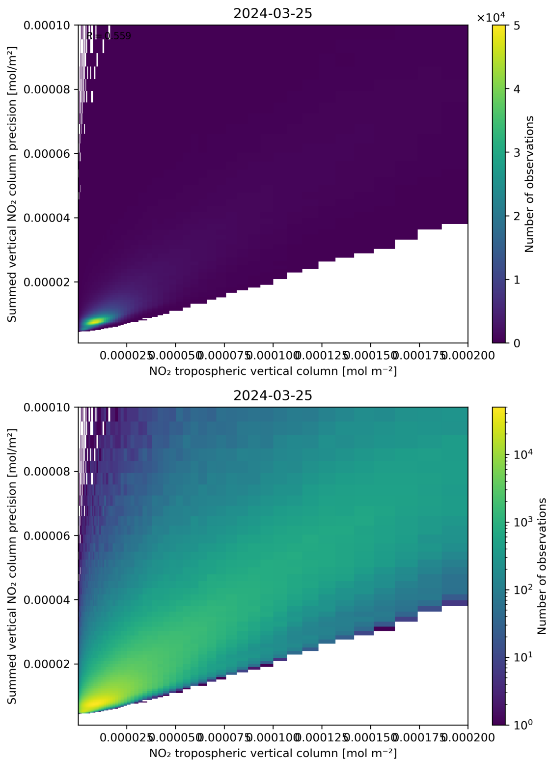
Figure 127: Scatter density plot of “NO 2 tropospheric vertical column” against “Summed vertical NO 2 column precision” for 2024-03-25 to 2024-03-26.
