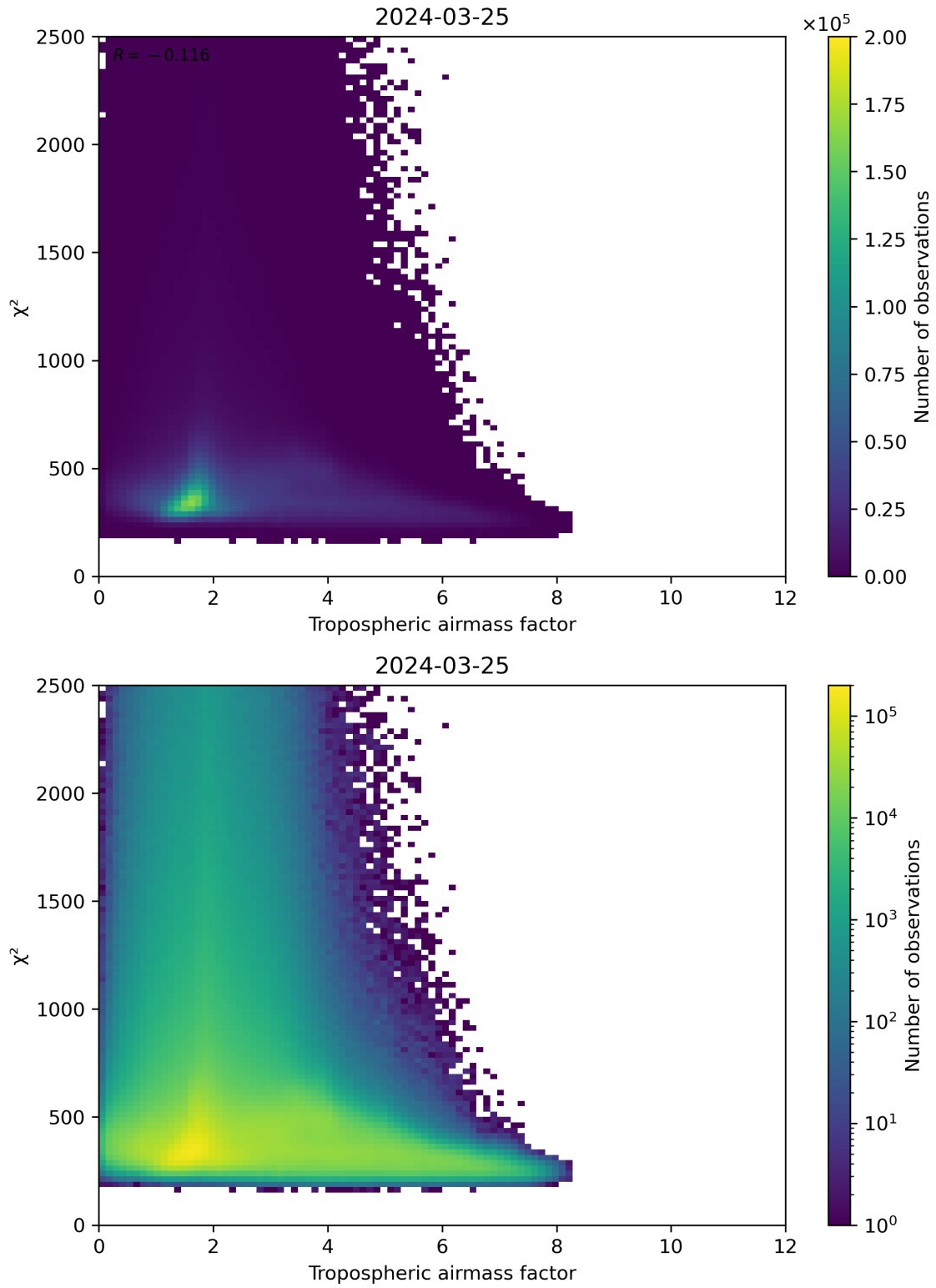
Figure 73: Scatter density plot of “Tropospheric airmass factor” against “ \chi^2 ” for 2024-03-25 to 2024-03-26.
