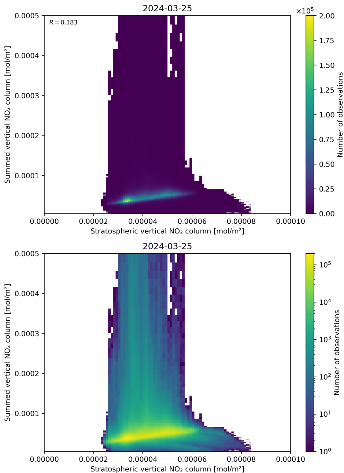
Figure 98: Scatter density plot of “Stratospheric vertical NO 2 column” against “Summed vertical NO 2 column” for 2024-03-25 to 2024-03-26.
