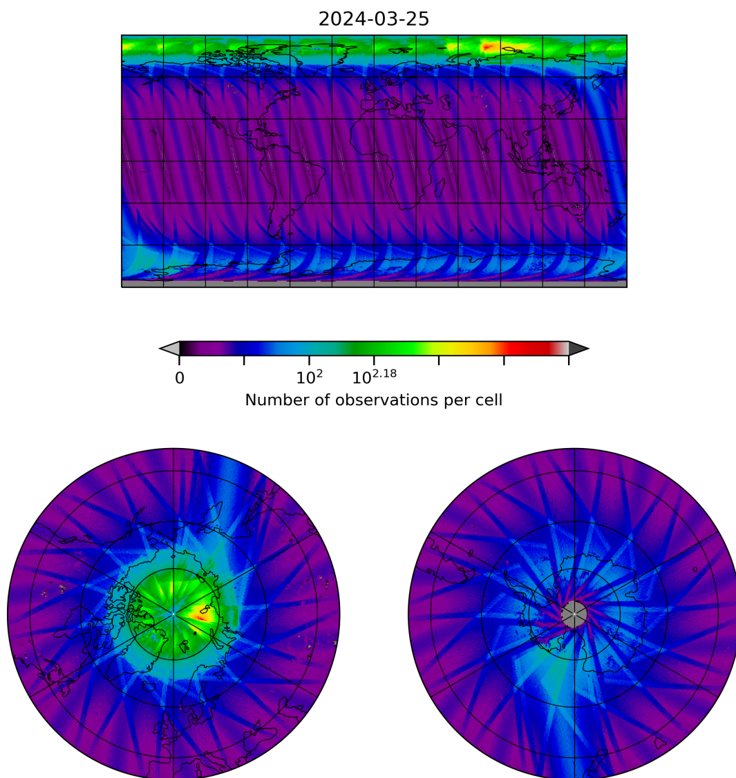
Figure 10: Map of the number of observations for 2024-03-25 to 2024-03-26
