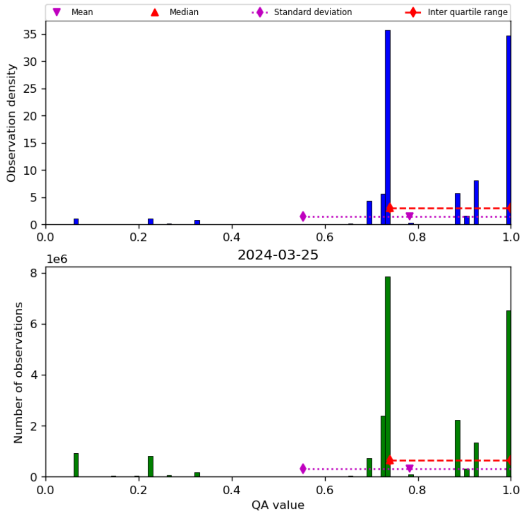
Figure 28: Histogram of “QA value” for 2024-03-25 to 2024-03-26
