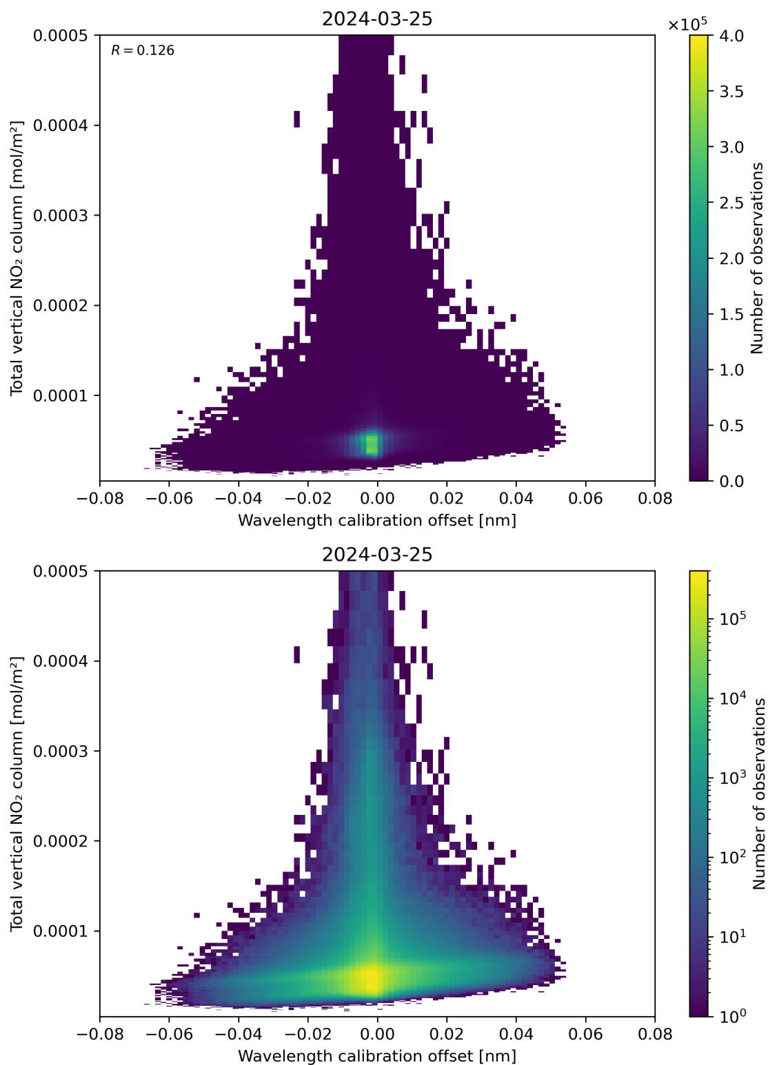
Figure 179: Scatter density plot of “Wavelength calibration offset” against “Total vertical NO 2 column” for 2024-03-25 to 2024-03-26.
