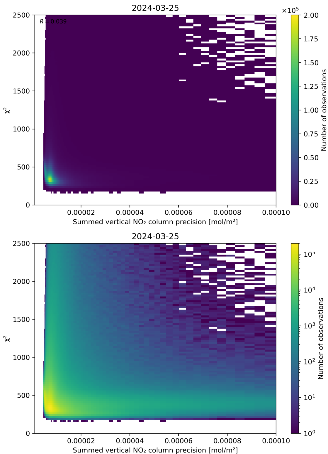
Figure 107: Scatter density plot of “Summed vertical NO 2 column precision” against “ \chi^2 ” for 2024-03-25 to 2024-03-26.
