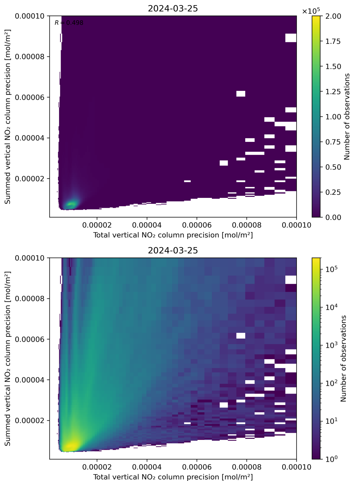
Figure 118: Scatter density plot of “Total vertical NO 2 column precision” against “Summed vertical NO 2 column precision” for 2024-03-25 to 2024-03-26.
