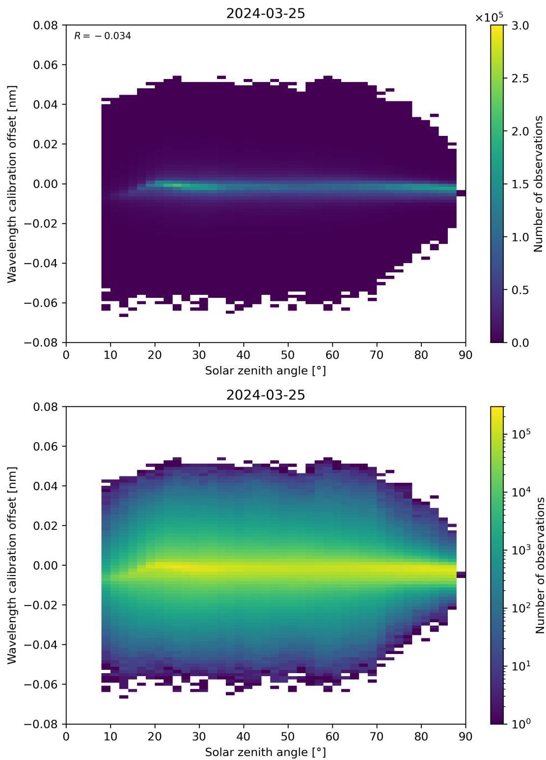
Figure 158: Scatter density plot of “Solar zenith angle” against “Wavelength calibration offset” for 2024-03-25 to 2024-03-26.
