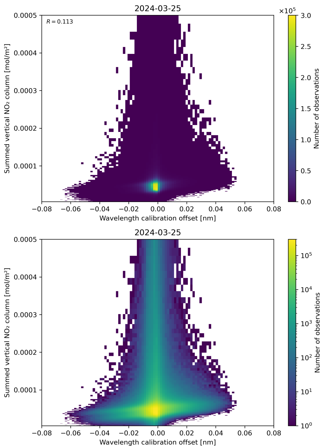
Figure 177: Scatter density plot of “Wavelength calibration offset” against “Summed vertical NO 2 column” for 2024-03-25 to 2024-03-26.
