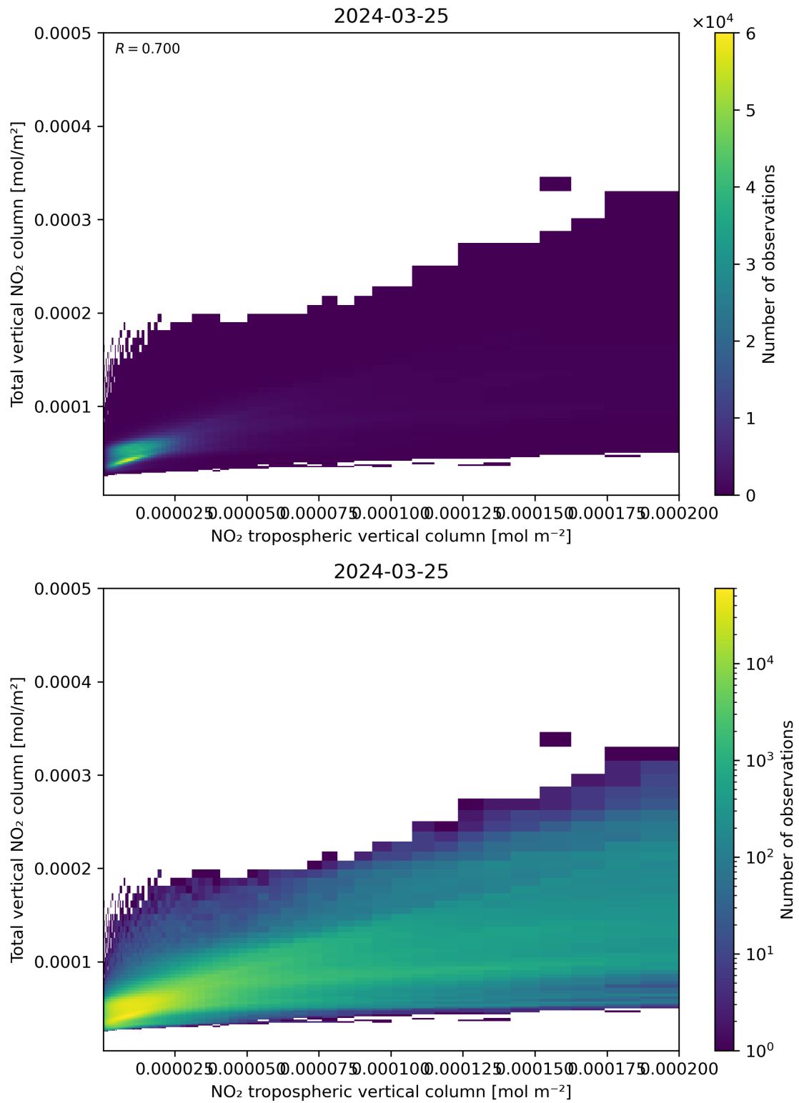
Figure 128: Scatter density plot of “NO 2 tropospheric vertical column” against “Total vertical NO 2 column” for 2024-03-25 to 2024-03-26.
