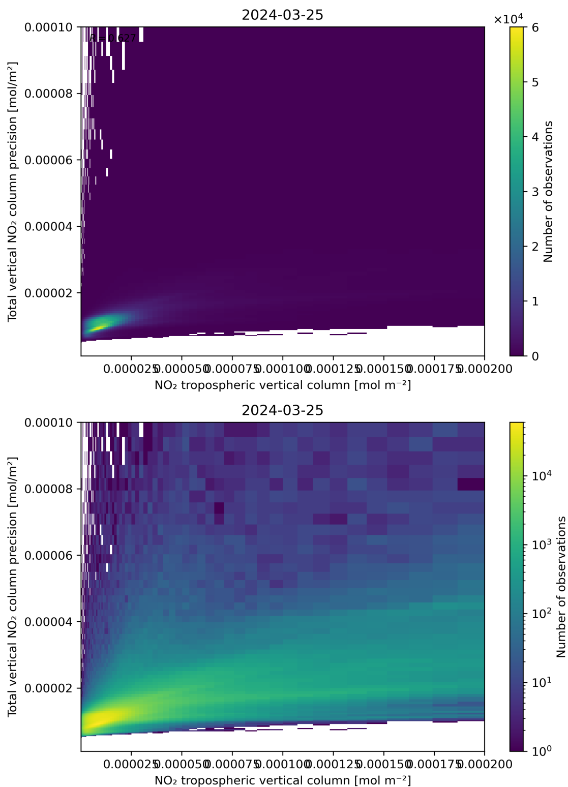
Figure 129: Scatter density plot of “NO 2 tropospheric vertical column” against “Total vertical NO 2 column precision” for 2024-03-25 to 2024-03-26.
