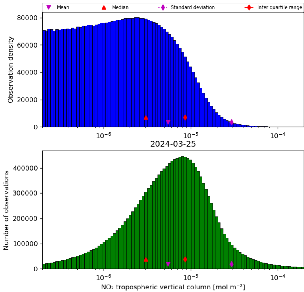
Figure 29: Histogram of “NO 2 tropospheric vertical column” for 2024-03-25 to 2024-03-26
