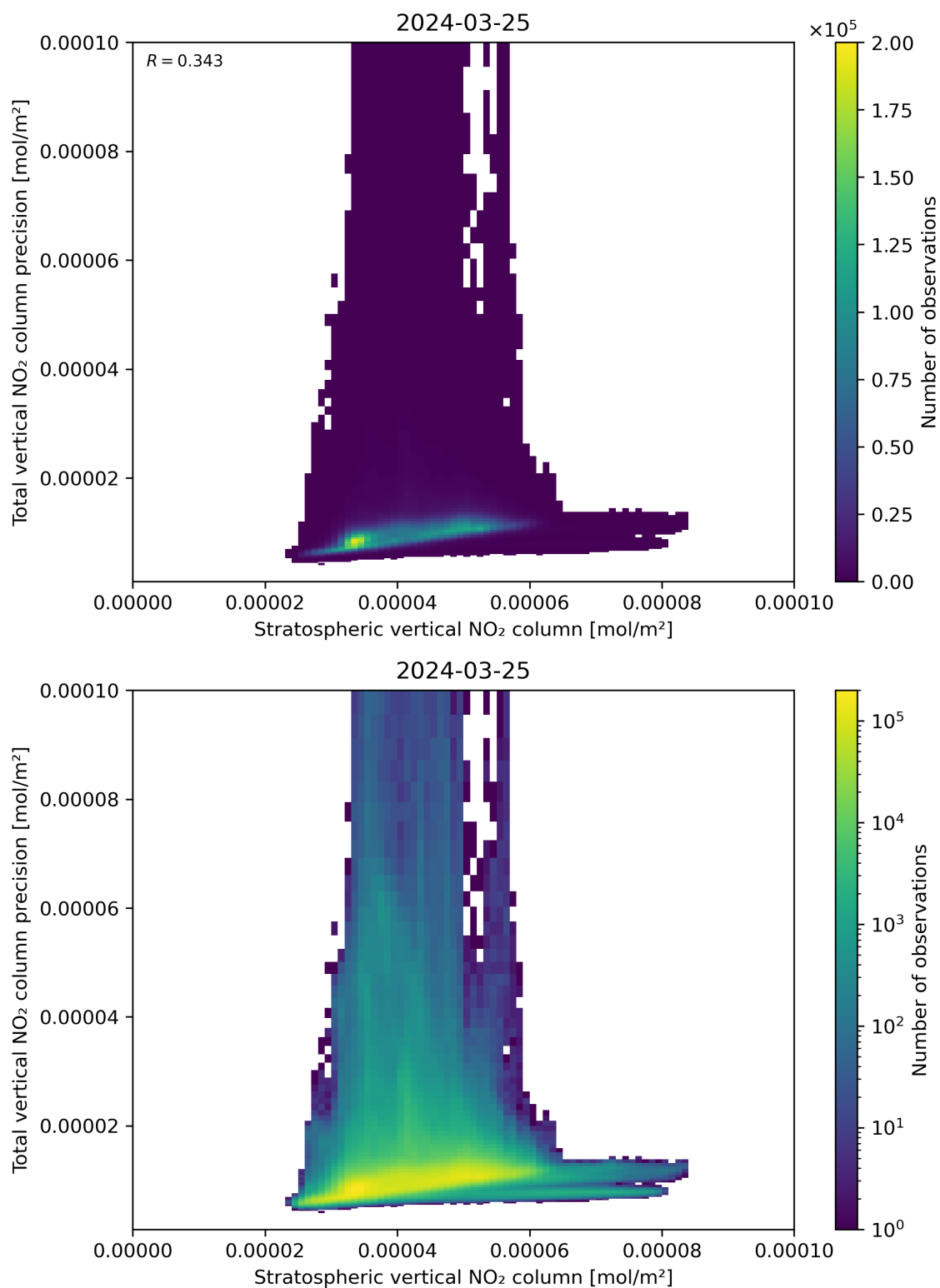
Figure 101: Scatter density plot of “Stratospheric vertical NO 2 column” against “Total vertical NO 2 column precision” for 2024-03-25 to 2024-03-26.
