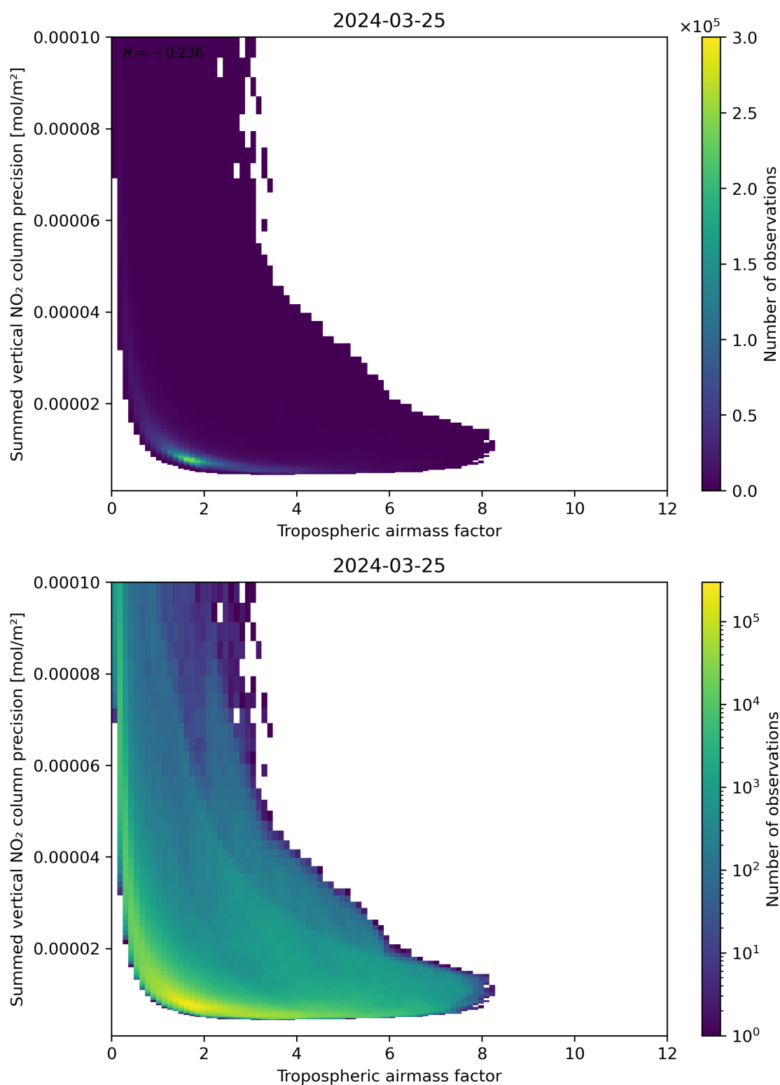
Figure 76: Scatter density plot of “Tropospheric air mass factor” against “Summed vertical NO 2 column precision” for 2024-03-25 to 2024-03-26.
