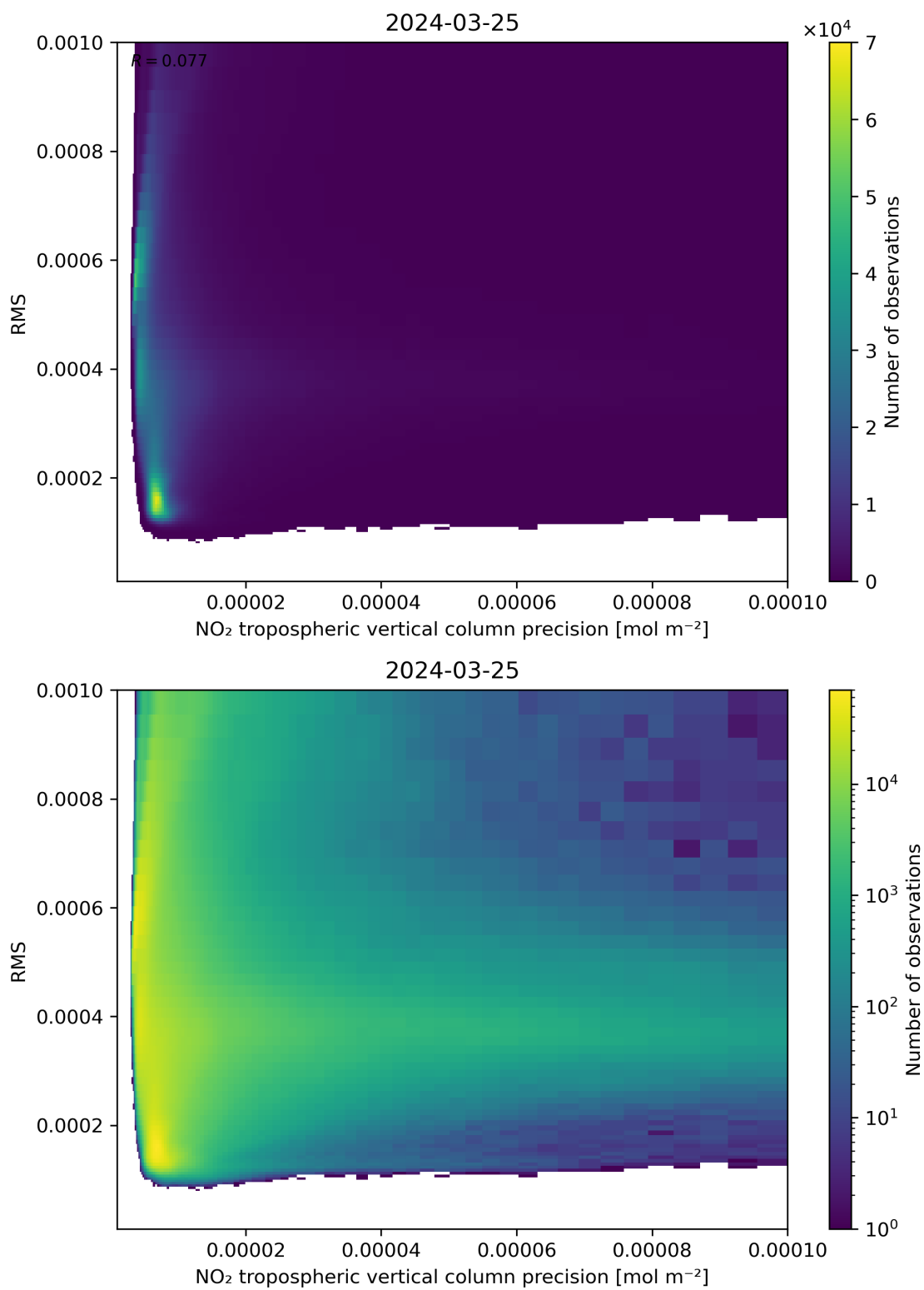
Figure 140: Scatter density plot of “NO 2 tropospheric vertical column precision” against “RMS” for 2024-03-25 to 2024-03-26.
