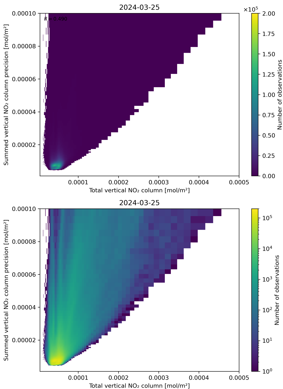
Figure 113: Scatter density plot of “Total vertical NO 2 column” against “Summed vertical NO 2 column precision” for 2024-03-25 to 2024-03-26.
