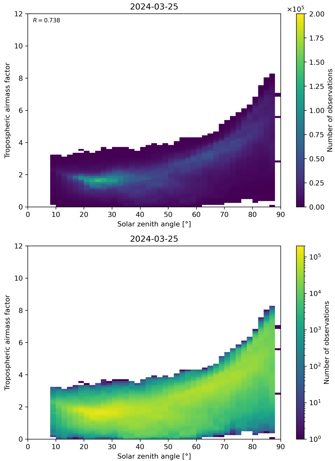
Figure 147: Scatter density plot of “Solar zenith angle” against “Tropospheric airmass factor” for 2024-03-25 to 2024-03-26.
