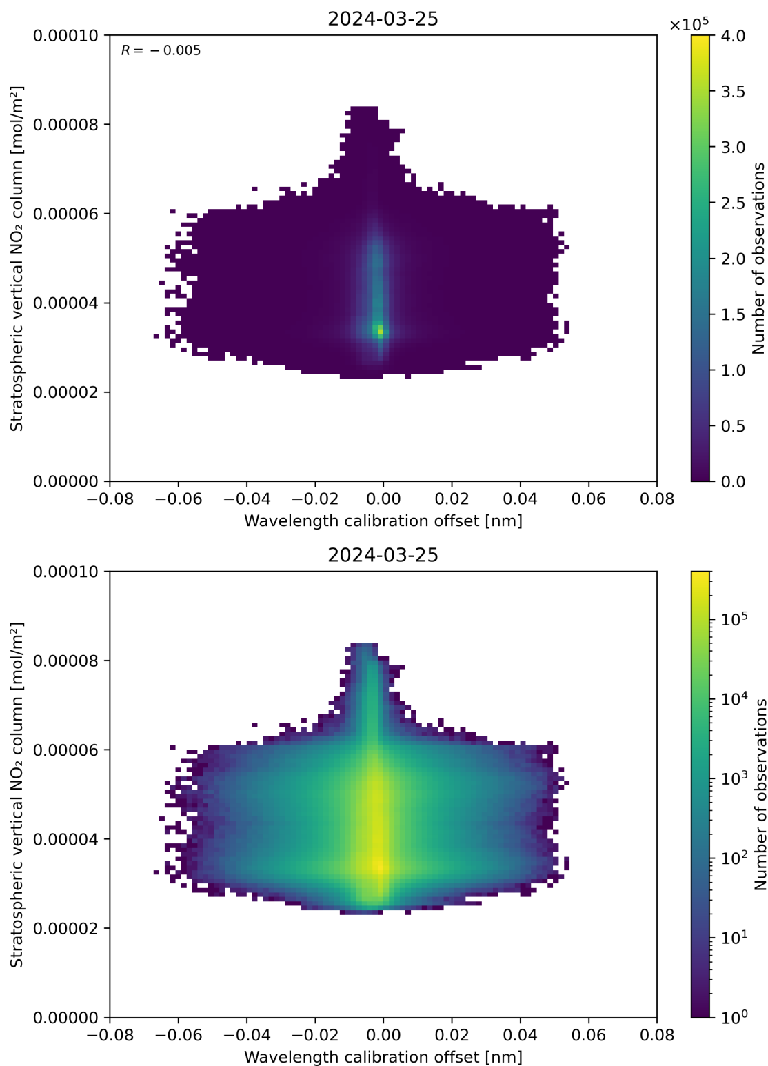
Figure 176: Scatter density plot of “Wavelength calibration offset” against “Stratospheric vertical NO 2 column” for 2024-03-25 to 2024-03-26.
