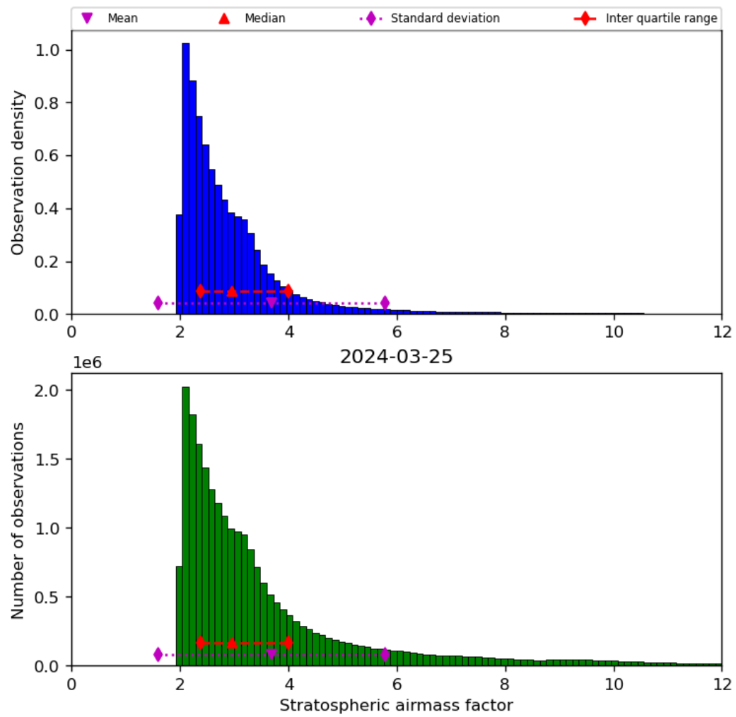
Figure 44: Histogram of "Stratospheric airmass factor" for 2024-03-25 to 2024-03-26
