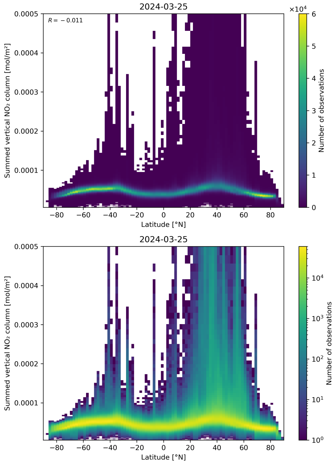
Figure 88: Scatter density plot of “Latitude” against “Summed vertical NO 2 column” for 2024-03-25 to 2024-03-26.
