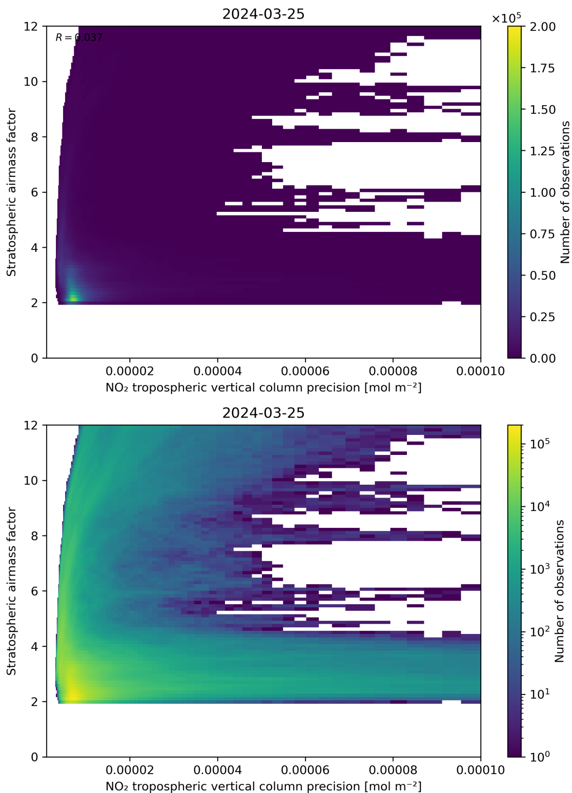
Figure 131: Scatter density plot of “NO 2 tropospheric vertical column precision” against “Stratospheric airmass factor” for 2024-03-25 to 2024-03-26.
