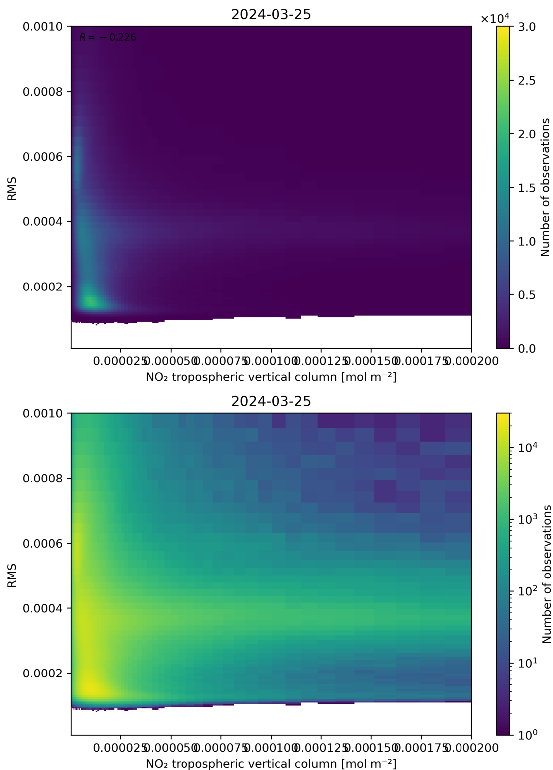
Figure 142: Scatter density plot of “NO 2 tropospheric vertical column” against “RMS” for 2024-03-25 to 2024-03-26.
