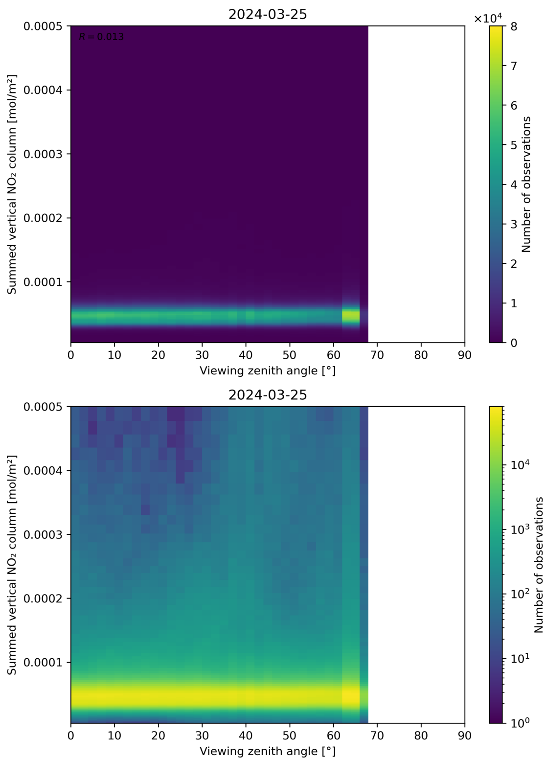
Figure 165: Scatter density plot of “Viewing zenith angle” against “Summed vertical NO 2 column” for 2024-03-25 to 2024-03-26.
