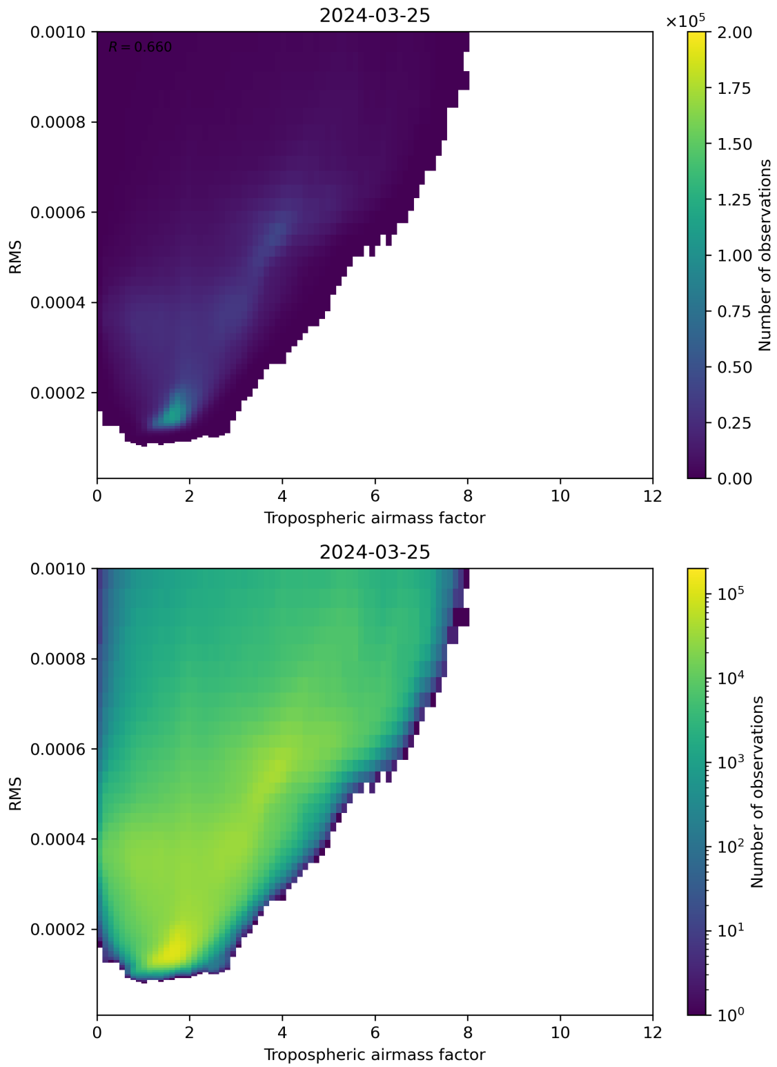
Figure 79: Scatter density plot of “Tropospheric airmass factor” against “RMS” for 2024-03-25 to 2024-03-26.
