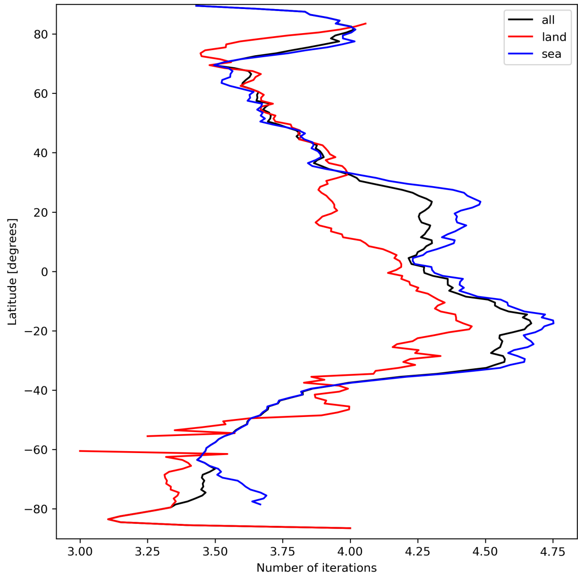
Figure 17: Zonal average of “Number of iterations” for 2024-03-25 to 2024-03-26.
