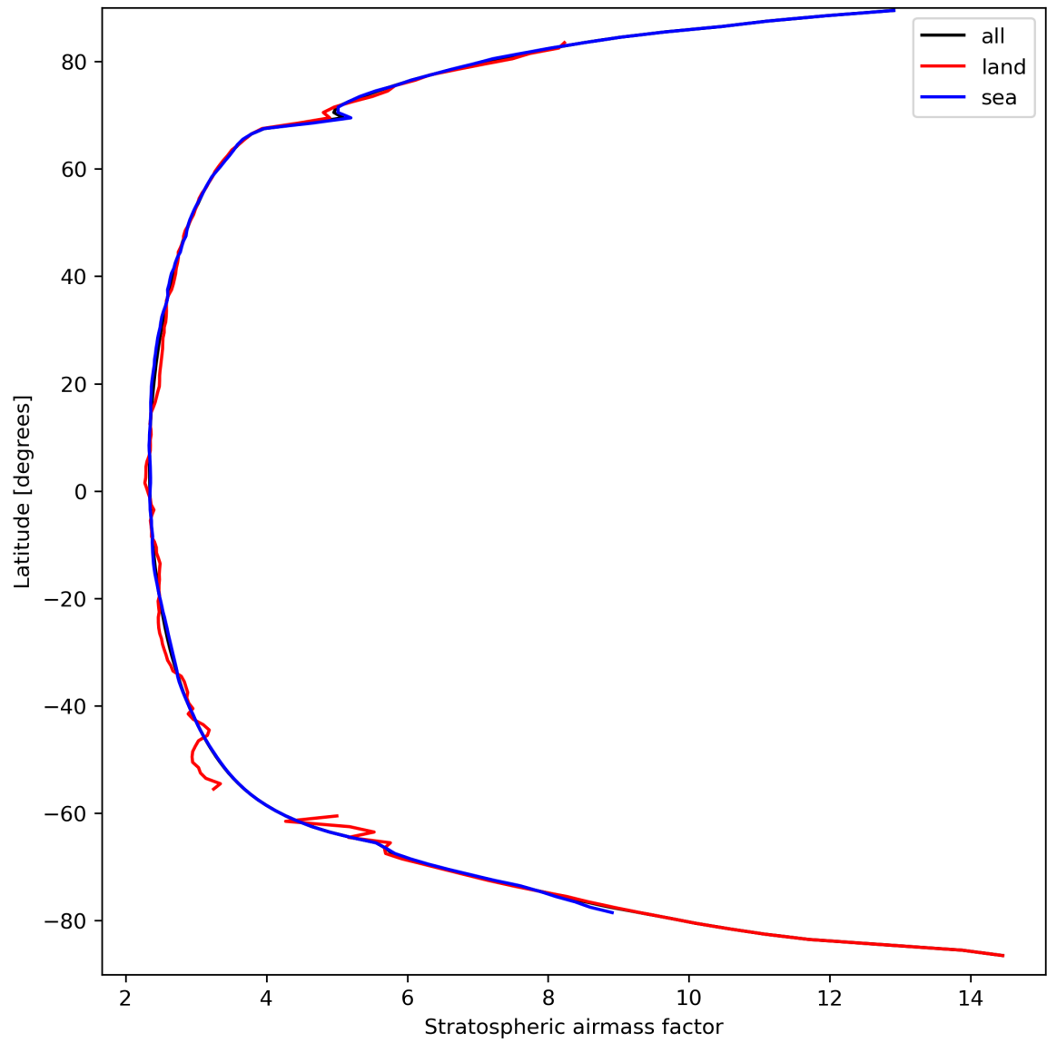
Figure 27: Zonal average of “Stratospheric airmass factor” for 2024-03-25 to 2024-03-26.
