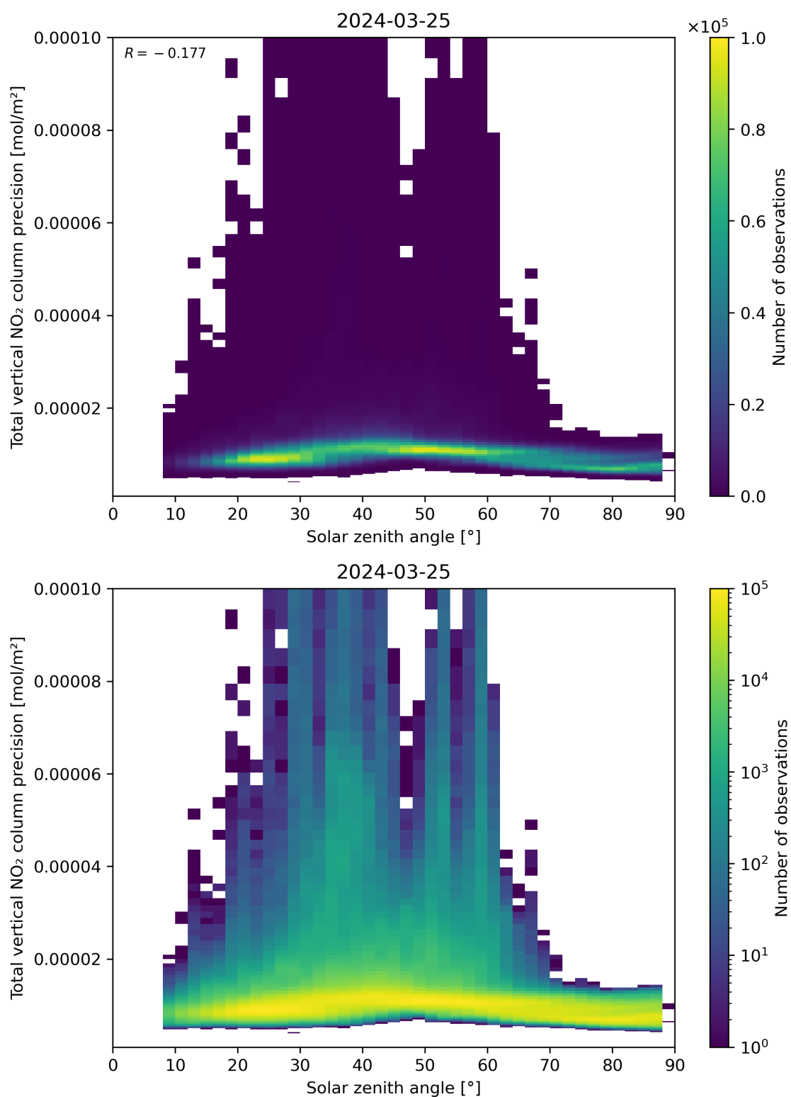
Figure 154: Scatter density plot of “Solar zenith angle” against “Total vertical NO 2 column precision” for 2024-03-25 to 2024-03-26.
