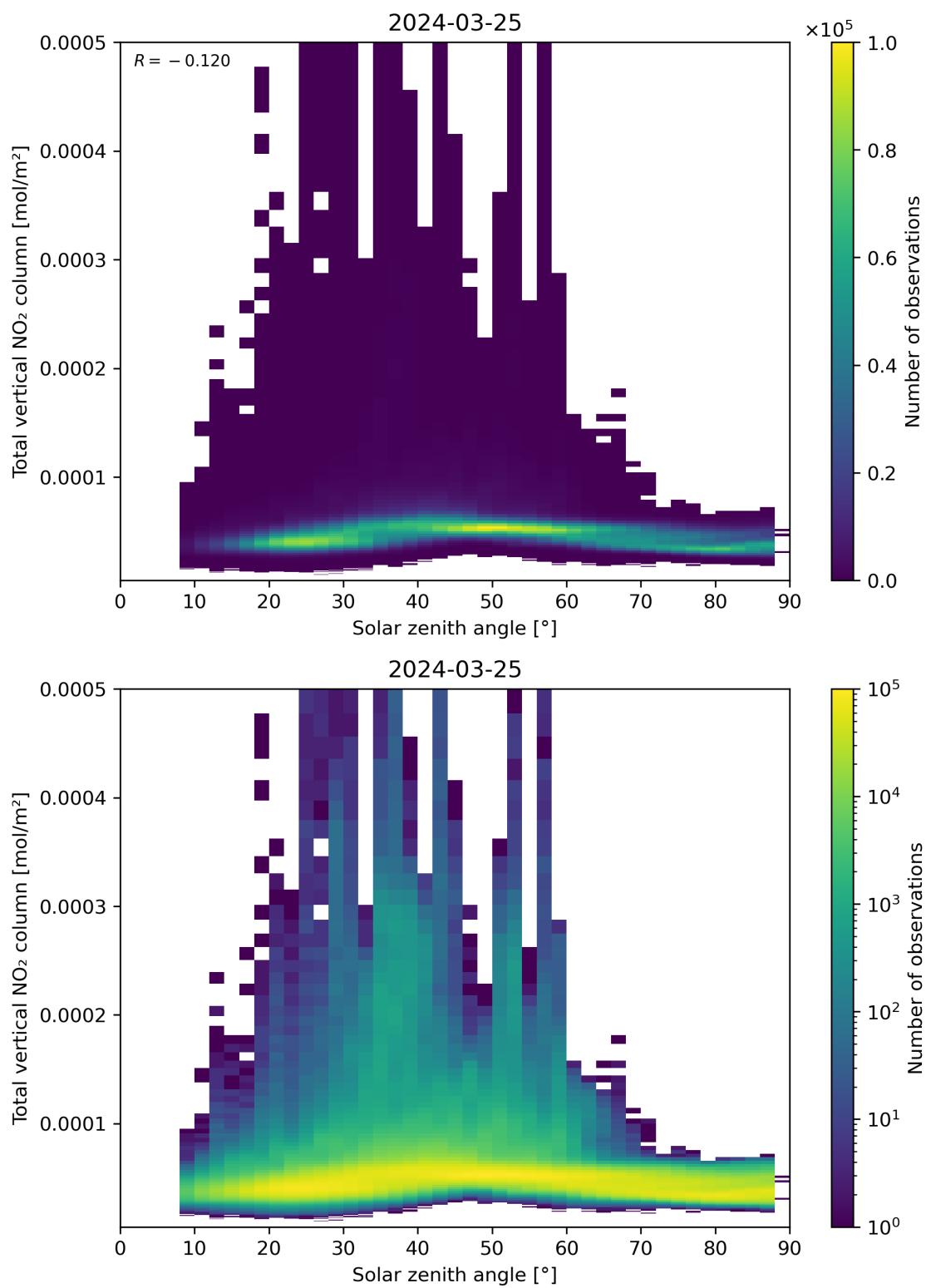
Figure 153: Scatter density plot of “Solar zenith angle” against “Total vertical NO 2 column” for 2024-03-25 to 2024-03-26.
