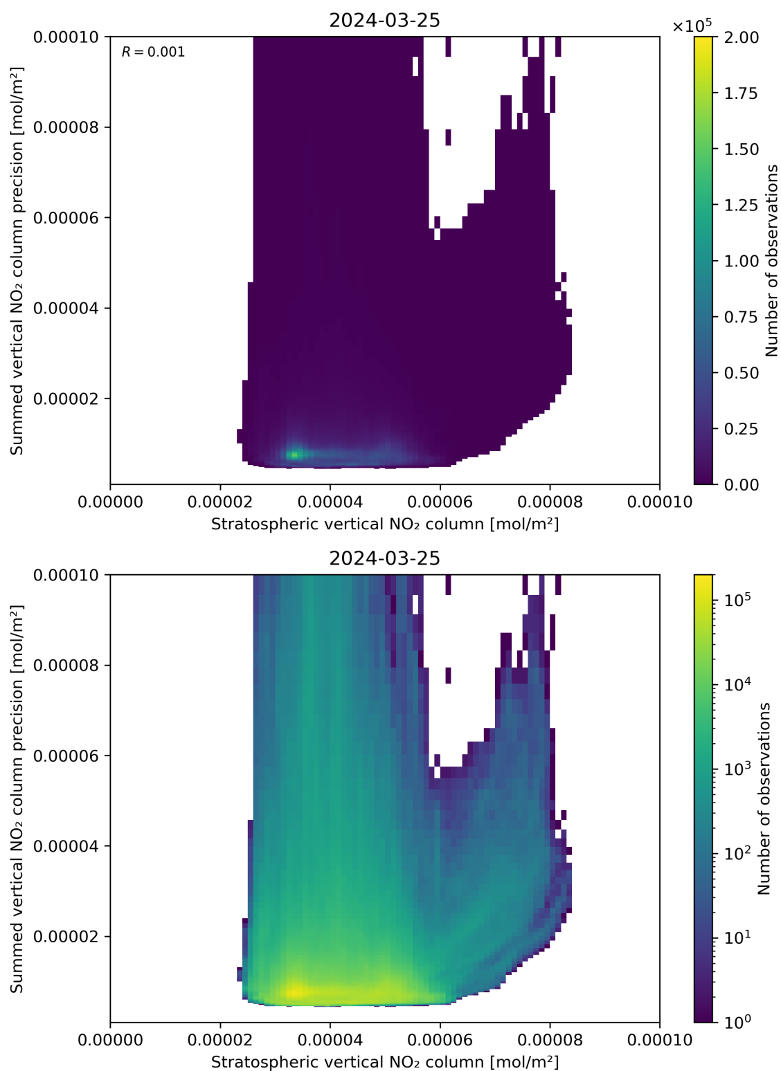
Figure 99: Scatter density plot of “Stratospheric vertical NO 2 column” against “Summed vertical NO 2 column precision” for 2024-03-25 to 2024-03-26.
