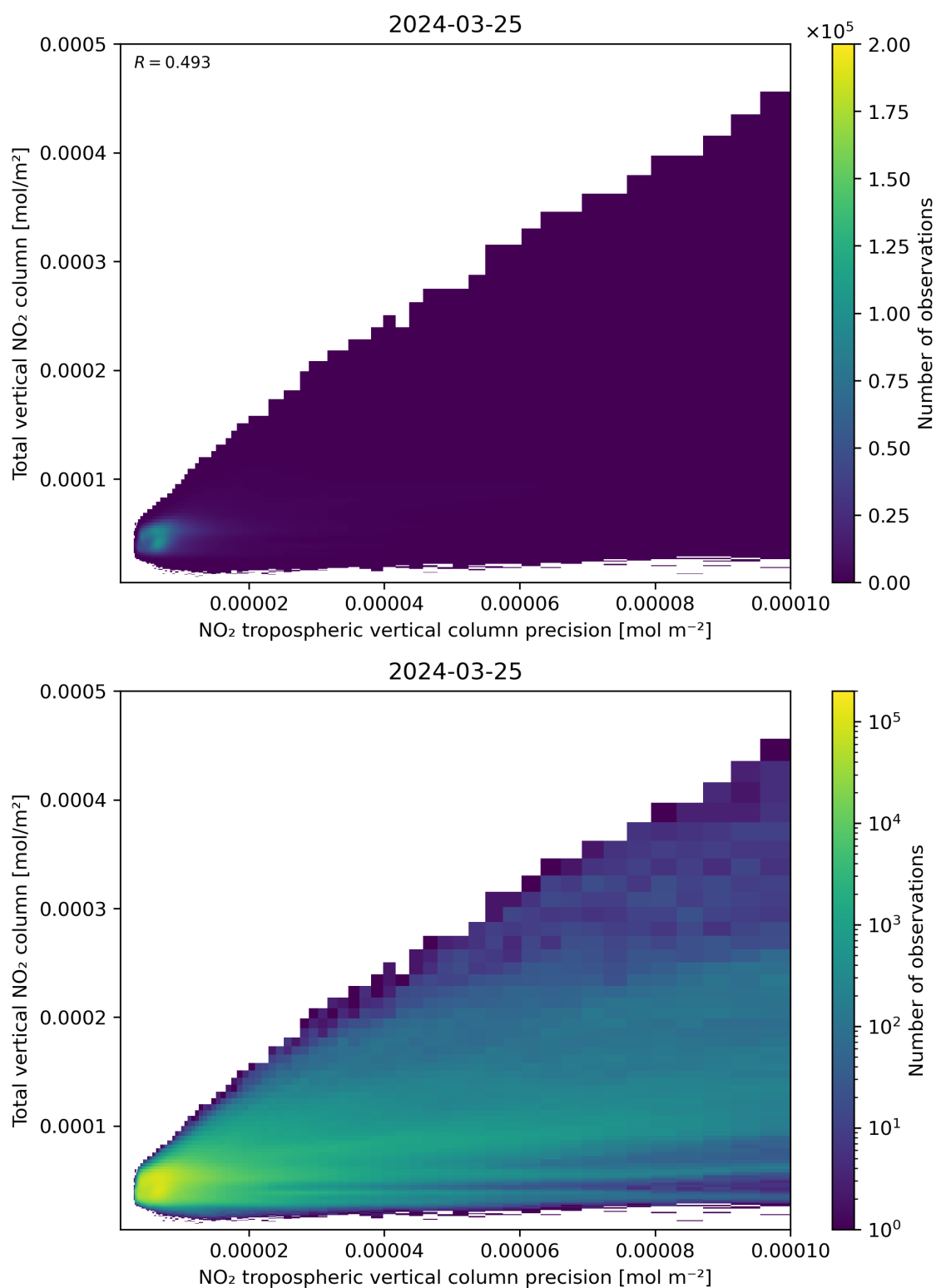
Figure 138: Scatter density plot of “NO 2 tropospheric vertical column precision” against “Total vertical NO 2 column” for 2024-03-25 to 2024-03-26.
