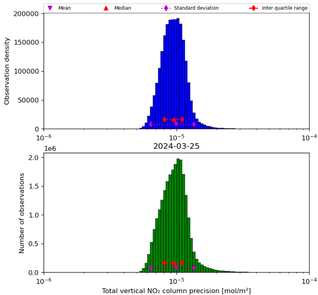
Figure 39: Histogram of “Total vertical NO 2 column precision” for 2024-03-25 to 2024-03-26
