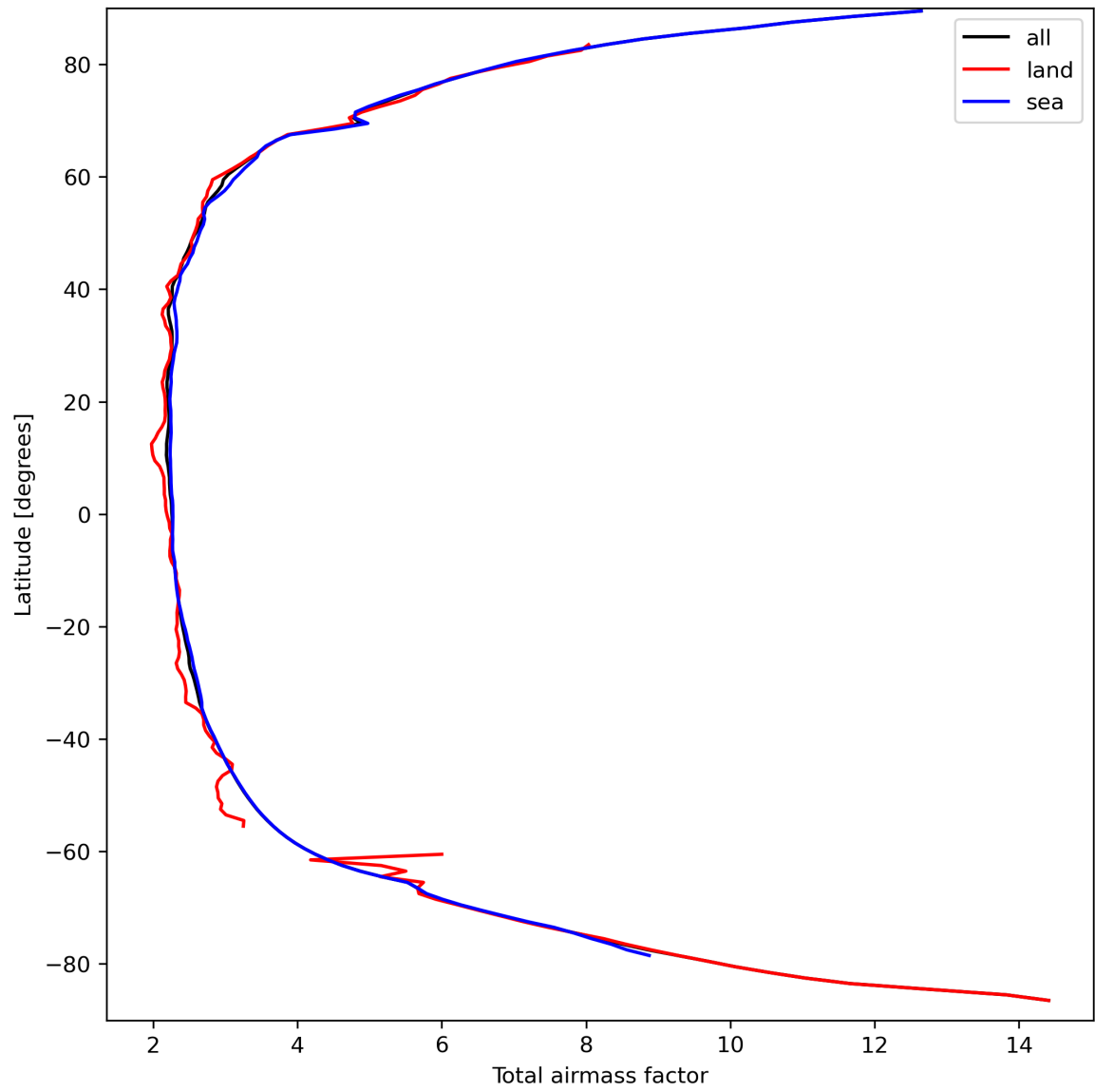
Figure 15: Zonal average of “Total airmass factor” for 2024-03-25 to 2024-03-26.
