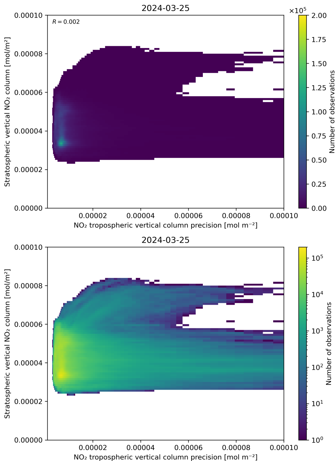
Figure 135: Scatter density plot of “NO 2 tropospheric vertical column precision” against “Stratospheric vertical NO 2 column” for 2024-03-25 to 2024-03-26.
