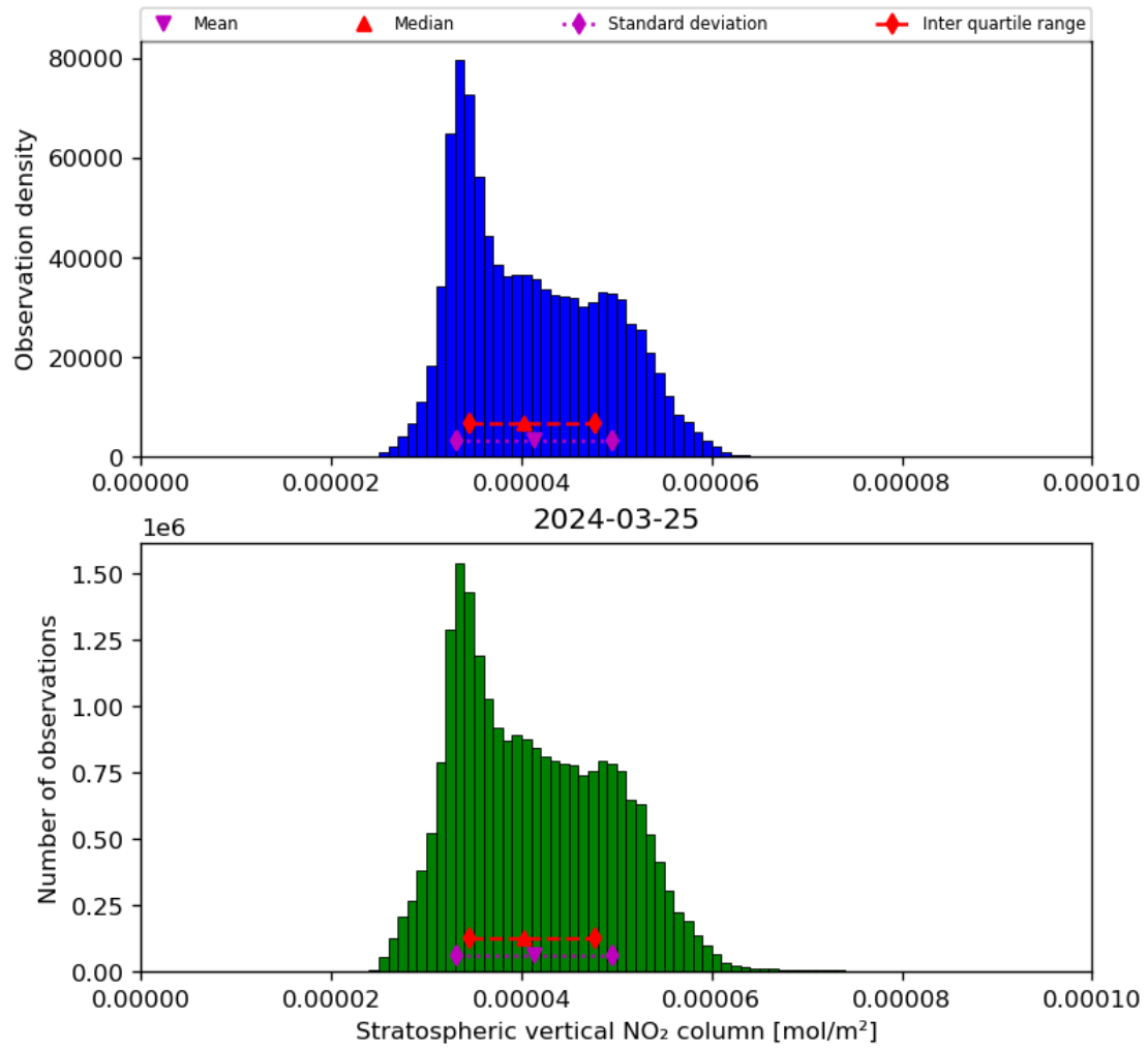
Figure 36: Histogram of “Stratospheric vertical NO 2 column” for 2024-03-25 to 2024-03-26
