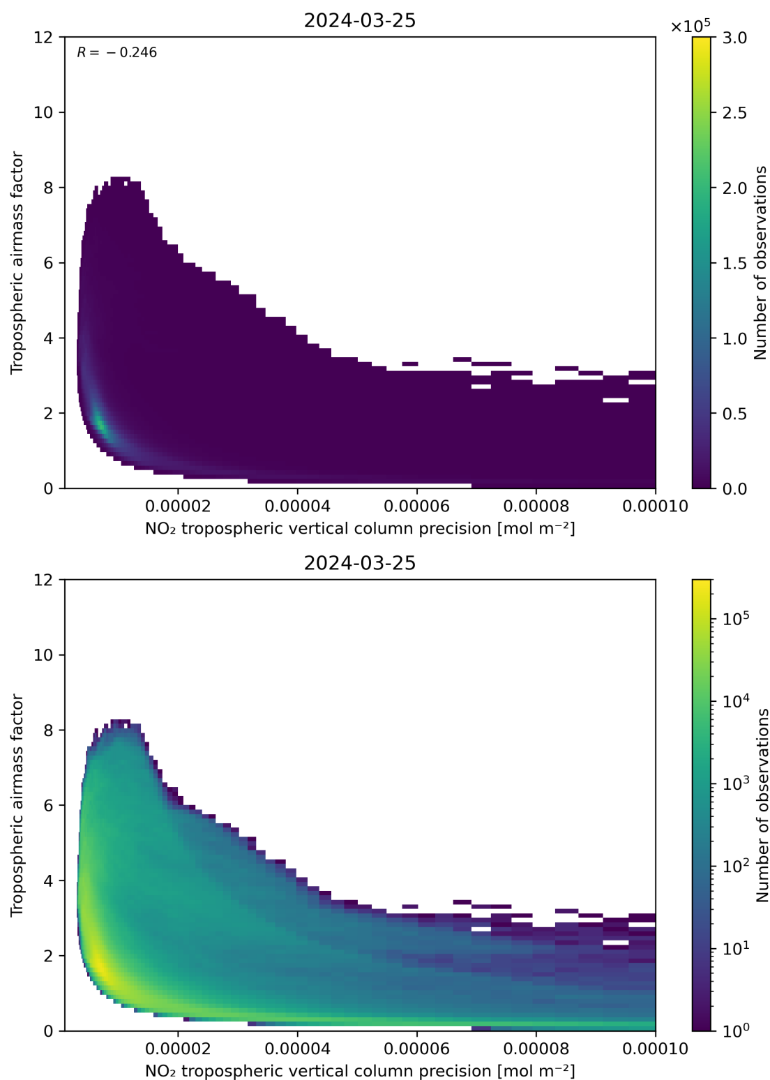
Figure 133: Scatter density plot of “NO 2 tropospheric vertical column precision” against “Tropospheric airmass factor” for 2024-03-25 to 2024-03-26.
