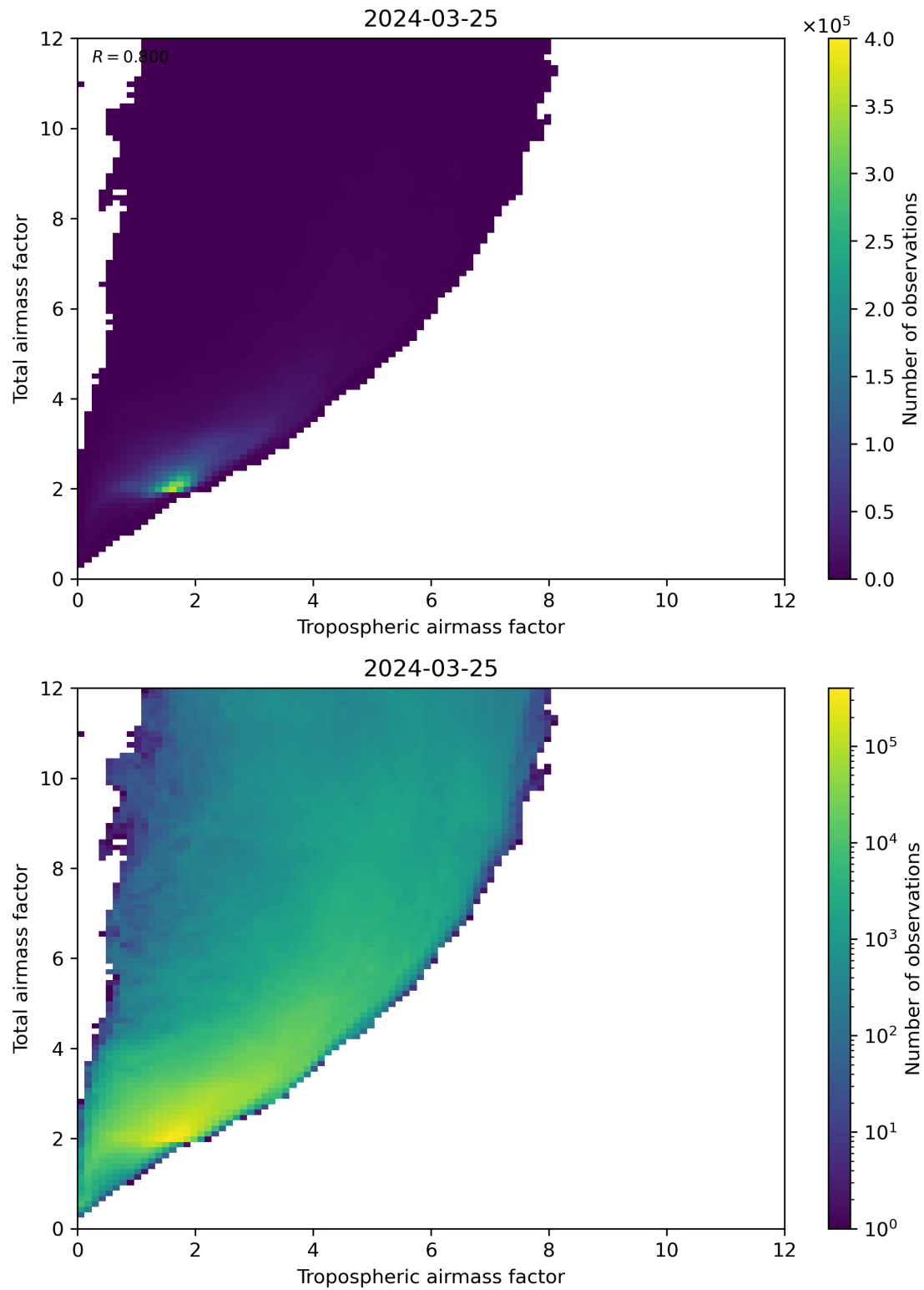
Figure 72: Scatter density plot of “Tropospheric airmass factor” against “Total airmass factor” for 2024-03-25 to 2024-03-26.
