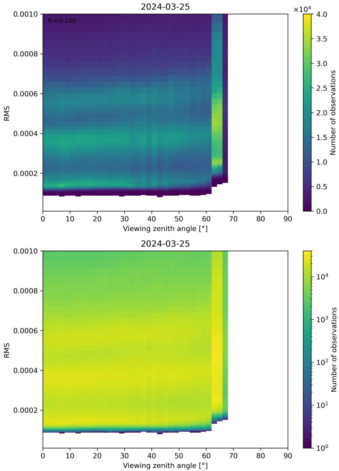
Figure 171: Scatter density plot of “Viewing zenith angle” against “RMS” for 2024-03-25 to 2024-03-26.
