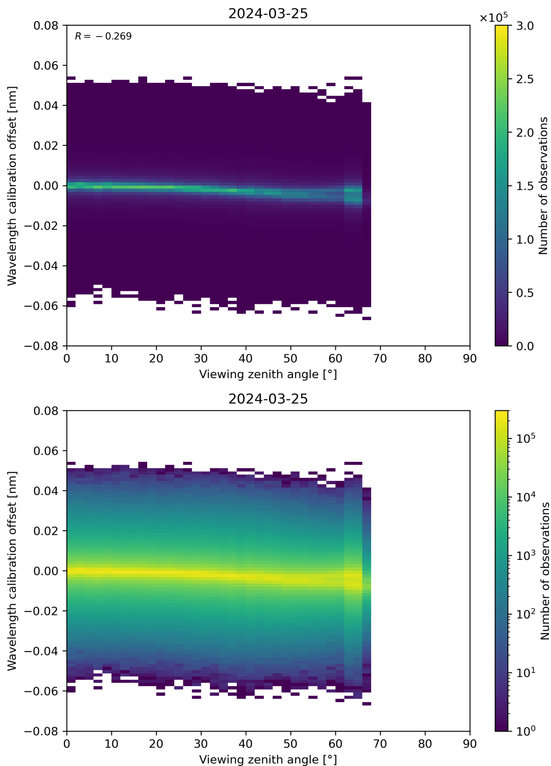
Figure 173: Scatter density plot of “Viewing zenith angle” against “Wavelength calibration offset” for 2024-03-25 to 2024-03-26.
