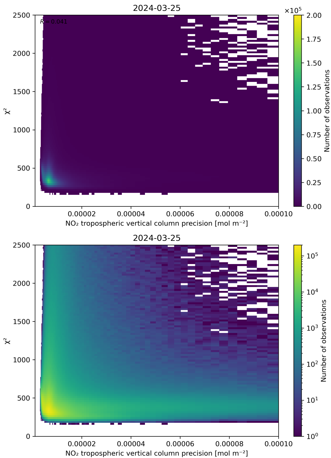
Figure 134: Scatter density plot of “NO 2 tropospheric vertical column precision” against “ \chi^2 ” for 2024-03-25 to 2024-03-26.
