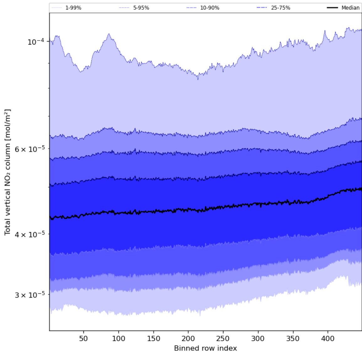
Figure 55: Along track statistics of “Total vertical NO 2 column” for 2024-03-25 to 2024-03-26
