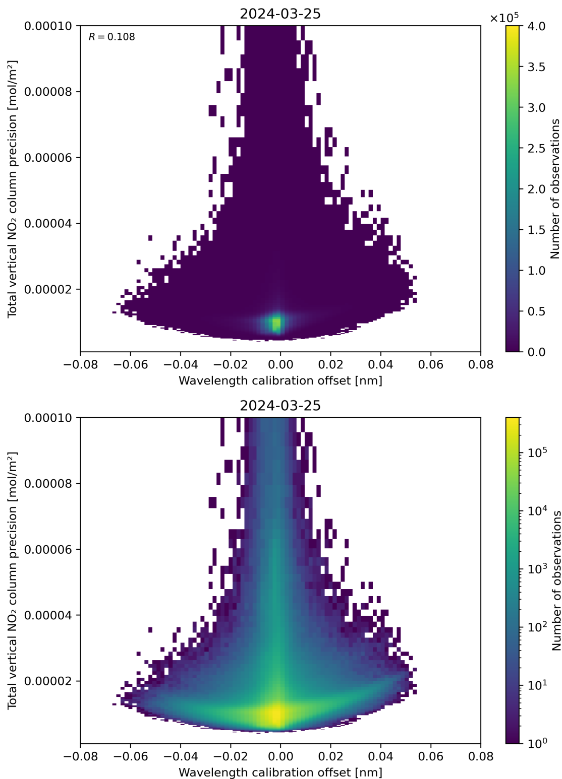
Figure 180: Scatter density plot of “Wavelength calibration offset” against “Total vertical NO 2 column precision” for 2024-03-25 to 2024-03-26.
