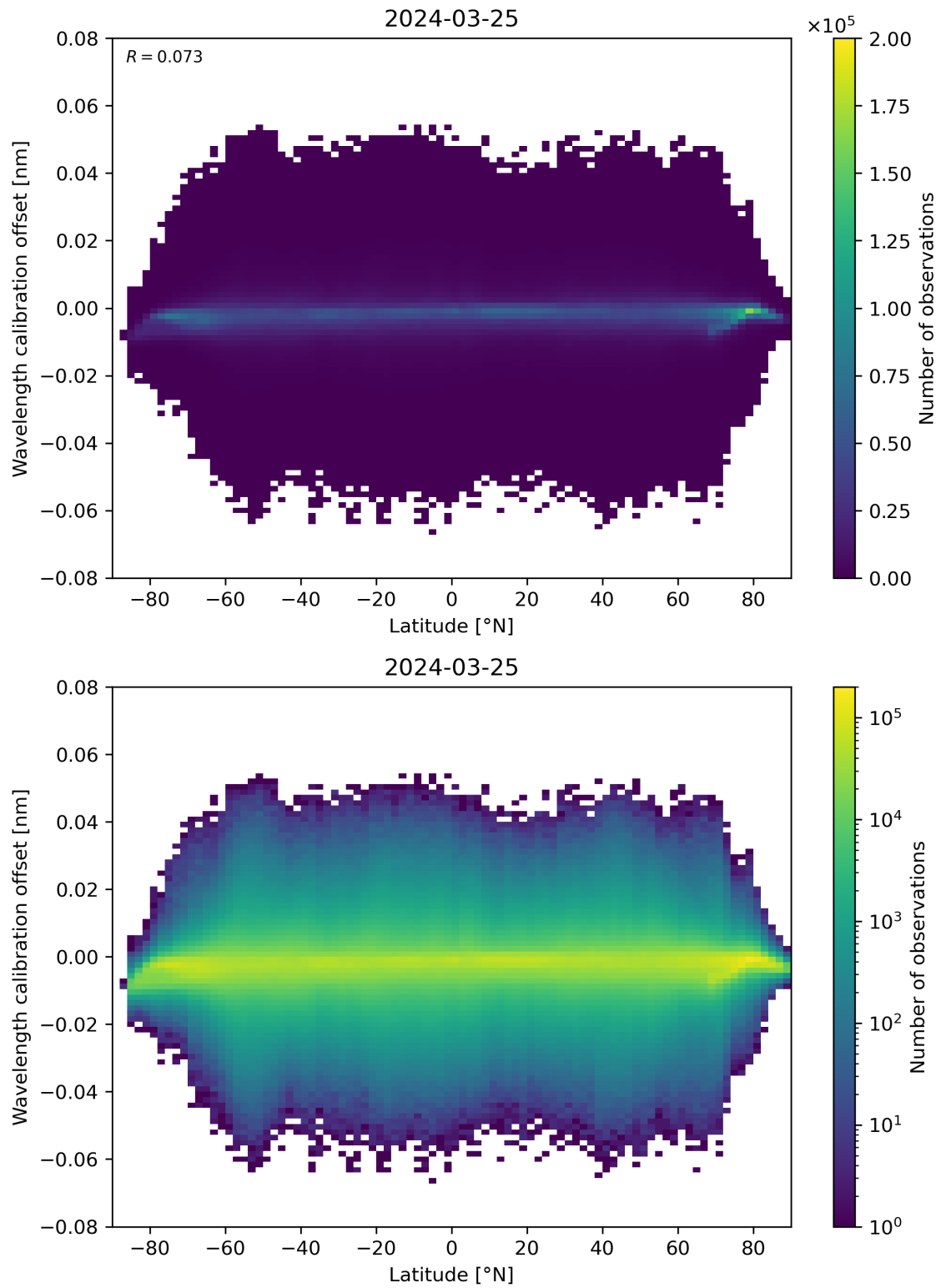
Figure 95: Scatter density plot of “Latitude” against “Wavelength calibration offset” for 2024-03-25 to 2024-03-26.
