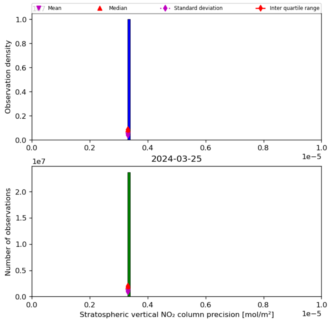
Figure 37: Histogram of “Stratospheric vertical NO 2 column precision” for 2024-03-25 to 2024-03-26
