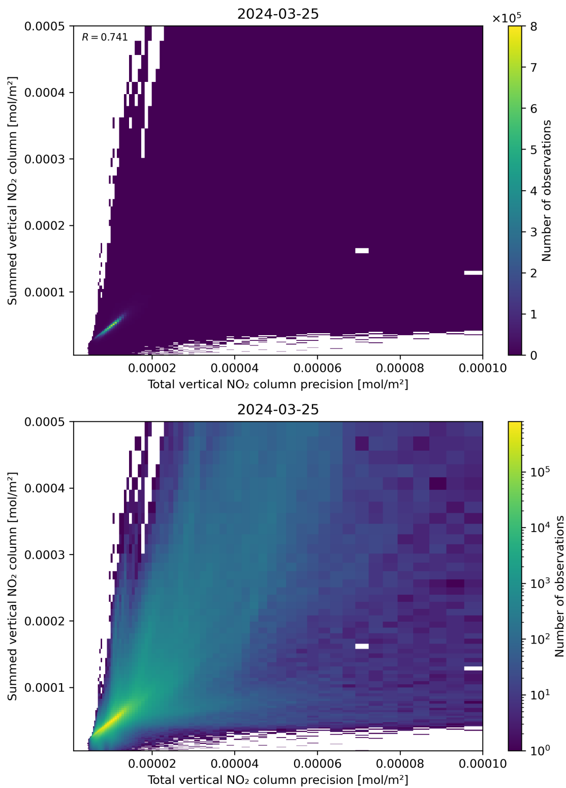
Figure 117: Scatter density plot of “Total vertical NO 2 column precision” against “Summed vertical NO 2 column” for 2024-03-25 to 2024-03-26.
