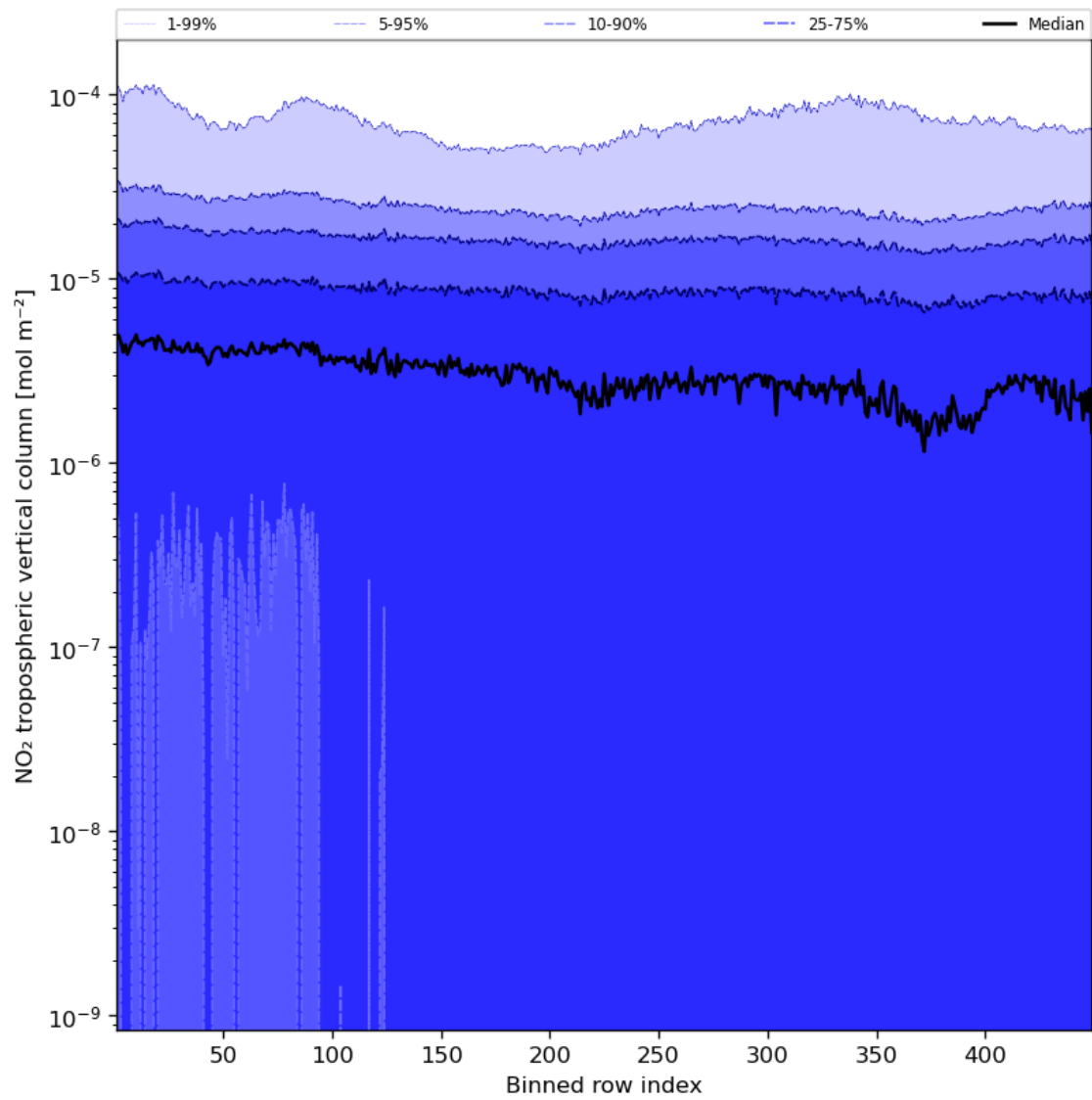
Figure 46: Along track statistics of “NO 2 tropospheric vertical column” for 2024-03-25 to 2024-03-26
