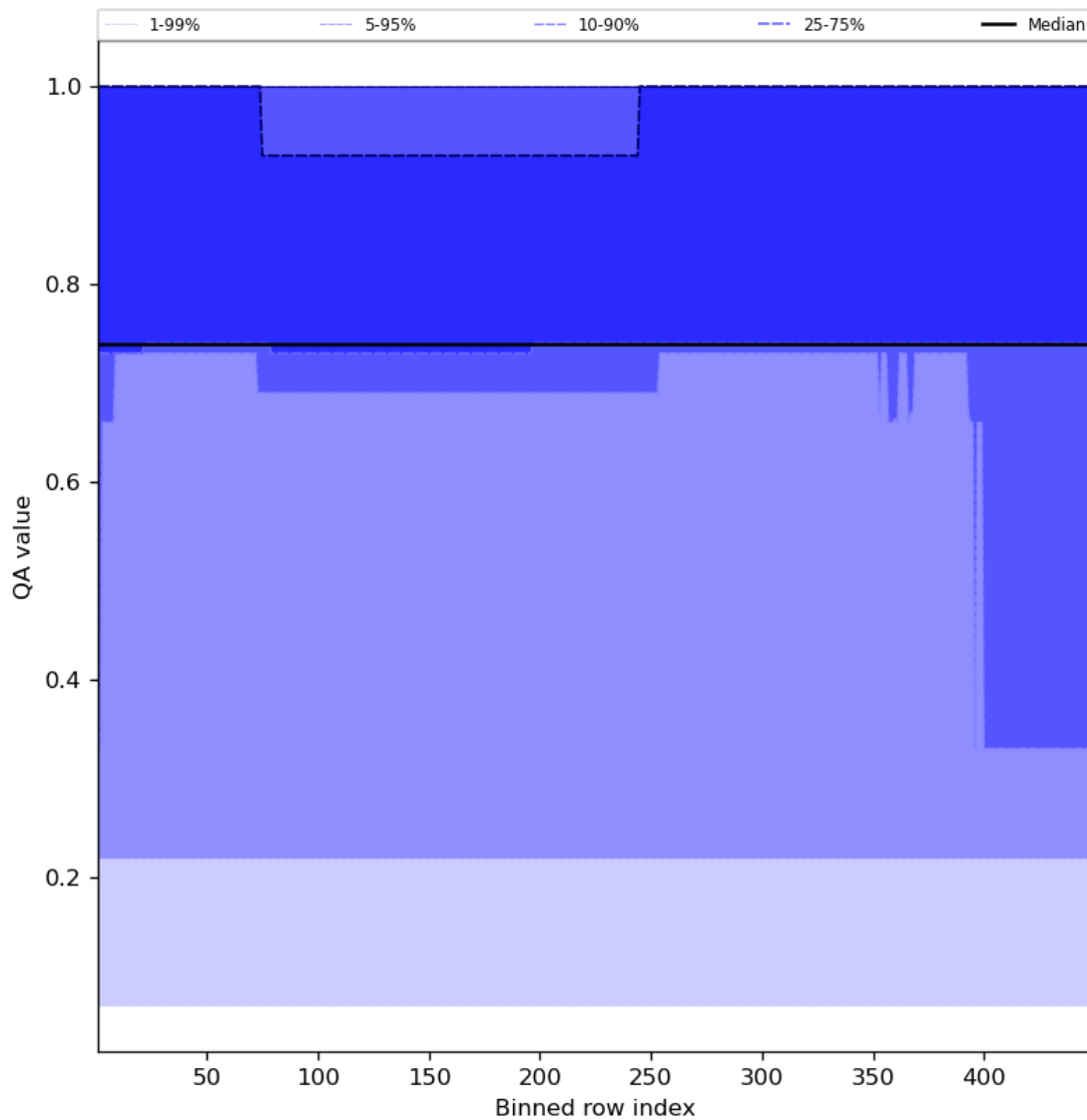
Figure 45: Along track statistics of “QA value” for 2024-03-25 to 2024-03-26
