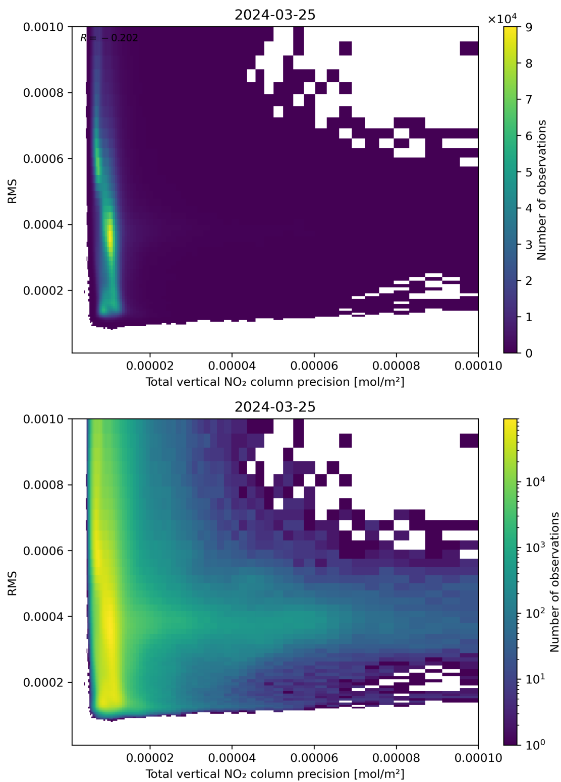
Figure 119: Scatter density plot of “Total vertical NO 2 column precision” against “RMS” for 2024-03-25 to 2024-03-26.
