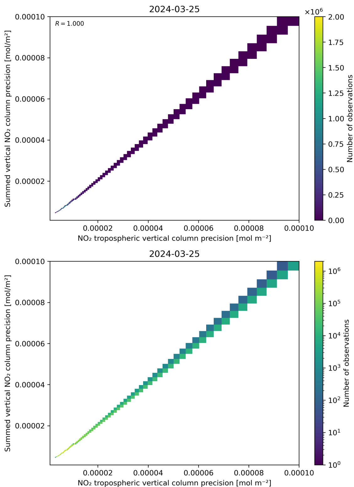
Figure 137: Scatter density plot of “NO 2 tropospheric vertical column precision” against “Summed vertical NO 2 column precision” for 2024-03-25 to 2024-03-26.
