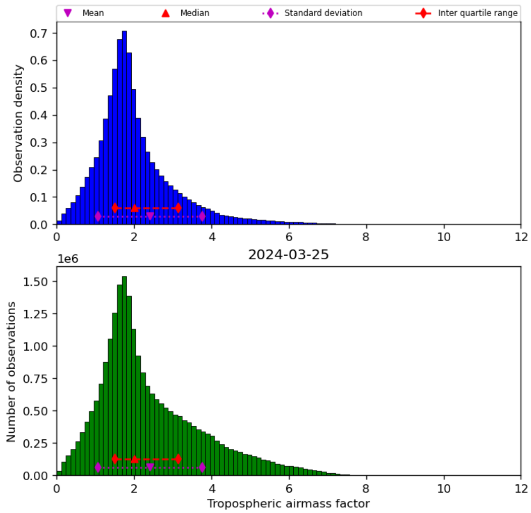
Figure 31: Histogram of “Tropospheric airmass factor” for 2024-03-25 to 2024-03-26
