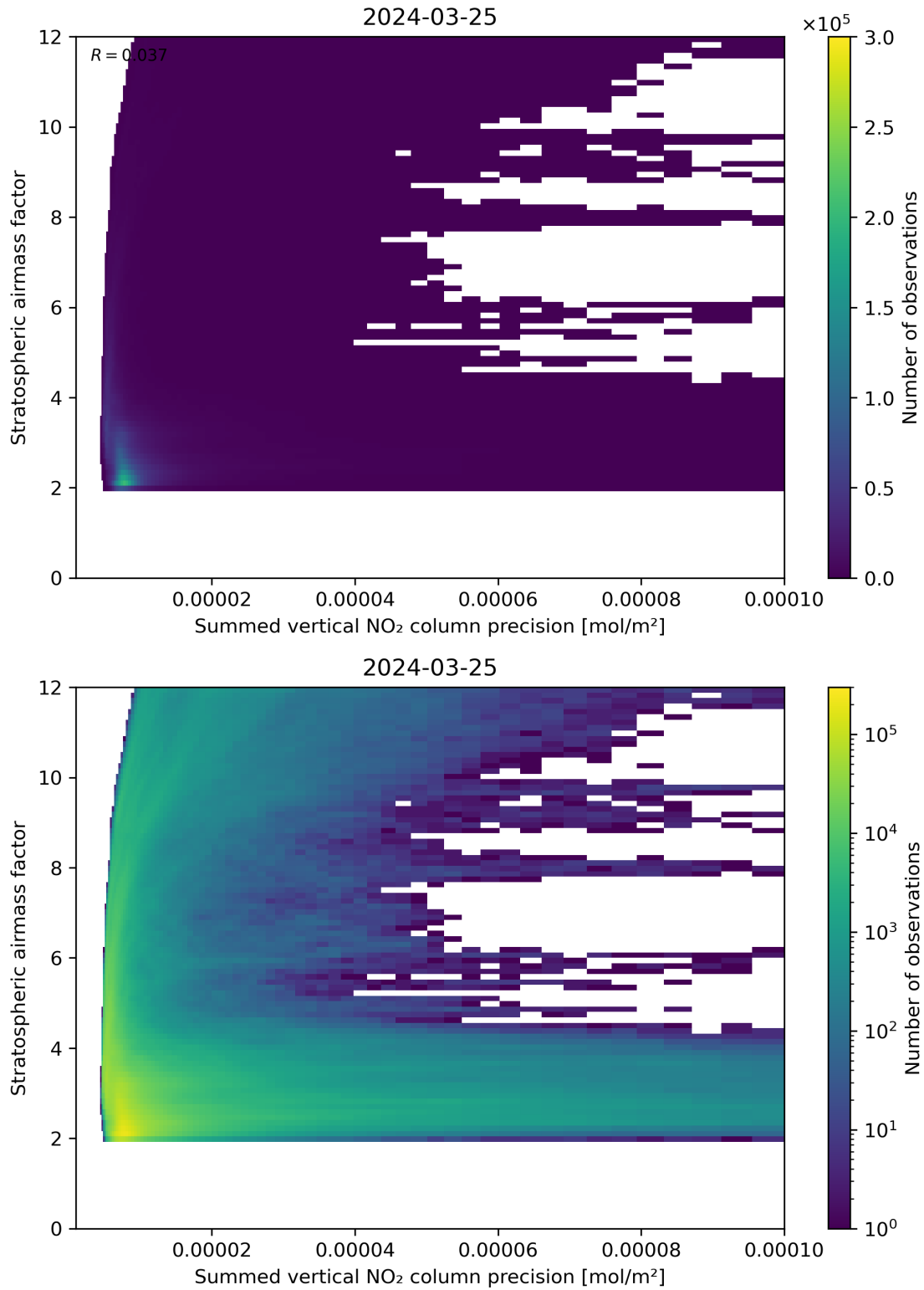
Figure 106: Scatter density plot of “Summed vertical NO 2 column precision” against “Stratospheric airmass factor” for 2024-03-25 to 2024-03-26.
