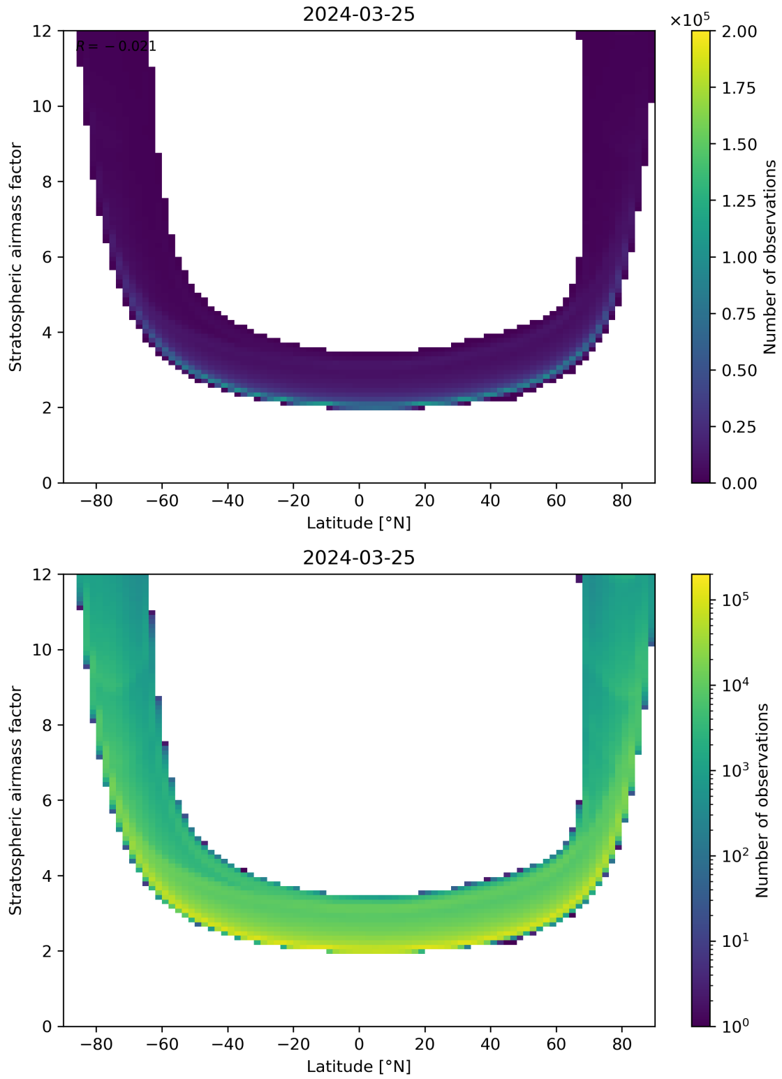
Figure 83: Scatter density plot of “Latitude” against “Stratospheric air mass factor” for 2024-03-25 to 2024-03-26.
