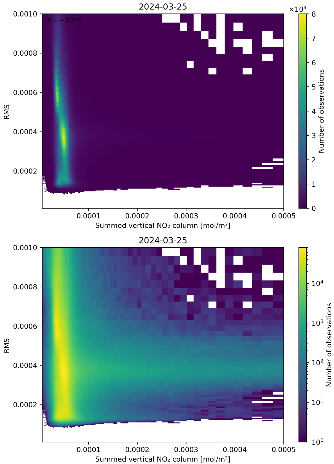
Figure 109: Scatter density plot of “Summed vertical NO 2 column” against “RMS” for 2024-03-25 to 2024-03-26.
