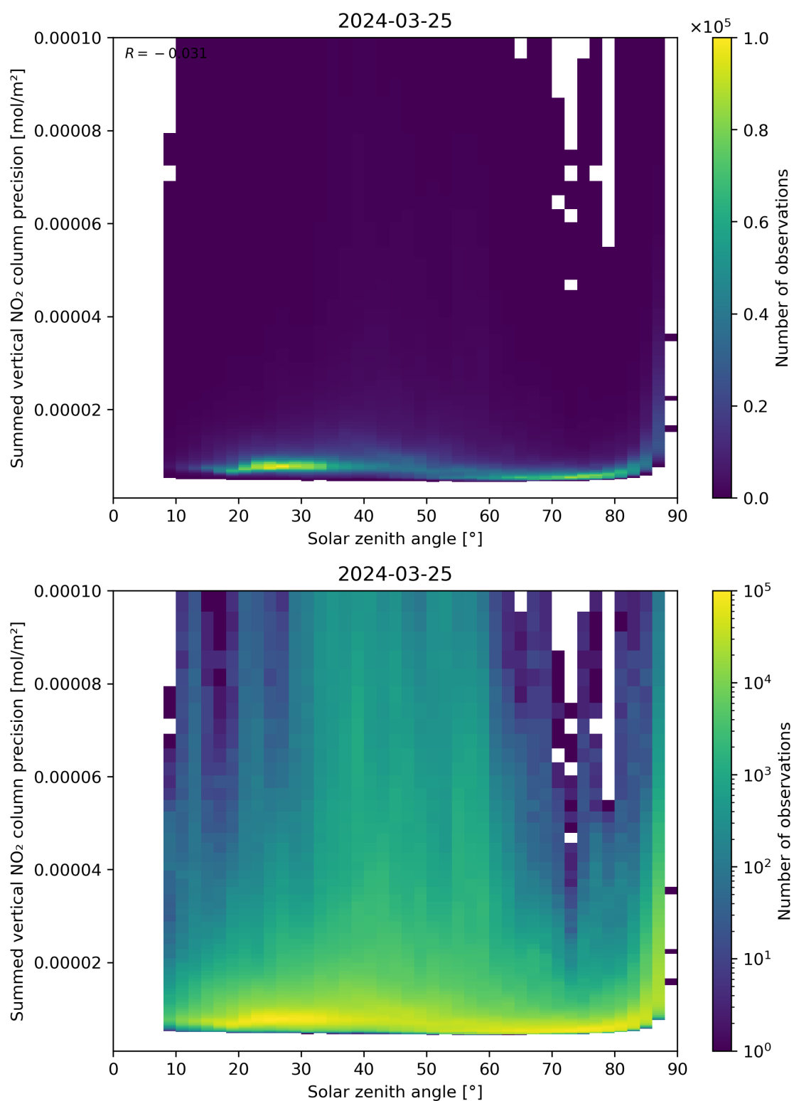
Figure 152: Scatter density plot of “Solar zenith angle” against “Summed vertical NO 2 column precision” for 2024-03-25 to 2024-03-26.
