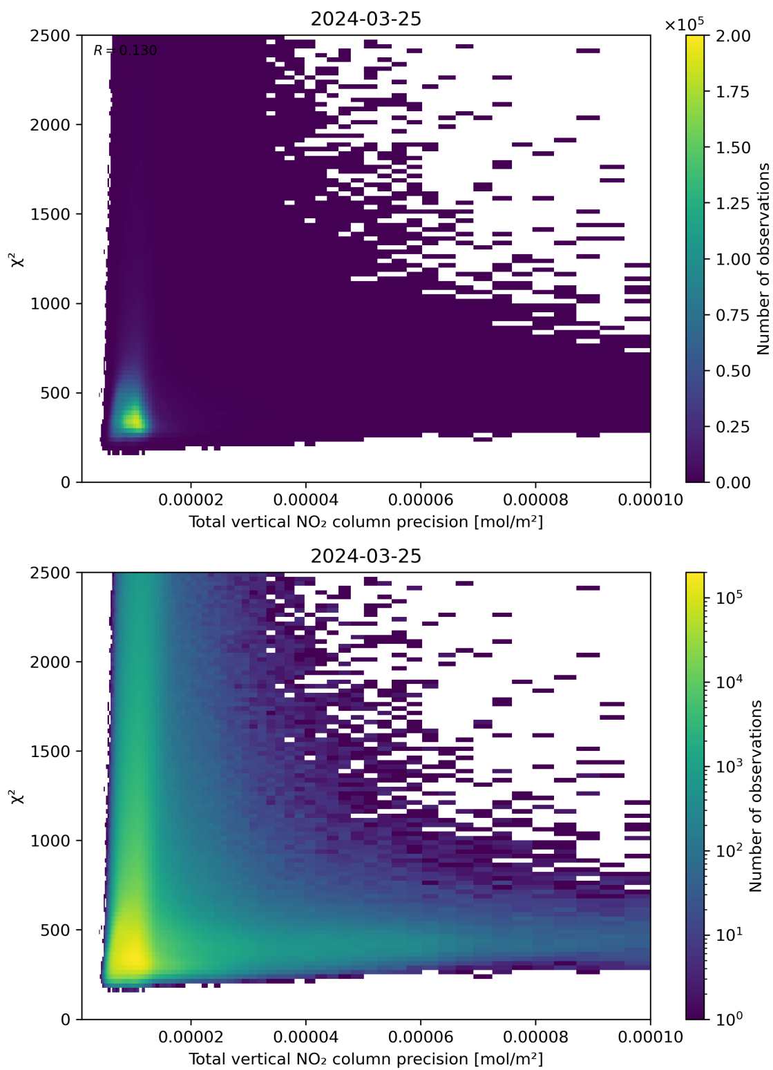
Figure 116: Scatter density plot of “Total vertical NO 2 column precision” against “ \chi^2 ” for 2024-03-25 to 2024-03-26.
