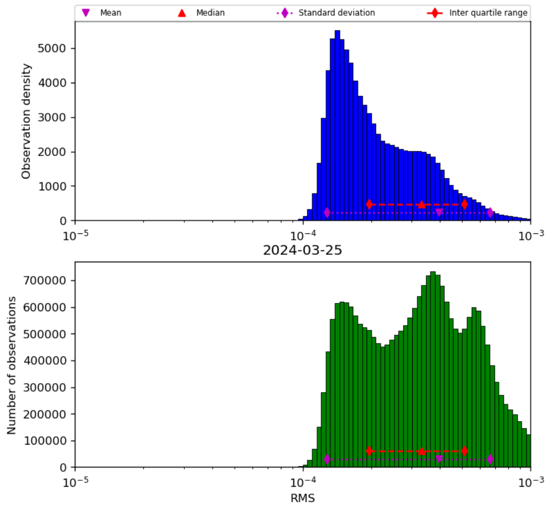
Figure 43: Histogram of “RMS” for 2024-03-25 to 2024-03-26
