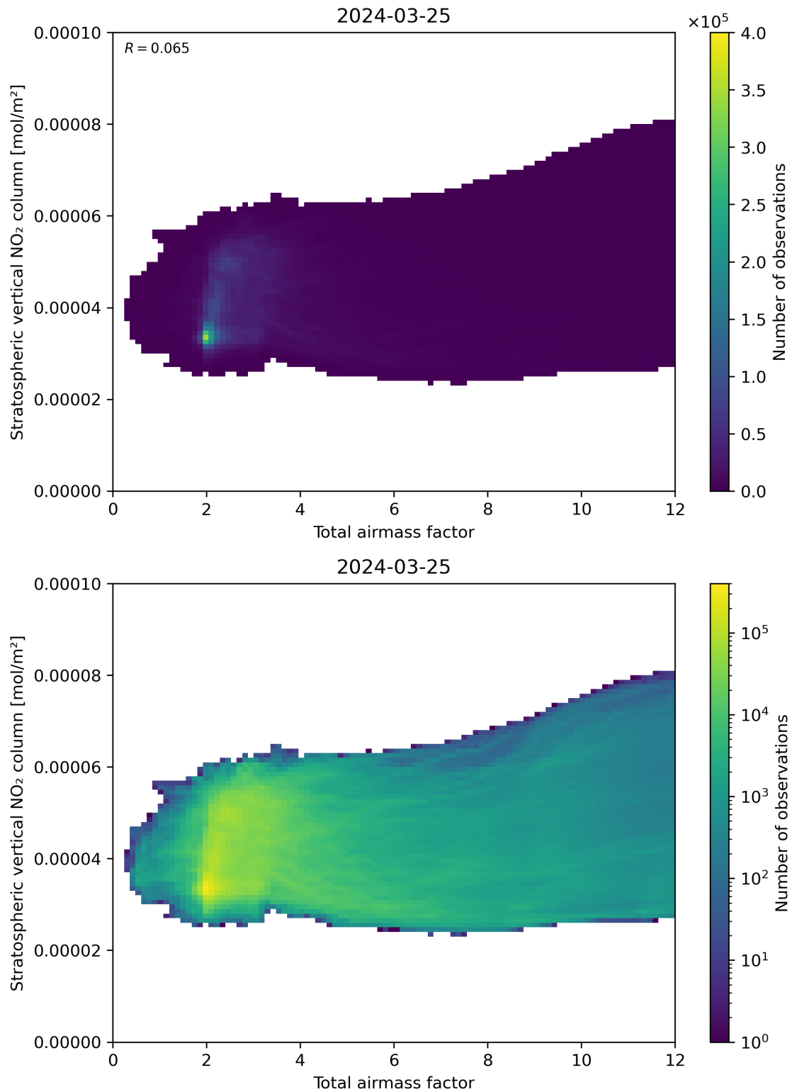
Figure 64: Scatter density plot of “Total airmass factor” against “Stratospheric vertical \text{NO}_2 column” for 2024-03-25 to 2024-03-26.
