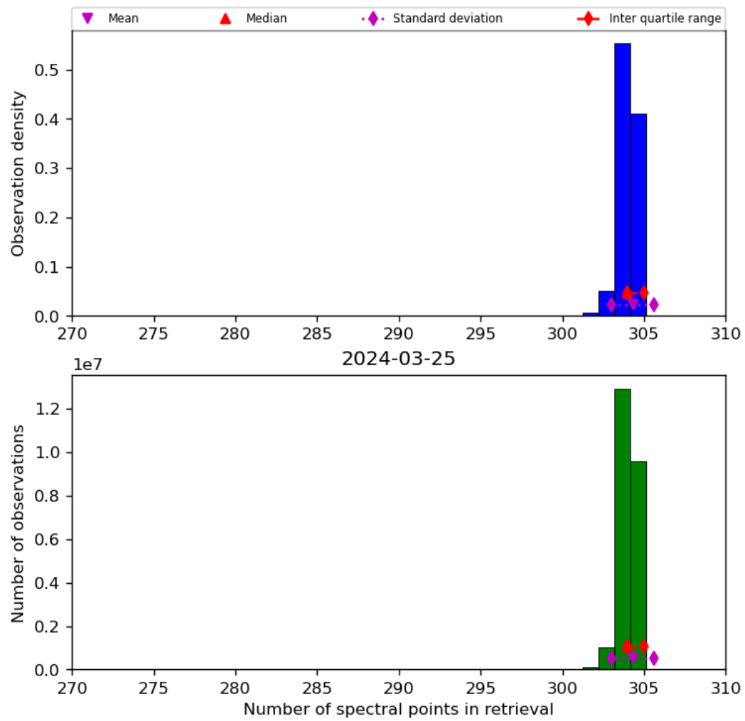
Figure 33: Histogram of “Number of spectral points in retrieval” for 2024-03-25 to 2024-03-26
