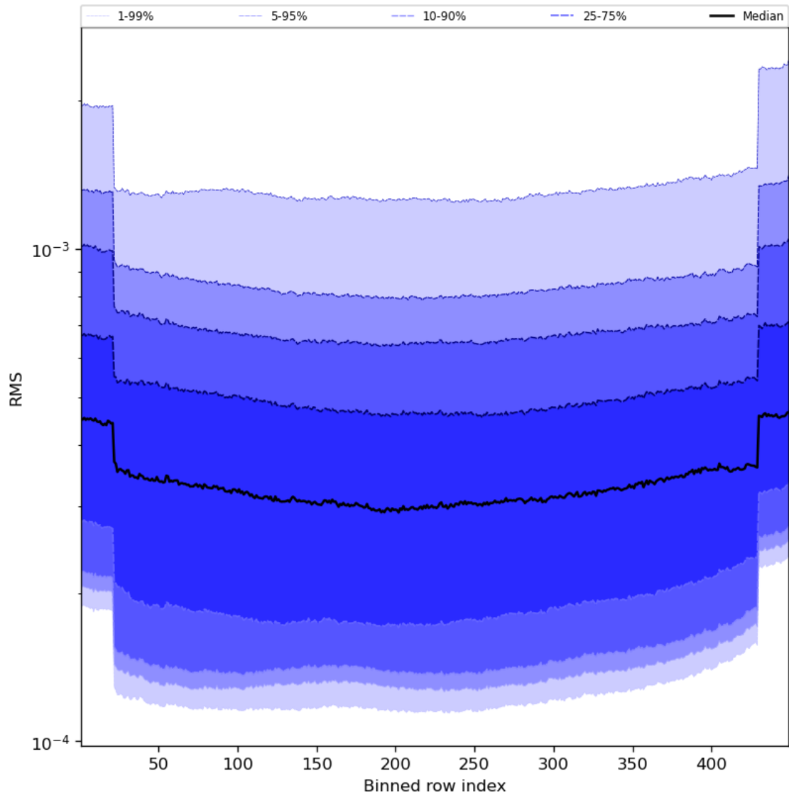
Figure 60: Along track statistics of “RMS” for 2024-03-25 to 2024-03-26
