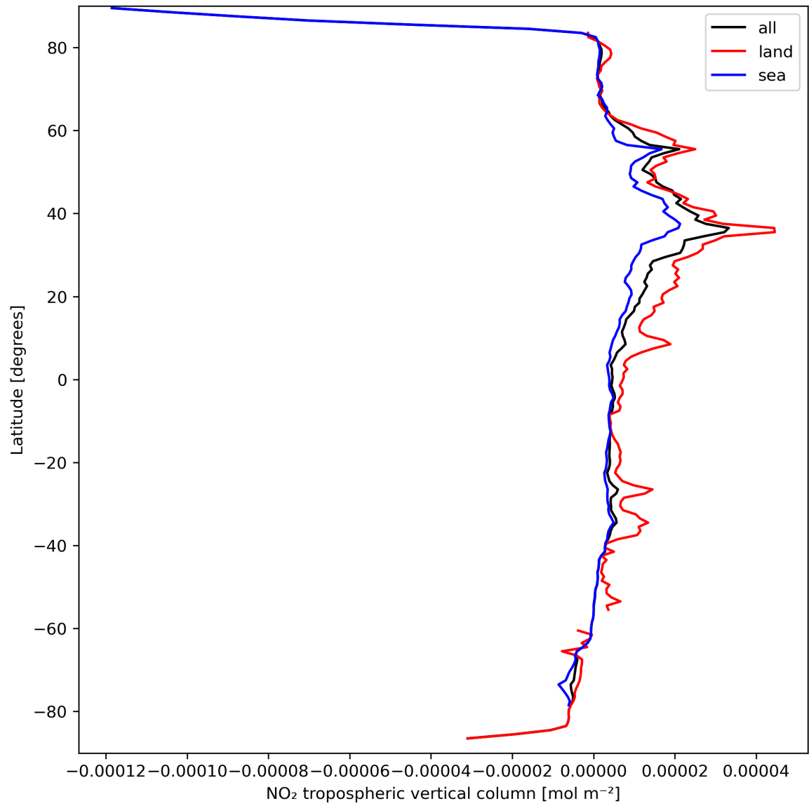
Figure 12: Zonal average of “NO 2 tropospheric vertical column” for 2024-03-25 to 2024-03-26.
