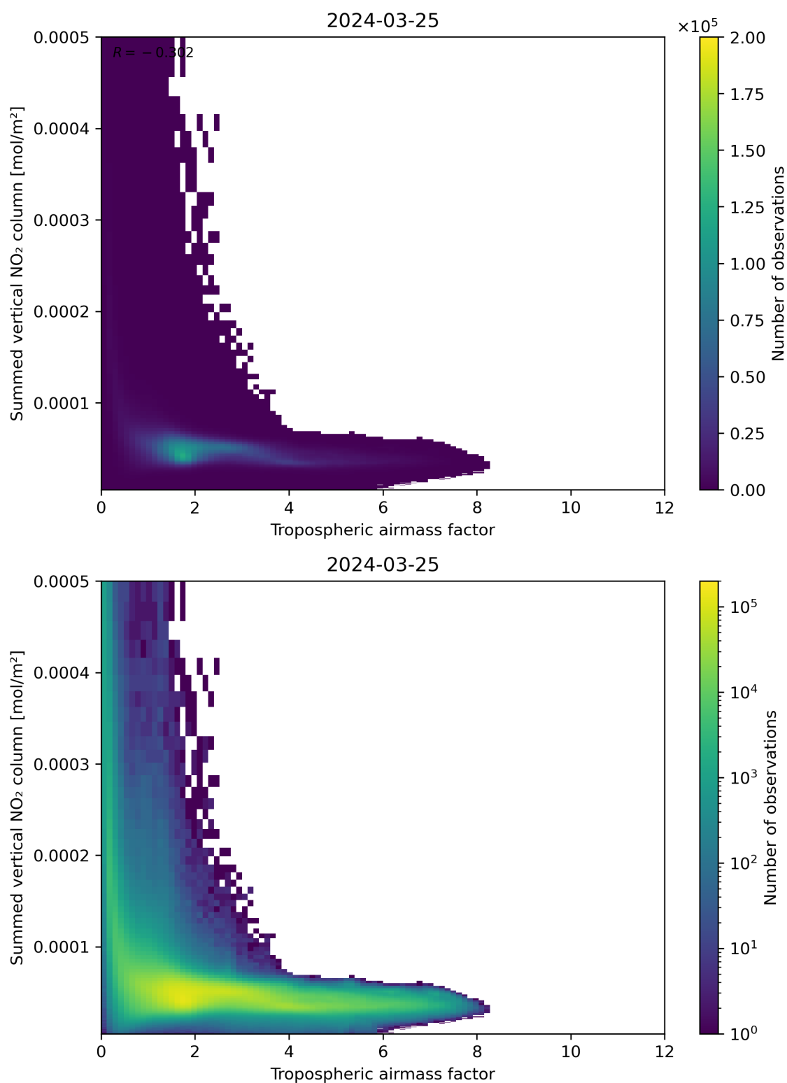
Figure 75: Scatter density plot of “Tropospheric air mass factor” against “Summed vertical NO 2 column” for 2024-03-25 to 2024-03-26.
