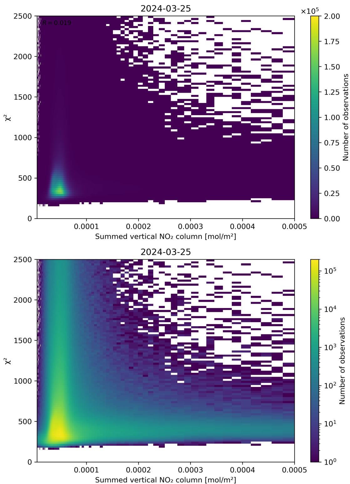
Figure 104: Scatter density plot of “Summed vertical NO 2 column” against “ \chi^2 ” for 2024-03-25 to 2024-03-26.
