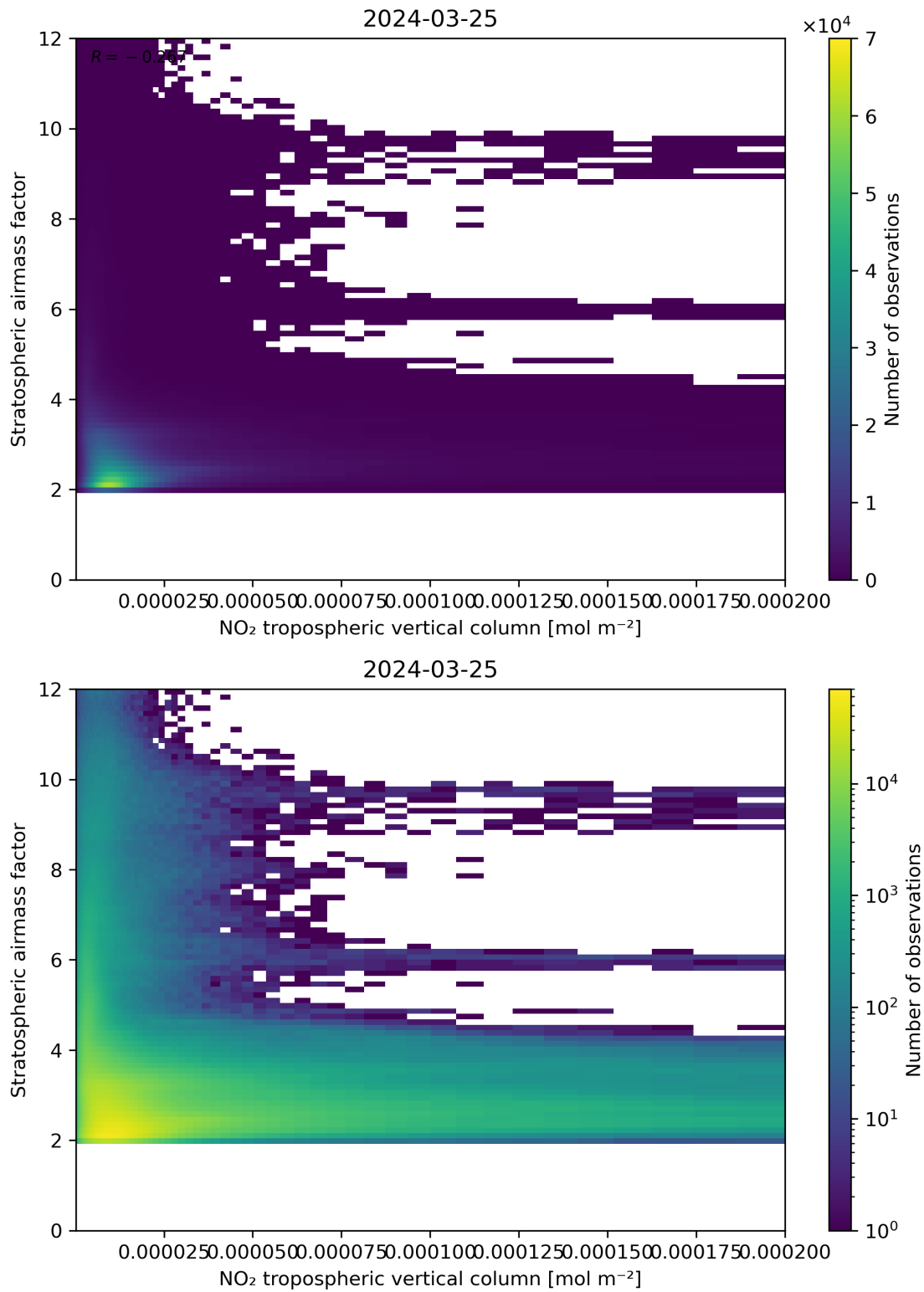
Figure 121: Scatter density plot of “NO 2 tropospheric vertical column” against “Stratospheric air mass factor” for 2024-03-25 to 2024-03-26.
