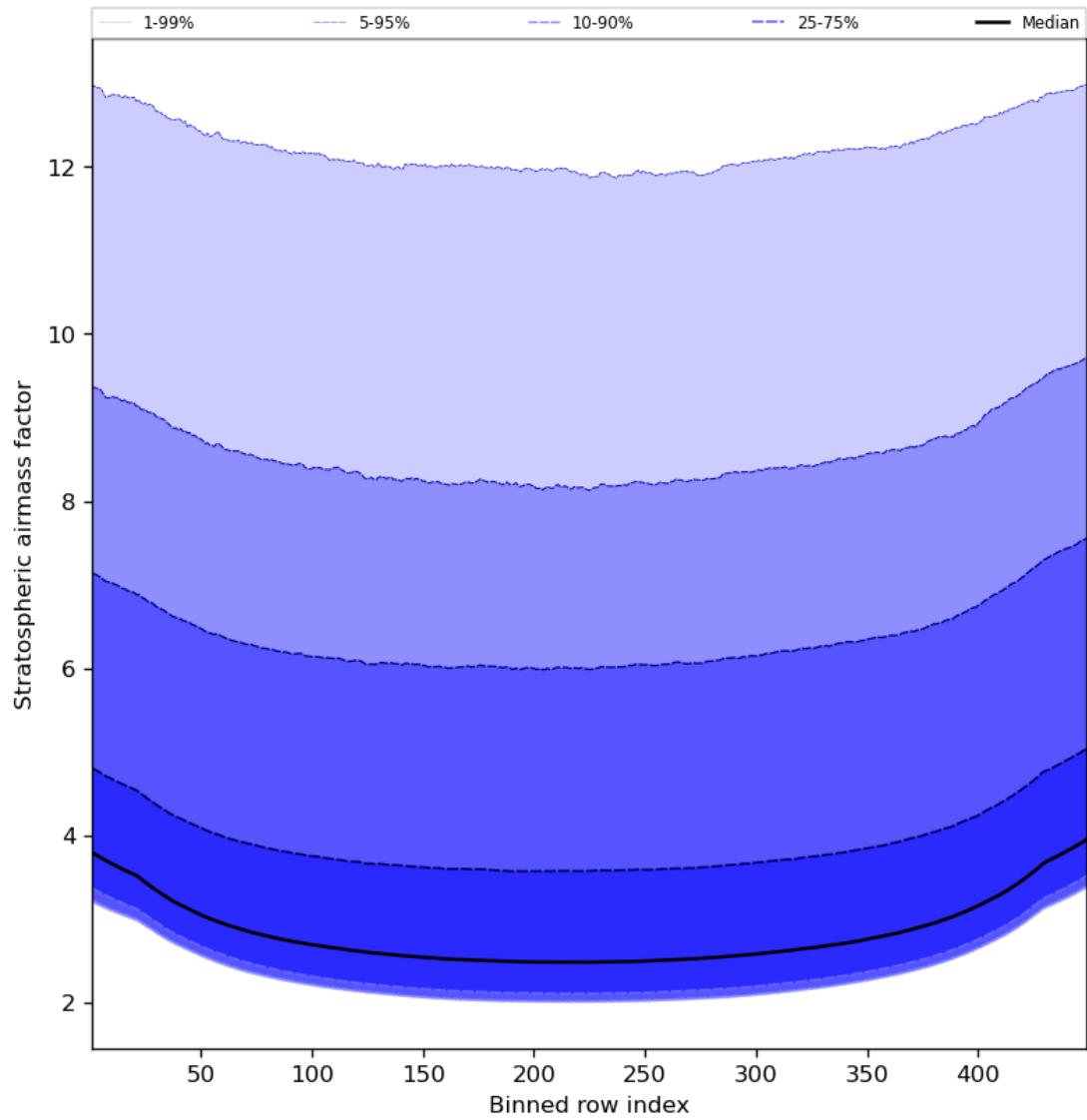
Figure 61: Along track statistics of “Stratospheric airmass factor” for 2024-03-25 to 2024-03-26
