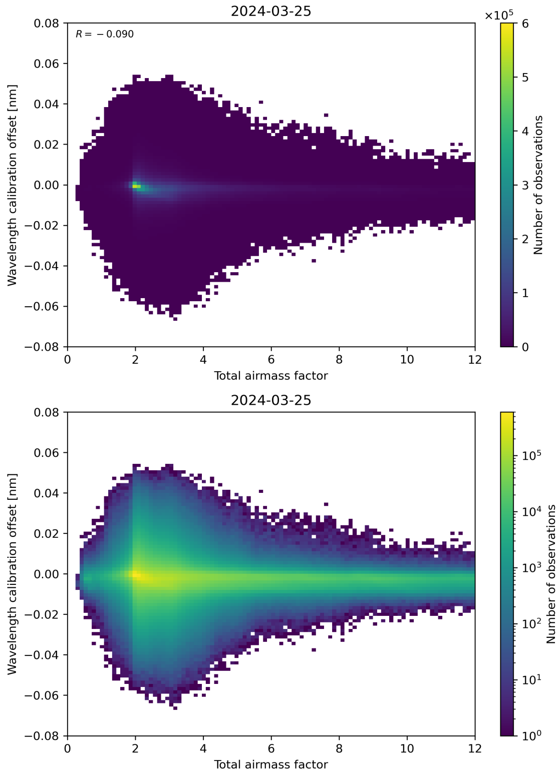
Figure 70: Scatter density plot of “Total airmass factor” against “Wavelength calibration offset” for 2024-03-25 to 2024-03-26.
