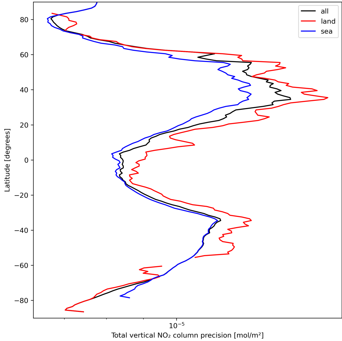
Figure 22: Zonal average of “Total vertical NO 2 column precision” for 2024-03-25 to 2024-03-26.
