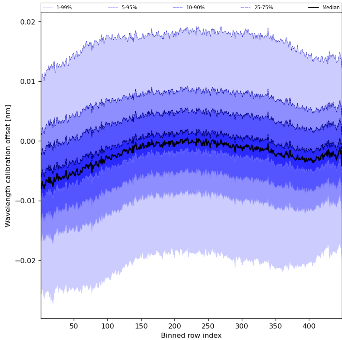
Figure 52: Along track statistics of “Wavelength calibration offset” for 2024-03-25 to 2024-03-26
