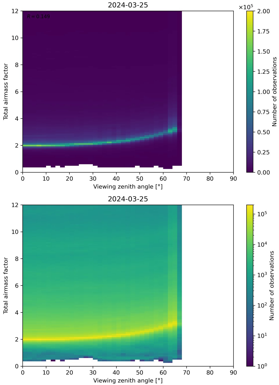
Figure 160: Scatter density plot of “Viewing zenith angle” against “Total airmass factor” for 2024-03-25 to 2024-03-26.
