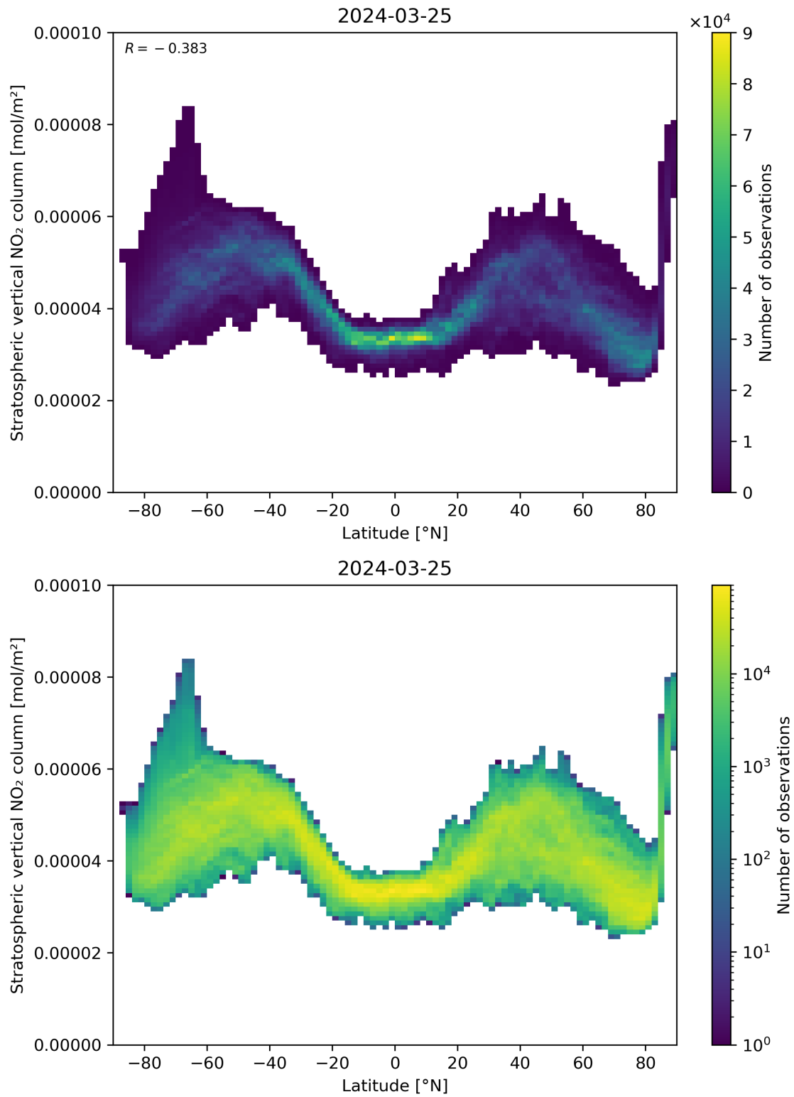
Figure 87: Scatter density plot of “Latitude” against “Stratospheric vertical NO 2 column” for 2024-03-25 to 2024-03-26.
