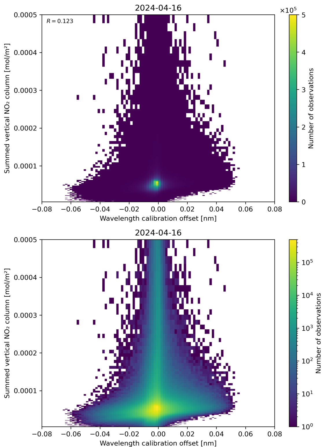
Figure 177: Scatter density plot of “Wavelength calibration offset” against “Summed vertical NO 2 column” for 2024-04-16 to 2024-04-17.
