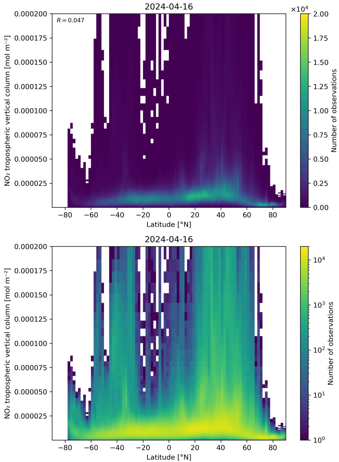
Figure 92: Scatter density plot of “Latitude” against “NO 2 tropospheric vertical column” for 2024-04-16 to 2024-04-17.
