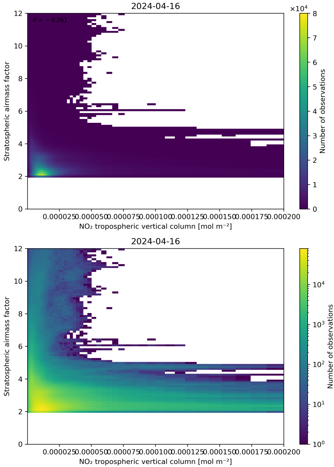
Figure 121: Scatter density plot of “NO 2 tropospheric vertical column” against “Stratospheric air mass factor” for 2024-04-16 to 2024-04-17.
