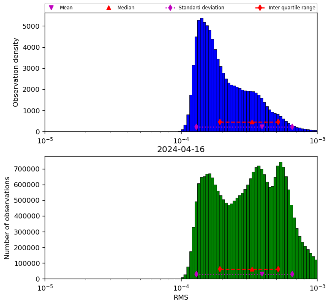
Figure 43: Histogram of “RMS” for 2024-04-16 to 2024-04-17
