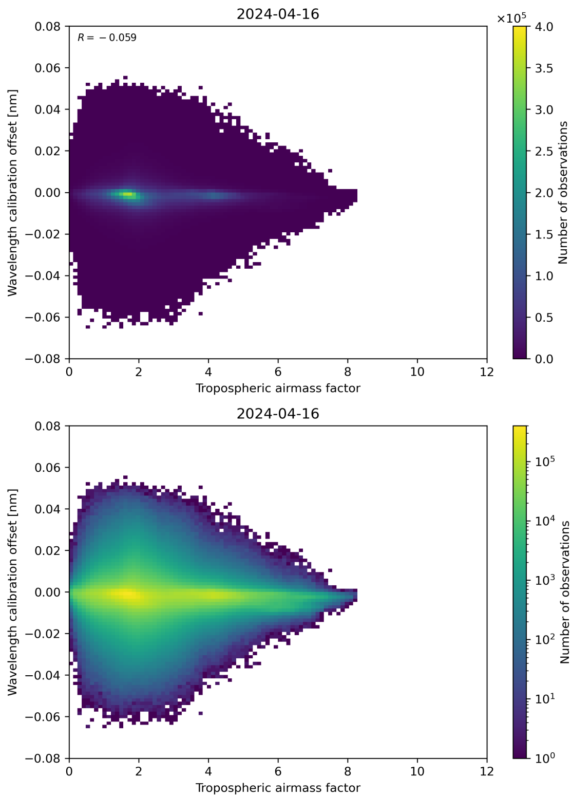
Figure 80: Scatter density plot of “Tropospheric airmass factor” against “Wavelength calibration offset” for 2024-04-16 to 2024-04-17.
