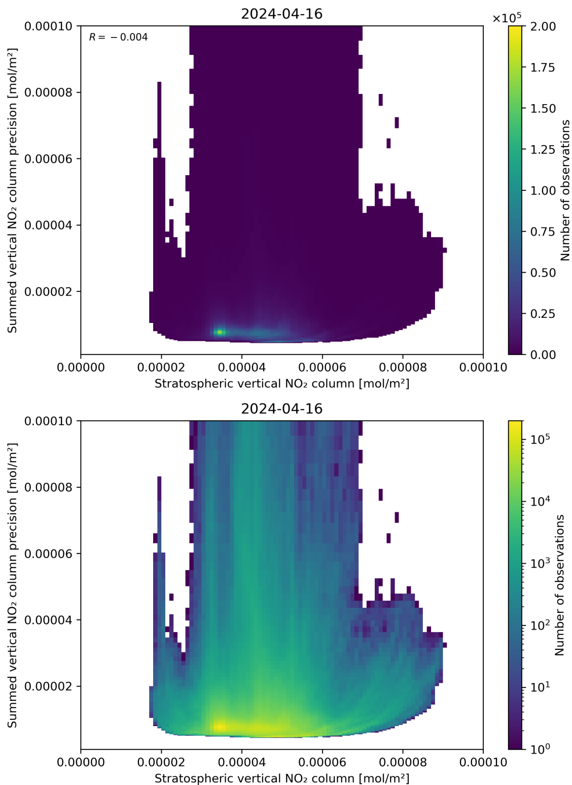
Figure 99: Scatter density plot of “Stratospheric vertical NO 2 column” against “Summed vertical NO 2 column precision” for 2024-04-16 to 2024-04-17.
