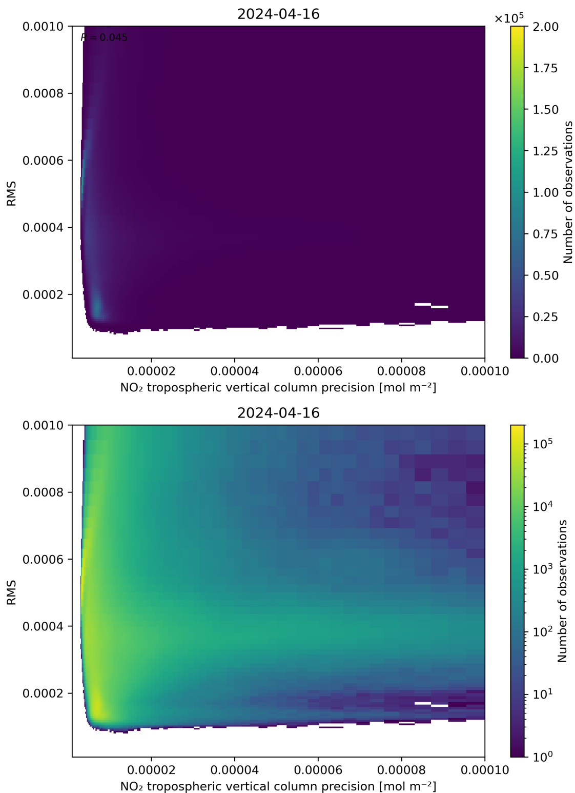
Figure 140: Scatter density plot of “NO 2 tropospheric vertical column precision” against “RMS” for 2024-04-16 to 2024-04-17.
