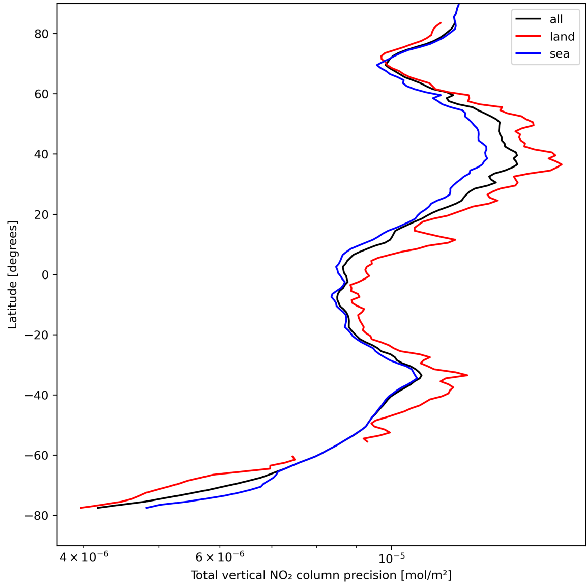
Figure 22: Zonal average of “Total vertical NO 2 column precision” for 2024-04-16 to 2024-04-17.
