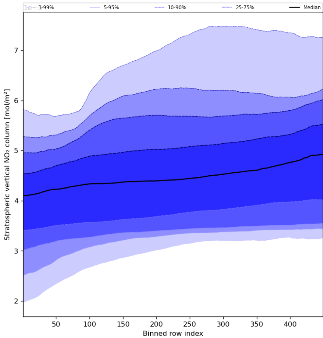
Figure 53: Along track statistics of “Stratospheric vertical NO 2 column” for 2024-04-16 to 2024-04-17
