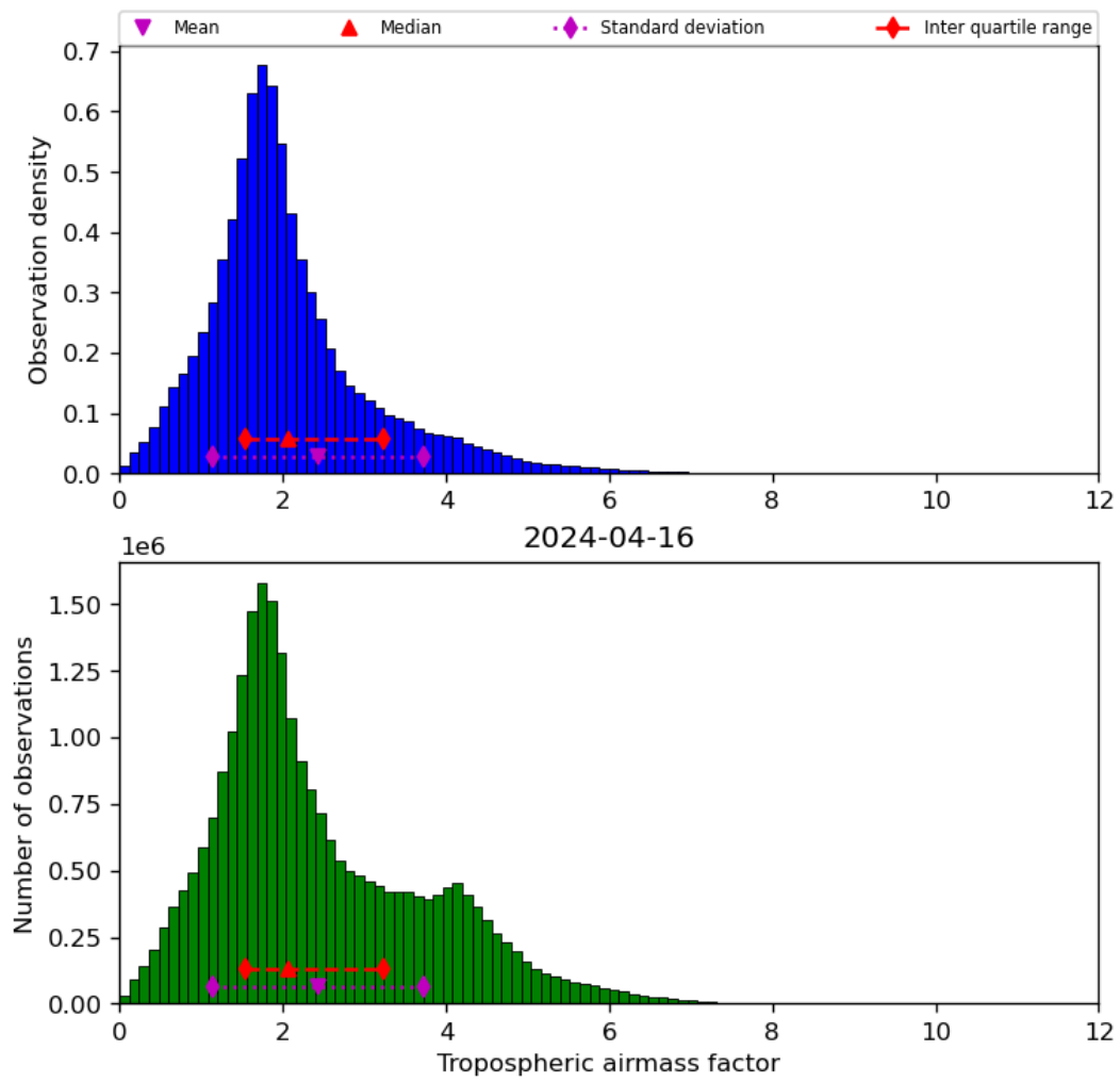
Figure 31: Histogram of “Tropospheric airmass factor” for 2024-04-16 to 2024-04-17
