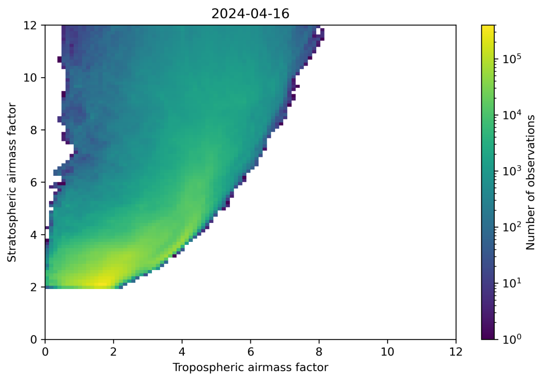
Figure 71: Scatter density plot of “Tropospheric airmass factor” against “Stratospheric airmass factor” for 2024-04-16 to 2024-04-17.
