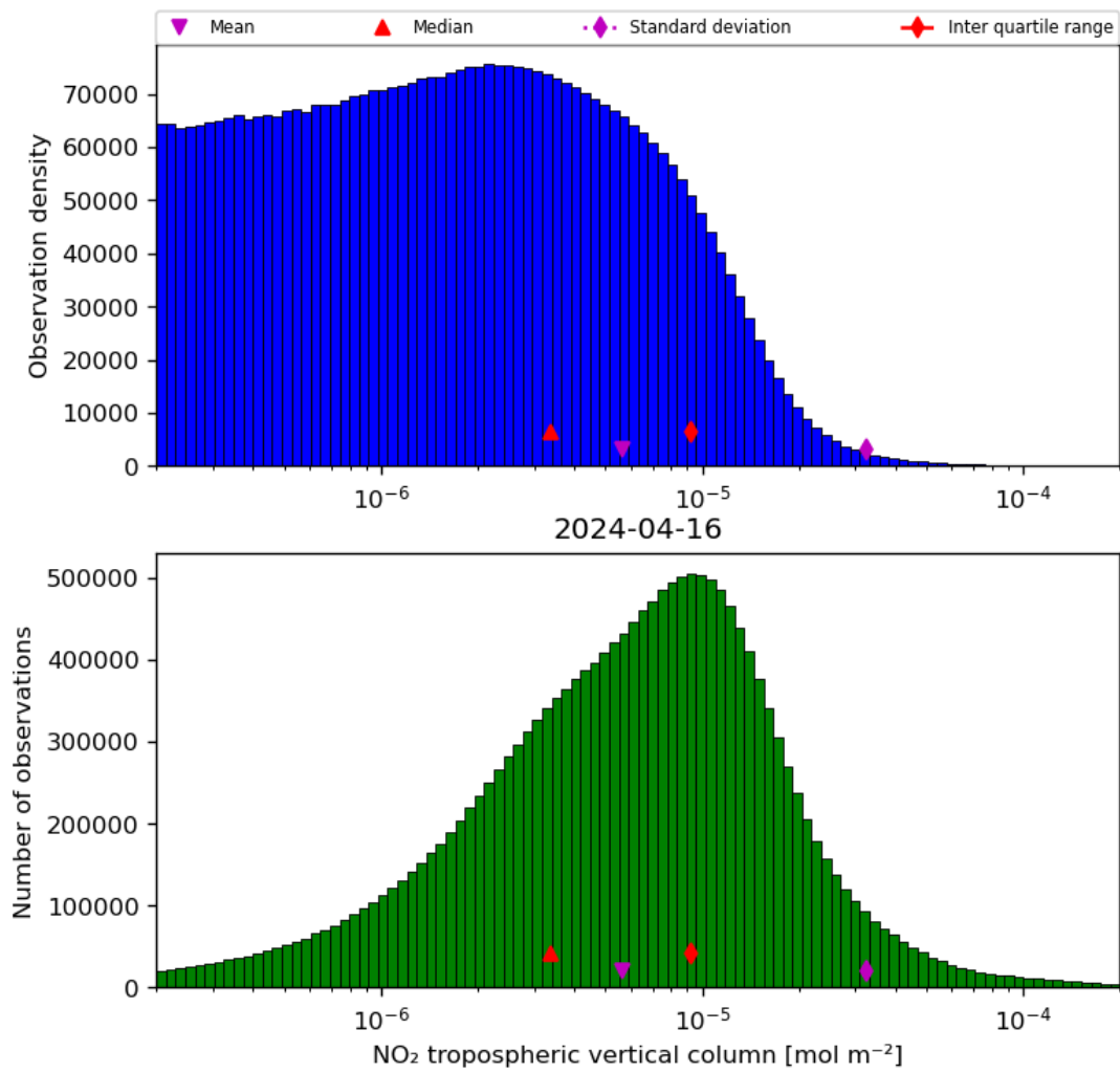
Figure 29: Histogram of “NO 2 tropospheric vertical column” for 2024-04-16 to 2024-04-17
