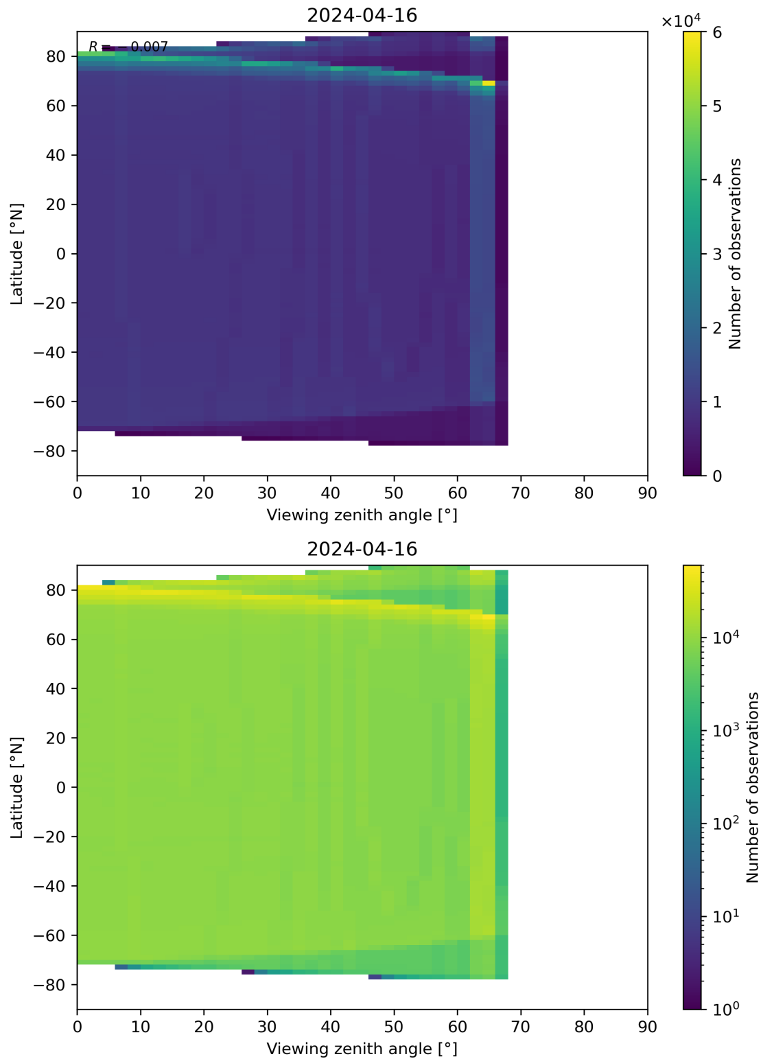
Figure 163: Scatter density plot of “Viewing zenith angle” against “Latitude” for 2024-04-16 to 2024-04-17.
