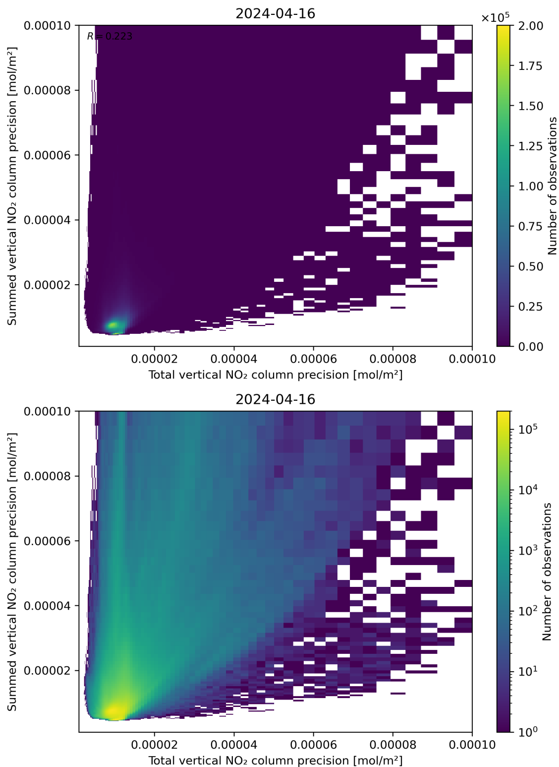
Figure 118: Scatter density plot of “Total vertical NO 2 column precision” against “Summed vertical NO 2 column precision” for 2024-04-16 to 2024-04-17.
