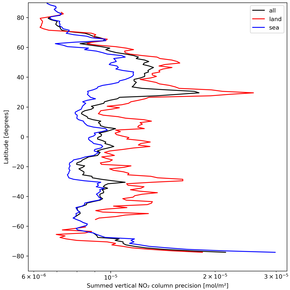
Figure 24: Zonal average of “Summed vertical NO 2 column precision” for 2024-04-16 to 2024-04-17.
