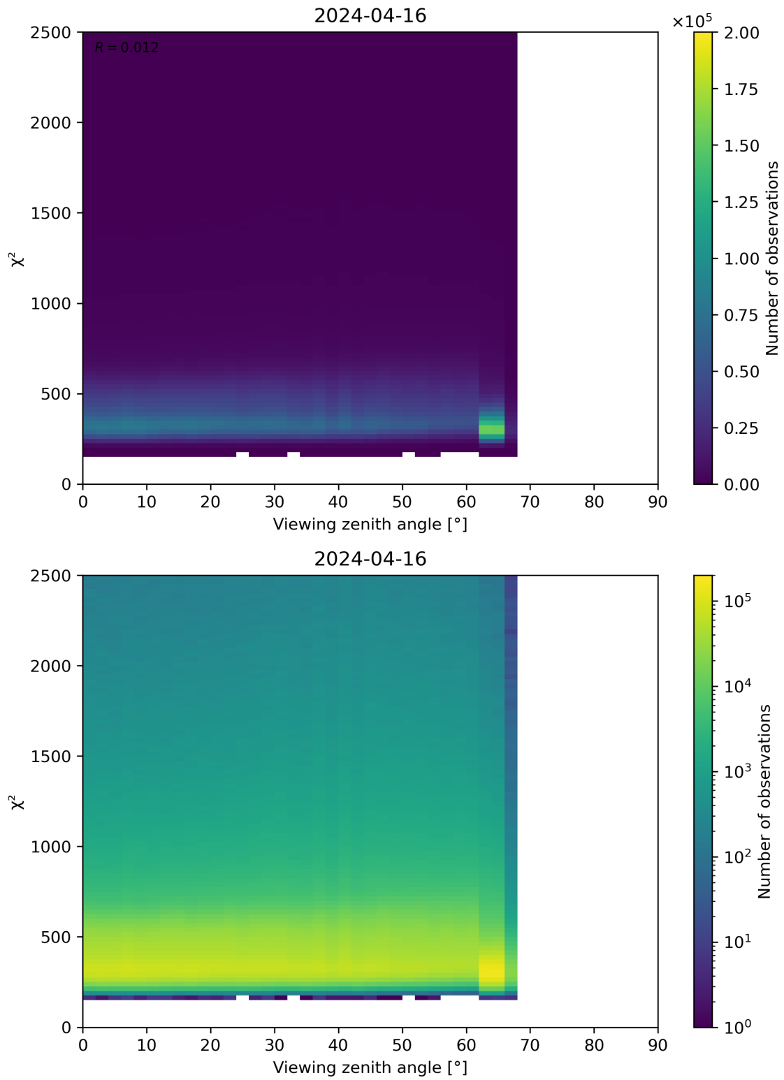
Figure 162: Scatter density plot of “Viewing zenith angle” against “ \chi^2 ” for 2024-04-16 to 2024-04-17.
