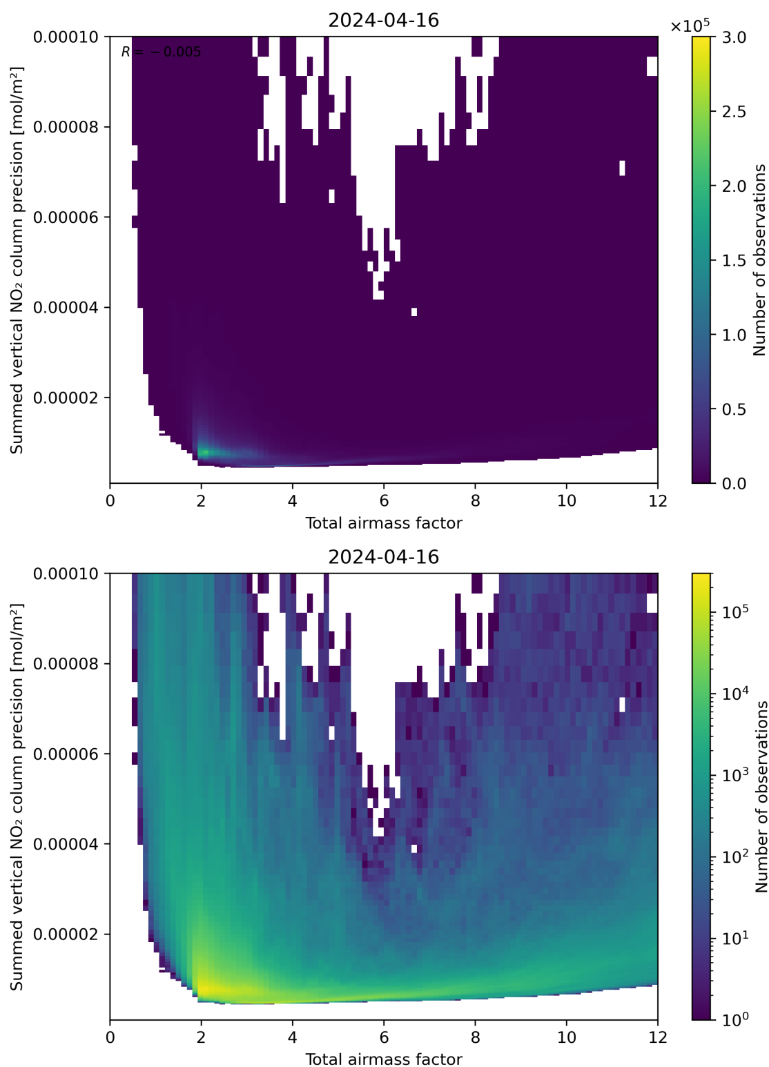
Figure 66: Scatter density plot of “Total airmass factor” against “Summed vertical NO 2 column precision” for 2024-04-16 to 2024-04-17.
