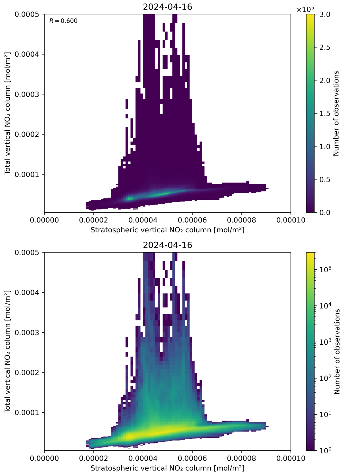
Figure 100: Scatter density plot of “Stratospheric vertical NO 2 column” against “Total vertical NO 2 column” for 2024-04-16 to 2024-04-17.
