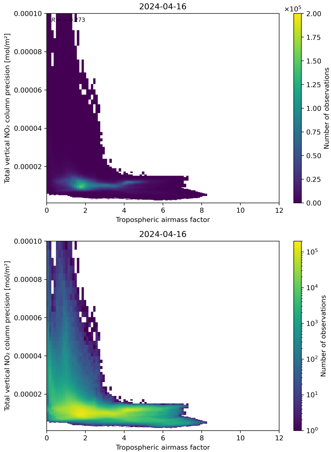
Figure 78: Scatter density plot of “Tropospheric air mass factor” against “Total vertical NO 2 column precision” for 2024-04-16 to 2024-04-17.
