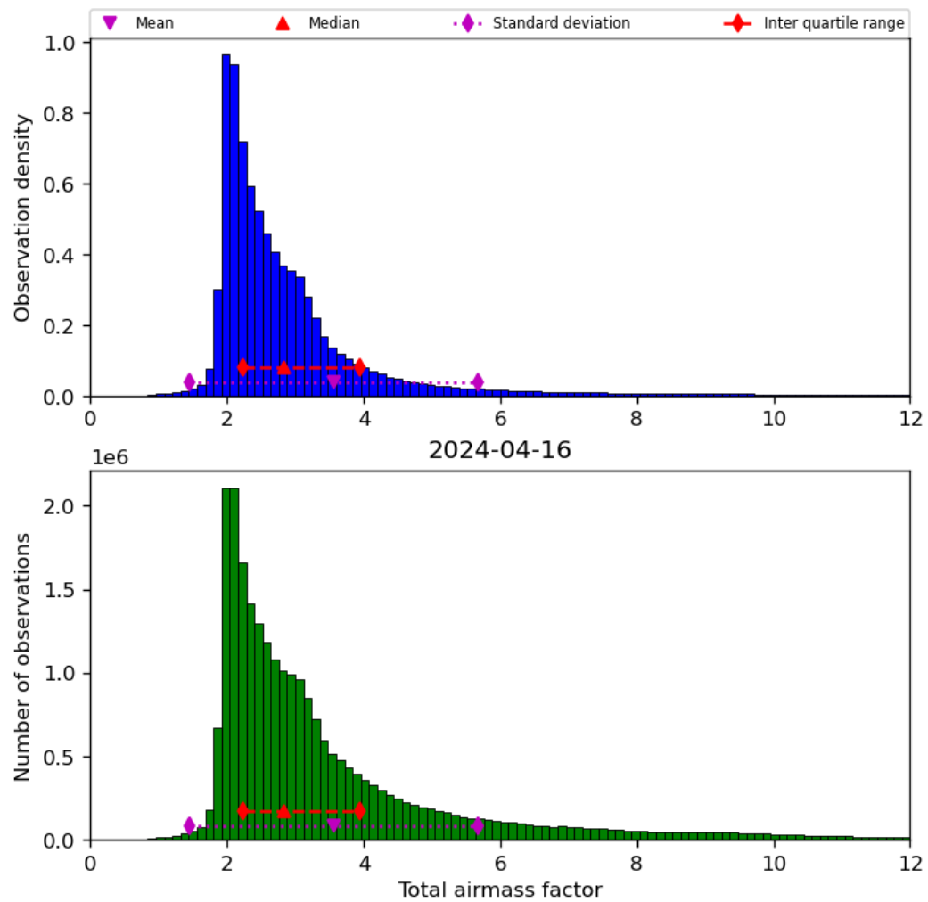
Figure 32: Histogram of “Total airmass factor” for 2024-04-16 to 2024-04-17
