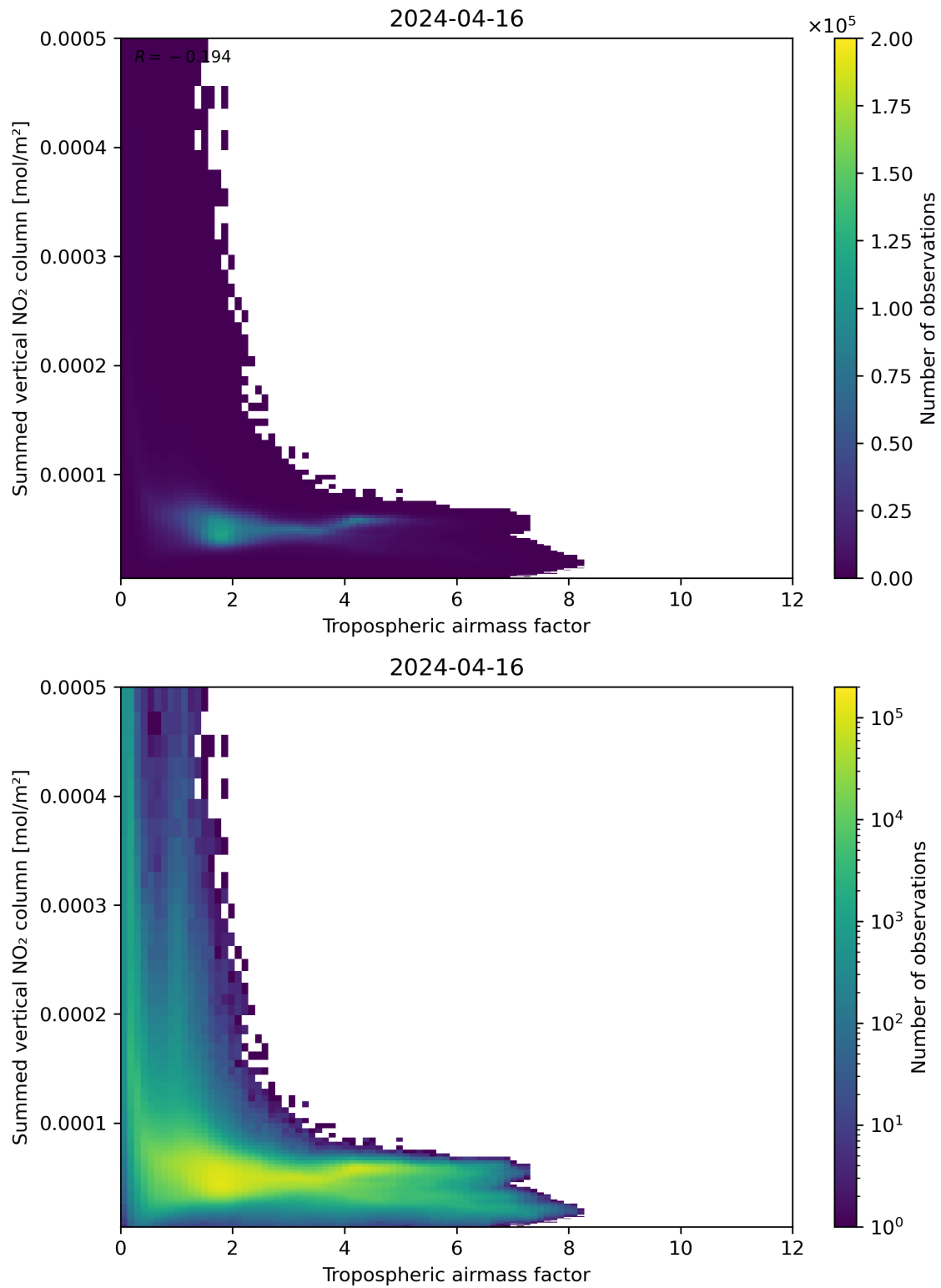
Figure 75: Scatter density plot of “Tropospheric air mass factor” against “Summed vertical NO 2 column” for 2024-04-16 to 2024-04-17.
