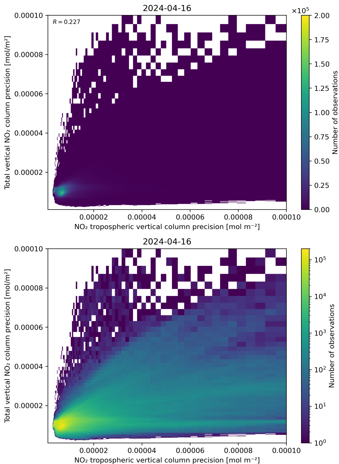
Figure 139: Scatter density plot of “NO 2 tropospheric vertical column precision” against “Total vertical NO 2 column precision” for 2024-04-16 to 2024-04-17.
