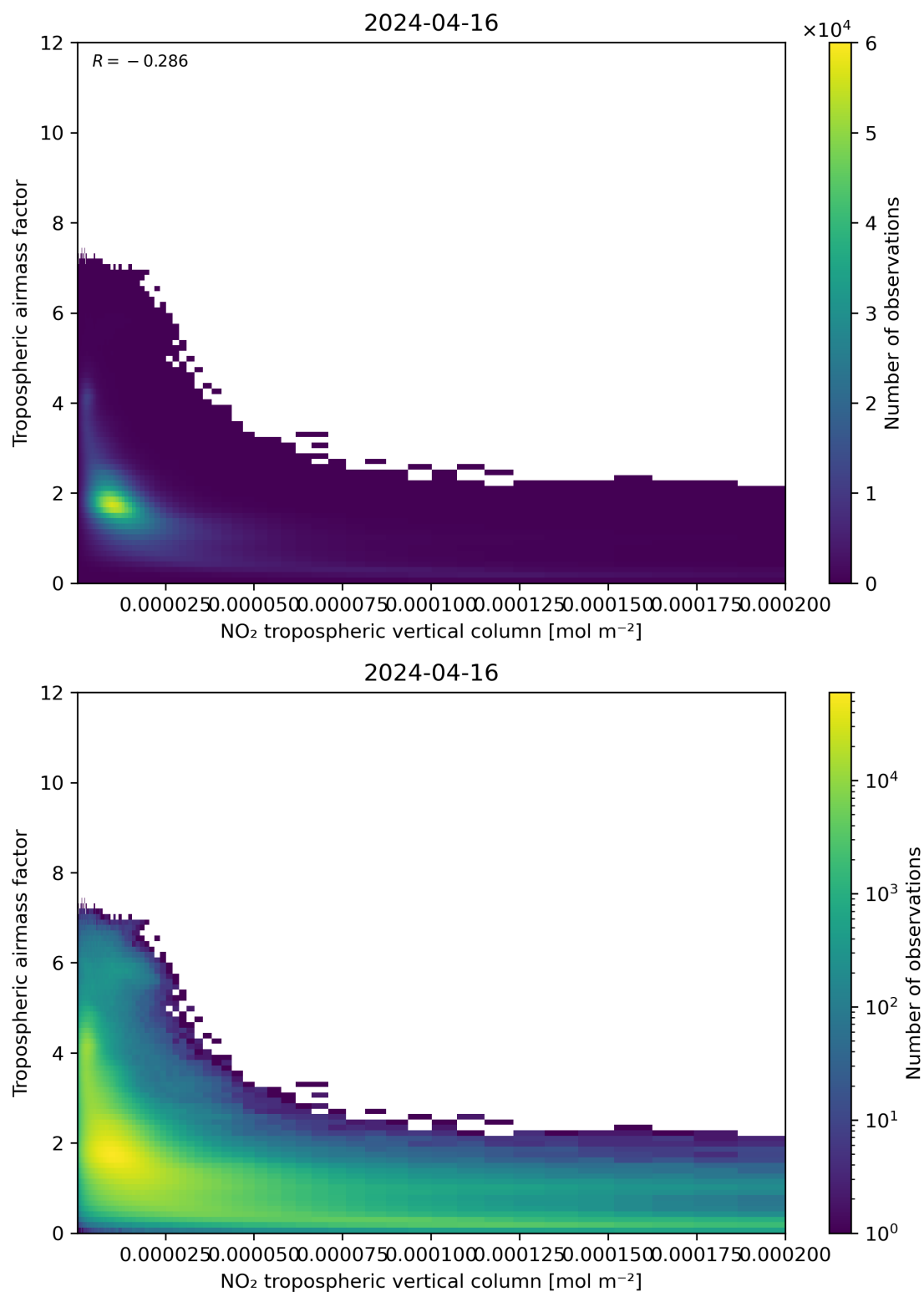
Figure 123: Scatter density plot of “NO 2 tropospheric vertical column” against “Tropospheric air mass factor” for 2024-04-16 to 2024-04-17.
