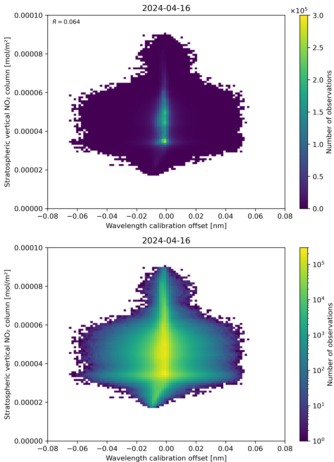
Figure 176: Scatter density plot of “Wavelength calibration offset” against “Stratospheric vertical NO 2 column” for 2024-04-16 to 2024-04-17.
