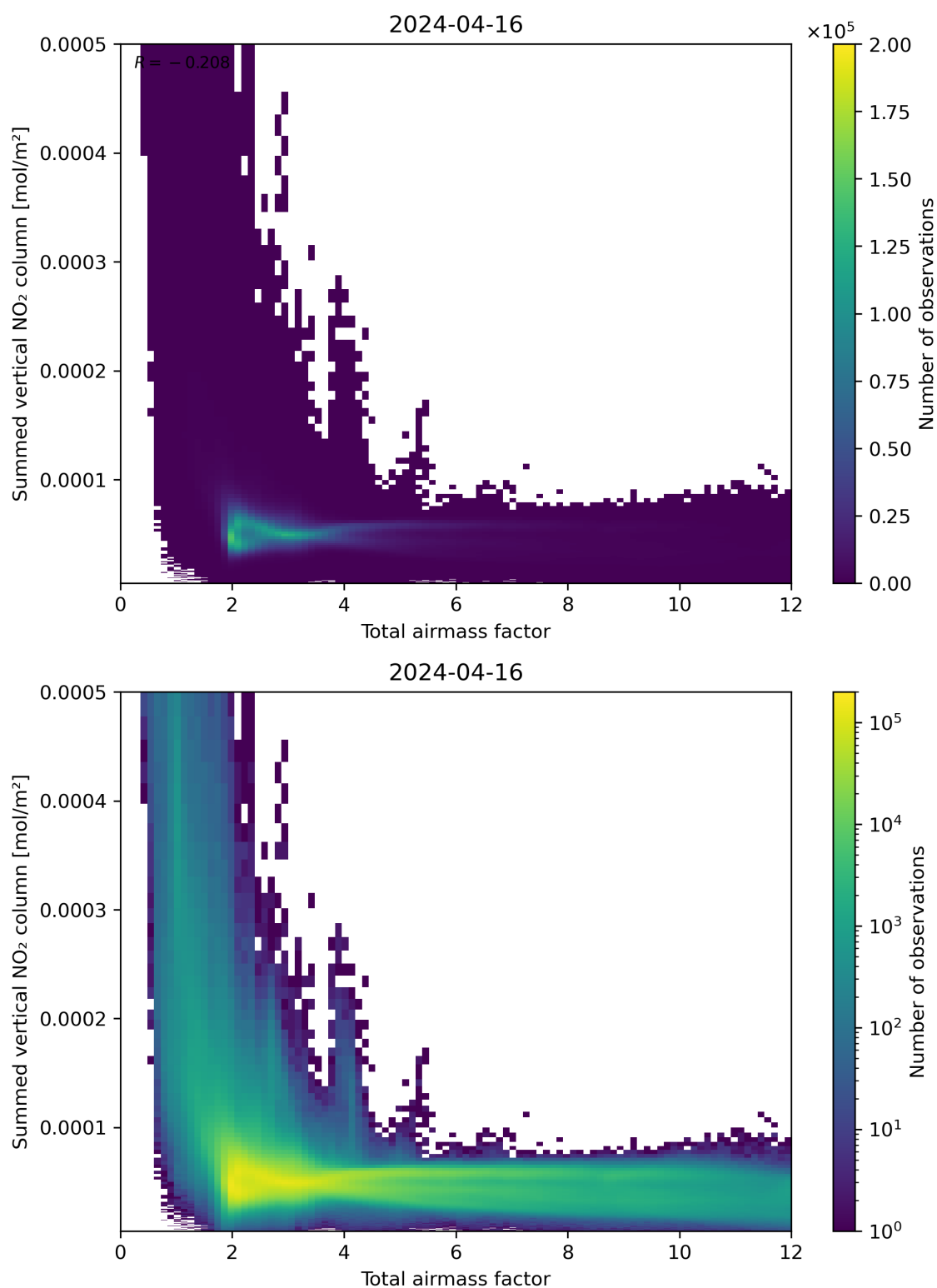
Figure 65: Scatter density plot of “Total airmass factor” against “Summed vertical NO 2 column” for 2024-04-16 to 2024-04-17.
