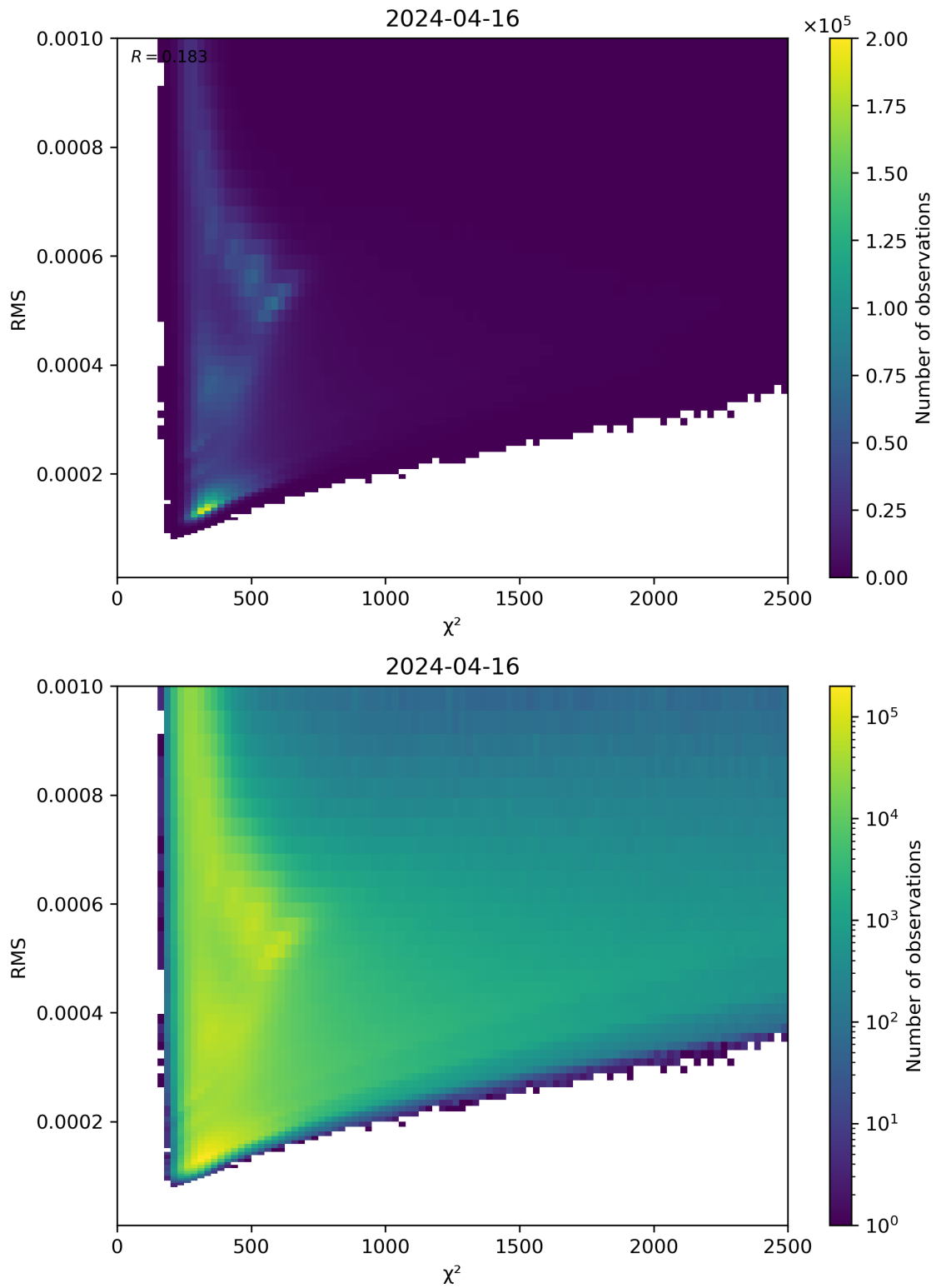
Figure 82: Scatter density plot of “ \chi^2 ” against “RMS” for 2024-04-16 to 2024-04-17.
