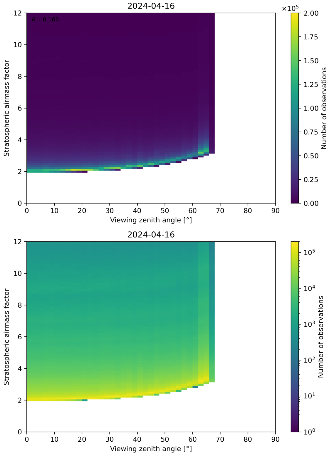
Figure 159: Scatter density plot of “Viewing zenith angle” against “Stratospheric airmass factor” for 2024-04-16 to 2024-04-17.
