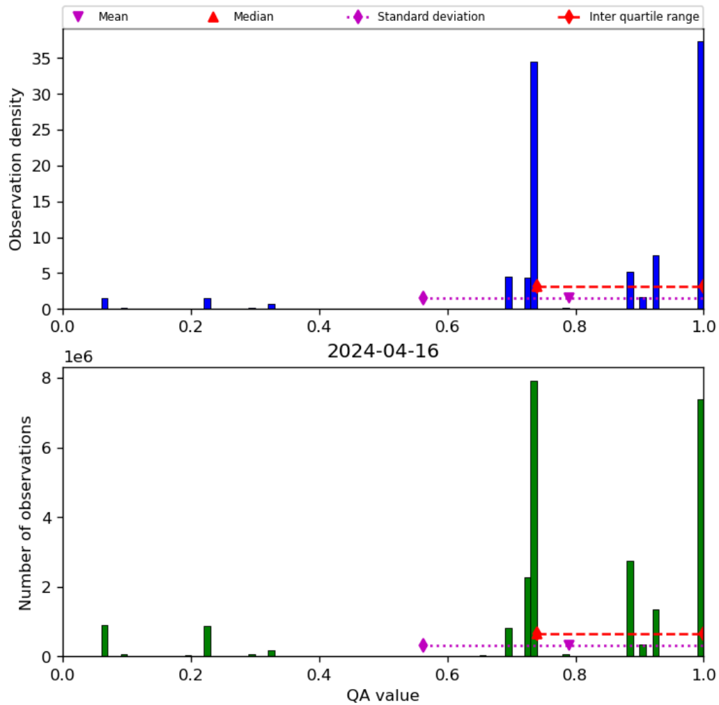
Figure 28: Histogram of “QA value” for 2024-04-16 to 2024-04-17
