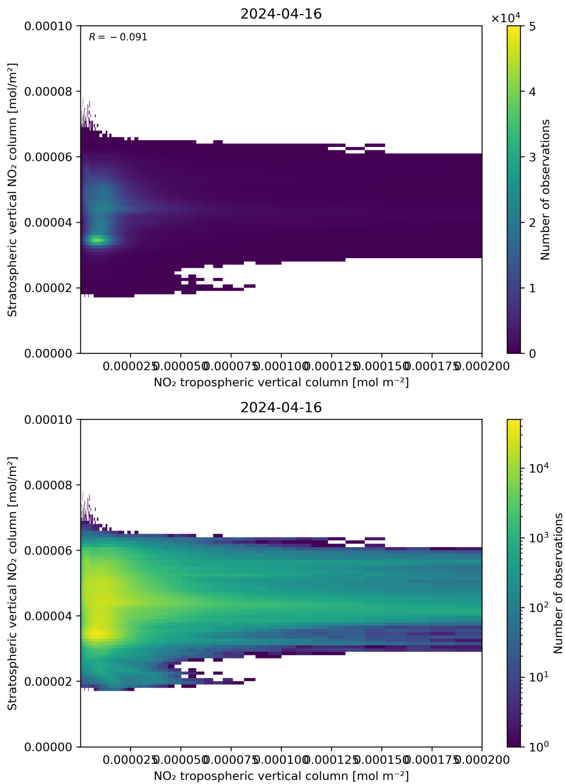
Figure 125: Scatter density plot of “NO 2 tropospheric vertical column” against “Stratospheric vertical NO 2 column” for 2024-04-16 to 2024-04-17.
