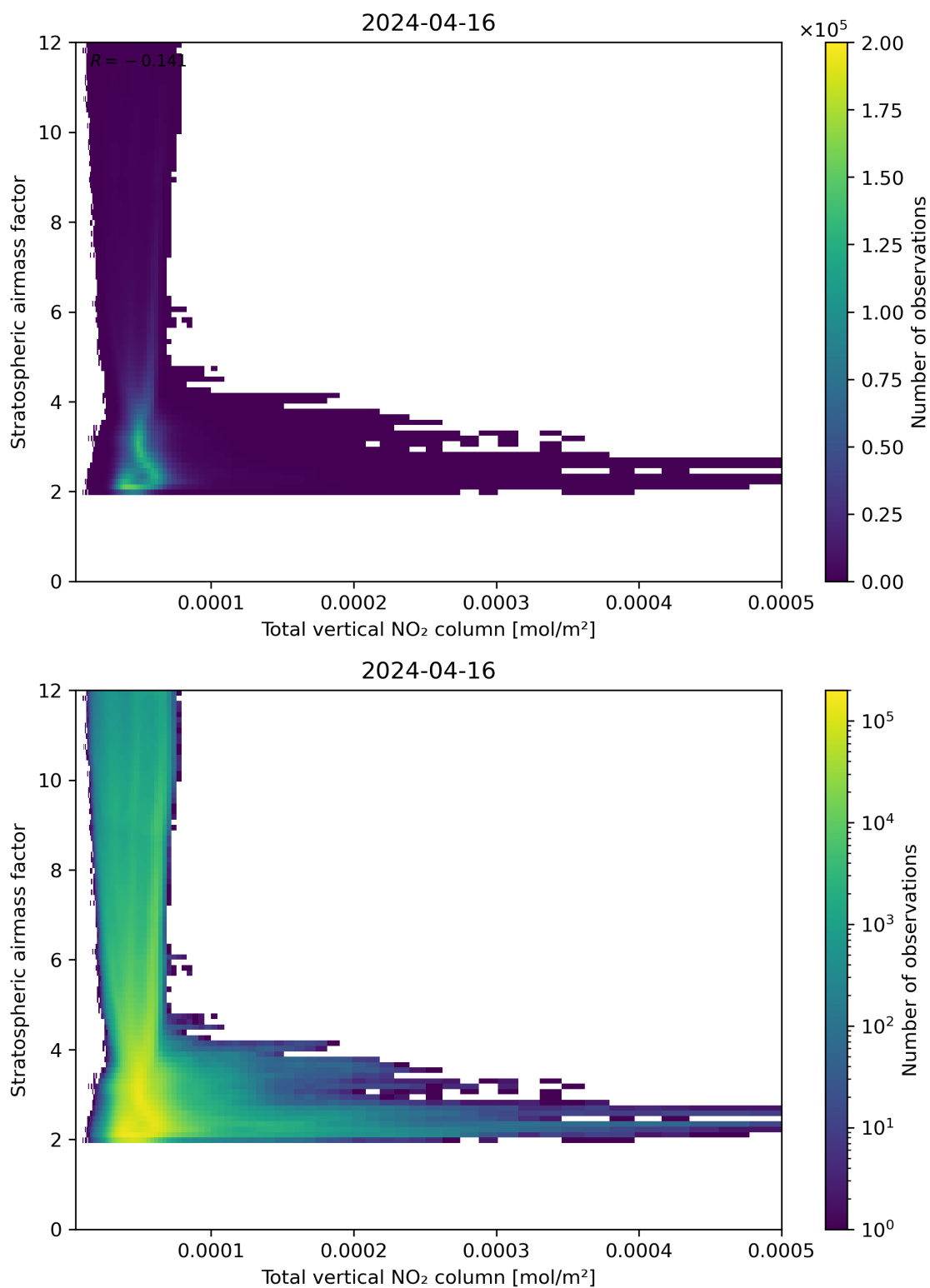
Figure 110: Scatter density plot of “Total vertical NO 2 column” against “Stratospheric airmass factor” for 2024-04-16 to 2024-04-17.
