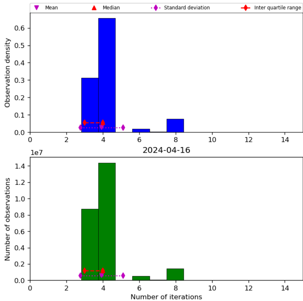
Figure 34: Histogram of “Number of iterations” for 2024-04-16 to 2024-04-17
