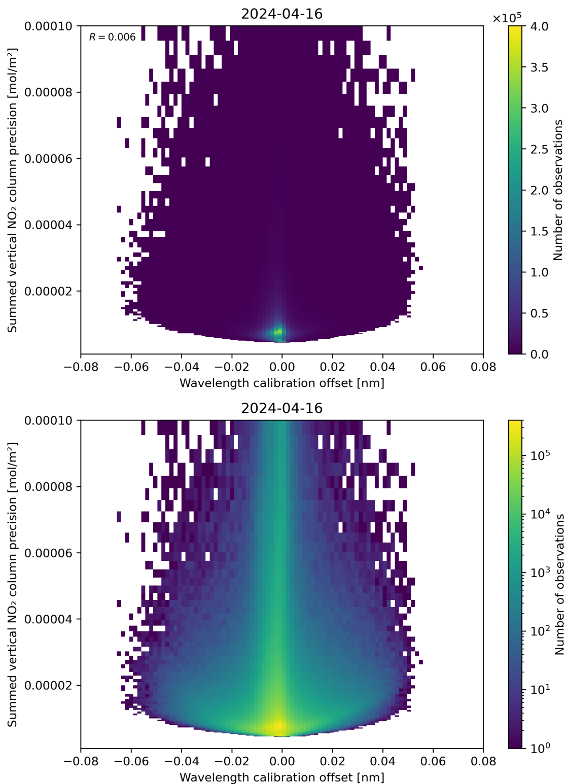
Figure 178: Scatter density plot of “Wavelength calibration offset” against “Summed vertical NO 2 column precision” for 2024-04-16 to 2024-04-17.
