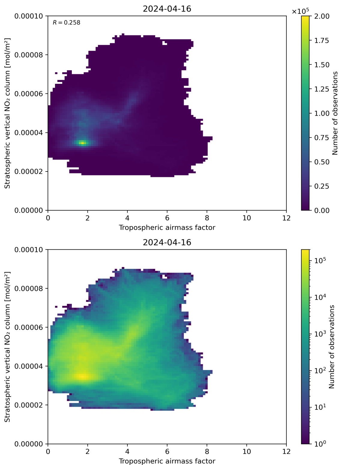
Figure 74: Scatter density plot of “Tropospheric air mass factor” against “Stratospheric vertical NO 2 column” for 2024-04-16 to 2024-04-17.
