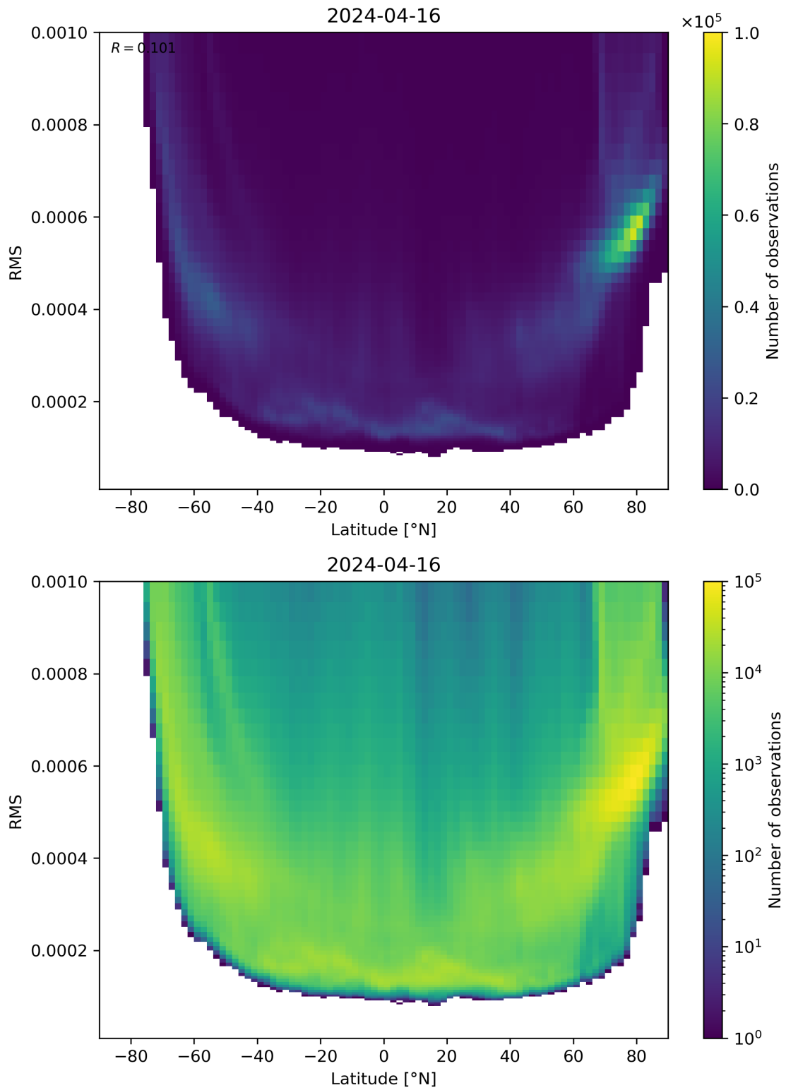
Figure 94: Scatter density plot of “Latitude” against “RMS” for 2024-04-16 to 2024-04-17.
