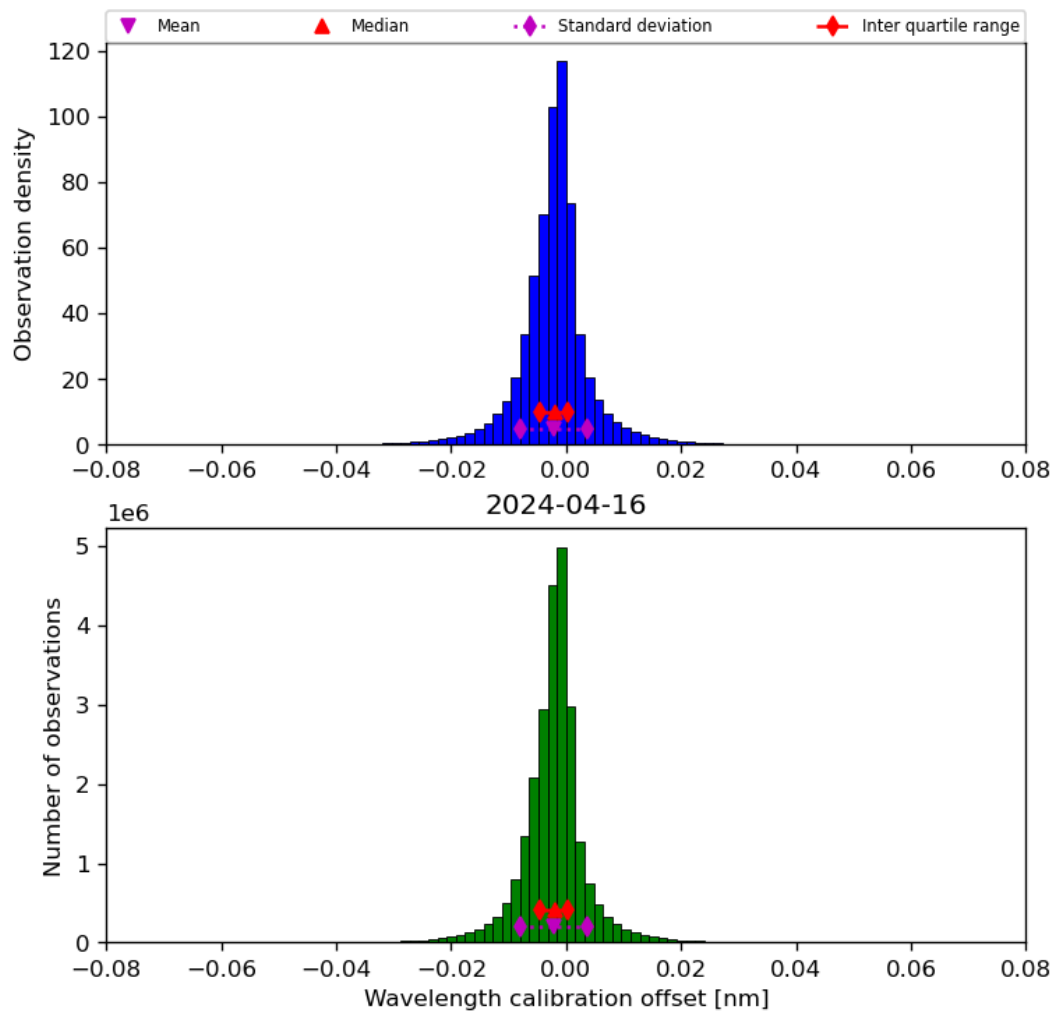
Figure 35: Histogram of “Wavelength calibration offset” for 2024-04-16 to 2024-04-17
