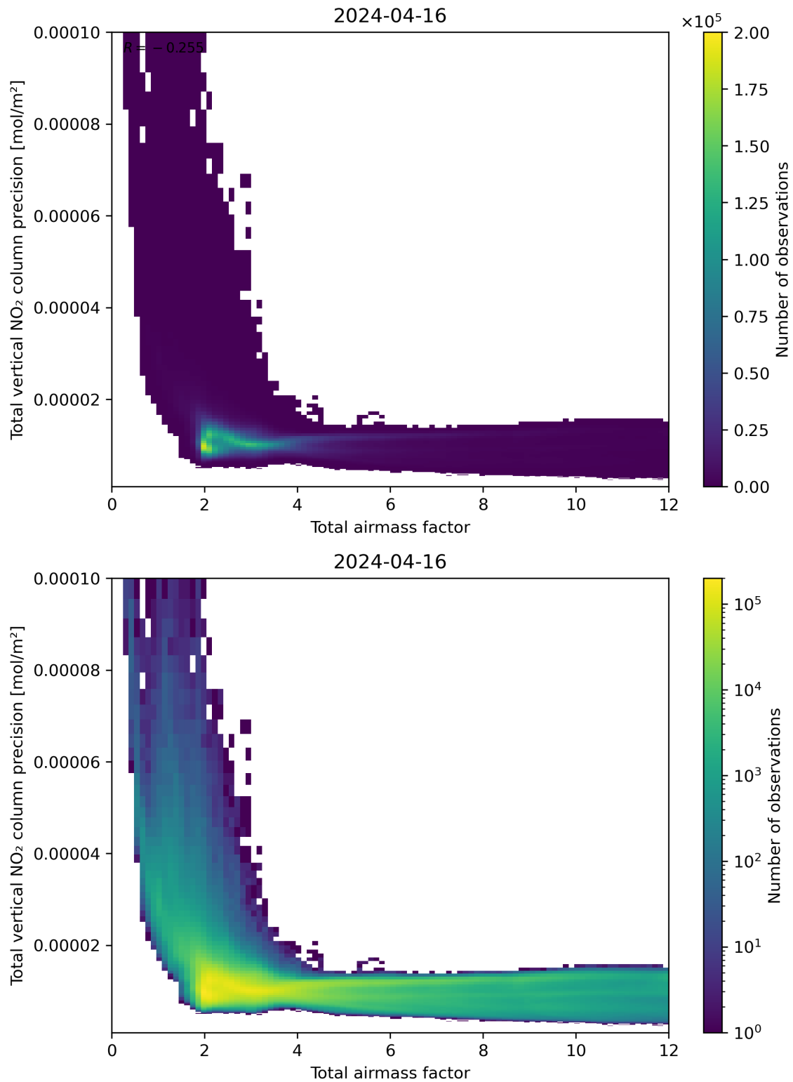
Figure 68: Scatter density plot of “Total airmass factor” against “Total vertical NO 2 column precision” for 2024-04-16 to 2024-04-17.
