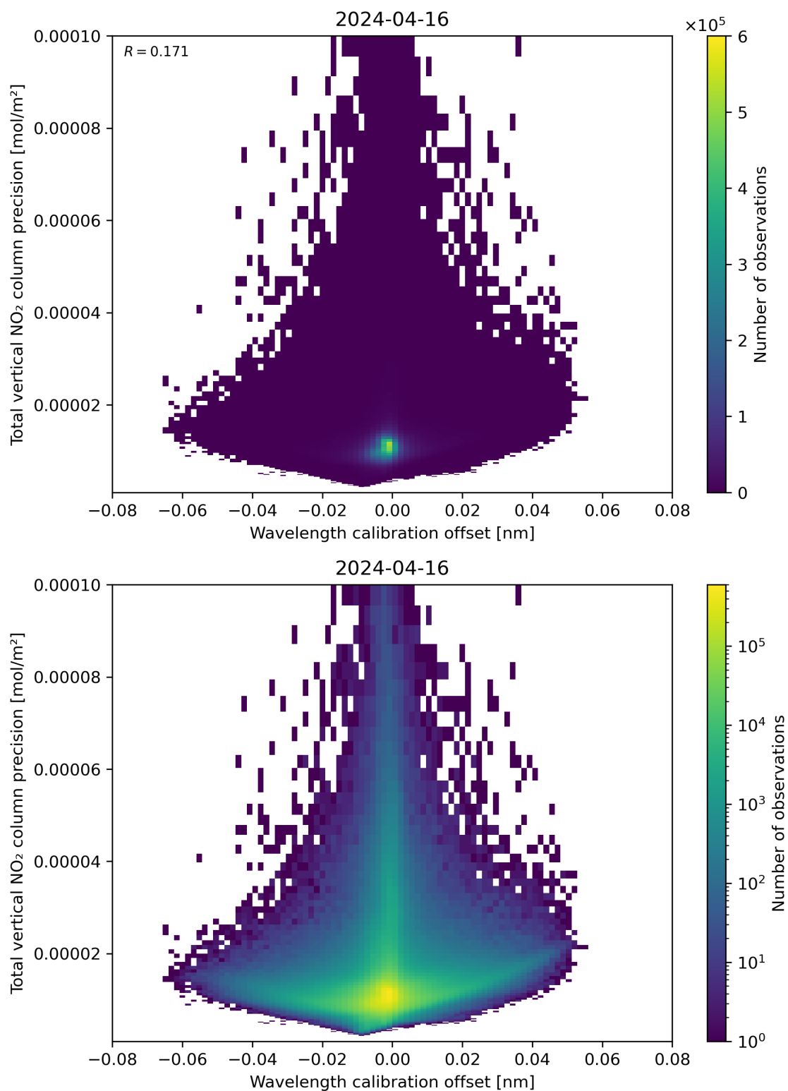
Figure 180: Scatter density plot of “Wavelength calibration offset” against “Total vertical NO 2 column precision” for 2024-04-16 to 2024-04-17.
