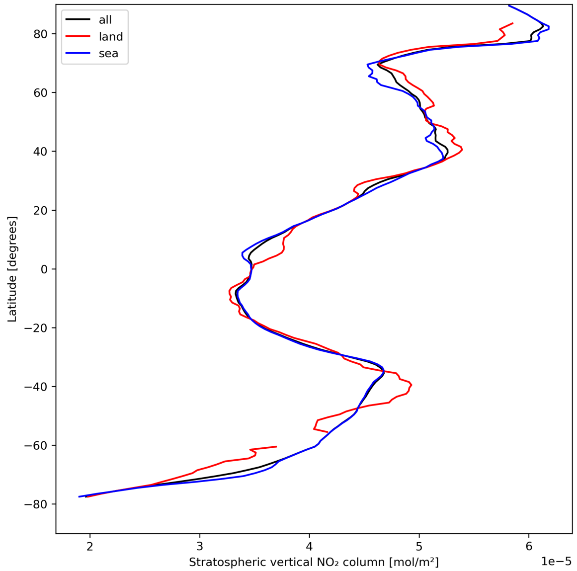
Figure 19: Zonal average of “Stratospheric vertical NO 2 column” for 2024-04-16 to 2024-04-17.
