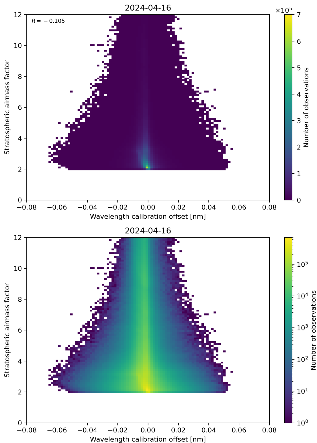
Figure 174: Scatter density plot of “Wavelength calibration offset” against “Stratospheric airmass factor” for 2024-04-16 to 2024-04-17.
