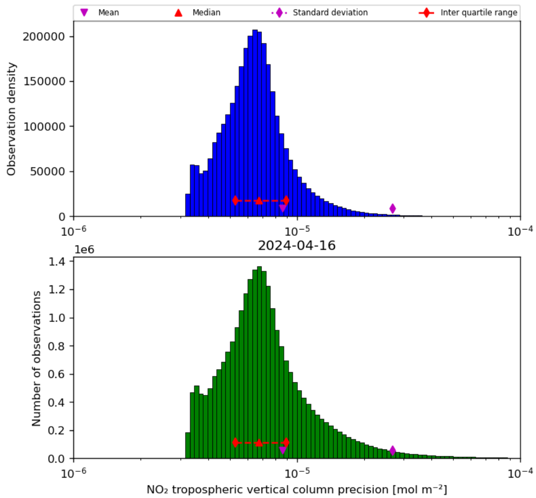
Figure 30: Histogram of “NO 2 tropospheric vertical column precision” for 2024-04-16 to 2024-04-17
