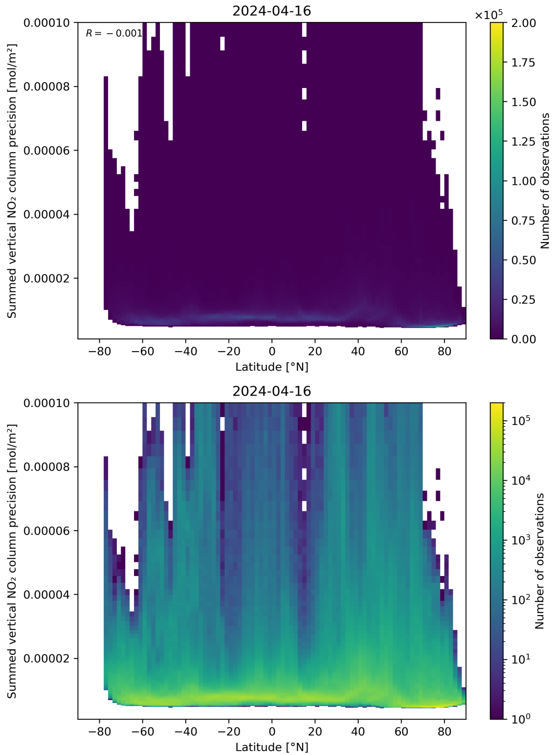
Figure 89: Scatter density plot of “Latitude” against “Summed vertical NO 2 column precision” for 2024-04-16 to 2024-04-17.
