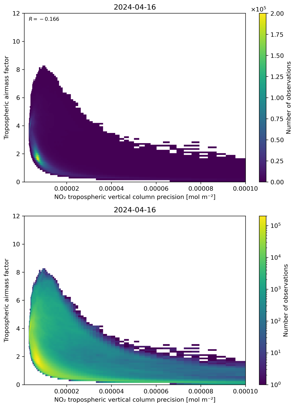
Figure 133: Scatter density plot of “NO 2 tropospheric vertical column precision” against “Tropospheric airmass factor” for 2024-04-16 to 2024-04-17.
