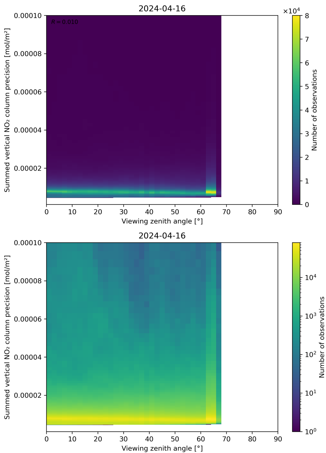
Figure 166: Scatter density plot of “Viewing zenith angle” against “Summed vertical NO 2 column precision” for 2024-04-16 to 2024-04-17.
