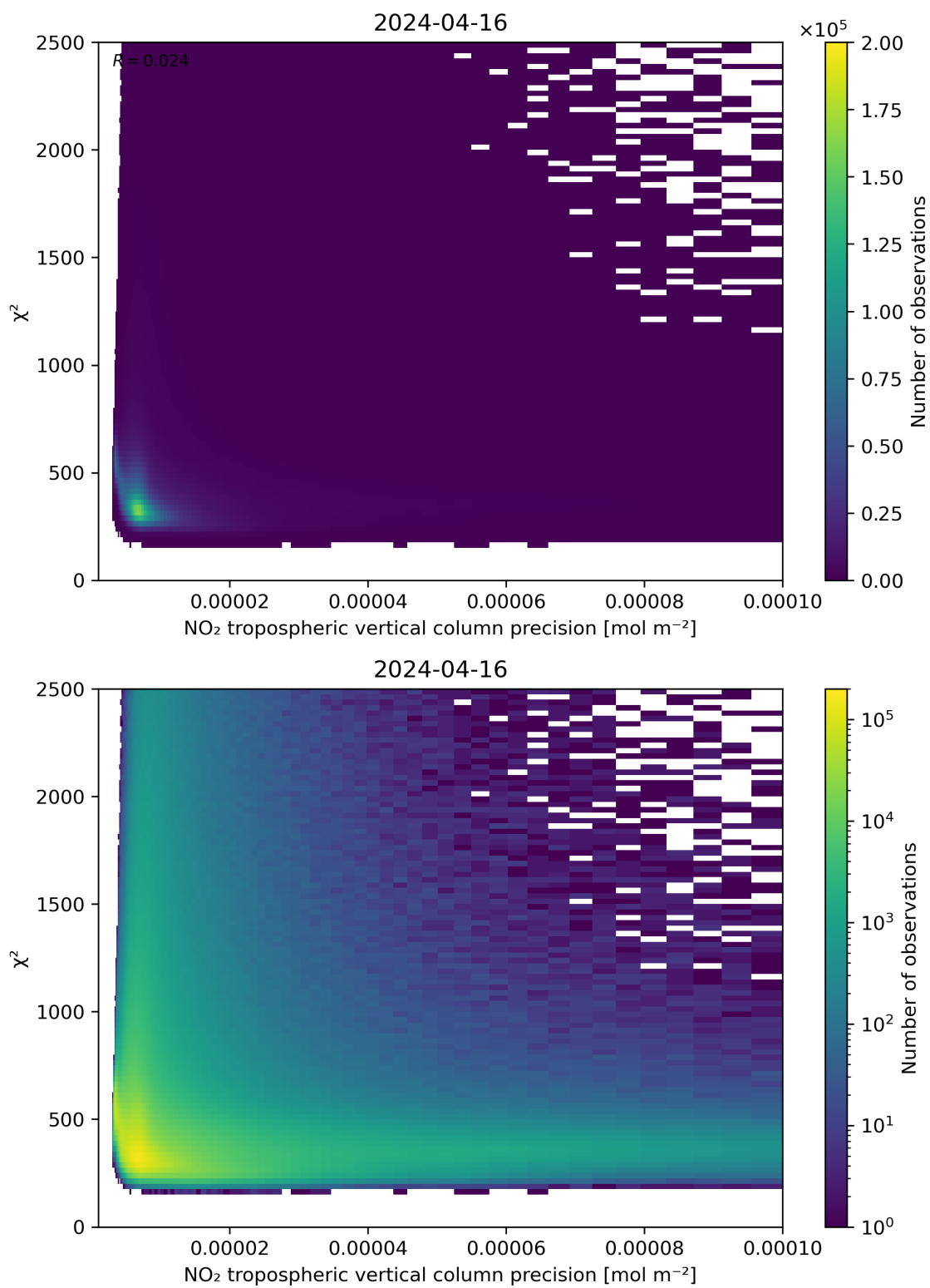
Figure 134: Scatter density plot of “NO 2 tropospheric vertical column precision” against “ \chi^2 ” for 2024-04-16 to 2024-04-17.
