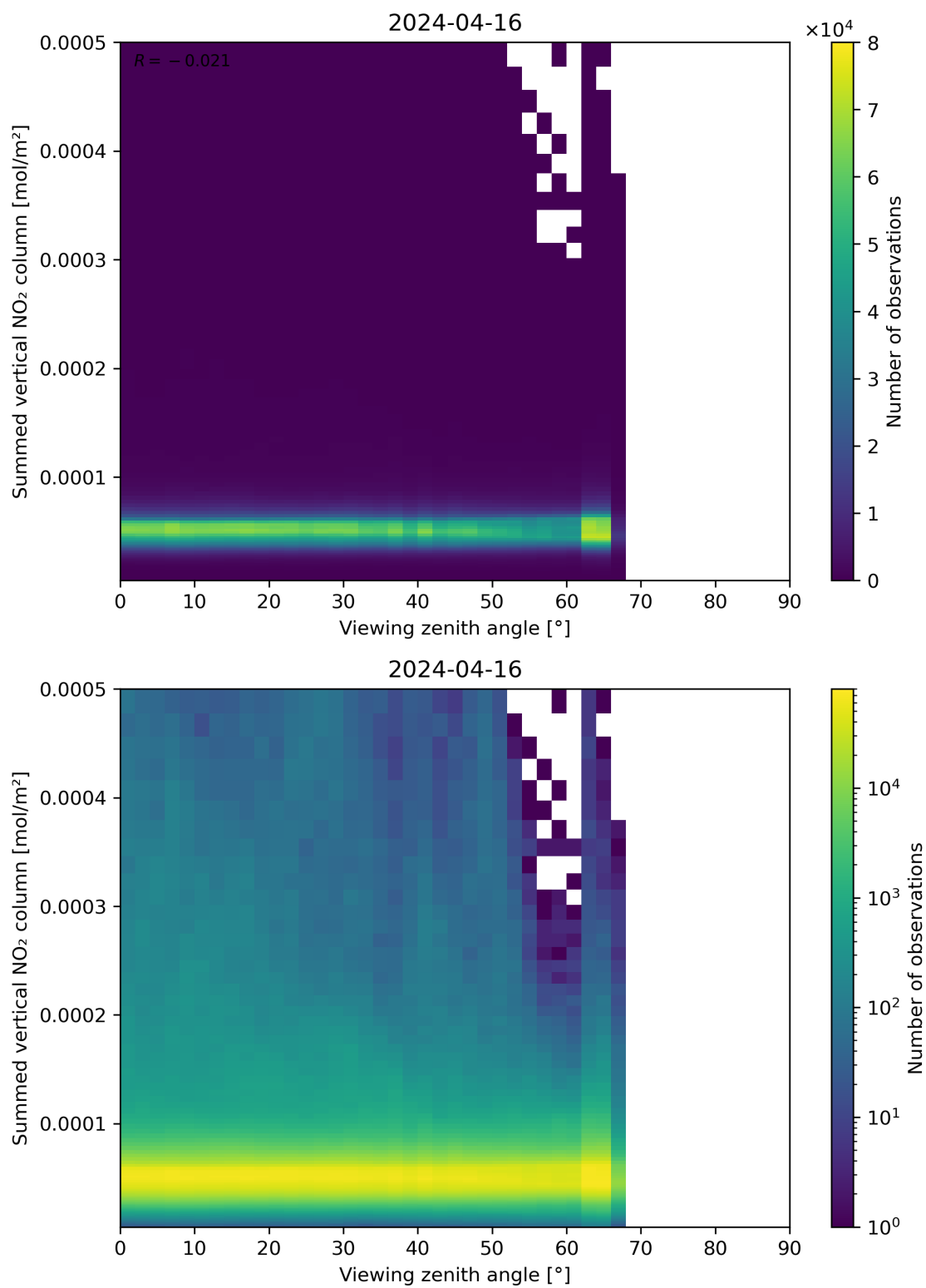
Figure 165: Scatter density plot of “Viewing zenith angle” against “Summed vertical NO 2 column” for 2024-04-16 to 2024-04-17.
