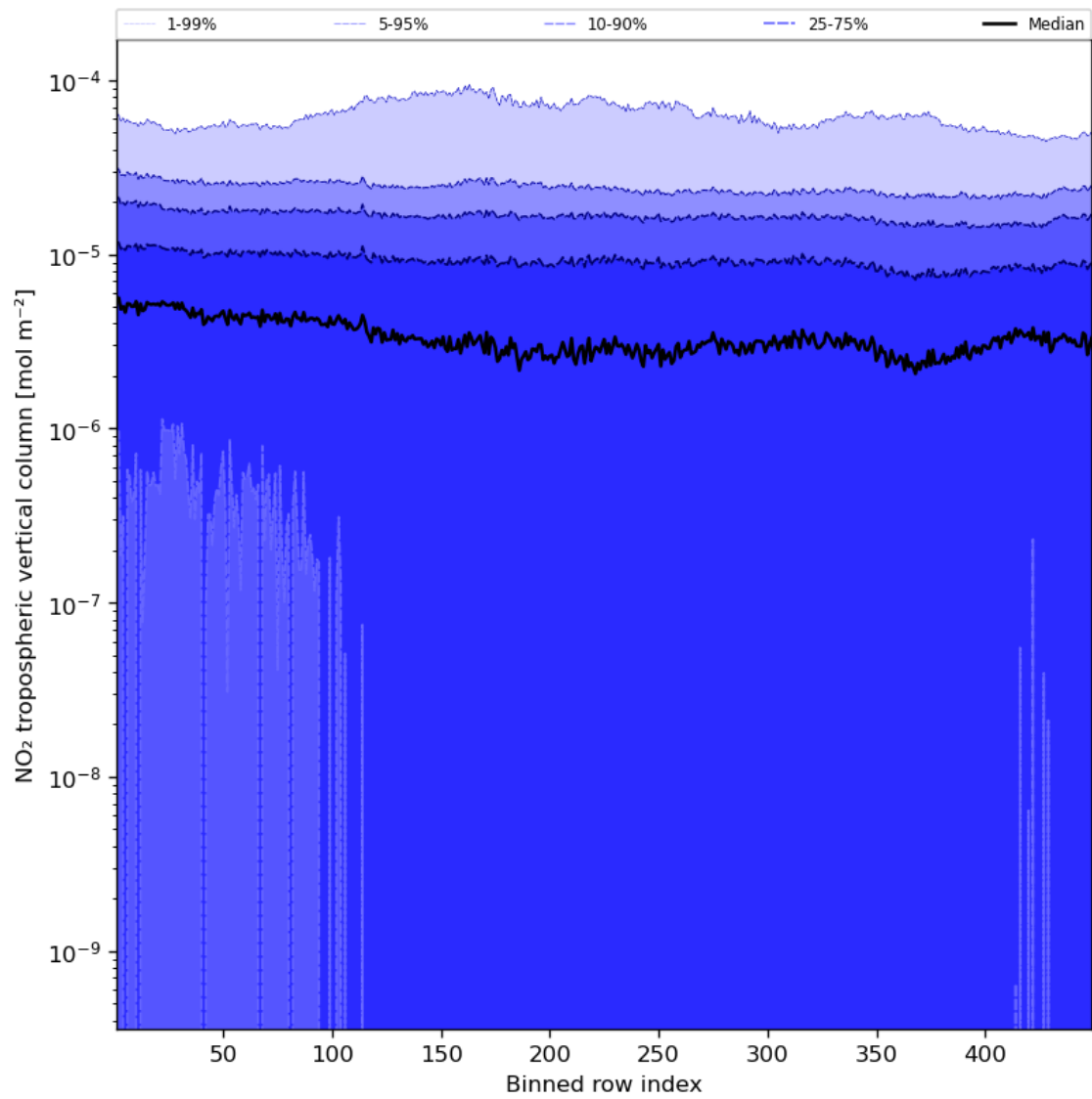
Figure 46: Along track statistics of “NO 2 tropospheric vertical column” for 2024-04-16 to 2024-04-17
