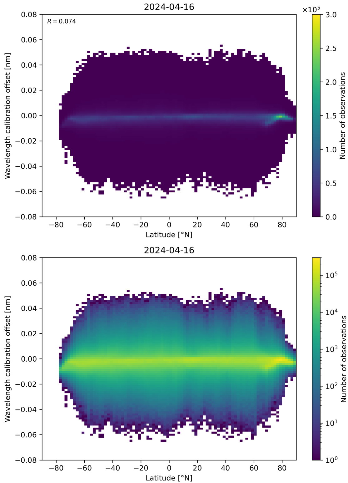
Figure 95: Scatter density plot of “Latitude” against “Wavelength calibration offset” for 2024-04-16 to 2024-04-17.
