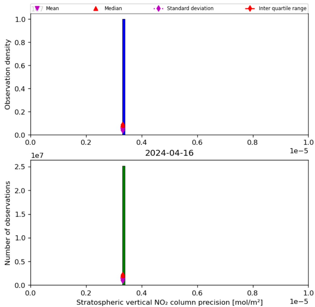
Figure 37: Histogram of “Stratospheric vertical NO 2 column precision” for 2024-04-16 to 2024-04-17
