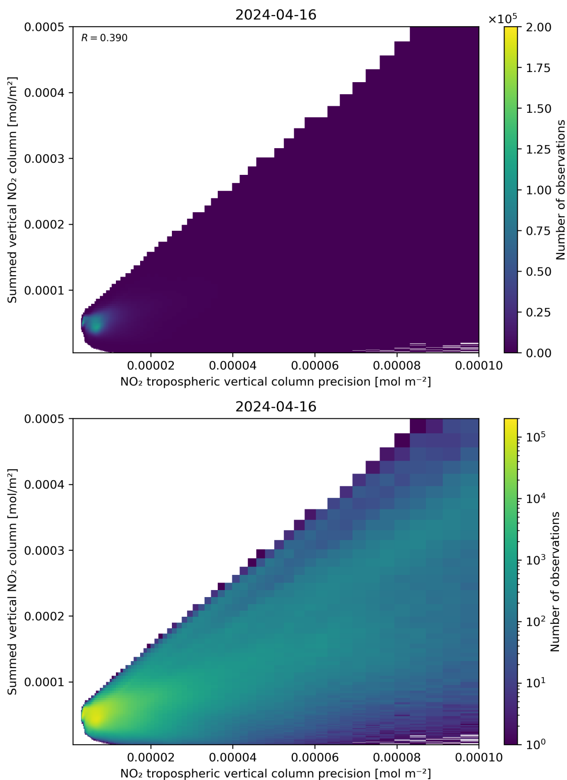
Figure 136: Scatter density plot of “NO 2 tropospheric vertical column precision” against “Summed vertical NO 2 column” for 2024-04-16 to 2024-04-17.
