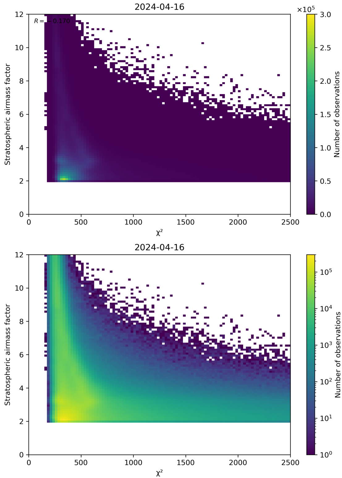
Figure 81: Scatter density plot of “ \chi^2 ” against “Stratospheric airmass factor” for 2024-04-16 to 2024-04-17.
