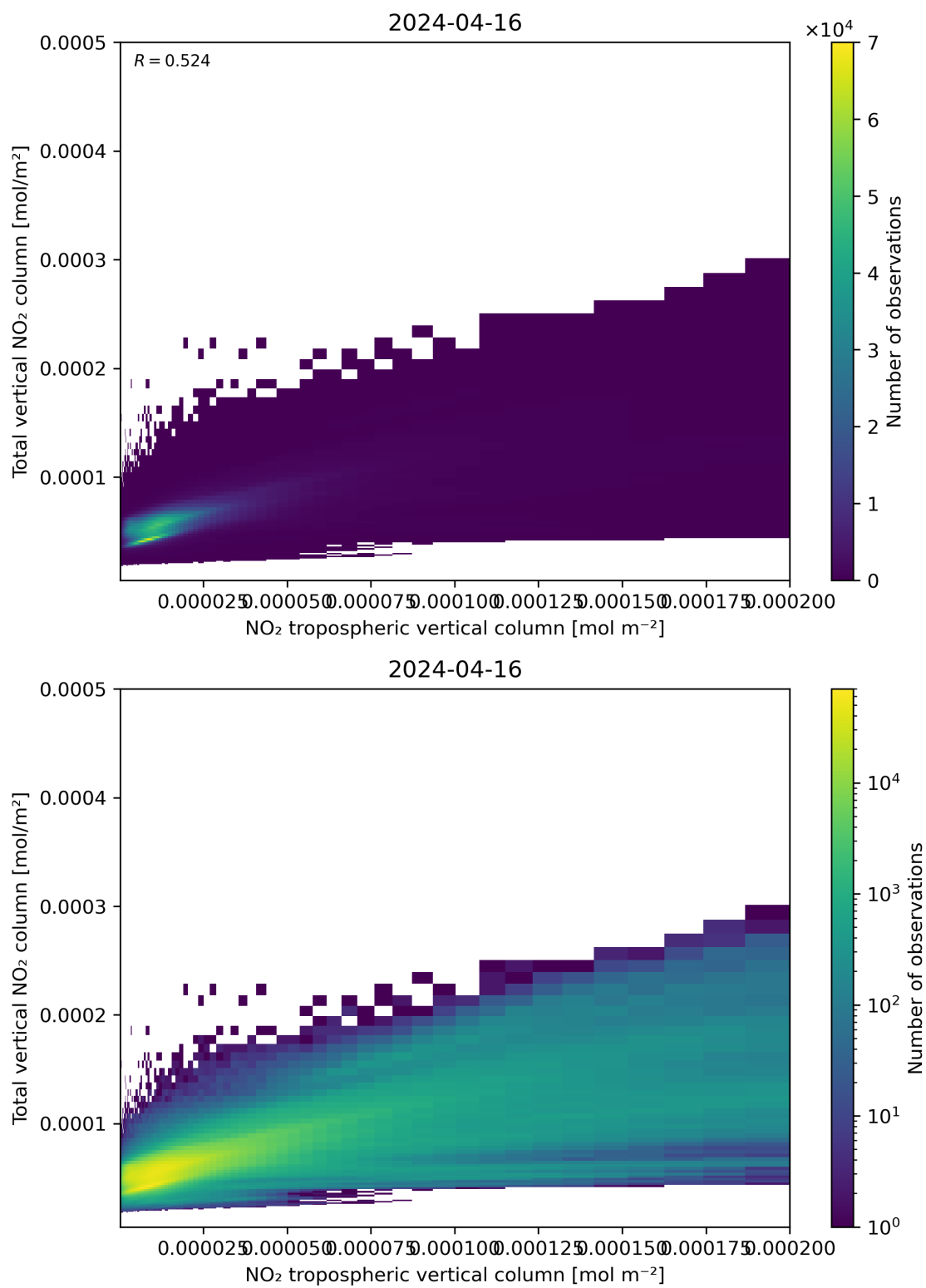
Figure 128: Scatter density plot of “NO 2 tropospheric vertical column” against “Total vertical NO 2 column” for 2024-04-16 to 2024-04-17.
