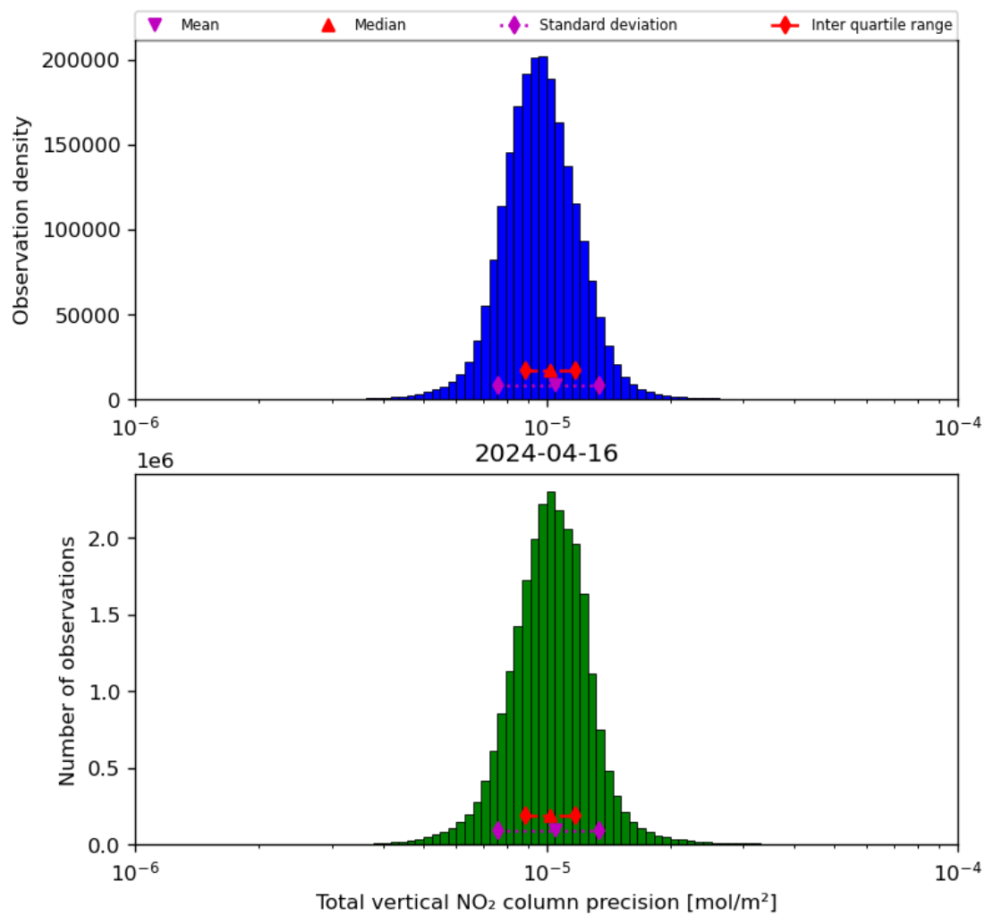
Figure 39: Histogram of “Total vertical NO 2 column precision” for 2024-04-16 to 2024-04-17
