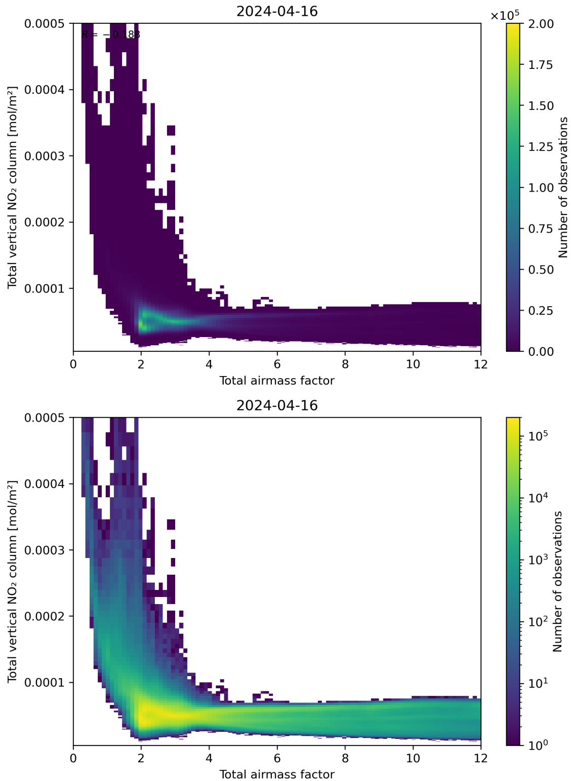
Figure 67: Scatter density plot of “Total airmass factor” against “Total vertical NO 2 column” for 2024-04-16 to 2024-04-17.
