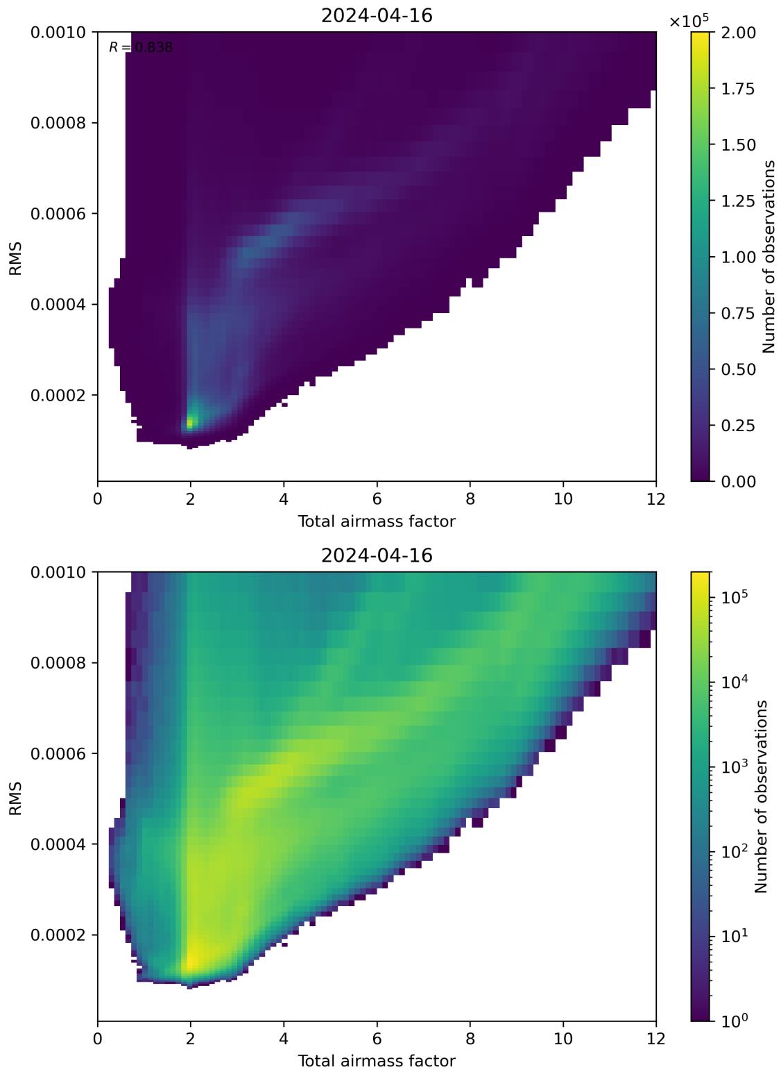
Figure 69: Scatter density plot of “Total airmass factor” against “RMS” for 2024-04-16 to 2024-04-17.
