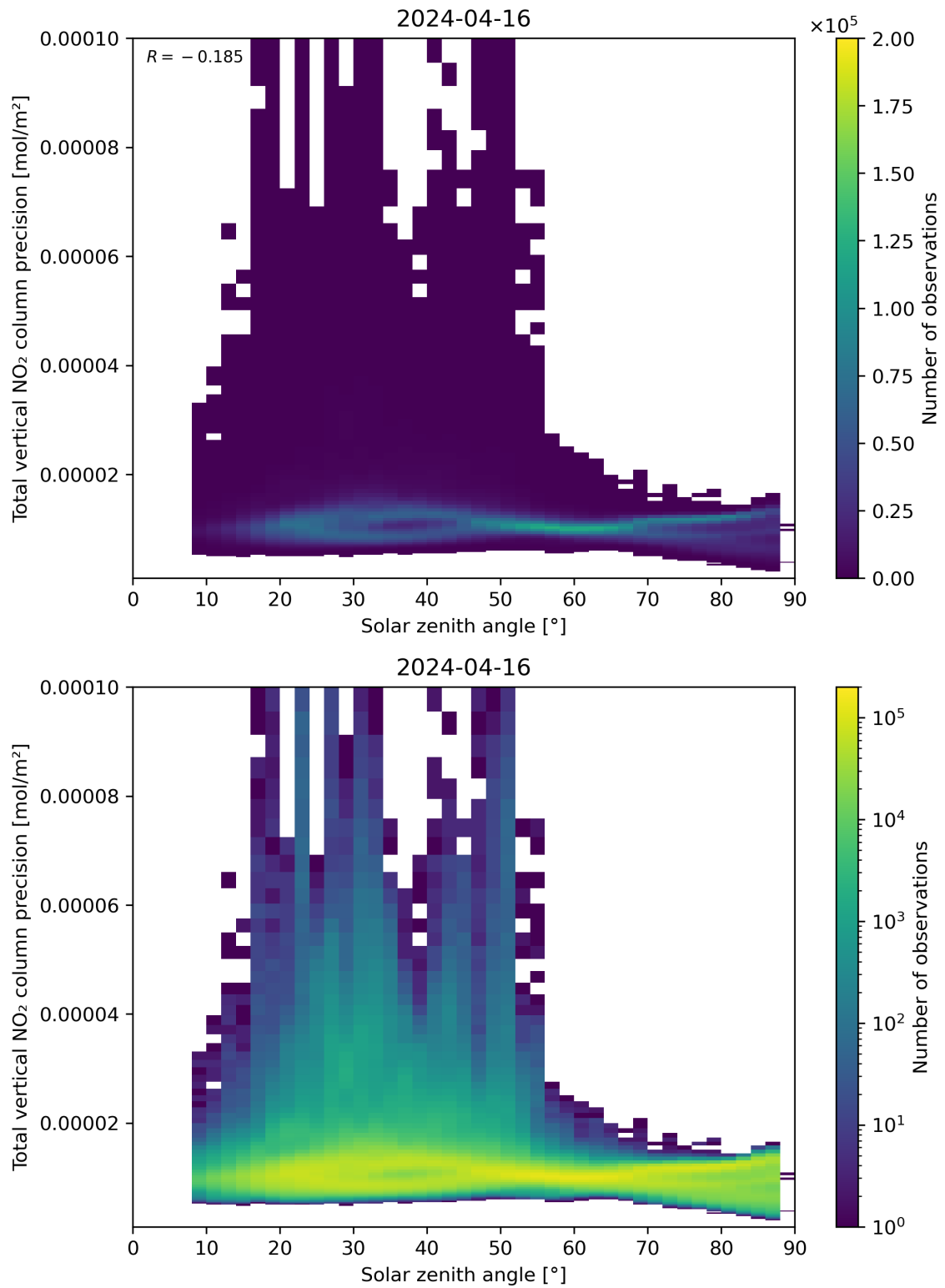
Figure 154: Scatter density plot of “Solar zenith angle” against “Total vertical NO 2 column precision” for 2024-04-16 to 2024-04-17.
