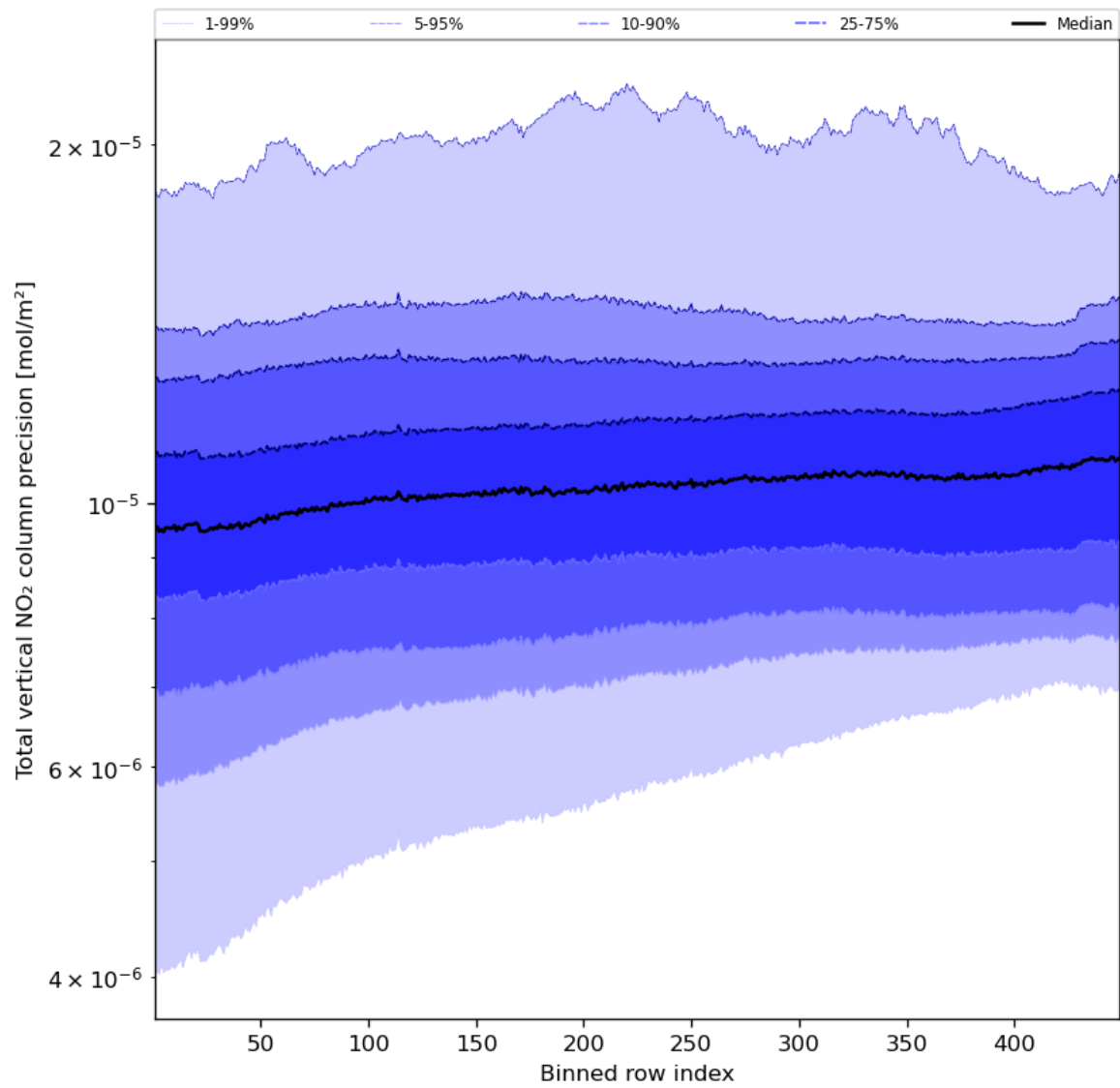
Figure 56: Along track statistics of "Total vertical NO 2 column precision" for 2024-04-16 to 2024-04-17
