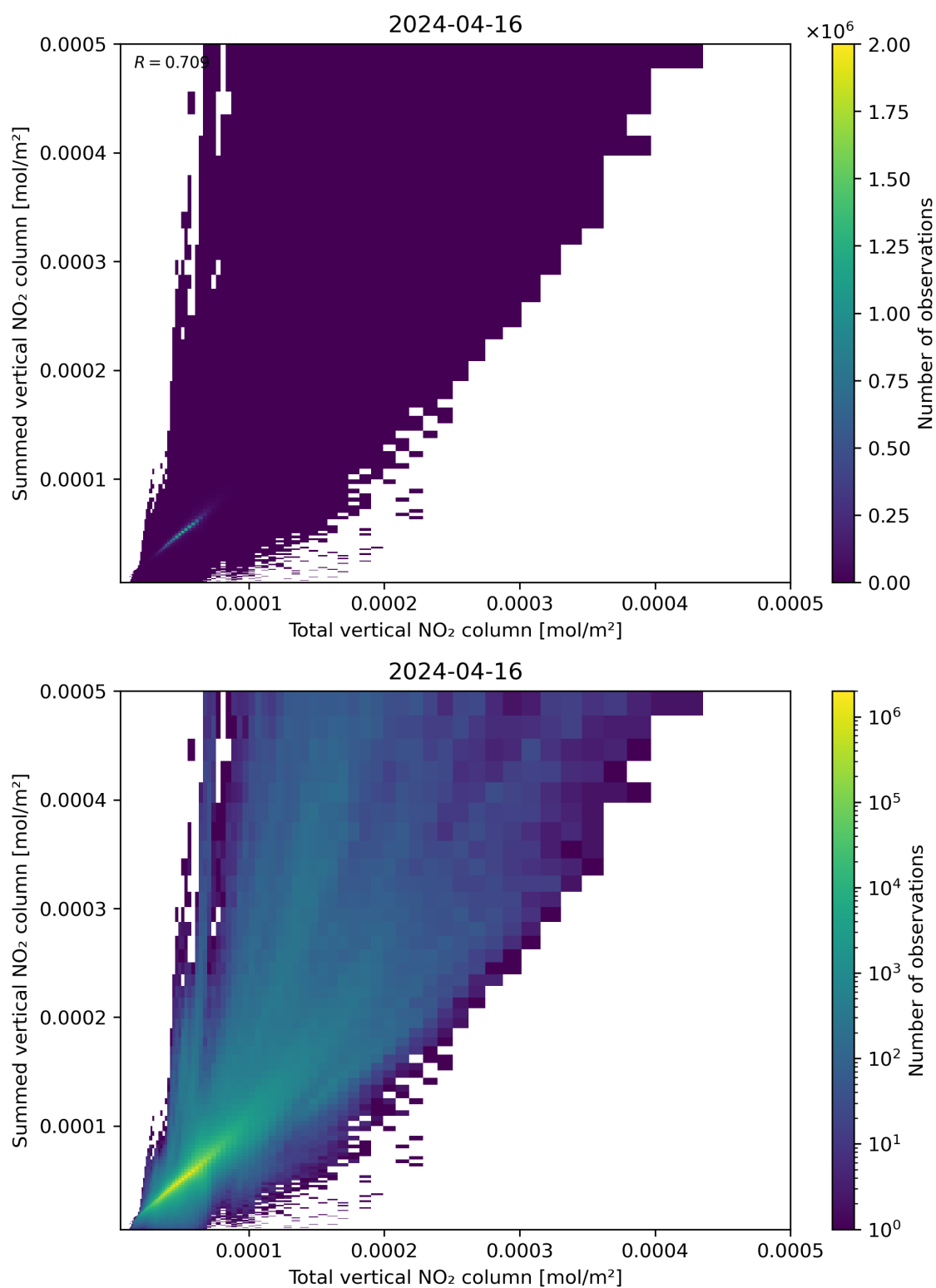
Figure 112: Scatter density plot of “Total vertical NO 2 column” against “Summed vertical NO 2 column” for 2024-04-16 to 2024-04-17.
