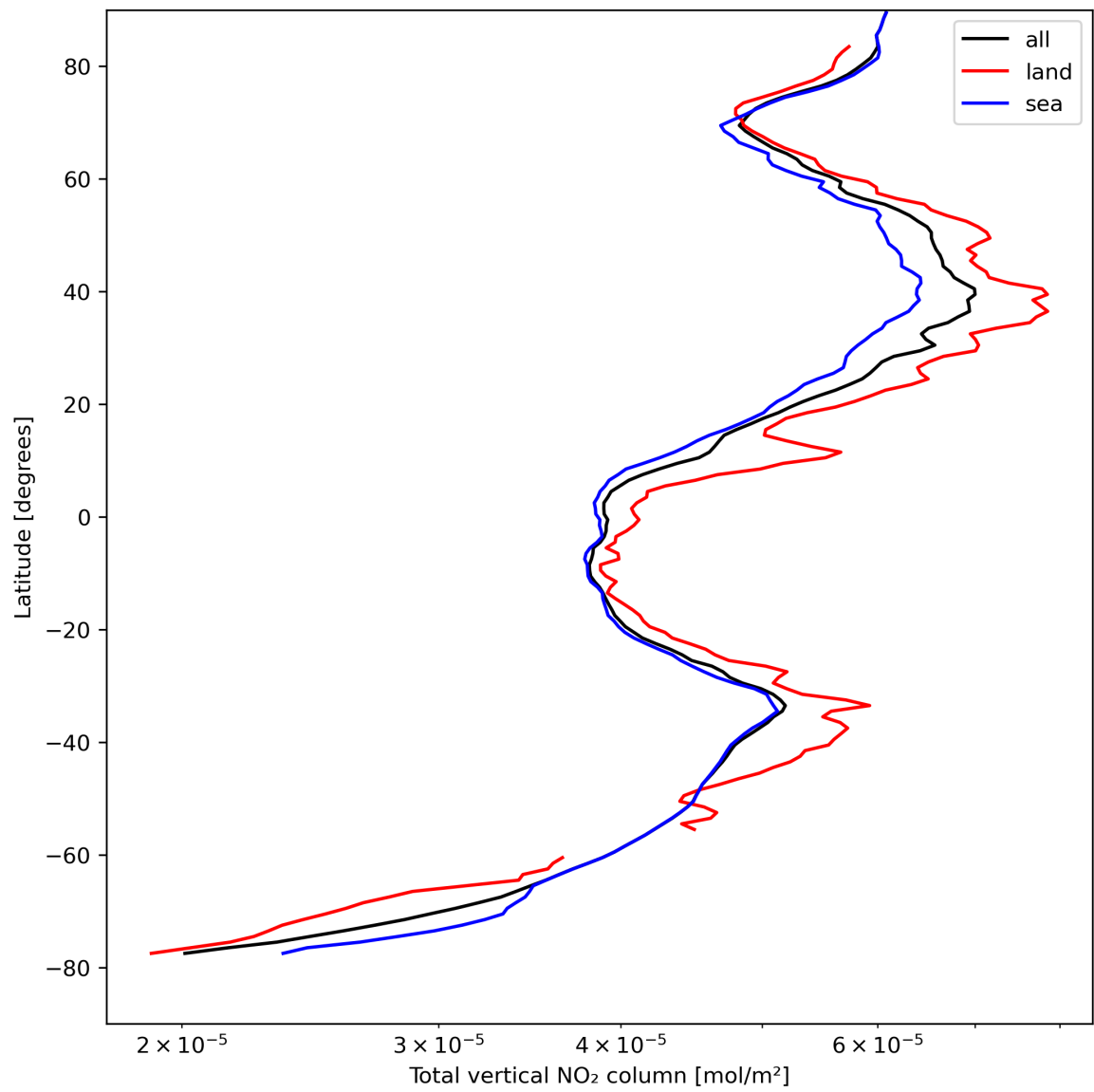
Figure 21: Zonal average of “Total vertical NO 2 column” for 2024-04-16 to 2024-04-17.
