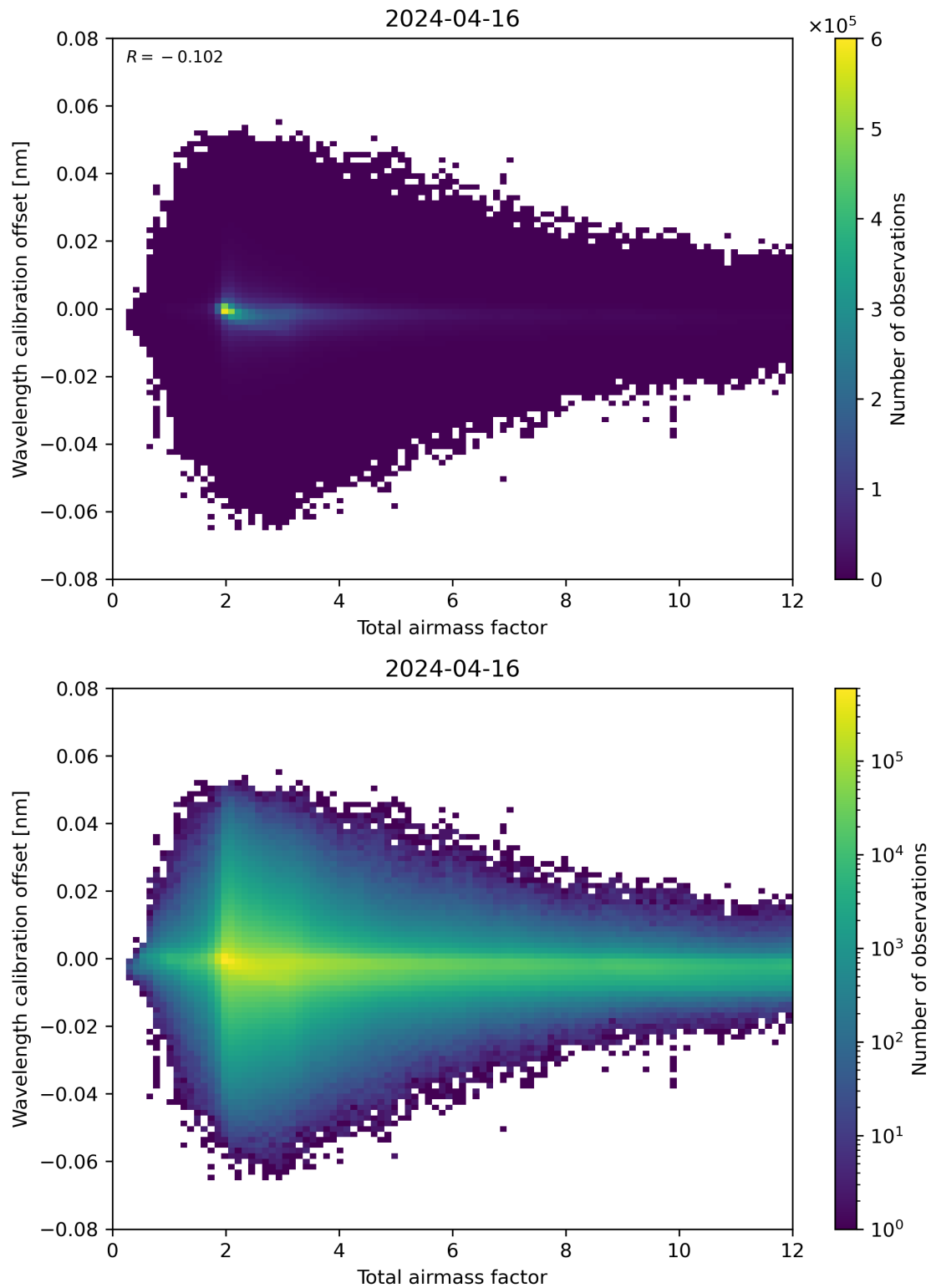
Figure 70: Scatter density plot of “Total airmass factor” against “Wavelength calibration offset” for 2024-04-16 to 2024-04-17.
