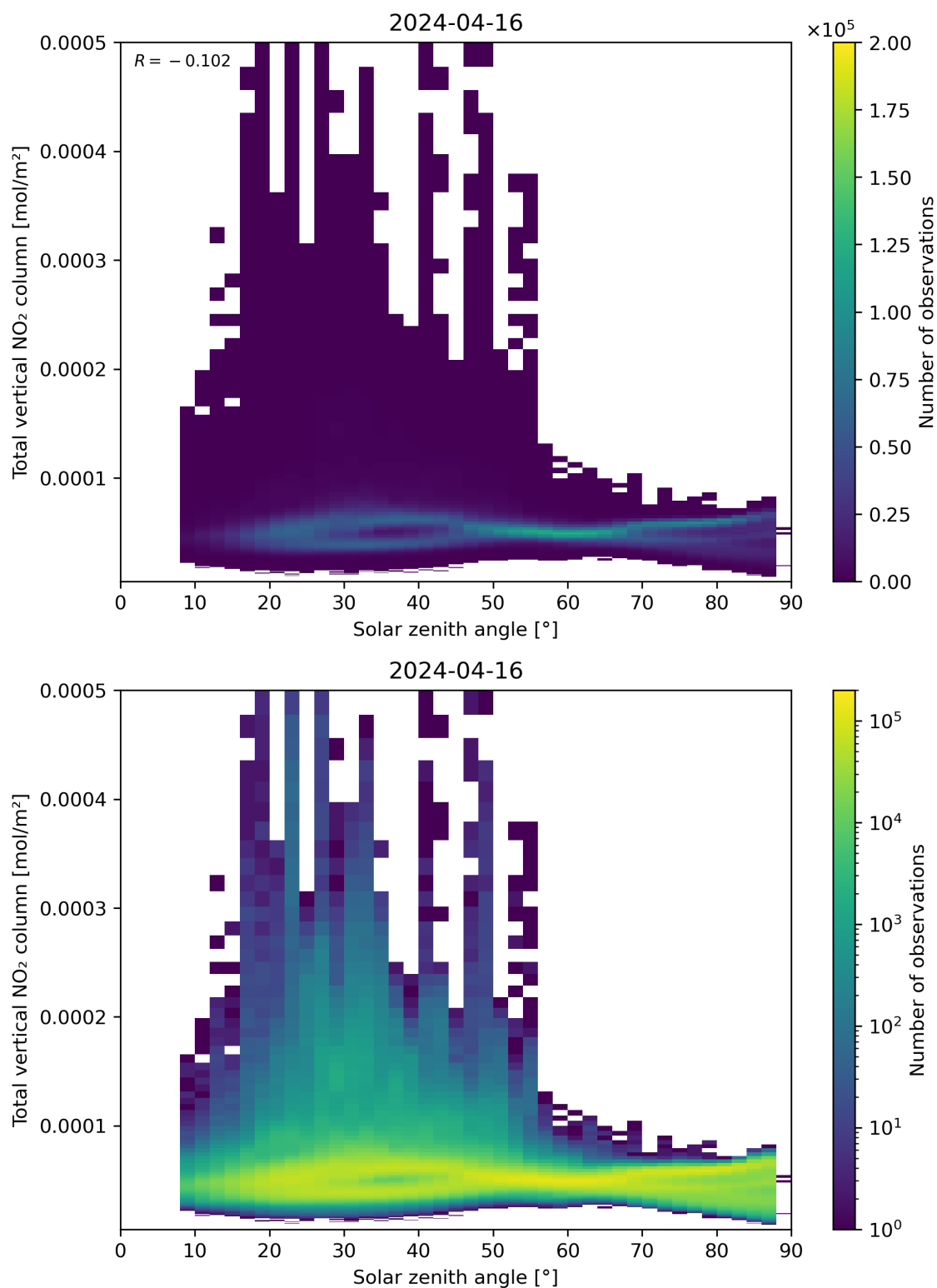
Figure 153: Scatter density plot of “Solar zenith angle” against “Total vertical NO 2 column” for 2024-04-16 to 2024-04-17.
