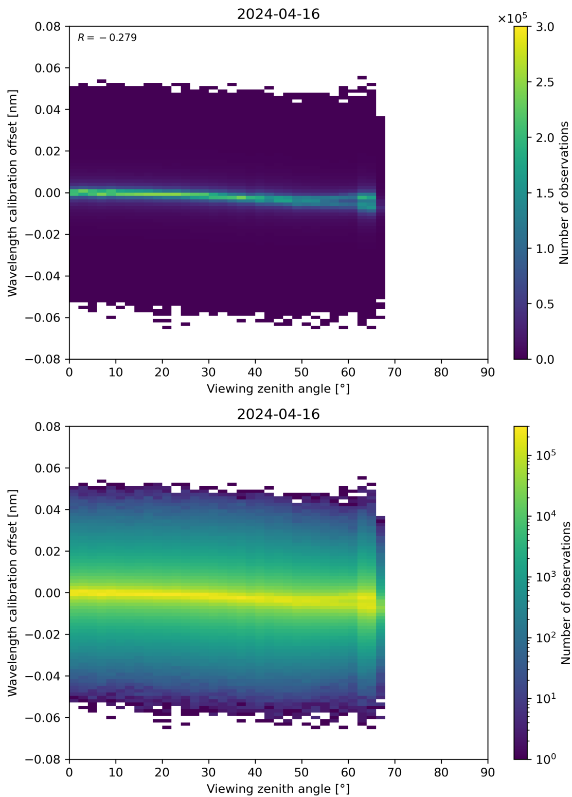
Figure 173: Scatter density plot of “Viewing zenith angle” against “Wavelength calibration offset” for 2024-04-16 to 2024-04-17.
