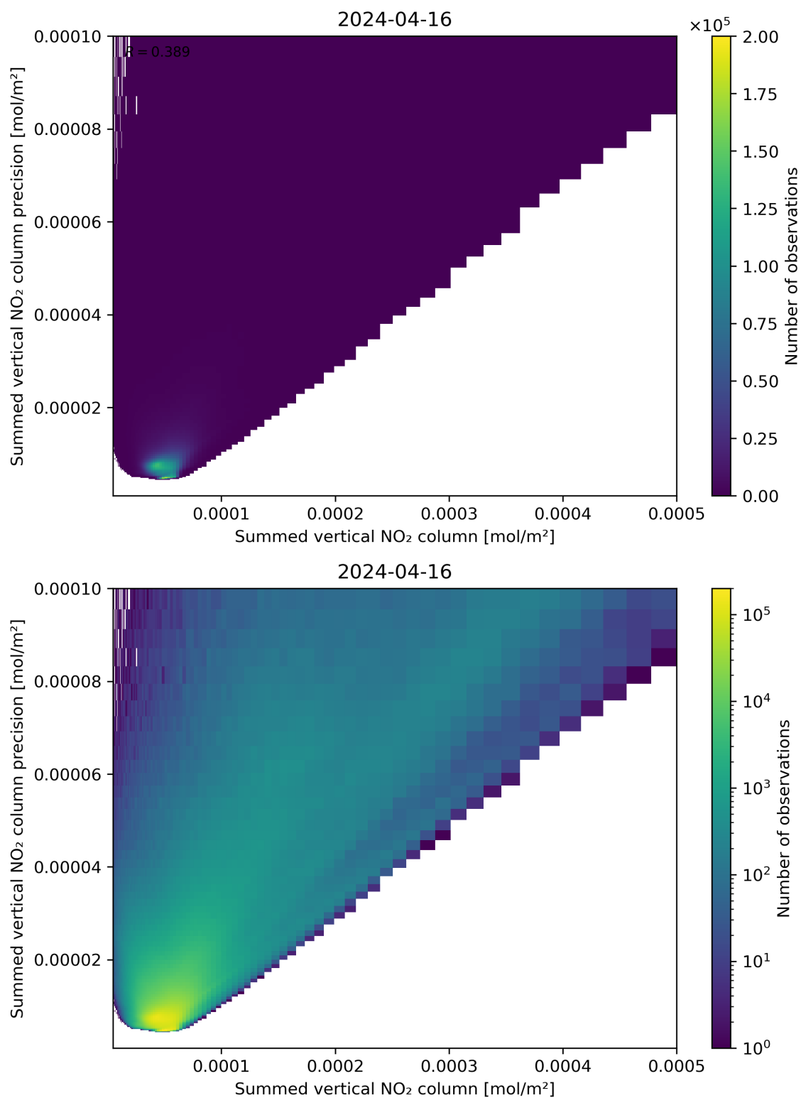
Figure 105: Scatter density plot of “Summed vertical NO 2 column” against “Summed vertical NO 2 column precision” for 2024-04-16 to 2024-04-17.
