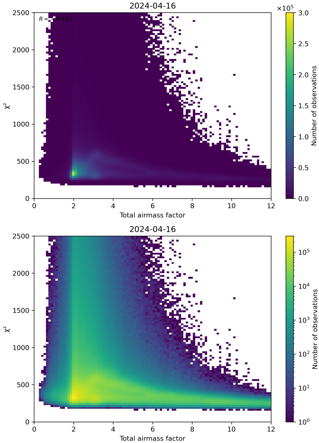
Figure 63: Scatter density plot of “Total airmass factor” against “ \chi^2 ” for 2024-04-16 to 2024-04-17.
