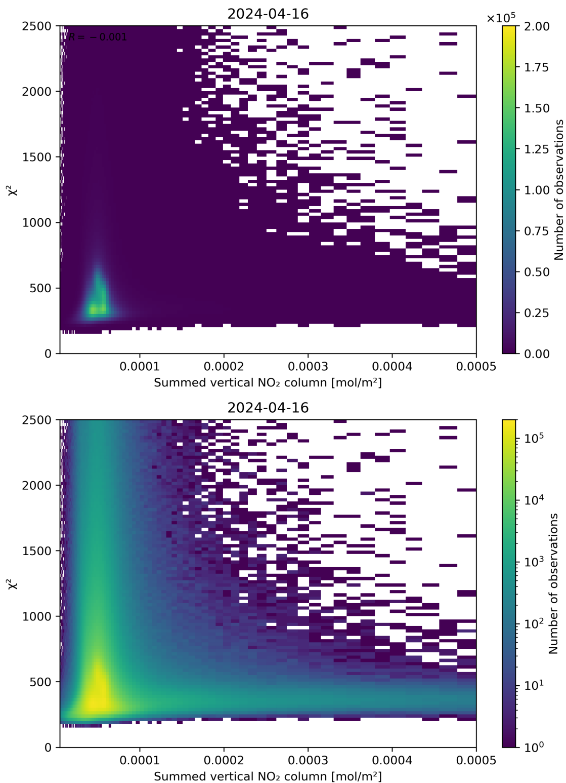
Figure 104: Scatter density plot of “Summed vertical NO 2 column” against “ \chi^2 ” for 2024-04-16 to 2024-04-17.
