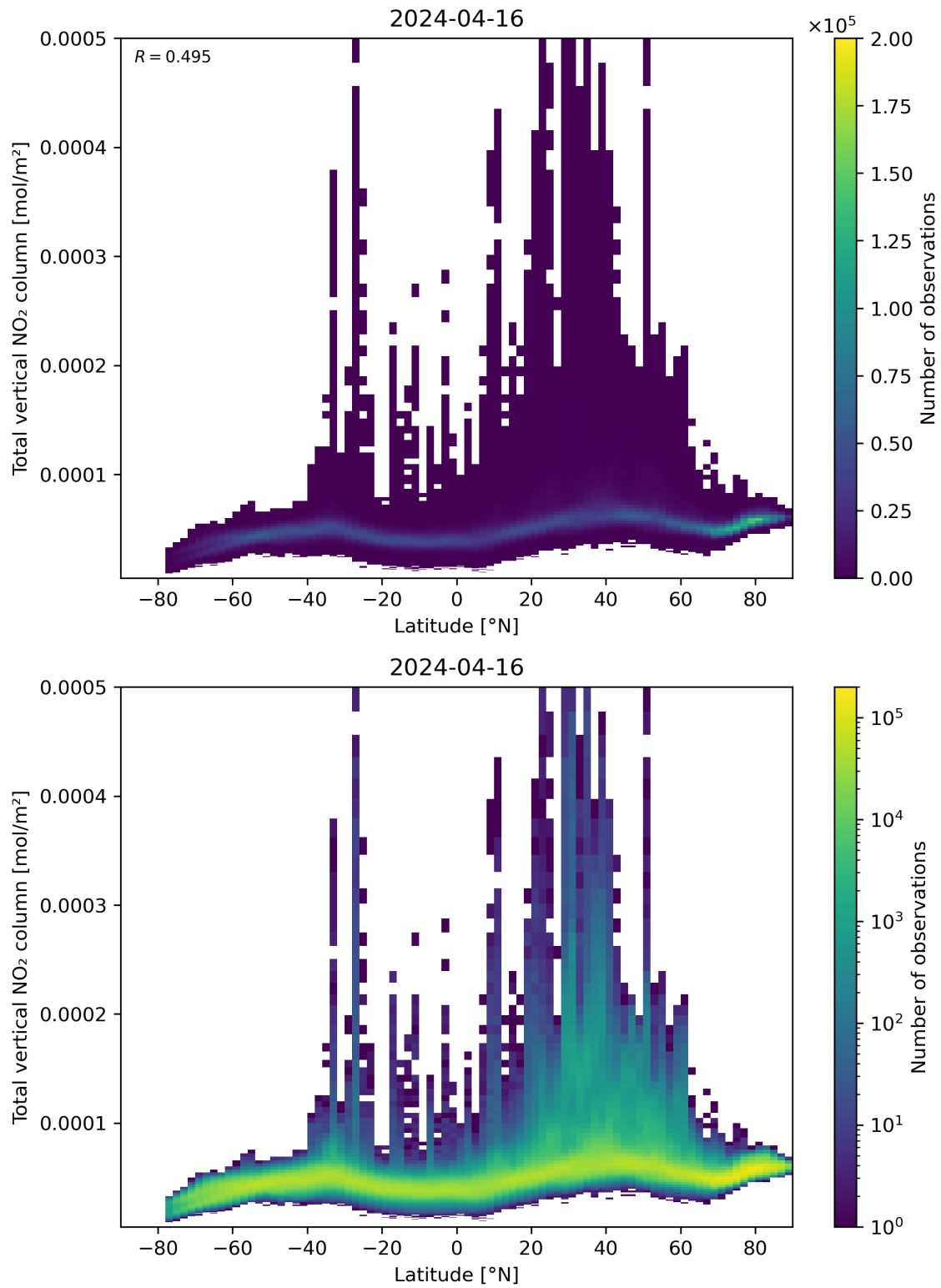
Figure 90: Scatter density plot of “Latitude” against “Total vertical NO 2 column” for 2024-04-16 to 2024-04-17.
