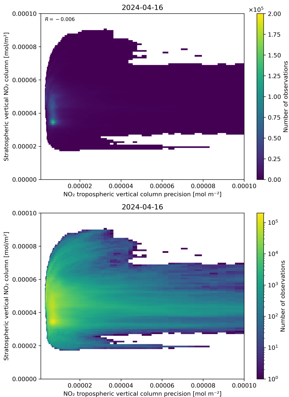
Figure 135: Scatter density plot of “NO 2 tropospheric vertical column precision” against “Stratospheric vertical NO 2 column” for 2024-04-16 to 2024-04-17.
