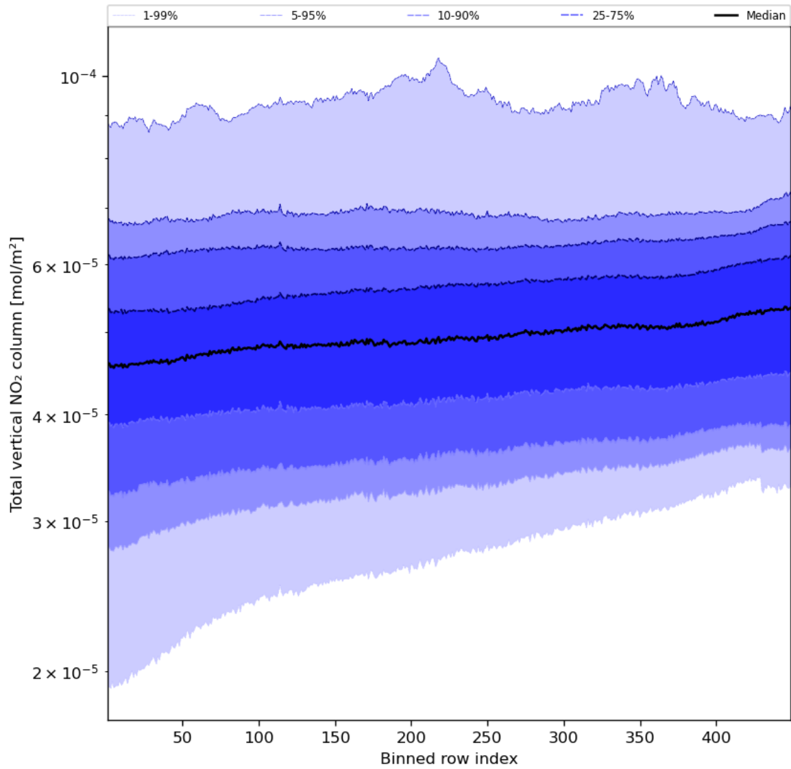
Figure 55: Along track statistics of “Total vertical NO 2 column” for 2024-04-16 to 2024-04-17
