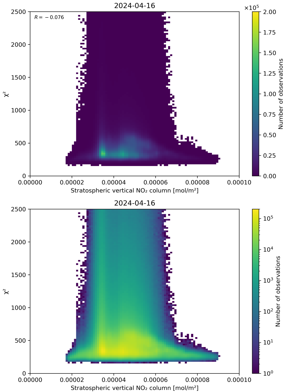
Figure 97: Scatter density plot of “Stratospheric vertical NO 2 column” against “ \chi^2 ” for 2024-04-16 to 2024-04-17.
