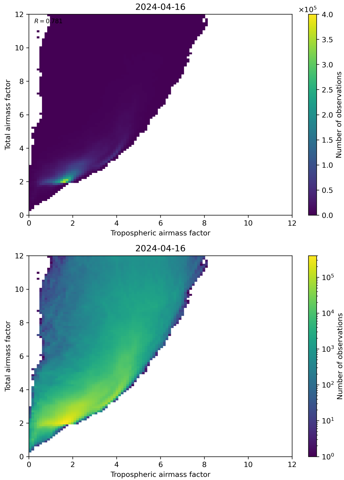
Figure 72: Scatter density plot of “Tropospheric airmass factor” against “Total airmass factor” for 2024-04-16 to 2024-04-17.
