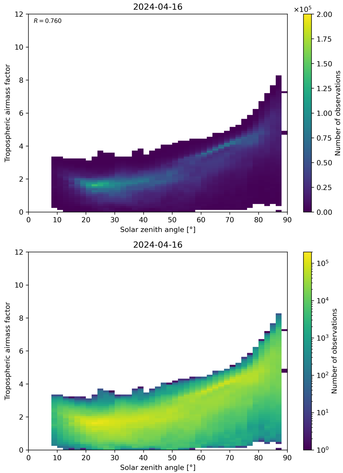
Figure 147: Scatter density plot of “Solar zenith angle” against “Tropospheric airmass factor” for 2024-04-16 to 2024-04-17.
