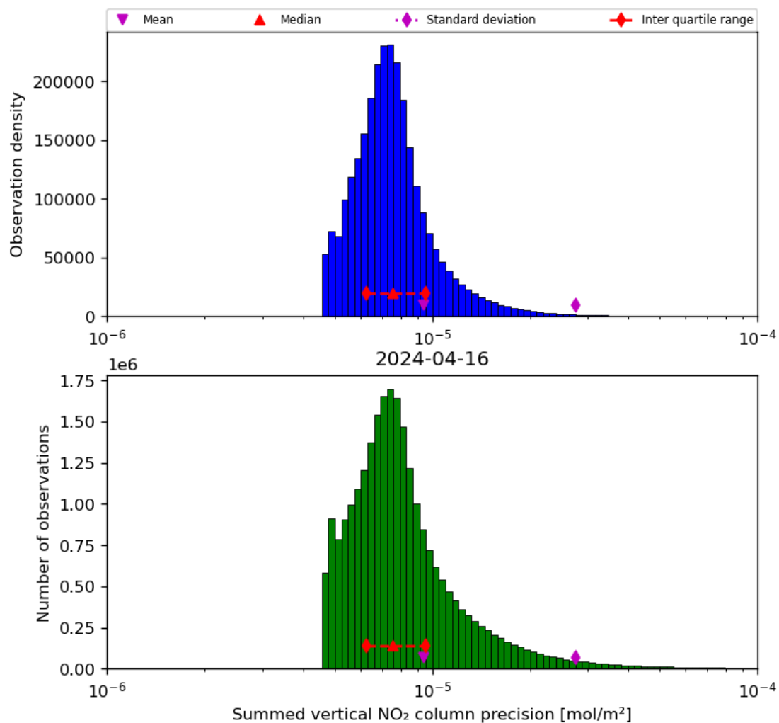
Figure 41: Histogram of “Summed vertical NO 2 column precision” for 2024-04-16 to 2024-04-17
