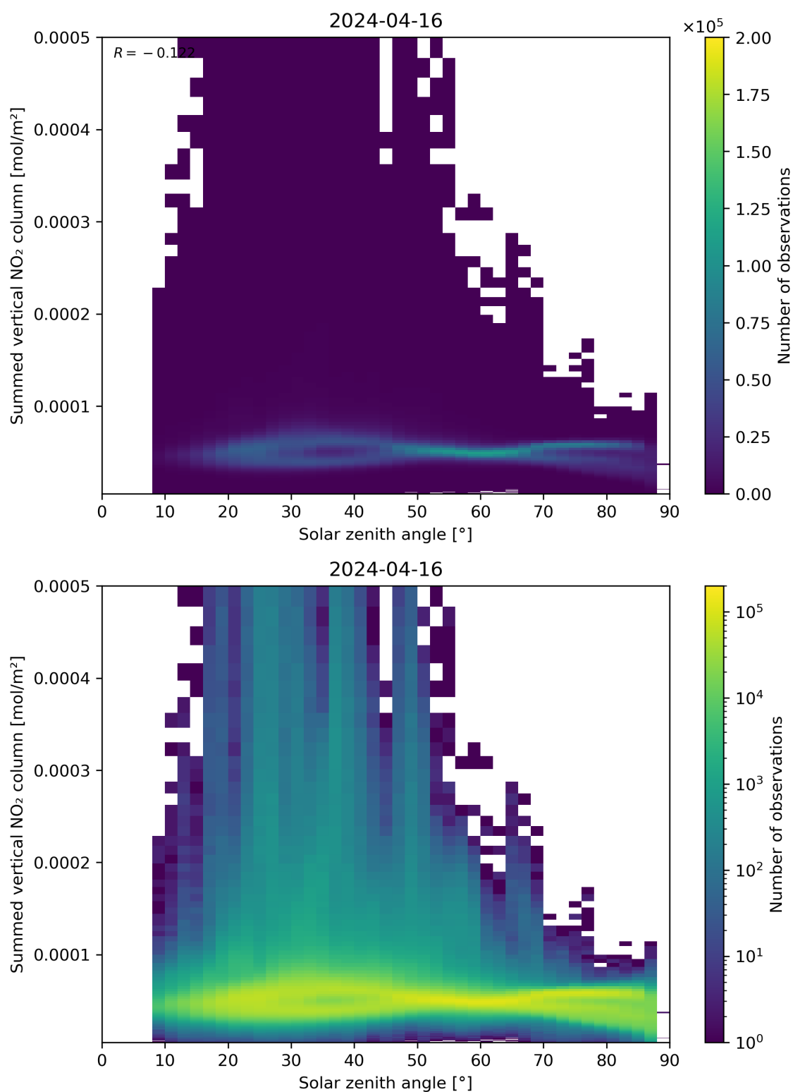
Figure 151: Scatter density plot of “Solar zenith angle” against “Summed vertical NO 2 column” for 2024-04-16 to 2024-04-17.
