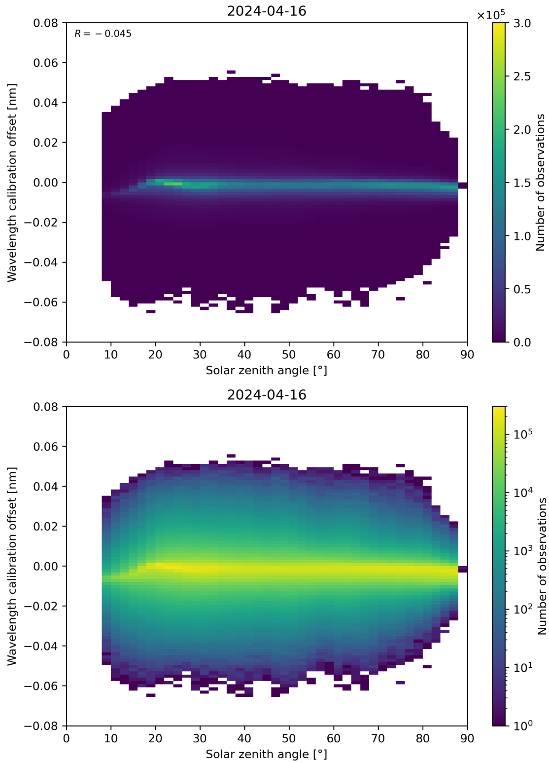
Figure 158: Scatter density plot of “Solar zenith angle” against “Wavelength calibration offset” for 2024-04-16 to 2024-04-17.
