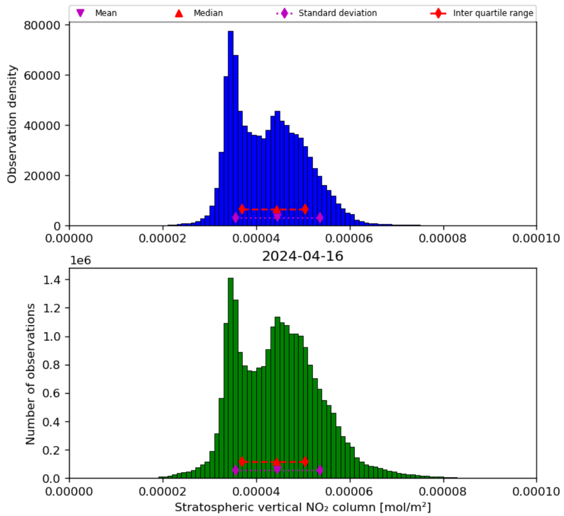
Figure 36: Histogram of “Stratospheric vertical NO 2 column” for 2024-04-16 to 2024-04-17
