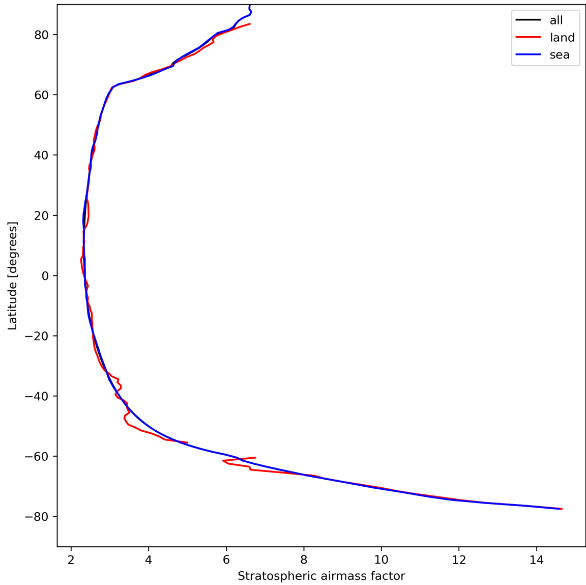
Figure 27: Zonal average of “Stratospheric airmass factor” for 2024-04-16 to 2024-04-17.
