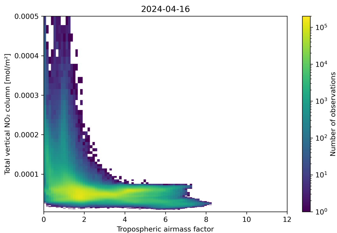
Figure 77: Scatter density plot of “Tropospheric airmass factor” against “Total vertical NO 2 column” for 2024-04-16 to 2024-04-17.
