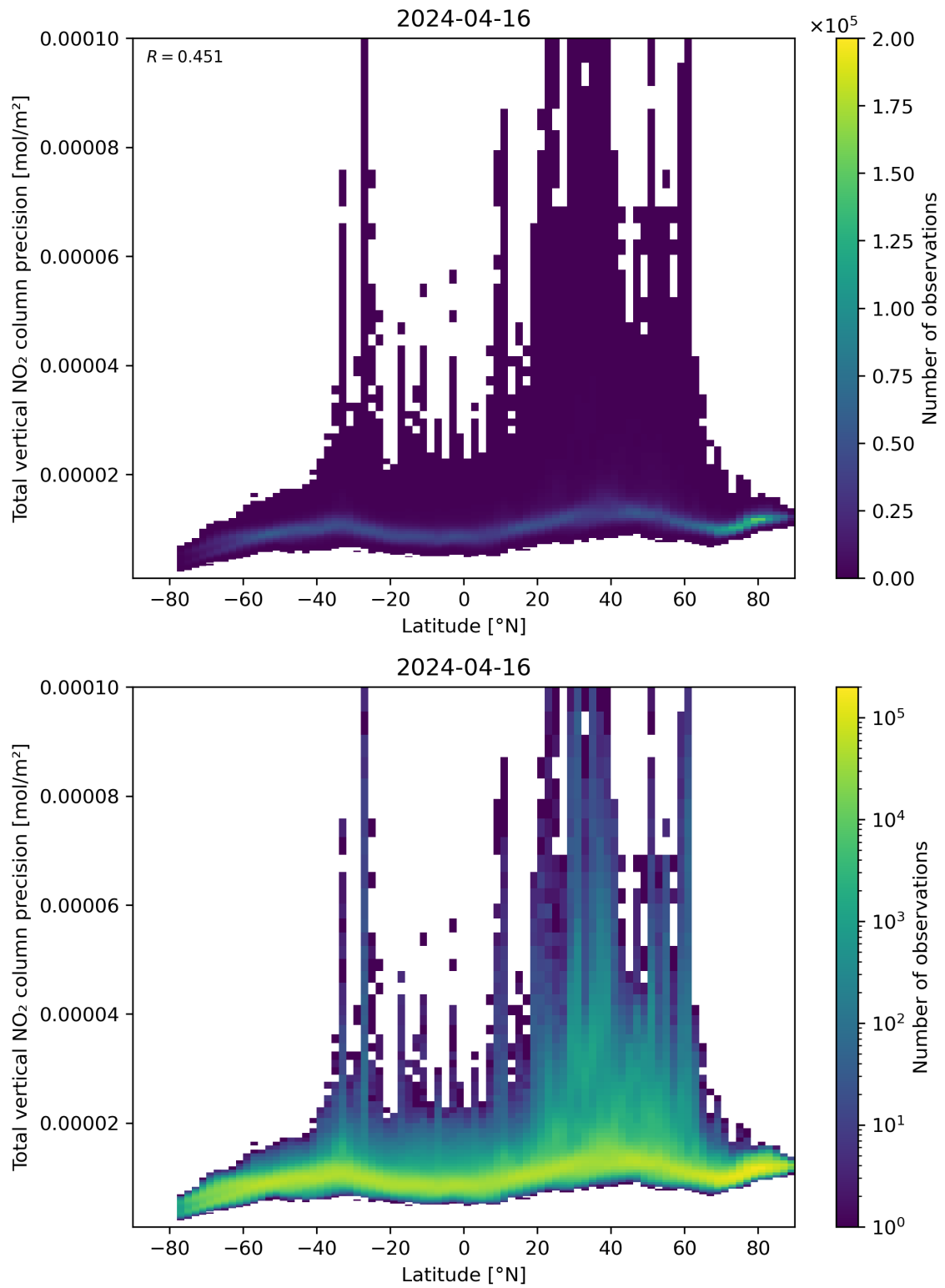
Figure 91: Scatter density plot of “Latitude” against “Total vertical NO 2 column precision” for 2024-04-16 to 2024-04-17.
