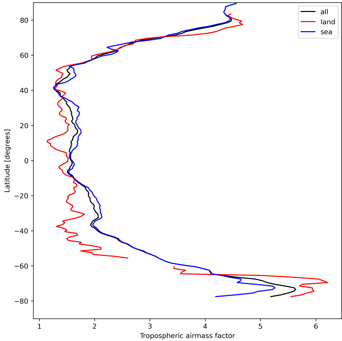
Figure 14: Zonal average of “Tropospheric airmass factor” for 2024-04-16 to 2024-04-17.
