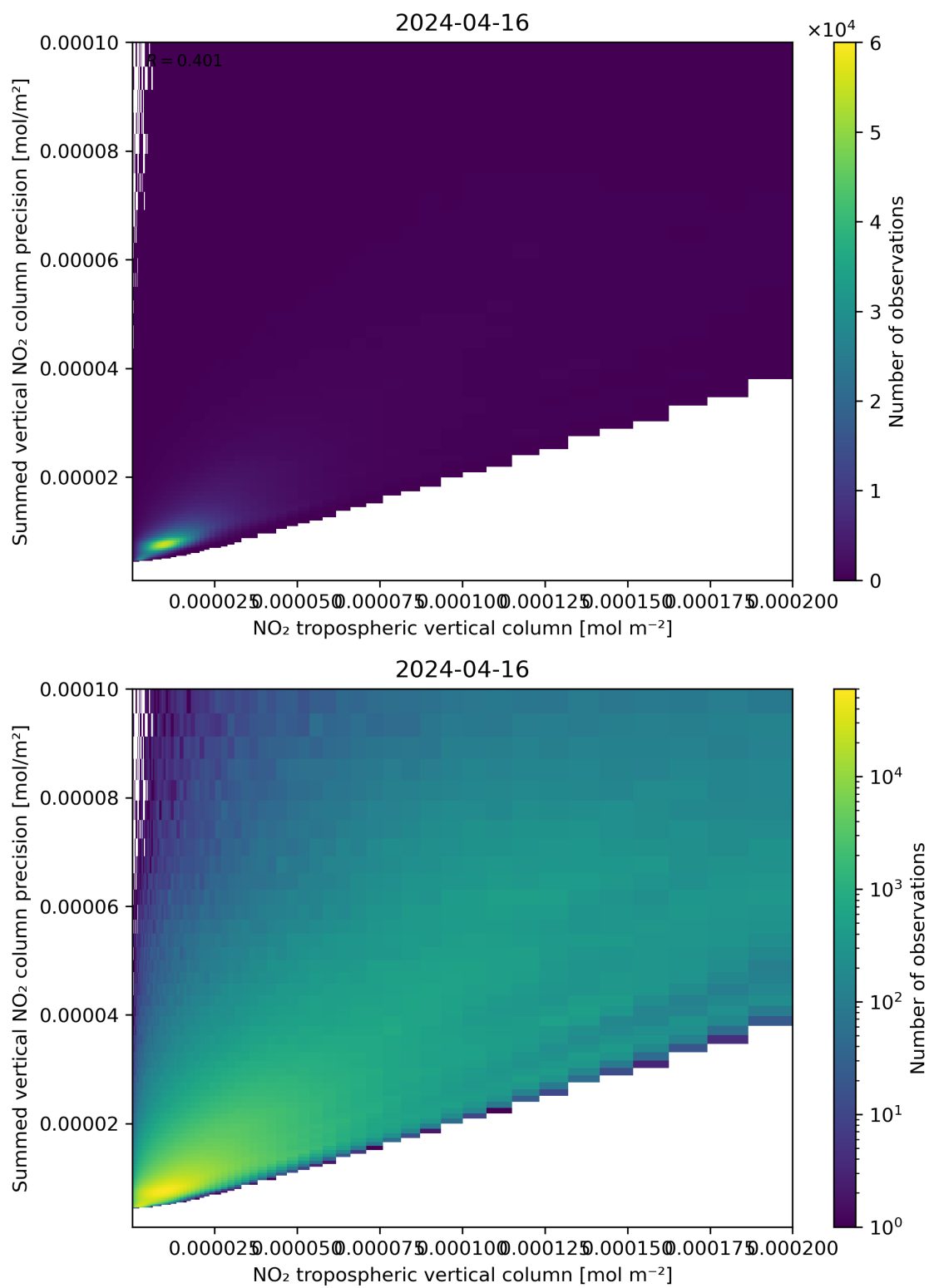
Figure 127: Scatter density plot of “NO 2 tropospheric vertical column” against “Summed vertical NO 2 column precision” for 2024-04-16 to 2024-04-17.
