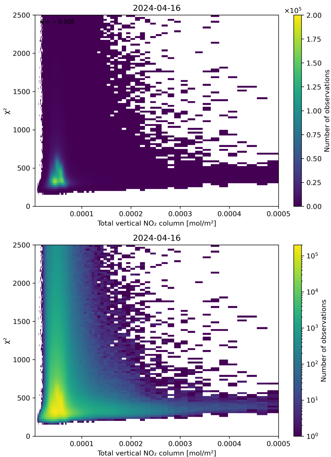
Figure 111: Scatter density plot of “Total vertical NO 2 column” against “ \chi^2 ” for 2024-04-16 to 2024-04-17.
