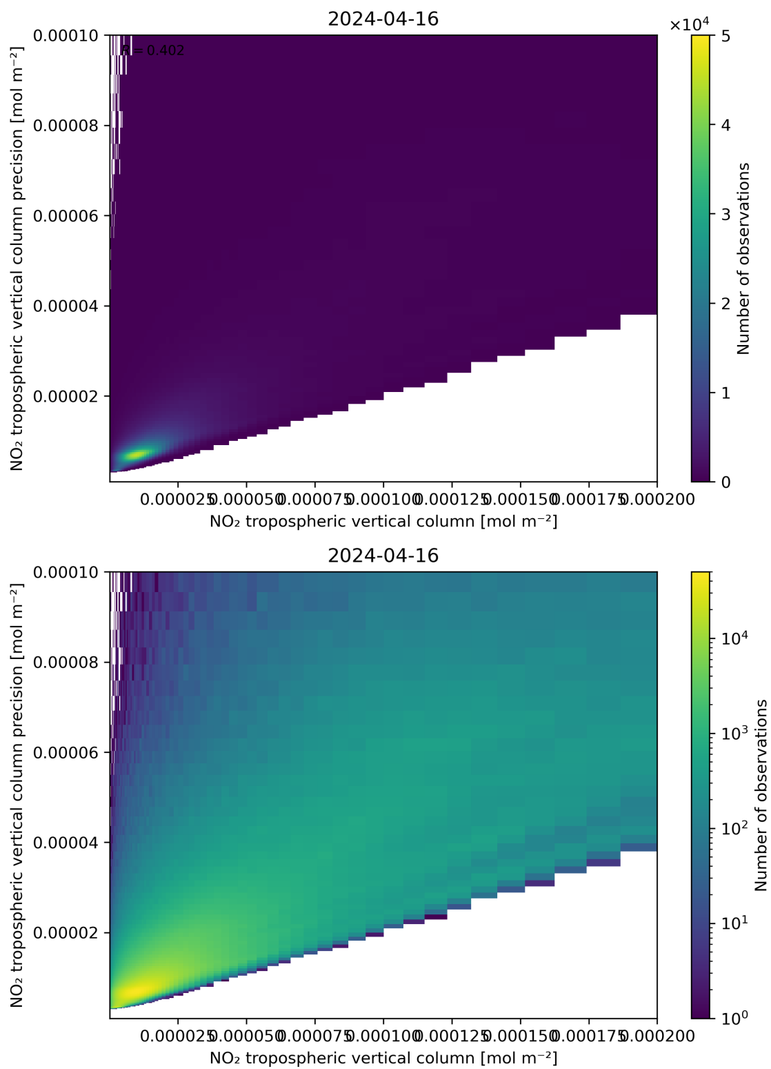
Figure 130: Scatter density plot of “NO 2 tropospheric vertical column” against “NO 2 tropospheric vertical column precision” for 2024-04-16 to 2024-04-17.
