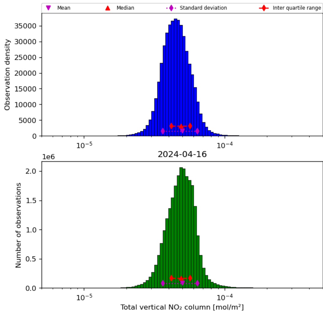
Figure 38: Histogram of “Total vertical NO 2 column” for 2024-04-16 to 2024-04-17
