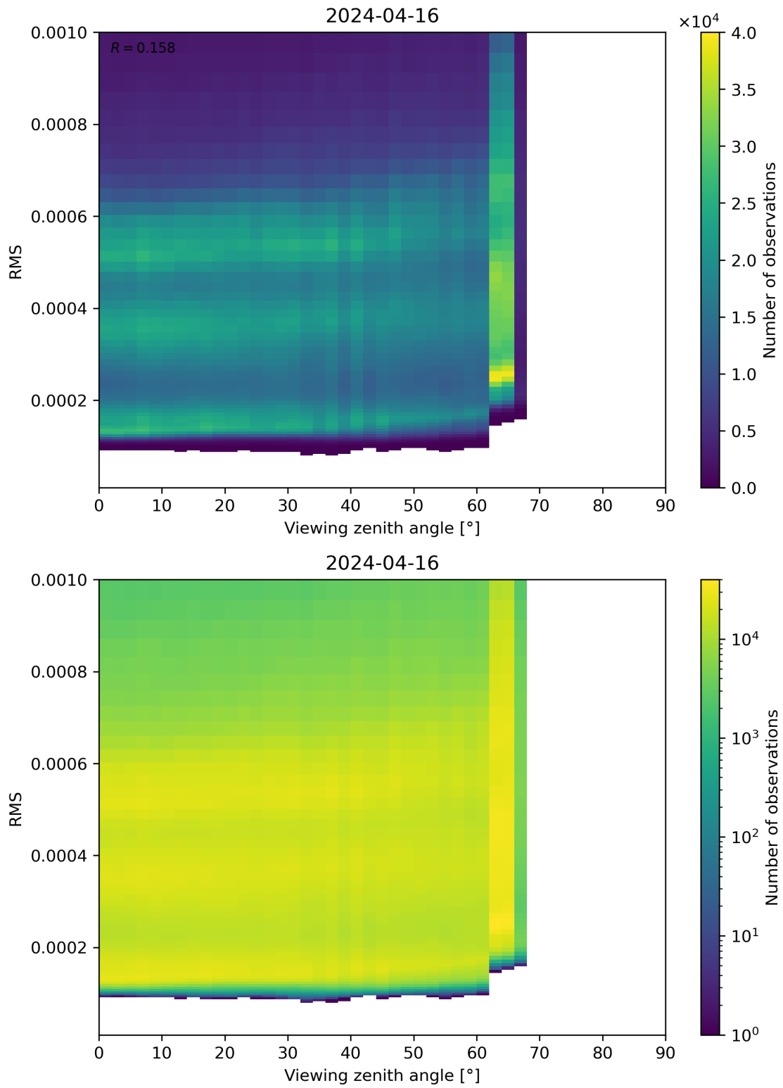
Figure 171: Scatter density plot of “Viewing zenith angle” against “RMS” for 2024-04-16 to 2024-04-17.
