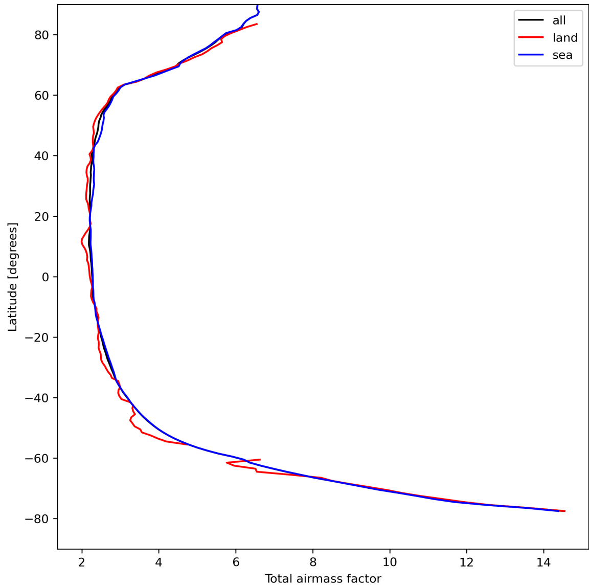
Figure 15: Zonal average of “Total airmass factor” for 2024-04-16 to 2024-04-17.
