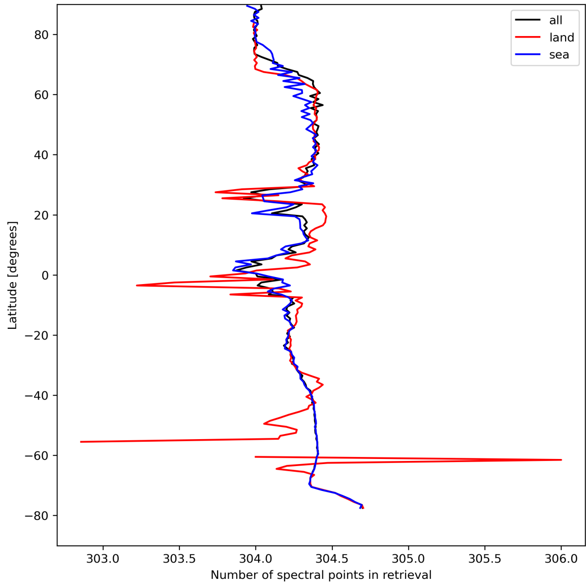
Figure 16: Zonal average of “Number of spectral points in retrieval” for 2024-04-16 to 2024-04-17.
