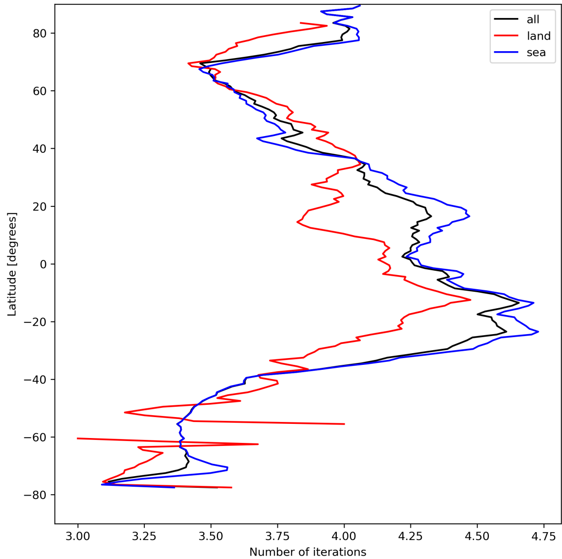
Figure 17: Zonal average of “Number of iterations” for 2024-04-16 to 2024-04-17.
