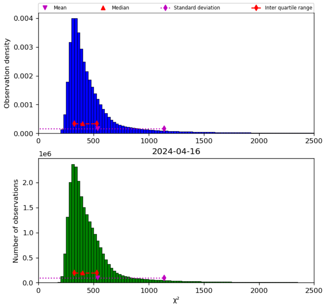
Figure 42: Histogram of “ \chi^2 ” for 2024-04-16 to 2024-04-17
