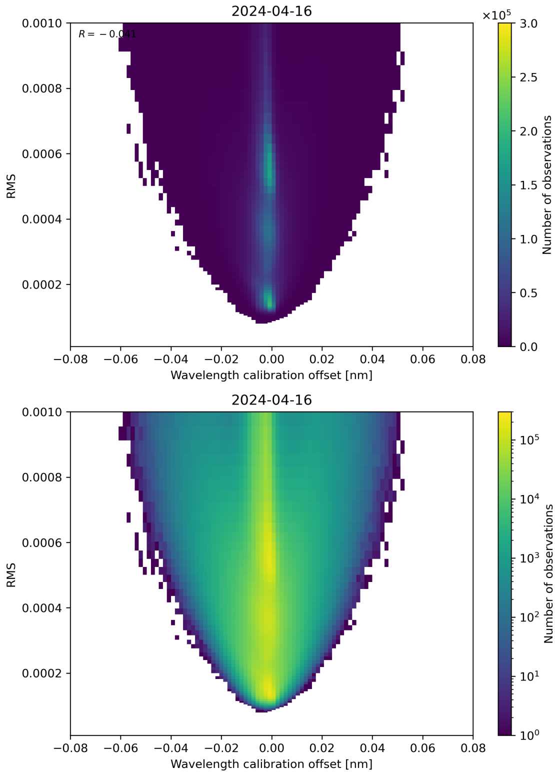
Figure 181: Scatter density plot of “Wavelength calibration offset” against “RMS” for 2024-04-16 to 2024-04-17.
