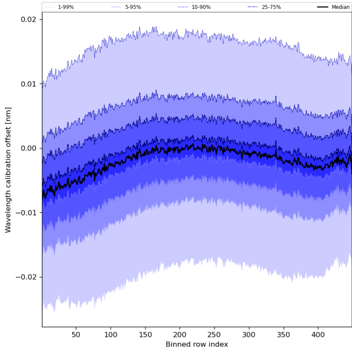
Figure 52: Along track statistics of “Wavelength calibration offset” for 2024-04-16 to 2024-04-17
