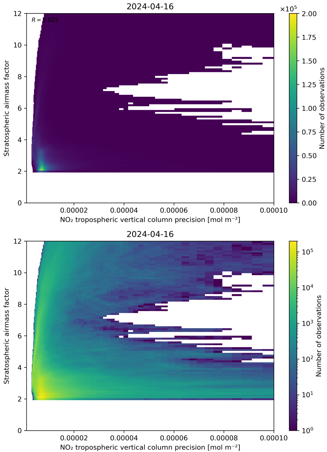
Figure 131: Scatter density plot of “NO 2 tropospheric vertical column precision” against “Stratospheric airmass factor” for 2024-04-16 to 2024-04-17.
