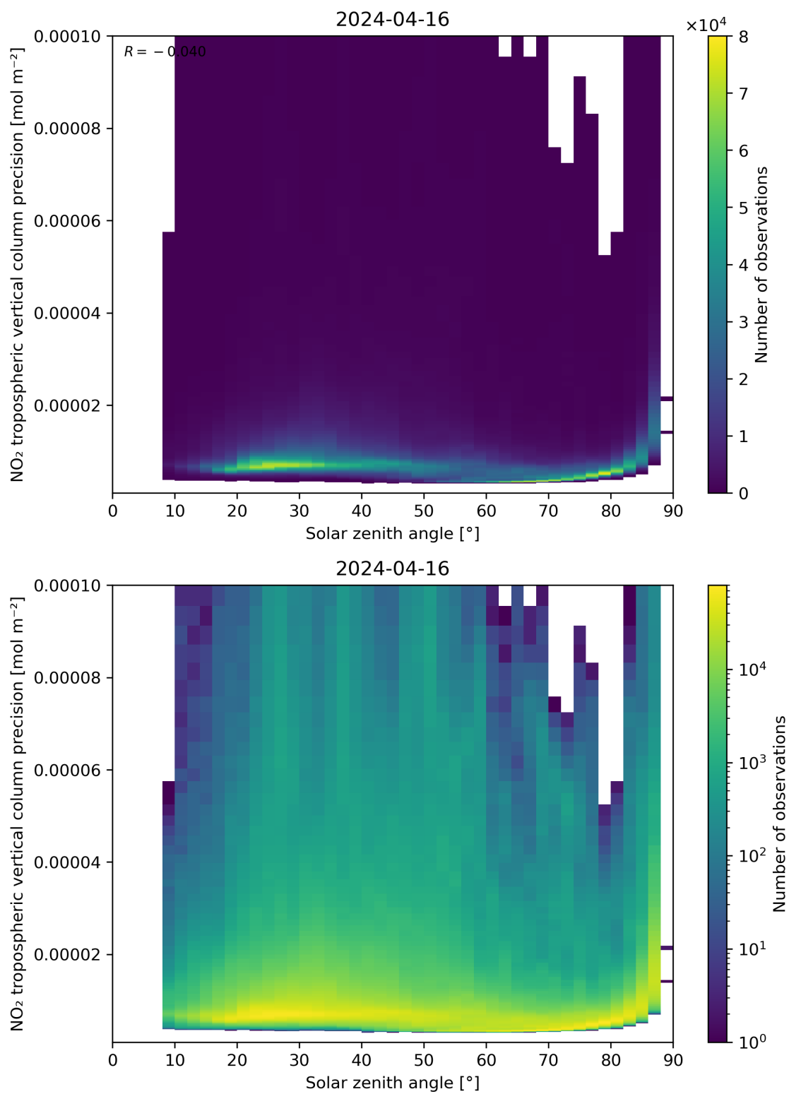
Figure 156: Scatter density plot of “Solar zenith angle” against “NO 2 tropospheric vertical column precision” for 2024-04-16 to 2024-04-17.
