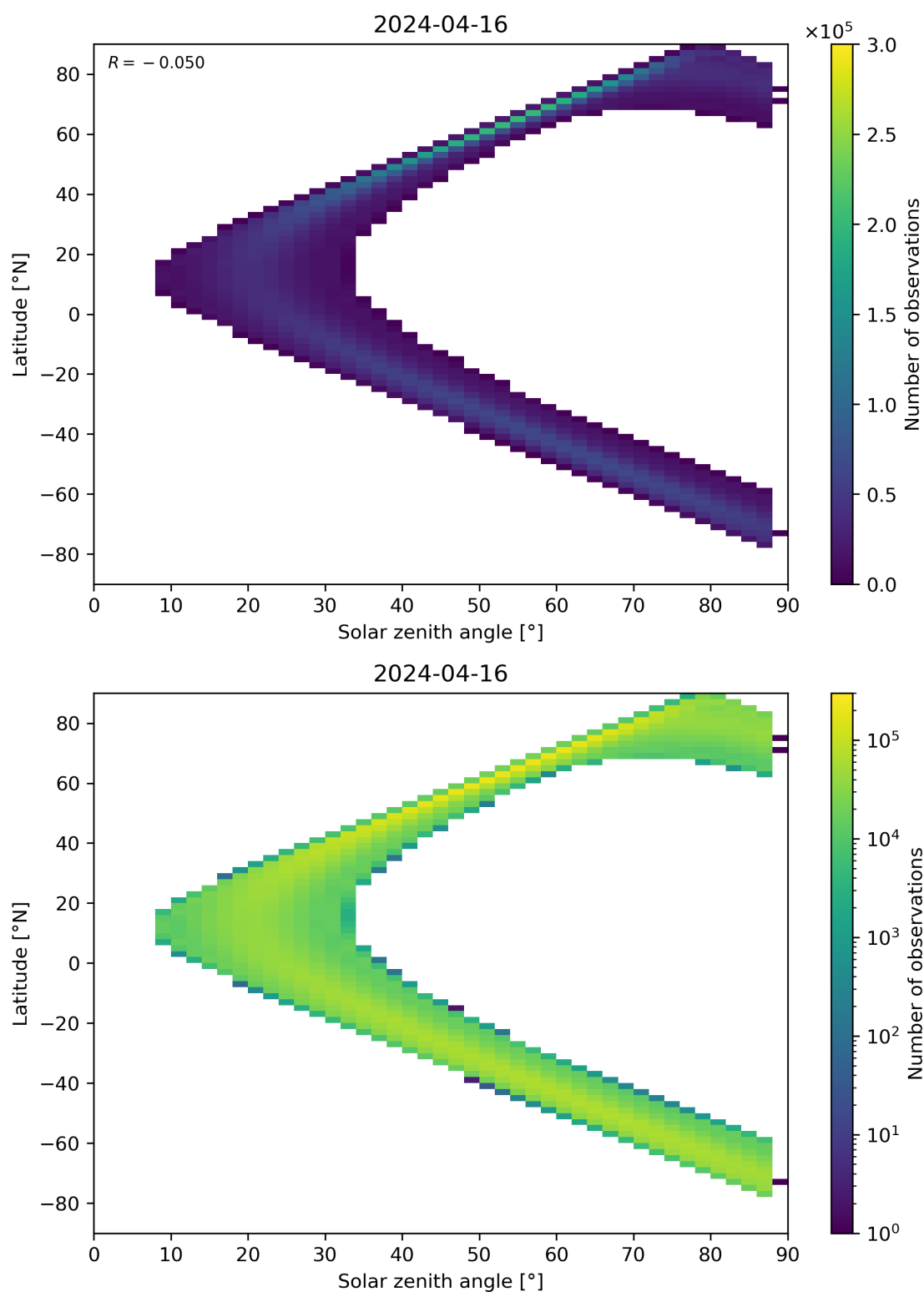
Figure 149: Scatter density plot of “Solar zenith angle” against “Latitude” for 2024-04-16 to 2024-04-17.
