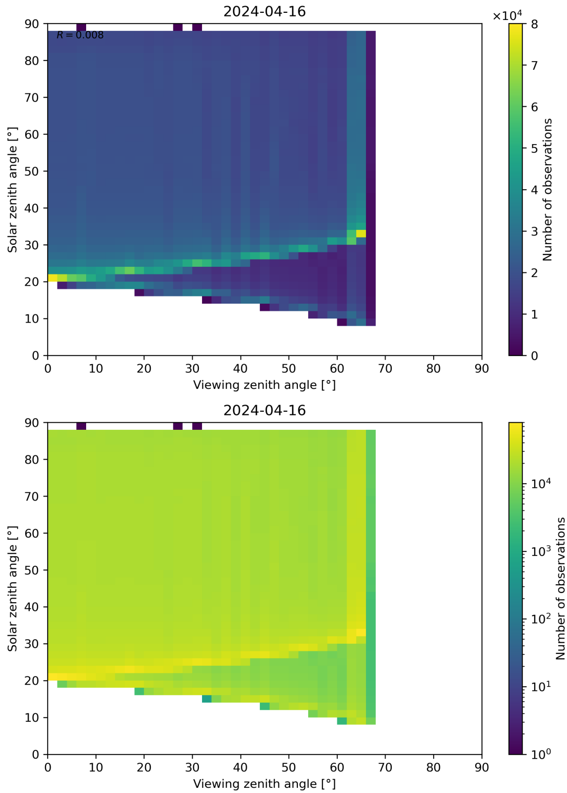
Figure 172: Scatter density plot of “Viewing zenith angle” against “Solar zenith angle” for 2024-04-16 to 2024-04-17.
