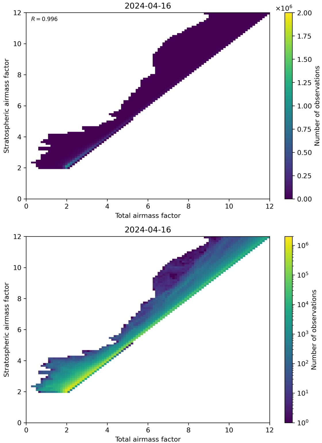
Figure 62: Scatter density plot of “Total airmass factor” against “Stratospheric airmass factor” for 2024-04-16 to 2024-04-17.
