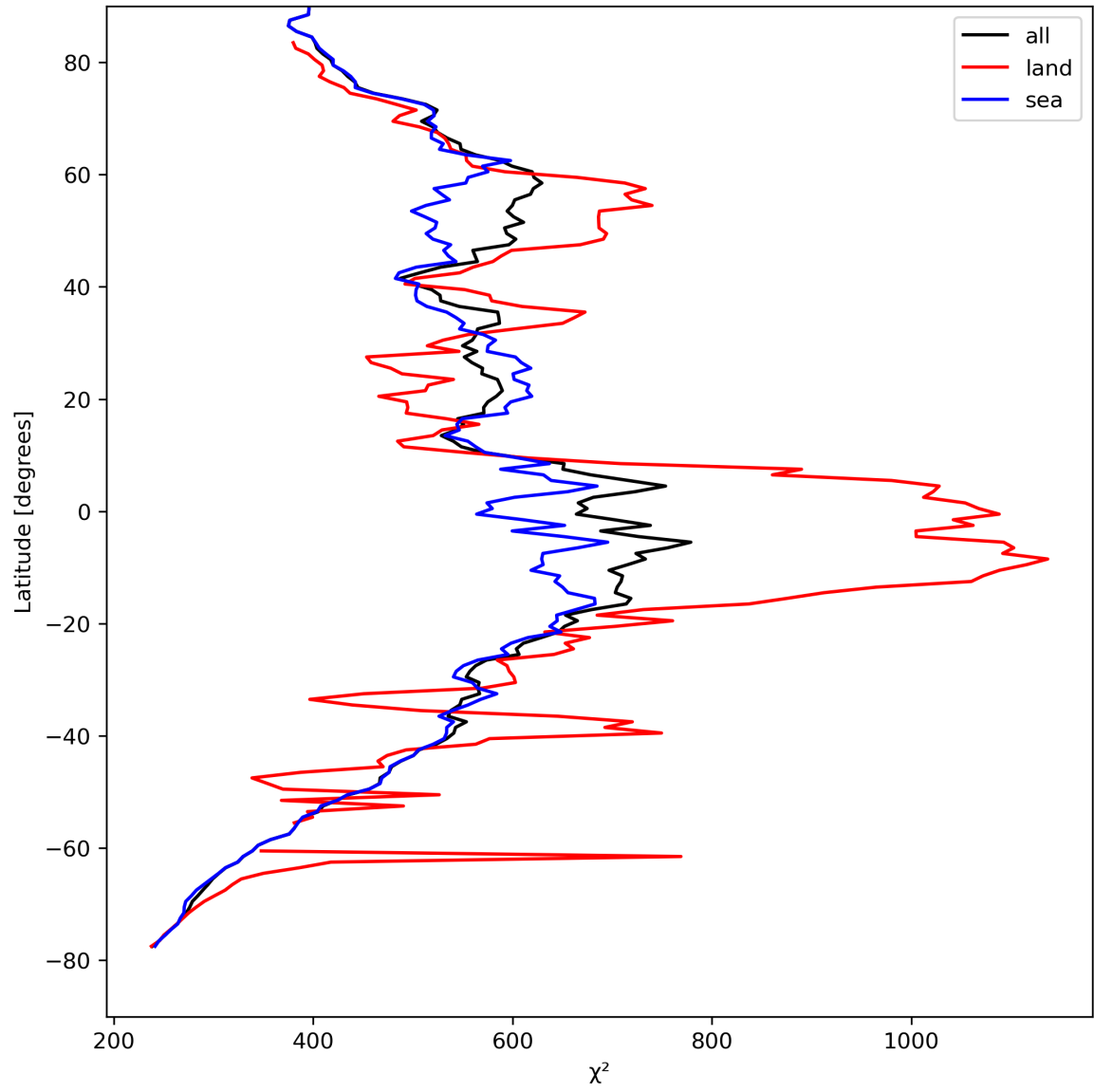
Figure 25: Zonal average of “ \chi^2 ” for 2024-04-16 to 2024-04-17.
