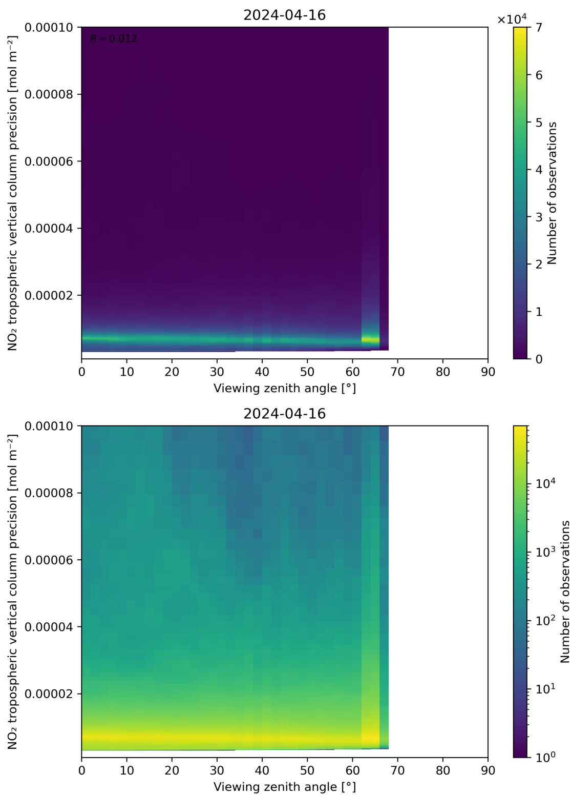
Figure 170: Scatter density plot of “Viewing zenith angle” against “NO 2 tropospheric vertical column precision” for 2024-04-16 to 2024-04-17.
