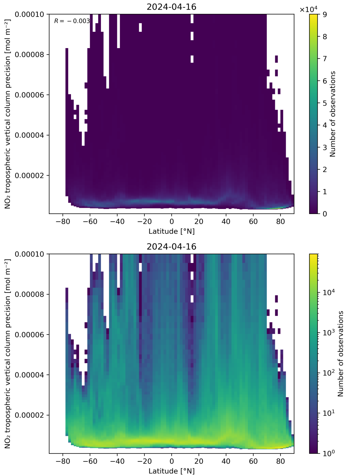
Figure 93: Scatter density plot of “Latitude” against “NO 2 tropospheric vertical column precision” for 2024-04-16 to 2024-04-17.
