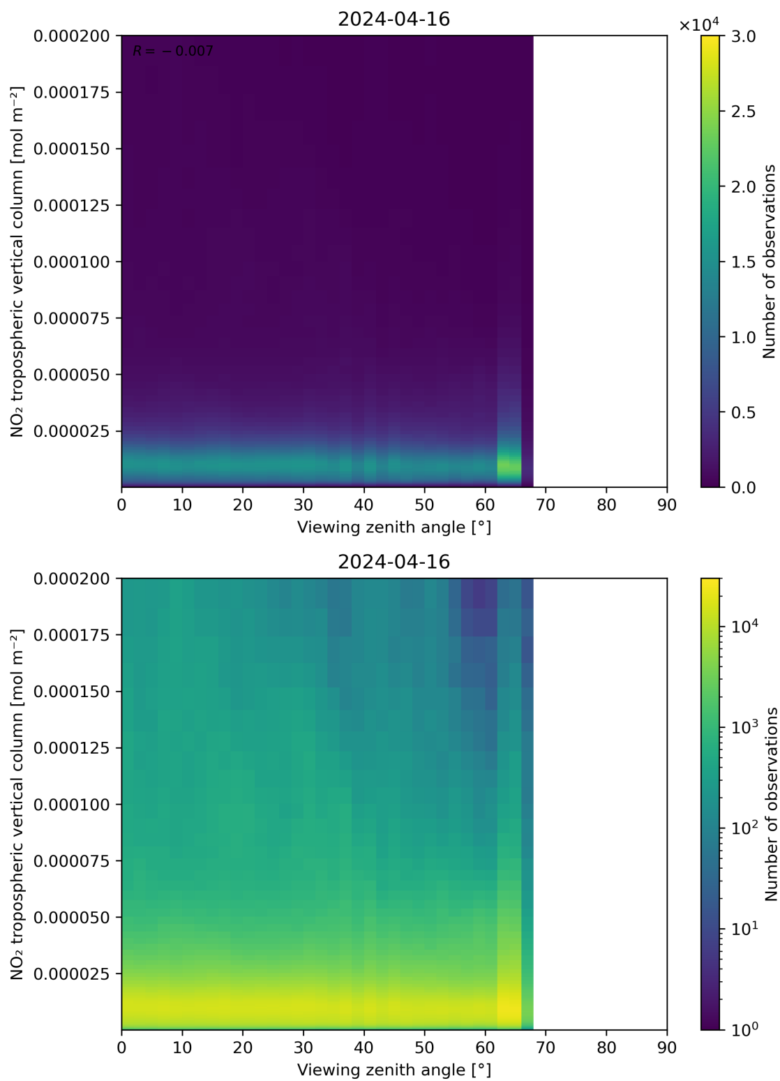
Figure 169: Scatter density plot of “Viewing zenith angle” against “NO 2 tropospheric vertical column” for 2024-04-16 to 2024-04-17.
