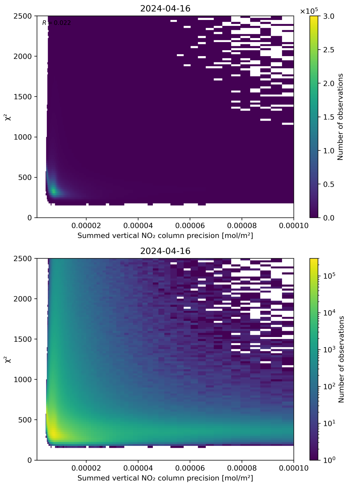
Figure 107: Scatter density plot of “Summed vertical NO 2 column precision” against “ \chi^2 ” for 2024-04-16 to 2024-04-17.
