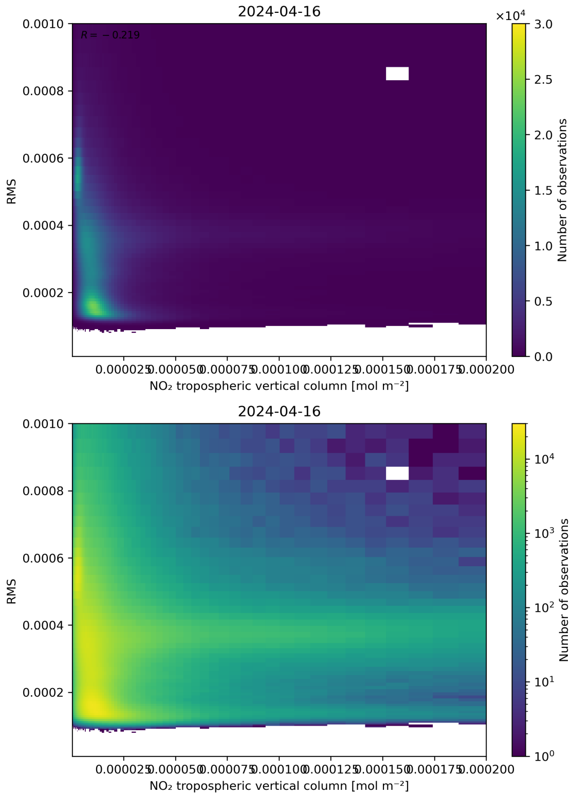
Figure 142: Scatter density plot of “NO 2 tropospheric vertical column” against “RMS” for 2024-04-16 to 2024-04-17.
