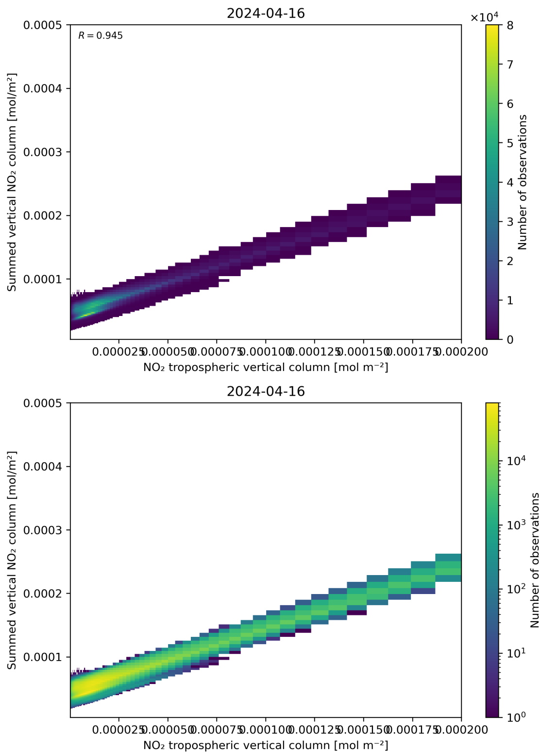
Figure 126: Scatter density plot of “NO 2 tropospheric vertical column” against “Summed vertical NO 2 column” for 2024-04-16 to 2024-04-17.
