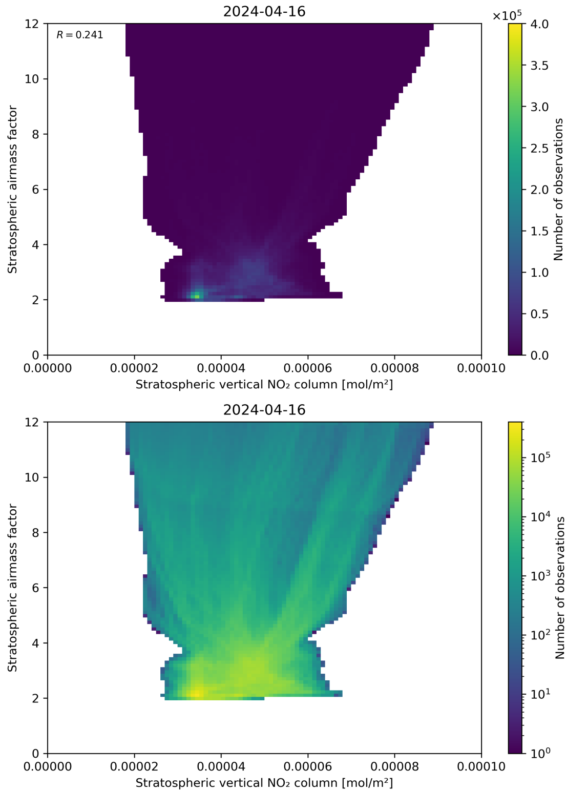
Figure 96: Scatter density plot of “Stratospheric vertical NO 2 column” against “Stratospheric airmass factor” for 2024-04-16 to 2024-04-17.
