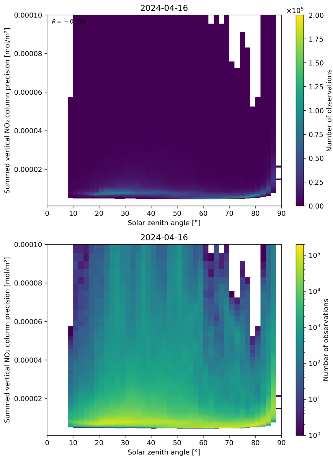
Figure 152: Scatter density plot of “Solar zenith angle” against “Summed vertical NO 2 column precision” for 2024-04-16 to 2024-04-17.
