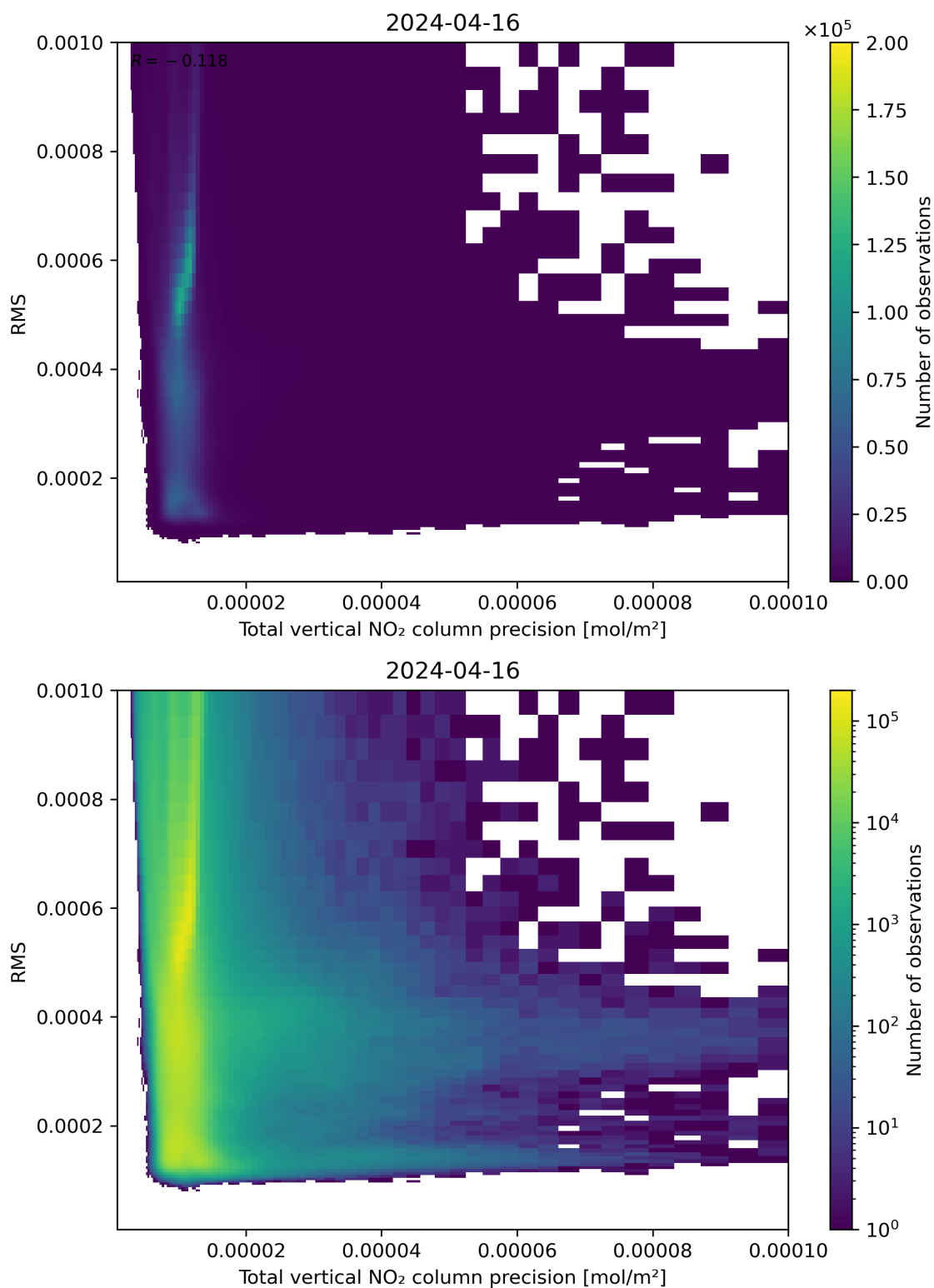
Figure 119: Scatter density plot of “Total vertical NO 2 column precision” against “RMS” for 2024-04-16 to 2024-04-17.
