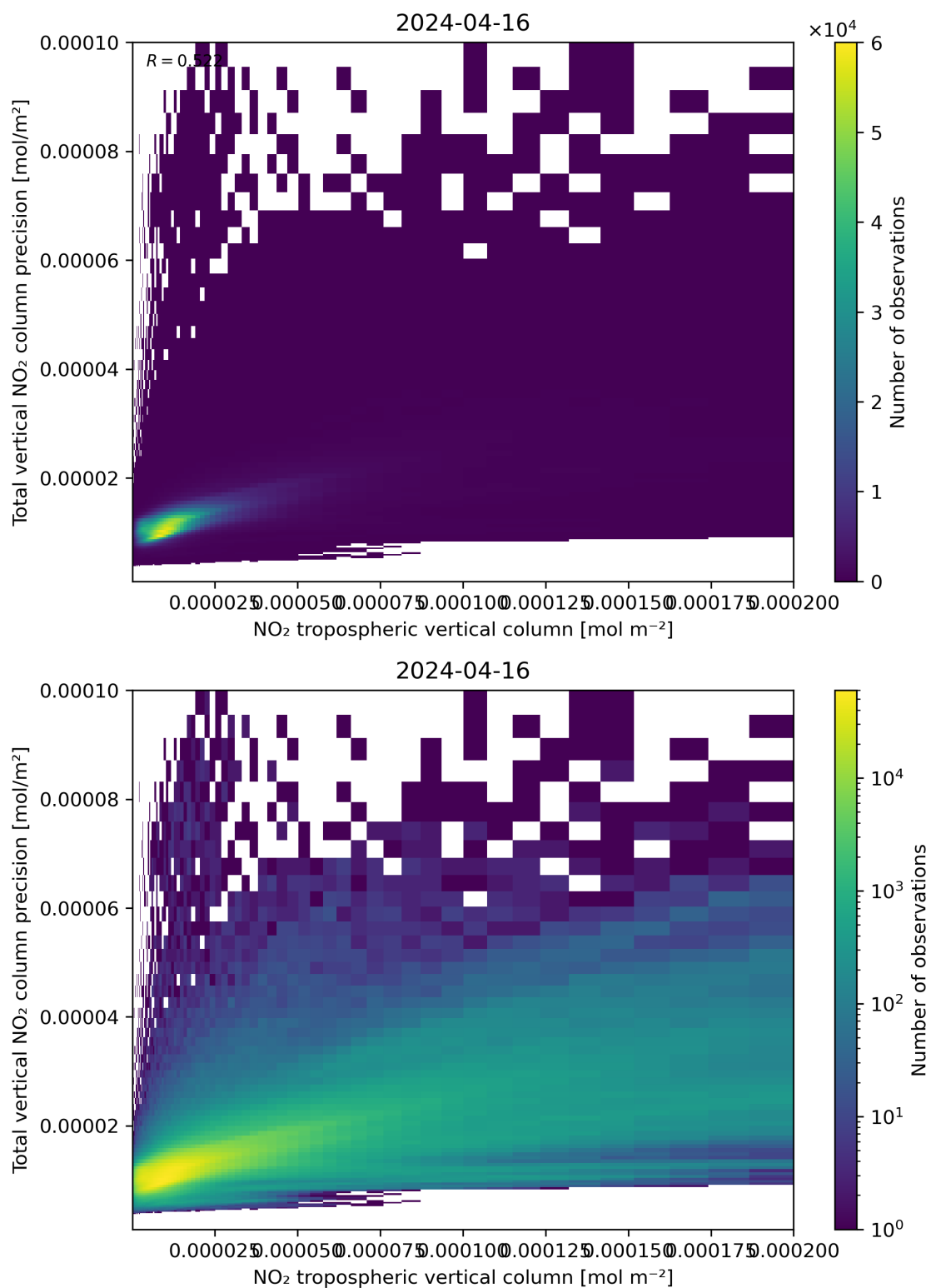
Figure 129: Scatter density plot of “NO 2 tropospheric vertical column” against “Total vertical NO 2 column precision” for 2024-04-16 to 2024-04-17.
