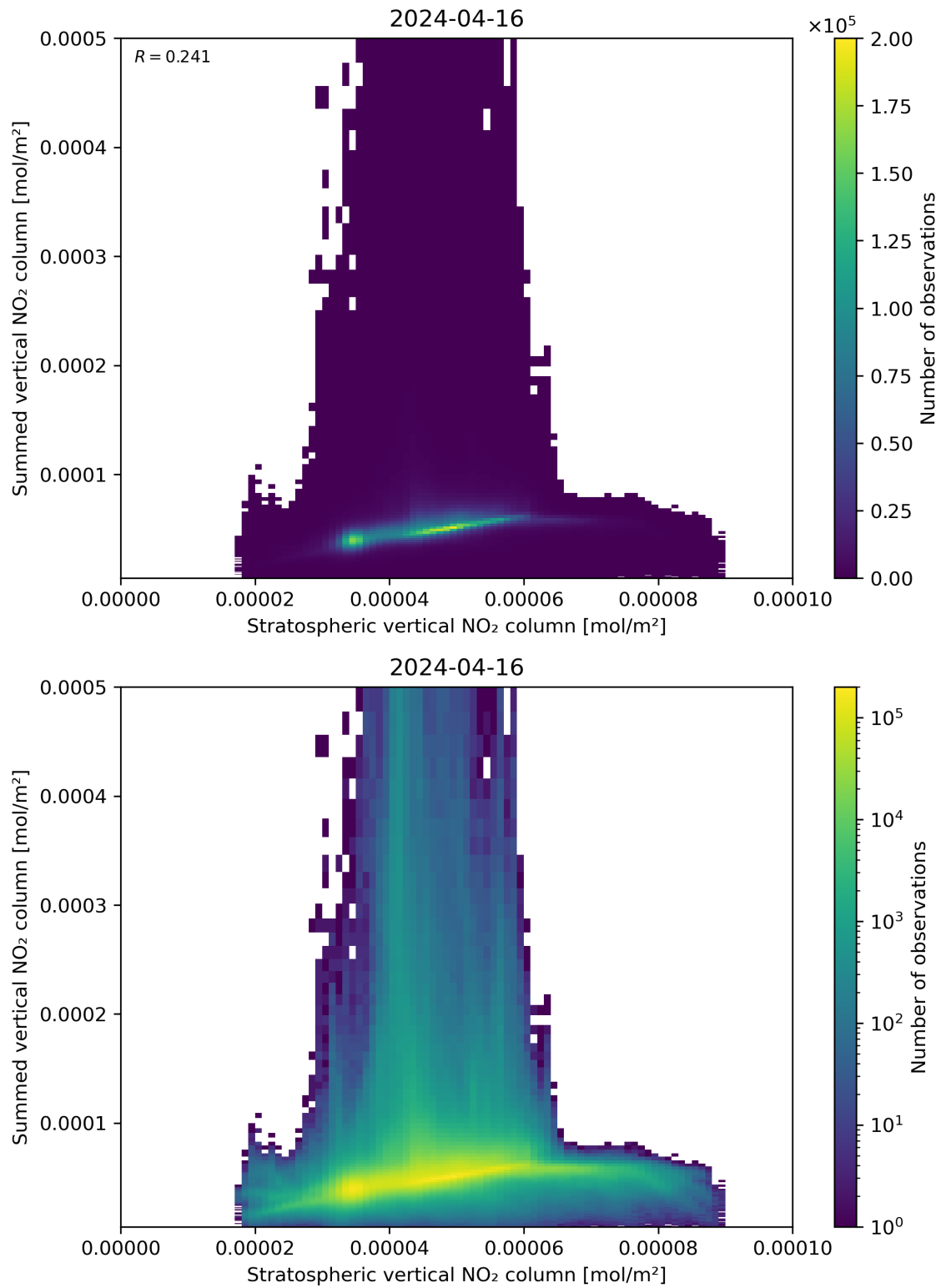
Figure 98: Scatter density plot of “Stratospheric vertical NO 2 column” against “Summed vertical NO 2 column” for 2024-04-16 to 2024-04-17.
