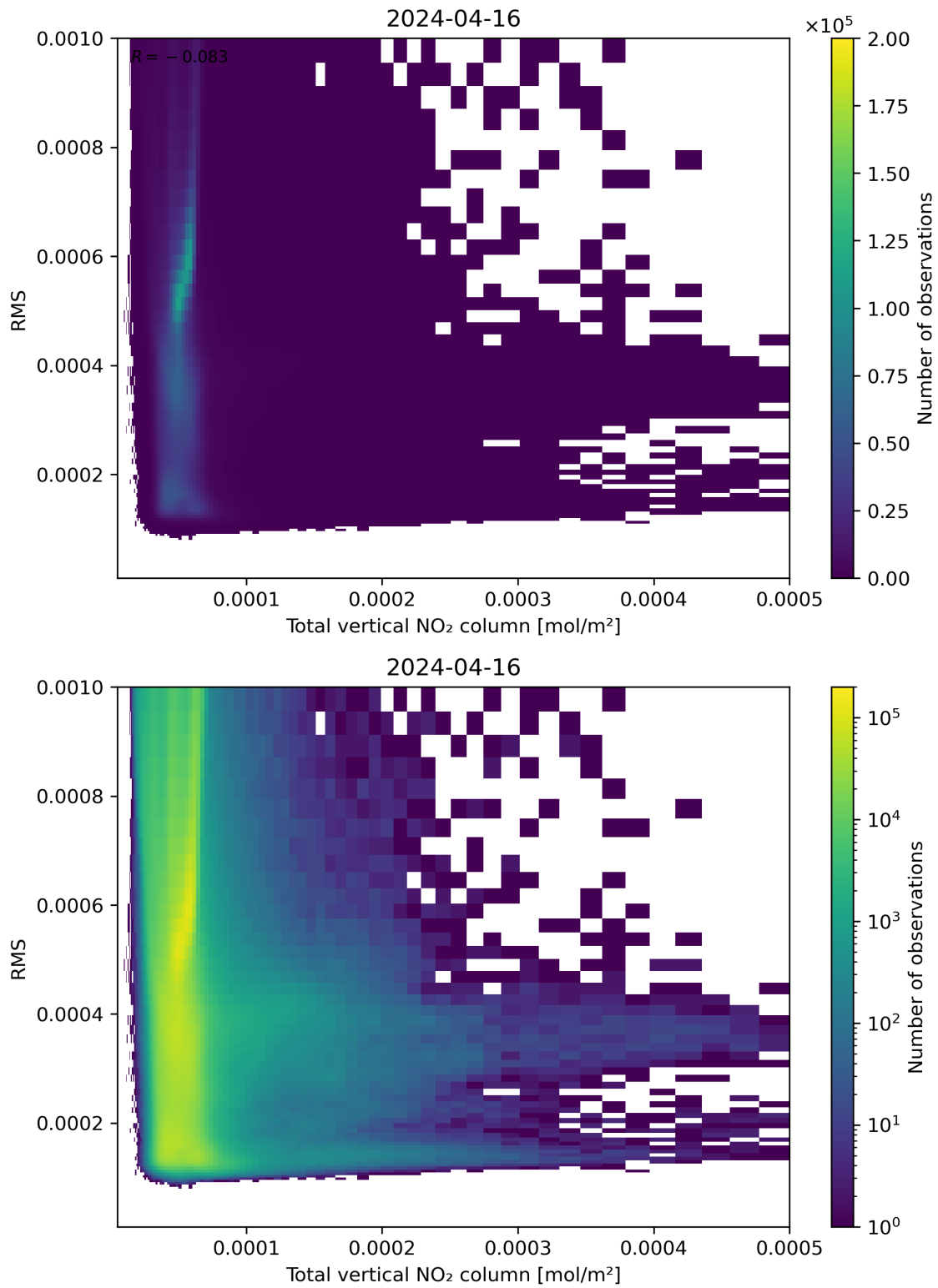
Figure 120: Scatter density plot of “Total vertical NO 2 column” against “RMS” for 2024-04-16 to 2024-04-17.
