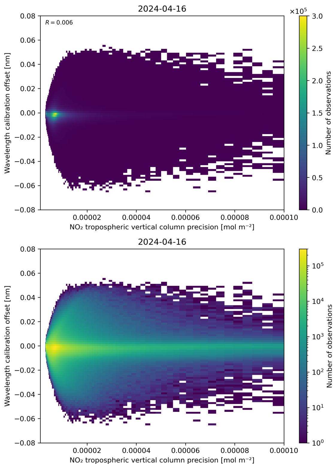
Figure 141: Scatter density plot of “NO 2 tropospheric vertical column precision” against “Wavelength calibration offset” for 2024-04-16 to 2024-04-17.
