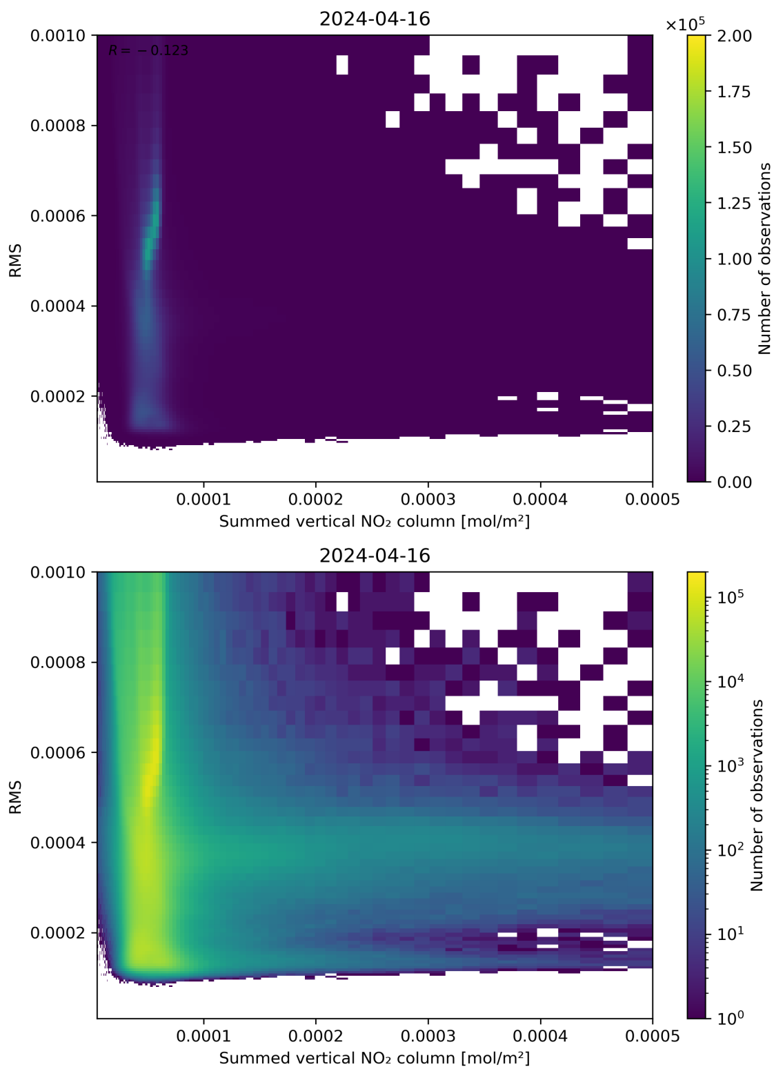
Figure 109: Scatter density plot of “Summed vertical NO 2 column” against “RMS” for 2024-04-16 to 2024-04-17.
