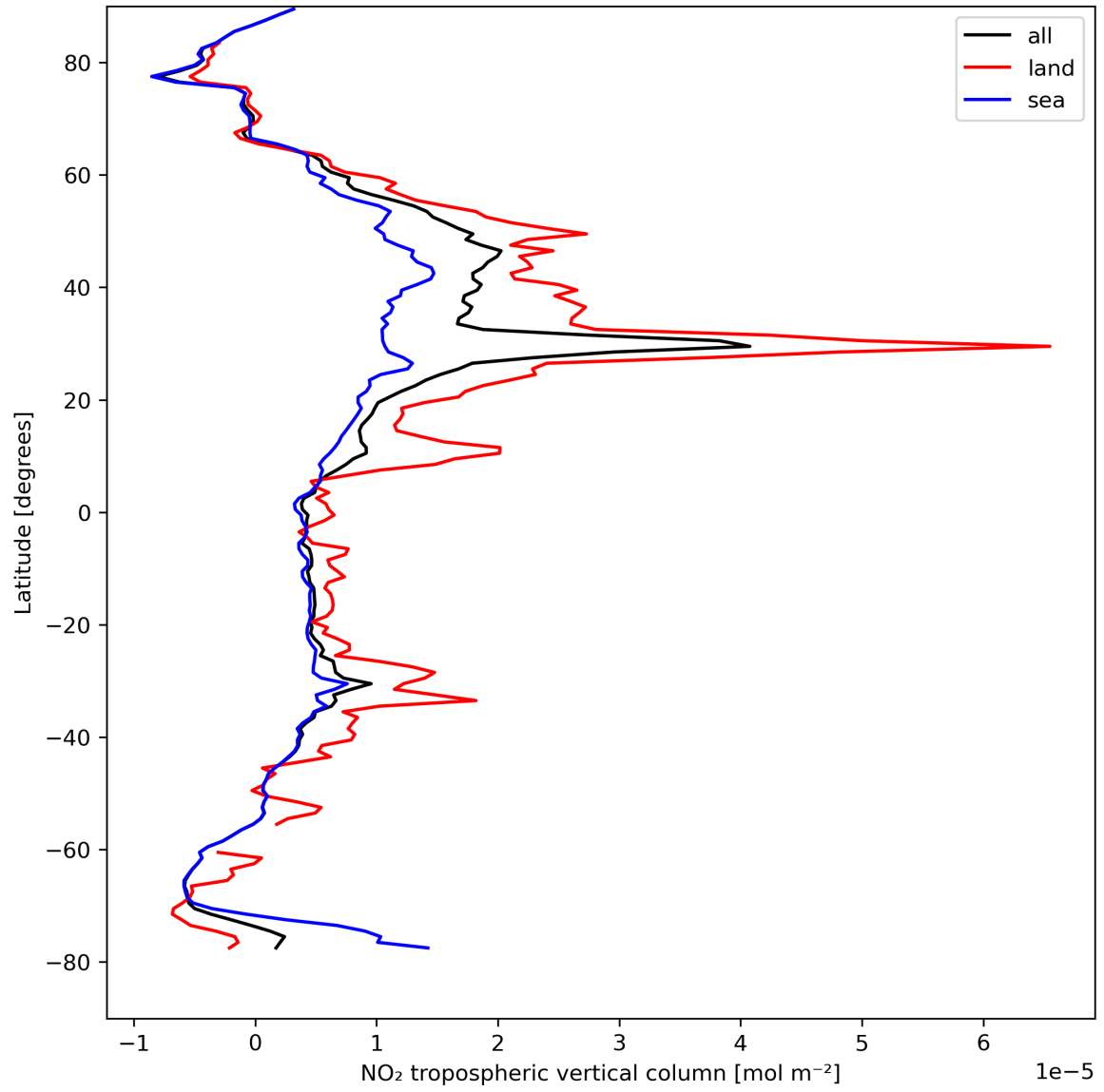
Figure 12: Zonal average of “NO 2 tropospheric vertical column” for 2024-04-16 to 2024-04-17.
