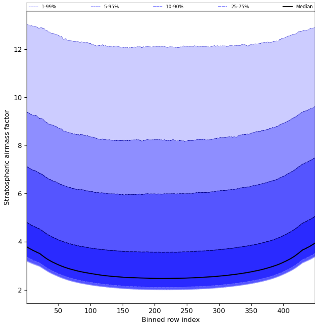
Figure 61: Along track statistics of “Stratospheric air mass factor” for 2024-04-16 to 2024-04-17
