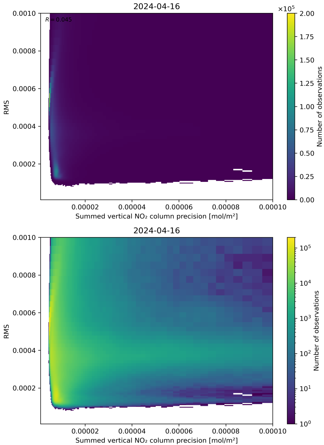
Figure 108: Scatter density plot of “Summed vertical NO 2 column precision” against “RMS” for 2024-04-16 to 2024-04-17.
