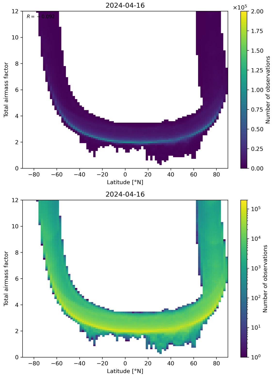
Figure 84: Scatter density plot of “Latitude” against “Total airmass factor” for 2024-04-16 to 2024-04-17.
