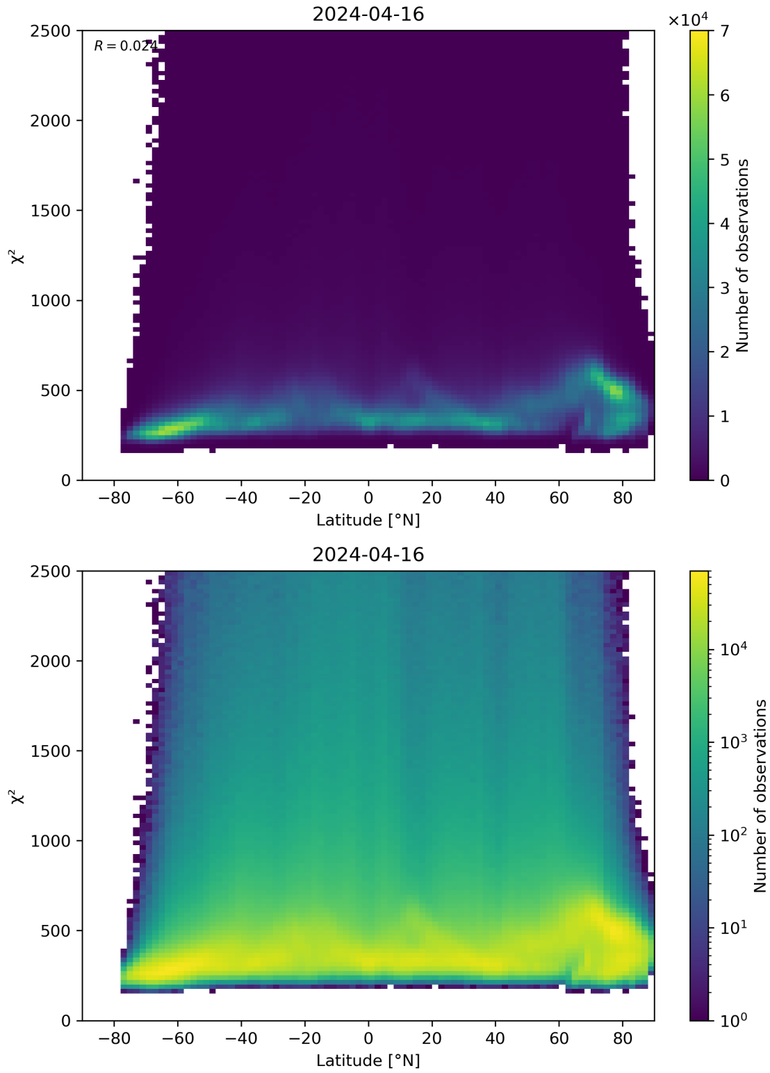
Figure 86: Scatter density plot of “Latitude” against “ \chi^2 ” for 2024-04-16 to 2024-04-17.
