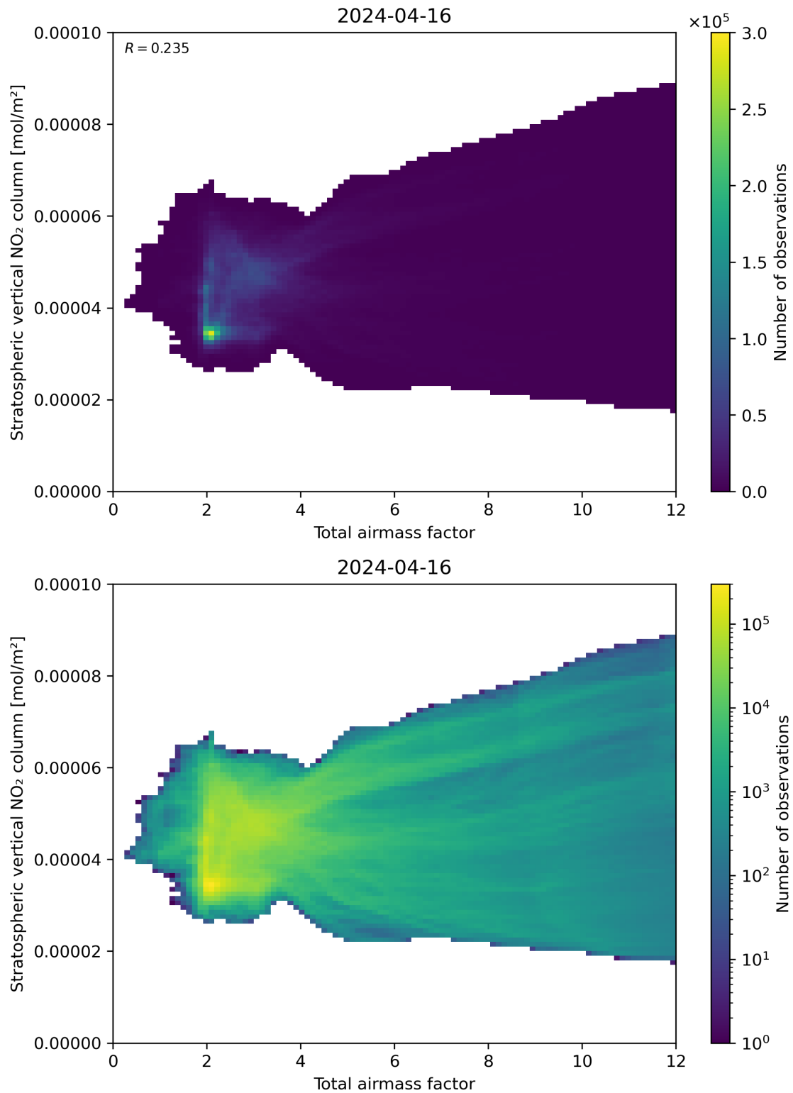
Figure 64: Scatter density plot of “Total airmass factor” against “Stratospheric vertical \text{NO}_2 column” for 2024-04-16 to 2024-04-17.
