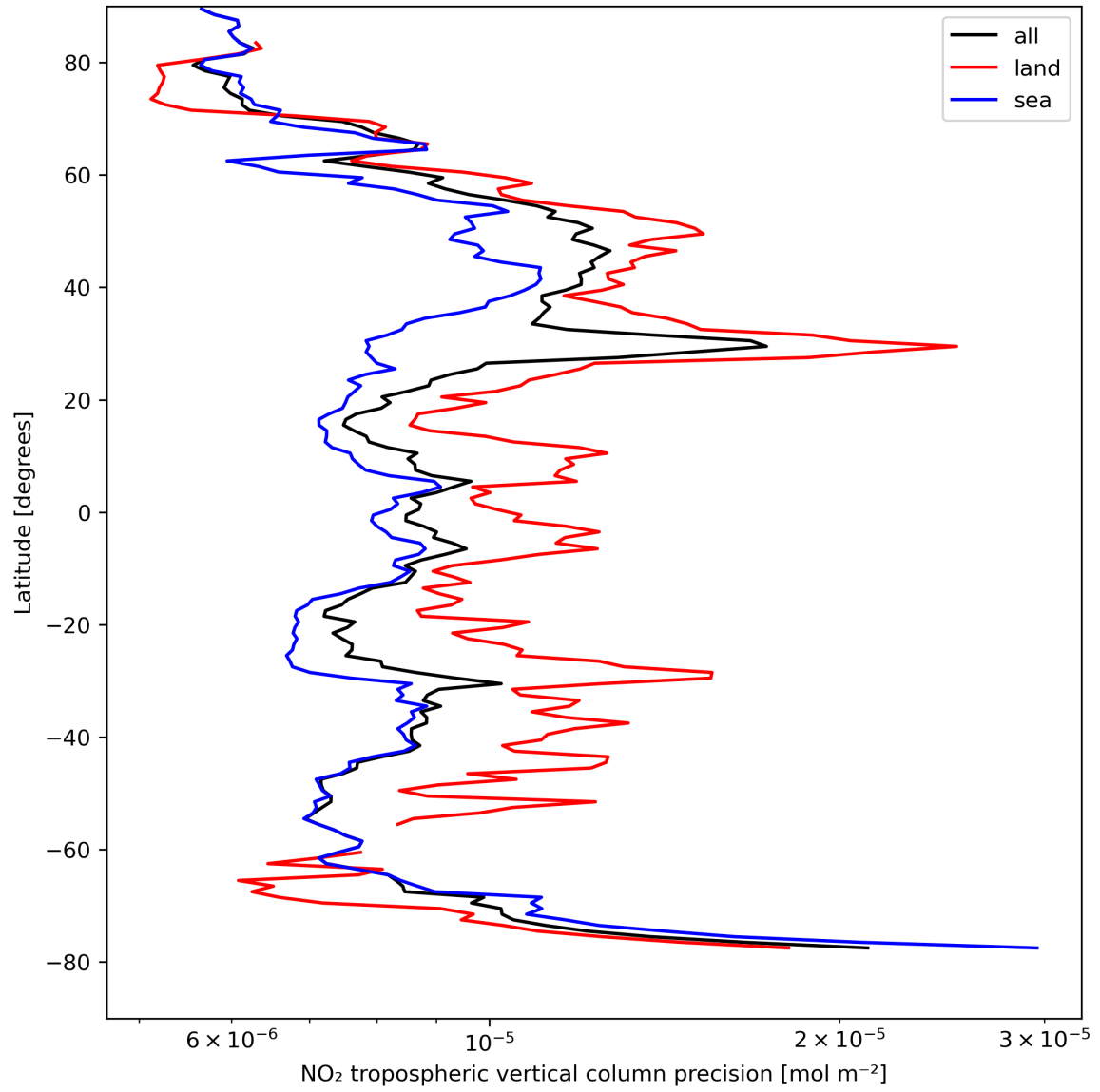
Figure 13: Zonal average of “NO 2 tropospheric vertical column precision” for 2024-04-16 to 2024-04-17.
