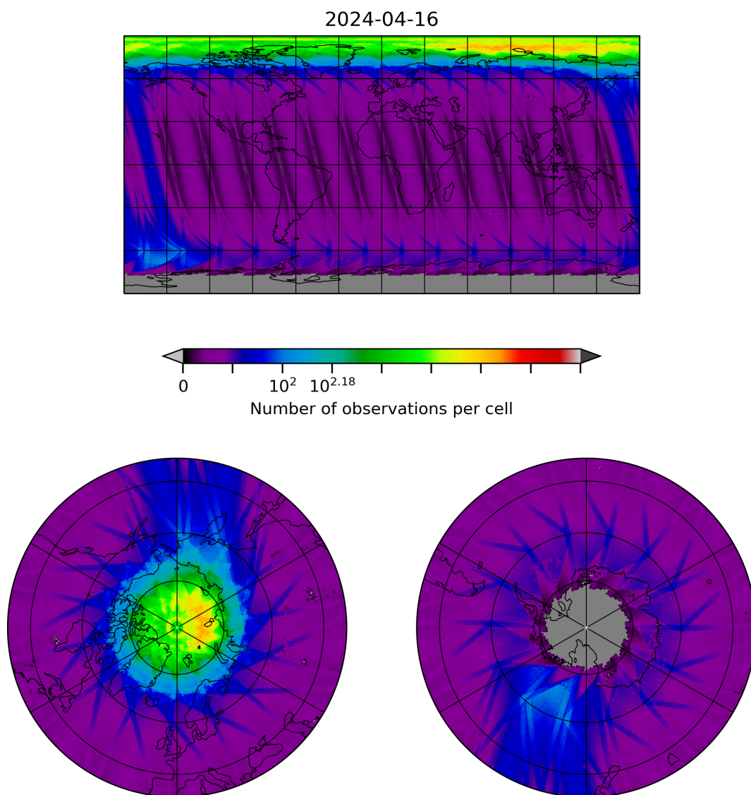
Figure 10: Map of the number of observations for 2024-04-16 to 2024-04-17
