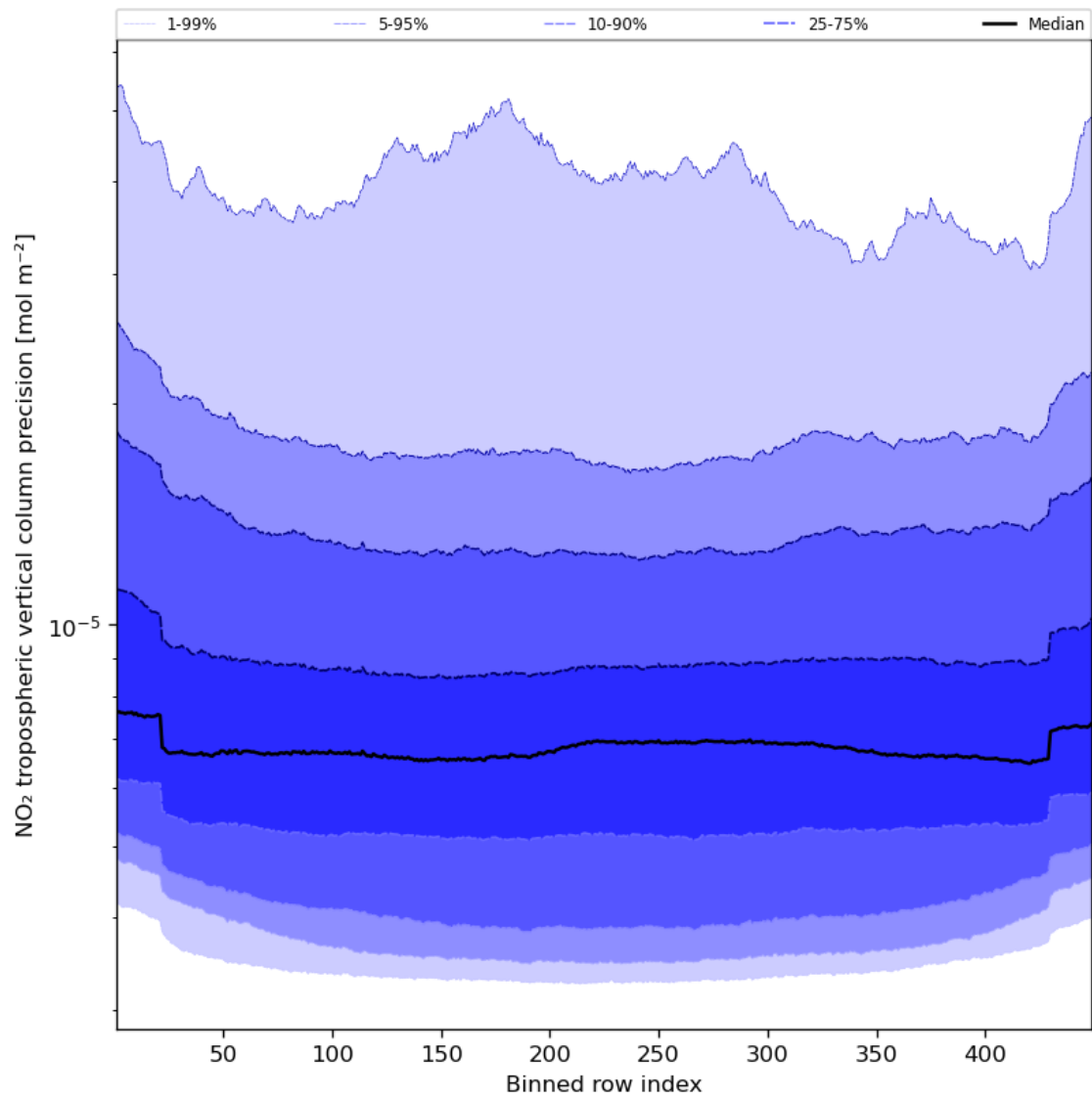
Figure 47: Along track statistics of “NO 2 tropospheric vertical column precision” for 2024-04-16 to 2024-04-17
