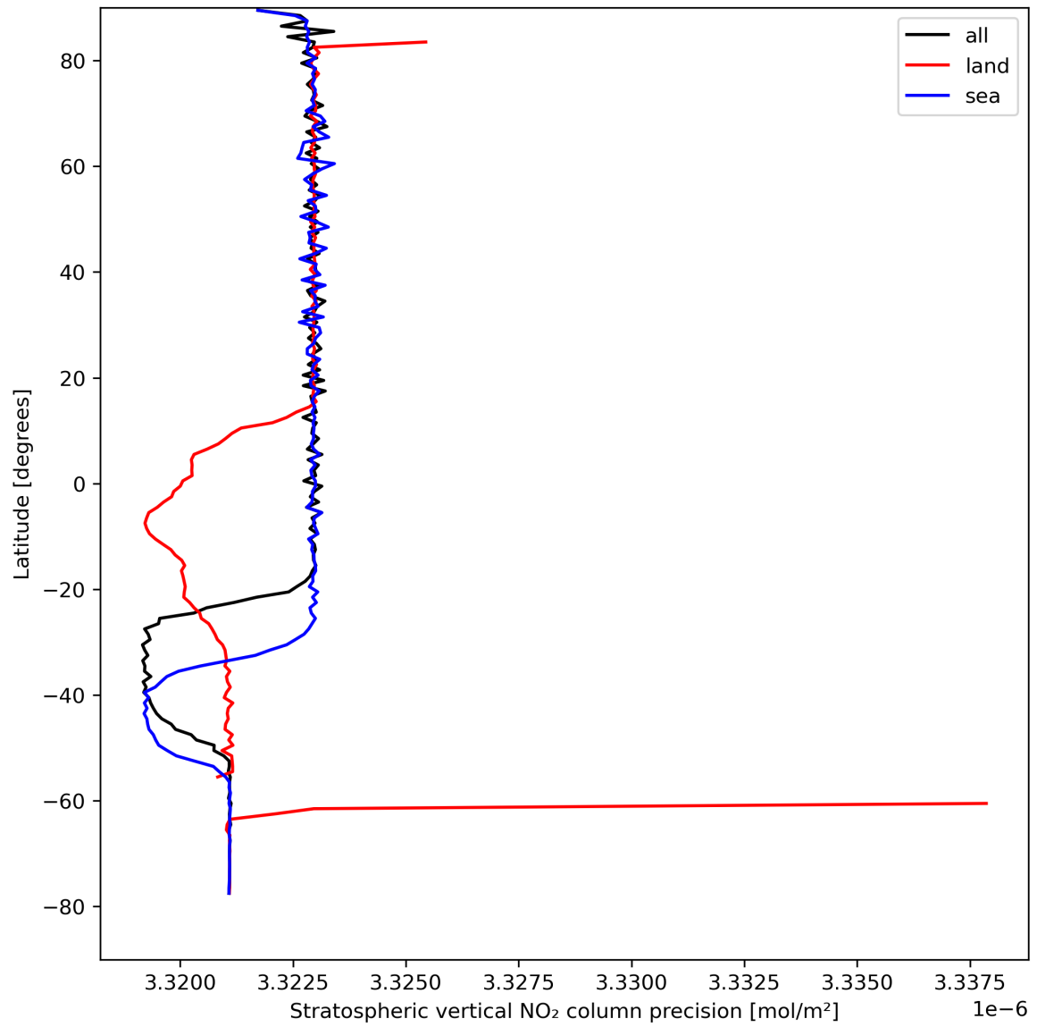
Figure 20: Zonal average of “Stratospheric vertical NO 2 column precision” for 2024-04-16 to 2024-04-17.
