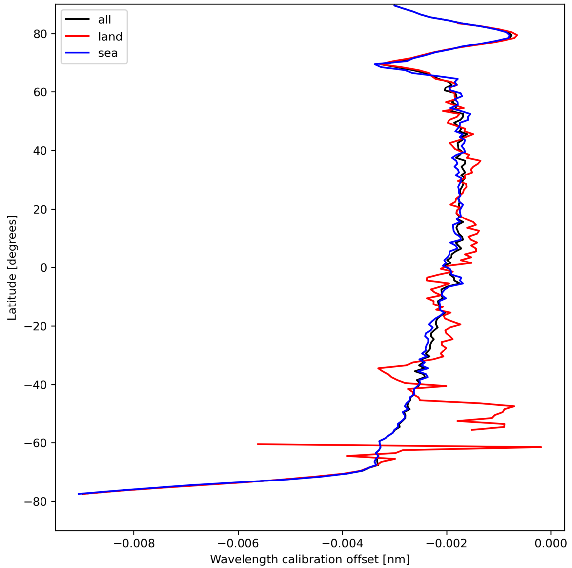
Figure 18: Zonal average of “Wavelength calibration offset” for 2024-04-16 to 2024-04-17.
