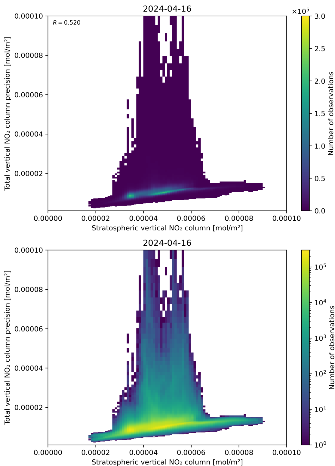
Figure 101: Scatter density plot of “Stratospheric vertical NO 2 column” against “Total vertical NO 2 column precision” for 2024-04-16 to 2024-04-17.
