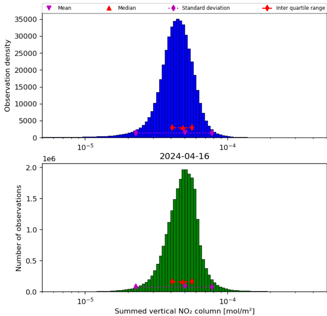
Figure 40: Histogram of “Summed vertical NO 2 column” for 2024-04-16 to 2024-04-17
