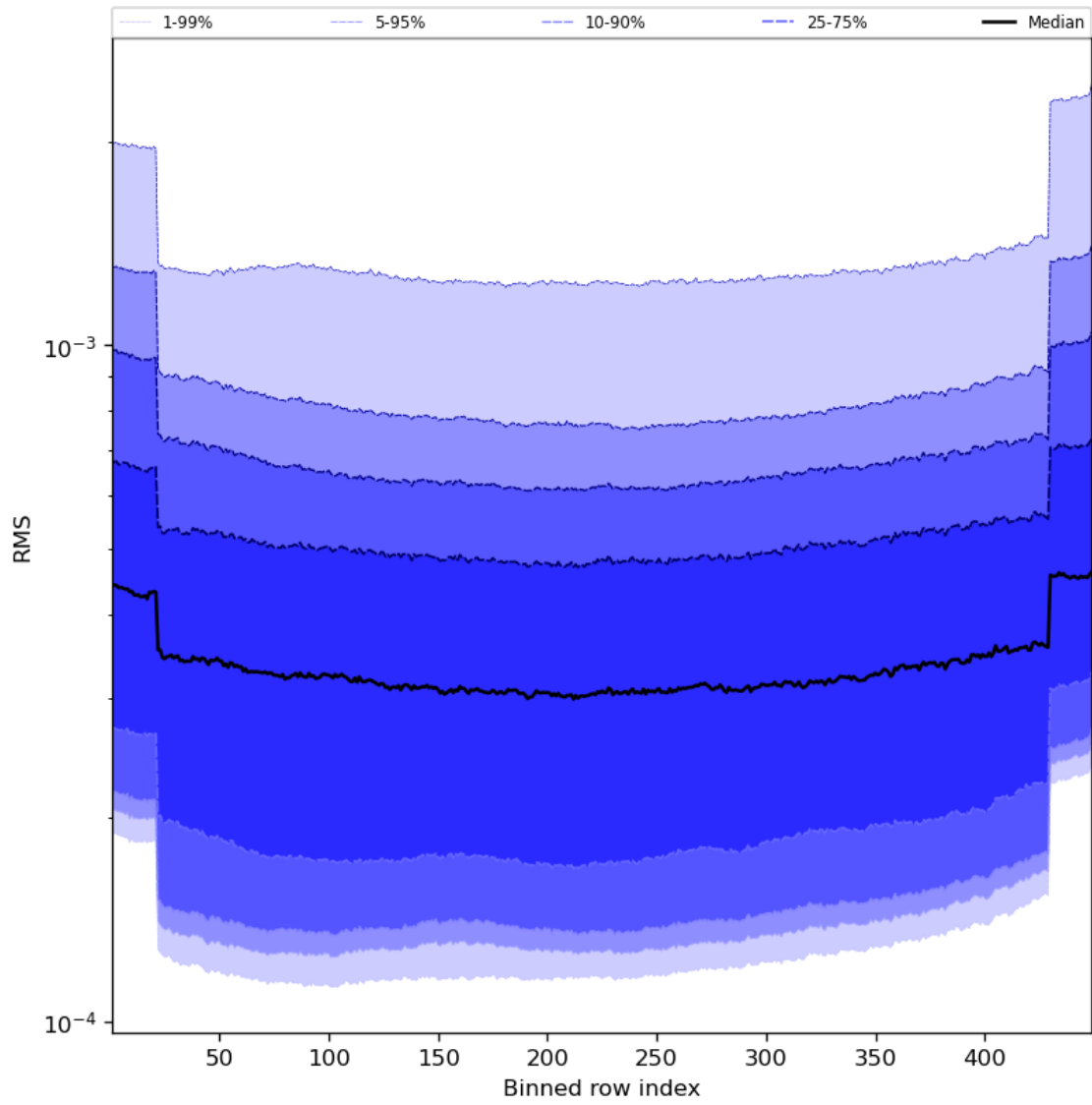
Figure 60: Along track statistics of “RMS” for 2024-04-16 to 2024-04-17
