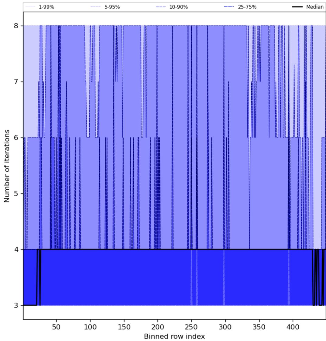
Figure 51: Along track statistics of “Number of iterations” for 2024-04-16 to 2024-04-17
