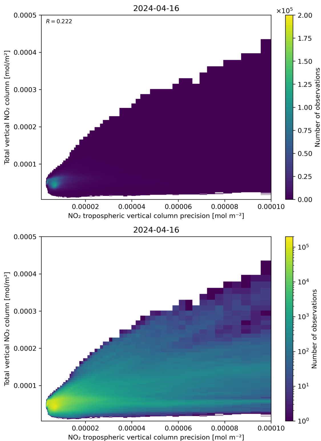
Figure 138: Scatter density plot of “NO 2 tropospheric vertical column precision” against “Total vertical NO 2 column” for 2024-04-16 to 2024-04-17.
