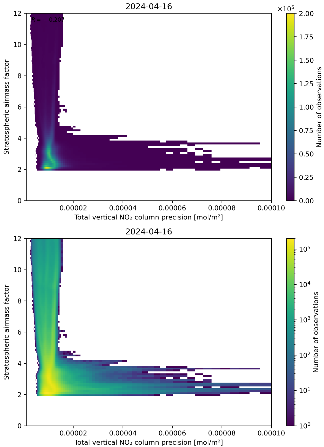
Figure 115: Scatter density plot of “Total vertical NO 2 column precision” against “Stratospheric airmass factor” for 2024-04-16 to 2024-04-17.
