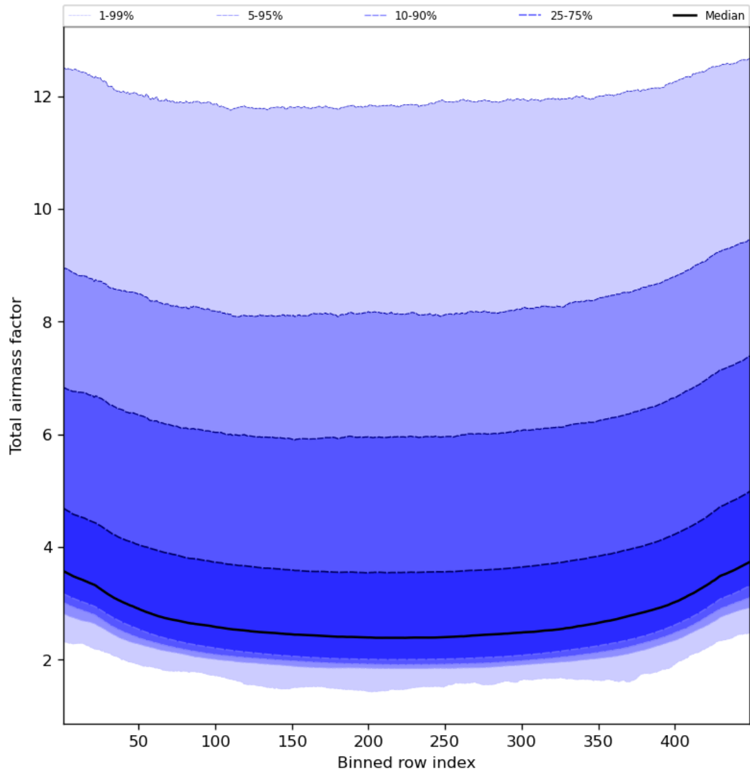
Figure 49: Along track statistics of “Total airmass factor” for 2024-04-16 to 2024-04-17
