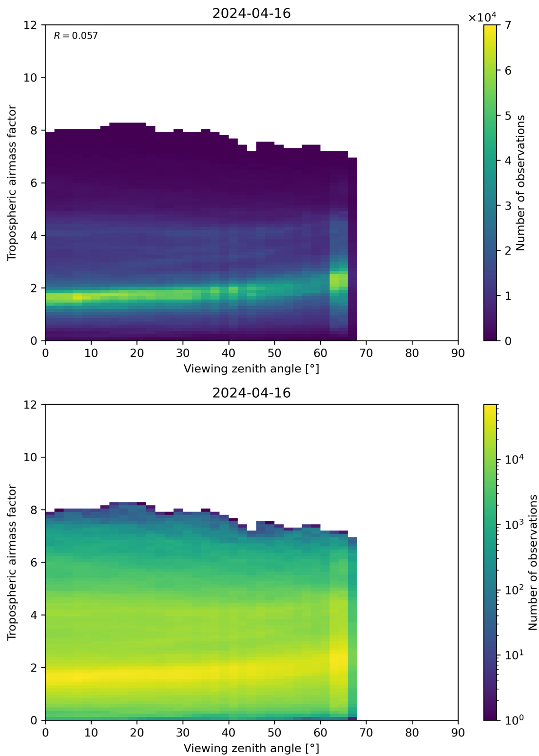
Figure 161: Scatter density plot of “Viewing zenith angle” against “Tropospheric airmass factor” for 2024-04-16 to 2024-04-17.
