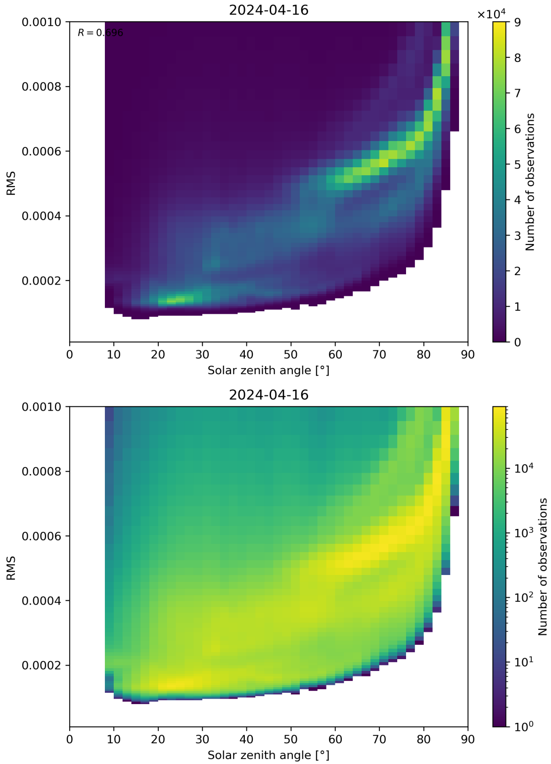
Figure 157: Scatter density plot of “Solar zenith angle” against “RMS” for 2024-04-16 to 2024-04-17.
