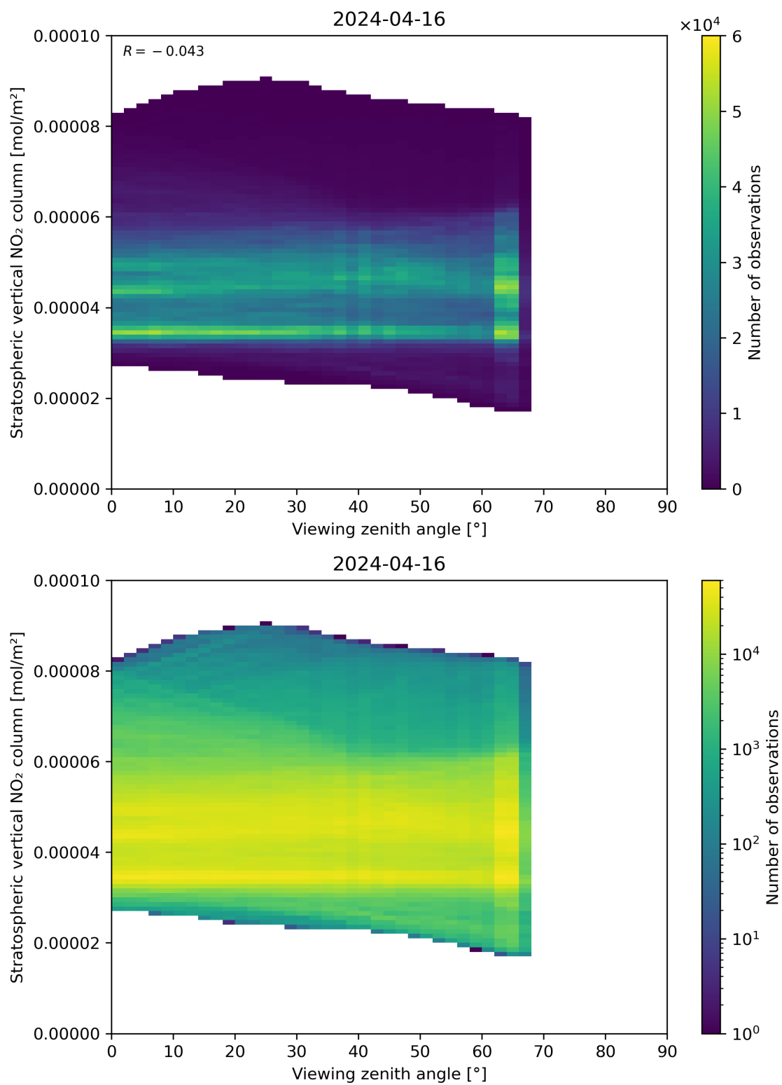
Figure 164: Scatter density plot of “Viewing zenith angle” against “Stratospheric vertical NO 2 column” for 2024-04-16 to 2024-04-17.
