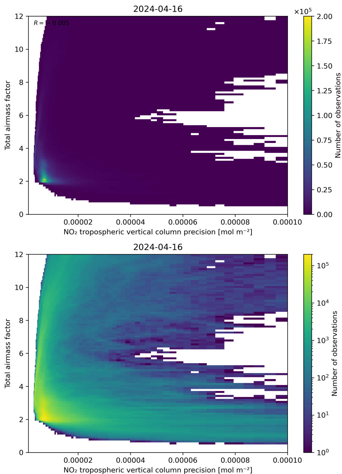
Figure 132: Scatter density plot of “NO 2 tropospheric vertical column precision” against “Total air mass factor” for 2024-04-16 to 2024-04-17.
