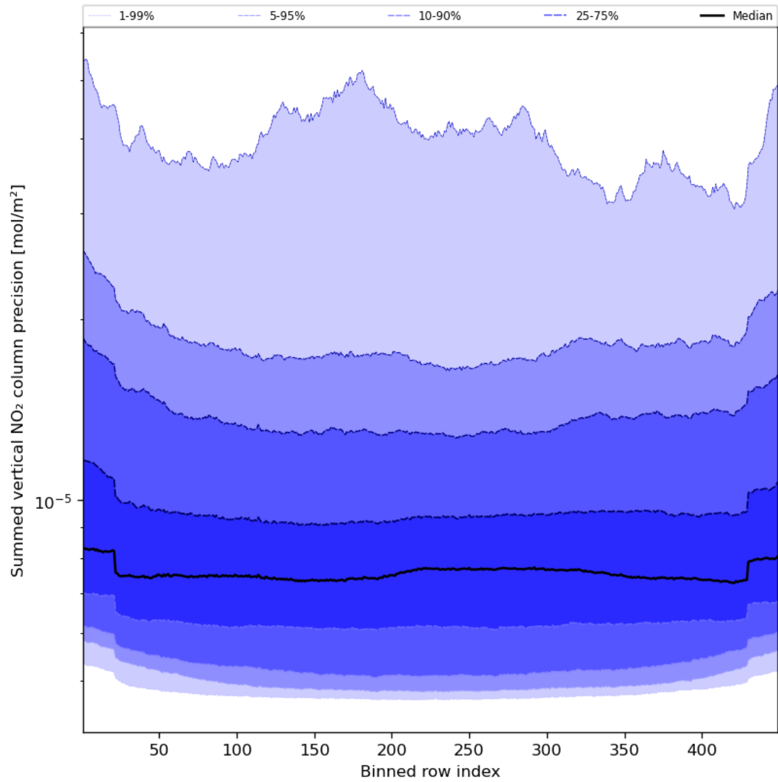
Figure 58: Along track statistics of “Summed vertical NO 2 column precision” for 2024-04-16 to 2024-04-17
