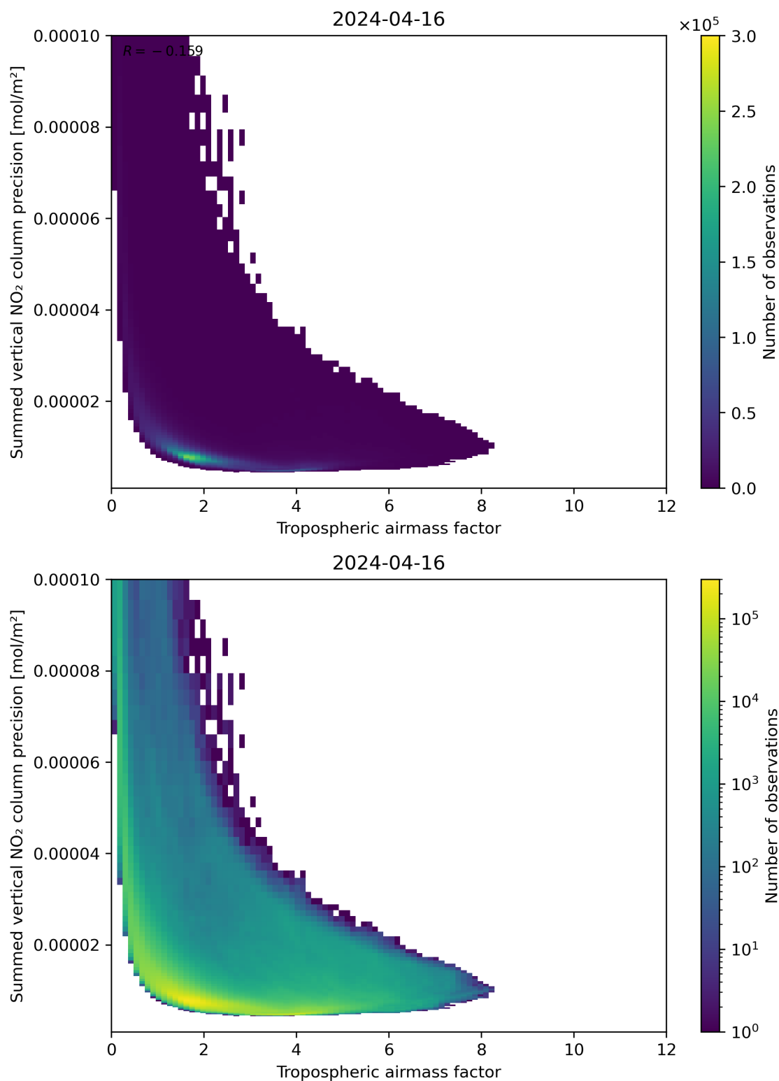
Figure 76: Scatter density plot of “Tropospheric air mass factor” against “Summed vertical NO 2 column precision” for 2024-04-16 to 2024-04-17.
