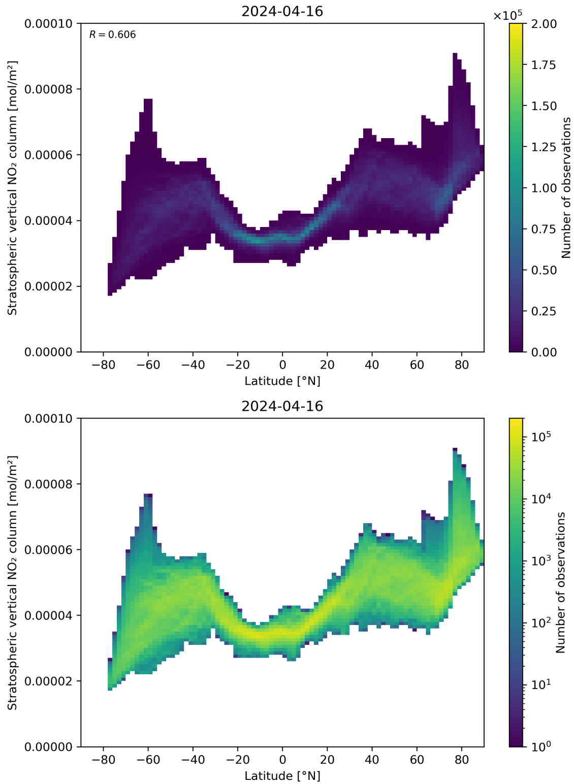
Figure 87: Scatter density plot of “Latitude” against “Stratospheric vertical NO 2 column” for 2024-04-16 to 2024-04-17.
