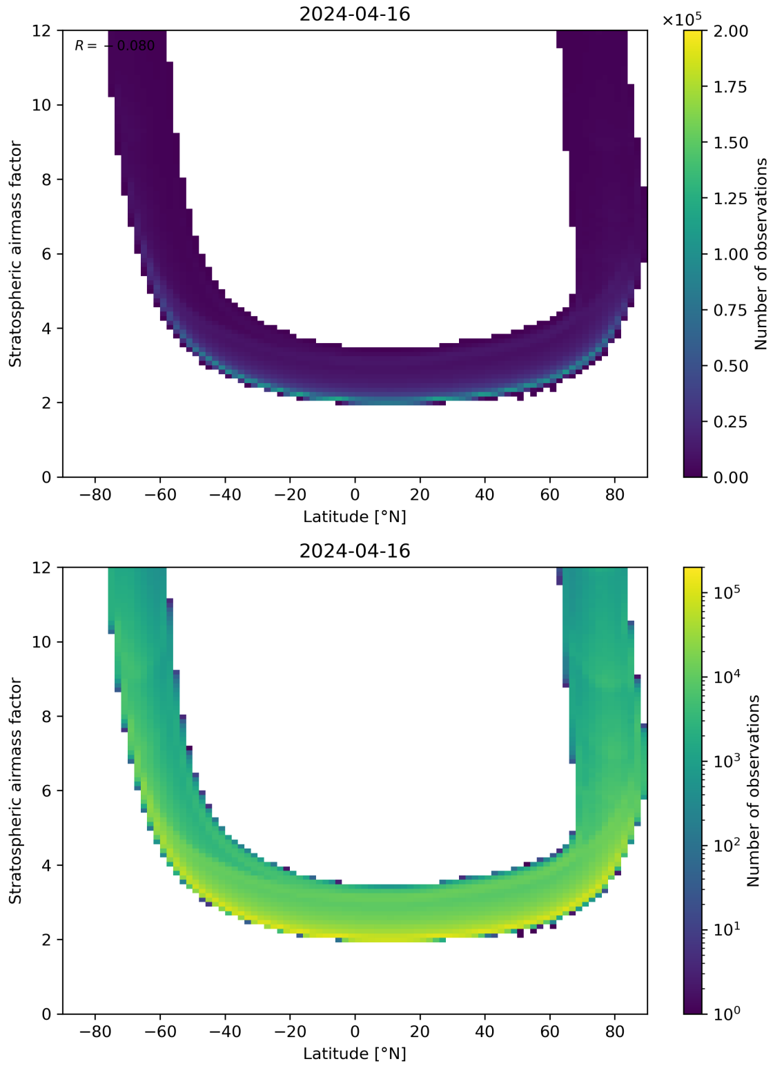
Figure 83: Scatter density plot of “Latitude” against “Stratospheric air mass factor” for 2024-04-16 to 2024-04-17.
