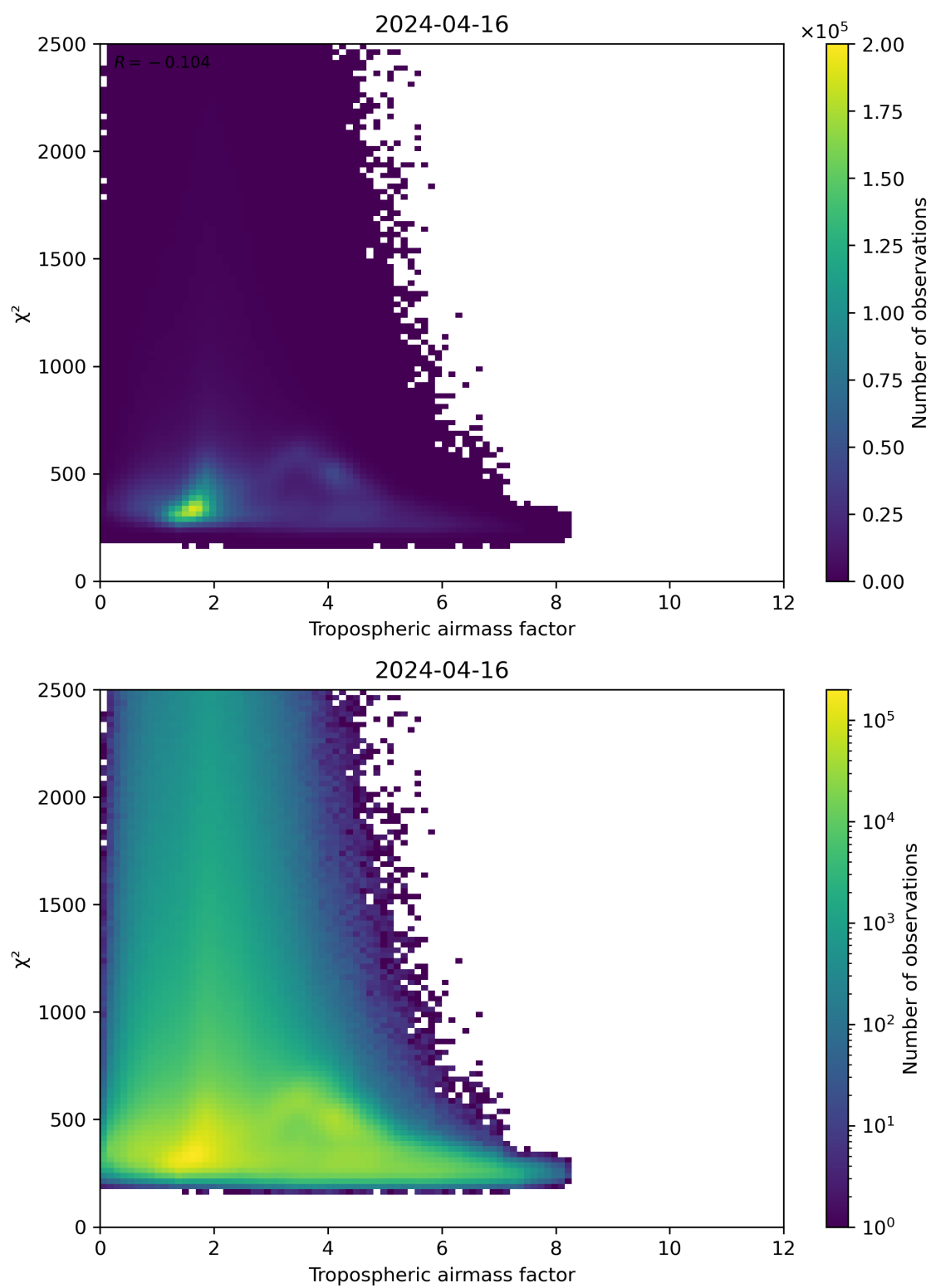
Figure 73: Scatter density plot of “Tropospheric airmass factor” against “ \chi^2 ” for 2024-04-16 to 2024-04-17.
