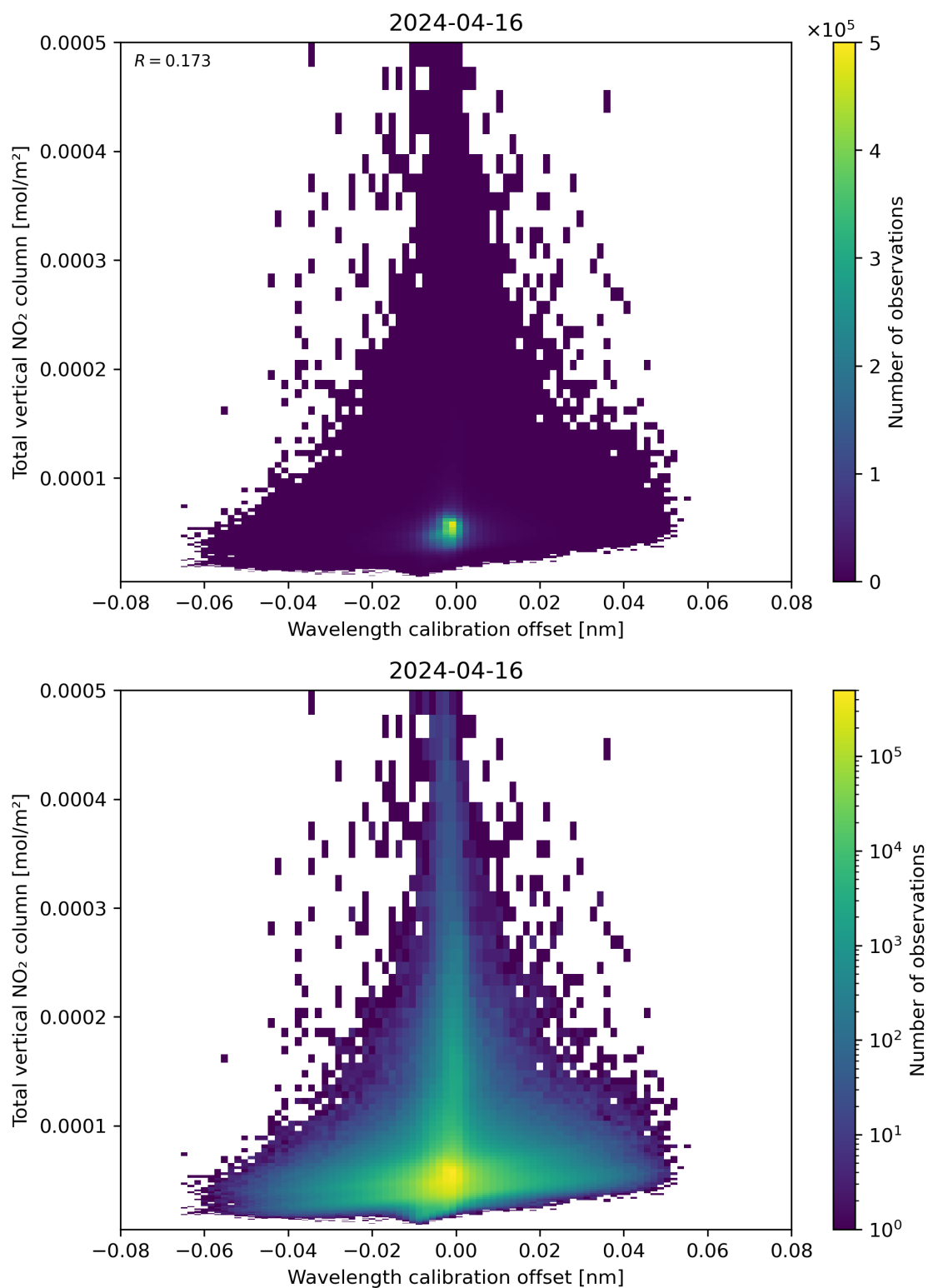
Figure 179: Scatter density plot of “Wavelength calibration offset” against “Total vertical NO 2 column” for 2024-04-16 to 2024-04-17.
