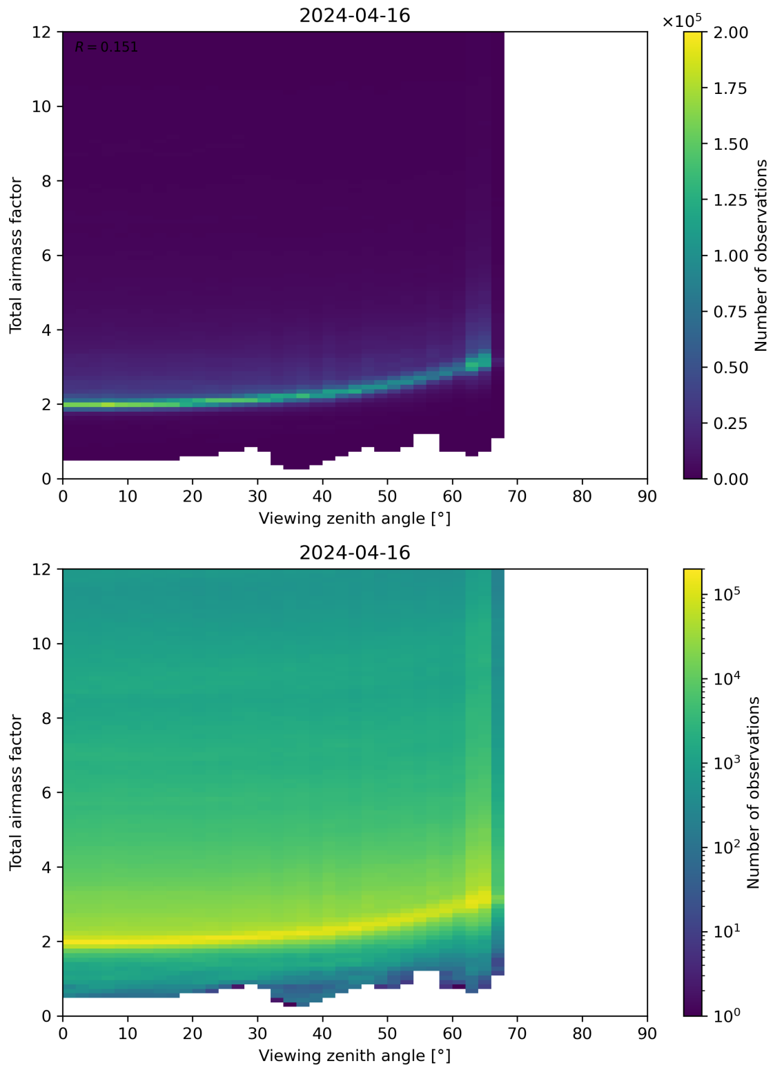
Figure 160: Scatter density plot of “Viewing zenith angle” against “Total airmass factor” for 2024-04-16 to 2024-04-17.
