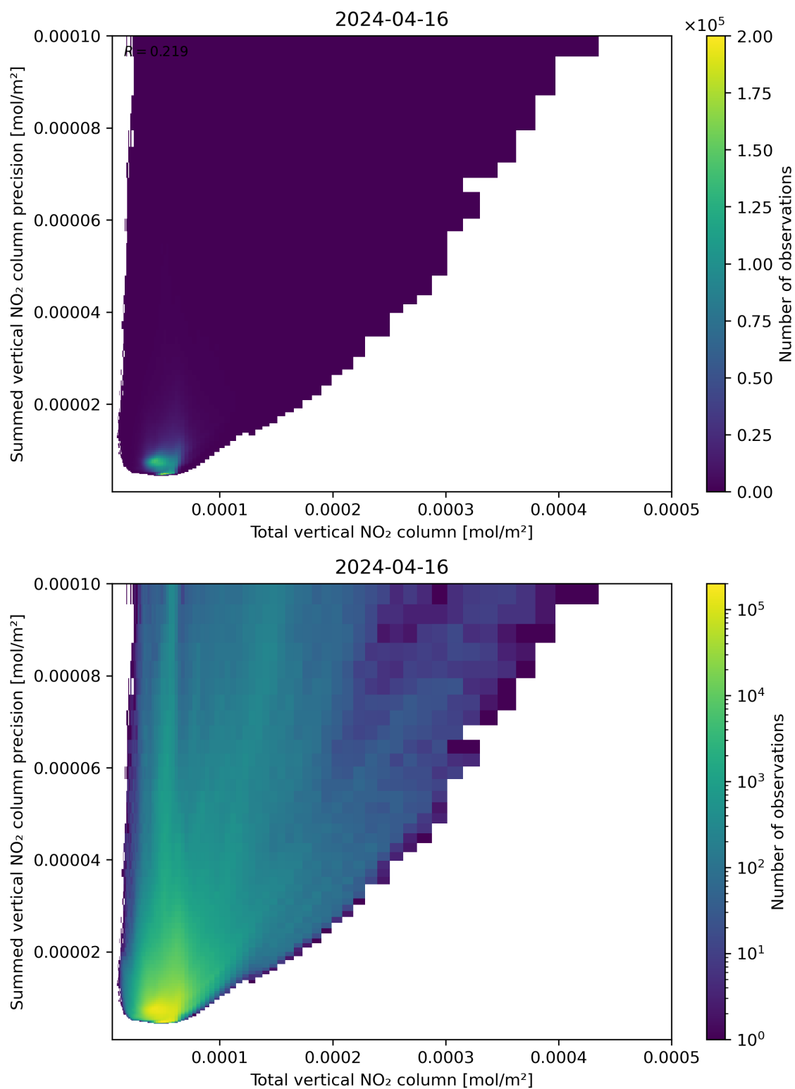
Figure 113: Scatter density plot of “Total vertical NO 2 column” against “Summed vertical NO 2 column precision” for 2024-04-16 to 2024-04-17.
