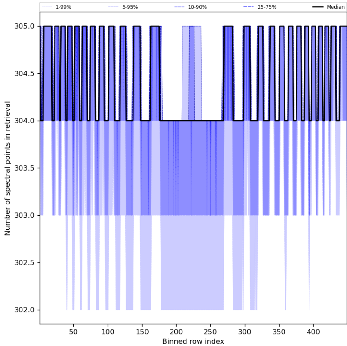
Figure 50: Along track statistics of “Number of spectral points in retrieval” for 2024-04-16 to 2024-04-17
