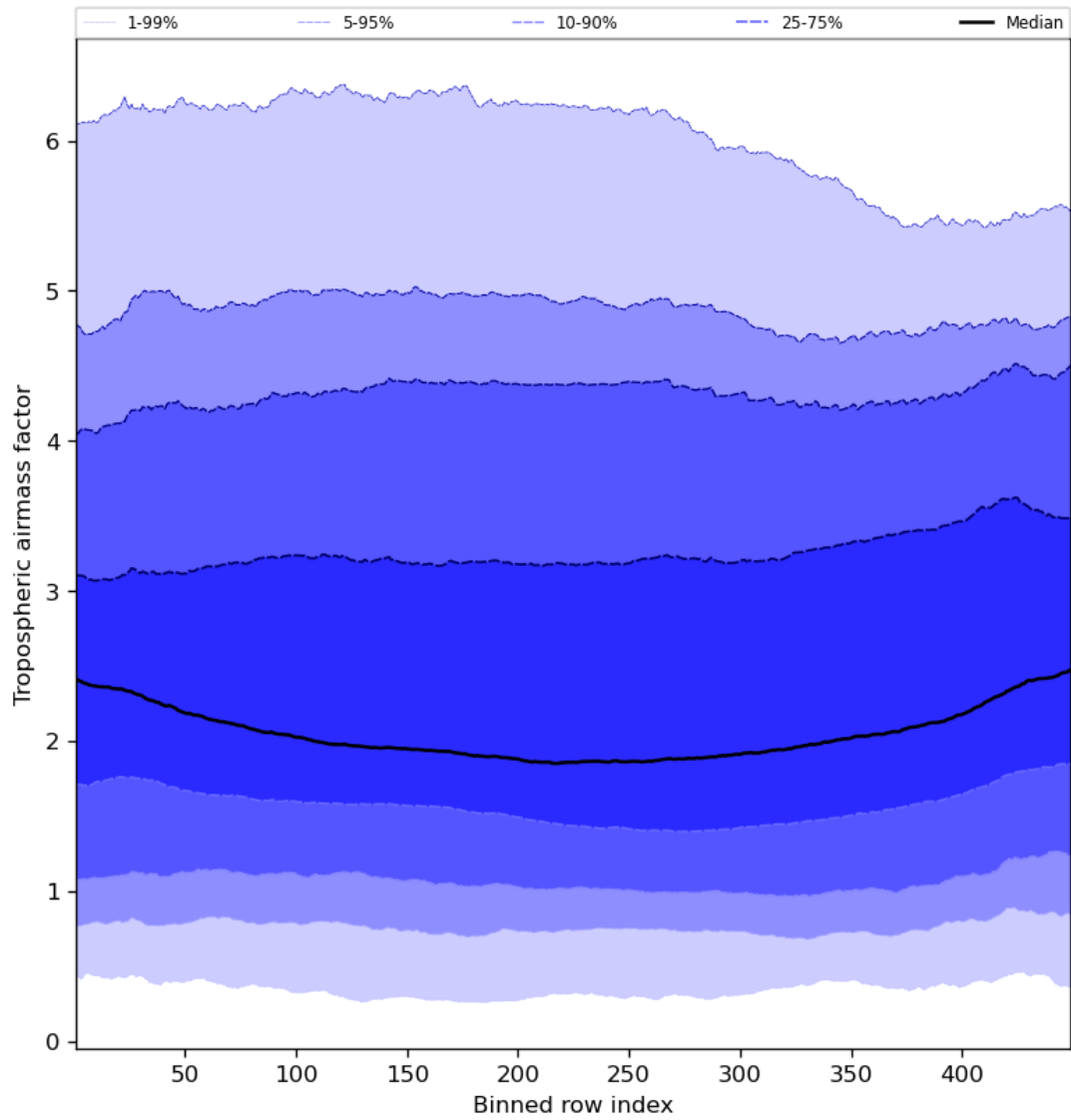
Figure 48: Along track statistics of “Tropospheric airmass factor” for 2024-04-16 to 2024-04-17
