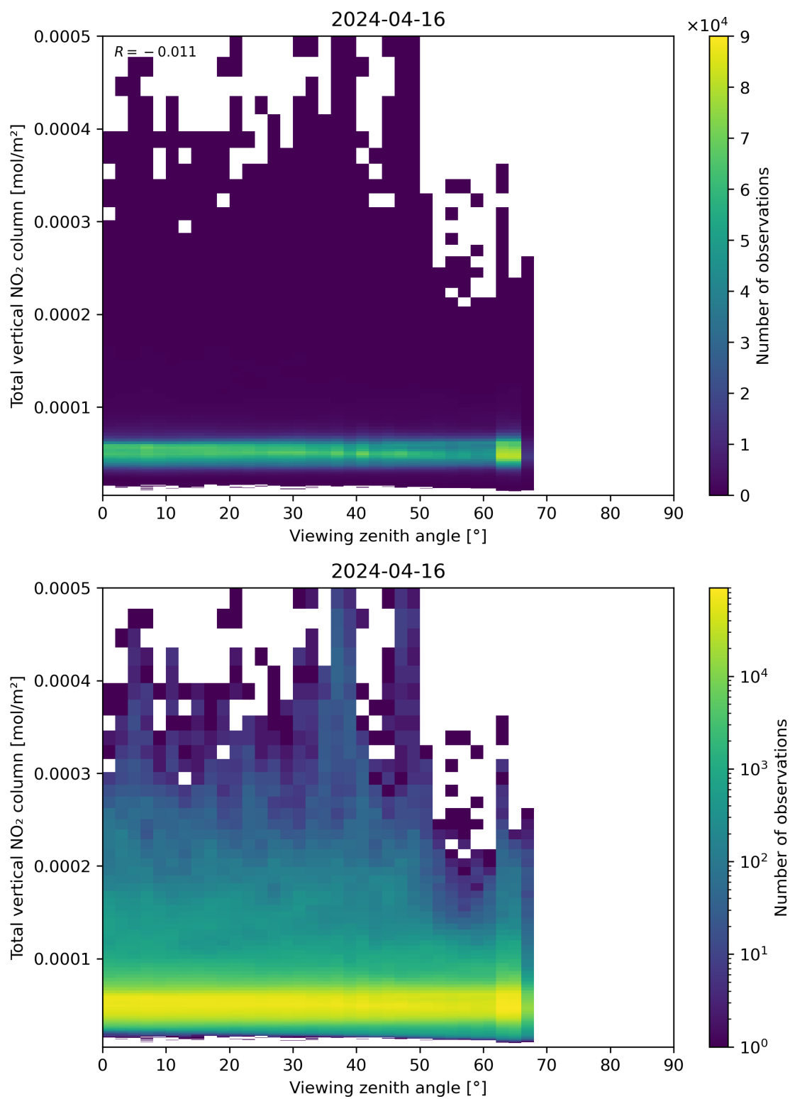
Figure 167: Scatter density plot of “Viewing zenith angle” against “Total vertical NO 2 column” for 2024-04-16 to 2024-04-17.
