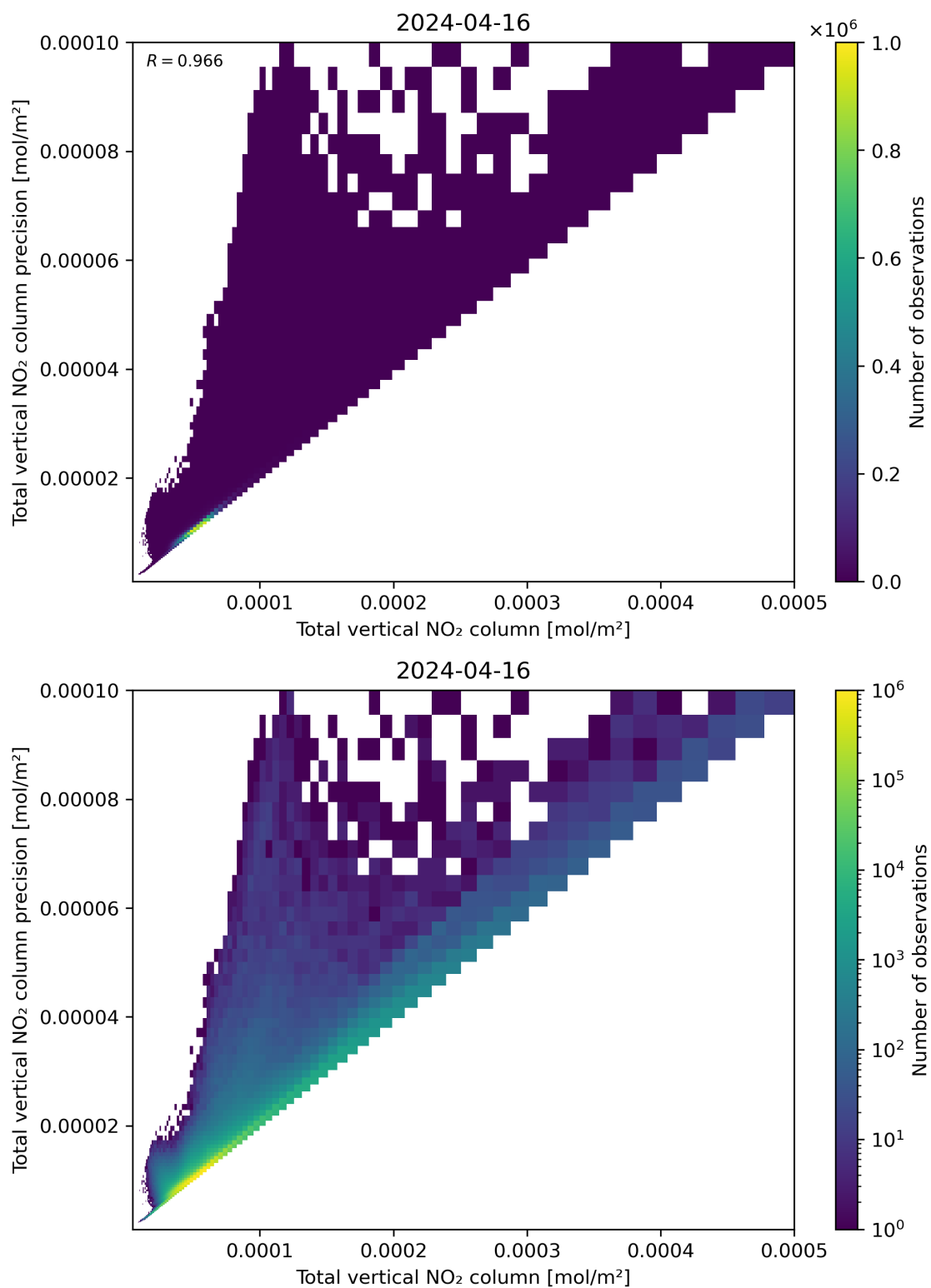
Figure 114: Scatter density plot of “Total vertical NO 2 column” against “Total vertical NO 2 column precision” for 2024-04-16 to 2024-04-17.
