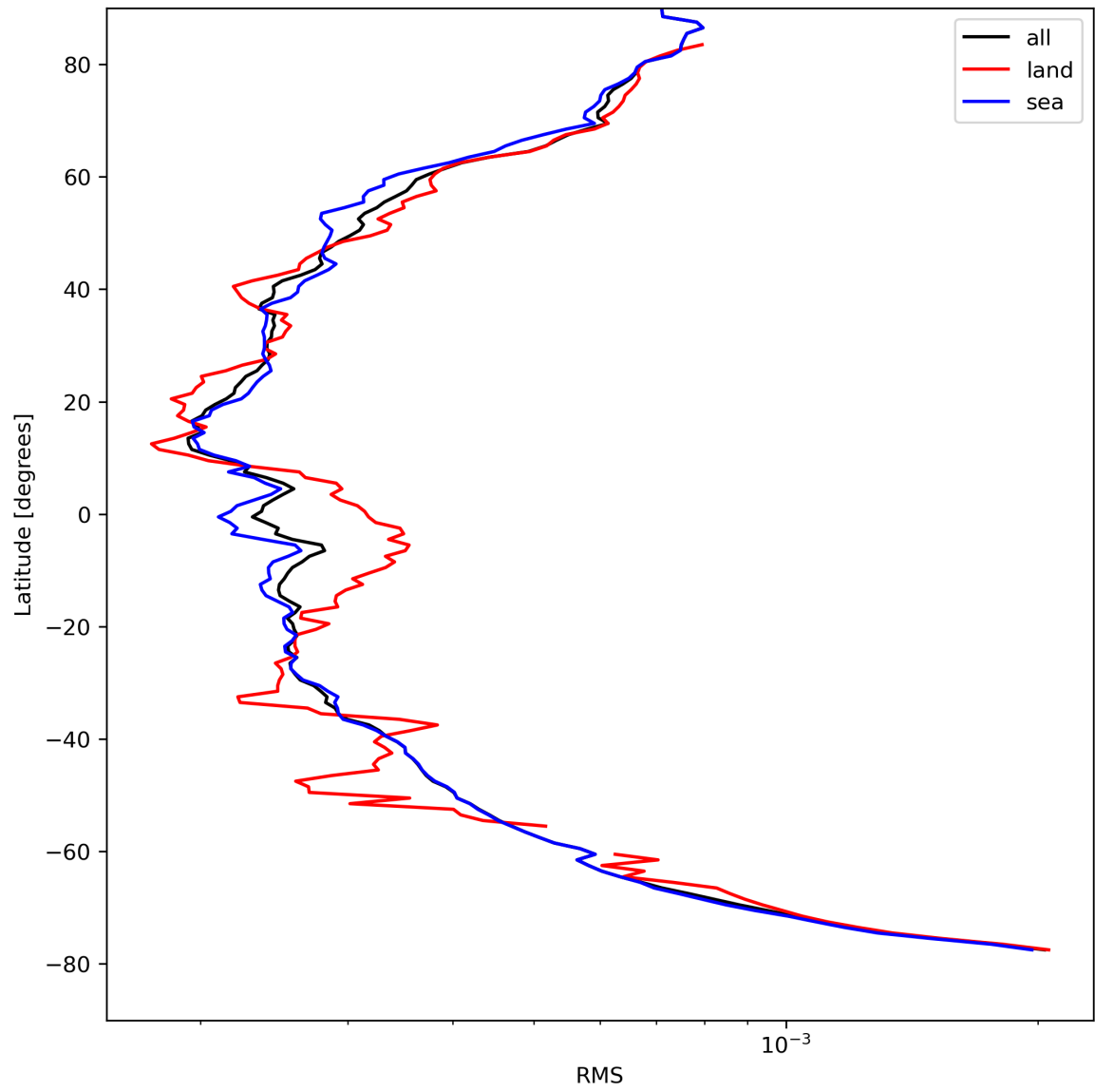
Figure 26: Zonal average of “RMS” for 2024-04-16 to 2024-04-17.
