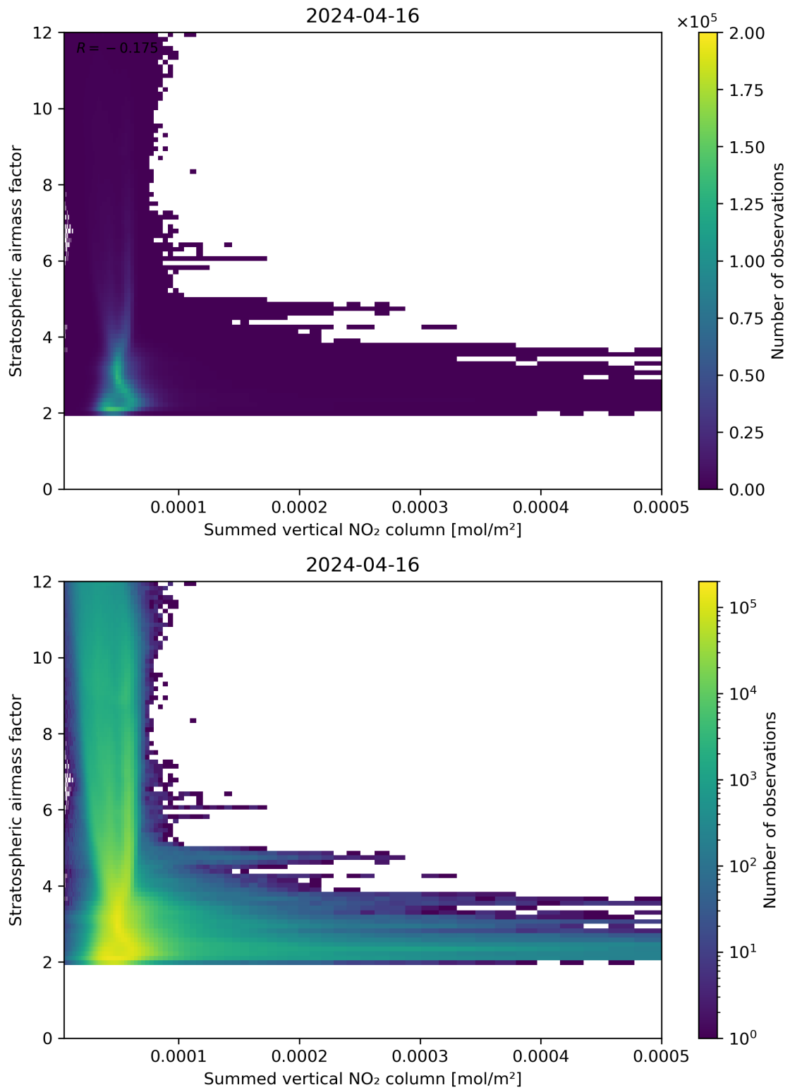
Figure 103: Scatter density plot of “Summed vertical NO 2 column” against “Stratospheric air mass factor” for 2024-04-16 to 2024-04-17.
