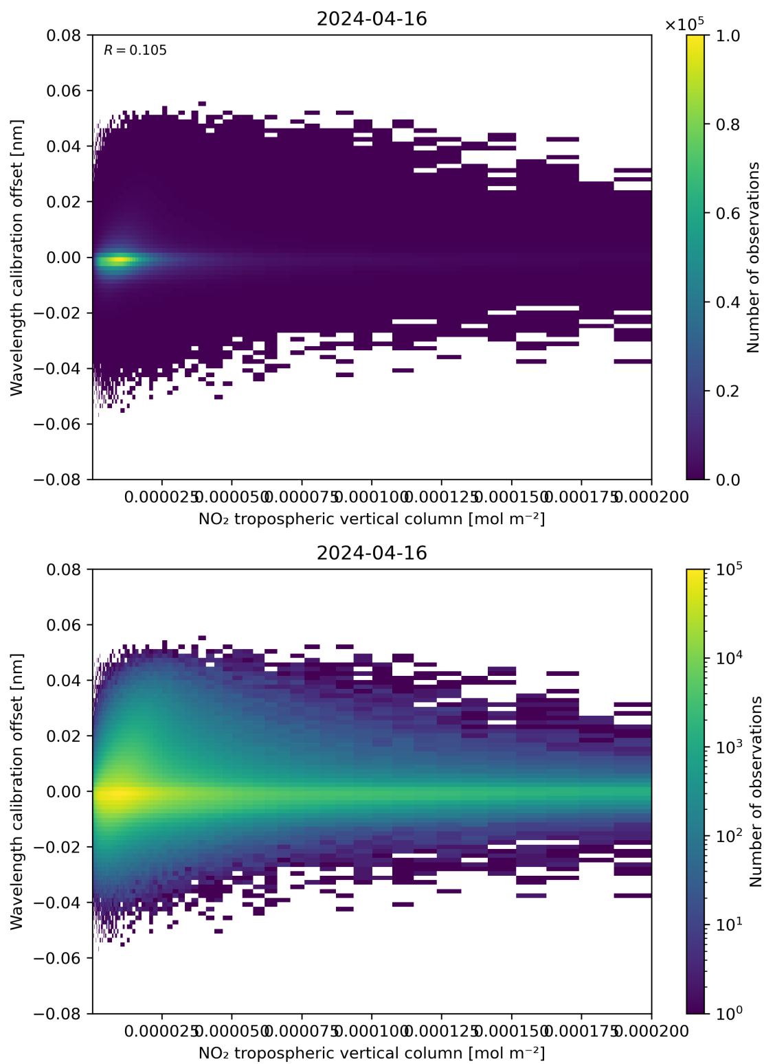
Figure 143: Scatter density plot of “NO 2 tropospheric vertical column” against “Wavelength calibration offset” for 2024-04-16 to 2024-04-17.
