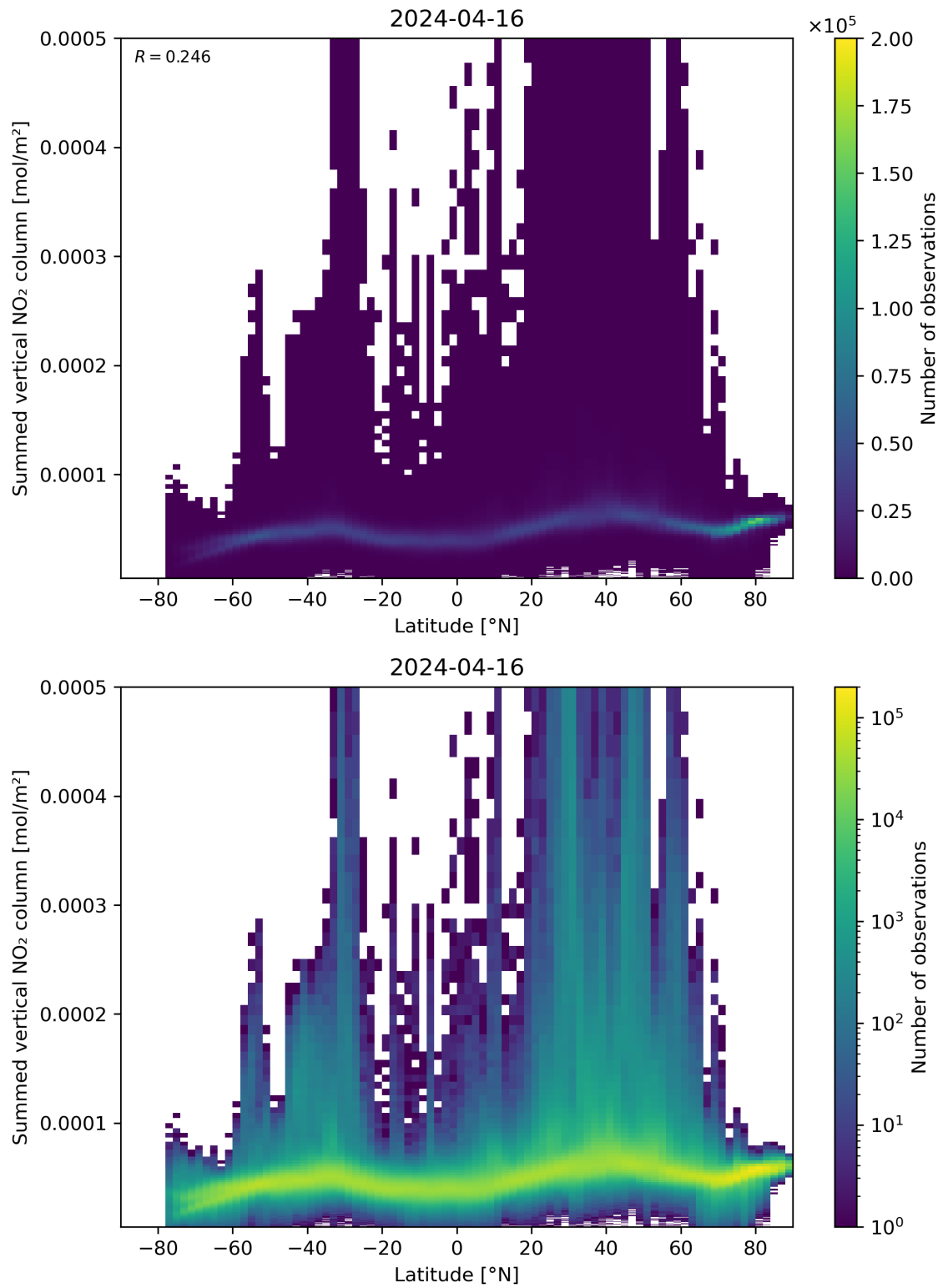
Figure 88: Scatter density plot of “Latitude” against “Summed vertical NO 2 column” for 2024-04-16 to 2024-04-17.
