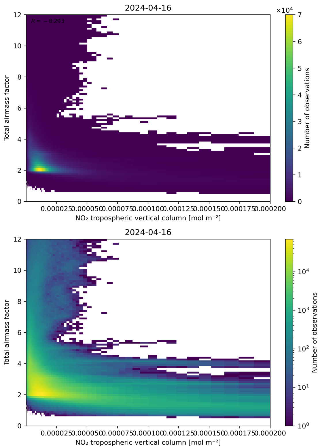
Figure 122: Scatter density plot of “NO 2 tropospheric vertical column” against “Total air mass factor” for 2024-04-16 to 2024-04-17.
