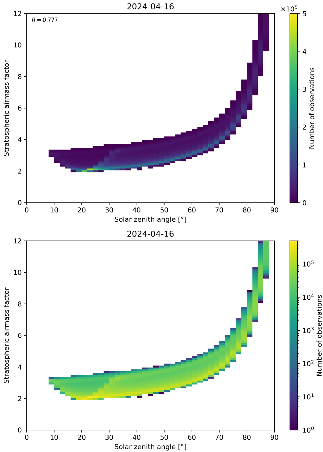
Figure 145: Scatter density plot of “Solar zenith angle” against “Stratospheric airmass factor” for 2024-04-16 to 2024-04-17.
