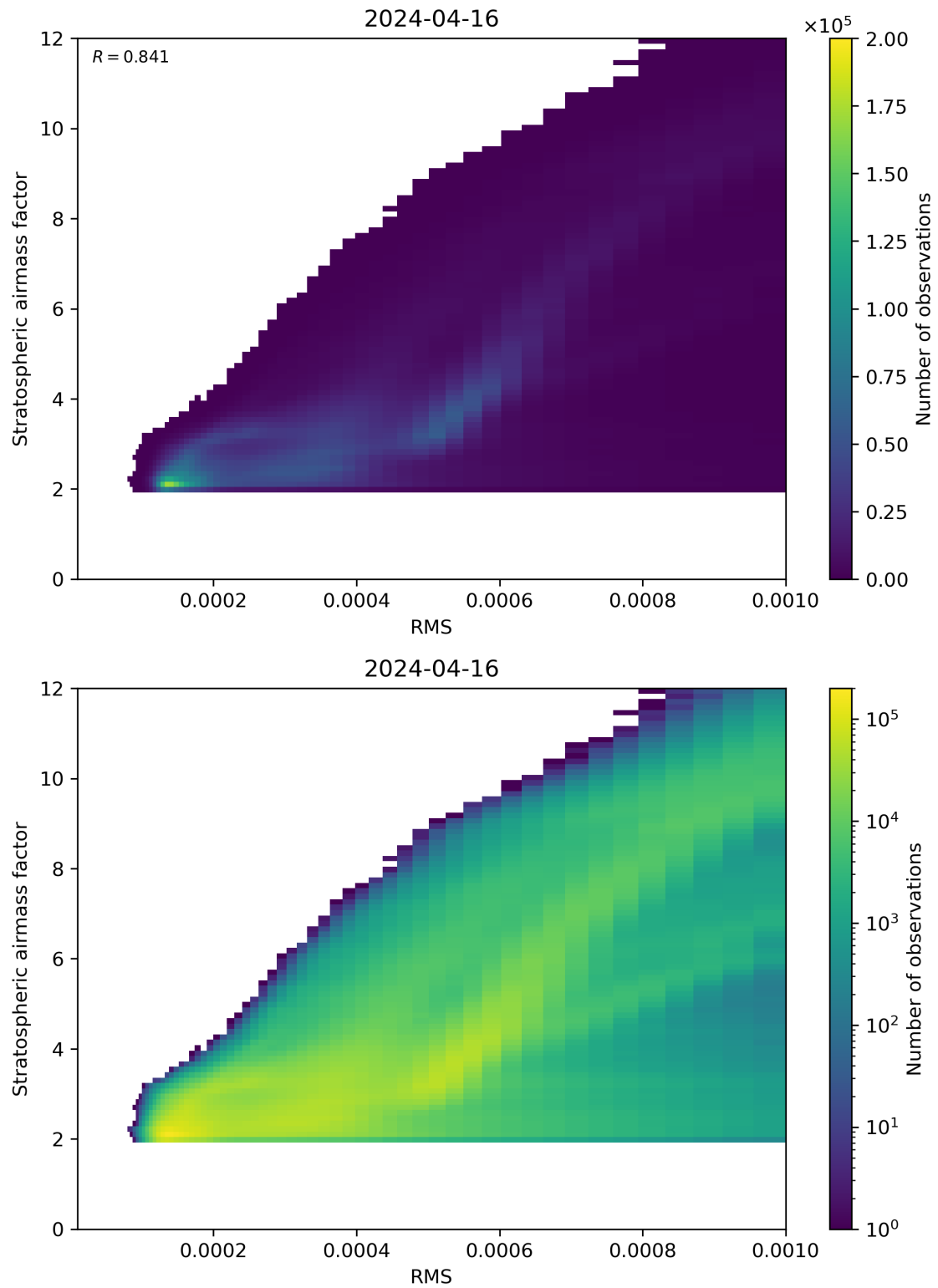
Figure 144: Scatter density plot of “RMS” against “Stratospheric airmass factor” for 2024-04-16 to 2024-04-17.
