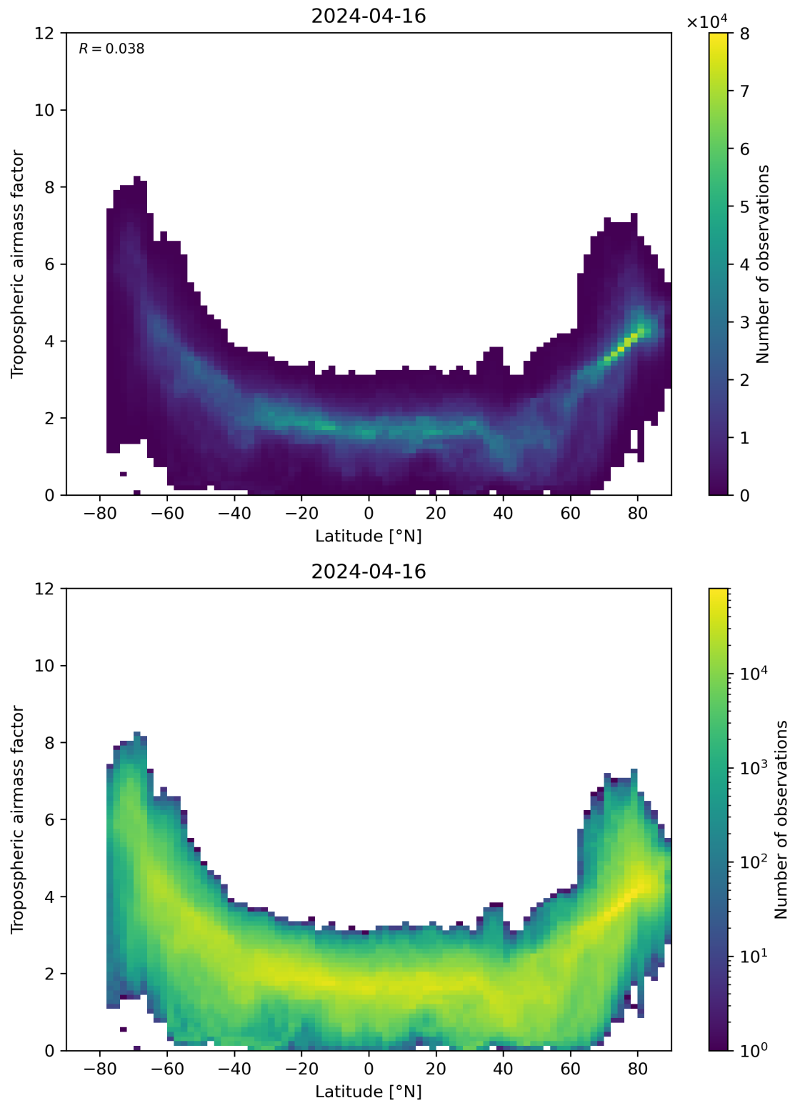
Figure 85: Scatter density plot of “Latitude” against “Tropospheric air mass factor” for 2024-04-16 to 2024-04-17.
