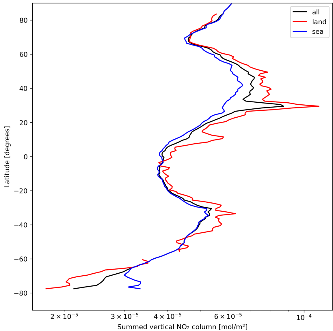
Figure 23: Zonal average of “Summed vertical NO 2 column” for 2024-04-16 to 2024-04-17.
