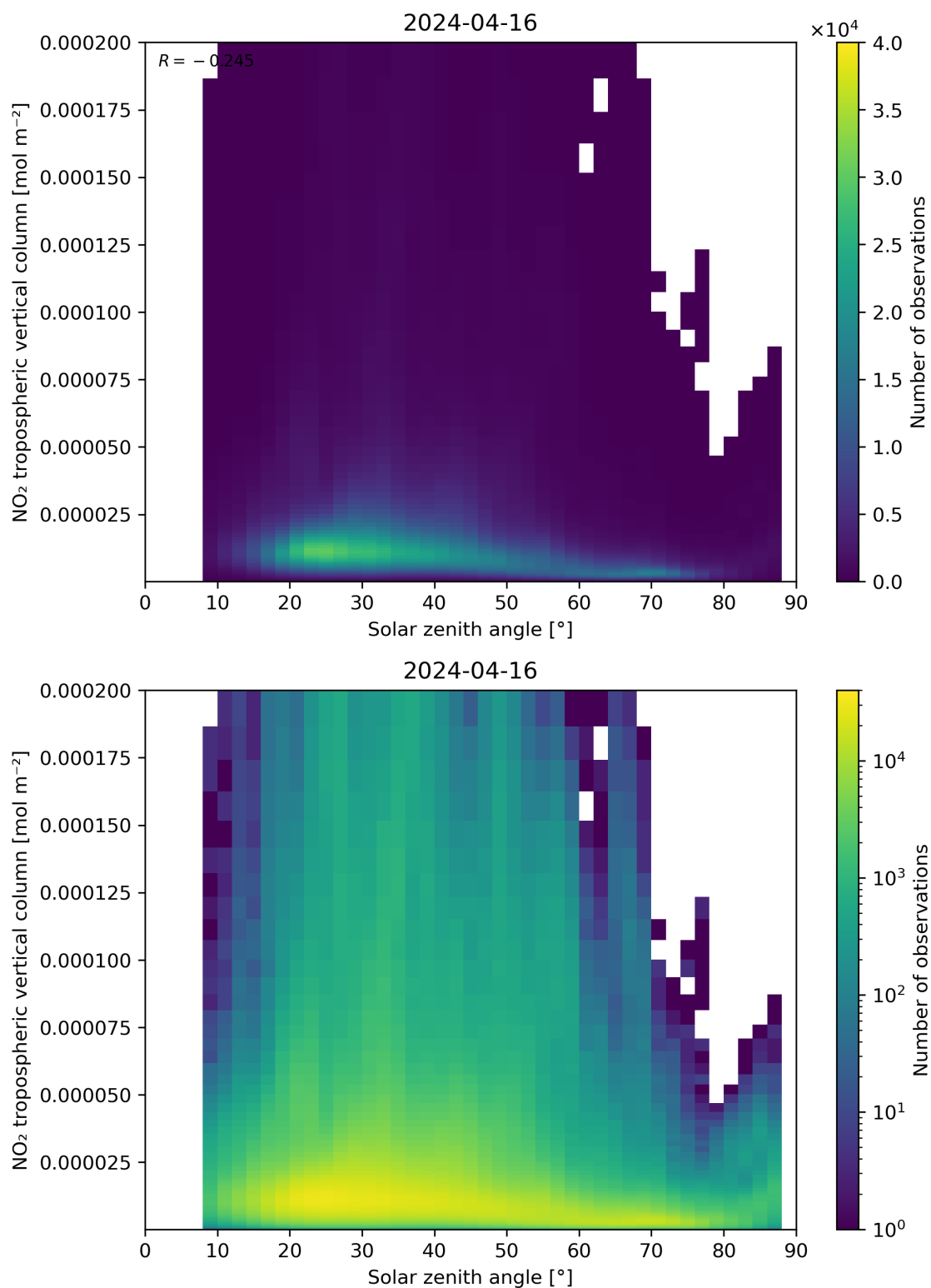
Figure 155: Scatter density plot of “Solar zenith angle” against “NO 2 tropospheric vertical column” for 2024-04-16 to 2024-04-17.
