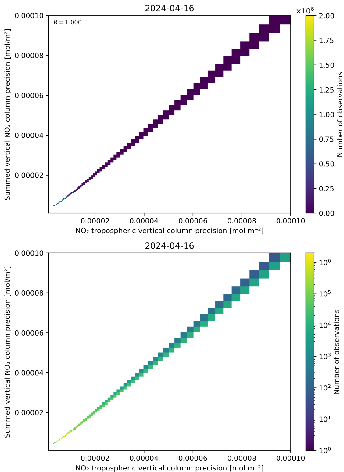
Figure 137: Scatter density plot of “NO 2 tropospheric vertical column precision” against “Summed vertical NO 2 column precision” for 2024-04-16 to 2024-04-17.
