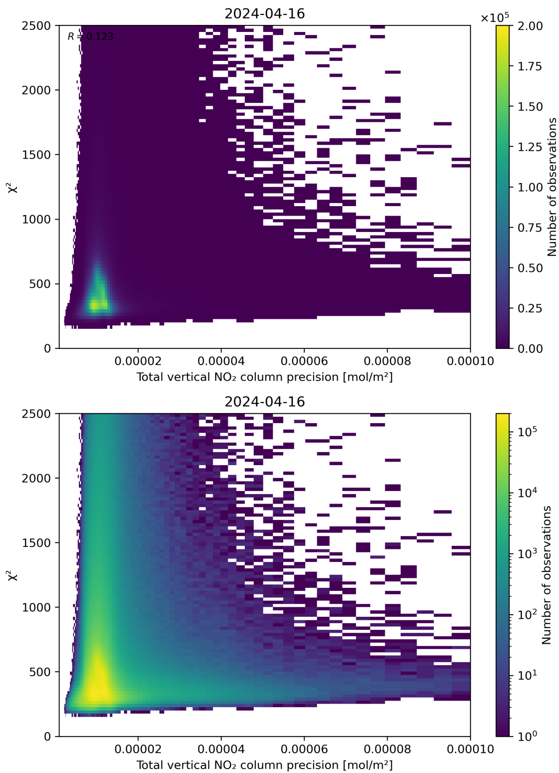
Figure 116: Scatter density plot of “Total vertical NO 2 column precision” against “ \chi^2 ” for 2024-04-16 to 2024-04-17.
