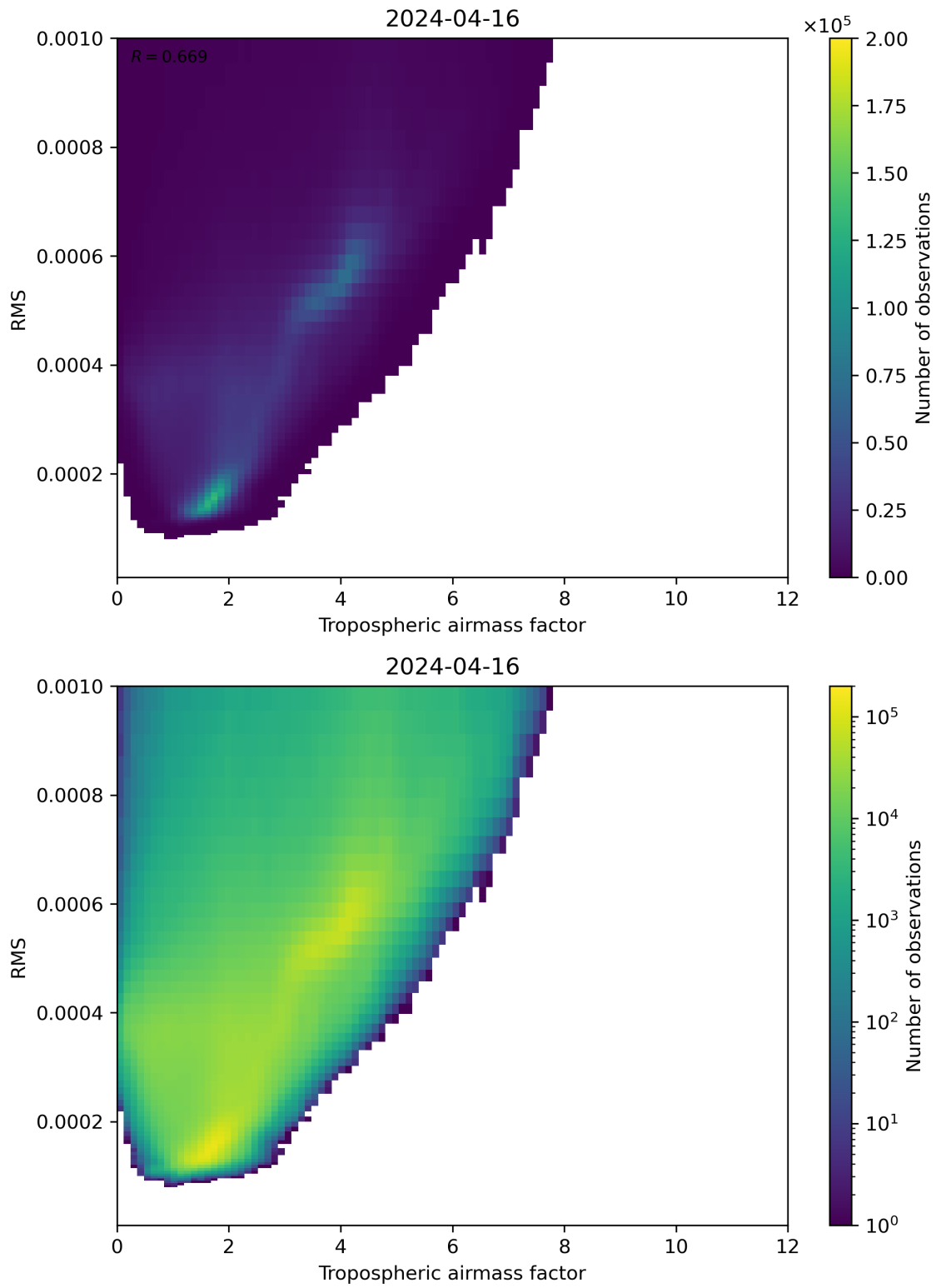
Figure 79: Scatter density plot of “Tropospheric airmass factor” against “RMS” for 2024-04-16 to 2024-04-17.
