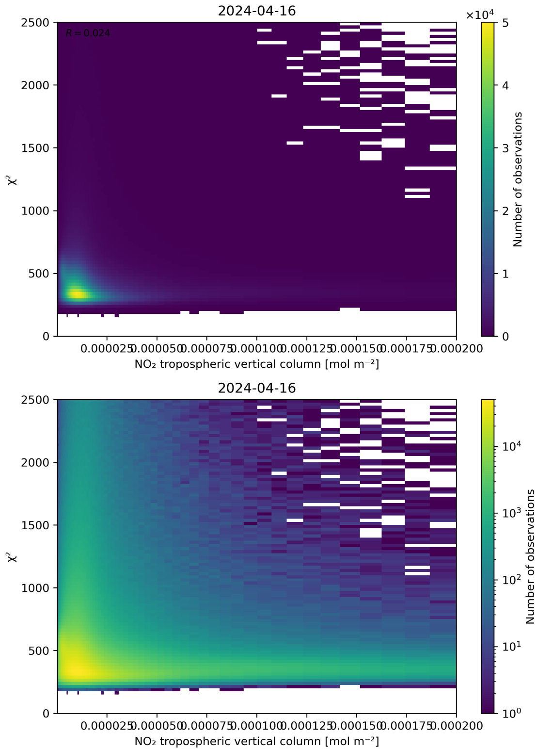
Figure 124: Scatter density plot of “NO 2 tropospheric vertical column” against “ \chi^2 ” for 2024-04-16 to 2024-04-17.
