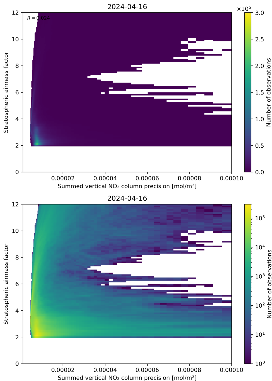
Figure 106: Scatter density plot of “Summed vertical NO 2 column precision” against “Stratospheric airmass factor” for 2024-04-16 to 2024-04-17.
