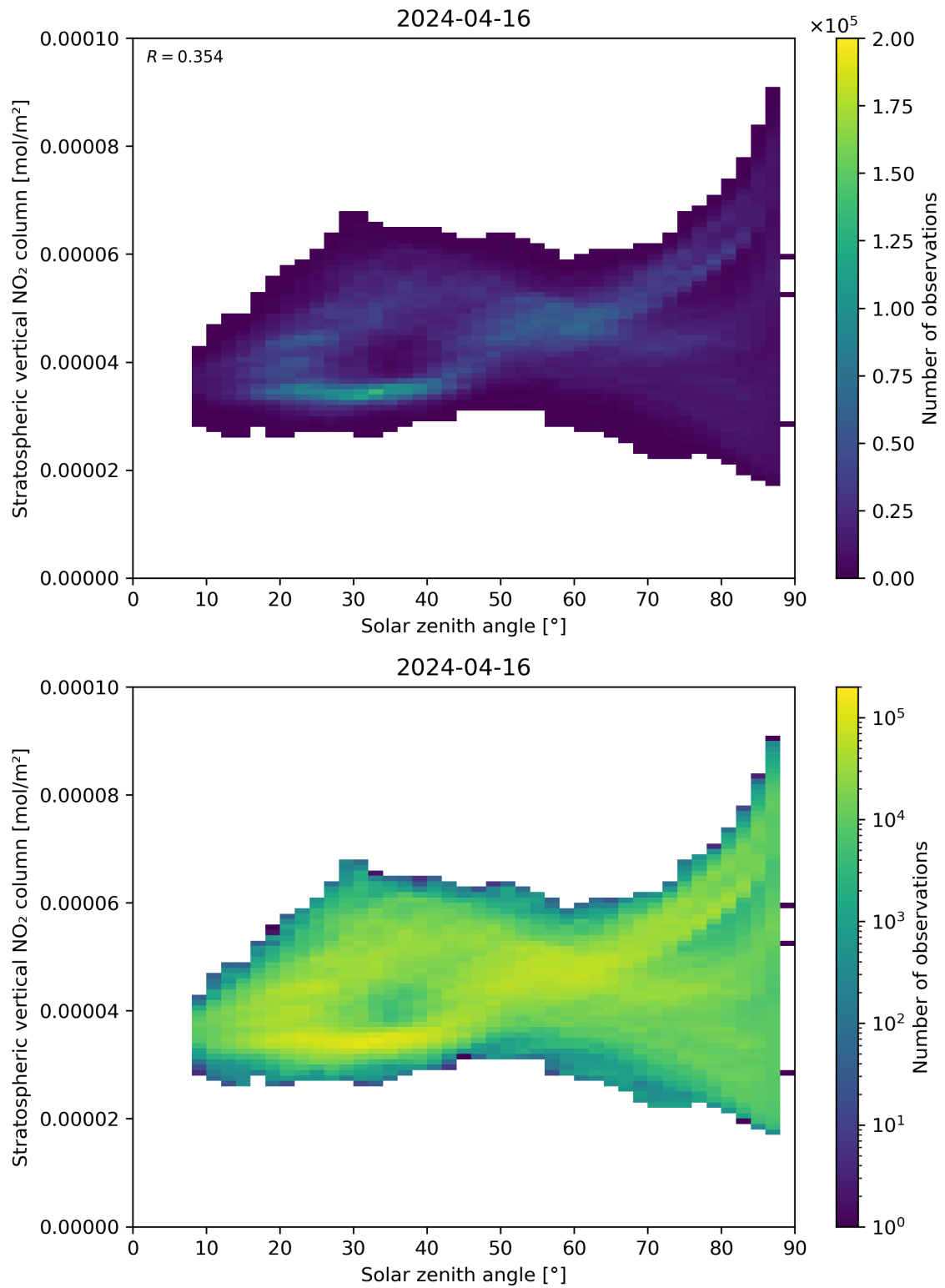
Figure 150: Scatter density plot of “Solar zenith angle” against “Stratospheric vertical \text{NO}_2 column” for 2024-04-16 to 2024-04-17.
