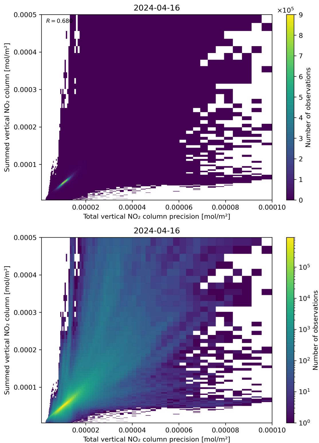
Figure 117: Scatter density plot of “Total vertical NO 2 column precision” against “Summed vertical NO 2 column” for 2024-04-16 to 2024-04-17.
