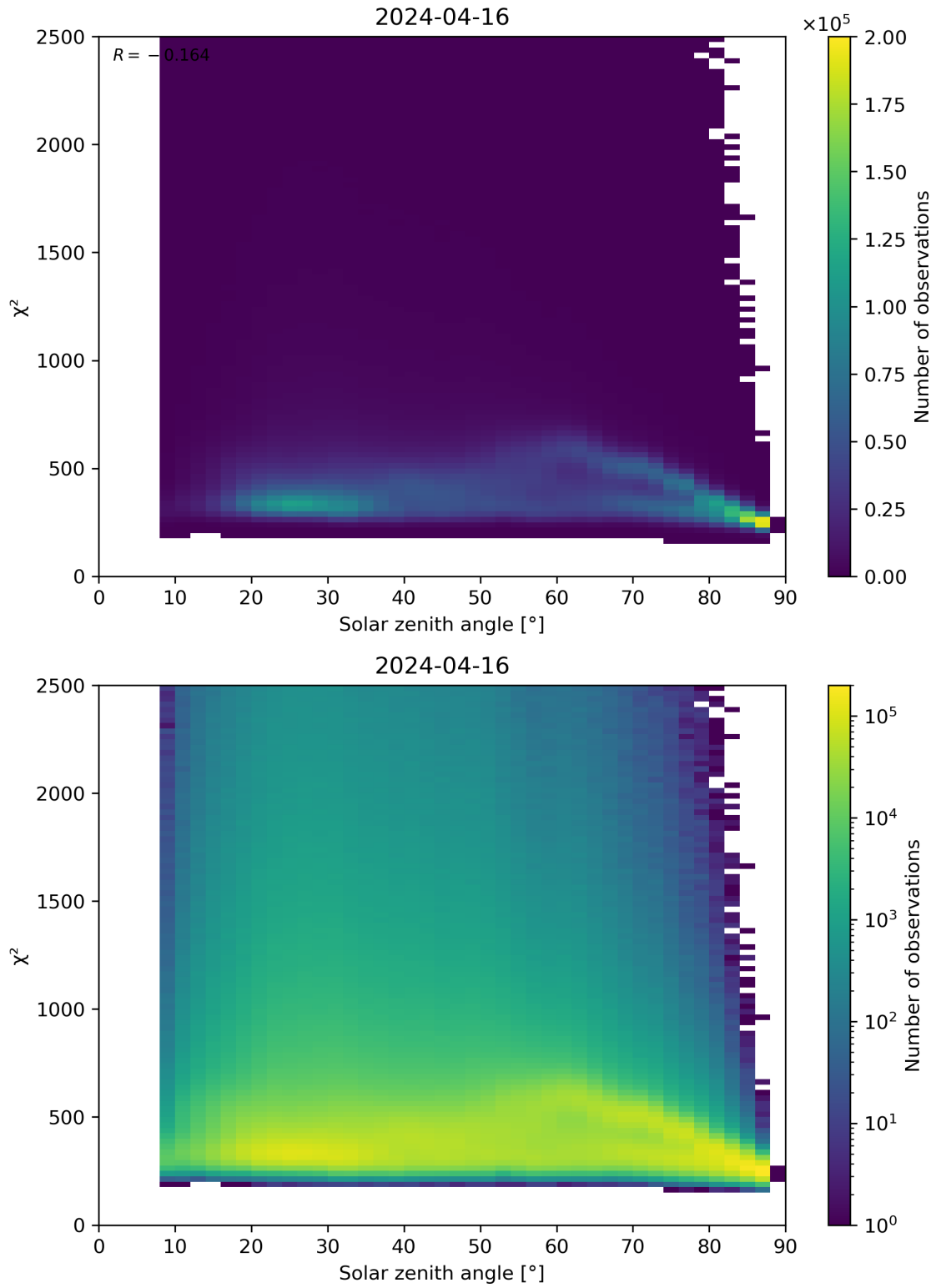
Figure 148: Scatter density plot of “Solar zenith angle” against “ \chi^2 ” for 2024-04-16 to 2024-04-17.
