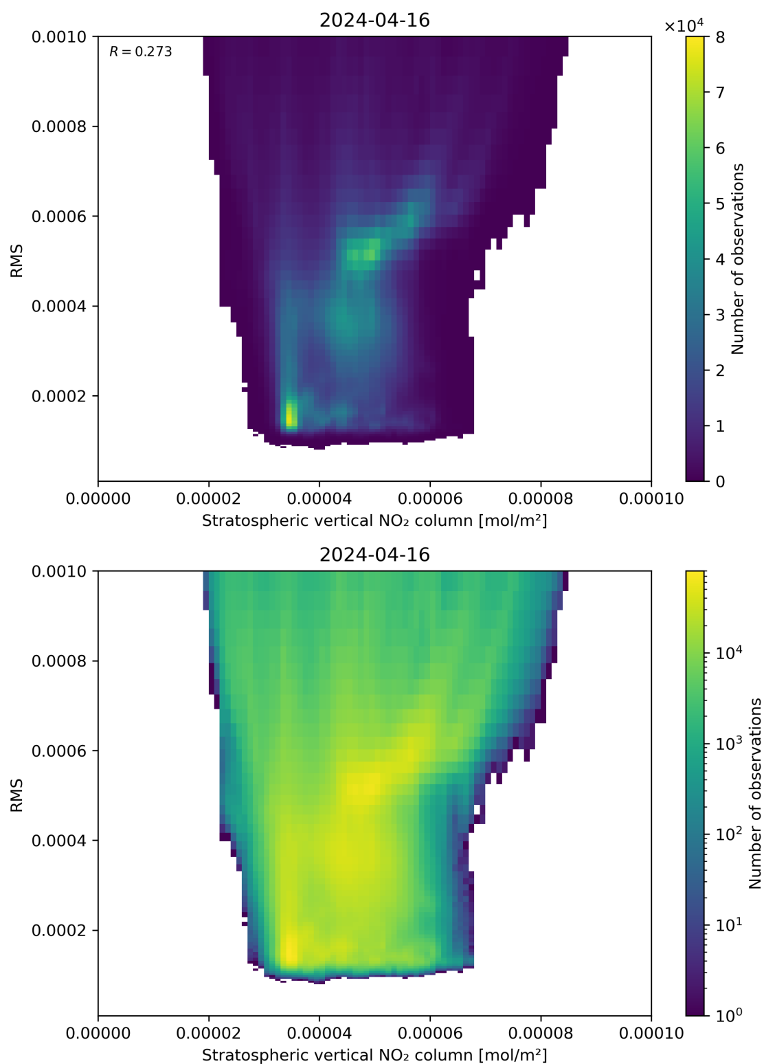
Figure 102: Scatter density plot of “Stratospheric vertical NO 2 column” against “RMS” for 2024-04-16 to 2024-04-17.
