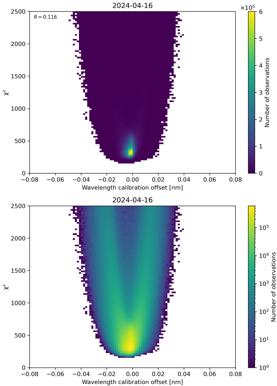
Figure 175: Scatter density plot of “Wavelength calibration offset” against “ \chi^2 ” for 2024-04-16 to 2024-04-17.
