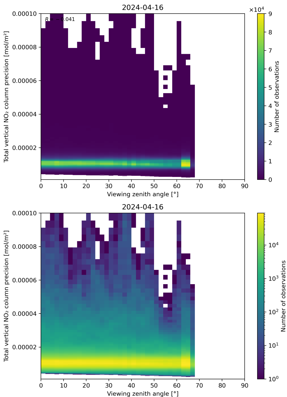
Figure 168: Scatter density plot of “Viewing zenith angle” against “Total vertical NO 2 column precision” for 2024-04-16 to 2024-04-17.
