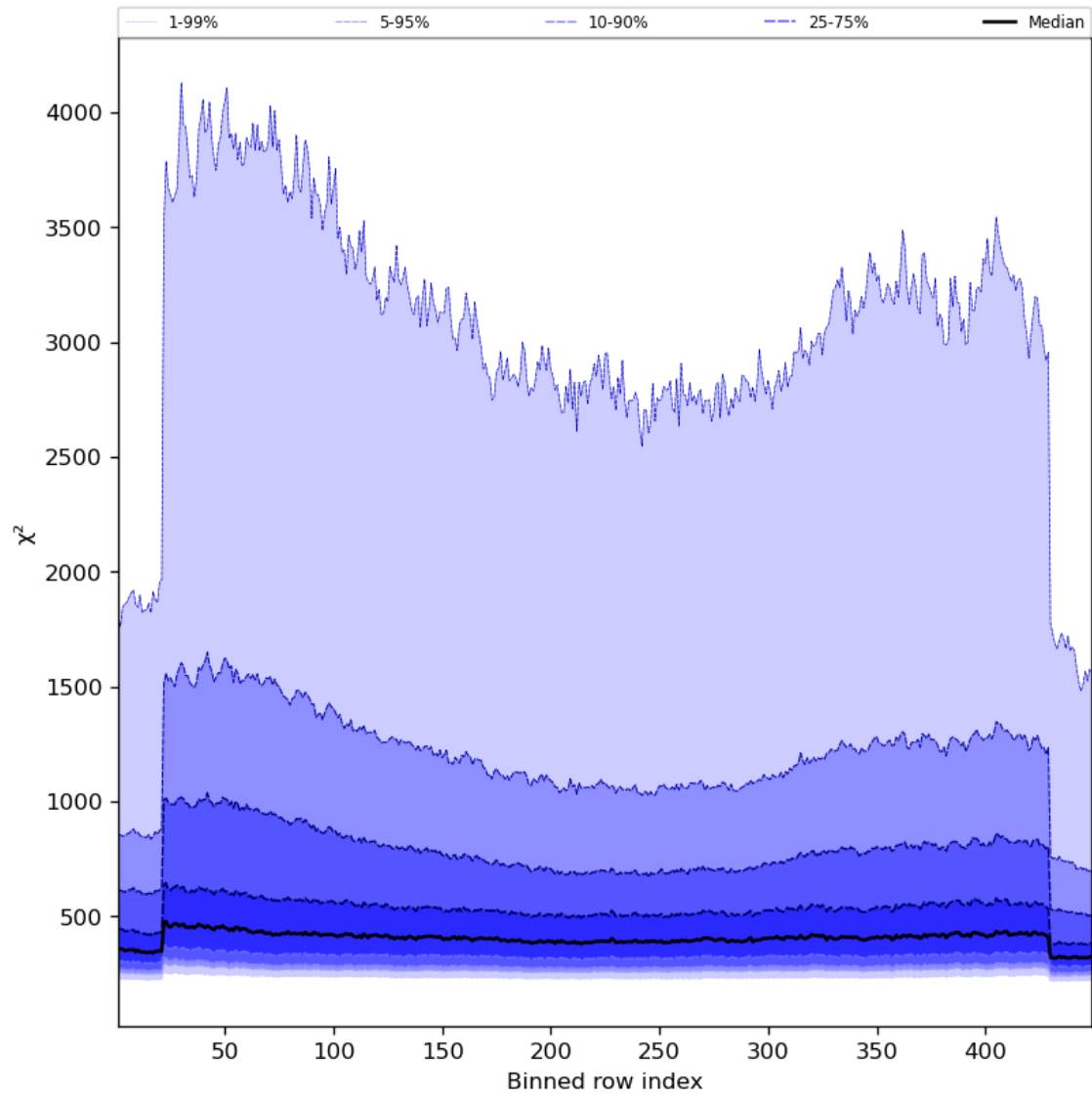
Figure 59: Along track statistics of “ \chi^2 ” for 2024-04-16 to 2024-04-17
