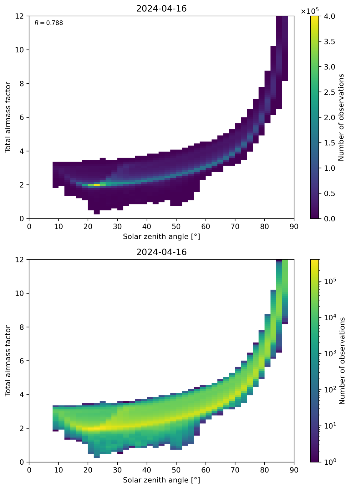
Figure 146: Scatter density plot of “Solar zenith angle” against “Total airmass factor” for 2024-04-16 to 2024-04-17.
