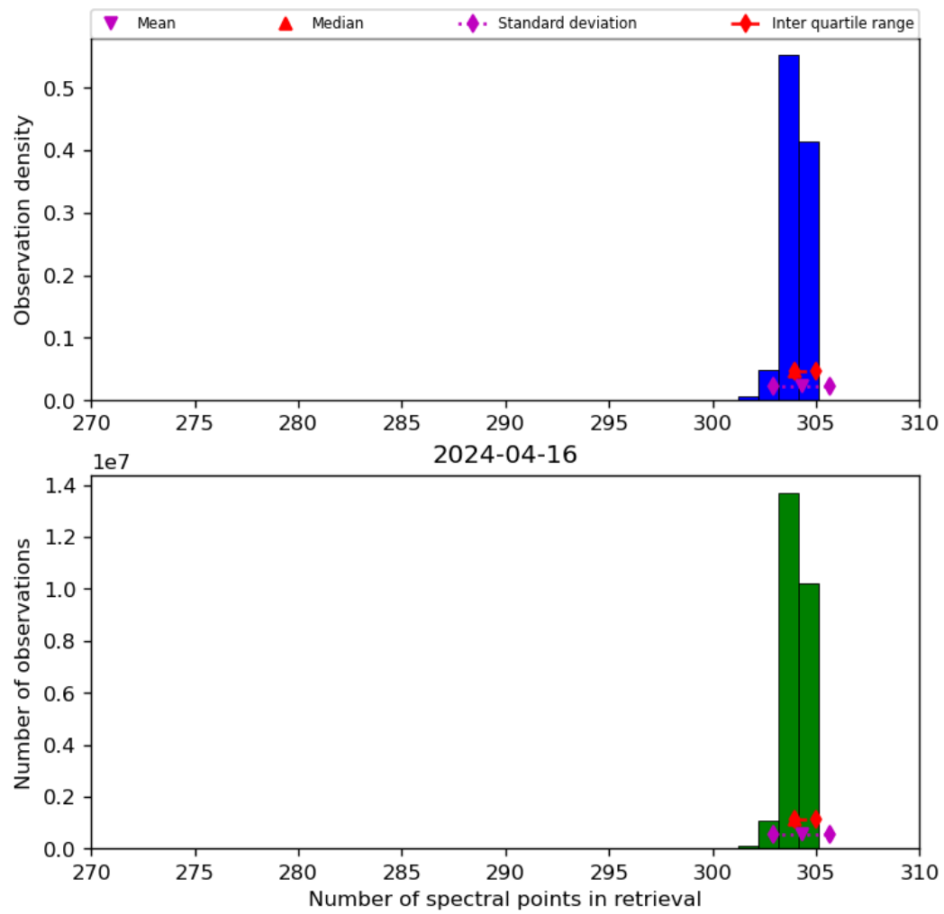
Figure 33: Histogram of “Number of spectral points in retrieval” for 2024-04-16 to 2024-04-17
