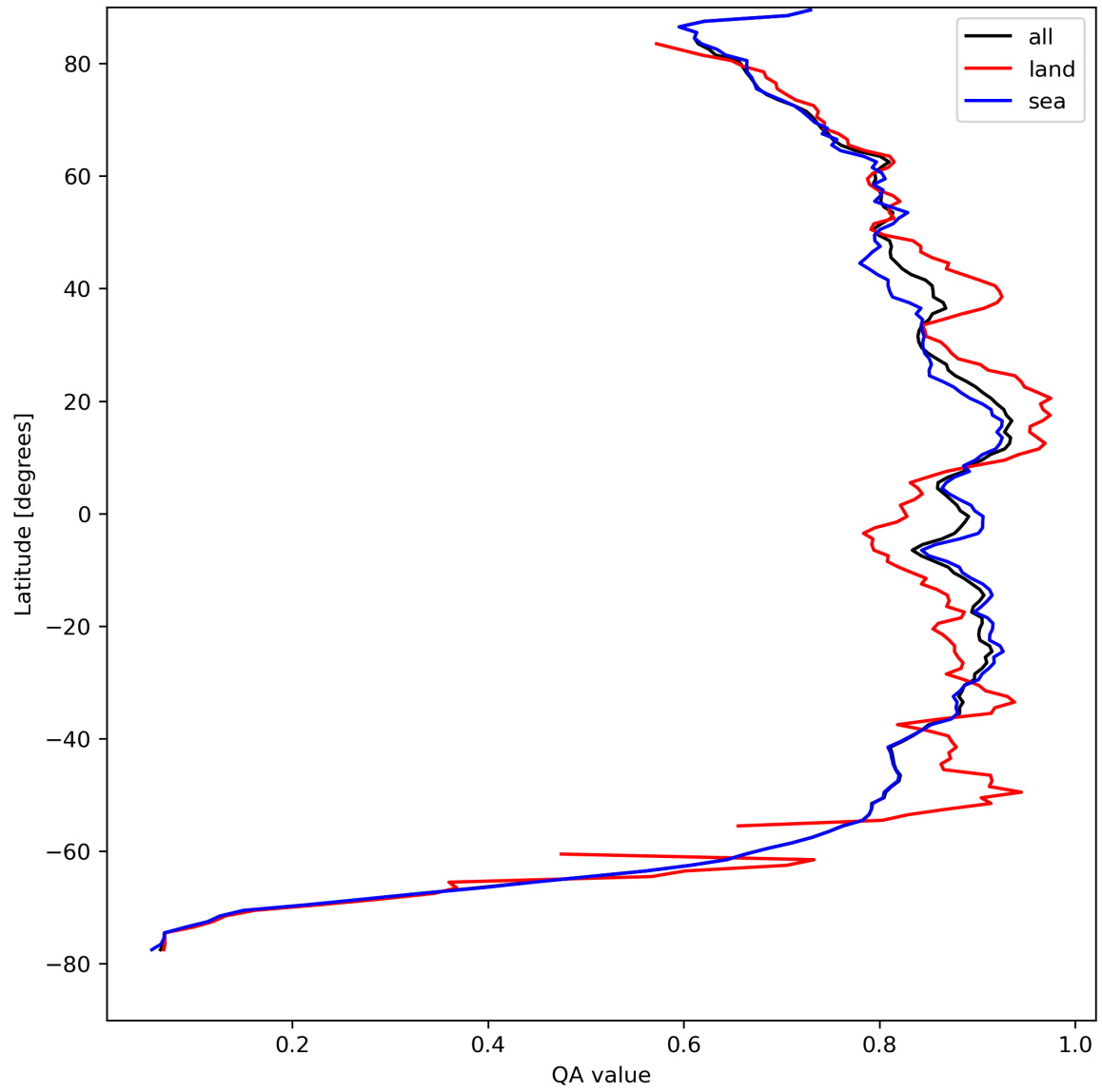
Figure 11: Zonal average of “QA value” for 2024-04-16 to 2024-04-17.
