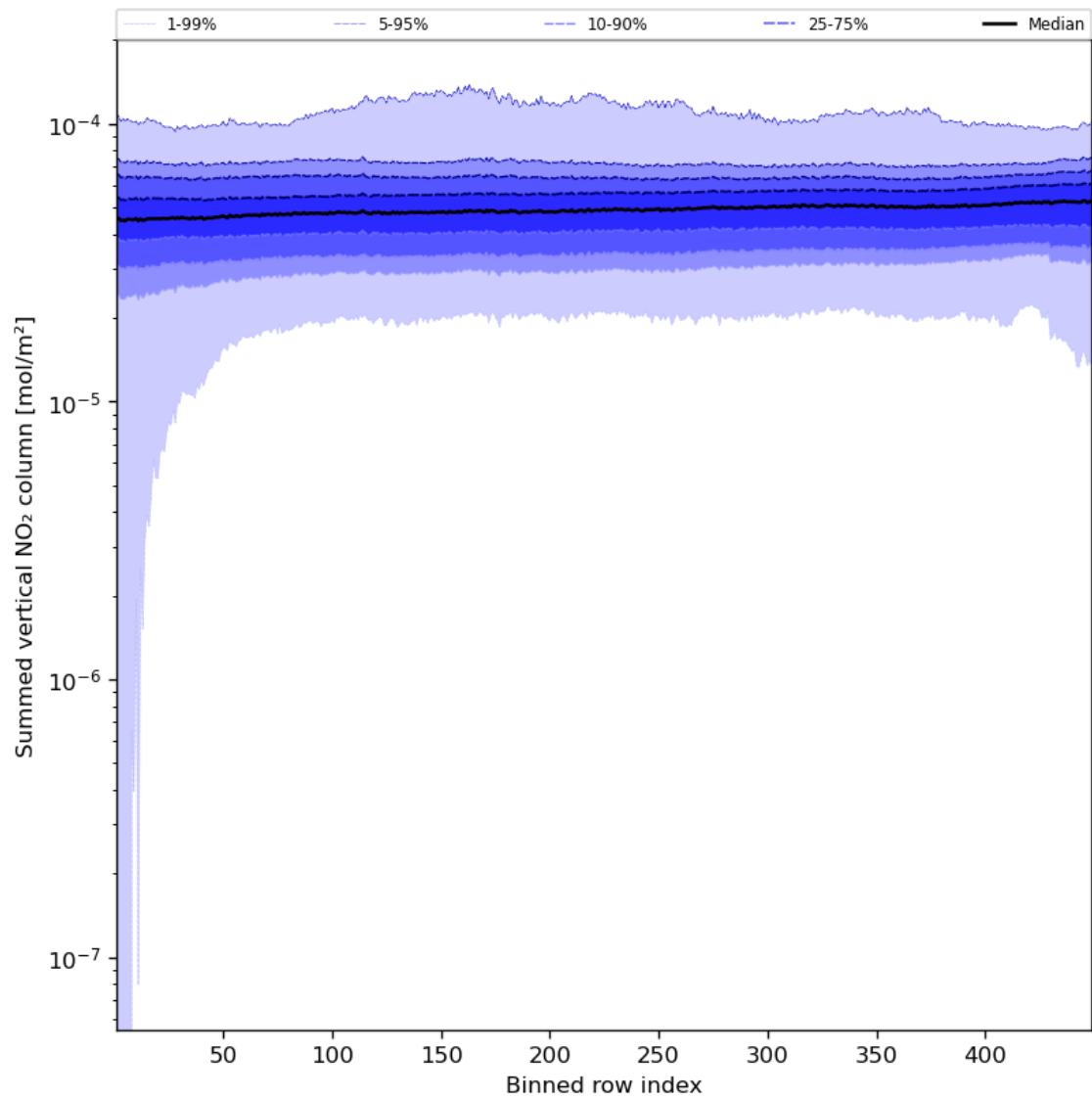
Figure 57: Along track statistics of “Summed vertical NO 2 column” for 2024-04-16 to 2024-04-17
