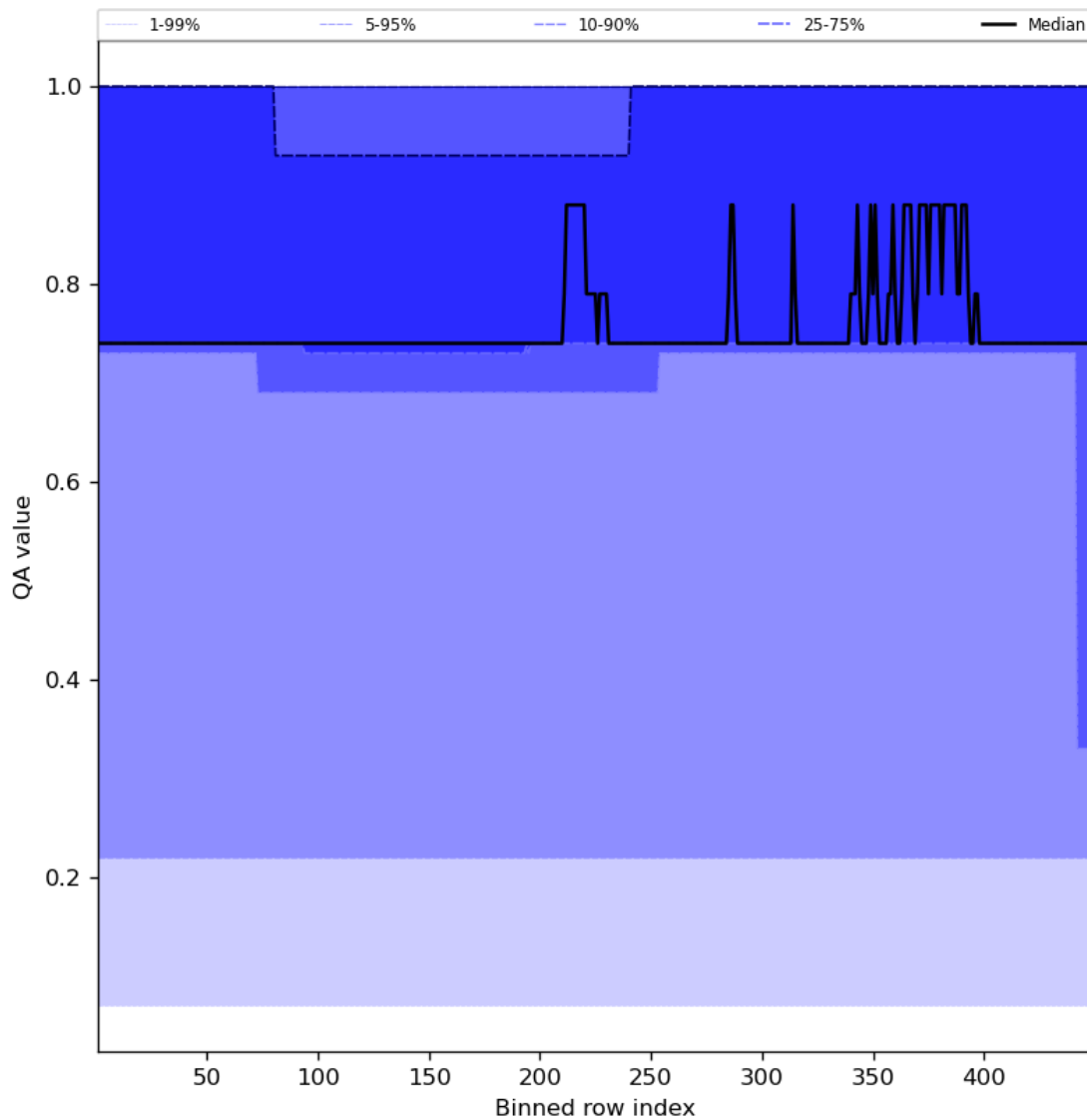
Figure 45: Along track statistics of “QA value” for 2024-04-16 to 2024-04-17
