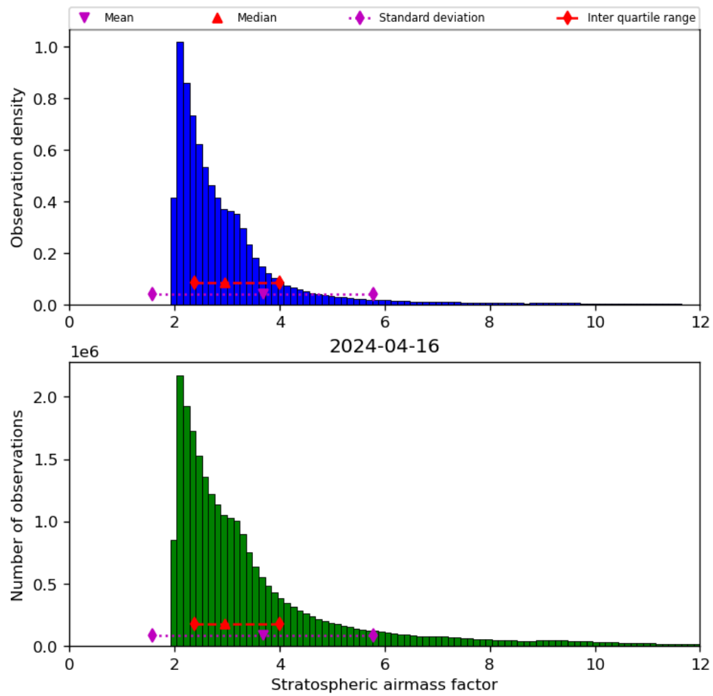
Figure 44: Histogram of “Stratospheric airmass factor” for 2024-04-16 to 2024-04-17
