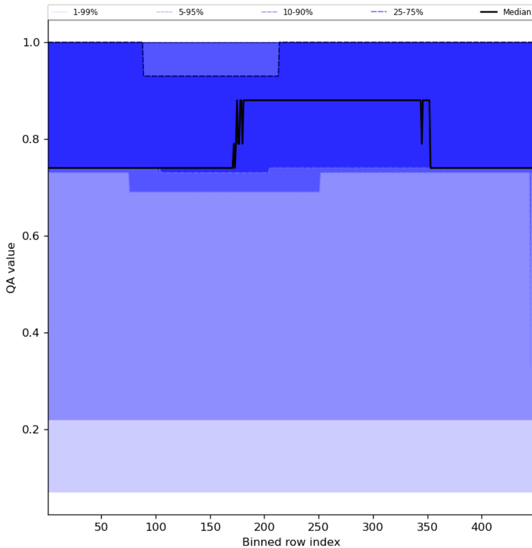
Figure 45: Along track statistics of “QA value” for 2024-04-23 to 2024-04-25
