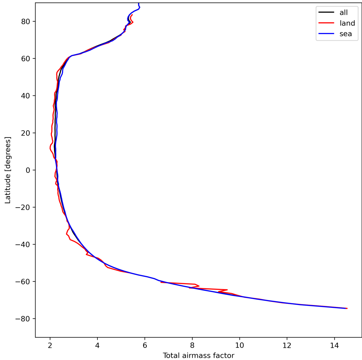
Figure 15: Zonal average of “Total airmass factor” for 2024-04-23 to 2024-04-25.
