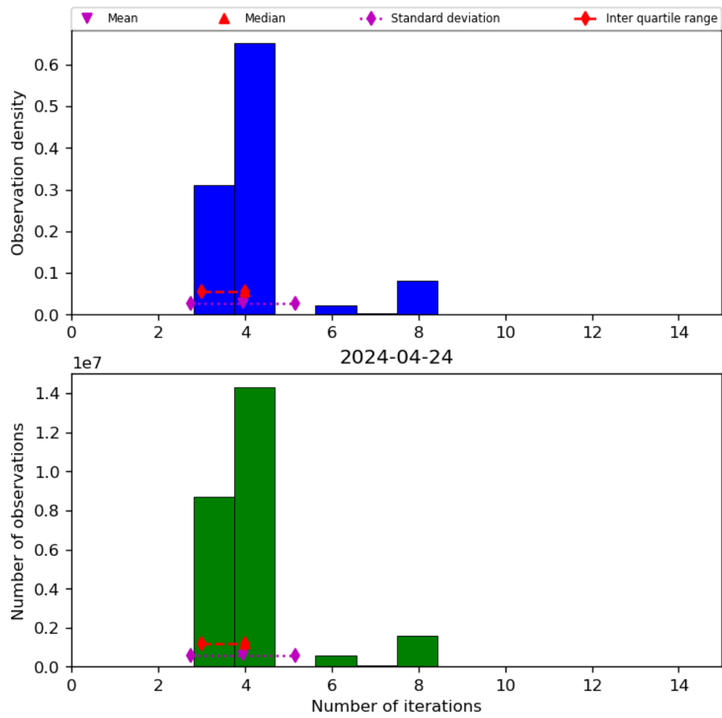
Figure 34: Histogram of “Number of iterations” for 2024-04-23 to 2024-04-25
