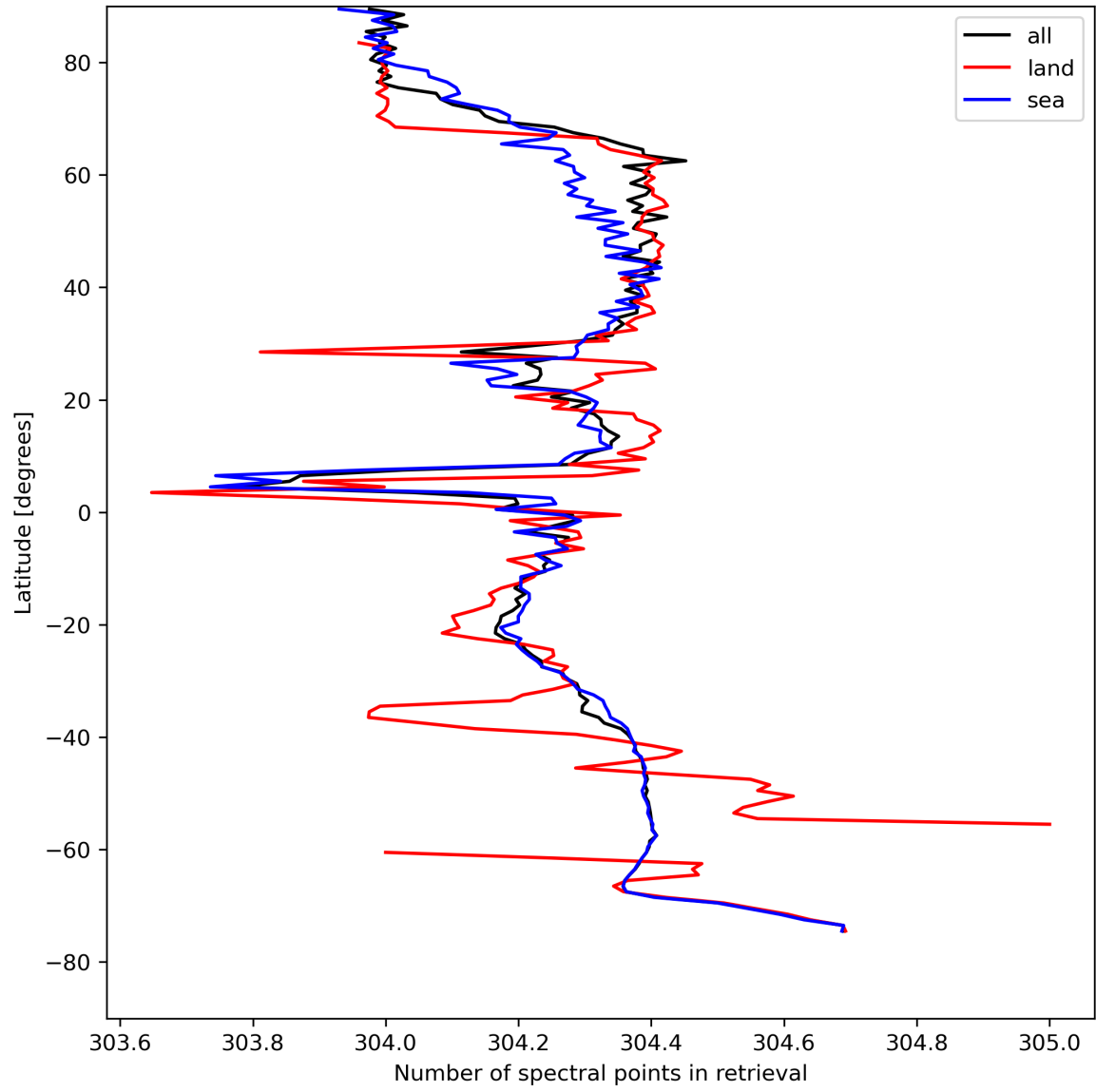
Figure 16: Zonal average of “Number of spectral points in retrieval” for 2024-04-23 to 2024-04-25.
