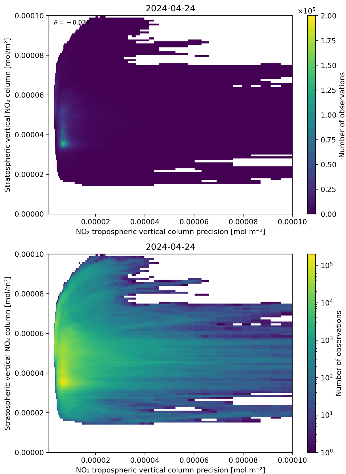
Figure 135: Scatter density plot of “NO 2 tropospheric vertical column precision” against “Stratospheric vertical NO 2 column” for 2024-04-23 to 2024-04-25.
