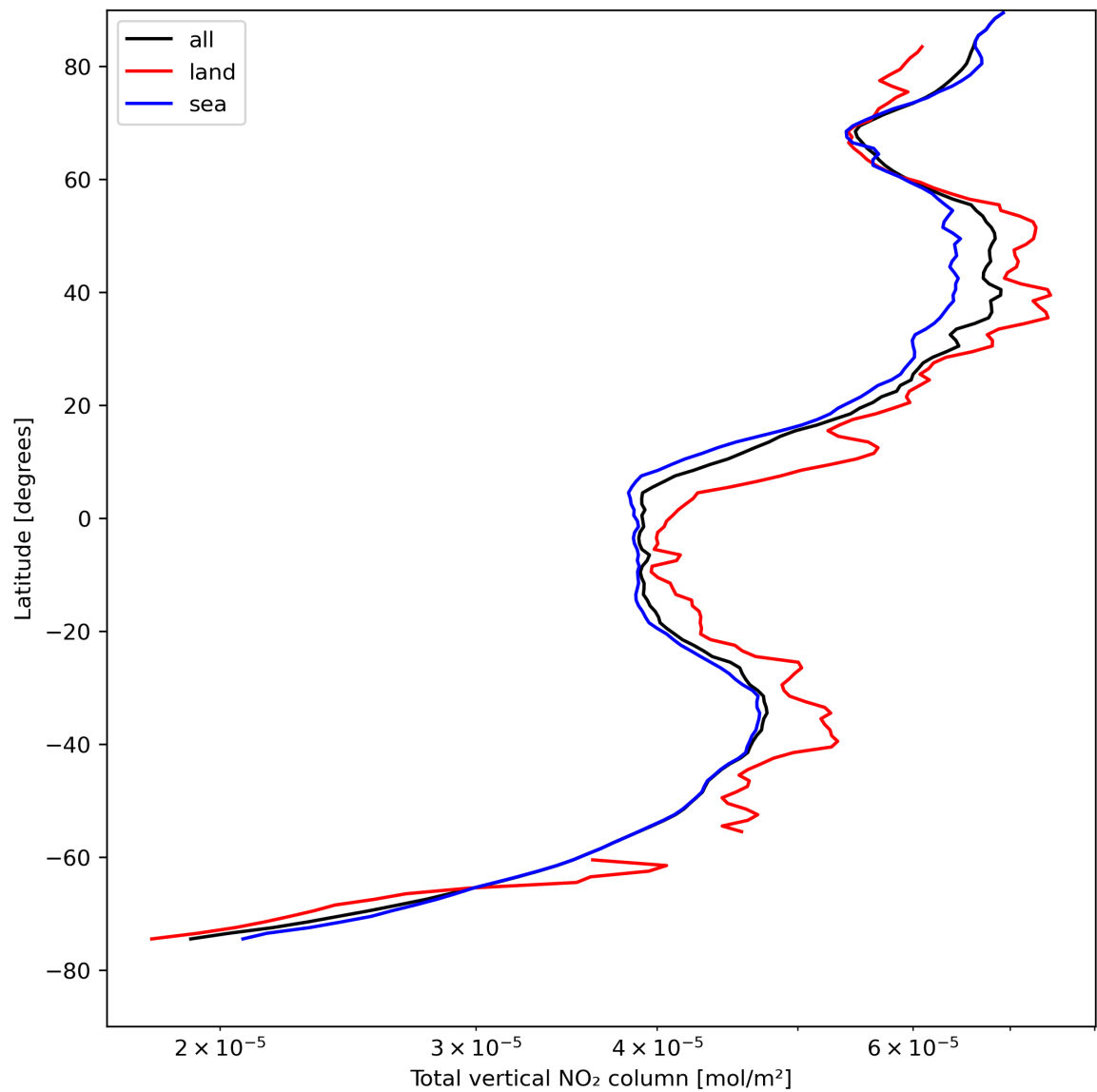
Figure 21: Zonal average of “Total vertical NO 2 column” for 2024-04-23 to 2024-04-25.
