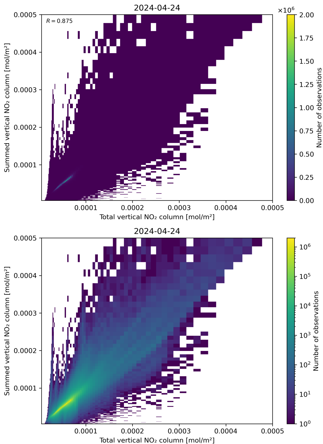
Figure 112: Scatter density plot of “Total vertical NO 2 column” against “Summed vertical NO 2 column” for 2024-04-23 to 2024-04-25.
