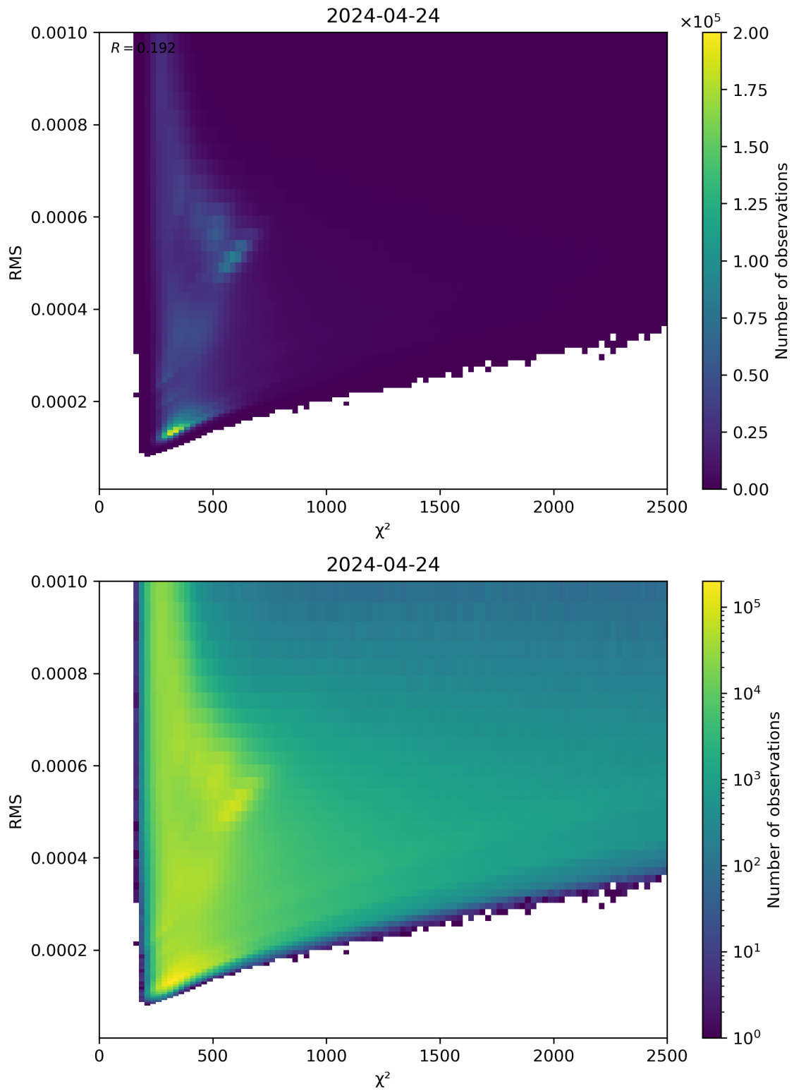
Figure 82: Scatter density plot of “ \chi^2 ” against “RMS” for 2024-04-23 to 2024-04-25.
