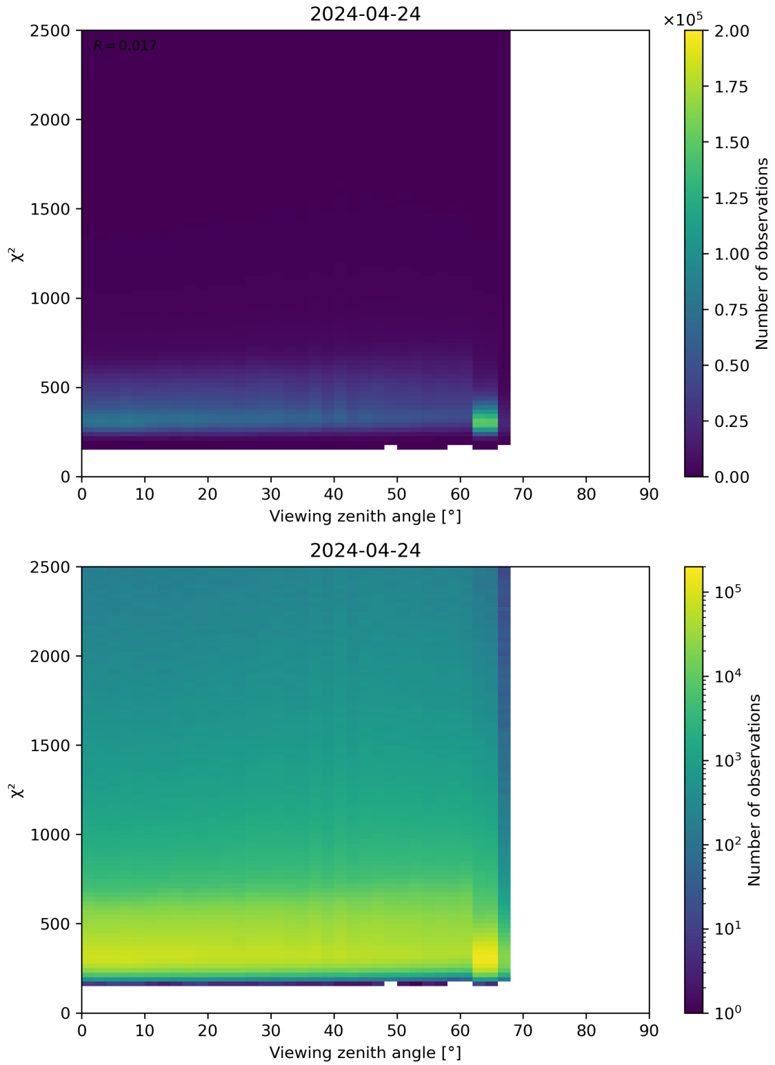
Figure 162: Scatter density plot of “Viewing zenith angle” against “ \chi^2 ” for 2024-04-23 to 2024-04-25.
