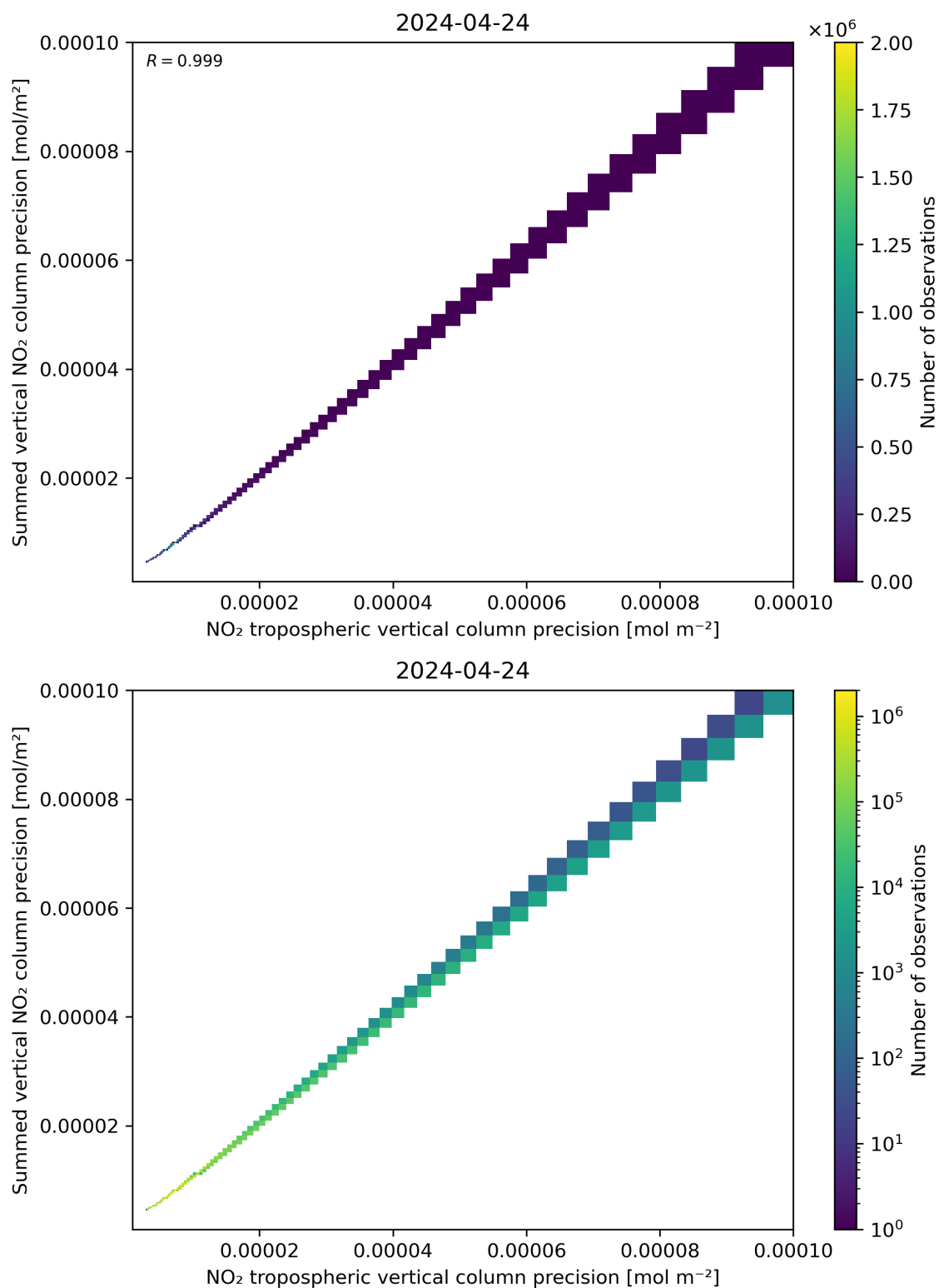
Figure 137: Scatter density plot of “NO 2 tropospheric vertical column precision” against “Summed vertical NO 2 column precision” for 2024-04-23 to 2024-04-25.
