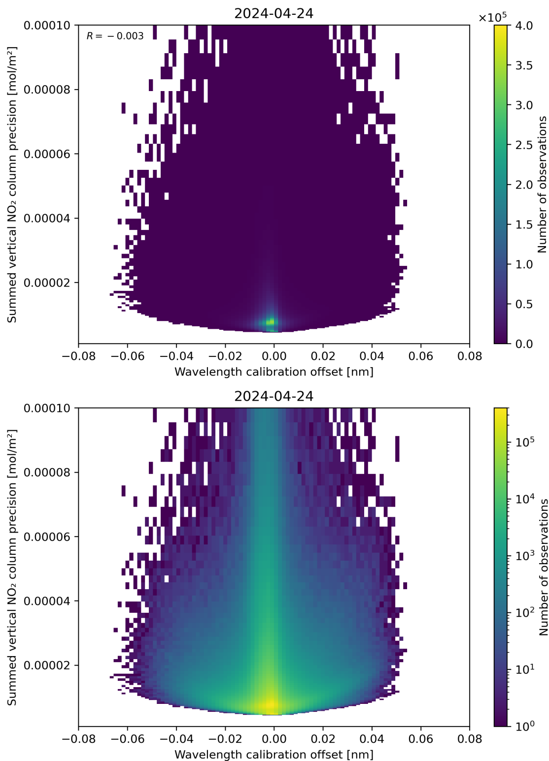
Figure 178: Scatter density plot of “Wavelength calibration offset” against “Summed vertical NO 2 column precision” for 2024-04-23 to 2024-04-25.
