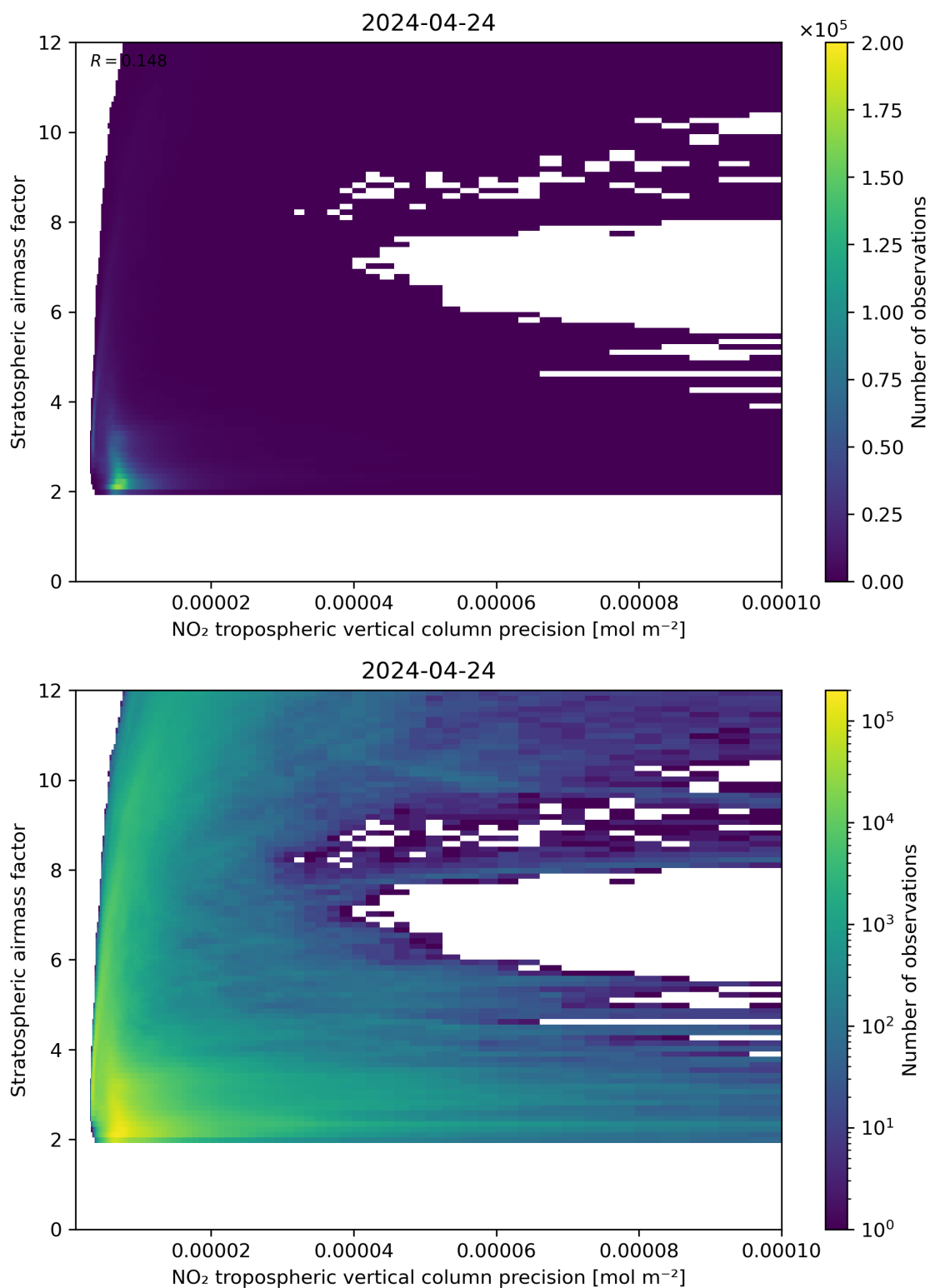
Figure 131: Scatter density plot of “NO 2 tropospheric vertical column precision” against “Stratospheric airmass factor” for 2024-04-23 to 2024-04-25.
