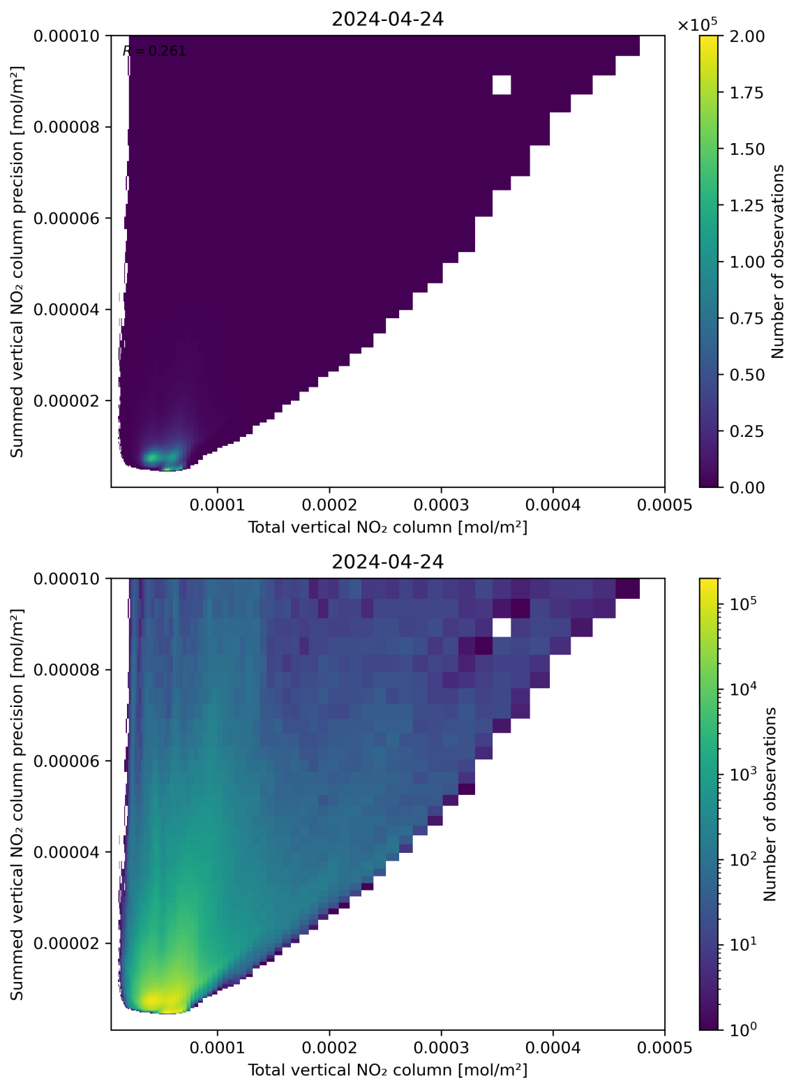
Figure 113: Scatter density plot of “Total vertical NO 2 column” against “Summed vertical NO 2 column precision” for 2024-04-23 to 2024-04-25.
