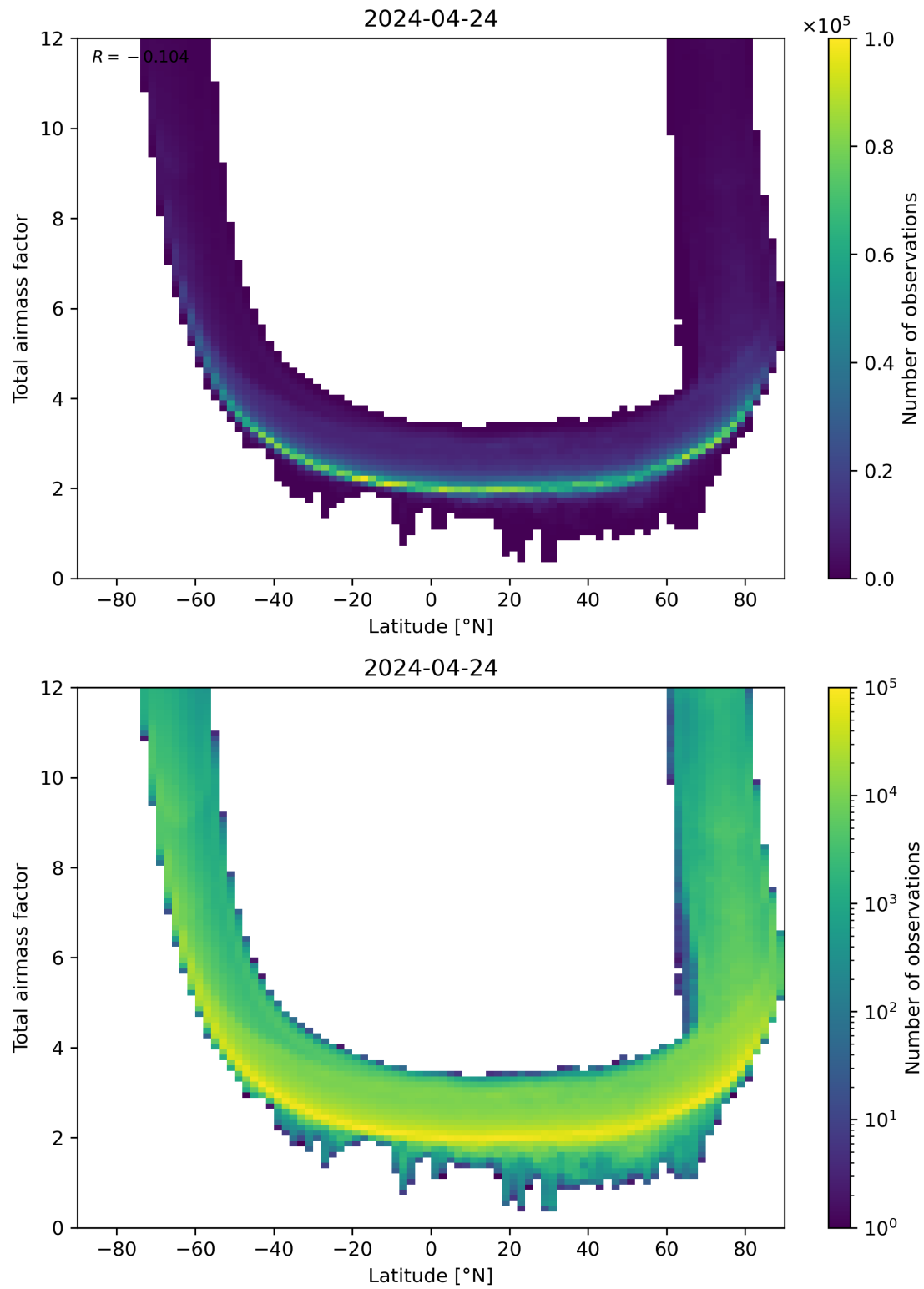
Figure 84: Scatter density plot of “Latitude” against “Total airmass factor” for 2024-04-23 to 2024-04-25.
