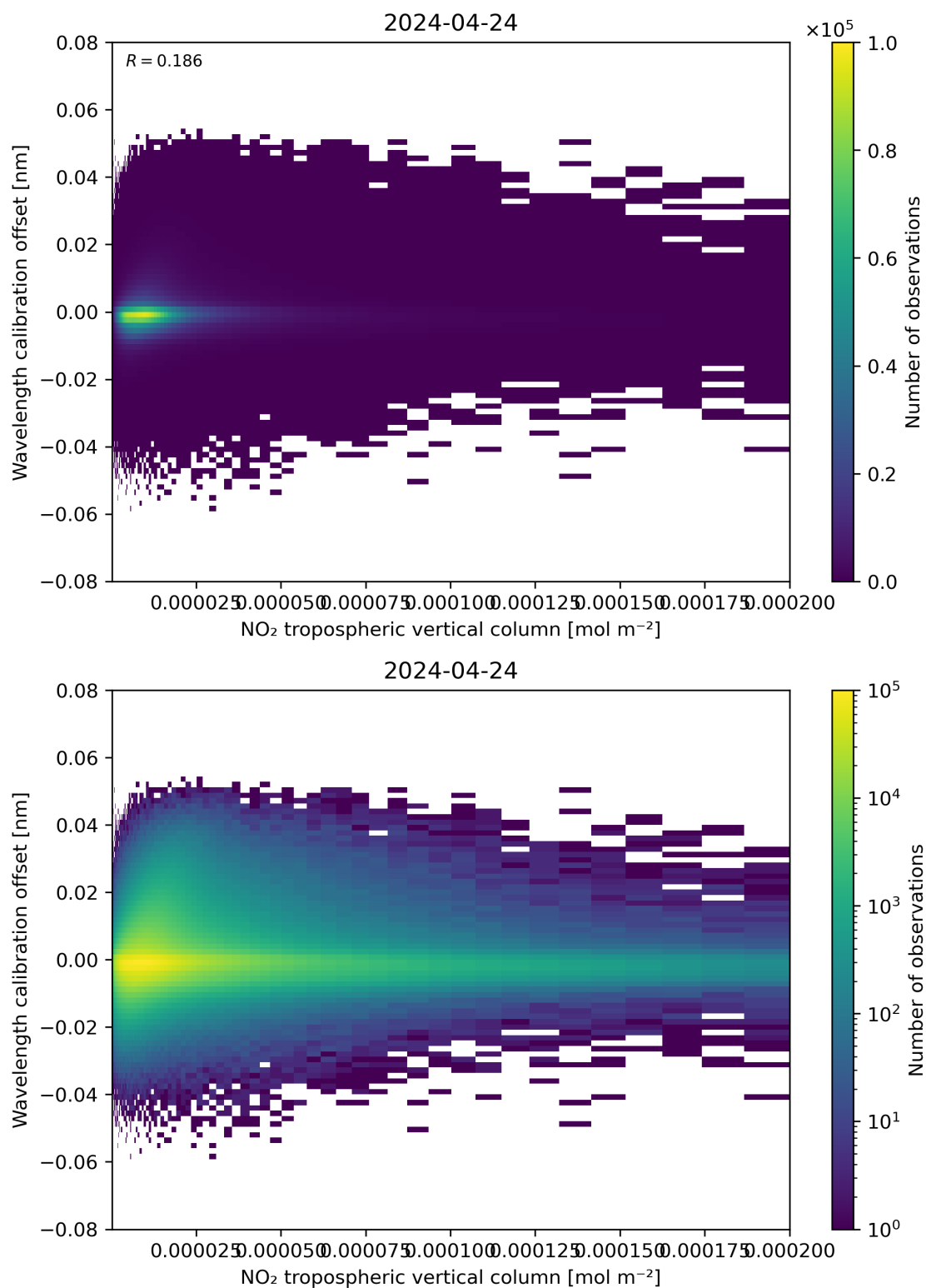
Figure 143: Scatter density plot of “NO 2 tropospheric vertical column” against “Wavelength calibration offset” for 2024-04-23 to 2024-04-25.
