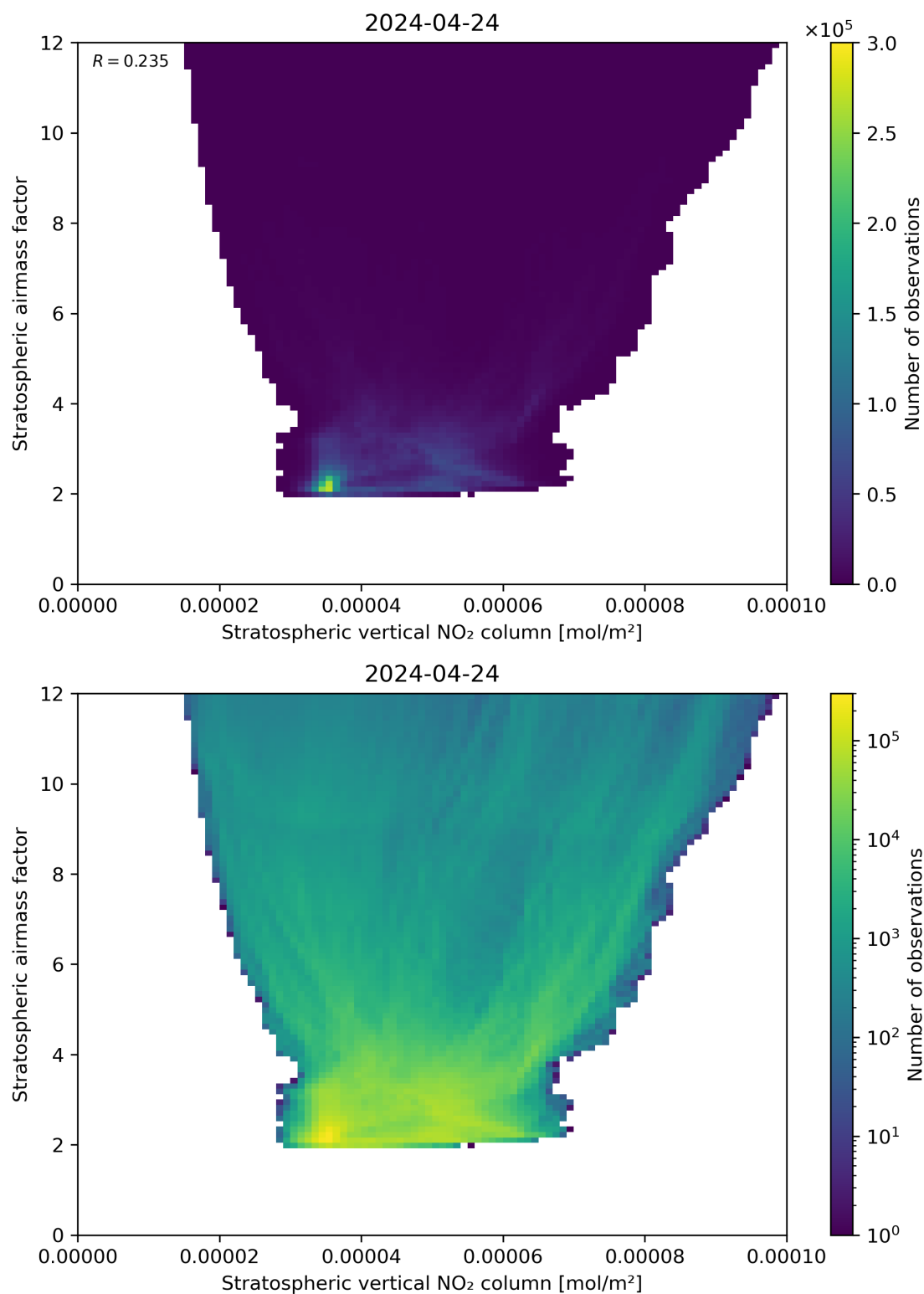
Figure 96: Scatter density plot of “Stratospheric vertical NO 2 column” against “Stratospheric airmass factor” for 2024-04-23 to 2024-04-25.
