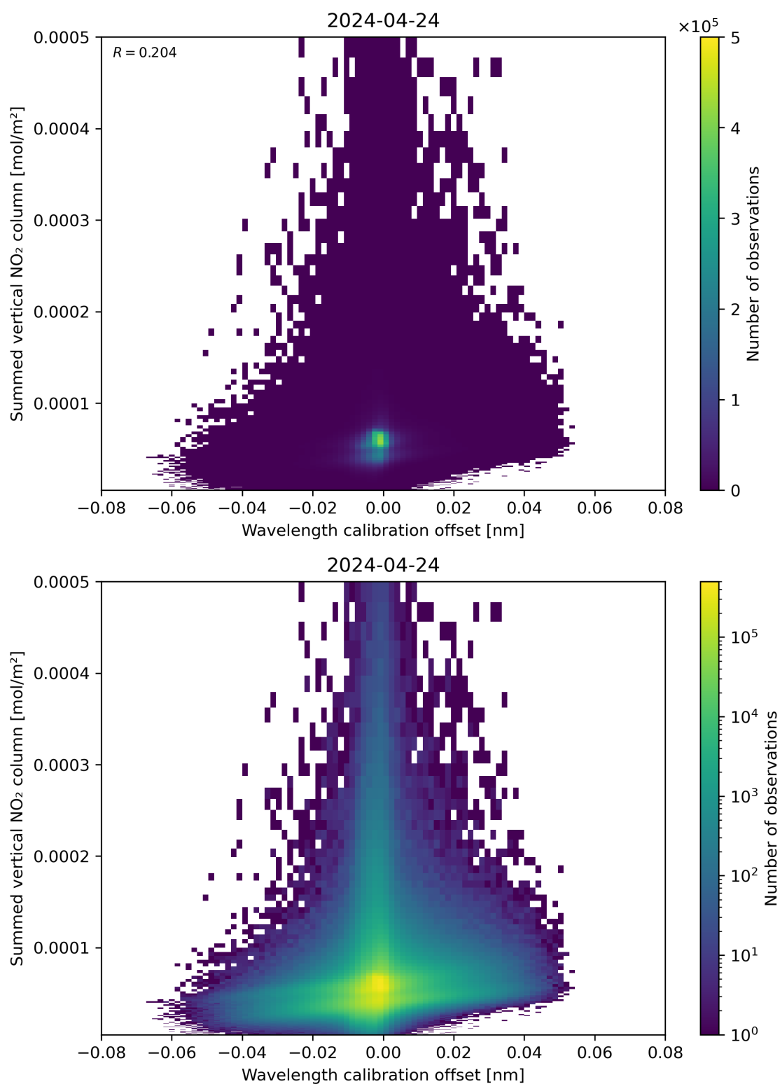
Figure 177: Scatter density plot of “Wavelength calibration offset” against “Summed vertical NO 2 column” for 2024-04-23 to 2024-04-25.
