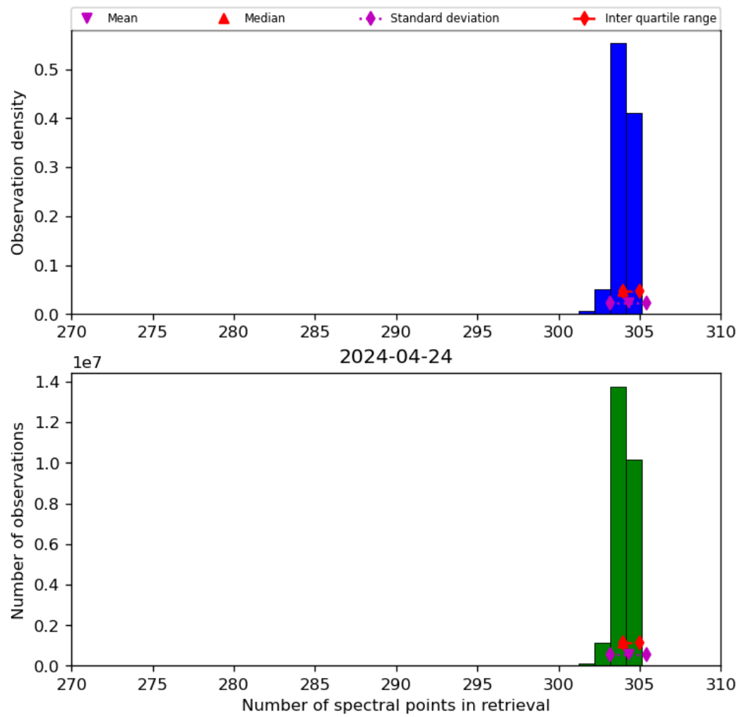
Figure 33: Histogram of “Number of spectral points in retrieval” for 2024-04-23 to 2024-04-25
