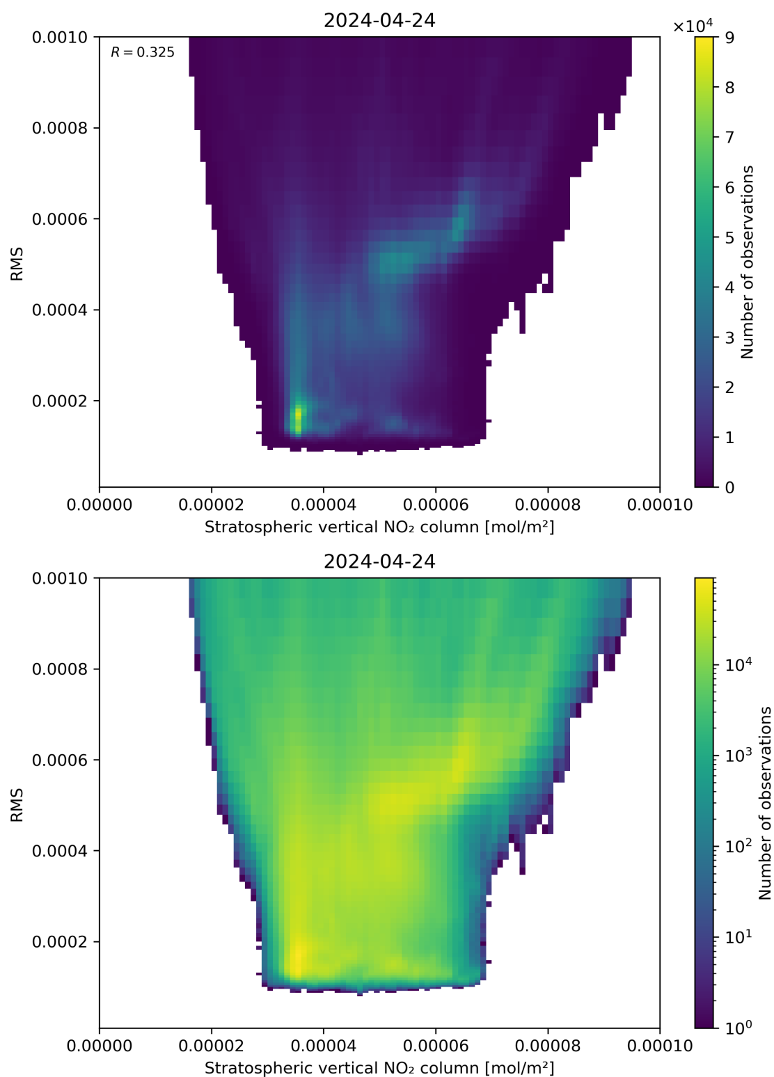
Figure 102: Scatter density plot of “Stratospheric vertical NO 2 column” against “RMS” for 2024-04-23 to 2024-04-25.
