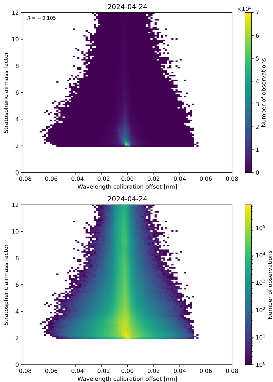
Figure 174: Scatter density plot of “Wavelength calibration offset” against “Stratospheric air mass factor” for 2024-04-23 to 2024-04-25.
