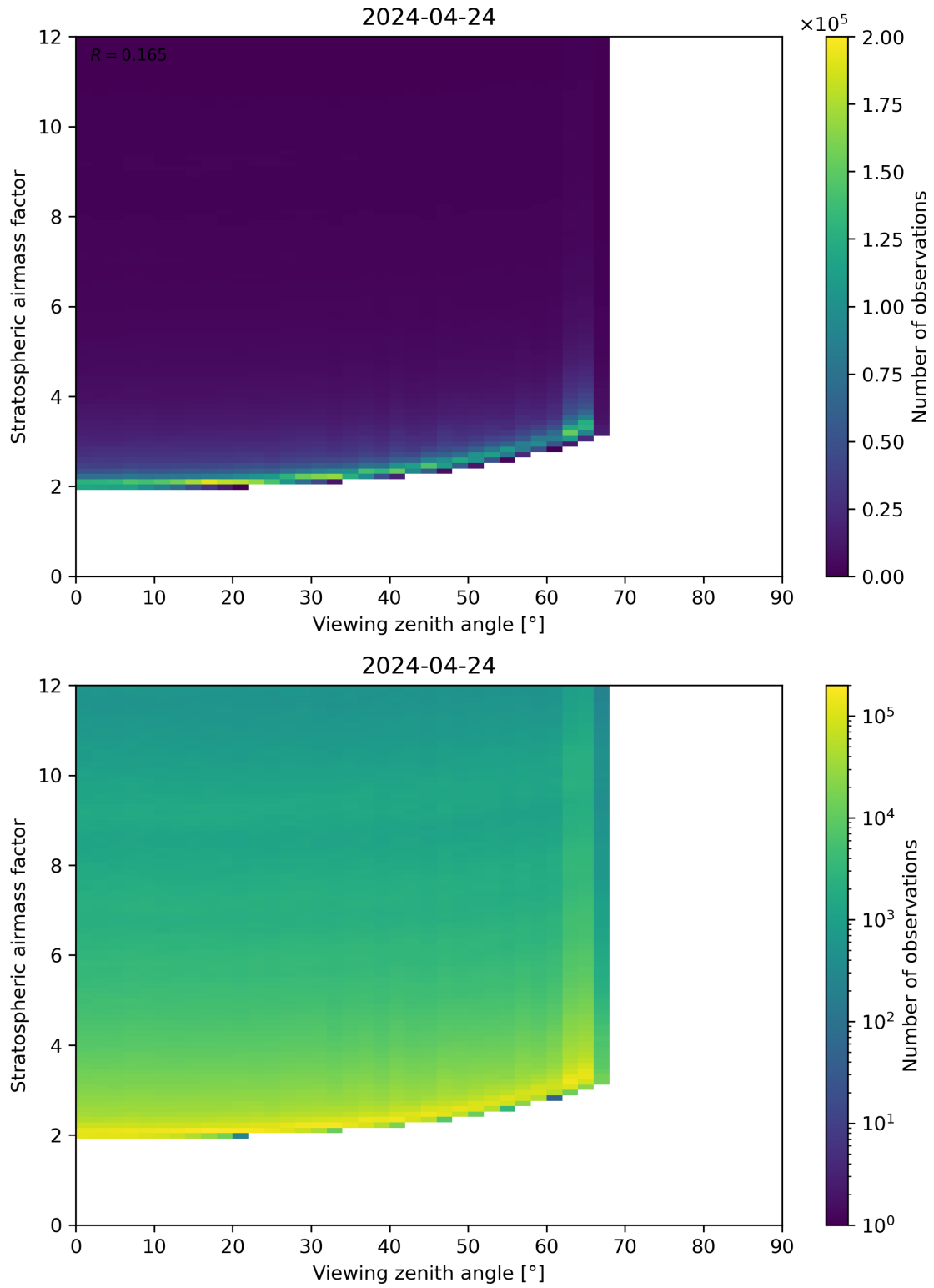
Figure 159: Scatter density plot of “Viewing zenith angle” against “Stratospheric airmass factor” for 2024-04-23 to 2024-04-25.
