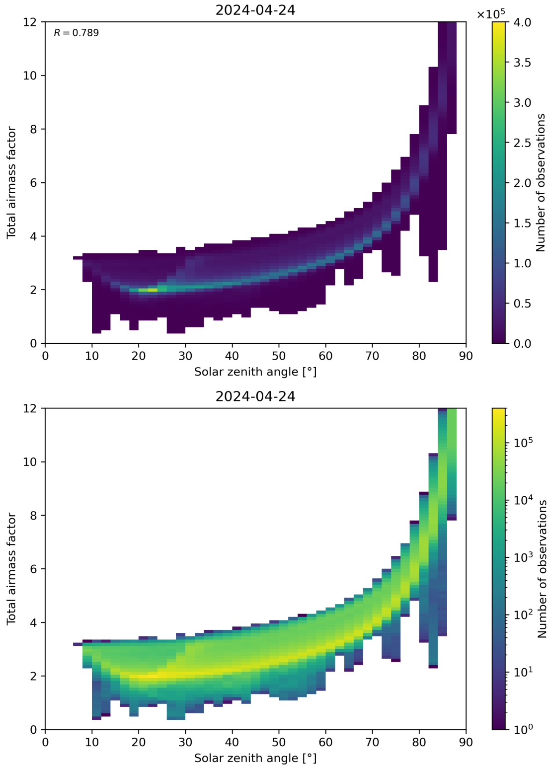
Figure 146: Scatter density plot of “Solar zenith angle” against “Total air mass factor” for 2024-04-23 to 2024-04-25.
