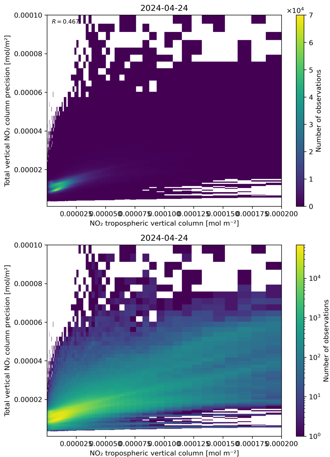
Figure 129: Scatter density plot of “NO 2 tropospheric vertical column” against “Total vertical NO 2 column precision” for 2024-04-23 to 2024-04-25.
