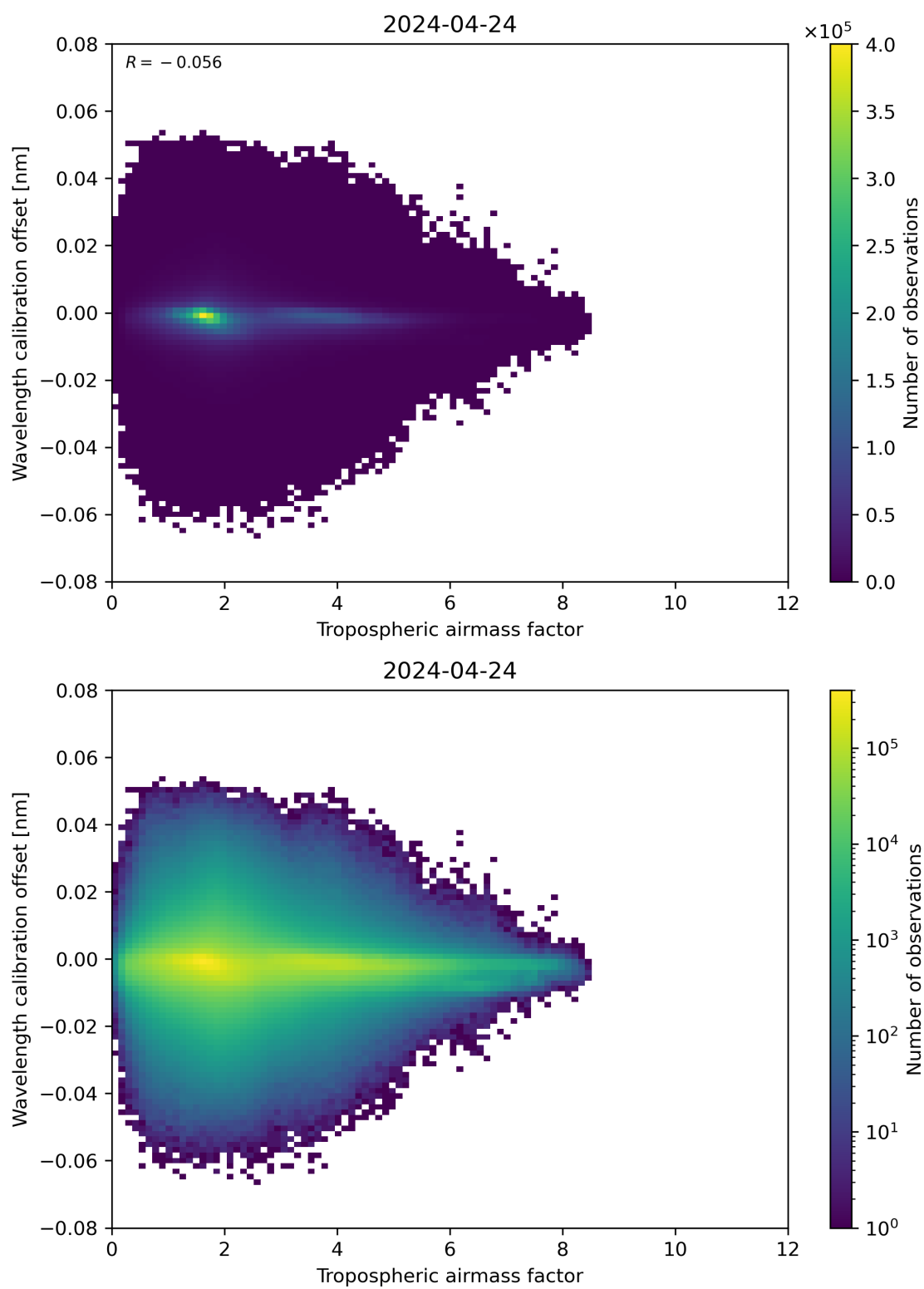
Figure 80: Scatter density plot of “Tropospheric air mass factor” against “Wavelength calibration offset” for 2024-04-23 to 2024-04-25.
