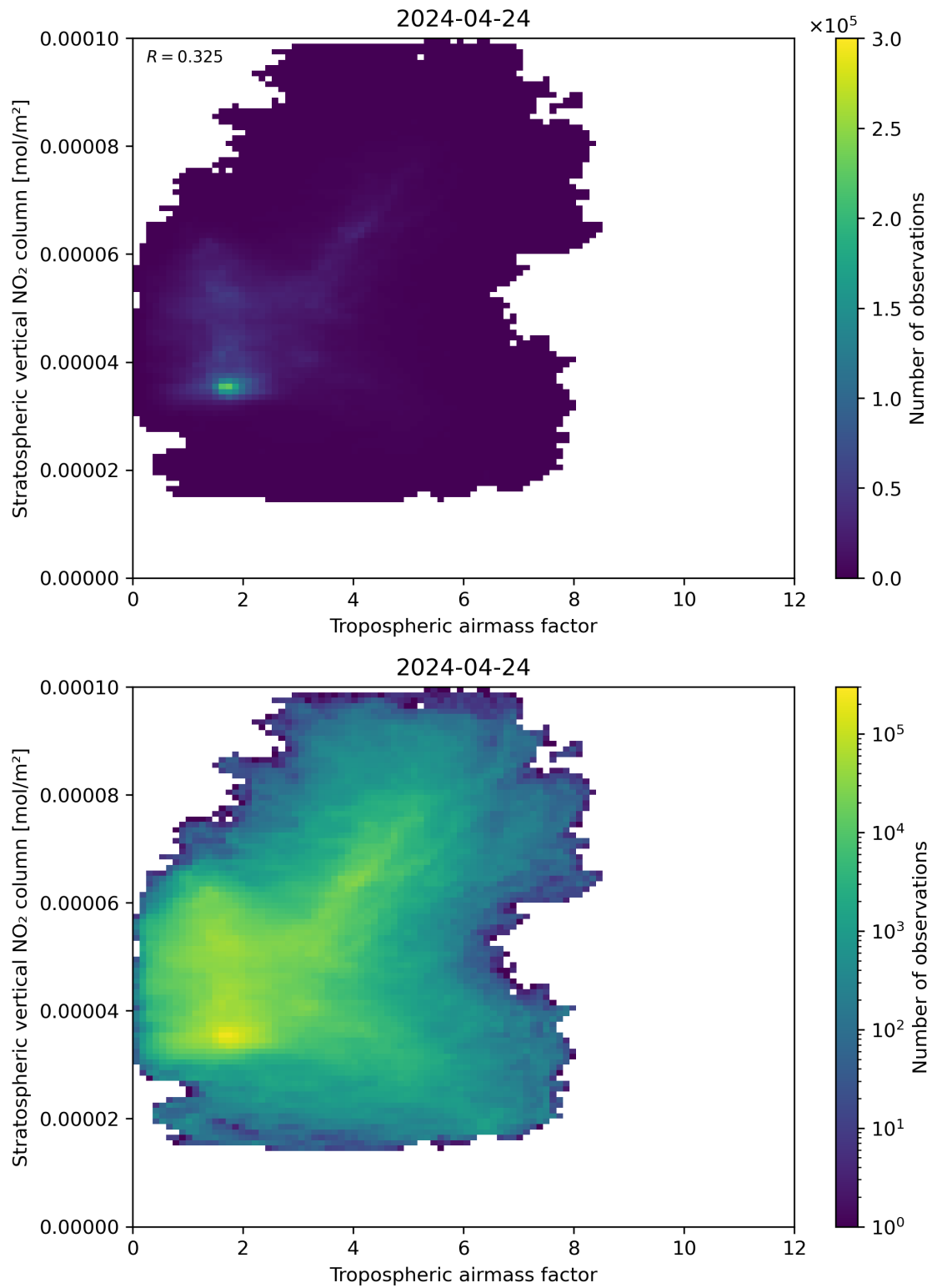
Figure 74: Scatter density plot of “Tropospheric air mass factor” against “Stratospheric vertical \text{NO}_2 column” for 2024-04-23 to 2024-04-25.
