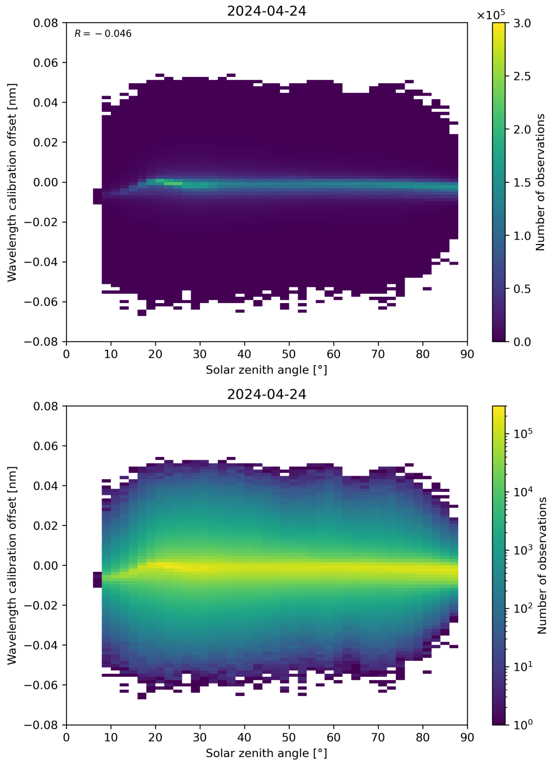
Figure 158: Scatter density plot of “Solar zenith angle” against “Wavelength calibration offset” for 2024-04-23 to 2024-04-25.
