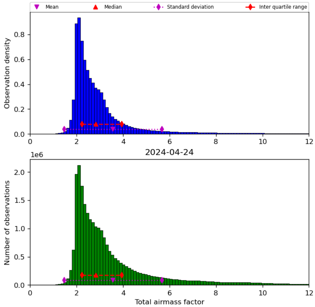
Figure 32: Histogram of “Total airmass factor” for 2024-04-23 to 2024-04-25
