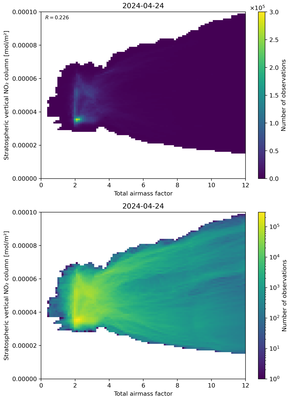
Figure 64: Scatter density plot of “Total airmass factor” against “Stratospheric vertical \text{NO}_2 column” for 2024-04-23 to 2024-04-25.
