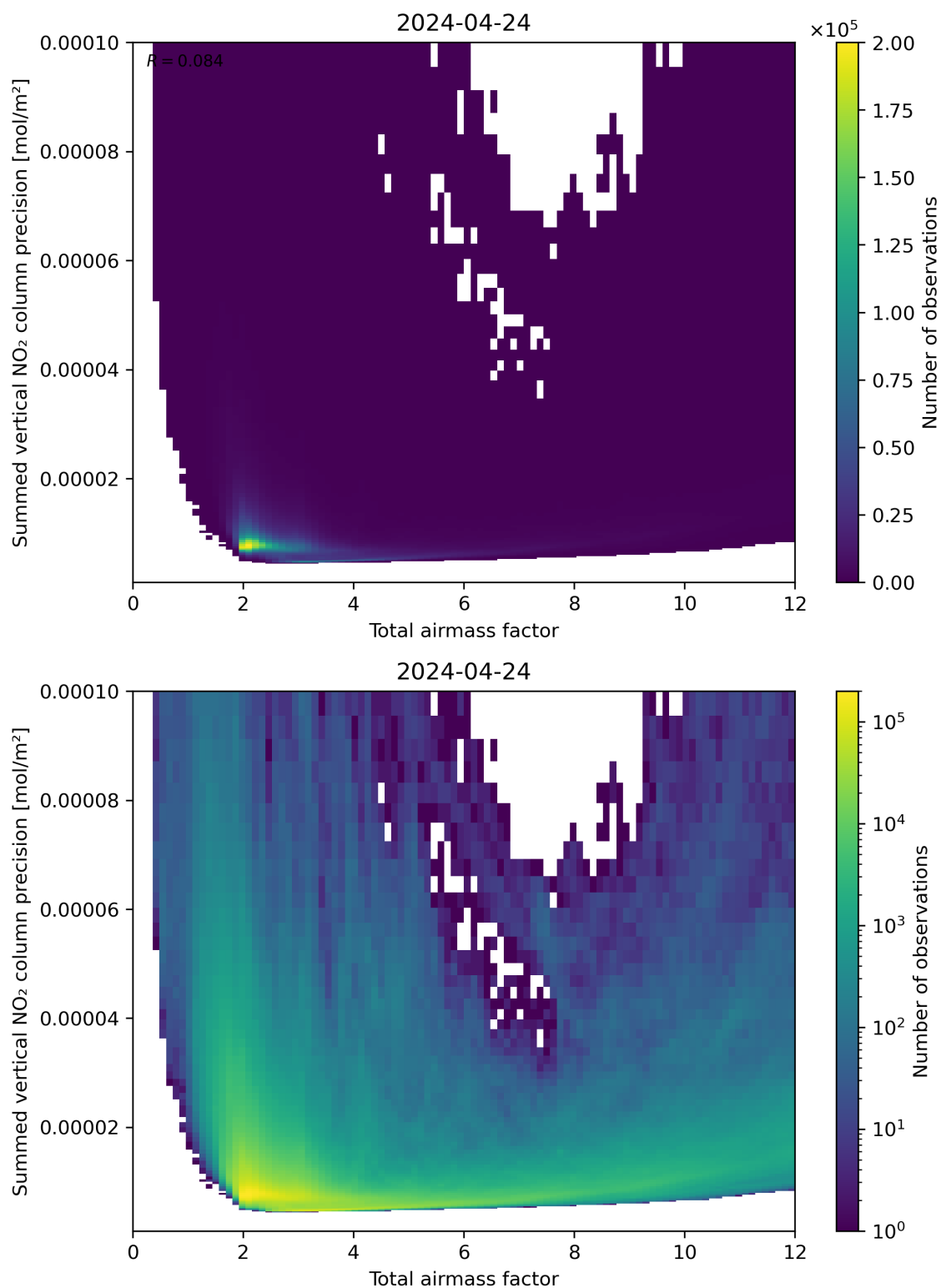
Figure 66: Scatter density plot of “Total airmass factor” against “Summed vertical NO 2 column precision” for 2024-04-23 to 2024-04-25.
