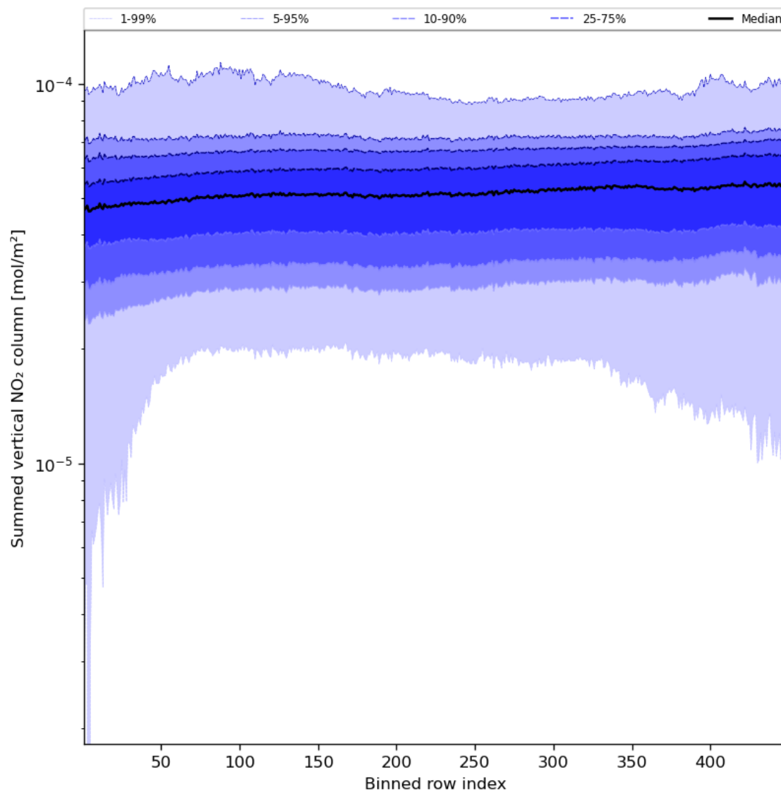
Figure 57: Along track statistics of “Summed vertical NO 2 column” for 2024-04-23 to 2024-04-25
