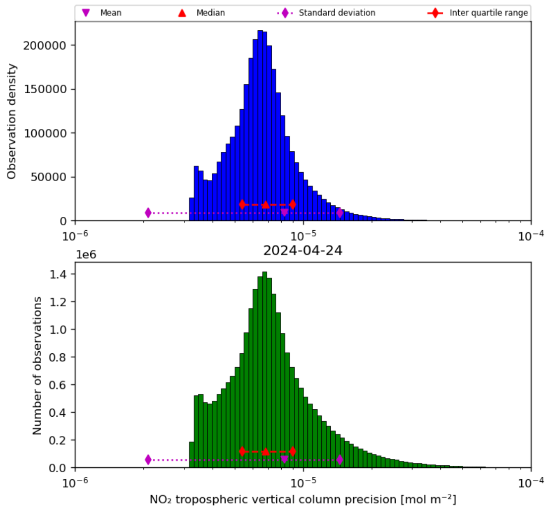
Figure 30: Histogram of “NO 2 tropospheric vertical column precision” for 2024-04-23 to 2024-04-25
