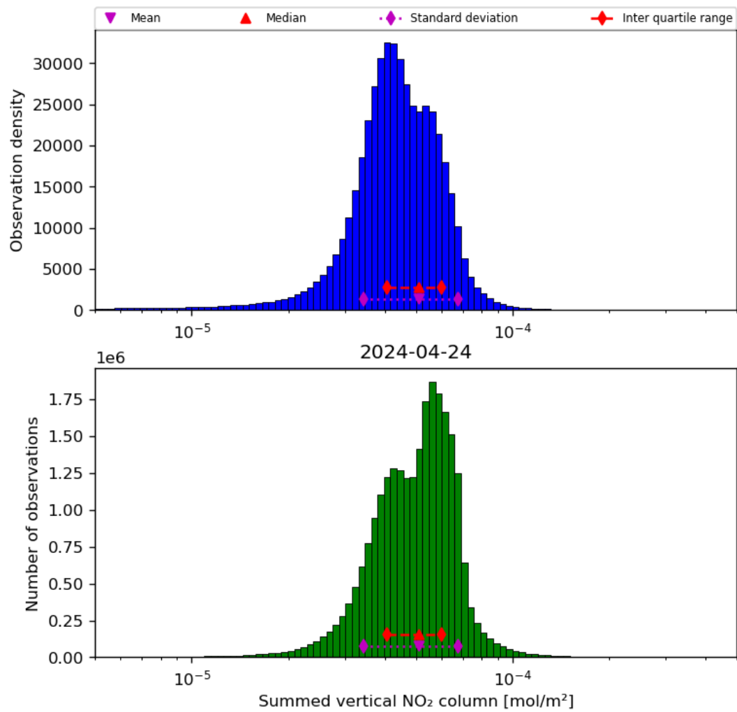
Figure 40: Histogram of “Summed vertical NO 2 column” for 2024-04-23 to 2024-04-25
