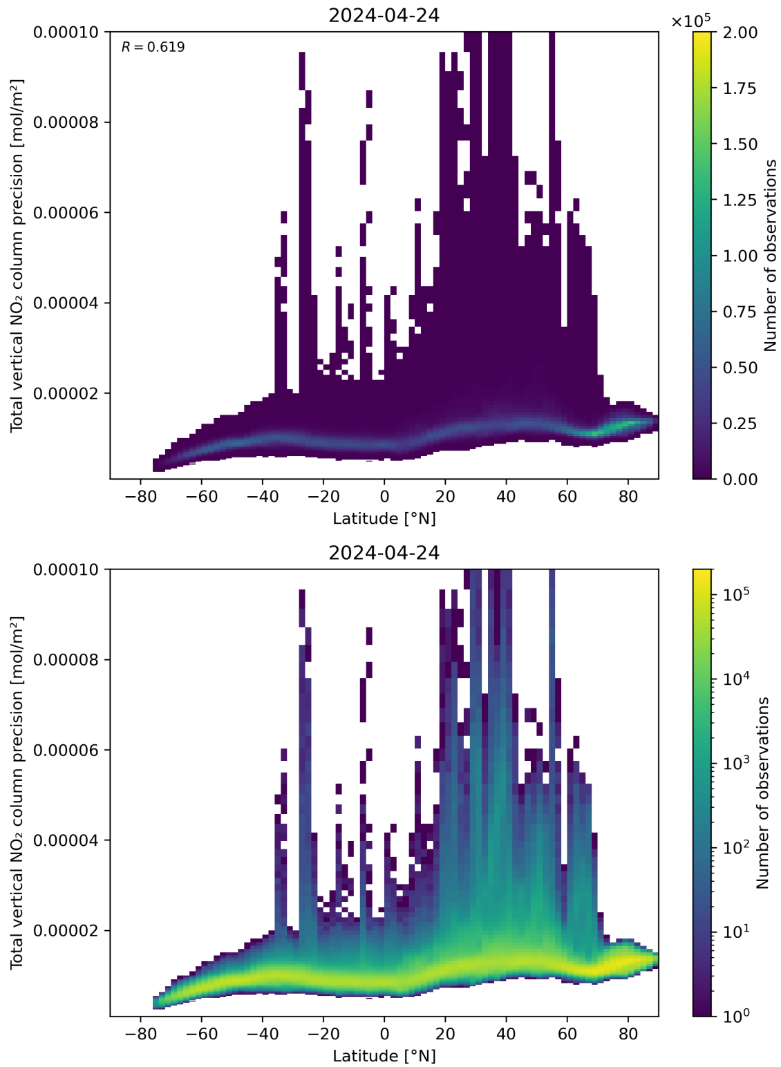
Figure 91: Scatter density plot of “Latitude” against “Total vertical NO 2 column precision” for 2024-04-23 to 2024-04-25.
