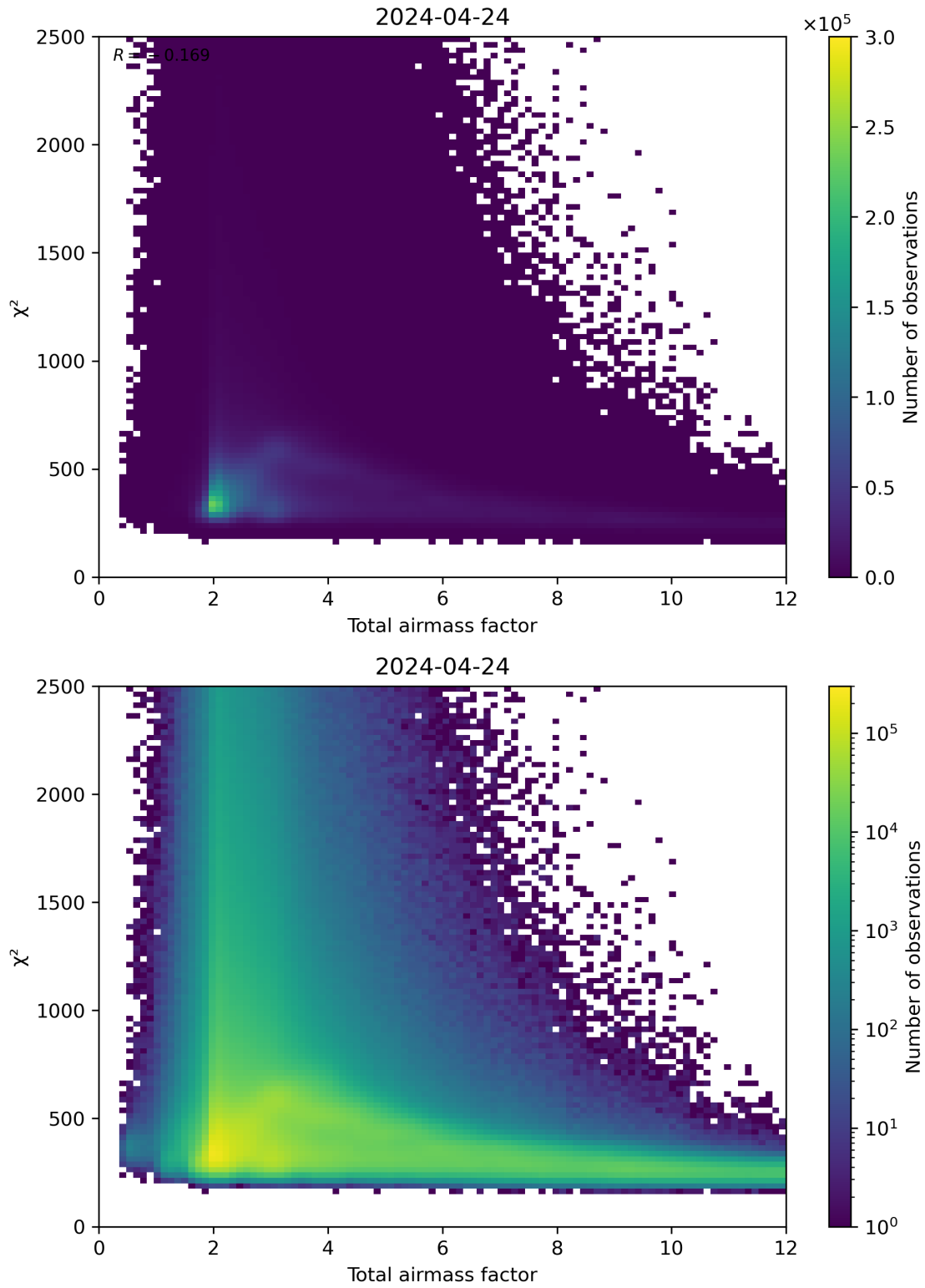
Figure 63: Scatter density plot of “Total airmass factor” against “ \chi^2 ” for 2024-04-23 to 2024-04-25.
