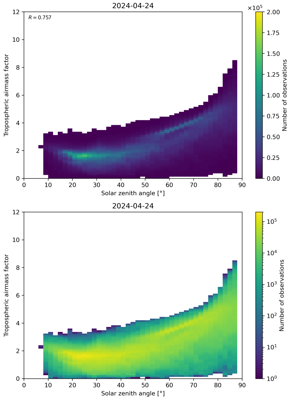
Figure 147: Scatter density plot of “Solar zenith angle” against “Tropospheric airmass factor” for 2024-04-23 to 2024-04-25.
