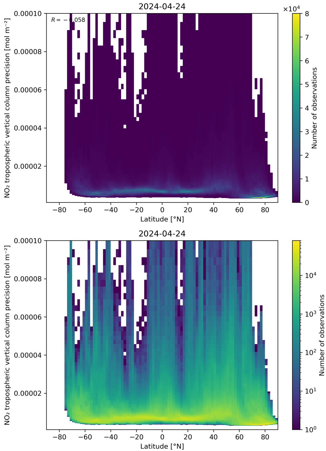
Figure 93: Scatter density plot of “Latitude” against “NO 2 tropospheric vertical column precision” for 2024-04-23 to 2024-04-25.
