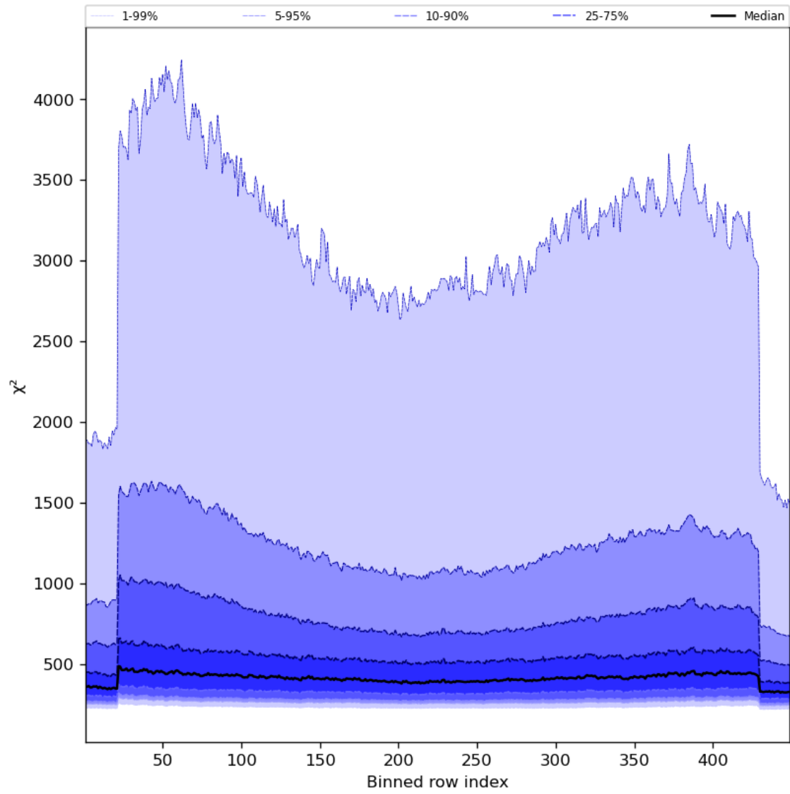
Figure 59: Along track statistics of “ \chi^2 ” for 2024-04-23 to 2024-04-25
