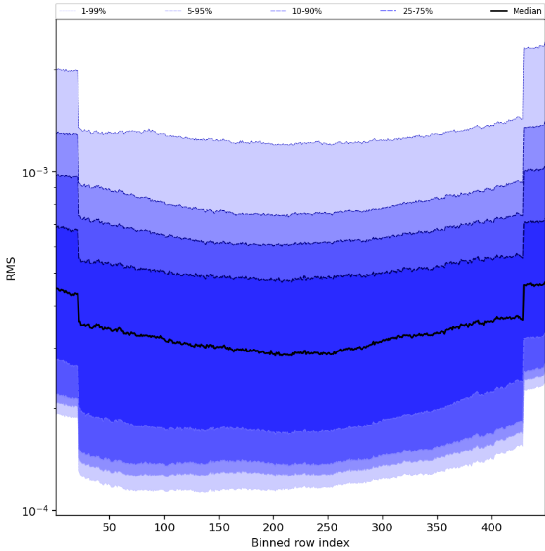
Figure 60: Along track statistics of “RMS” for 2024-04-23 to 2024-04-25
