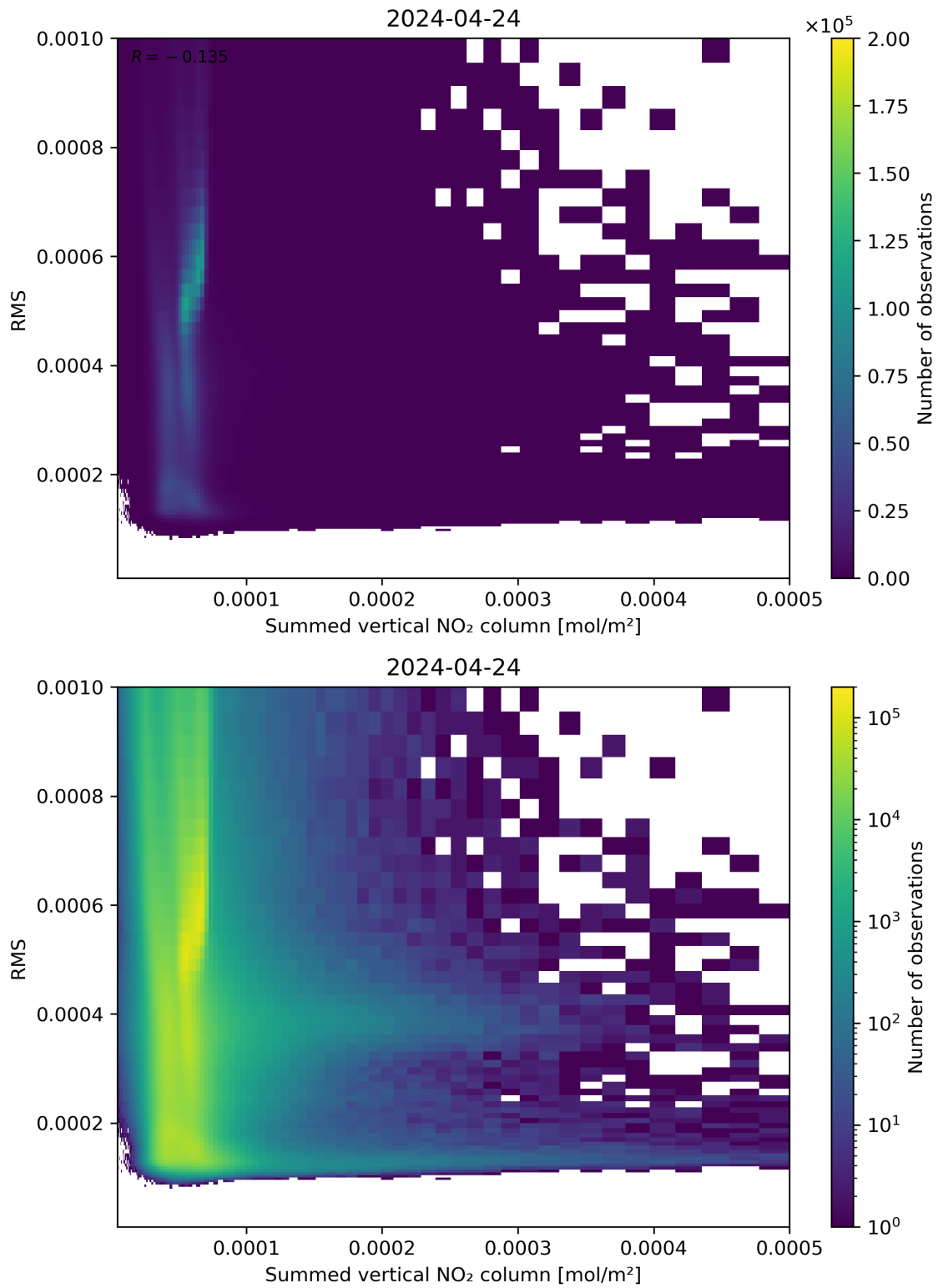
Figure 109: Scatter density plot of “Summed vertical NO 2 column” against “RMS” for 2024-04-23 to 2024-04-25.
