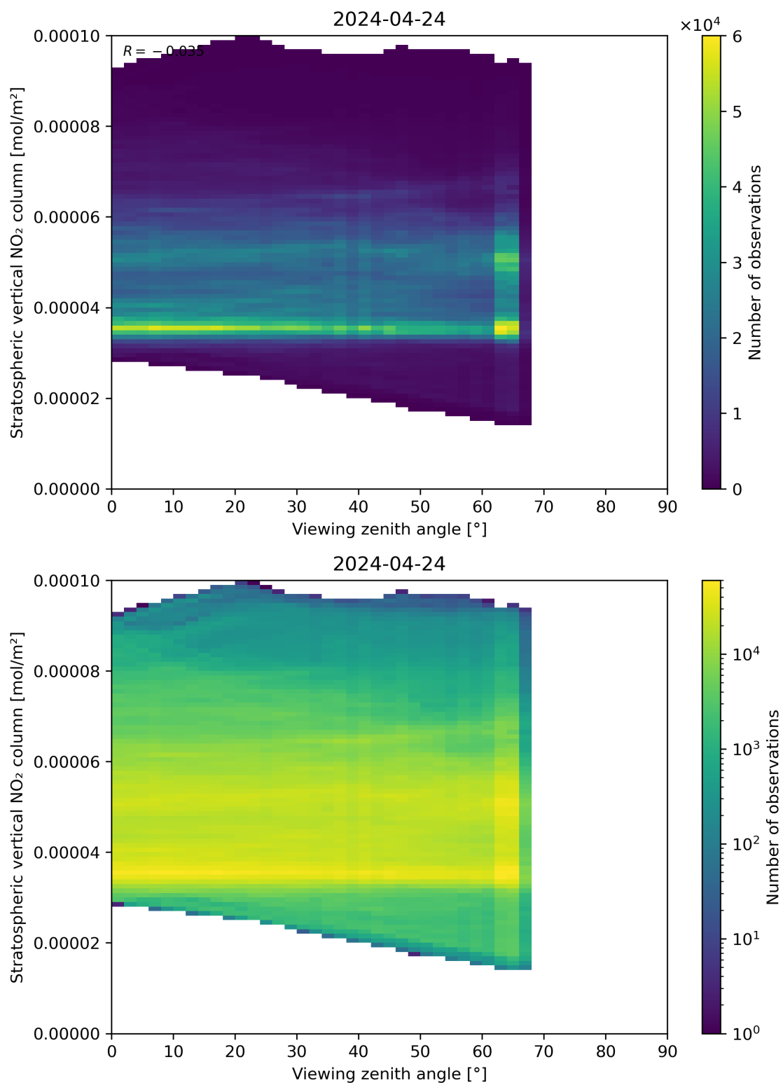
Figure 164: Scatter density plot of “Viewing zenith angle” against “Stratospheric vertical NO 2 column” for 2024-04-23 to 2024-04-25.
