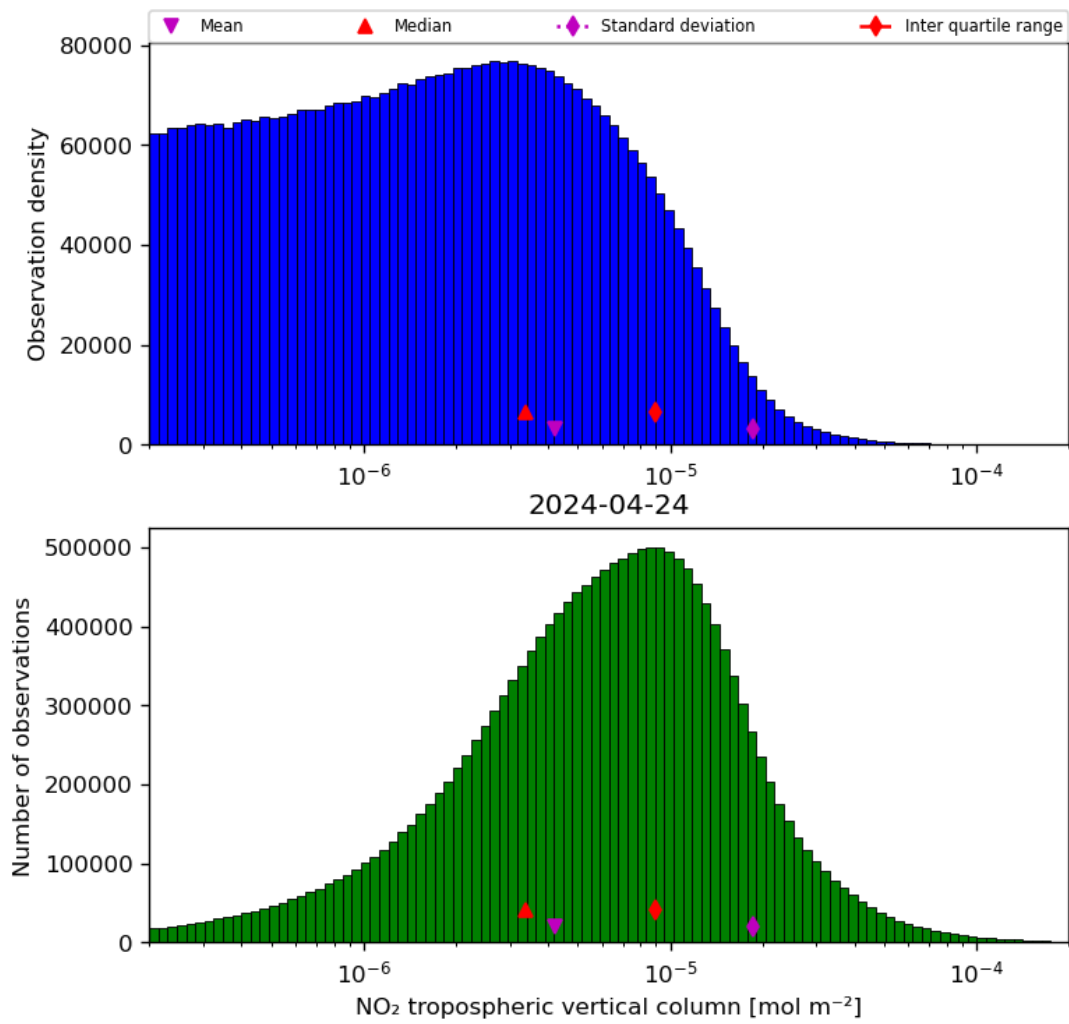
Figure 29: Histogram of “NO 2 tropospheric vertical column” for 2024-04-23 to 2024-04-25
