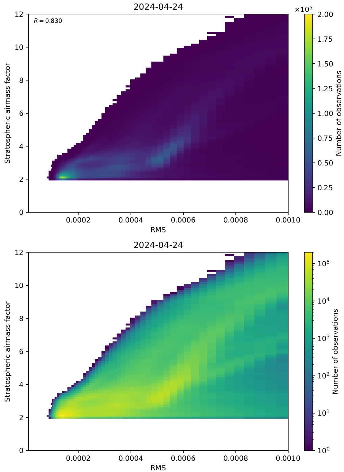
Figure 144: Scatter density plot of “RMS” against “Stratospheric airmass factor” for 2024-04-23 to 2024-04-25.
