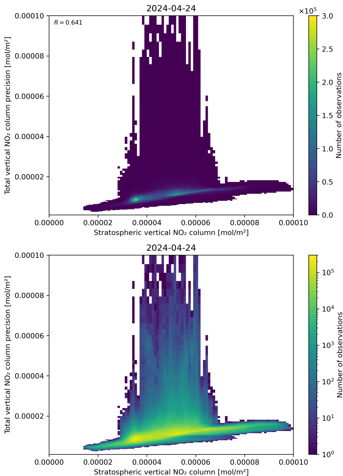
Figure 101: Scatter density plot of “Stratospheric vertical NO 2 column” against “Total vertical NO 2 column precision” for 2024-04-23 to 2024-04-25.
