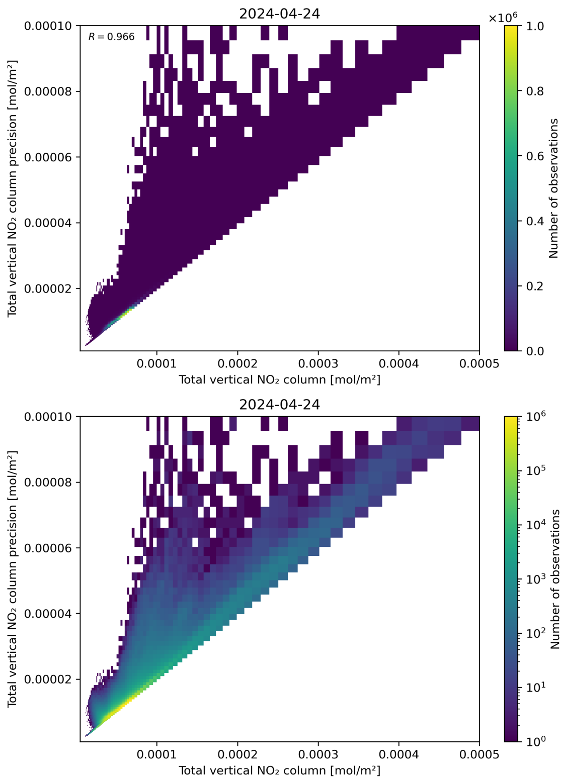
Figure 114: Scatter density plot of “Total vertical NO 2 column” against “Total vertical NO 2 column precision” for 2024-04-23 to 2024-04-25.
