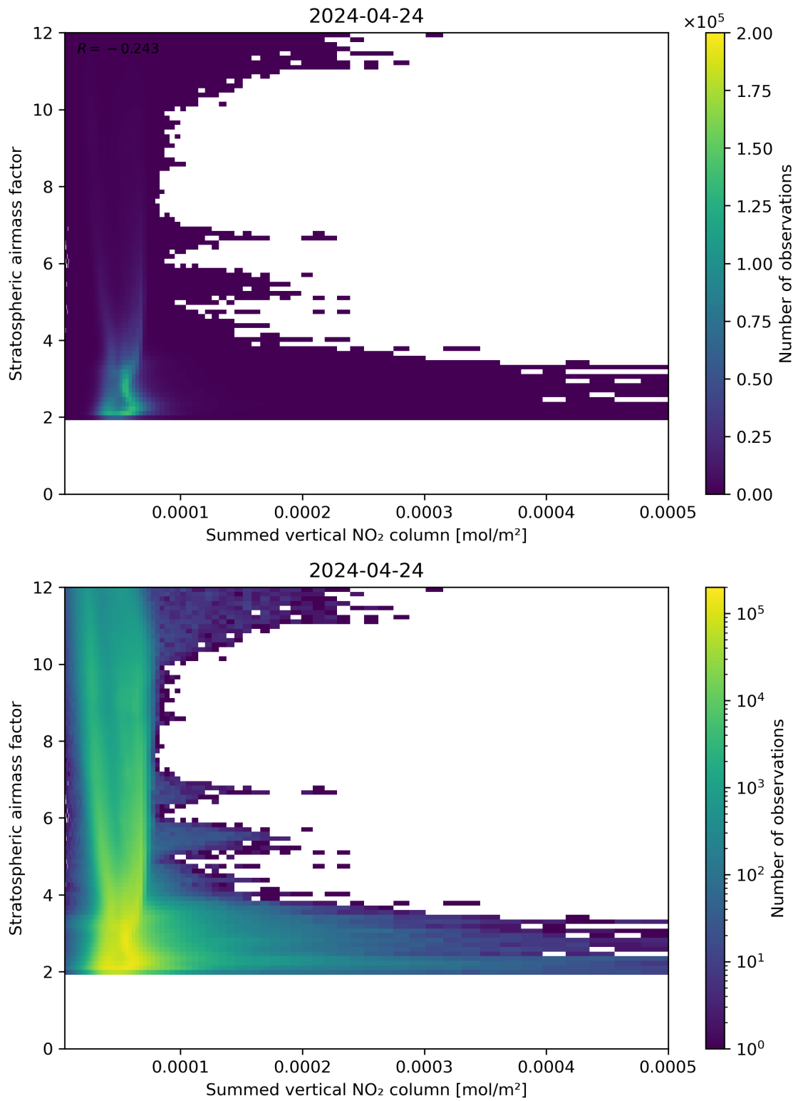
Figure 103: Scatter density plot of “Summed vertical NO 2 column” against “Stratospheric airmass factor” for 2024-04-23 to 2024-04-25.
