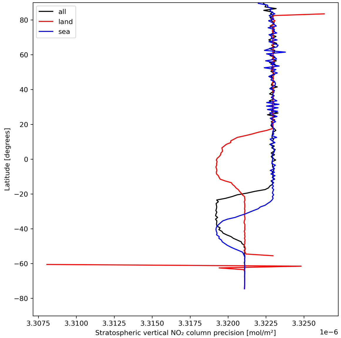
Figure 20: Zonal average of “Stratospheric vertical NO 2 column precision” for 2024-04-23 to 2024-04-25.
