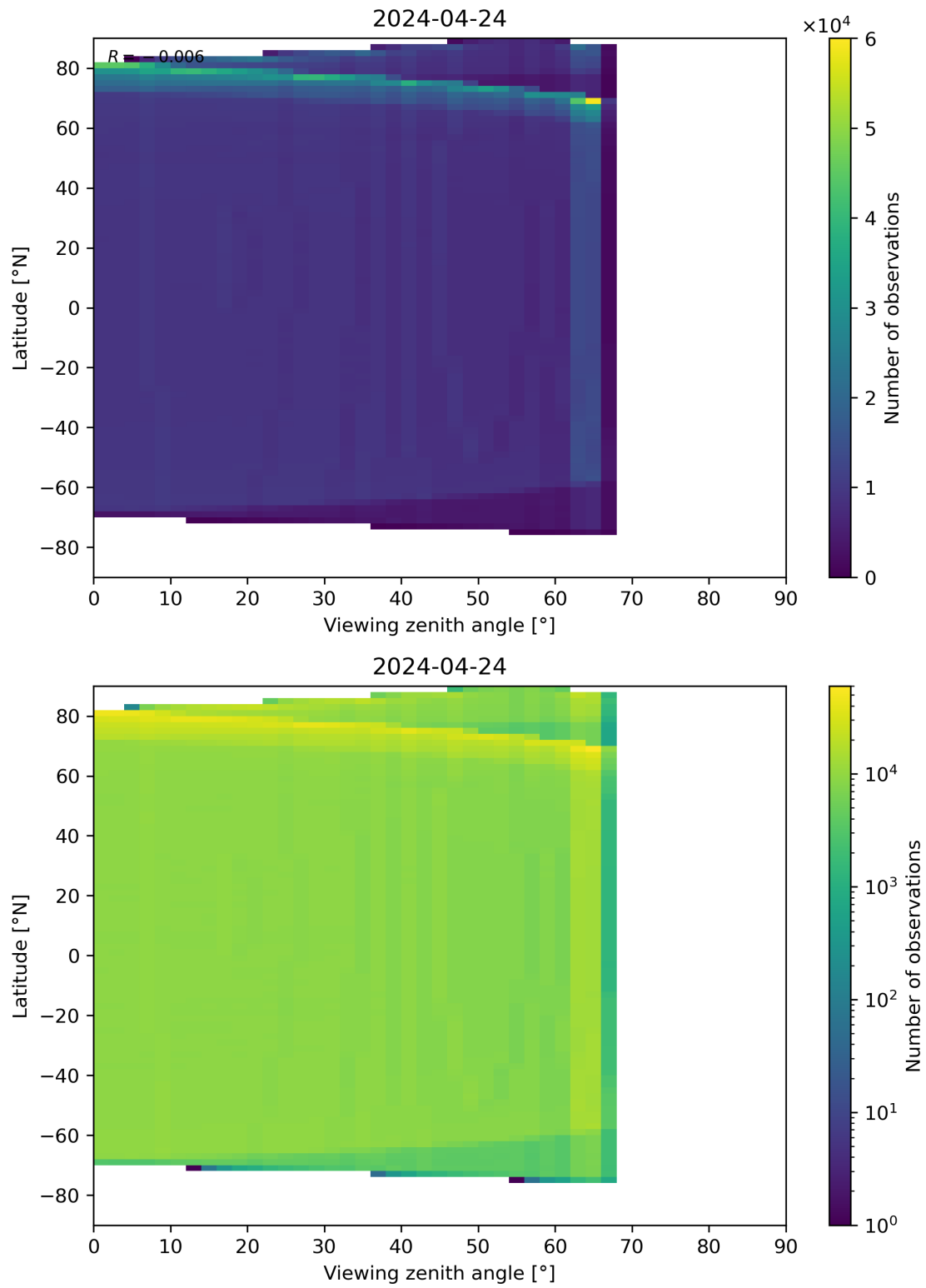
Figure 163: Scatter density plot of “Viewing zenith angle” against “Latitude” for 2024-04-23 to 2024-04-25.
