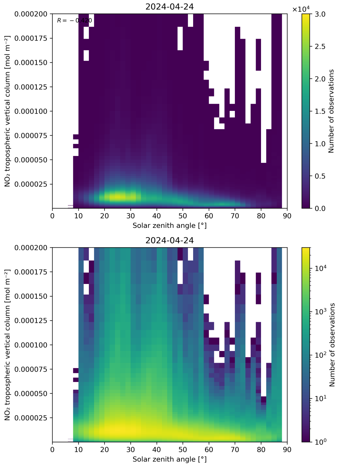
Figure 155: Scatter density plot of “Solar zenith angle” against “NO 2 tropospheric vertical column” for 2024-04-23 to 2024-04-25.
