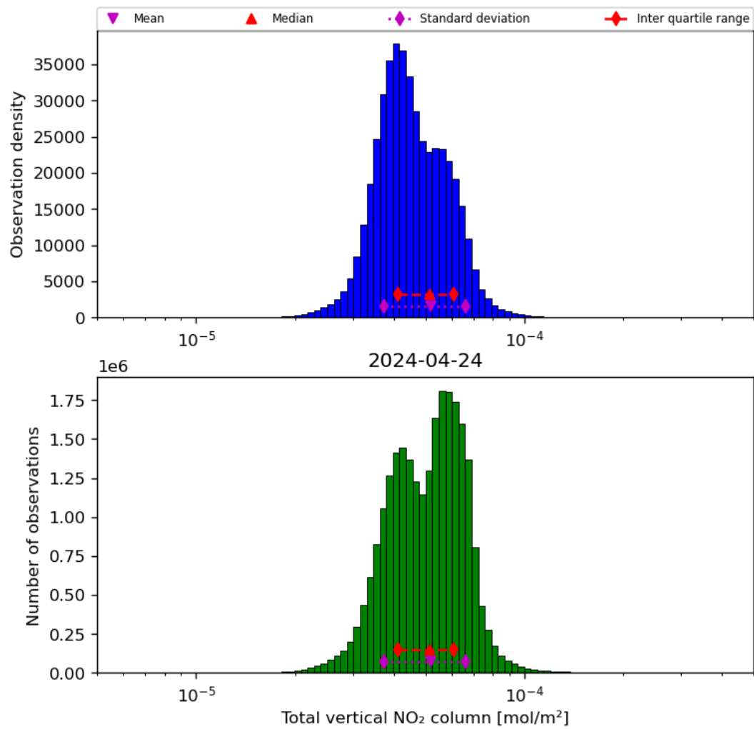
Figure 38: Histogram of “Total vertical NO 2 column” for 2024-04-23 to 2024-04-25
