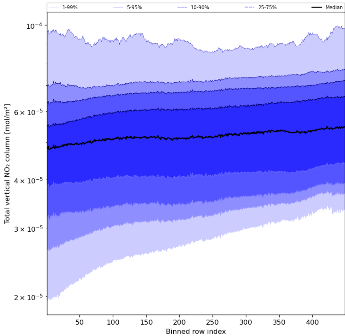
Figure 55: Along track statistics of “Total vertical NO 2 column” for 2024-04-23 to 2024-04-25
