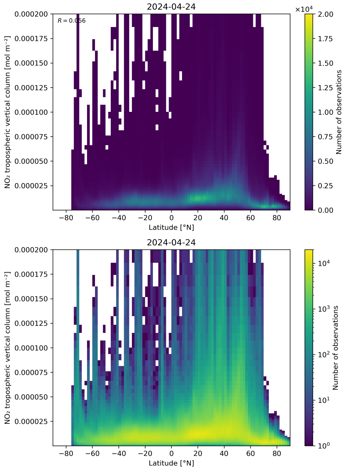
Figure 92: Scatter density plot of “Latitude” against “NO 2 tropospheric vertical column” for 2024-04-23 to 2024-04-25.
