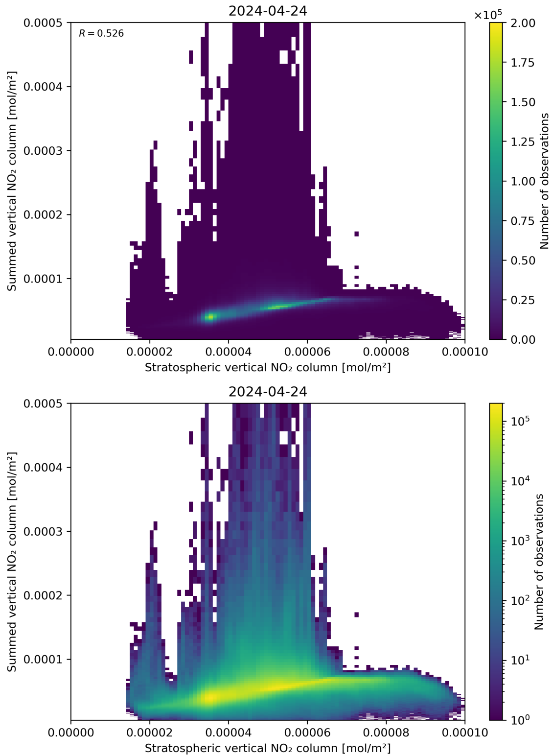
Figure 98: Scatter density plot of “Stratospheric vertical NO 2 column” against “Summed vertical NO 2 column” for 2024-04-23 to 2024-04-25.
