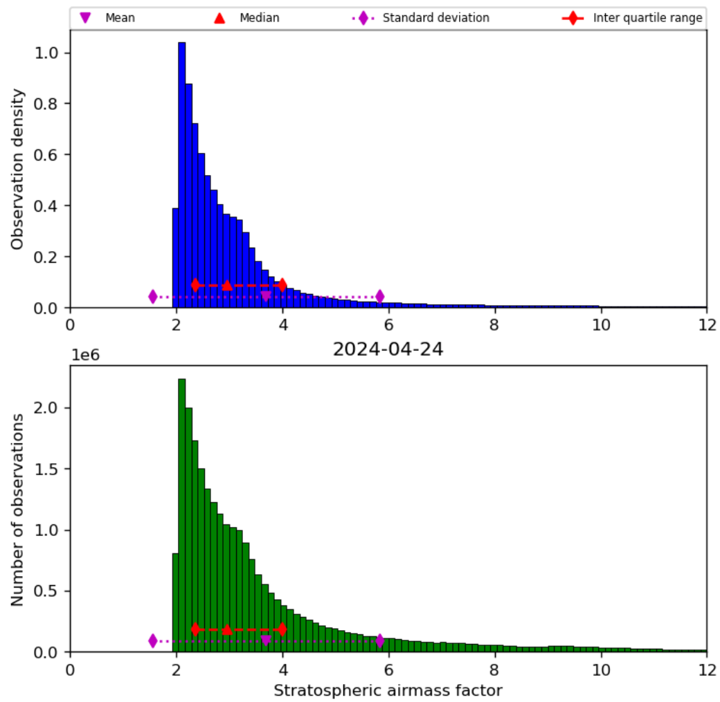
Figure 44: Histogram of “Stratospheric airmass factor” for 2024-04-23 to 2024-04-25
