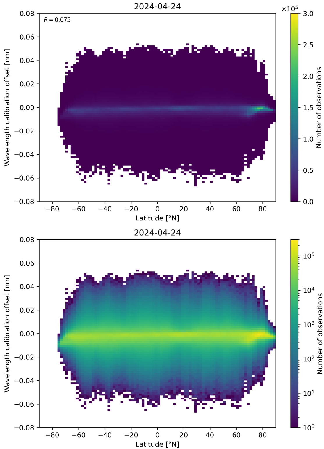
Figure 95: Scatter density plot of “Latitude” against “Wavelength calibration offset” for 2024-04-23 to 2024-04-25.
