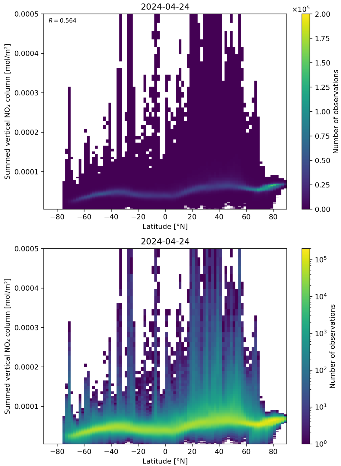
Figure 88: Scatter density plot of “Latitude” against “Summed vertical NO 2 column” for 2024-04-23 to 2024-04-25.
