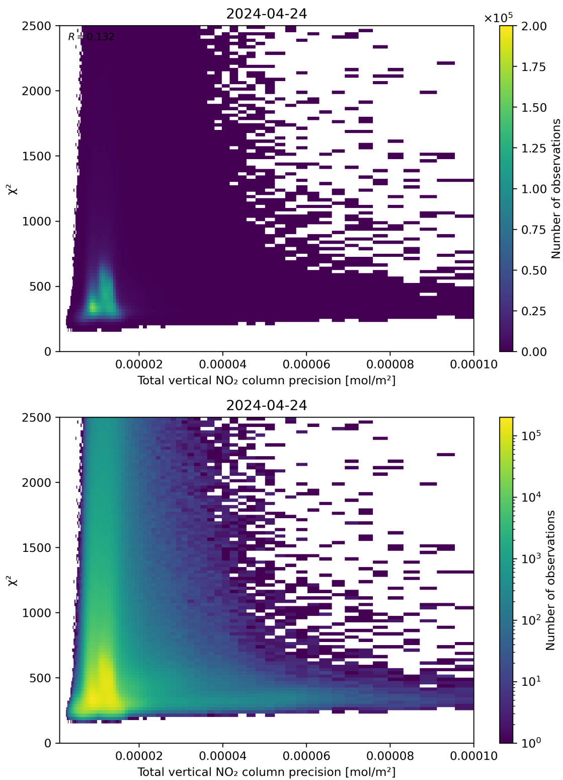
Figure 116: Scatter density plot of “Total vertical NO 2 column precision” against “ \chi^2 ” for 2024-04-23 to 2024-04-25.
