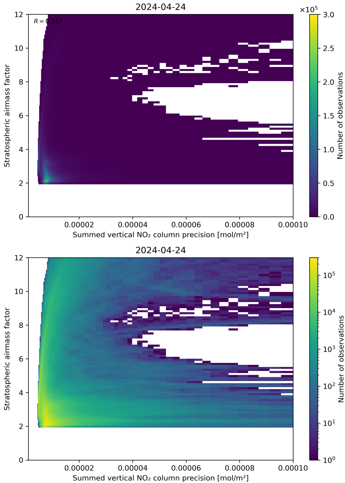
Figure 106: Scatter density plot of “Summed vertical NO 2 column precision” against “Stratospheric airmass factor” for 2024-04-23 to 2024-04-25.
