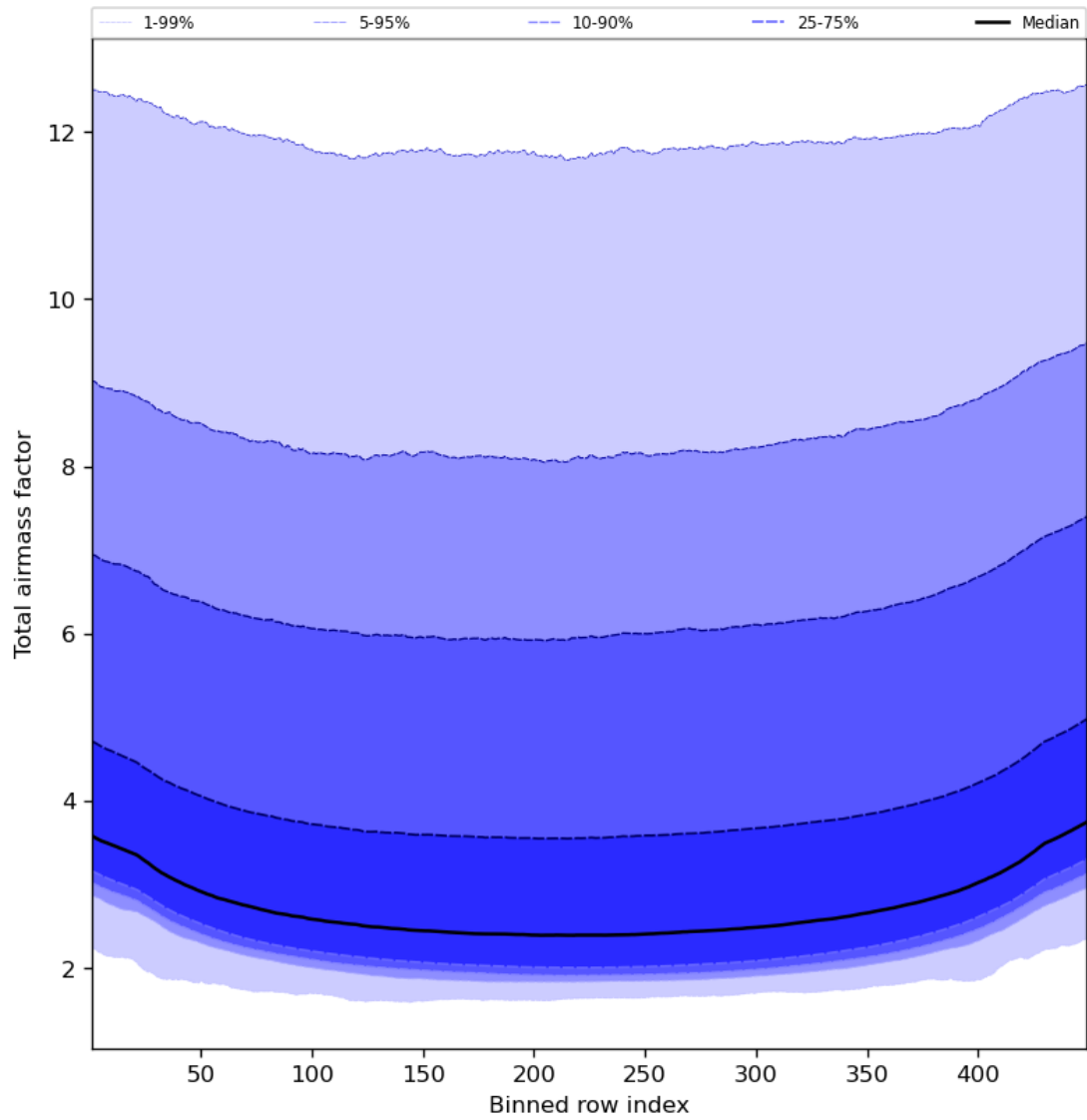
Figure 49: Along track statistics of “Total airmass factor” for 2024-04-23 to 2024-04-25
