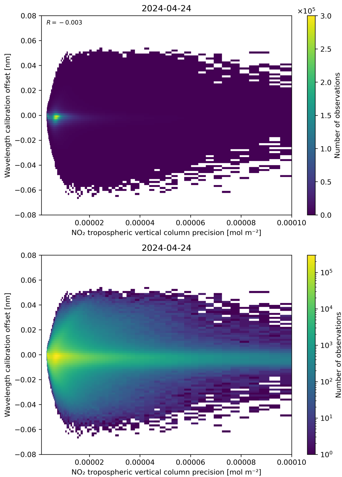
Figure 141: Scatter density plot of “NO 2 tropospheric vertical column precision” against “Wavelength calibration offset” for 2024-04-23 to 2024-04-25.
