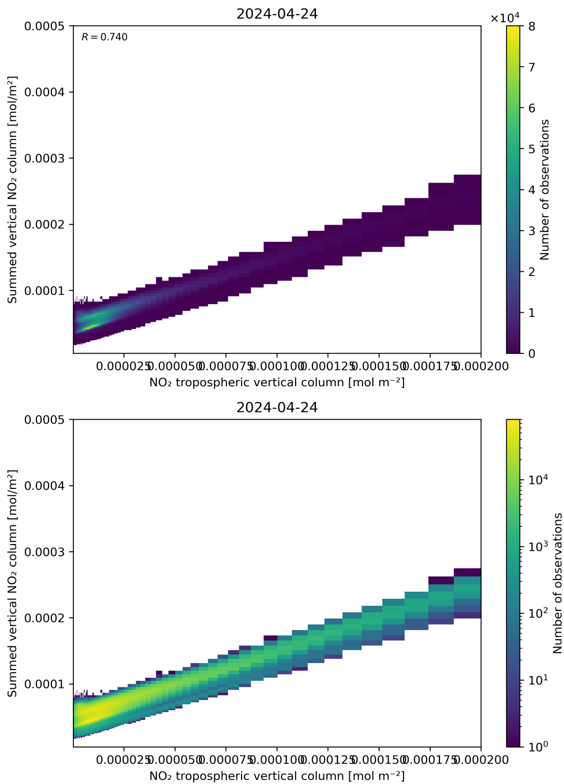
Figure 126: Scatter density plot of “NO 2 tropospheric vertical column” against “Summed vertical NO 2 column” for 2024-04-23 to 2024-04-25.
