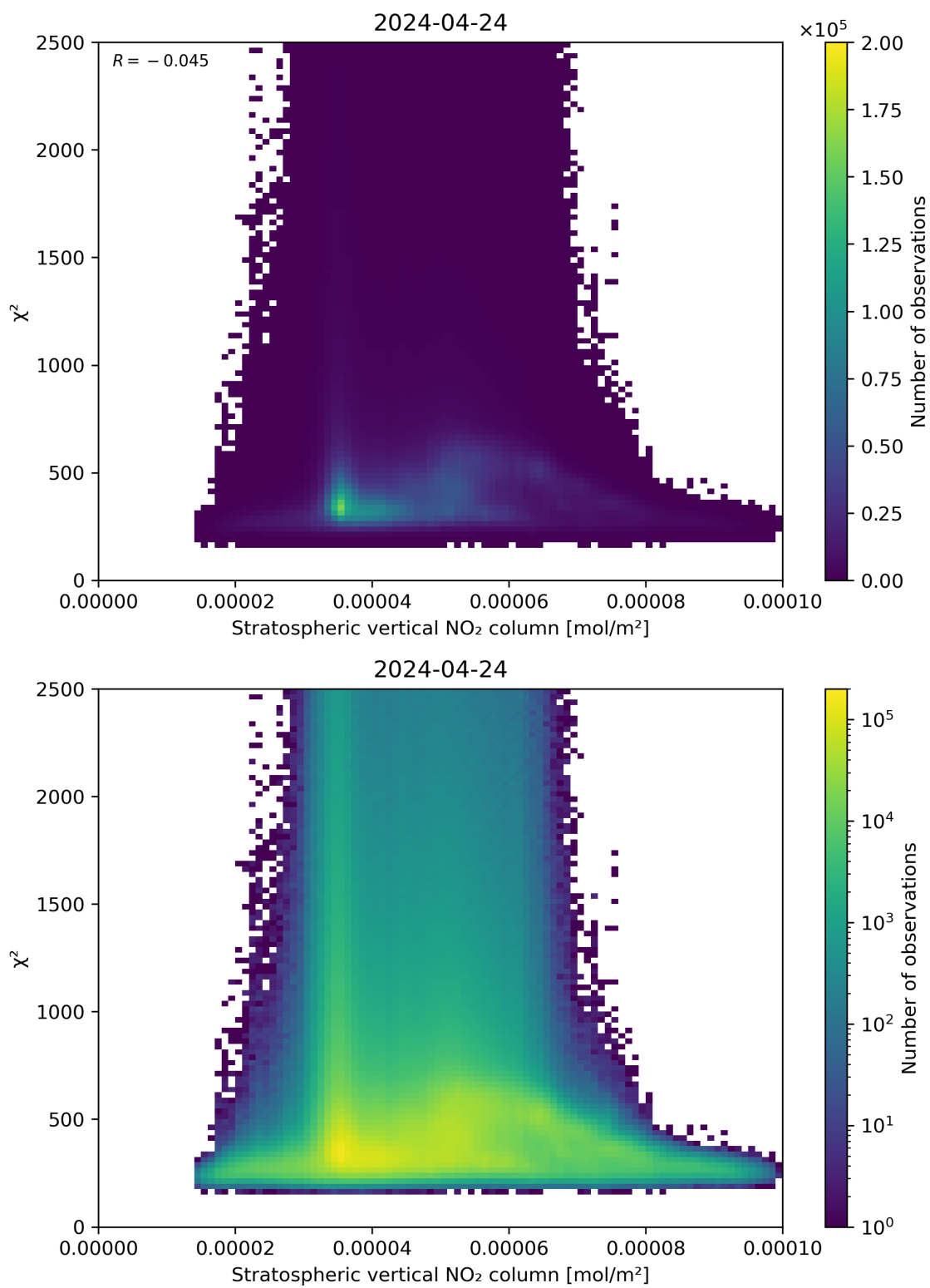
Figure 97: Scatter density plot of “Stratospheric vertical NO 2 column” against “ \chi^2 ” for 2024-04-23 to 2024-04-25.
