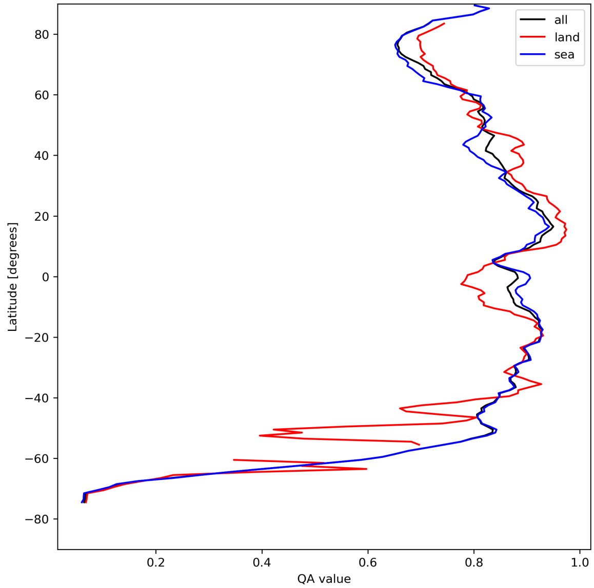
Figure 11: Zonal average of “QA value” for 2024-04-23 to 2024-04-25.
