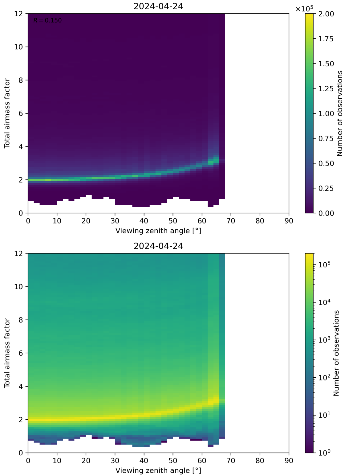
Figure 160: Scatter density plot of “Viewing zenith angle” against “Total airmass factor” for 2024-04-23 to 2024-04-25.
