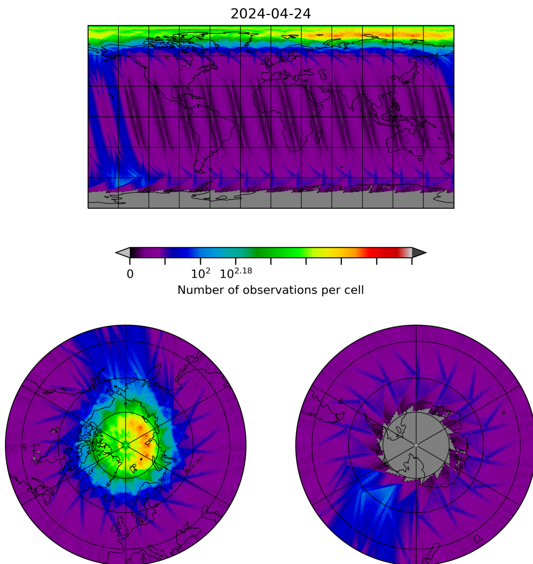
Figure 10: Map of the number of observations for 2024-04-23 to 2024-04-25
