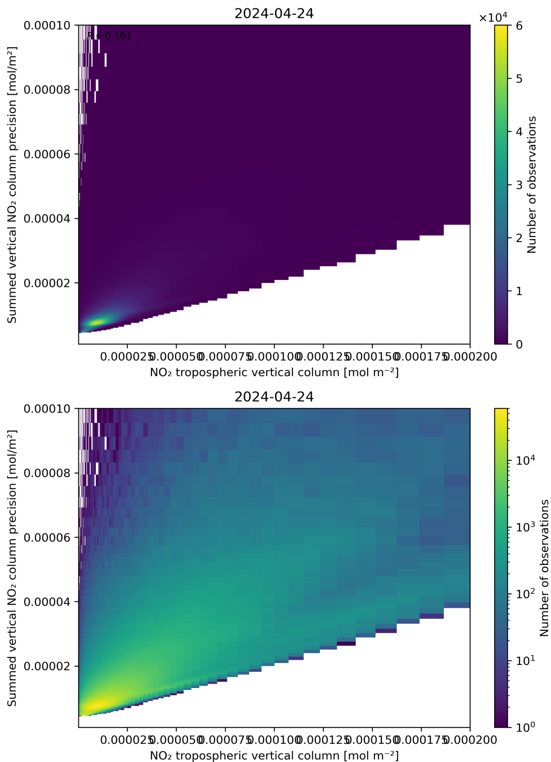
Figure 127: Scatter density plot of “NO 2 tropospheric vertical column” against “Summed vertical NO 2 column precision” for 2024-04-23 to 2024-04-25.
