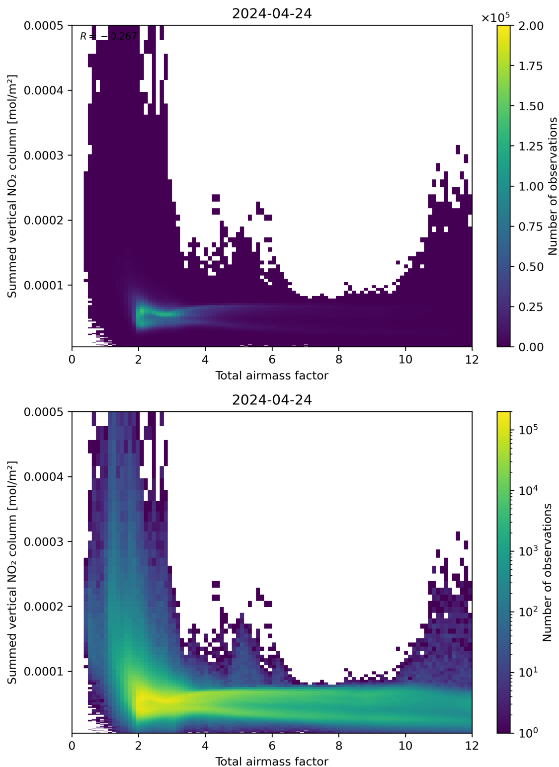
Figure 65: Scatter density plot of “Total airmass factor” against “Summed vertical NO 2 column” for 2024-04-23 to 2024-04-25.
