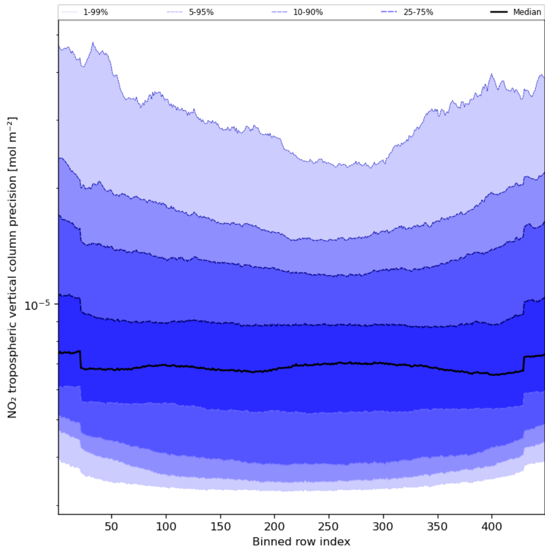
Figure 47: Along track statistics of “NO 2 tropospheric vertical column precision” for 2024-04-23 to 2024-04-25
