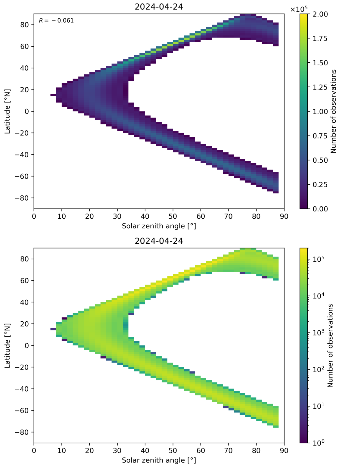
Figure 149: Scatter density plot of “Solar zenith angle” against “Latitude” for 2024-04-23 to 2024-04-25.
