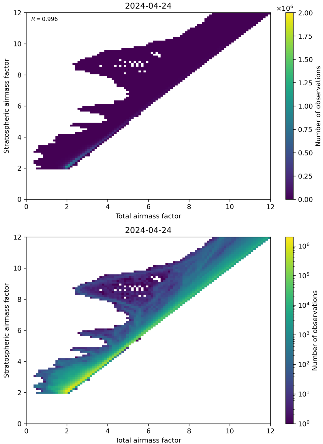
Figure 62: Scatter density plot of “Total airmass factor” against “Stratospheric airmass factor” for 2024-04-23 to 2024-04-25.
