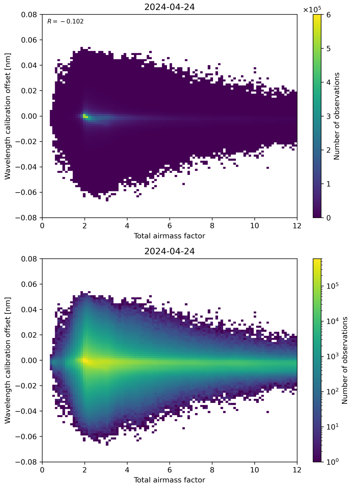
Figure 70: Scatter density plot of “Total airmass factor” against “Wavelength calibration offset” for 2024-04-23 to 2024-04-25.
