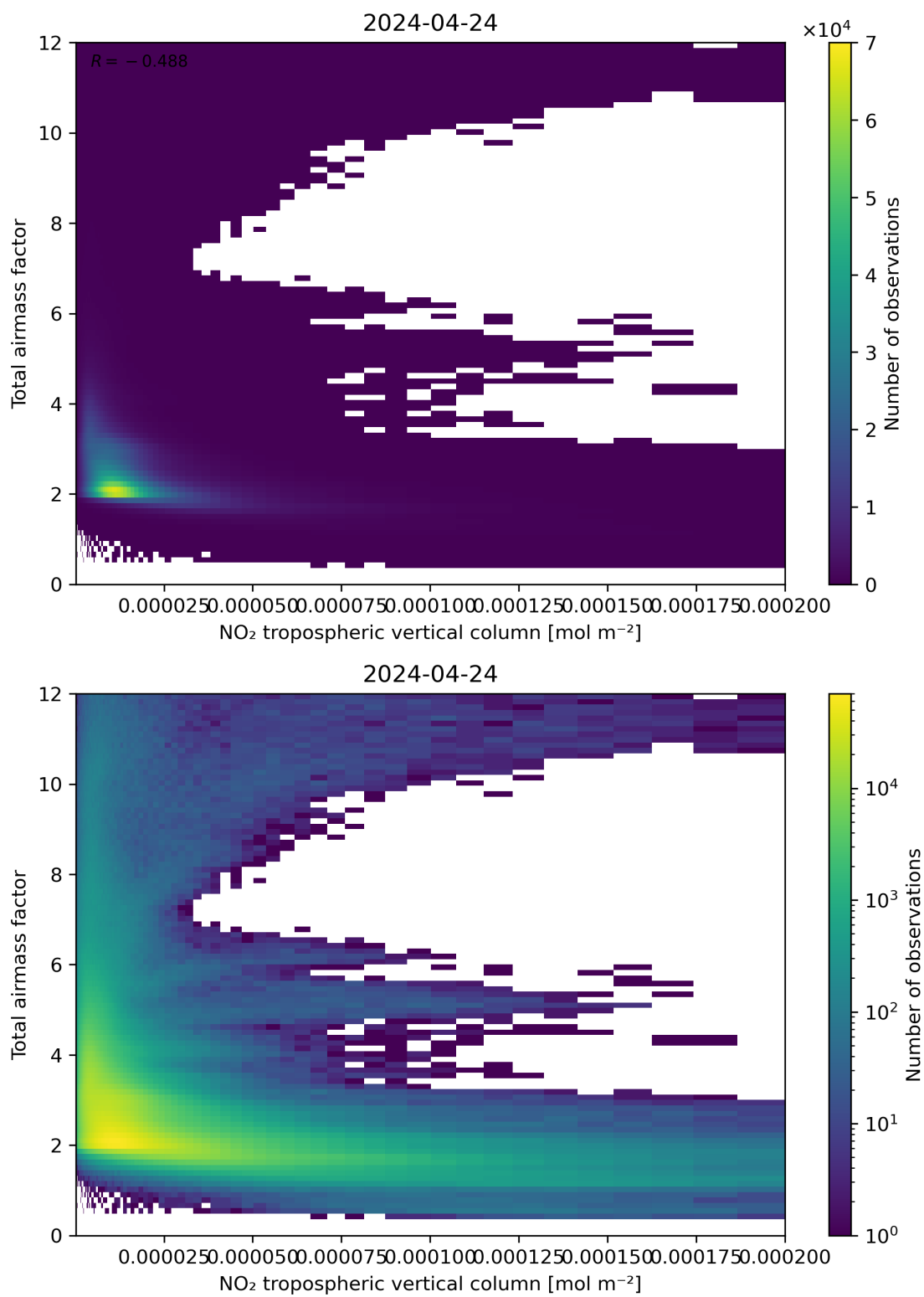
Figure 122: Scatter density plot of “NO 2 tropospheric vertical column” against “Total air mass factor” for 2024-04-23 to 2024-04-25.
