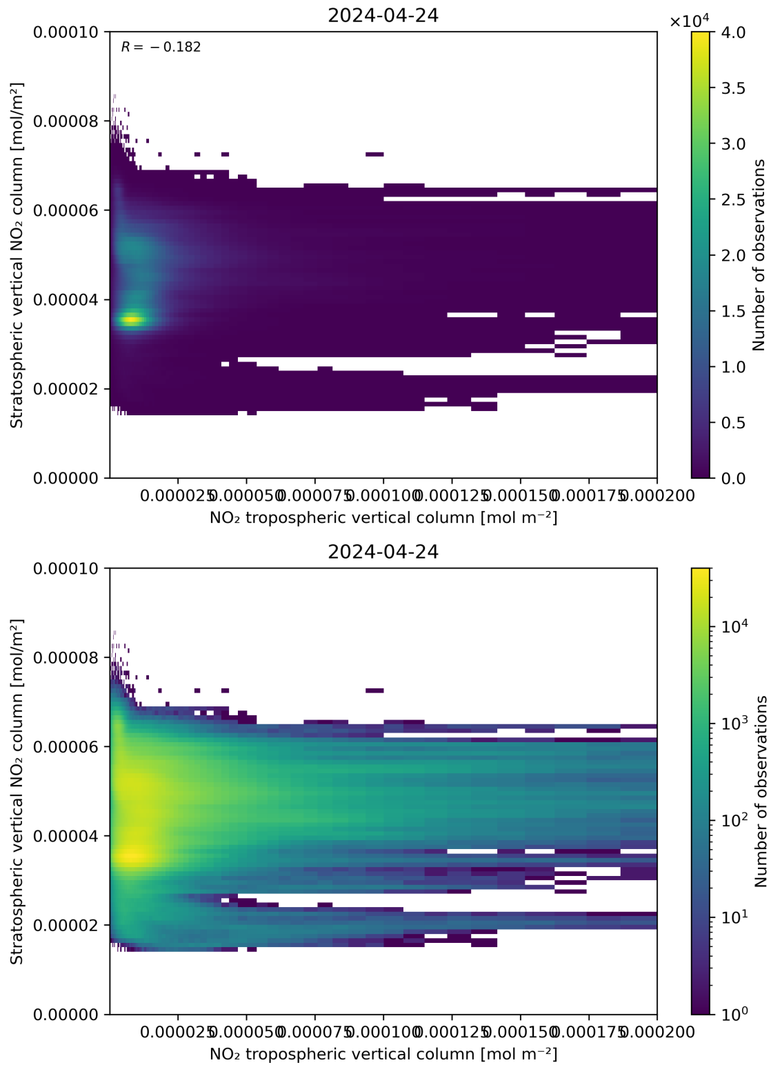
Figure 125: Scatter density plot of “NO 2 tropospheric vertical column” against “Stratospheric vertical NO 2 column” for 2024-04-23 to 2024-04-25.
