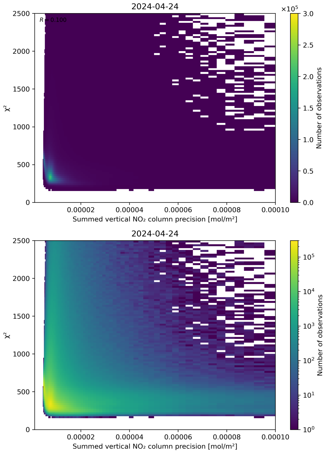
Figure 107: Scatter density plot of “Summed vertical NO 2 column precision” against “ \chi^2 ” for 2024-04-23 to 2024-04-25.
