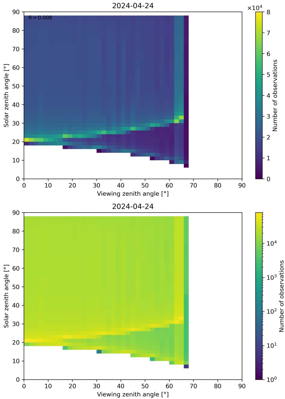
Figure 172: Scatter density plot of “Viewing zenith angle” against “Solar zenith angle” for 2024-04-23 to 2024-04-25.
