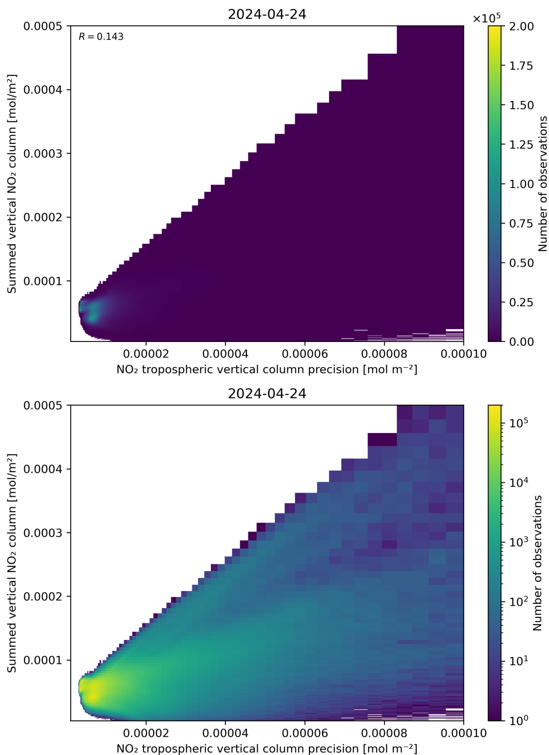
Figure 136: Scatter density plot of “NO 2 tropospheric vertical column precision” against “Summed vertical NO 2 column” for 2024-04-23 to 2024-04-25.
