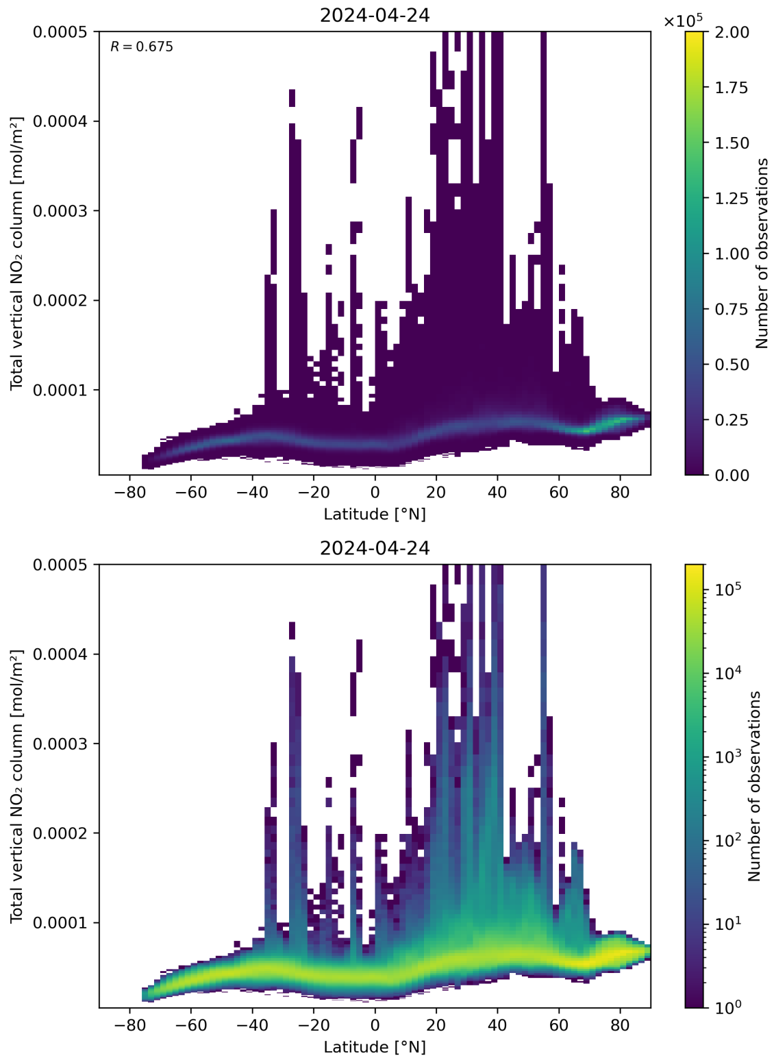
Figure 90: Scatter density plot of “Latitude” against “Total vertical NO 2 column” for 2024-04-23 to 2024-04-25.
