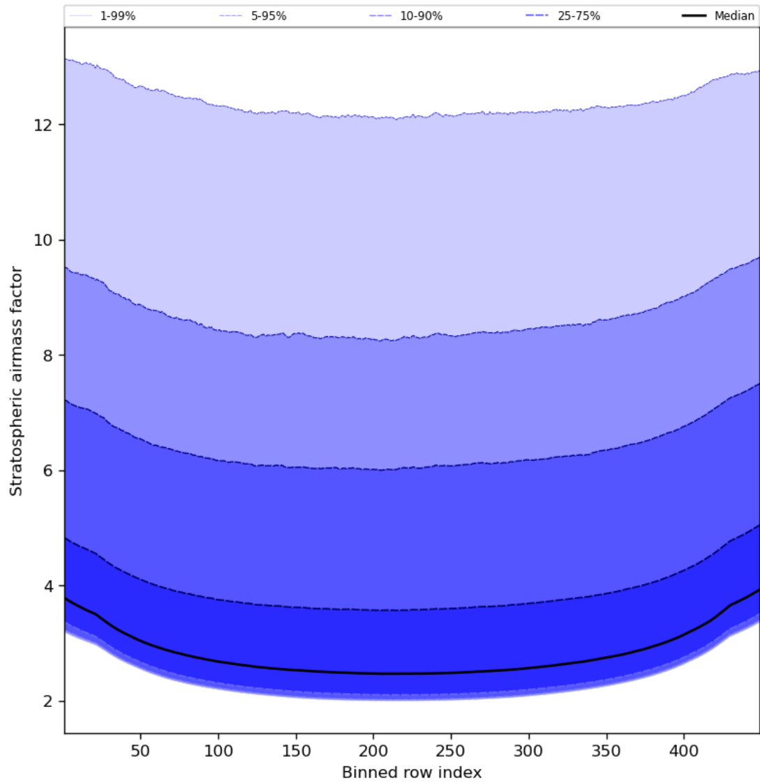
Figure 61: Along track statistics of “Stratospheric airmass factor” for 2024-04-23 to 2024-04-25
