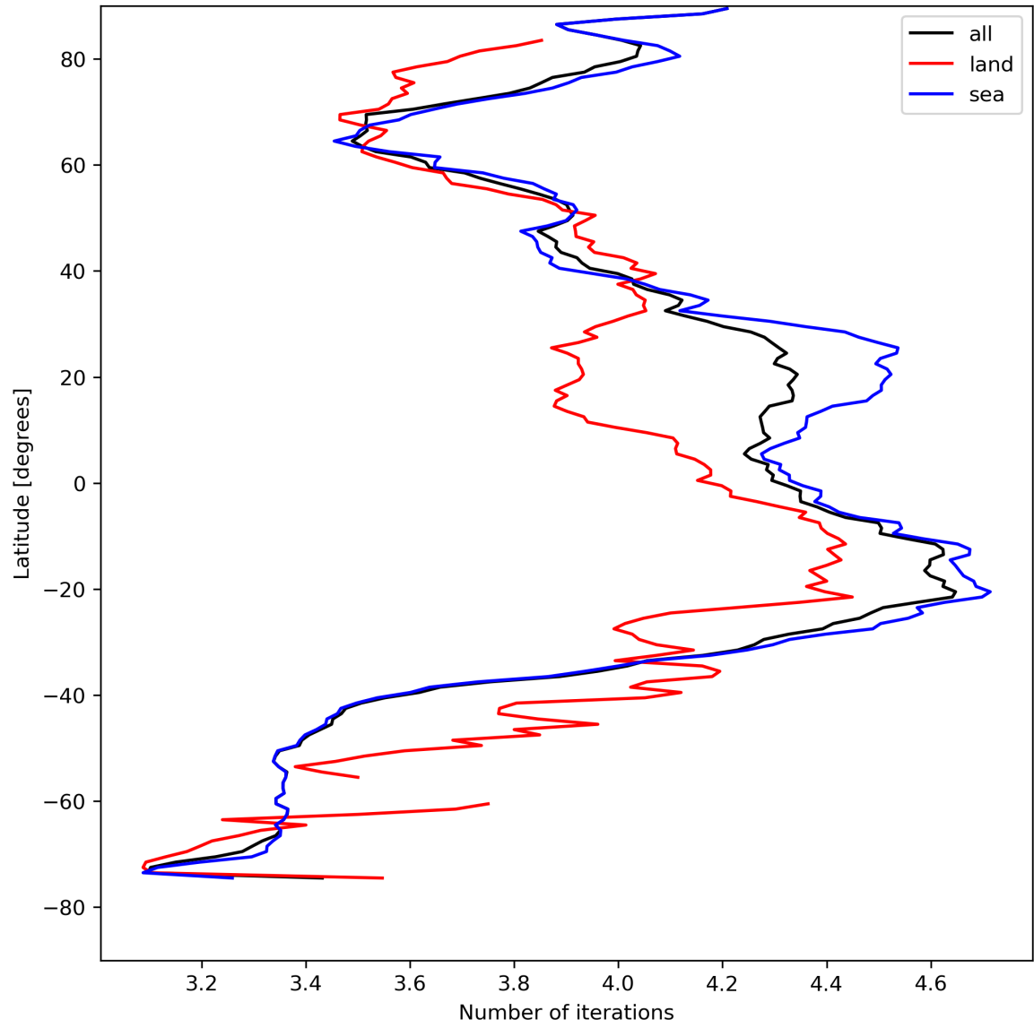
Figure 17: Zonal average of “Number of iterations” for 2024-04-23 to 2024-04-25.
