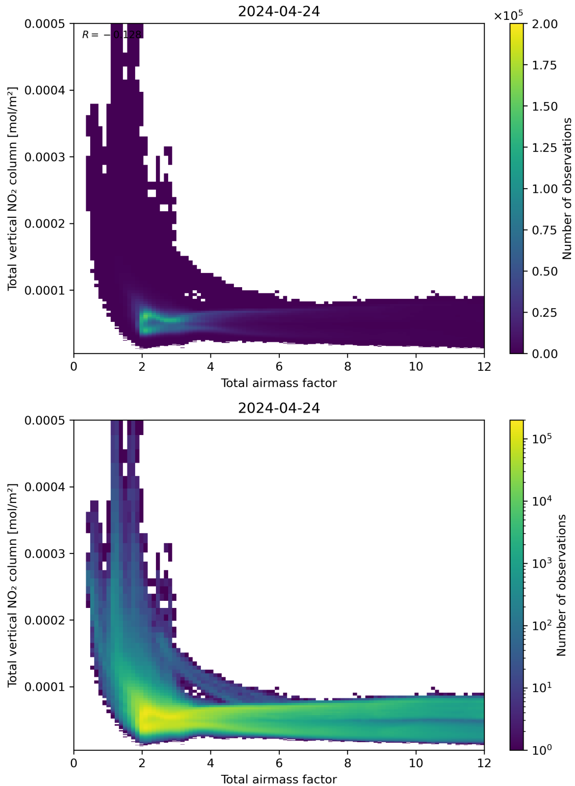
Figure 67: Scatter density plot of “Total airmass factor” against “Total vertical NO 2 column” for 2024-04-23 to 2024-04-25.
