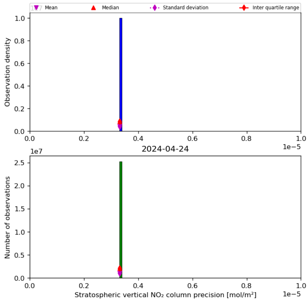
Figure 37: Histogram of “Stratospheric vertical NO 2 column precision” for 2024-04-23 to 2024-04-25
