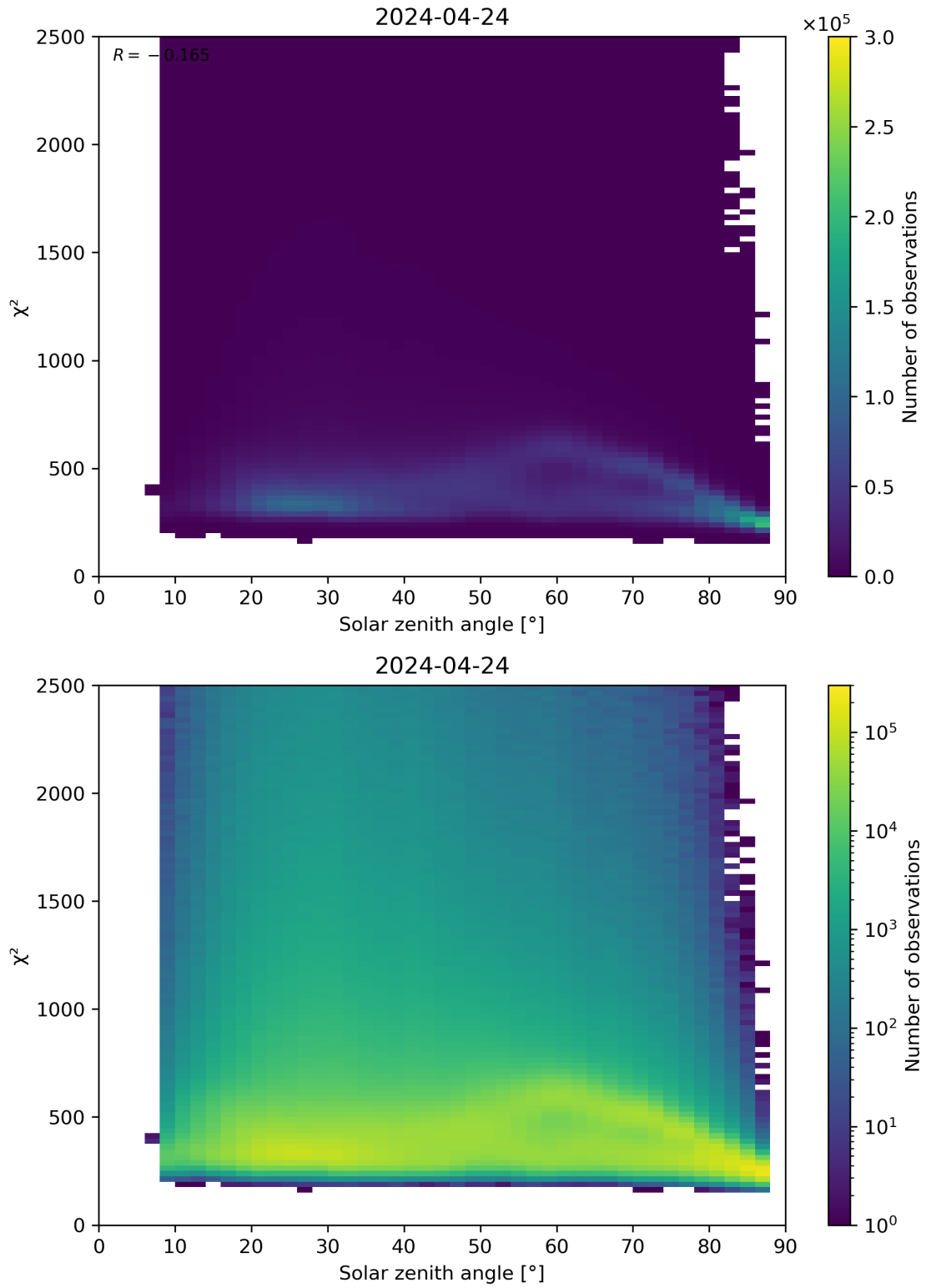
Figure 148: Scatter density plot of “Solar zenith angle” against “ \chi^2 ” for 2024-04-23 to 2024-04-25.
