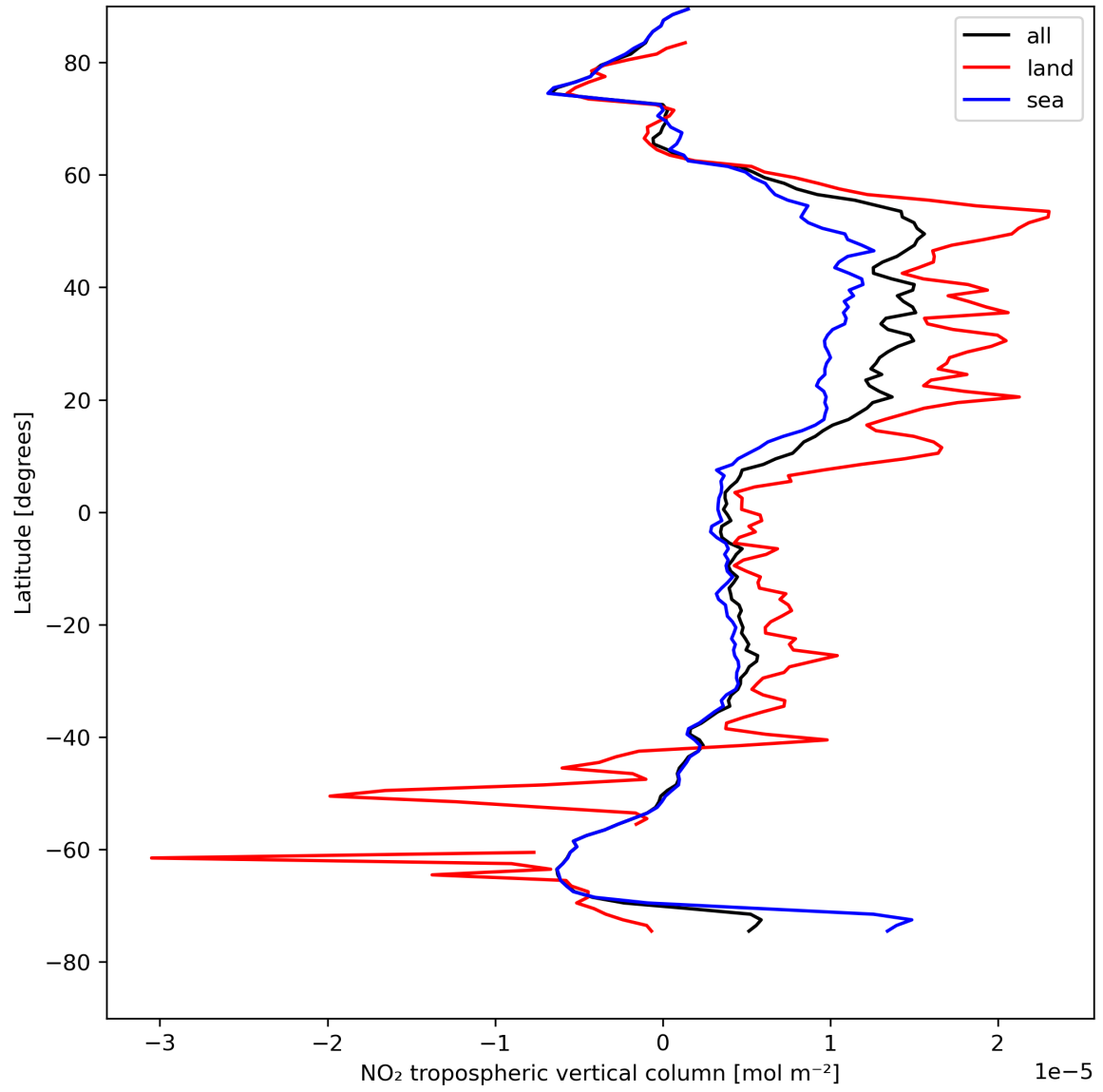
Figure 12: Zonal average of “NO 2 tropospheric vertical column” for 2024-04-23 to 2024-04-25.
