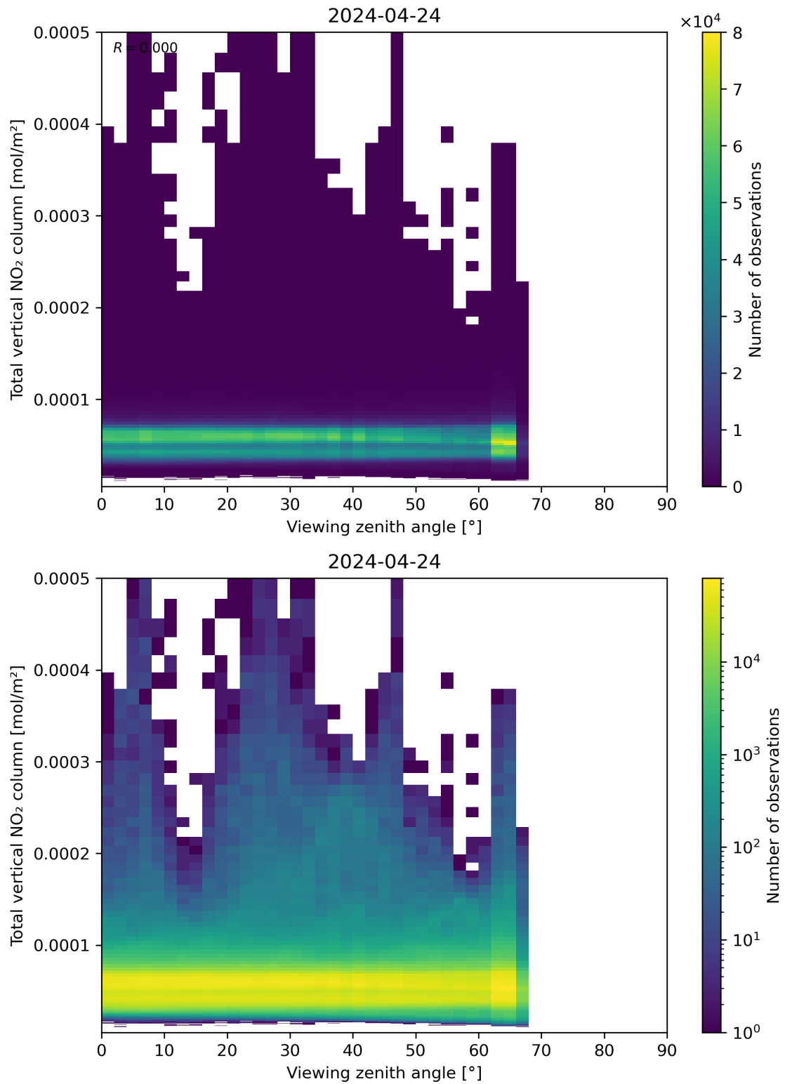
Figure 167: Scatter density plot of “Viewing zenith angle” against “Total vertical NO 2 column” for 2024-04-23 to 2024-04-25.
