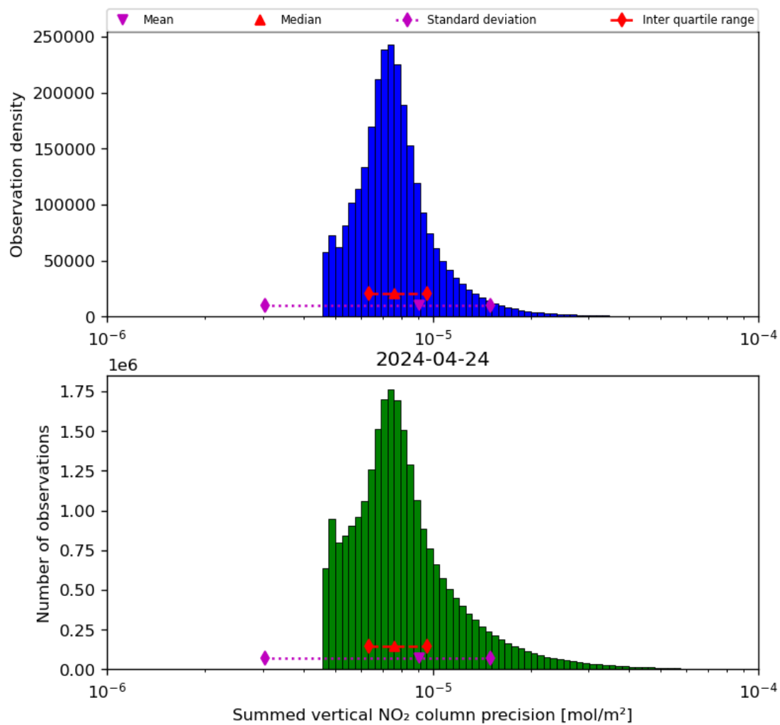
Figure 41: Histogram of “Summed vertical NO 2 column precision” for 2024-04-23 to 2024-04-25
