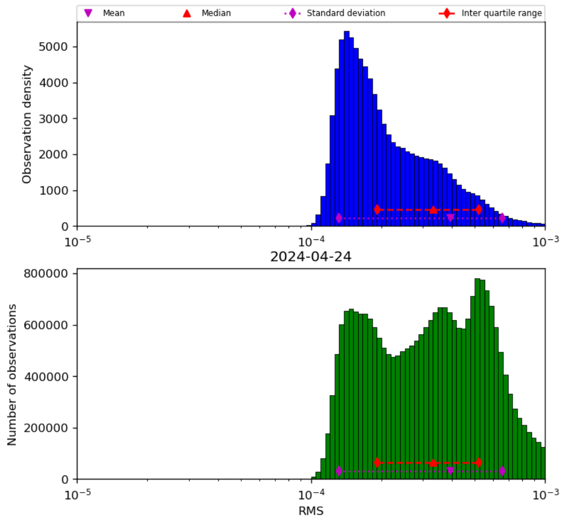
Figure 43: Histogram of “RMS” for 2024-04-23 to 2024-04-25
