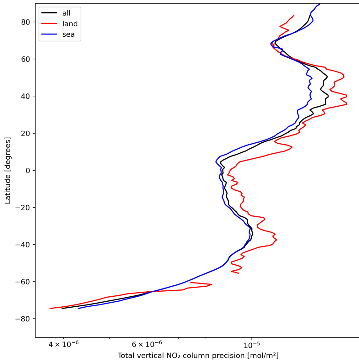
Figure 22: Zonal average of “Total vertical NO 2 column precision” for 2024-04-23 to 2024-04-25.
