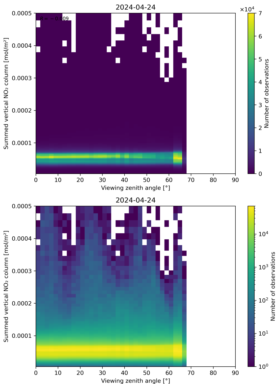
Figure 165: Scatter density plot of “Viewing zenith angle” against “Summed vertical NO 2 column” for 2024-04-23 to 2024-04-25.
