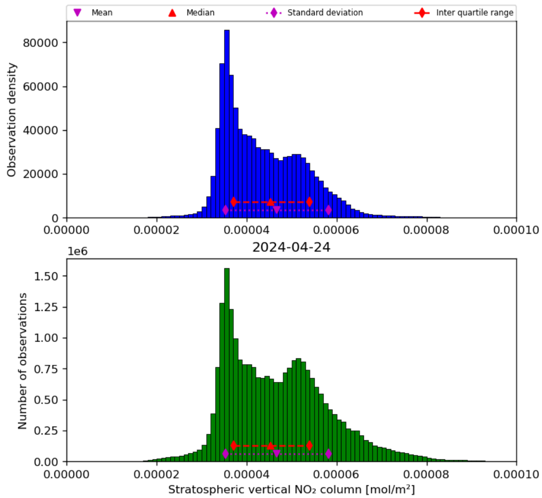
Figure 36: Histogram of “Stratospheric vertical NO 2 column” for 2024-04-23 to 2024-04-25
