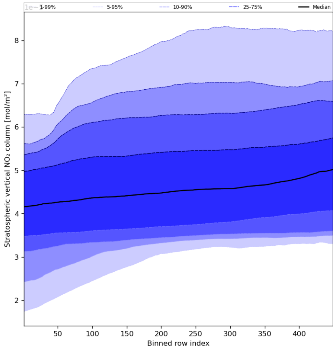
Figure 53: Along track statistics of “Stratospheric vertical NO 2 column” for 2024-04-23 to 2024-04-25
