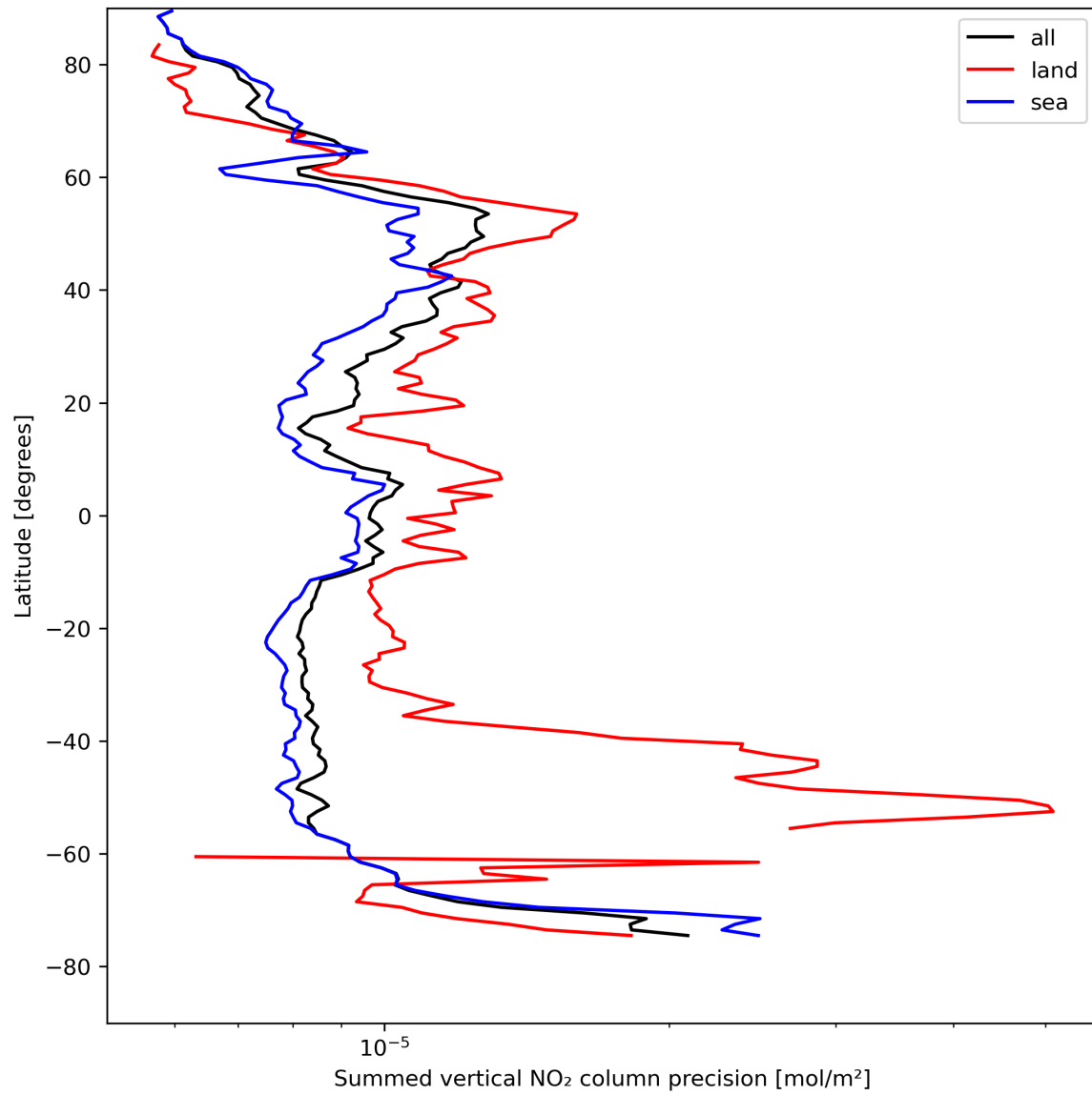
Figure 24: Zonal average of “Summed vertical NO 2 column precision” for 2024-04-23 to 2024-04-25.
