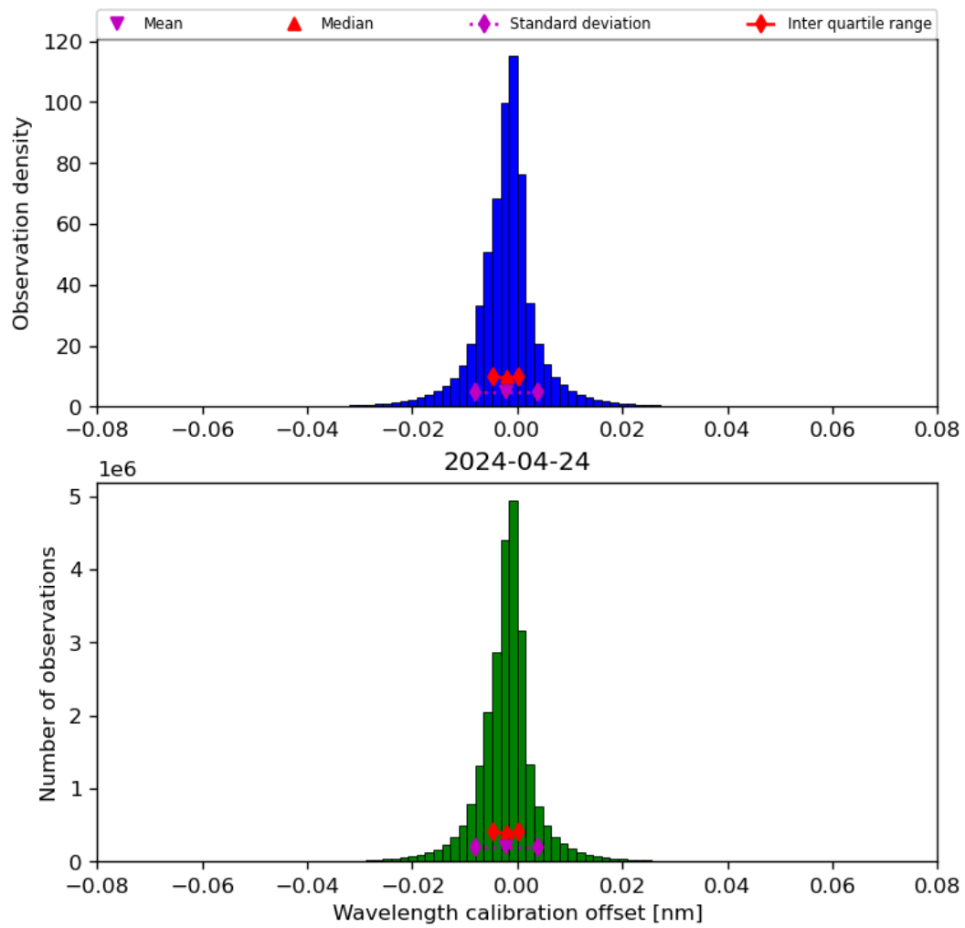
Figure 35: Histogram of “Wavelength calibration offset” for 2024-04-23 to 2024-04-25
