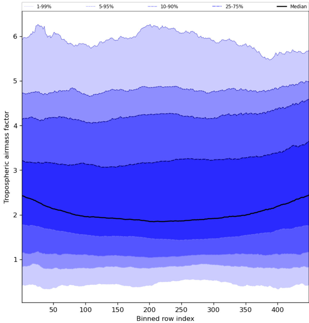
Figure 48: Along track statistics of “Tropospheric air mass factor” for 2024-04-23 to 2024-04-25
