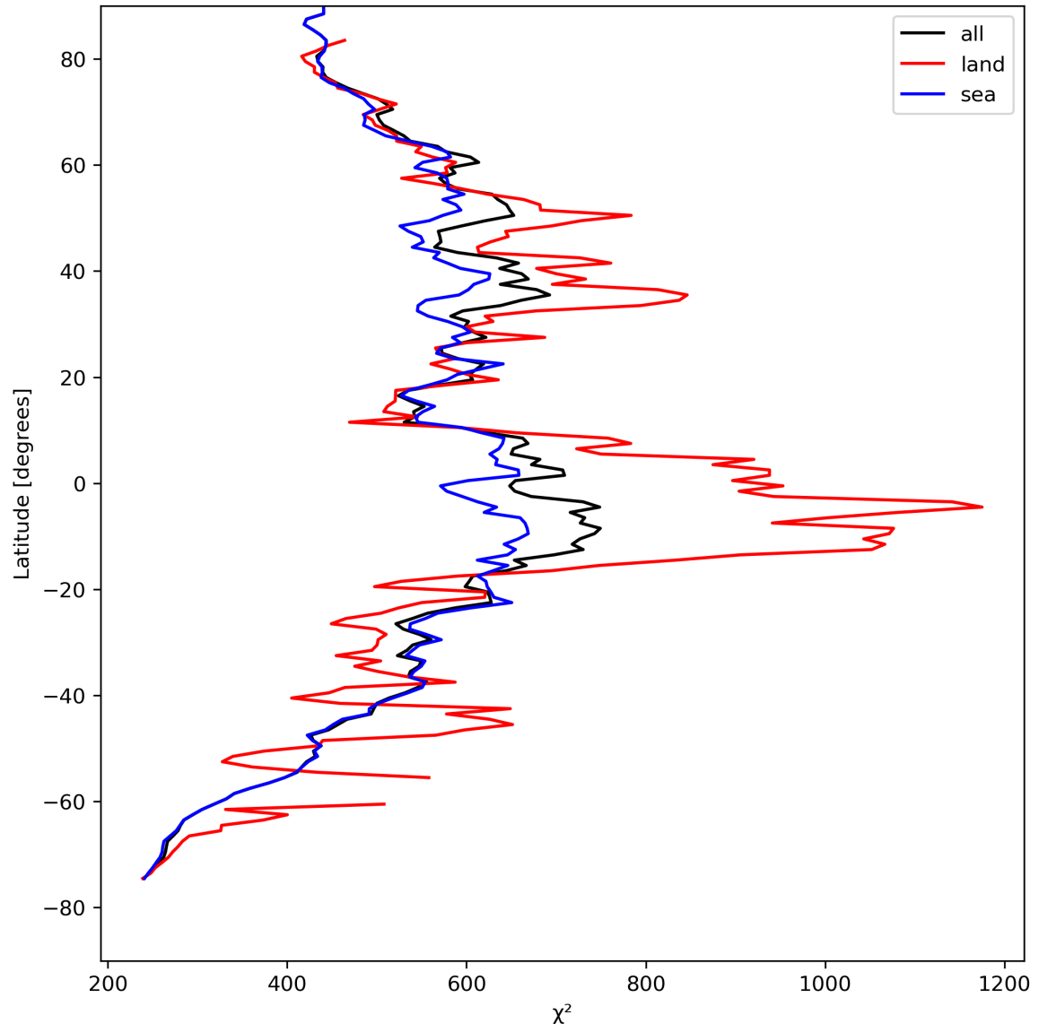
Figure 25: Zonal average of “ \chi^2 ” for 2024-04-23 to 2024-04-25.
