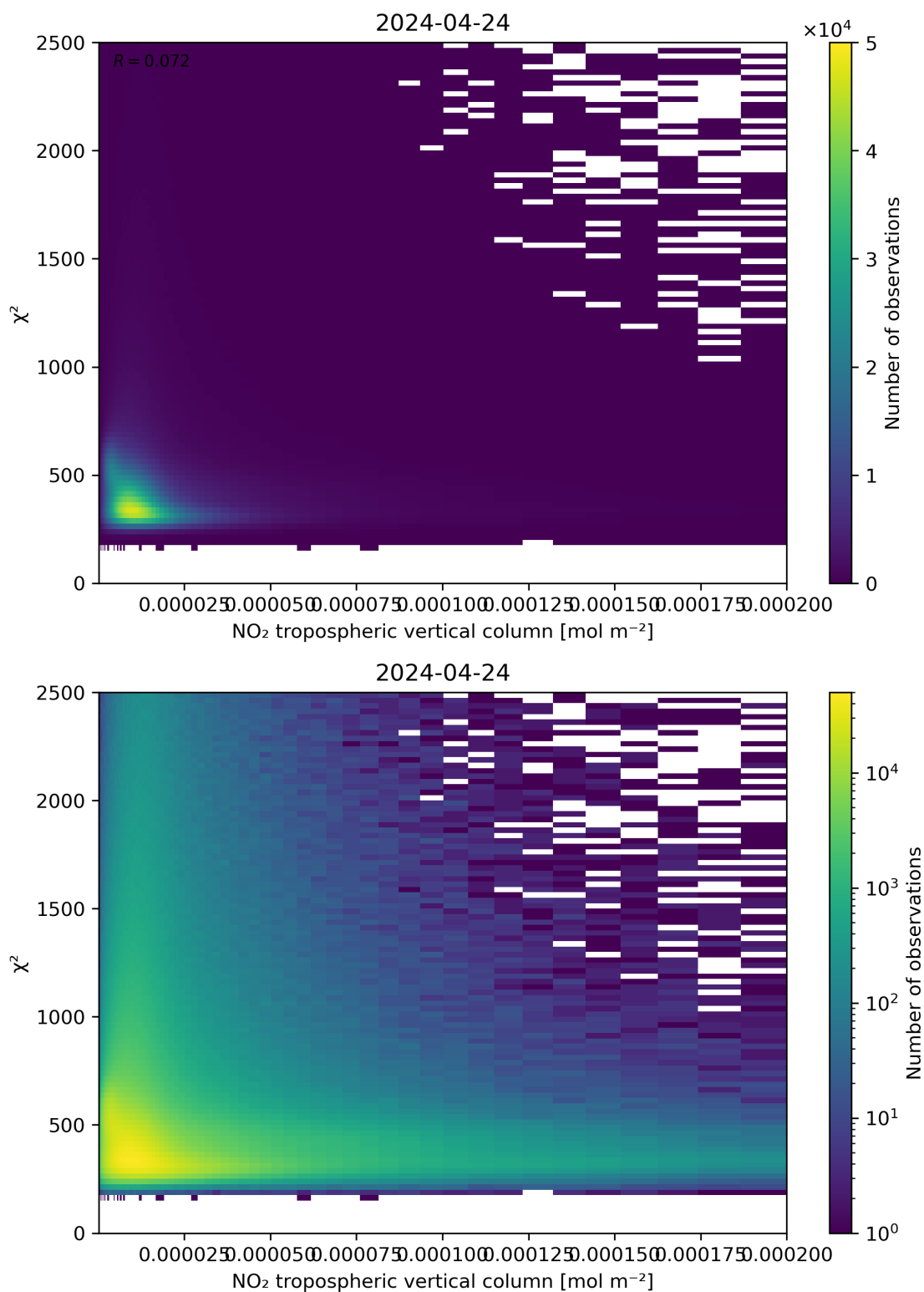
Figure 124: Scatter density plot of “NO 2 tropospheric vertical column” against “ \chi^2 ” for 2024-04-23 to 2024-04-25.
