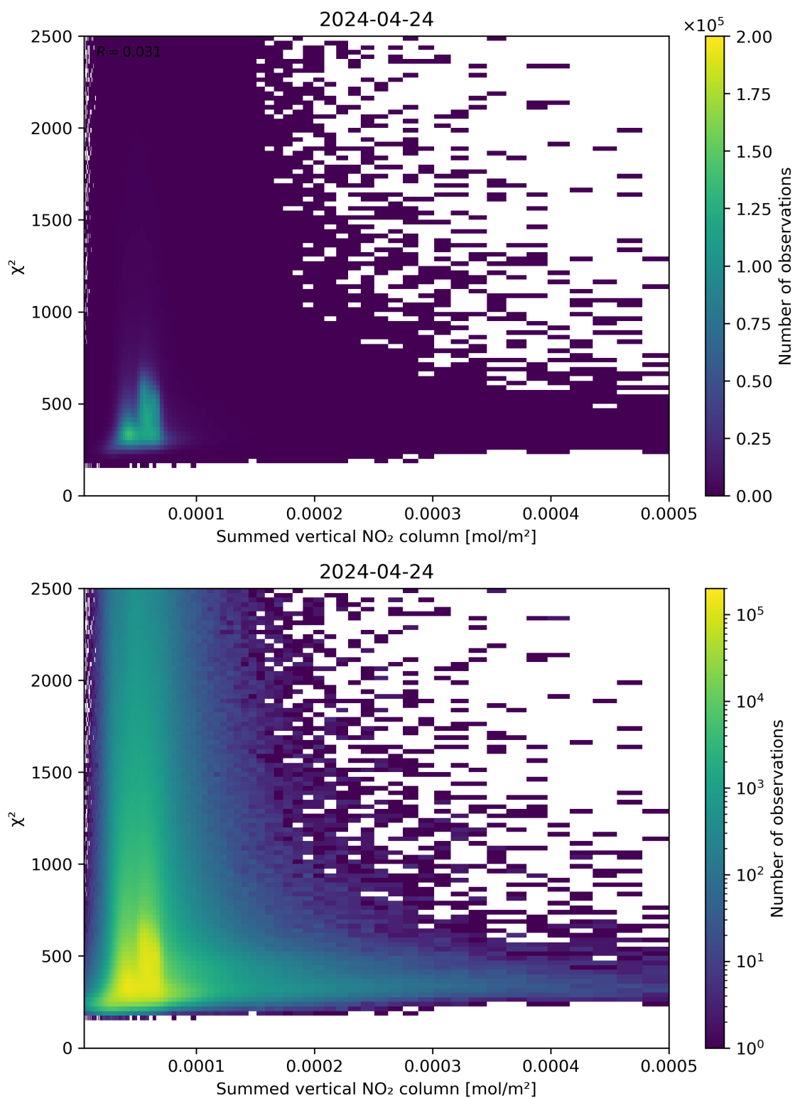
Figure 104: Scatter density plot of “Summed vertical NO 2 column” against “ \chi^2 ” for 2024-04-23 to 2024-04-25.
