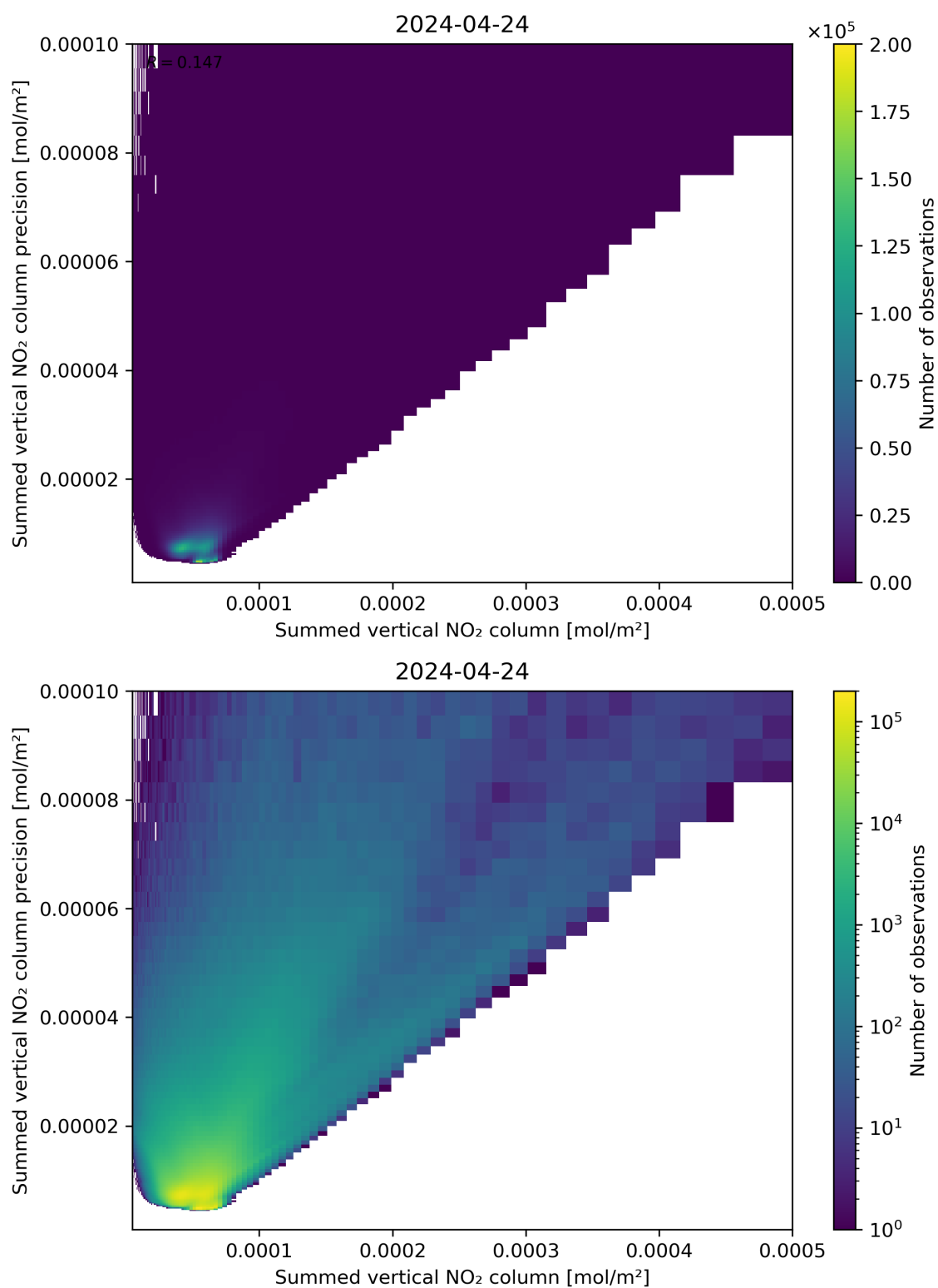
Figure 105: Scatter density plot of “Summed vertical NO 2 column” against “Summed vertical NO 2 column precision” for 2024-04-23 to 2024-04-25.
