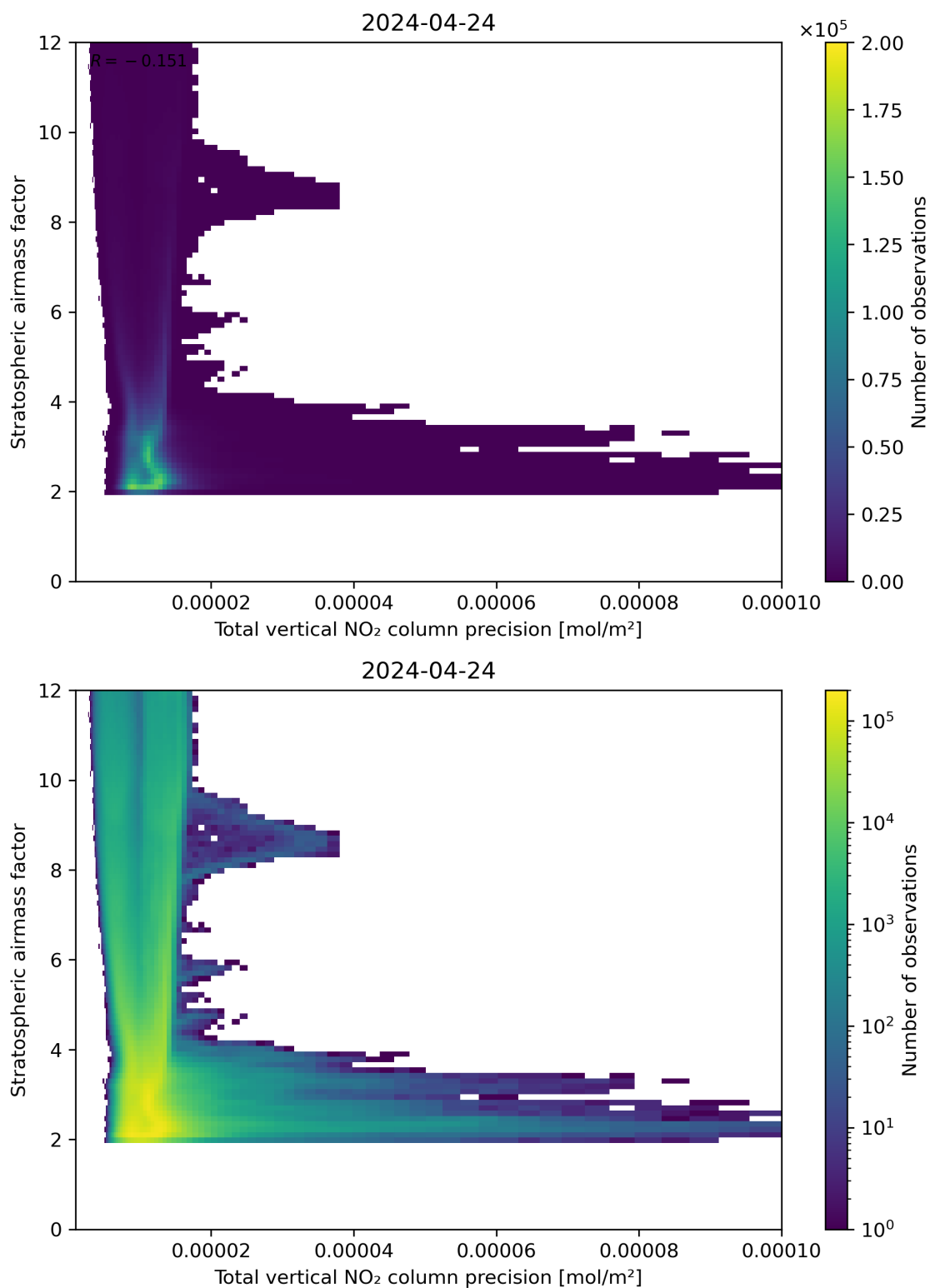
Figure 115: Scatter density plot of “Total vertical NO 2 column precision” against “Stratospheric air mass factor” for 2024-04-23 to 2024-04-25.
