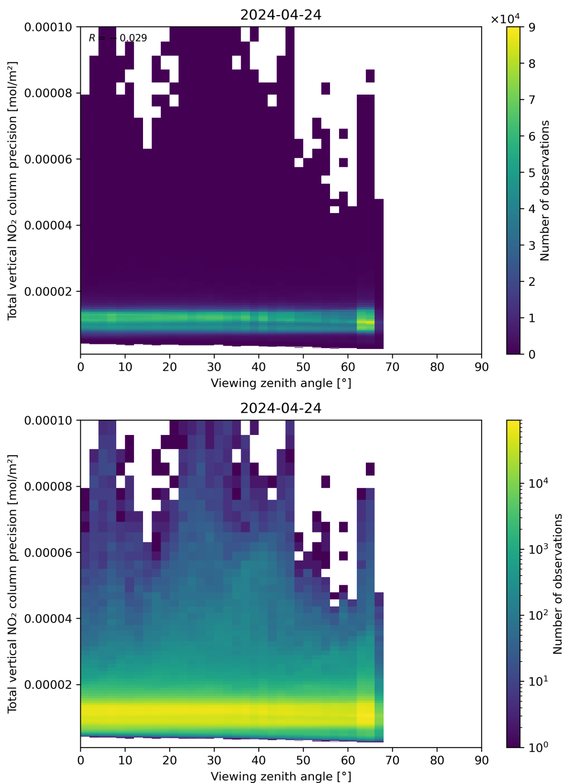
Figure 168: Scatter density plot of “Viewing zenith angle” against “Total vertical NO 2 column precision” for 2024-04-23 to 2024-04-25.
