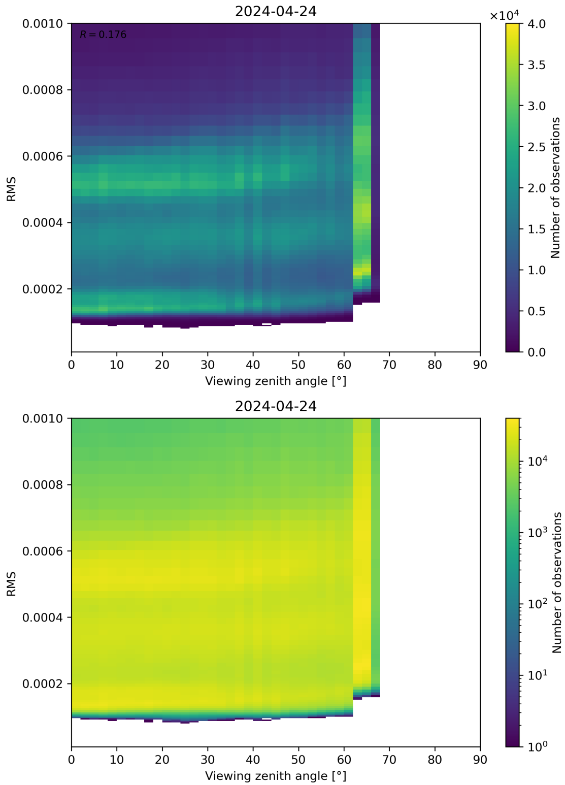
Figure 171: Scatter density plot of “Viewing zenith angle” against “RMS” for 2024-04-23 to 2024-04-25.
