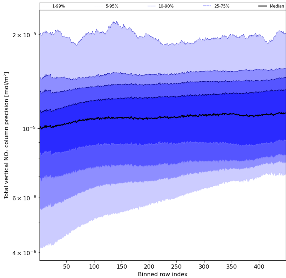
Figure 56: Along track statistics of “Total vertical NO 2 column precision” for 2024-04-23 to 2024-04-25
