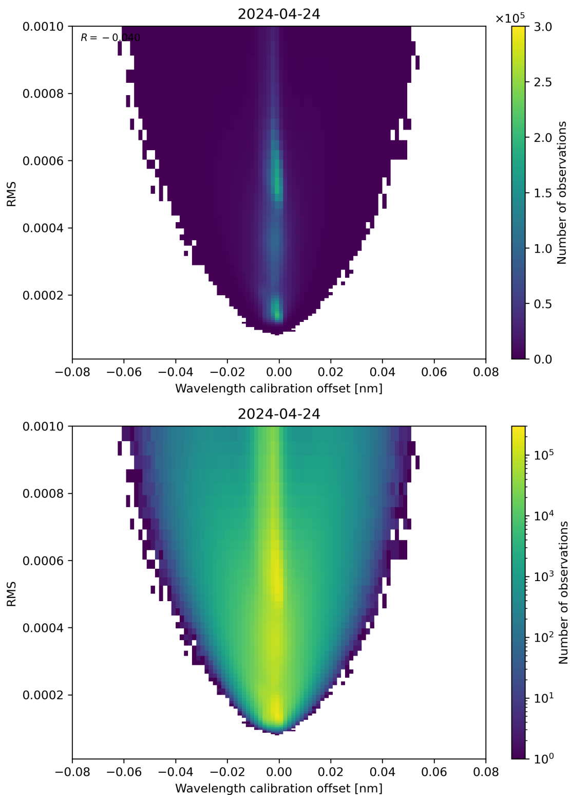
Figure 181: Scatter density plot of “Wavelength calibration offset” against “RMS” for 2024-04-23 to 2024-04-25.
