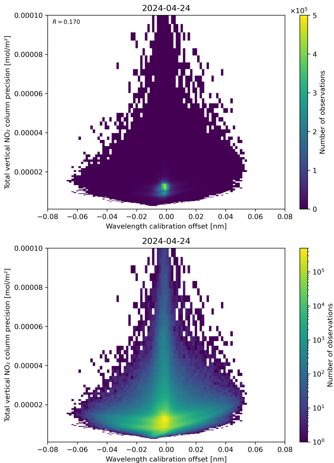
Figure 180: Scatter density plot of “Wavelength calibration offset” against “Total vertical NO 2 column precision” for 2024-04-23 to 2024-04-25.
