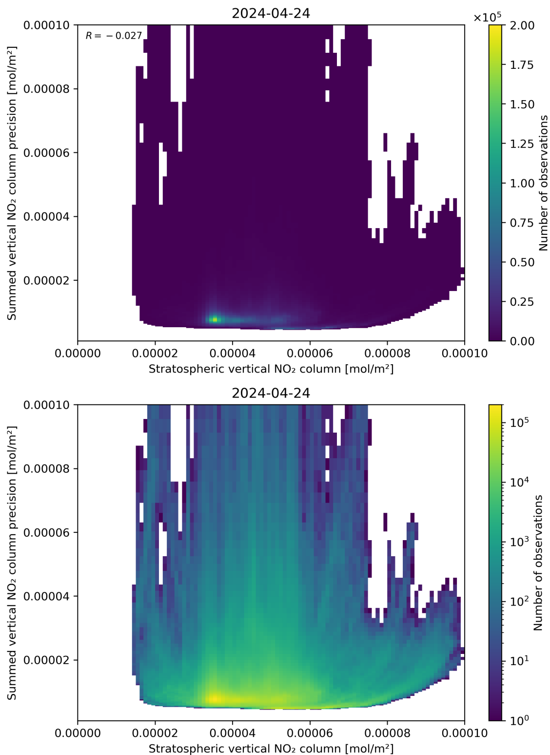
Figure 99: Scatter density plot of “Stratospheric vertical NO 2 column” against “Summed vertical NO 2 column precision” for 2024-04-23 to 2024-04-25.
