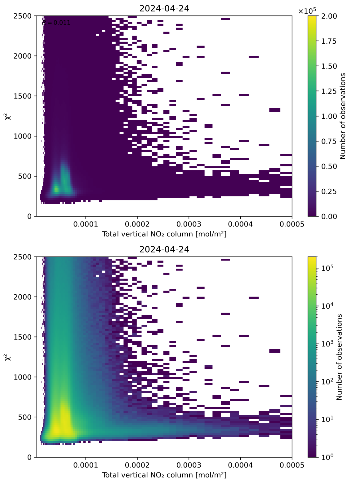
Figure 111: Scatter density plot of “Total vertical NO 2 column” against “ \chi^2 ” for 2024-04-23 to 2024-04-25.
