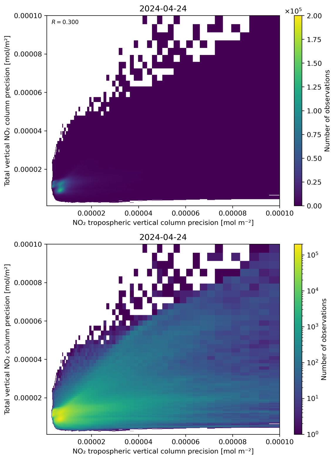
Figure 139: Scatter density plot of “NO 2 tropospheric vertical column precision” against “Total vertical NO 2 column precision” for 2024-04-23 to 2024-04-25.
