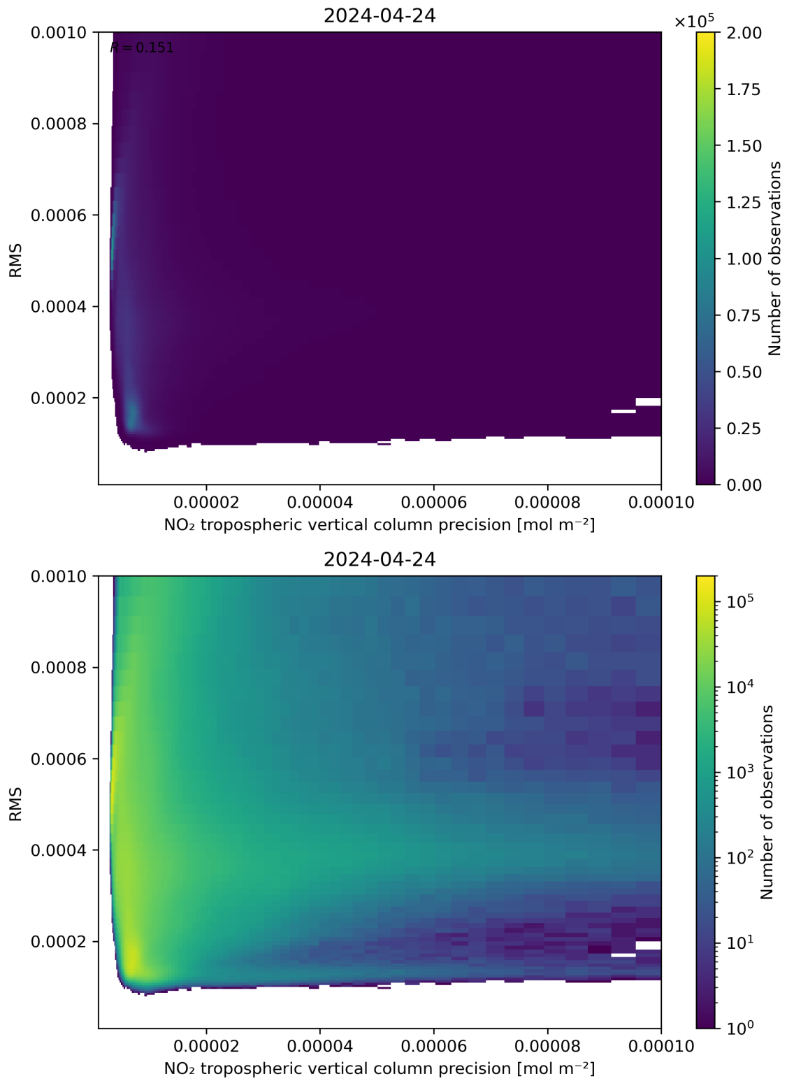
Figure 140: Scatter density plot of “NO 2 tropospheric vertical column precision” against “RMS” for 2024-04-23 to 2024-04-25.
