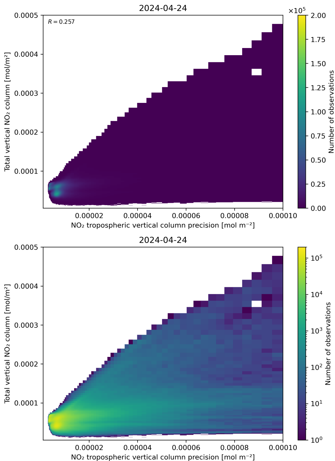
Figure 138: Scatter density plot of “NO 2 tropospheric vertical column precision” against “Total vertical NO 2 column” for 2024-04-23 to 2024-04-25.
