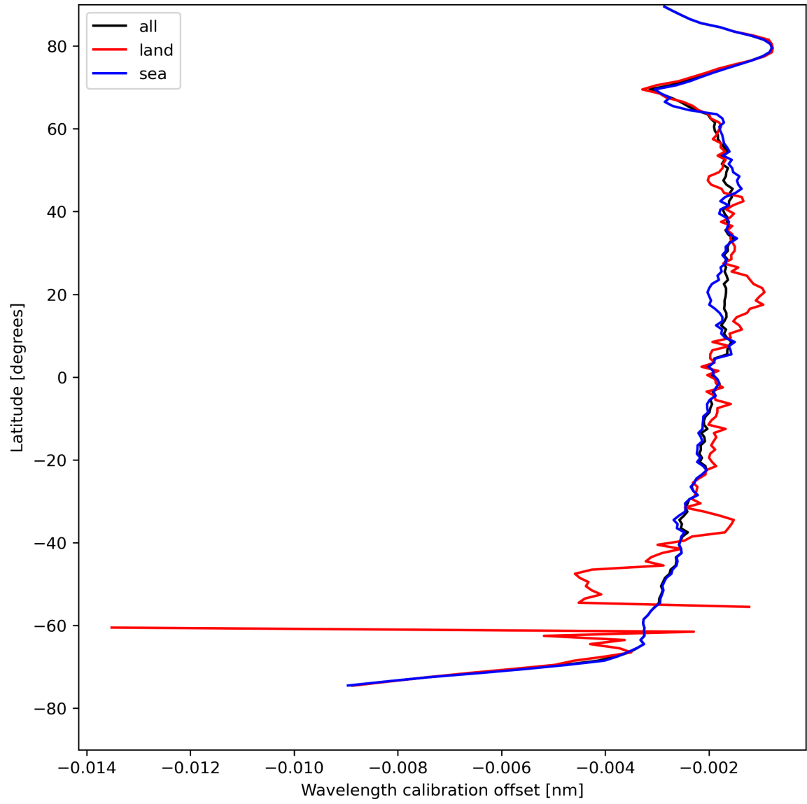
Figure 18: Zonal average of “Wavelength calibration offset” for 2024-04-23 to 2024-04-25.
