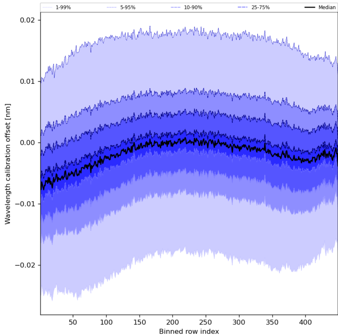
Figure 52: Along track statistics of “Wavelength calibration offset” for 2024-04-23 to 2024-04-25
