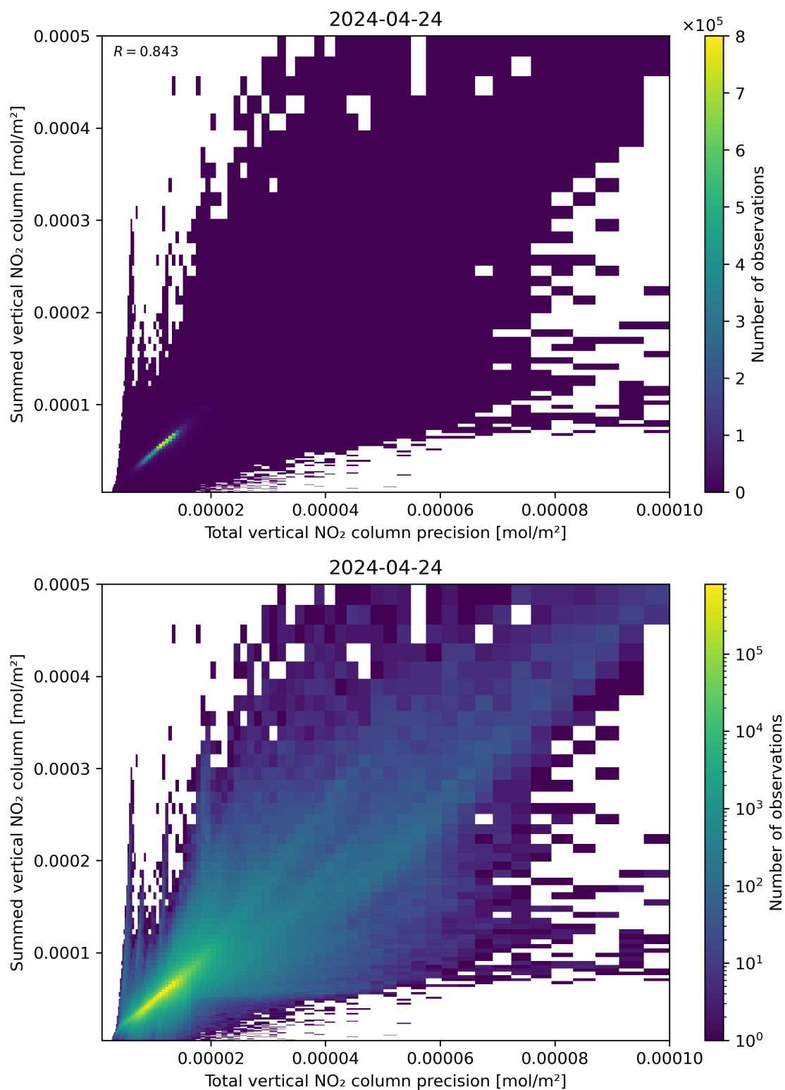
Figure 117: Scatter density plot of “Total vertical NO 2 column precision” against “Summed vertical NO 2 column” for 2024-04-23 to 2024-04-25.
