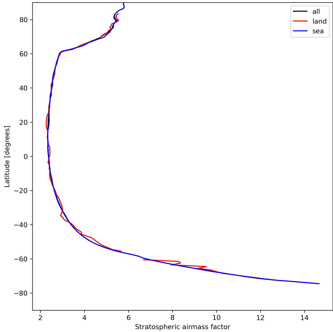
Figure 27: Zonal average of “Stratospheric air mass factor” for 2024-04-23 to 2024-04-25.
