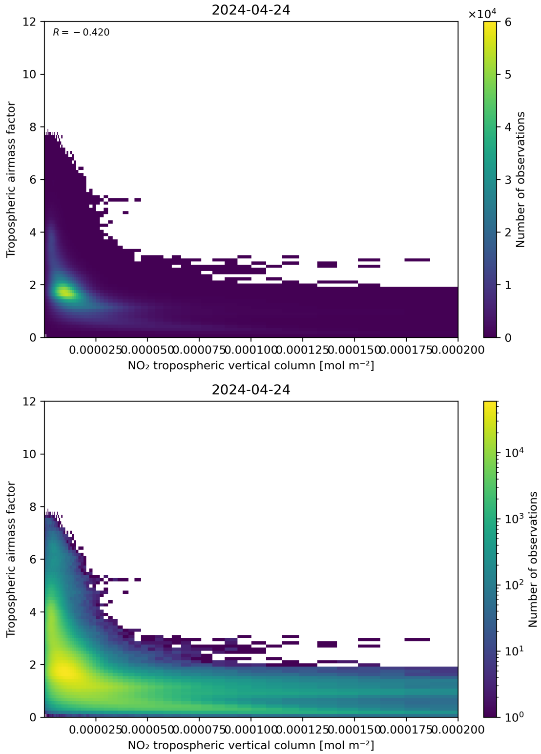
Figure 123: Scatter density plot of “NO 2 tropospheric vertical column” against “Tropospheric air mass factor” for 2024-04-23 to 2024-04-25.
