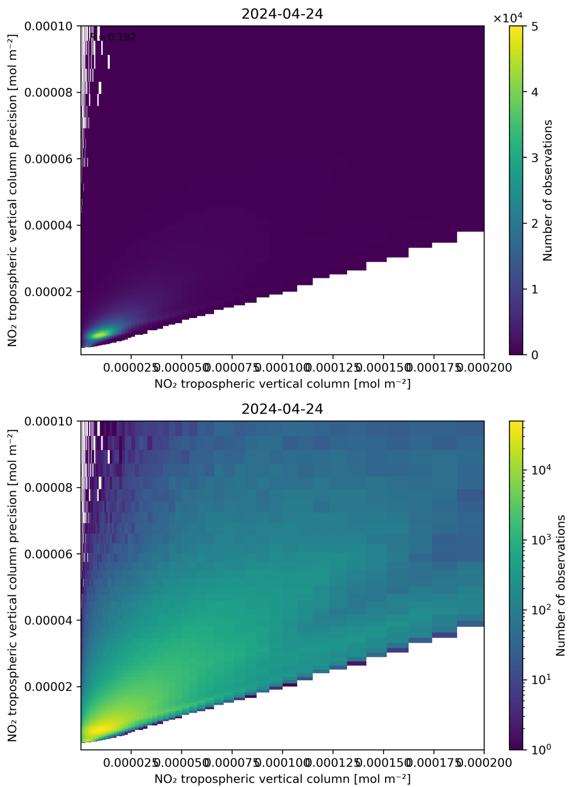
Figure 130: Scatter density plot of “NO 2 tropospheric vertical column” against “NO 2 tropospheric vertical column precision” for 2024-04-23 to 2024-04-25.
