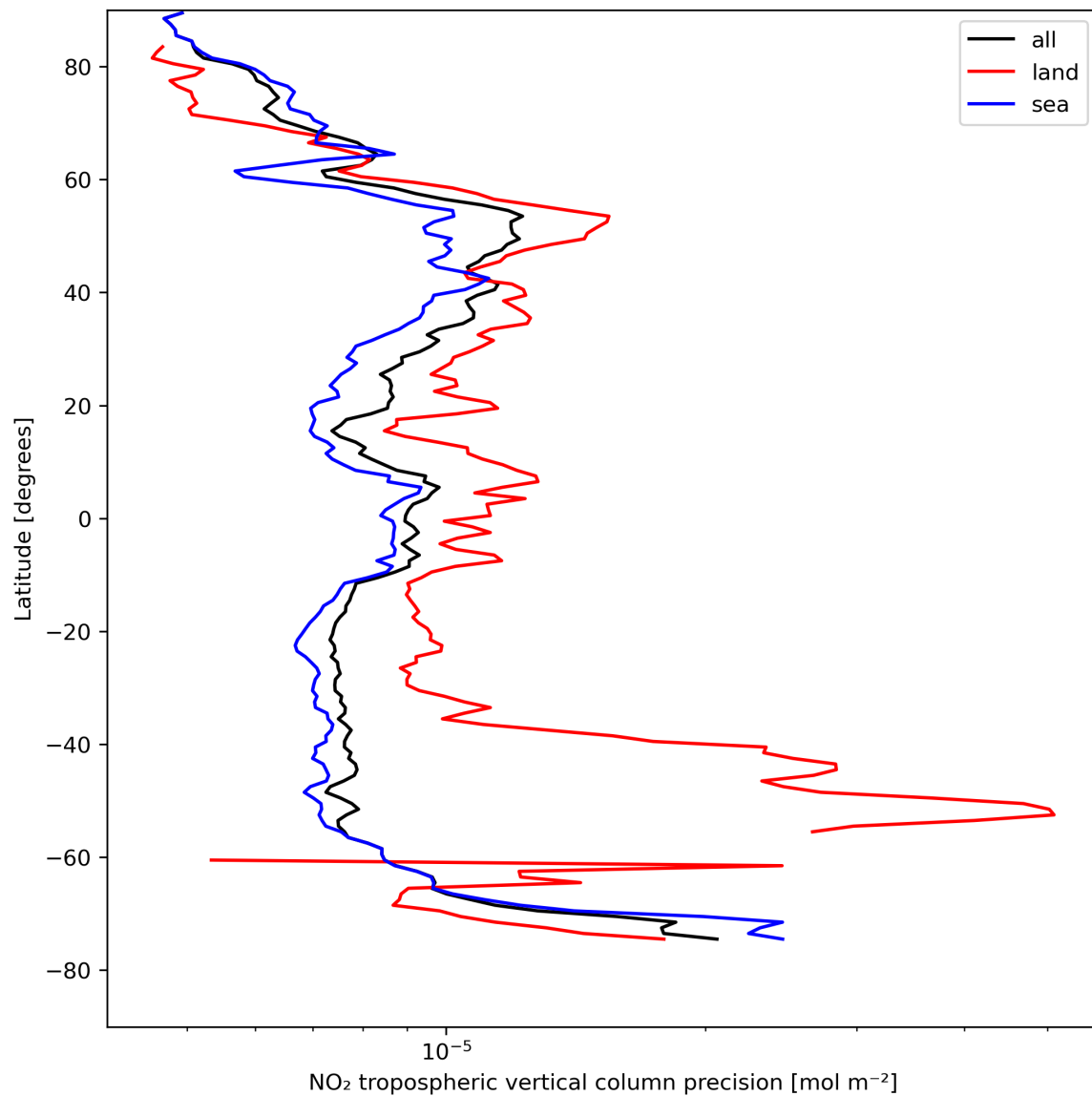
Figure 13: Zonal average of “NO 2 tropospheric vertical column precision” for 2024-04-23 to 2024-04-25.
