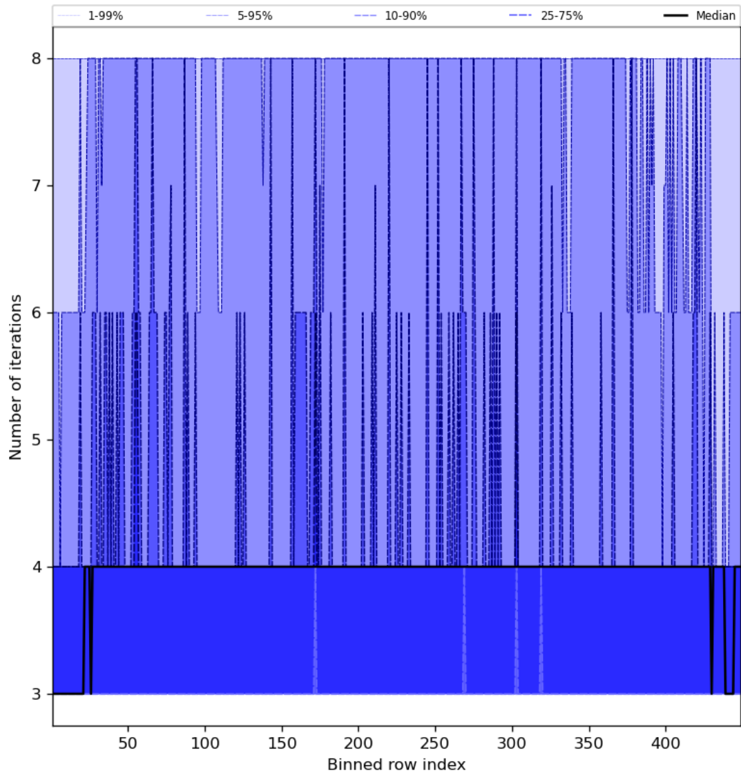
Figure 51: Along track statistics of “Number of iterations” for 2024-04-23 to 2024-04-25
