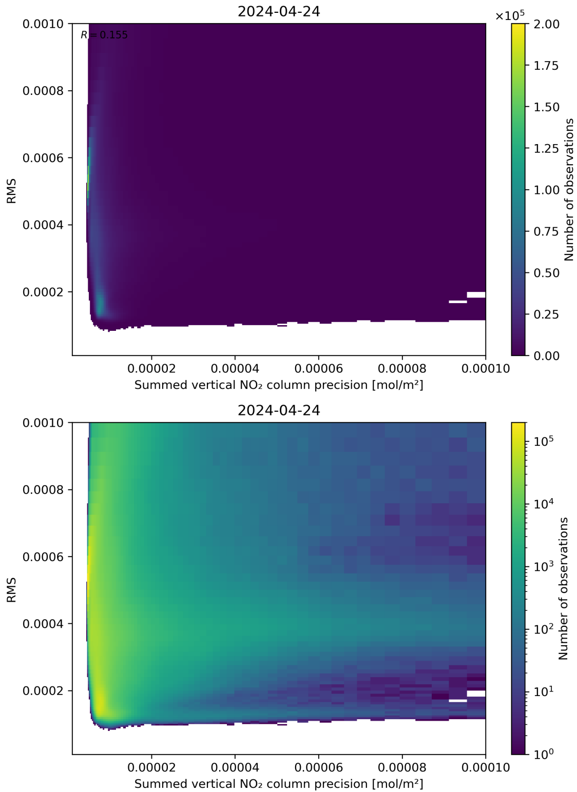
Figure 108: Scatter density plot of “Summed vertical NO 2 column precision” against “RMS” for 2024-04-23 to 2024-04-25.
