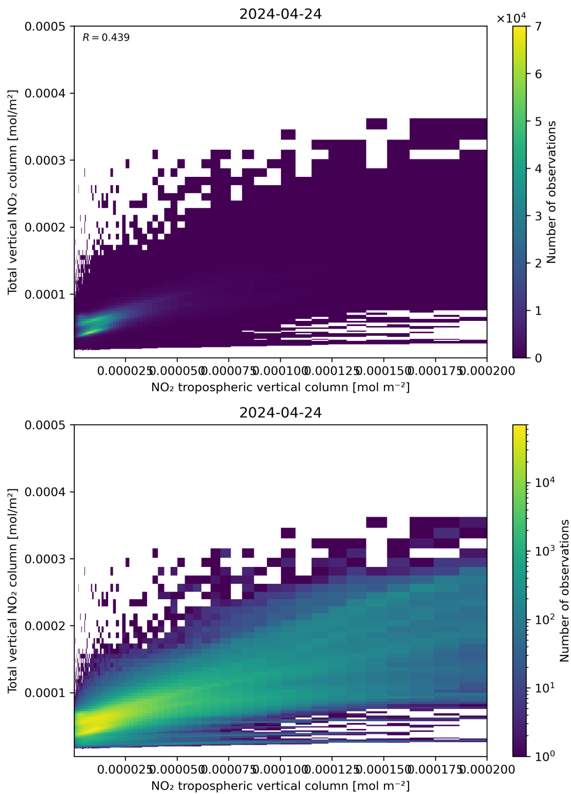
Figure 128: Scatter density plot of “NO 2 tropospheric vertical column” against “Total vertical NO 2 column” for 2024-04-23 to 2024-04-25.
