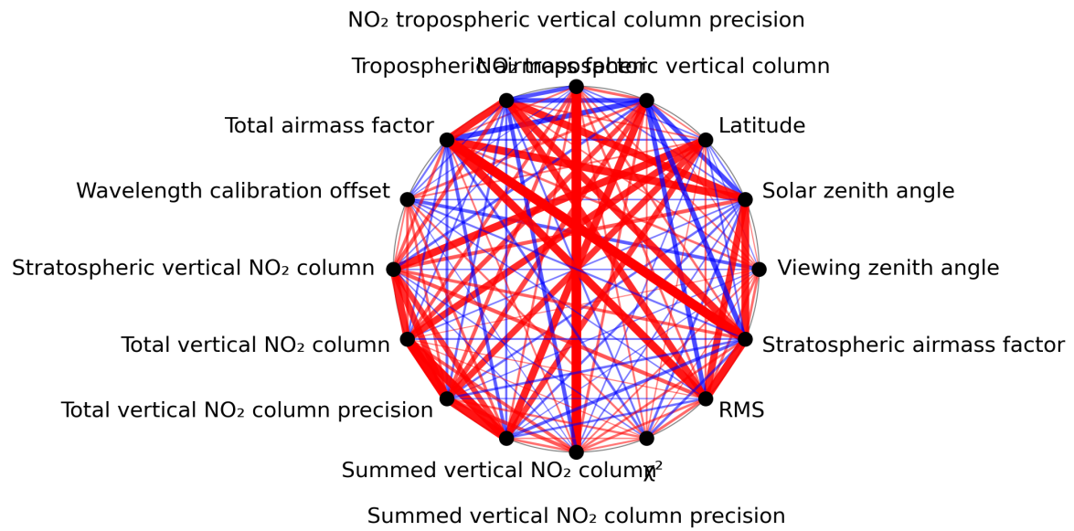
Figure 1: Map of correlation graph for 2024-04-23 to 2024-04-25.
