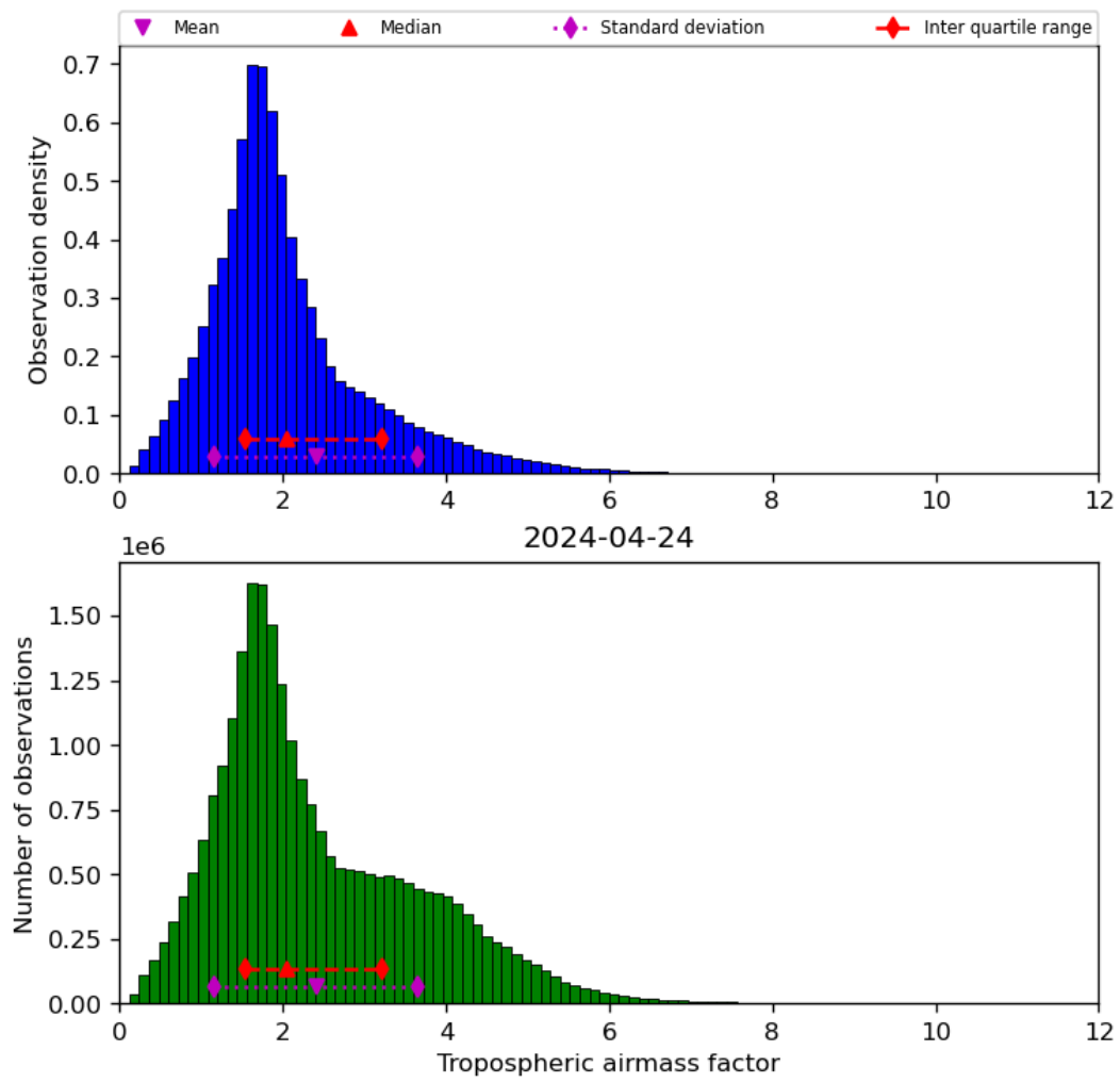
Figure 31: Histogram of “Tropospheric airmass factor” for 2024-04-23 to 2024-04-25
