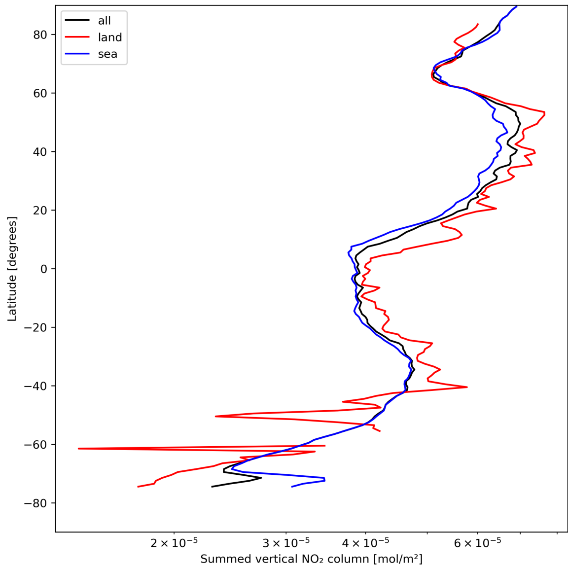
Figure 23: Zonal average of “Summed vertical NO 2 column” for 2024-04-23 to 2024-04-25.
