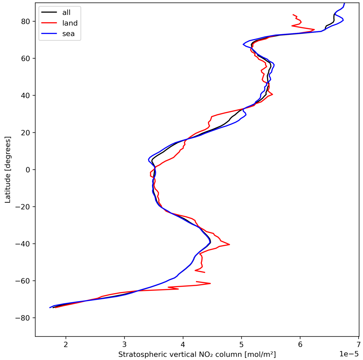
Figure 19: Zonal average of “Stratospheric vertical NO 2 column” for 2024-04-23 to 2024-04-25.
