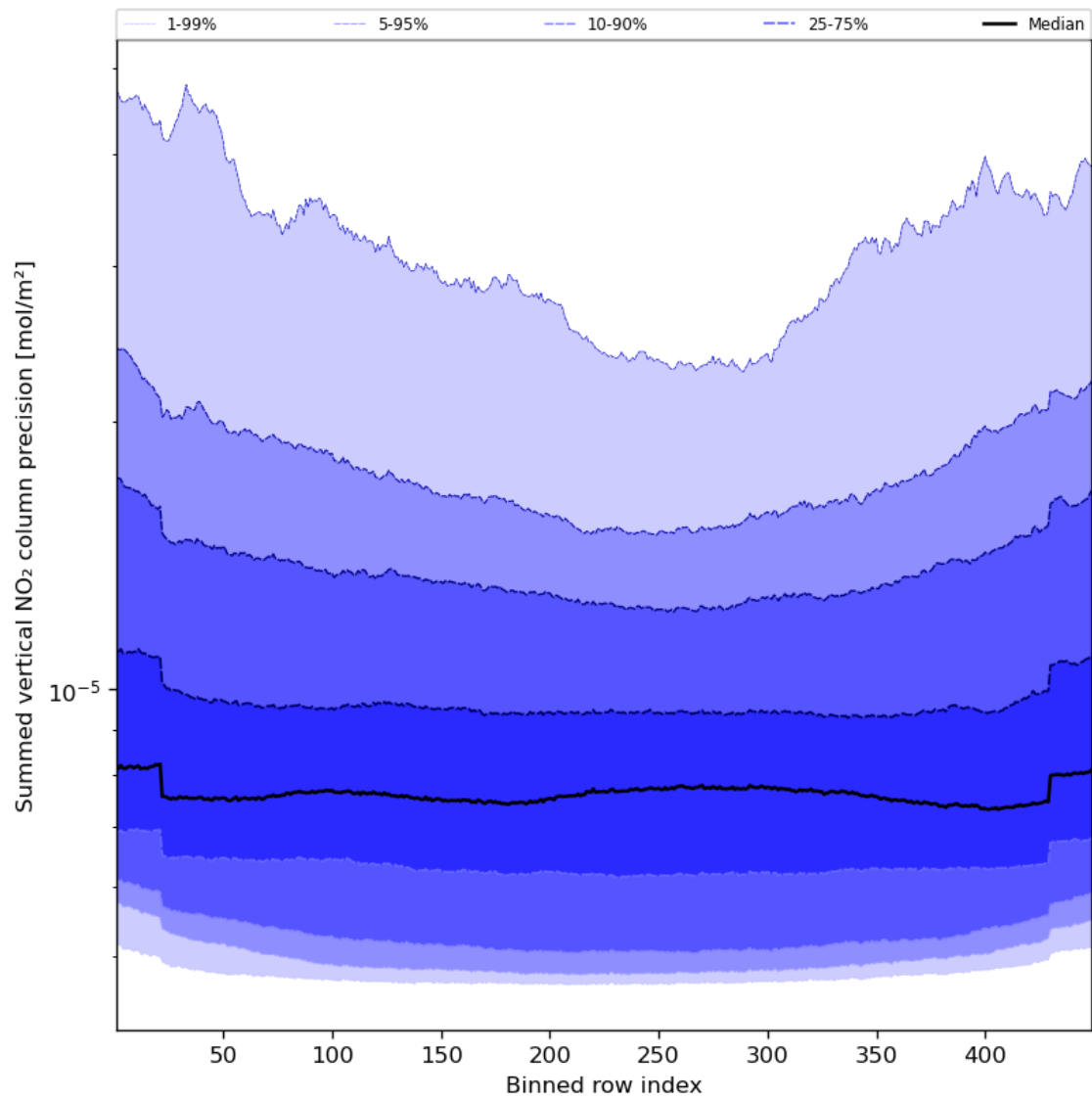
Figure 58: Along track statistics of “Summed vertical NO 2 column precision” for 2024-04-23 to 2024-04-25
