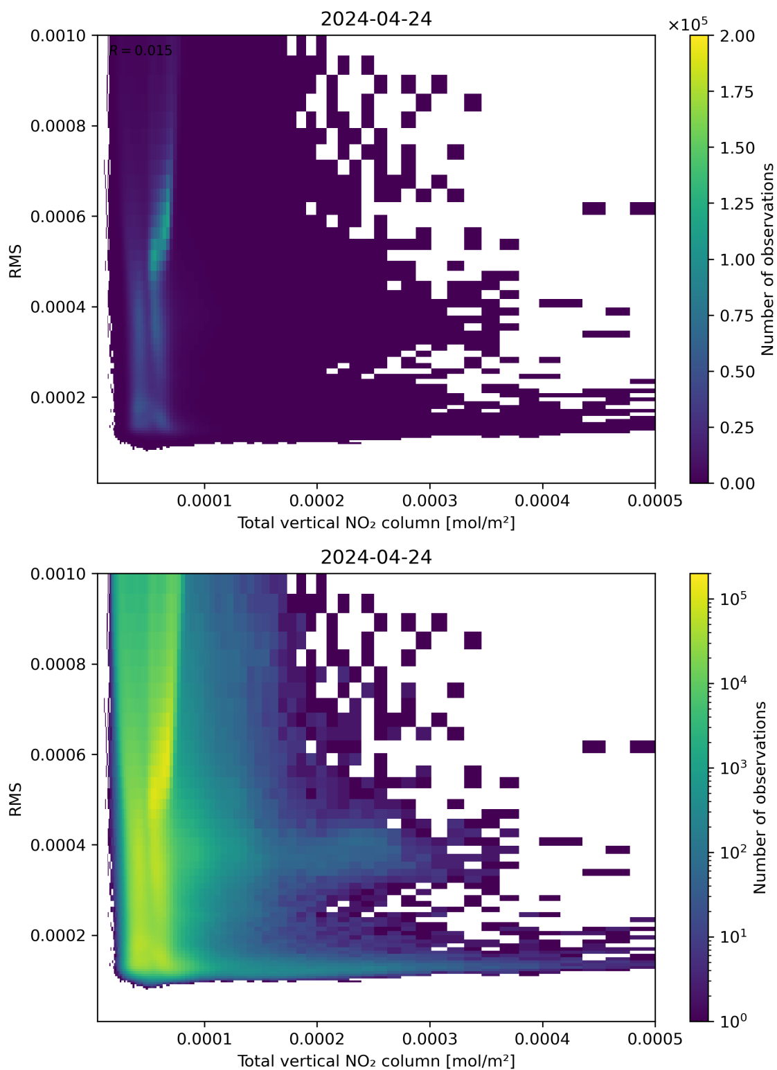
Figure 120: Scatter density plot of “Total vertical NO 2 column” against “RMS” for 2024-04-23 to 2024-04-25.
