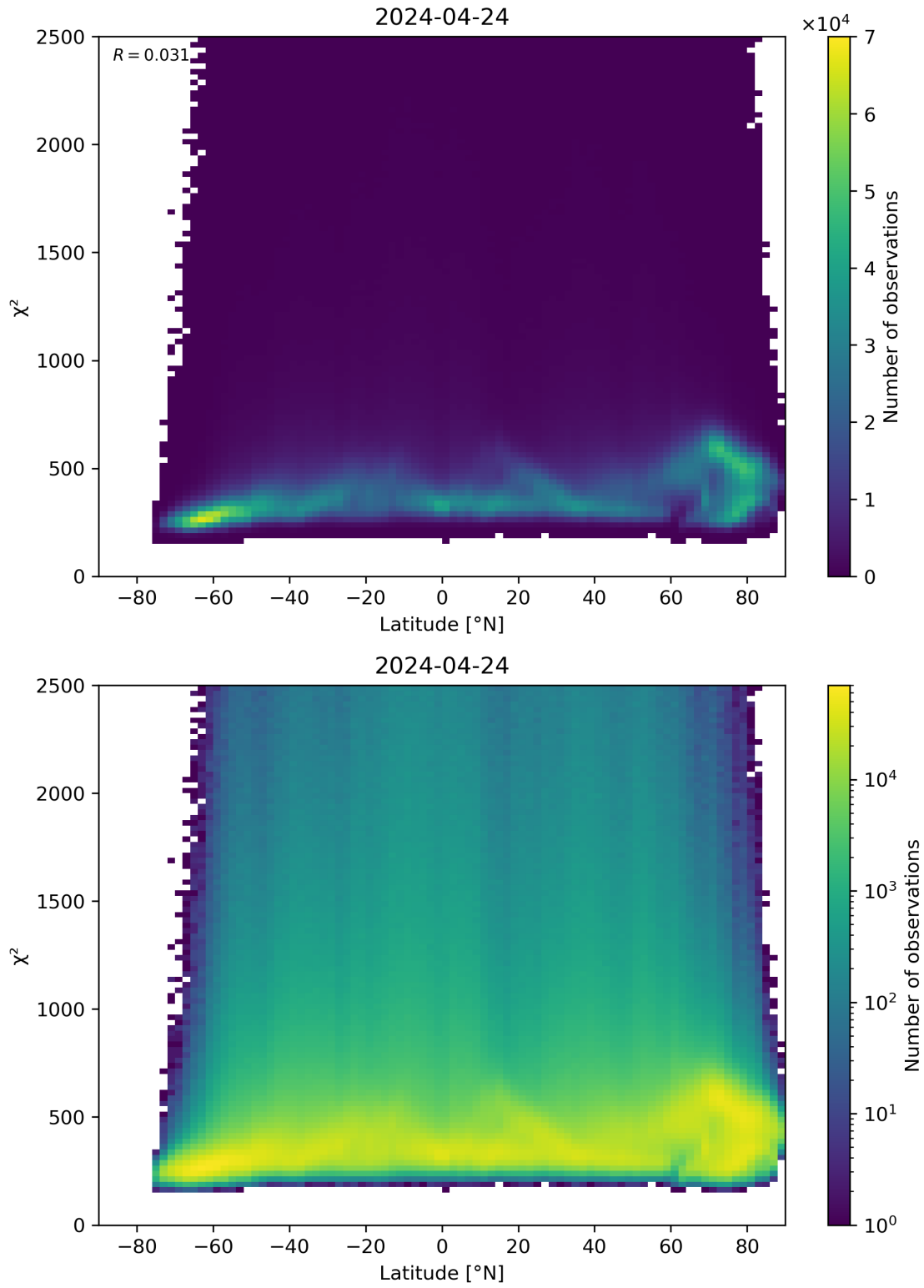
Figure 86: Scatter density plot of “Latitude” against “ \chi^2 ” for 2024-04-23 to 2024-04-25.
