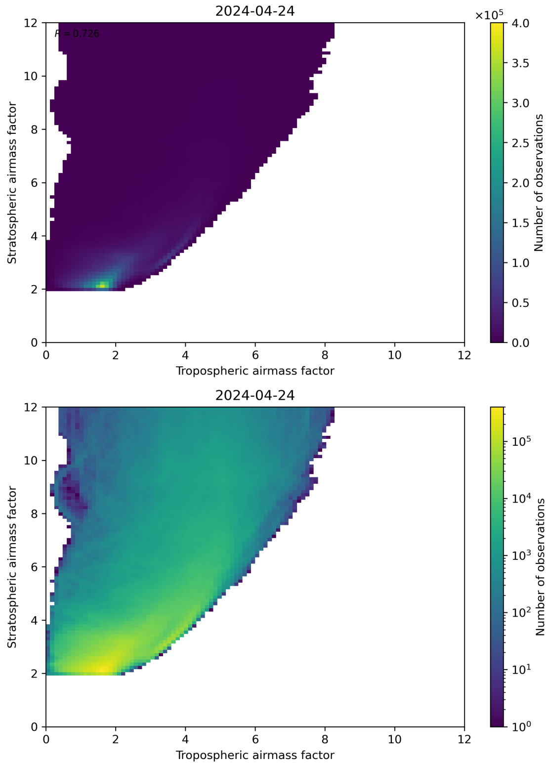
Figure 71: Scatter density plot of “Tropospheric airmass factor” against “Stratospheric airmass factor” for 2024-04-23 to 2024-04-25.
