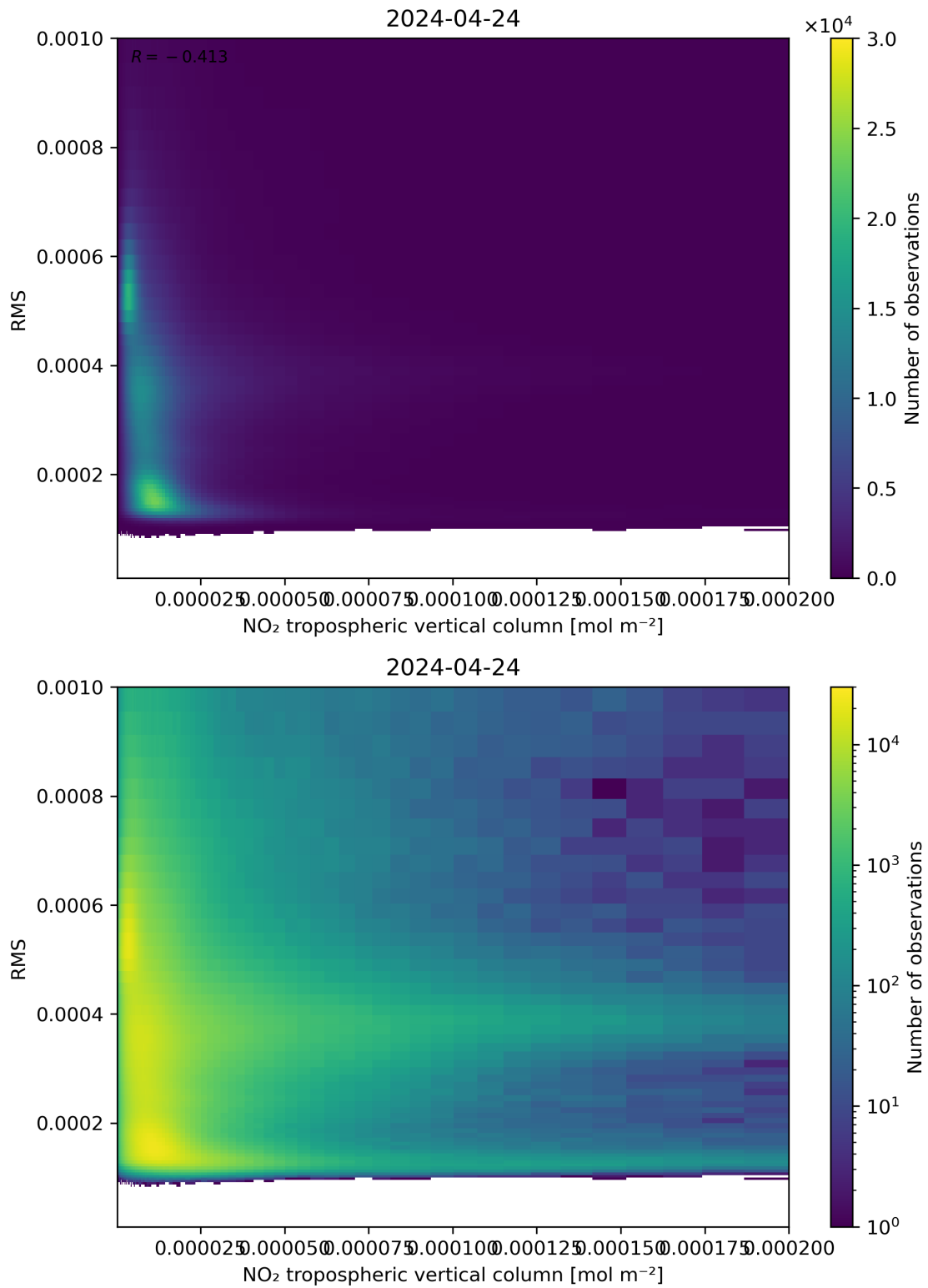
Figure 142: Scatter density plot of “NO 2 tropospheric vertical column” against “RMS” for 2024-04-23 to 2024-04-25.
