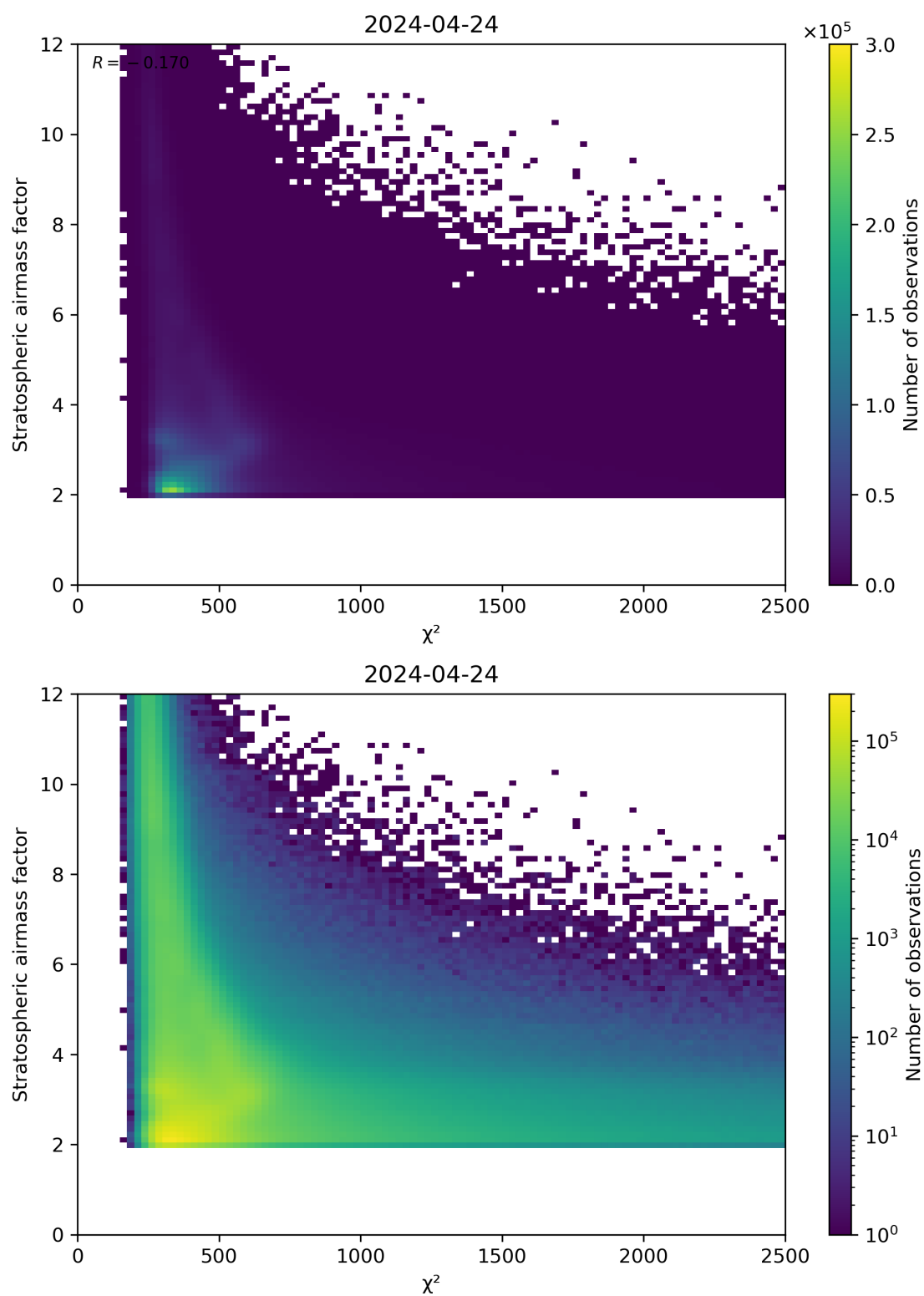
Figure 81: Scatter density plot of “ \chi^2 ” against “Stratospheric airmass factor” for 2024-04-23 to 2024-04-25.
