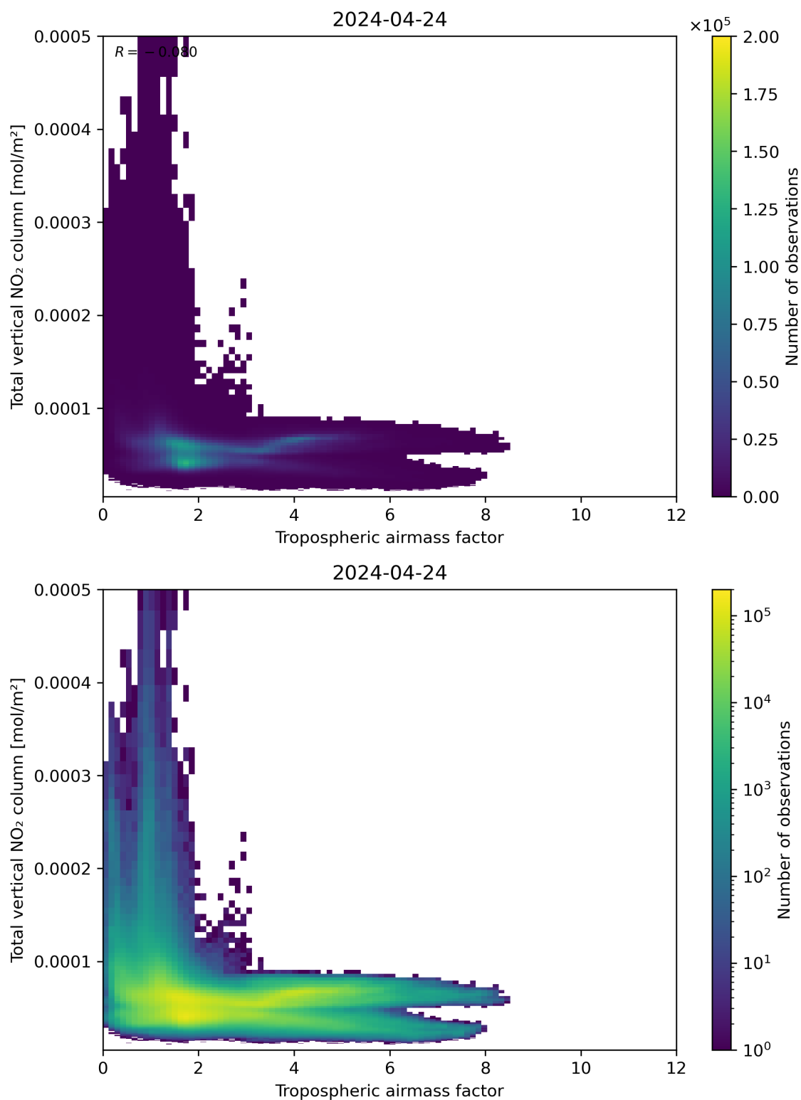
Figure 77: Scatter density plot of “Tropospheric airmass factor” against “Total vertical NO 2 column” for 2024-04-23 to 2024-04-25.
