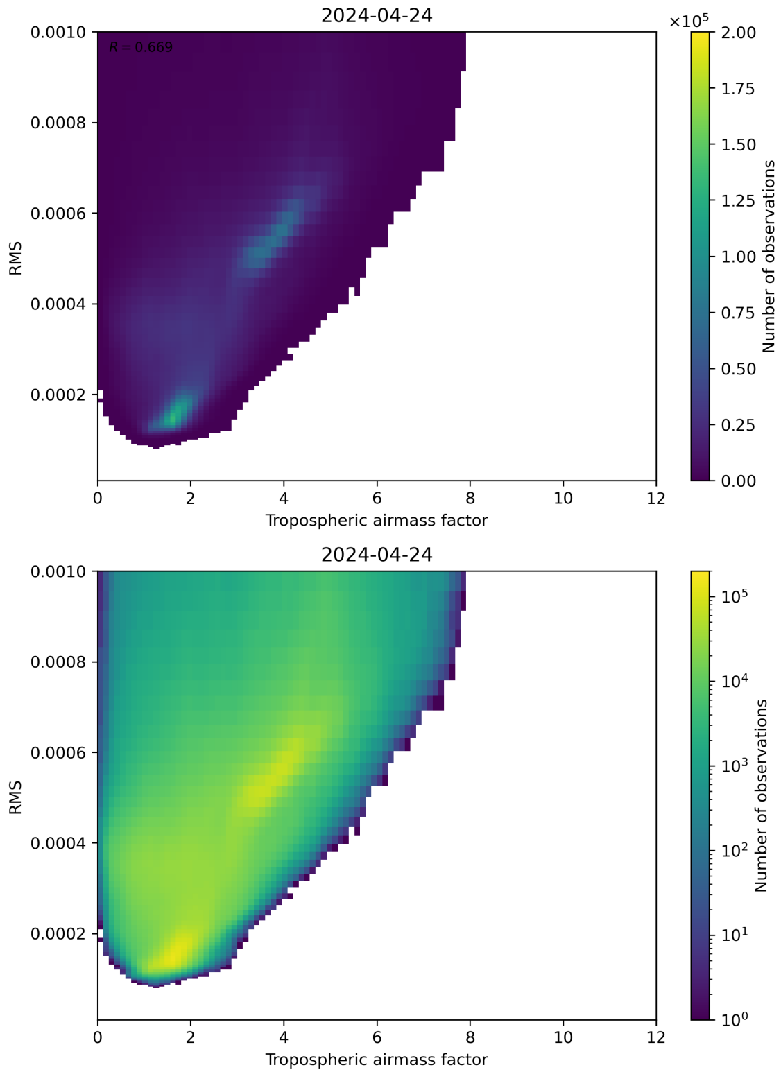
Figure 79: Scatter density plot of “Tropospheric airmass factor” against “RMS” for 2024-04-23 to 2024-04-25.
