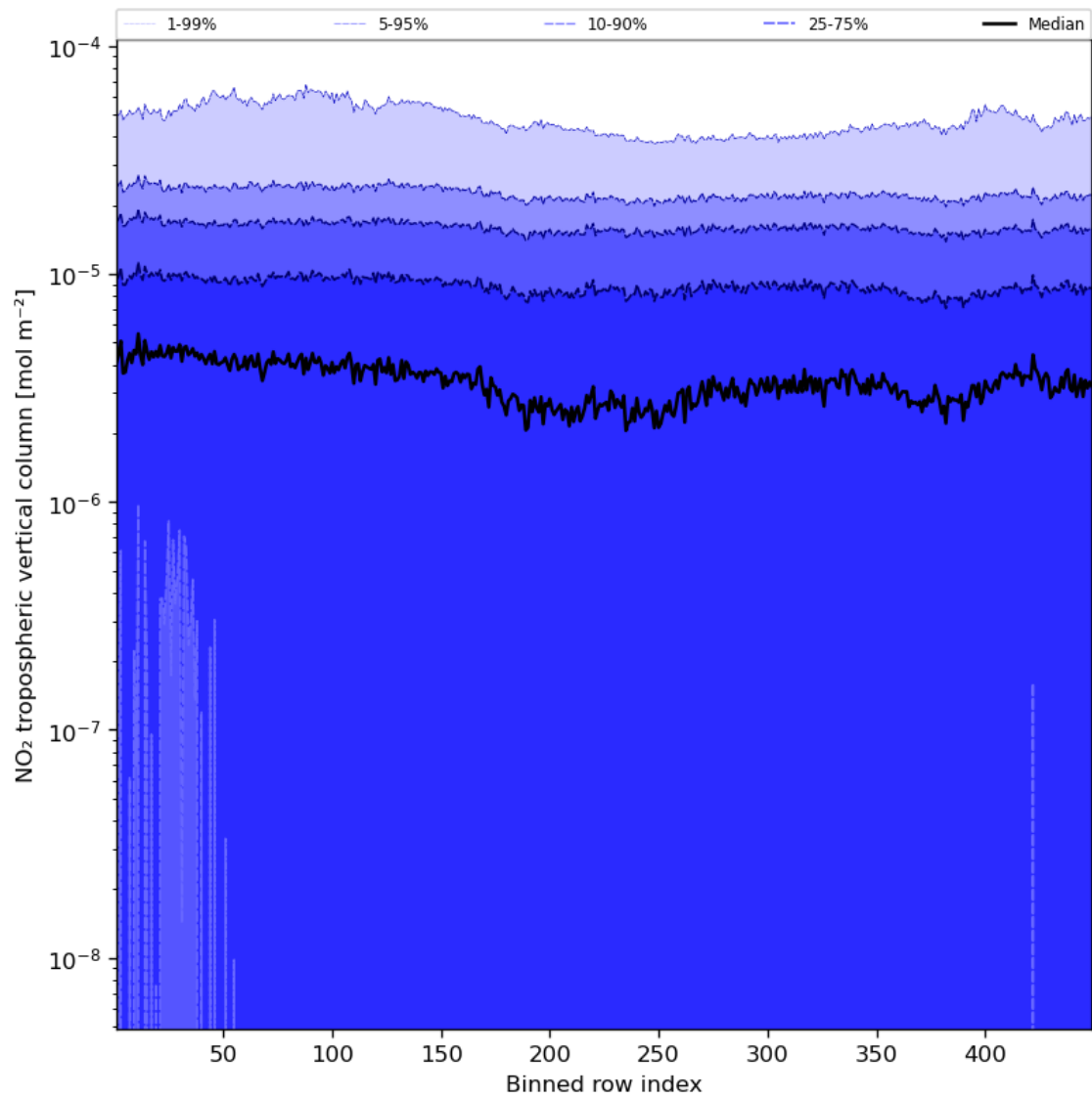
Figure 46: Along track statistics of “NO 2 tropospheric vertical column” for 2024-04-23 to 2024-04-25
