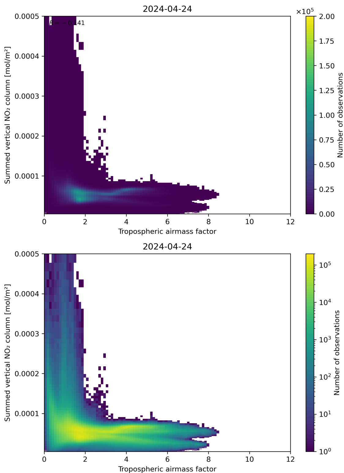
Figure 75: Scatter density plot of “Tropospheric airmass factor” against “Summed vertical NO 2 column” for 2024-04-23 to 2024-04-25.
