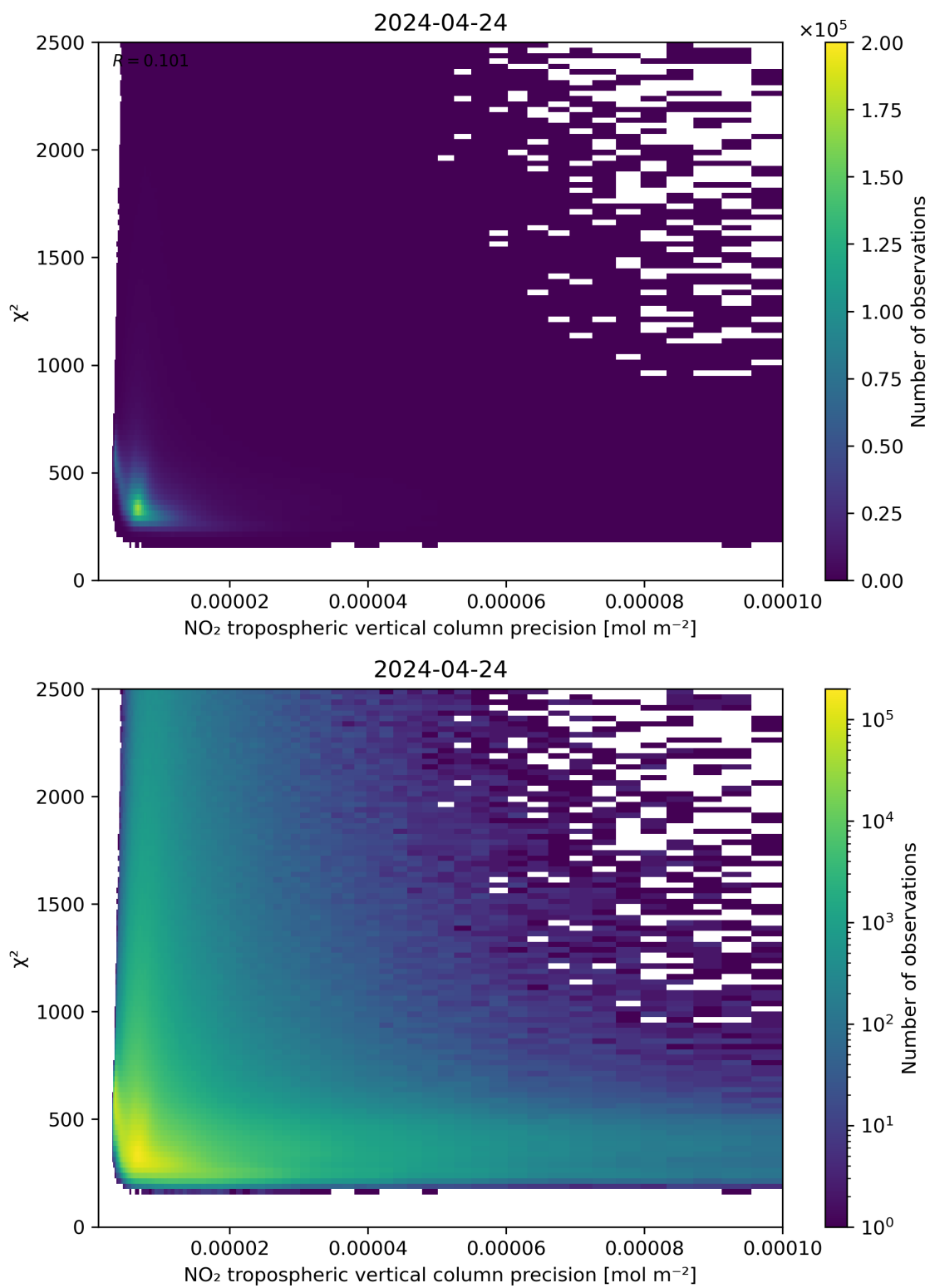
Figure 134: Scatter density plot of “NO 2 tropospheric vertical column precision” against “ \chi^2 ” for 2024-04-23 to 2024-04-25.
