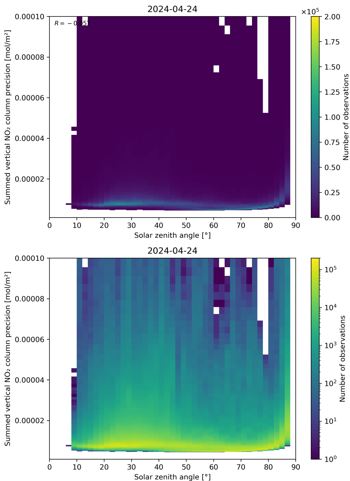
Figure 152: Scatter density plot of “Solar zenith angle” against “Summed vertical NO 2 column precision” for 2024-04-23 to 2024-04-25.
