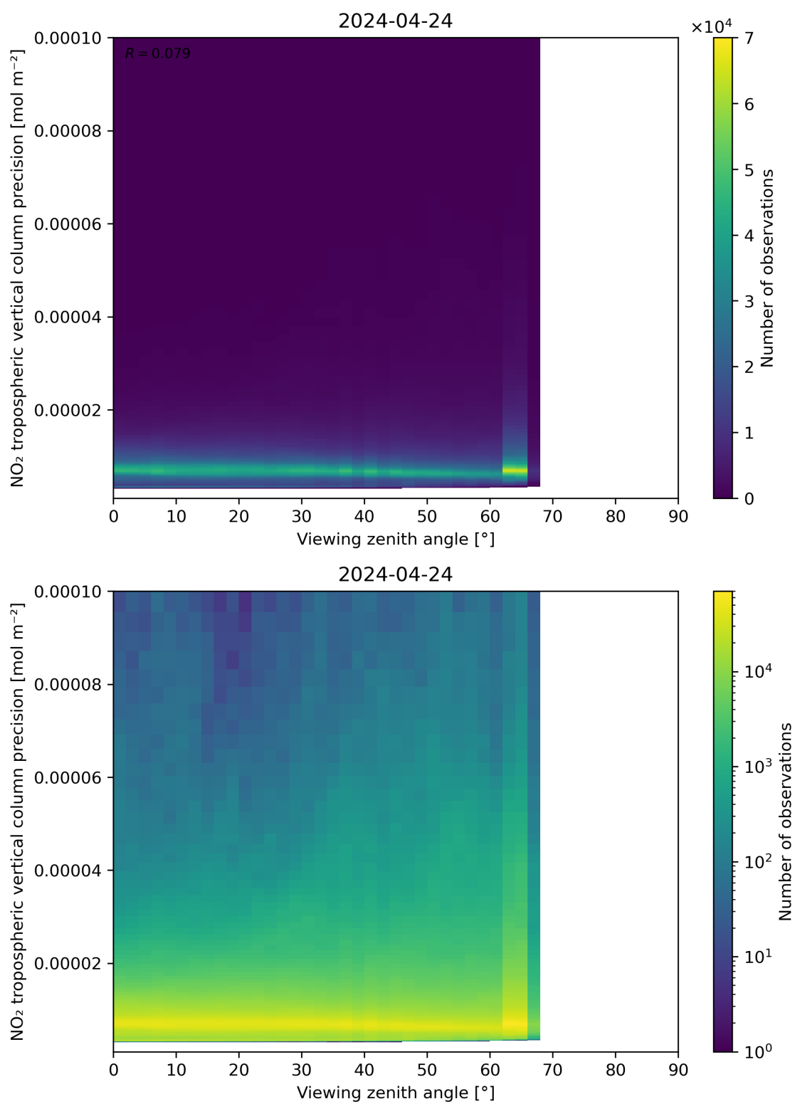
Figure 170: Scatter density plot of “Viewing zenith angle” against “NO 2 tropospheric vertical column precision” for 2024-04-23 to 2024-04-25.
