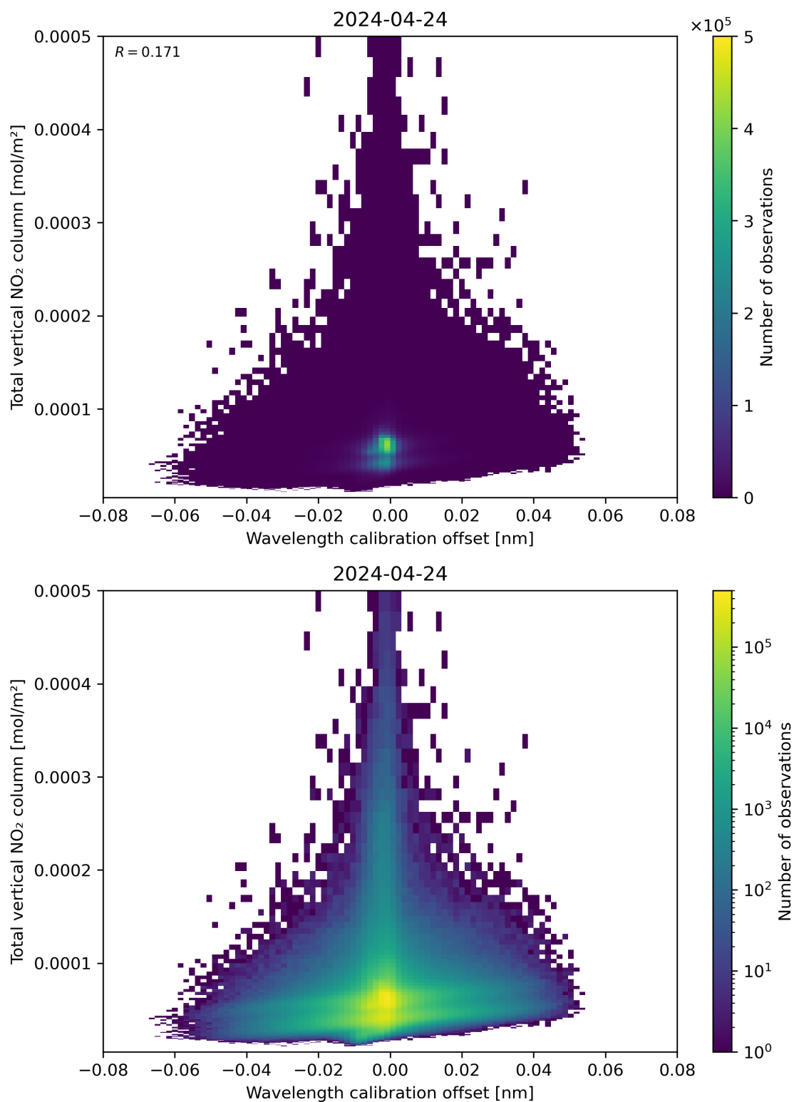
Figure 179: Scatter density plot of “Wavelength calibration offset” against “Total vertical NO 2 column” for 2024-04-23 to 2024-04-25.
