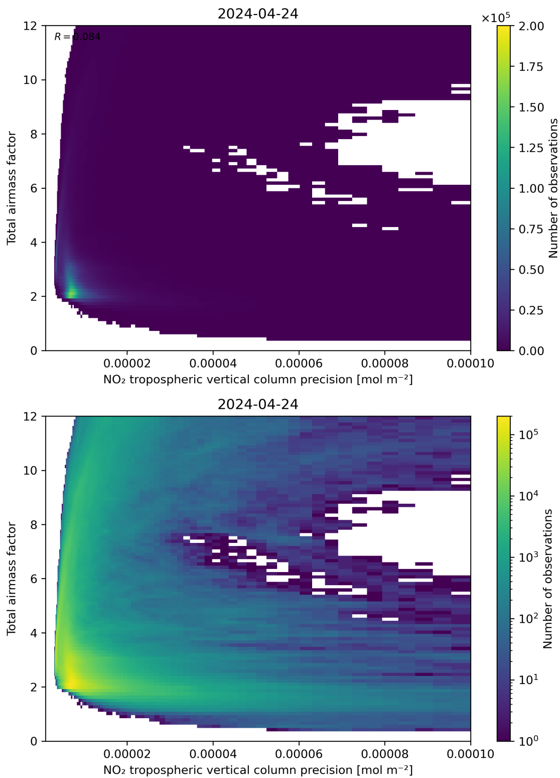
Figure 132: Scatter density plot of “NO 2 tropospheric vertical column precision” against “Total air mass factor” for 2024-04-23 to 2024-04-25.
