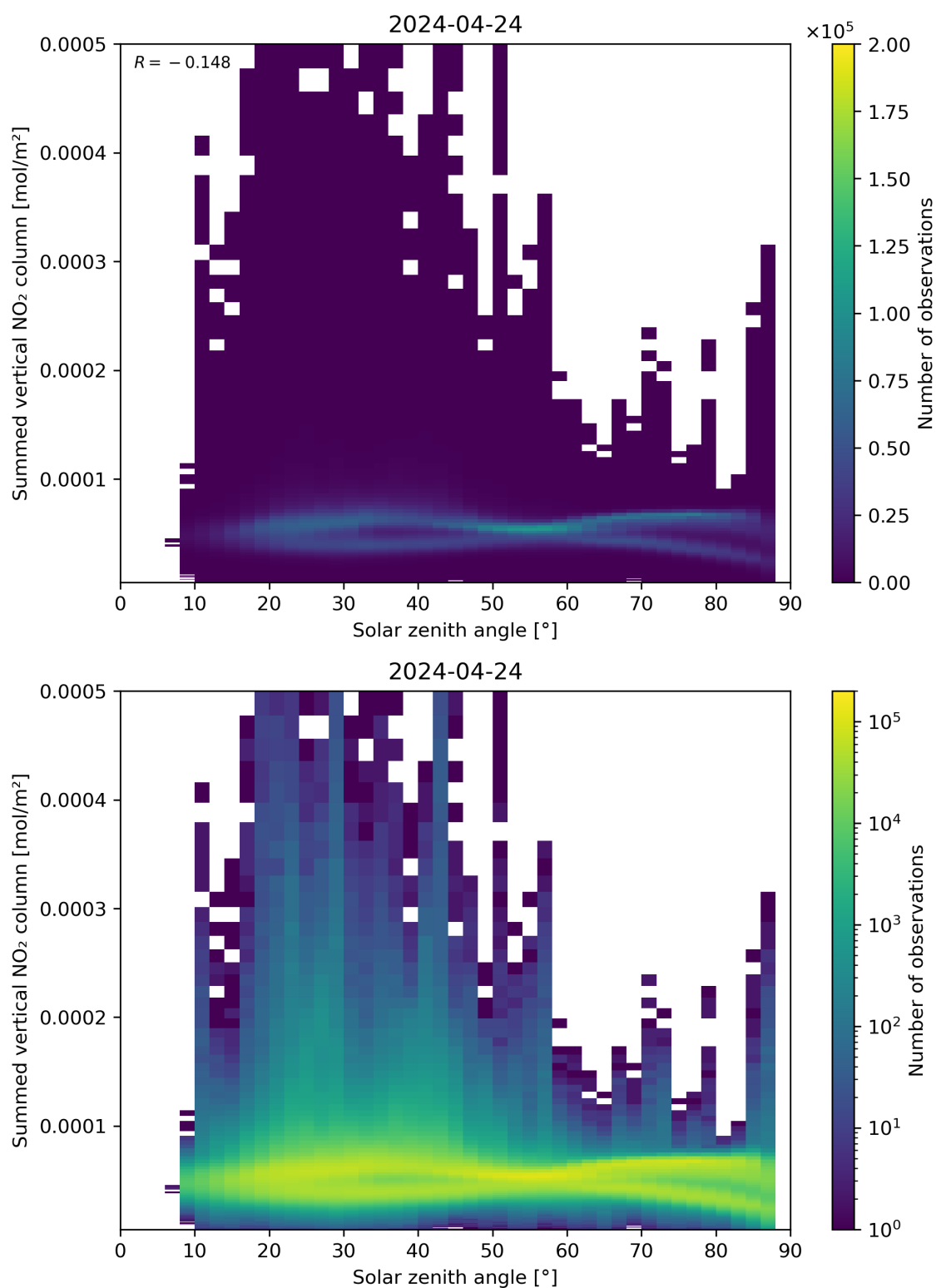
Figure 151: Scatter density plot of “Solar zenith angle” against “Summed vertical NO 2 column” for 2024-04-23 to 2024-04-25.
