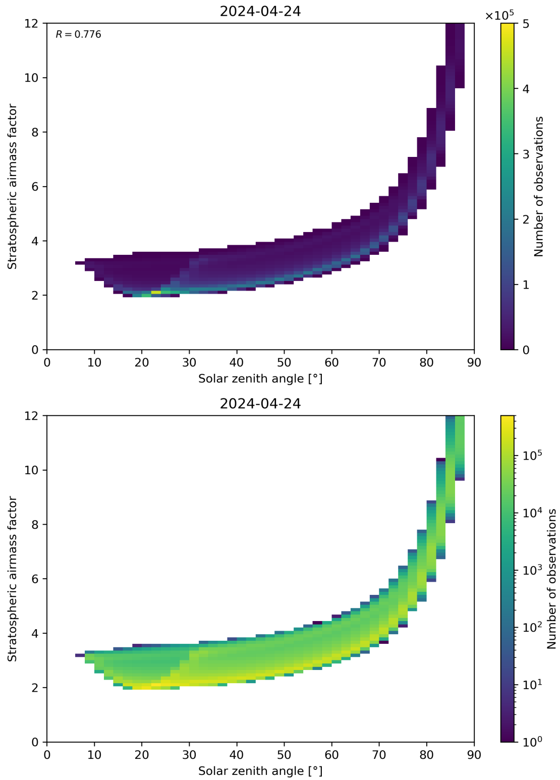
Figure 145: Scatter density plot of “Solar zenith angle” against “Stratospheric airmass factor” for 2024-04-23 to 2024-04-25.
