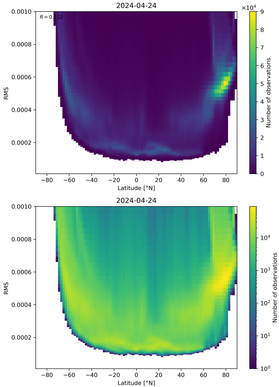
Figure 94: Scatter density plot of “Latitude” against “RMS” for 2024-04-23 to 2024-04-25.
