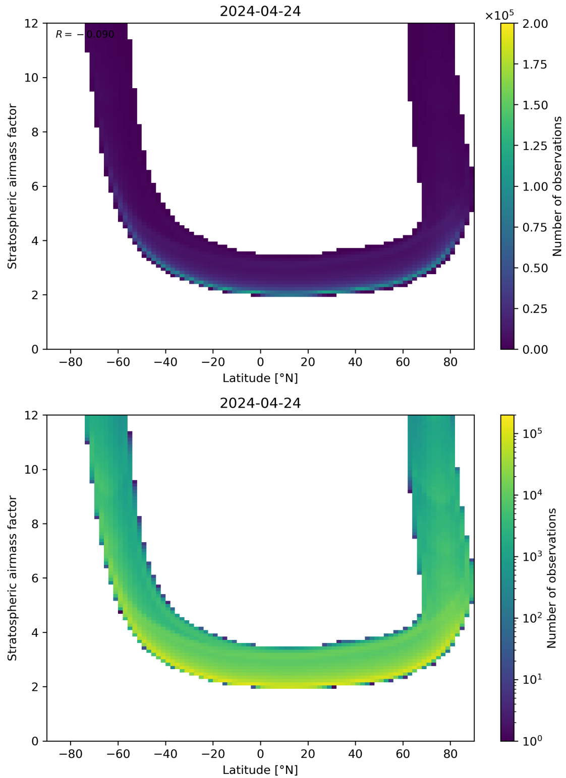
Figure 83: Scatter density plot of “Latitude” against “Stratospheric airmass factor” for 2024-04-23 to 2024-04-25.
