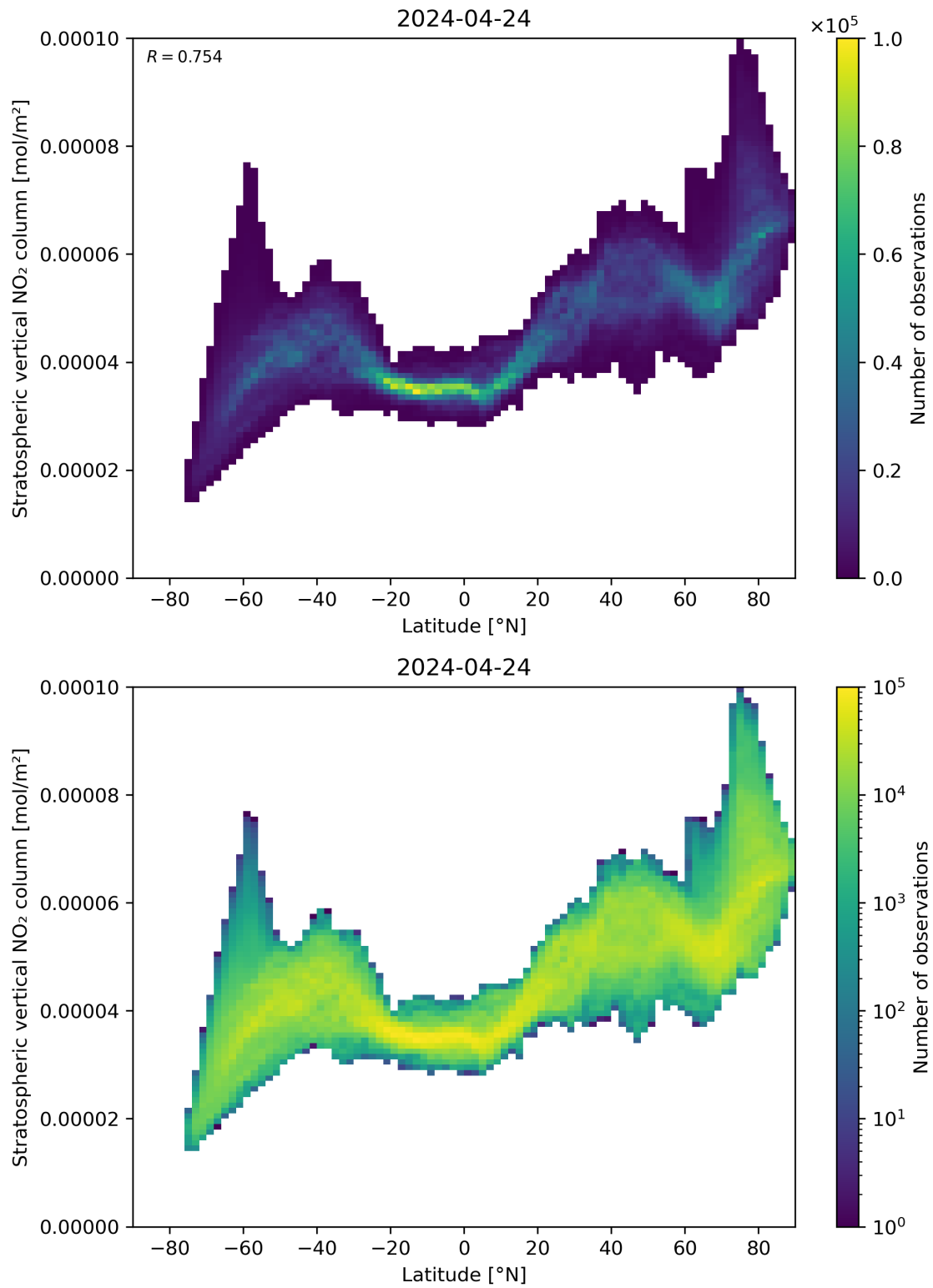
Figure 87: Scatter density plot of “Latitude” against “Stratospheric vertical NO 2 column” for 2024-04-23 to 2024-04-25.
