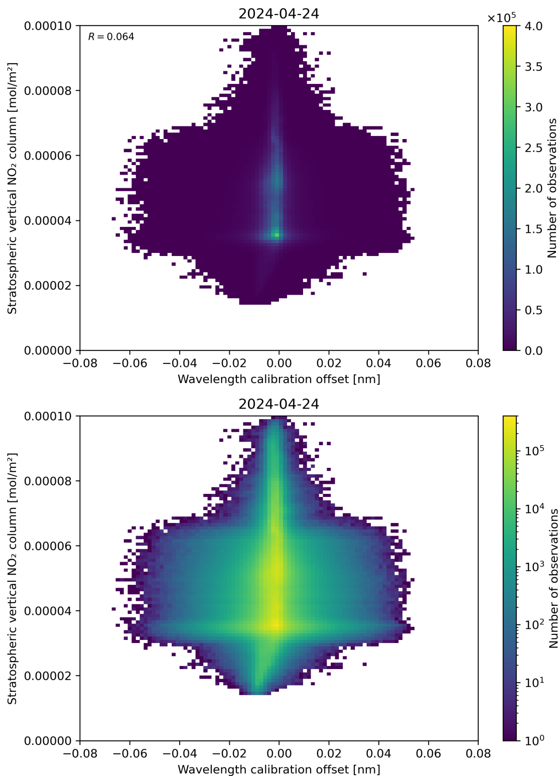
Figure 176: Scatter density plot of “Wavelength calibration offset” against “Stratospheric vertical \text{NO}_2 column” for 2024-04-23 to 2024-04-25.
