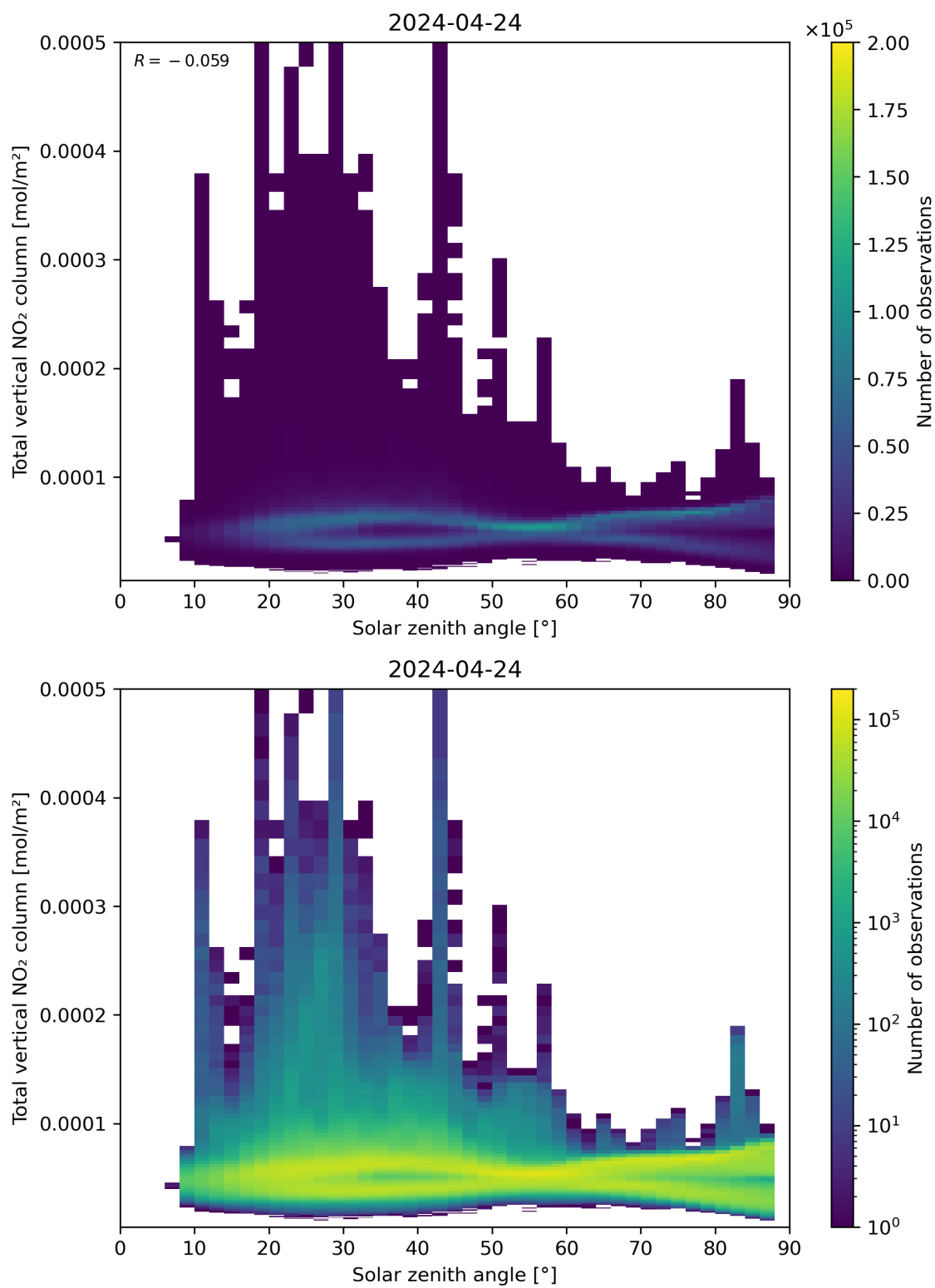
Figure 153: Scatter density plot of “Solar zenith angle” against “Total vertical NO 2 column” for 2024-04-23 to 2024-04-25.
