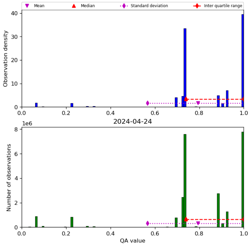
Figure 28: Histogram of “QA value” for 2024-04-23 to 2024-04-25
