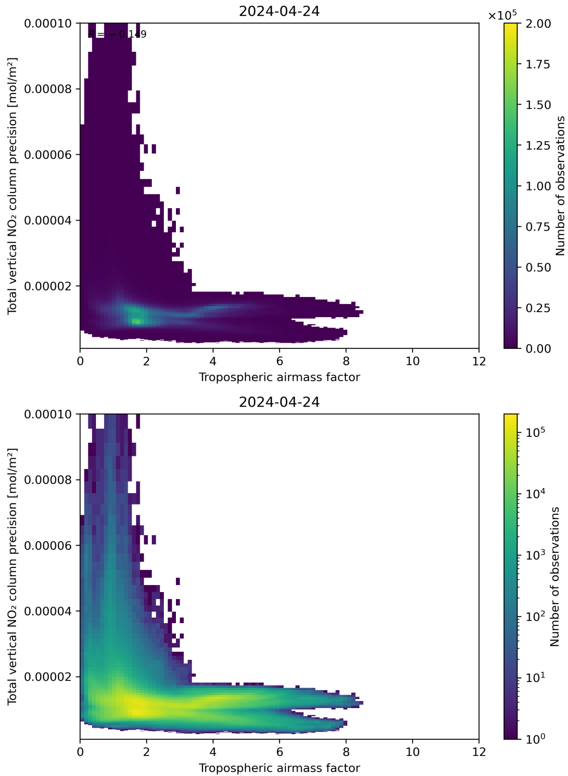
Figure 78: Scatter density plot of “Tropospheric air mass factor” against “Total vertical NO 2 column precision” for 2024-04-23 to 2024-04-25.
