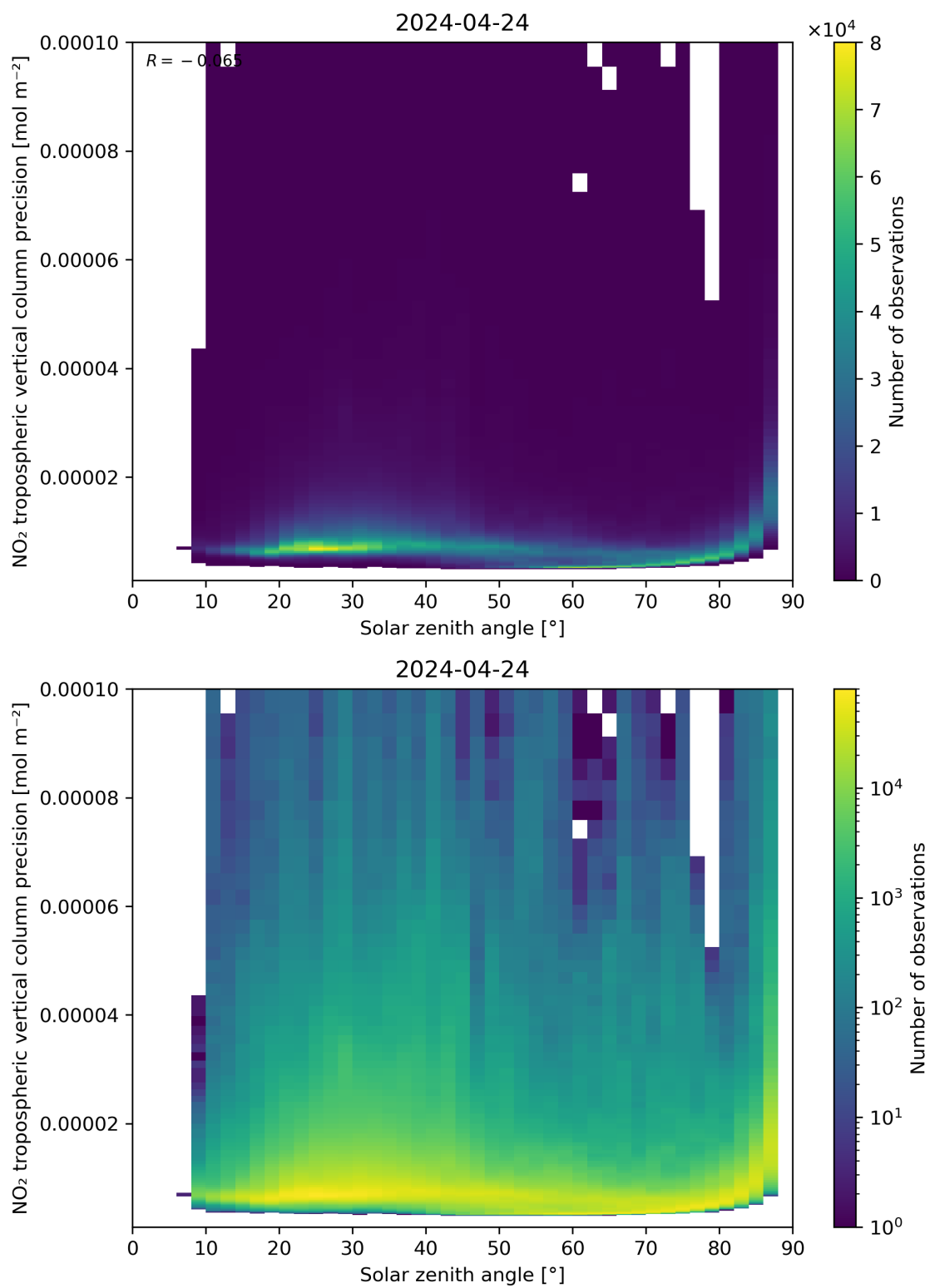
Figure 156: Scatter density plot of “Solar zenith angle” against “NO 2 tropospheric vertical column precision” for 2024-04-23 to 2024-04-25.
