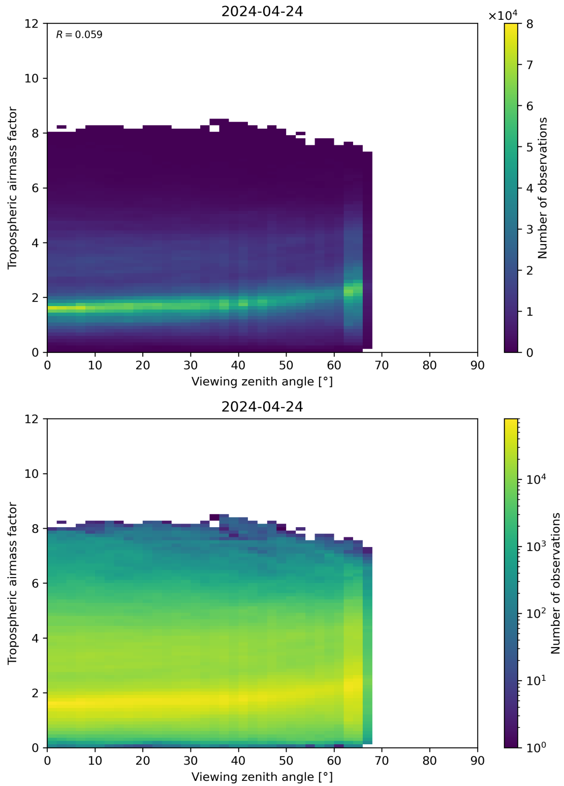
Figure 161: Scatter density plot of “Viewing zenith angle” against “Tropospheric airmass factor” for 2024-04-23 to 2024-04-25.
