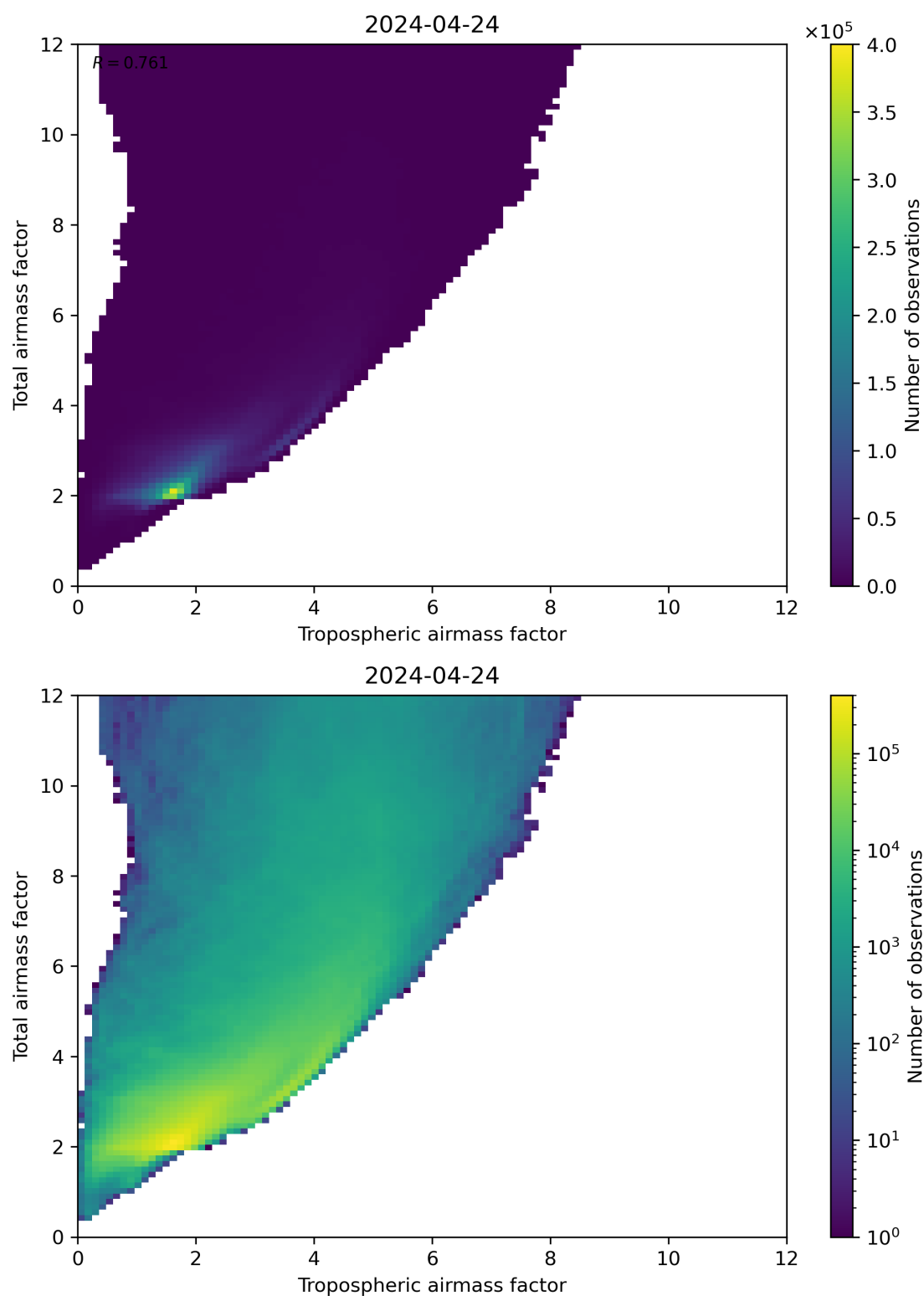
Figure 72: Scatter density plot of “Tropospheric airmass factor” against “Total airmass factor” for 2024-04-23 to 2024-04-25.
