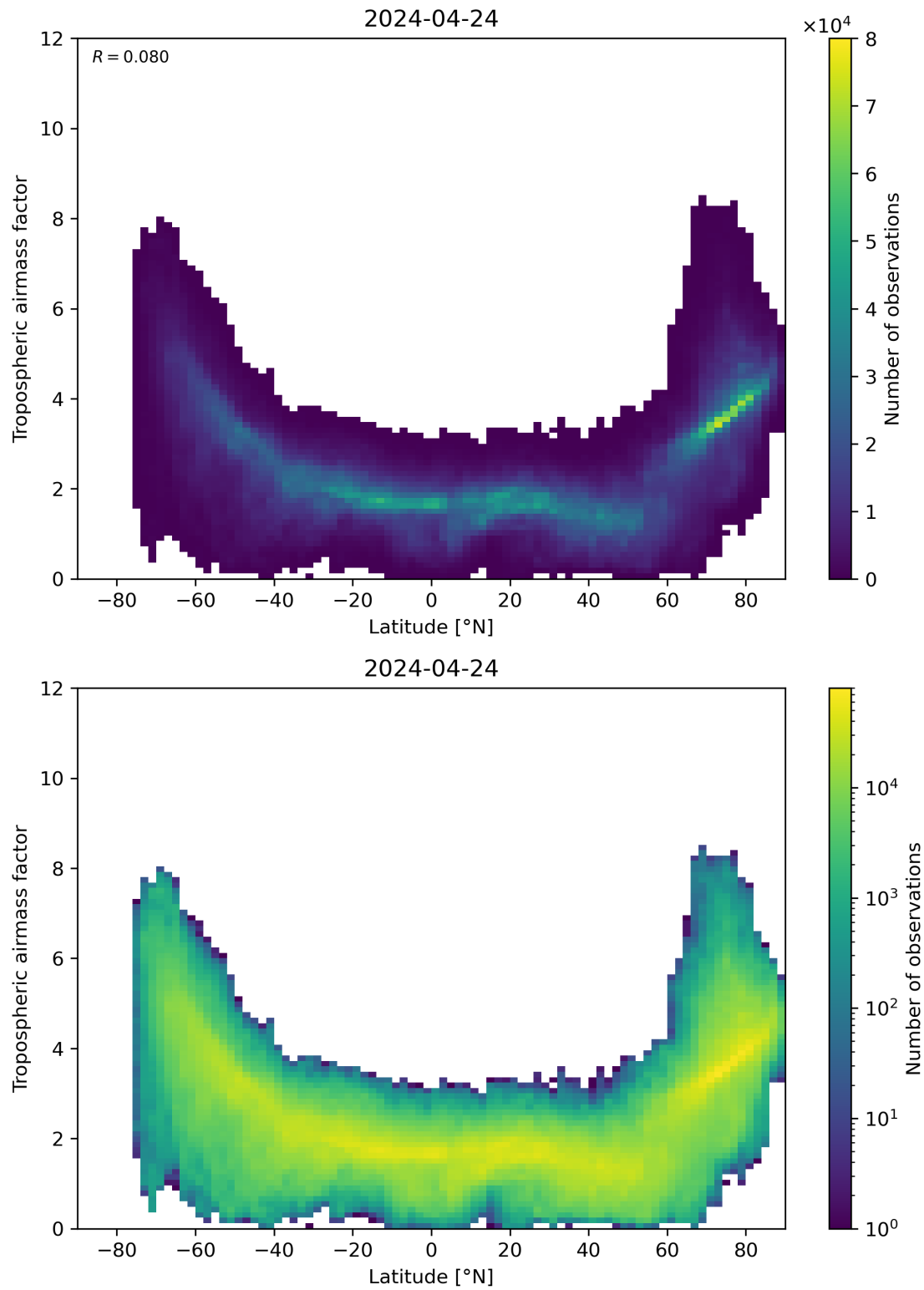
Figure 85: Scatter density plot of “Latitude” against “Tropospheric airmass factor” for 2024-04-23 to 2024-04-25.
