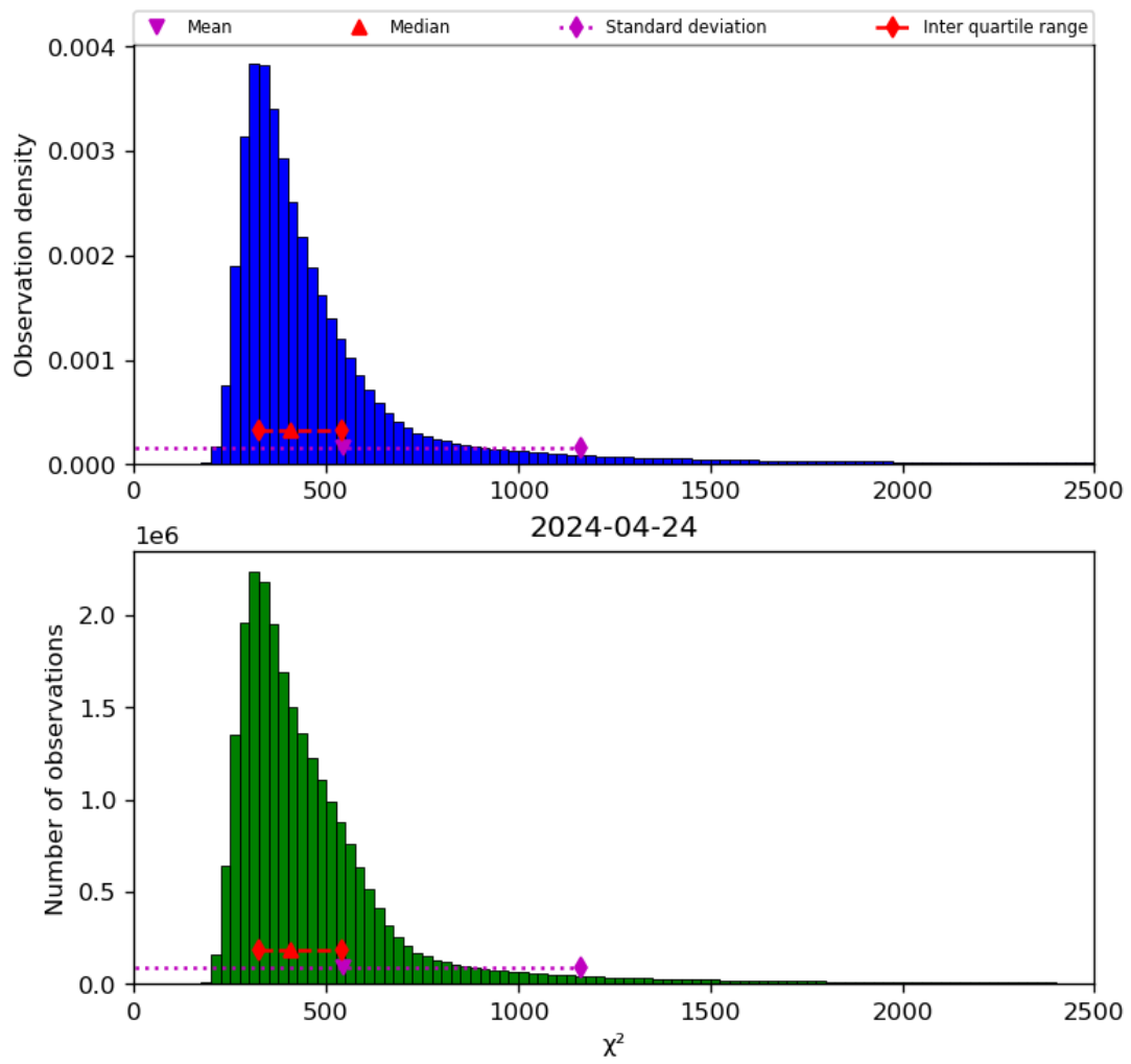
Figure 42: Histogram of " \chi^2 " for 2024-04-23 to 2024-04-25
