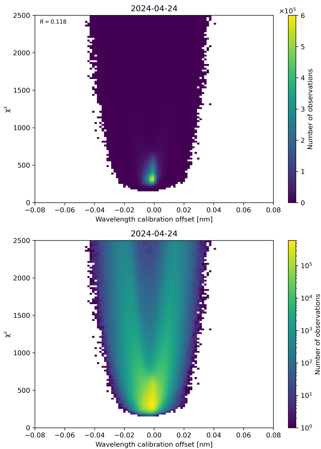
Figure 175: Scatter density plot of “Wavelength calibration offset” against “ \chi^2 ” for 2024-04-23 to 2024-04-25.
