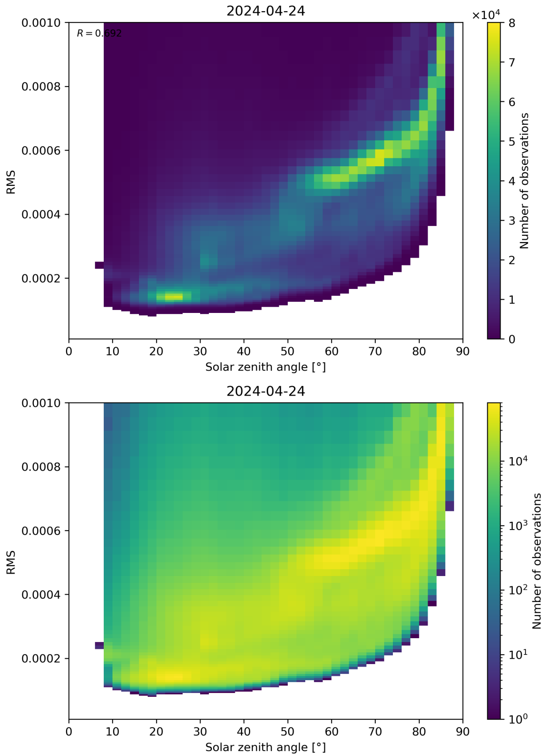
Figure 157: Scatter density plot of “Solar zenith angle” against “RMS” for 2024-04-23 to 2024-04-25.
