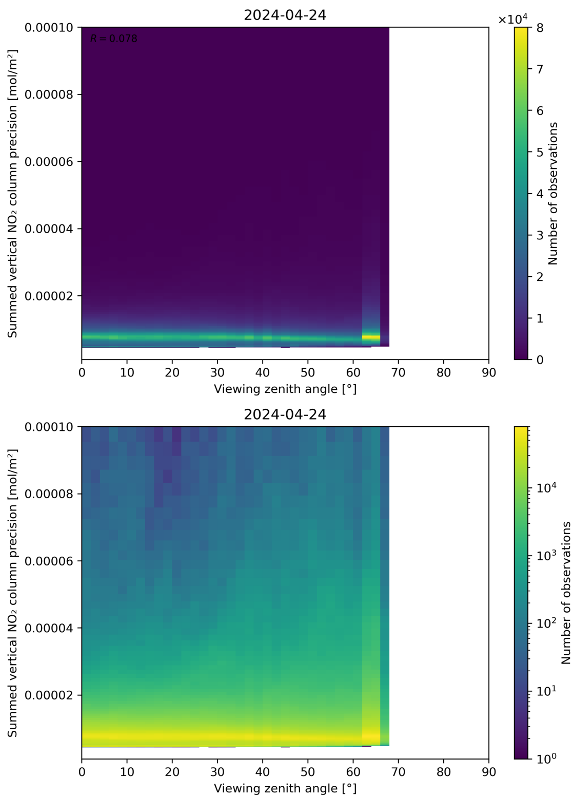
Figure 166: Scatter density plot of “Viewing zenith angle” against “Summed vertical NO 2 column precision” for 2024-04-23 to 2024-04-25.
