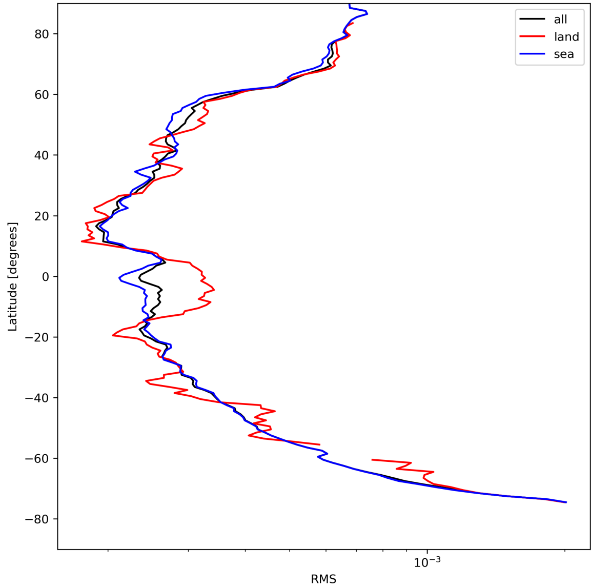
Figure 26: Zonal average of “RMS” for 2024-04-23 to 2024-04-25.
