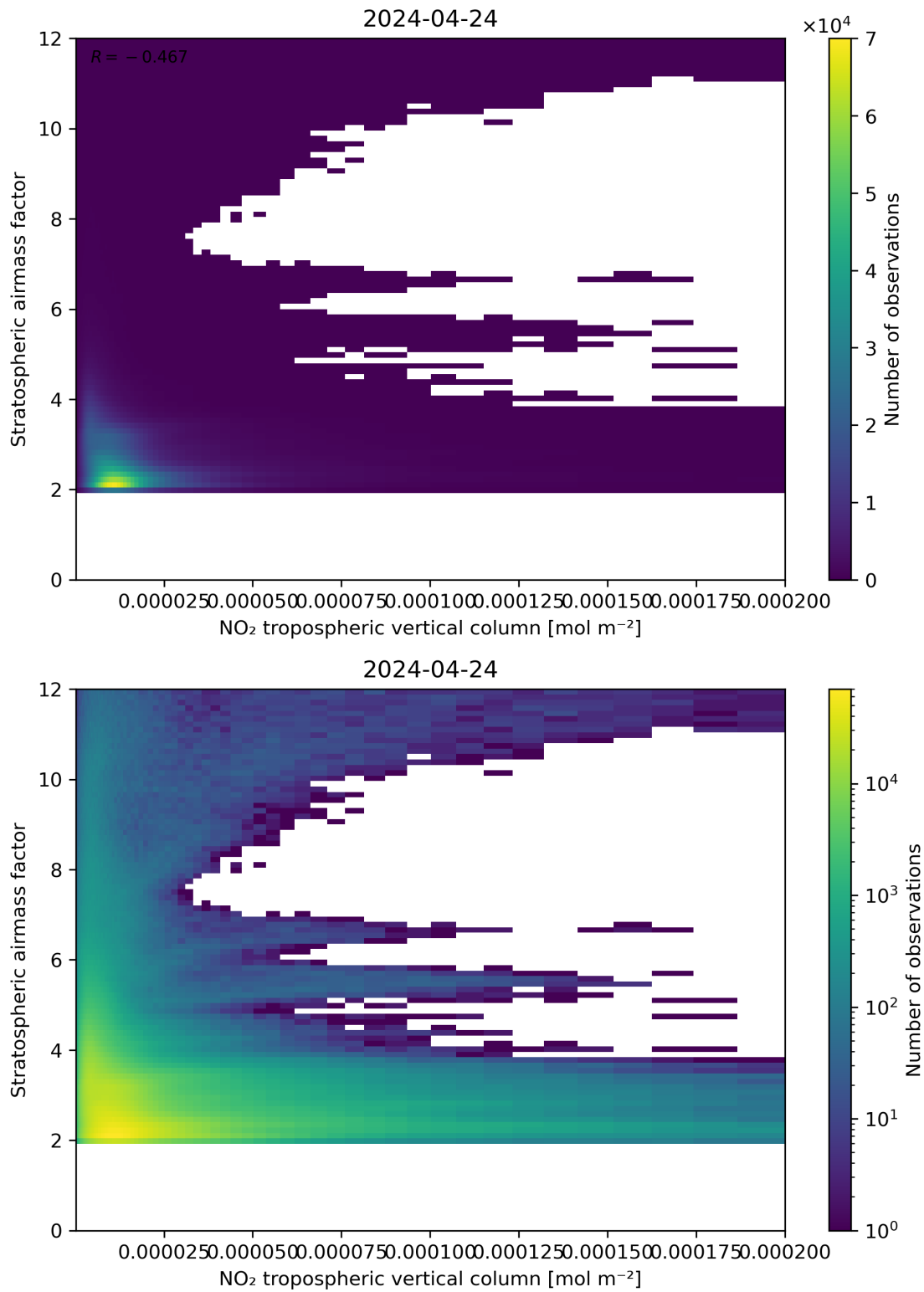
Figure 121: Scatter density plot of “NO 2 tropospheric vertical column” against “Stratospheric air mass factor” for 2024-04-23 to 2024-04-25.
