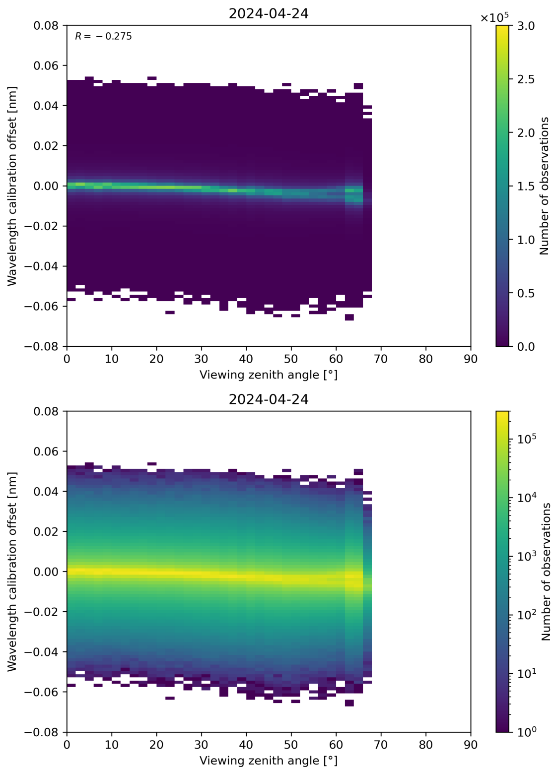
Figure 173: Scatter density plot of “Viewing zenith angle” against “Wavelength calibration offset” for 2024-04-23 to 2024-04-25.
