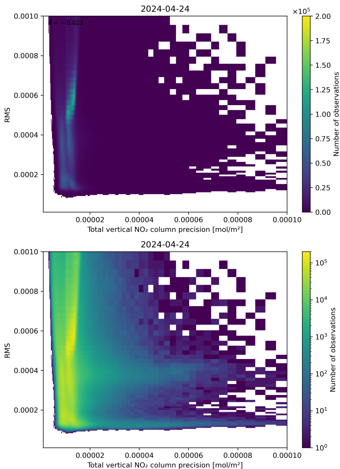
Figure 119: Scatter density plot of “Total vertical NO 2 column precision” against “RMS” for 2024-04-23 to 2024-04-25.
