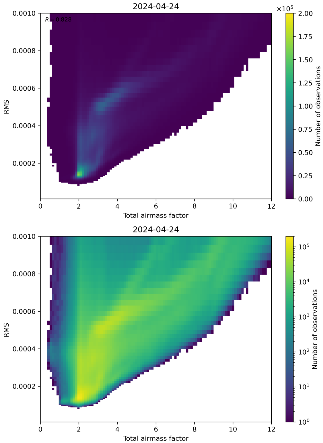
Figure 69: Scatter density plot of “Total airmass factor” against “RMS” for 2024-04-23 to 2024-04-25.
