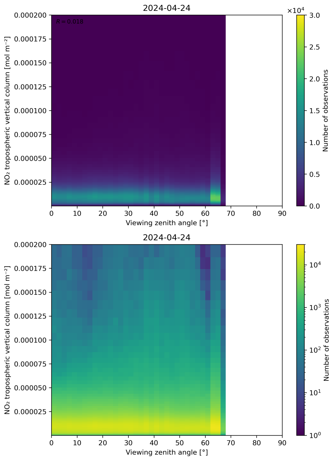
Figure 169: Scatter density plot of “Viewing zenith angle” against “NO 2 tropospheric vertical column” for 2024-04-23 to 2024-04-25.
