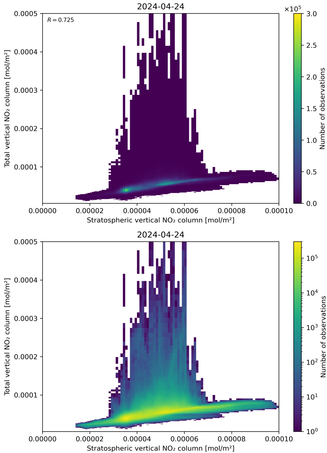
Figure 100: Scatter density plot of “Stratospheric vertical NO 2 column” against “Total vertical NO 2 column” for 2024-04-23 to 2024-04-25.
