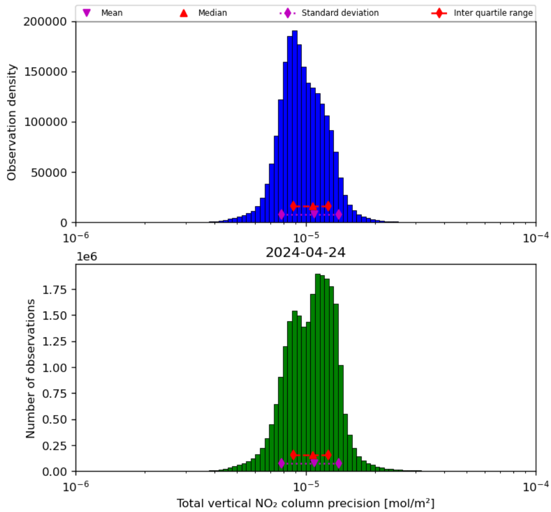
Figure 39: Histogram of "Total vertical NO 2 column precision" for 2024-04-23 to 2024-04-25
