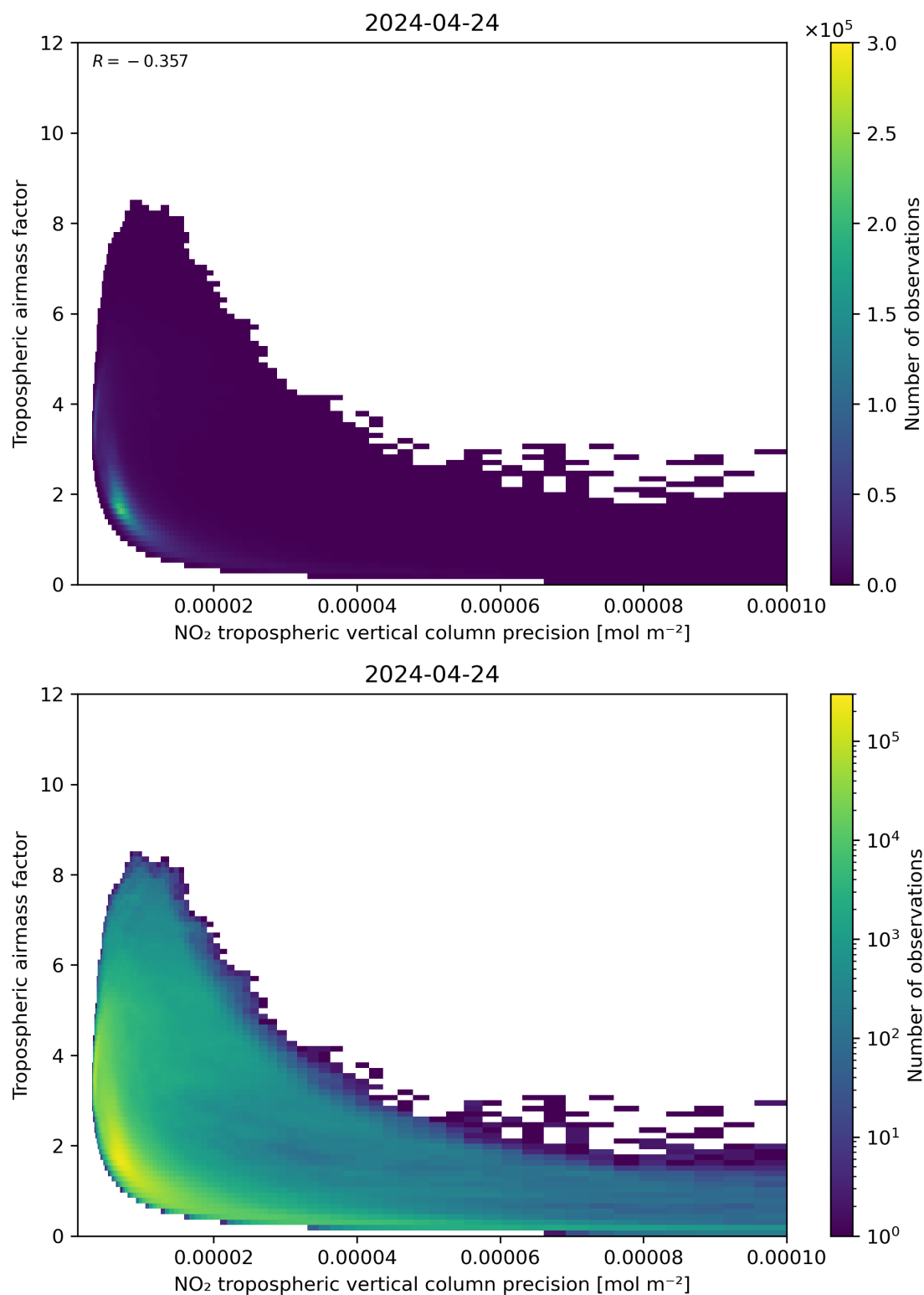
Figure 133: Scatter density plot of “NO 2 tropospheric vertical column precision” against “Tropospheric airmass factor” for 2024-04-23 to 2024-04-25.
