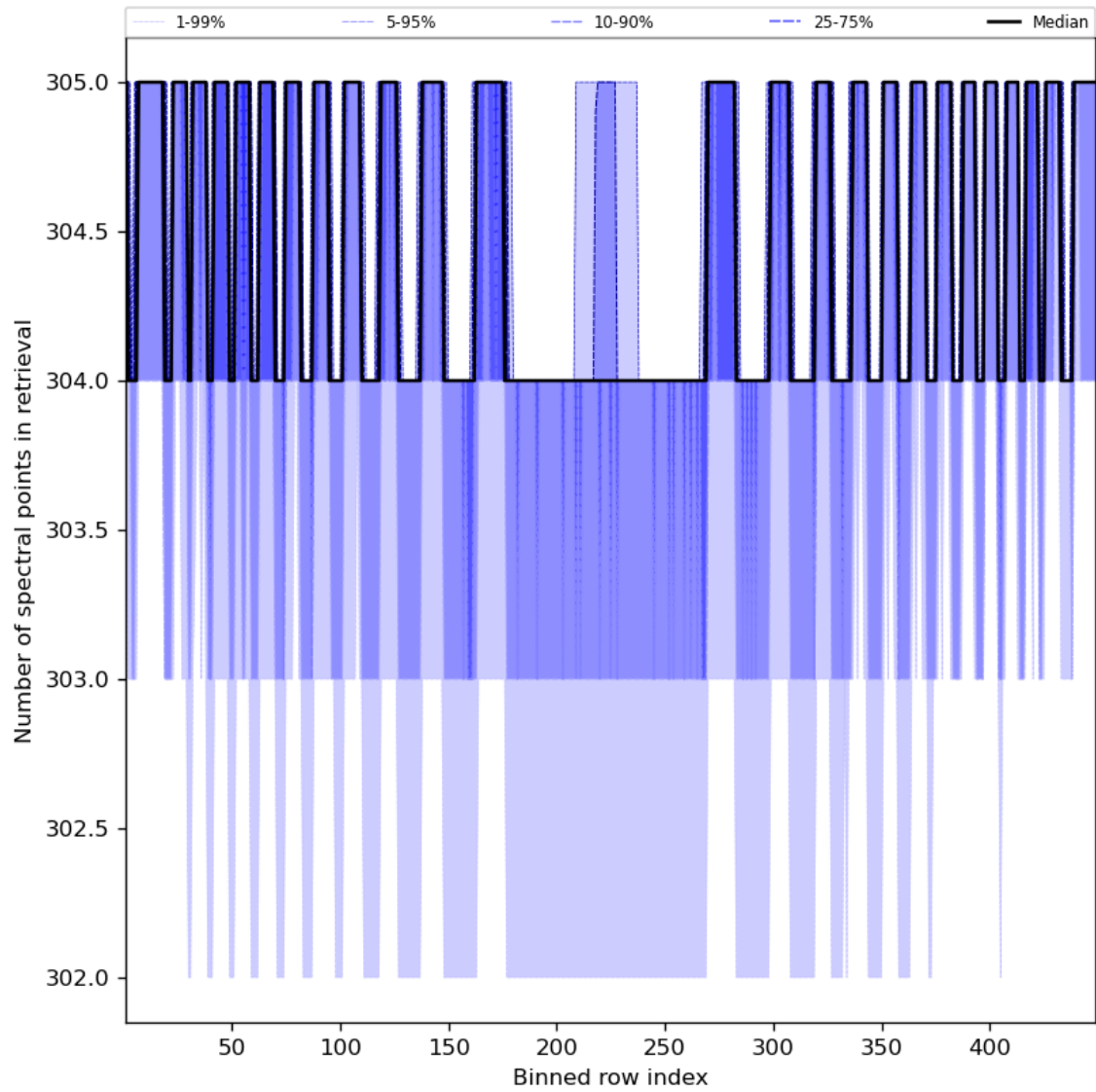
Figure 50: Along track statistics of “Number of spectral points in retrieval” for 2024-04-23 to 2024-04-25
