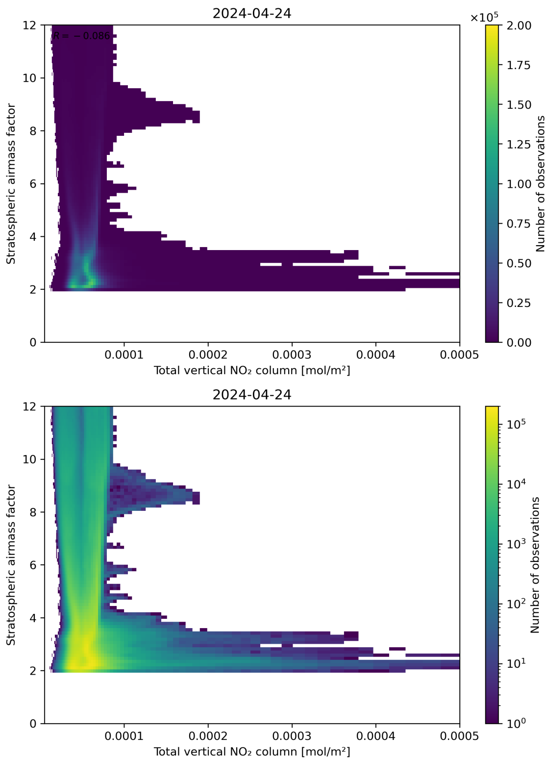
Figure 110: Scatter density plot of “Total vertical NO 2 column” against “Stratospheric airmass factor” for 2024-04-23 to 2024-04-25.
