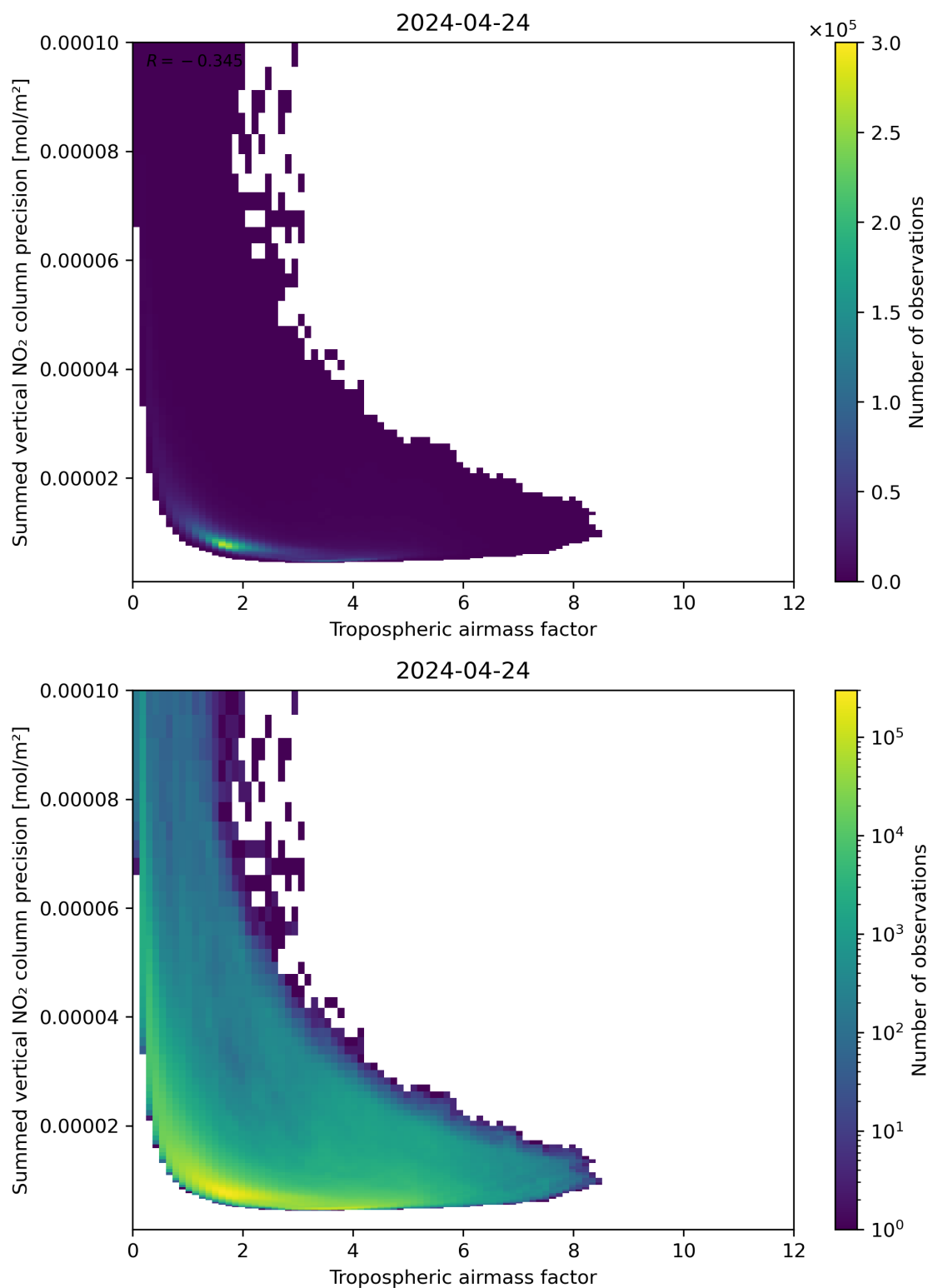
Figure 76: Scatter density plot of “Tropospheric air mass factor” against “Summed vertical NO 2 column precision” for 2024-04-23 to 2024-04-25.
