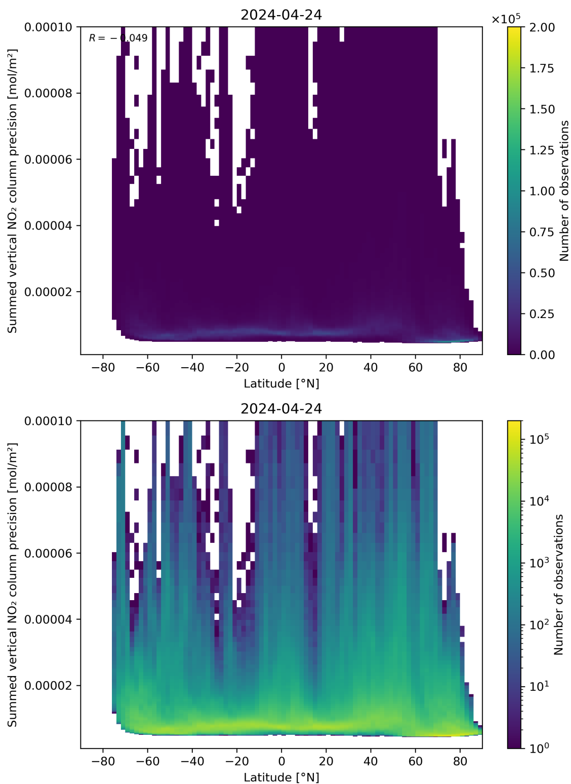
Figure 89: Scatter density plot of “Latitude” against “Summed vertical NO 2 column precision” for 2024-04-23 to 2024-04-25.
