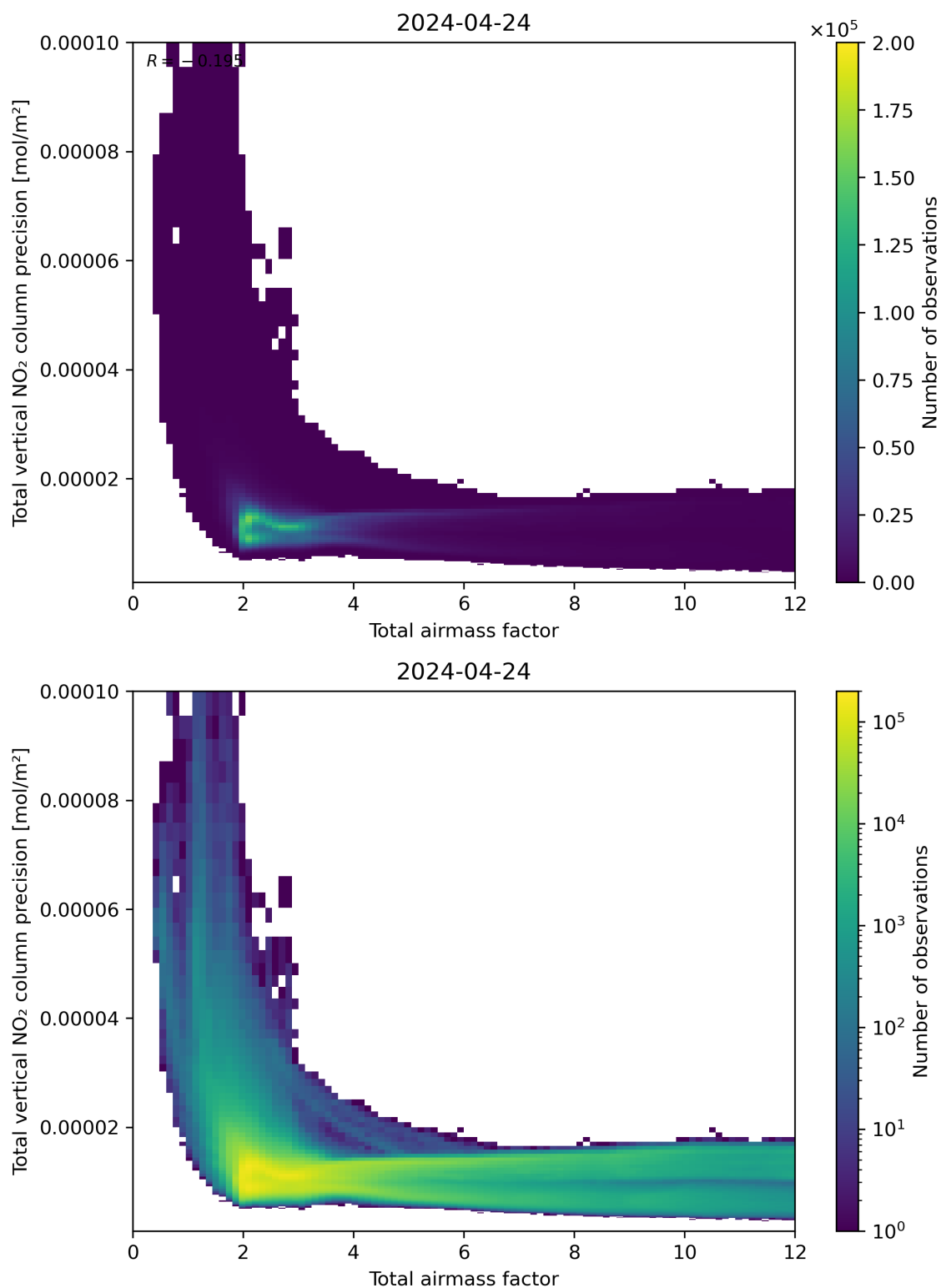
Figure 68: Scatter density plot of “Total airmass factor” against “Total vertical NO 2 column precision” for 2024-04-23 to 2024-04-25.
