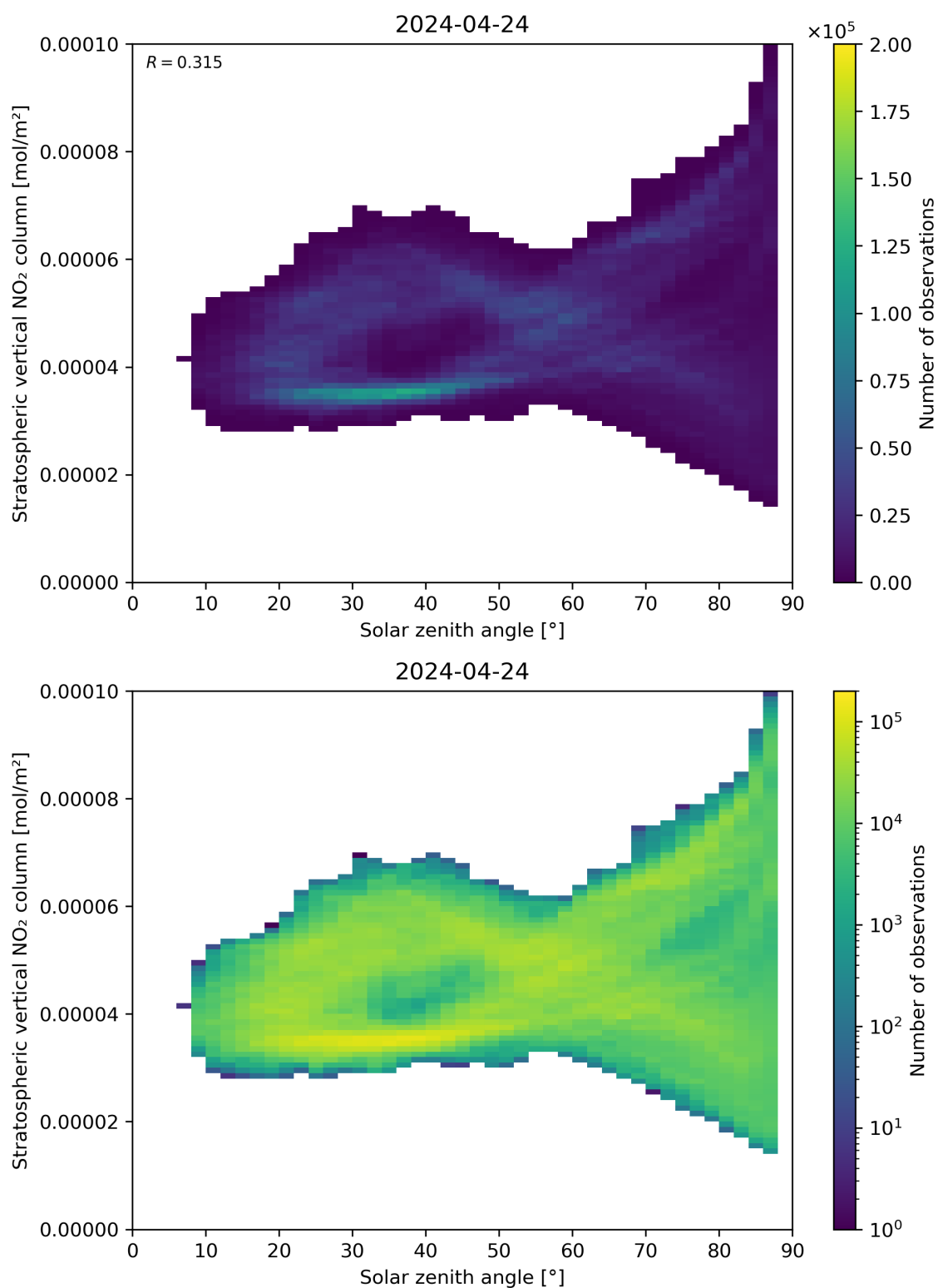
Figure 150: Scatter density plot of “Solar zenith angle” against “Stratospheric vertical NO 2 column” for 2024-04-23 to 2024-04-25.
