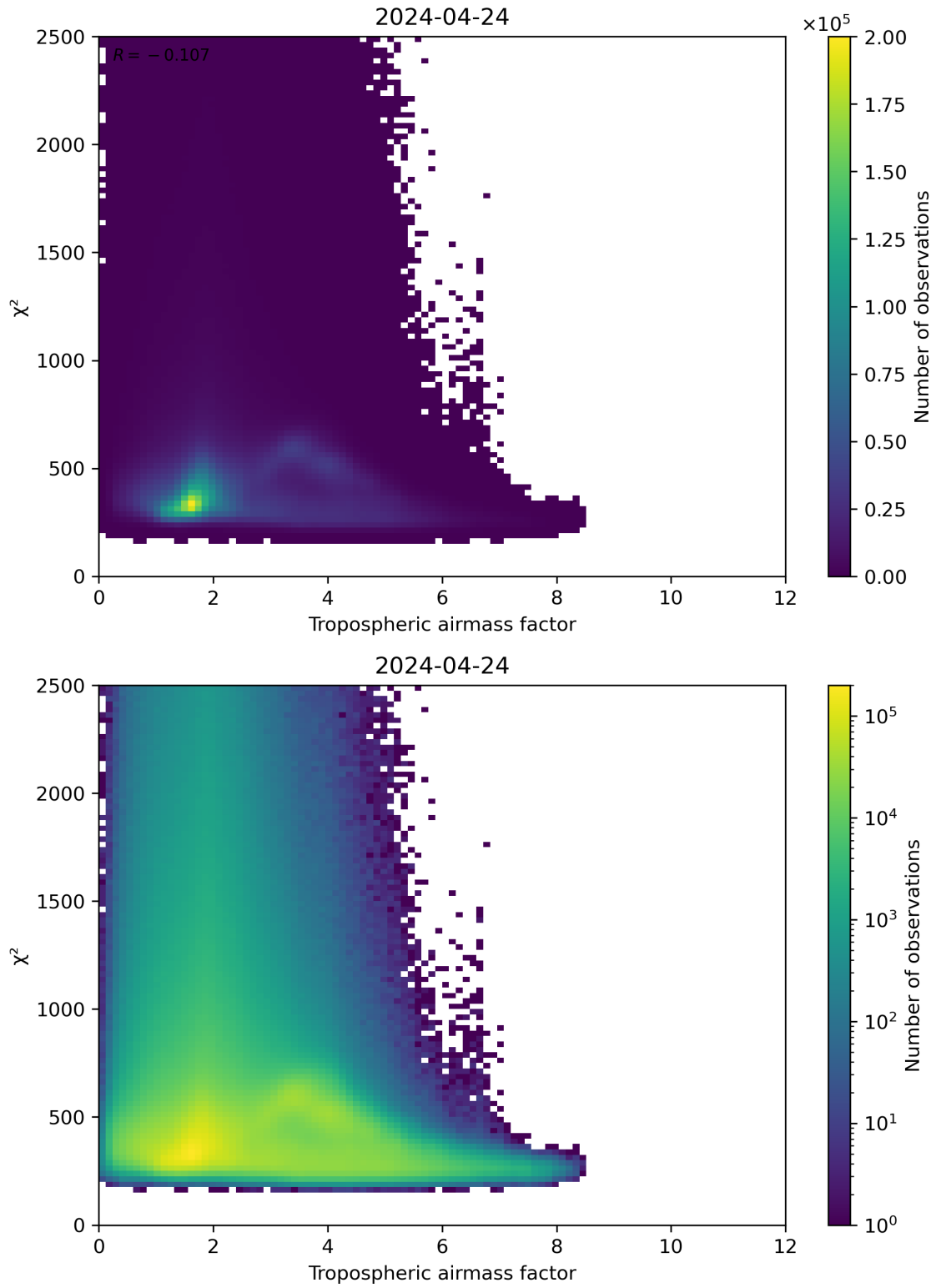
Figure 73: Scatter density plot of “Tropospheric airmass factor” against “ \chi^2 ” for 2024-04-23 to 2024-04-25.
