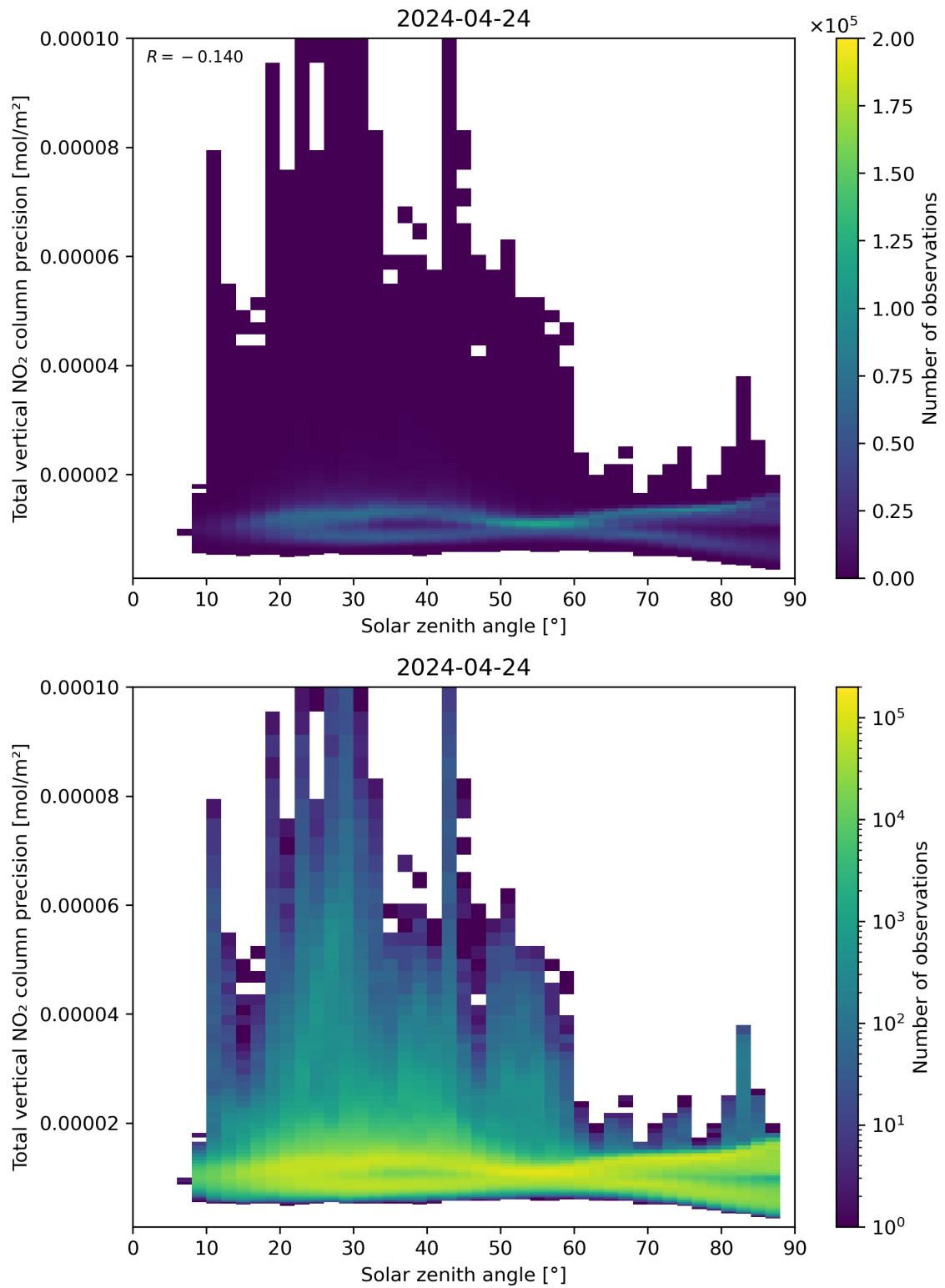
Figure 154: Scatter density plot of “Solar zenith angle” against “Total vertical NO 2 column precision” for 2024-04-23 to 2024-04-25.
