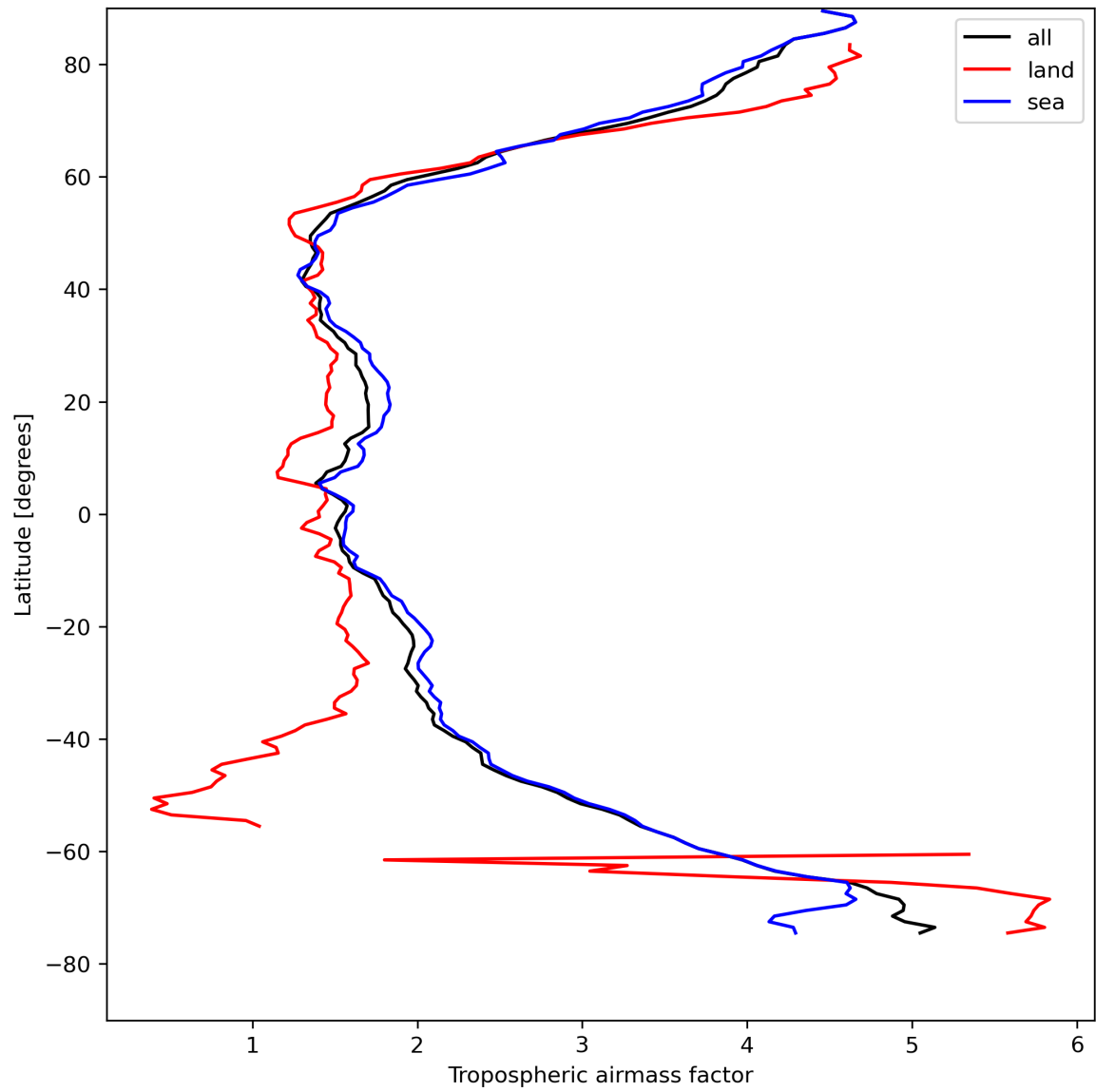
Figure 14: Zonal average of “Tropospheric airmass factor” for 2024-04-23 to 2024-04-25.
