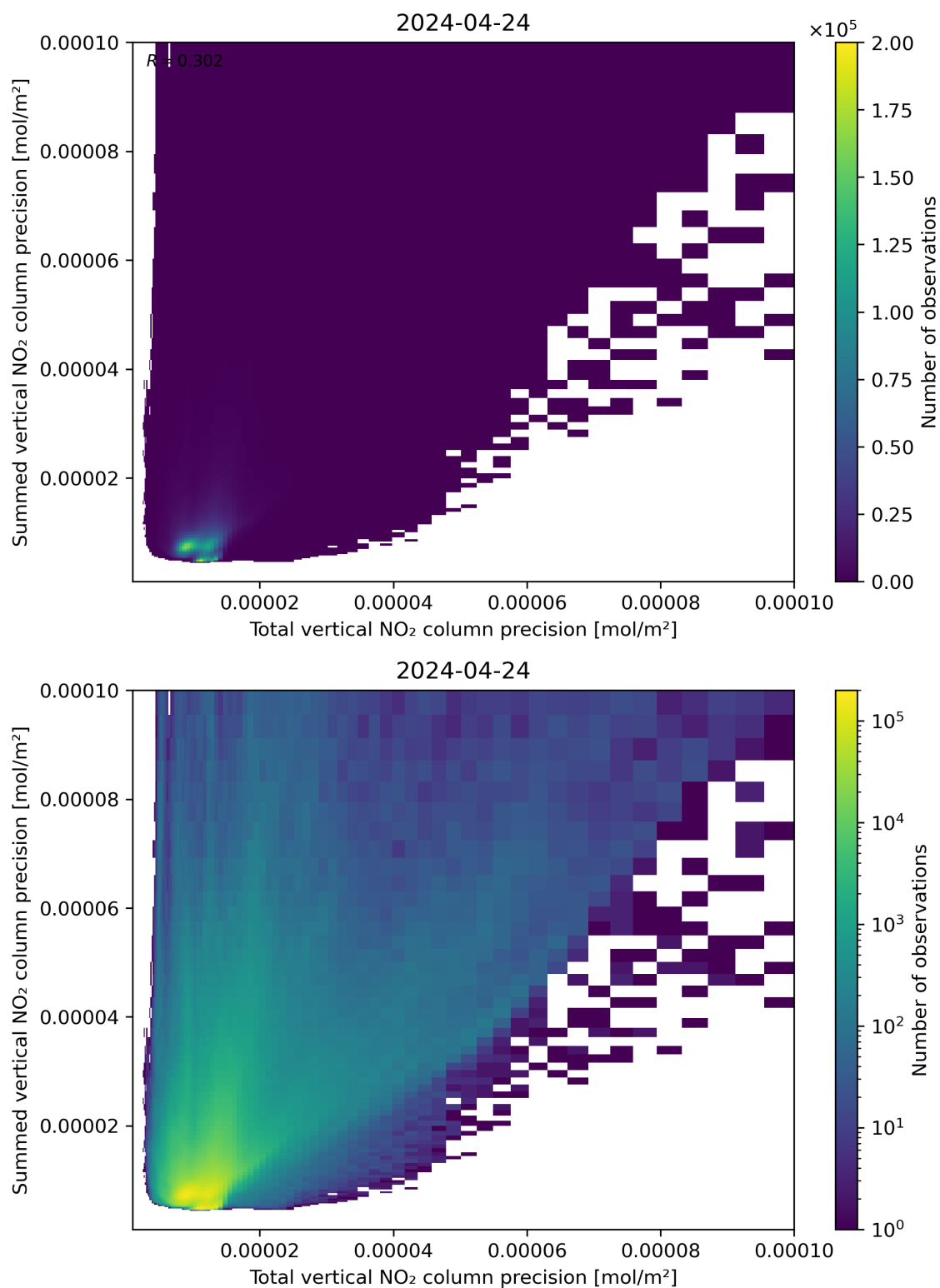
Figure 118: Scatter density plot of “Total vertical NO 2 column precision” against “Summed vertical NO 2 column precision” for 2024-04-23 to 2024-04-25.
