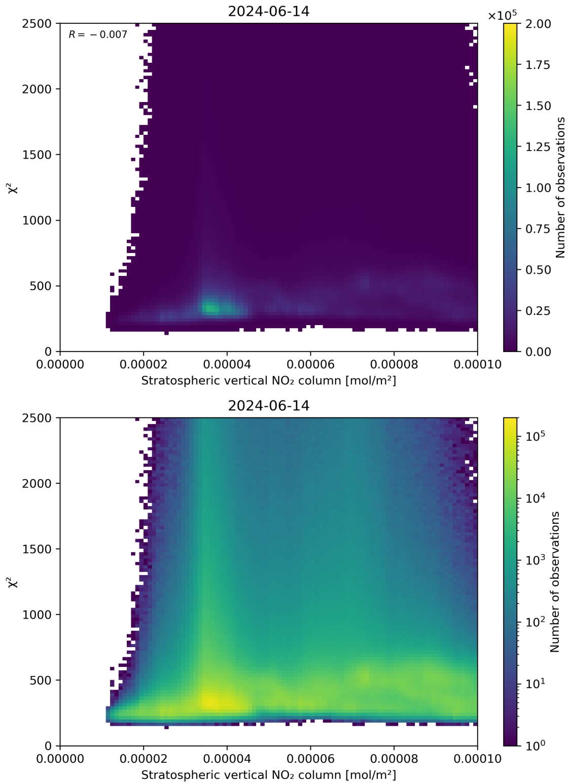
Figure 97: Scatter density plot of “Stratospheric vertical NO 2 column” against “ \chi^2 ” for 2024-06-13 to 2024-06-15.
