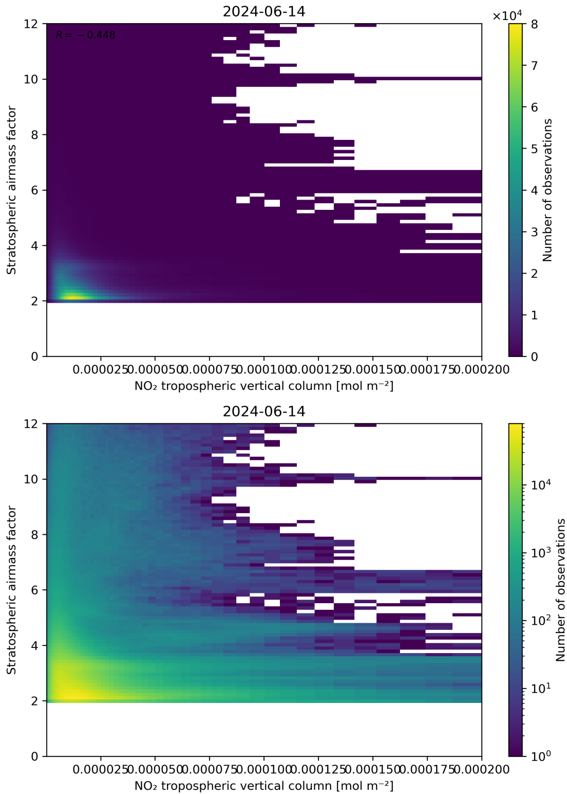
Figure 121: Scatter density plot of “NO 2 tropospheric vertical column” against “Stratospheric air mass factor” for 2024-06-13 to 2024-06-15.
