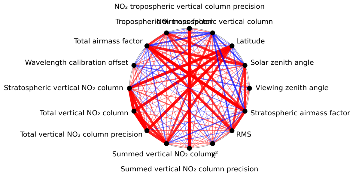
Figure 1: Map of correlation graph for 2024-06-13 to 2024-06-15.
