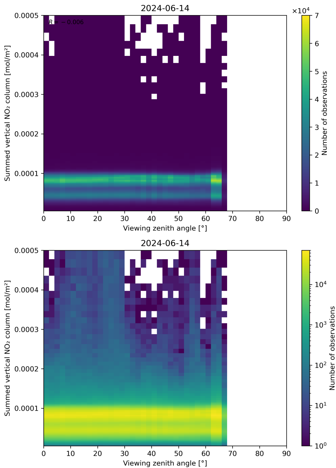
Figure 165: Scatter density plot of “Viewing zenith angle” against “Summed vertical NO 2 column” for 2024-06-13 to 2024-06-15.
