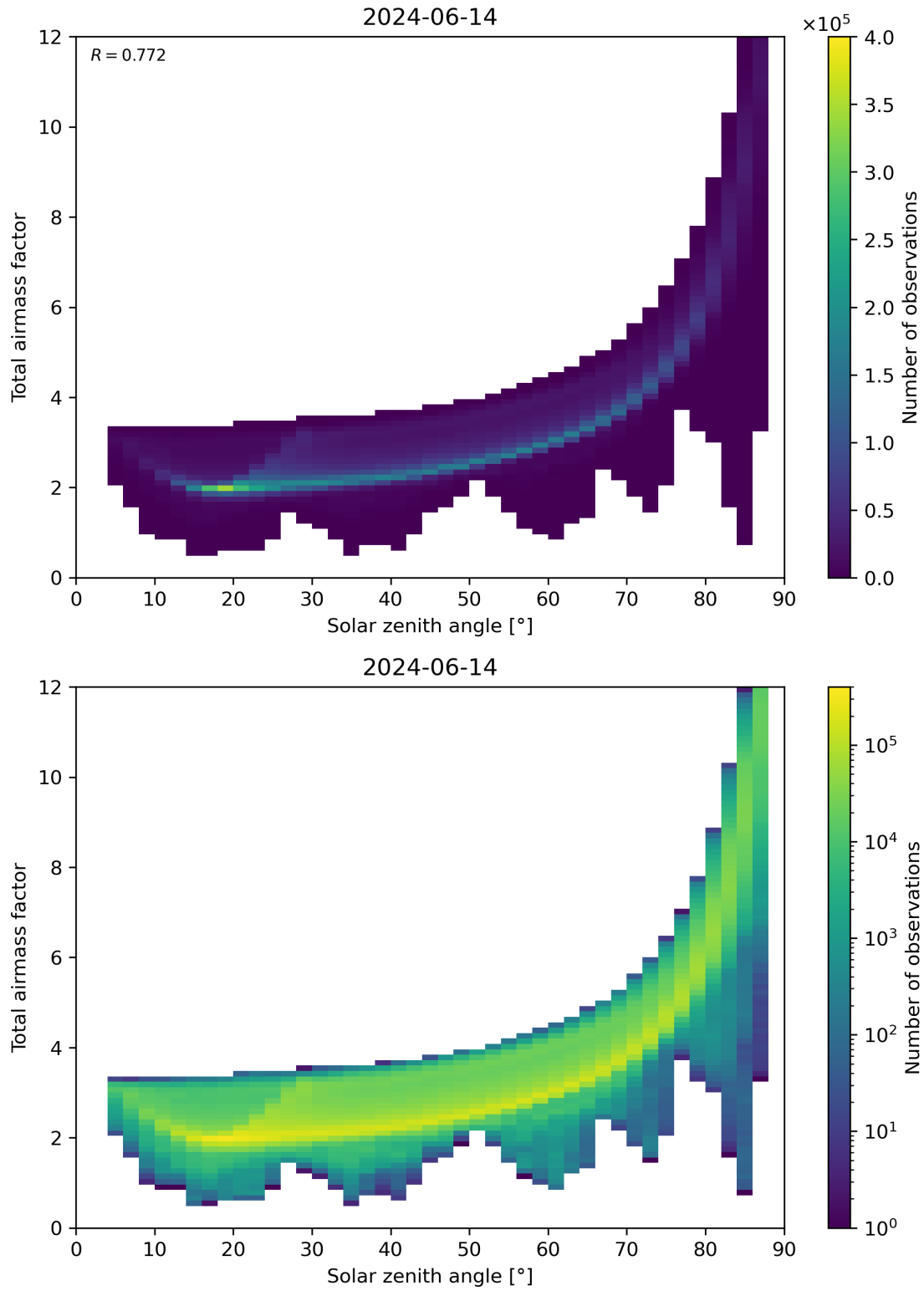
Figure 146: Scatter density plot of “Solar zenith angle” against “Total air mass factor” for 2024-06-13 to 2024-06-15.
