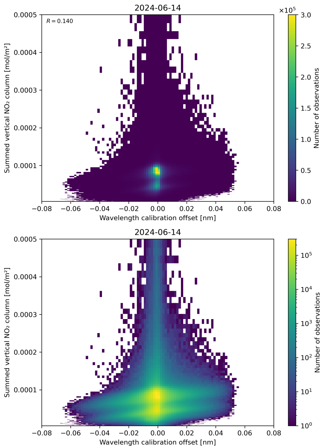
Figure 177: Scatter density plot of “Wavelength calibration offset” against “Summed vertical NO 2 column” for 2024-06-13 to 2024-06-15.
