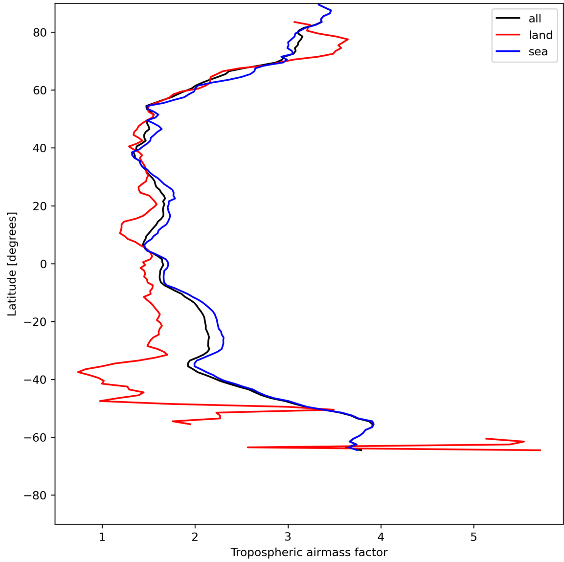
Figure 14: Zonal average of “Tropospheric airmass factor” for 2024-06-13 to 2024-06-15.
