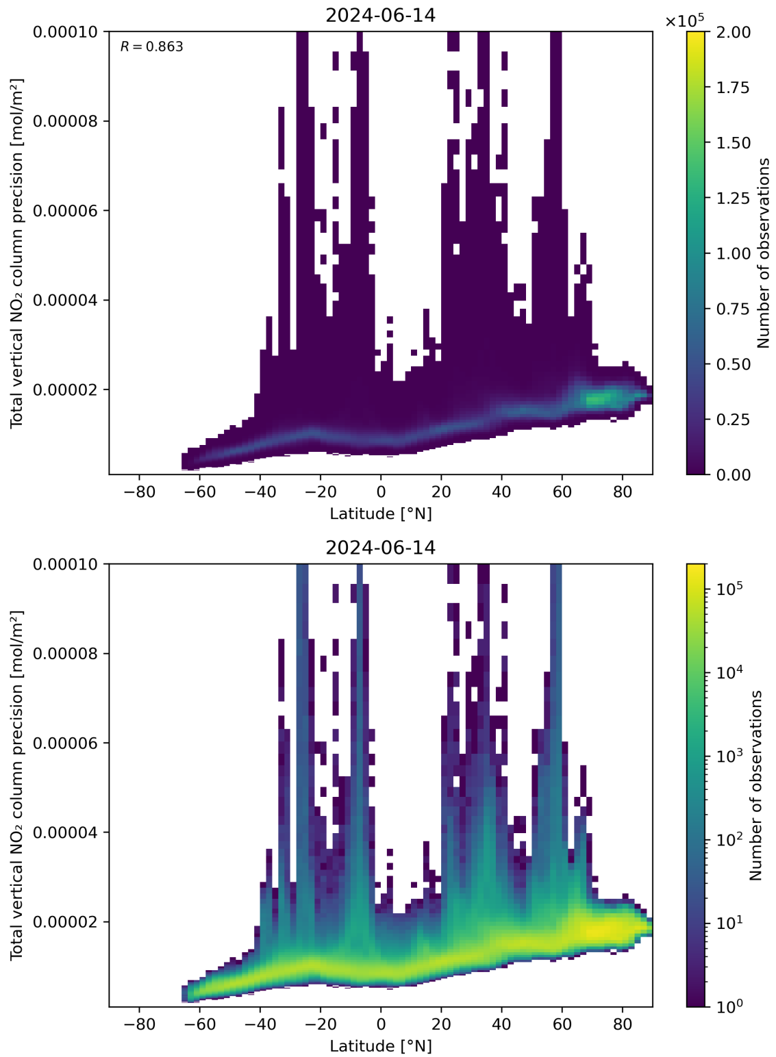
Figure 91: Scatter density plot of “Latitude” against “Total vertical NO 2 column precision” for 2024-06-13 to 2024-06-15.
