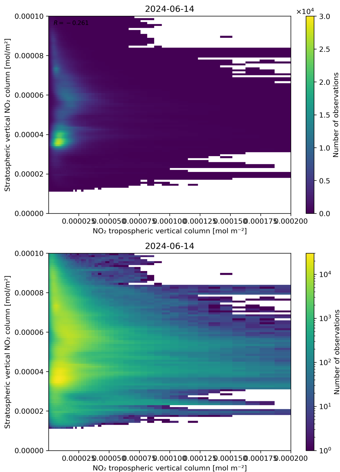
Figure 125: Scatter density plot of “NO 2 tropospheric vertical column” against “Stratospheric vertical NO 2 column” for 2024-06-13 to 2024-06-15.
