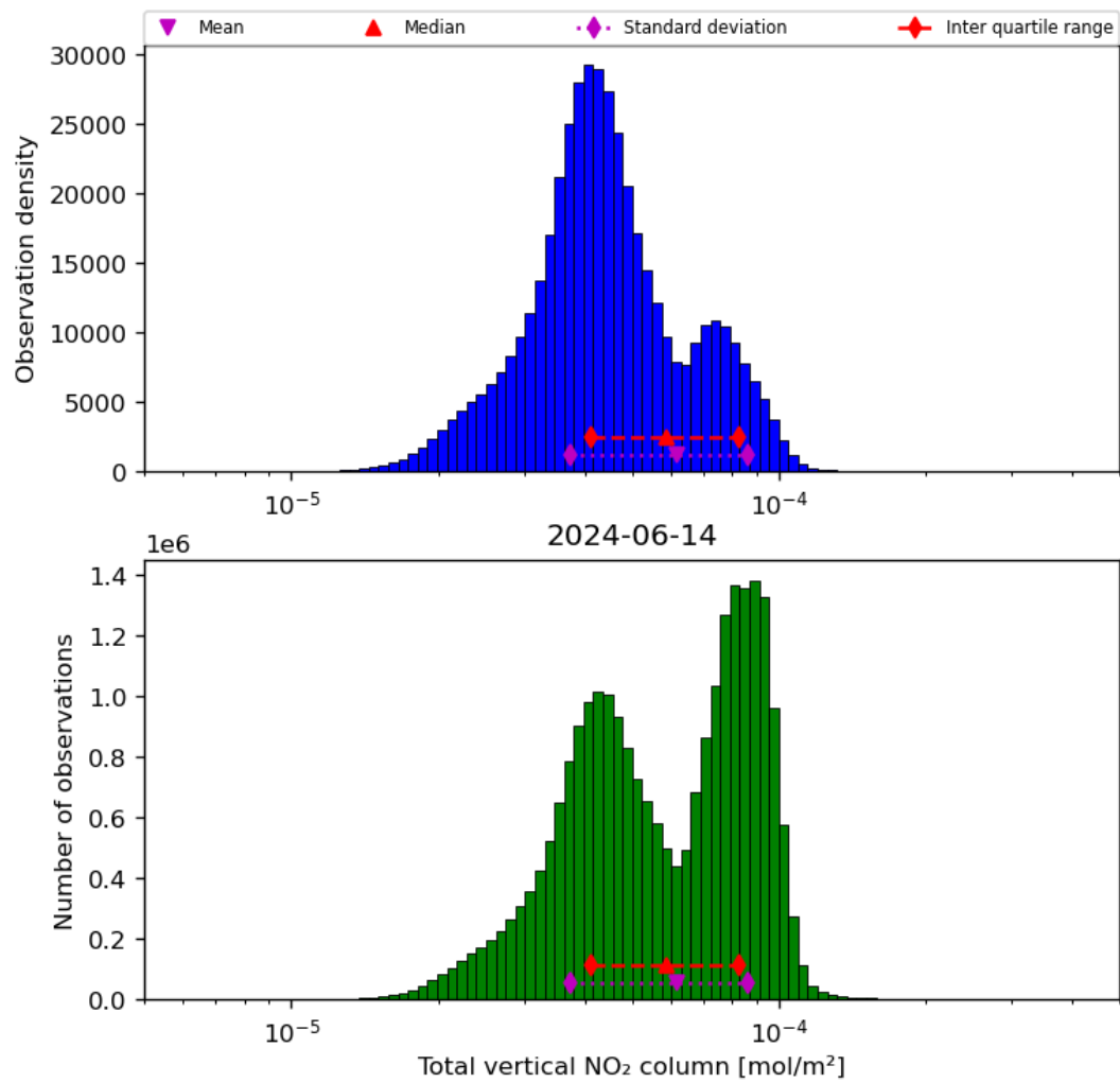
Figure 38: Histogram of “Total vertical NO 2 column” for 2024-06-13 to 2024-06-15
