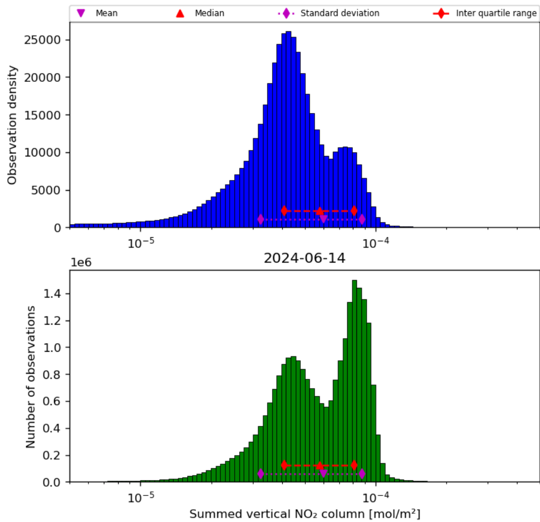
Figure 40: Histogram of “Summed vertical NO 2 column” for 2024-06-13 to 2024-06-15
