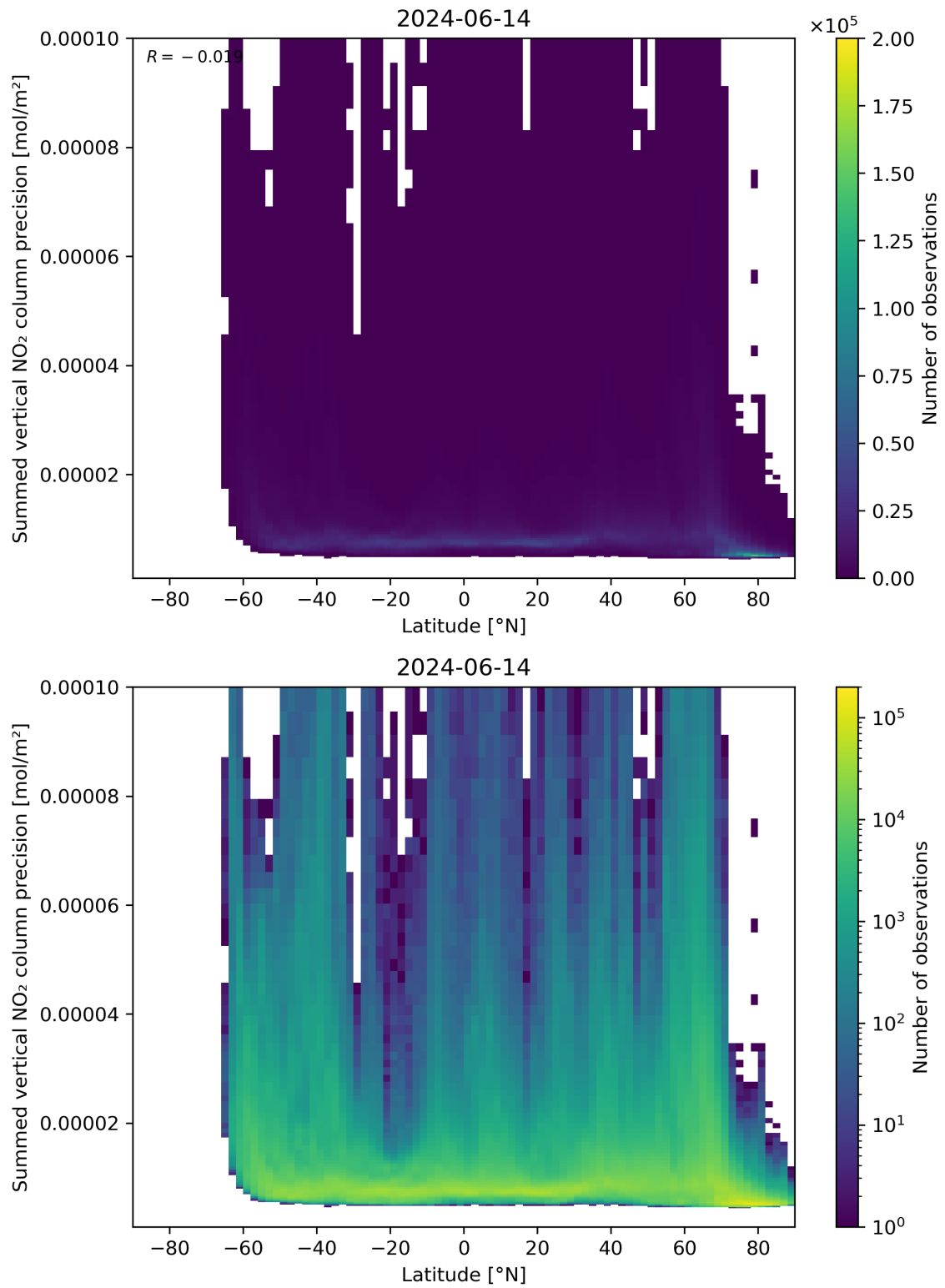
Figure 89: Scatter density plot of “Latitude” against “Summed vertical NO 2 column precision” for 2024-06-13 to 2024-06-15.
