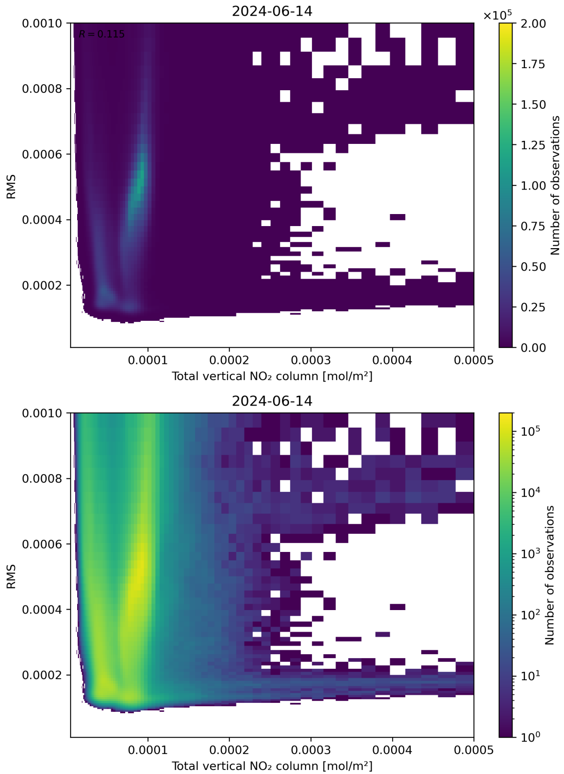
Figure 120: Scatter density plot of “Total vertical NO 2 column” against “RMS” for 2024-06-13 to 2024-06-15.
