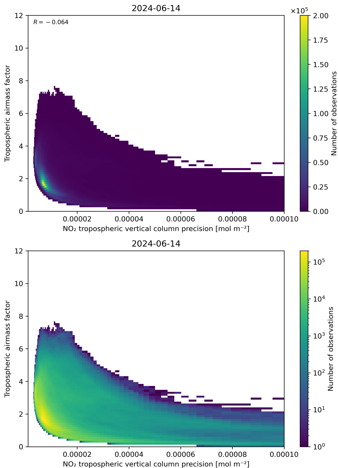
Figure 133: Scatter density plot of “NO 2 tropospheric vertical column precision” against “Tropospheric airmass factor” for 2024-06-13 to 2024-06-15.
