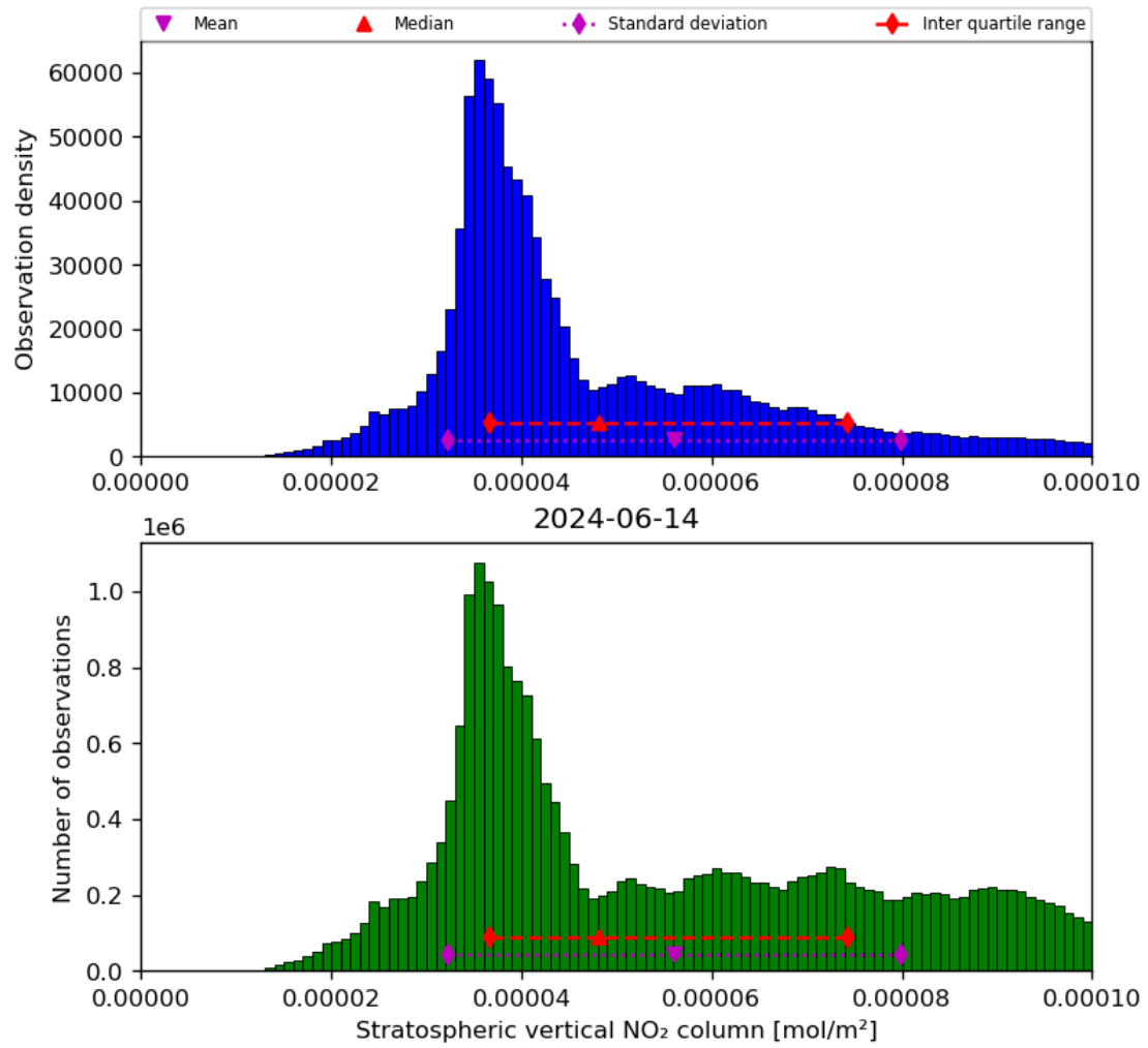
Figure 36: Histogram of “Stratospheric vertical NO 2 column” for 2024-06-13 to 2024-06-15
