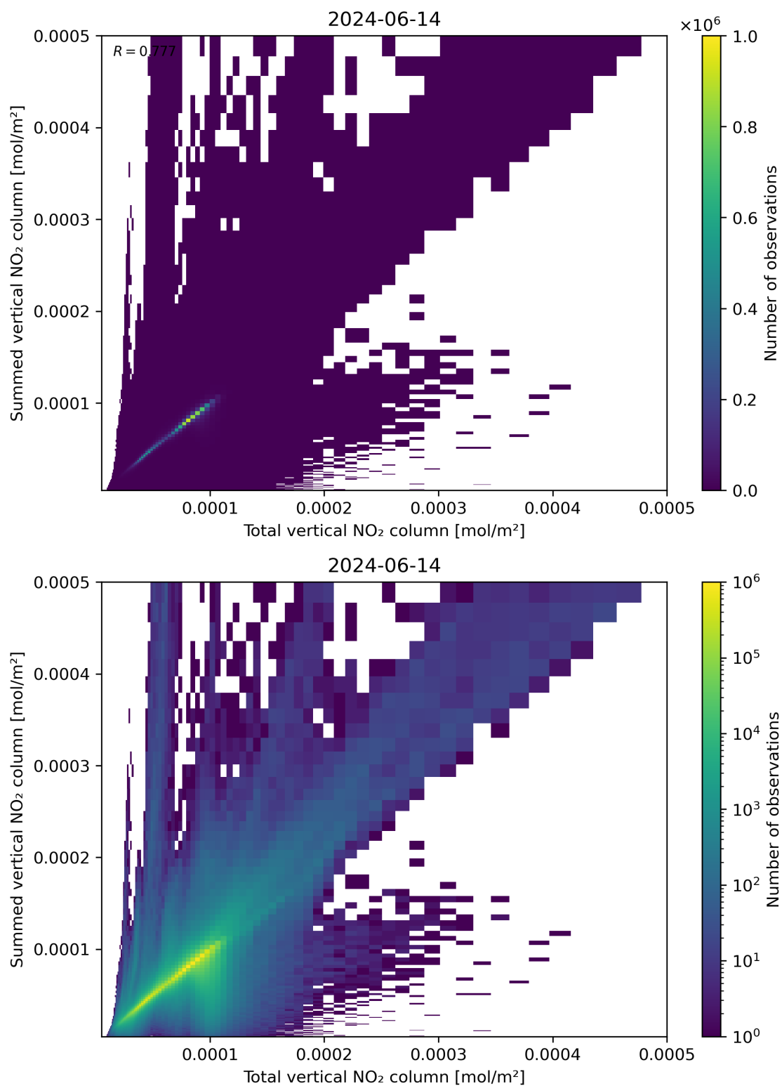
Figure 112: Scatter density plot of “Total vertical NO 2 column” against “Summed vertical NO 2 column” for 2024-06-13 to 2024-06-15.
