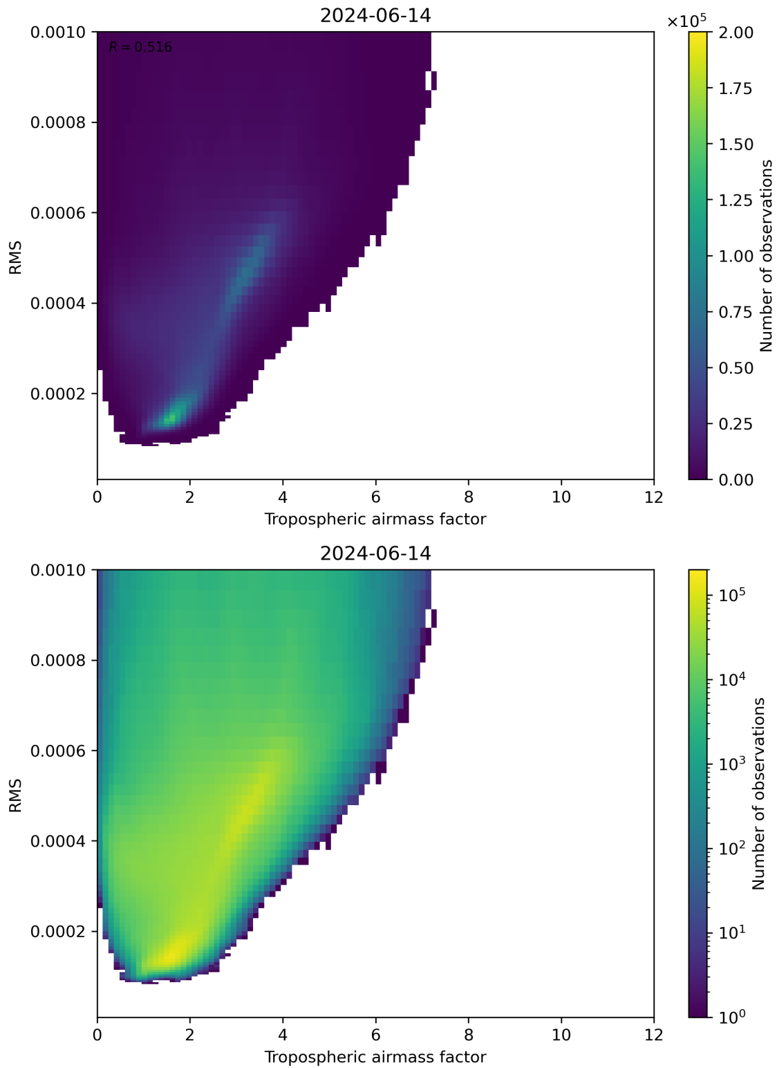
Figure 79: Scatter density plot of “Tropospheric airmass factor” against “RMS” for 2024-06-13 to 2024-06-15.
