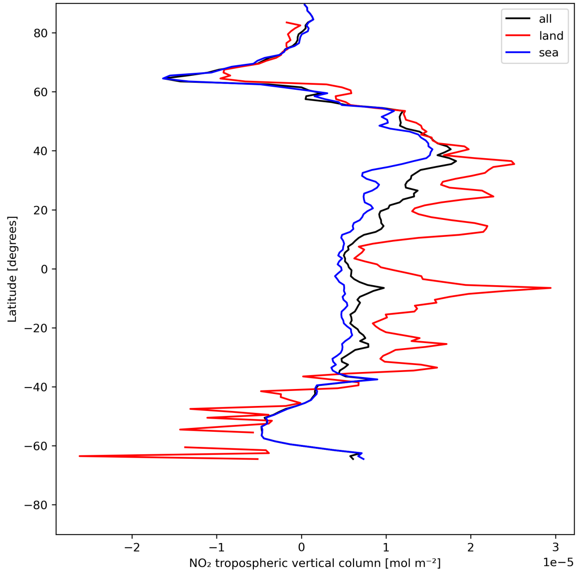
Figure 12: Zonal average of “NO 2 tropospheric vertical column” for 2024-06-13 to 2024-06-15.
