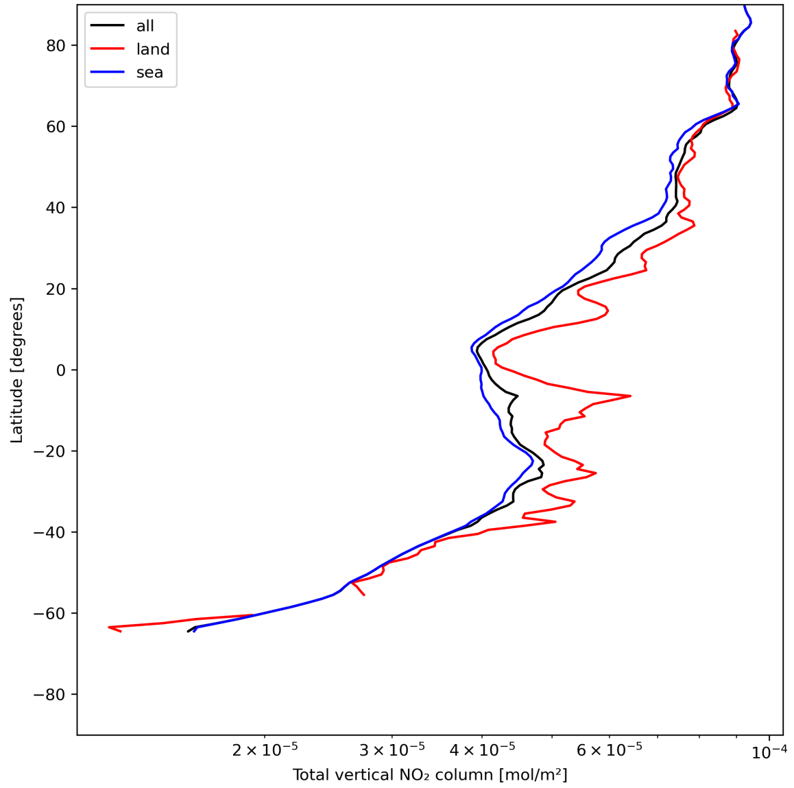
Figure 21: Zonal average of “Total vertical NO 2 column” for 2024-06-13 to 2024-06-15.
