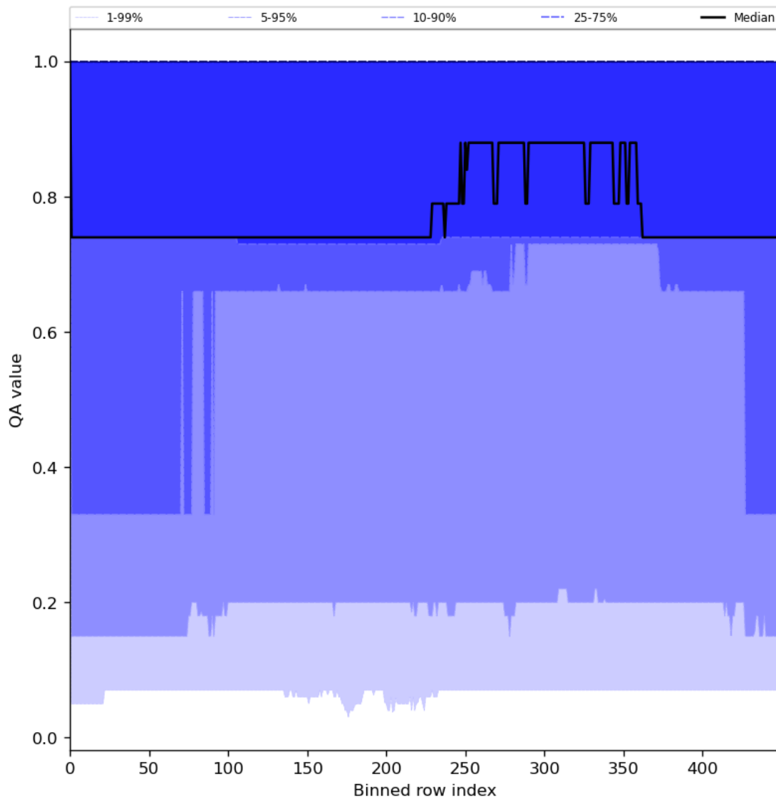
Figure 45: Along track statistics of “QA value” for 2024-06-13 to 2024-06-15
