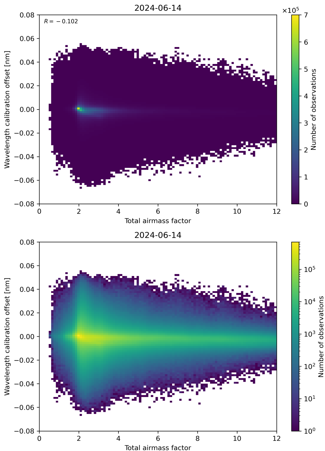
Figure 70: Scatter density plot of “Total airmass factor” against “Wavelength calibration offset” for 2024-06-13 to 2024-06-15.
