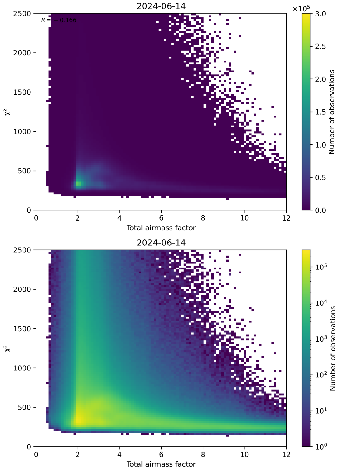
Figure 63: Scatter density plot of “Total airmass factor” against “ \chi^2 ” for 2024-06-13 to 2024-06-15.
