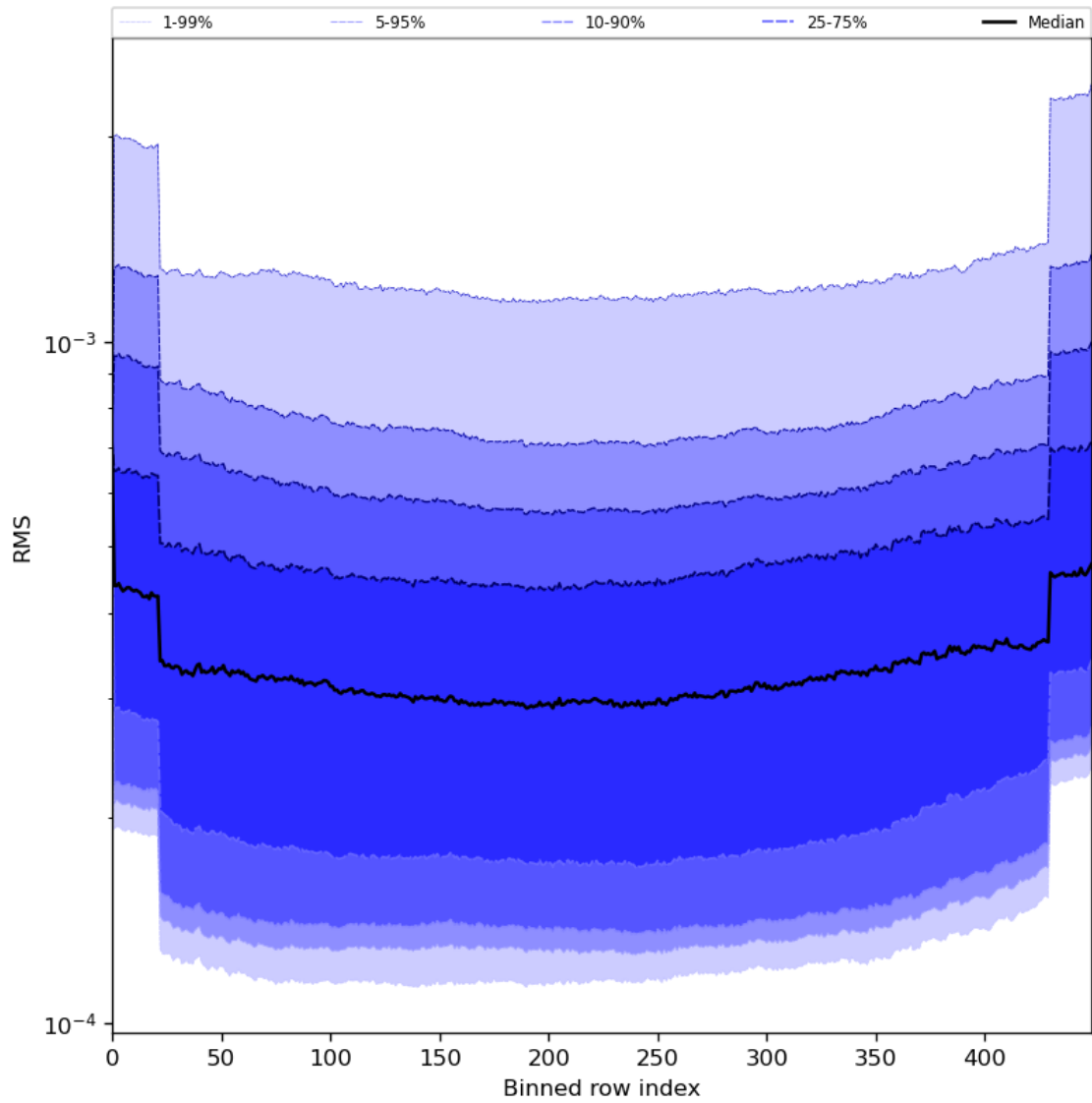
Figure 60: Along track statistics of “RMS” for 2024-06-13 to 2024-06-15
