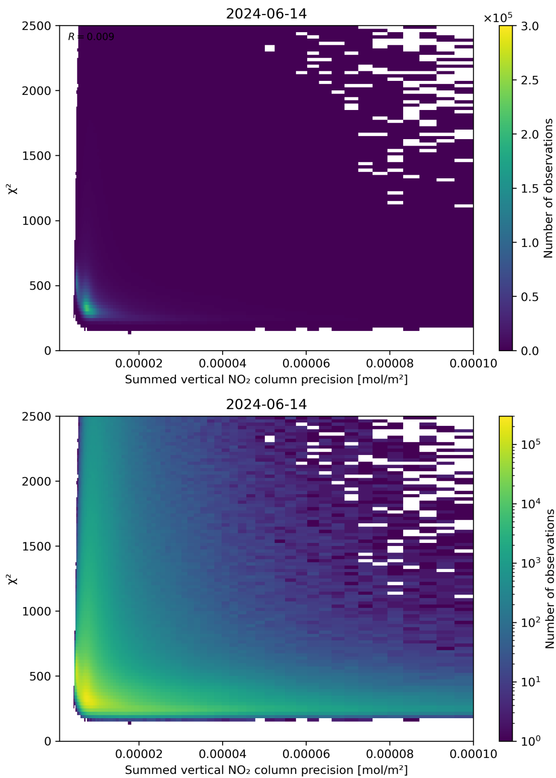
Figure 107: Scatter density plot of “Summed vertical NO 2 column precision” against “ \chi^2 ” for 2024-06-13 to 2024-06-15.
