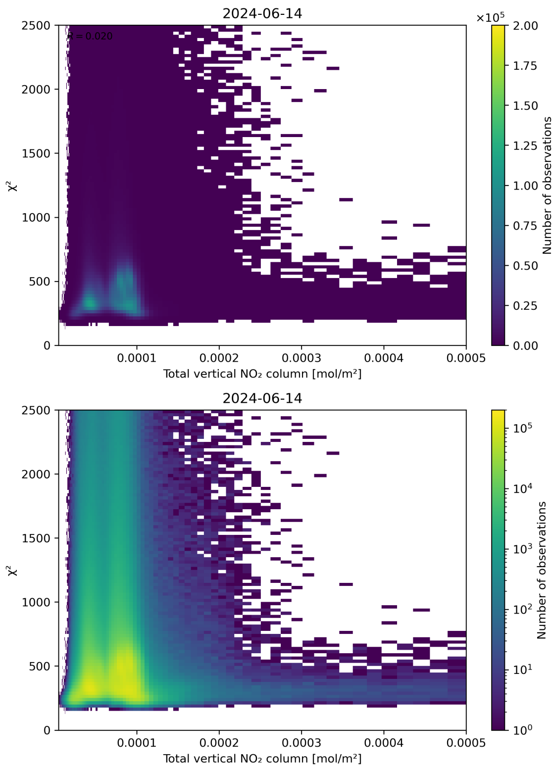
Figure 111: Scatter density plot of “Total vertical NO 2 column” against “ \chi^2 ” for 2024-06-13 to 2024-06-15.
