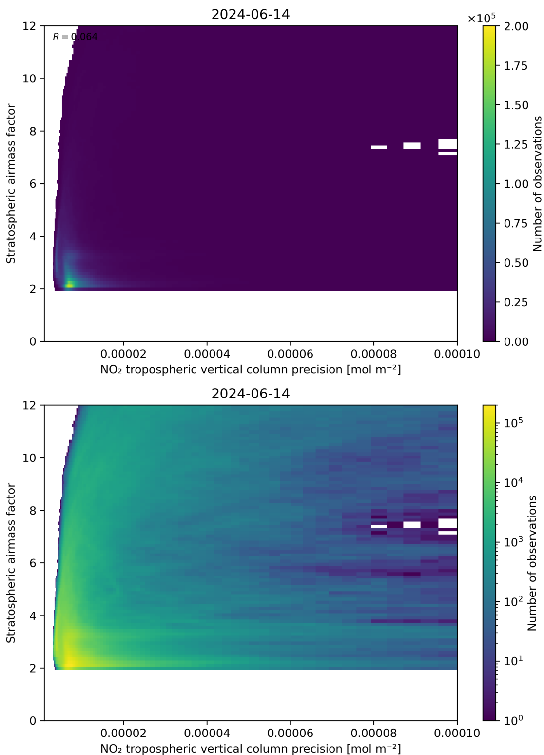
Figure 131: Scatter density plot of “NO 2 tropospheric vertical column precision” against “Stratospheric airmass factor” for 2024-06-13 to 2024-06-15.
