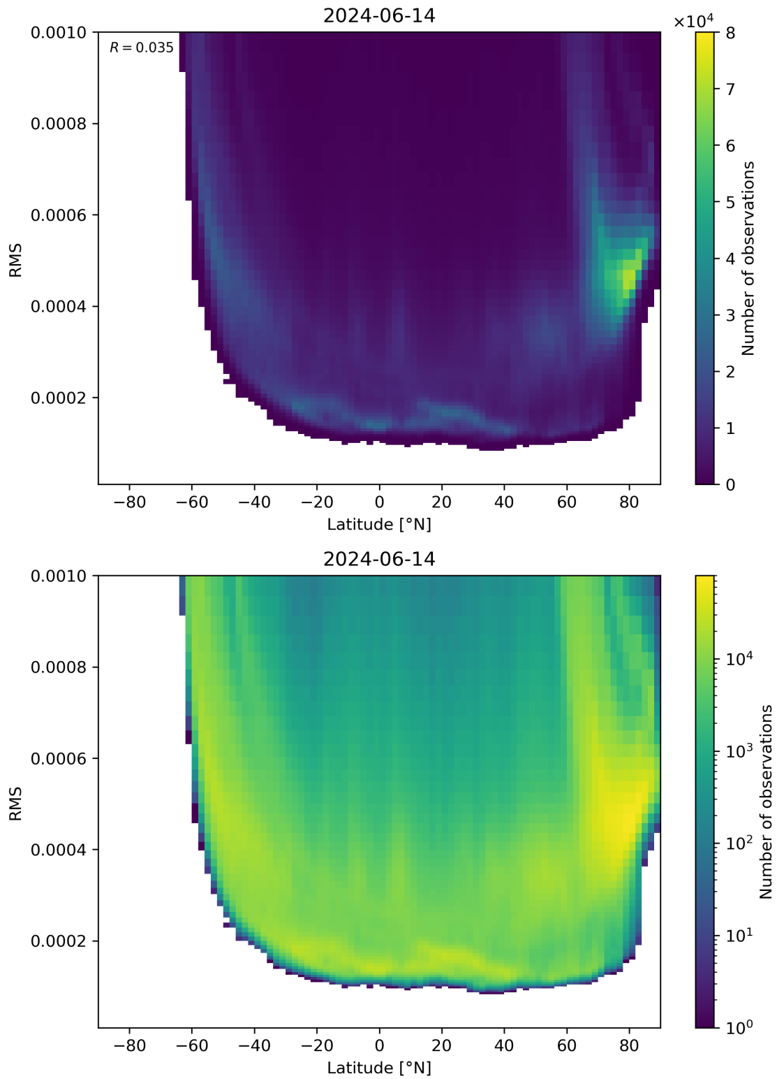
Figure 94: Scatter density plot of “Latitude” against “RMS” for 2024-06-13 to 2024-06-15.
