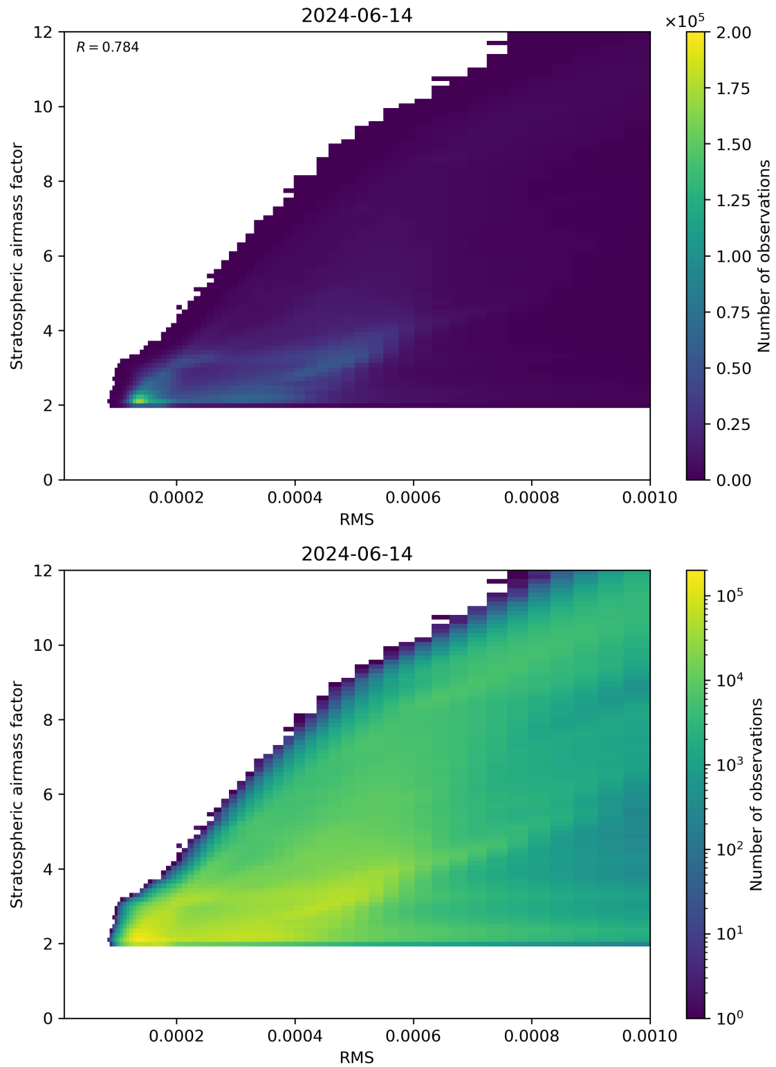
Figure 144: Scatter density plot of “RMS” against “Stratospheric airmass factor” for 2024-06-13 to 2024-06-15.
