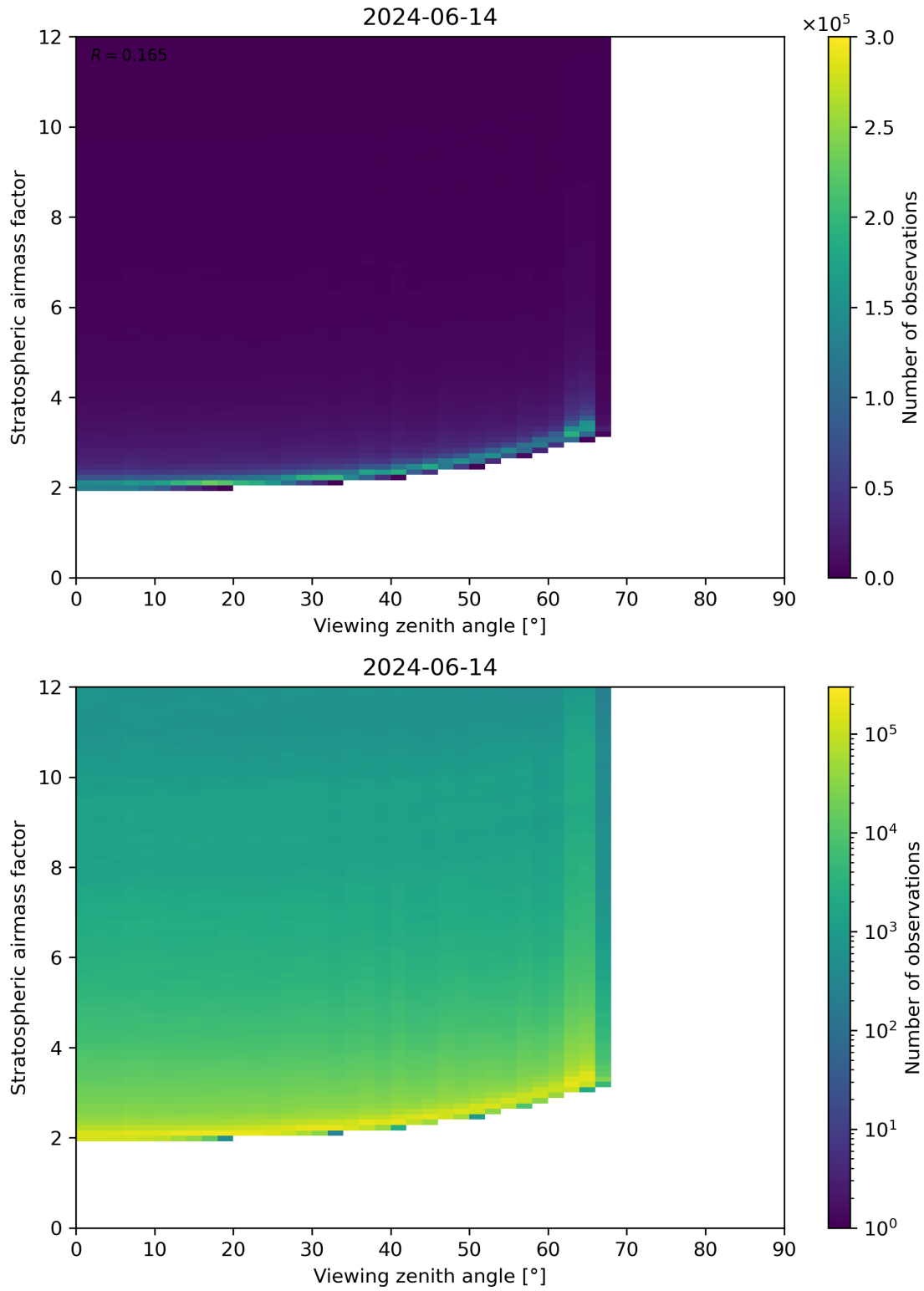
Figure 159: Scatter density plot of “Viewing zenith angle” against “Stratospheric airmass factor” for 2024-06-13 to 2024-06-15.
