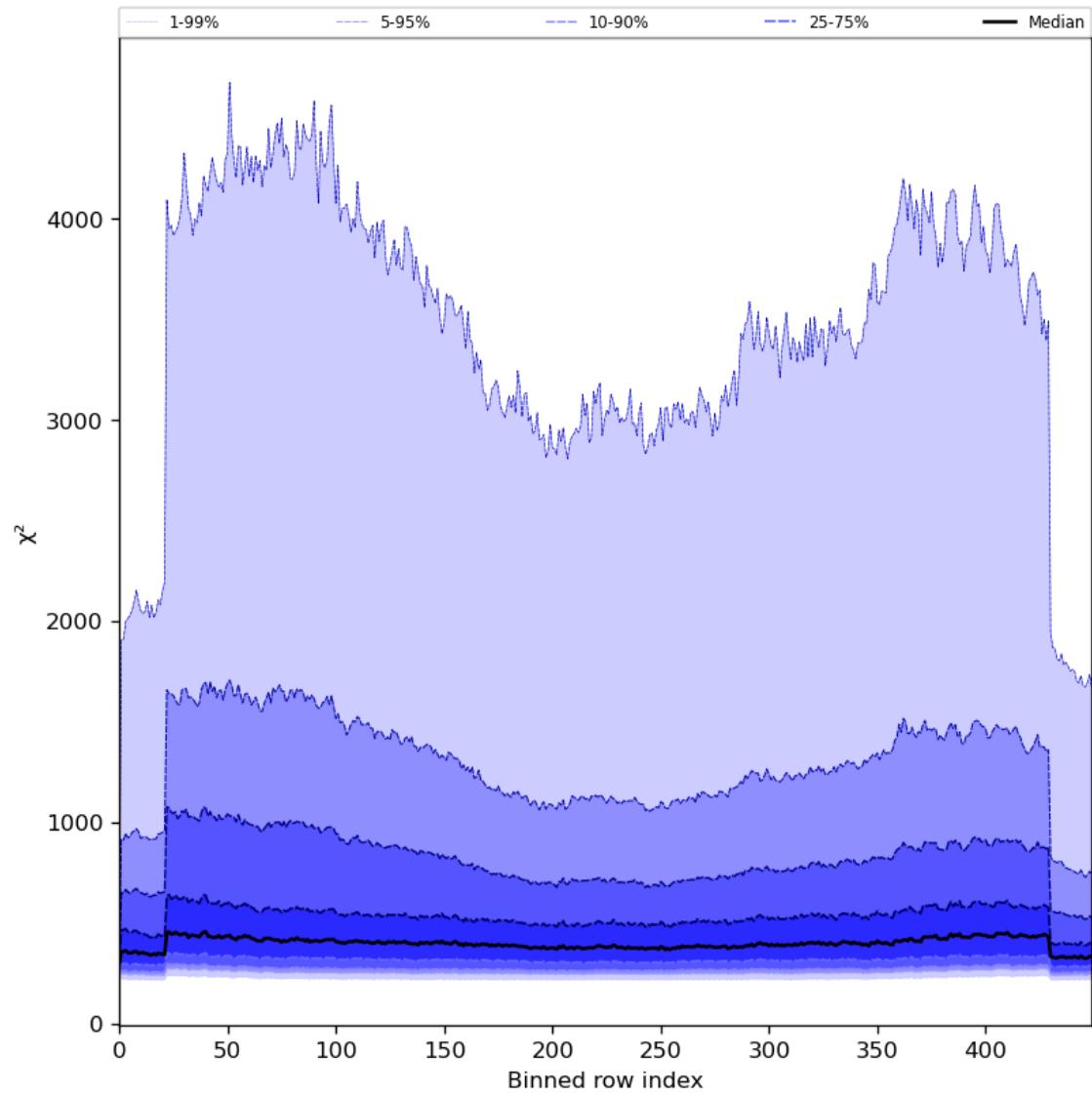
Figure 59: Along track statistics of “ \chi^2 ” for 2024-06-13 to 2024-06-15
