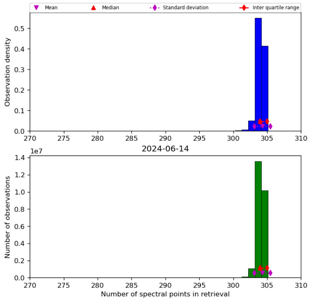
Figure 33: Histogram of “Number of spectral points in retrieval” for 2024-06-13 to 2024-06-15
