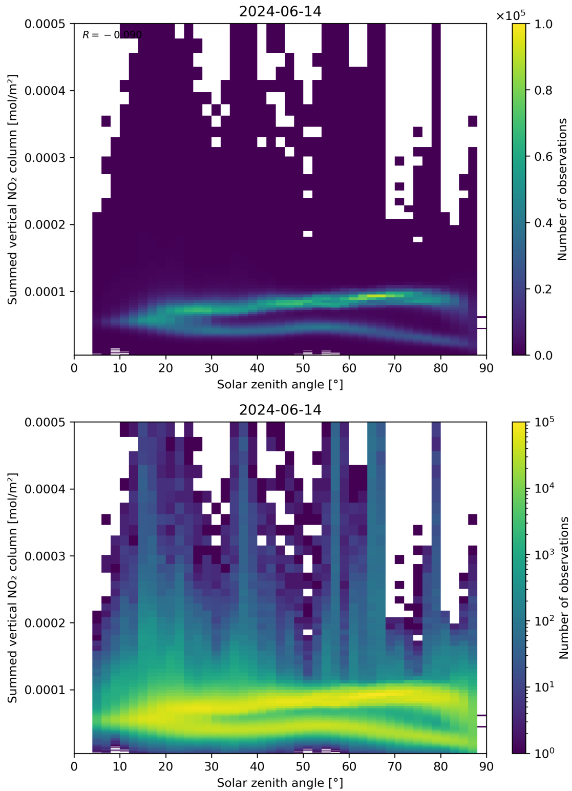
Figure 151: Scatter density plot of “Solar zenith angle” against “Summed vertical NO 2 column” for 2024-06-13 to 2024-06-15.
