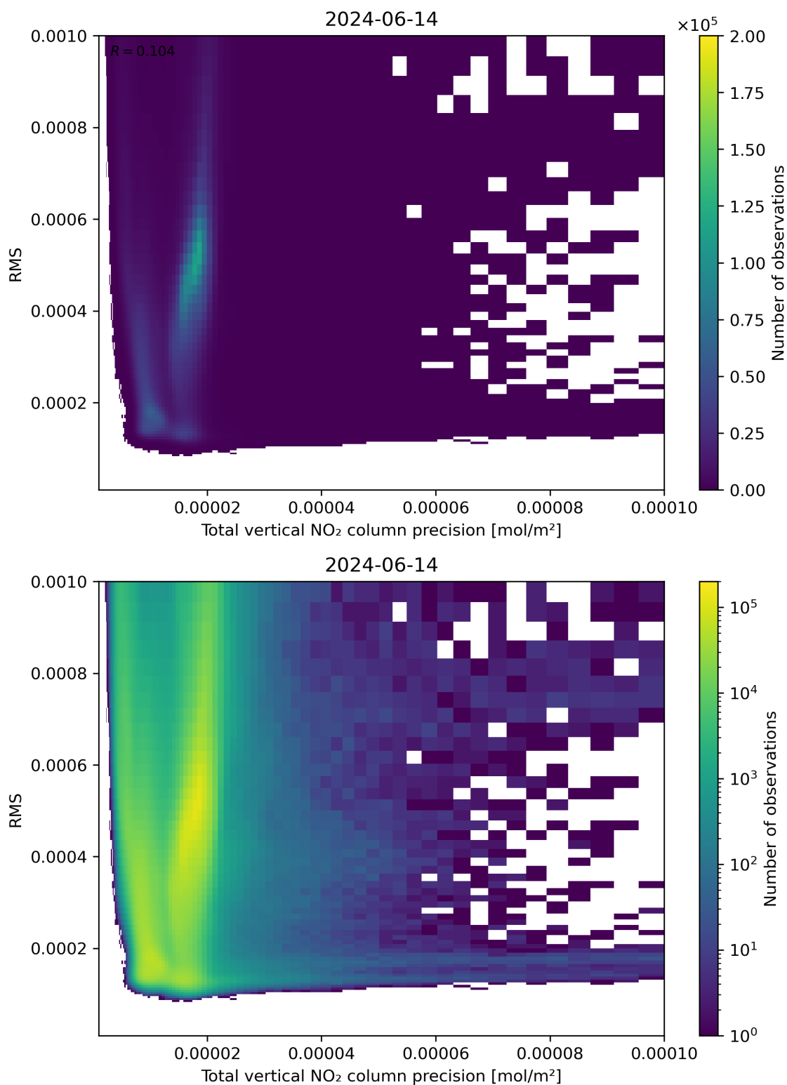
Figure 119: Scatter density plot of “Total vertical NO 2 column precision” against “RMS” for 2024-06-13 to 2024-06-15.
