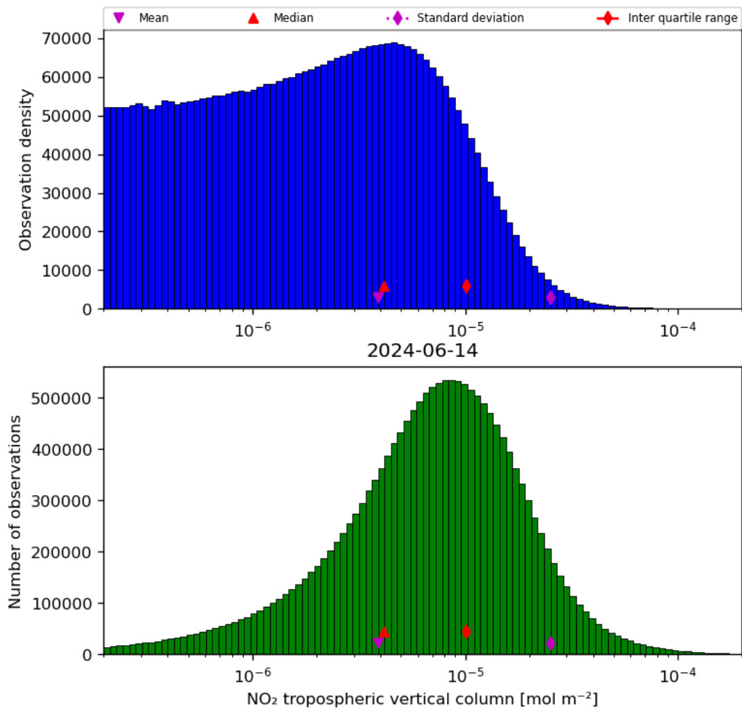
Figure 29: Histogram of “NO 2 tropospheric vertical column” for 2024-06-13 to 2024-06-15
