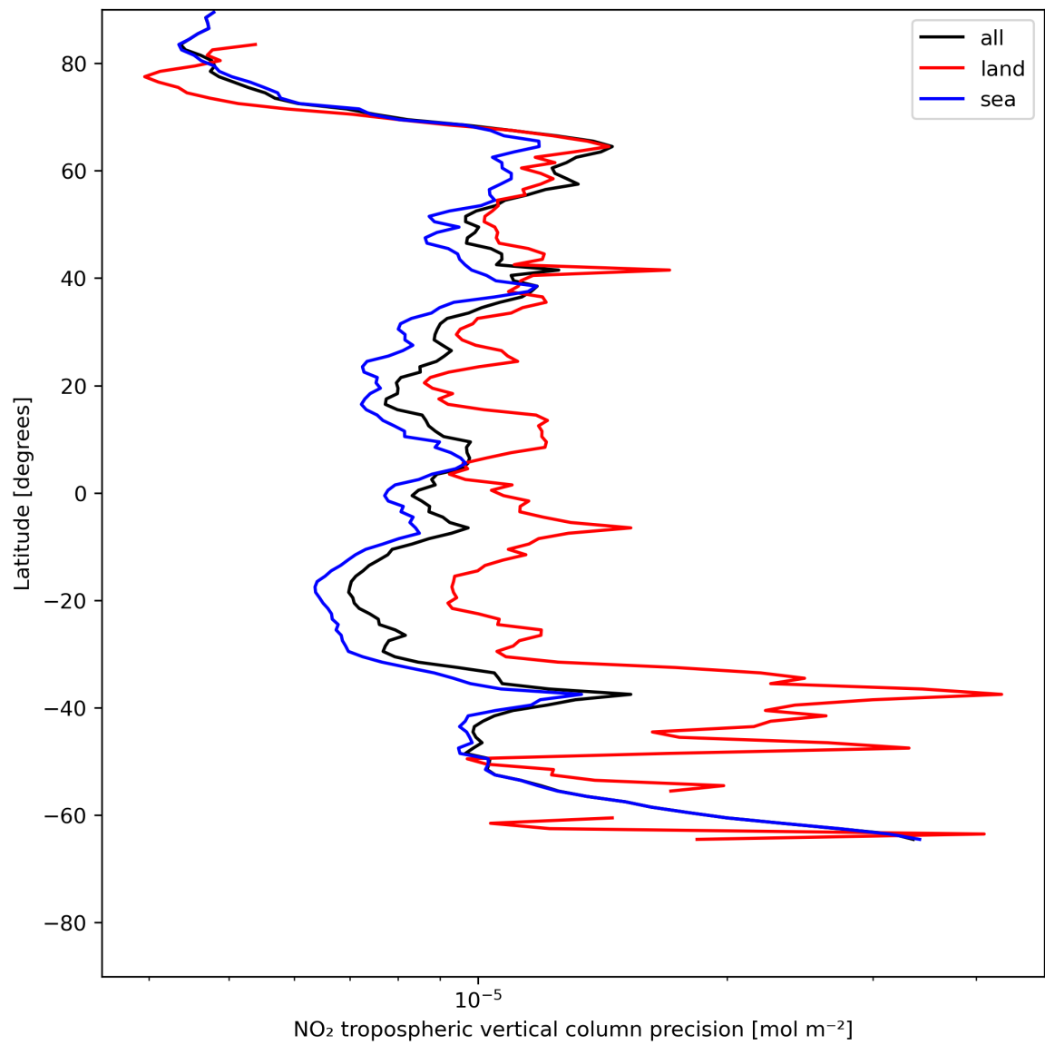
Figure 13: Zonal average of “NO 2 tropospheric vertical column precision” for 2024-06-13 to 2024-06-15.
