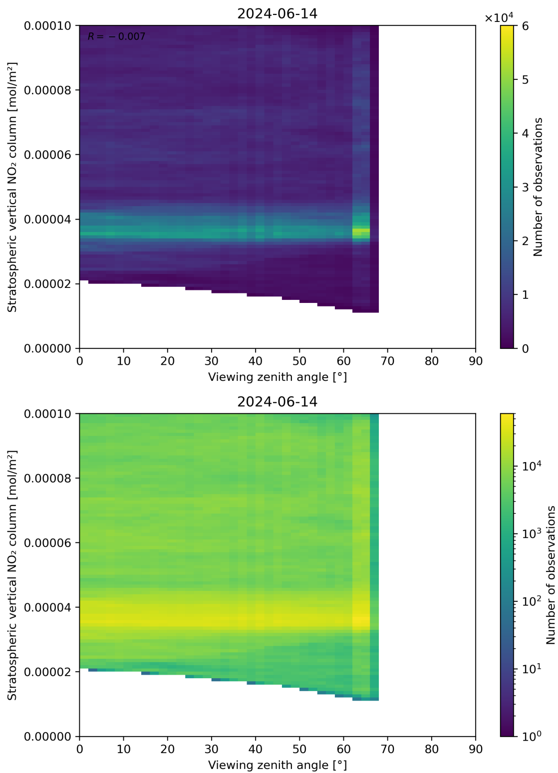
Figure 164: Scatter density plot of “Viewing zenith angle” against “Stratospheric vertical NO 2 column” for 2024-06-13 to 2024-06-15.
