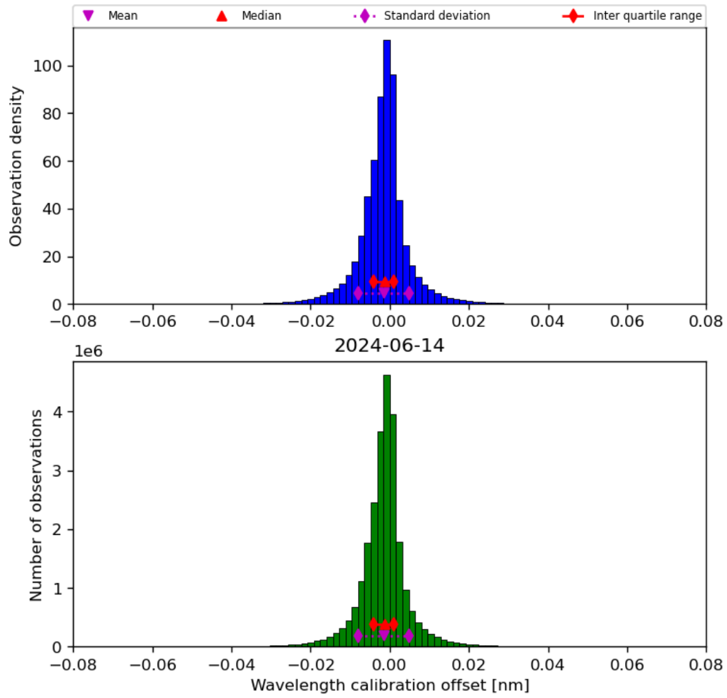
Figure 35: Histogram of “Wavelength calibration offset” for 2024-06-13 to 2024-06-15
