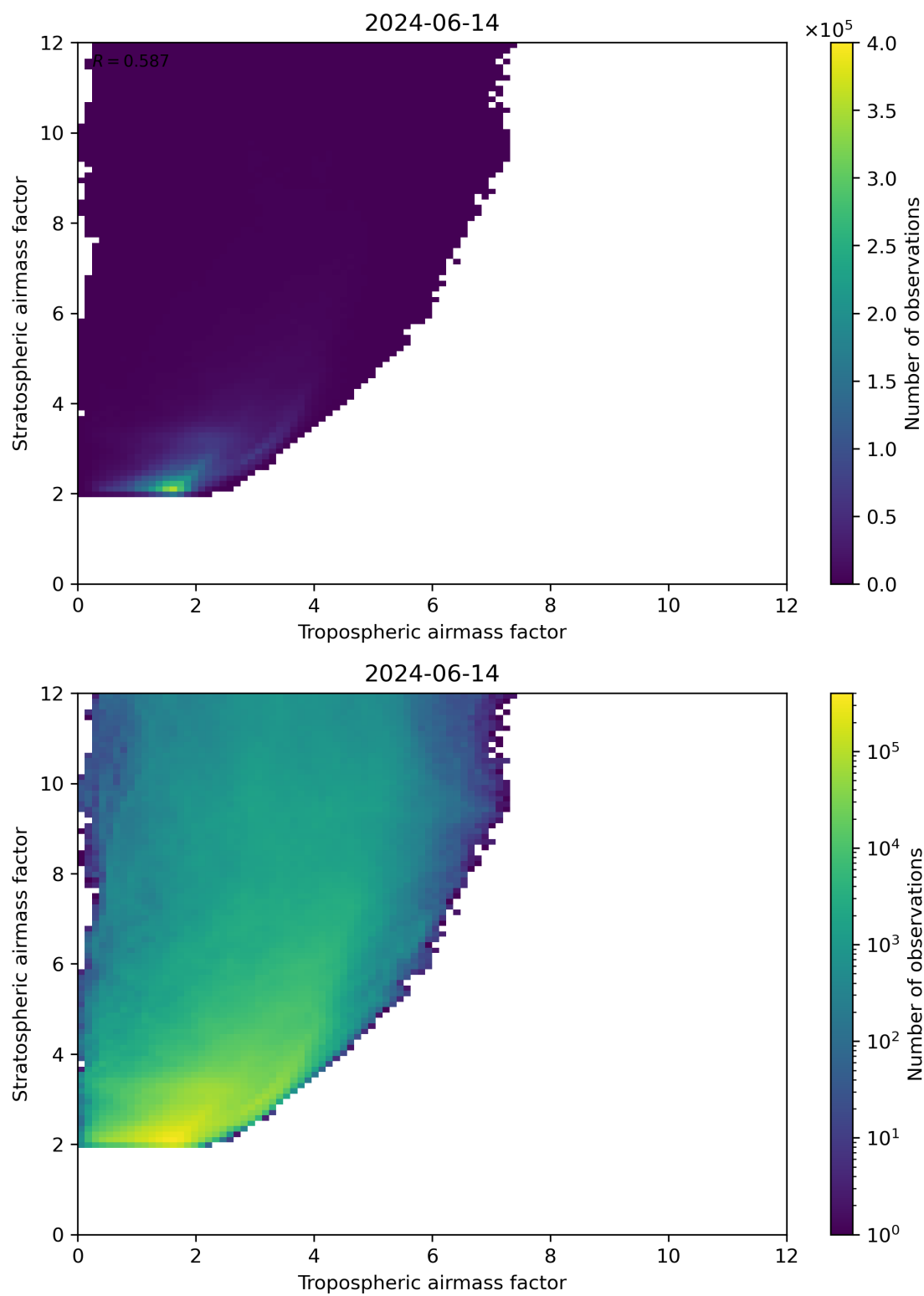
Figure 71: Scatter density plot of “Tropospheric airmass factor” against “Stratospheric airmass factor” for 2024-06-13 to 2024-06-15.
