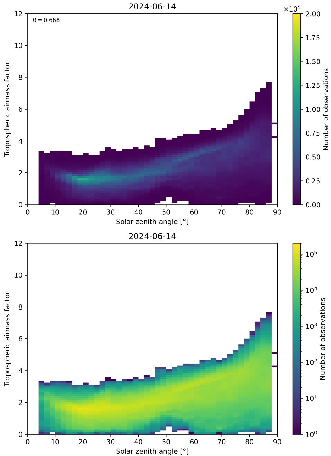
Figure 147: Scatter density plot of “Solar zenith angle” against “Tropospheric airmass factor” for 2024-06-13 to 2024-06-15.
