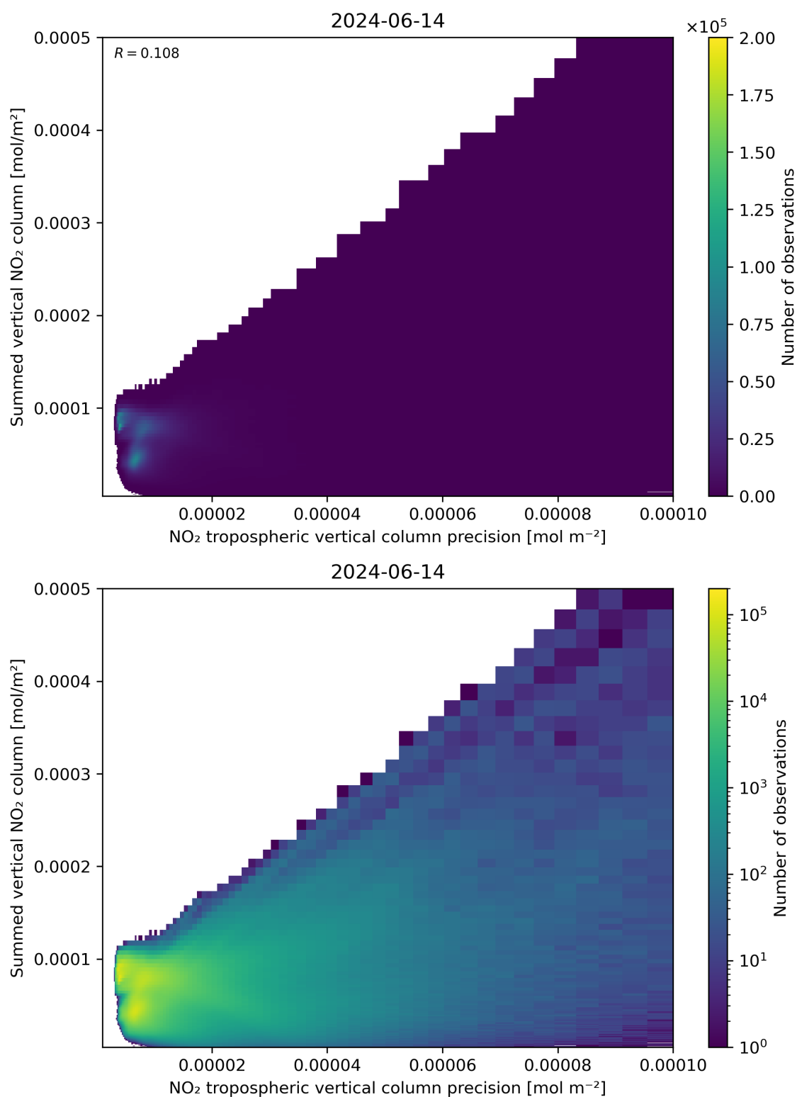
Figure 136: Scatter density plot of “NO 2 tropospheric vertical column precision” against “Summed vertical NO 2 column” for 2024-06-13 to 2024-06-15.
