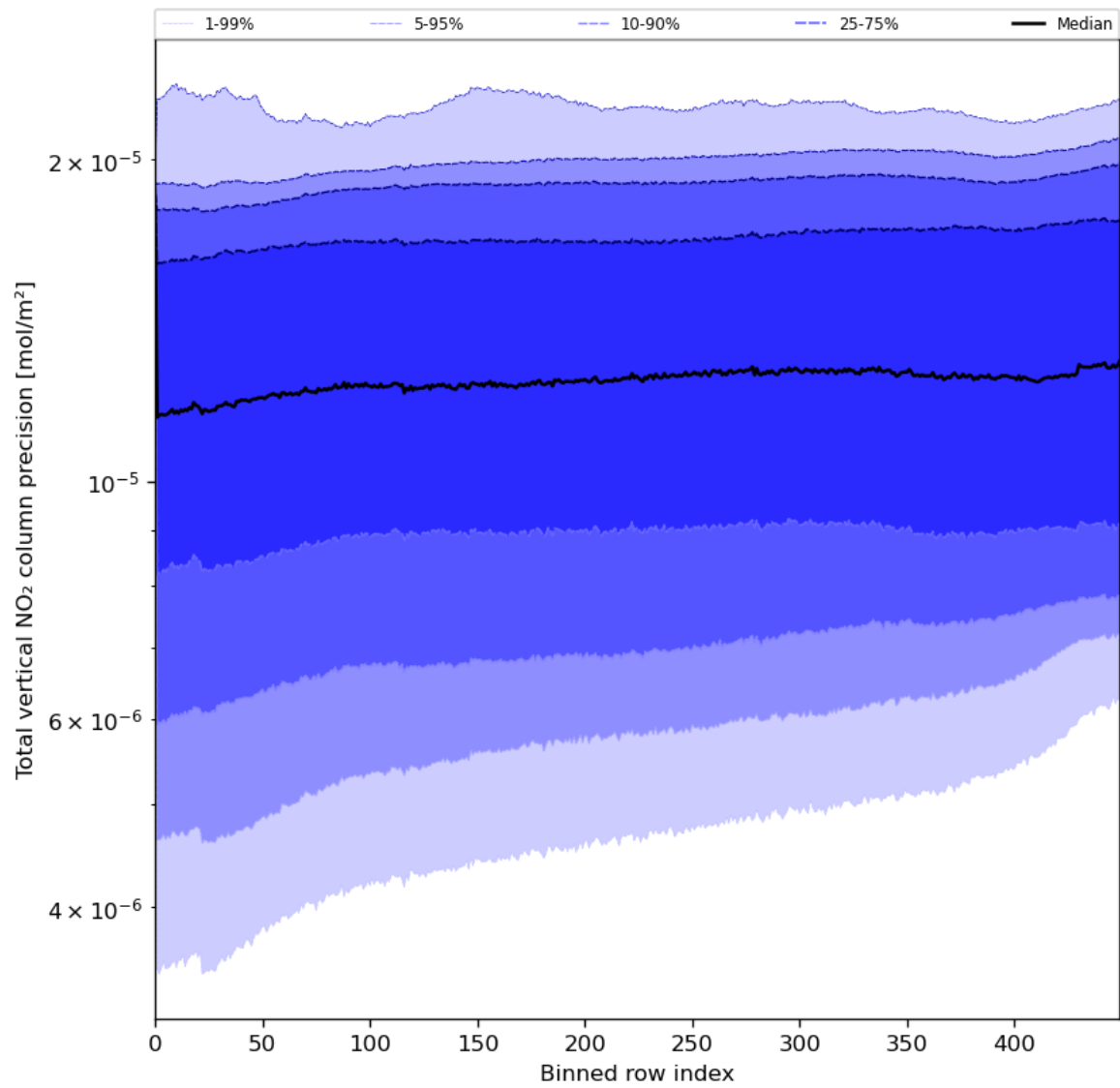
Figure 56: Along track statistics of “Total vertical NO 2 column precision” for 2024-06-13 to 2024-06-15
