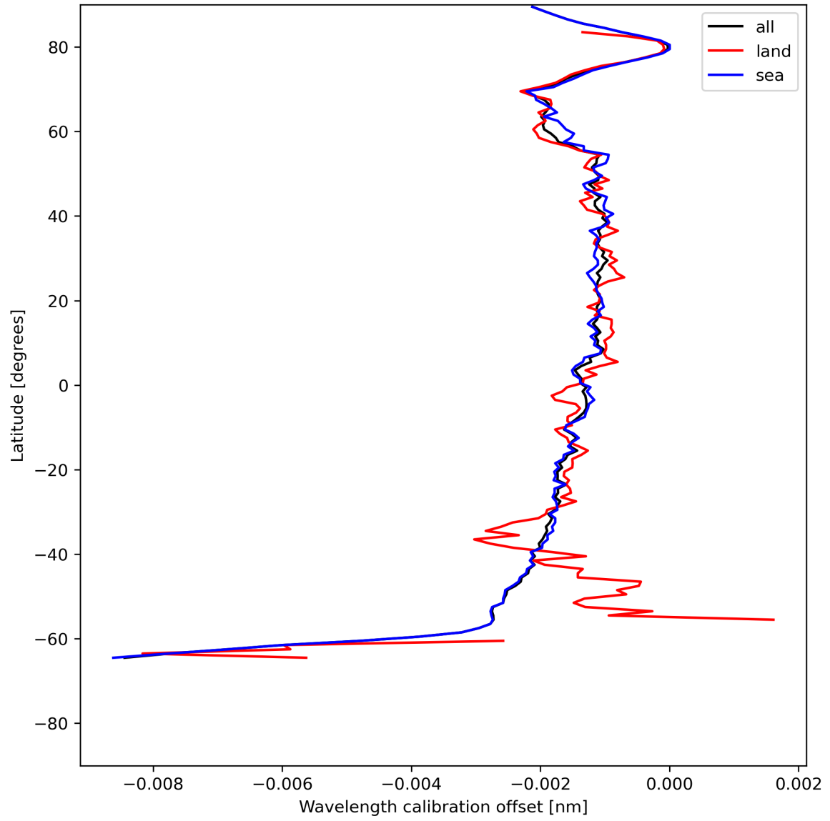
Figure 18: Zonal average of “Wavelength calibration offset” for 2024-06-13 to 2024-06-15.
