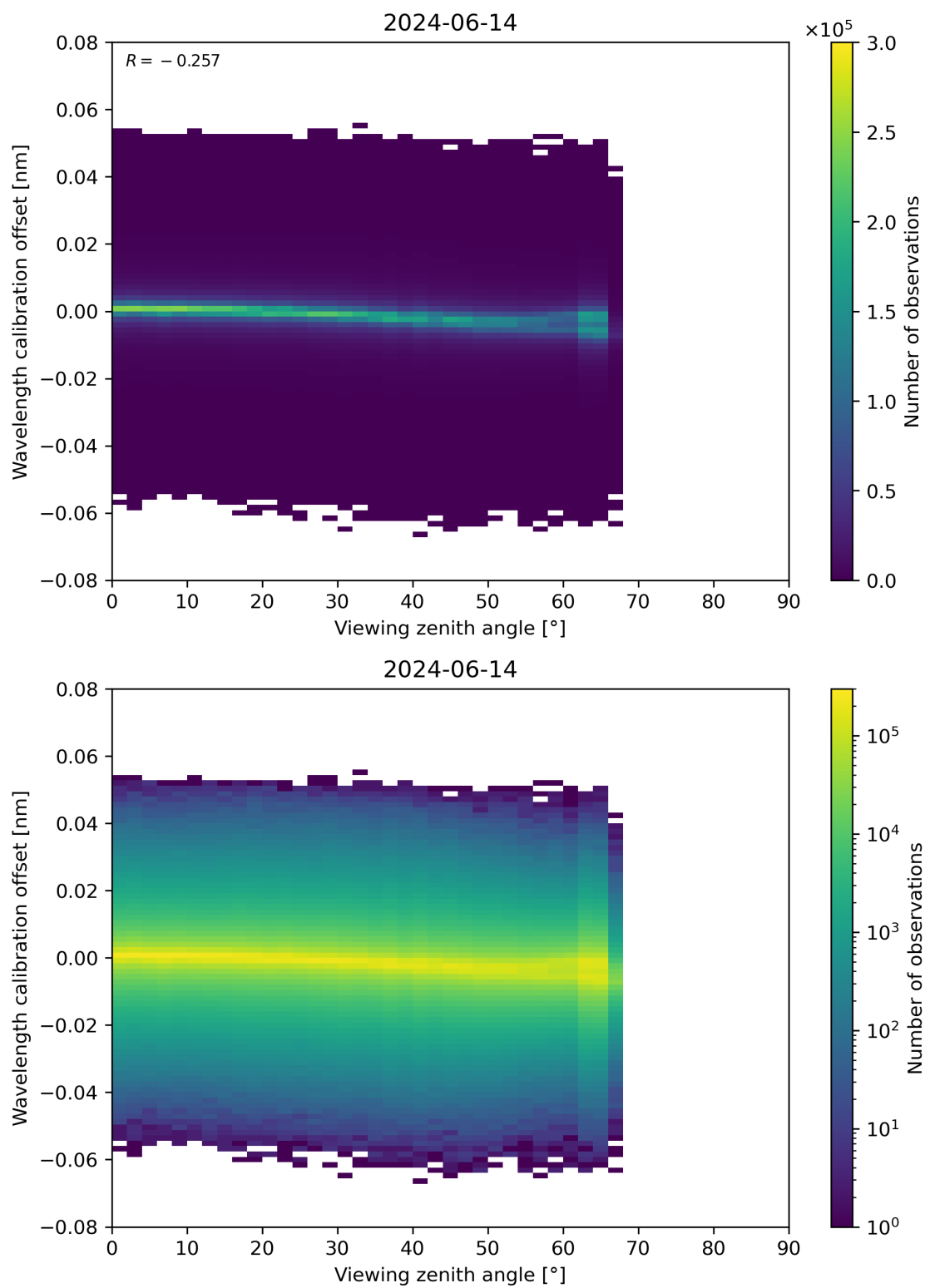
Figure 173: Scatter density plot of “Viewing zenith angle” against “Wavelength calibration offset” for 2024-06-13 to 2024-06-15.
