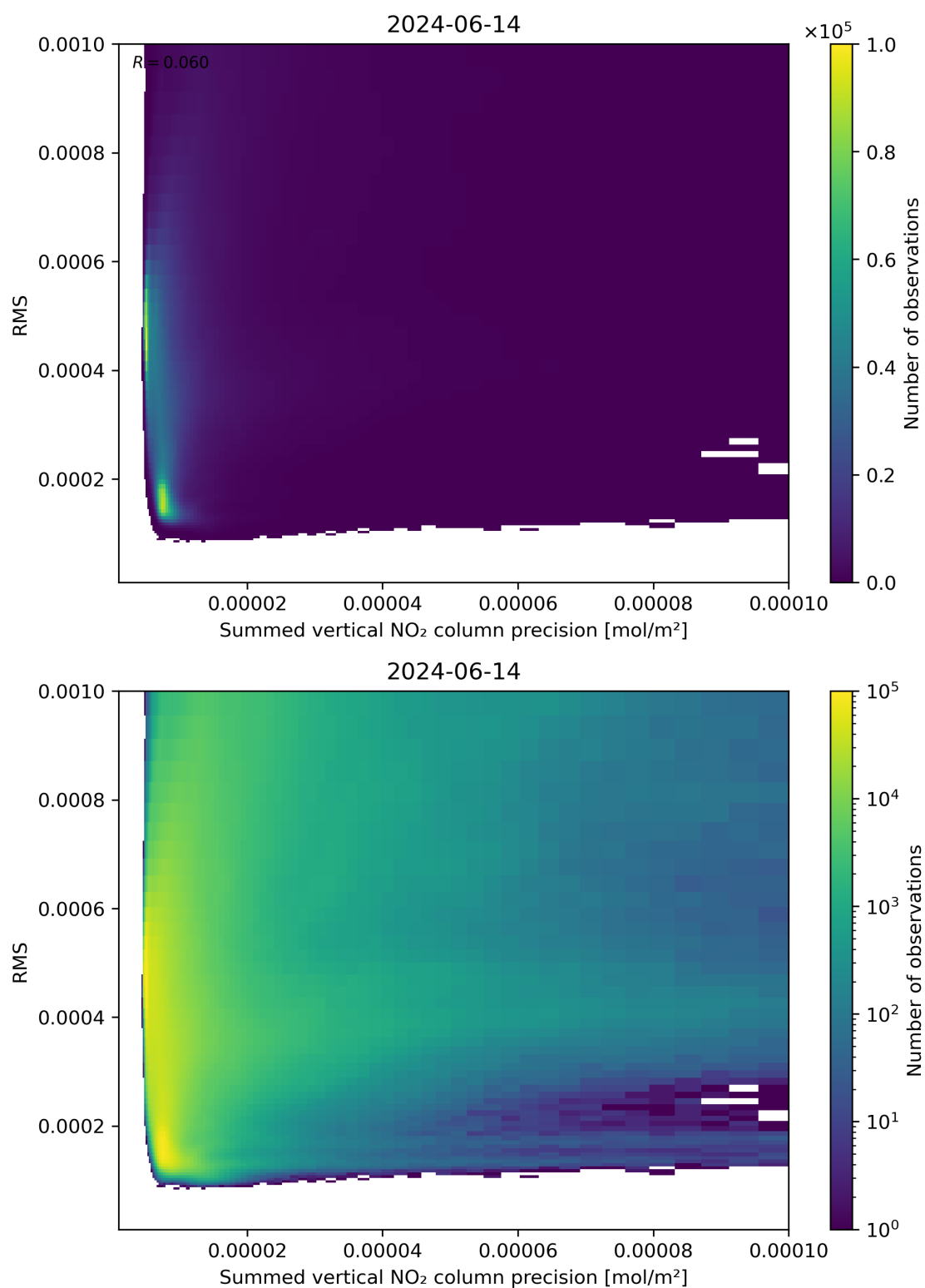
Figure 108: Scatter density plot of “Summed vertical NO 2 column precision” against “RMS” for 2024-06-13 to 2024-06-15.
