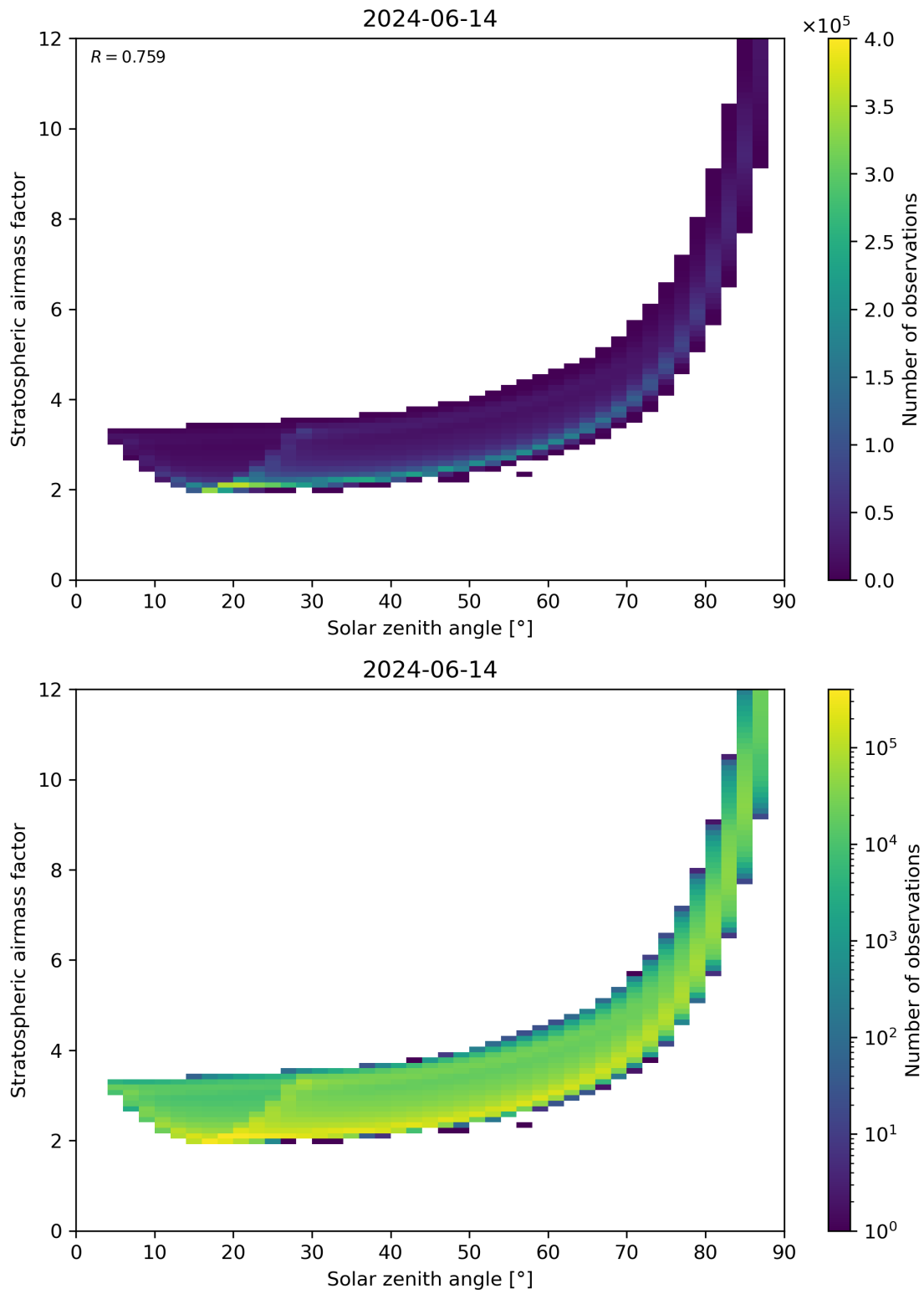
Figure 145: Scatter density plot of “Solar zenith angle” against “Stratospheric airmass factor” for 2024-06-13 to 2024-06-15.
