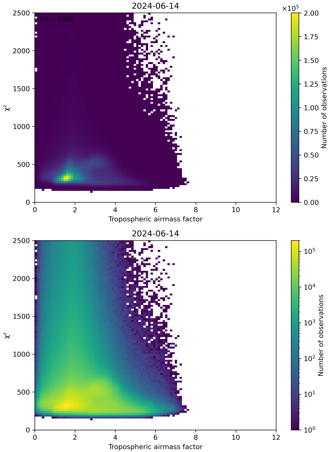
Figure 73: Scatter density plot of “Tropospheric airmass factor” against “ \chi^2 ” for 2024-06-13 to 2024-06-15.
