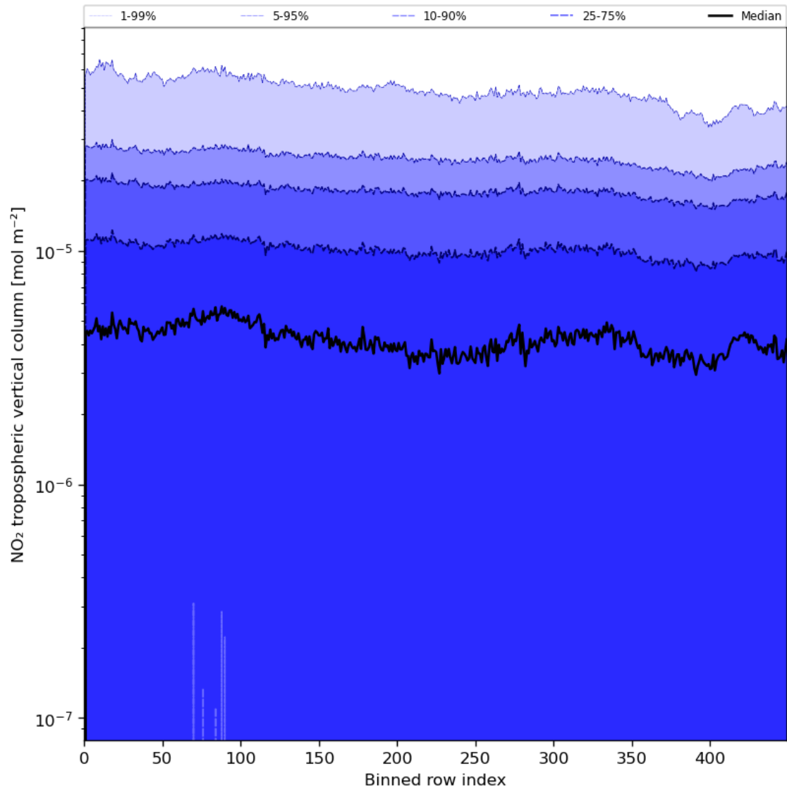
Figure 46: Along track statistics of “NO 2 tropospheric vertical column” for 2024-06-13 to 2024-06-15
