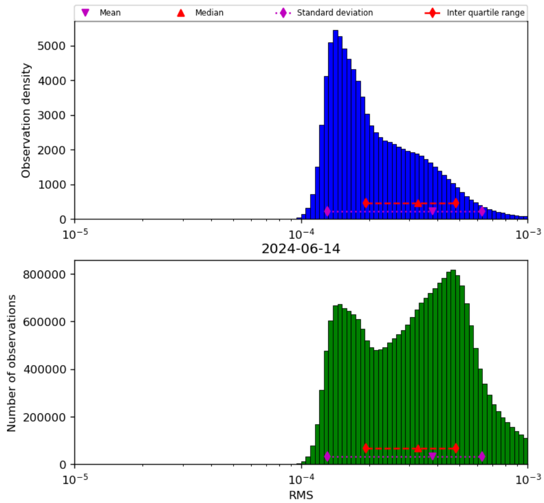
Figure 43: Histogram of “RMS” for 2024-06-13 to 2024-06-15
