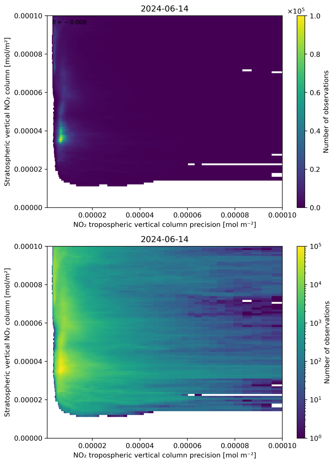
Figure 135: Scatter density plot of “NO 2 tropospheric vertical column precision” against “Stratospheric vertical NO 2 column” for 2024-06-13 to 2024-06-15.
