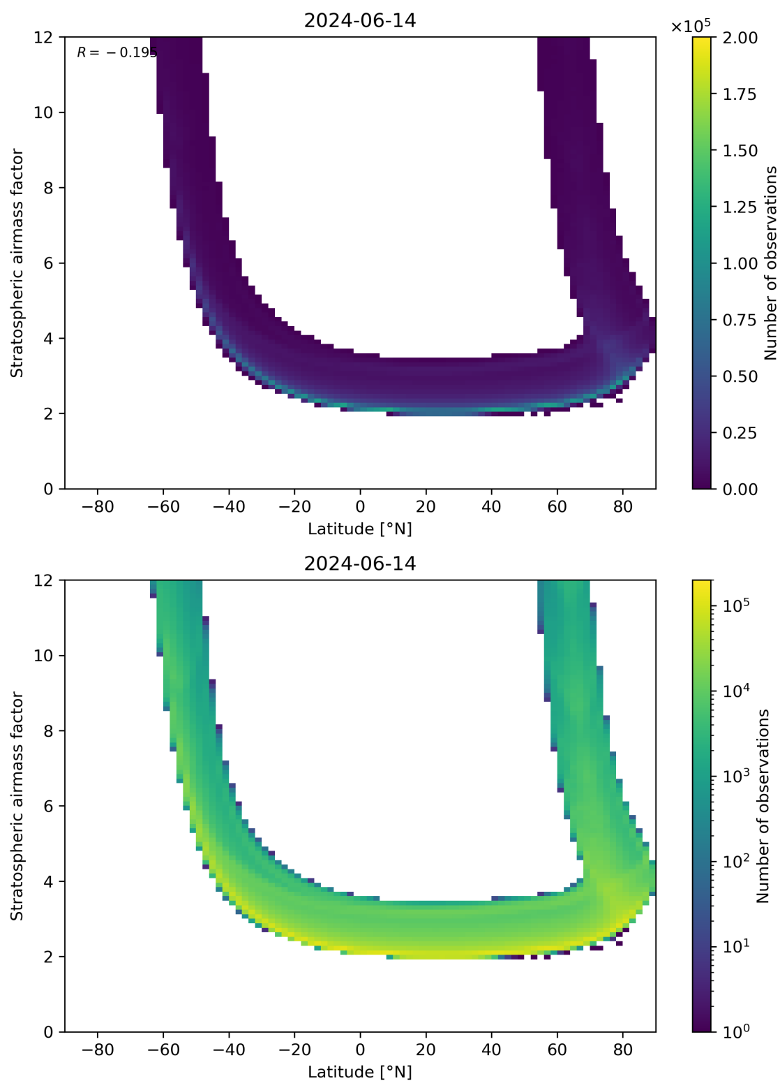
Figure 83: Scatter density plot of “Latitude” against “Stratospheric air mass factor” for 2024-06-13 to 2024-06-15.
