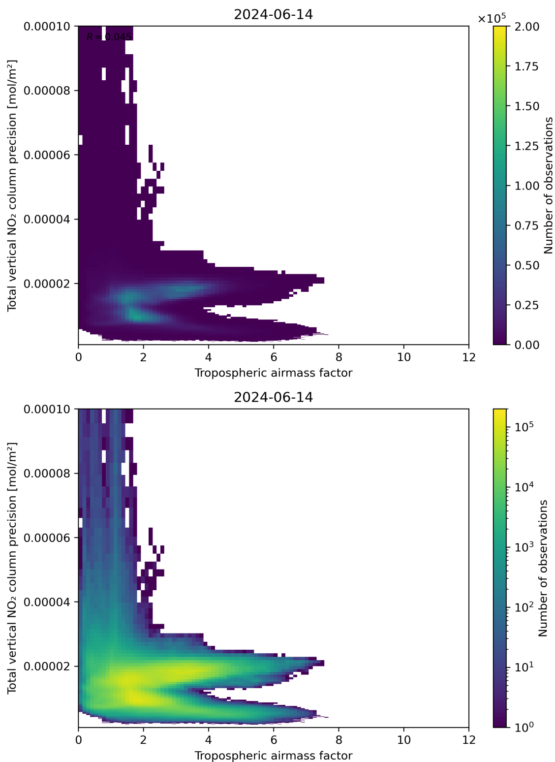
Figure 78: Scatter density plot of “Tropospheric air mass factor” against “Total vertical NO 2 column precision” for 2024-06-13 to 2024-06-15.
