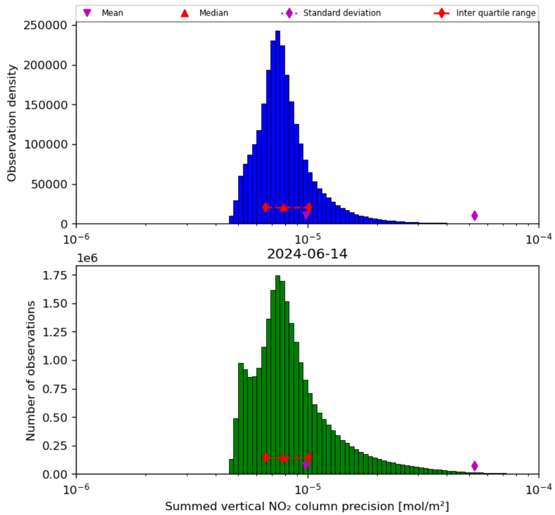
Figure 41: Histogram of "Summed vertical NO 2 column precision" for 2024-06-13 to 2024-06-15
