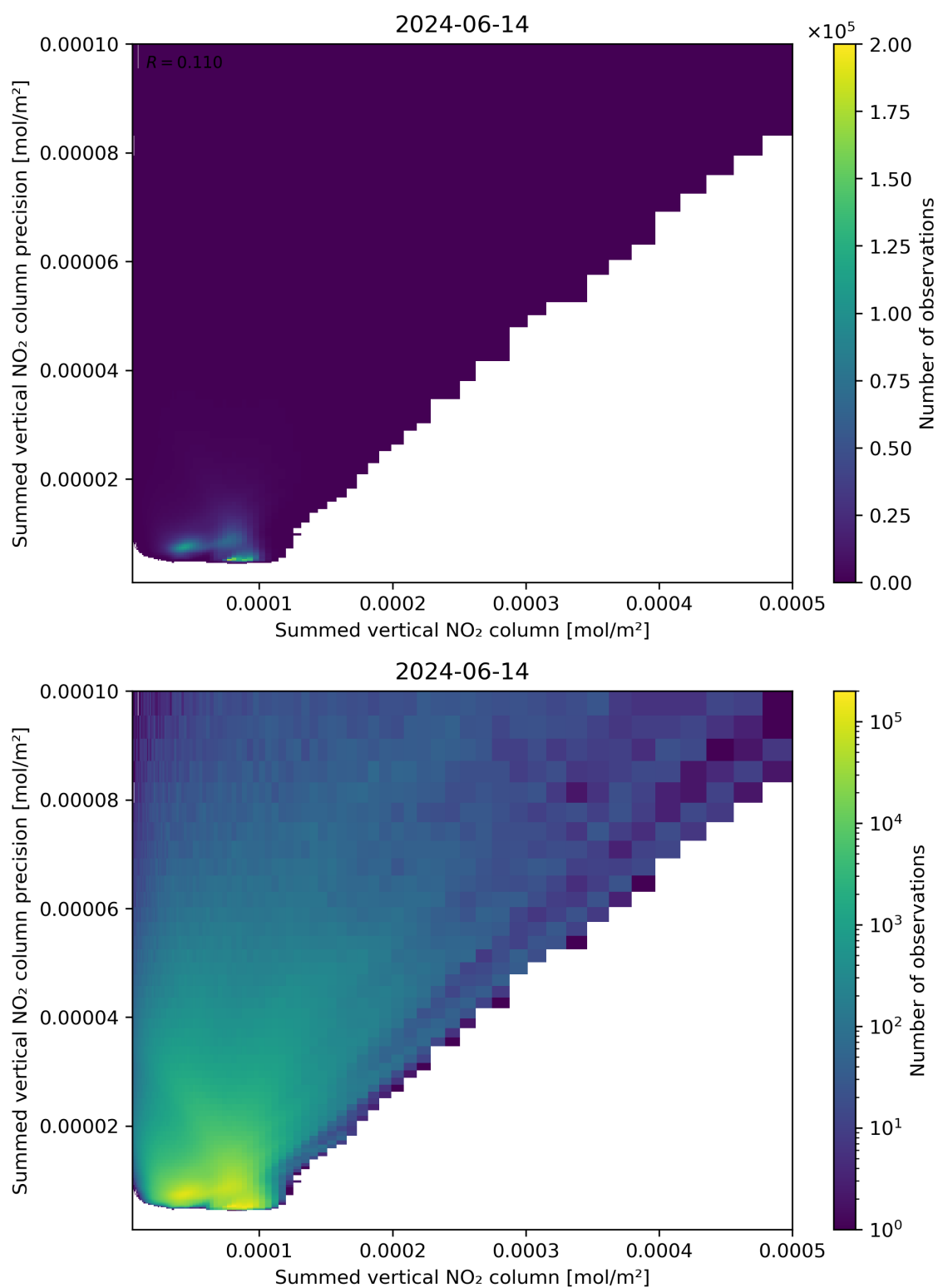
Figure 105: Scatter density plot of “Summed vertical NO 2 column” against “Summed vertical NO 2 column precision” for 2024-06-13 to 2024-06-15.
