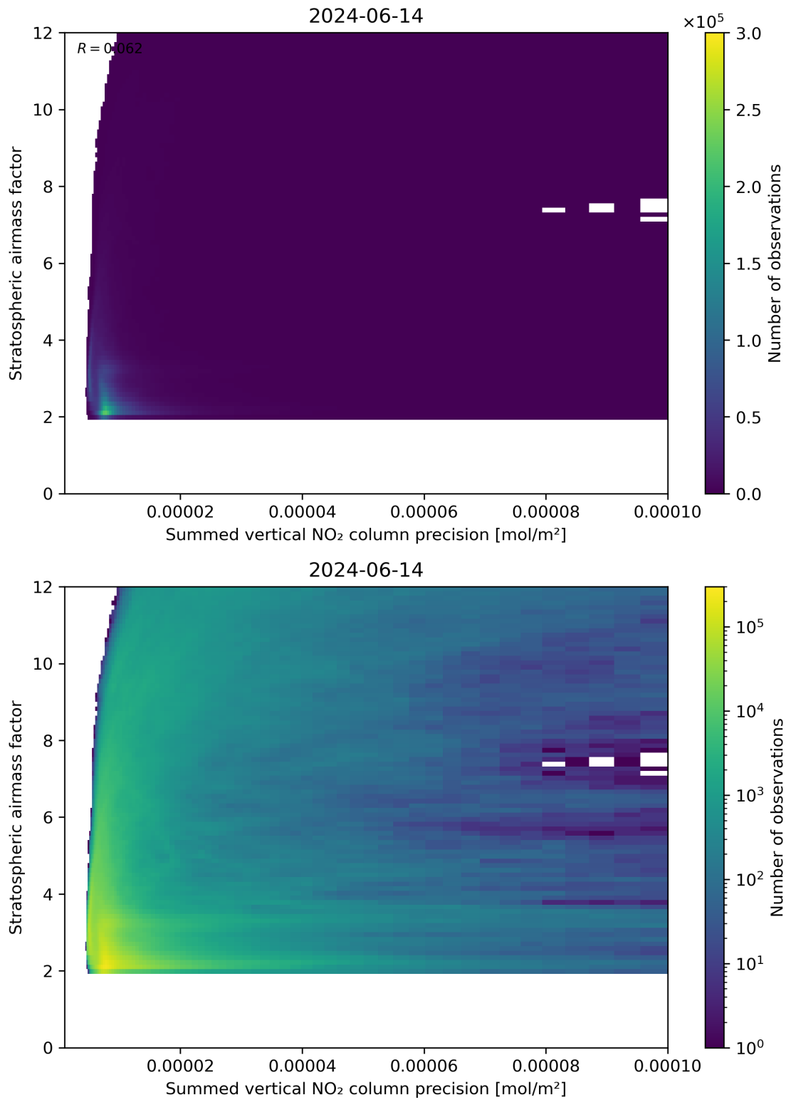
Figure 106: Scatter density plot of “Summed vertical NO 2 column precision” against “Stratospheric air mass factor” for 2024-06-13 to 2024-06-15.
