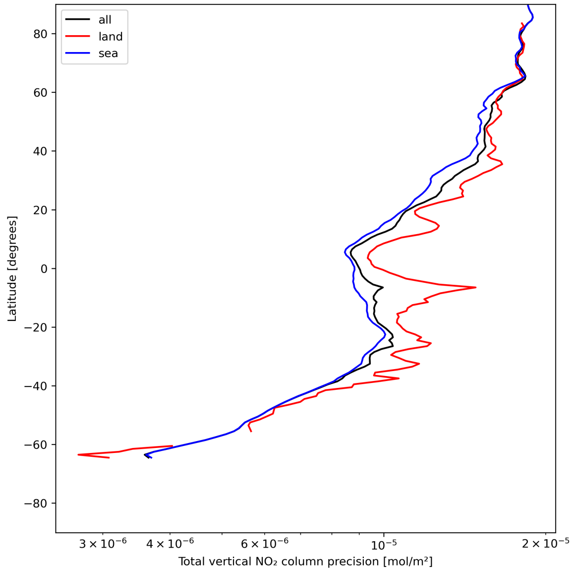
Figure 22: Zonal average of “Total vertical NO 2 column precision” for 2024-06-13 to 2024-06-15.
