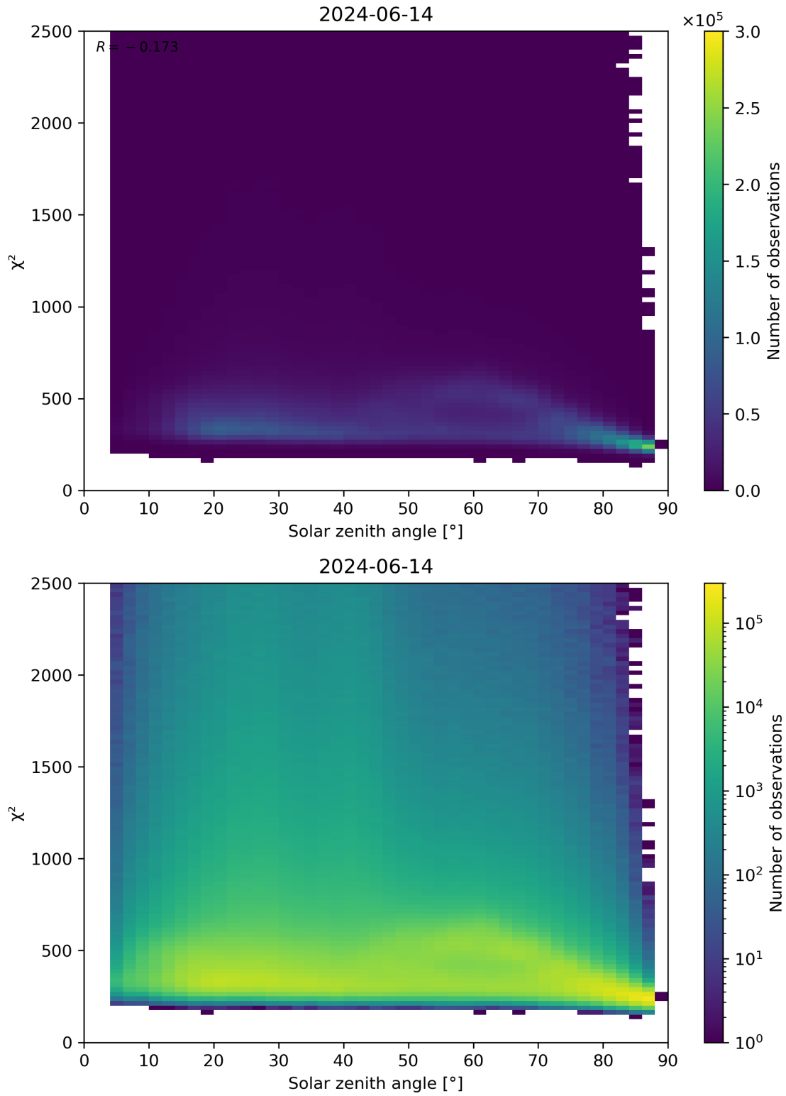
Figure 148: Scatter density plot of “Solar zenith angle” against “ \chi^2 ” for 2024-06-13 to 2024-06-15.
