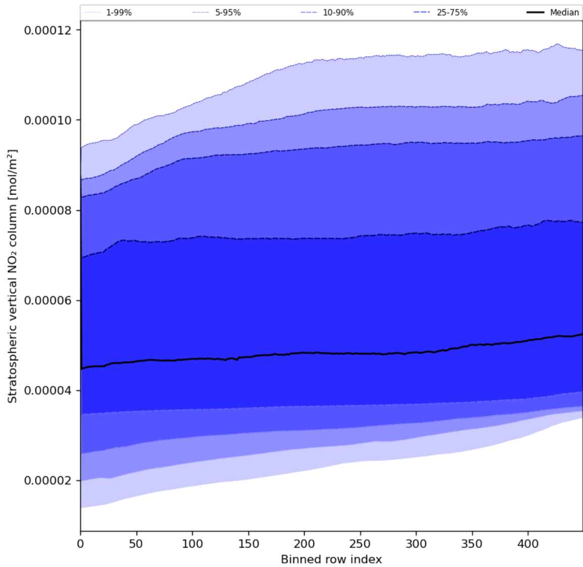
Figure 53: Along track statistics of “Stratospheric vertical NO 2 column” for 2024-06-13 to 2024-06-15
