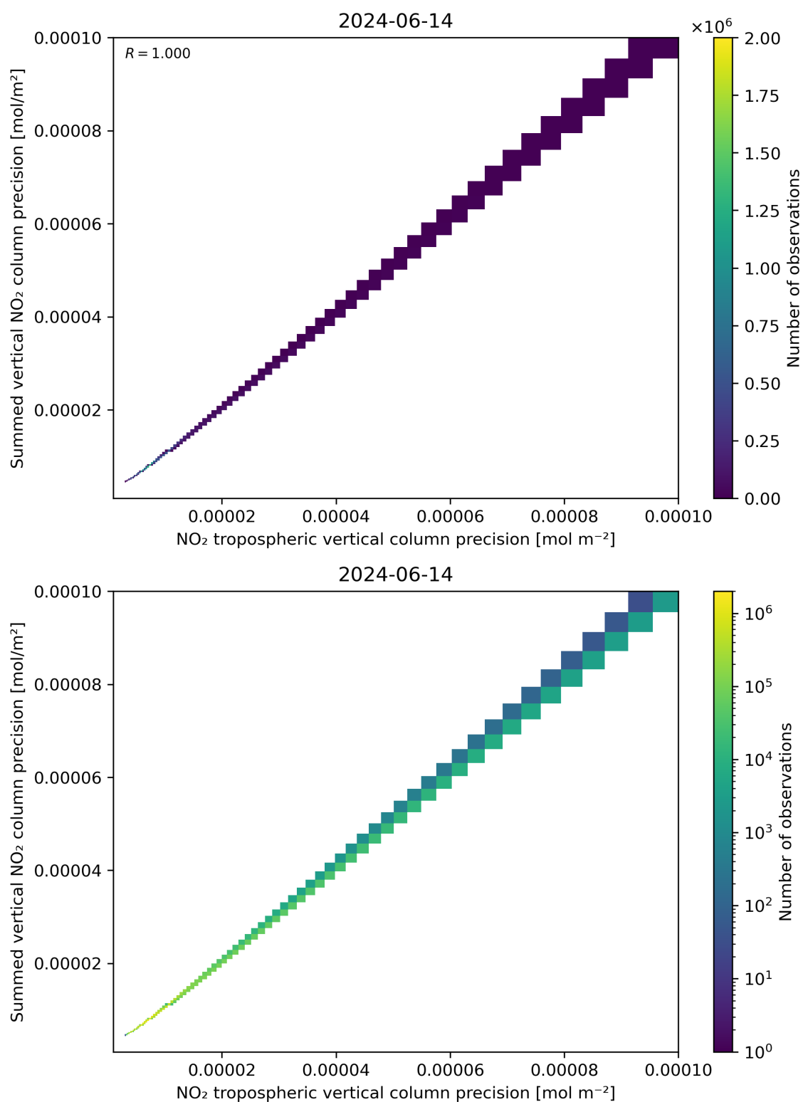
Figure 137: Scatter density plot of “NO 2 tropospheric vertical column precision” against “Summed vertical NO 2 column precision” for 2024-06-13 to 2024-06-15.
