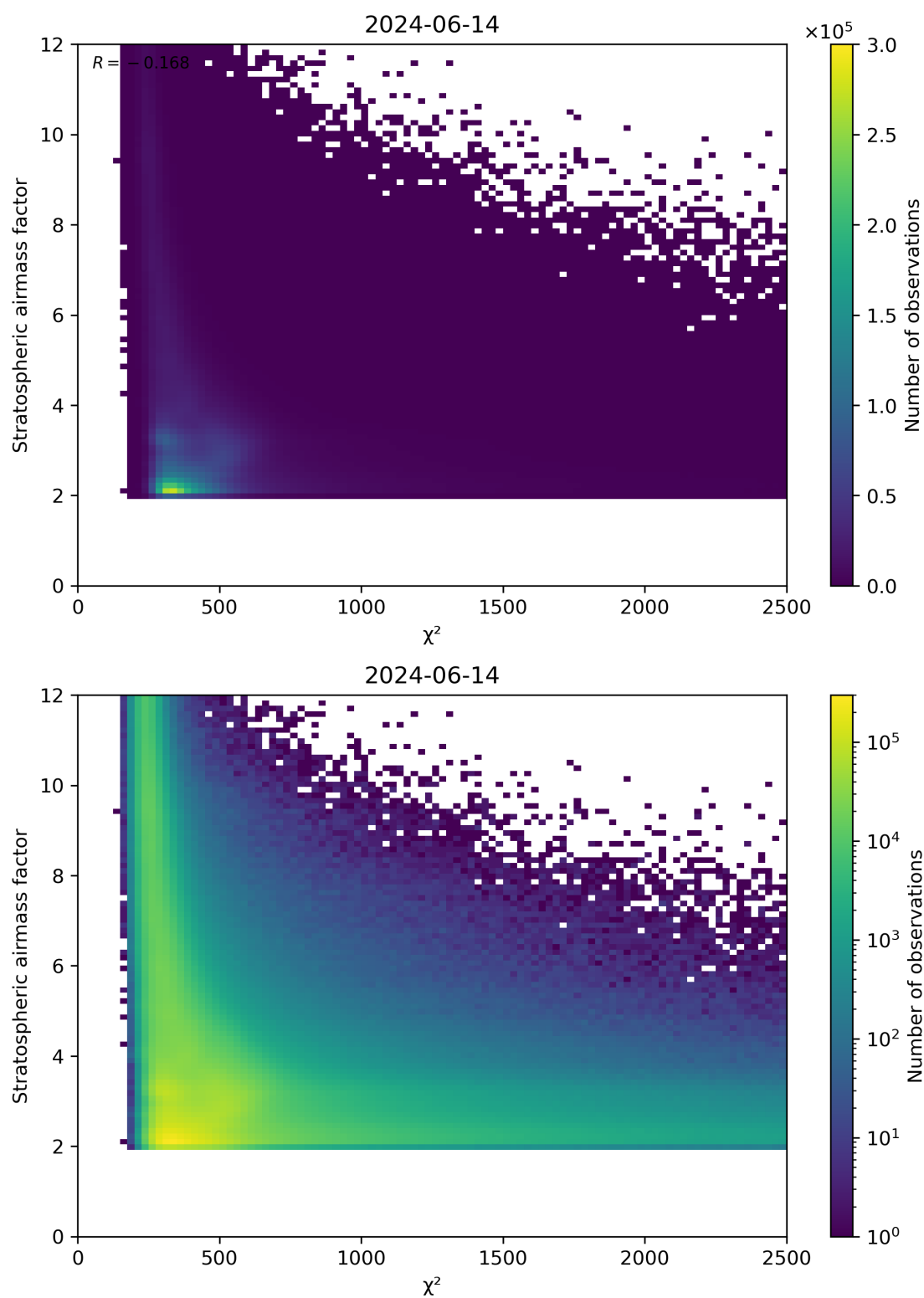
Figure 81: Scatter density plot of “ \chi^2 ” against “Stratospheric airmass factor” for 2024-06-13 to 2024-06-15.
