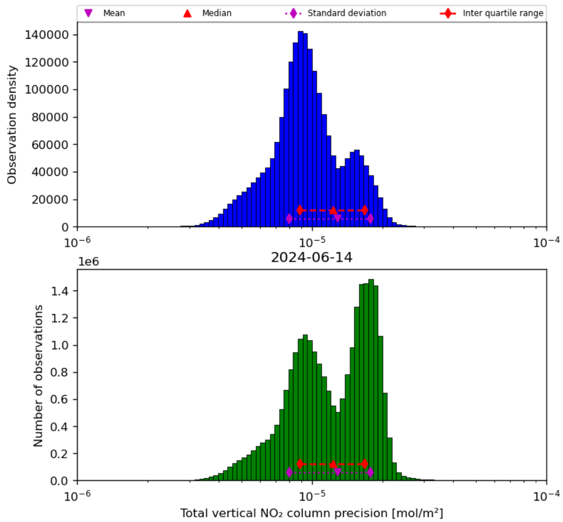
Figure 39: Histogram of “Total vertical NO 2 column precision” for 2024-06-13 to 2024-06-15
