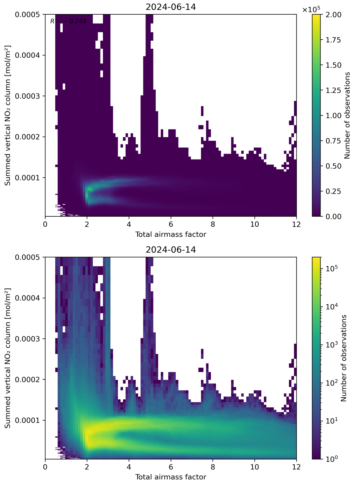
Figure 65: Scatter density plot of “Total airmass factor” against “Summed vertical NO 2 column” for 2024-06-13 to 2024-06-15.
