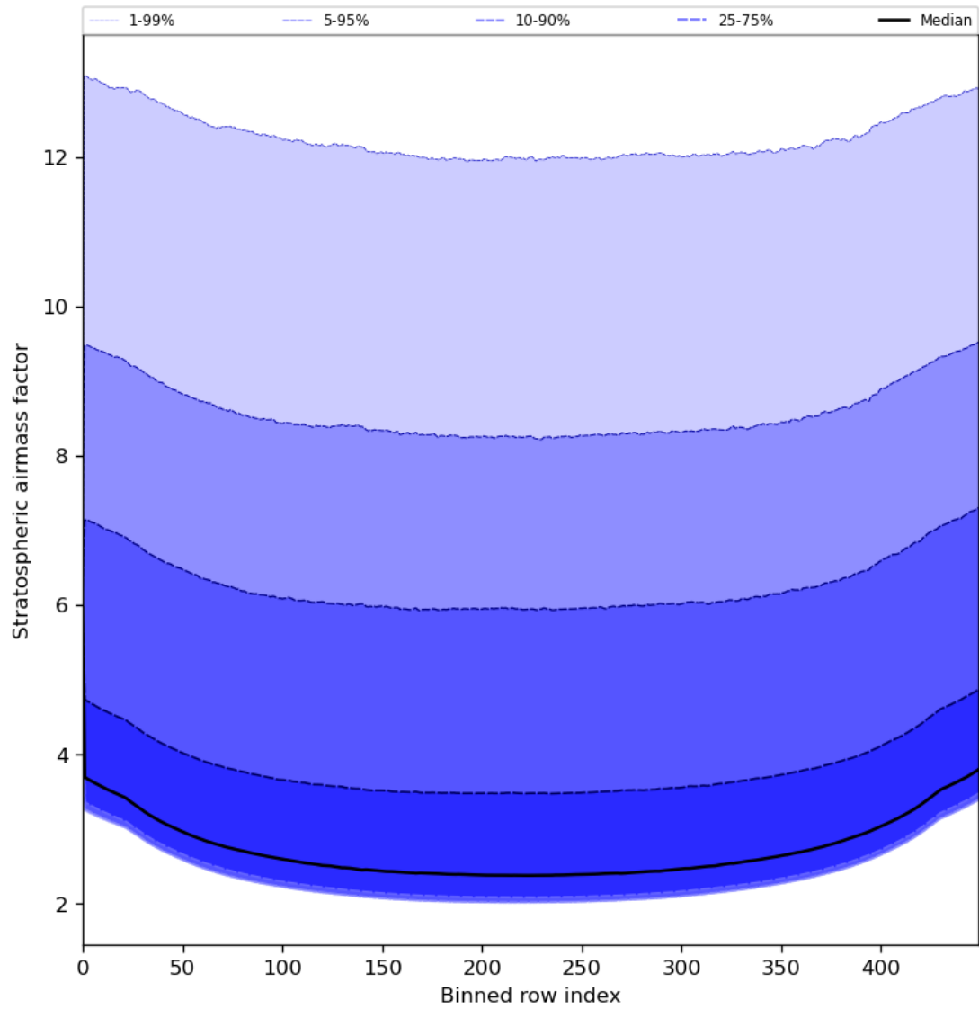
Figure 61: Along track statistics of “Stratospheric airmass factor” for 2024-06-13 to 2024-06-15
