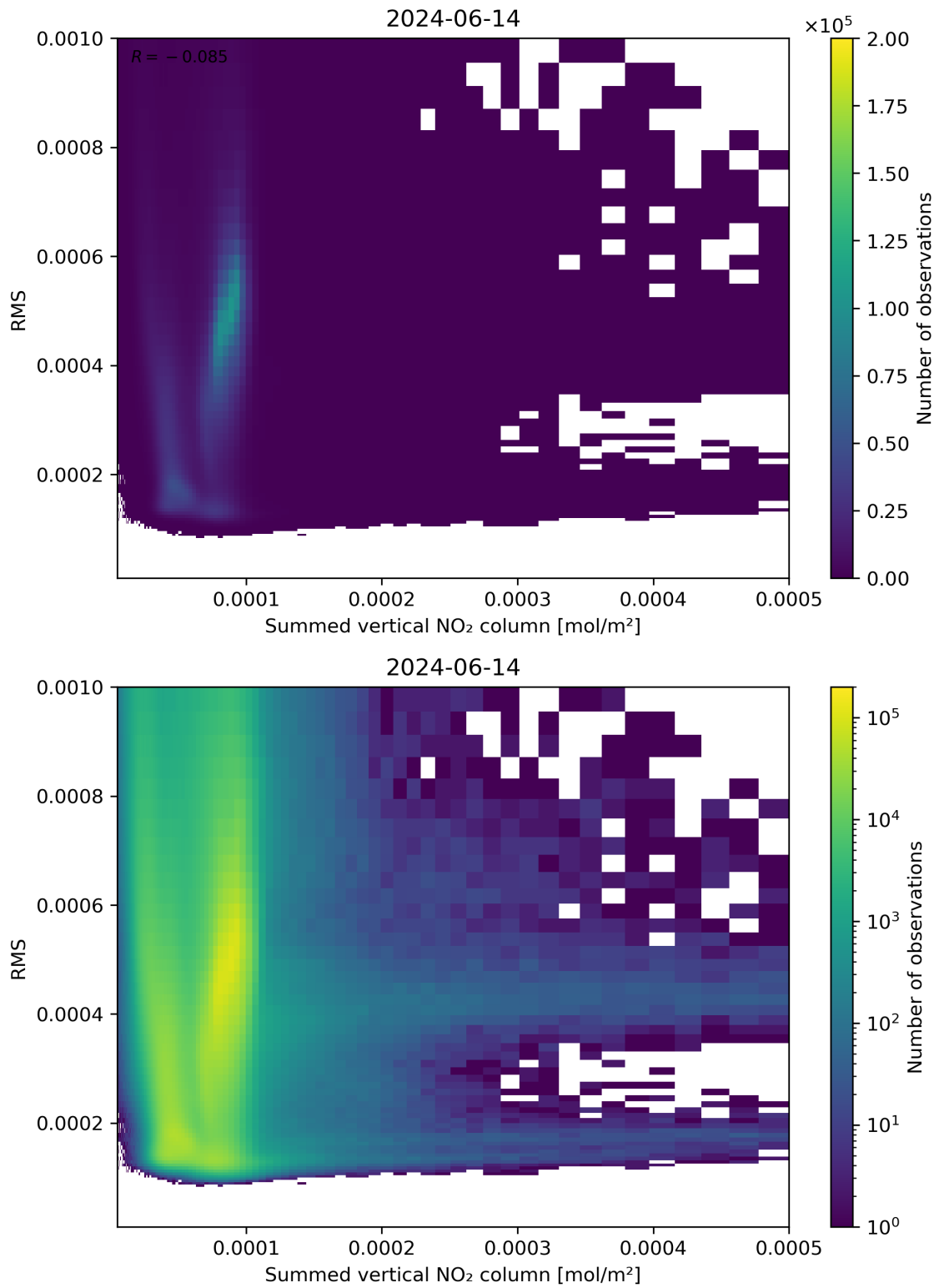
Figure 109: Scatter density plot of “Summed vertical NO 2 column” against “RMS” for 2024-06-13 to 2024-06-15.
