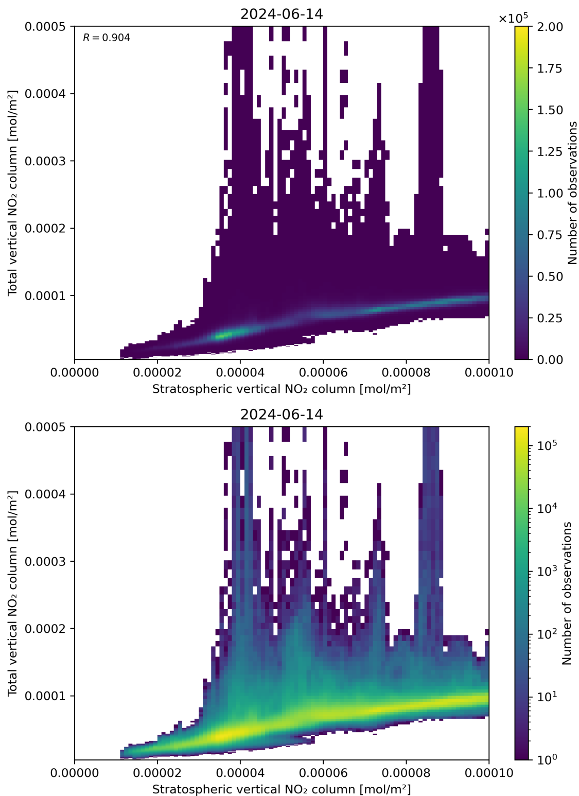
Figure 100: Scatter density plot of “Stratospheric vertical NO 2 column” against “Total vertical NO 2 column” for 2024-06-13 to 2024-06-15.
