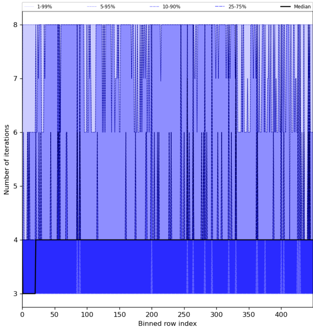
Figure 51: Along track statistics of “Number of iterations” for 2024-06-13 to 2024-06-15
