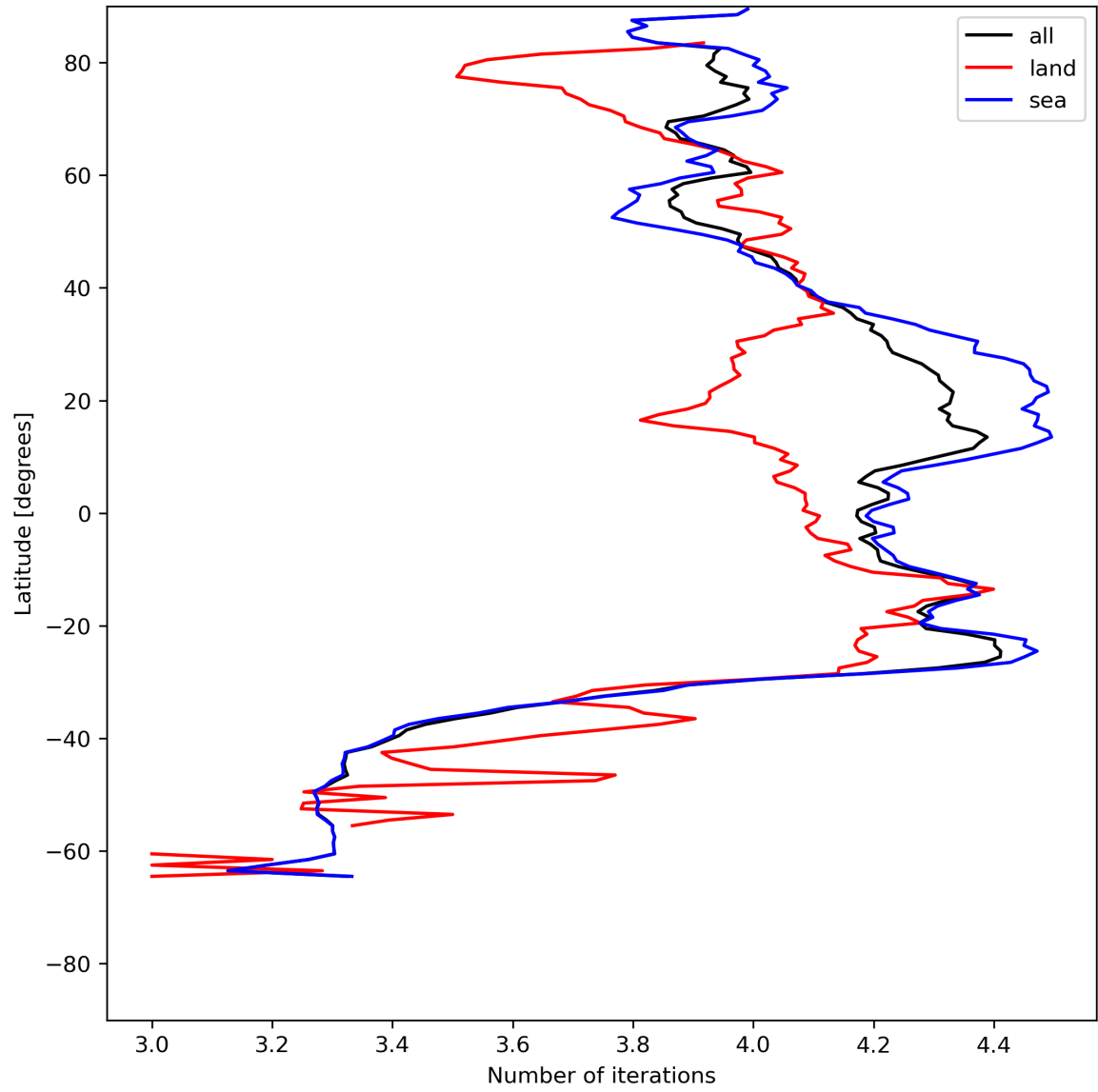
Figure 17: Zonal average of “Number of iterations” for 2024-06-13 to 2024-06-15.
