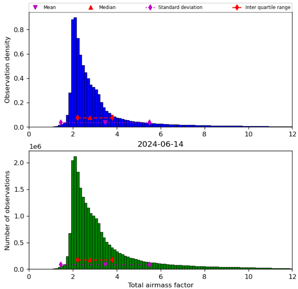
Figure 32: Histogram of “Total airmass factor” for 2024-06-13 to 2024-06-15
