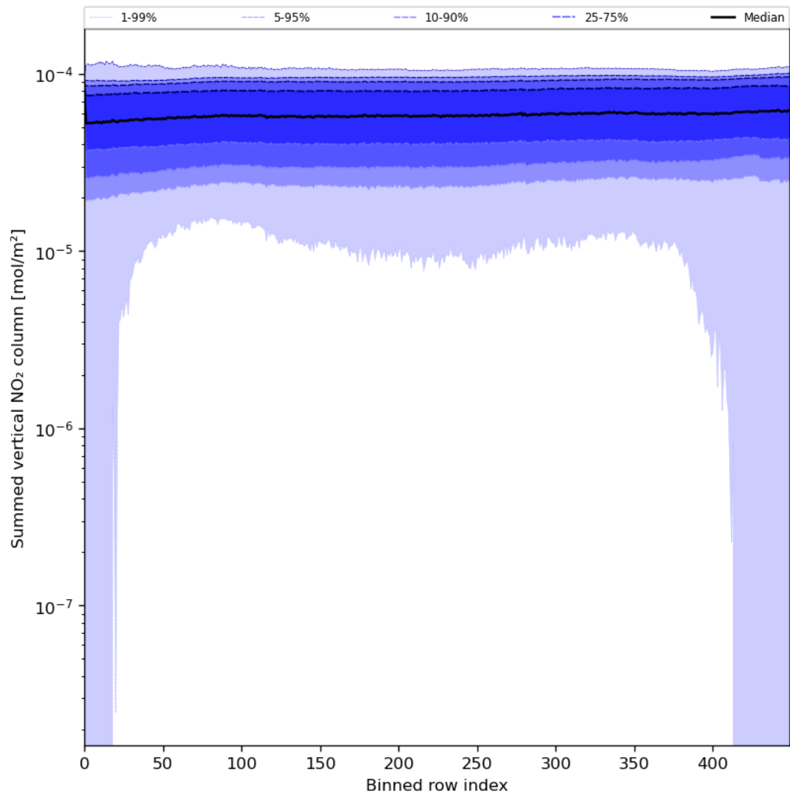
Figure 57: Along track statistics of “Summed vertical NO 2 column” for 2024-06-13 to 2024-06-15
