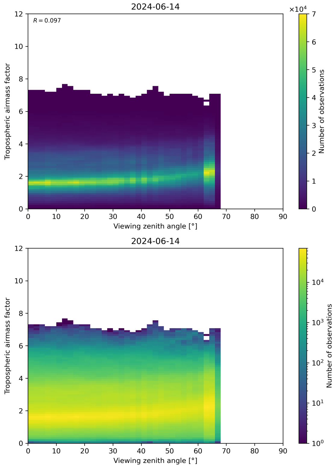
Figure 161: Scatter density plot of “Viewing zenith angle” against “Tropospheric airmass factor” for 2024-06-13 to 2024-06-15.
