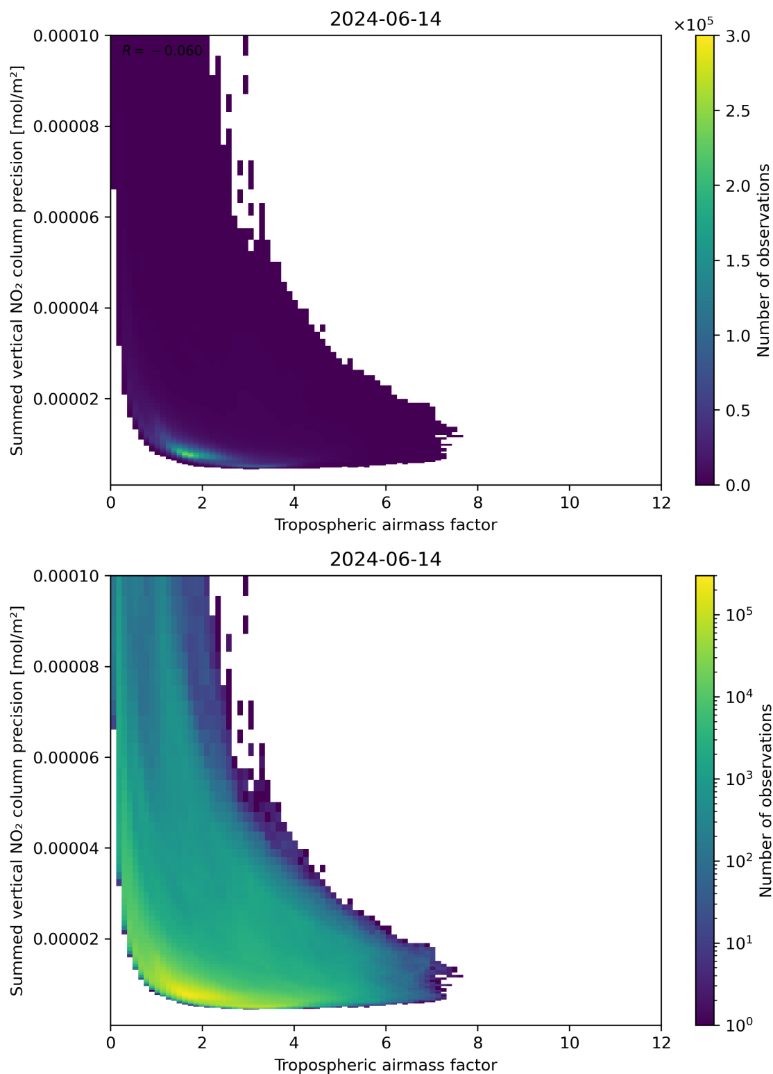
Figure 76: Scatter density plot of “Tropospheric air mass factor” against “Summed vertical NO 2 column precision” for 2024-06-13 to 2024-06-15.
