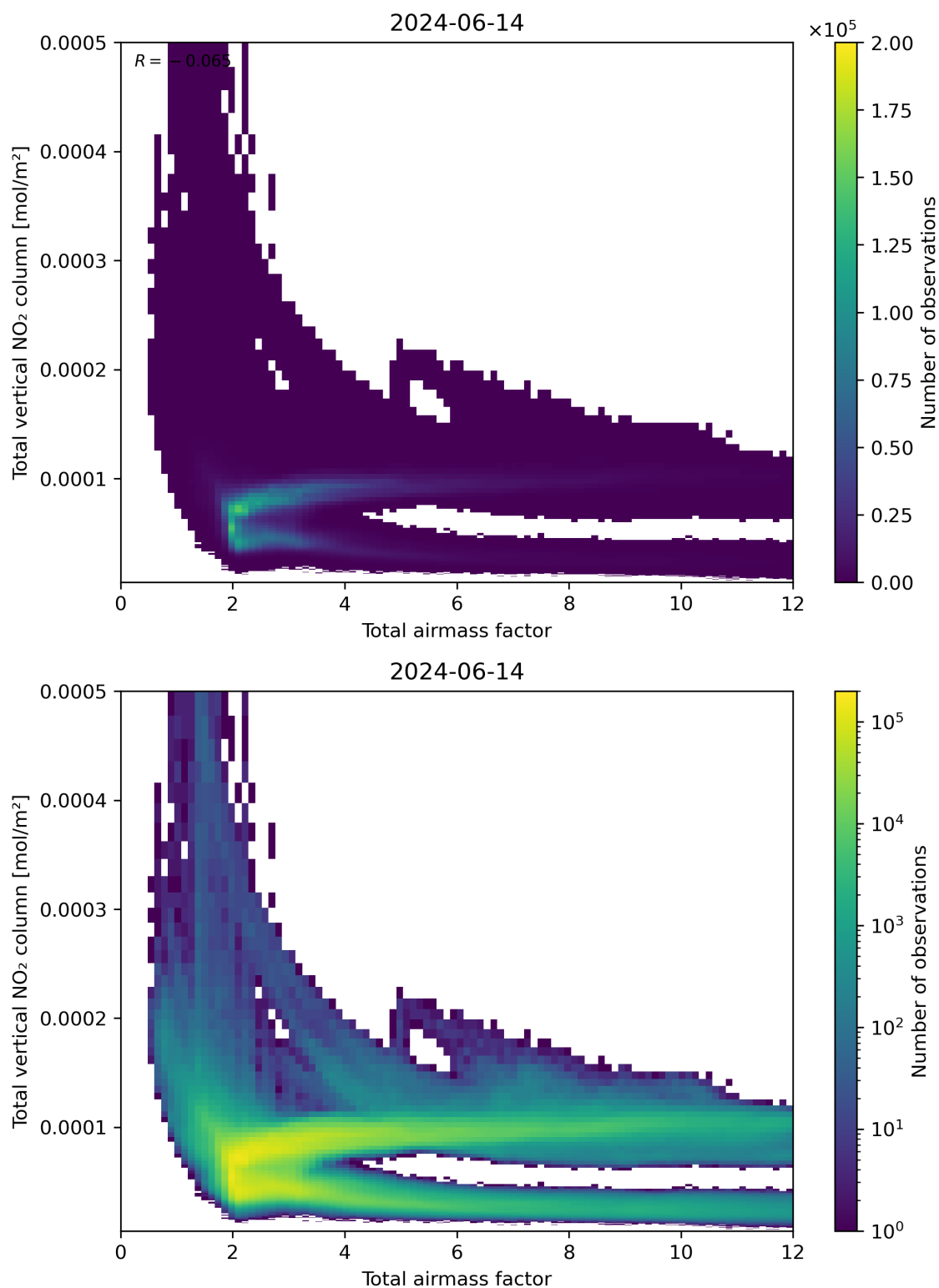
Figure 67: Scatter density plot of “Total airmass factor” against “Total vertical NO 2 column” for 2024-06-13 to 2024-06-15.
