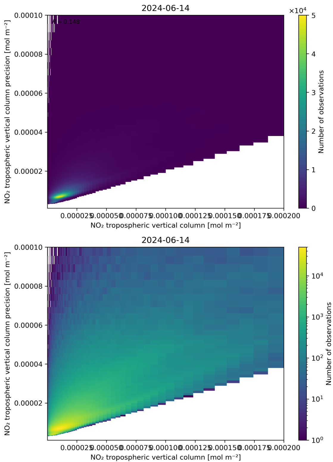
Figure 130: Scatter density plot of “NO 2 tropospheric vertical column” against “NO 2 tropospheric vertical column precision” for 2024-06-13 to 2024-06-15.
