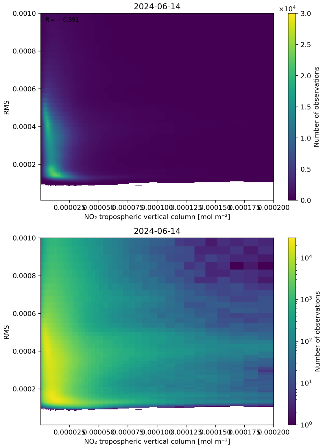
Figure 142: Scatter density plot of “NO 2 tropospheric vertical column” against “RMS” for 2024-06-13 to 2024-06-15.
