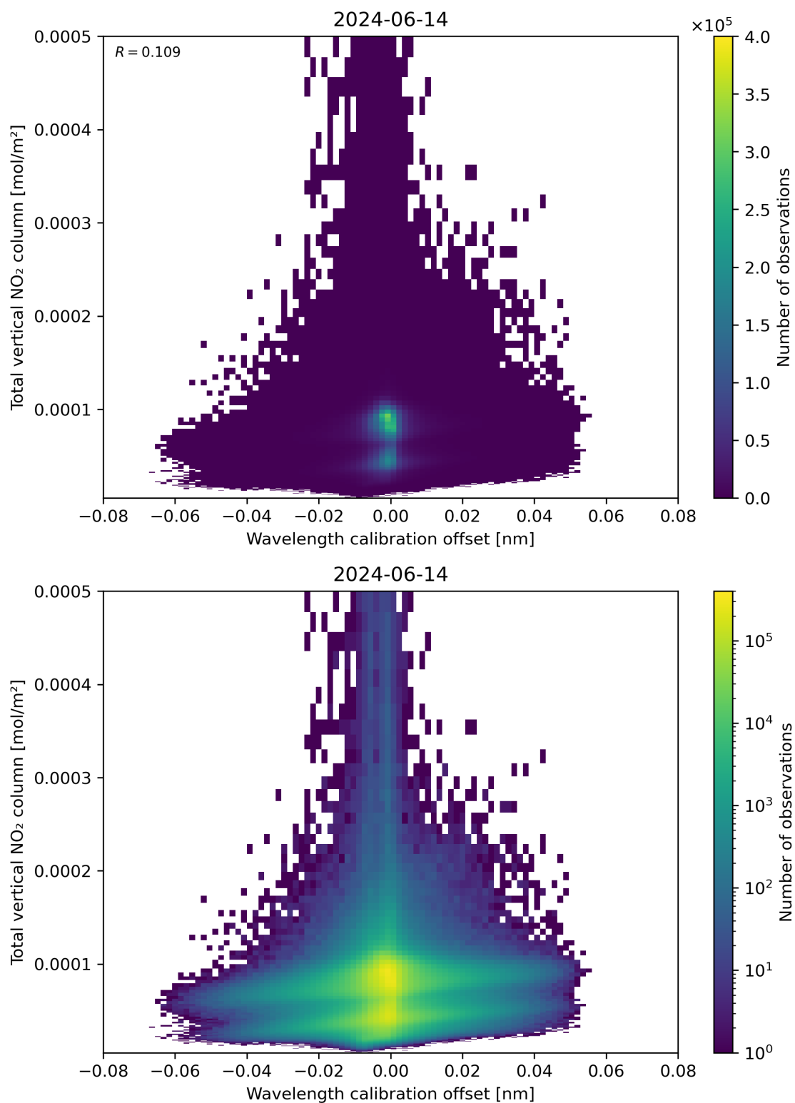
Figure 179: Scatter density plot of “Wavelength calibration offset” against “Total vertical NO 2 column” for 2024-06-13 to 2024-06-15.
