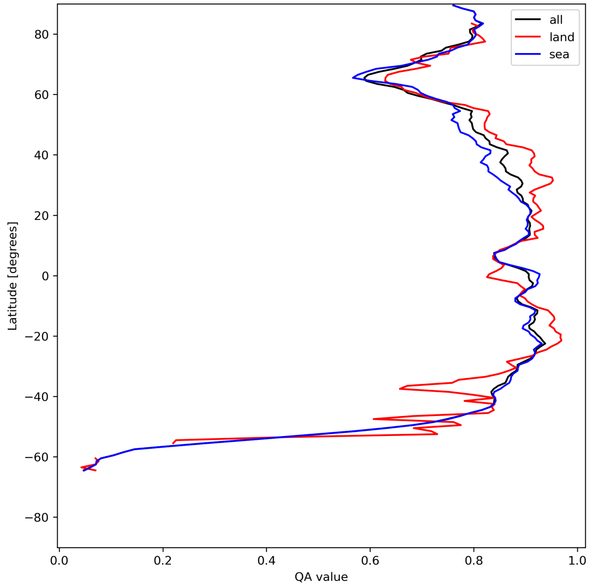
Figure 11: Zonal average of “QA value” for 2024-06-13 to 2024-06-15.
