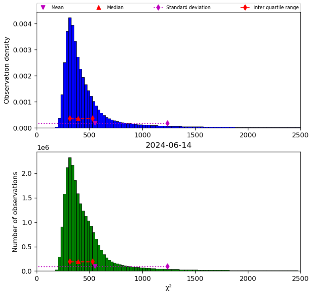
Figure 42: Histogram of “ \chi^2 ” for 2024-06-13 to 2024-06-15
