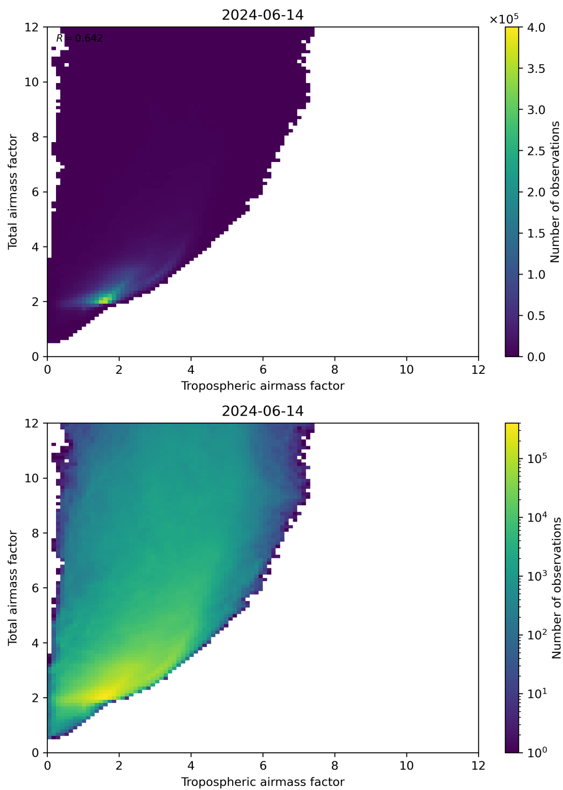
Figure 72: Scatter density plot of “Tropospheric airmass factor” against “Total airmass factor” for 2024-06-13 to 2024-06-15.
