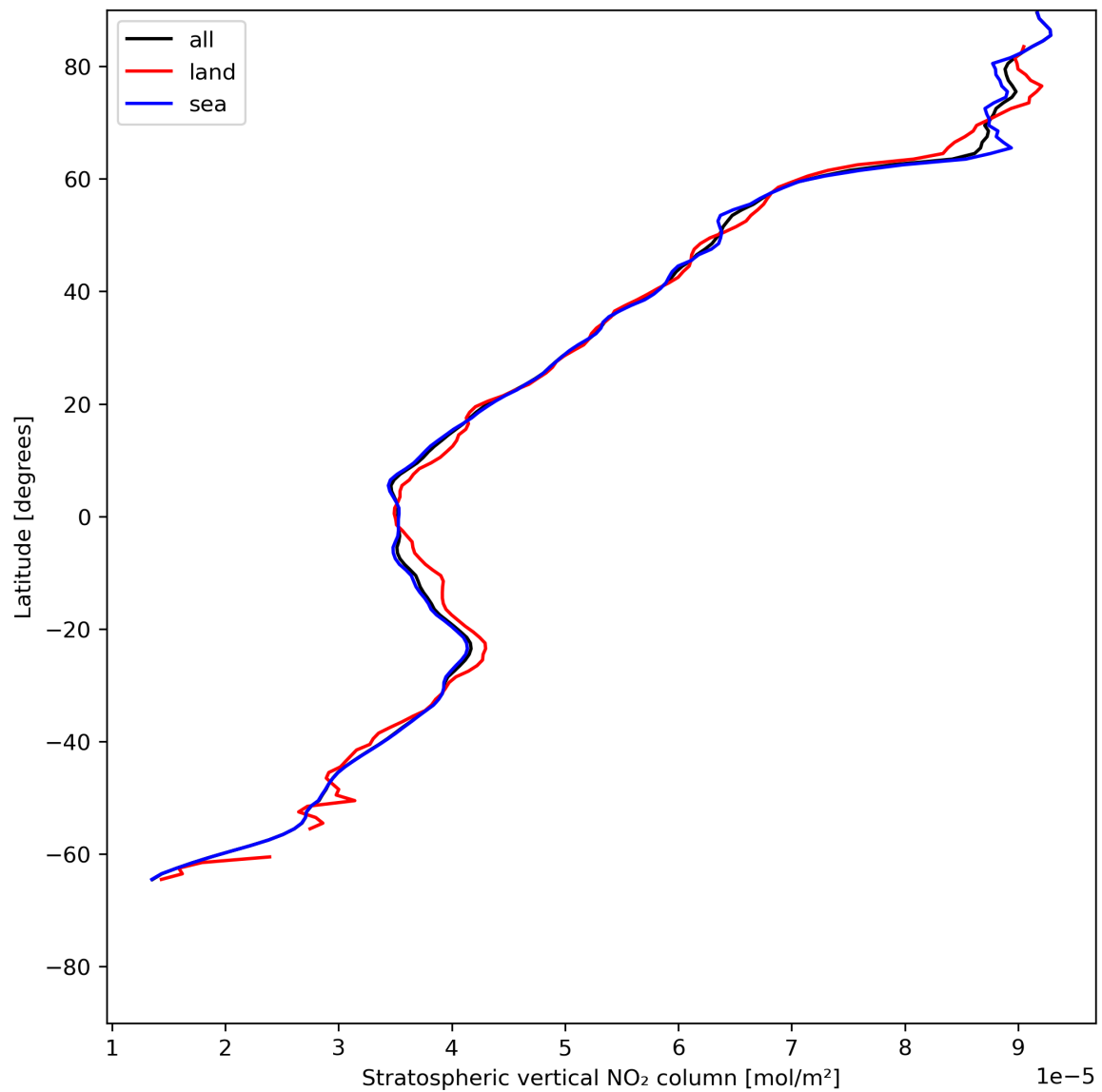
Figure 19: Zonal average of “Stratospheric vertical NO 2 column” for 2024-06-13 to 2024-06-15.
