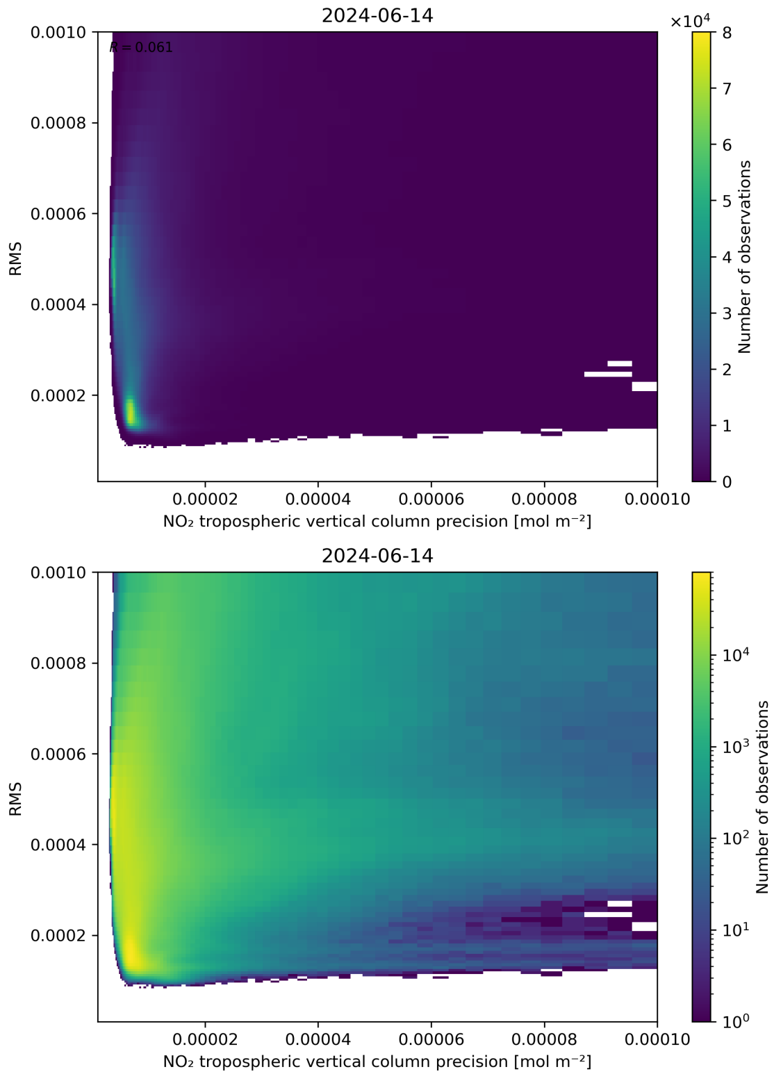
Figure 140: Scatter density plot of “NO 2 tropospheric vertical column precision” against “RMS” for 2024-06-13 to 2024-06-15.
