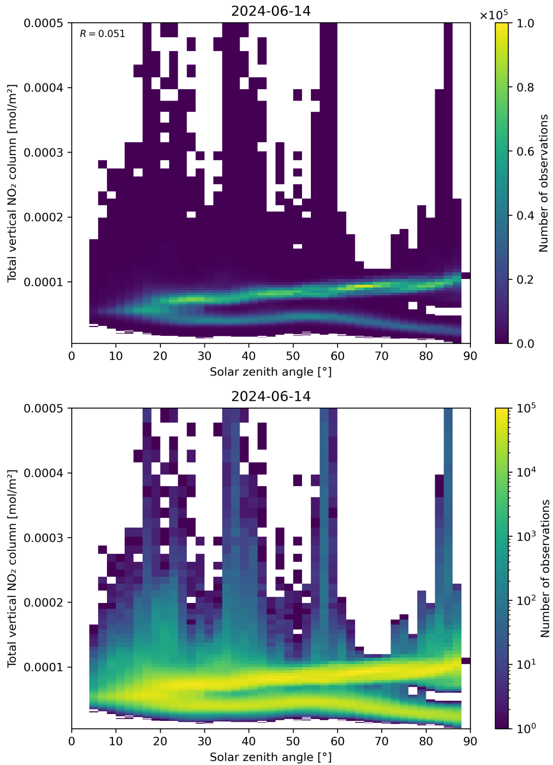
Figure 153: Scatter density plot of “Solar zenith angle” against “Total vertical NO 2 column” for 2024-06-13 to 2024-06-15.
