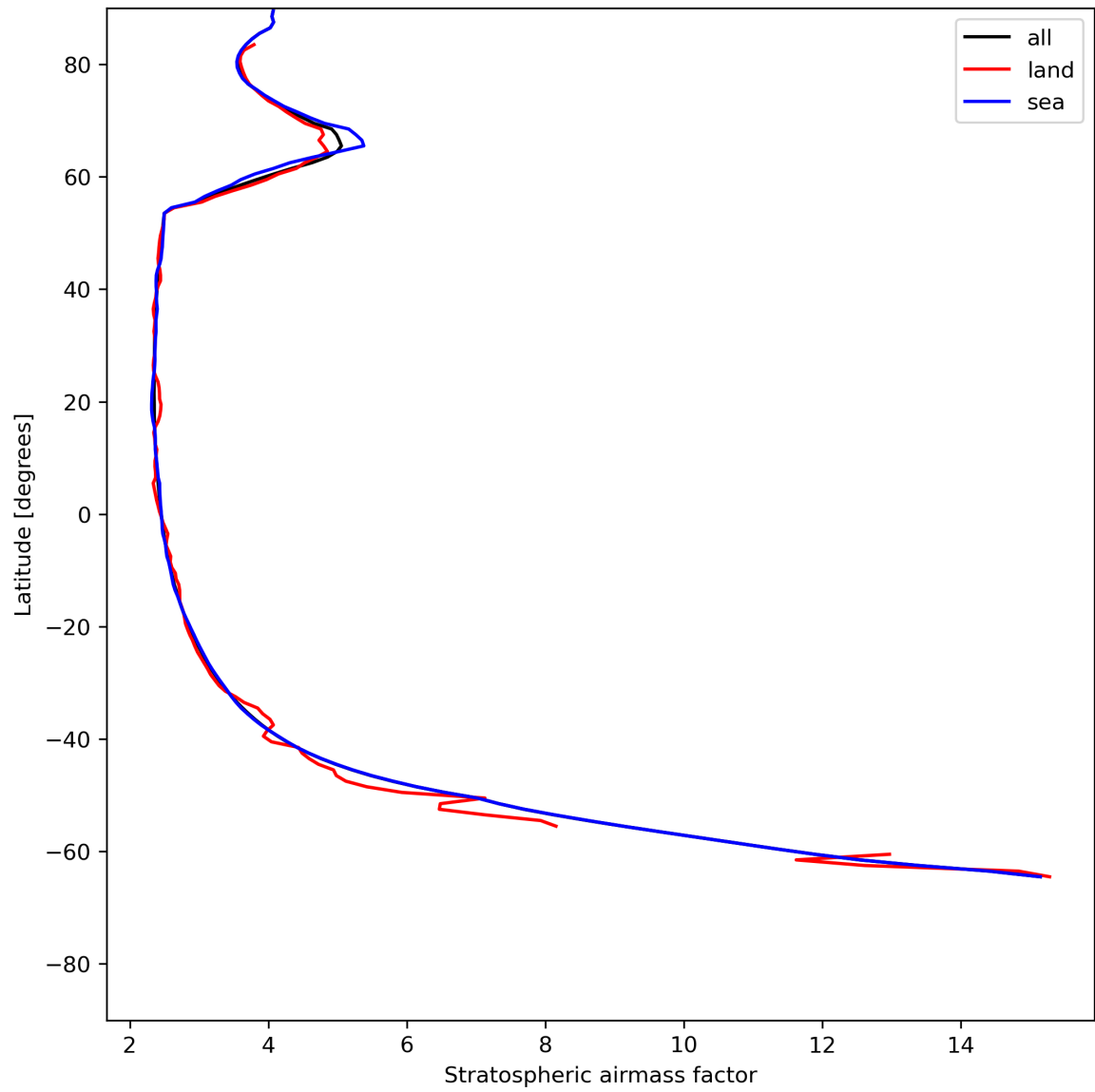
Figure 27: Zonal average of “Stratospheric air mass factor” for 2024-06-13 to 2024-06-15.
