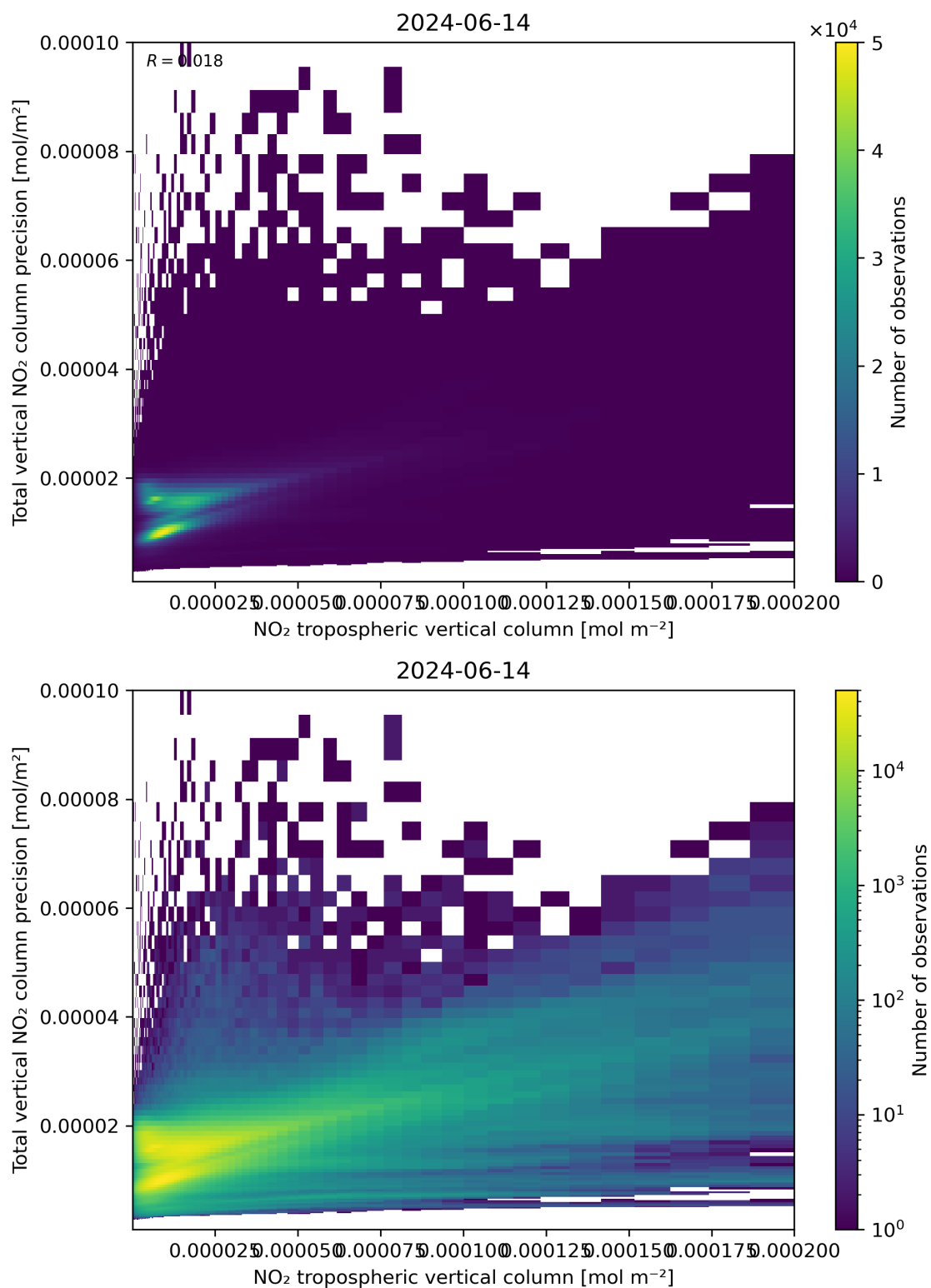
Figure 129: Scatter density plot of “NO 2 tropospheric vertical column” against “Total vertical NO 2 column precision” for 2024-06-13 to 2024-06-15.
