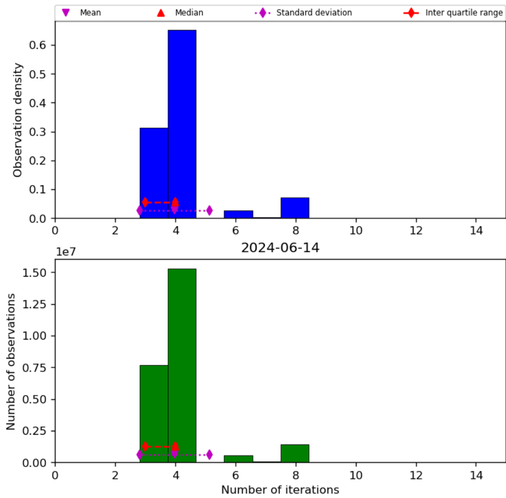
Figure 34: Histogram of “Number of iterations” for 2024-06-13 to 2024-06-15
