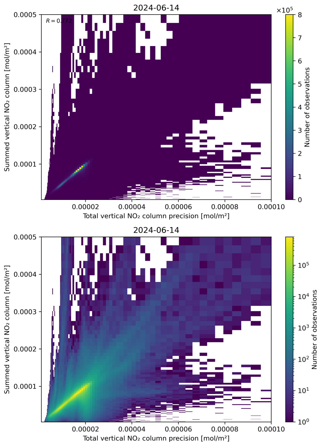
Figure 117: Scatter density plot of “Total vertical NO 2 column precision” against “Summed vertical NO 2 column” for 2024-06-13 to 2024-06-15.
