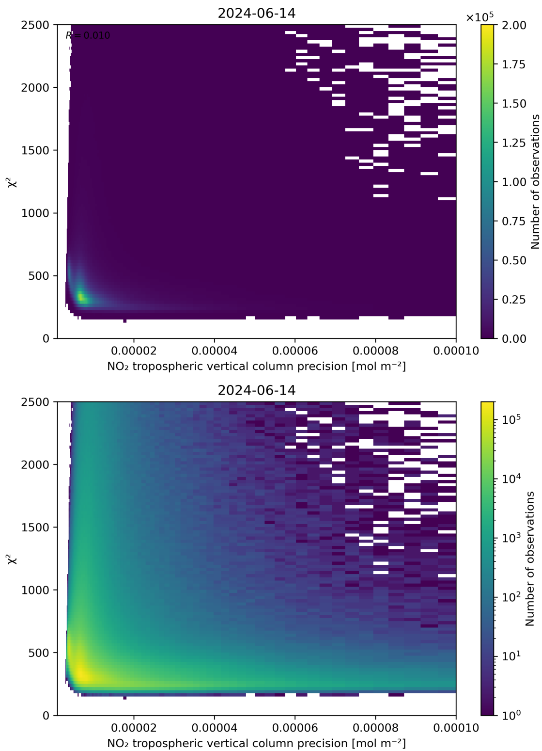
Figure 134: Scatter density plot of “NO 2 tropospheric vertical column precision” against “ \chi^2 ” for 2024-06-13 to 2024-06-15.
