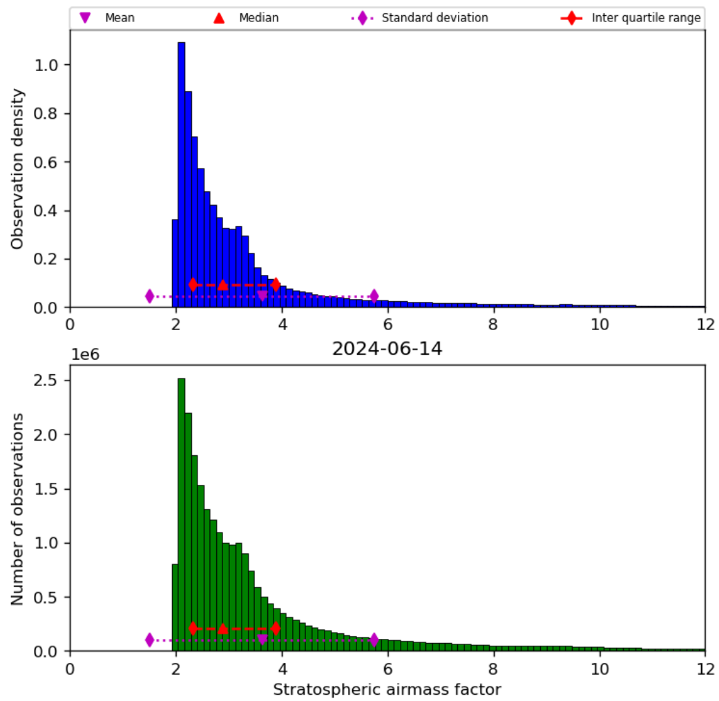
Figure 44: Histogram of “Stratospheric airmass factor” for 2024-06-13 to 2024-06-15
