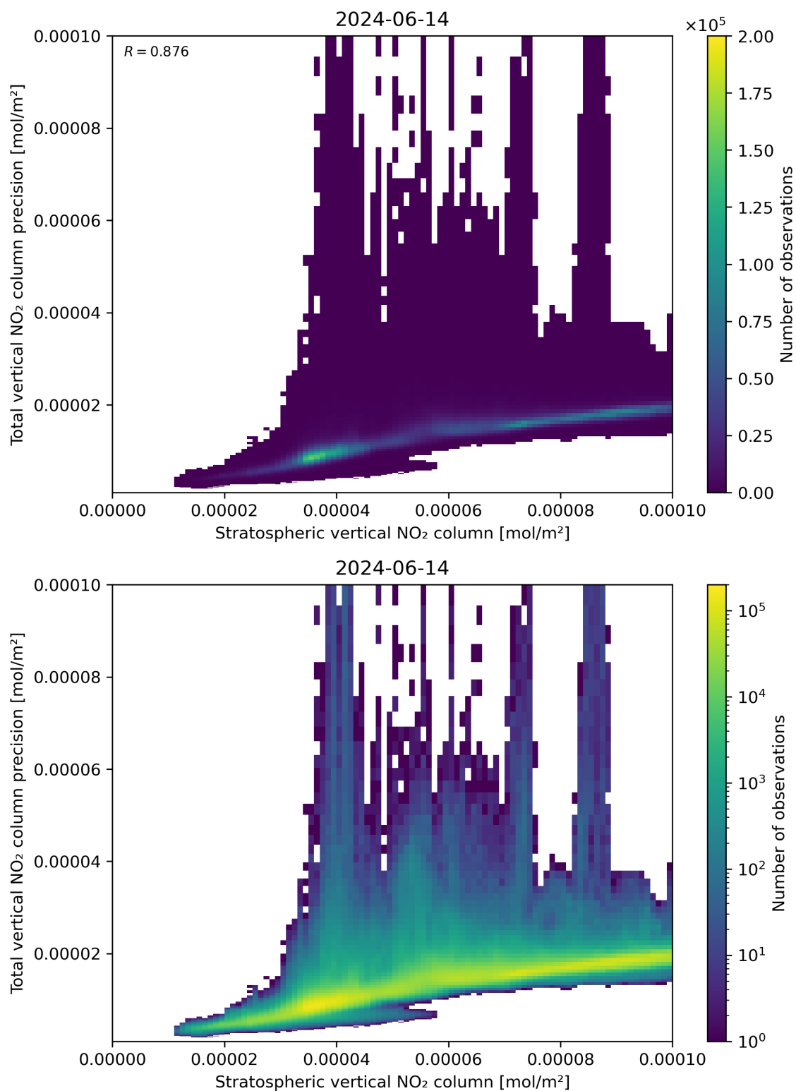
Figure 101: Scatter density plot of “Stratospheric vertical NO 2 column” against “Total vertical NO 2 column precision” for 2024-06-13 to 2024-06-15.
