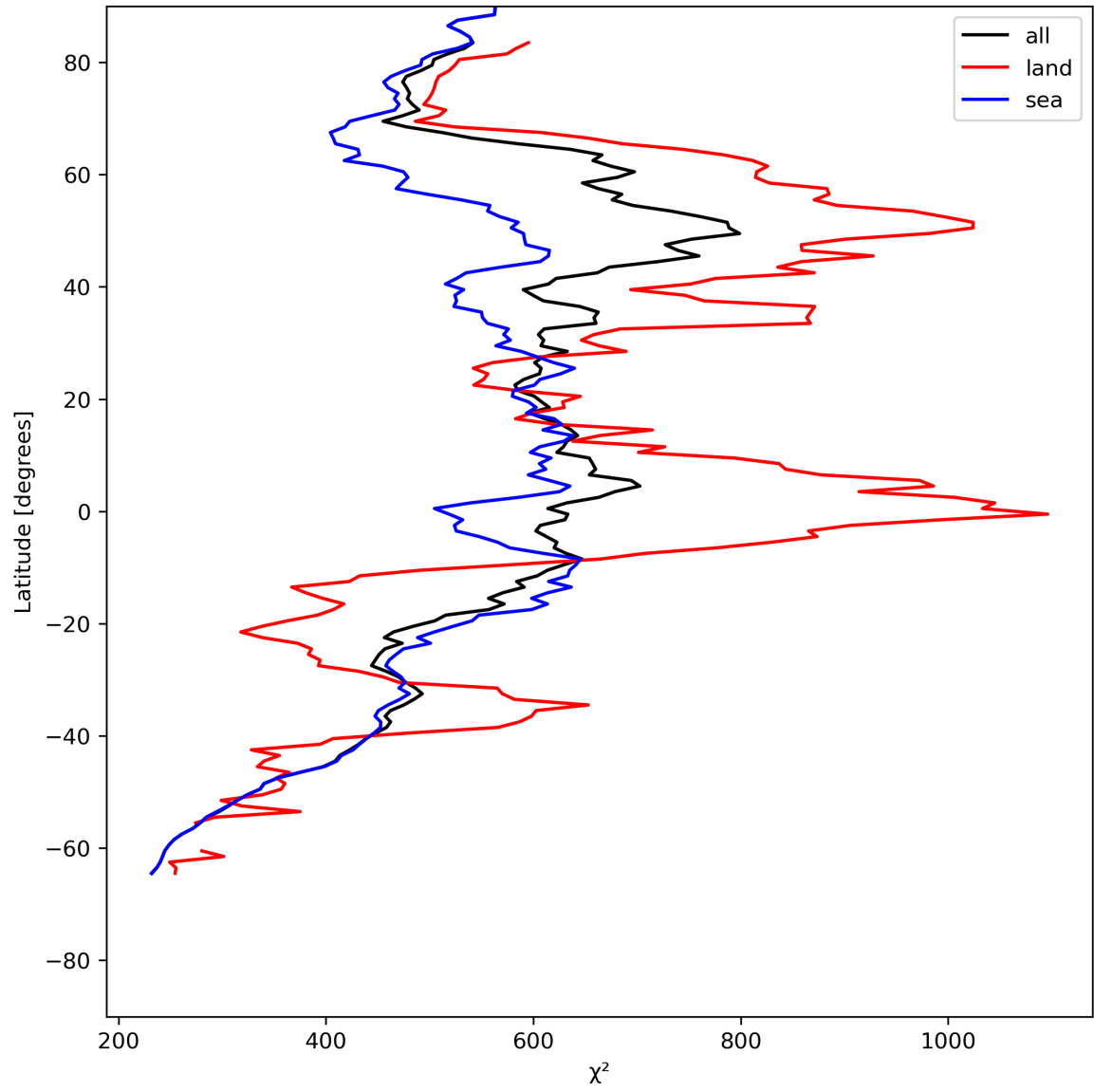
Figure 25: Zonal average of “ \chi^2 ” for 2024-06-13 to 2024-06-15.
