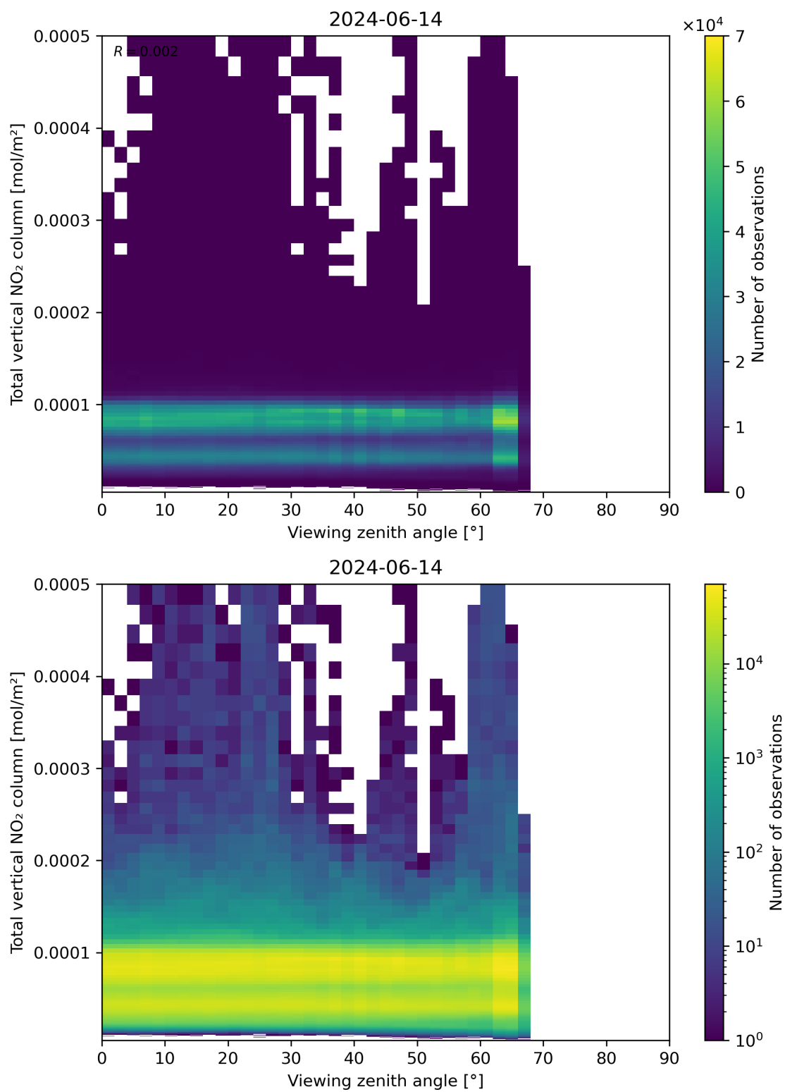
Figure 167: Scatter density plot of “Viewing zenith angle” against “Total vertical NO 2 column” for 2024-06-13 to 2024-06-15.
