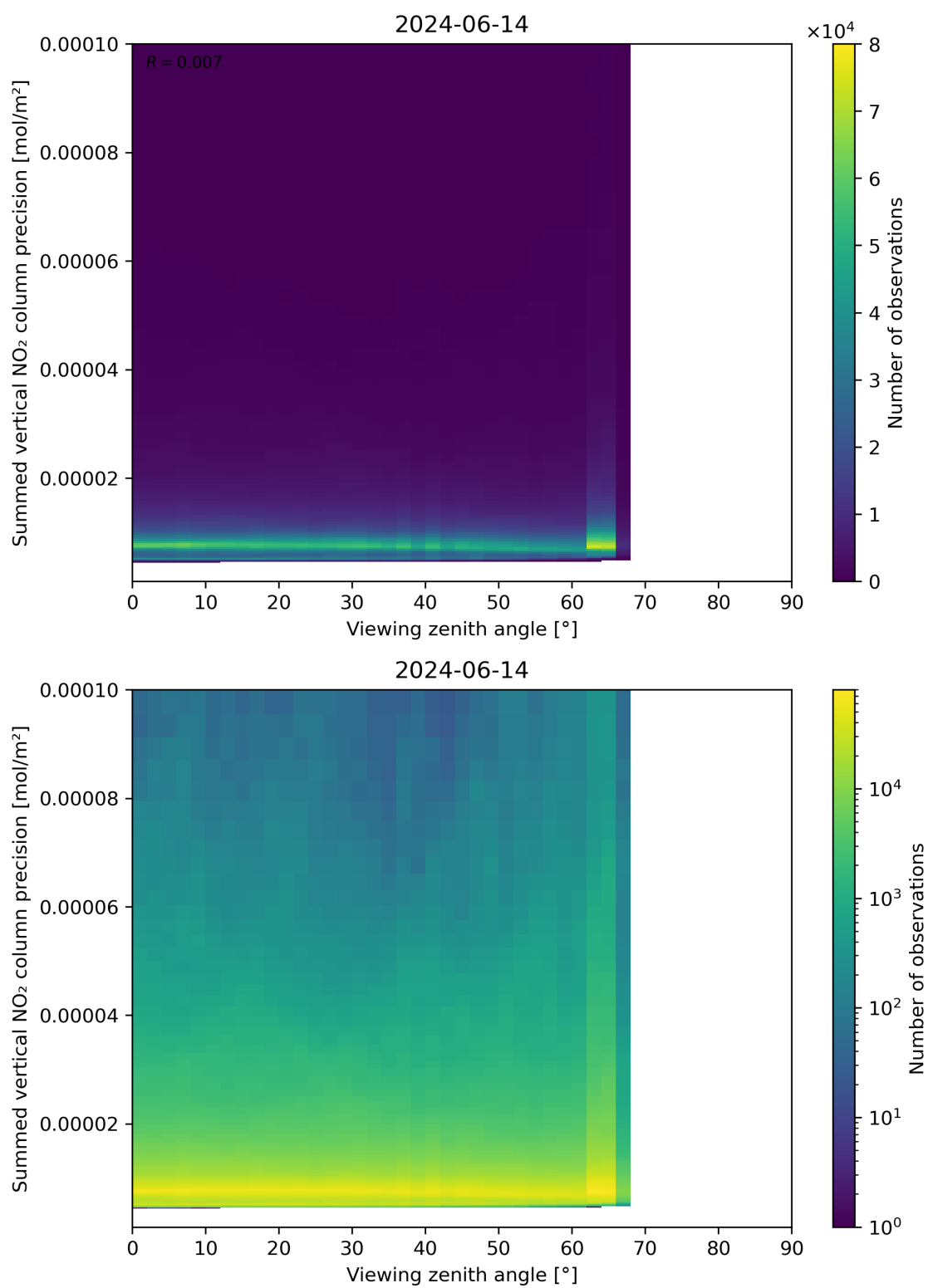
Figure 166: Scatter density plot of “Viewing zenith angle” against “Summed vertical NO 2 column precision” for 2024-06-13 to 2024-06-15.
