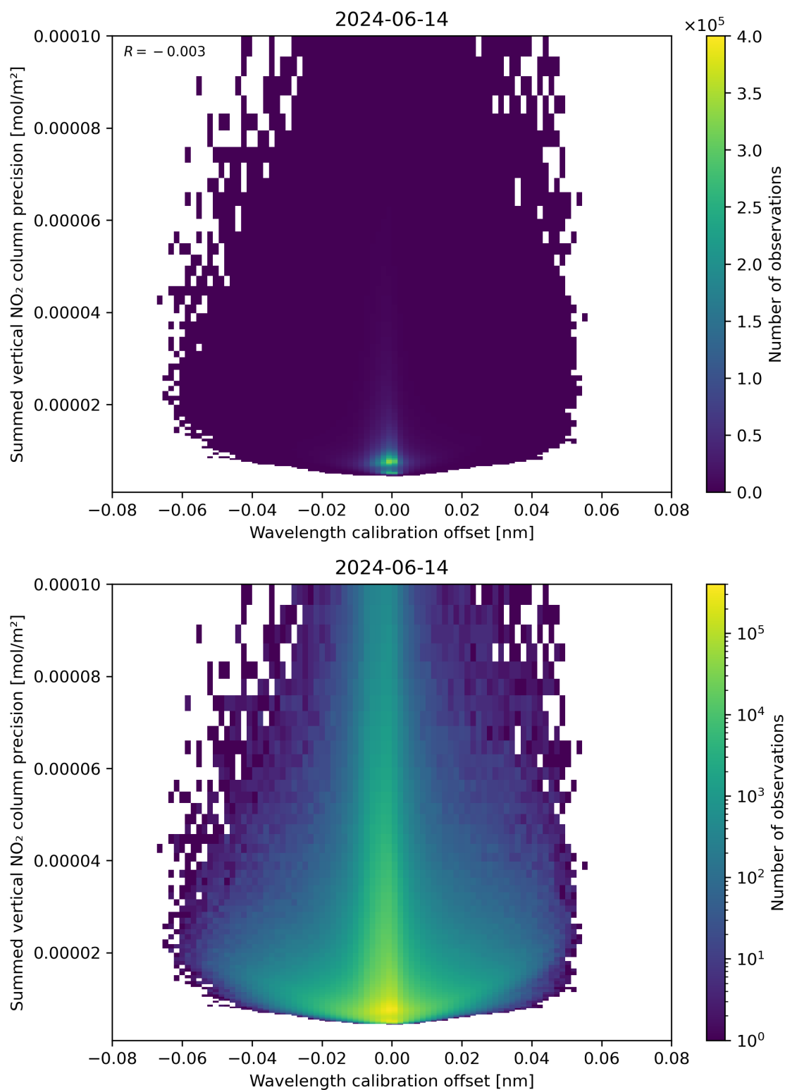
Figure 178: Scatter density plot of “Wavelength calibration offset” against “Summed vertical NO 2 column precision” for 2024-06-13 to 2024-06-15.
