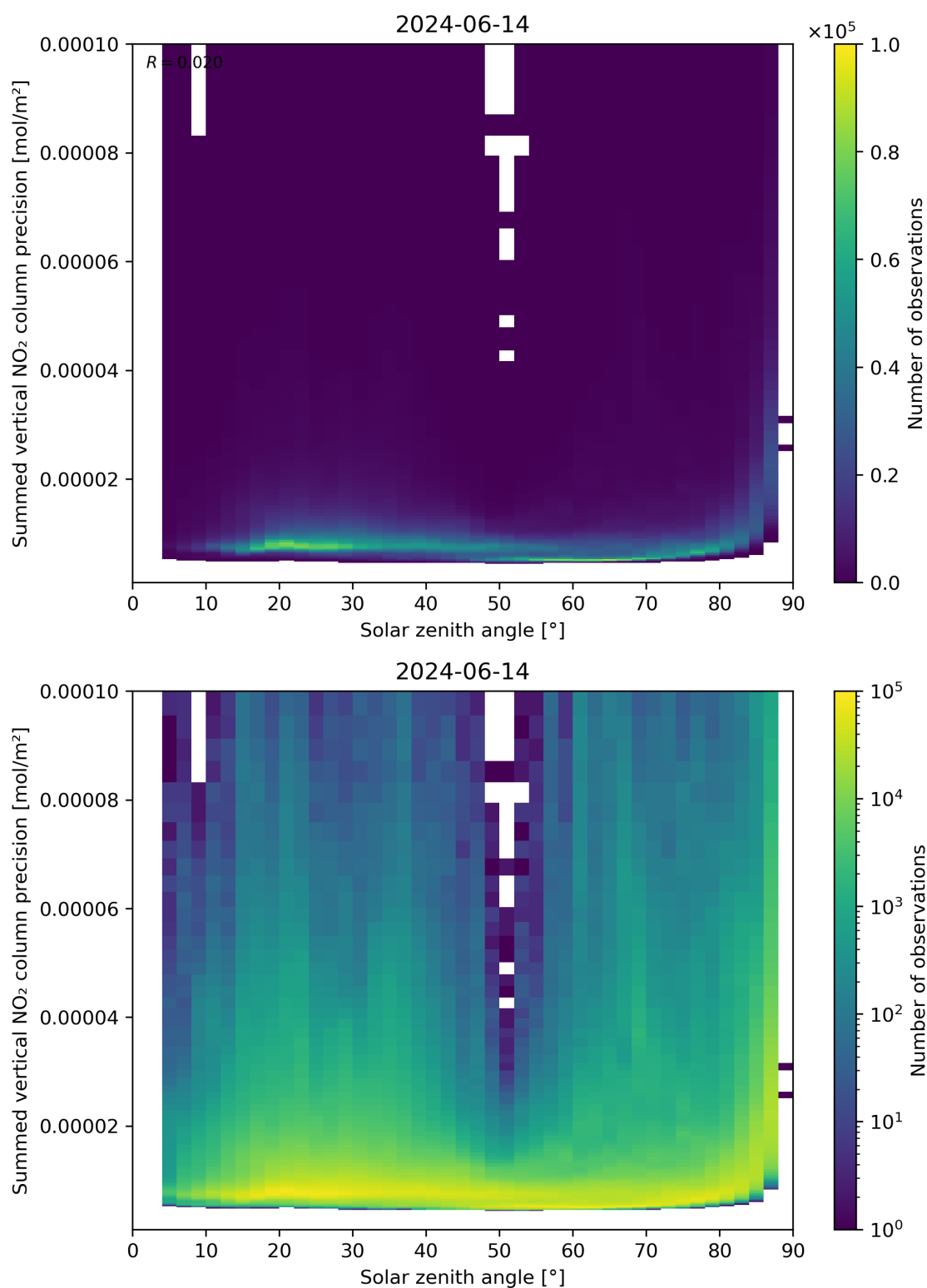
Figure 152: Scatter density plot of “Solar zenith angle” against “Summed vertical NO 2 column precision” for 2024-06-13 to 2024-06-15.
