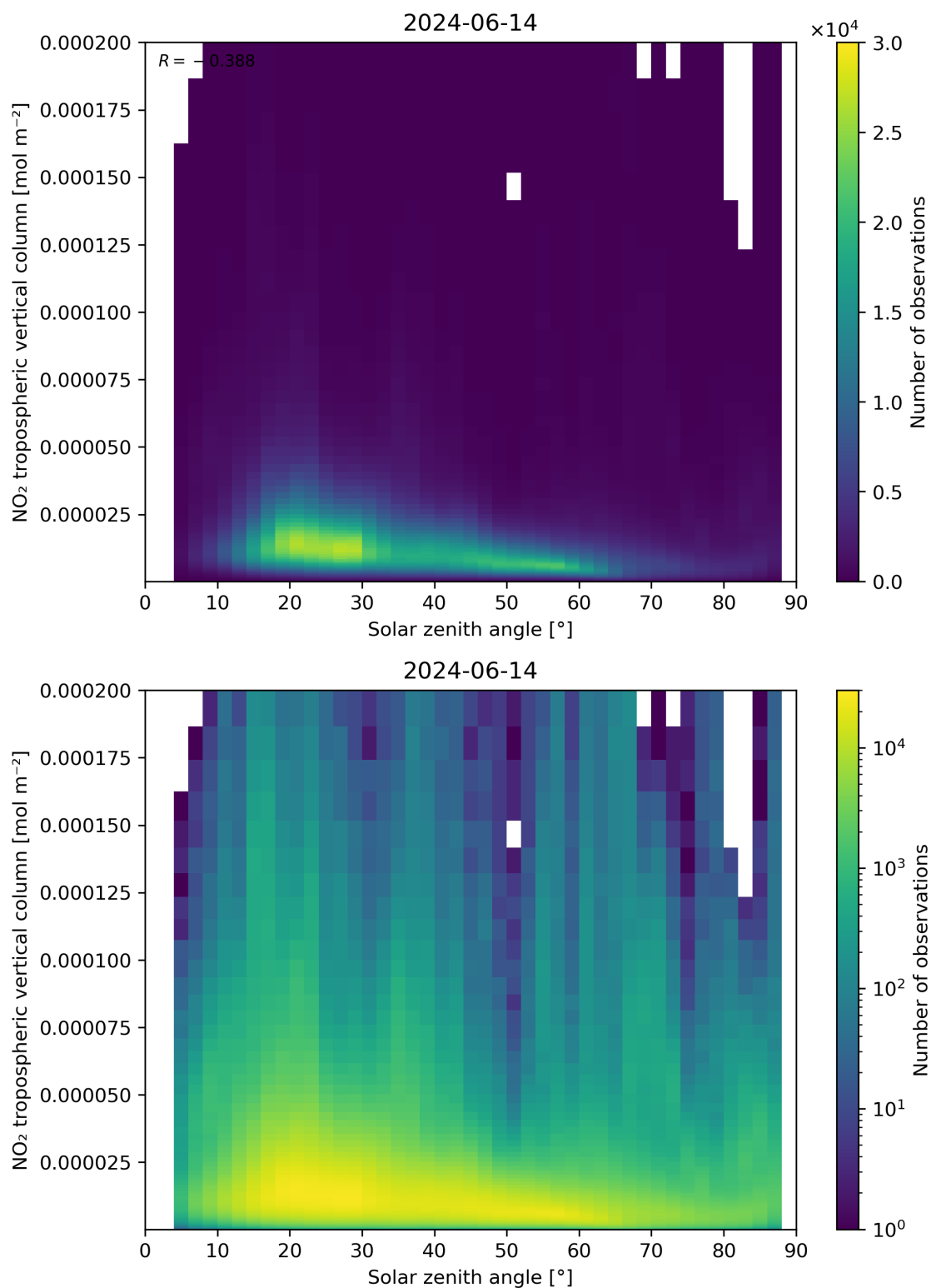
Figure 155: Scatter density plot of “Solar zenith angle” against “NO 2 tropospheric vertical column” for 2024-06-13 to 2024-06-15.
