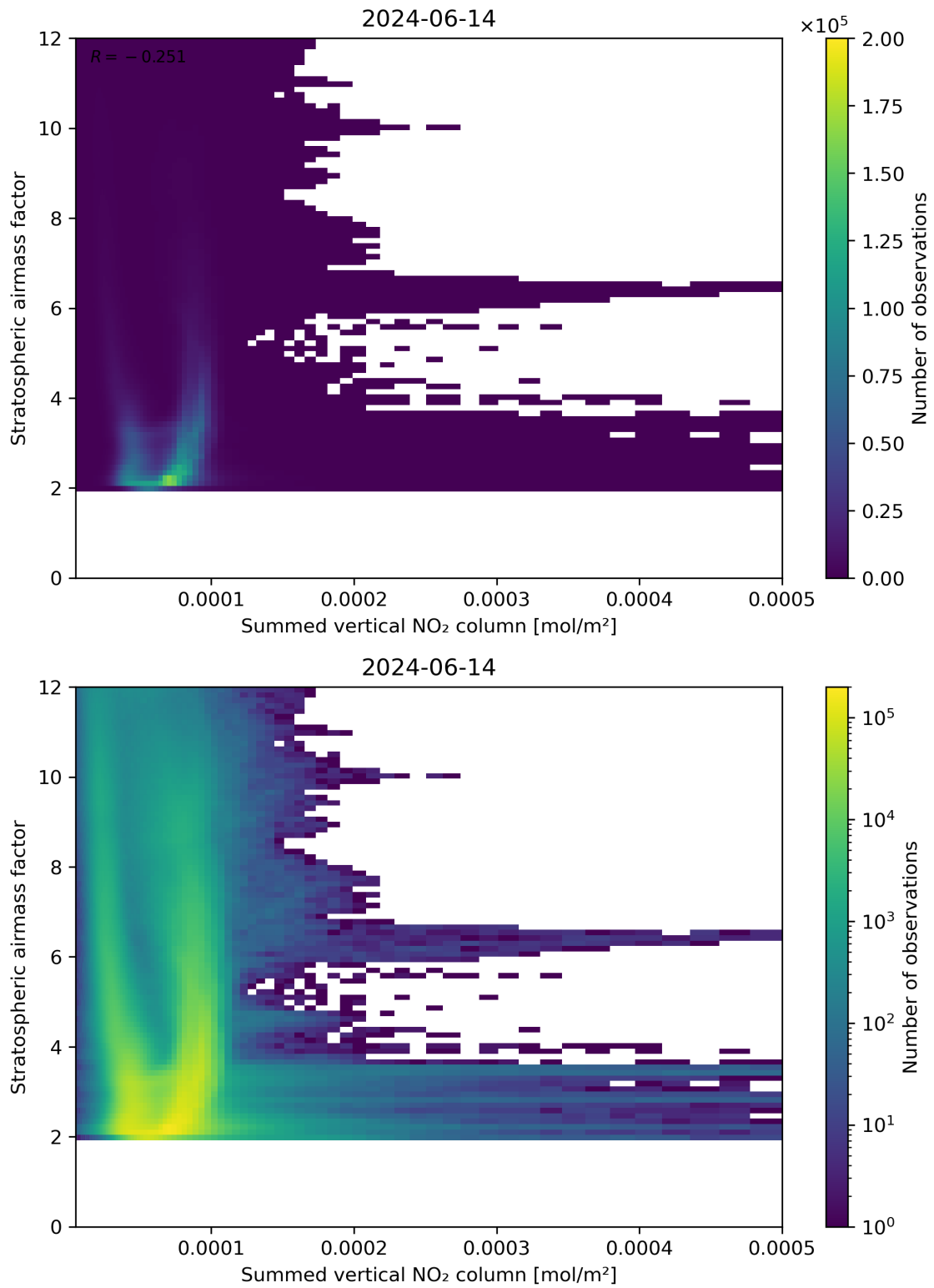
Figure 103: Scatter density plot of “Summed vertical NO 2 column” against “Stratospheric air mass factor” for 2024-06-13 to 2024-06-15.
