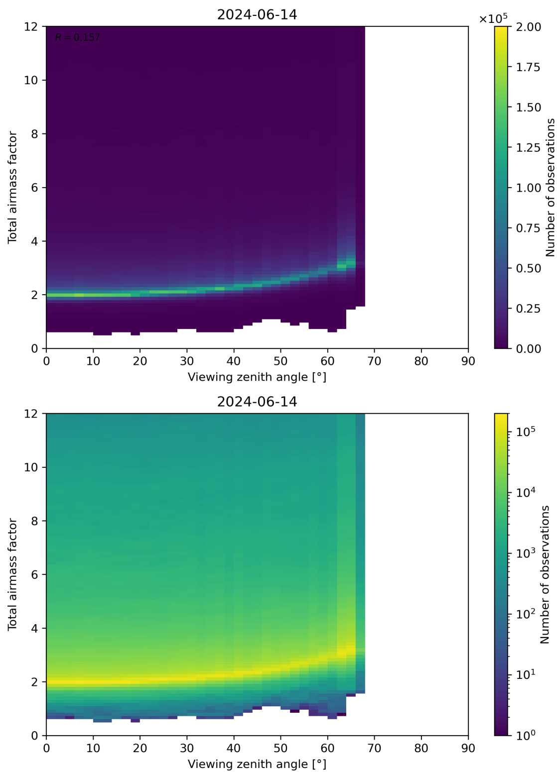
Figure 160: Scatter density plot of “Viewing zenith angle” against “Total airmass factor” for 2024-06-13 to 2024-06-15.
