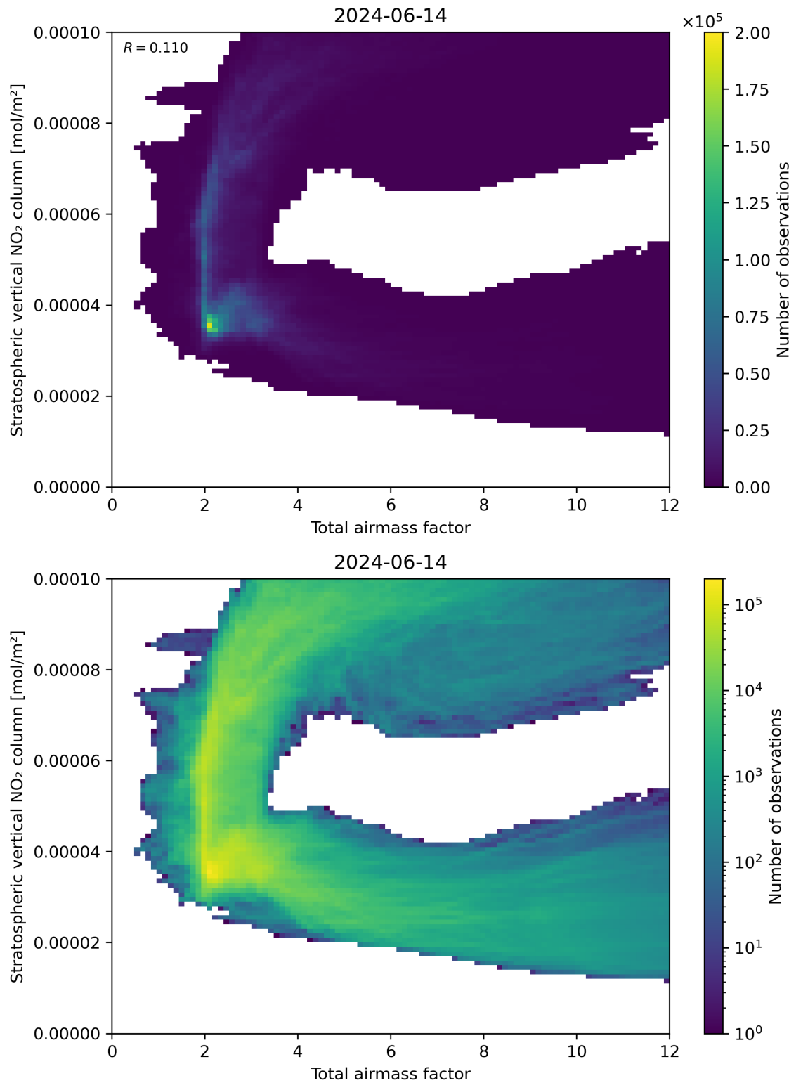
Figure 64: Scatter density plot of “Total airmass factor” against “Stratospheric vertical NO 2 column” for 2024-06-13 to 2024-06-15.
