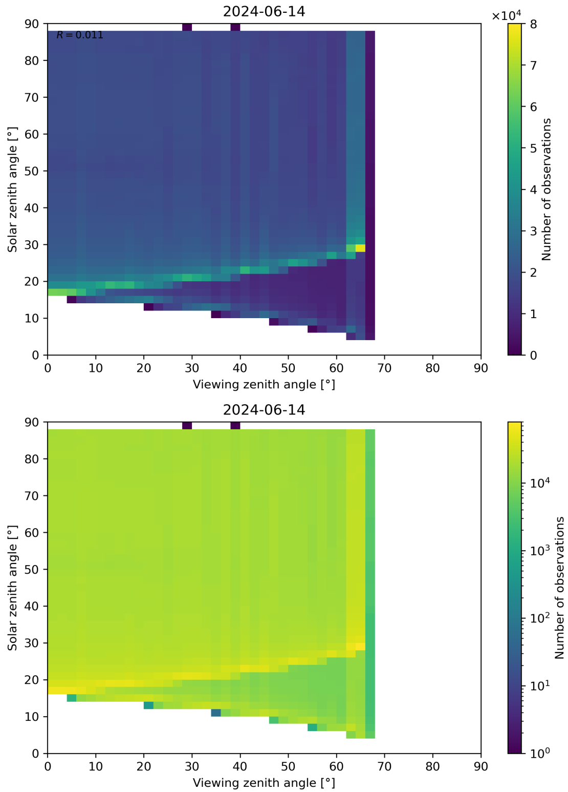
Figure 172: Scatter density plot of “Viewing zenith angle” against “Solar zenith angle” for 2024-06-13 to 2024-06-15.
