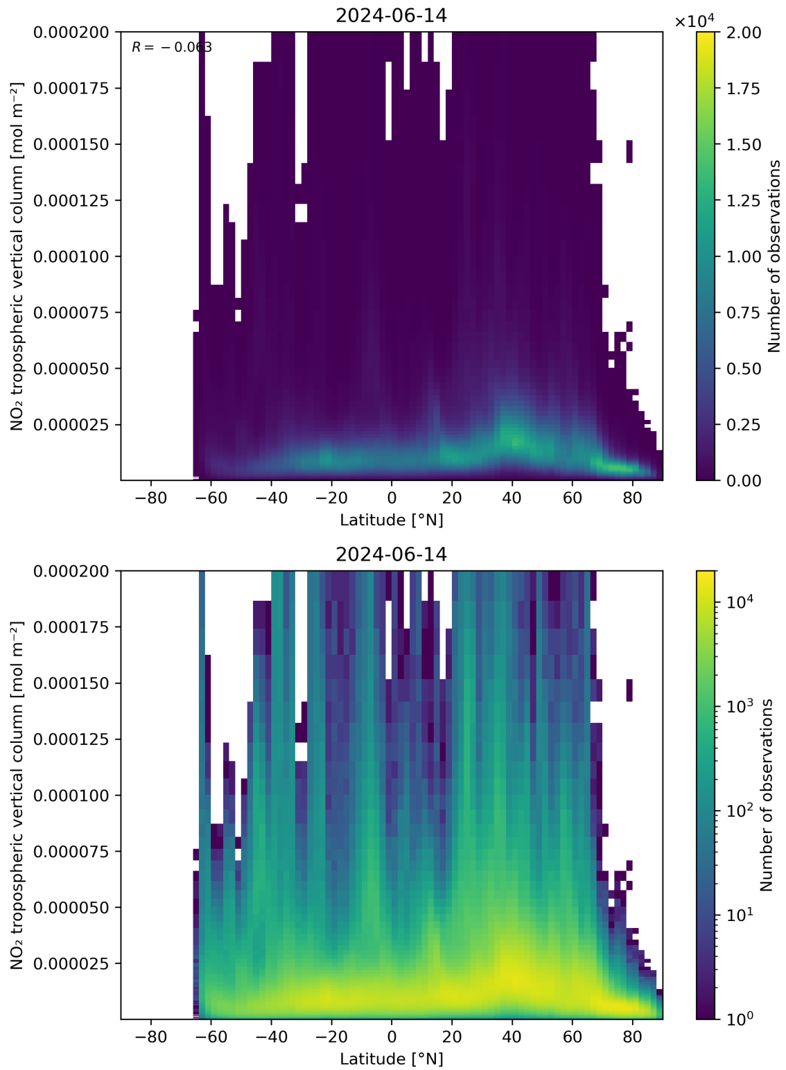
Figure 92: Scatter density plot of “Latitude” against “NO 2 tropospheric vertical column” for 2024-06-13 to 2024-06-15.
