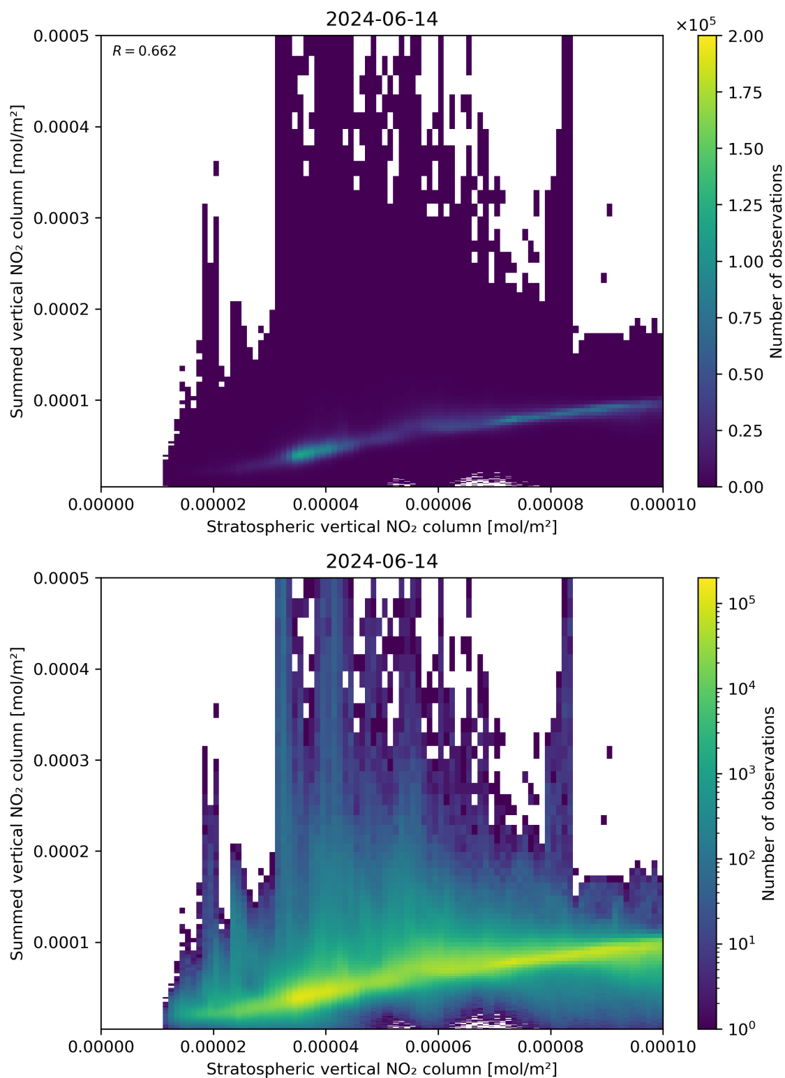
Figure 98: Scatter density plot of “Stratospheric vertical NO 2 column” against “Summed vertical NO 2 column” for 2024-06-13 to 2024-06-15.
