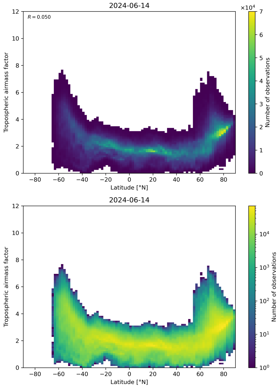
Figure 85: Scatter density plot of “Latitude” against “Tropospheric airmass factor” for 2024-06-13 to 2024-06-15.
