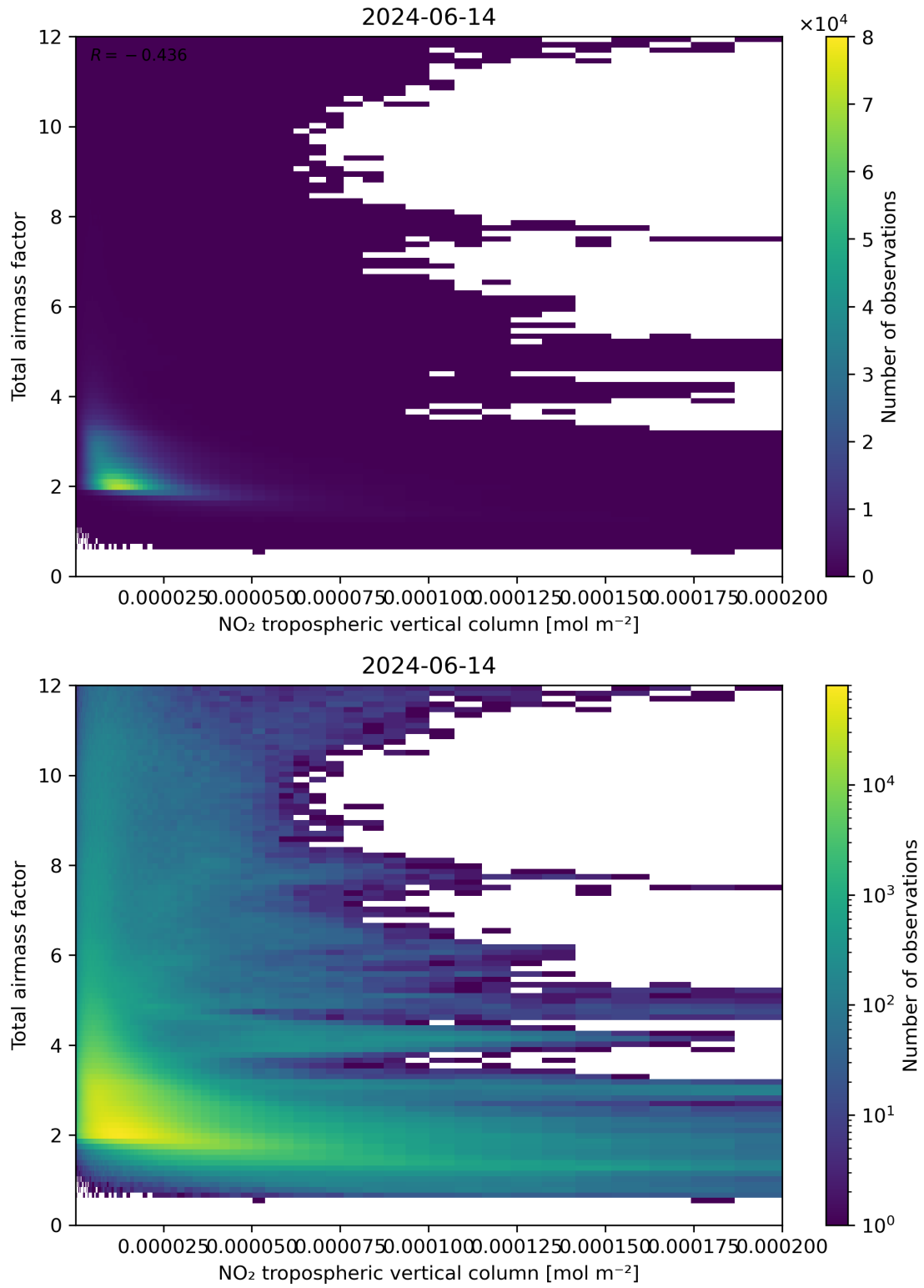
Figure 122: Scatter density plot of “NO 2 tropospheric vertical column” against “Total air mass factor” for 2024-06-13 to 2024-06-15.
