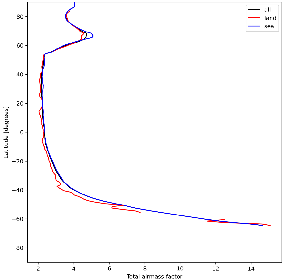
Figure 15: Zonal average of “Total airmass factor” for 2024-06-13 to 2024-06-15.
