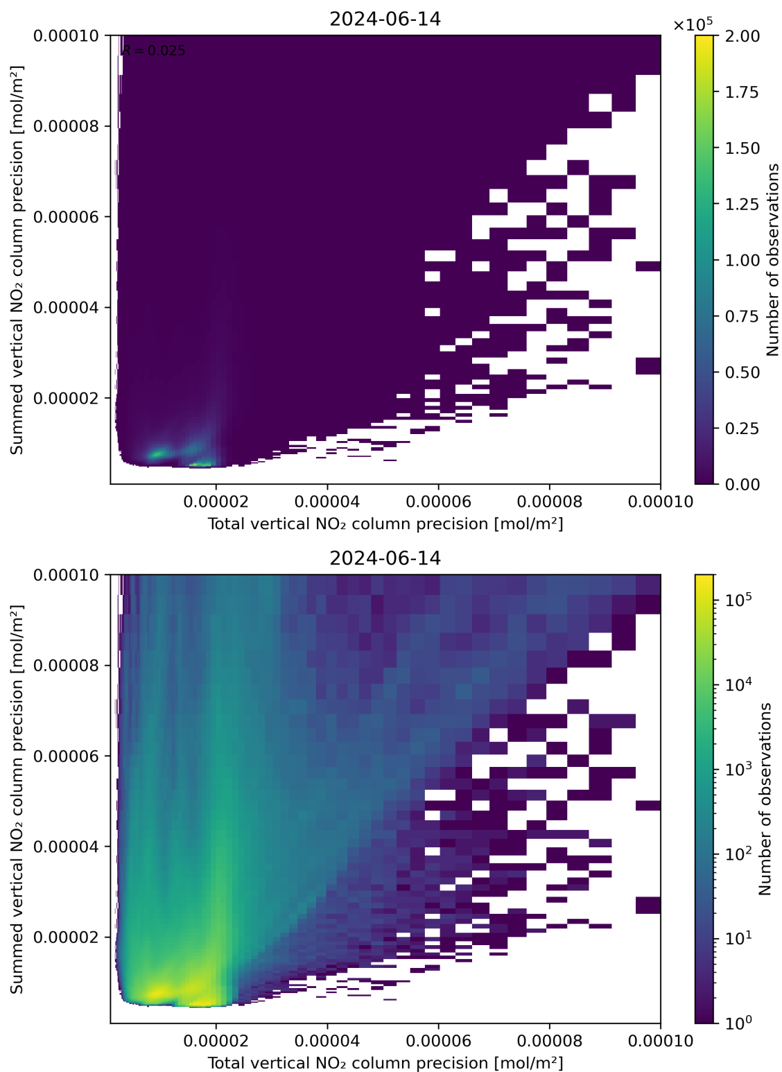
Figure 118: Scatter density plot of “Total vertical NO 2 column precision” against “Summed vertical NO 2 column precision” for 2024-06-13 to 2024-06-15.
