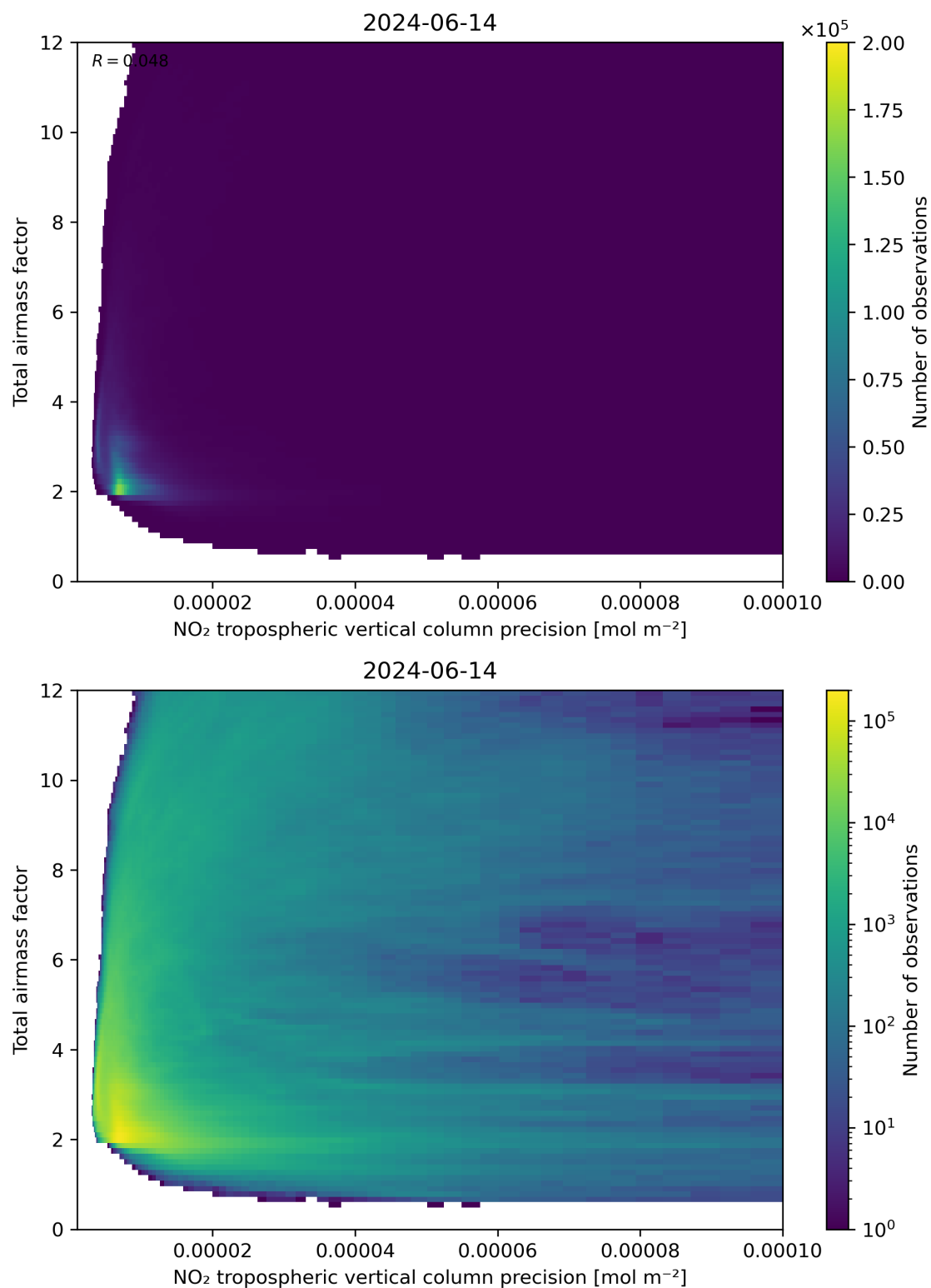
Figure 132: Scatter density plot of “NO 2 tropospheric vertical column precision” against “Total air mass factor” for 2024-06-13 to 2024-06-15.
