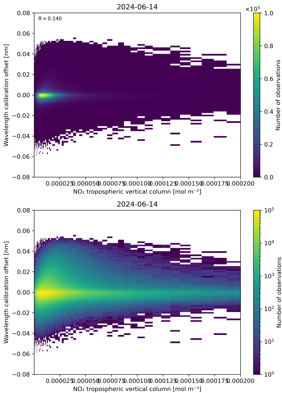
Figure 143: Scatter density plot of “NO 2 tropospheric vertical column” against “Wavelength calibration offset” for 2024-06-13 to 2024-06-15.
