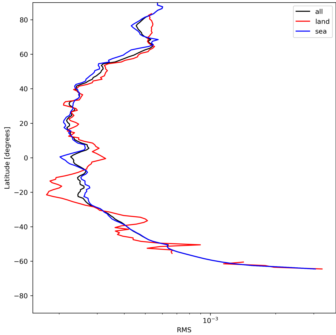
Figure 26: Zonal average of “RMS” for 2024-06-13 to 2024-06-15.
