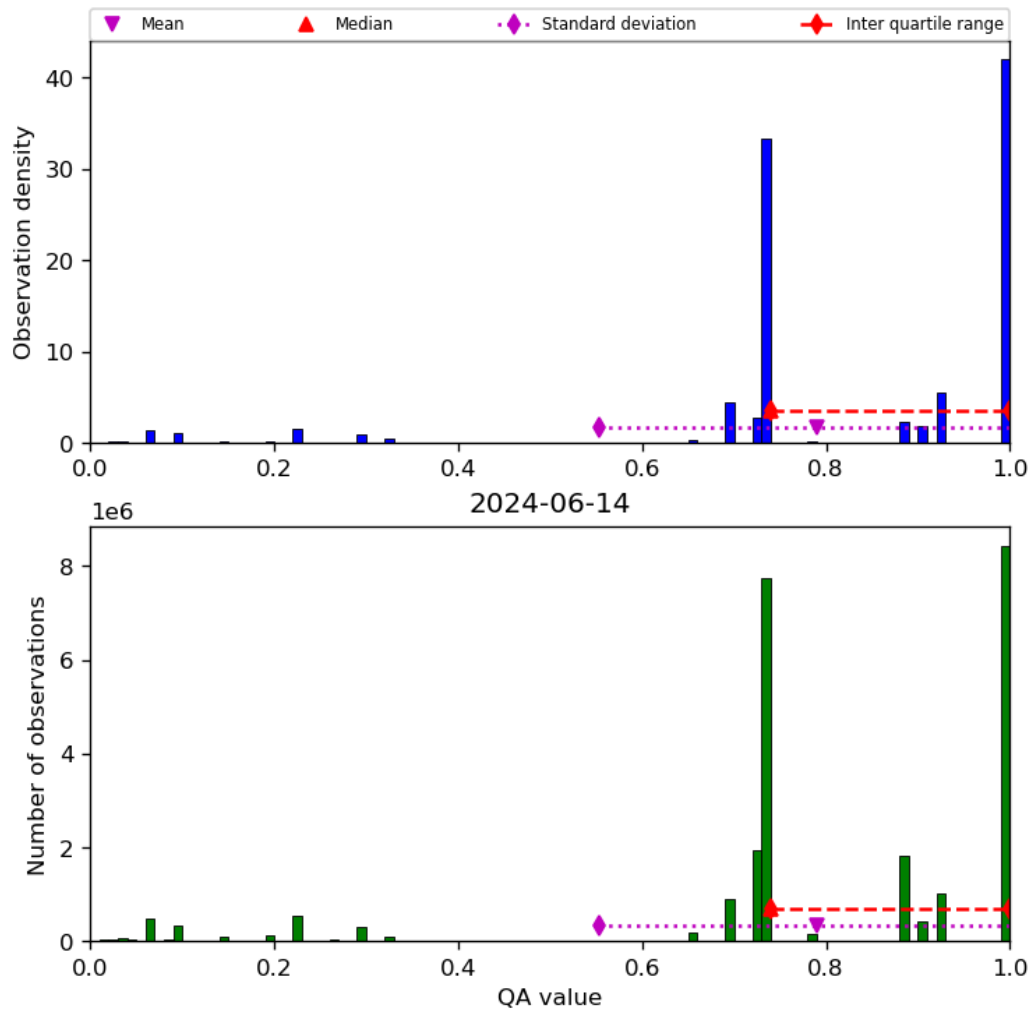
Figure 28: Histogram of “QA value” for 2024-06-13 to 2024-06-15
