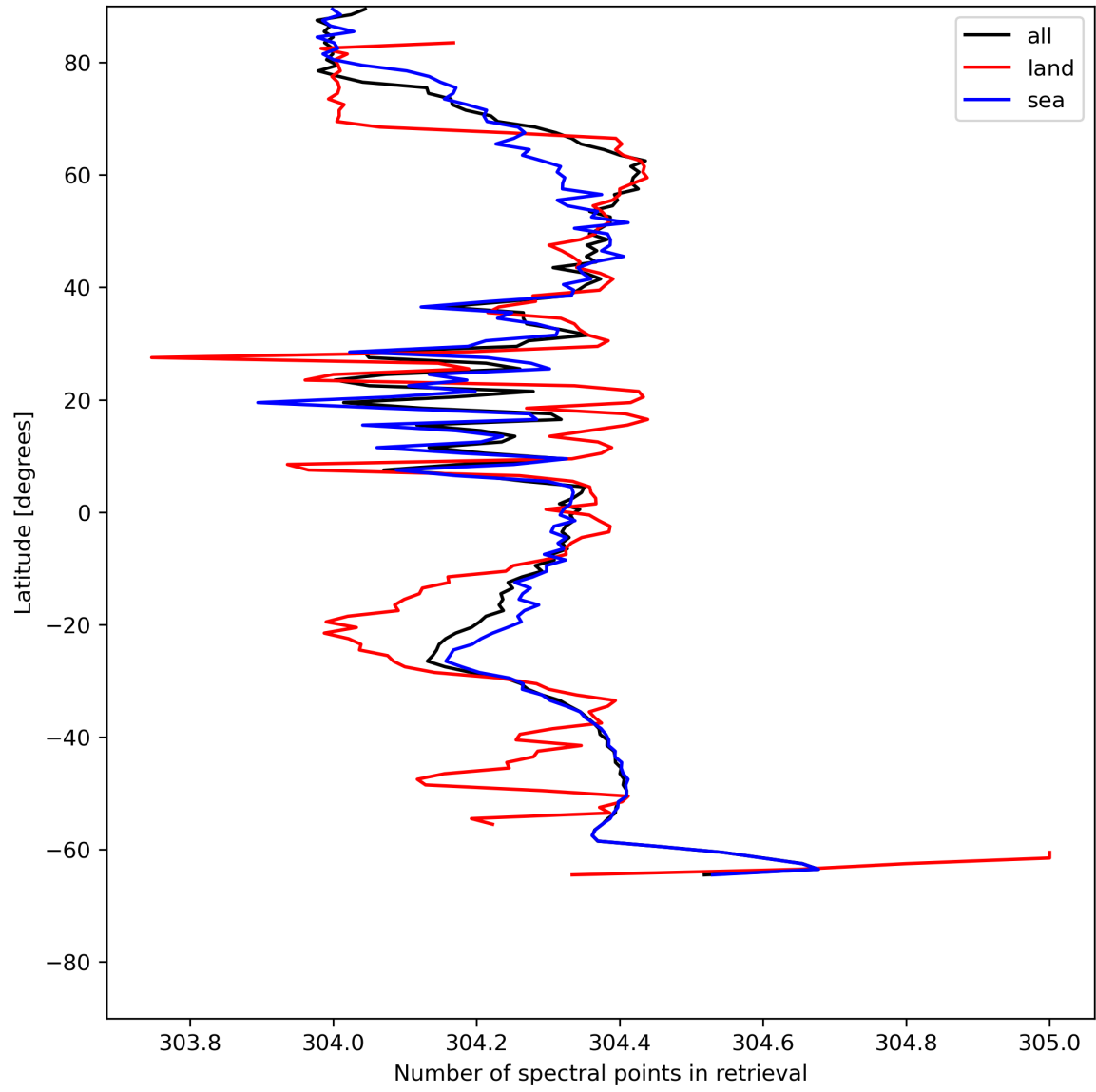
Figure 16: Zonal average of “Number of spectral points in retrieval” for 2024-06-13 to 2024-06-15.
