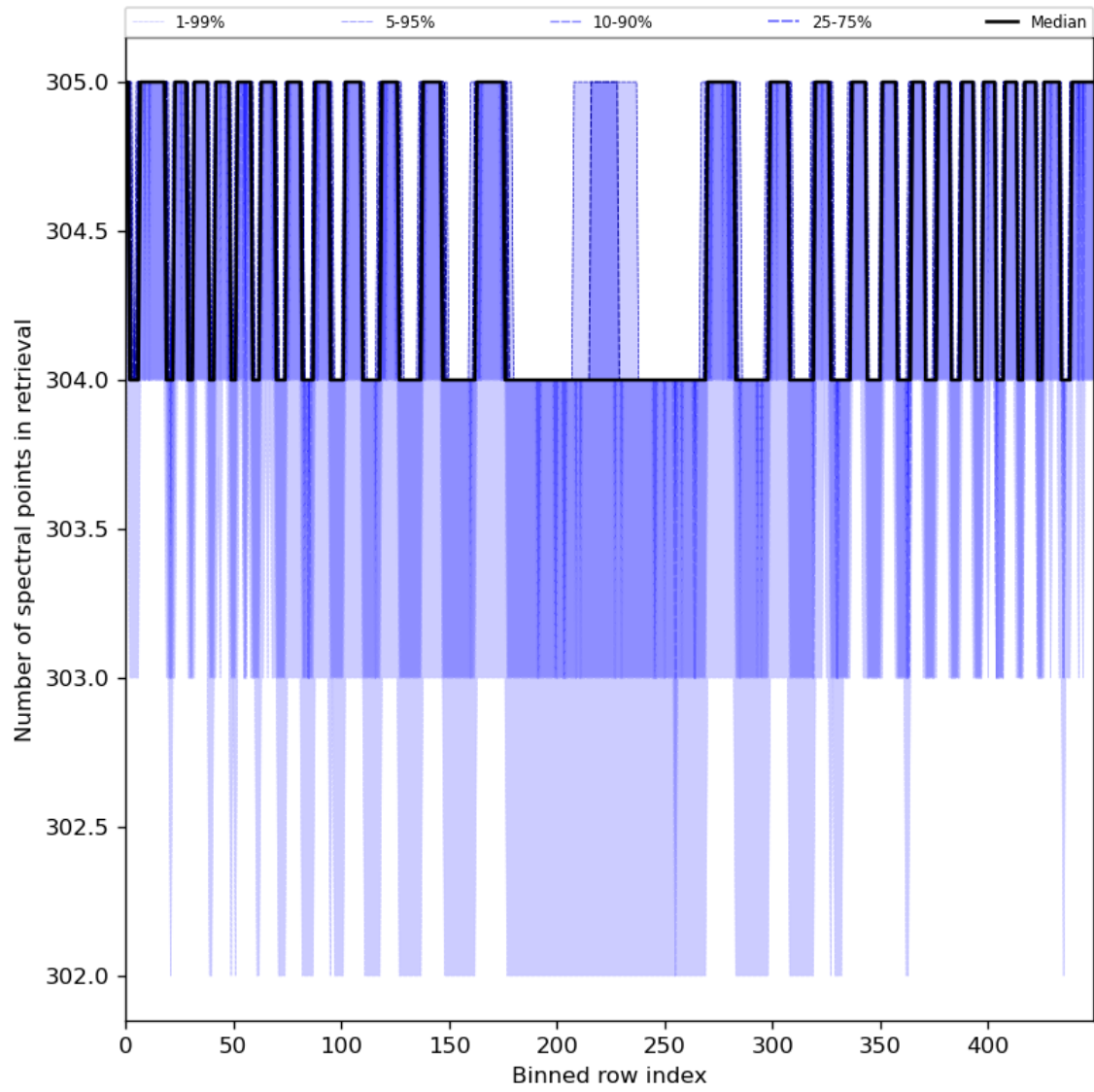
Figure 50: Along track statistics of “Number of spectral points in retrieval” for 2024-06-13 to 2024-06-15
