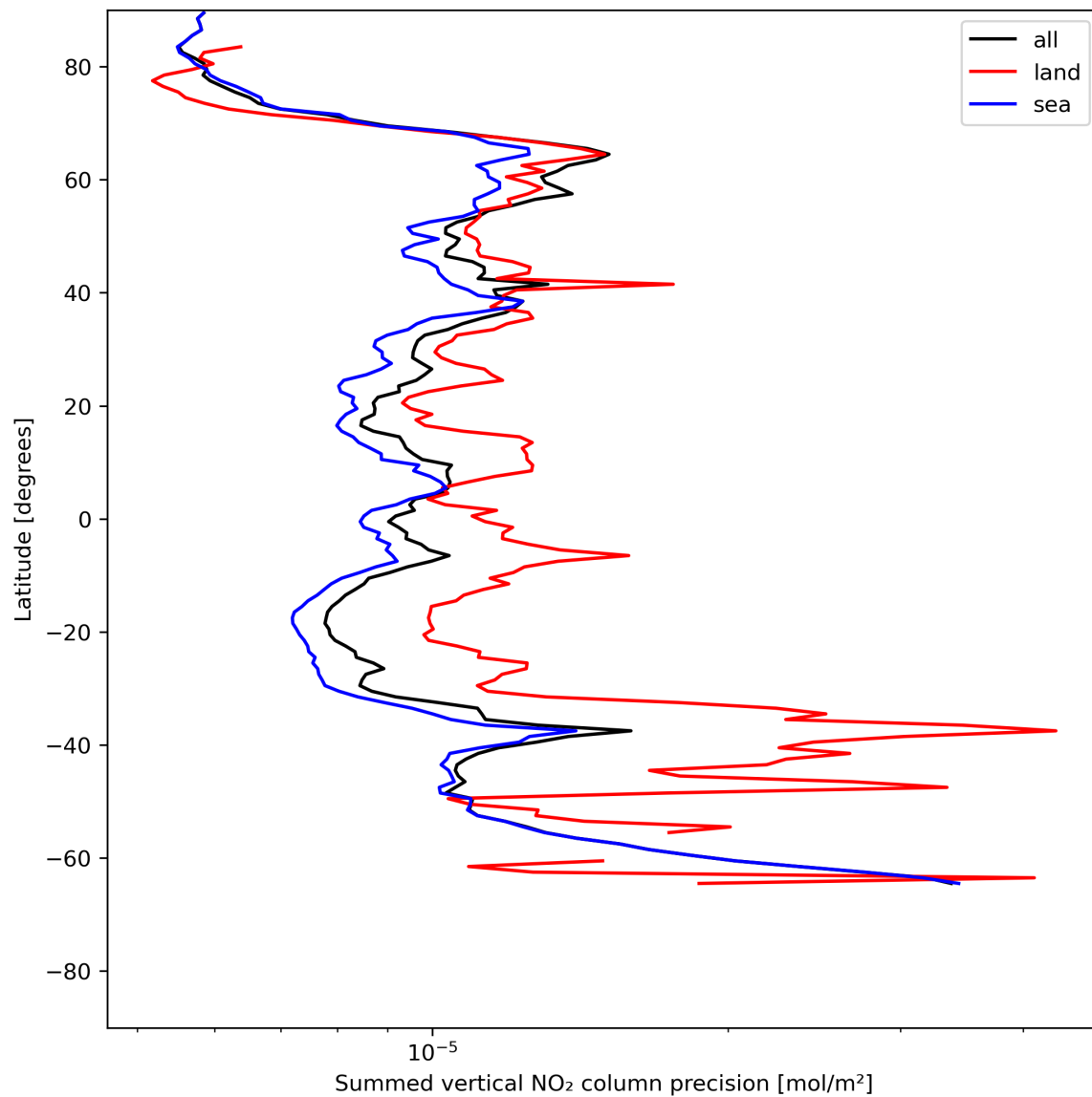
Figure 24: Zonal average of “Summed vertical NO 2 column precision” for 2024-06-13 to 2024-06-15.
