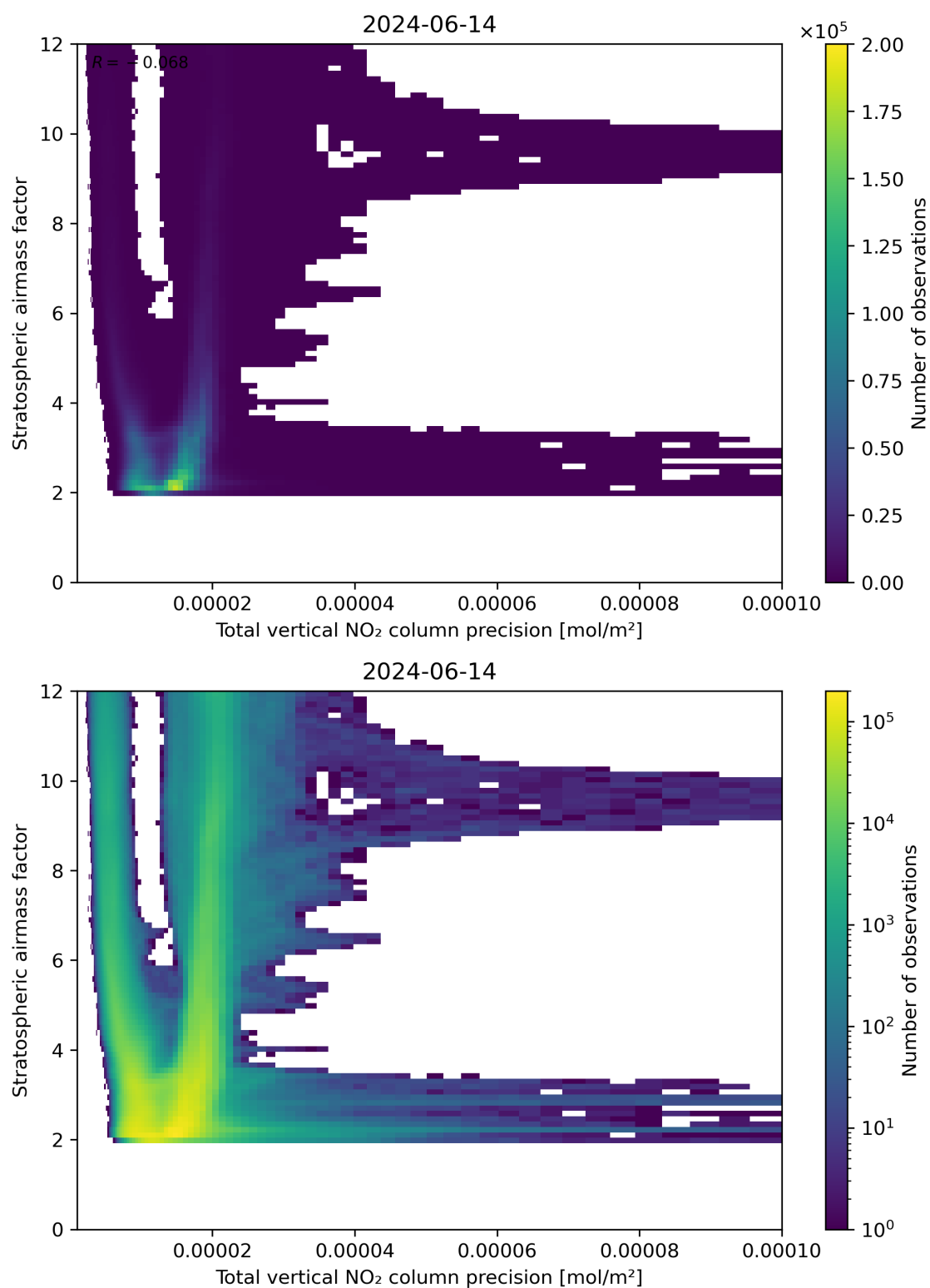
Figure 115: Scatter density plot of “Total vertical NO 2 column precision” against “Stratospheric airmass factor” for 2024-06-13 to 2024-06-15.
