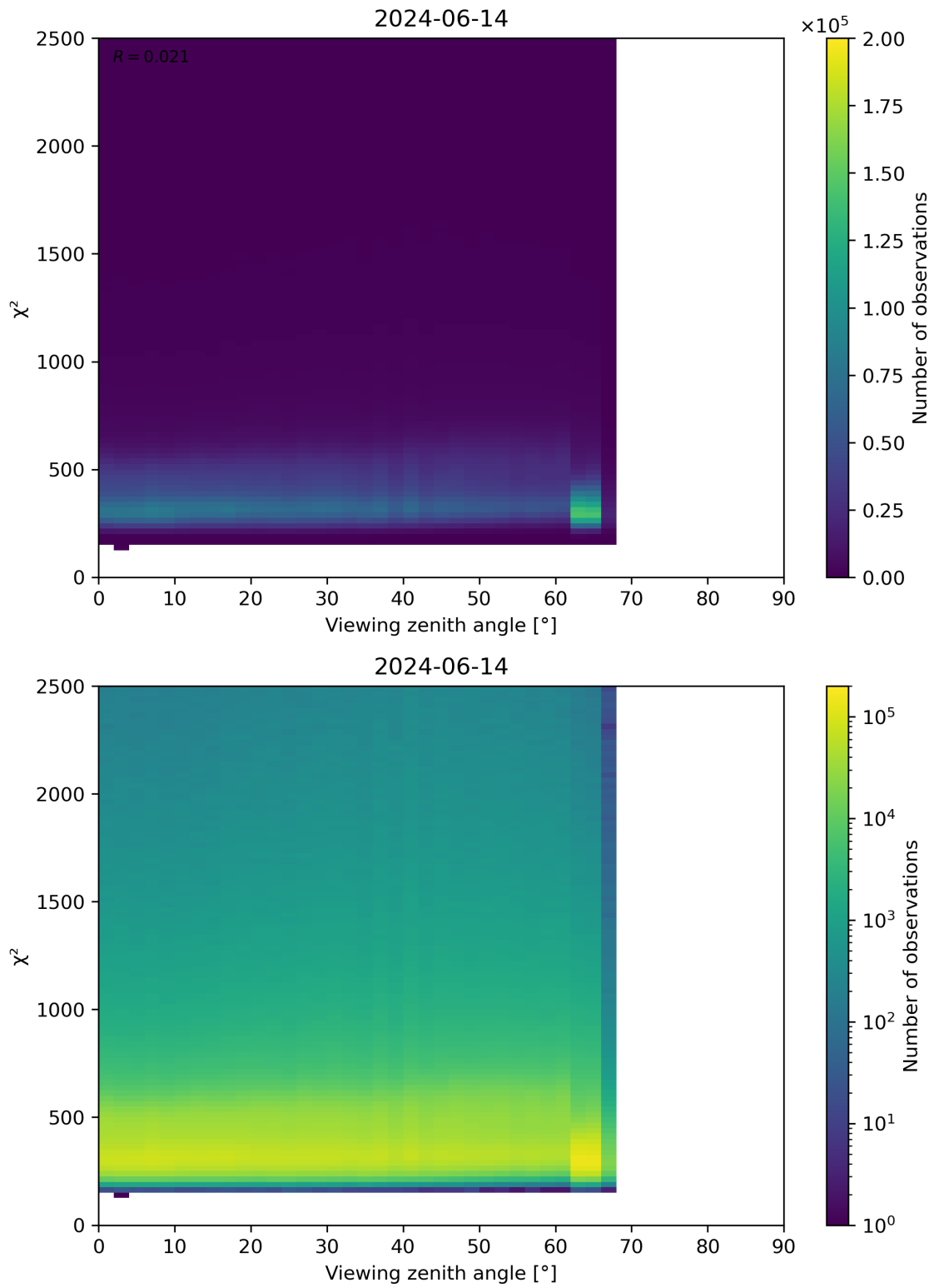
Figure 162: Scatter density plot of “Viewing zenith angle” against “ \chi^2 ” for 2024-06-13 to 2024-06-15.
