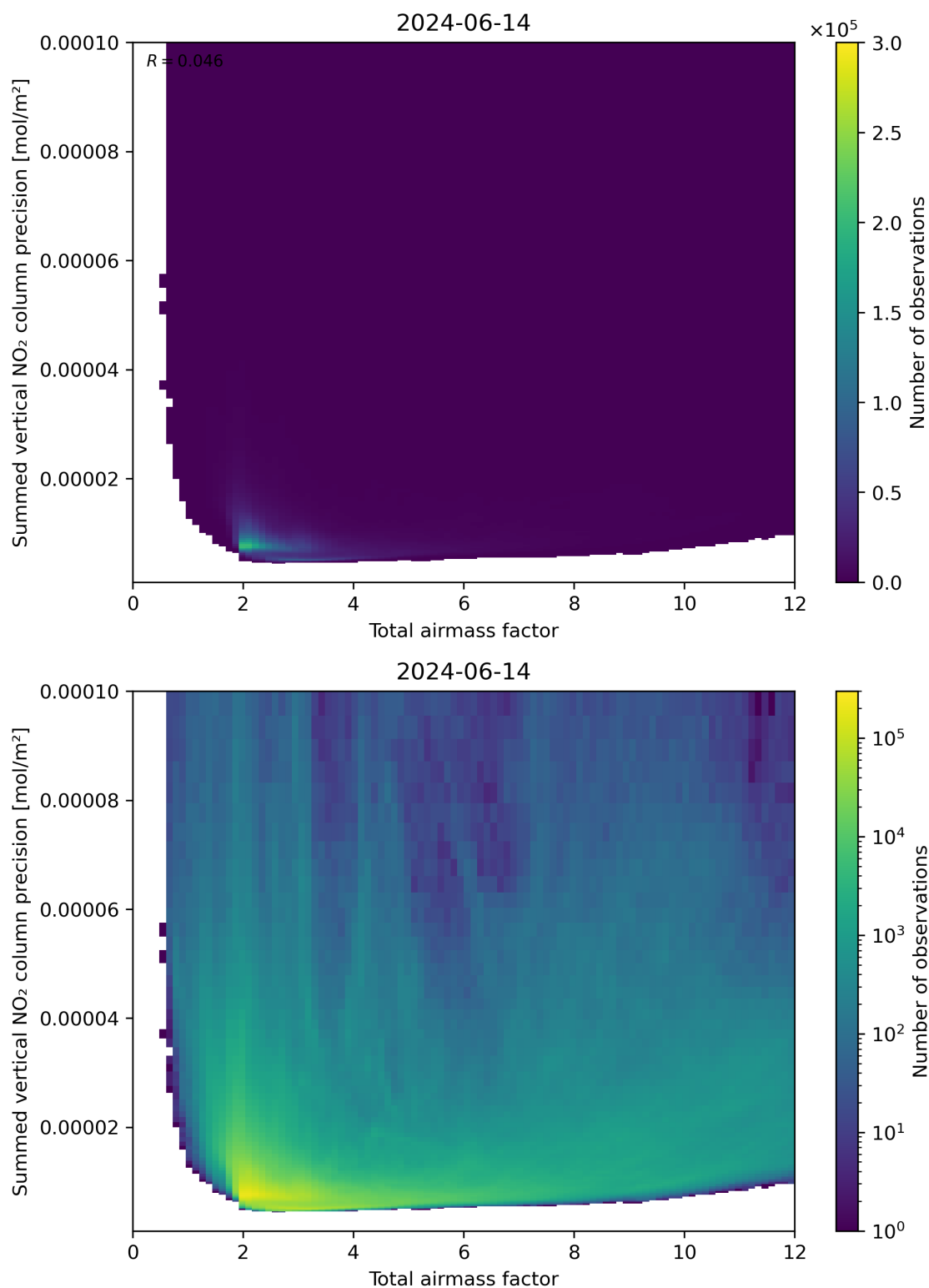
Figure 66: Scatter density plot of “Total airmass factor” against “Summed vertical NO 2 column precision” for 2024-06-13 to 2024-06-15.
