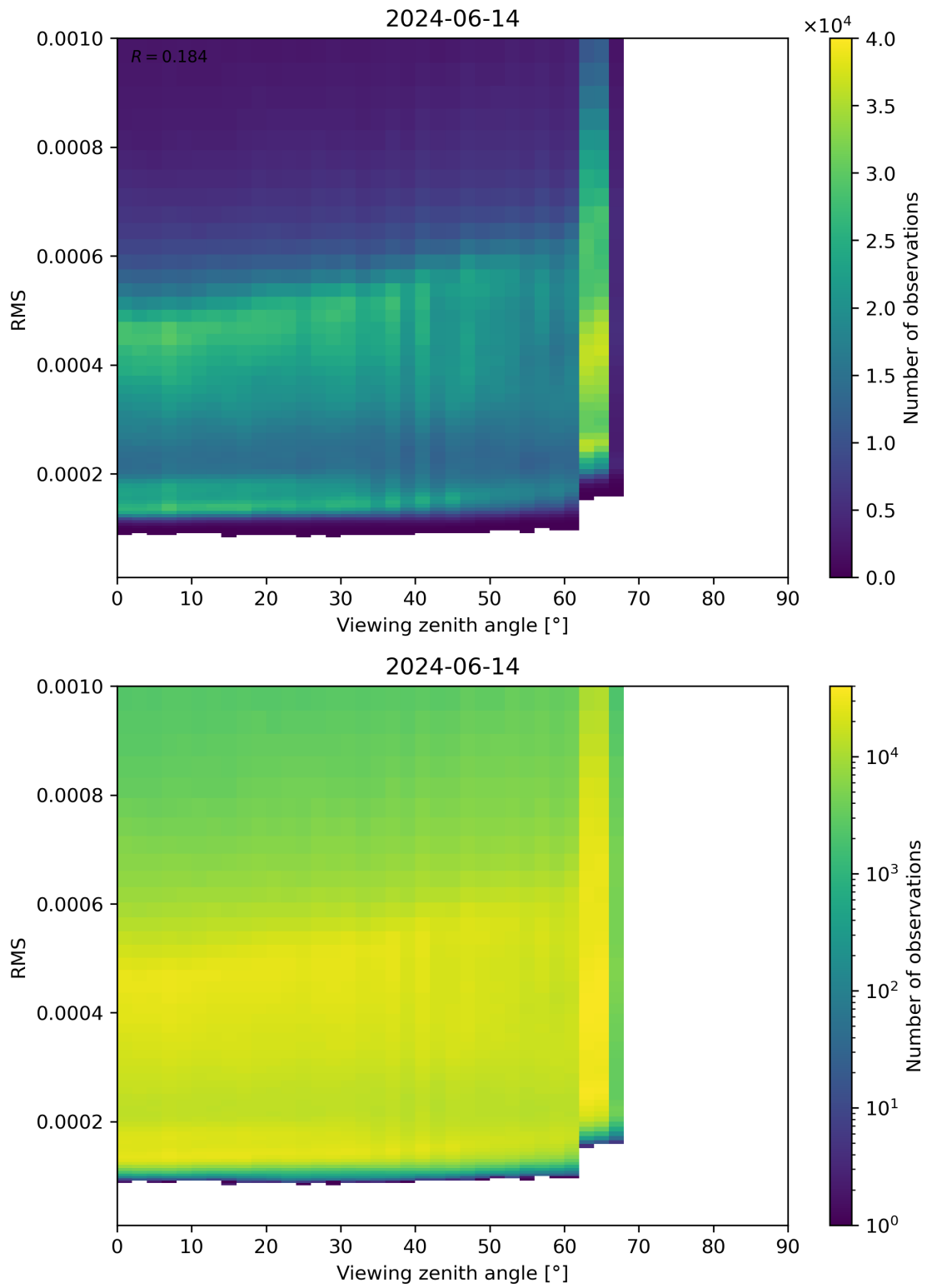
Figure 171: Scatter density plot of “Viewing zenith angle” against “RMS” for 2024-06-13 to 2024-06-15.
