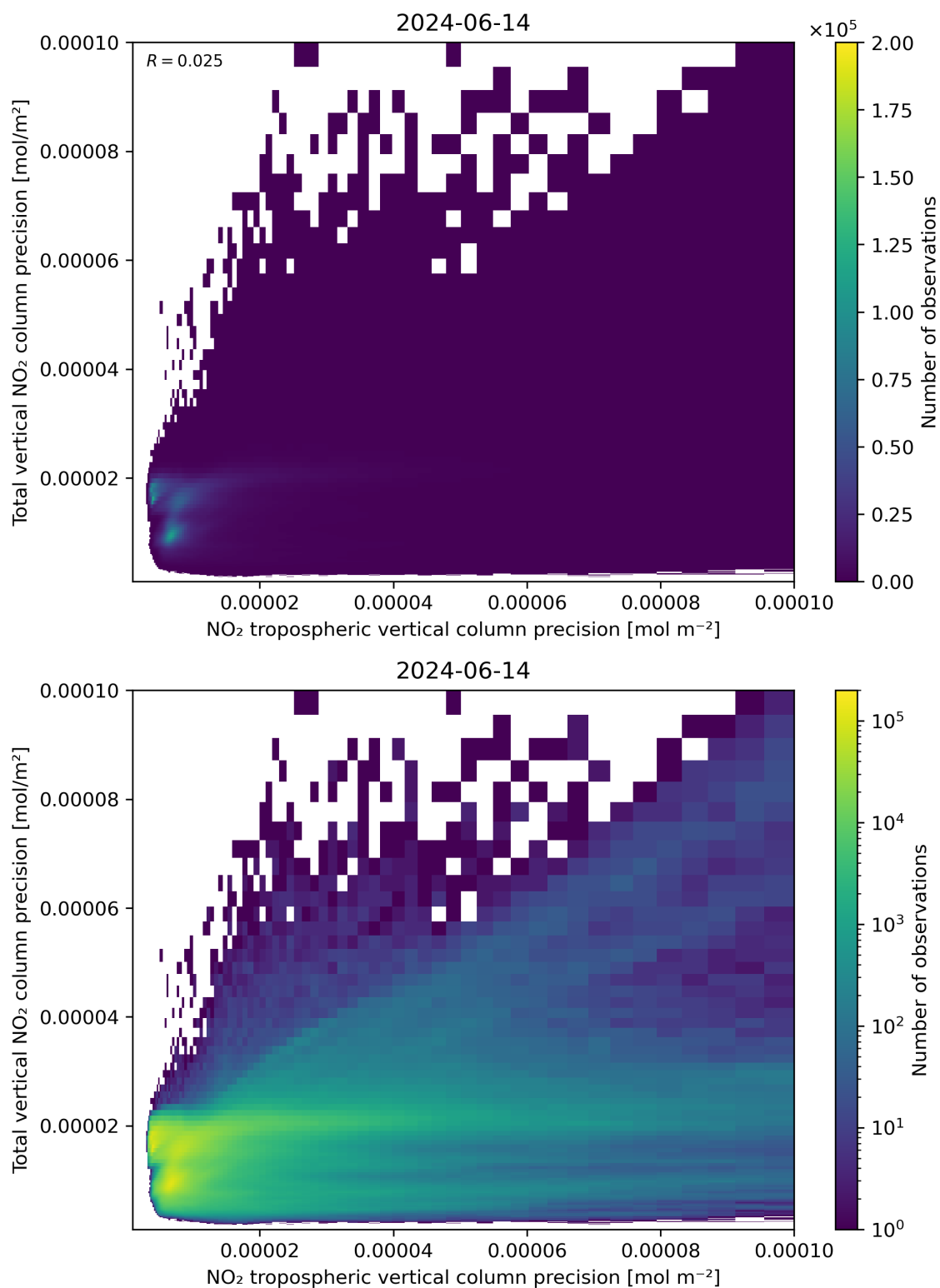
Figure 139: Scatter density plot of “NO 2 tropospheric vertical column precision” against “Total vertical NO 2 column precision” for 2024-06-13 to 2024-06-15.
