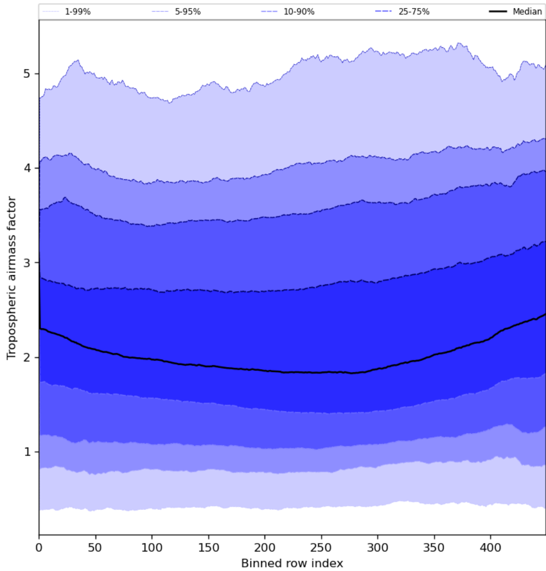
Figure 48: Along track statistics of “Tropospheric airmass factor” for 2024-06-13 to 2024-06-15
