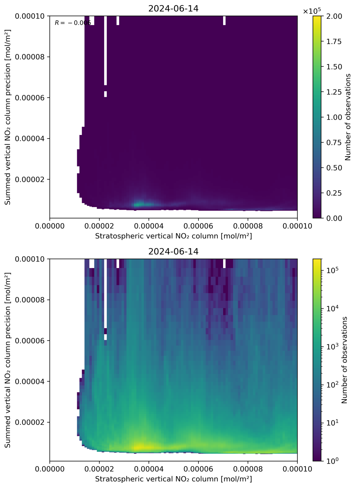
Figure 99: Scatter density plot of “Stratospheric vertical NO 2 column” against “Summed vertical NO 2 column precision” for 2024-06-13 to 2024-06-15.
