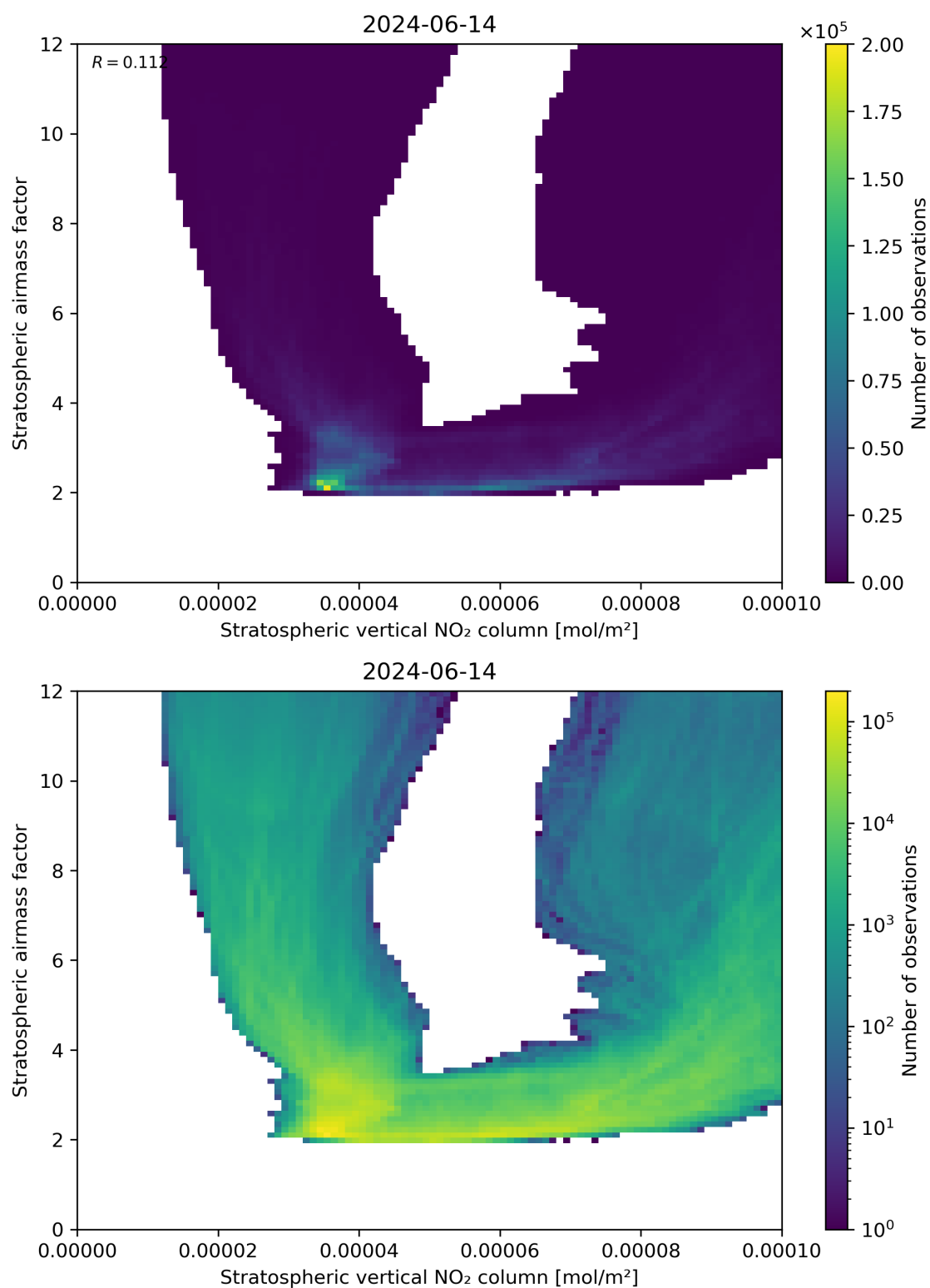
Figure 96: Scatter density plot of “Stratospheric vertical NO 2 column” against “Stratospheric airmass factor” for 2024-06-13 to 2024-06-15.
