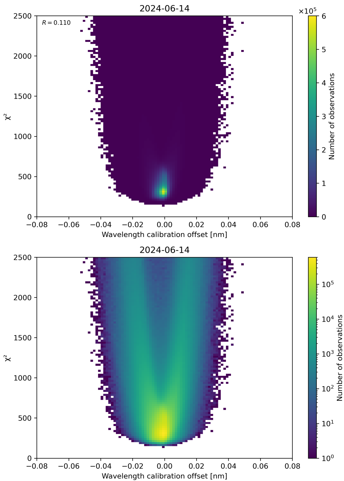
Figure 175: Scatter density plot of “Wavelength calibration offset” against “ \chi^2 ” for 2024-06-13 to 2024-06-15.
