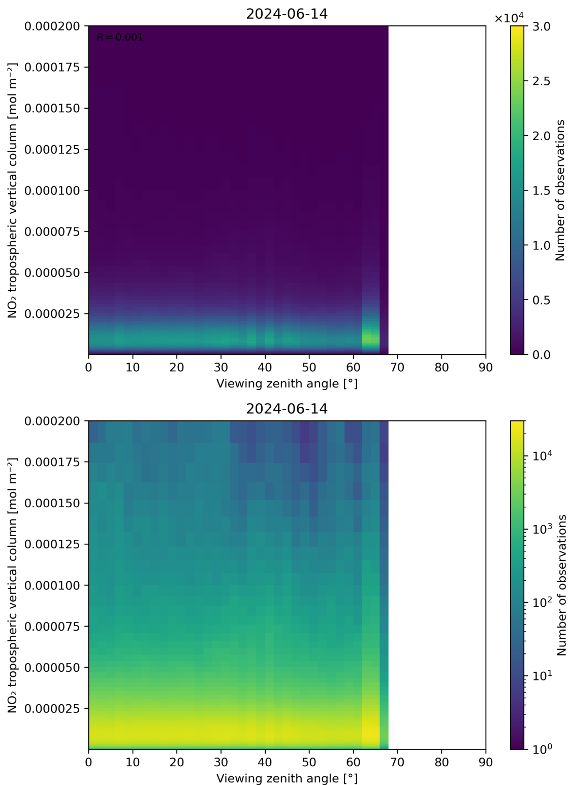
Figure 169: Scatter density plot of “Viewing zenith angle” against “NO 2 tropospheric vertical column” for 2024-06-13 to 2024-06-15.
