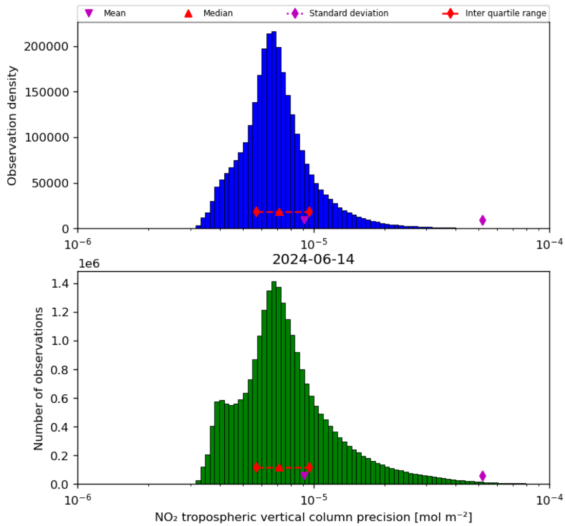
Figure 30: Histogram of “NO 2 tropospheric vertical column precision” for 2024-06-13 to 2024-06-15
