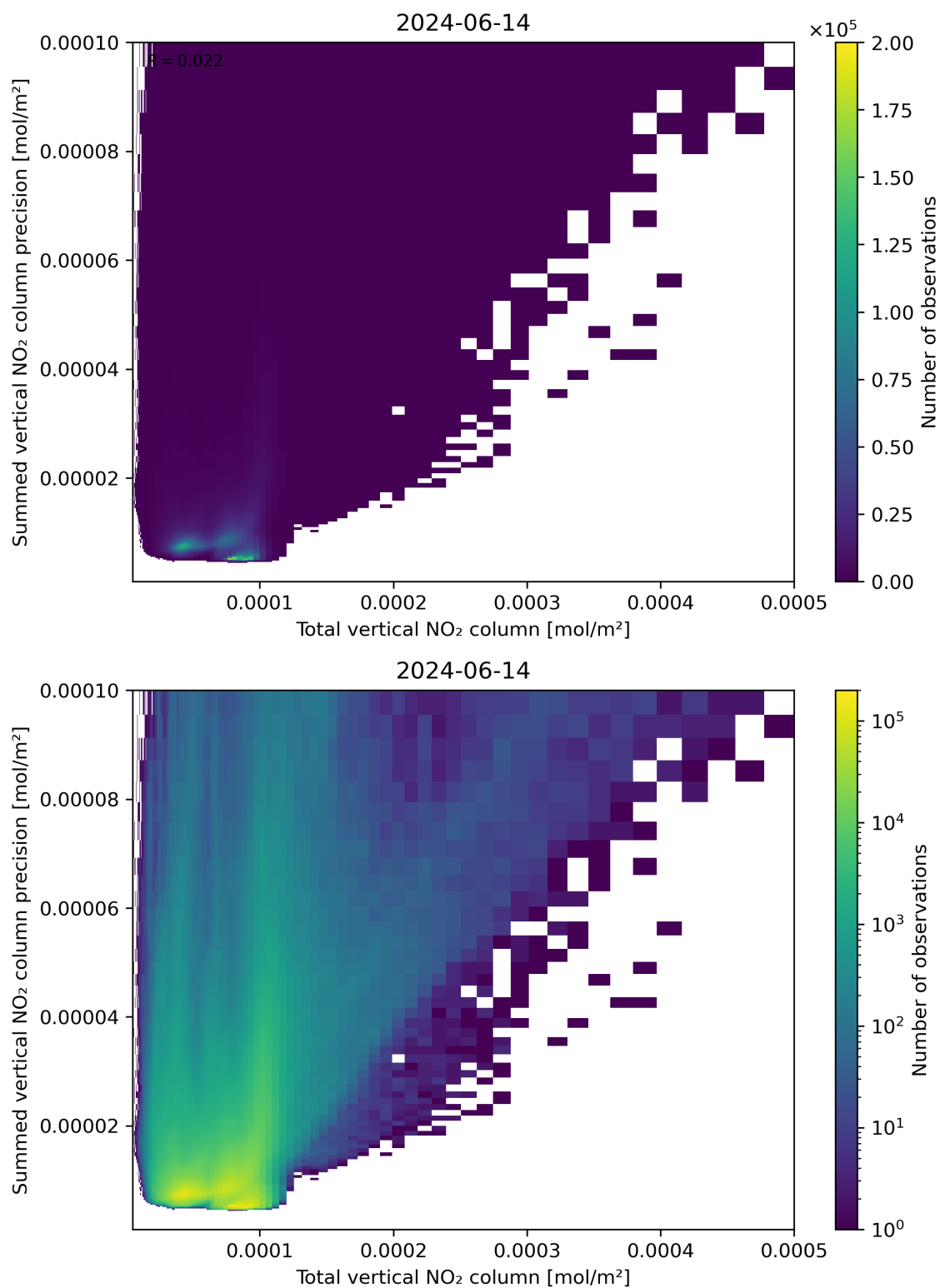
Figure 113: Scatter density plot of “Total vertical NO 2 column” against “Summed vertical NO 2 column precision” for 2024-06-13 to 2024-06-15.
