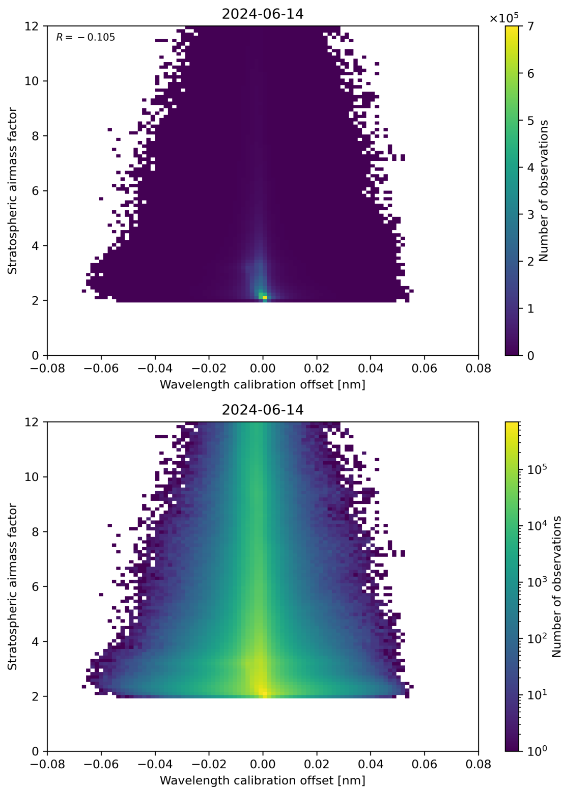
Figure 174: Scatter density plot of “Wavelength calibration offset” against “Stratospheric air mass factor” for 2024-06-13 to 2024-06-15.
