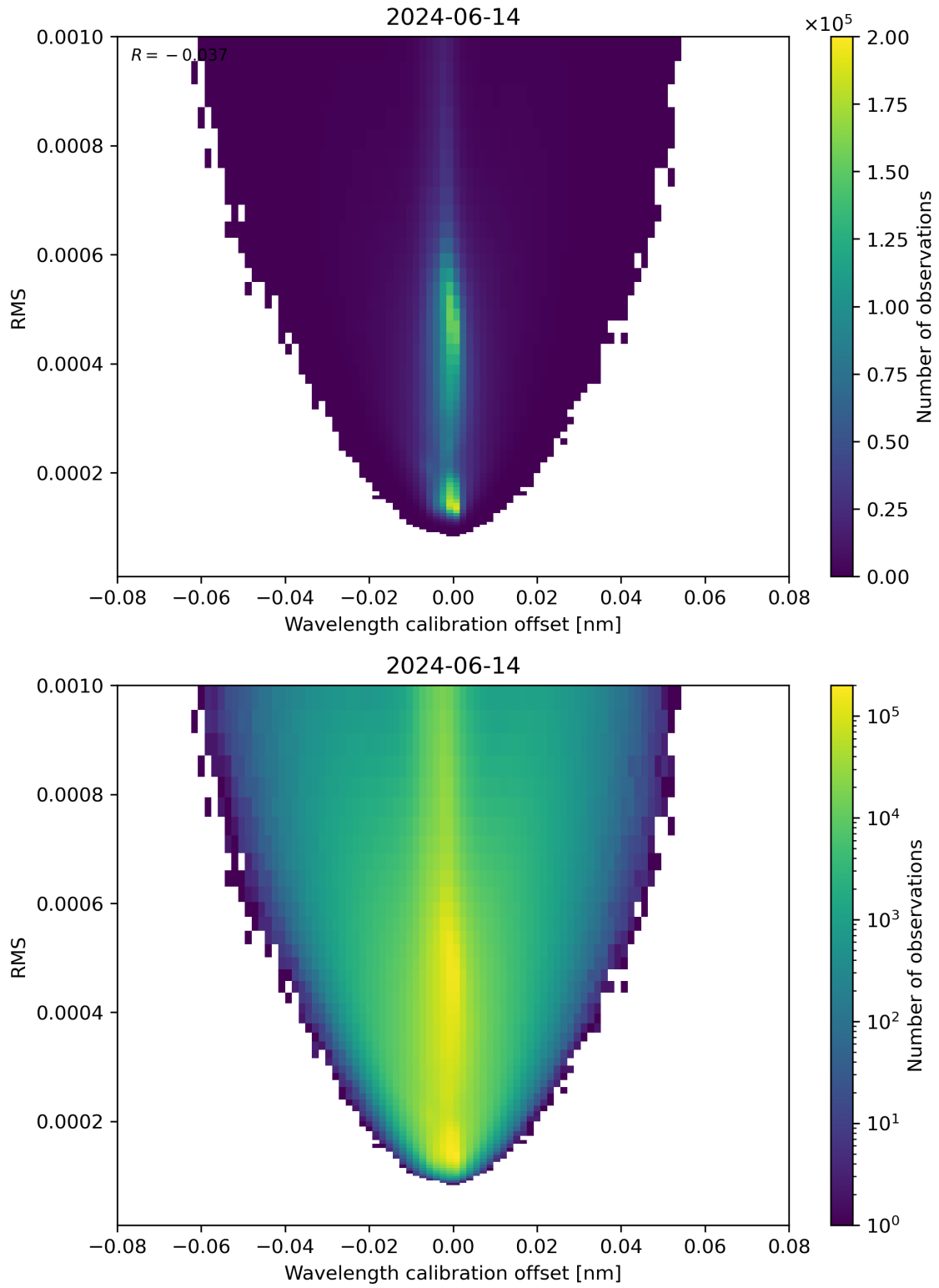
Figure 181: Scatter density plot of “Wavelength calibration offset” against “RMS” for 2024-06-13 to 2024-06-15.
