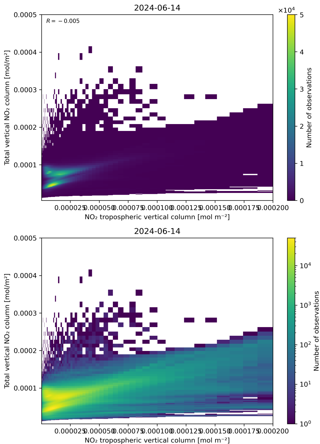
Figure 128: Scatter density plot of “NO 2 tropospheric vertical column” against “Total vertical NO 2 column” for 2024-06-13 to 2024-06-15.
