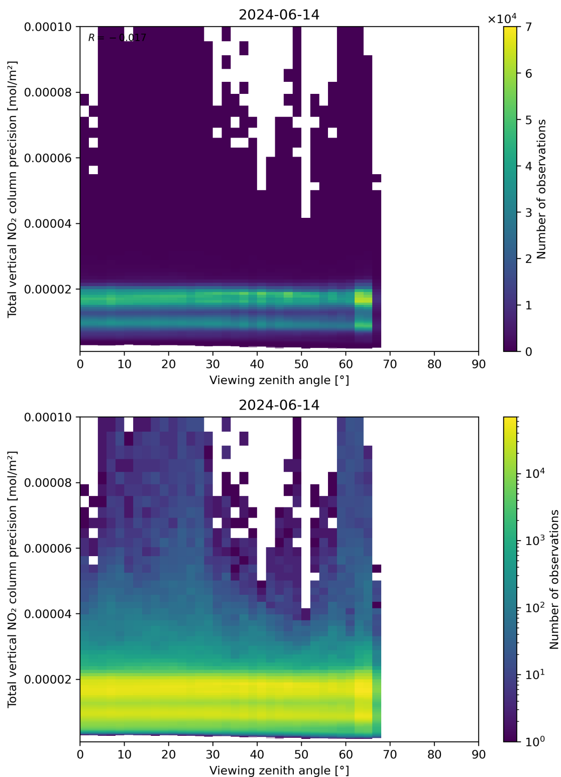
Figure 168: Scatter density plot of “Viewing zenith angle” against “Total vertical NO 2 column precision” for 2024-06-13 to 2024-06-15.
