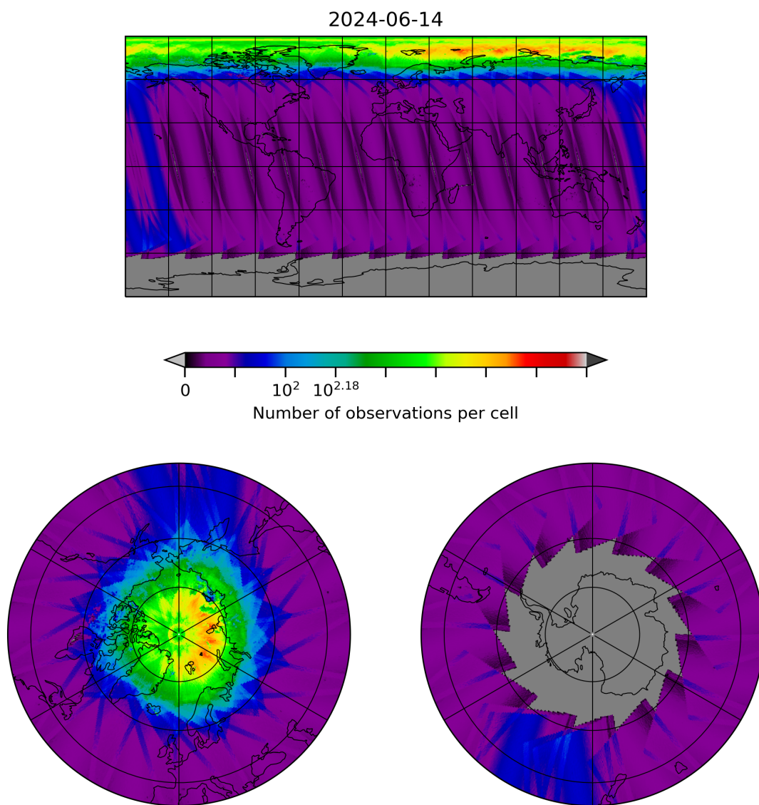
Figure 10: Map of the number of observations for 2024-06-13 to 2024-06-15
