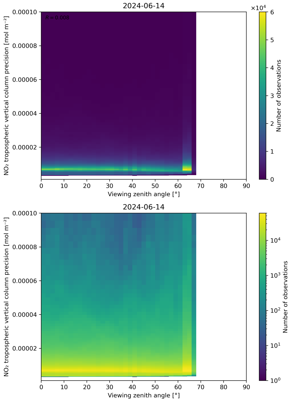
Figure 170: Scatter density plot of “Viewing zenith angle” against “NO 2 tropospheric vertical column precision” for 2024-06-13 to 2024-06-15.
