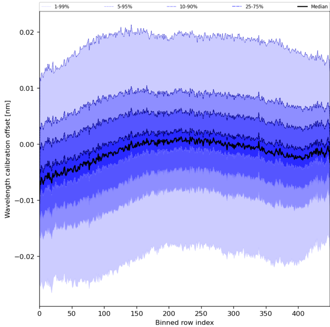
Figure 52: Along track statistics of “Wavelength calibration offset” for 2024-06-13 to 2024-06-15
