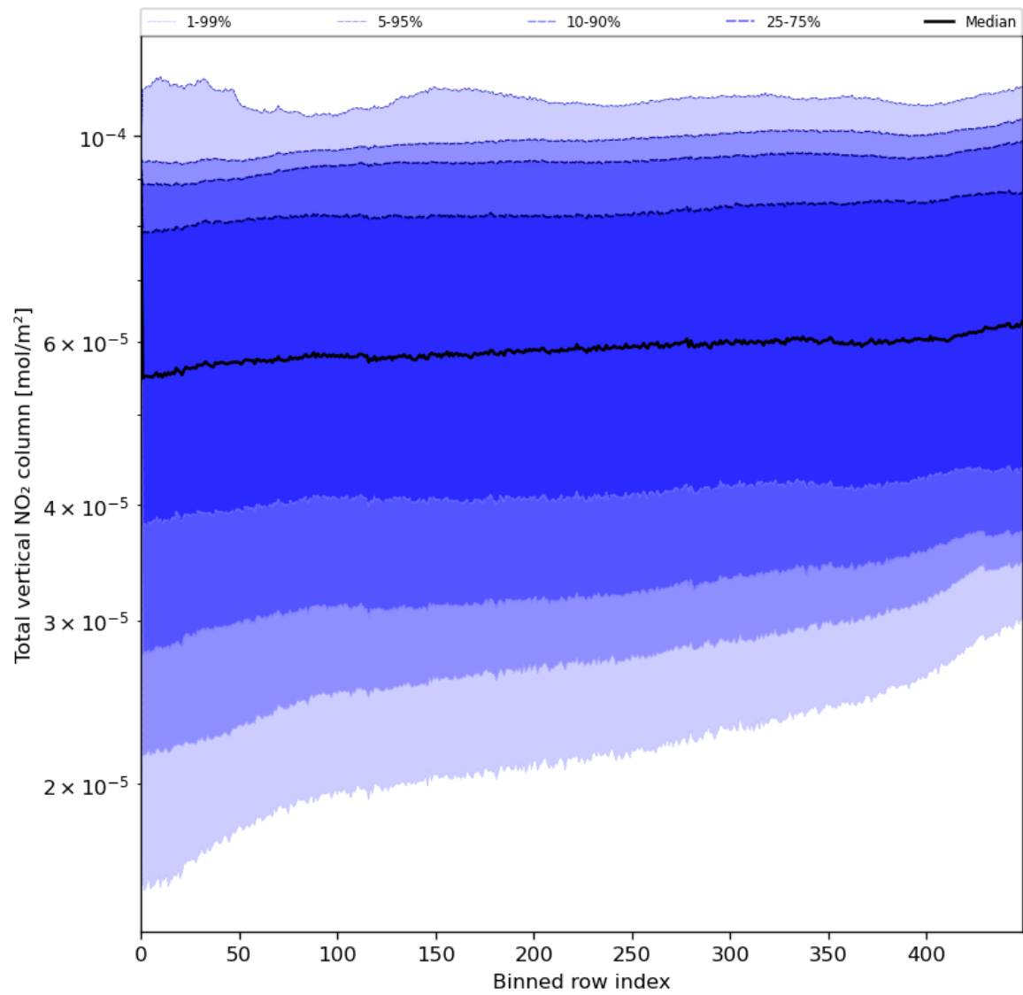
Figure 55: Along track statistics of “Total vertical NO 2 column” for 2024-06-13 to 2024-06-15
