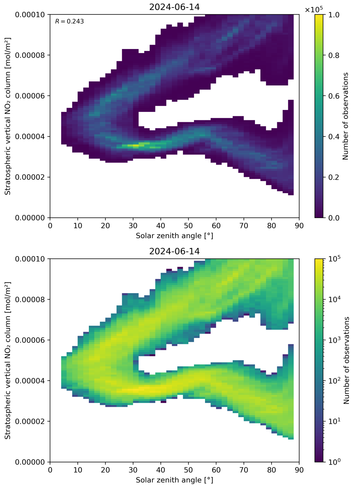
Figure 150: Scatter density plot of “Solar zenith angle” against “Stratospheric vertical NO 2 column” for 2024-06-13 to 2024-06-15.
