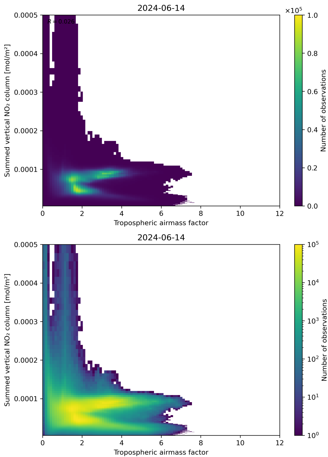
Figure 75: Scatter density plot of “Tropospheric airmass factor” against “Summed vertical NO 2 column” for 2024-06-13 to 2024-06-15.
