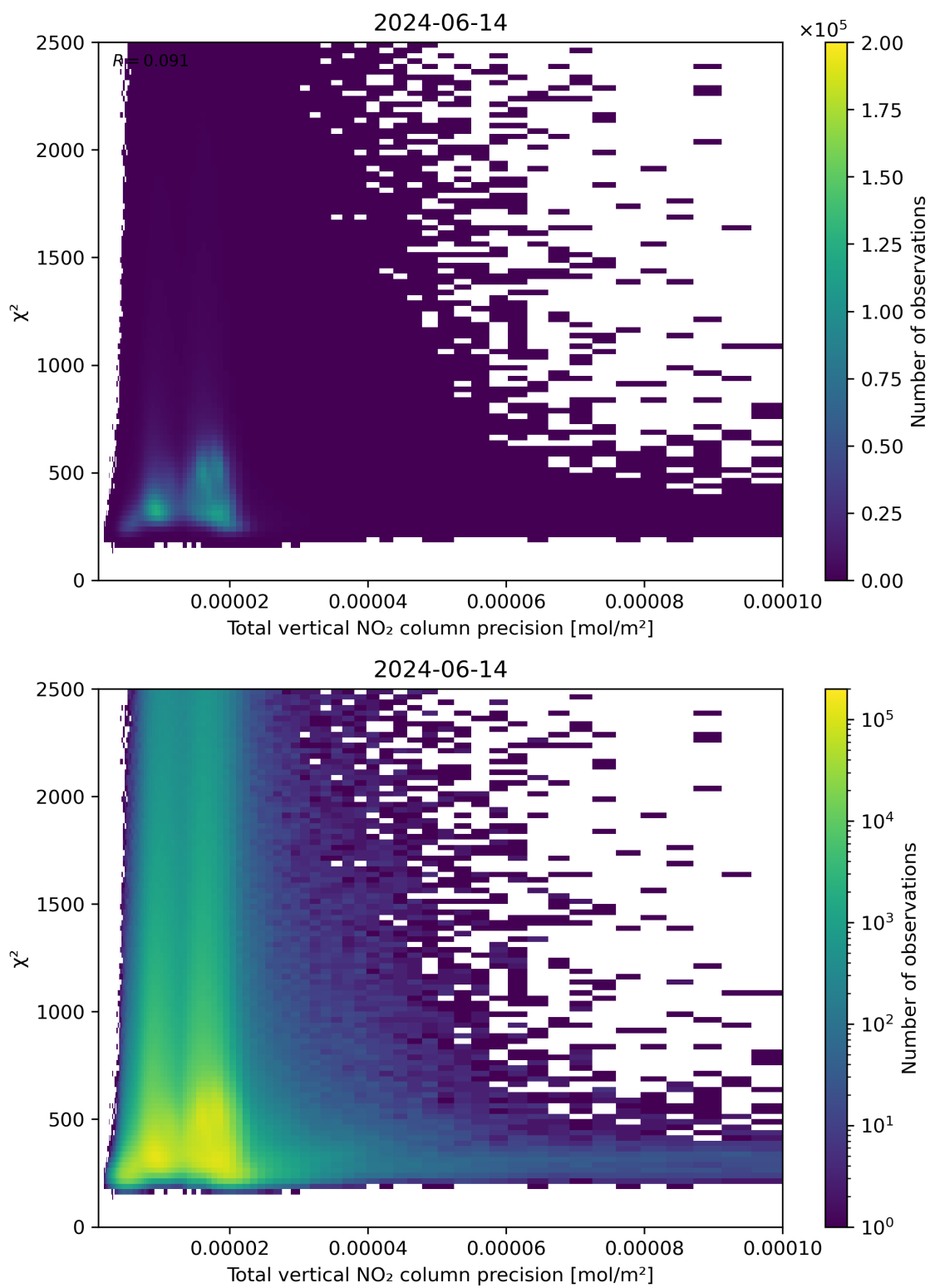
Figure 116: Scatter density plot of “Total vertical NO 2 column precision” against “ \chi^2 ” for 2024-06-13 to 2024-06-15.
