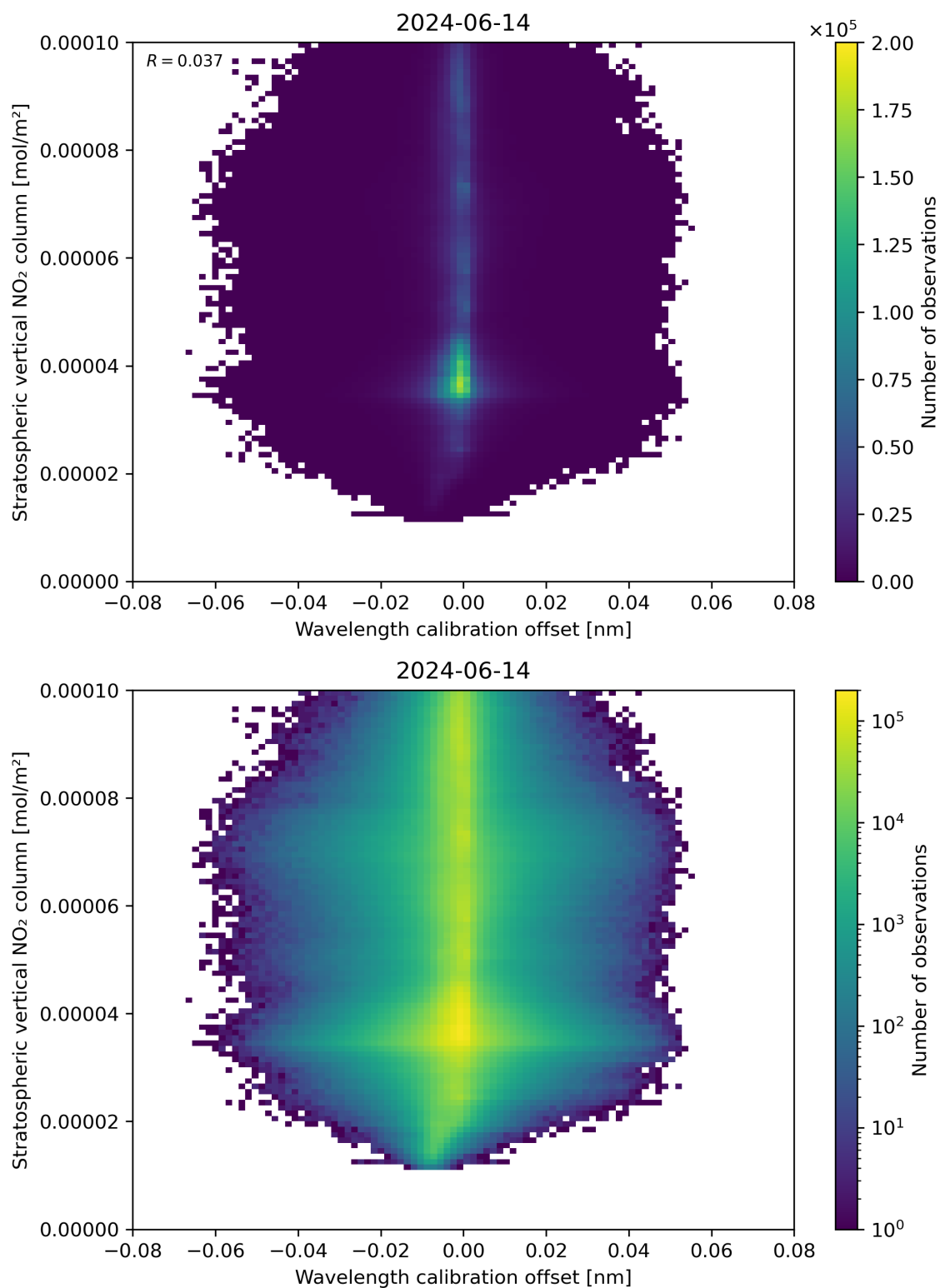
Figure 176: Scatter density plot of “Wavelength calibration offset” against “Stratospheric vertical NO 2 column” for 2024-06-13 to 2024-06-15.
