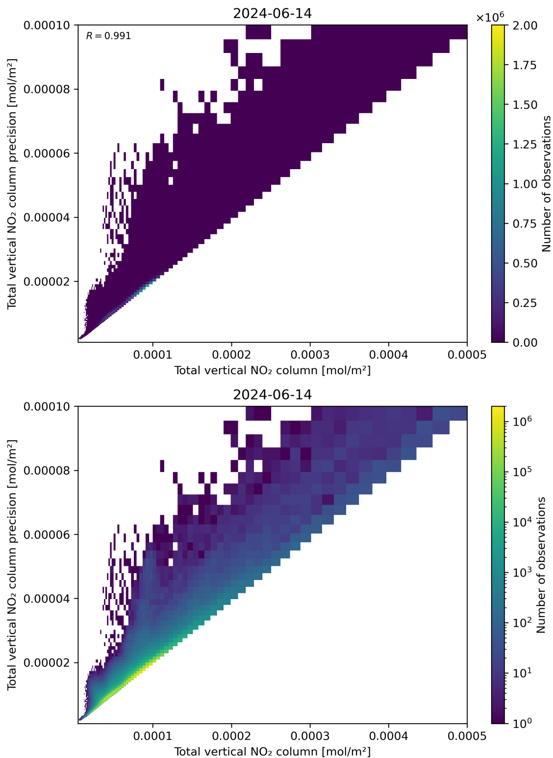
Figure 114: Scatter density plot of “Total vertical NO 2 column” against “Total vertical NO 2 column precision” for 2024-06-13 to 2024-06-15.
