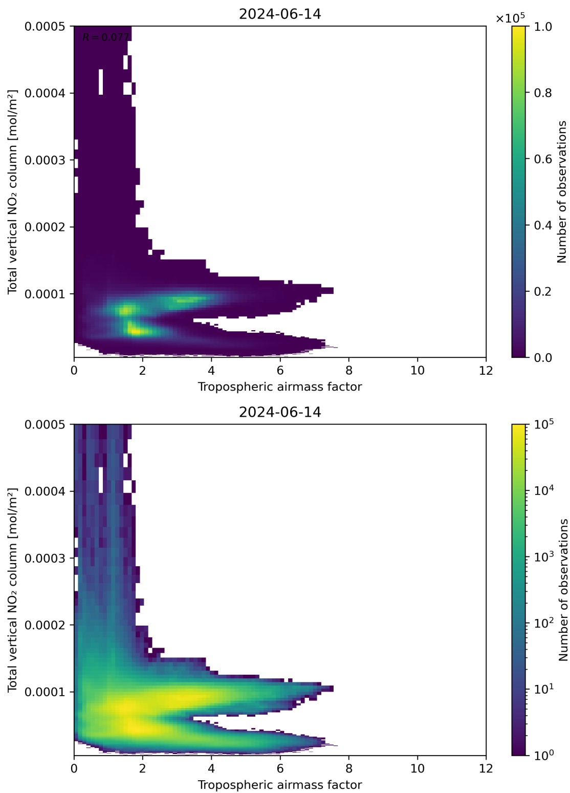
Figure 77: Scatter density plot of “Tropospheric airmass factor” against “Total vertical NO 2 column” for 2024-06-13 to 2024-06-15.
