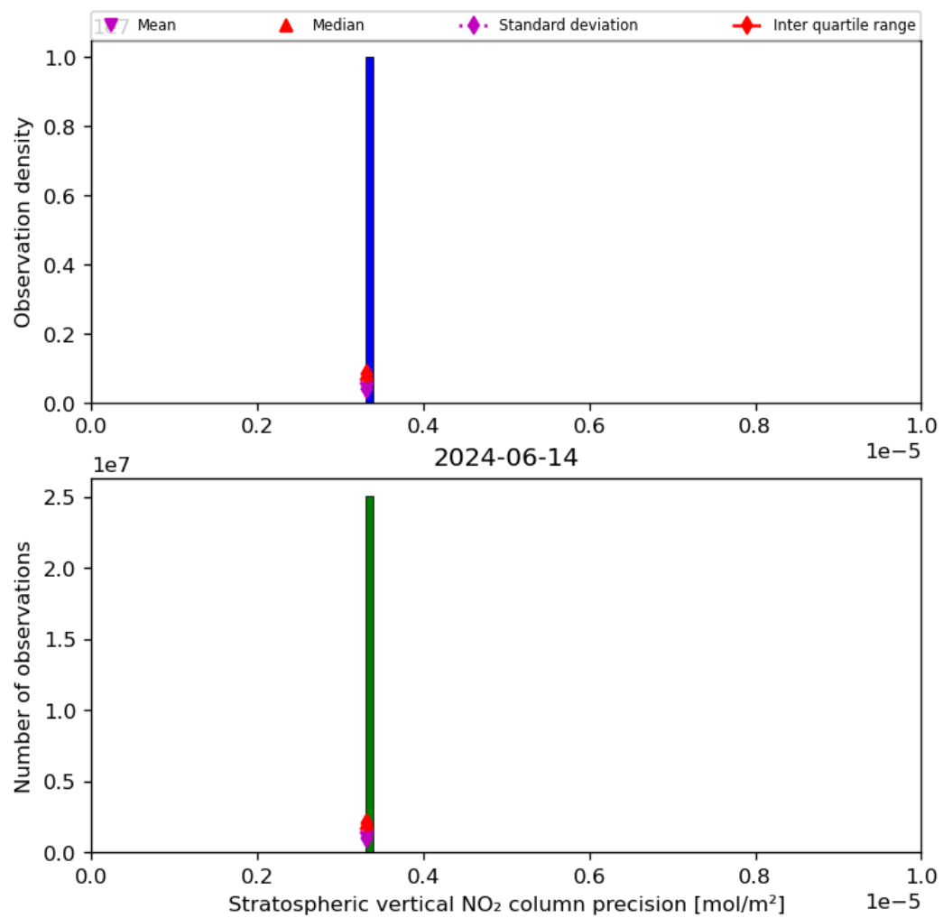
Figure 37: Histogram of “Stratospheric vertical NO 2 column precision” for 2024-06-13 to 2024-06-15
