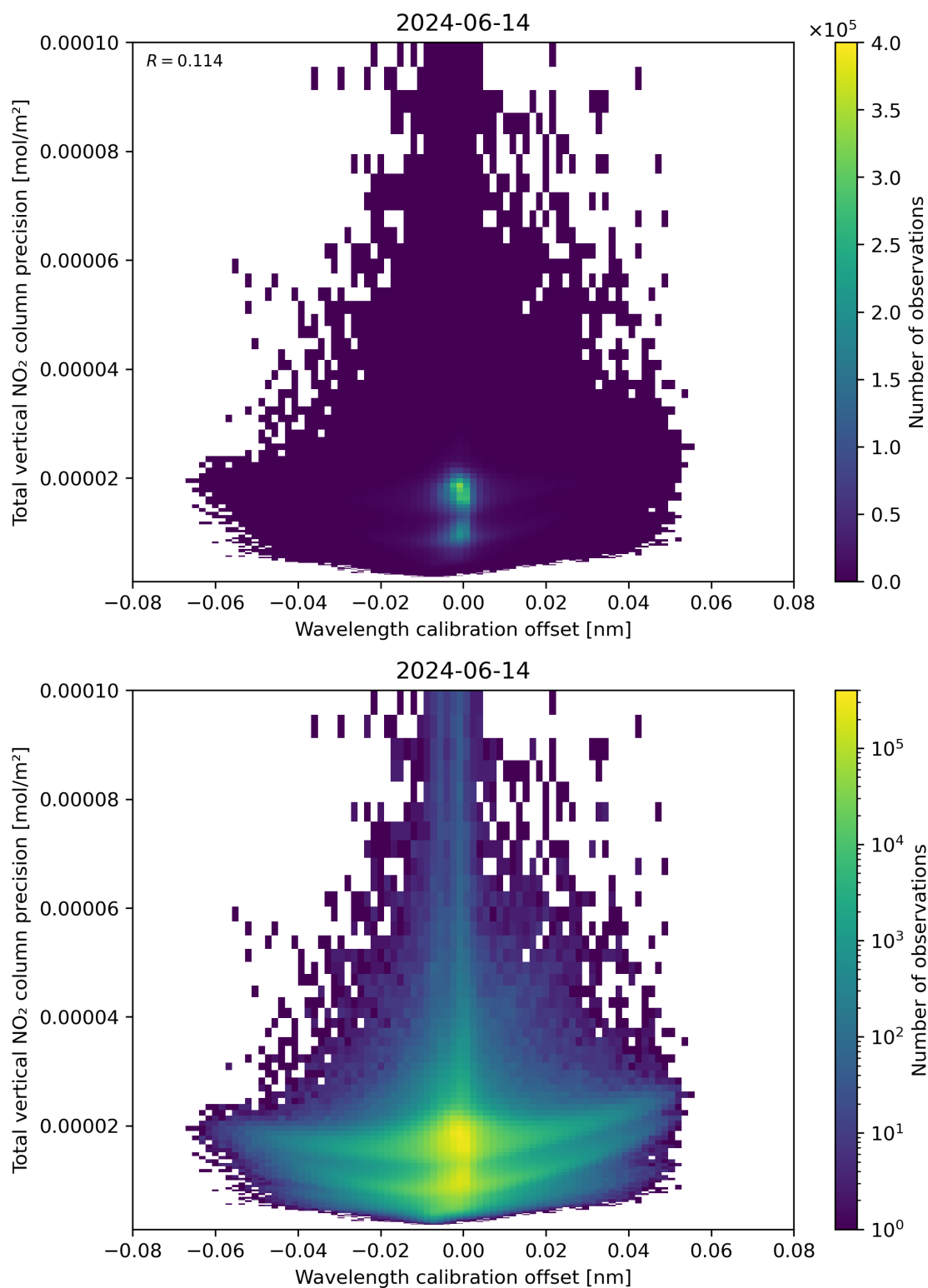
Figure 180: Scatter density plot of “Wavelength calibration offset” against “Total vertical NO 2 column precision” for 2024-06-13 to 2024-06-15.
