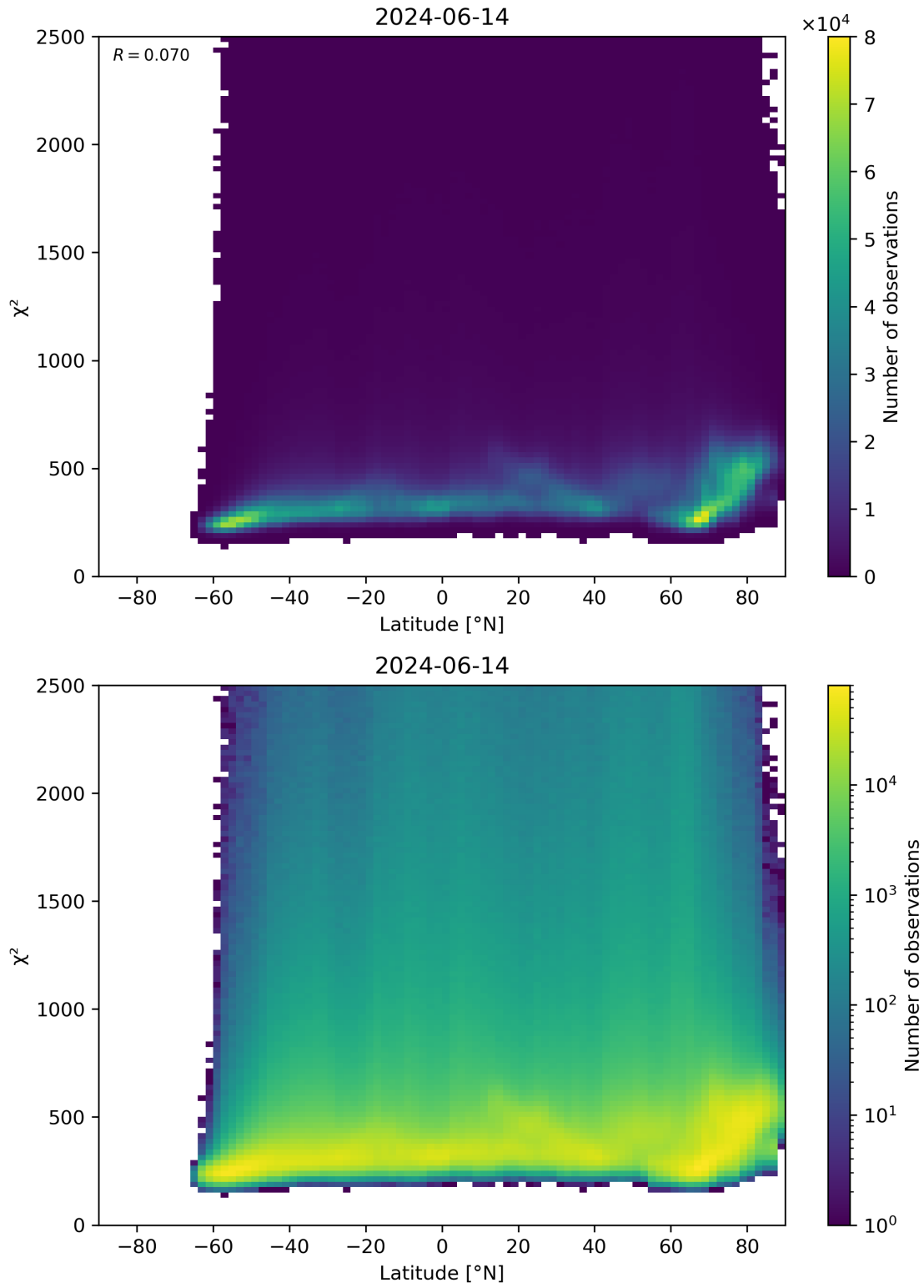
Figure 86: Scatter density plot of “Latitude” against “ \chi^2 ” for 2024-06-13 to 2024-06-15.
