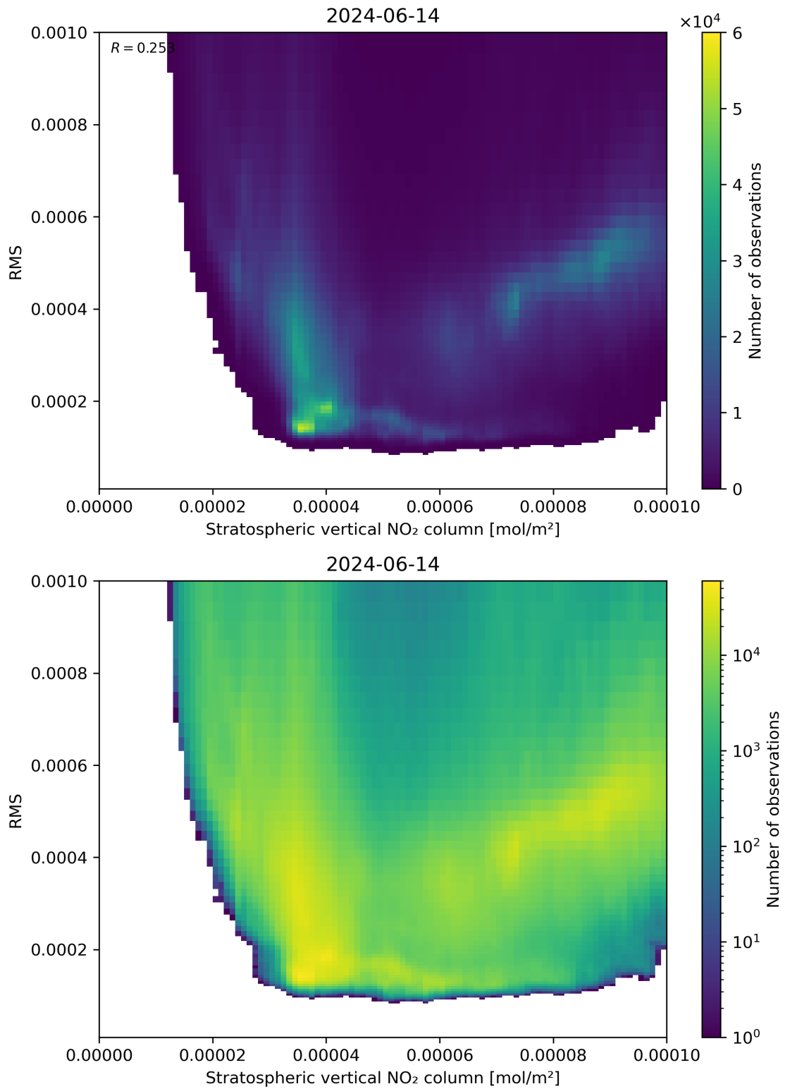
Figure 102: Scatter density plot of “Stratospheric vertical NO 2 column” against “RMS” for 2024-06-13 to 2024-06-15.
