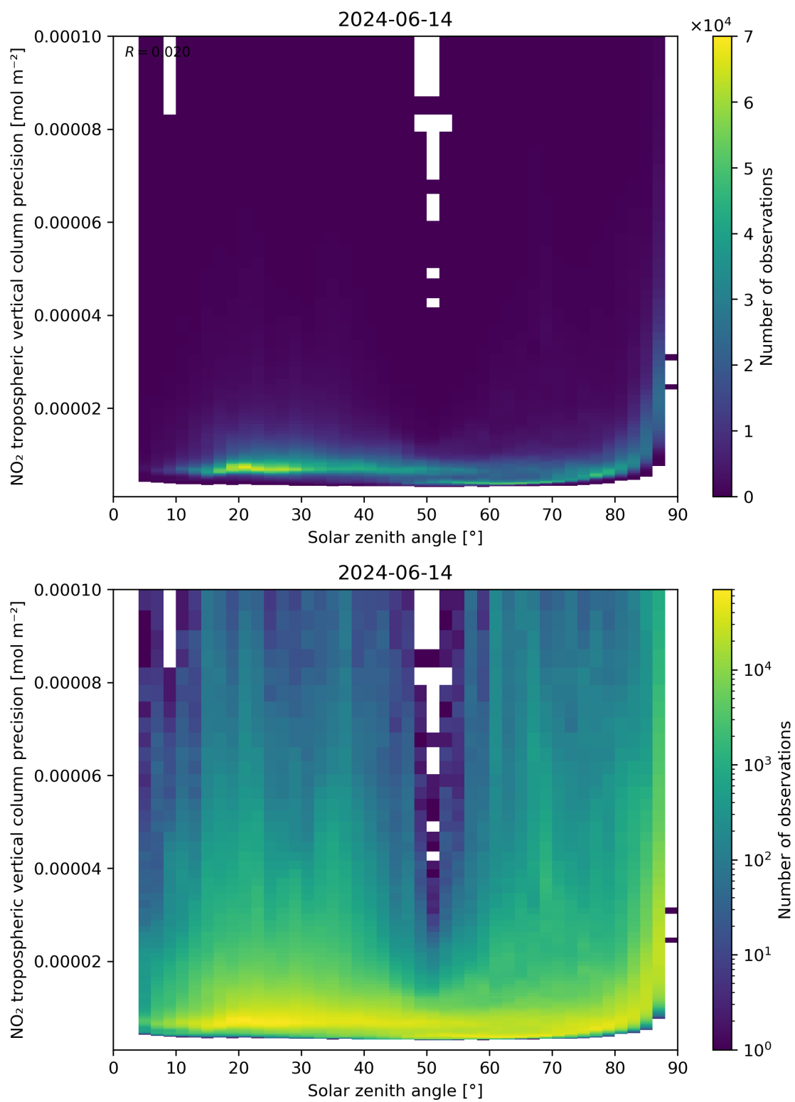
Figure 156: Scatter density plot of “Solar zenith angle” against “NO 2 tropospheric vertical column precision” for 2024-06-13 to 2024-06-15.
