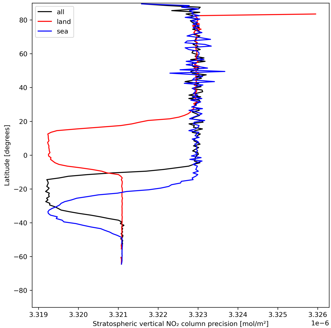
Figure 20: Zonal average of “Stratospheric vertical NO 2 column precision” for 2024-06-13 to 2024-06-15.
