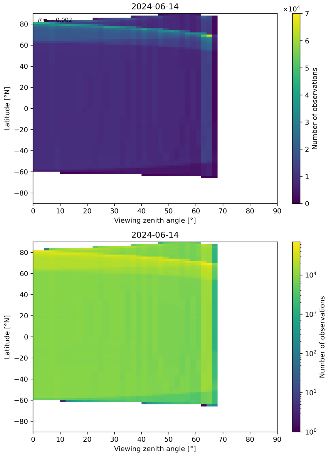
Figure 163: Scatter density plot of “Viewing zenith angle” against “Latitude” for 2024-06-13 to 2024-06-15.
