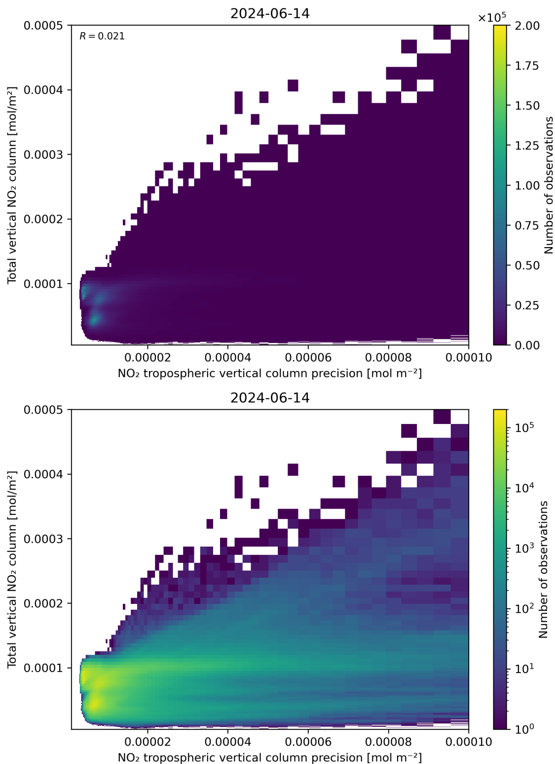
Figure 138: Scatter density plot of “NO 2 tropospheric vertical column precision” against “Total vertical NO 2 column” for 2024-06-13 to 2024-06-15.
