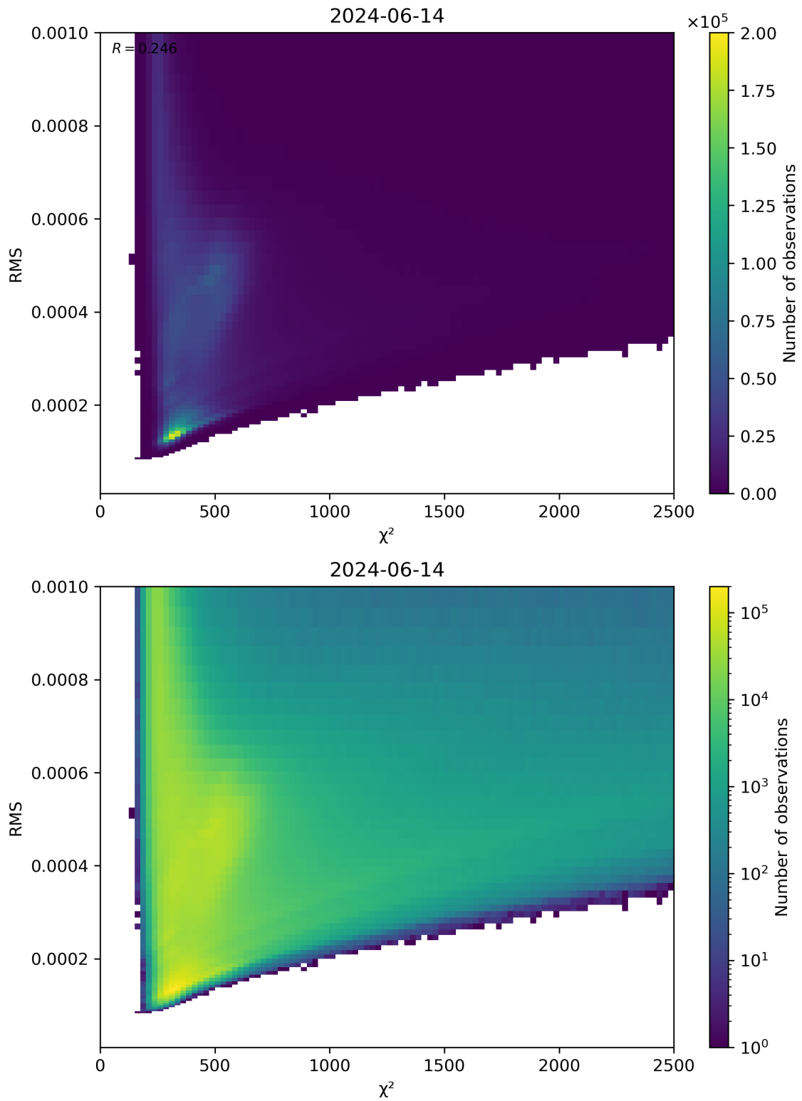
Figure 82: Scatter density plot of “ \chi^2 ” against “RMS” for 2024-06-13 to 2024-06-15.
