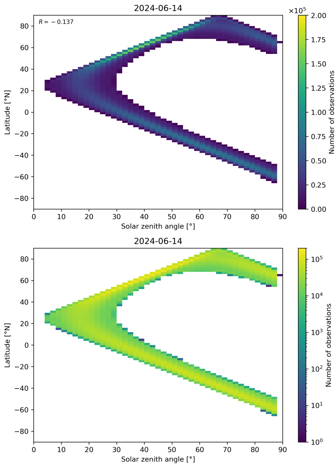
Figure 149: Scatter density plot of “Solar zenith angle” against “Latitude” for 2024-06-13 to 2024-06-15.
