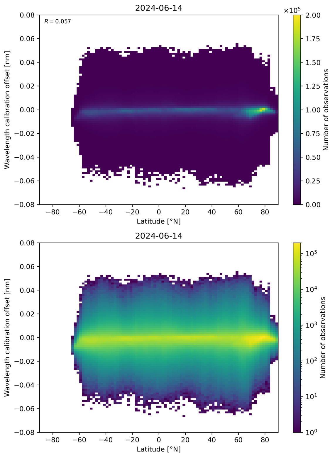
Figure 95: Scatter density plot of “Latitude” against “Wavelength calibration offset” for 2024-06-13 to 2024-06-15.
