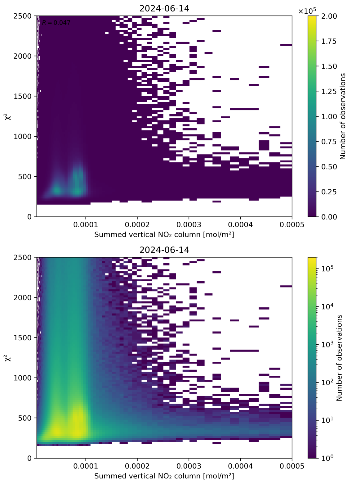
Figure 104: Scatter density plot of “Summed vertical NO 2 column” against “ \chi^2 ” for 2024-06-13 to 2024-06-15.
