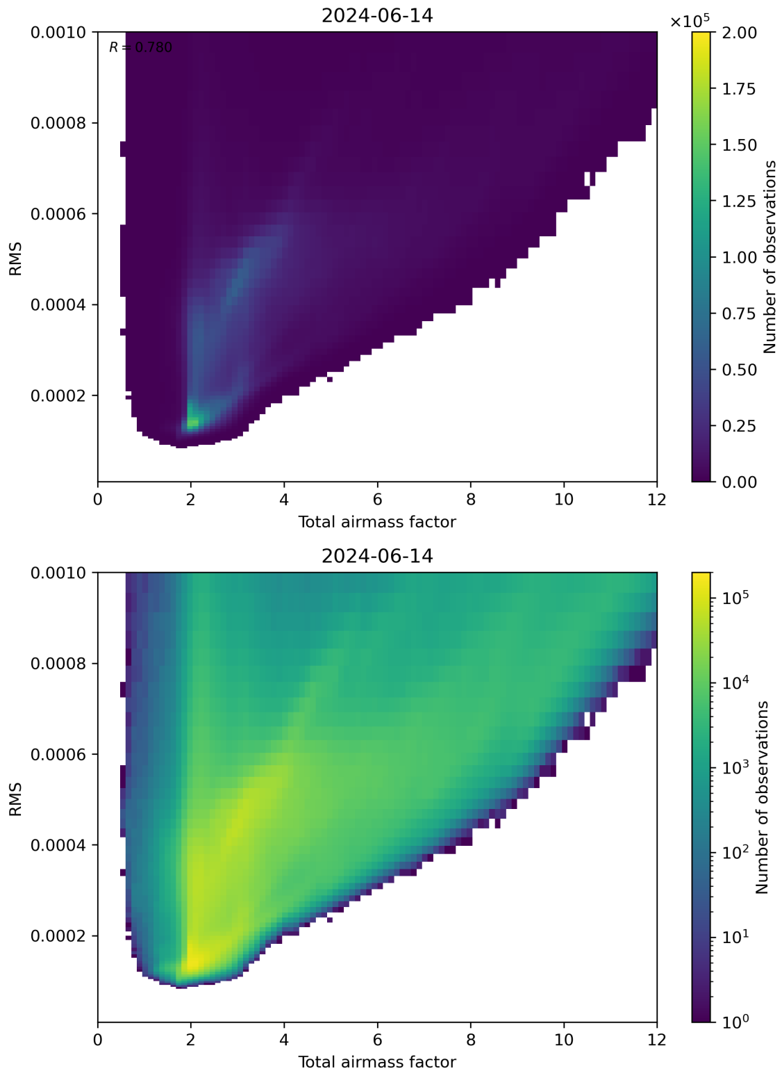
Figure 69: Scatter density plot of “Total airmass factor” against “RMS” for 2024-06-13 to 2024-06-15.
