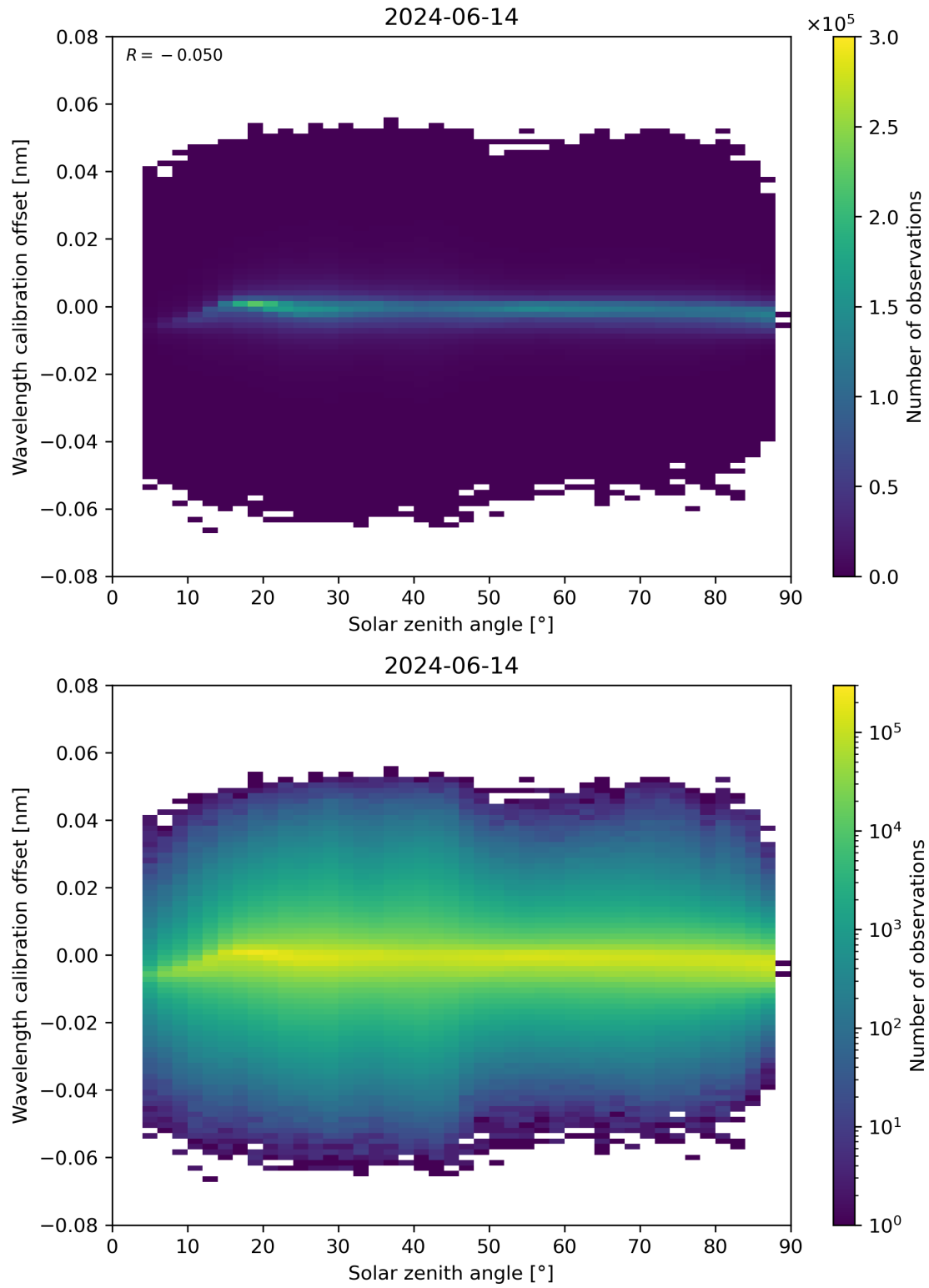
Figure 158: Scatter density plot of “Solar zenith angle” against “Wavelength calibration offset” for 2024-06-13 to 2024-06-15.
