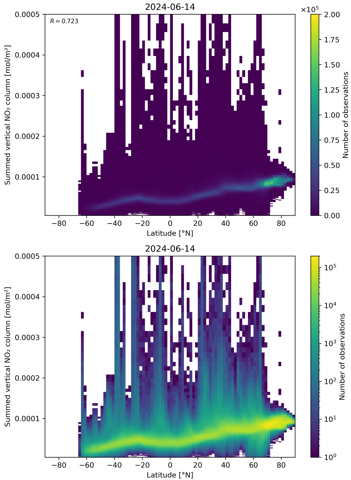
Figure 88: Scatter density plot of “Latitude” against “Summed vertical NO 2 column” for 2024-06-13 to 2024-06-15.
