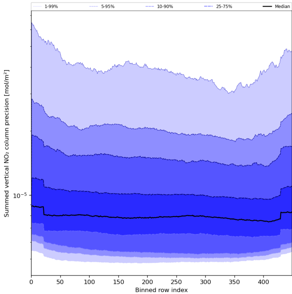
Figure 58: Along track statistics of “Summed vertical NO 2 column precision” for 2024-06-13 to 2024-06-15
