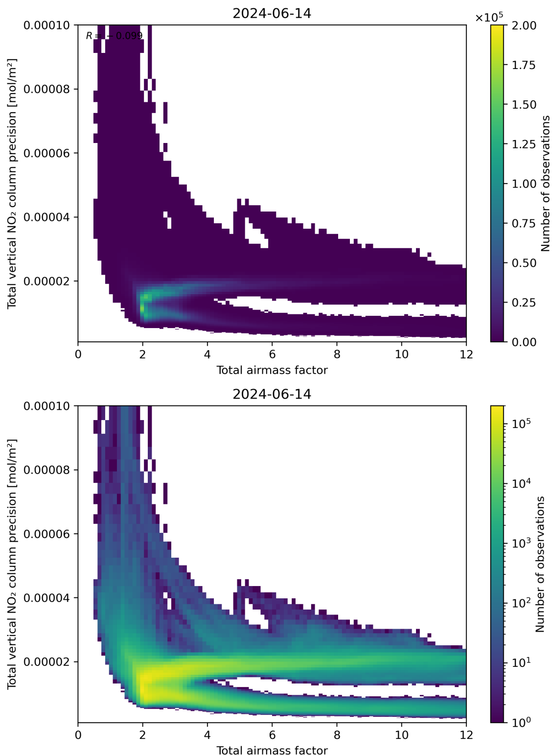
Figure 68: Scatter density plot of “Total airmass factor” against “Total vertical NO 2 column precision” for 2024-06-13 to 2024-06-15.
