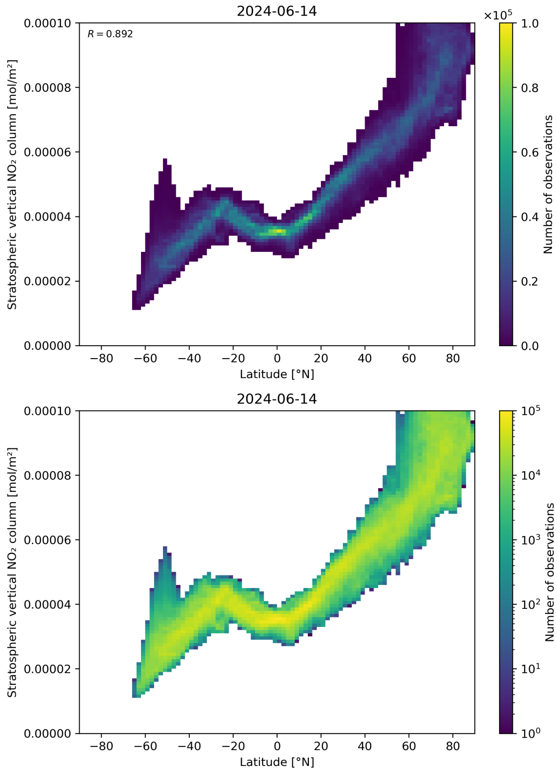
Figure 87: Scatter density plot of “Latitude” against “Stratospheric vertical \text{NO}_2 column” for 2024-06-13 to 2024-06-15.
