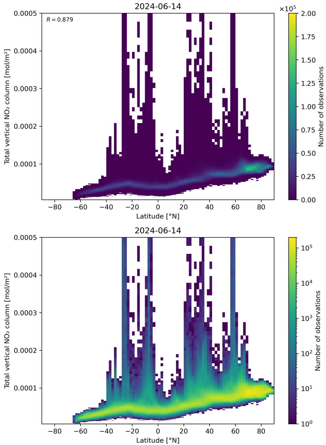
Figure 90: Scatter density plot of “Latitude” against “Total vertical NO 2 column” for 2024-06-13 to 2024-06-15.
