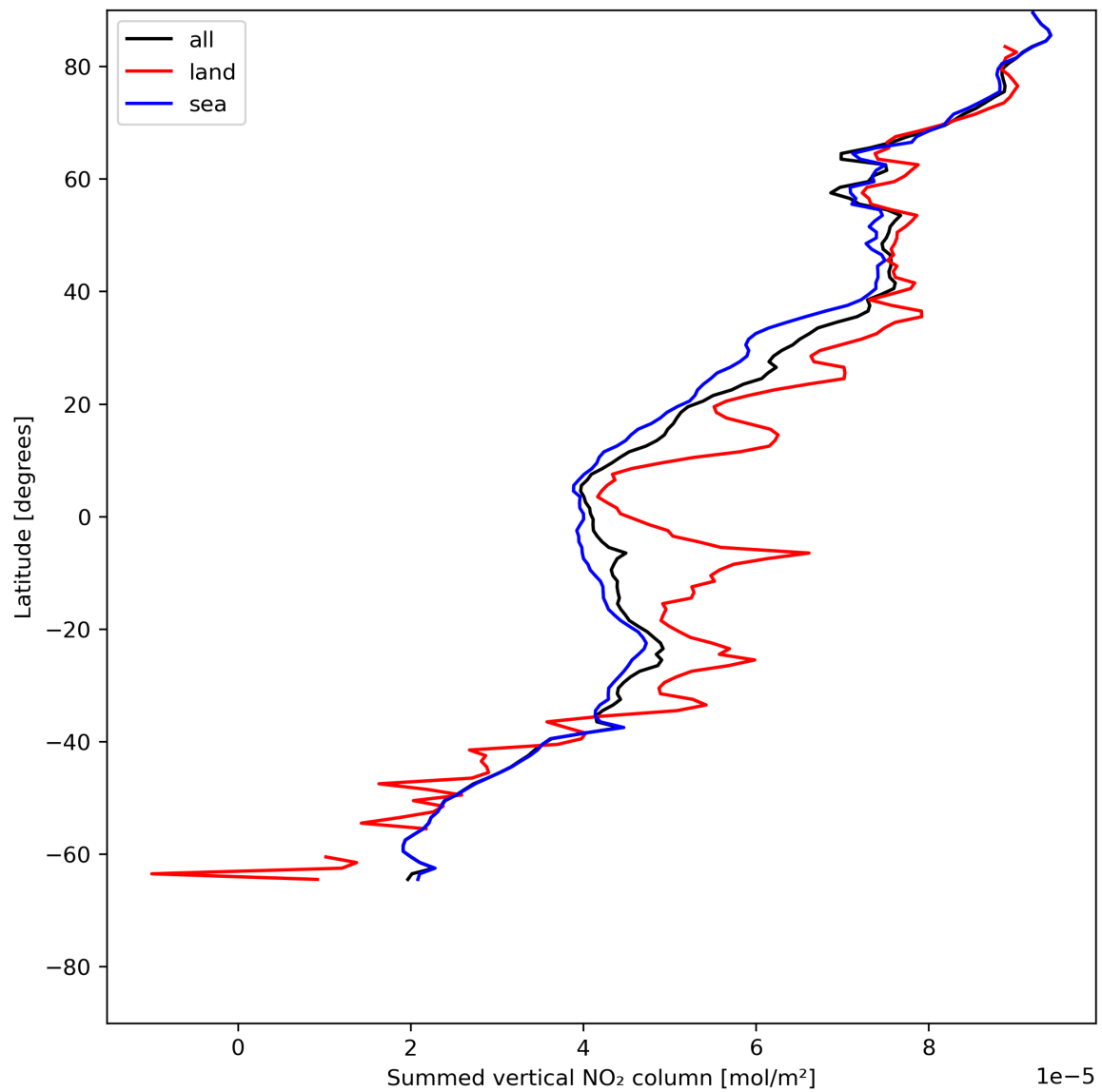
Figure 23: Zonal average of “Summed vertical NO 2 column” for 2024-06-13 to 2024-06-15.
