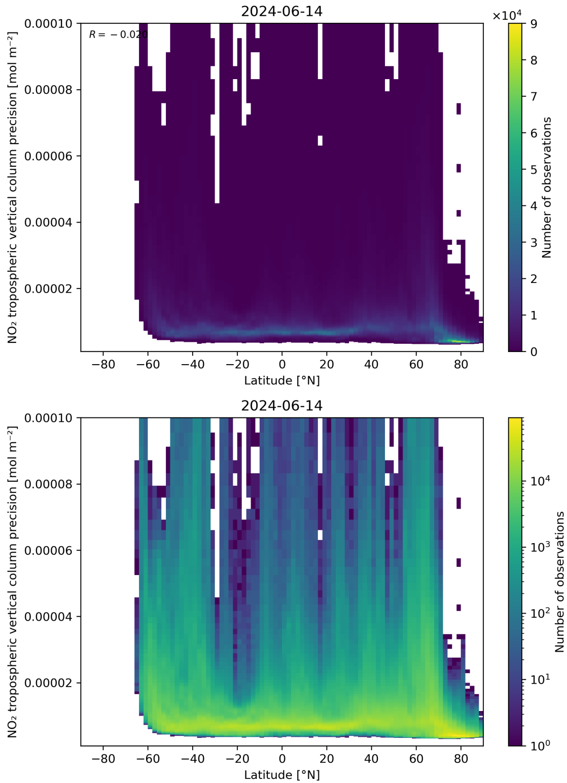
Figure 93: Scatter density plot of “Latitude” against “NO 2 tropospheric vertical column precision” for 2024-06-13 to 2024-06-15.
