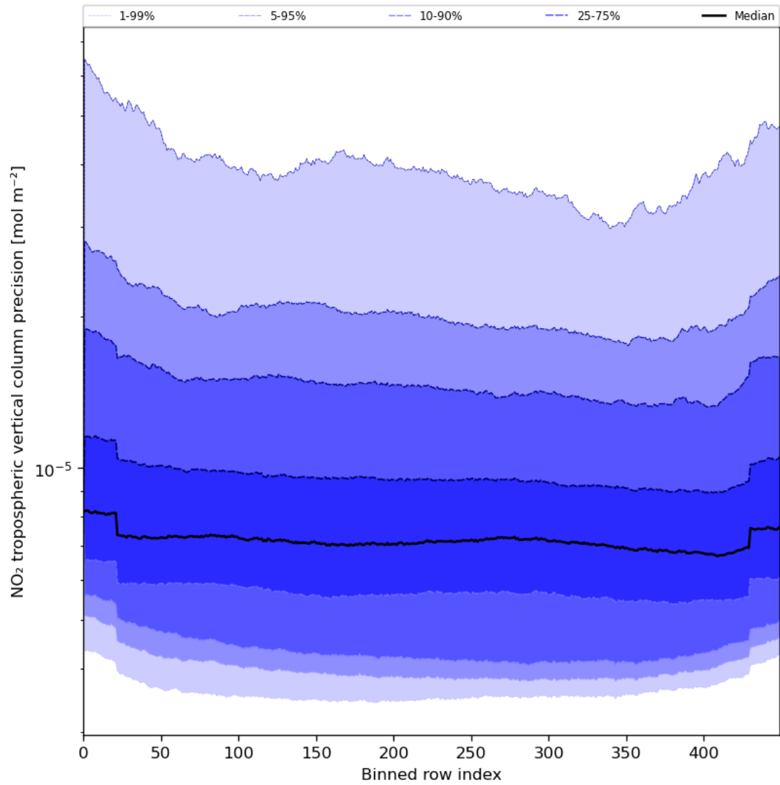
Figure 47: Along track statistics of “NO 2 tropospheric vertical column precision” for 2024-06-13 to 2024-06-15
