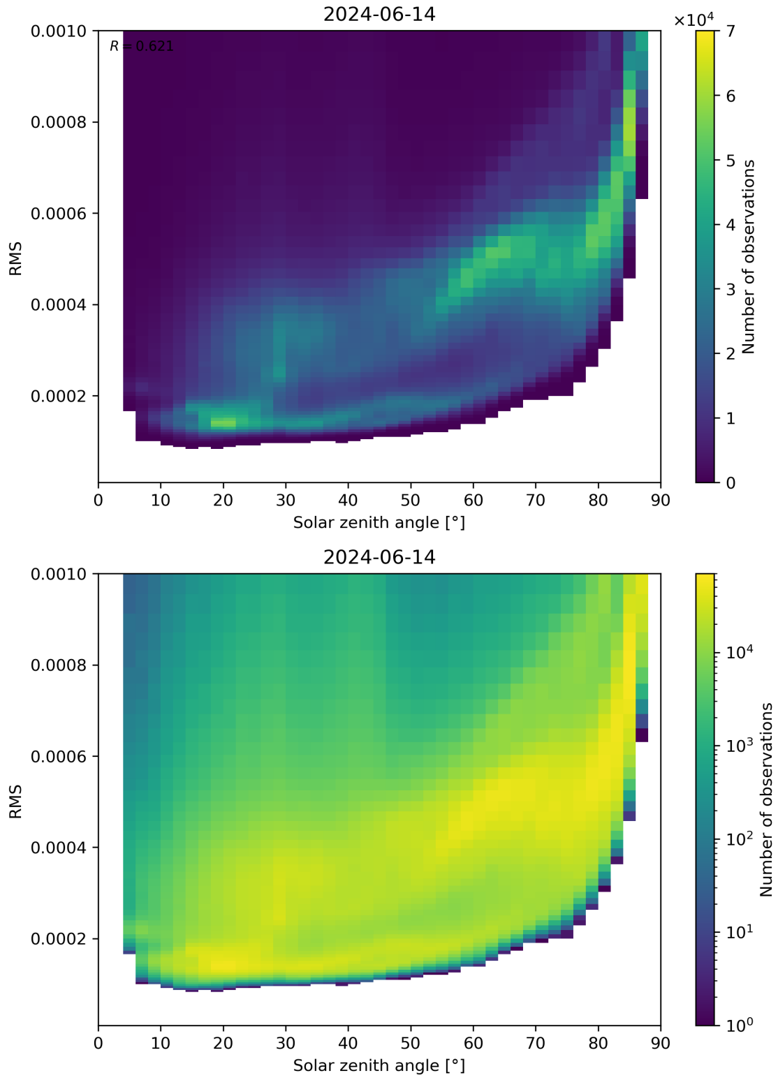
Figure 157: Scatter density plot of “Solar zenith angle” against “RMS” for 2024-06-13 to 2024-06-15.
