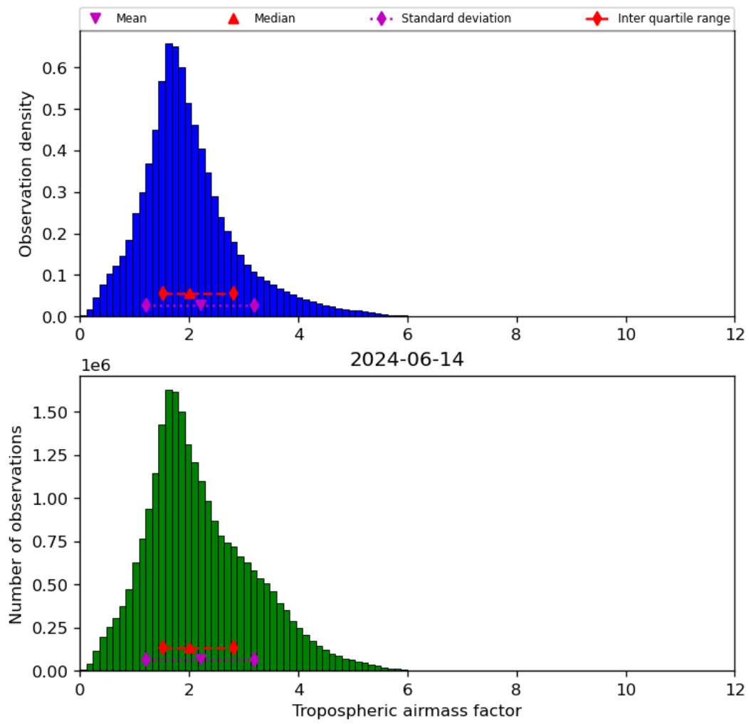
Figure 31: Histogram of “Tropospheric airmass factor” for 2024-06-13 to 2024-06-15
