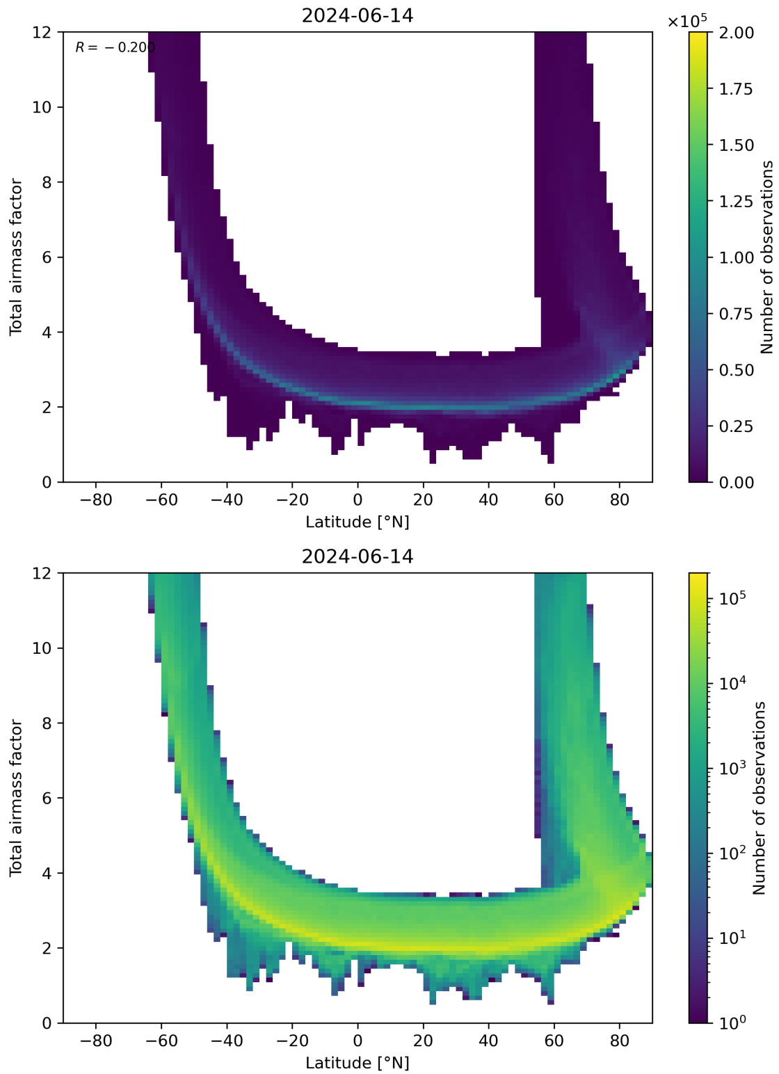
Figure 84: Scatter density plot of “Latitude” against “Total airmass factor” for 2024-06-13 to 2024-06-15.
