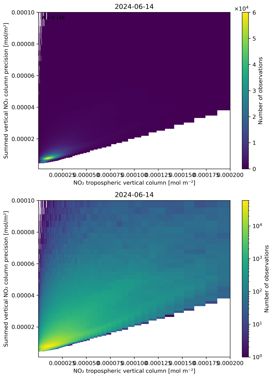
Figure 127: Scatter density plot of “NO 2 tropospheric vertical column” against “Summed vertical NO 2 column precision” for 2024-06-13 to 2024-06-15.
