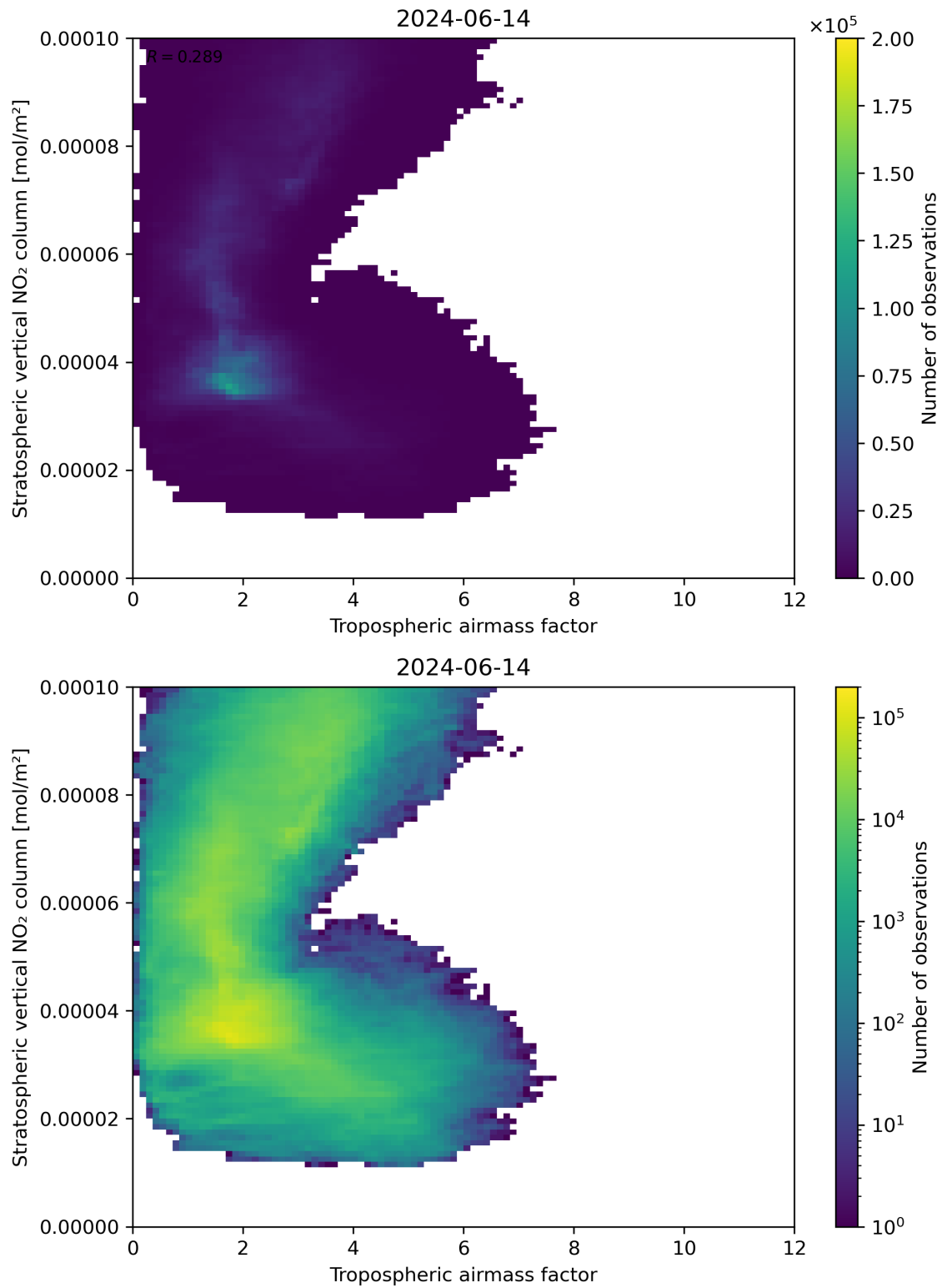
Figure 74: Scatter density plot of “Tropospheric air mass factor” against “Stratospheric vertical NO 2 column” for 2024-06-13 to 2024-06-15.
