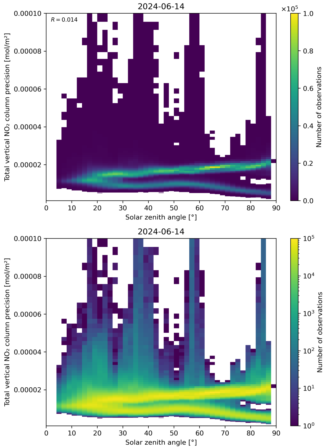
Figure 154: Scatter density plot of “Solar zenith angle” against “Total vertical NO 2 column precision” for 2024-06-13 to 2024-06-15.
