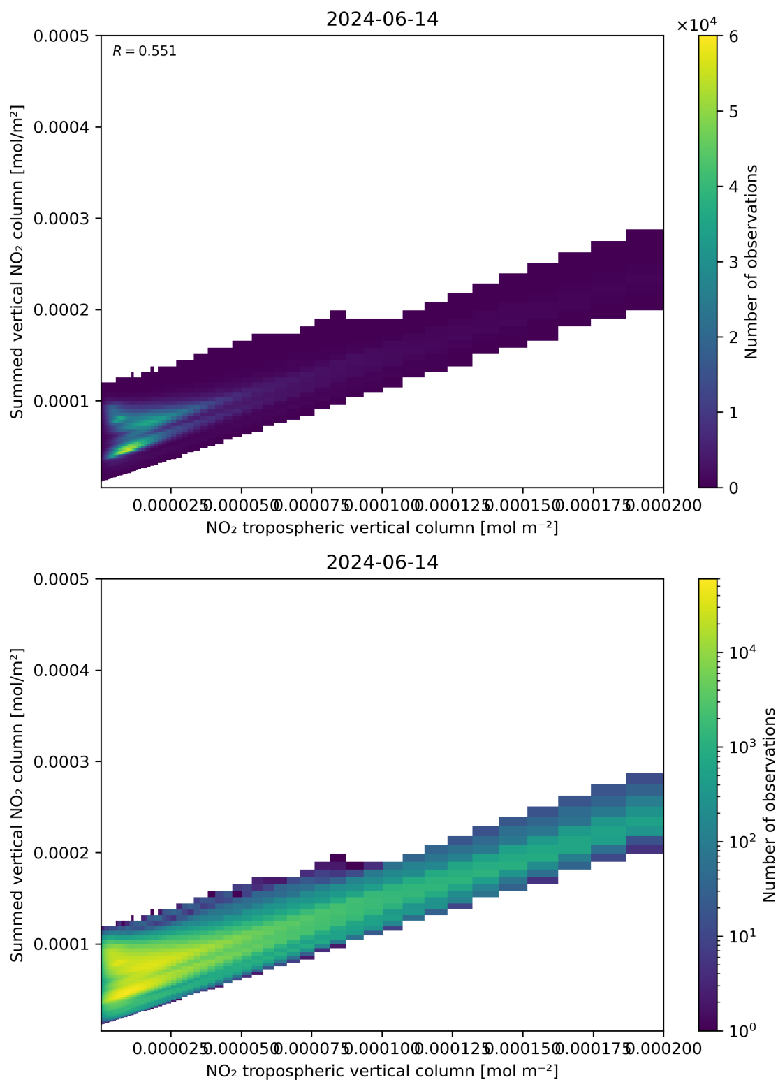
Figure 126: Scatter density plot of “NO 2 tropospheric vertical column” against “Summed vertical NO 2 column” for 2024-06-13 to 2024-06-15.
