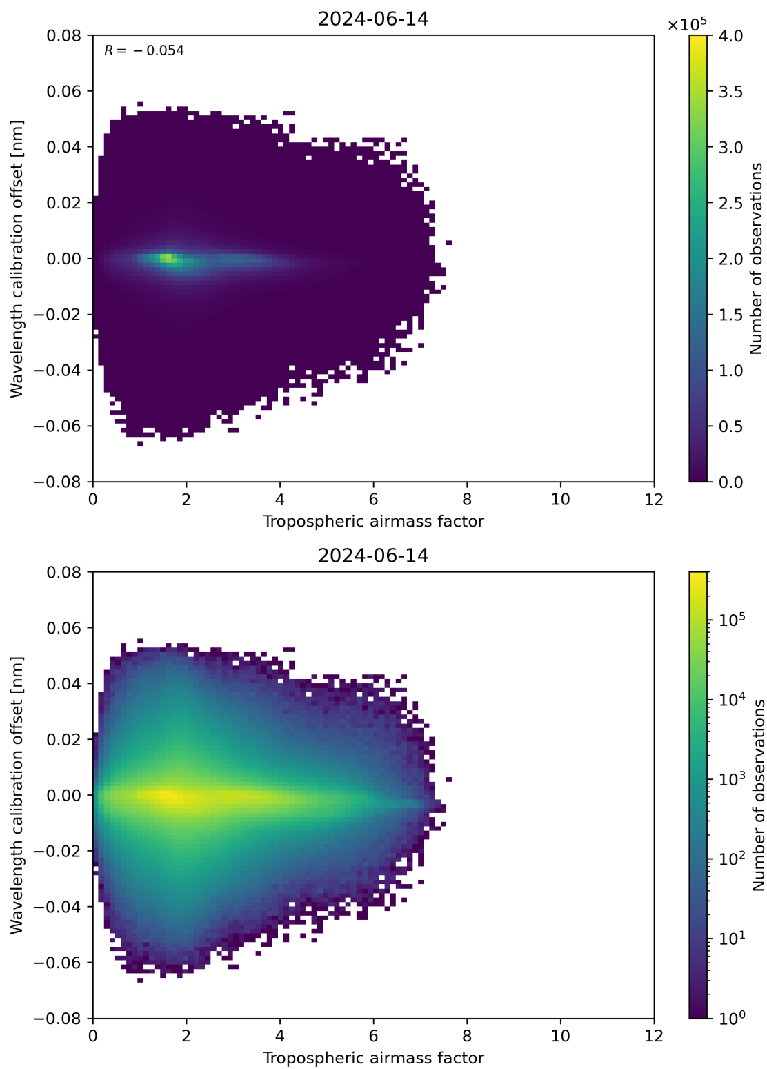
Figure 80: Scatter density plot of “Tropospheric airmass factor” against “Wavelength calibration offset” for 2024-06-13 to 2024-06-15.
