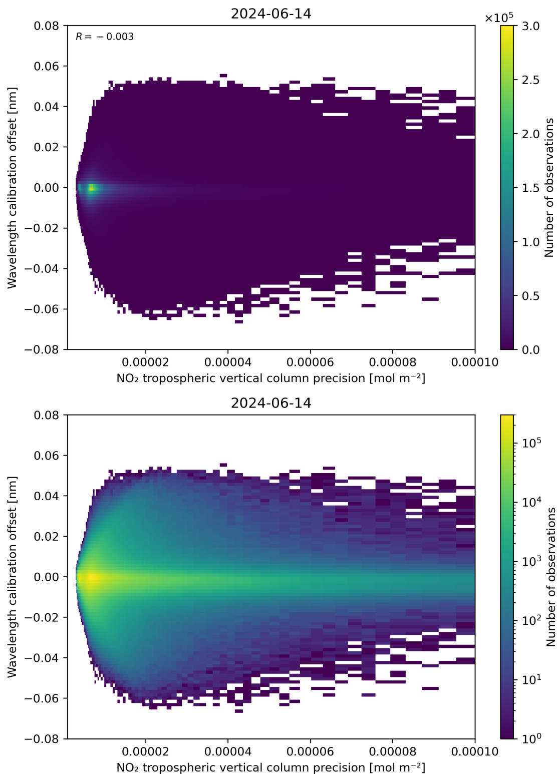
Figure 141: Scatter density plot of “NO 2 tropospheric vertical column precision” against “Wavelength calibration offset” for 2024-06-13 to 2024-06-15.
