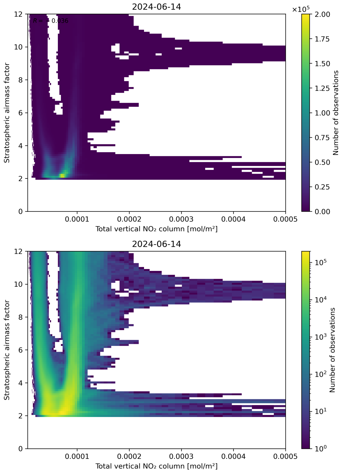
Figure 110: Scatter density plot of “Total vertical NO 2 column” against “Stratospheric airmass factor” for 2024-06-13 to 2024-06-15.
