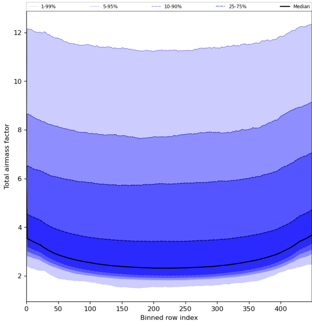
Figure 49: Along track statistics of “Total airmass factor” for 2024-06-13 to 2024-06-15
