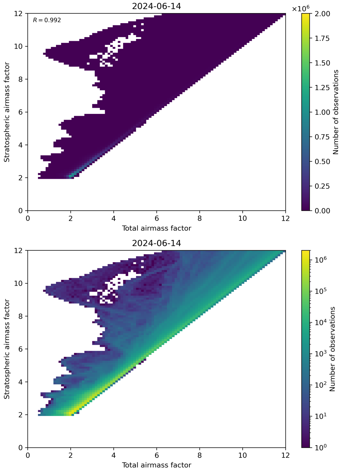
Figure 62: Scatter density plot of “Total airmass factor” against “Stratospheric airmass factor” for 2024-06-13 to 2024-06-15.
