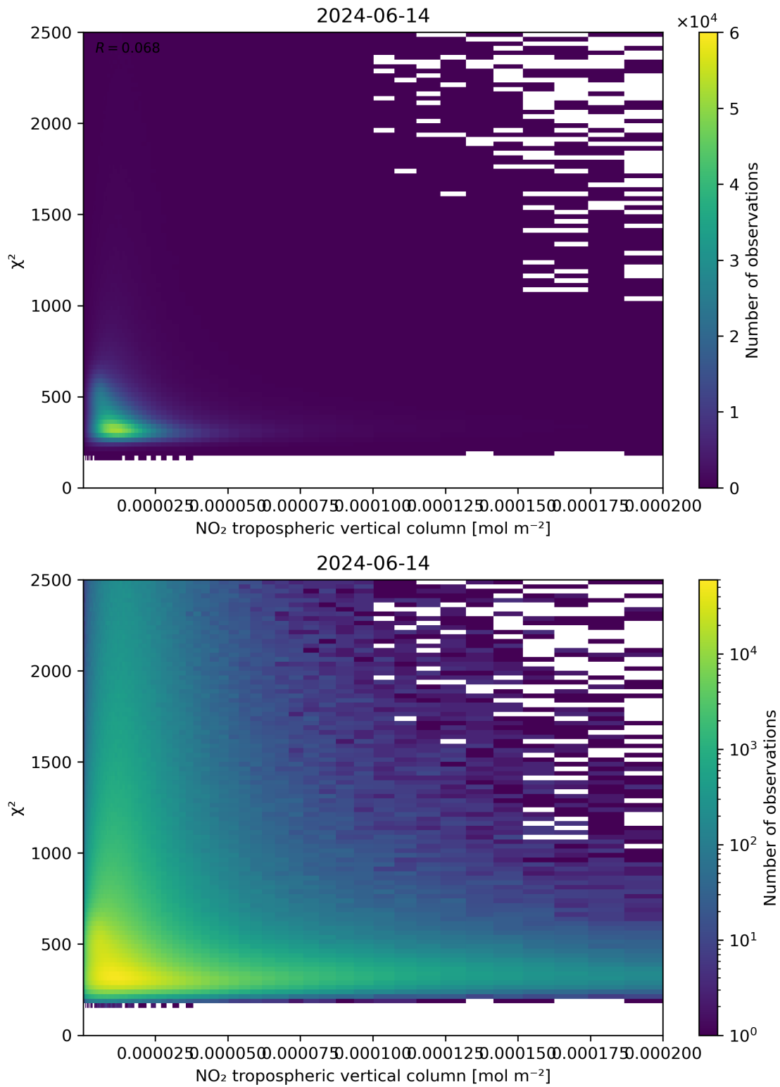
Figure 124: Scatter density plot of “NO 2 tropospheric vertical column” against “ \chi^2 ” for 2024-06-13 to 2024-06-15.
