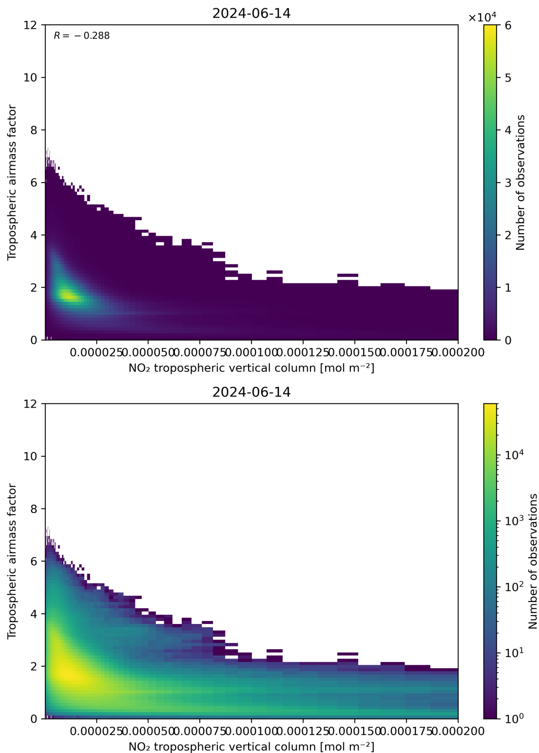
Figure 123: Scatter density plot of “NO 2 tropospheric vertical column” against “Tropospheric airmass factor” for 2024-06-13 to 2024-06-15.
