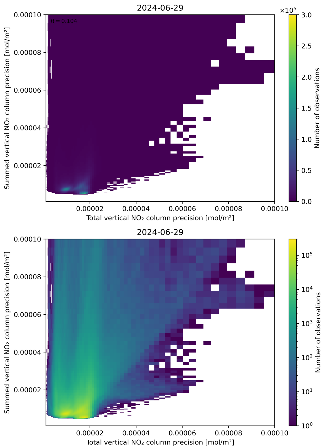
Figure 118: Scatter density plot of “Total vertical NO 2 column precision” against “Summed vertical NO 2 column precision” for 2024-06-29 to 2024-06-30.
