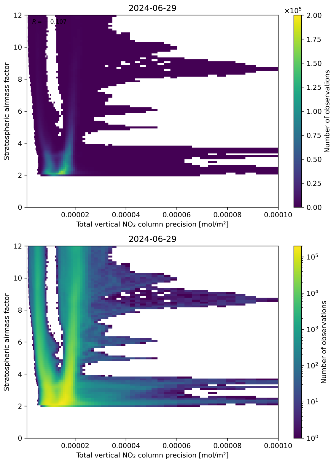
Figure 115: Scatter density plot of “Total vertical NO 2 column precision” against “Stratospheric air mass factor” for 2024-06-29 to 2024-06-30.
