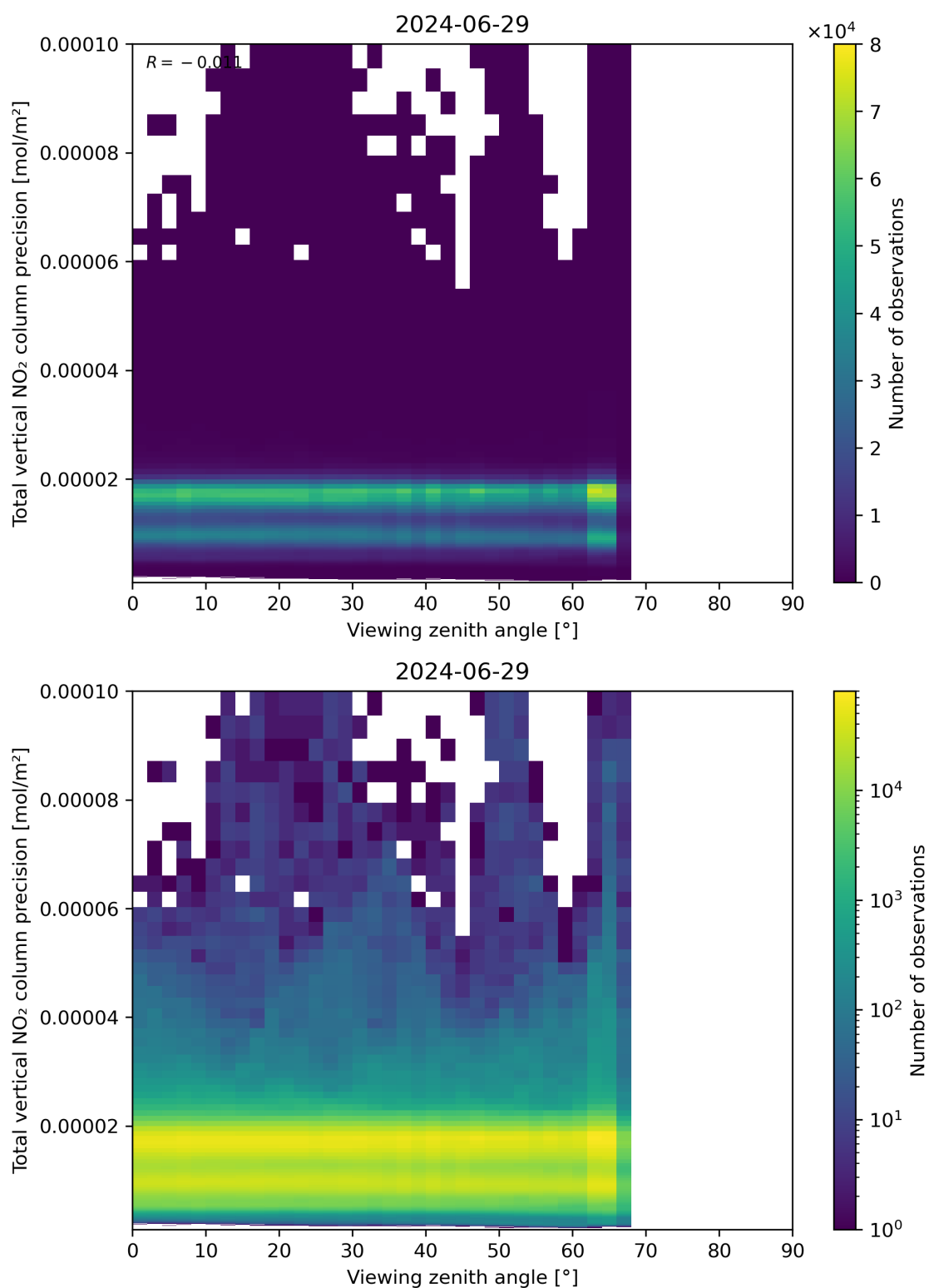
Figure 168: Scatter density plot of “Viewing zenith angle” against “Total vertical NO 2 column precision” for 2024-06-29 to 2024-06-30.
