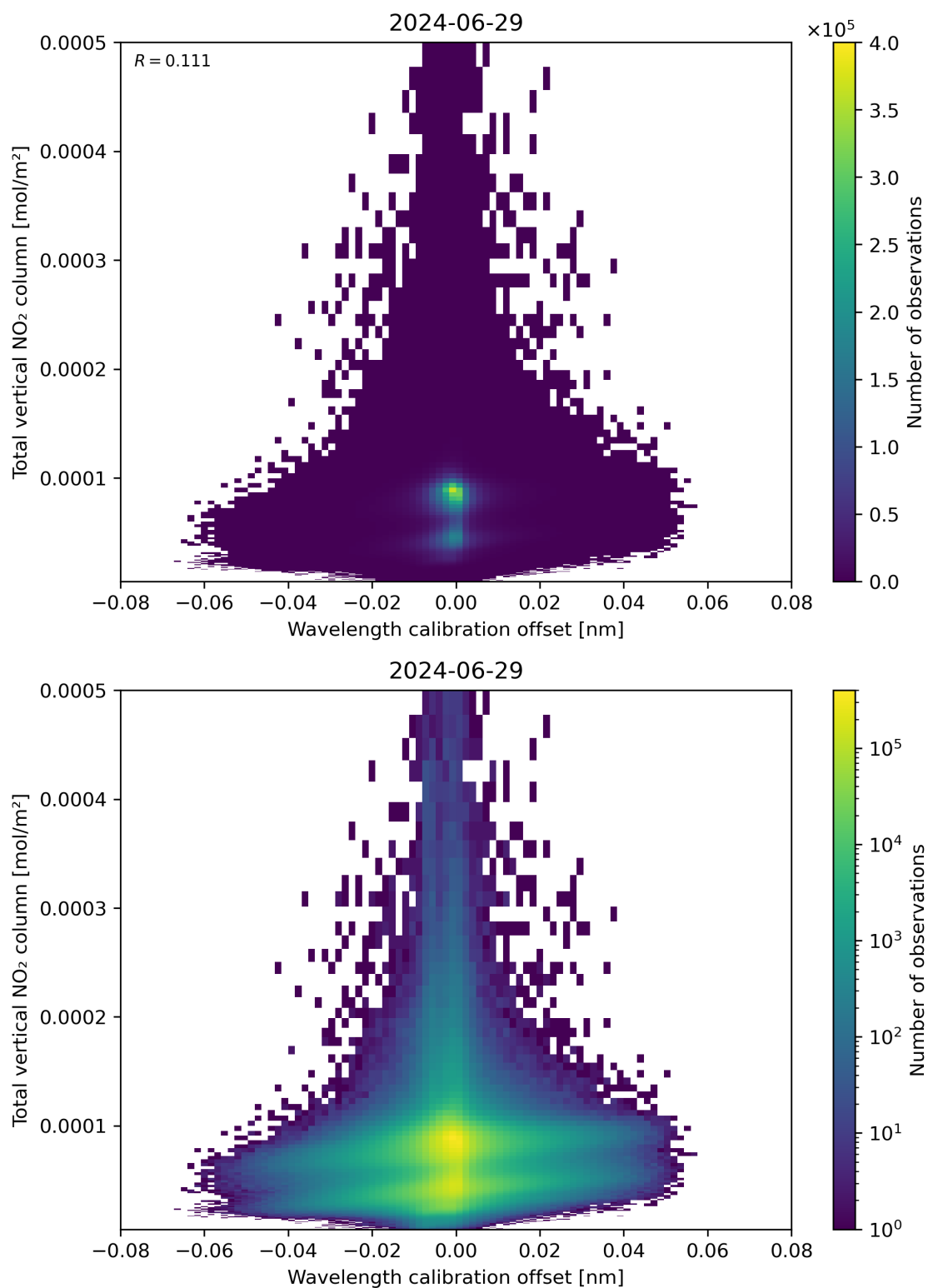
Figure 179: Scatter density plot of “Wavelength calibration offset” against “Total vertical NO 2 column” for 2024-06-29 to 2024-06-30.
