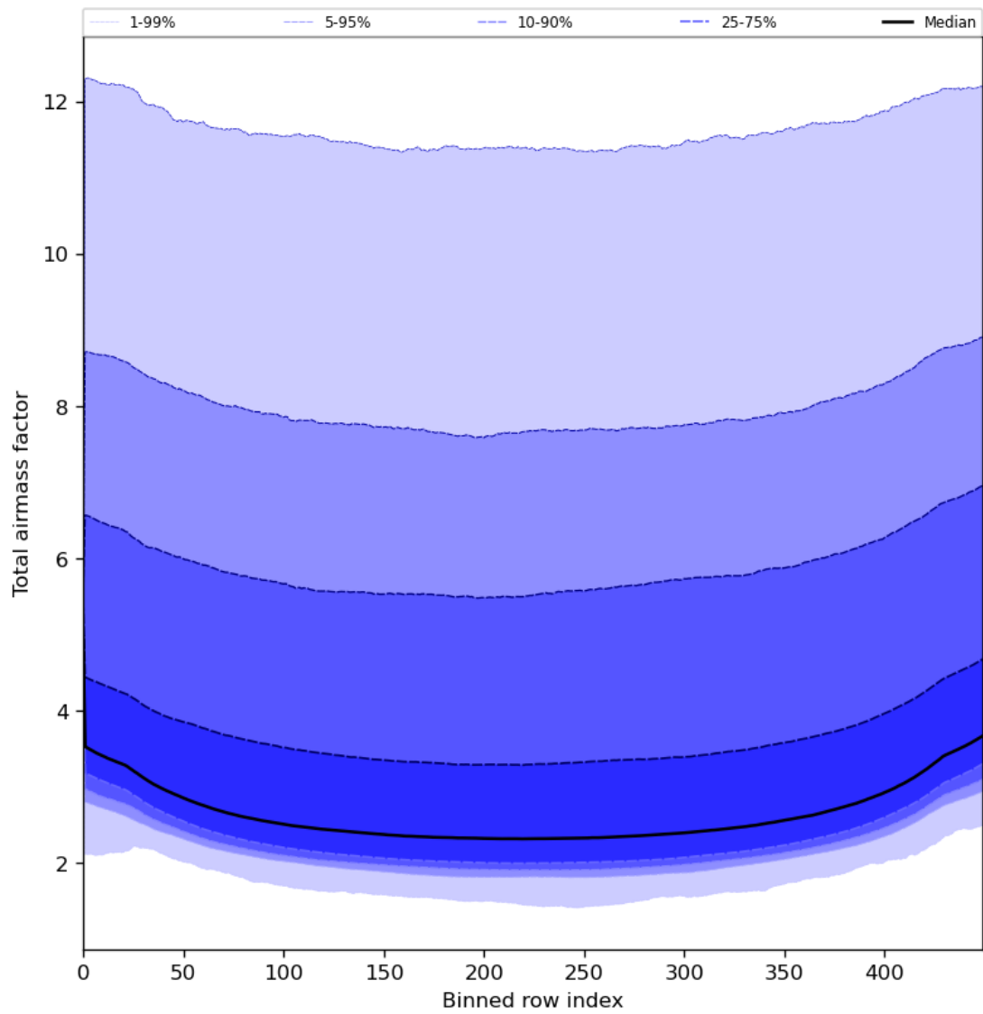
Figure 49: Along track statistics of “Total airmass factor” for 2024-06-29 to 2024-06-30
