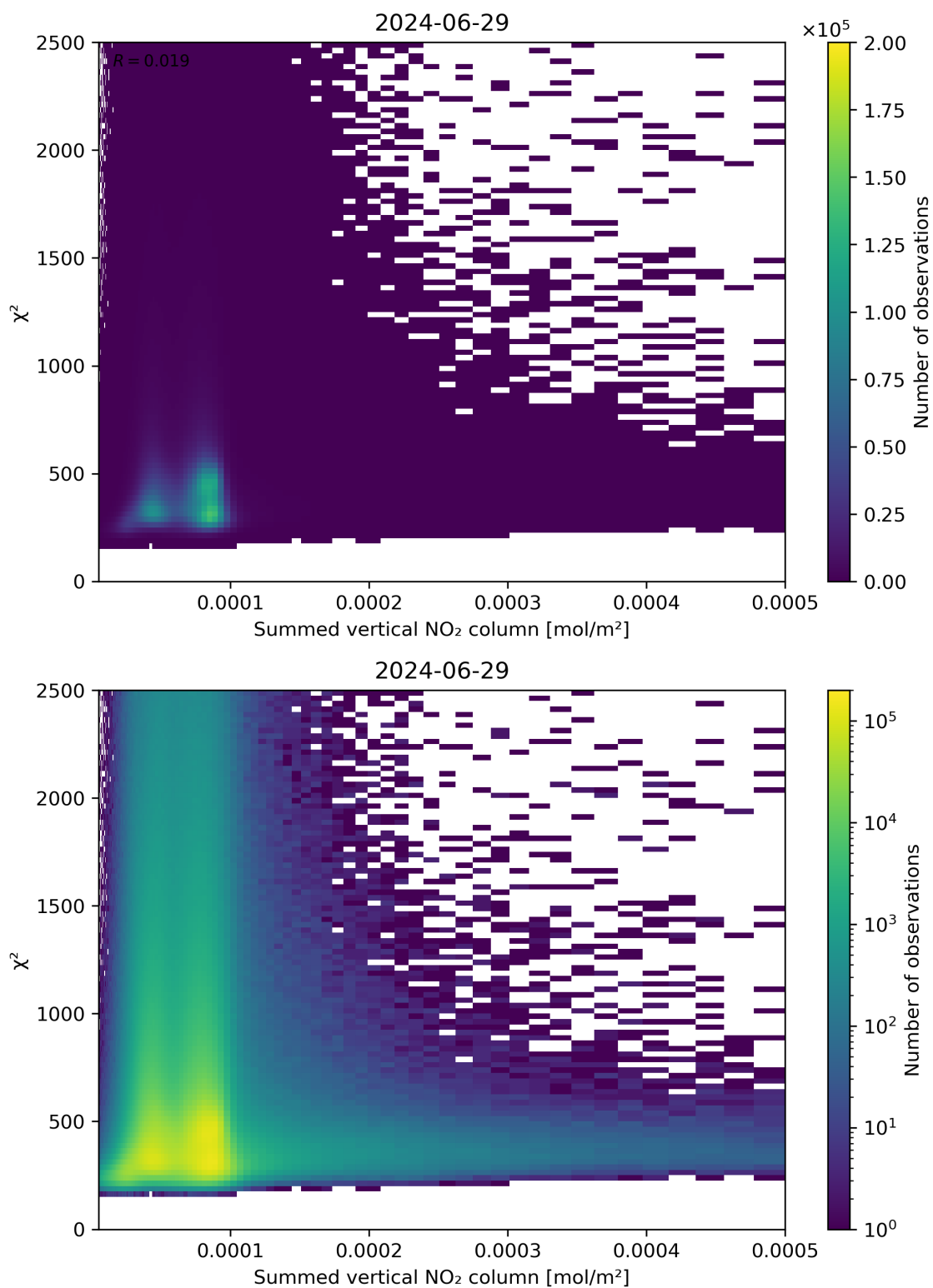
Figure 104: Scatter density plot of “Summed vertical NO 2 column” against “ \chi^2 ” for 2024-06-29 to 2024-06-30.
