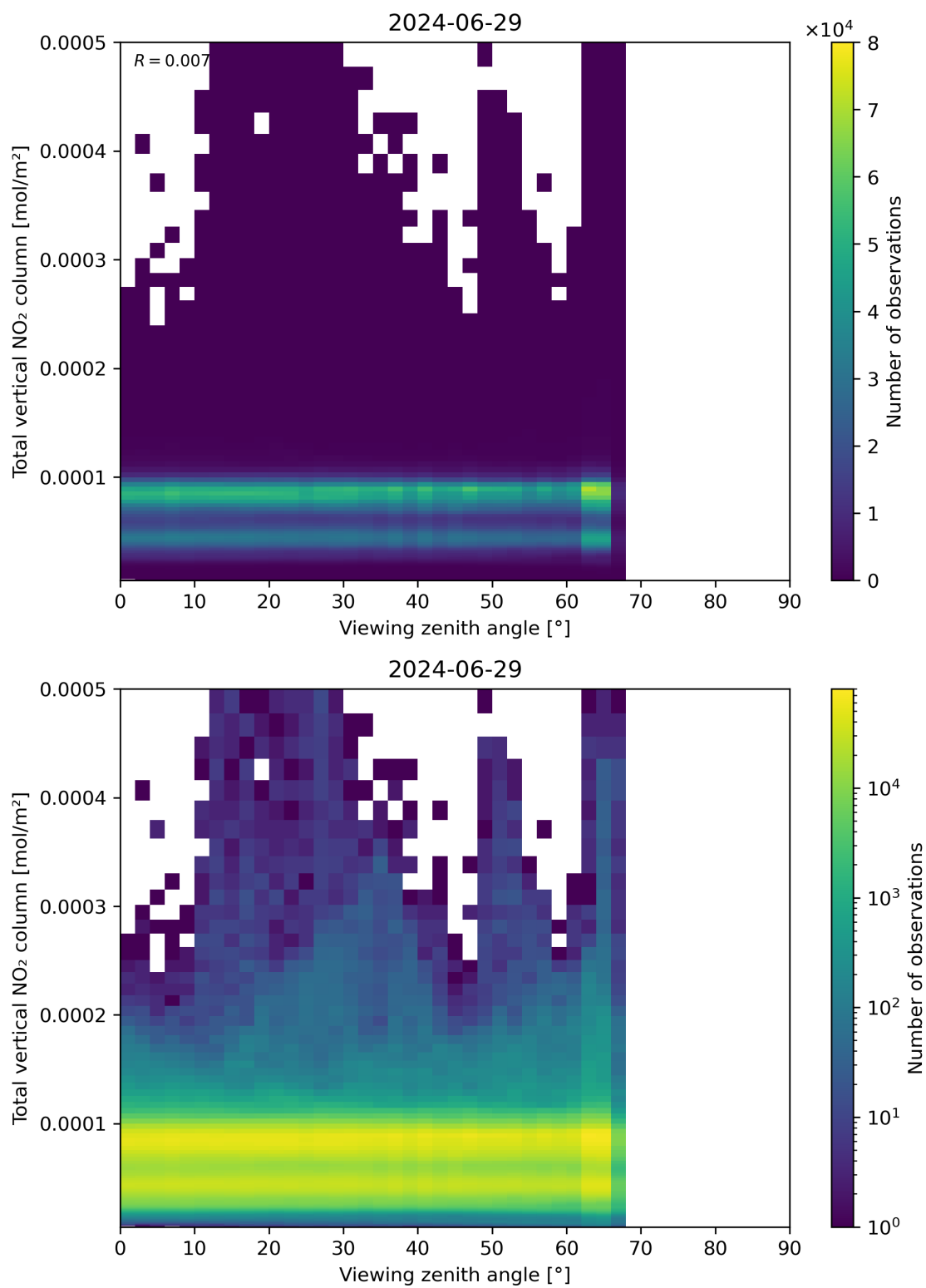
Figure 167: Scatter density plot of “Viewing zenith angle” against “Total vertical NO 2 column” for 2024-06-29 to 2024-06-30.
