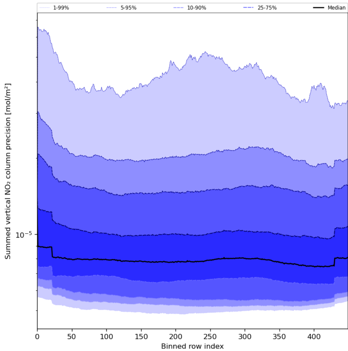
Figure 58: Along track statistics of “Summed vertical NO 2 column precision” for 2024-06-29 to 2024-06-30
