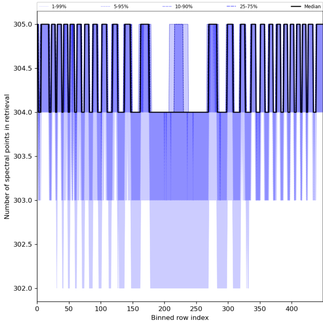
Figure 50: Along track statistics of “Number of spectral points in retrieval” for 2024-06-29 to 2024-06-30
