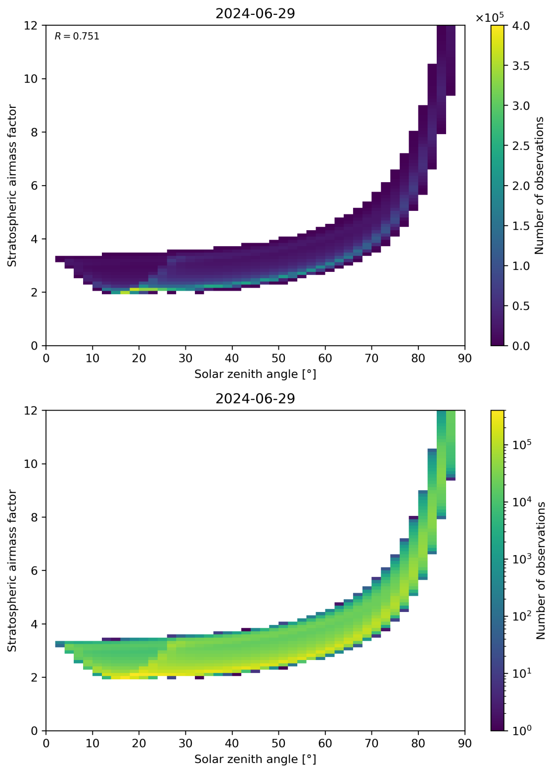
Figure 145: Scatter density plot of “Solar zenith angle” against “Stratospheric airmass factor” for 2024-06-29 to 2024-06-30.
