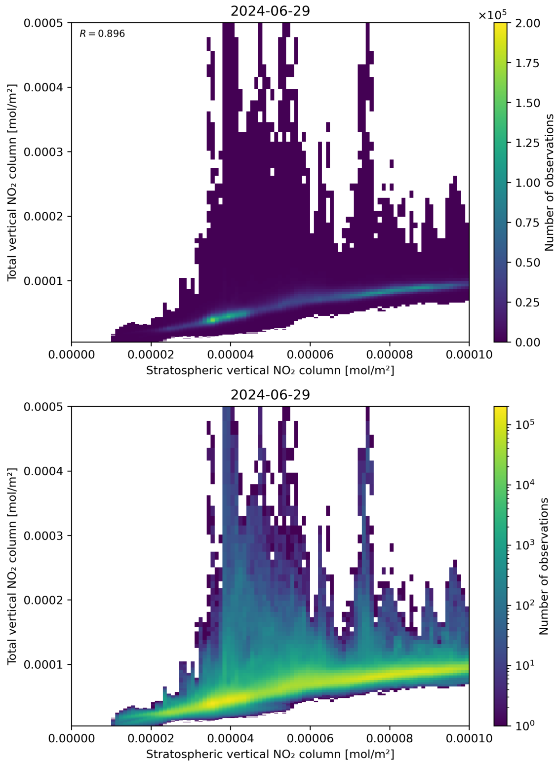
Figure 100: Scatter density plot of “Stratospheric vertical NO 2 column” against “Total vertical NO 2 column” for 2024-06-29 to 2024-06-30.
