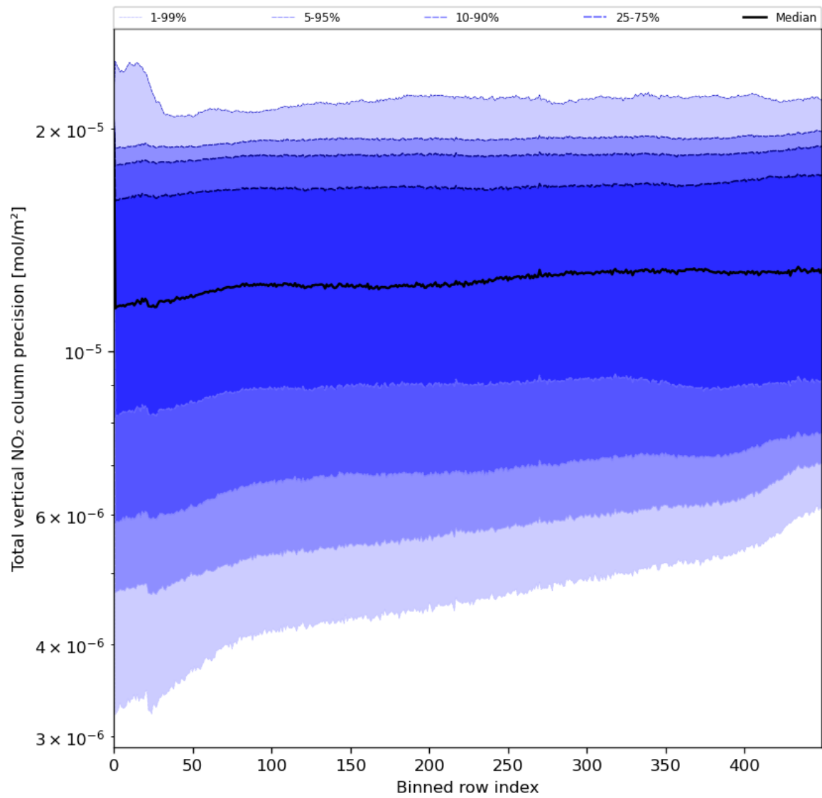
Figure 56: Along track statistics of “Total vertical NO 2 column precision” for 2024-06-29 to 2024-06-30
