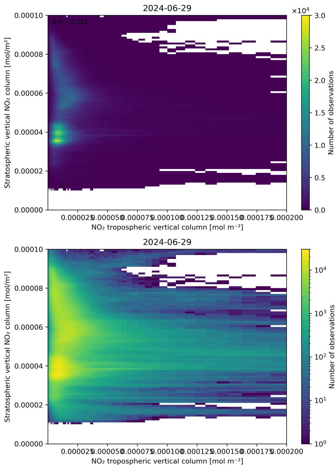
Figure 125: Scatter density plot of “NO 2 tropospheric vertical column” against “Stratospheric vertical NO 2 column” for 2024-06-29 to 2024-06-30.
