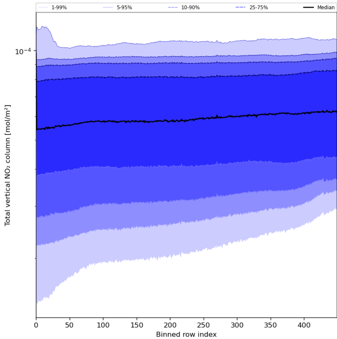
Figure 55: Along track statistics of “Total vertical NO 2 column” for 2024-06-29 to 2024-06-30
