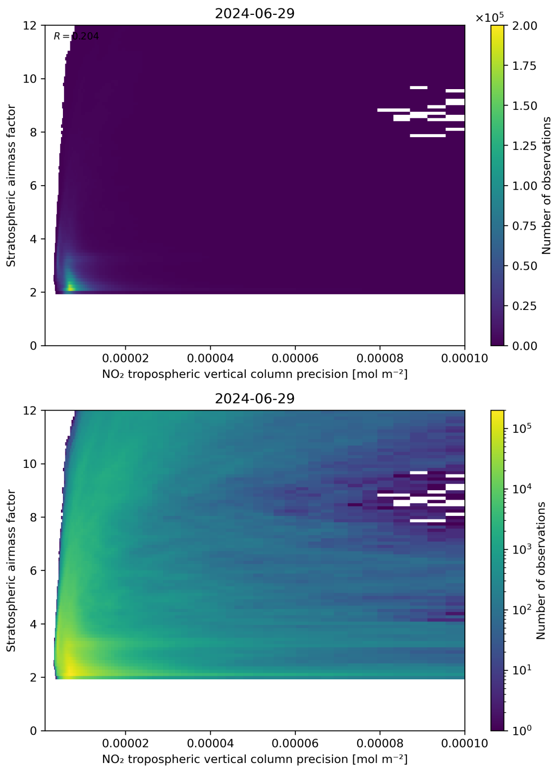
Figure 131: Scatter density plot of “NO 2 tropospheric vertical column precision” against “Stratospheric airmass factor” for 2024-06-29 to 2024-06-30.
