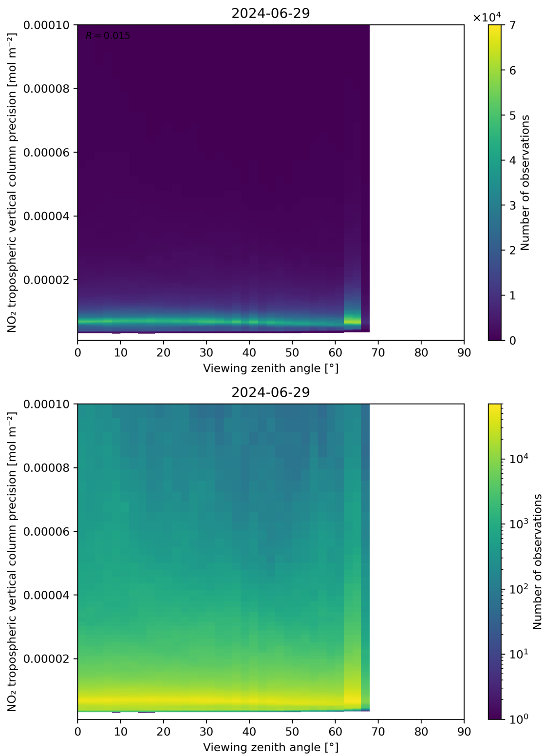
Figure 170: Scatter density plot of “Viewing zenith angle” against “NO 2 tropospheric vertical column precision” for 2024-06-29 to 2024-06-30.
