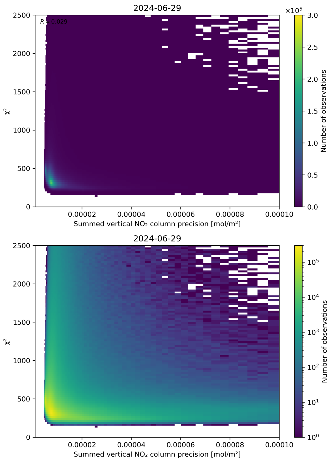
Figure 107: Scatter density plot of “Summed vertical NO 2 column precision” against “ \chi^2 ” for 2024-06-29 to 2024-06-30.
