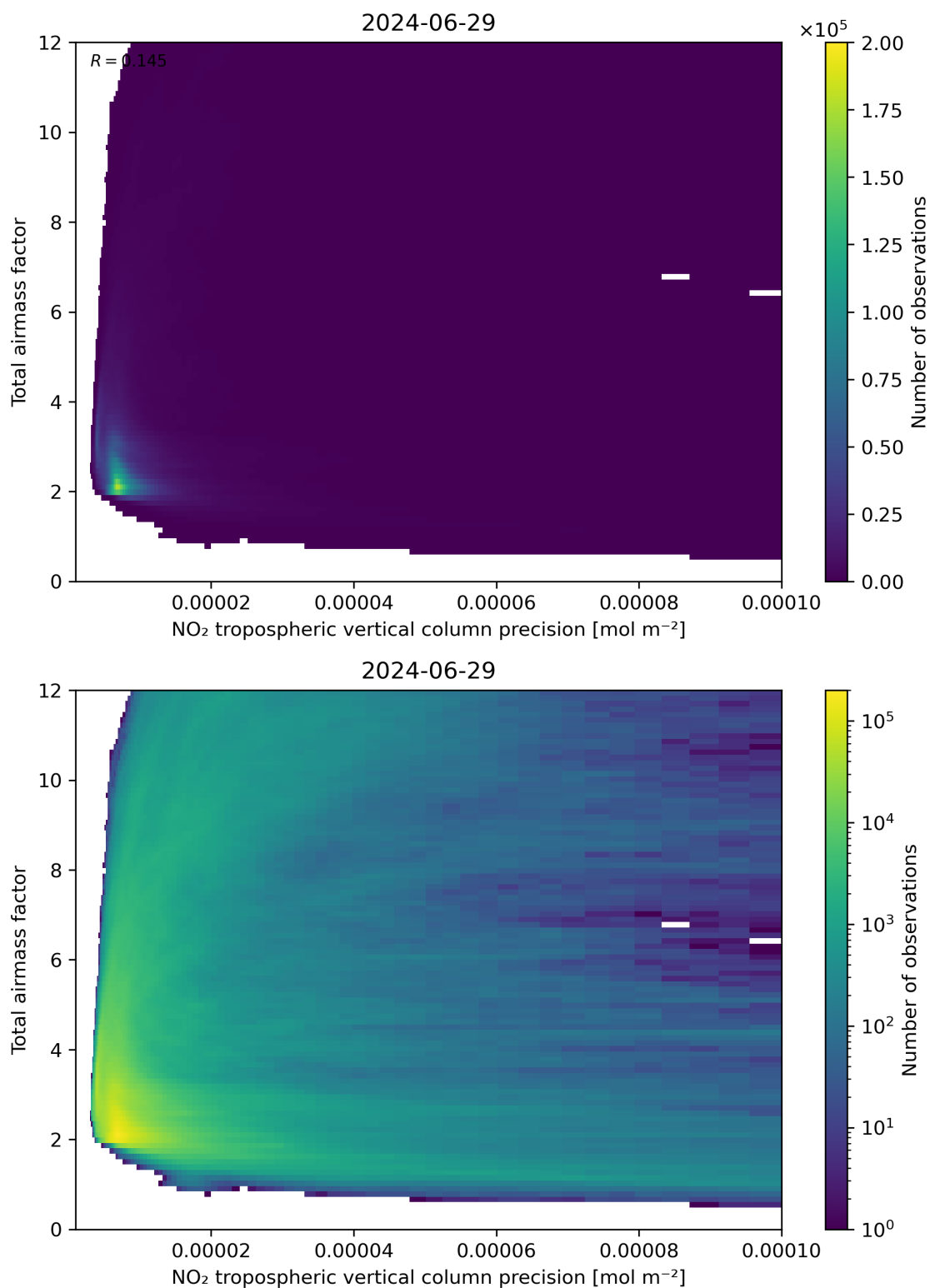
Figure 132: Scatter density plot of “NO 2 tropospheric vertical column precision” against “Total air mass factor” for 2024-06-29 to 2024-06-30.
