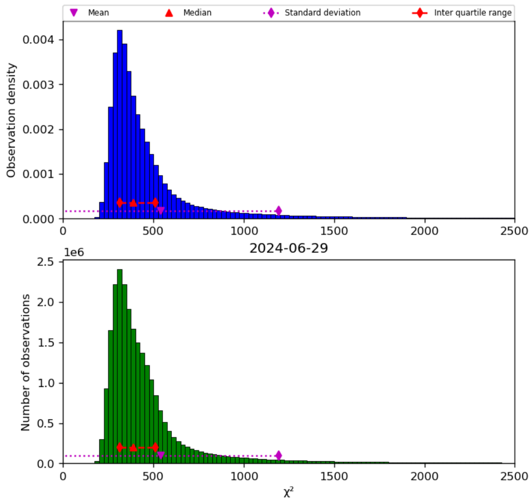
Figure 42: Histogram of “ \chi^2 ” for 2024-06-29 to 2024-06-30
