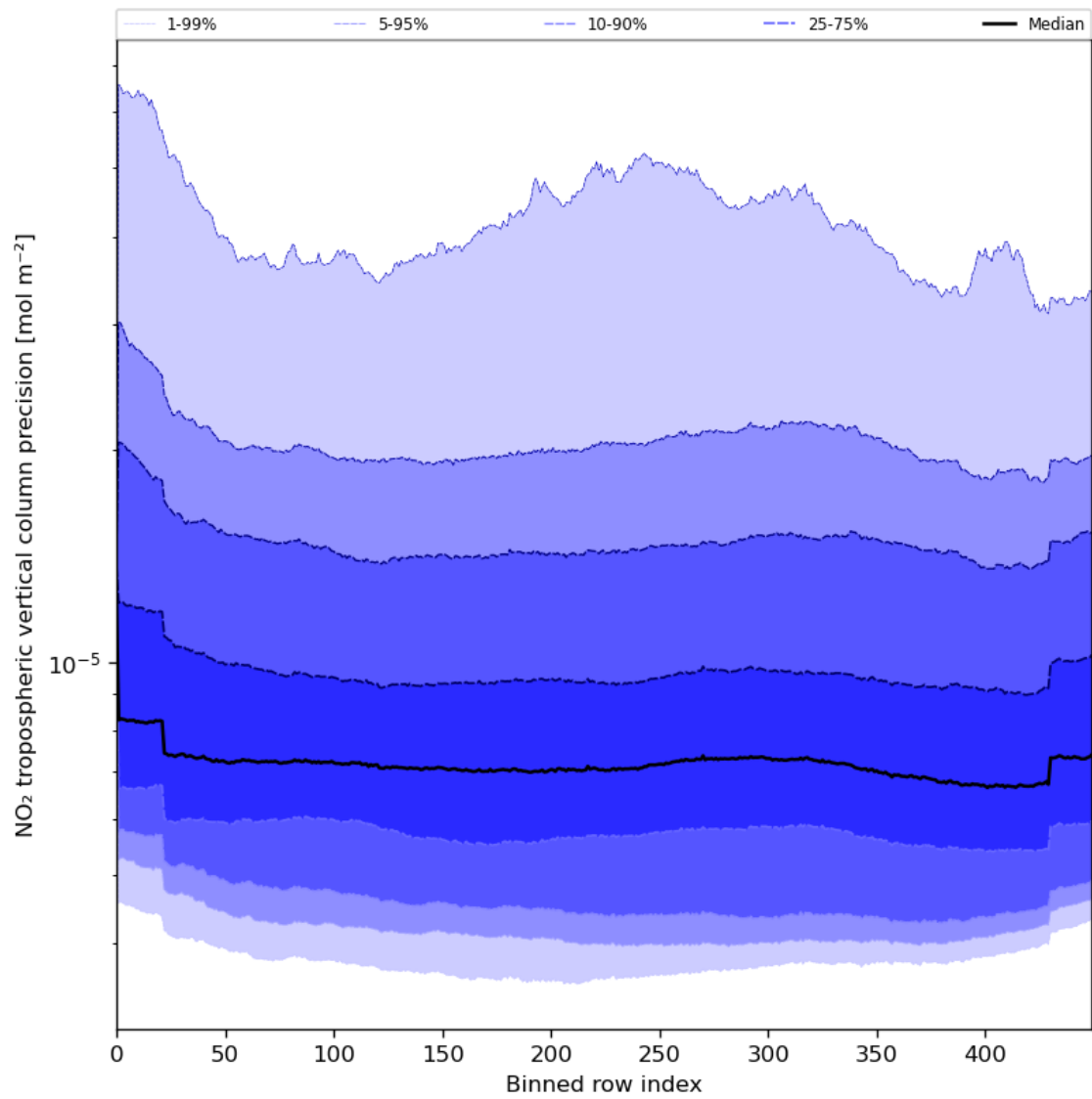
Figure 47: Along track statistics of “NO 2 tropospheric vertical column precision” for 2024-06-29 to 2024-06-30
