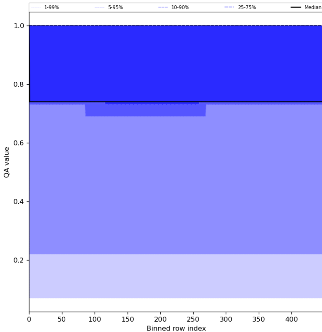
Figure 45: Along track statistics of “QA value” for 2024-06-29 to 2024-06-30
