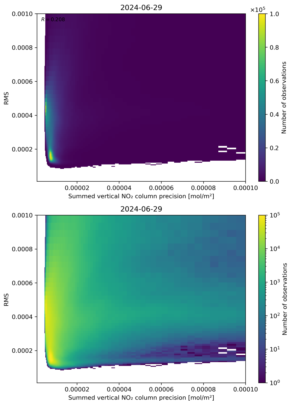
Figure 108: Scatter density plot of “Summed vertical NO 2 column precision” against “RMS” for 2024-06-29 to 2024-06-30.
