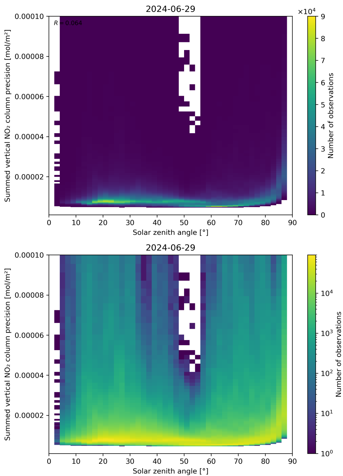
Figure 152: Scatter density plot of “Solar zenith angle” against “Summed vertical NO 2 column precision” for 2024-06-29 to 2024-06-30.
