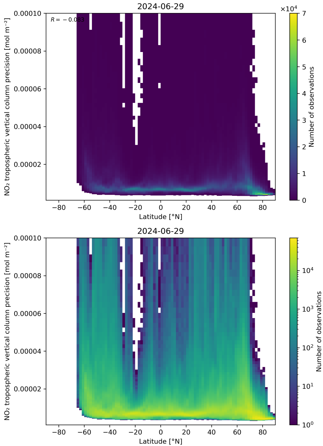
Figure 93: Scatter density plot of “Latitude” against “NO 2 tropospheric vertical column precision” for 2024-06-29 to 2024-06-30.
