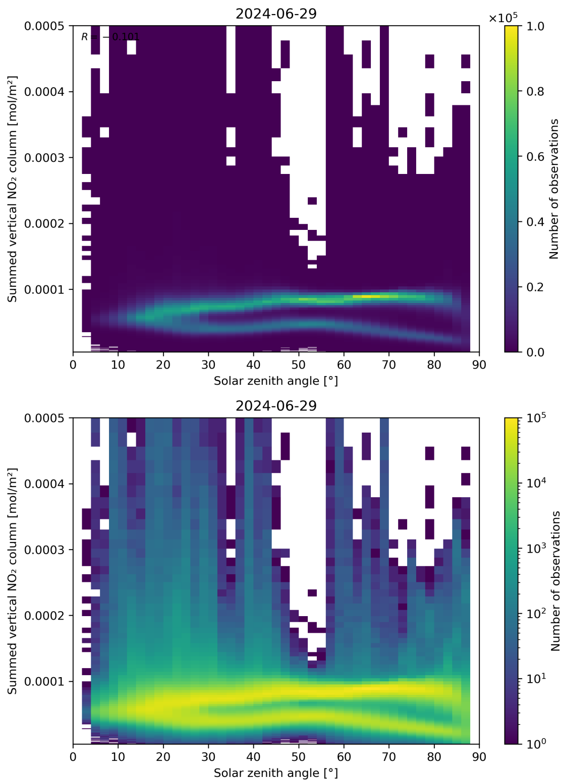
Figure 151: Scatter density plot of “Solar zenith angle” against “Summed vertical NO 2 column” for 2024-06-29 to 2024-06-30.
