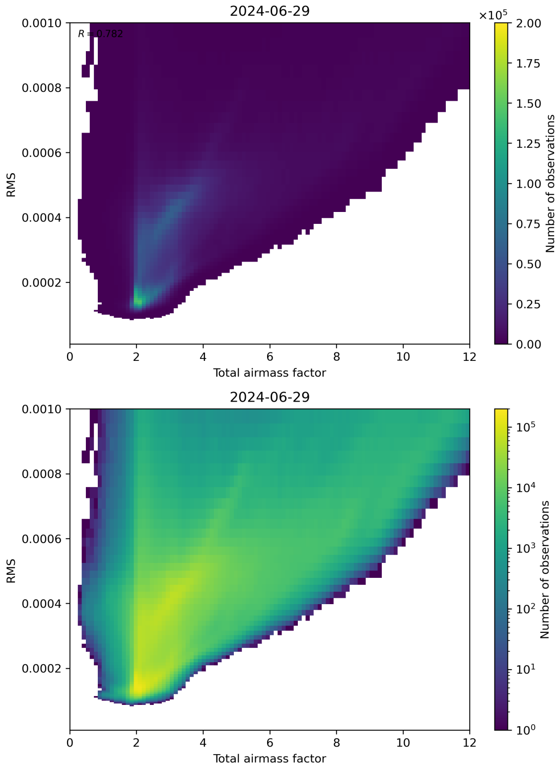
Figure 69: Scatter density plot of “Total airmass factor” against “RMS” for 2024-06-29 to 2024-06-30.
