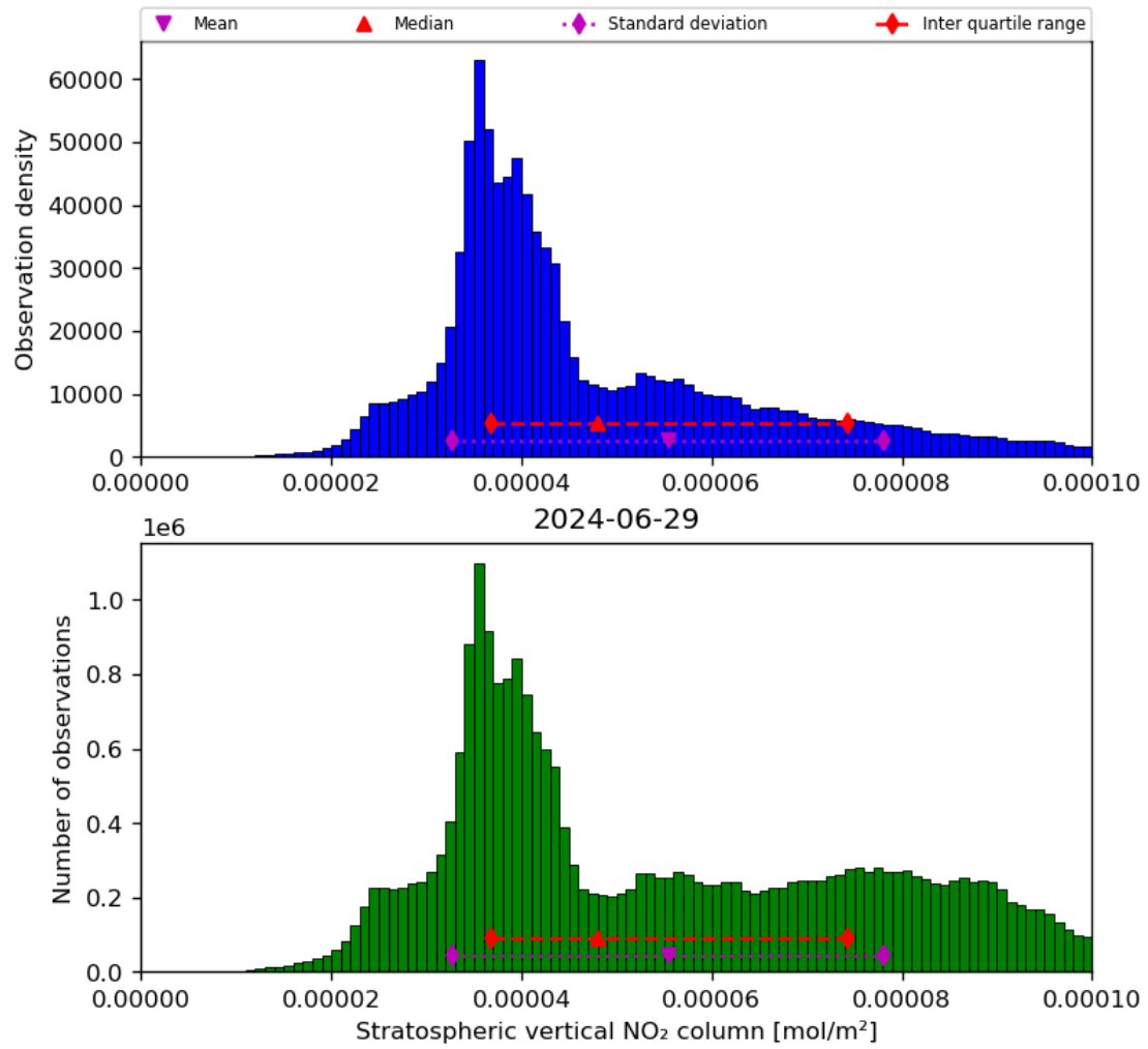
Figure 36: Histogram of “Stratospheric vertical NO 2 column” for 2024-06-29 to 2024-06-30
