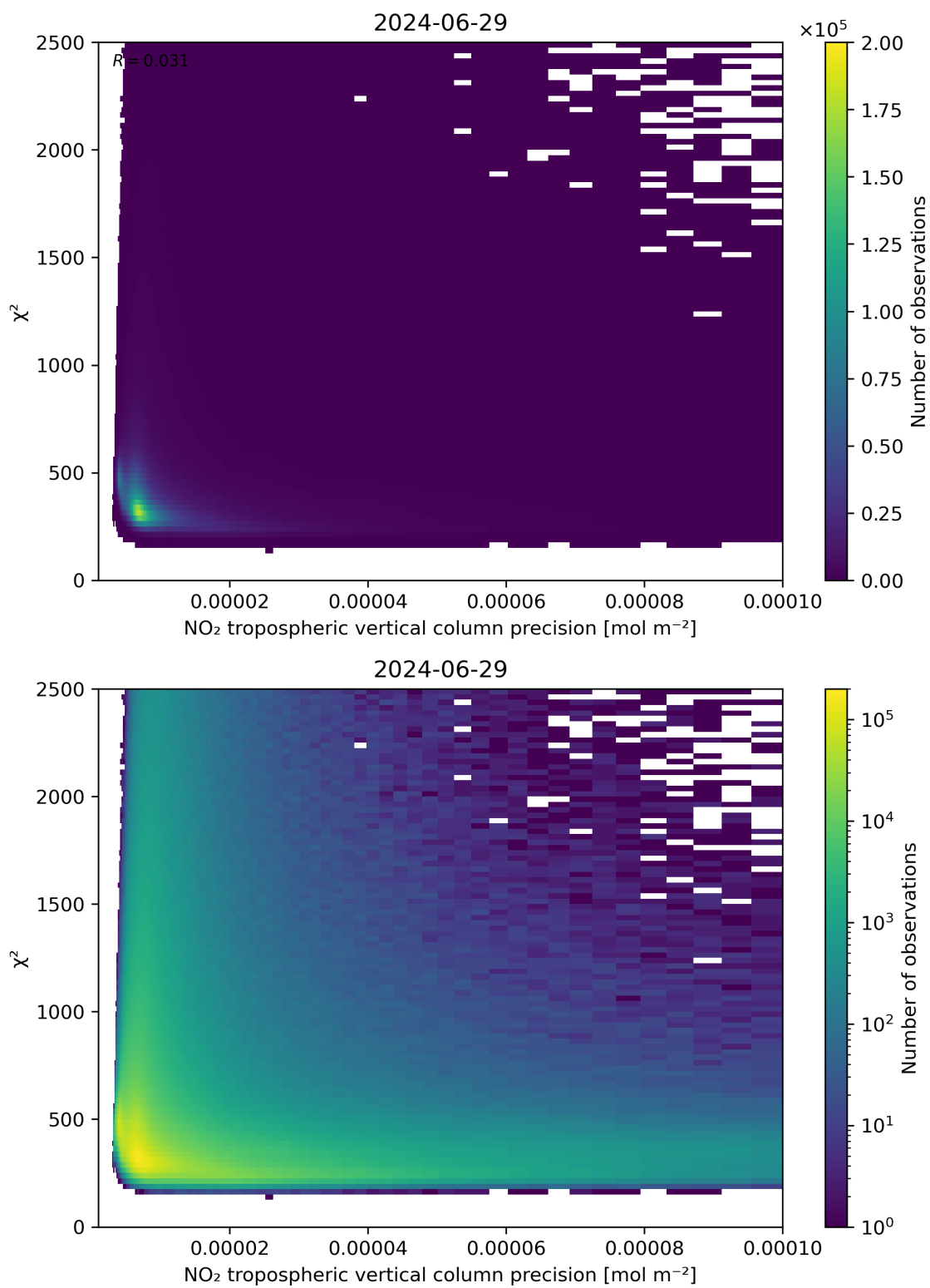
Figure 134: Scatter density plot of “NO 2 tropospheric vertical column precision” against “ \chi^2 ” for 2024-06-29 to 2024-06-30.
