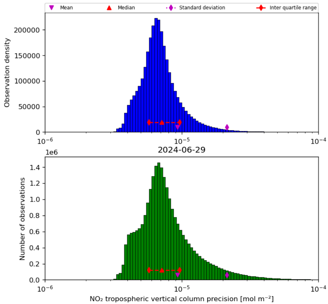
Figure 30: Histogram of “NO 2 tropospheric vertical column precision” for 2024-06-29 to 2024-06-30
