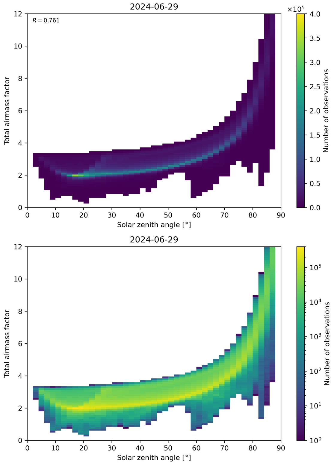
Figure 146: Scatter density plot of “Solar zenith angle” against “Total air mass factor” for 2024-06-29 to 2024-06-30.
