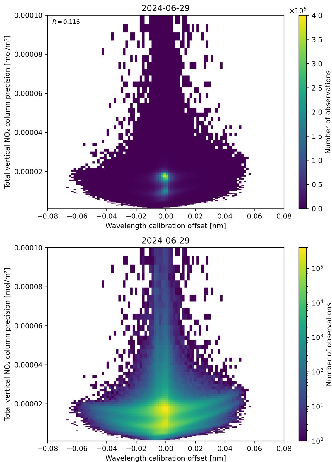
Figure 180: Scatter density plot of “Wavelength calibration offset” against “Total vertical NO 2 column precision” for 2024-06-29 to 2024-06-30.
