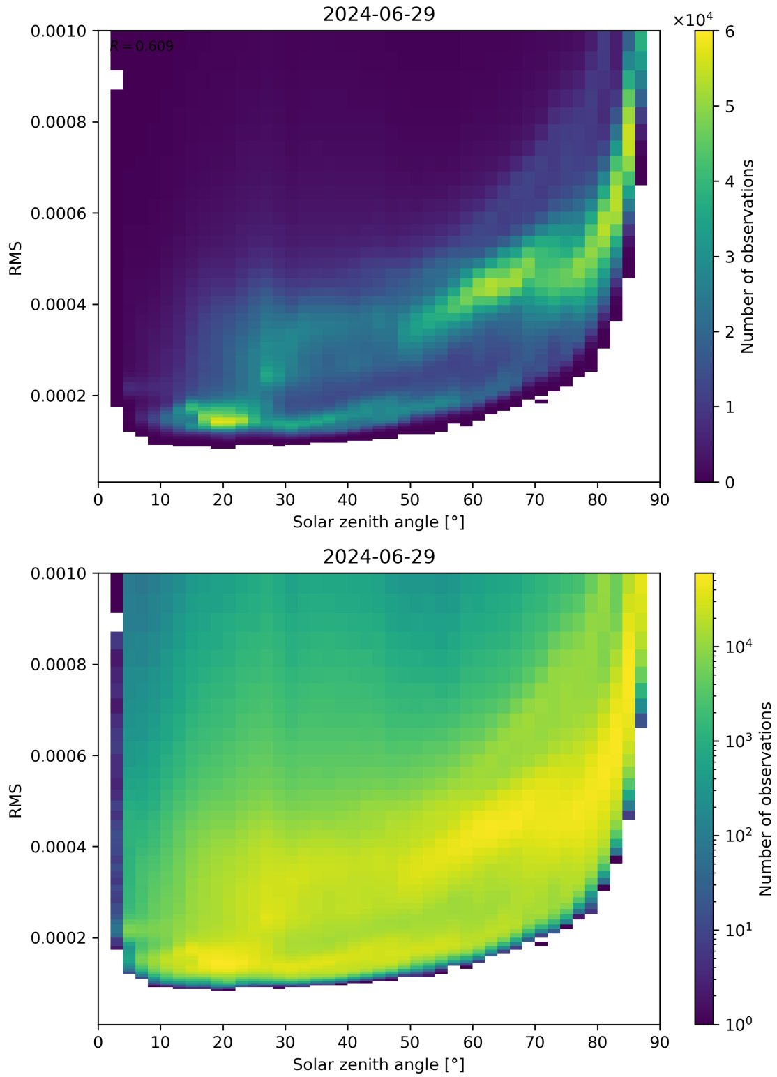
Figure 157: Scatter density plot of “Solar zenith angle” against “RMS” for 2024-06-29 to 2024-06-30.
