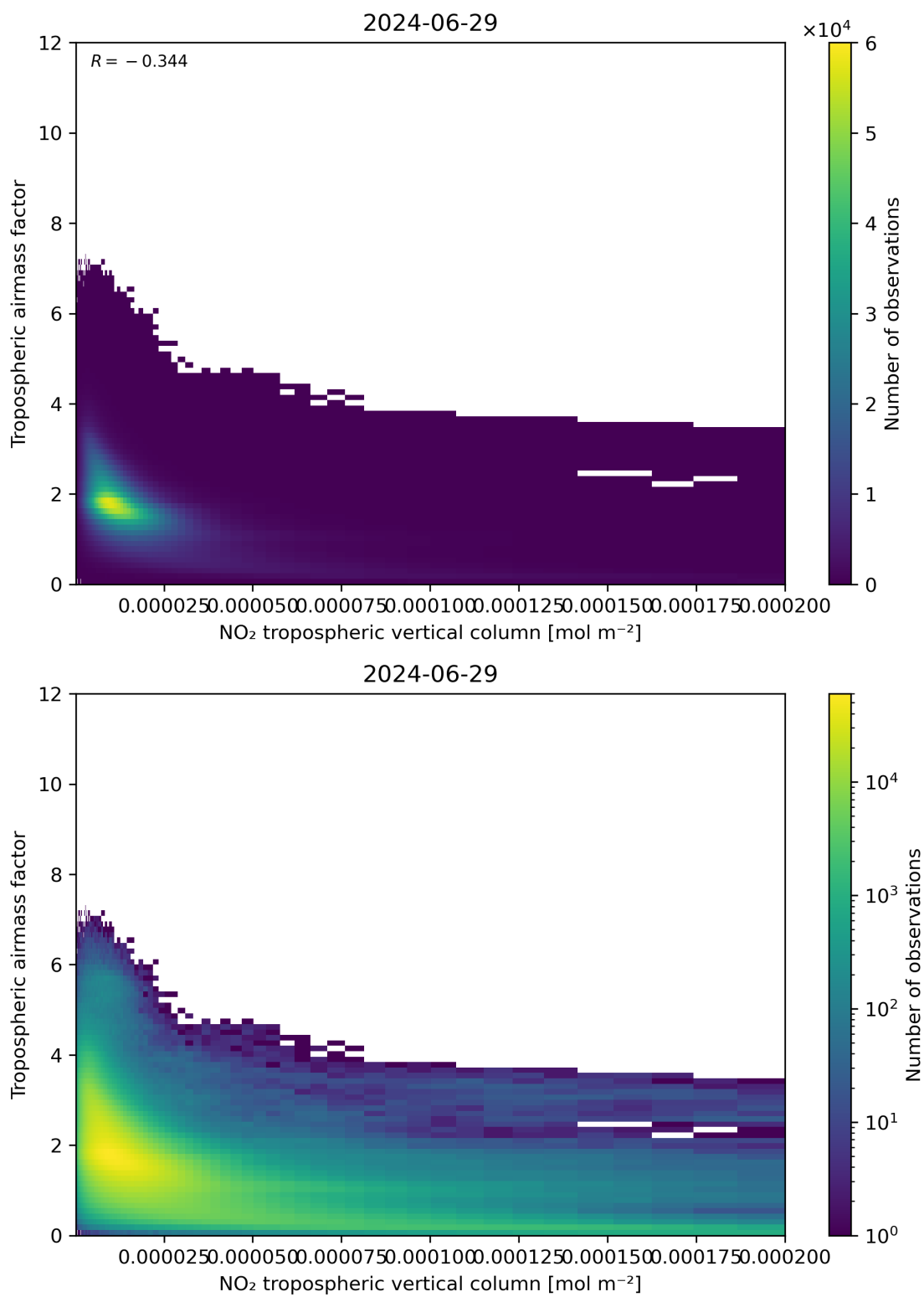
Figure 123: Scatter density plot of “NO 2 tropospheric vertical column” against “Tropospheric air mass factor” for 2024-06-29 to 2024-06-30.
