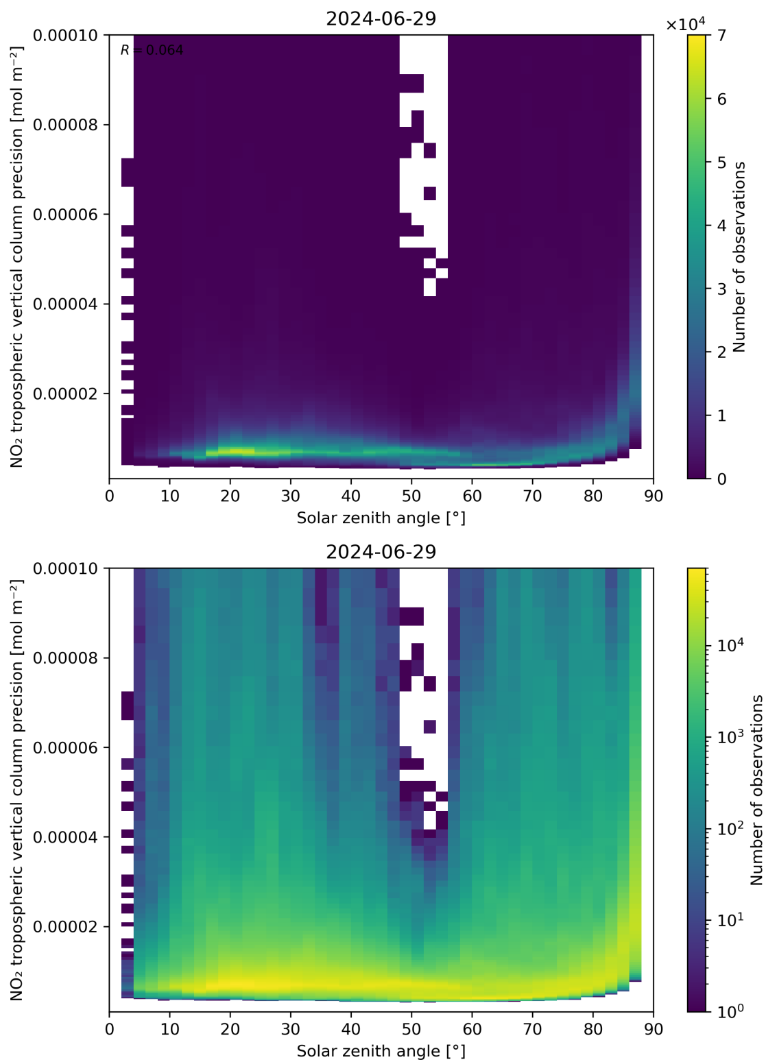
Figure 156: Scatter density plot of “Solar zenith angle” against “NO 2 tropospheric vertical column precision” for 2024-06-29 to 2024-06-30.
