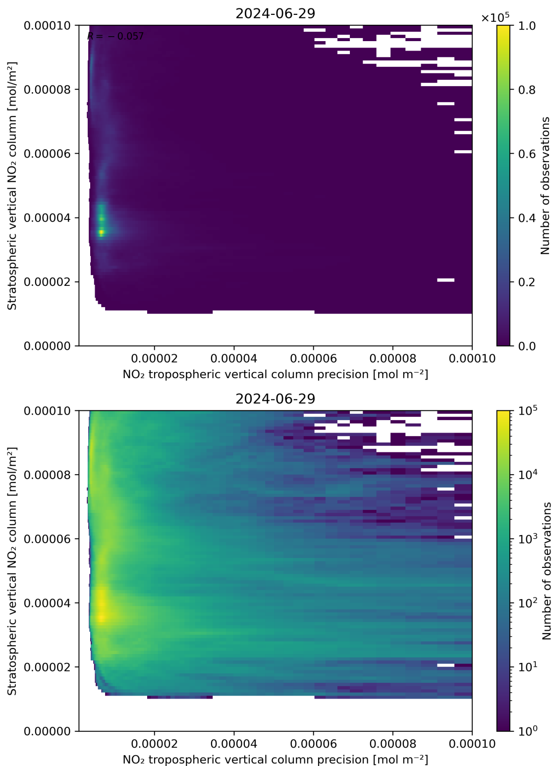
Figure 135: Scatter density plot of “NO 2 tropospheric vertical column precision” against “Stratospheric vertical NO 2 column” for 2024-06-29 to 2024-06-30.
