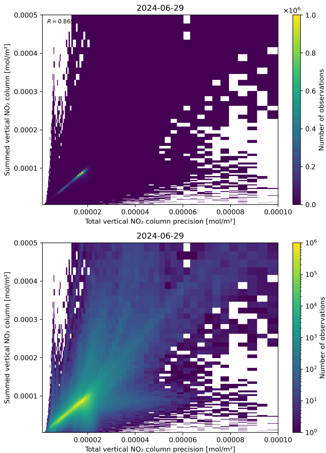
Figure 117: Scatter density plot of “Total vertical NO 2 column precision” against “Summed vertical NO 2 column” for 2024-06-29 to 2024-06-30.
