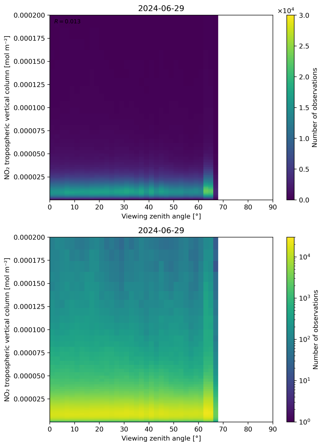
Figure 169: Scatter density plot of “Viewing zenith angle” against “NO 2 tropospheric vertical column” for 2024-06-29 to 2024-06-30.
