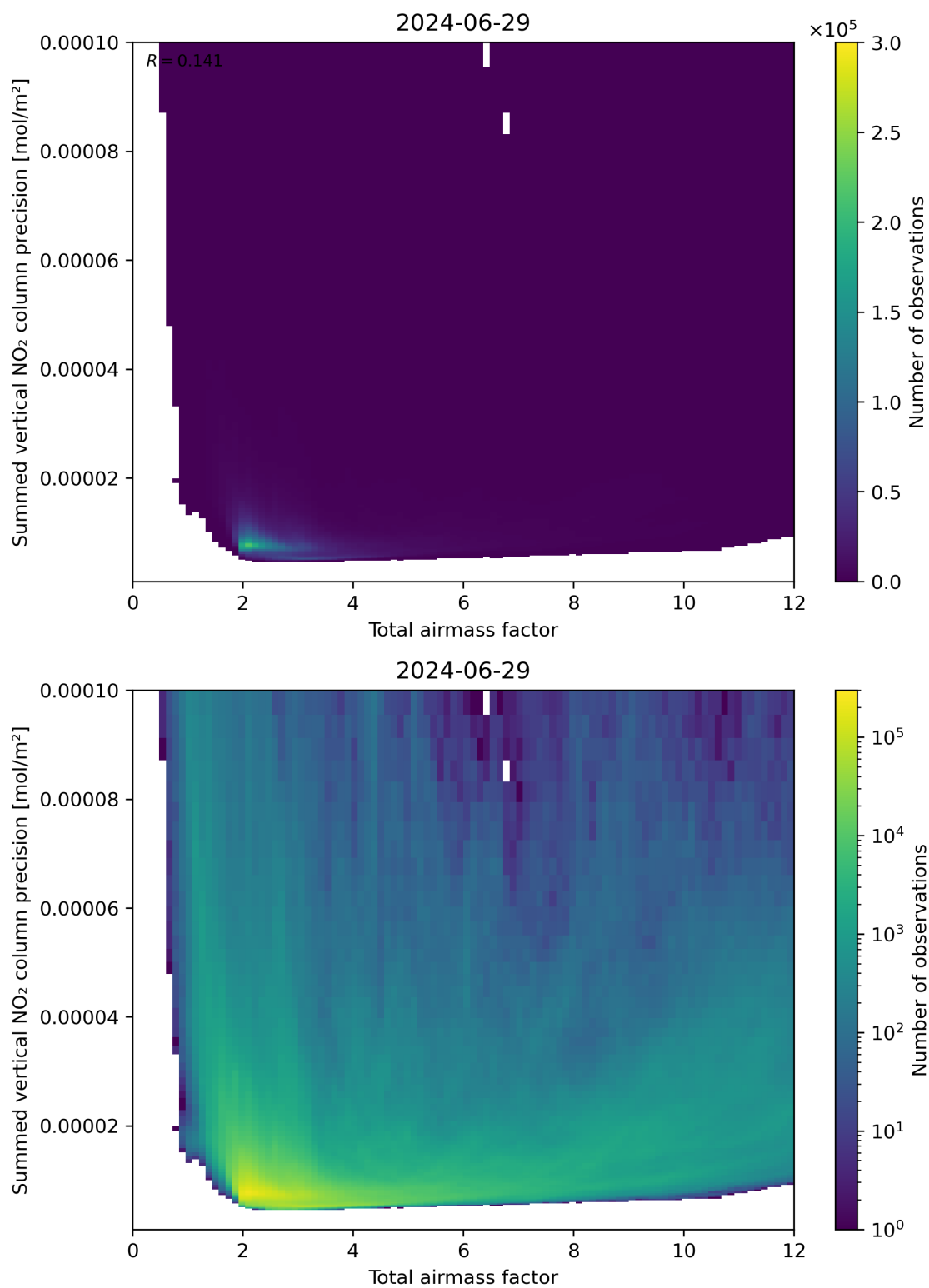
Figure 66: Scatter density plot of “Total airmass factor” against “Summed vertical NO 2 column precision” for 2024-06-29 to 2024-06-30.
