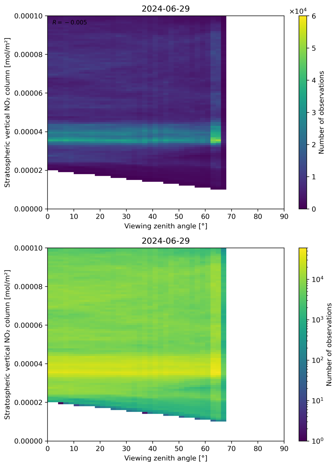
Figure 164: Scatter density plot of “Viewing zenith angle” against “Stratospheric vertical NO 2 column” for 2024-06-29 to 2024-06-30.
