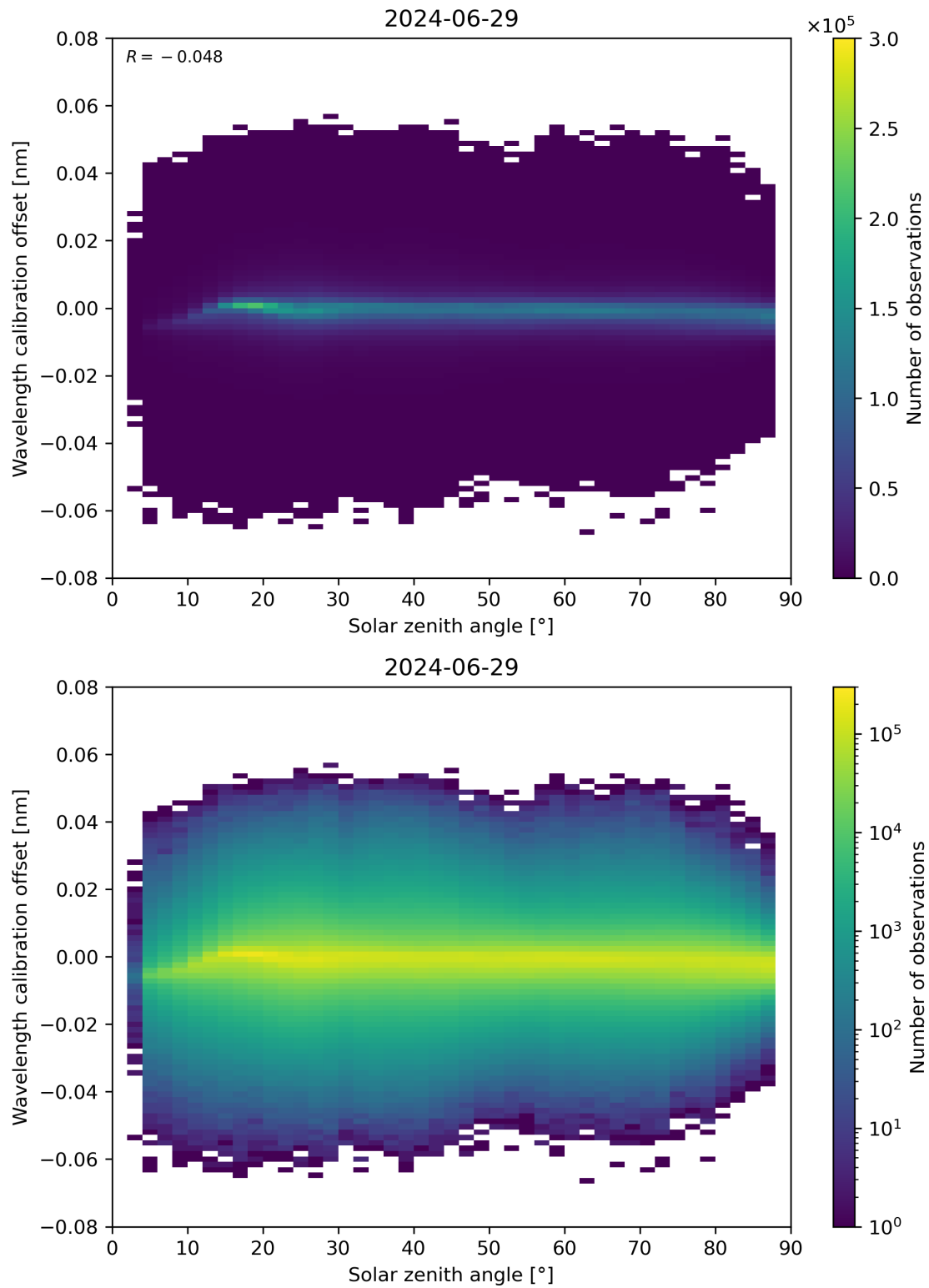
Figure 158: Scatter density plot of “Solar zenith angle” against “Wavelength calibration offset” for 2024-06-29 to 2024-06-30.
