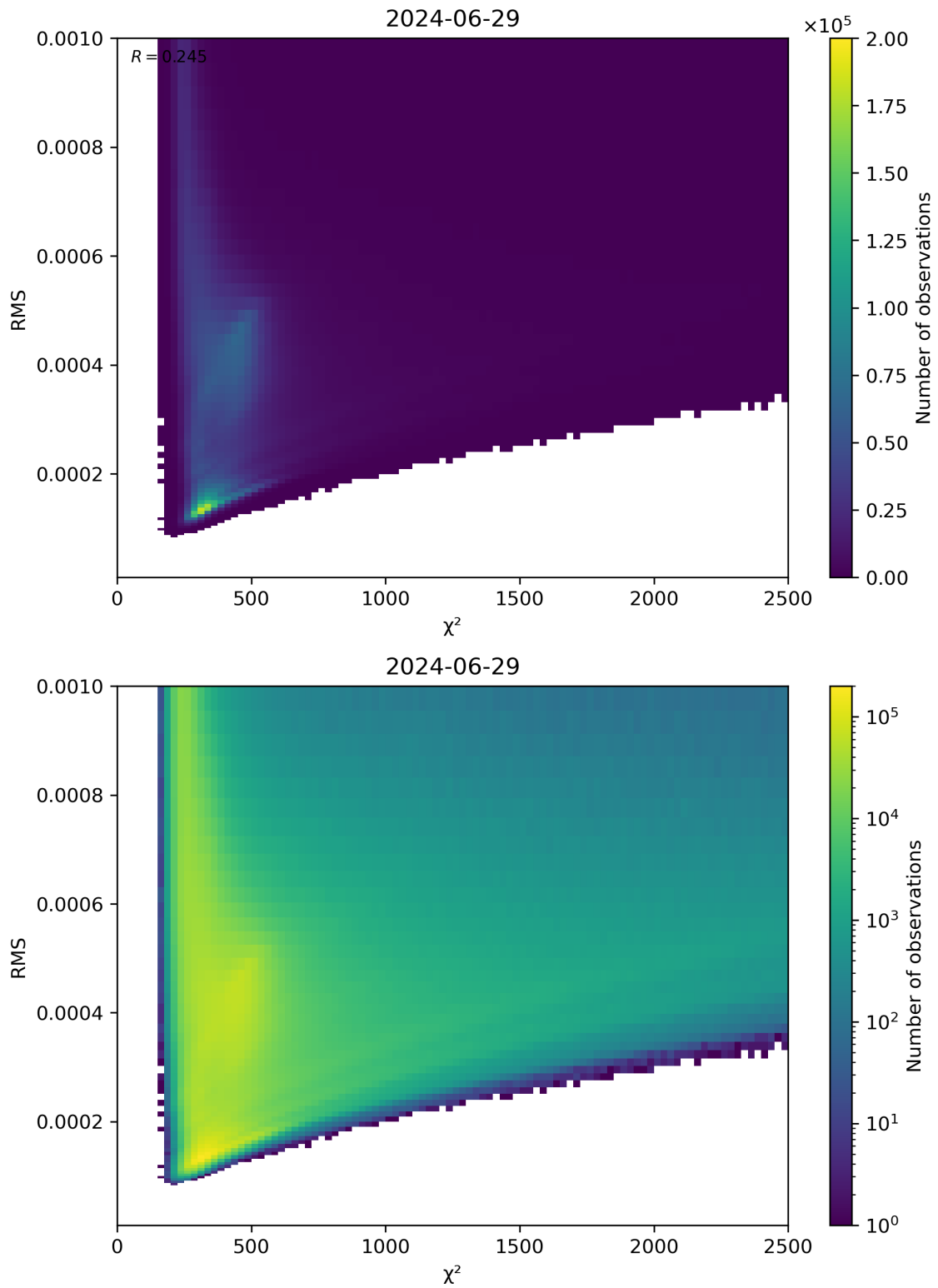
Figure 82: Scatter density plot of “ \chi^2 ” against “RMS” for 2024-06-29 to 2024-06-30.
