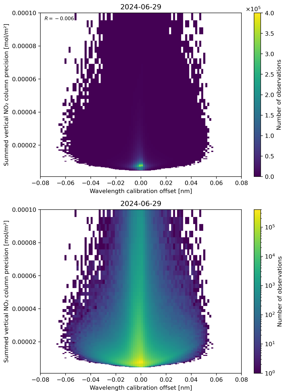
Figure 178: Scatter density plot of “Wavelength calibration offset” against “Summed vertical NO 2 column precision” for 2024-06-29 to 2024-06-30.
