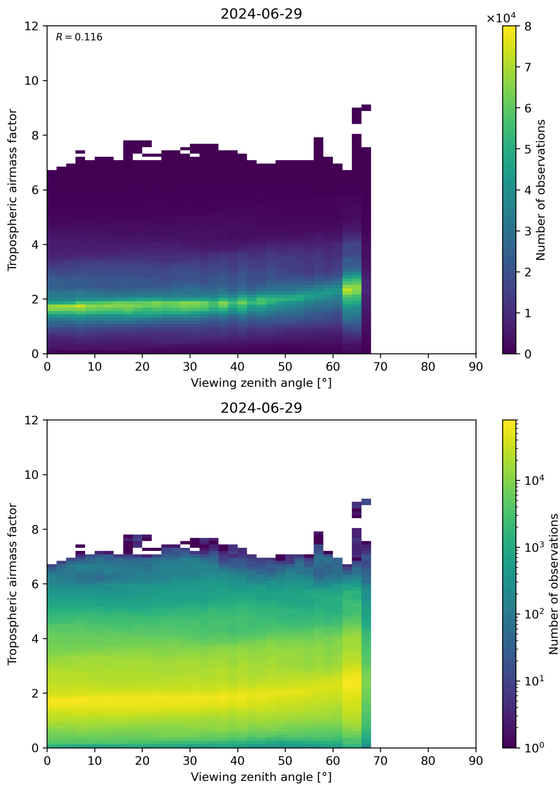
Figure 161: Scatter density plot of “Viewing zenith angle” against “Tropospheric airmass factor” for 2024-06-29 to 2024-06-30.
