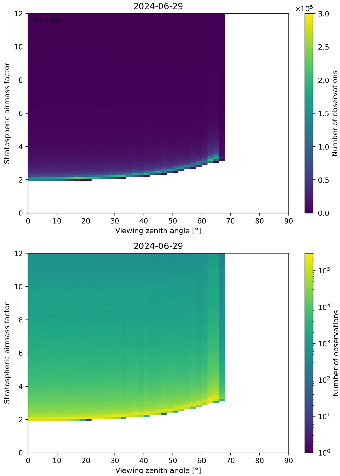
Figure 159: Scatter density plot of “Viewing zenith angle” against “Stratospheric airmass factor” for 2024-06-29 to 2024-06-30.
