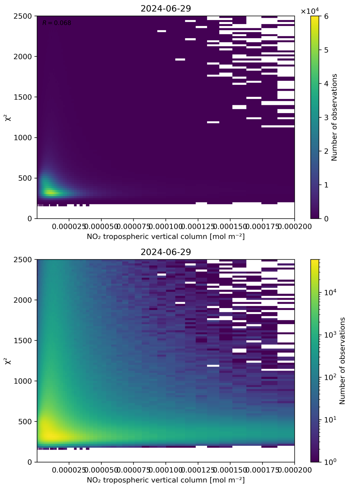
Figure 124: Scatter density plot of “NO 2 tropospheric vertical column” against “ \chi^2 ” for 2024-06-29 to 2024-06-30.
