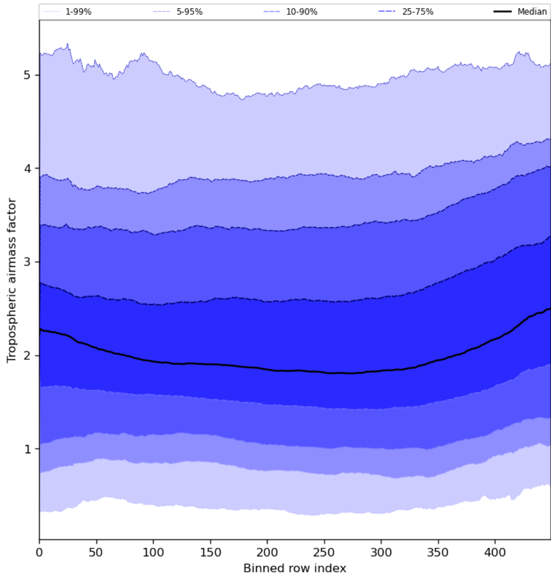
Figure 48: Along track statistics of “Tropospheric air mass factor” for 2024-06-29 to 2024-06-30
