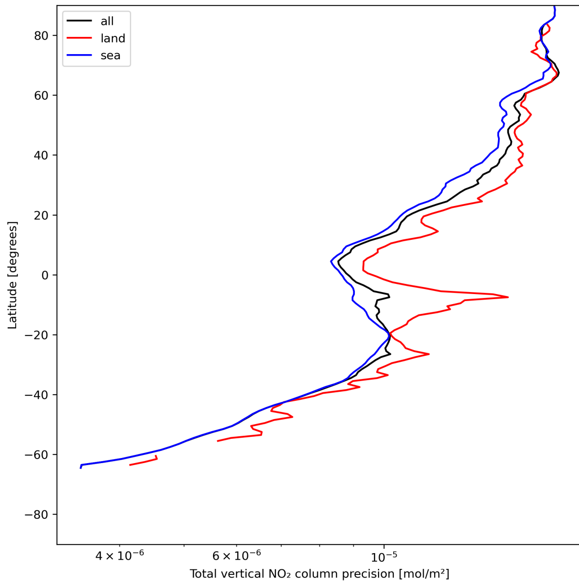
Figure 22: Zonal average of “Total vertical NO 2 column precision” for 2024-06-29 to 2024-06-30.
