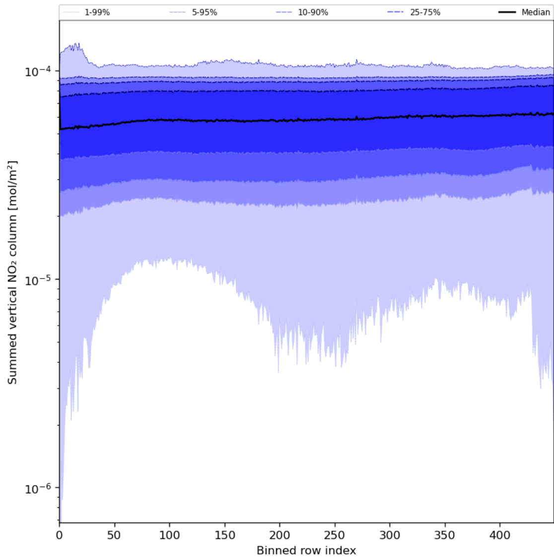
Figure 57: Along track statistics of “Summed vertical NO 2 column” for 2024-06-29 to 2024-06-30
