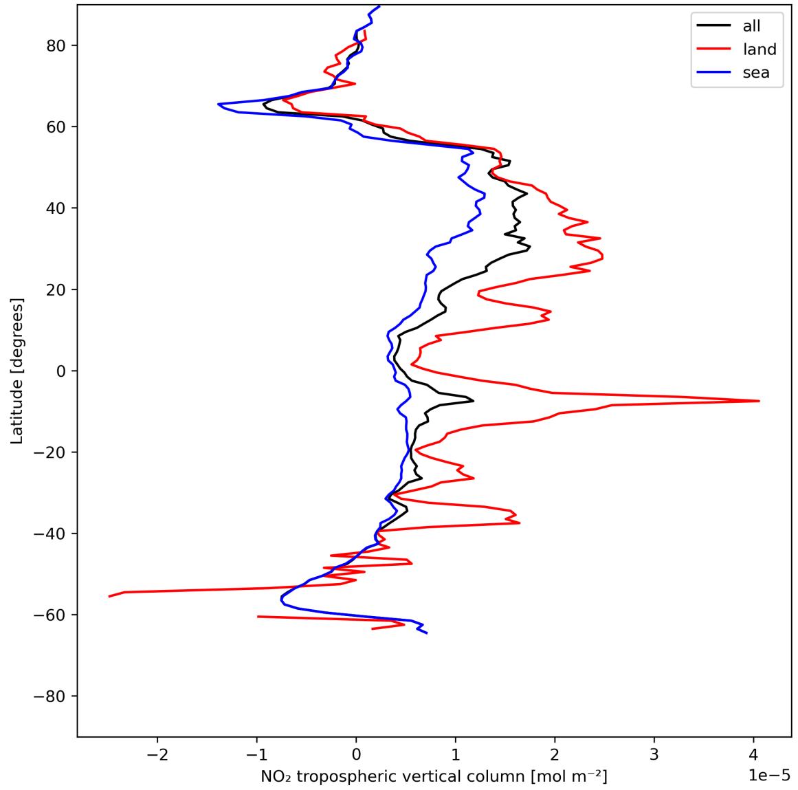
Figure 12: Zonal average of “NO 2 tropospheric vertical column” for 2024-06-29 to 2024-06-30.
