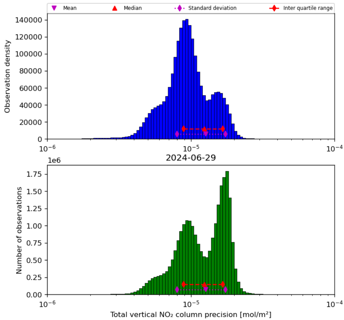
Figure 39: Histogram of “Total vertical NO 2 column precision” for 2024-06-29 to 2024-06-30
