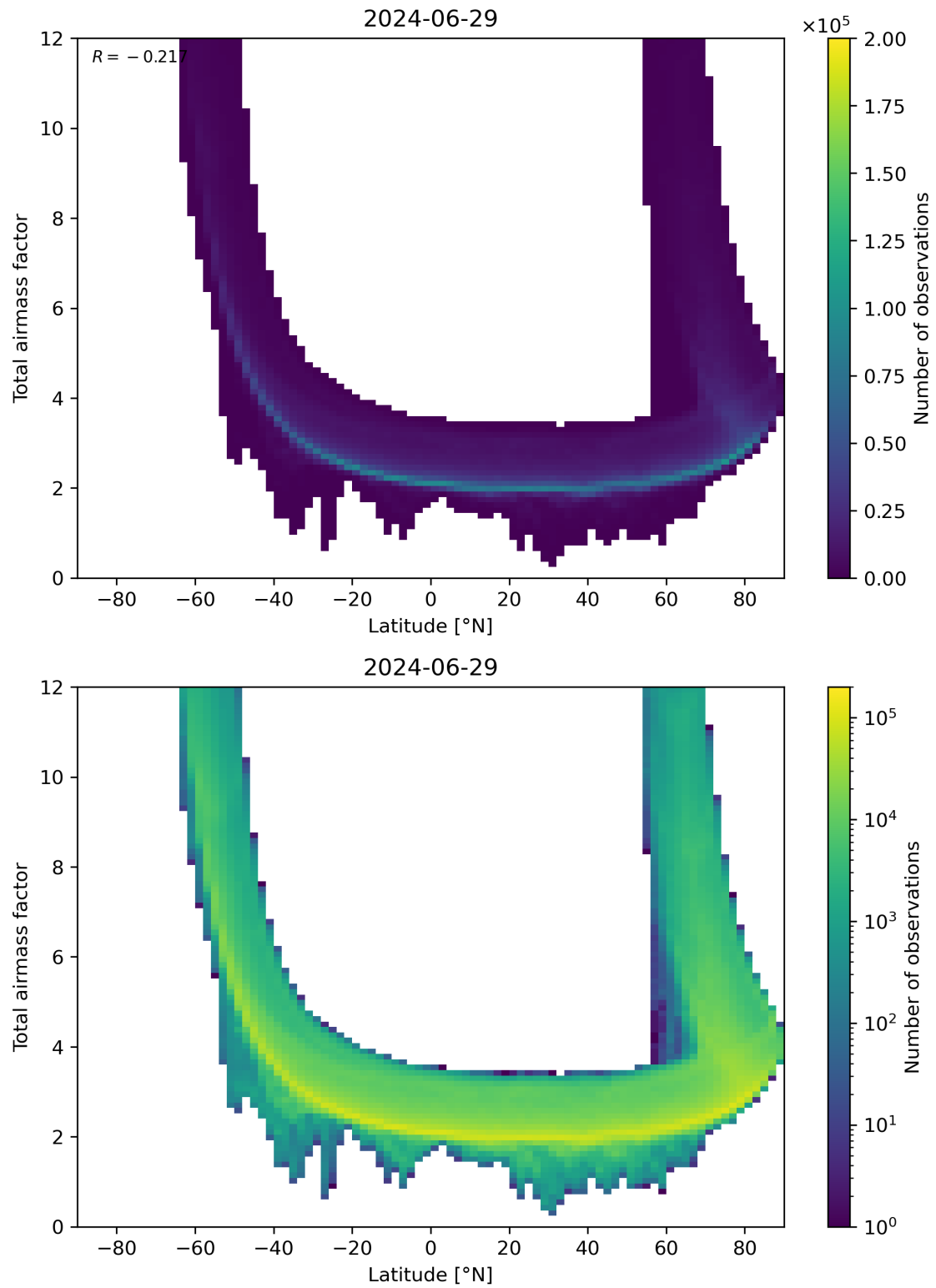
Figure 84: Scatter density plot of “Latitude” against “Total airmass factor” for 2024-06-29 to 2024-06-30.
