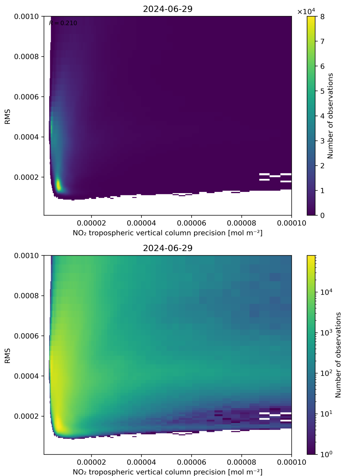
Figure 140: Scatter density plot of “NO 2 tropospheric vertical column precision” against “RMS” for 2024-06-29 to 2024-06-30.
