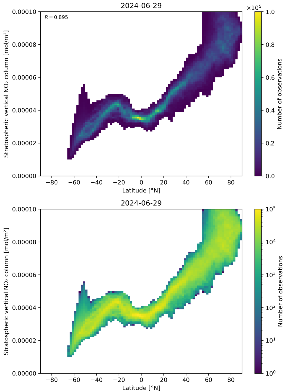
Figure 87: Scatter density plot of “Latitude” against “Stratospheric vertical NO 2 column” for 2024-06-29 to 2024-06-30.
