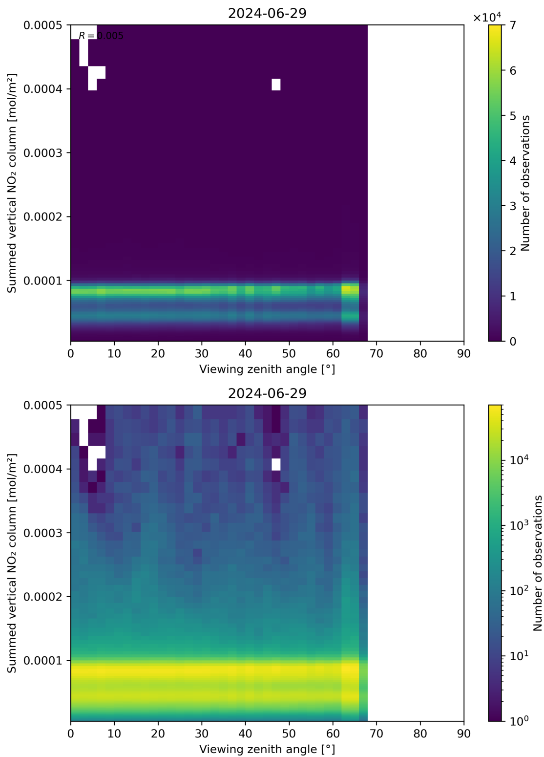
Figure 165: Scatter density plot of “Viewing zenith angle” against “Summed vertical NO 2 column” for 2024-06-29 to 2024-06-30.
