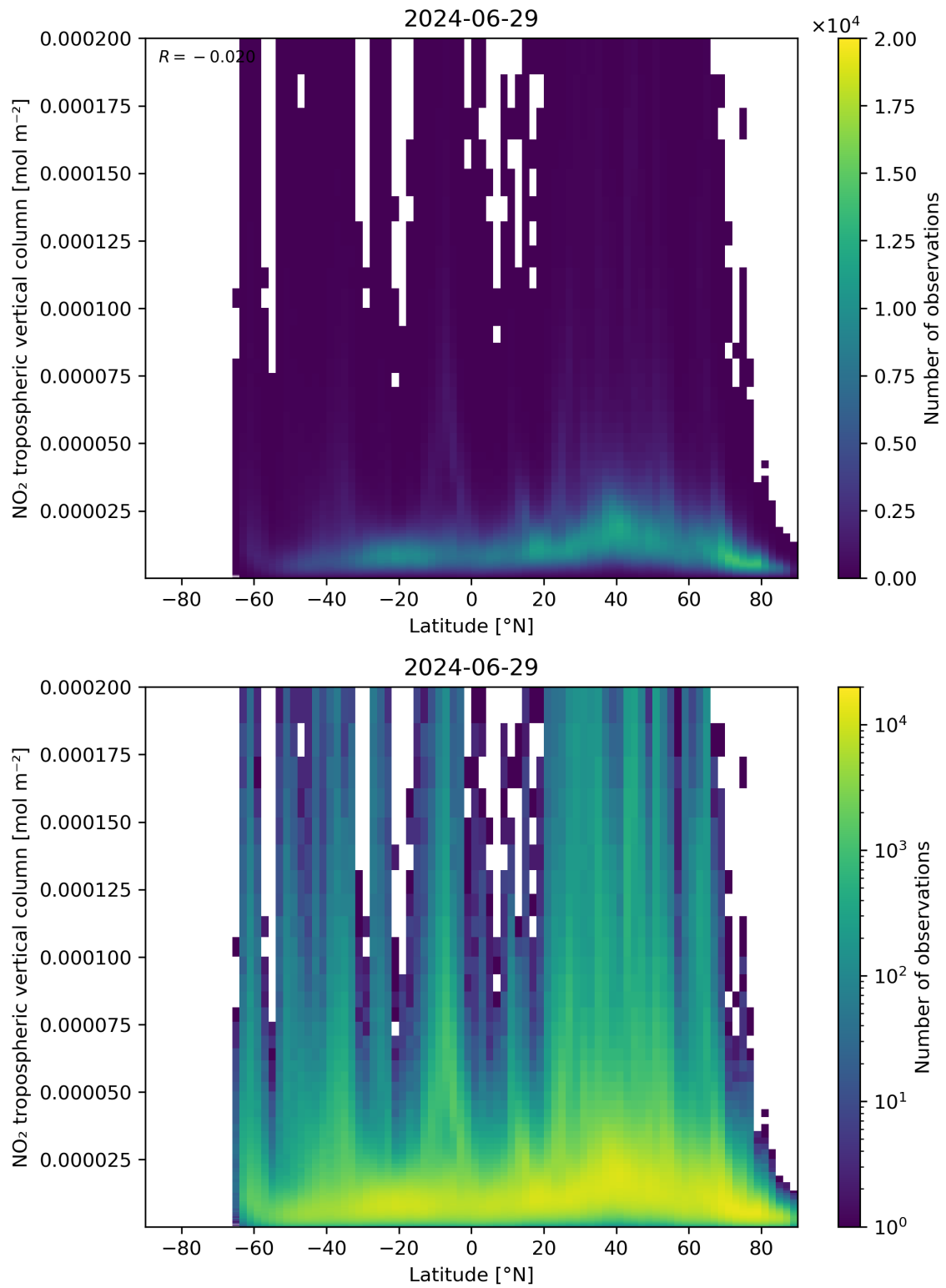
Figure 92: Scatter density plot of “Latitude” against “NO 2 tropospheric vertical column” for 2024-06-29 to 2024-06-30.
