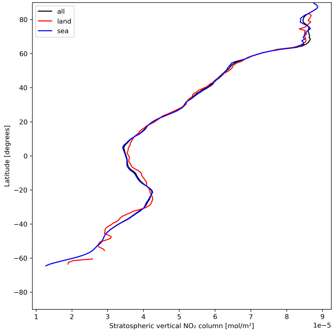
Figure 19: Zonal average of “Stratospheric vertical NO 2 column” for 2024-06-29 to 2024-06-30.
