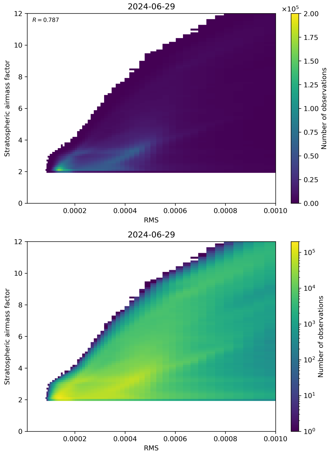
Figure 144: Scatter density plot of “RMS” against “Stratospheric airmass factor” for 2024-06-29 to 2024-06-30.
