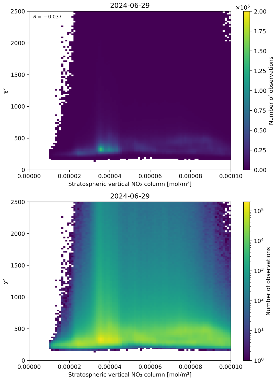
Figure 97: Scatter density plot of “Stratospheric vertical NO 2 column” against “ \chi^2 ” for 2024-06-29 to 2024-06-30.
