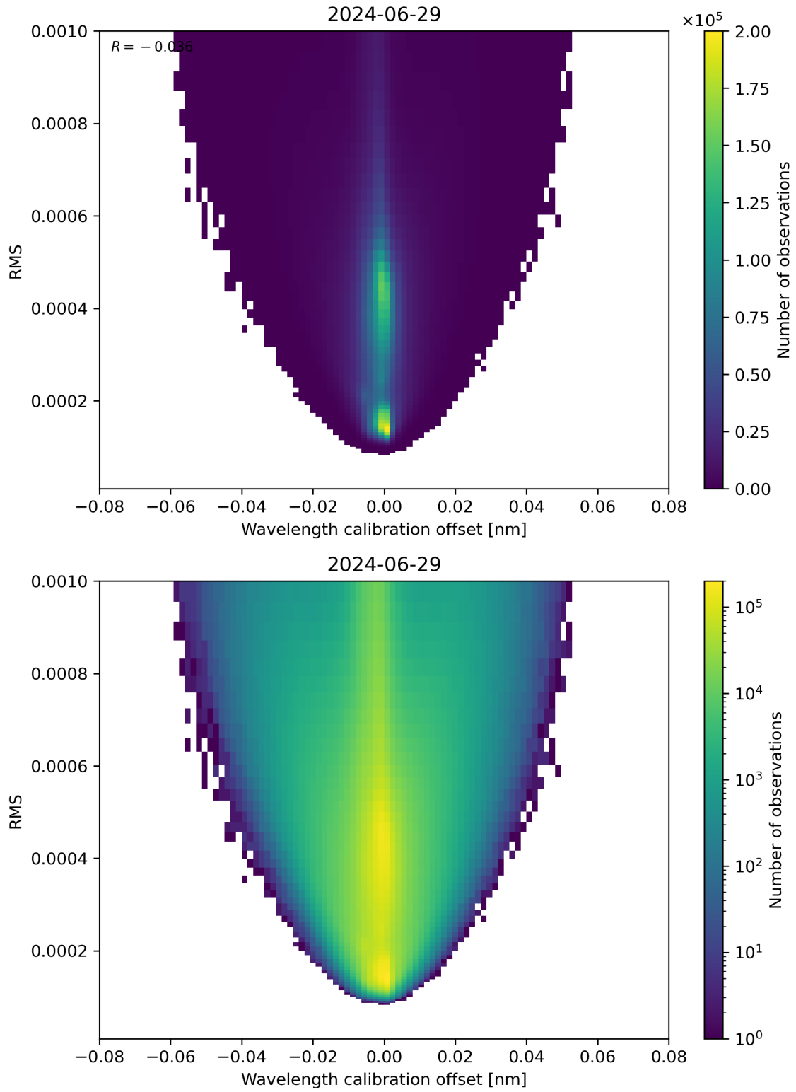
Figure 181: Scatter density plot of “Wavelength calibration offset” against “RMS” for 2024-06-29 to 2024-06-30.
