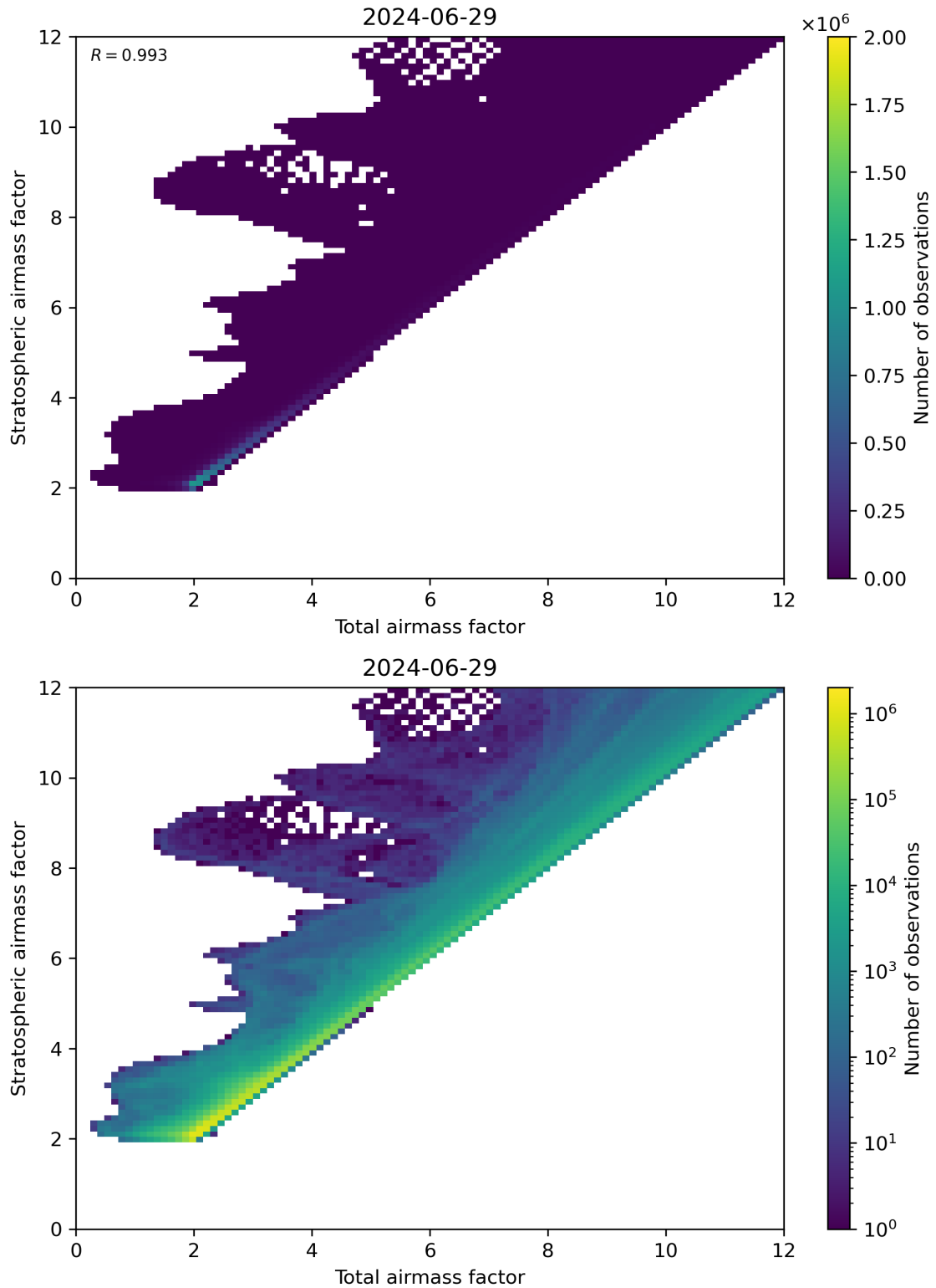
Figure 62: Scatter density plot of “Total airmass factor” against “Stratospheric airmass factor” for 2024-06-29 to 2024-06-30.
