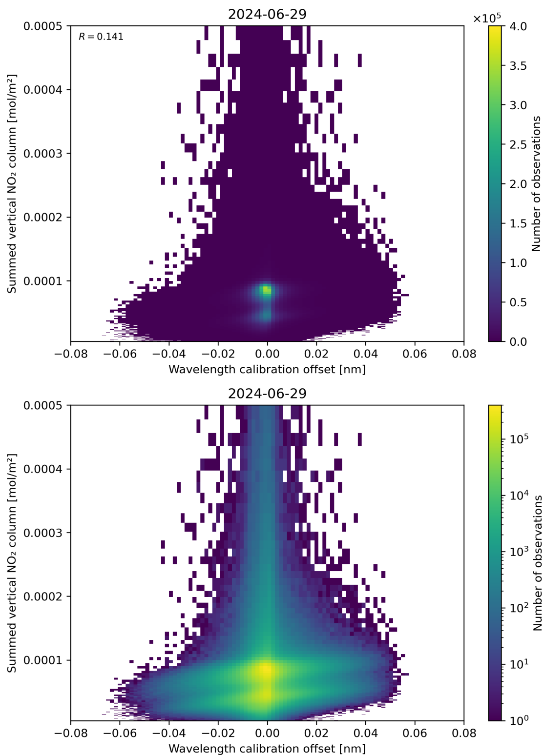
Figure 177: Scatter density plot of “Wavelength calibration offset” against “Summed vertical NO 2 column” for 2024-06-29 to 2024-06-30.
