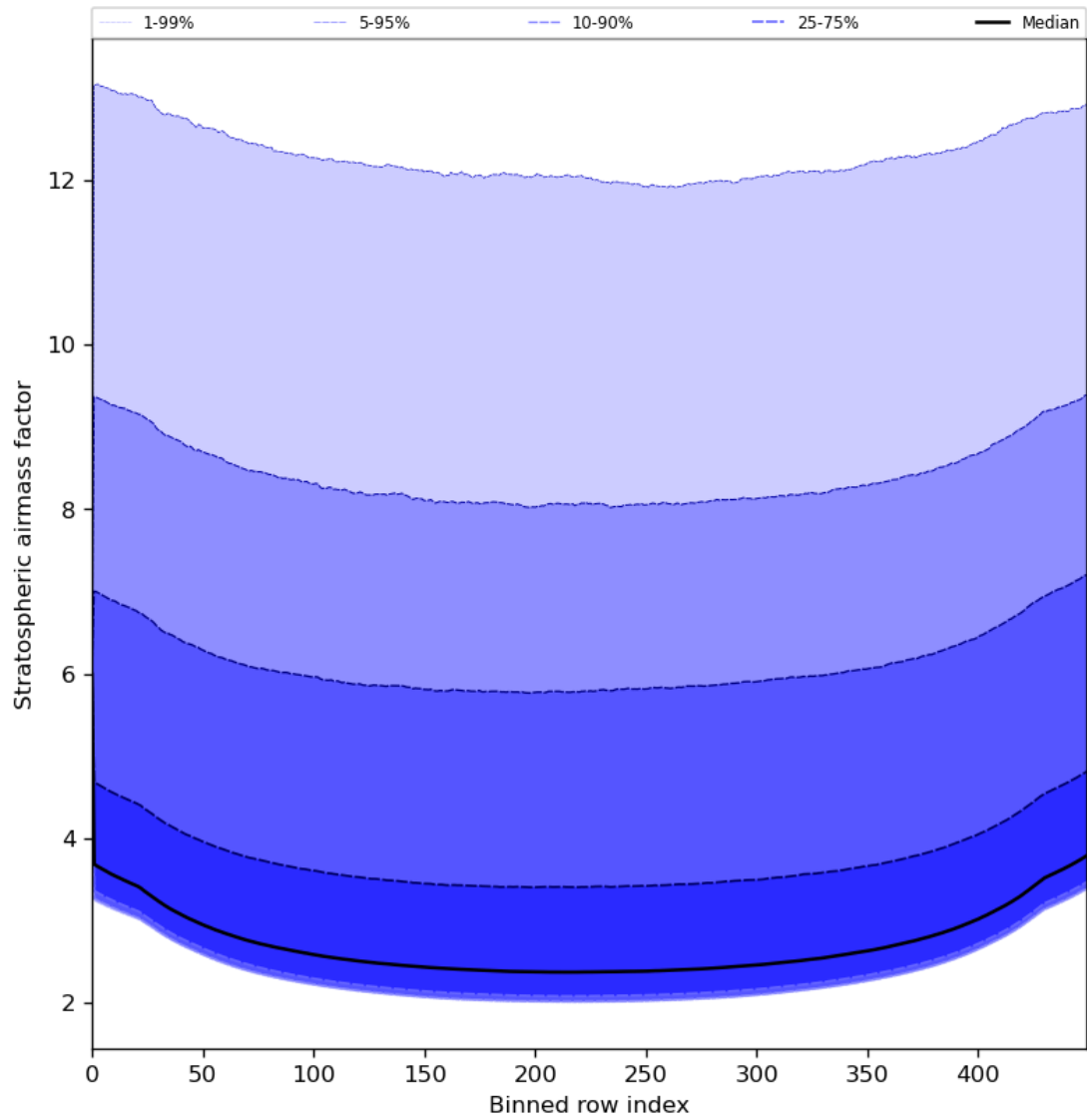
Figure 61: Along track statistics of “Stratospheric airmass factor” for 2024-06-29 to 2024-06-30
