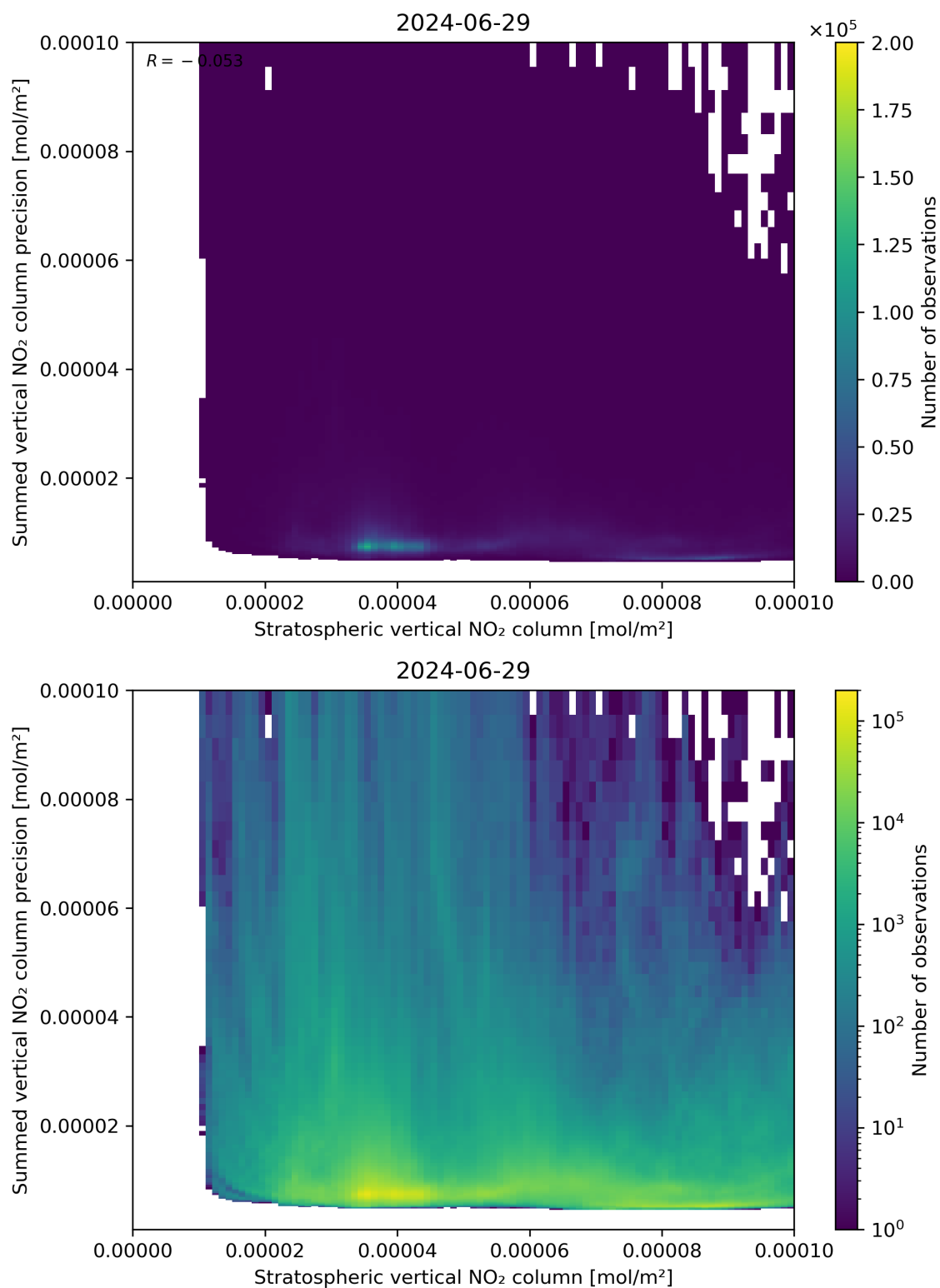
Figure 99: Scatter density plot of “Stratospheric vertical NO 2 column” against “Summed vertical NO 2 column precision” for 2024-06-29 to 2024-06-30.
