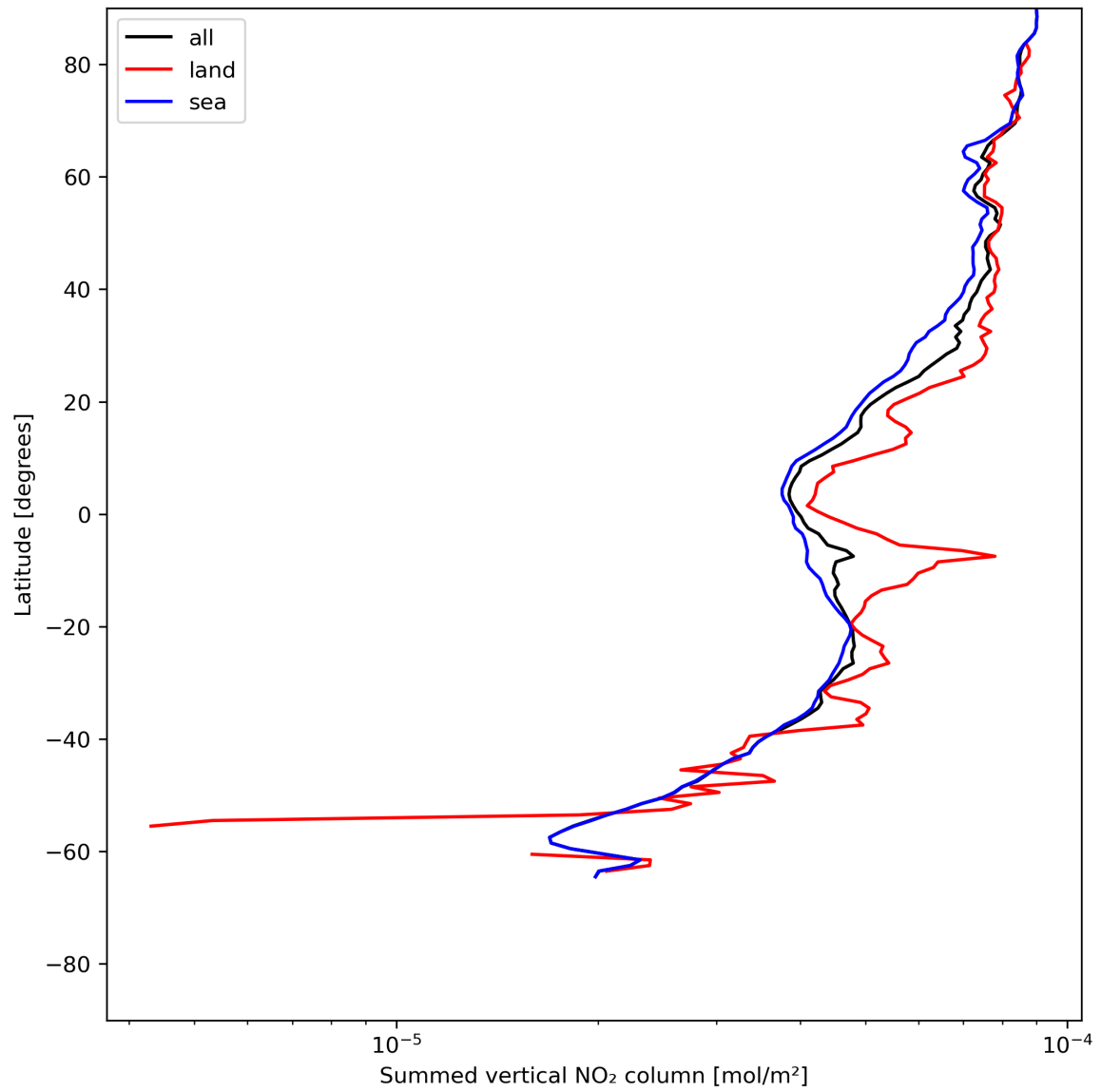
Figure 23: Zonal average of “Summed vertical NO 2 column” for 2024-06-29 to 2024-06-30.
