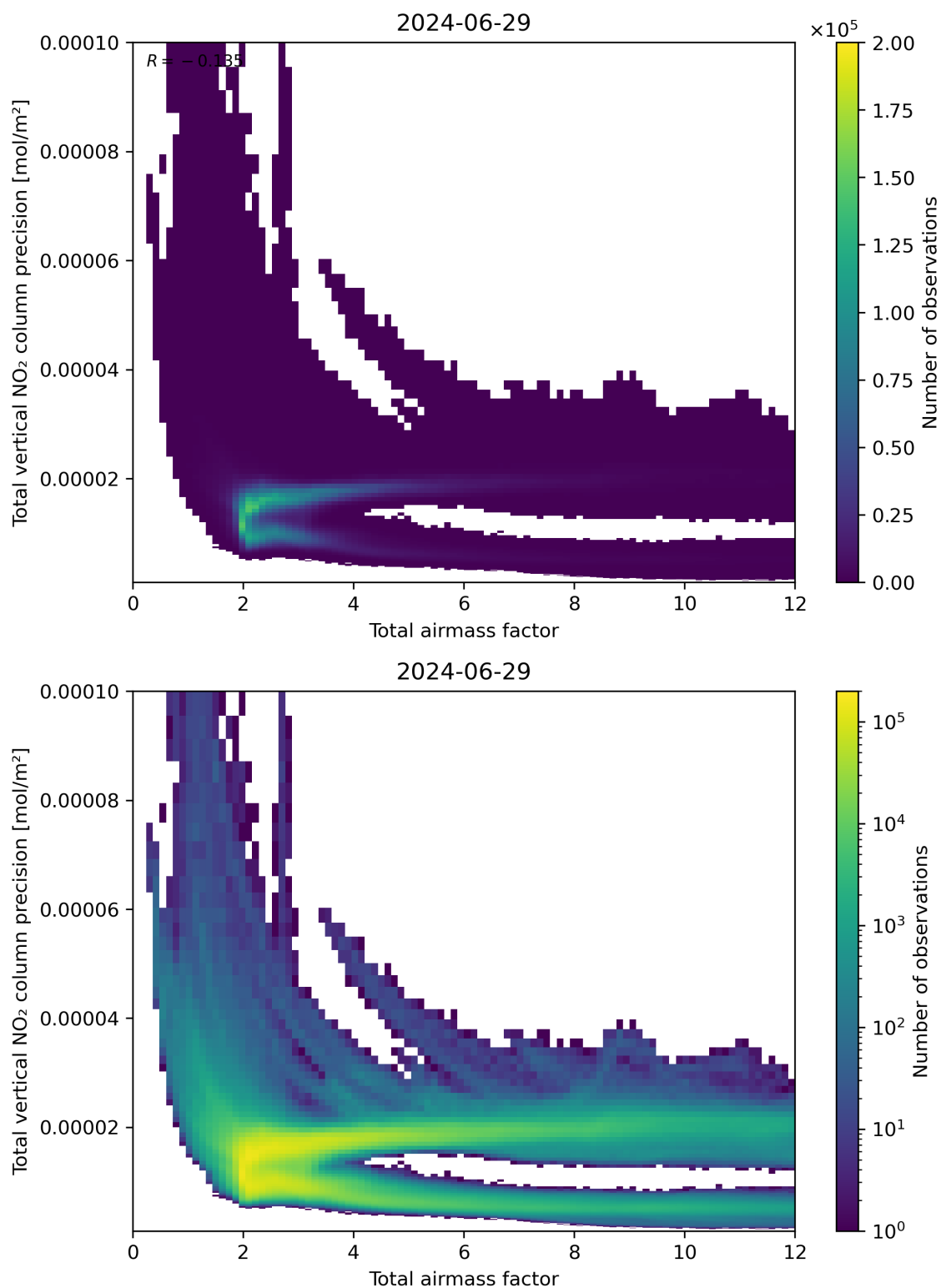
Figure 68: Scatter density plot of “Total airmass factor” against “Total vertical NO 2 column precision” for 2024-06-29 to 2024-06-30.
