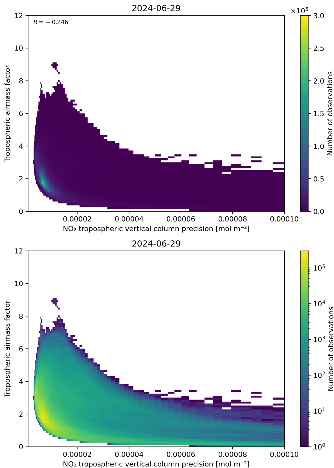
Figure 133: Scatter density plot of “NO 2 tropospheric vertical column precision” against “Tropospheric airmass factor” for 2024-06-29 to 2024-06-30.
