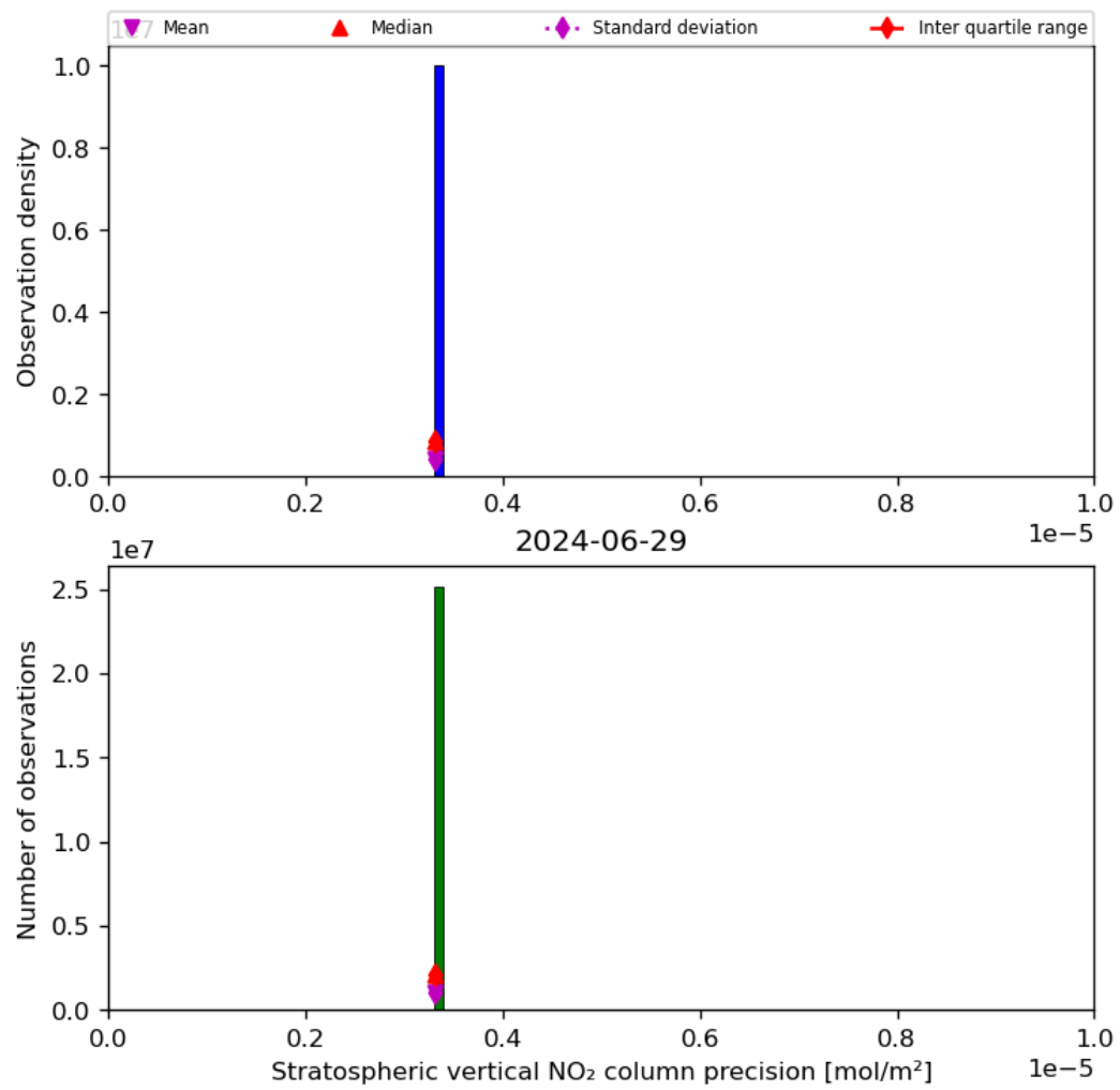
Figure 37: Histogram of “Stratospheric vertical NO 2 column precision” for 2024-06-29 to 2024-06-30
