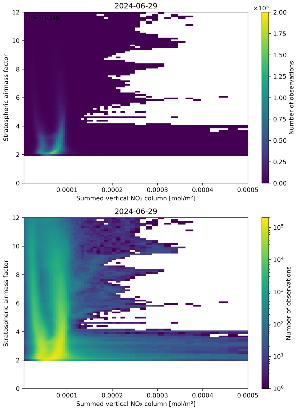
Figure 103: Scatter density plot of “Summed vertical NO 2 column” against “Stratospheric air mass factor” for 2024-06-29 to 2024-06-30.
