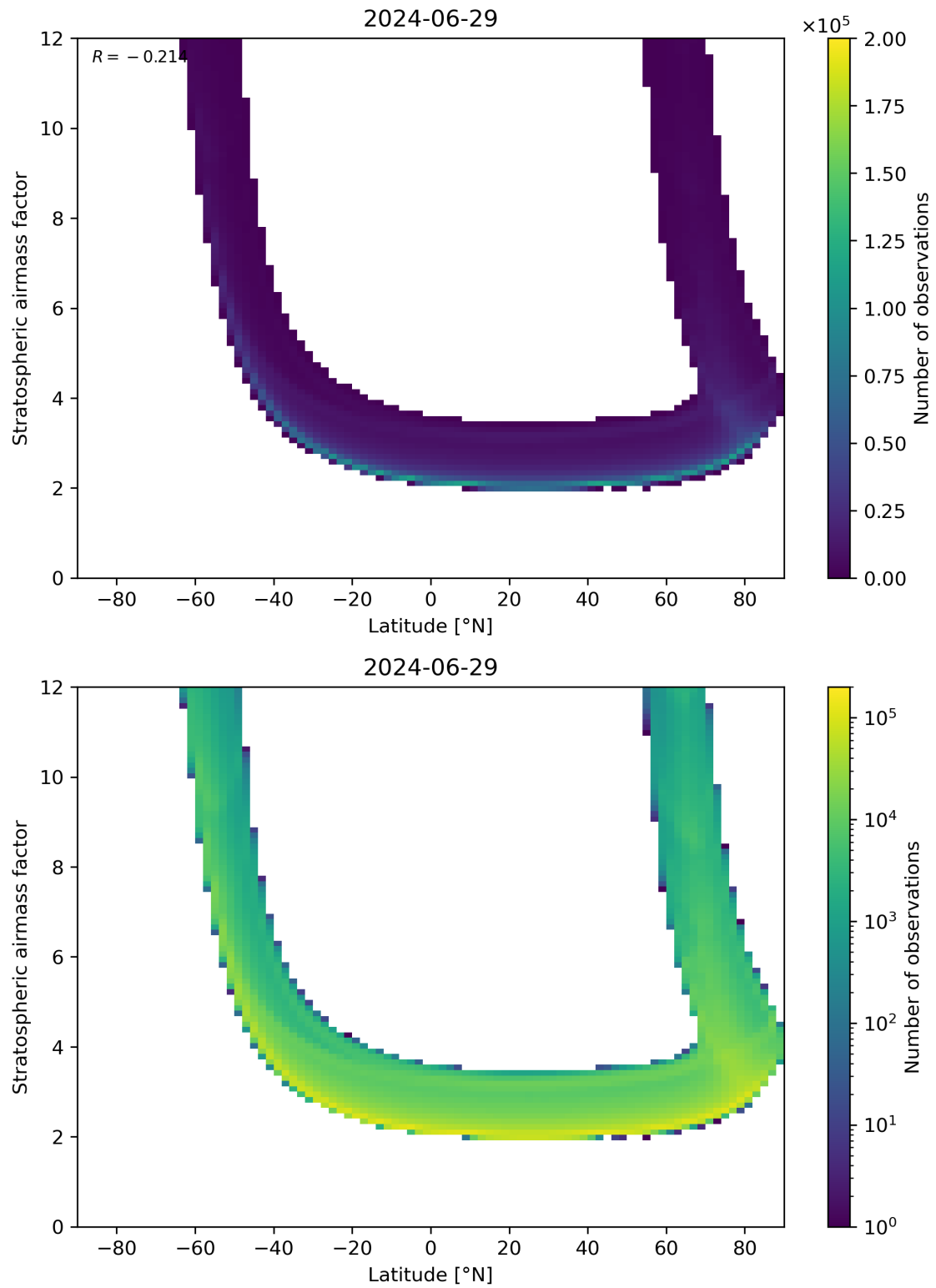
Figure 83: Scatter density plot of “Latitude” against “Stratospheric air mass factor” for 2024-06-29 to 2024-06-30.
