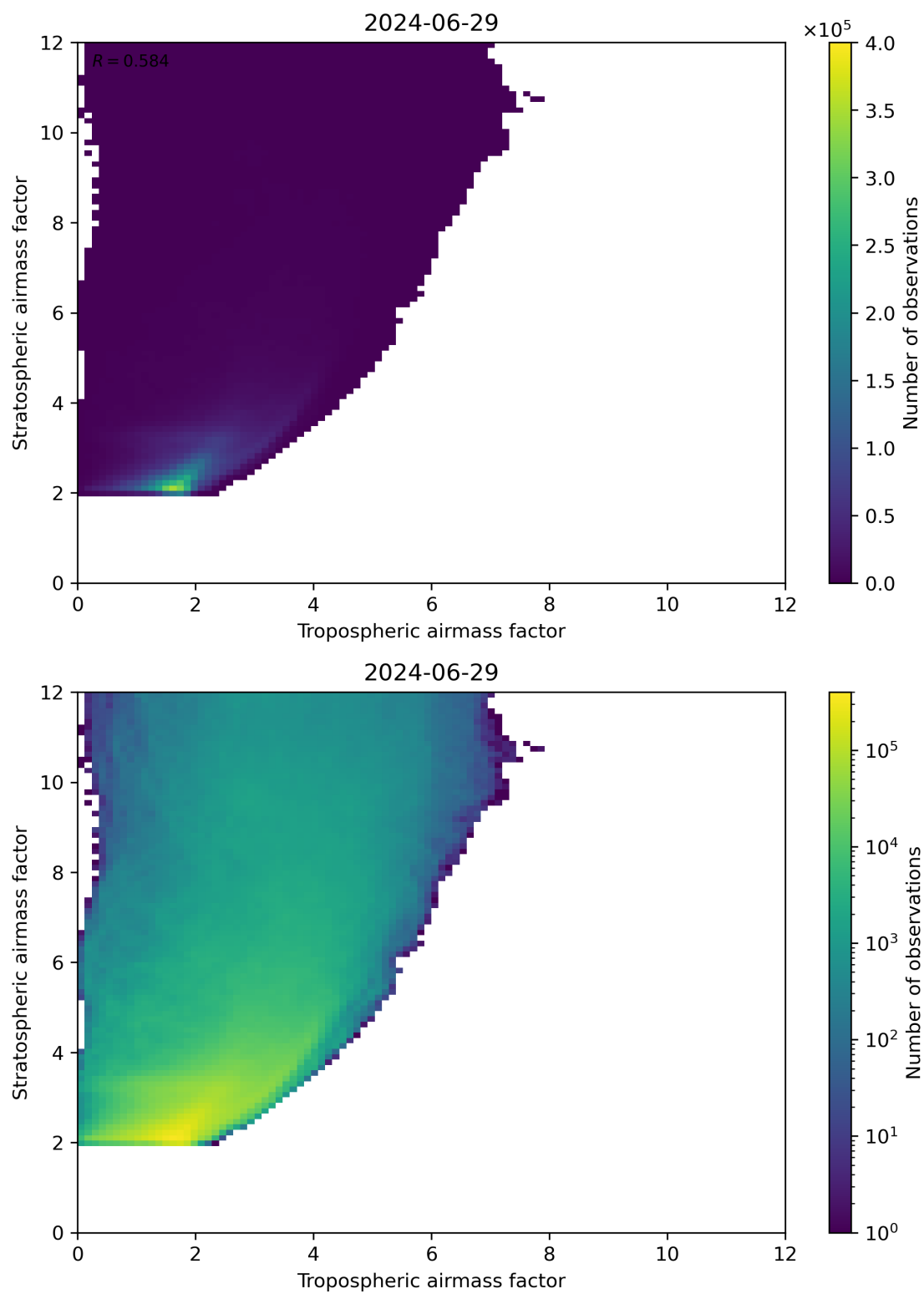
Figure 71: Scatter density plot of “Tropospheric airmass factor” against “Stratospheric airmass factor” for 2024-06-29 to 2024-06-30.
