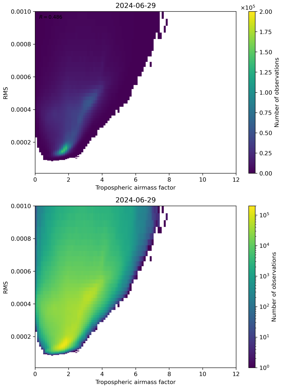
Figure 79: Scatter density plot of “Tropospheric airmass factor” against “RMS” for 2024-06-29 to 2024-06-30.
