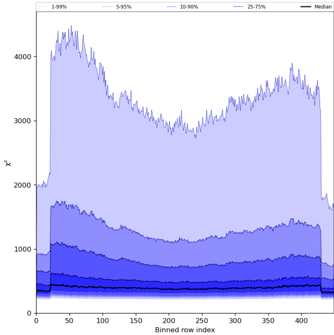
Figure 59: Along track statistics of “ \chi^2 ” for 2024-06-29 to 2024-06-30
