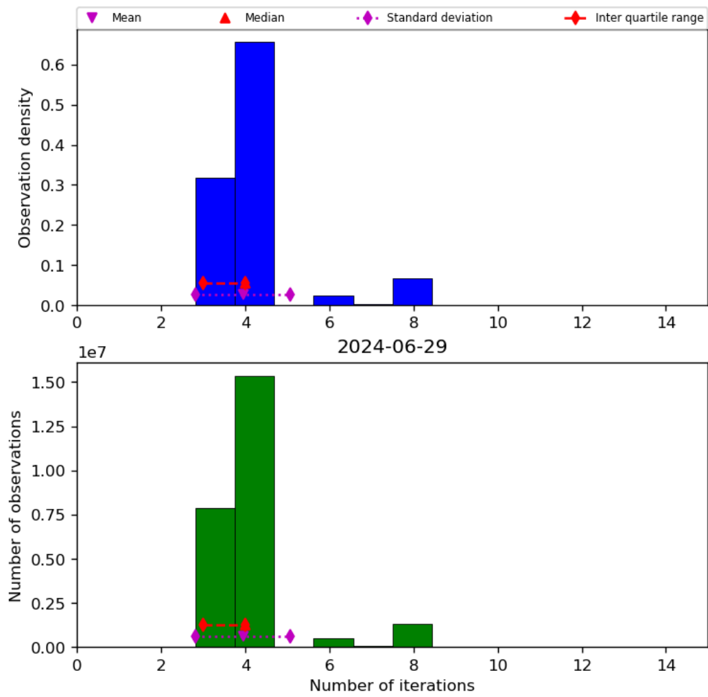
Figure 34: Histogram of “Number of iterations” for 2024-06-29 to 2024-06-30
