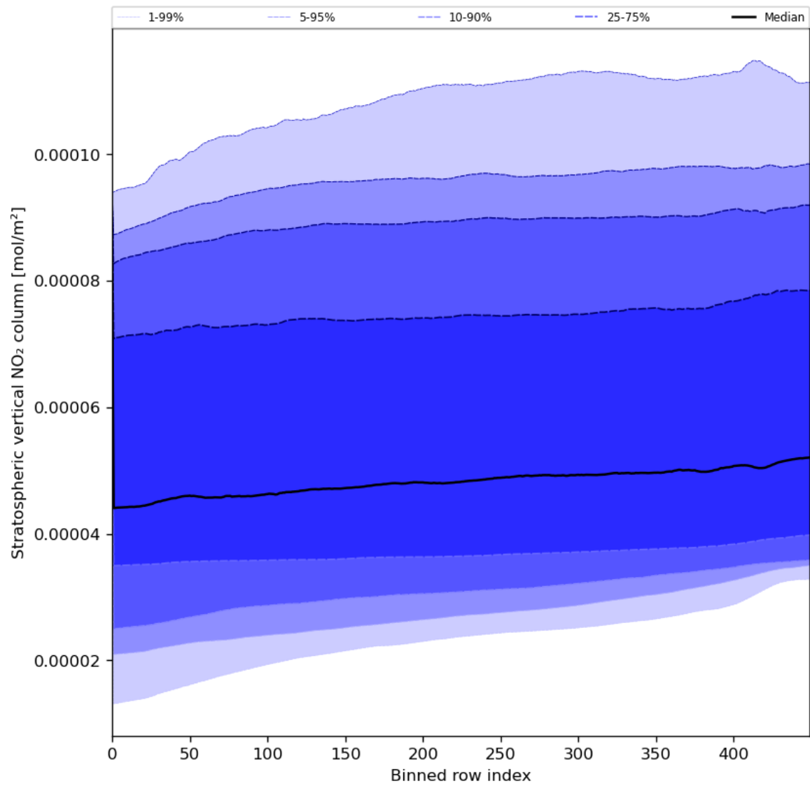
Figure 53: Along track statistics of “Stratospheric vertical NO 2 column” for 2024-06-29 to 2024-06-30
