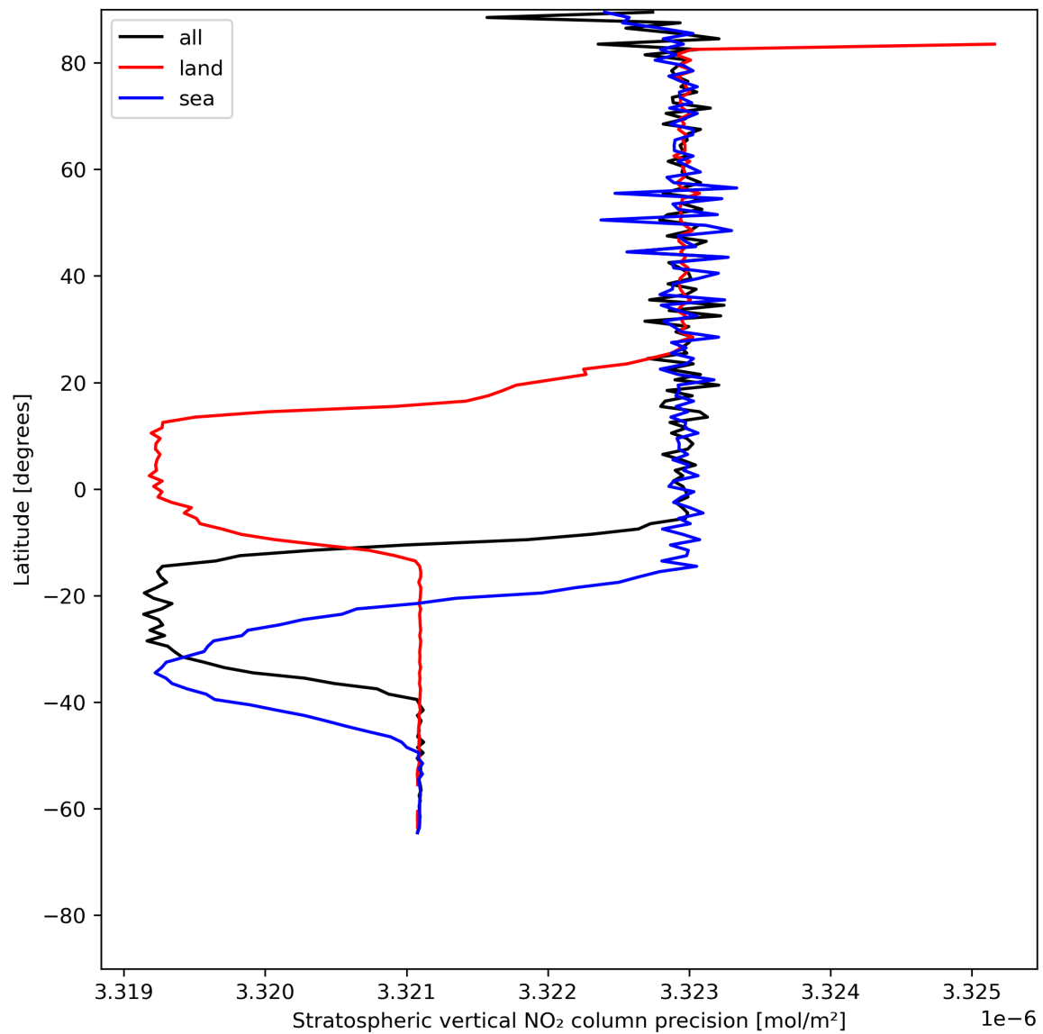
Figure 20: Zonal average of “Stratospheric vertical NO 2 column precision” for 2024-06-29 to 2024-06-30.
