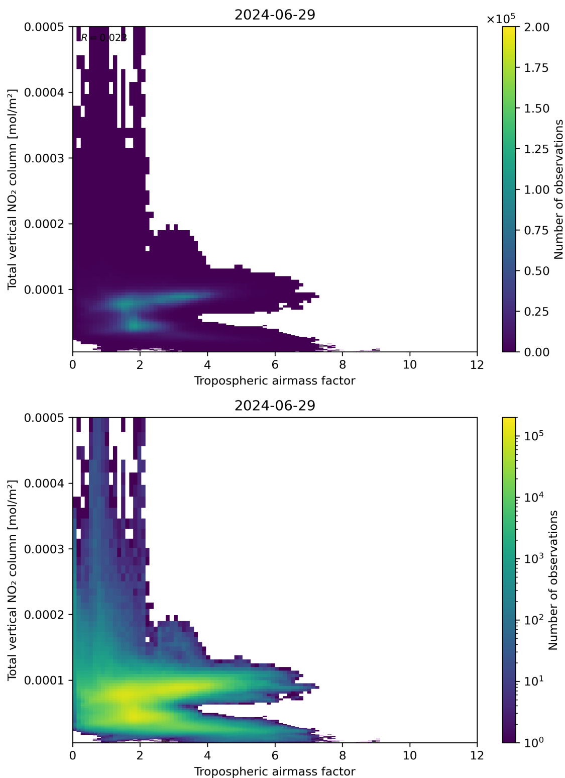
Figure 77: Scatter density plot of “Tropospheric airmass factor” against “Total vertical NO 2 column” for 2024-06-29 to 2024-06-30.
