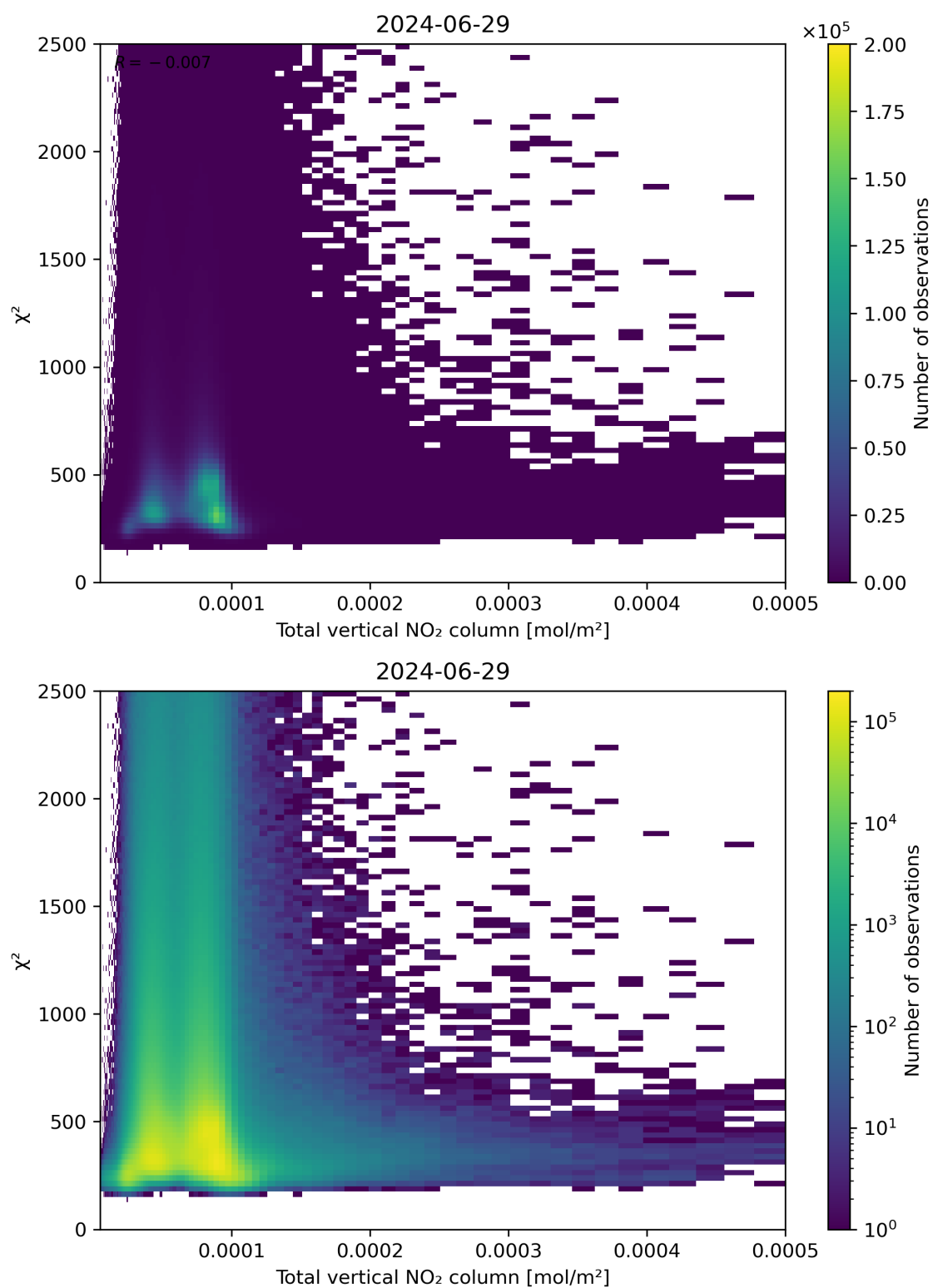
Figure 111: Scatter density plot of “Total vertical NO 2 column” against “ \chi^2 ” for 2024-06-29 to 2024-06-30.
