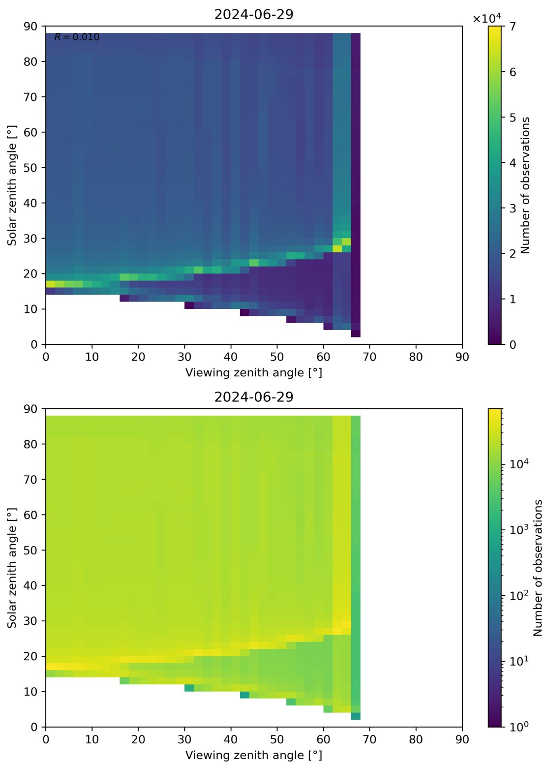
Figure 172: Scatter density plot of “Viewing zenith angle” against “Solar zenith angle” for 2024-06-29 to 2024-06-30.
