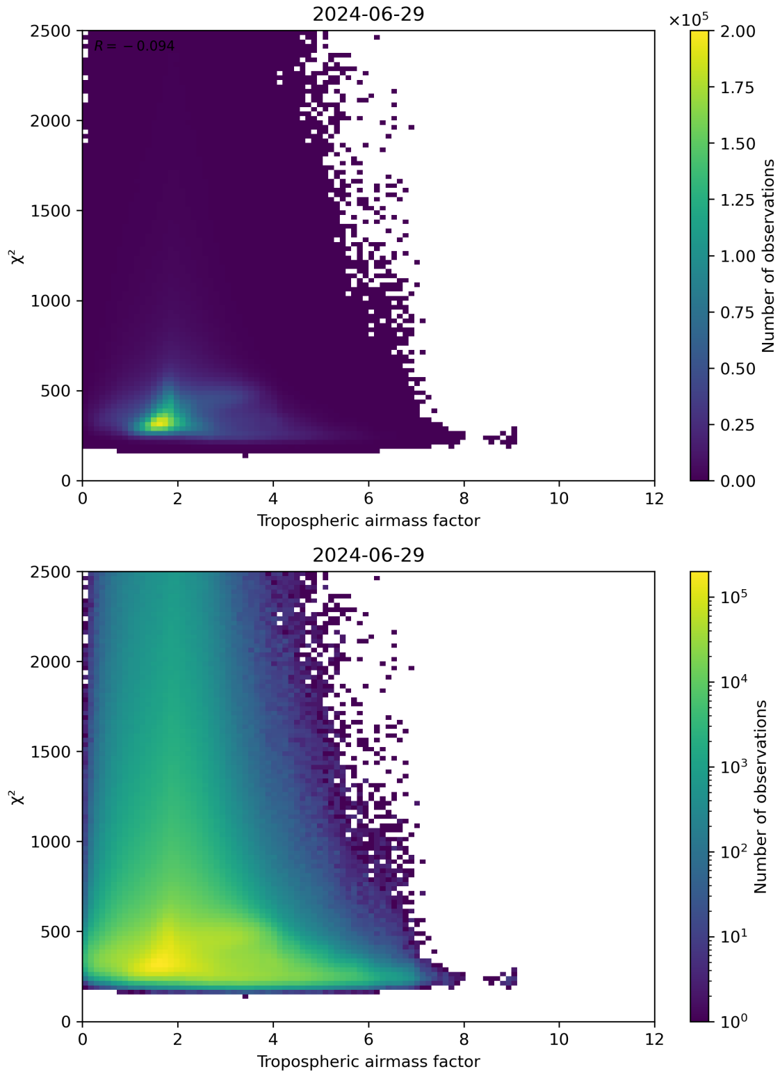
Figure 73: Scatter density plot of “Tropospheric airmass factor” against “ \chi^2 ” for 2024-06-29 to 2024-06-30.
