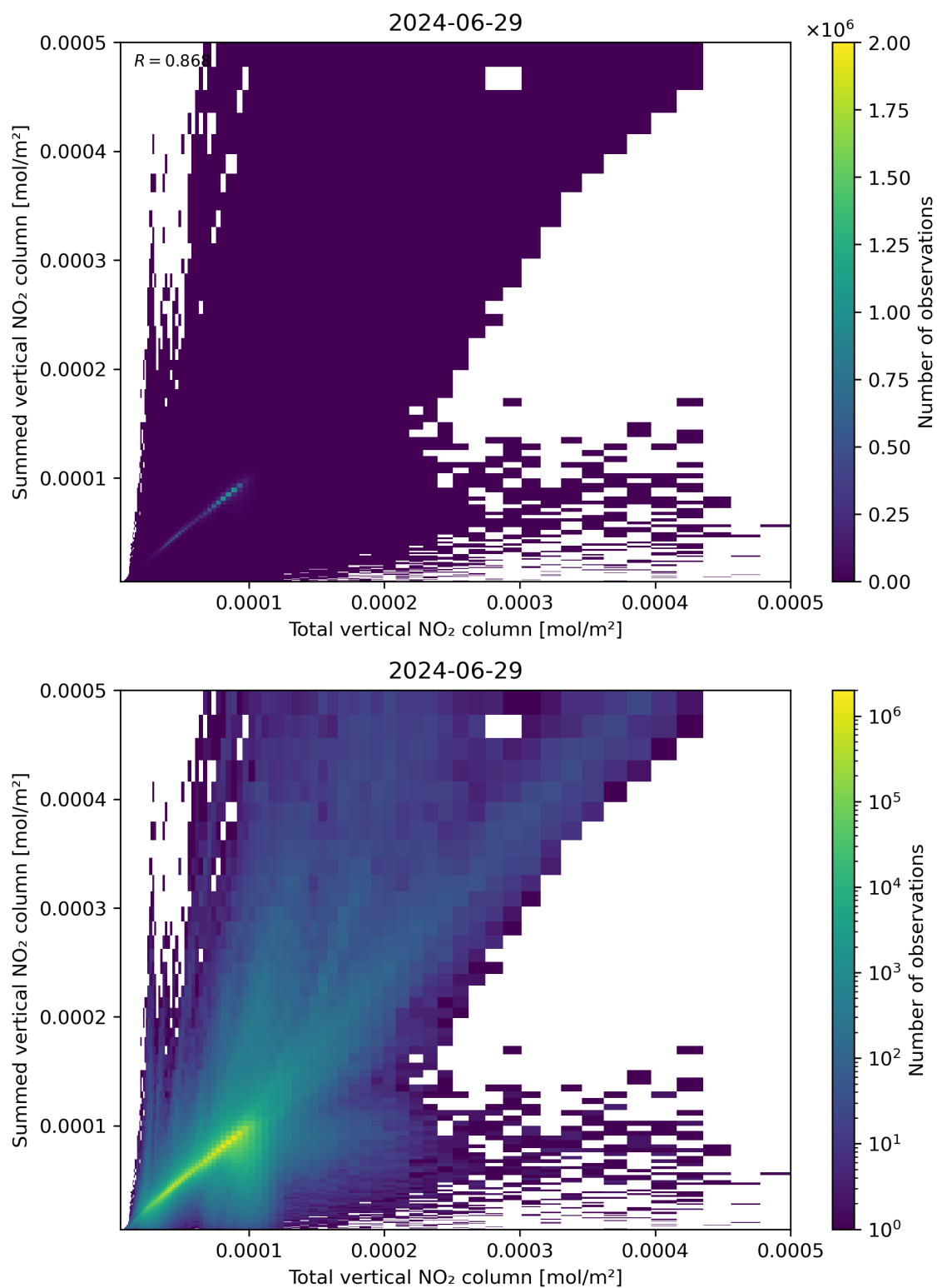
Figure 112: Scatter density plot of “Total vertical NO 2 column” against “Summed vertical NO 2 column” for 2024-06-29 to 2024-06-30.
