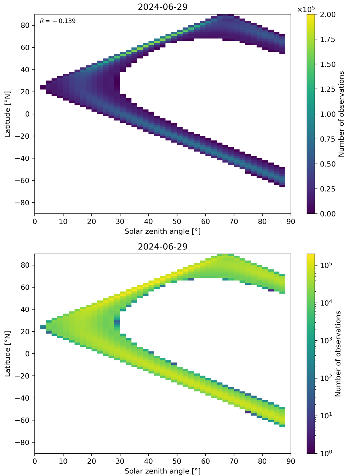
Figure 149: Scatter density plot of “Solar zenith angle” against “Latitude” for 2024-06-29 to 2024-06-30.
