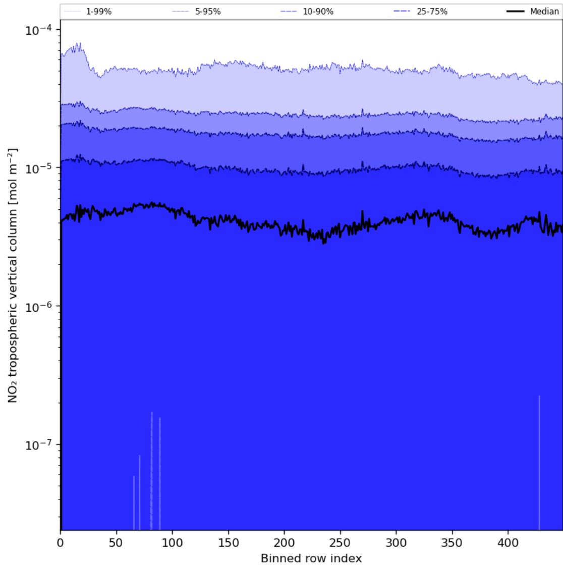
Figure 46: Along track statistics of “NO 2 tropospheric vertical column” for 2024-06-29 to 2024-06-30
