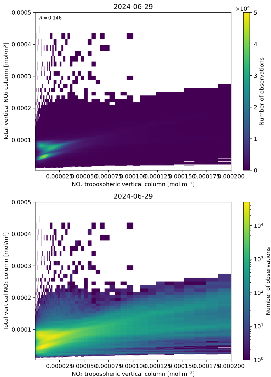
Figure 128: Scatter density plot of “NO 2 tropospheric vertical column” against “Total vertical NO 2 column” for 2024-06-29 to 2024-06-30.
