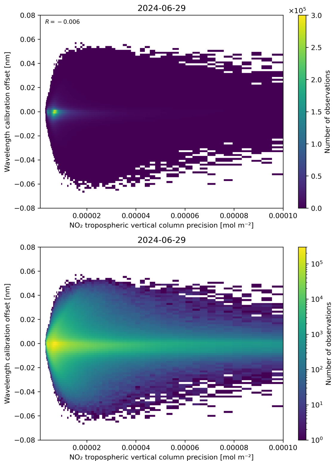
Figure 141: Scatter density plot of “NO 2 tropospheric vertical column precision” against “Wavelength calibration offset” for 2024-06-29 to 2024-06-30.
