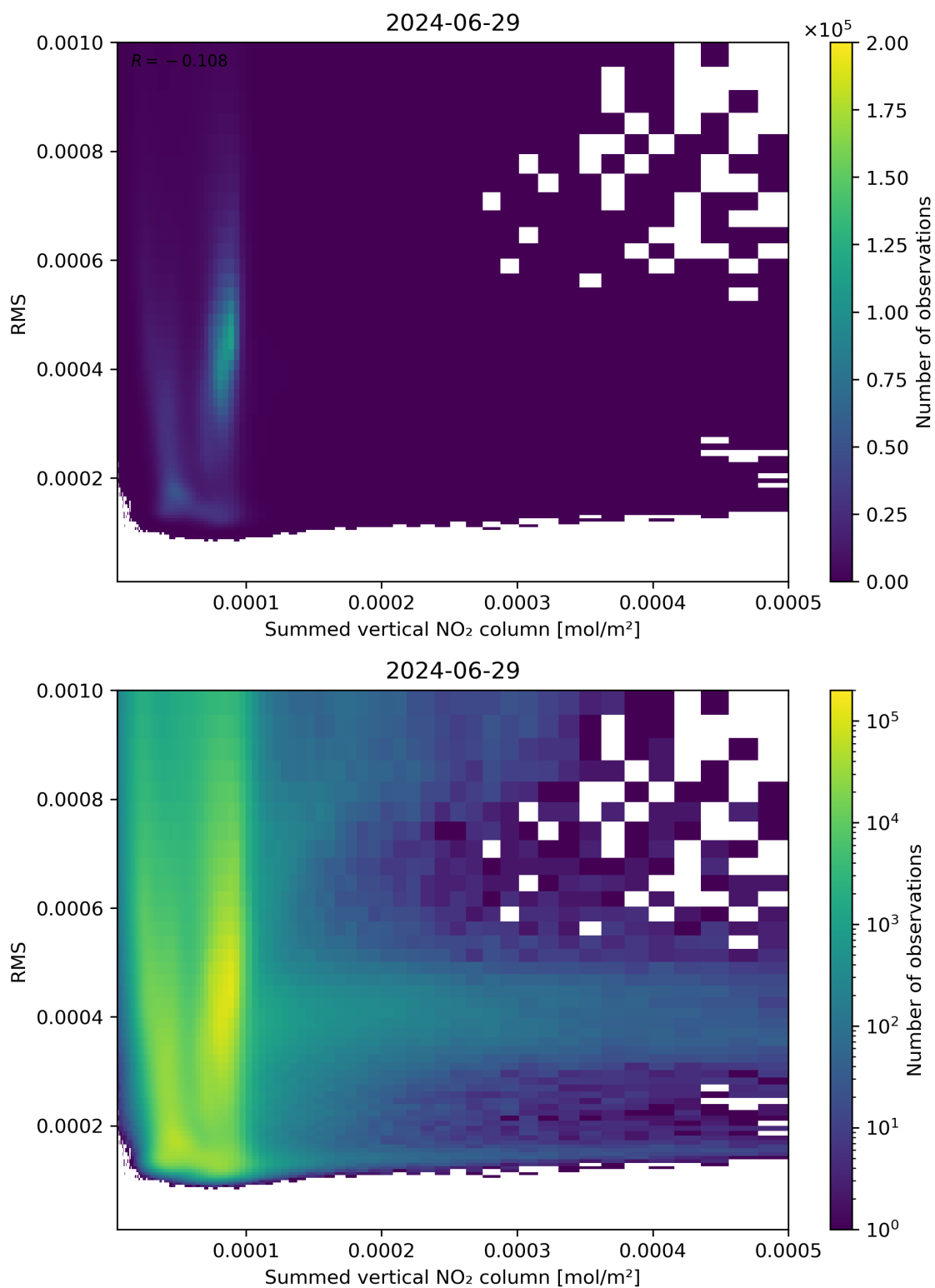
Figure 109: Scatter density plot of “Summed vertical NO 2 column” against “RMS” for 2024-06-29 to 2024-06-30.
