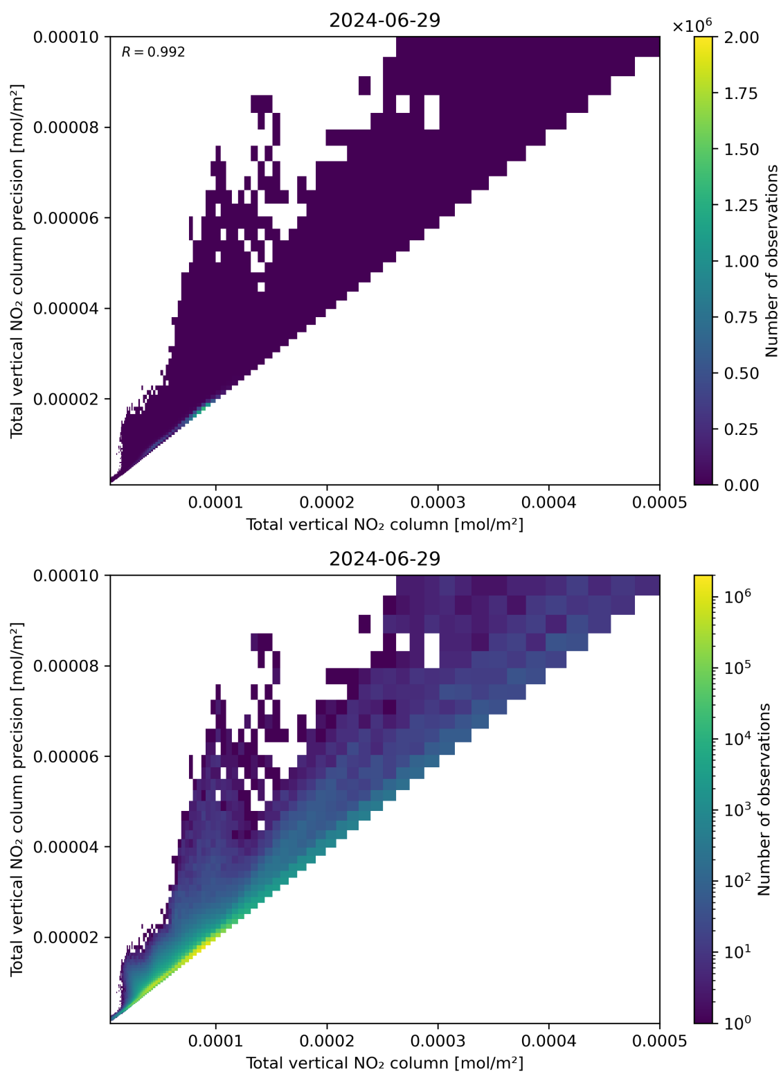
Figure 114: Scatter density plot of “Total vertical NO 2 column” against “Total vertical NO 2 column precision” for 2024-06-29 to 2024-06-30.
