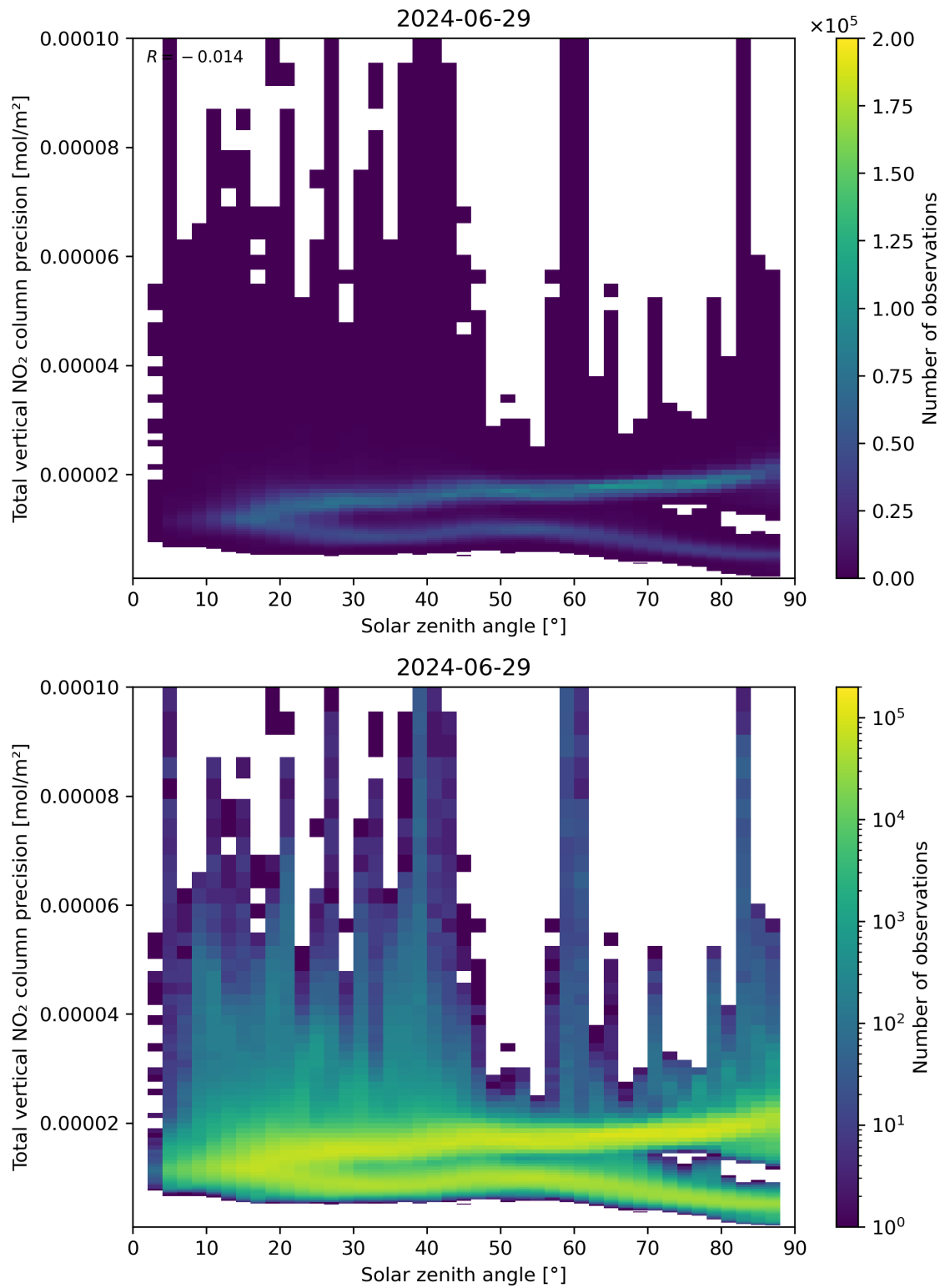
Figure 154: Scatter density plot of “Solar zenith angle” against “Total vertical NO 2 column precision” for 2024-06-29 to 2024-06-30.
