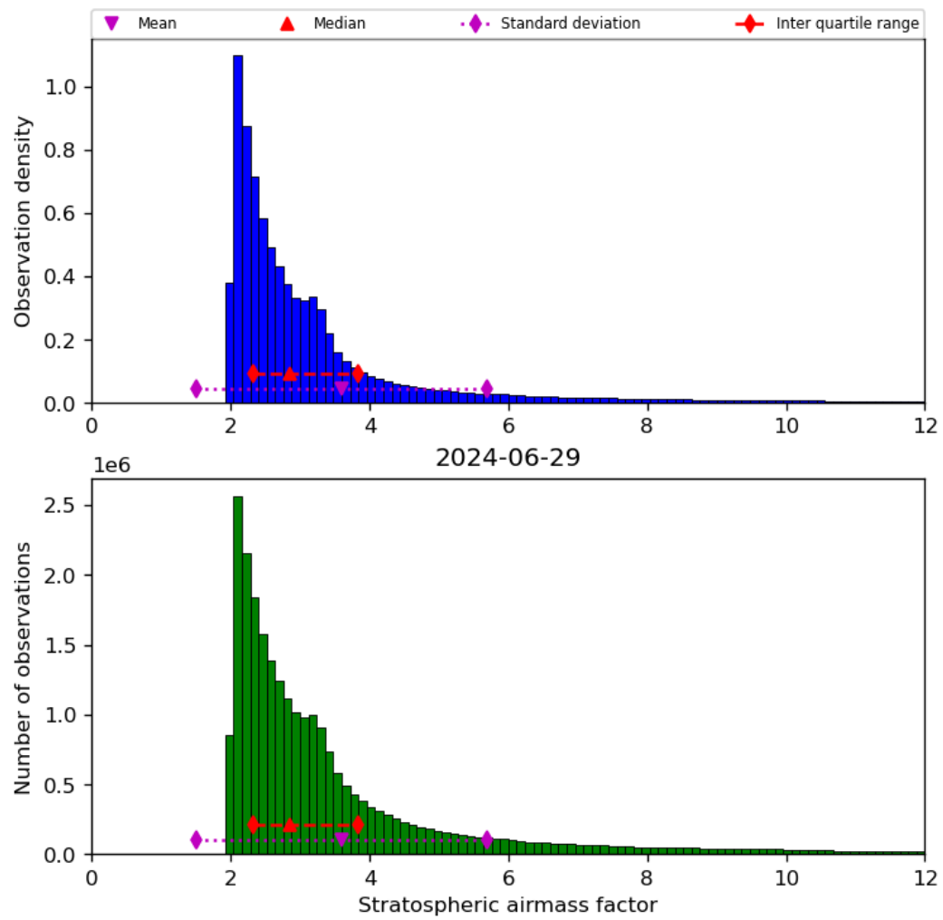
Figure 44: Histogram of “Stratospheric airmass factor” for 2024-06-29 to 2024-06-30
