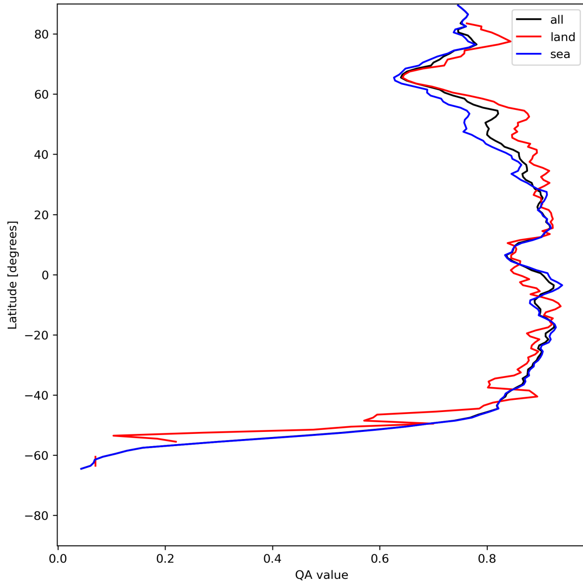
Figure 11: Zonal average of “QA value” for 2024-06-29 to 2024-06-30.
