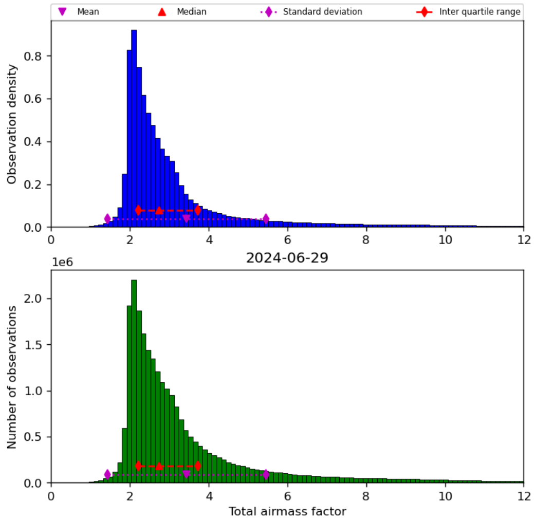
Figure 32: Histogram of “Total airmass factor” for 2024-06-29 to 2024-06-30
