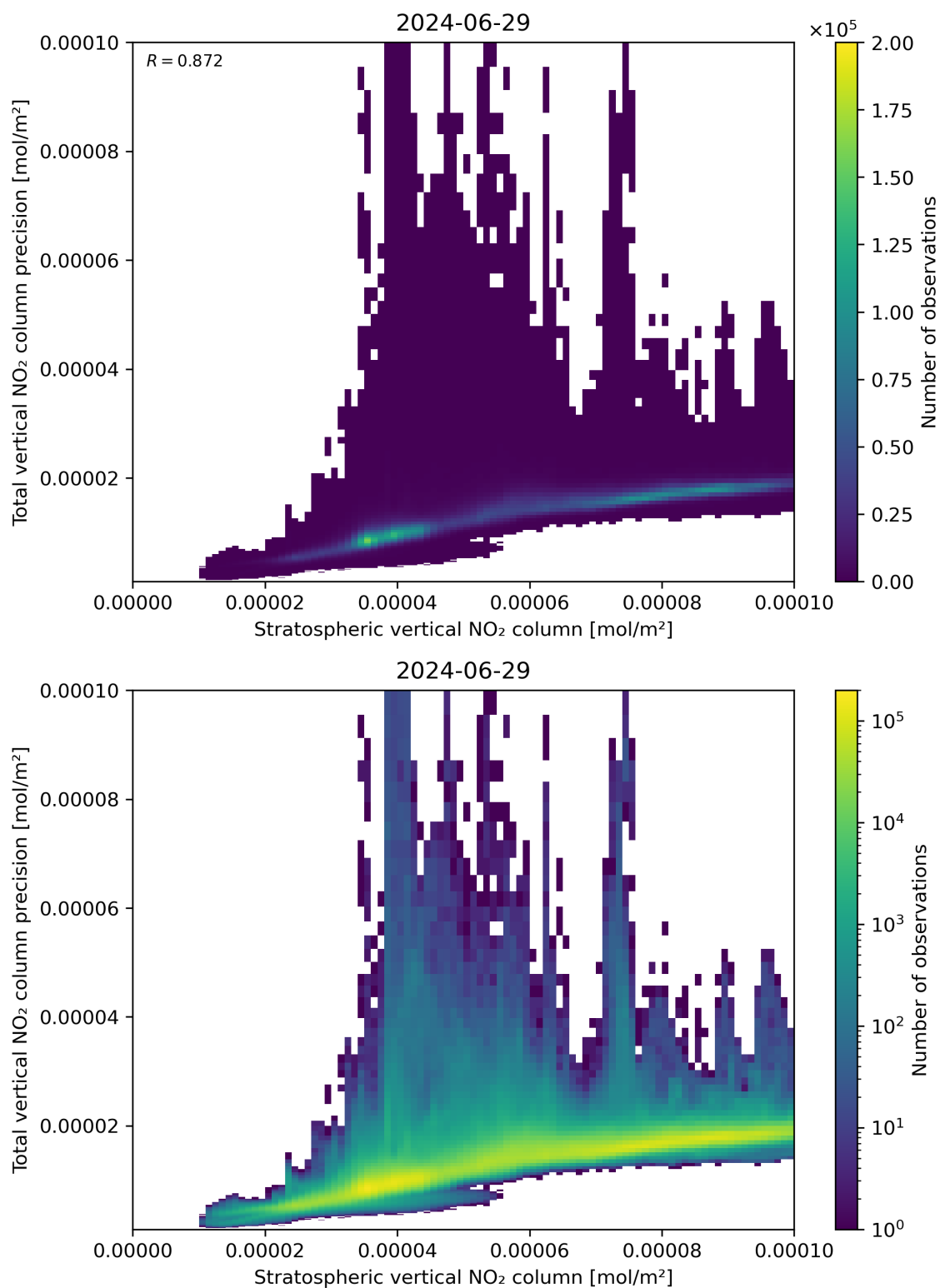
Figure 101: Scatter density plot of “Stratospheric vertical NO 2 column” against “Total vertical NO 2 column precision” for 2024-06-29 to 2024-06-30.
