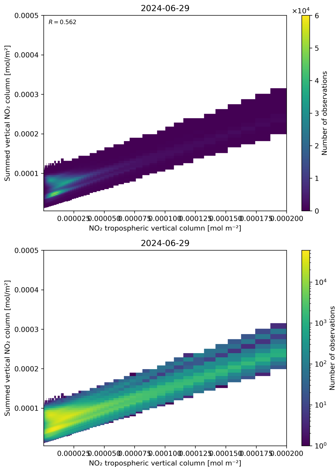
Figure 126: Scatter density plot of “NO 2 tropospheric vertical column” against “Summed vertical NO 2 column” for 2024-06-29 to 2024-06-30.
