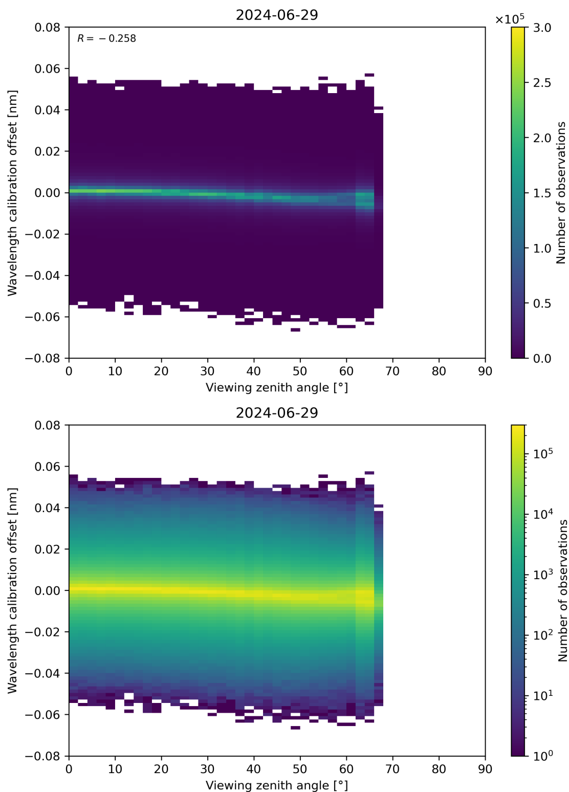
Figure 173: Scatter density plot of “Viewing zenith angle” against “Wavelength calibration offset” for 2024-06-29 to 2024-06-30.
