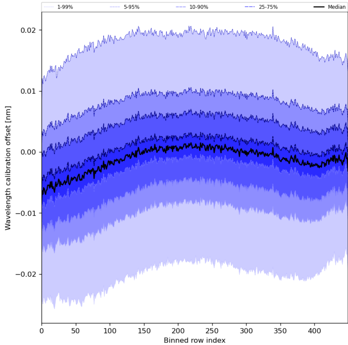
Figure 52: Along track statistics of “Wavelength calibration offset” for 2024-06-29 to 2024-06-30
