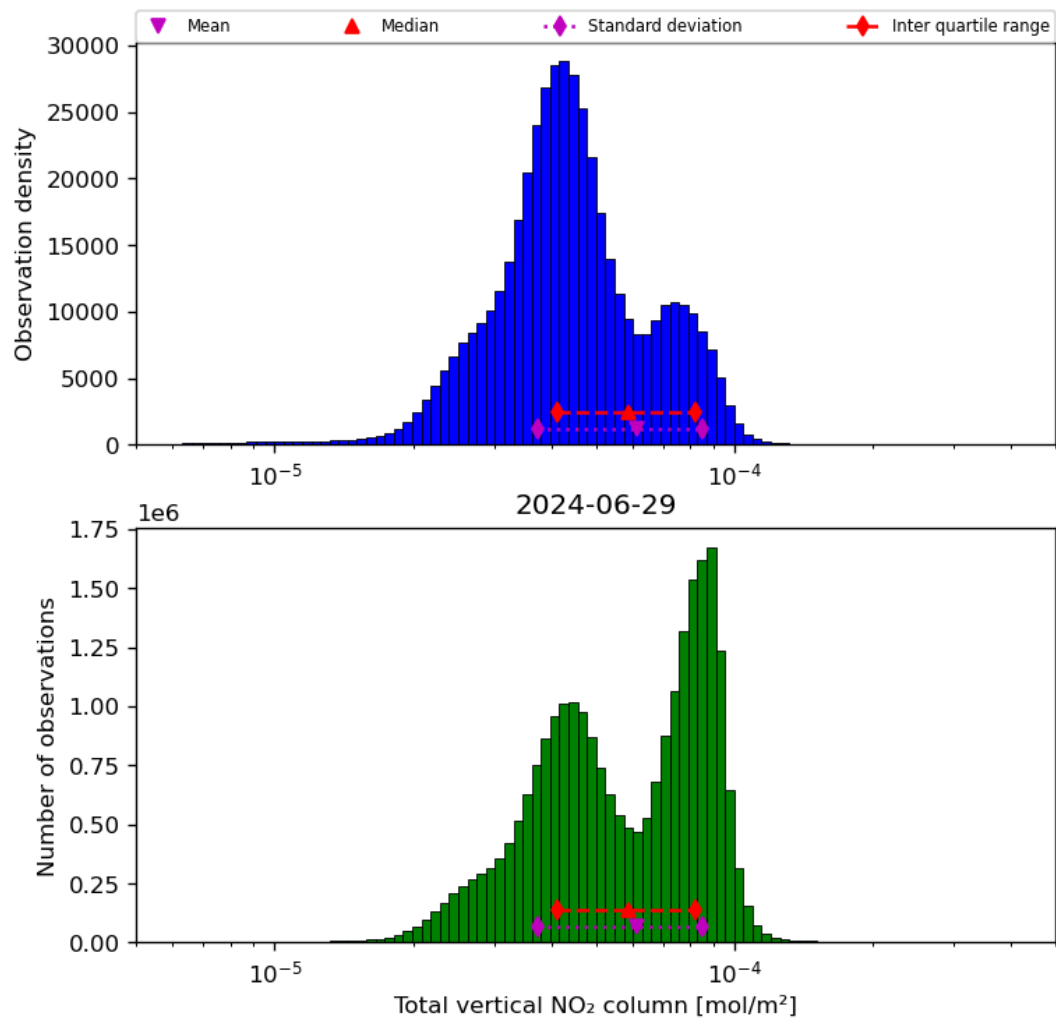
Figure 38: Histogram of "Total vertical NO 2 column" for 2024-06-29 to 2024-06-30
