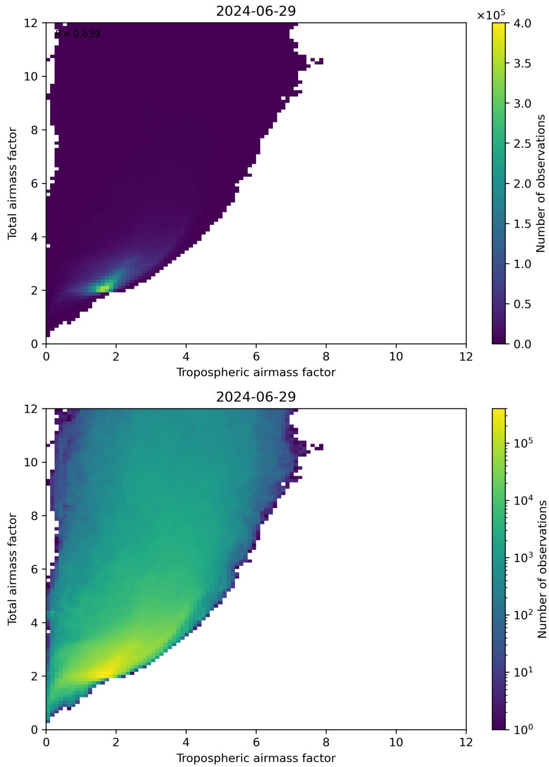
Figure 72: Scatter density plot of “Tropospheric airmass factor” against “Total airmass factor” for 2024-06-29 to 2024-06-30.
