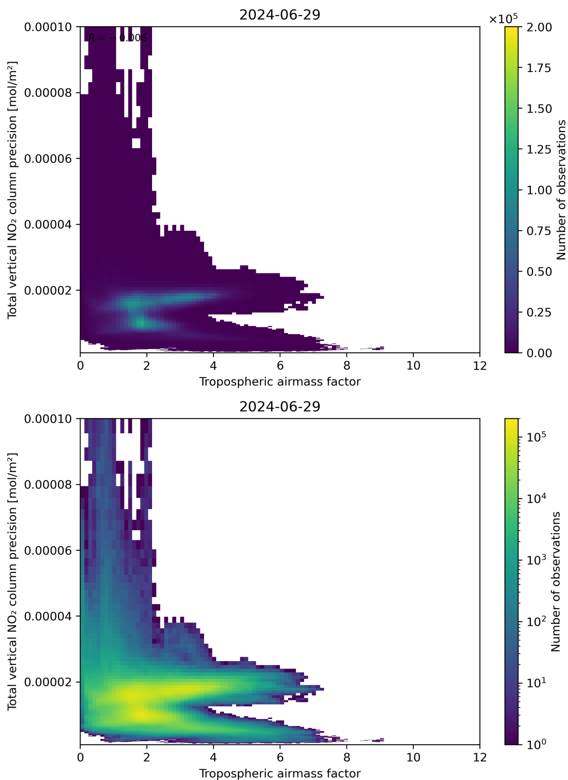
Figure 78: Scatter density plot of “Tropospheric air mass factor” against “Total vertical NO 2 column precision” for 2024-06-29 to 2024-06-30.
