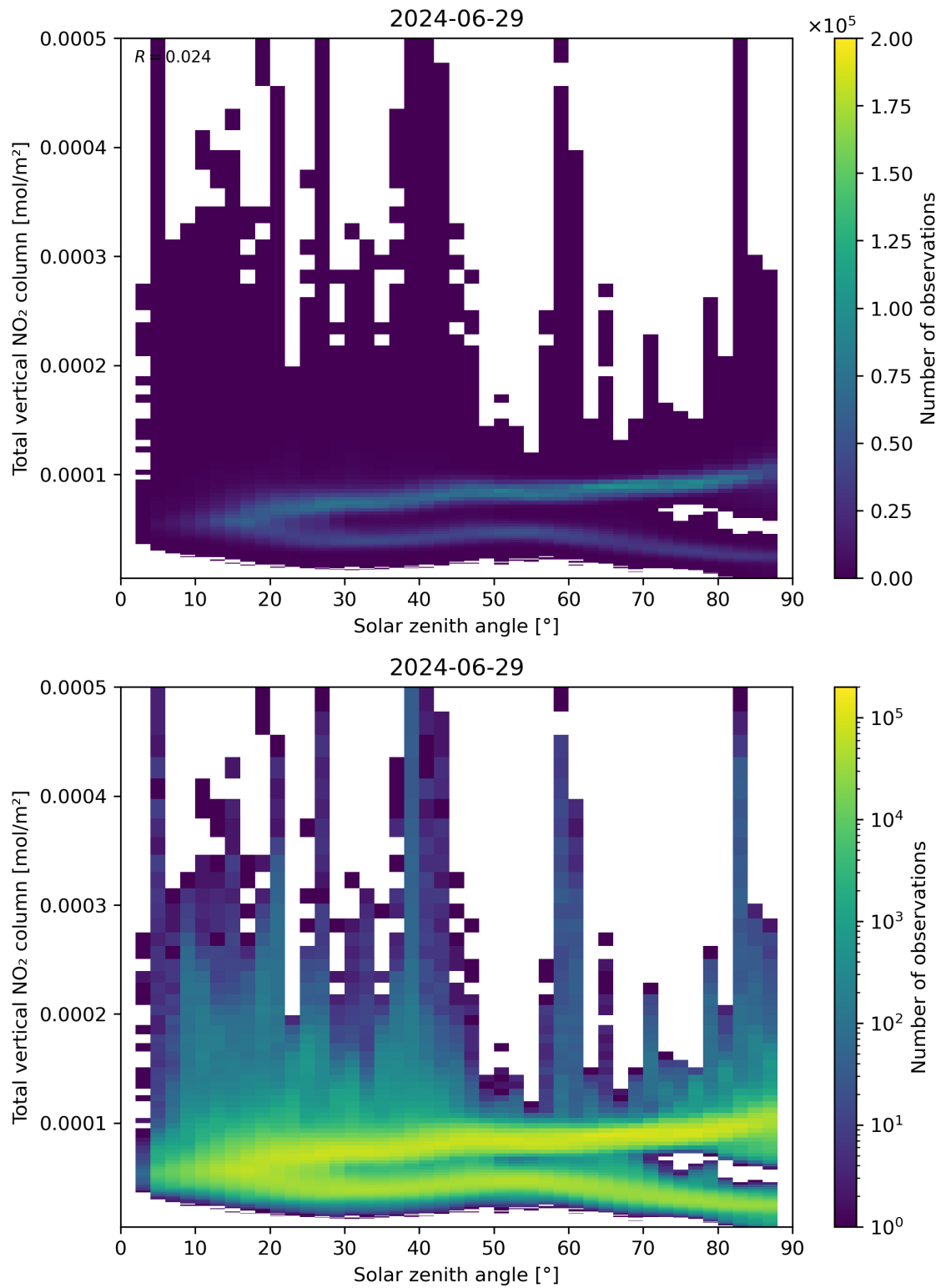
Figure 153: Scatter density plot of “Solar zenith angle” against “Total vertical NO 2 column” for 2024-06-29 to 2024-06-30.
