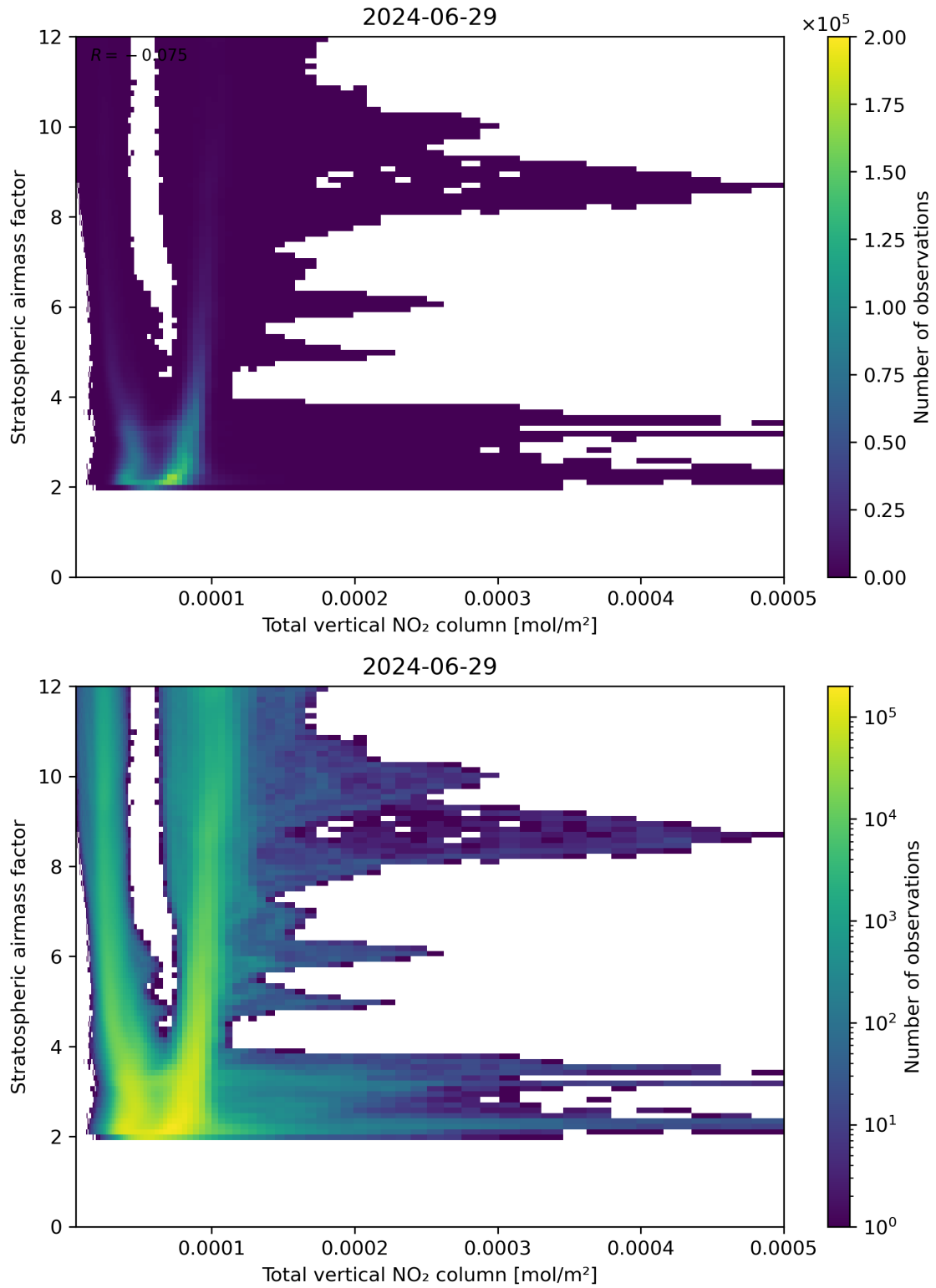
Figure 110: Scatter density plot of “Total vertical NO 2 column” against “Stratospheric airmass factor” for 2024-06-29 to 2024-06-30.
