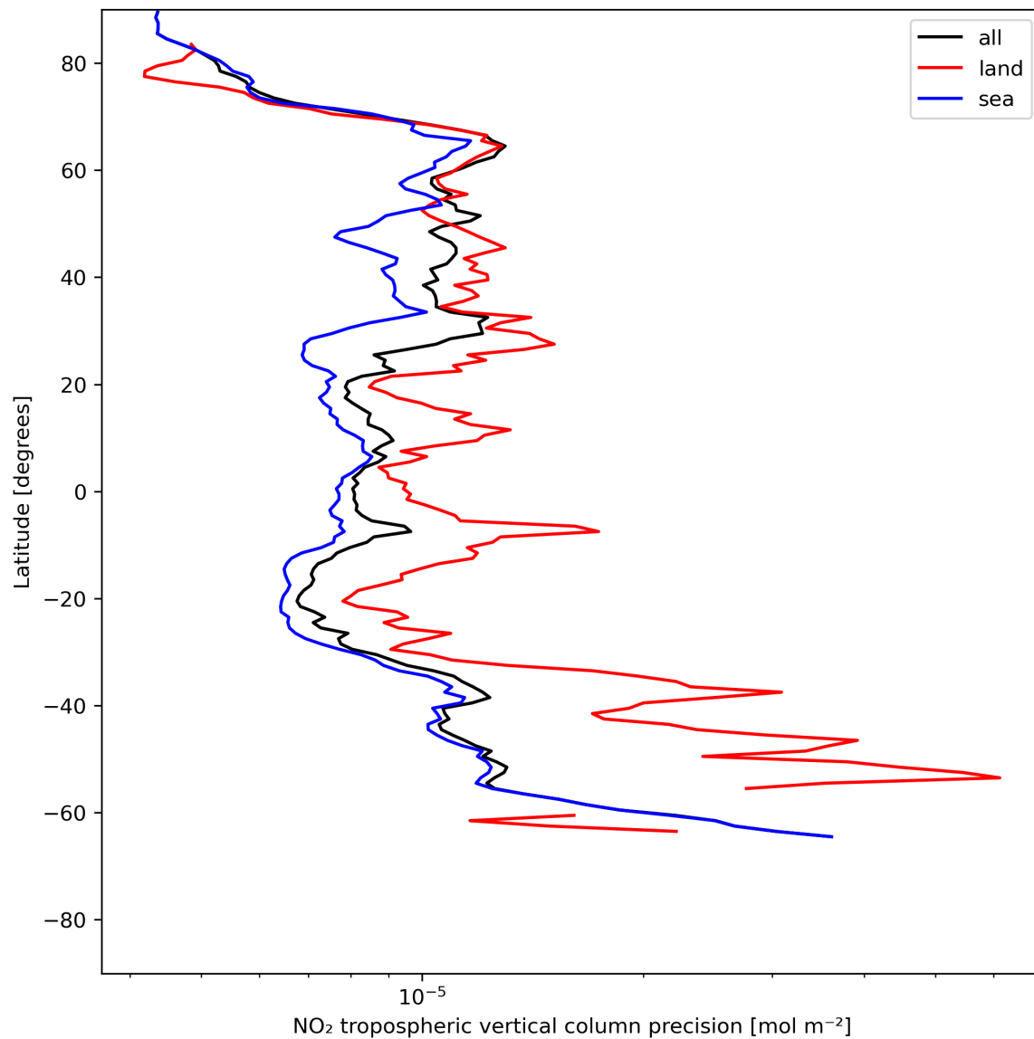
Figure 13: Zonal average of “NO 2 tropospheric vertical column precision” for 2024-06-29 to 2024-06-30.
