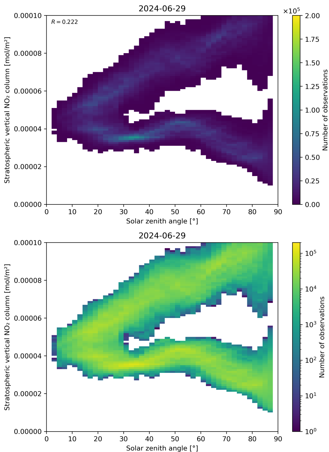
Figure 150: Scatter density plot of “Solar zenith angle” against “Stratospheric vertical NO 2 column” for 2024-06-29 to 2024-06-30.
