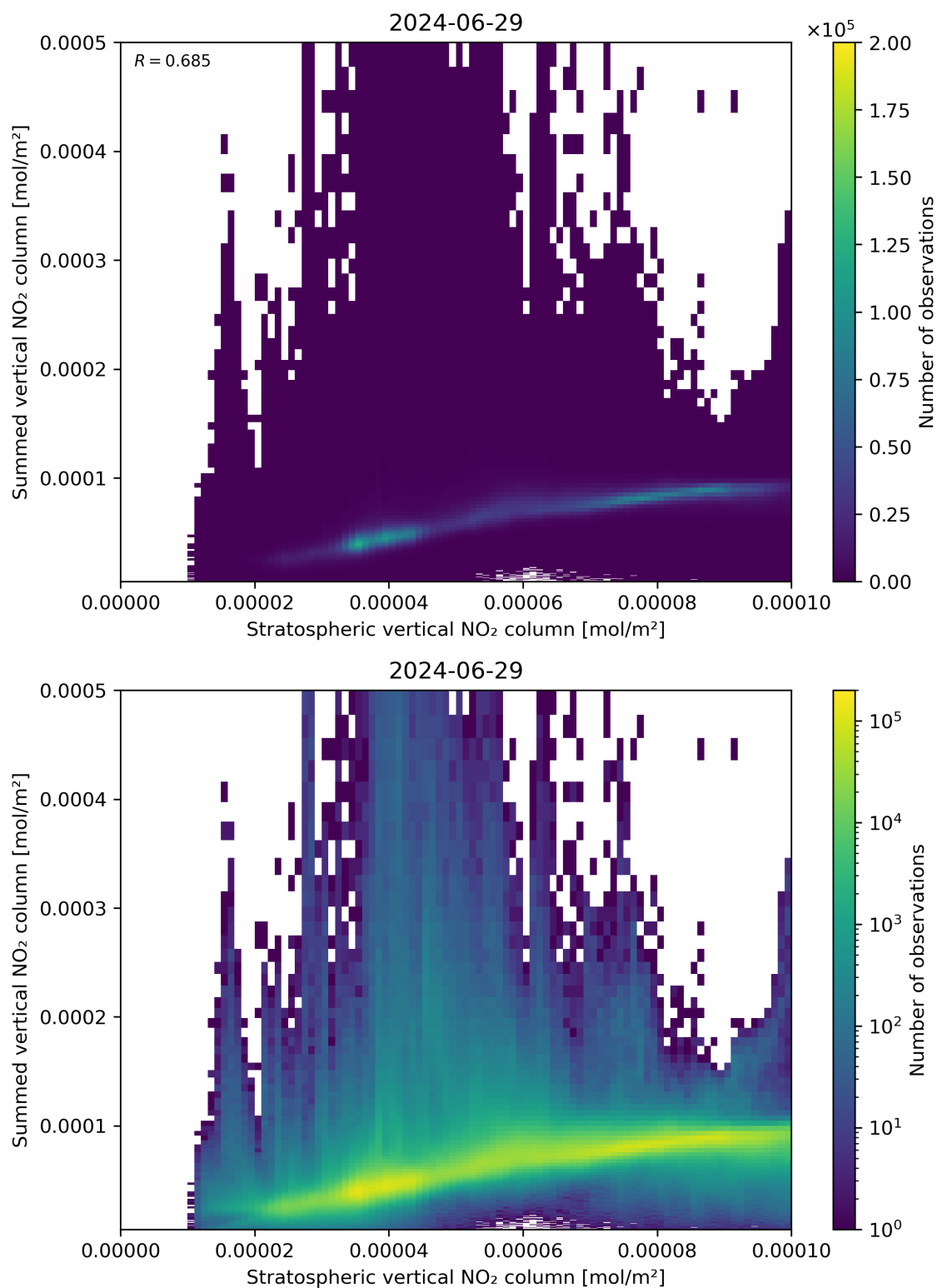
Figure 98: Scatter density plot of “Stratospheric vertical NO 2 column” against “Summed vertical NO 2 column” for 2024-06-29 to 2024-06-30.
