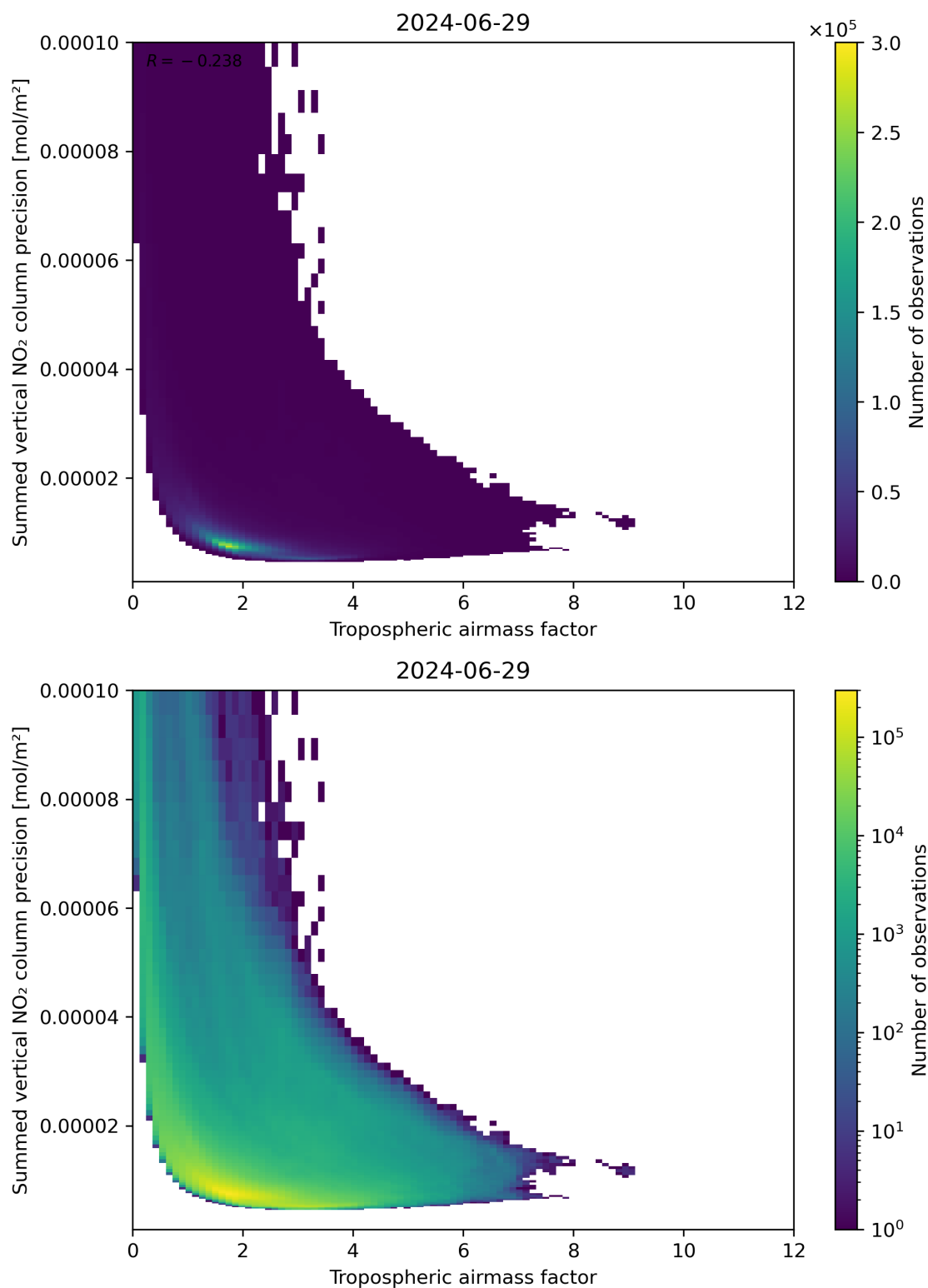
Figure 76: Scatter density plot of “Tropospheric air mass factor” against “Summed vertical NO 2 column precision” for 2024-06-29 to 2024-06-30.
