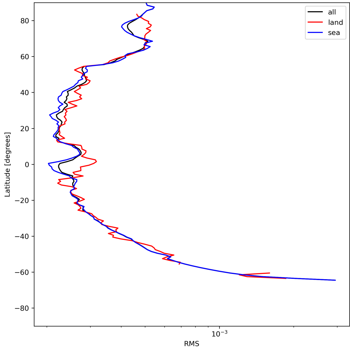
Figure 26: Zonal average of “RMS” for 2024-06-29 to 2024-06-30.
