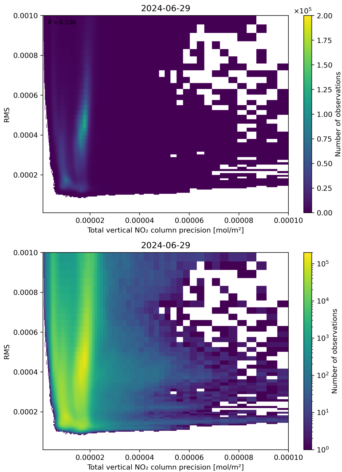
Figure 119: Scatter density plot of “Total vertical NO 2 column precision” against “RMS” for 2024-06-29 to 2024-06-30.
