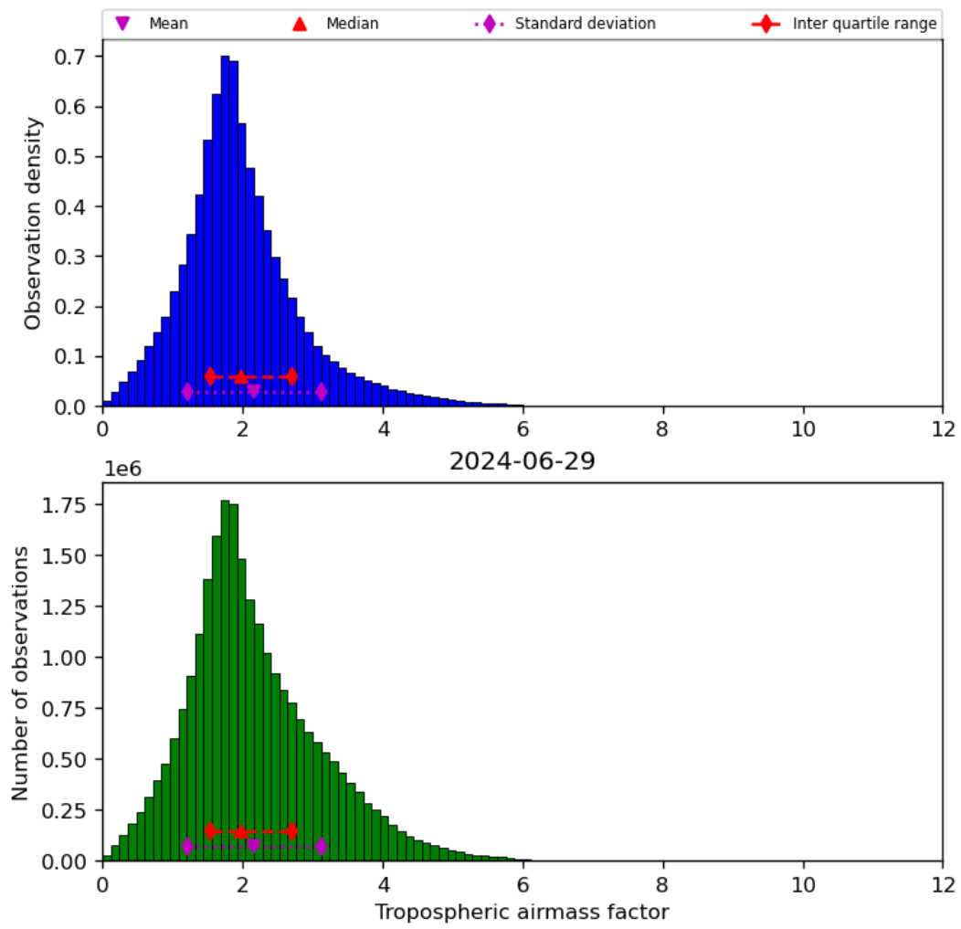
Figure 31: Histogram of “Tropospheric airmass factor” for 2024-06-29 to 2024-06-30
