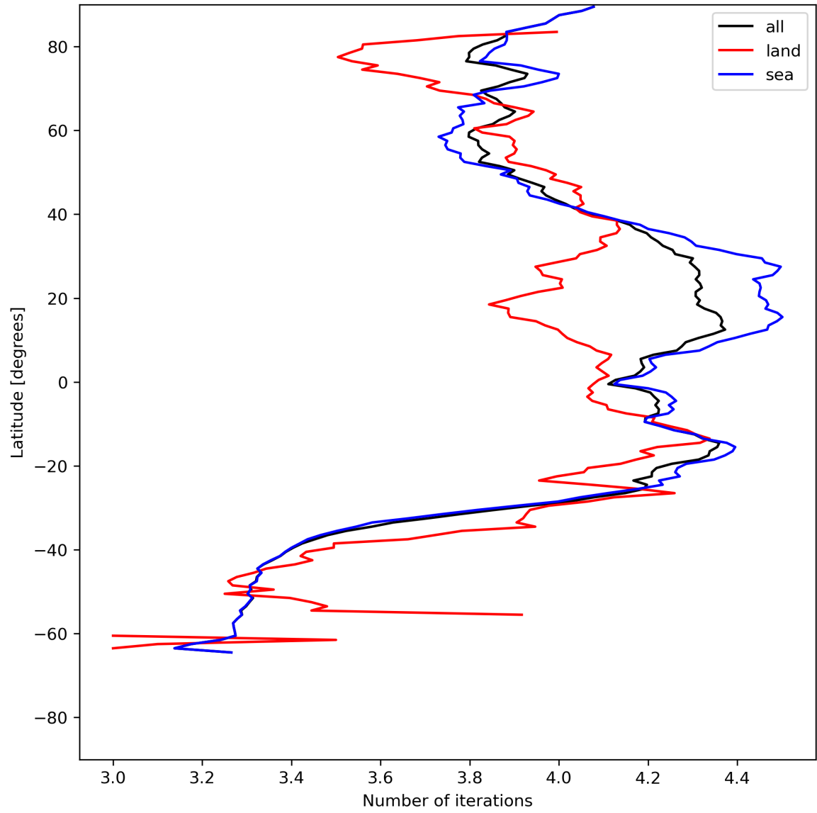
Figure 17: Zonal average of “Number of iterations” for 2024-06-29 to 2024-06-30.
