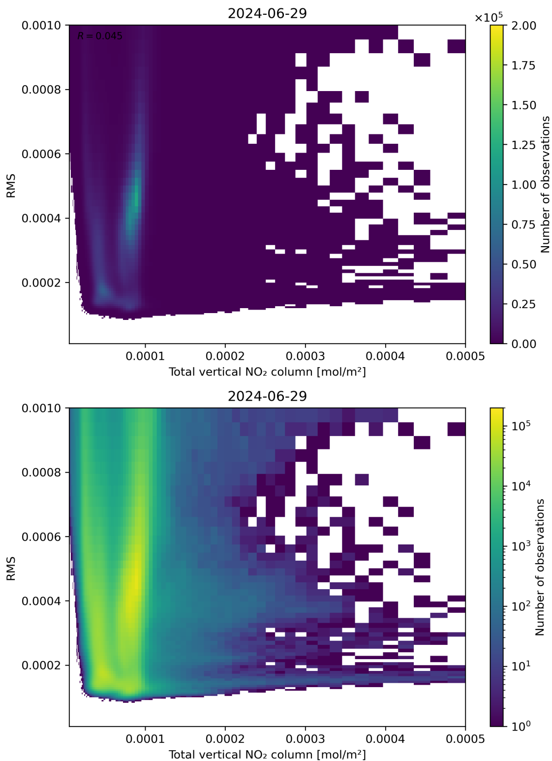
Figure 120: Scatter density plot of “Total vertical NO 2 column” against “RMS” for 2024-06-29 to 2024-06-30.
