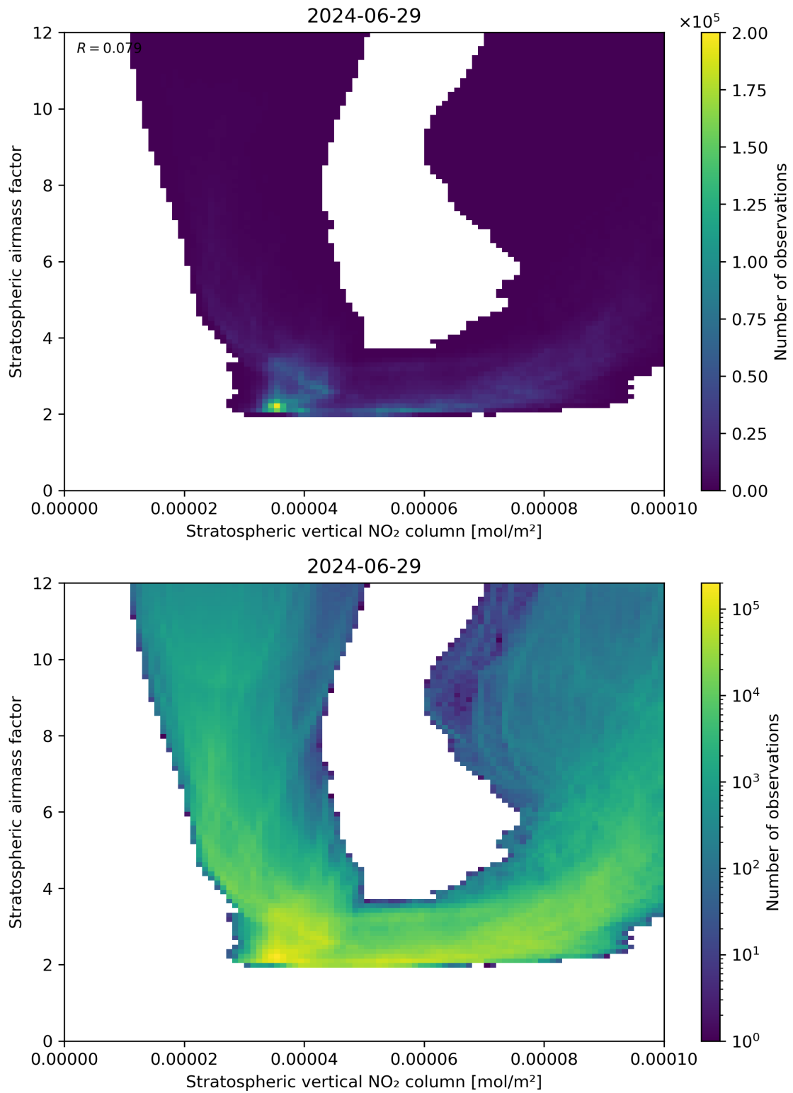
Figure 96: Scatter density plot of “Stratospheric vertical NO 2 column” against “Stratospheric airmass factor” for 2024-06-29 to 2024-06-30.
