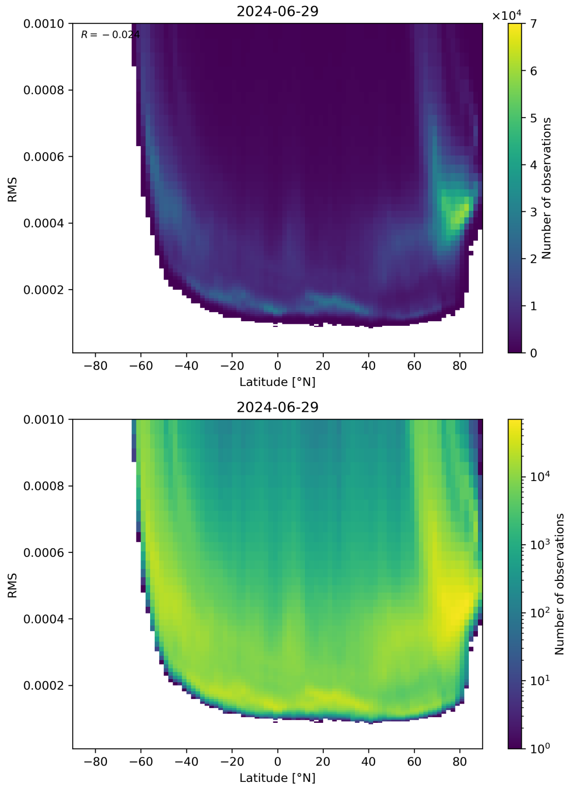
Figure 94: Scatter density plot of “Latitude” against “RMS” for 2024-06-29 to 2024-06-30.
