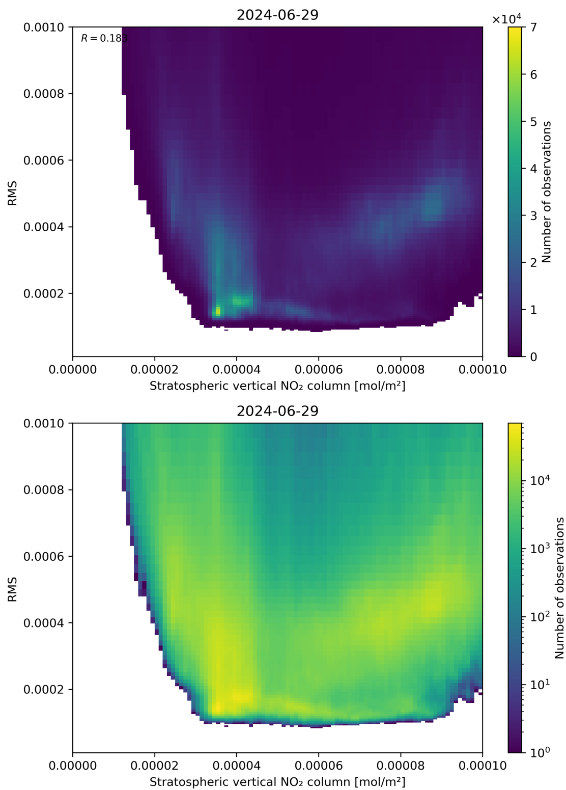
Figure 102: Scatter density plot of “Stratospheric vertical NO 2 column” against “RMS” for 2024-06-29 to 2024-06-30.
