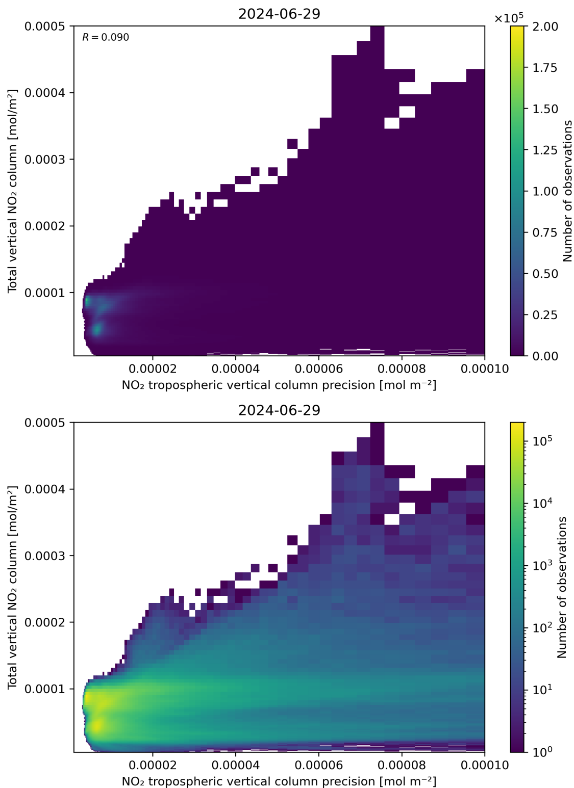
Figure 138: Scatter density plot of “NO 2 tropospheric vertical column precision” against “Total vertical NO 2 column” for 2024-06-29 to 2024-06-30.
