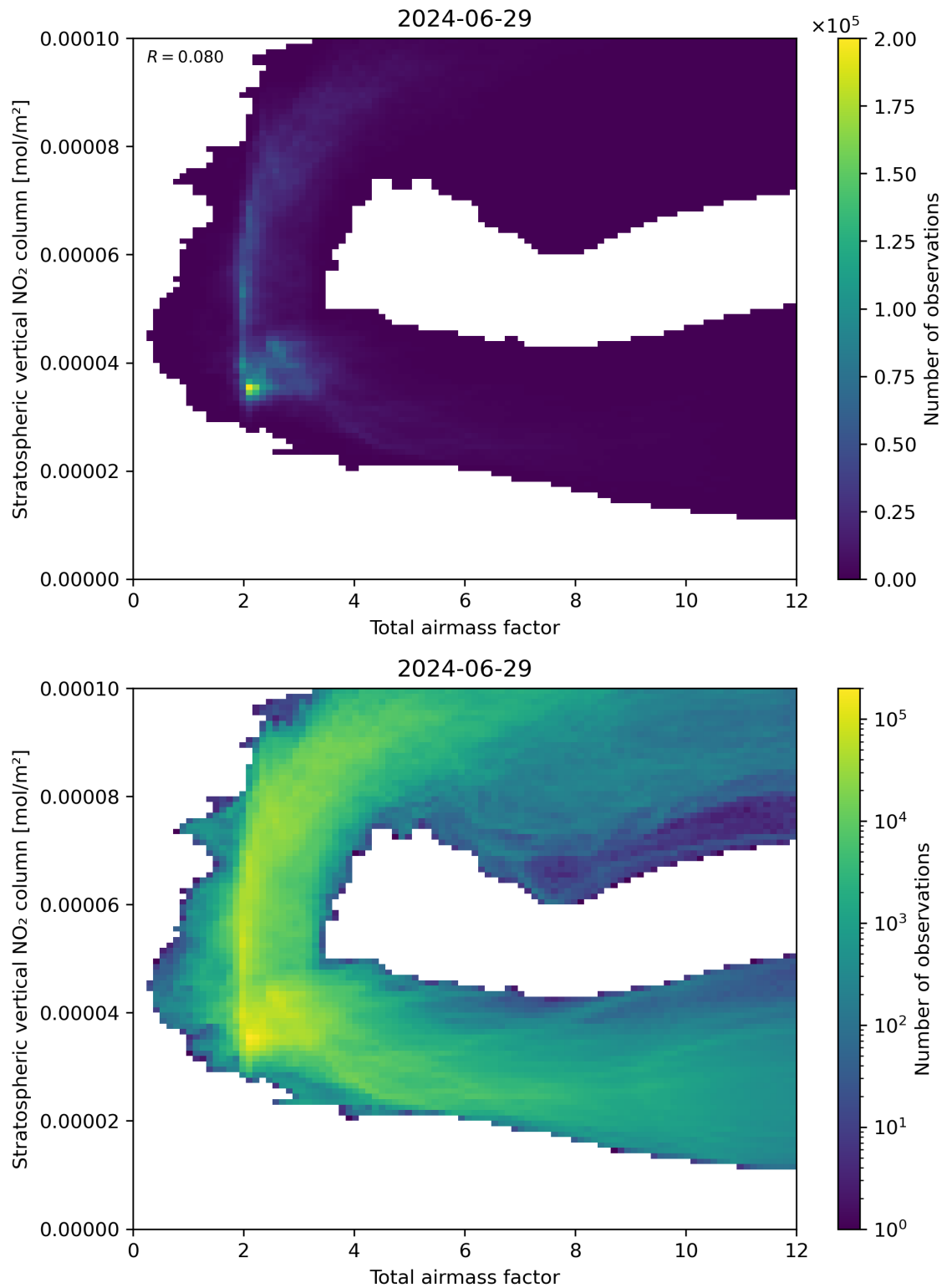
Figure 64: Scatter density plot of “Total airmass factor” against “Stratospheric vertical NO 2 column” for 2024-06-29 to 2024-06-30.
