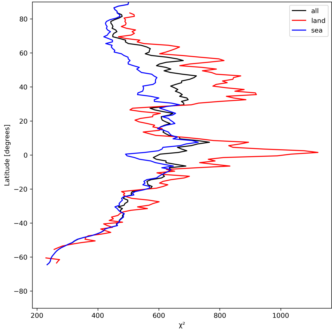
Figure 25: Zonal average of “ \chi^2 ” for 2024-06-29 to 2024-06-30.
