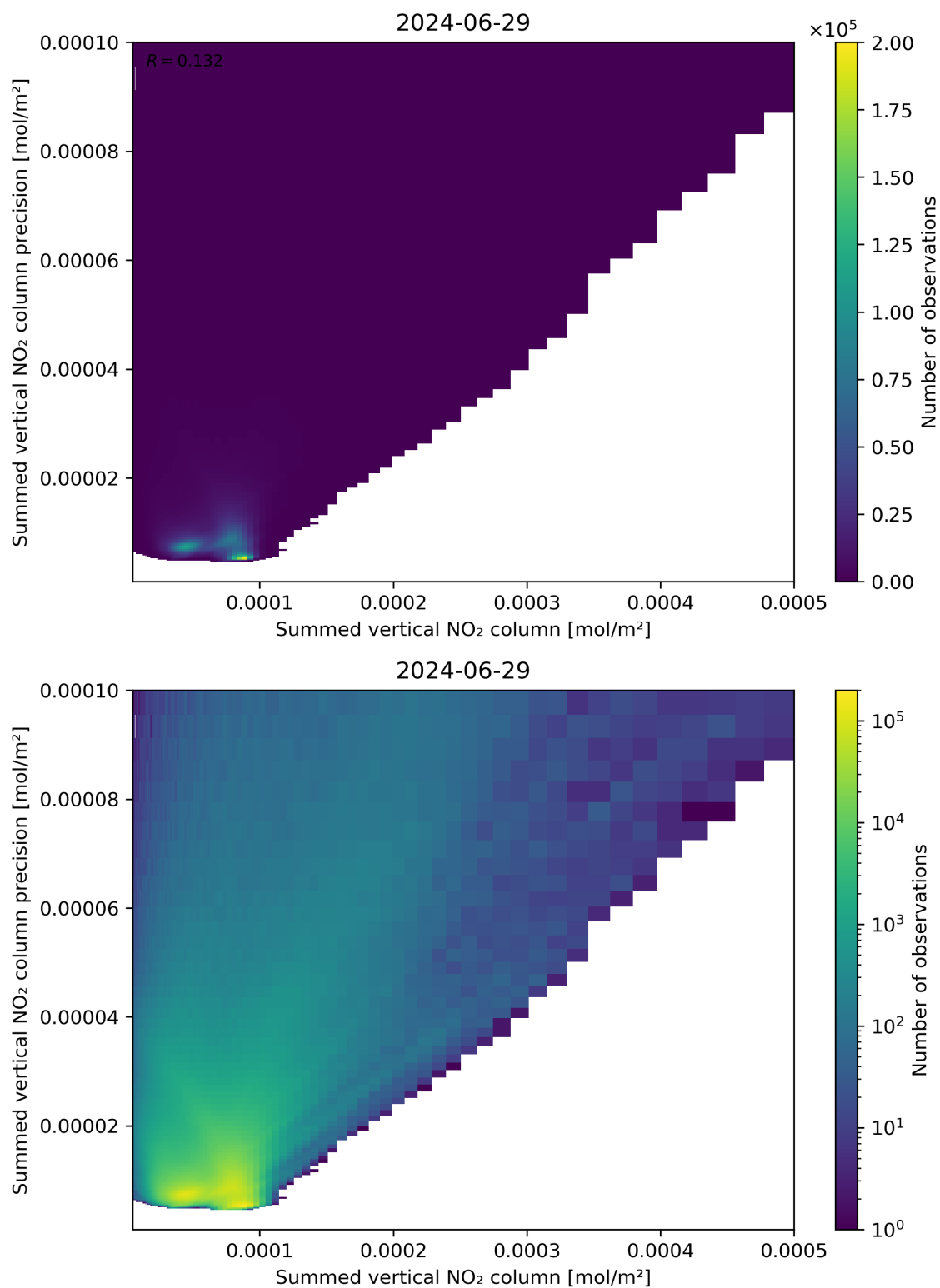
Figure 105: Scatter density plot of “Summed vertical NO 2 column” against “Summed vertical NO 2 column precision” for 2024-06-29 to 2024-06-30.
