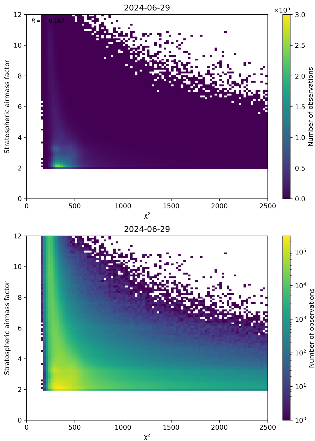
Figure 81: Scatter density plot of “ \chi^2 ” against “Stratospheric airmass factor” for 2024-06-29 to 2024-06-30.
