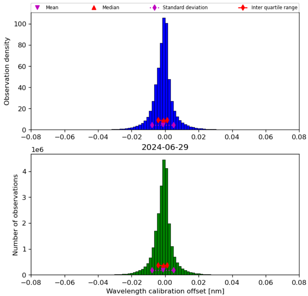
Figure 35: Histogram of “Wavelength calibration offset” for 2024-06-29 to 2024-06-30
