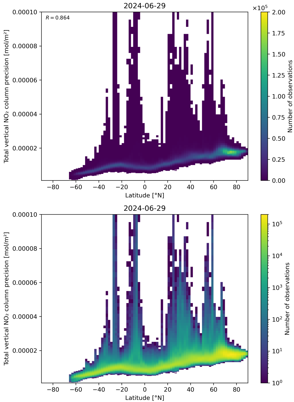
Figure 91: Scatter density plot of “Latitude” against “Total vertical NO 2 column precision” for 2024-06-29 to 2024-06-30.
