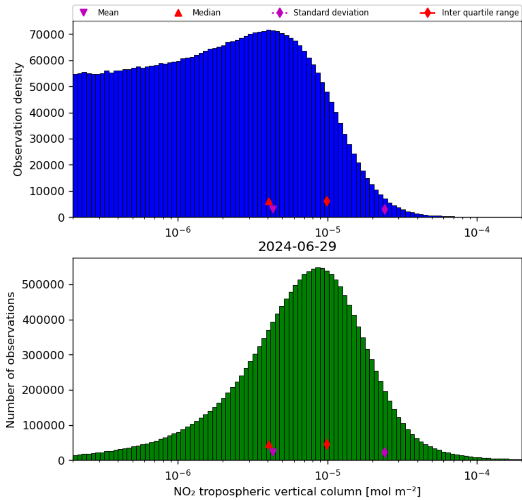
Figure 29: Histogram of “NO 2 tropospheric vertical column” for 2024-06-29 to 2024-06-30
