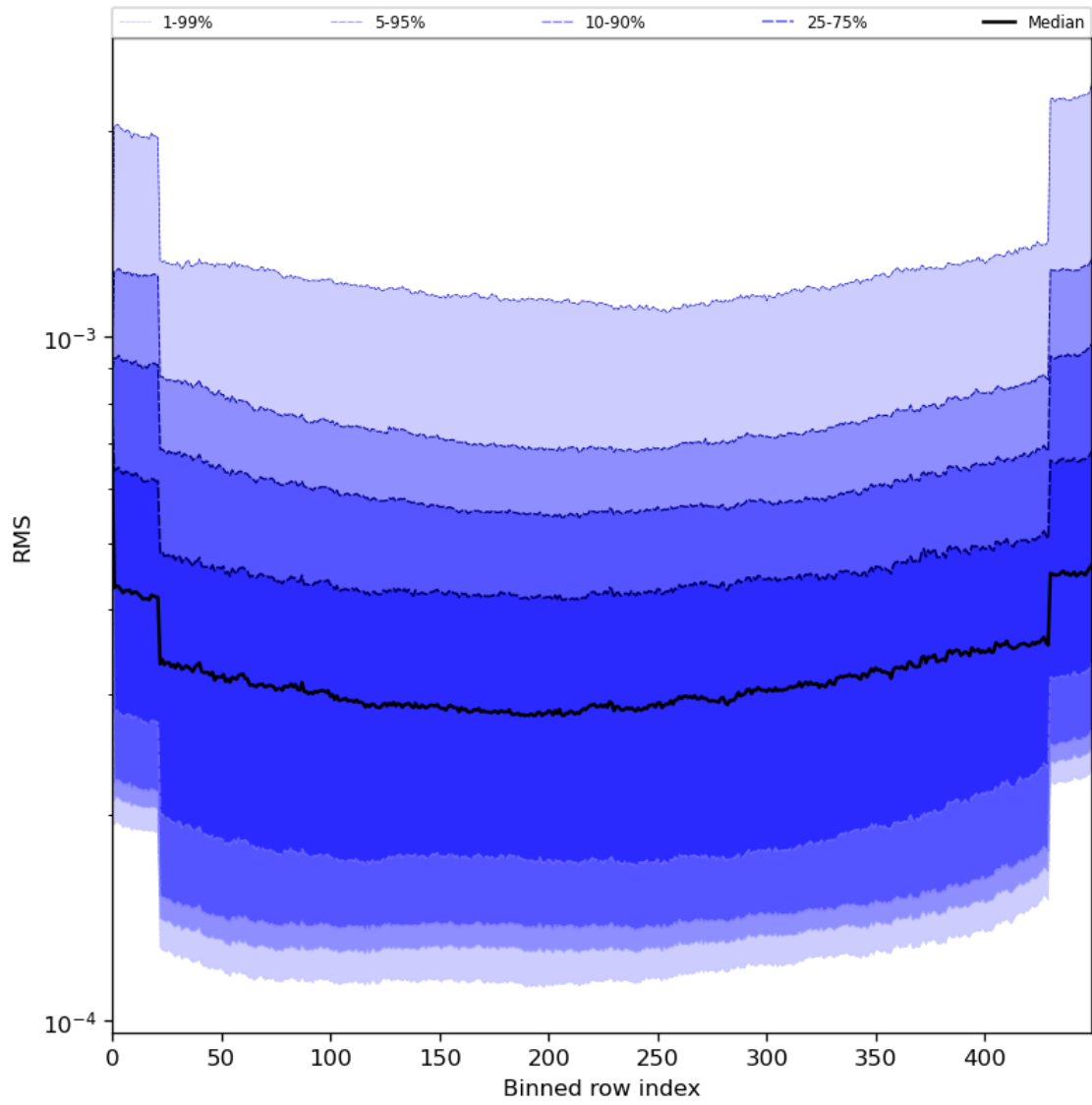
Figure 60: Along track statistics of “RMS” for 2024-06-29 to 2024-06-30
