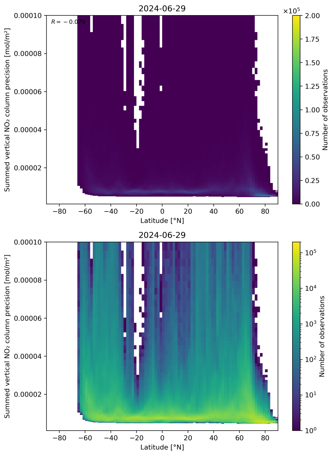
Figure 89: Scatter density plot of “Latitude” against “Summed vertical NO 2 column precision” for 2024-06-29 to 2024-06-30.
