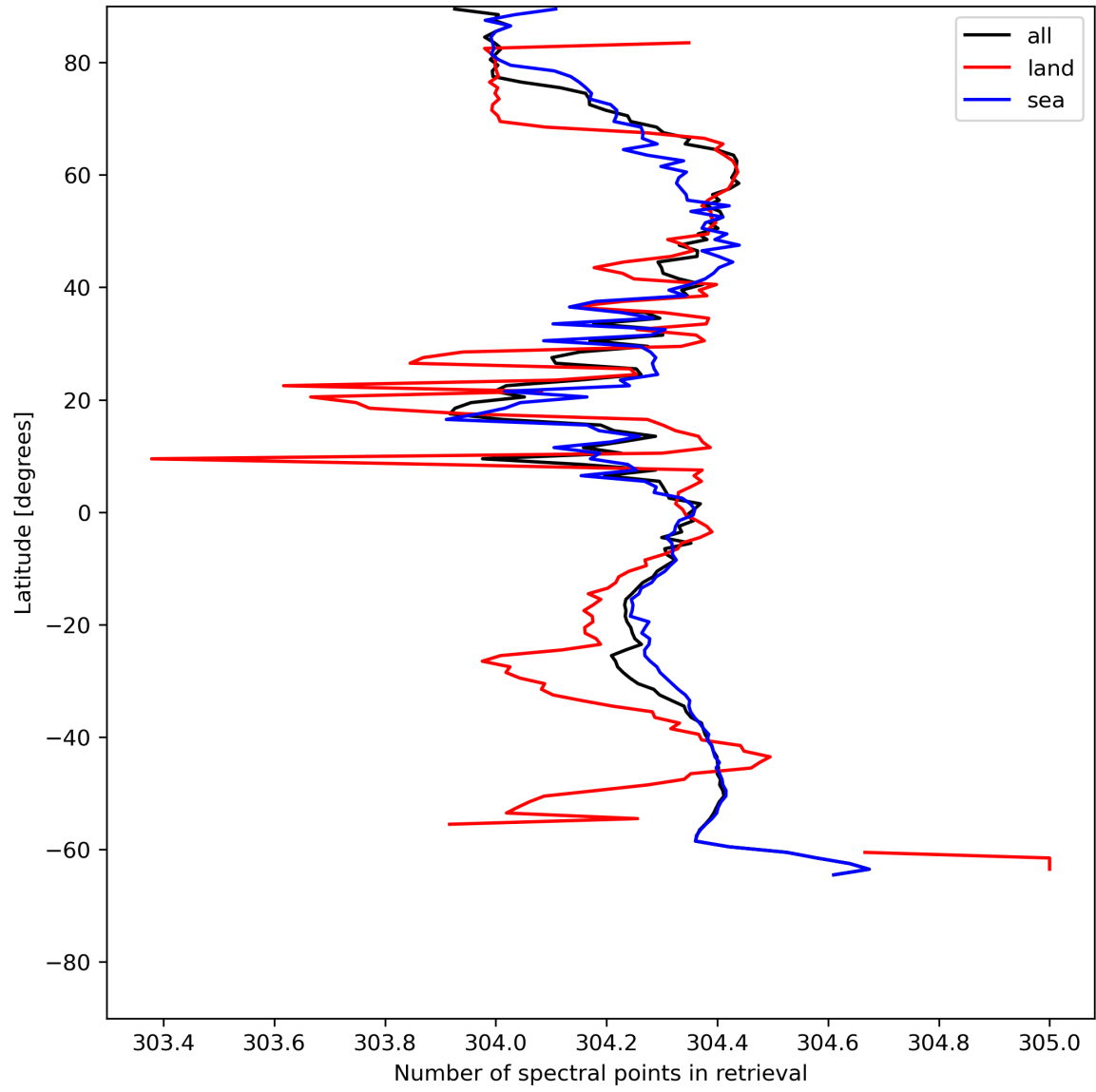
Figure 16: Zonal average of “Number of spectral points in retrieval” for 2024-06-29 to 2024-06-30.
