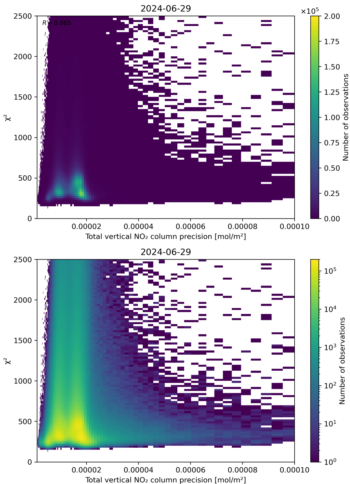
Figure 116: Scatter density plot of “Total vertical NO 2 column precision” against “ \chi^2 ” for 2024-06-29 to 2024-06-30.
