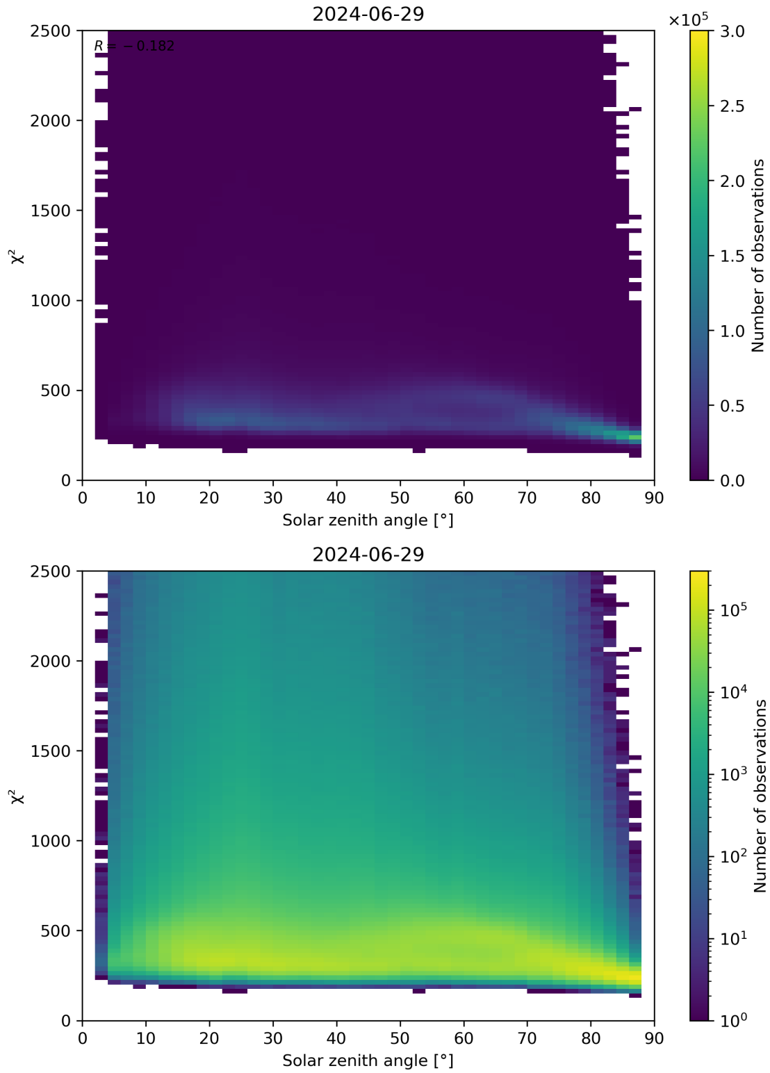
Figure 148: Scatter density plot of “Solar zenith angle” against “ \chi^2 ” for 2024-06-29 to 2024-06-30.
