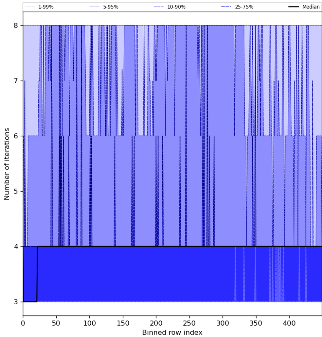
Figure 51: Along track statistics of “Number of iterations” for 2024-06-29 to 2024-06-30
