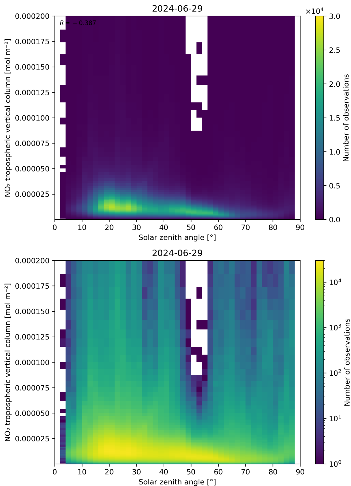
Figure 155: Scatter density plot of “Solar zenith angle” against “NO 2 tropospheric vertical column” for 2024-06-29 to 2024-06-30.
