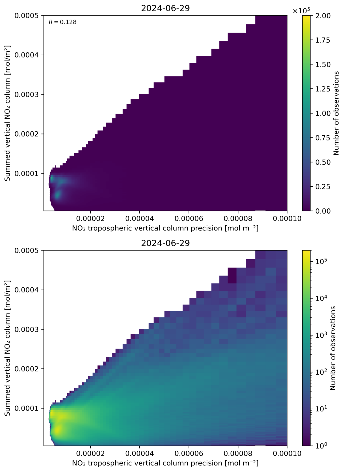
Figure 136: Scatter density plot of “NO 2 tropospheric vertical column precision” against “Summed vertical NO 2 column” for 2024-06-29 to 2024-06-30.
