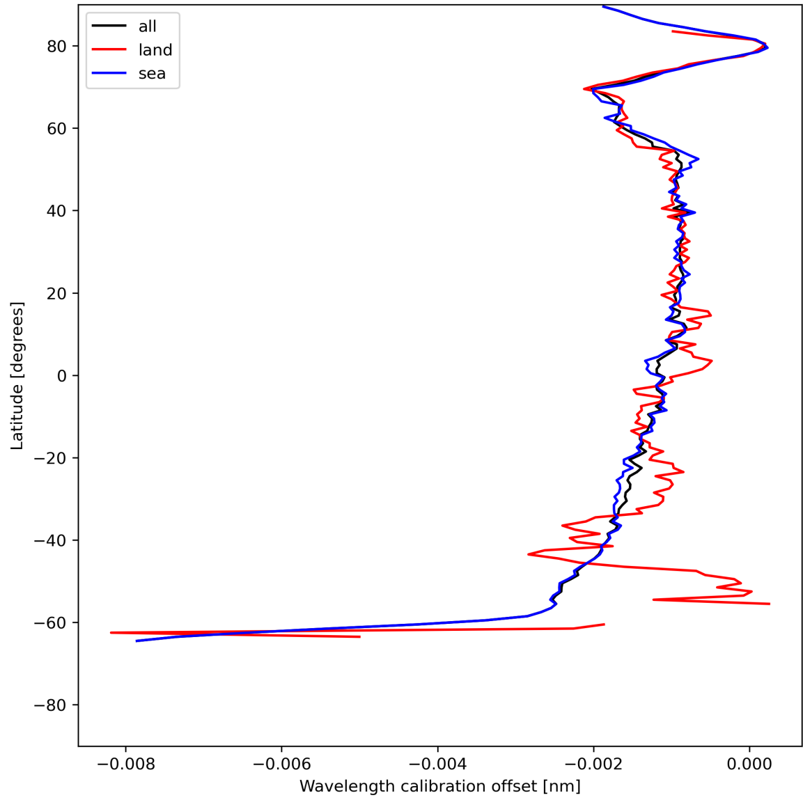
Figure 18: Zonal average of “Wavelength calibration offset” for 2024-06-29 to 2024-06-30.
