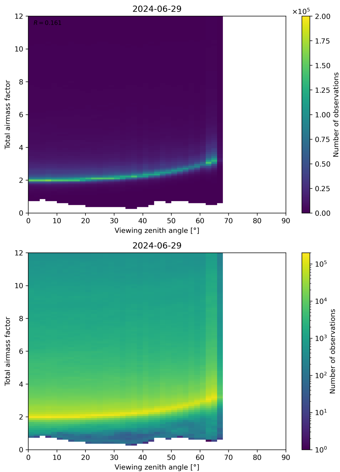
Figure 160: Scatter density plot of “Viewing zenith angle” against “Total airmass factor” for 2024-06-29 to 2024-06-30.
