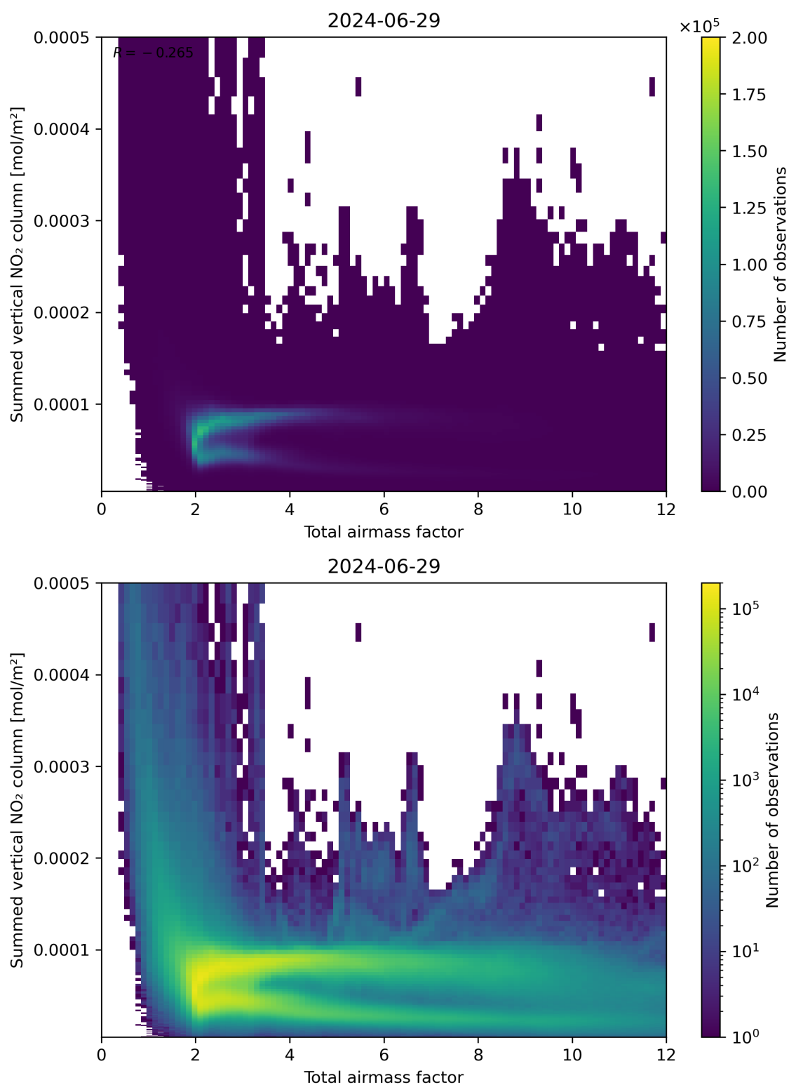
Figure 65: Scatter density plot of “Total airmass factor” against “Summed vertical NO 2 column” for 2024-06-29 to 2024-06-30.
