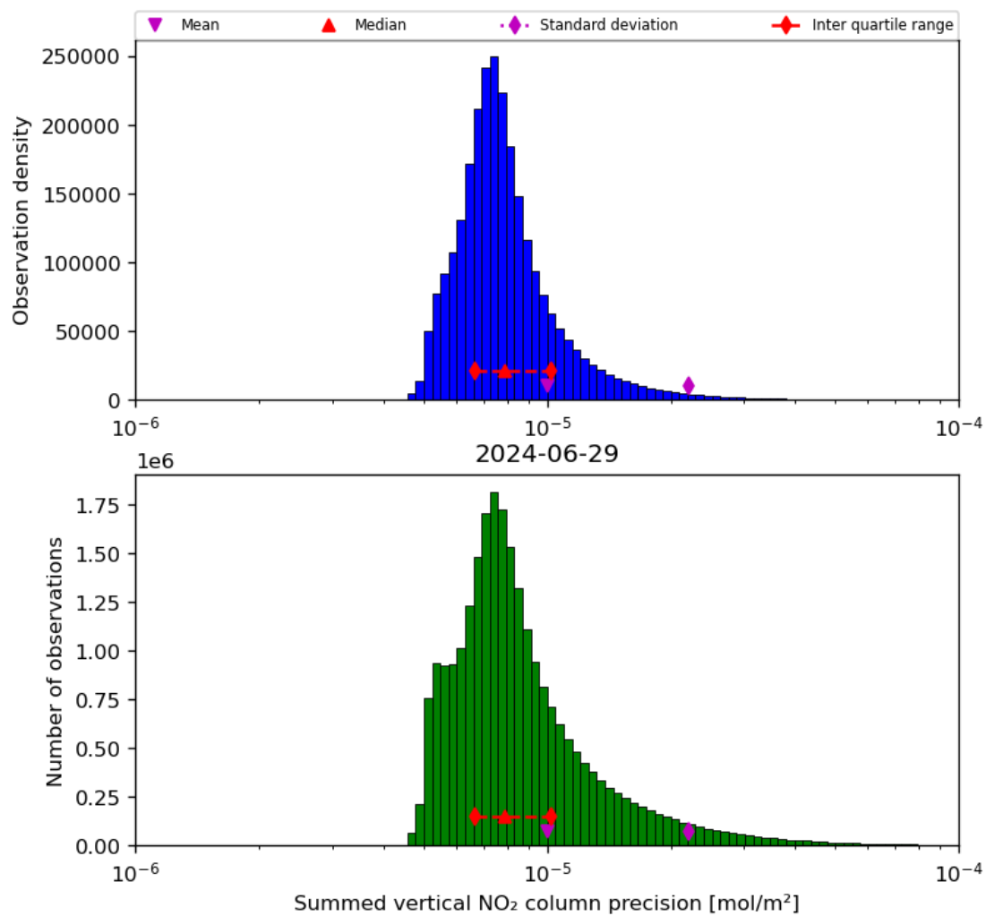
Figure 41: Histogram of “Summed vertical NO 2 column precision” for 2024-06-29 to 2024-06-30
