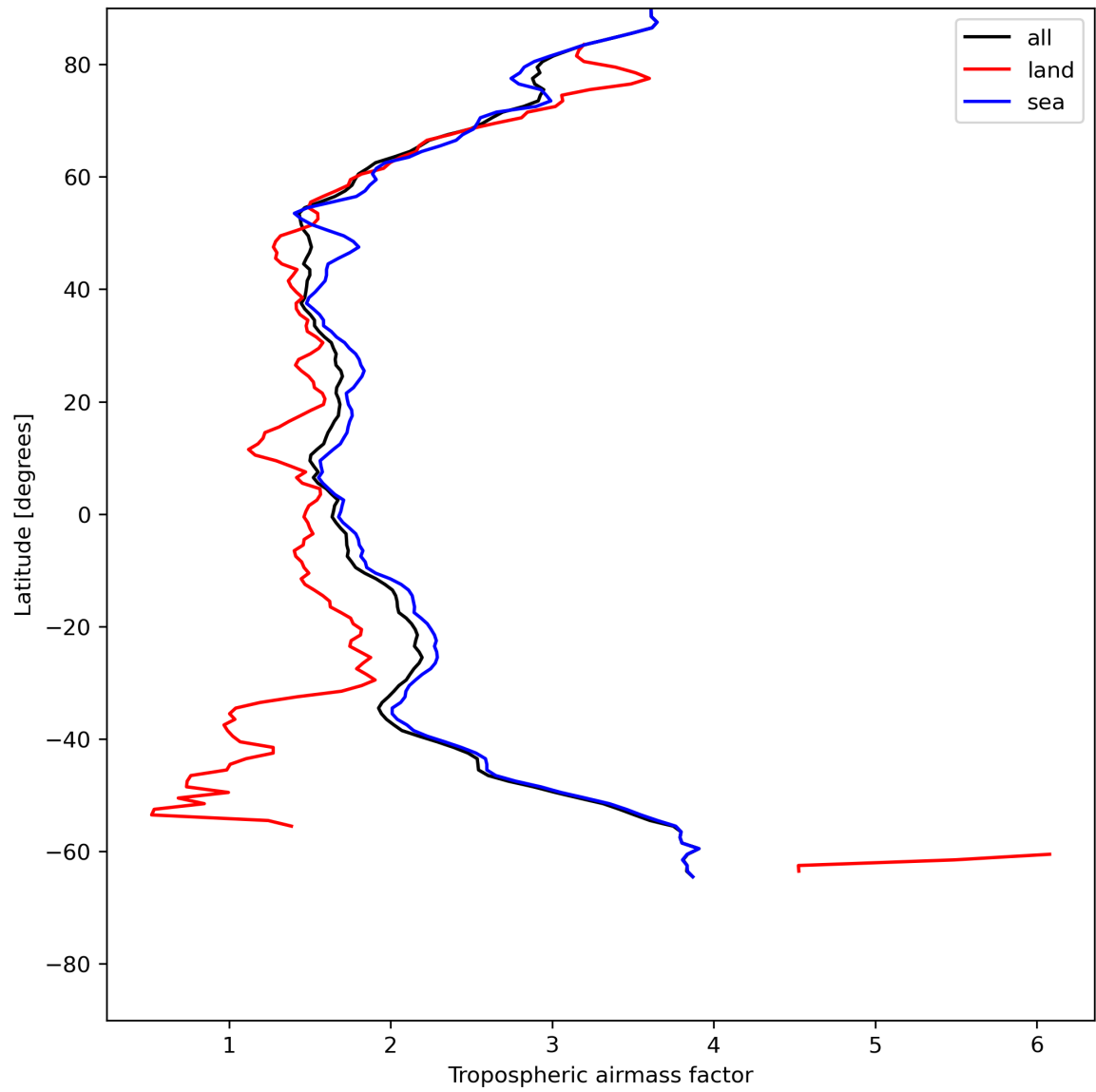
Figure 14: Zonal average of “Tropospheric airmass factor” for 2024-06-29 to 2024-06-30.
