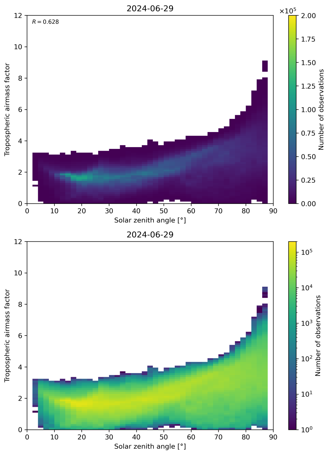
Figure 147: Scatter density plot of “Solar zenith angle” against “Tropospheric airmass factor” for 2024-06-29 to 2024-06-30.
