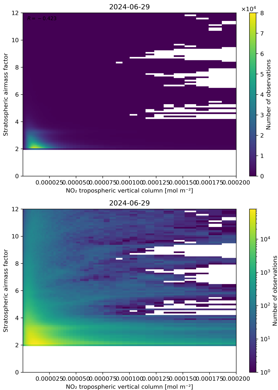
Figure 121: Scatter density plot of “NO 2 tropospheric vertical column” against “Stratospheric air mass factor” for 2024-06-29 to 2024-06-30.
