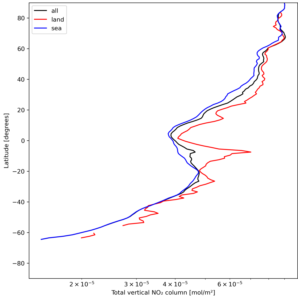
Figure 21: Zonal average of “Total vertical NO 2 column” for 2024-06-29 to 2024-06-30.
