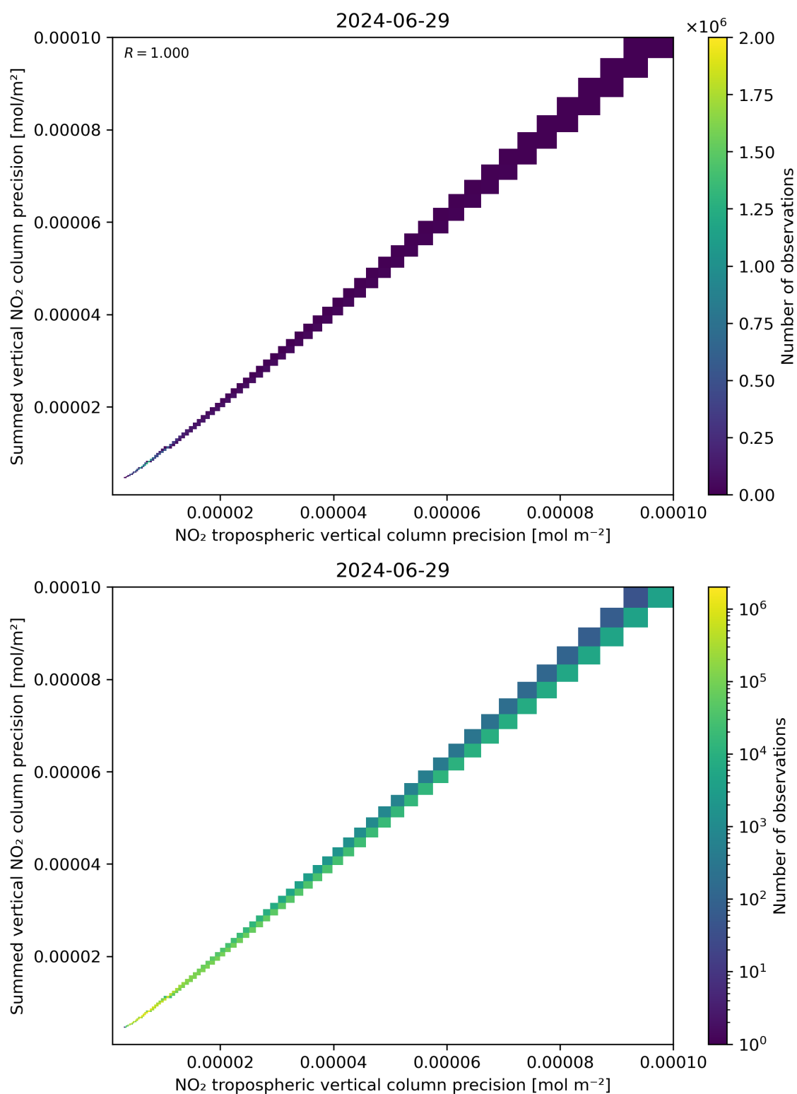
Figure 137: Scatter density plot of “NO 2 tropospheric vertical column precision” against “Summed vertical NO 2 column precision” for 2024-06-29 to 2024-06-30.
