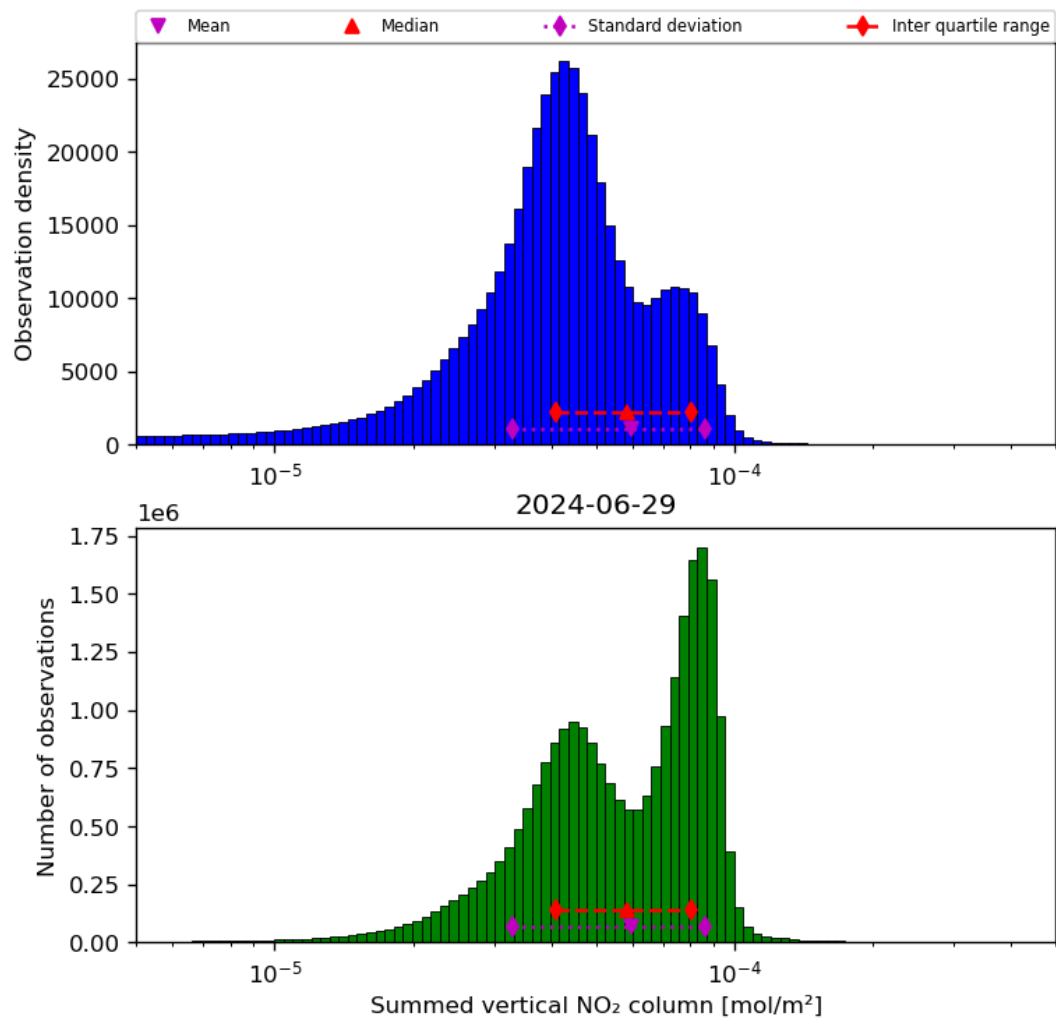
Figure 40: Histogram of “Summed vertical NO 2 column” for 2024-06-29 to 2024-06-30
