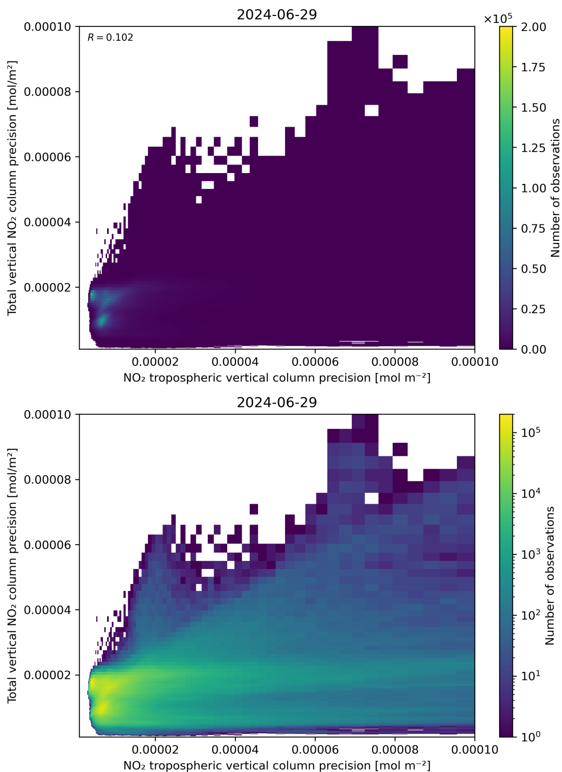
Figure 139: Scatter density plot of “NO 2 tropospheric vertical column precision” against “Total vertical NO 2 column precision” for 2024-06-29 to 2024-06-30.
