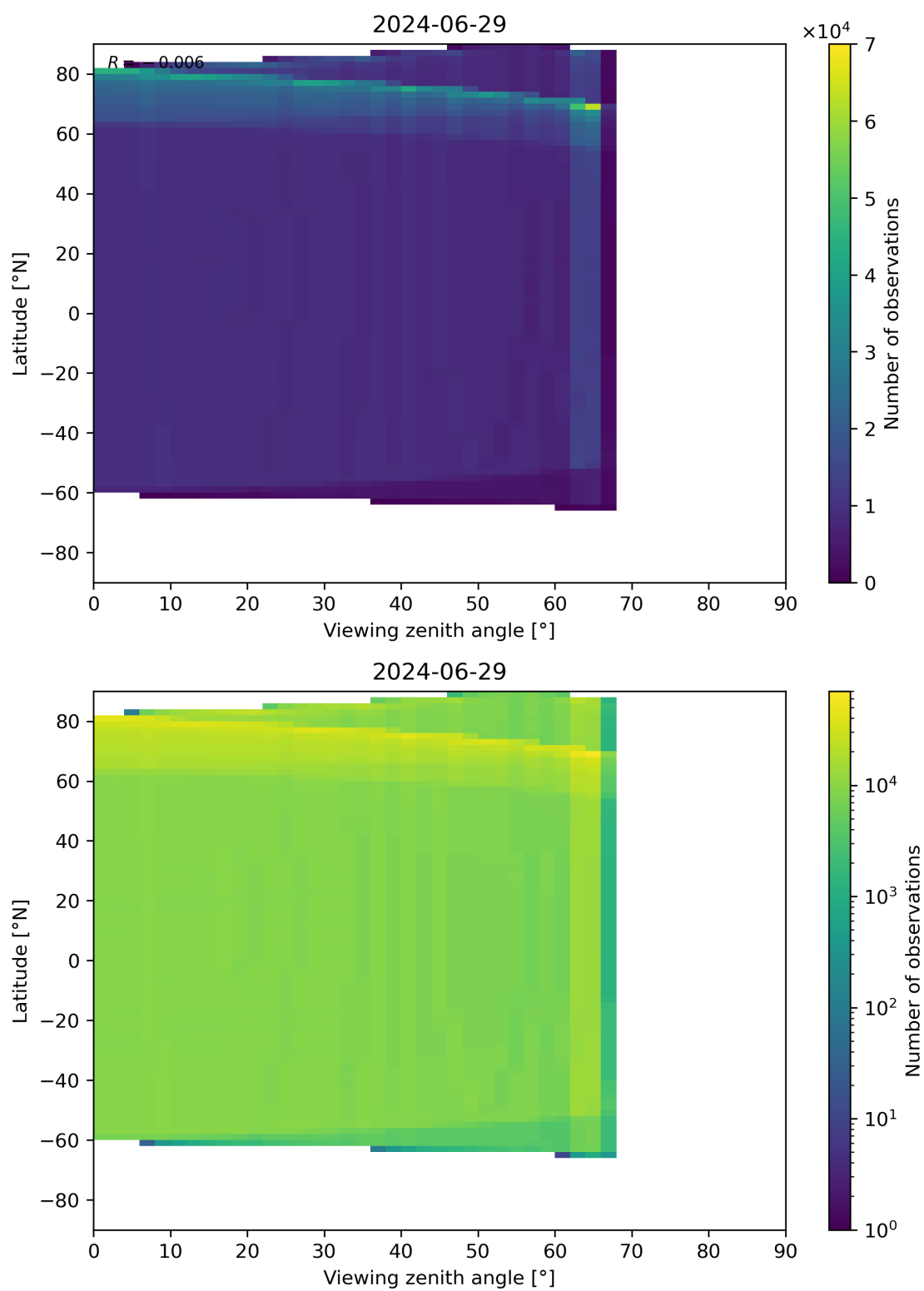
Figure 163: Scatter density plot of “Viewing zenith angle” against “Latitude” for 2024-06-29 to 2024-06-30.
