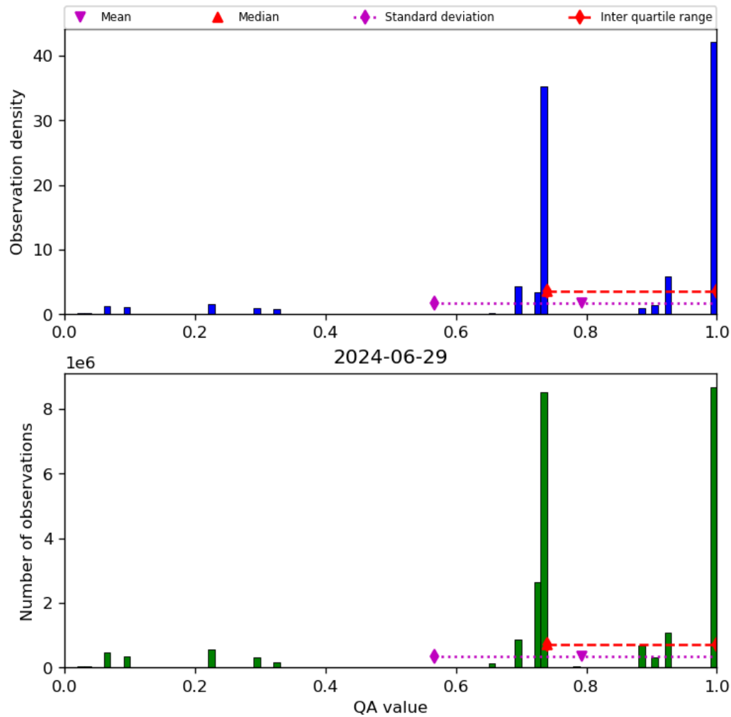
Figure 28: Histogram of “QA value” for 2024-06-29 to 2024-06-30
