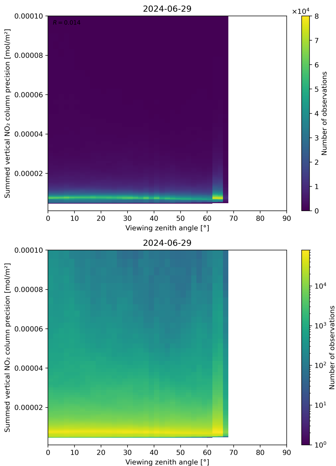
Figure 166: Scatter density plot of “Viewing zenith angle” against “Summed vertical NO 2 column precision” for 2024-06-29 to 2024-06-30.
