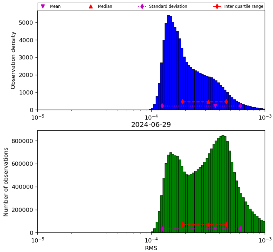
Figure 43: Histogram of “RMS” for 2024-06-29 to 2024-06-30
