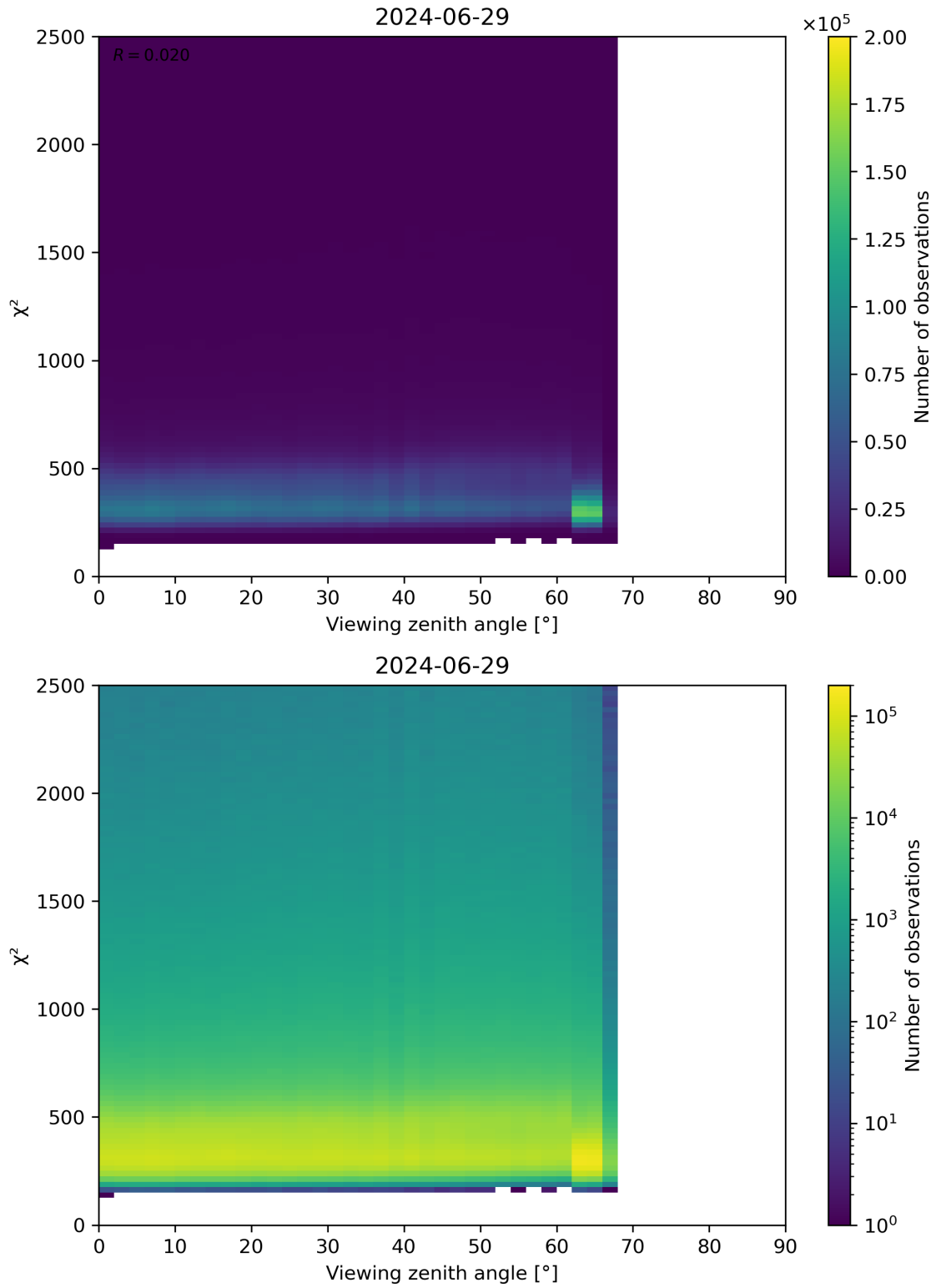
Figure 162: Scatter density plot of “Viewing zenith angle” against “ \chi^2 ” for 2024-06-29 to 2024-06-30.
