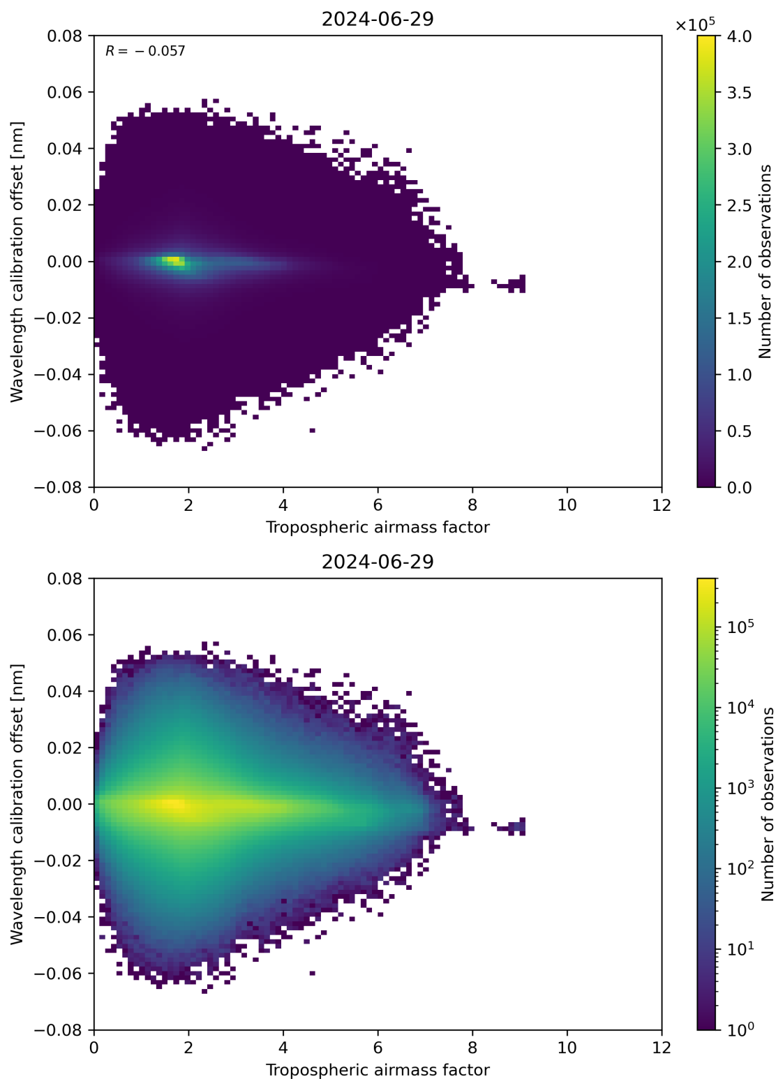
Figure 80: Scatter density plot of “Tropospheric airmass factor” against “Wavelength calibration offset” for 2024-06-29 to 2024-06-30.
