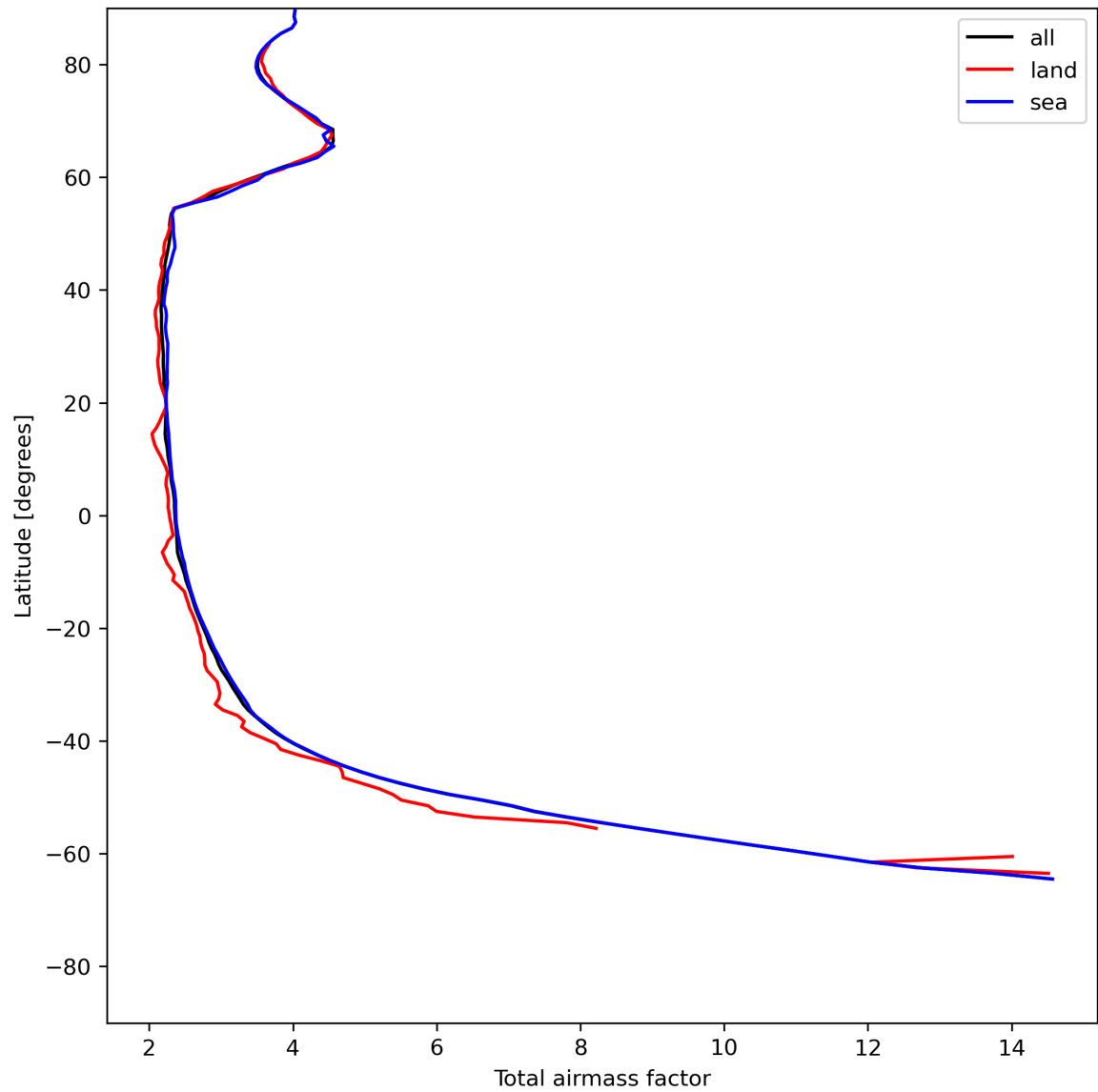
Figure 15: Zonal average of “Total airmass factor” for 2024-06-29 to 2024-06-30.
