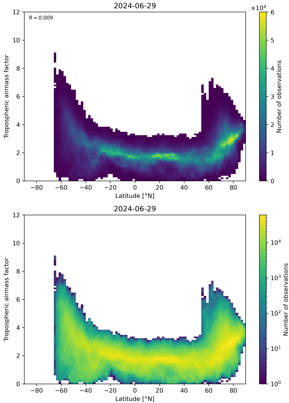
Figure 85: Scatter density plot of “Latitude” against “Tropospheric airmass factor” for 2024-06-29 to 2024-06-30.
