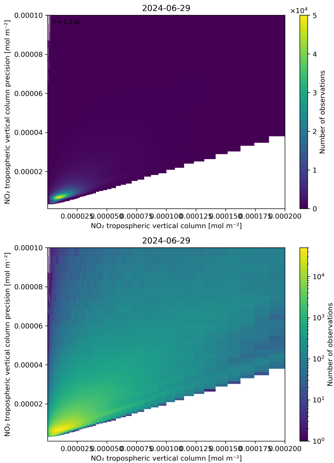
Figure 130: Scatter density plot of “NO 2 tropospheric vertical column” against “NO 2 tropospheric vertical column precision” for 2024-06-29 to 2024-06-30.
