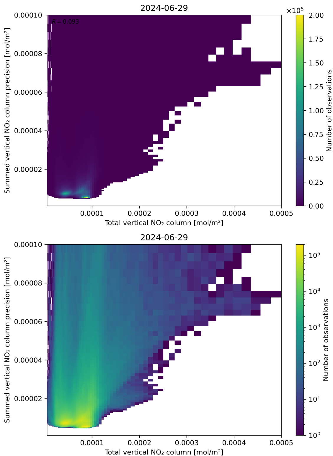
Figure 113: Scatter density plot of “Total vertical NO 2 column” against “Summed vertical NO 2 column precision” for 2024-06-29 to 2024-06-30.
