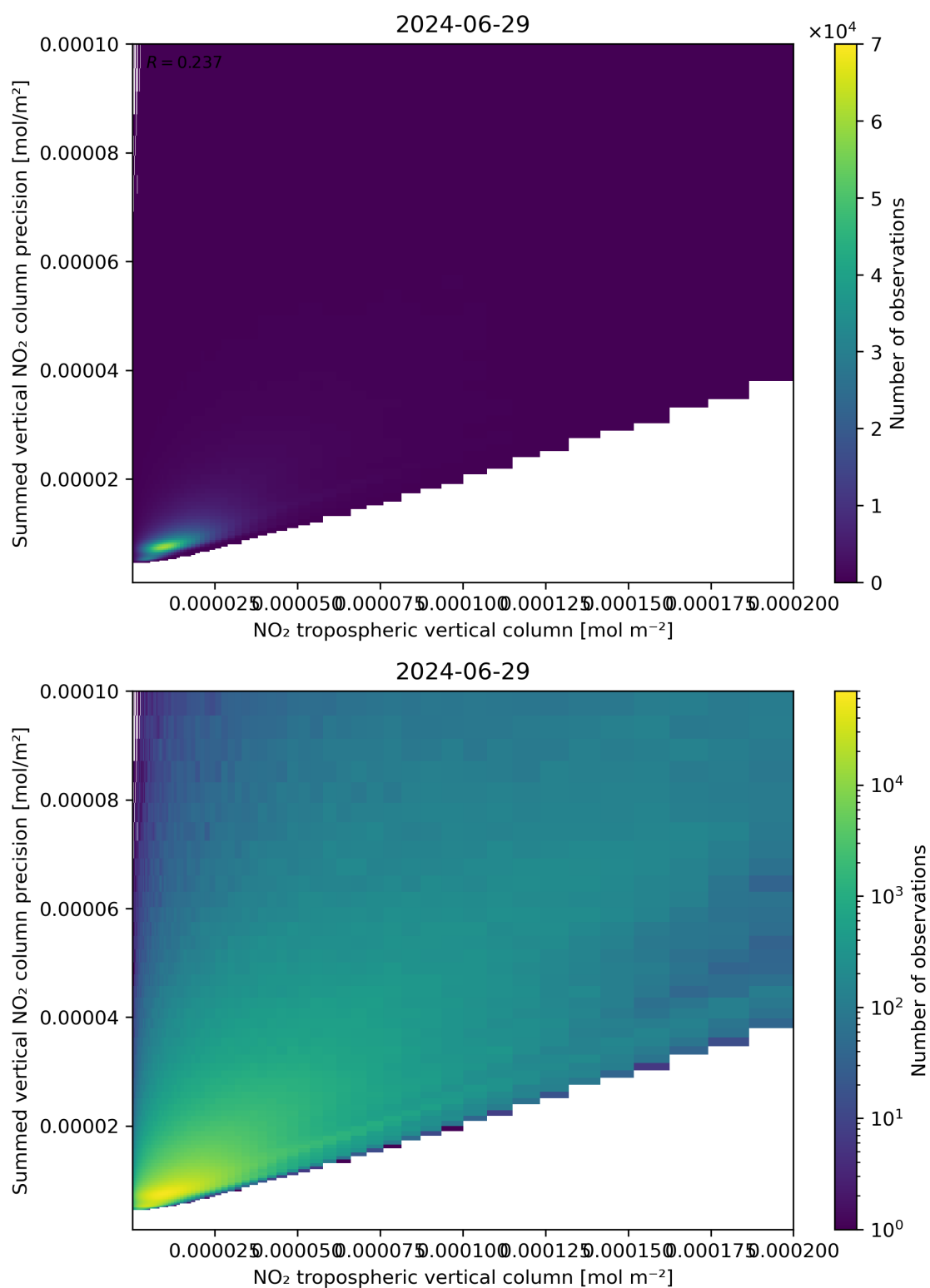
Figure 127: Scatter density plot of “NO 2 tropospheric vertical column” against “Summed vertical NO 2 column precision” for 2024-06-29 to 2024-06-30.
