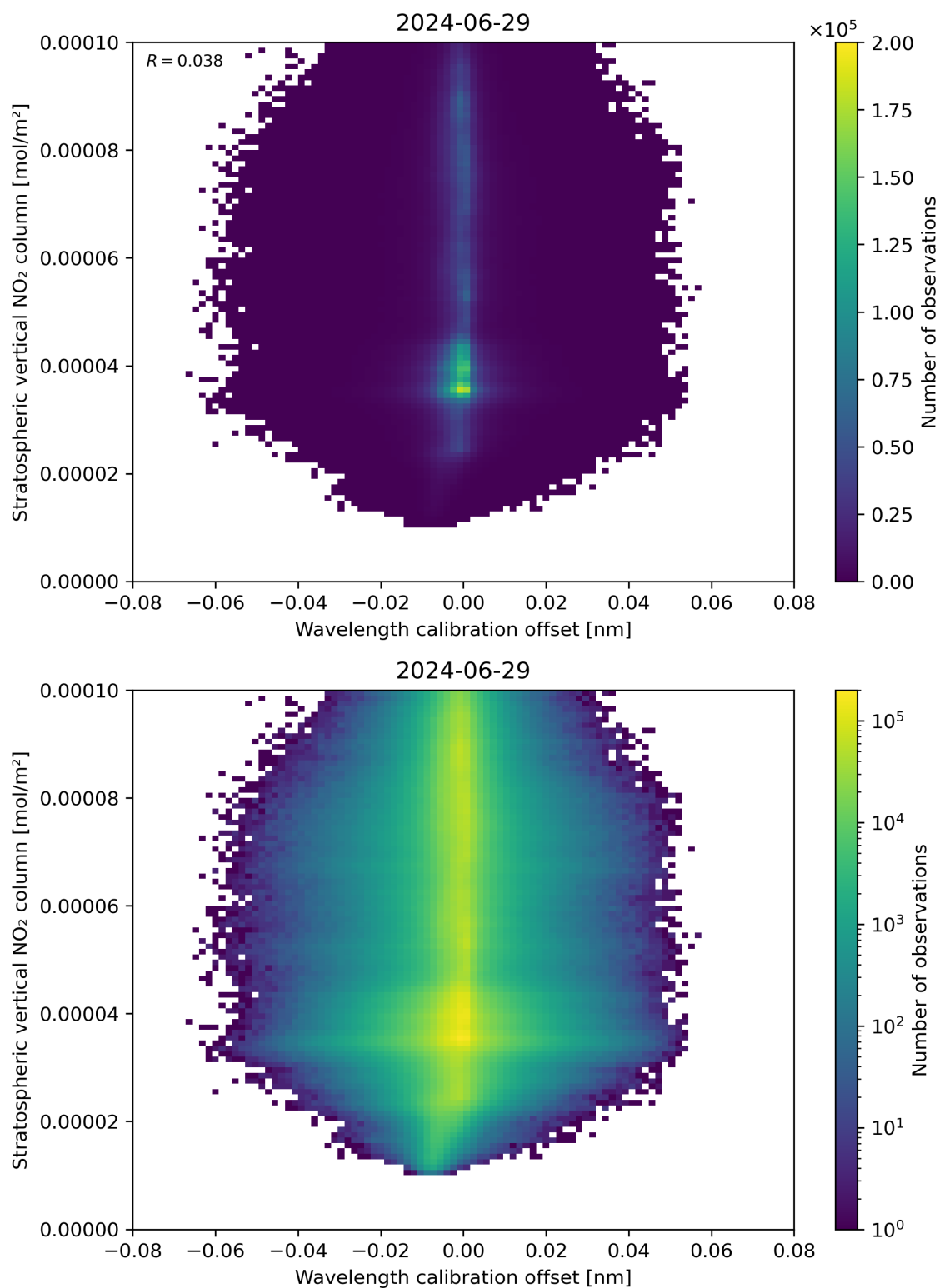
Figure 176: Scatter density plot of “Wavelength calibration offset” against “Stratospheric vertical NO 2 column” for 2024-06-29 to 2024-06-30.
