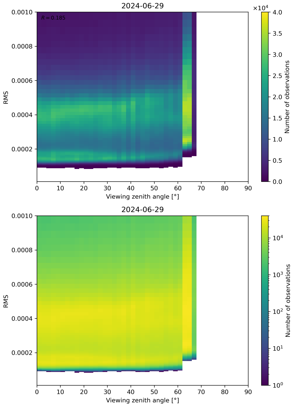
Figure 171: Scatter density plot of “Viewing zenith angle” against “RMS” for 2024-06-29 to 2024-06-30.
