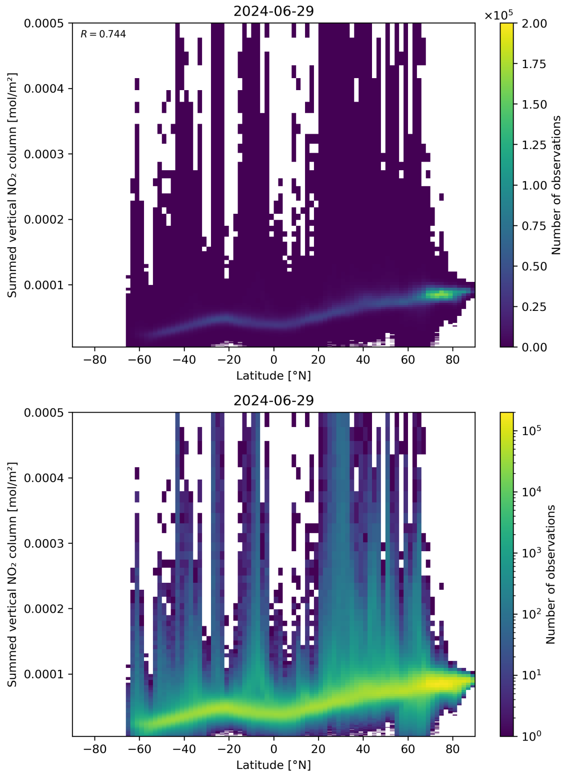
Figure 88: Scatter density plot of “Latitude” against “Summed vertical NO 2 column” for 2024-06-29 to 2024-06-30.
