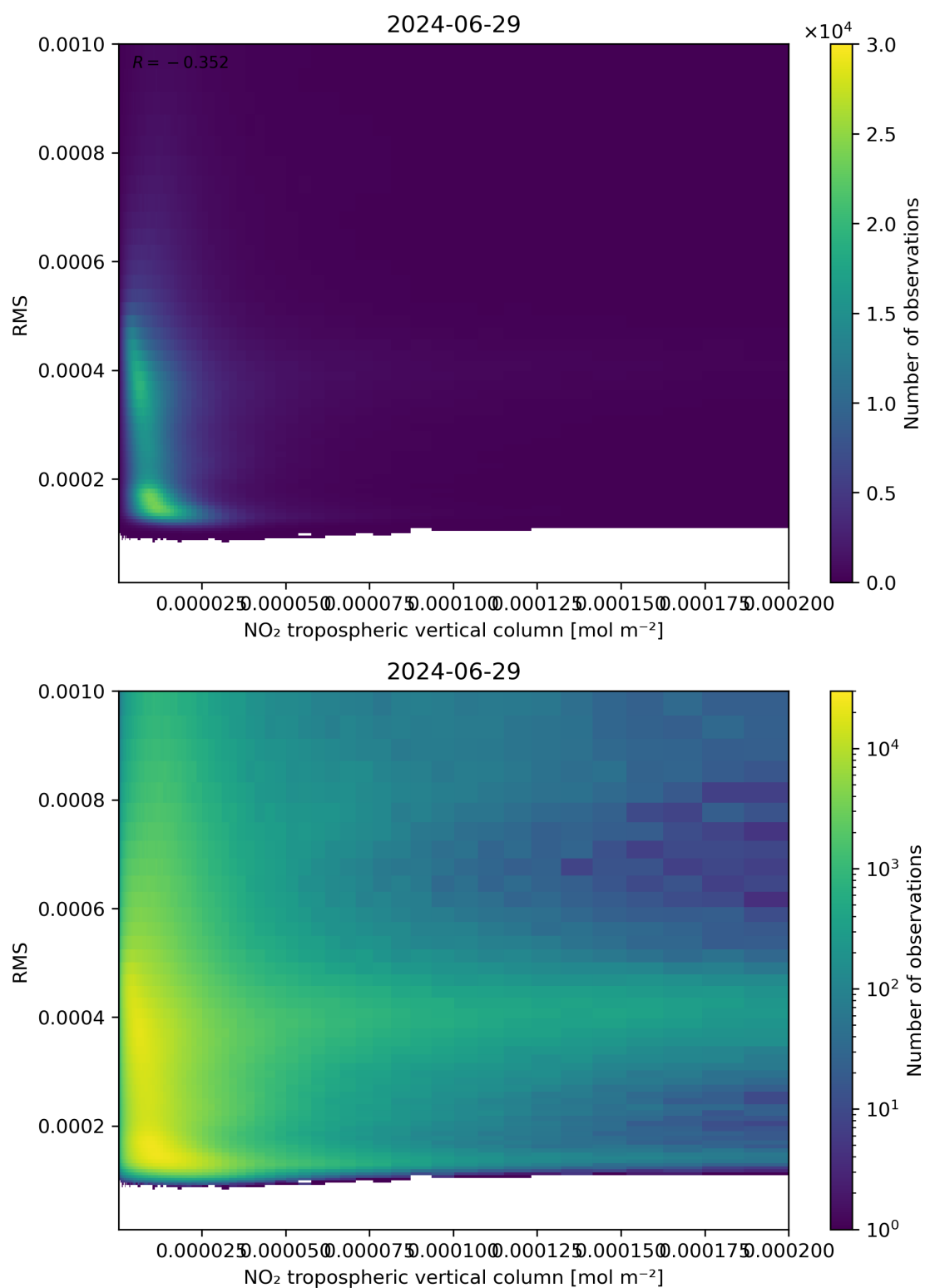
Figure 142: Scatter density plot of “NO 2 tropospheric vertical column” against “RMS” for 2024-06-29 to 2024-06-30.
