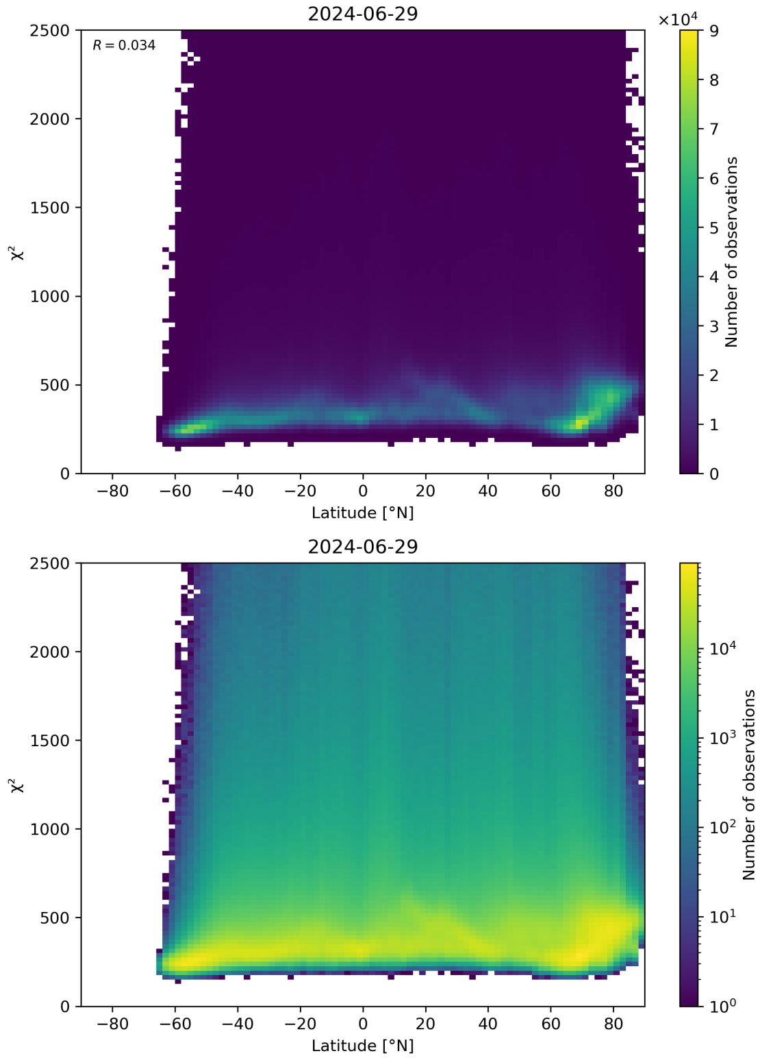
Figure 86: Scatter density plot of “Latitude” against “ \chi^2 ” for 2024-06-29 to 2024-06-30.
