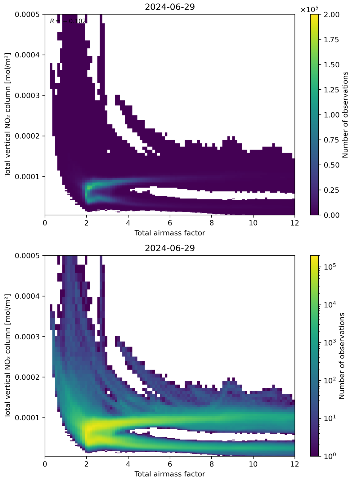
Figure 67: Scatter density plot of “Total airmass factor” against “Total vertical NO 2 column” for 2024-06-29 to 2024-06-30.
