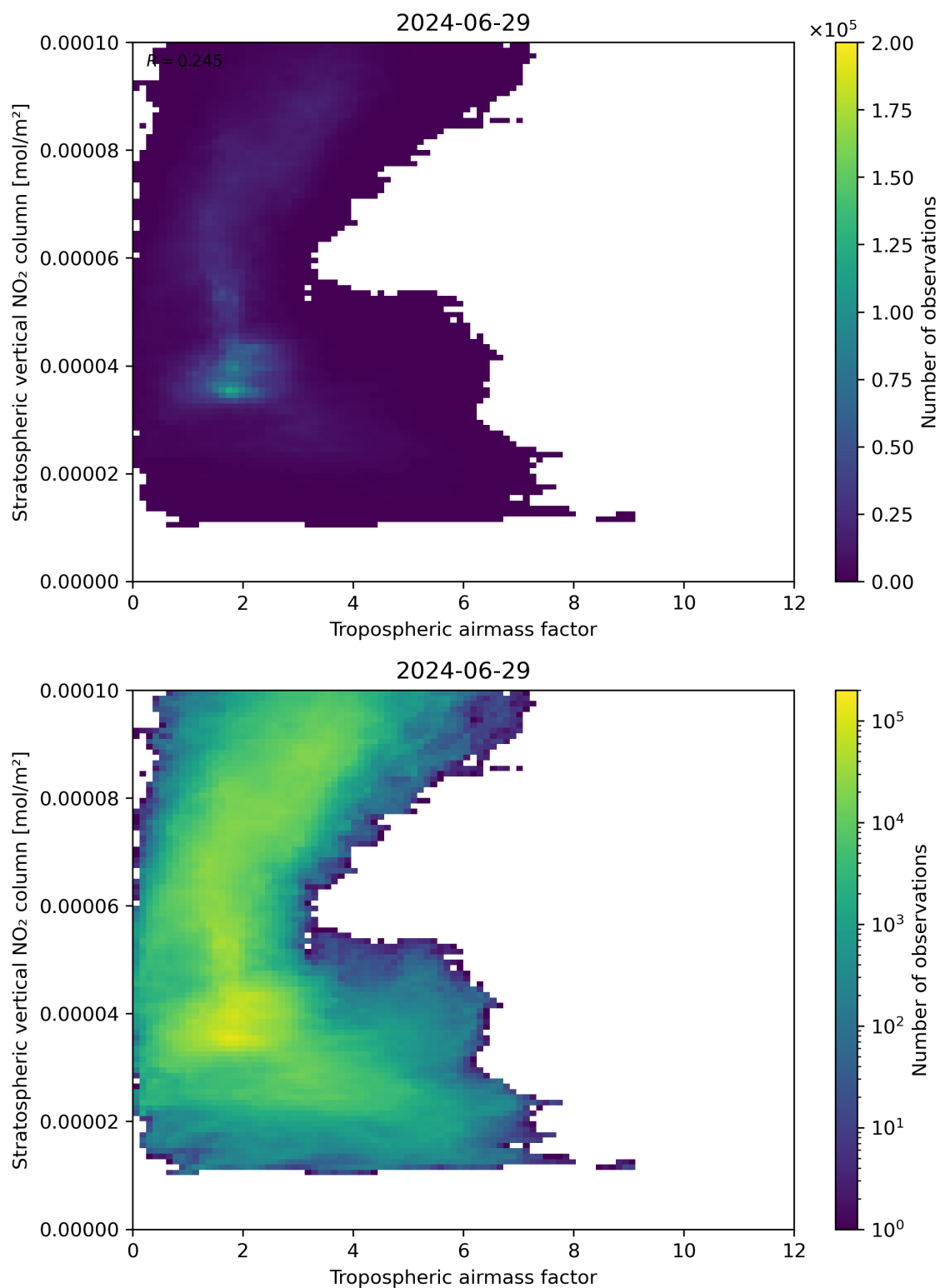
Figure 74: Scatter density plot of “Tropospheric air mass factor” against “Stratospheric vertical NO 2 column” for 2024-06-29 to 2024-06-30.
