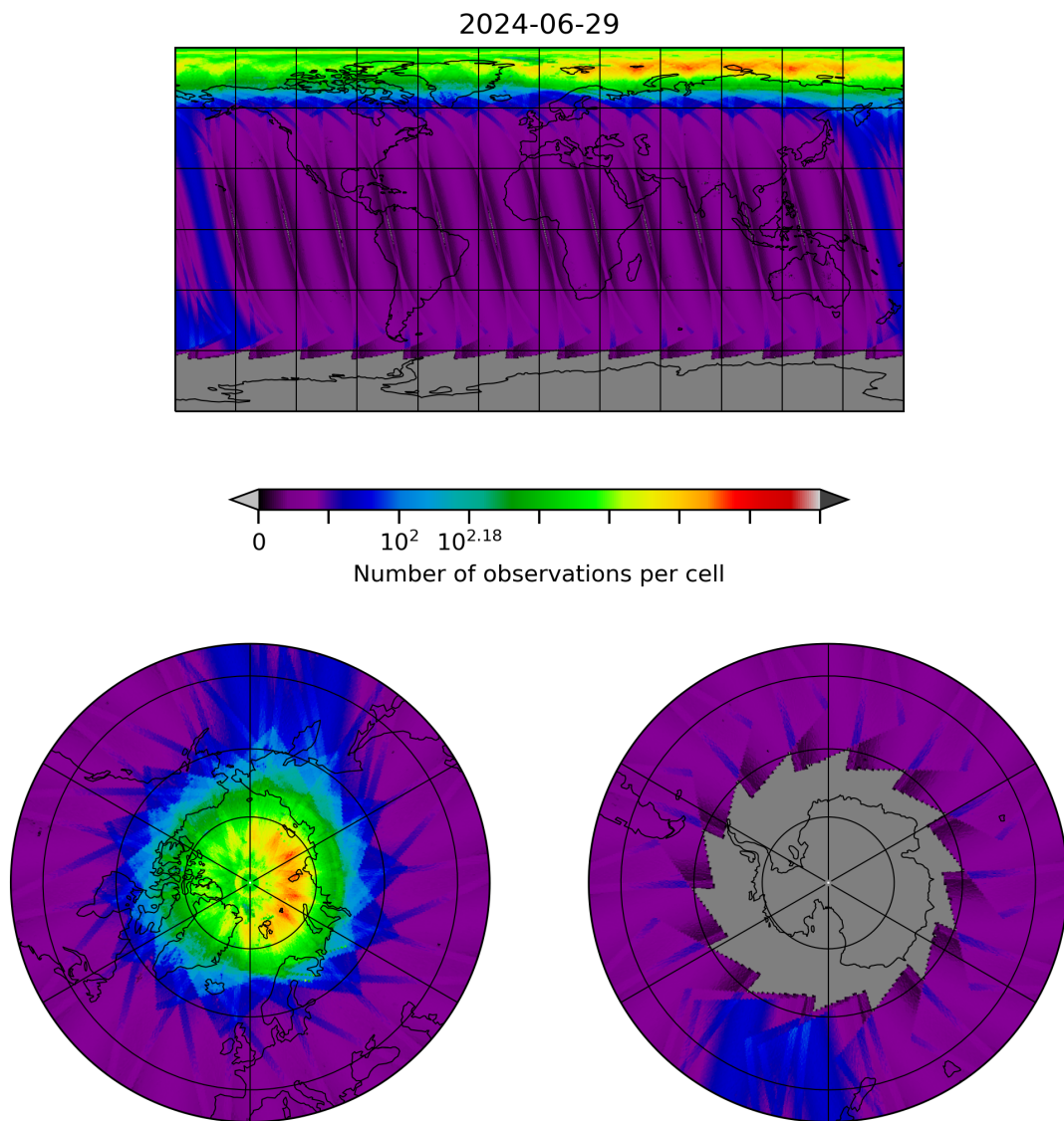
Figure 10: Map of the number of observations for 2024-06-29 to 2024-06-30
