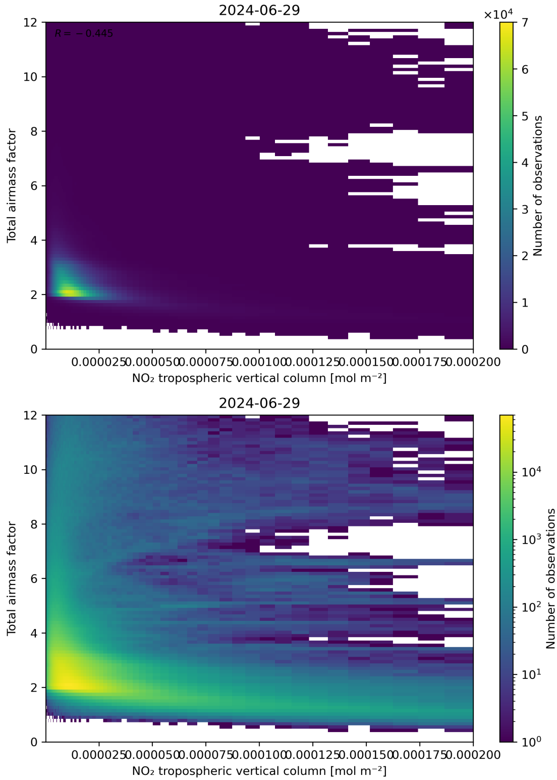
Figure 122: Scatter density plot of “NO 2 tropospheric vertical column” against “Total air mass factor” for 2024-06-29 to 2024-06-30.
