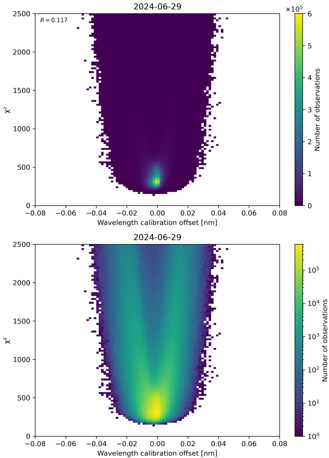
Figure 175: Scatter density plot of “Wavelength calibration offset” against “ \chi^2 ” for 2024-06-29 to 2024-06-30.
