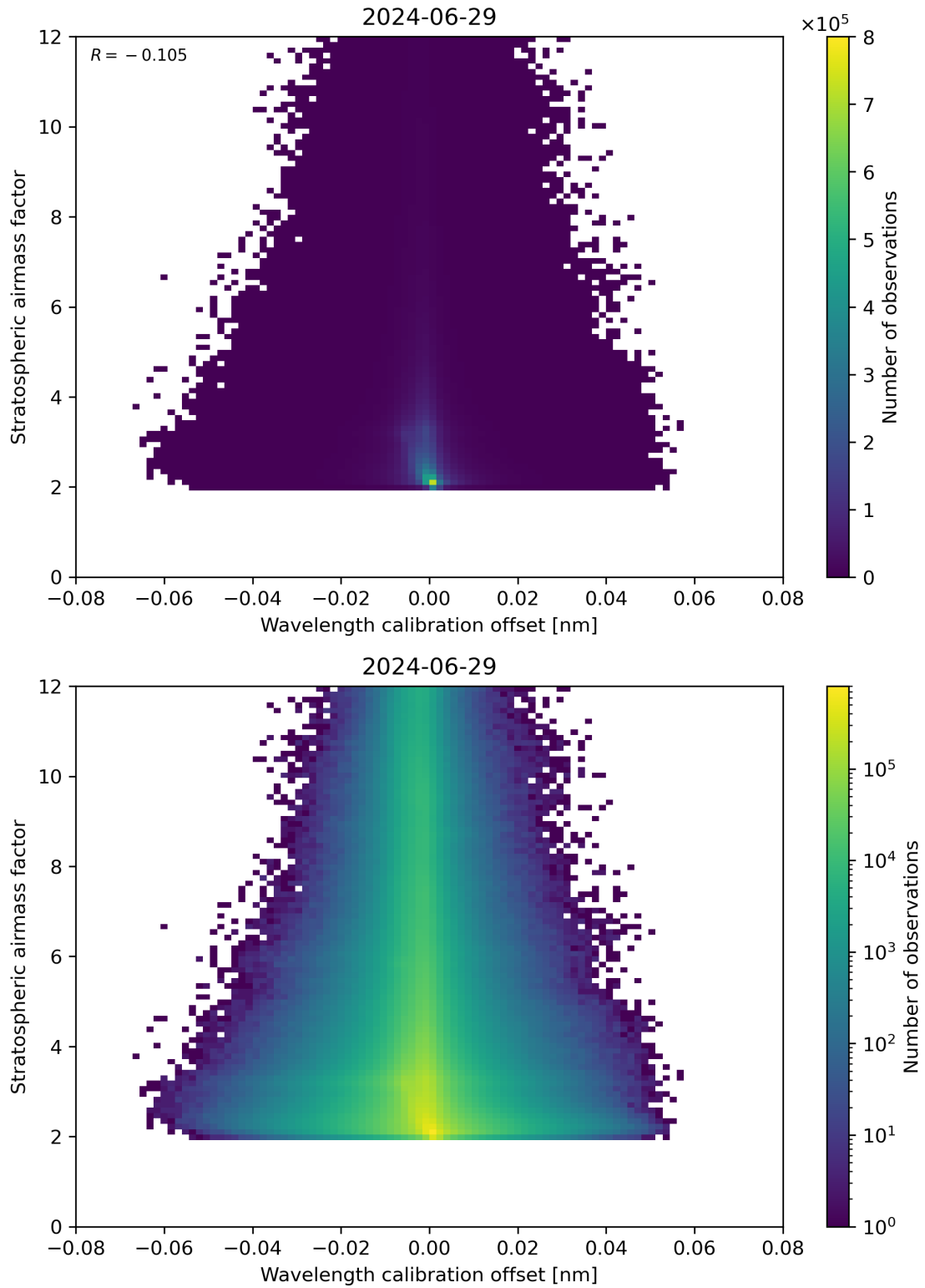
Figure 174: Scatter density plot of “Wavelength calibration offset” against “Stratospheric airmass factor” for 2024-06-29 to 2024-06-30.
