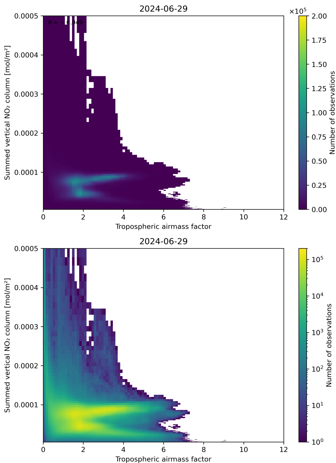
Figure 75: Scatter density plot of “Tropospheric air mass factor” against “Summed vertical NO 2 column” for 2024-06-29 to 2024-06-30.
