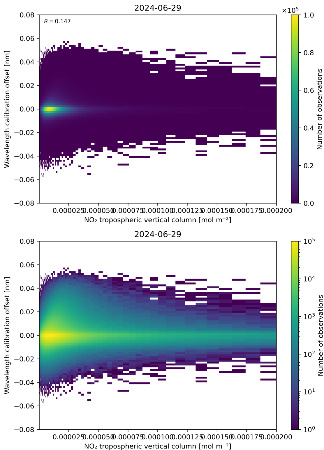
Figure 143: Scatter density plot of “NO 2 tropospheric vertical column” against “Wavelength calibration offset” for 2024-06-29 to 2024-06-30.
