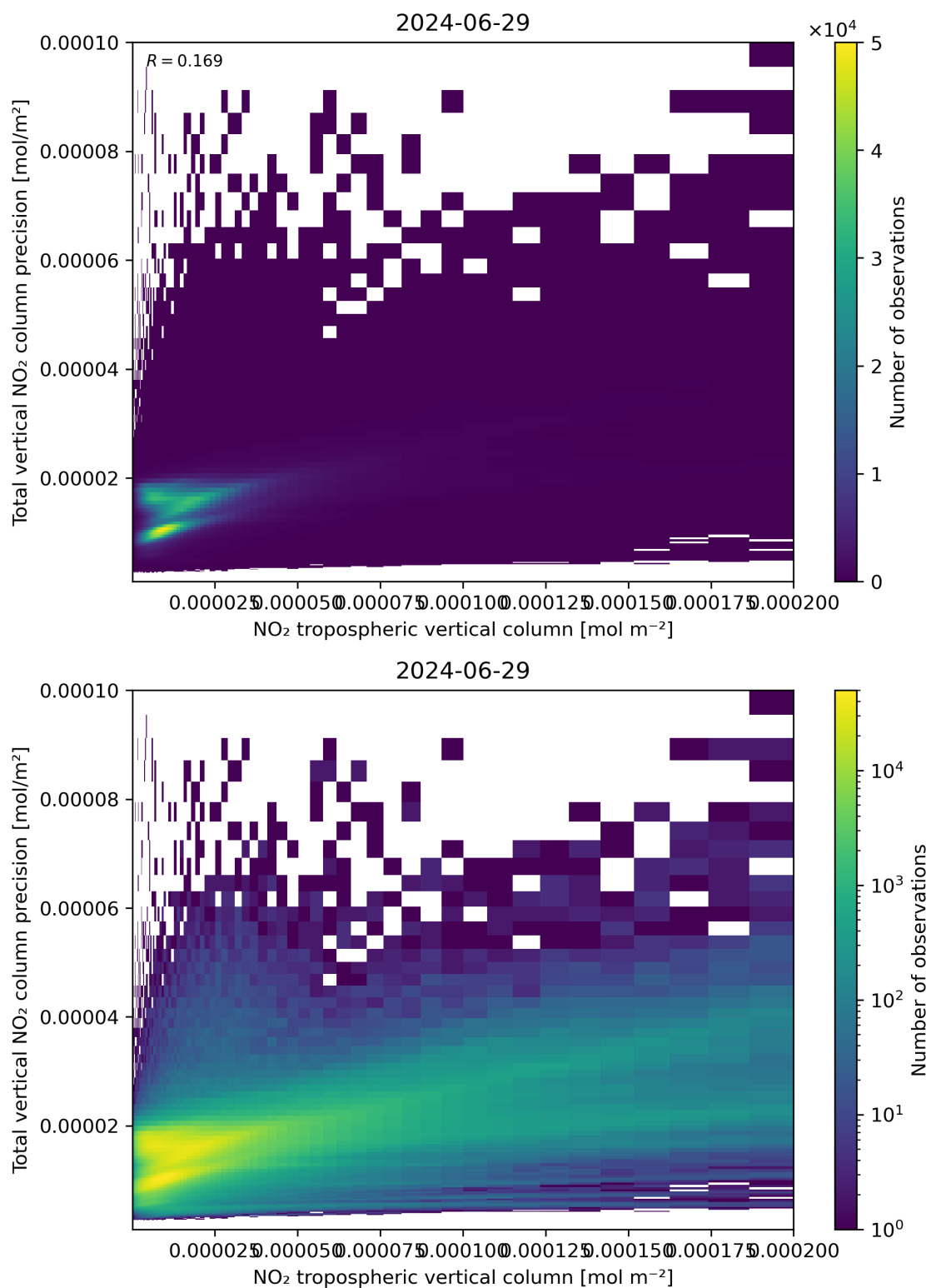
Figure 129: Scatter density plot of “NO 2 tropospheric vertical column” against “Total vertical NO 2 column precision” for 2024-06-29 to 2024-06-30.
