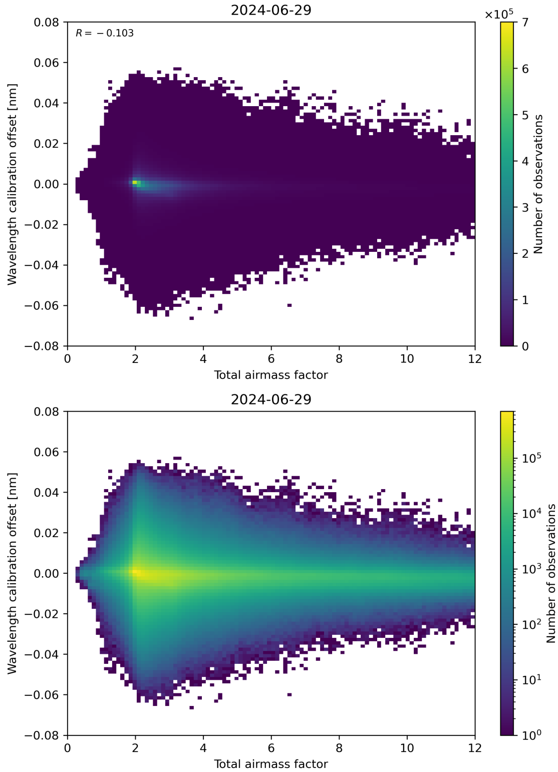
Figure 70: Scatter density plot of “Total airmass factor” against “Wavelength calibration offset” for 2024-06-29 to 2024-06-30.
