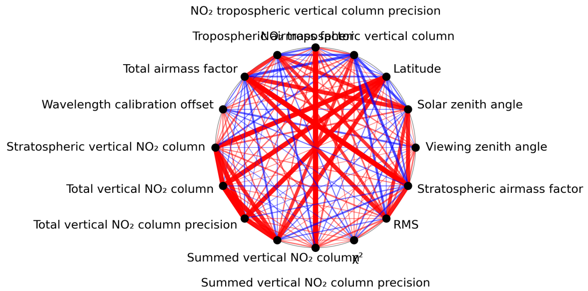
Figure 1: Map of correlation graph for 2024-06-29 to 2024-06-30.
