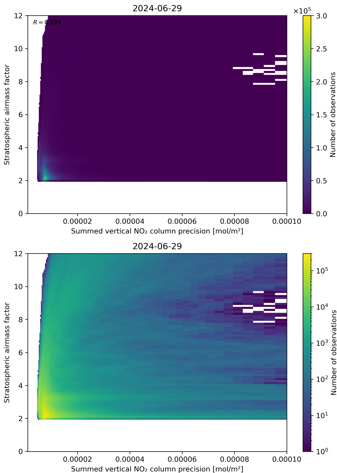
Figure 106: Scatter density plot of “Summed vertical NO 2 column precision” against “Stratospheric airmass factor” for 2024-06-29 to 2024-06-30.
