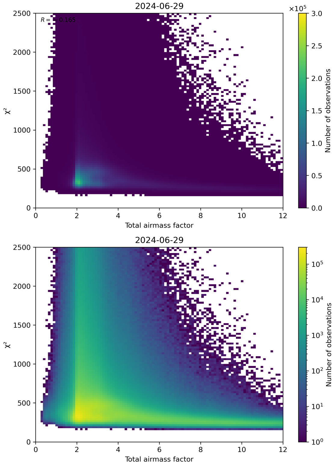
Figure 63: Scatter density plot of “Total airmass factor” against “ \chi^2 ” for 2024-06-29 to 2024-06-30.
