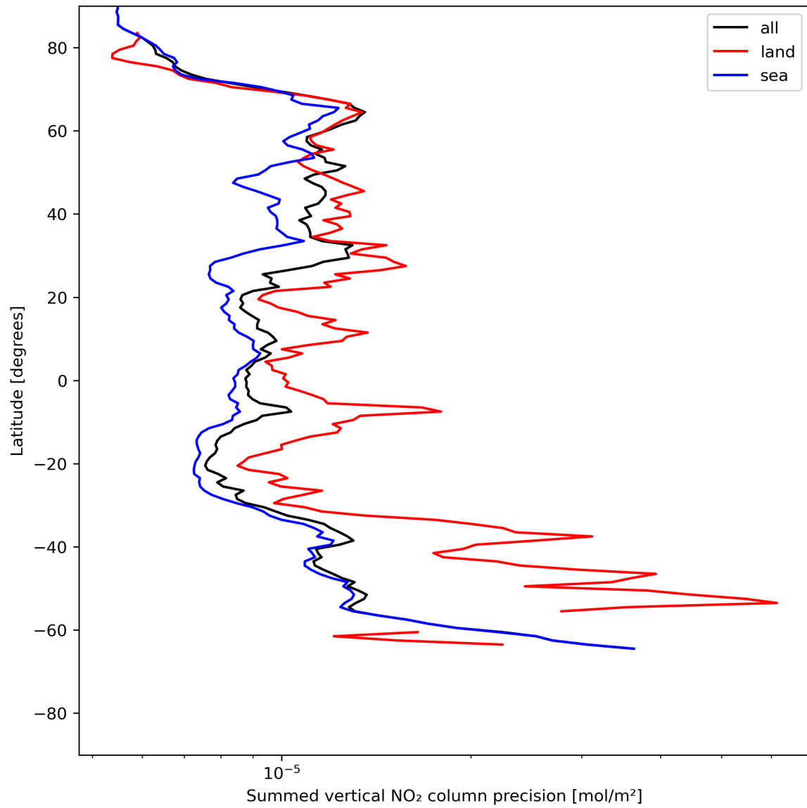
Figure 24: Zonal average of “Summed vertical NO 2 column precision” for 2024-06-29 to 2024-06-30.
