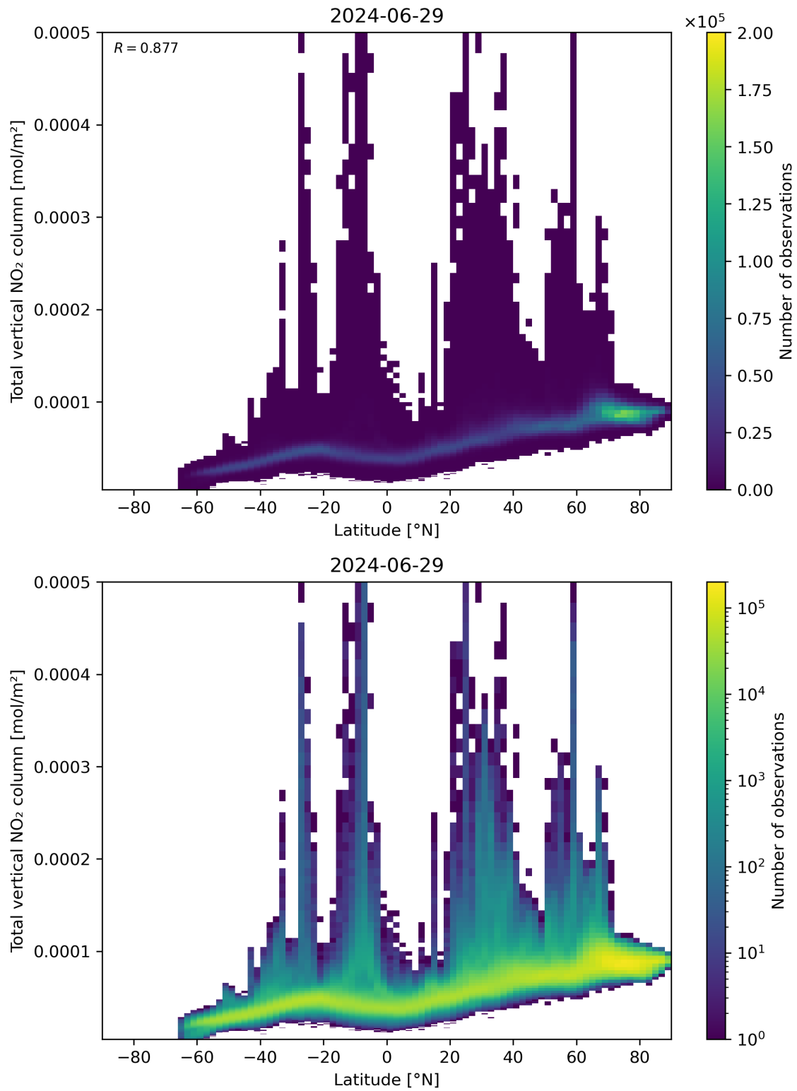
Figure 90: Scatter density plot of “Latitude” against “Total vertical NO 2 column” for 2024-06-29 to 2024-06-30.
