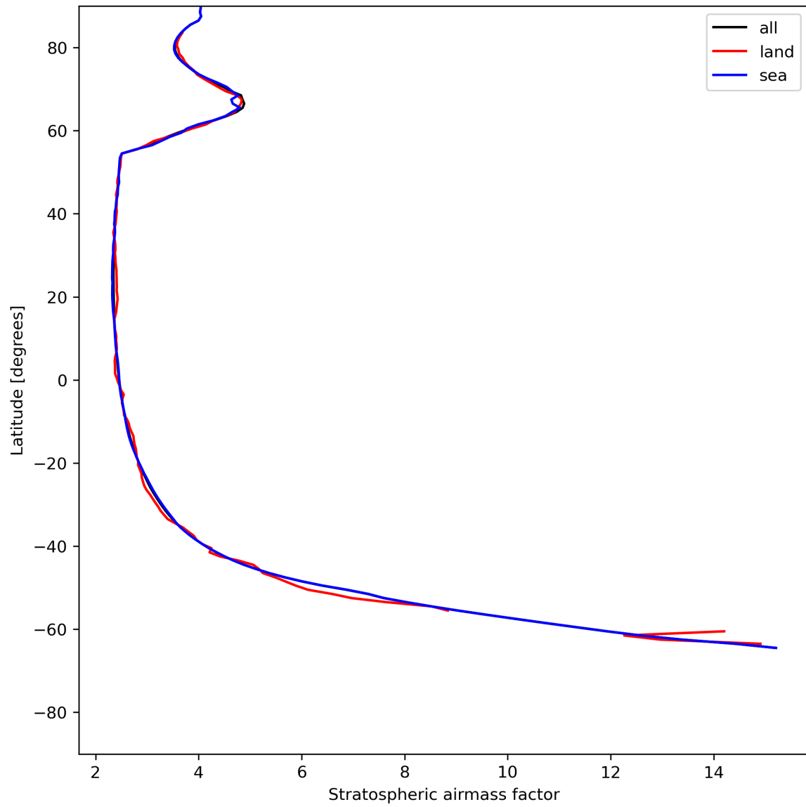
Figure 27: Zonal average of “Stratospheric airmass factor” for 2024-06-29 to 2024-06-30.
