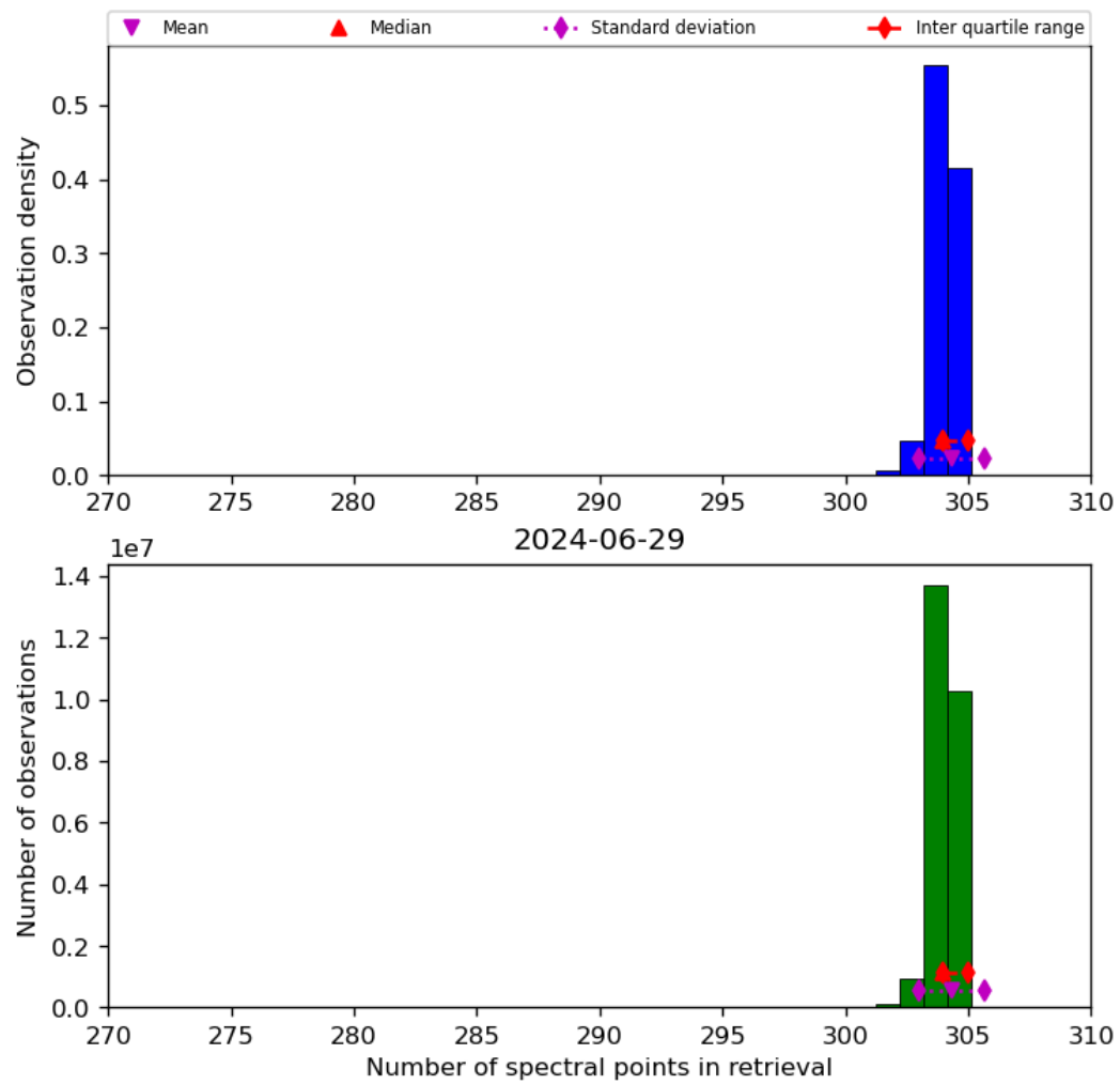
Figure 33: Histogram of “Number of spectral points in retrieval” for 2024-06-29 to 2024-06-30
