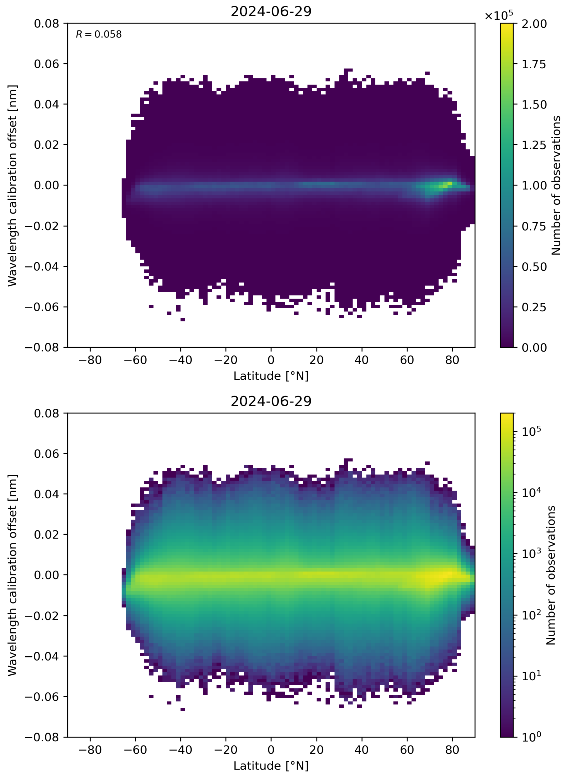
Figure 95: Scatter density plot of “Latitude” against “Wavelength calibration offset” for 2024-06-29 to 2024-06-30.
