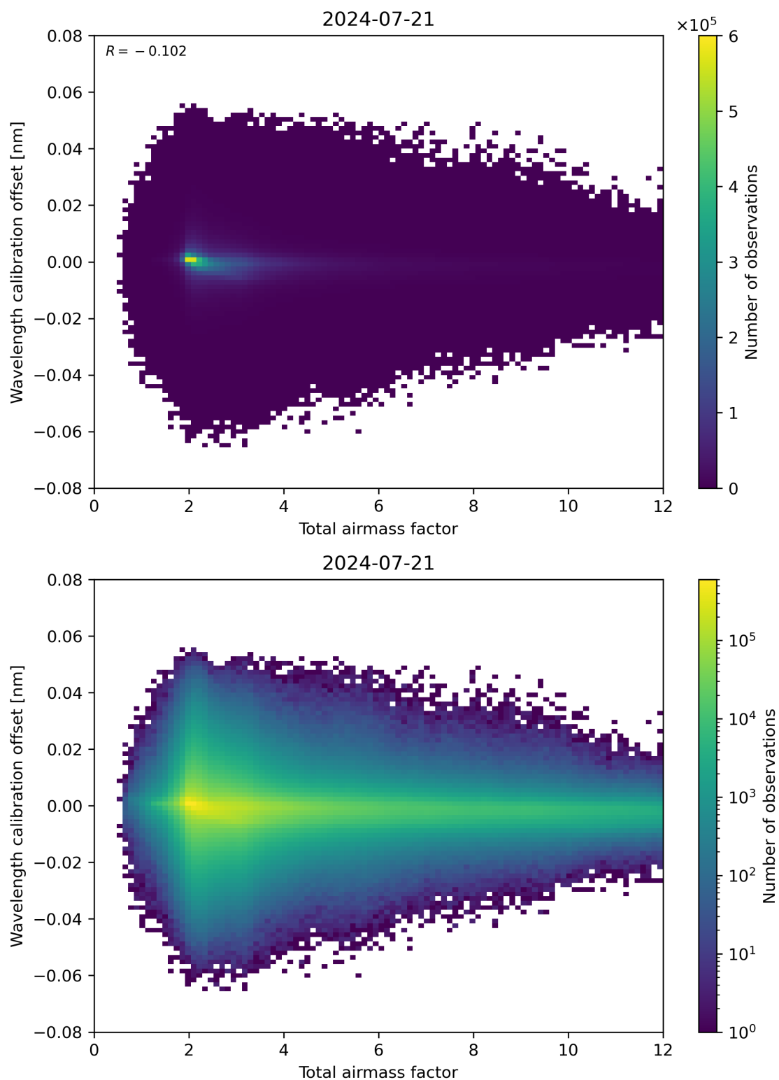
Figure 70: Scatter density plot of “Total airmass factor” against “Wavelength calibration offset” for 2024-07-21 to 2024-07-22.
