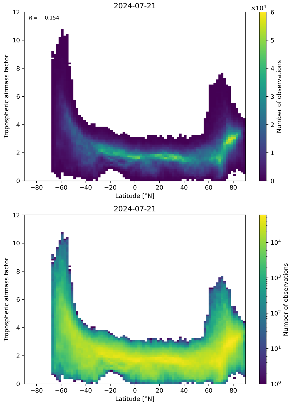
Figure 85: Scatter density plot of “Latitude” against “Tropospheric airmass factor” for 2024-07-21 to 2024-07-22.
