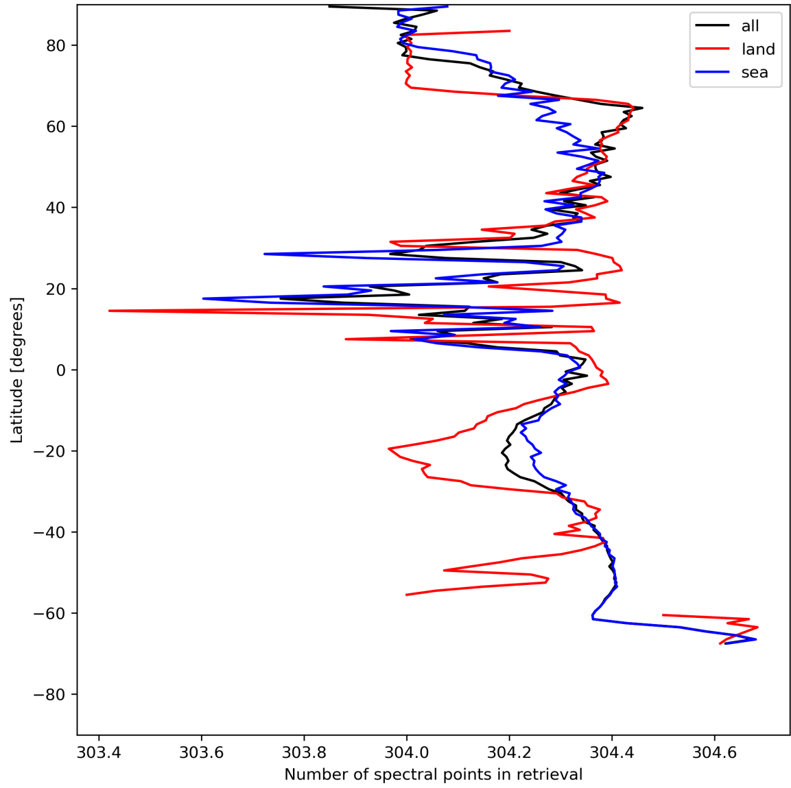
Figure 16: Zonal average of “Number of spectral points in retrieval” for 2024-07-21 to 2024-07-22.
