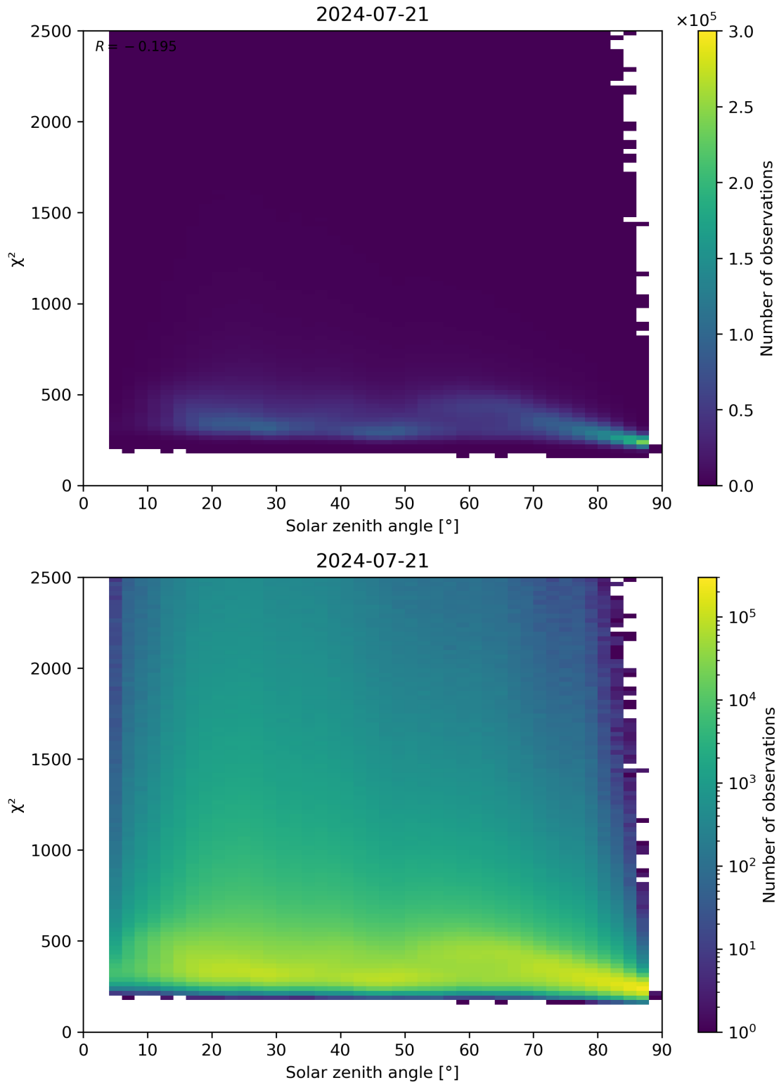
Figure 148: Scatter density plot of “Solar zenith angle” against “ \chi^2 ” for 2024-07-21 to 2024-07-22.
