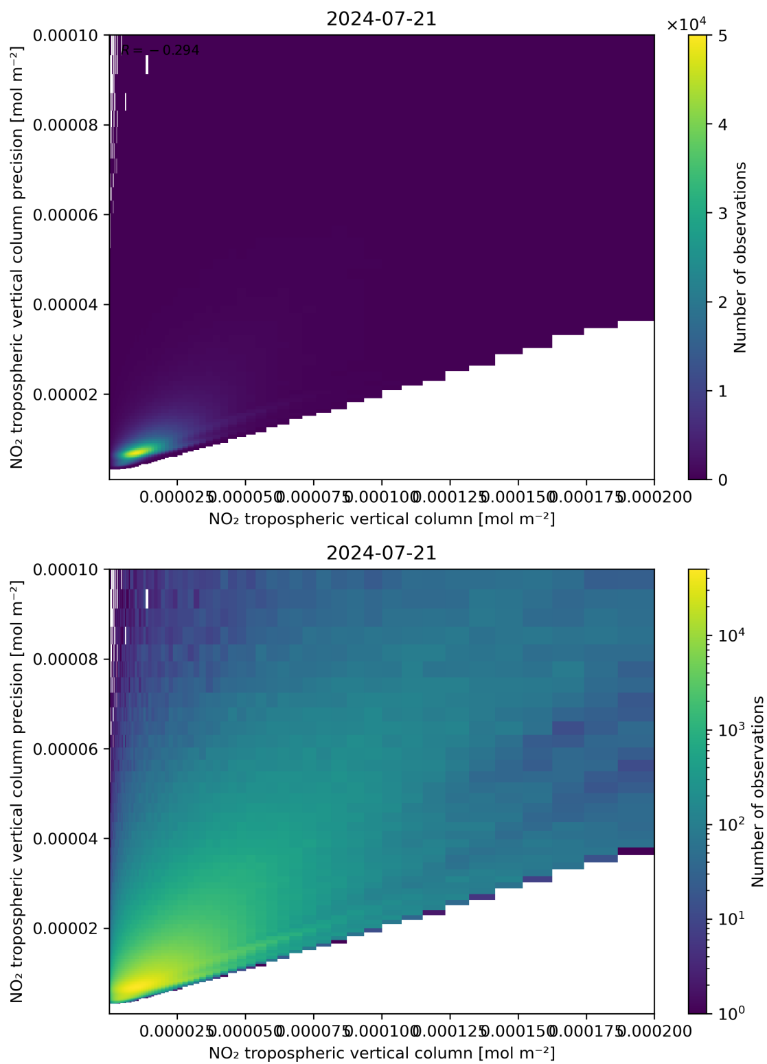
Figure 130: Scatter density plot of “NO 2 tropospheric vertical column” against “NO 2 tropospheric vertical column precision” for 2024-07-21 to 2024-07-22.
