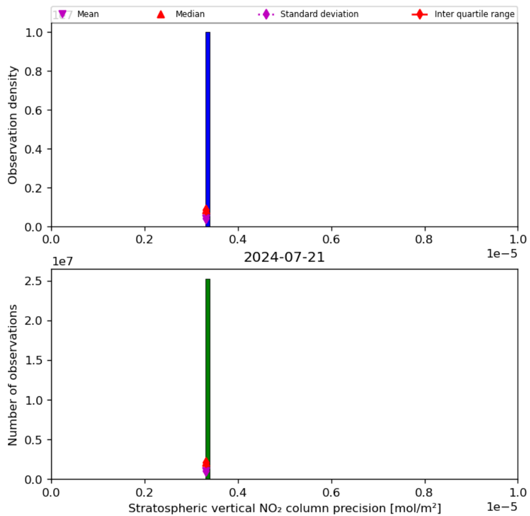
Figure 37: Histogram of “Stratospheric vertical NO 2 column precision” for 2024-07-21 to 2024-07-22
