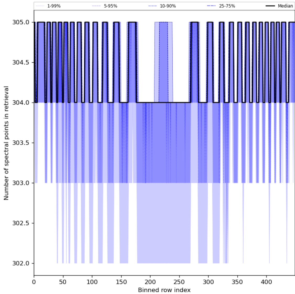
Figure 50: Along track statistics of “Number of spectral points in retrieval” for 2024-07-21 to 2024-07-22
