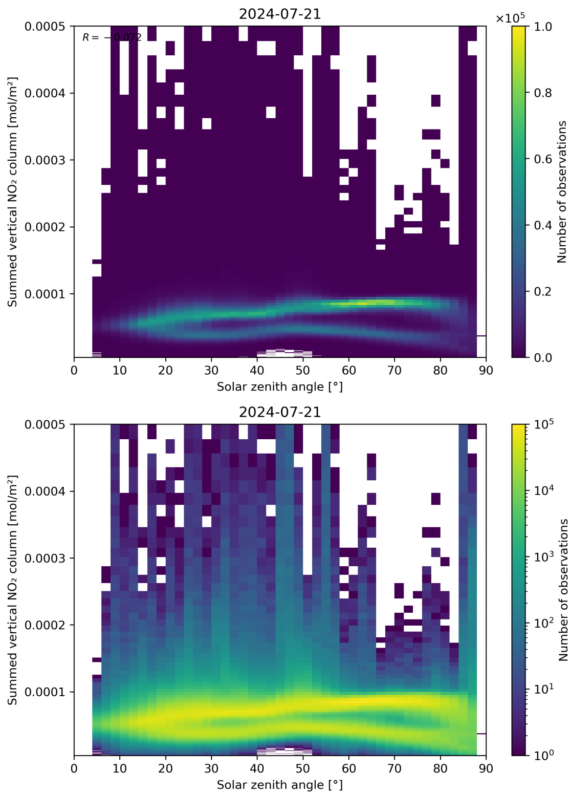
Figure 151: Scatter density plot of “Solar zenith angle” against “Summed vertical NO 2 column” for 2024-07-21 to 2024-07-22.
