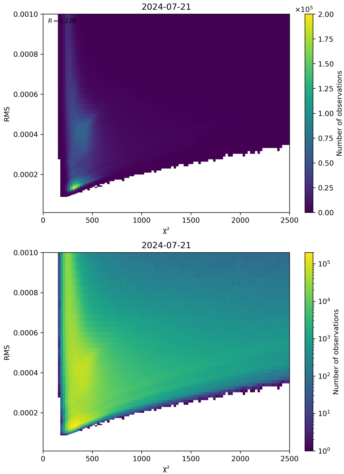
Figure 82: Scatter density plot of “ \chi^2 ” against “RMS” for 2024-07-21 to 2024-07-22.
