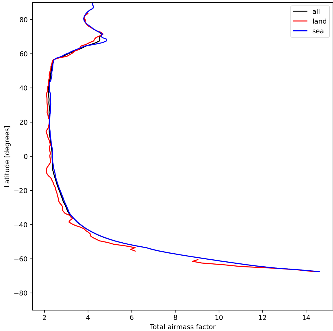
Figure 15: Zonal average of “Total airmass factor” for 2024-07-21 to 2024-07-22.
