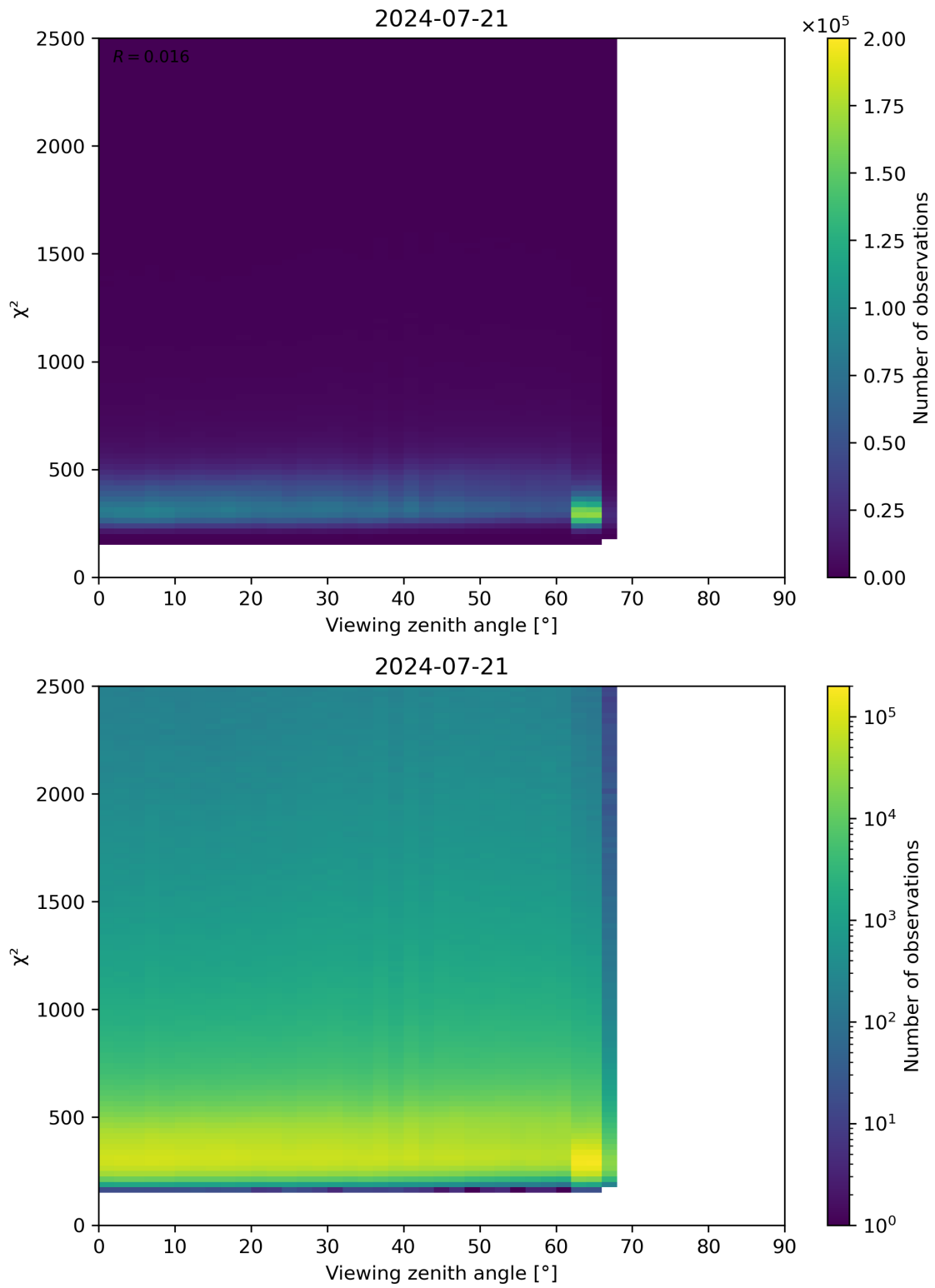
Figure 162: Scatter density plot of “Viewing zenith angle” against “ \chi^2 ” for 2024-07-21 to 2024-07-22.
