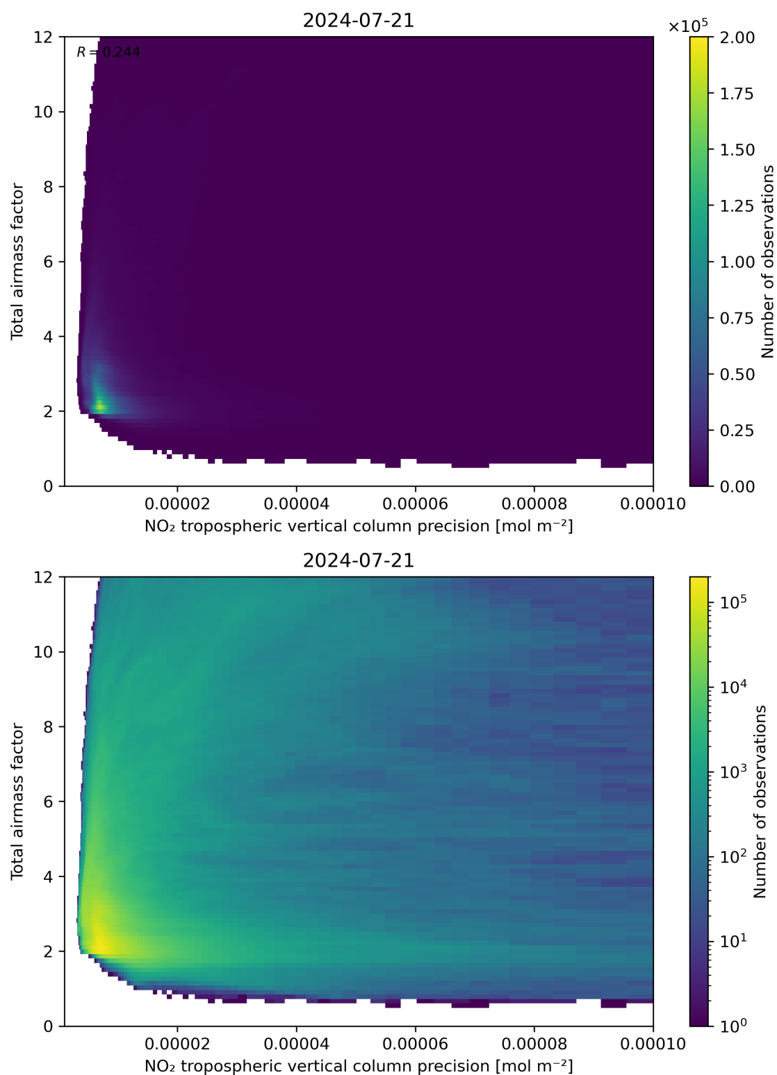
Figure 132: Scatter density plot of “NO 2 tropospheric vertical column precision” against “Total air mass factor” for 2024-07-21 to 2024-07-22.
