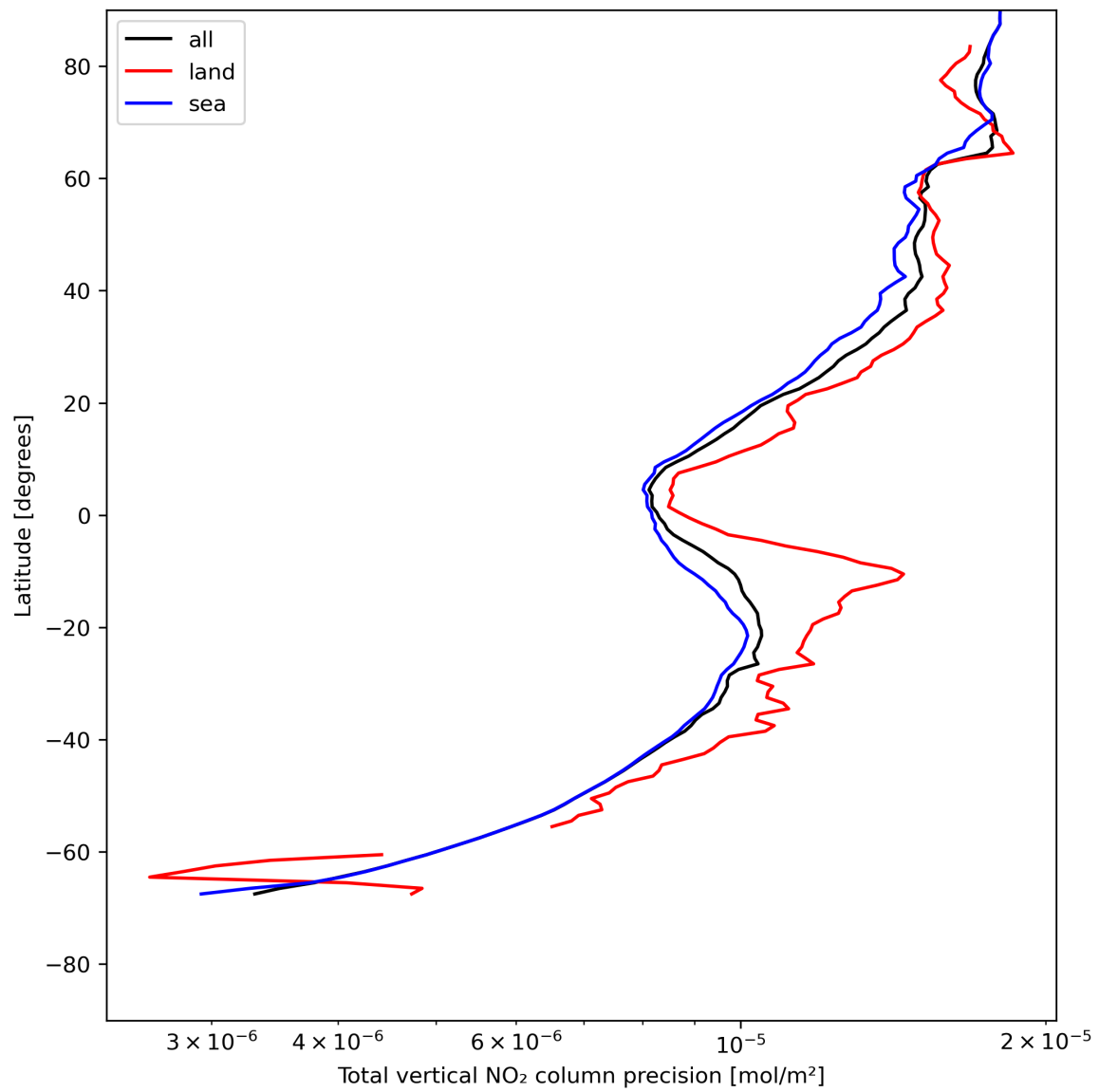
Figure 22: Zonal average of “Total vertical NO 2 column precision” for 2024-07-21 to 2024-07-22.
