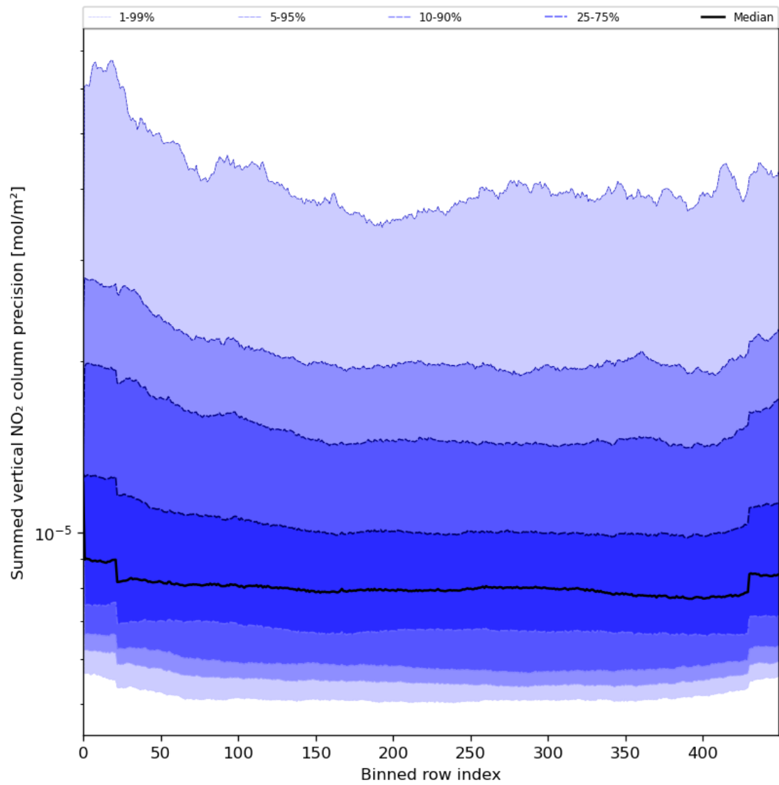
Figure 58: Along track statistics of “Summed vertical NO 2 column precision” for 2024-07-21 to 2024-07-22
