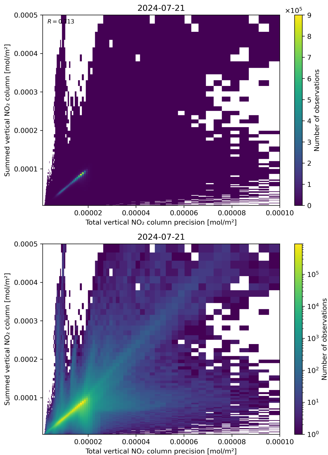
Figure 117: Scatter density plot of “Total vertical NO 2 column precision” against “Summed vertical NO 2 column” for 2024-07-21 to 2024-07-22.
