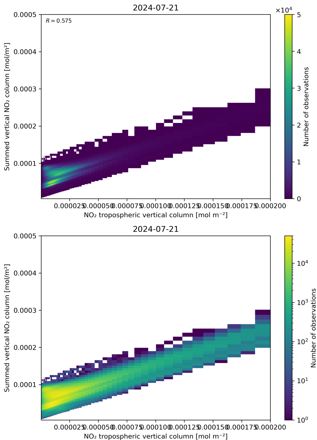
Figure 126: Scatter density plot of “NO 2 tropospheric vertical column” against “Summed vertical NO 2 column” for 2024-07-21 to 2024-07-22.
