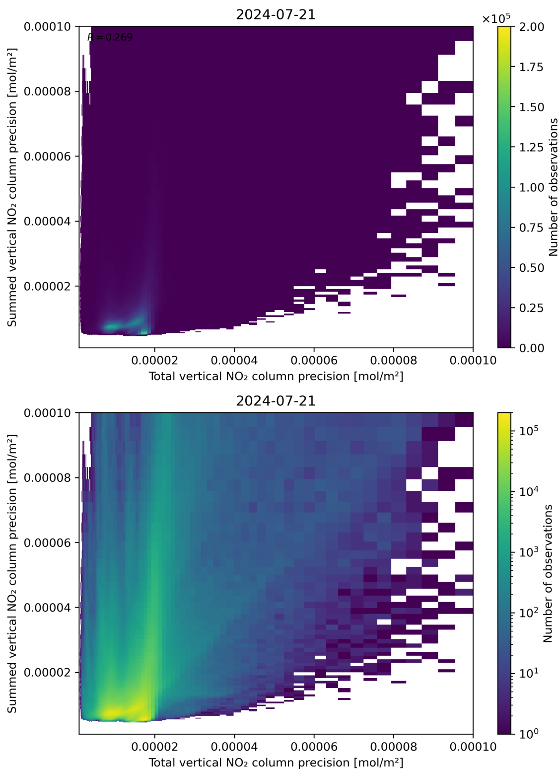
Figure 118: Scatter density plot of “Total vertical NO 2 column precision” against “Summed vertical NO 2 column precision” for 2024-07-21 to 2024-07-22.
