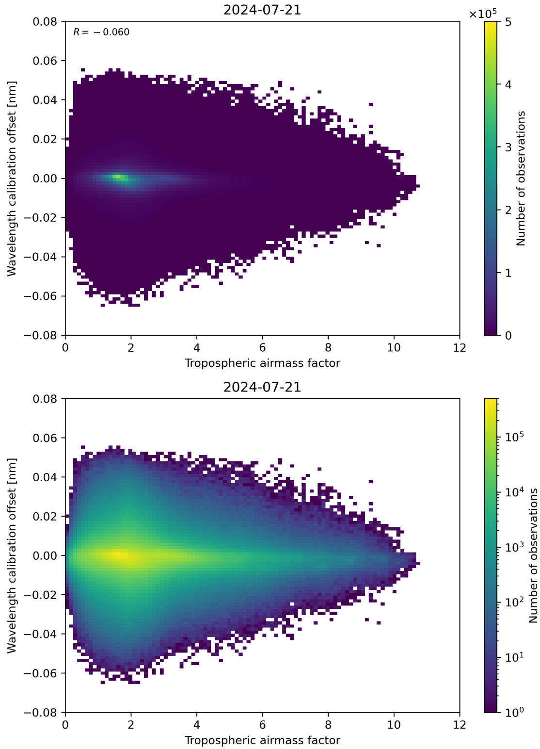
Figure 80: Scatter density plot of “Tropospheric air mass factor” against “Wavelength calibration offset” for 2024-07-21 to 2024-07-22.
