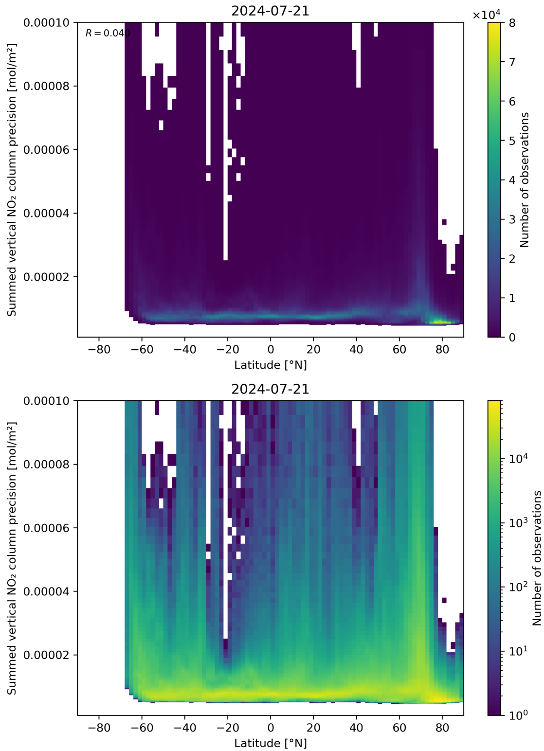
Figure 89: Scatter density plot of “Latitude” against “Summed vertical NO 2 column precision” for 2024-07-21 to 2024-07-22.
