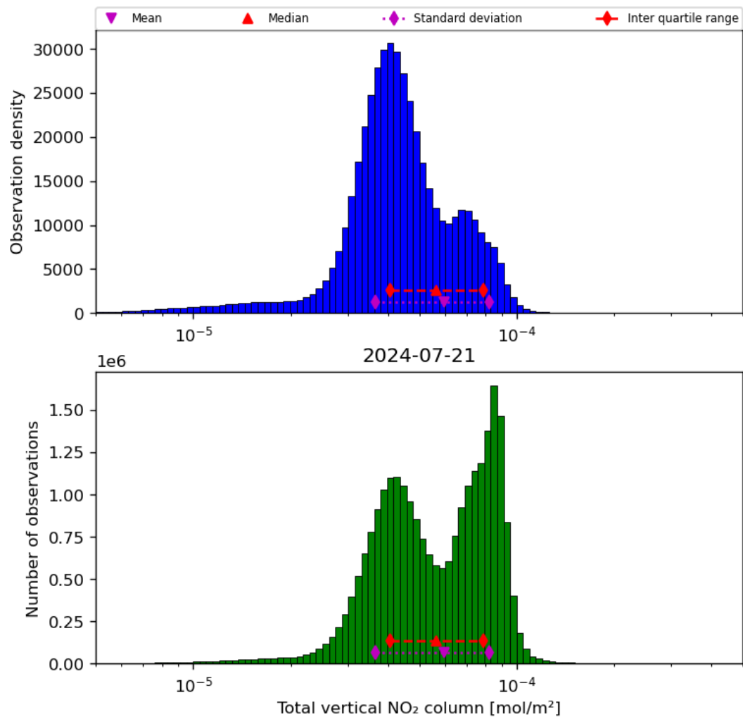
Figure 38: Histogram of “Total vertical NO 2 column” for 2024-07-21 to 2024-07-22
