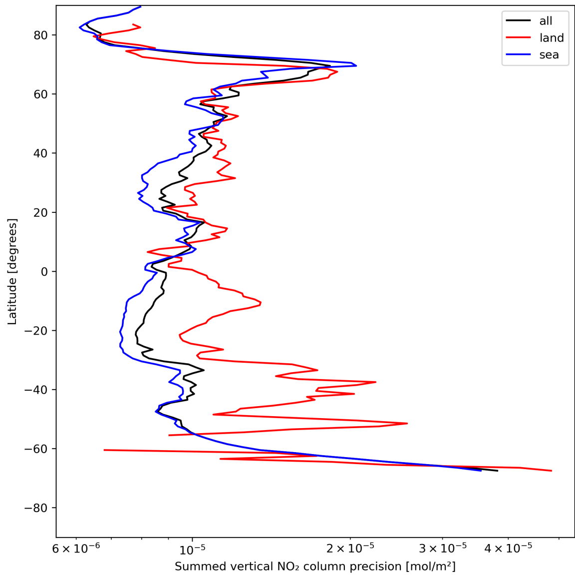
Figure 24: Zonal average of “Summed vertical NO 2 column precision” for 2024-07-21 to 2024-07-22.
