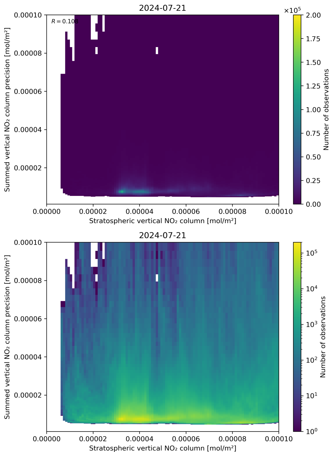
Figure 99: Scatter density plot of “Stratospheric vertical NO 2 column” against “Summed vertical NO 2 column precision” for 2024-07-21 to 2024-07-22.
