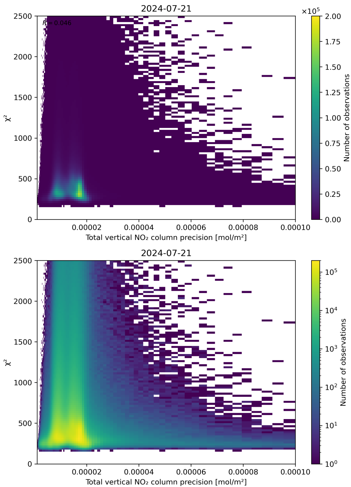
Figure 116: Scatter density plot of “Total vertical NO 2 column precision” against “ \chi^2 ” for 2024-07-21 to 2024-07-22.
