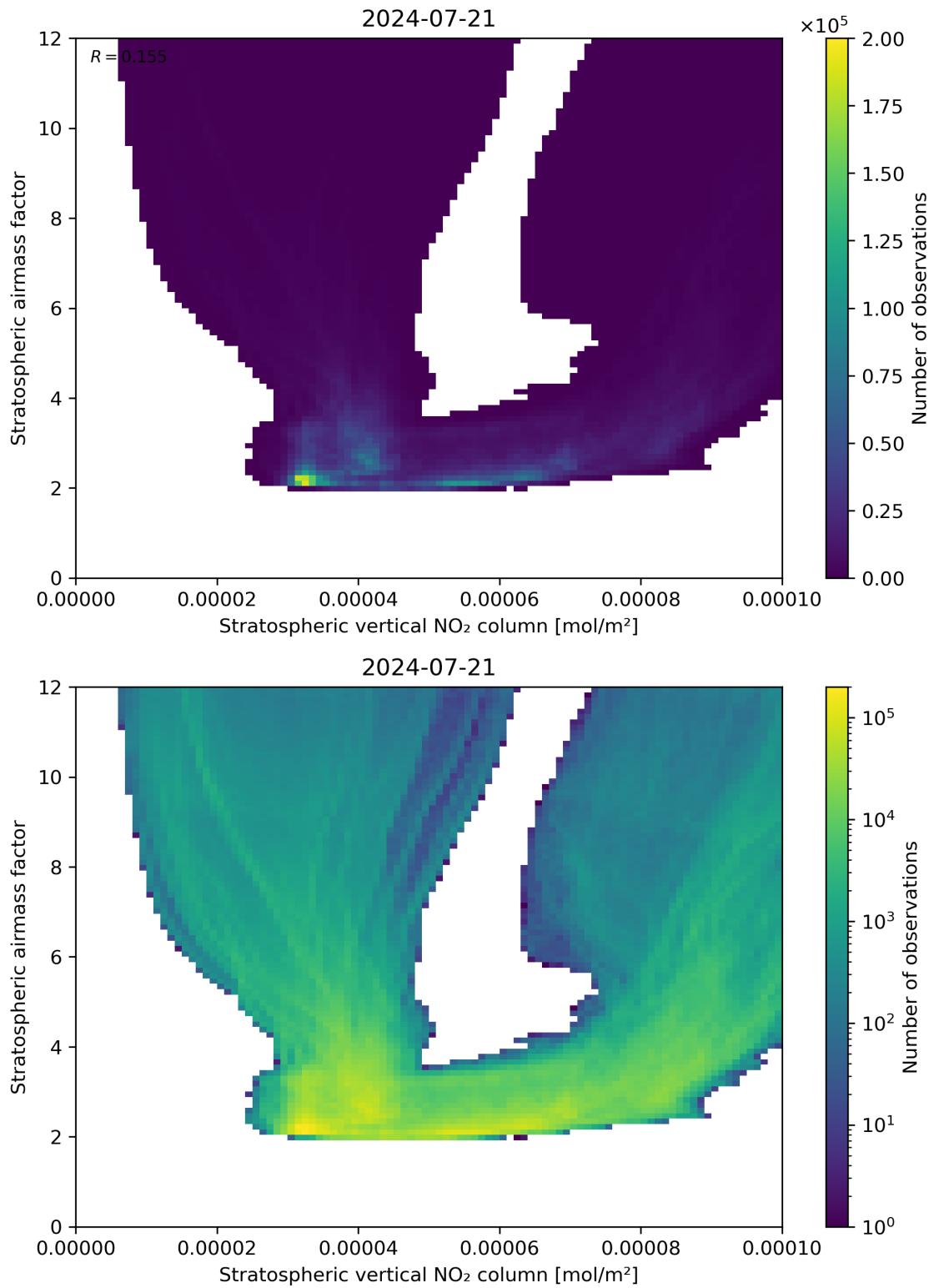
Figure 96: Scatter density plot of “Stratospheric vertical NO 2 column” against “Stratospheric airmass factor” for 2024-07-21 to 2024-07-22.
