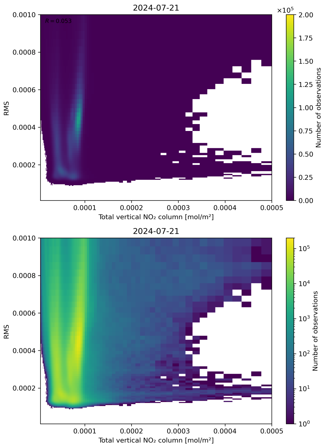
Figure 120: Scatter density plot of “Total vertical NO 2 column” against “RMS” for 2024-07-21 to 2024-07-22.
