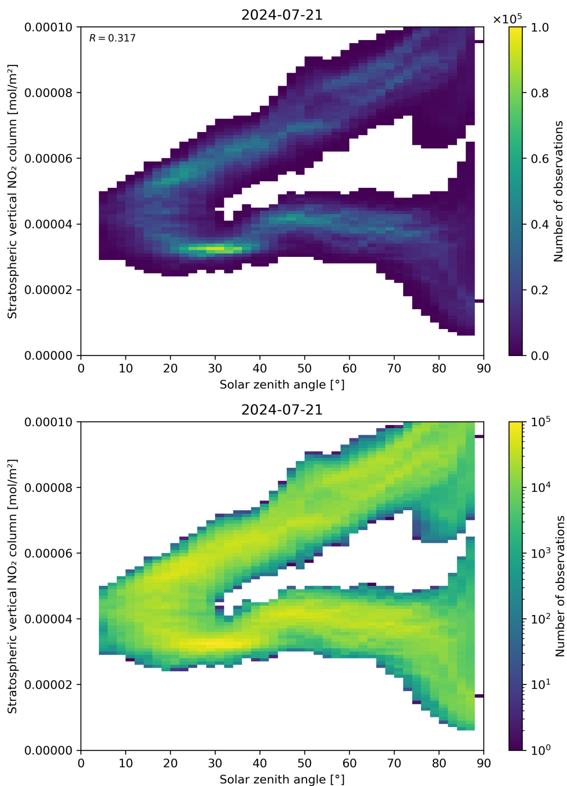
Figure 150: Scatter density plot of “Solar zenith angle” against “Stratospheric vertical NO 2 column” for 2024-07-21 to 2024-07-22.
