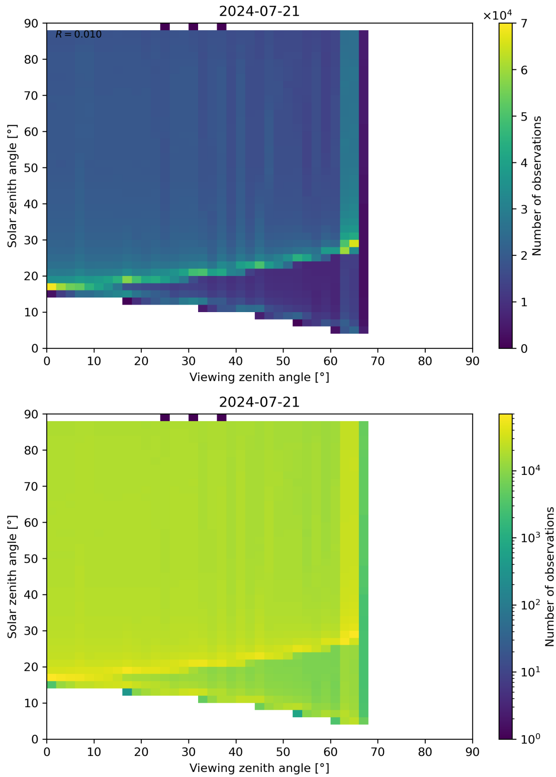
Figure 172: Scatter density plot of “Viewing zenith angle” against “Solar zenith angle” for 2024-07-21 to 2024-07-22.
