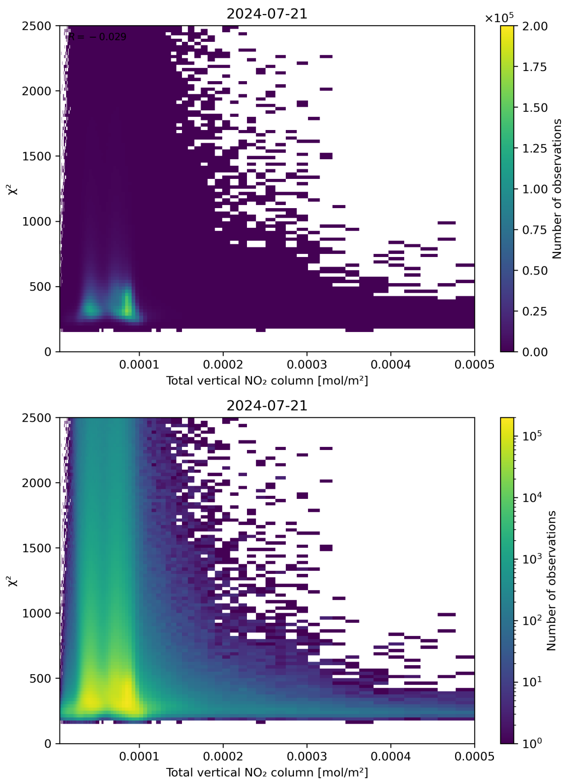
Figure 111: Scatter density plot of “Total vertical NO 2 column” against “ \chi^2 ” for 2024-07-21 to 2024-07-22.
