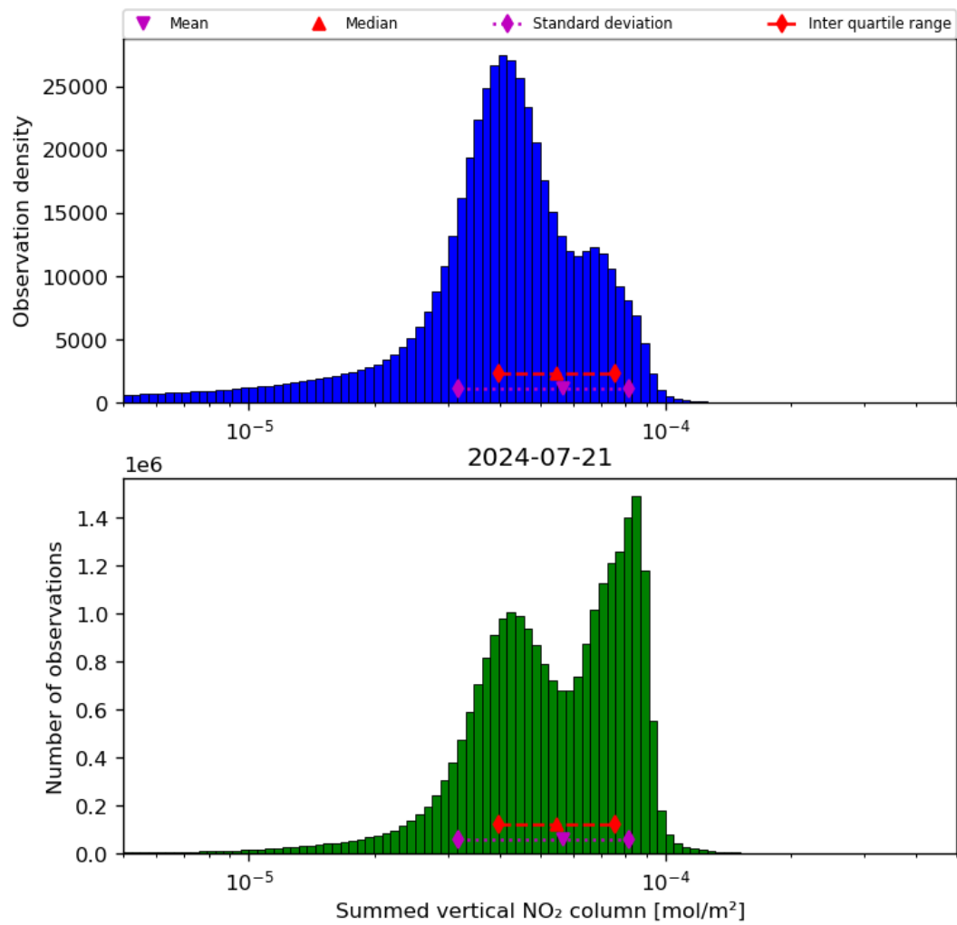
Figure 40: Histogram of “Summed vertical NO 2 column” for 2024-07-21 to 2024-07-22
