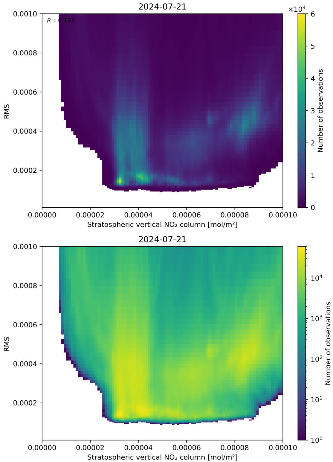
Figure 102: Scatter density plot of “Stratospheric vertical NO 2 column” against “RMS” for 2024-07-21 to 2024-07-22.
