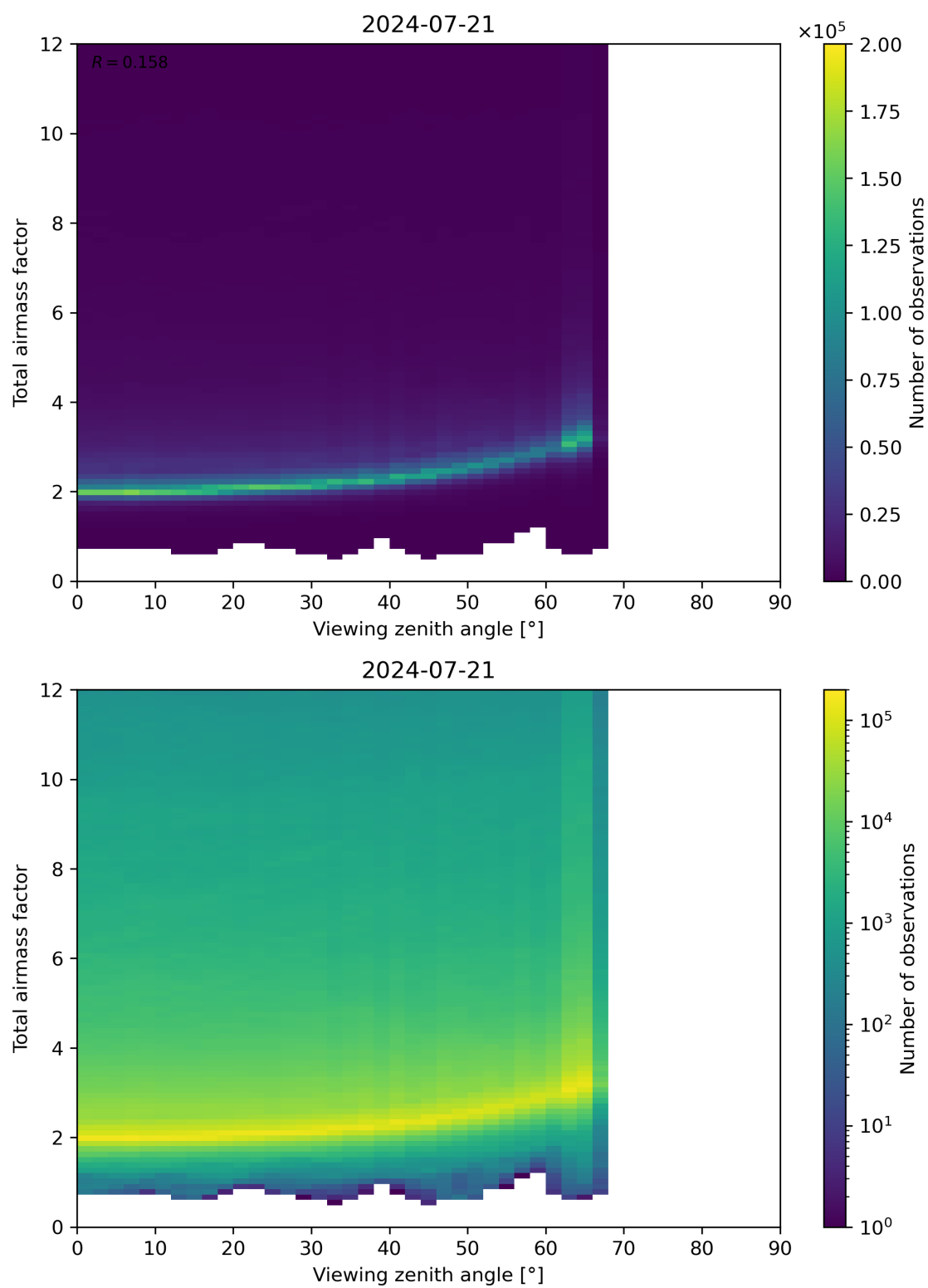
Figure 160: Scatter density plot of “Viewing zenith angle” against “Total airmass factor” for 2024-07-21 to 2024-07-22.
