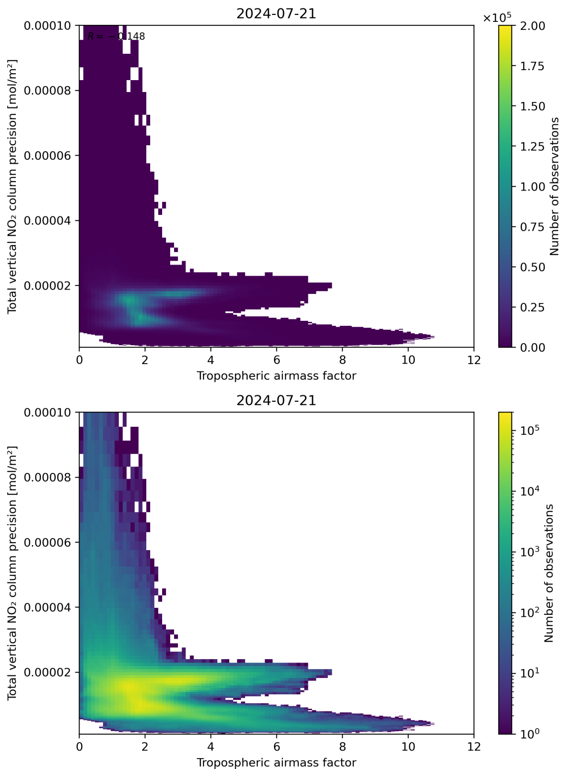
Figure 78: Scatter density plot of “Tropospheric air mass factor” against “Total vertical NO 2 column precision” for 2024-07-21 to 2024-07-22.
