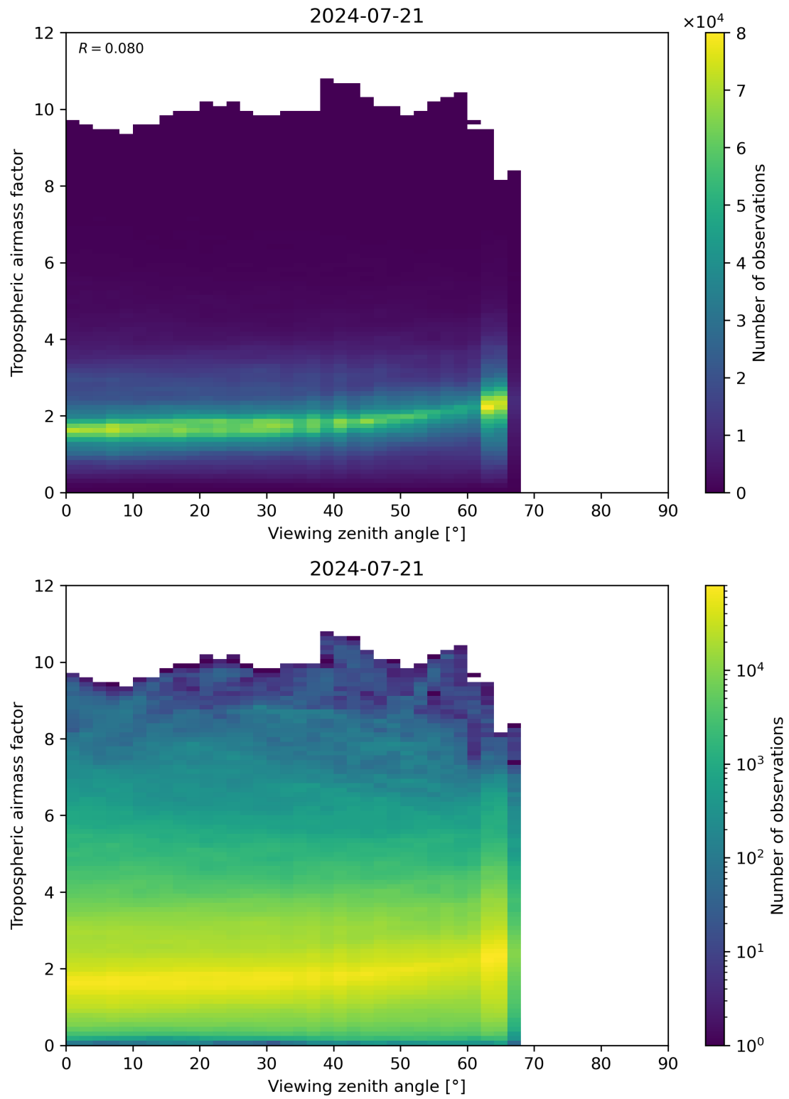
Figure 161: Scatter density plot of “Viewing zenith angle” against “Tropospheric airmass factor” for 2024-07-21 to 2024-07-22.
