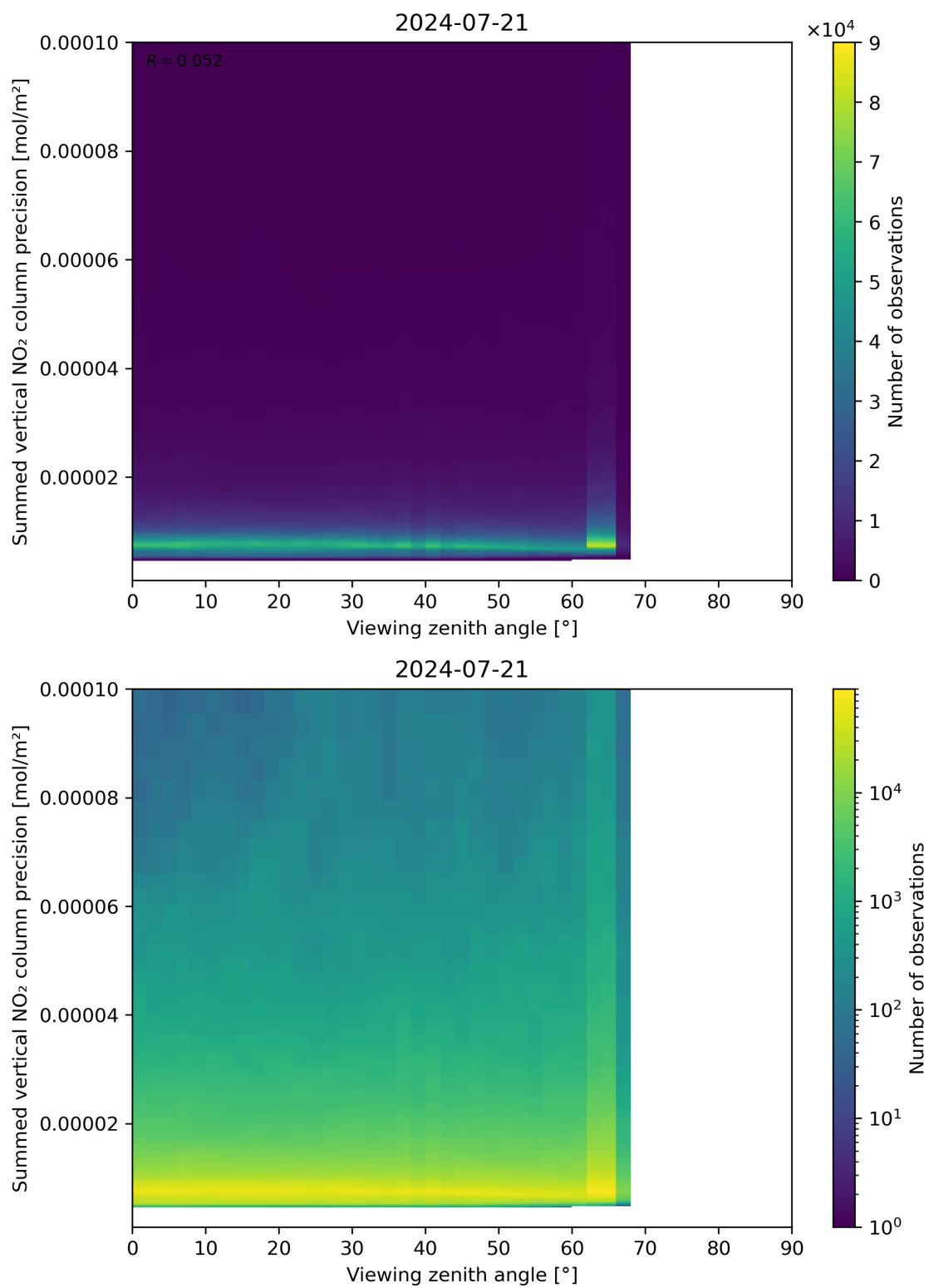
Figure 166: Scatter density plot of “Viewing zenith angle” against “Summed vertical NO 2 column precision” for 2024-07-21 to 2024-07-22.
