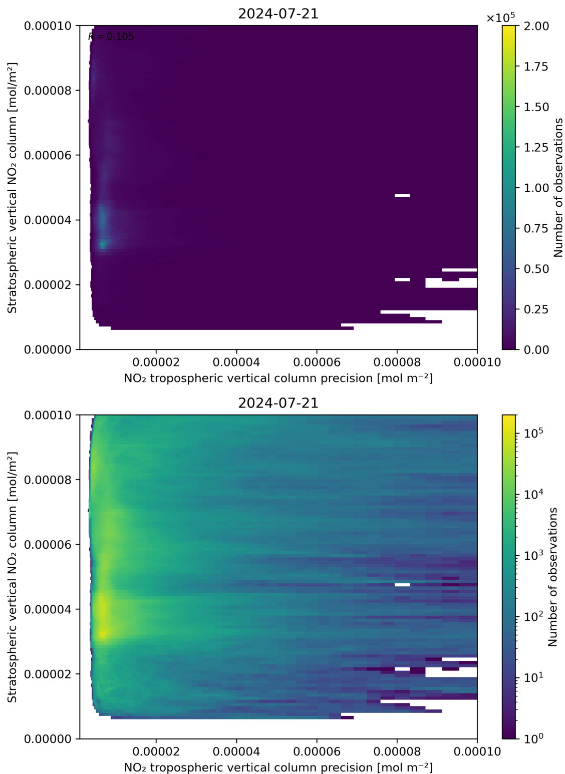
Figure 135: Scatter density plot of “NO 2 tropospheric vertical column precision” against “Stratospheric vertical NO 2 column” for 2024-07-21 to 2024-07-22.
