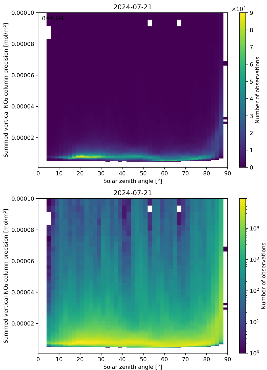
Figure 152: Scatter density plot of “Solar zenith angle” against “Summed vertical NO 2 column precision” for 2024-07-21 to 2024-07-22.
