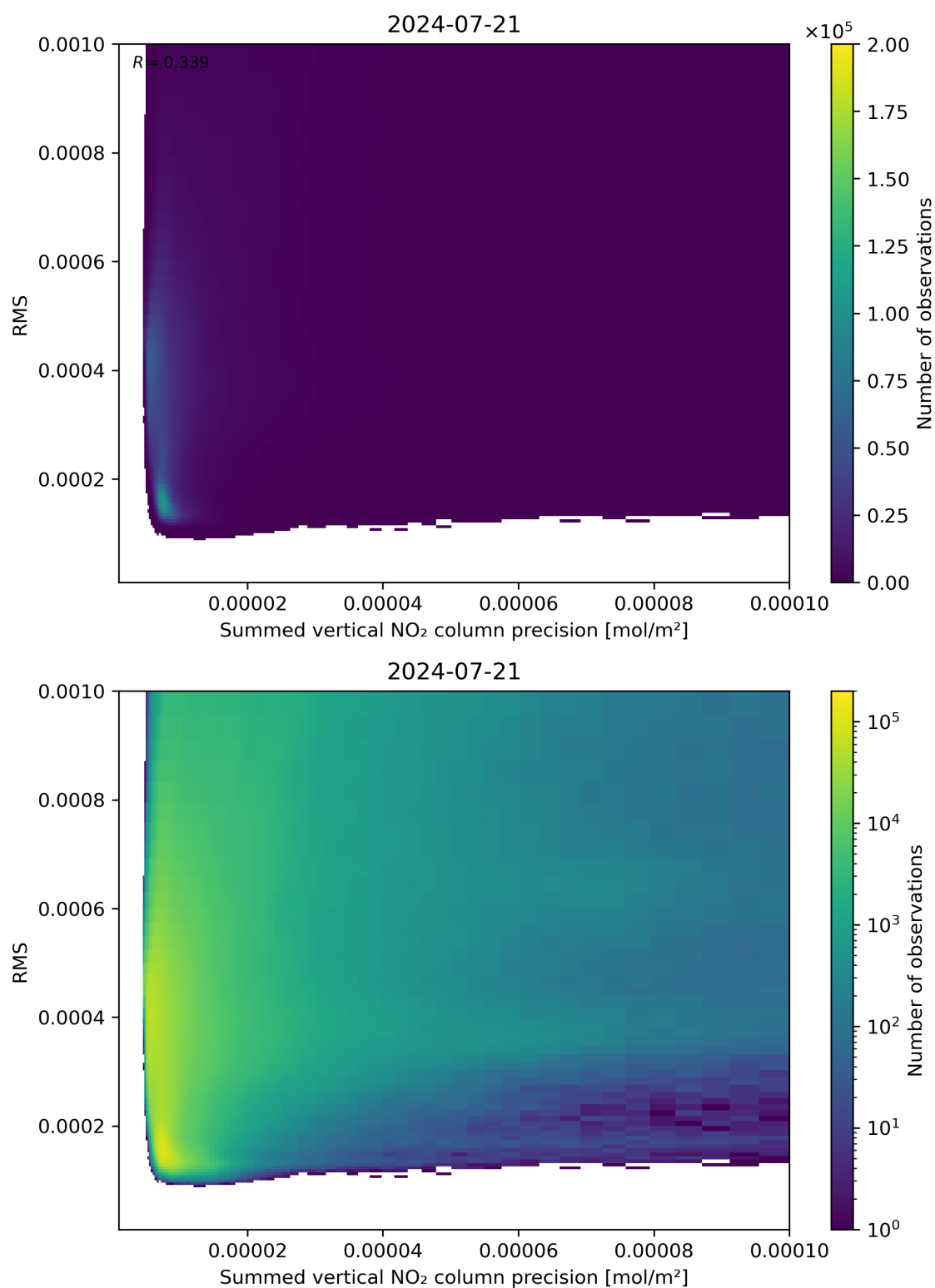
Figure 108: Scatter density plot of “Summed vertical NO 2 column precision” against “RMS” for 2024-07-21 to 2024-07-22.
