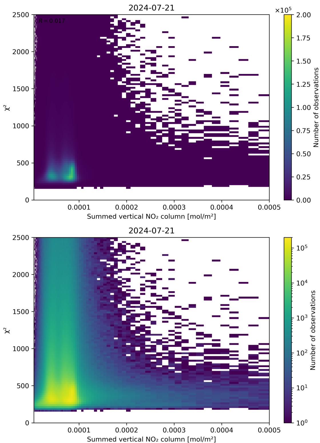
Figure 104: Scatter density plot of “Summed vertical NO 2 column” against “ \chi^2 ” for 2024-07-21 to 2024-07-22.
