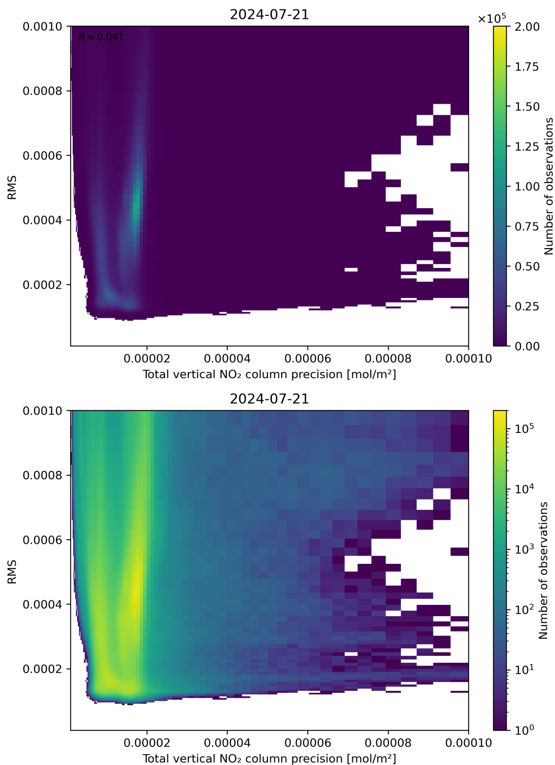
Figure 119: Scatter density plot of “Total vertical NO 2 column precision” against “RMS” for 2024-07-21 to 2024-07-22.
