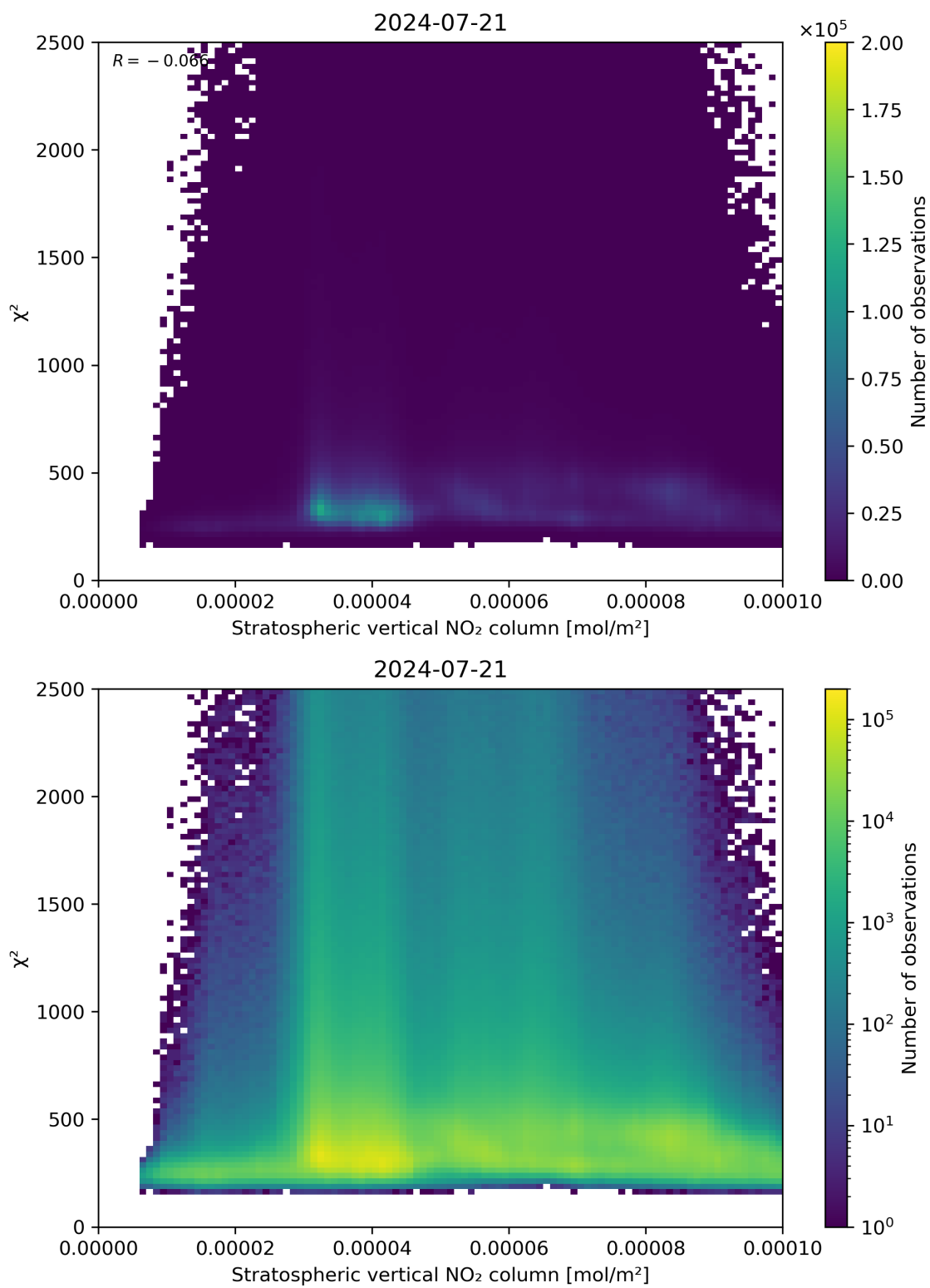
Figure 97: Scatter density plot of “Stratospheric vertical NO 2 column” against “ \chi^2 ” for 2024-07-21 to 2024-07-22.
