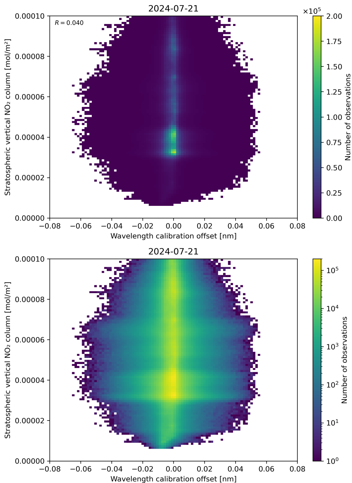
Figure 176: Scatter density plot of “Wavelength calibration offset” against “Stratospheric vertical NO 2 column” for 2024-07-21 to 2024-07-22.
