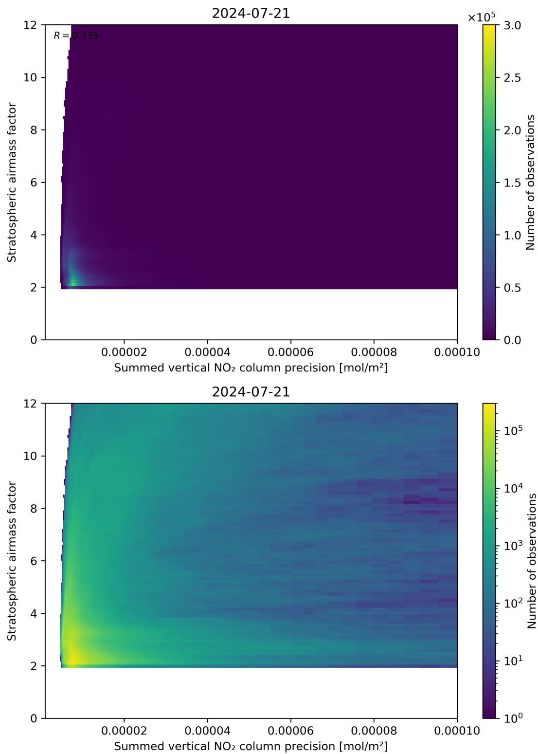
Figure 106: Scatter density plot of “Summed vertical NO 2 column precision” against “Stratospheric airmass factor” for 2024-07-21 to 2024-07-22.
