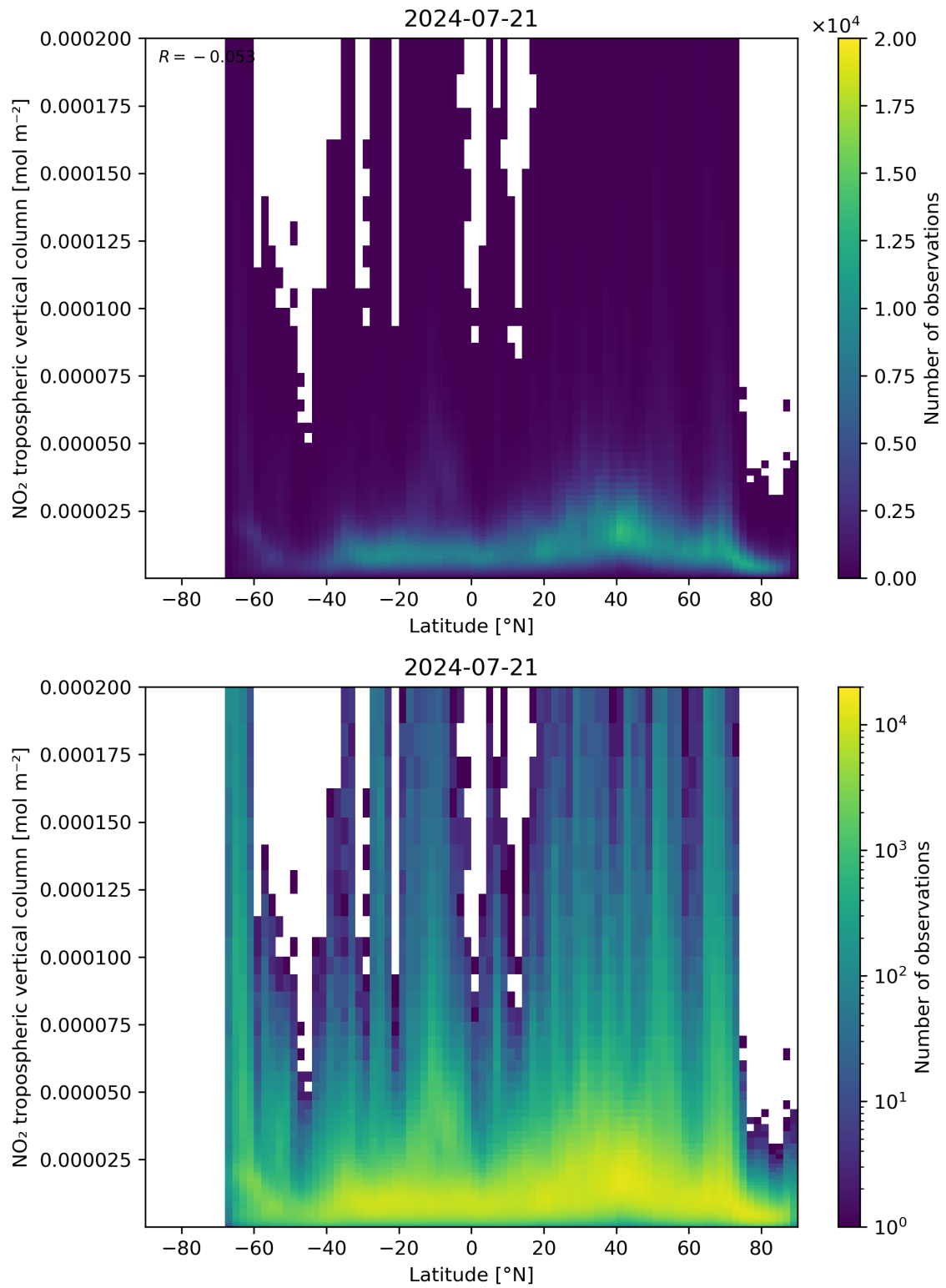
Figure 92: Scatter density plot of “Latitude” against “NO 2 tropospheric vertical column” for 2024-07-21 to 2024-07-22.
