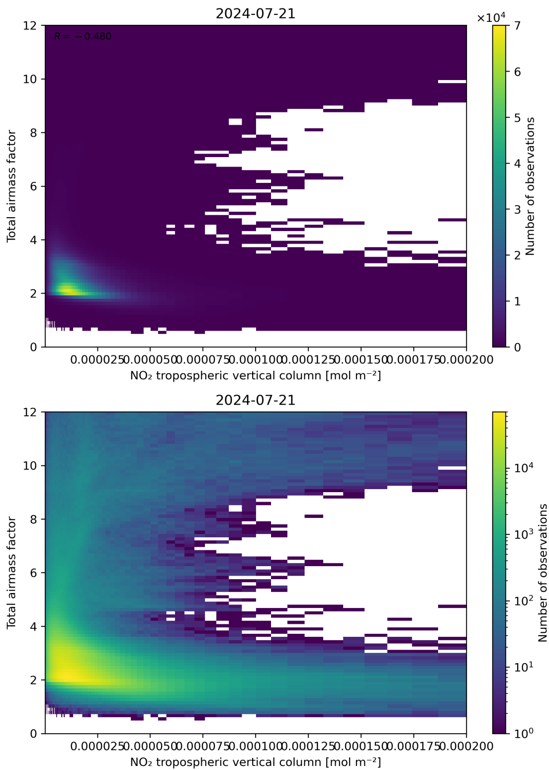
Figure 122: Scatter density plot of “NO 2 tropospheric vertical column” against “Total air mass factor” for 2024-07-21 to 2024-07-22.
