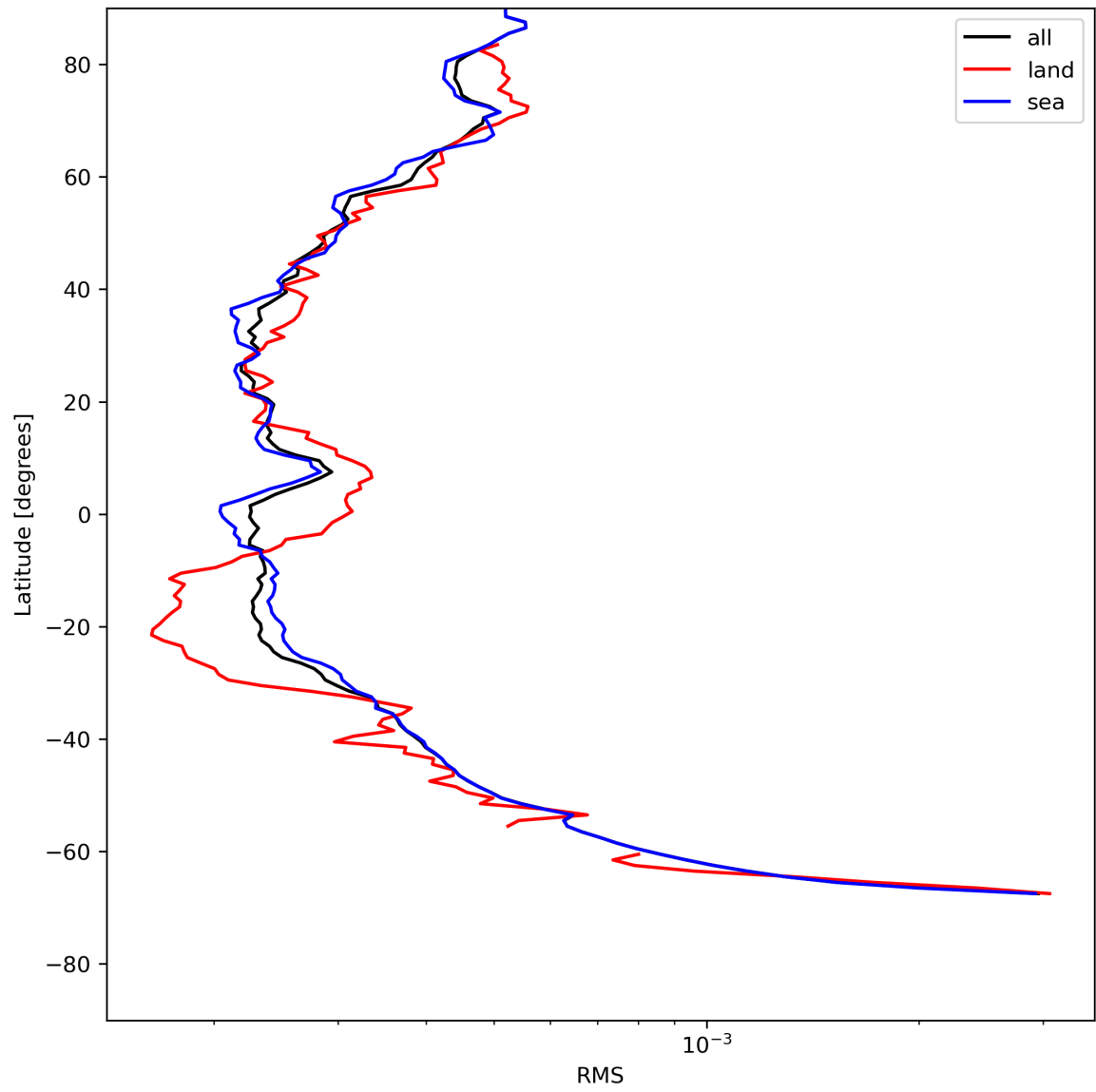
Figure 26: Zonal average of “RMS” for 2024-07-21 to 2024-07-22.
