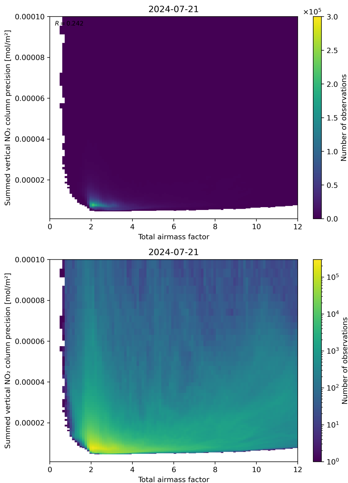
Figure 66: Scatter density plot of “Total airmass factor” against “Summed vertical NO 2 column precision” for 2024-07-21 to 2024-07-22.
