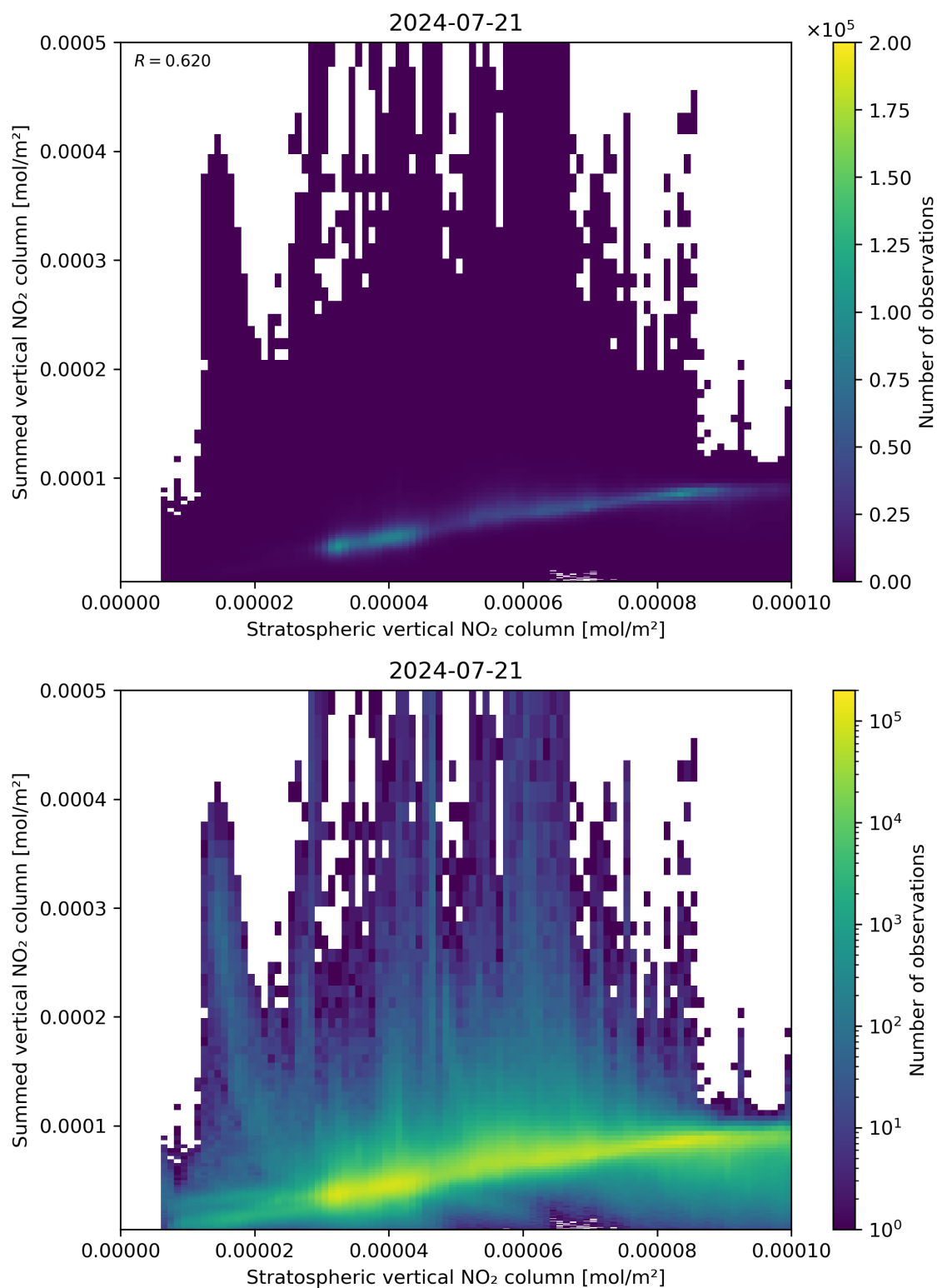
Figure 98: Scatter density plot of “Stratospheric vertical NO 2 column” against “Summed vertical NO 2 column” for 2024-07-21 to 2024-07-22.
