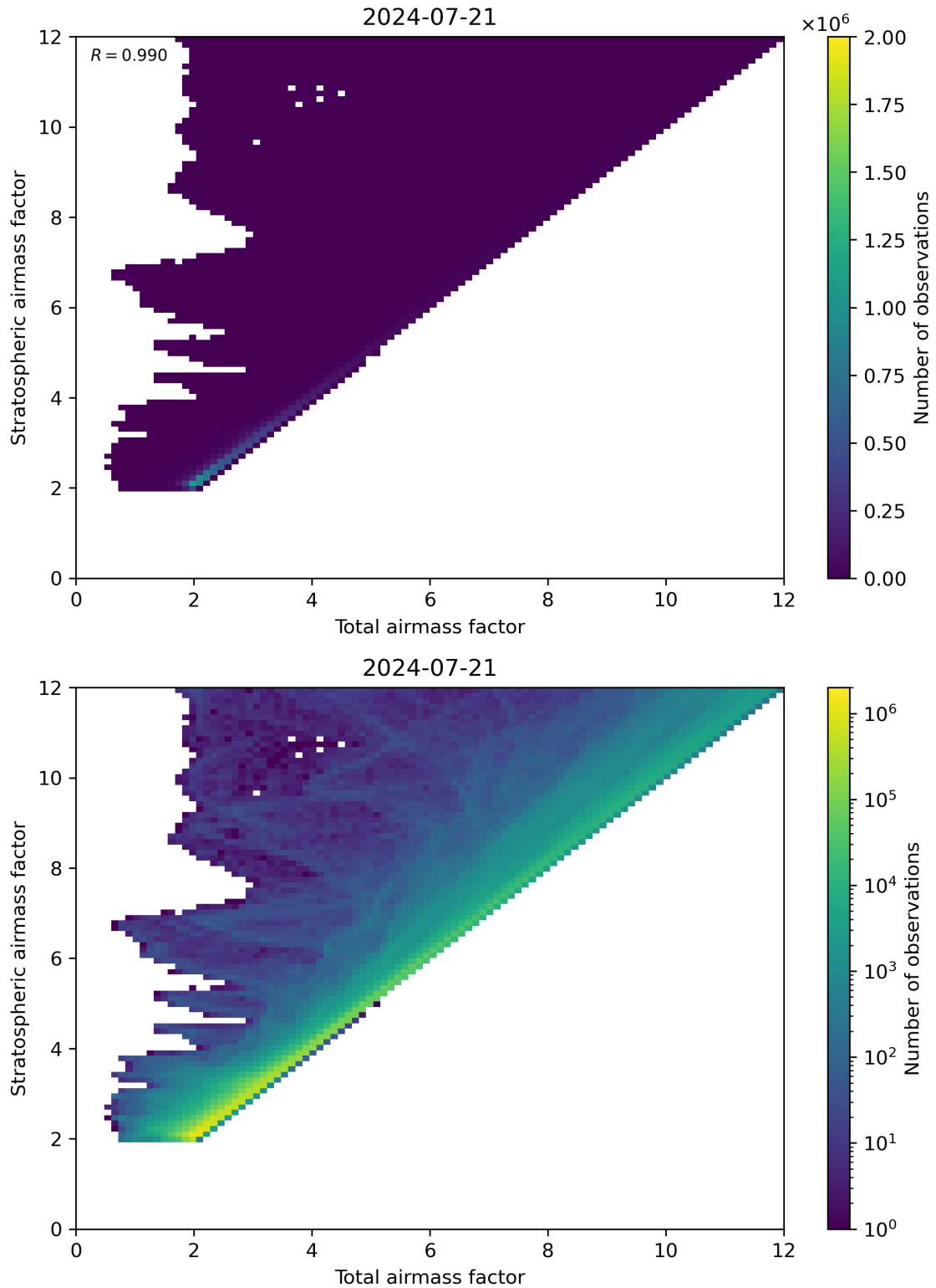
Figure 62: Scatter density plot of “Total airmass factor” against “Stratospheric airmass factor” for 2024-07-21 to 2024-07-22.
