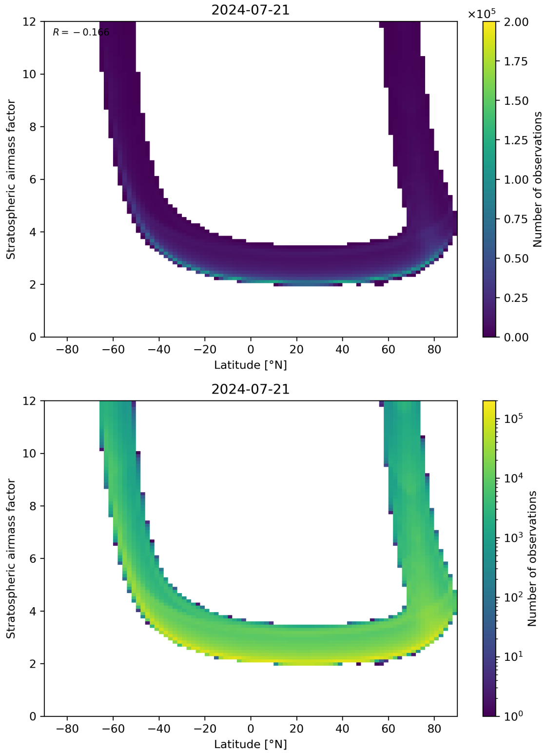
Figure 83: Scatter density plot of “Latitude” against “Stratospheric air mass factor” for 2024-07-21 to 2024-07-22.
