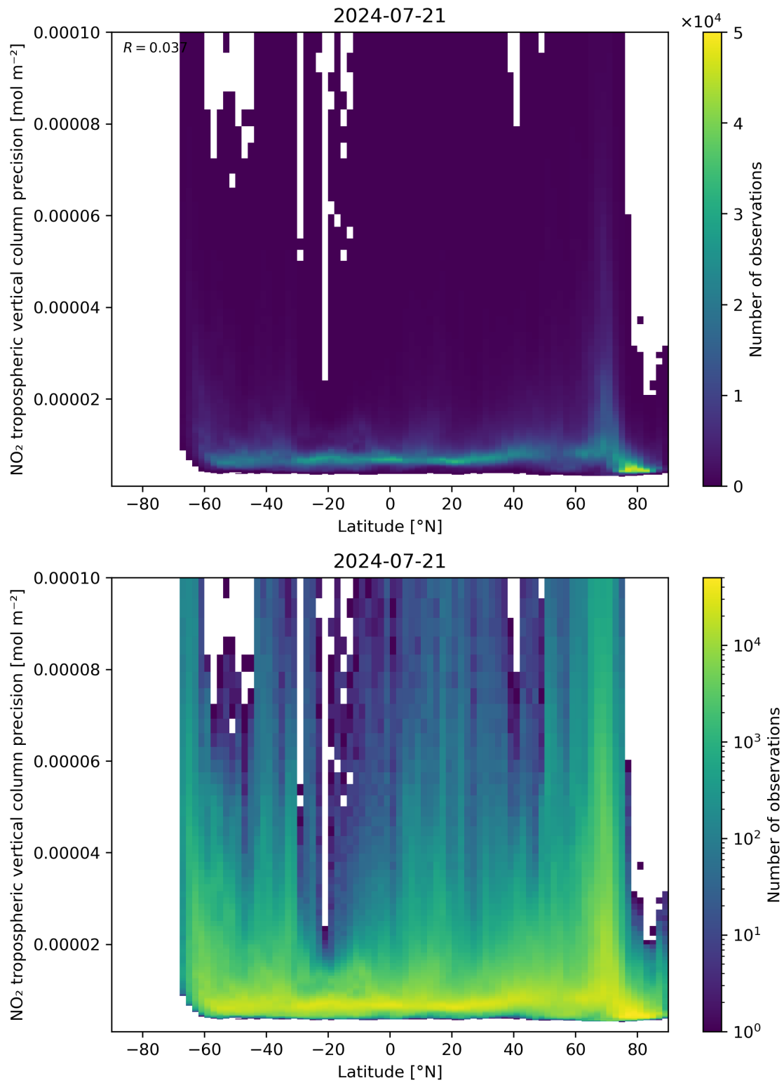
Figure 93: Scatter density plot of “Latitude” against “NO 2 tropospheric vertical column precision” for 2024-07-21 to 2024-07-22.
