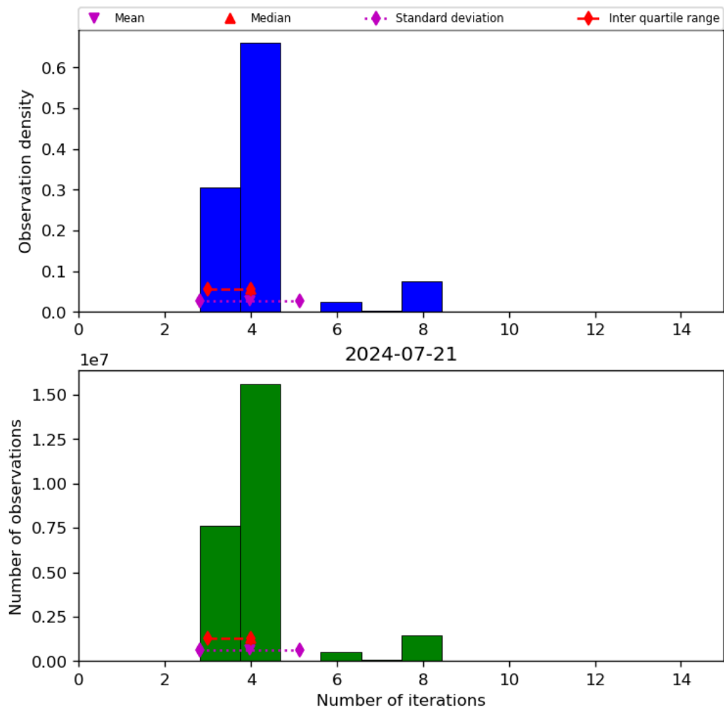
Figure 34: Histogram of “Number of iterations” for 2024-07-21 to 2024-07-22
