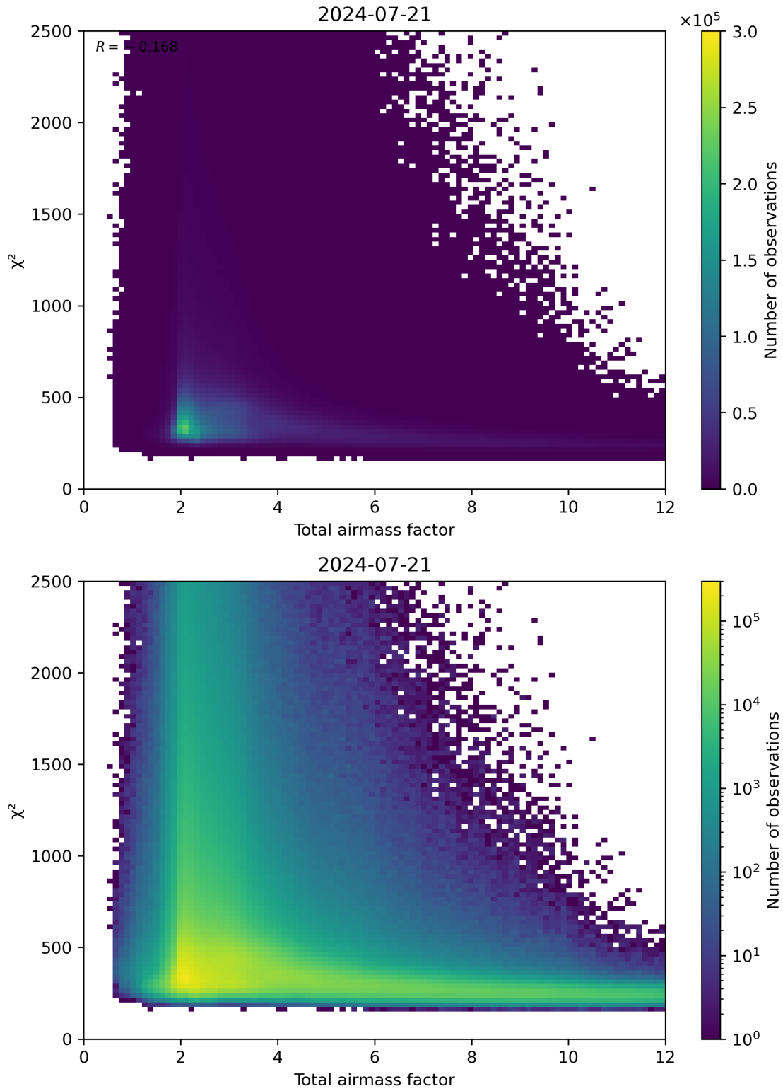
Figure 63: Scatter density plot of “Total airmass factor” against “ \chi^2 ” for 2024-07-21 to 2024-07-22.
