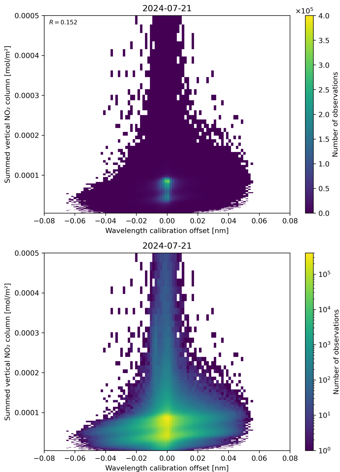
Figure 177: Scatter density plot of “Wavelength calibration offset” against “Summed vertical NO 2 column” for 2024-07-21 to 2024-07-22.
