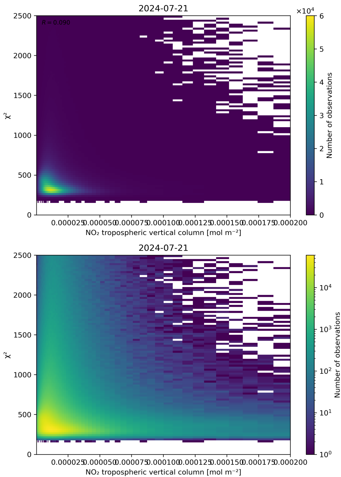
Figure 124: Scatter density plot of “NO 2 tropospheric vertical column” against “ \chi^2 ” for 2024-07-21 to 2024-07-22.
