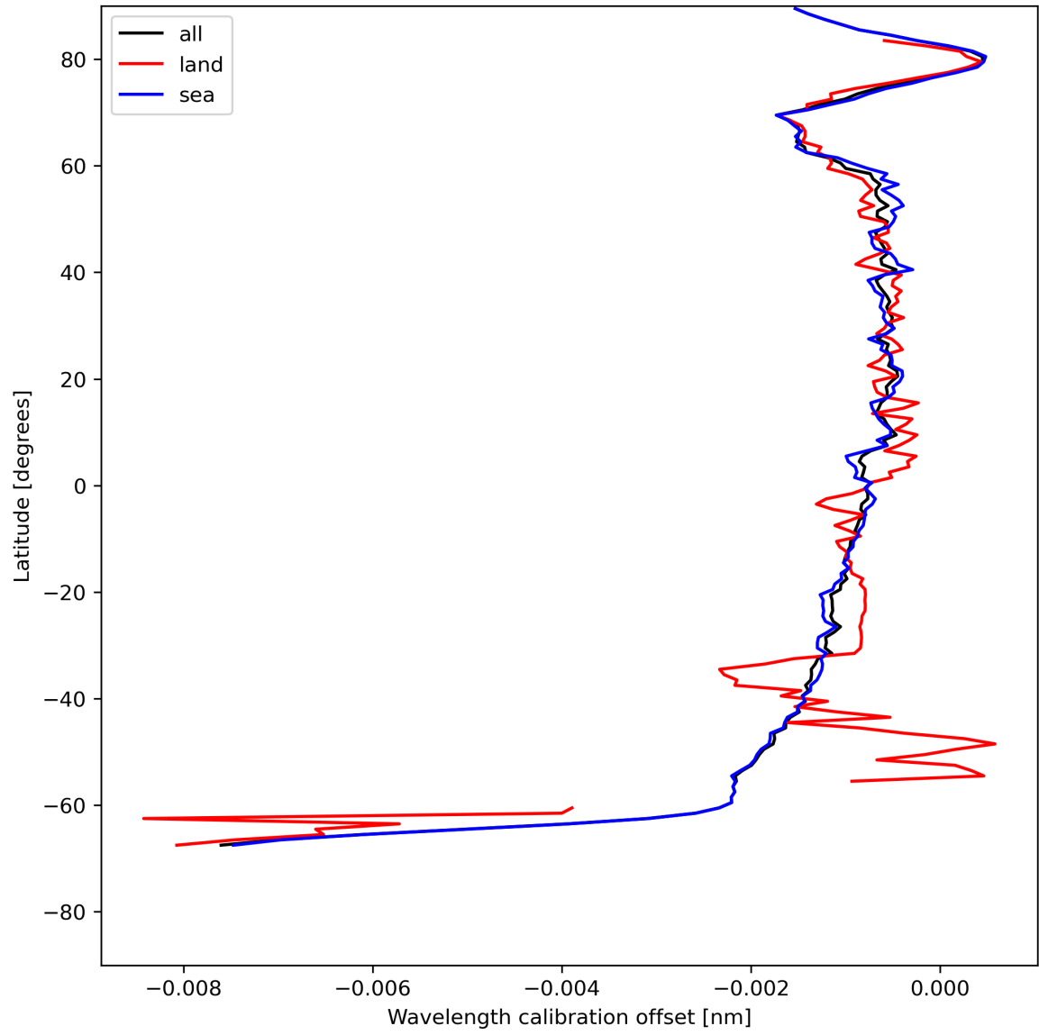
Figure 18: Zonal average of “Wavelength calibration offset” for 2024-07-21 to 2024-07-22.
