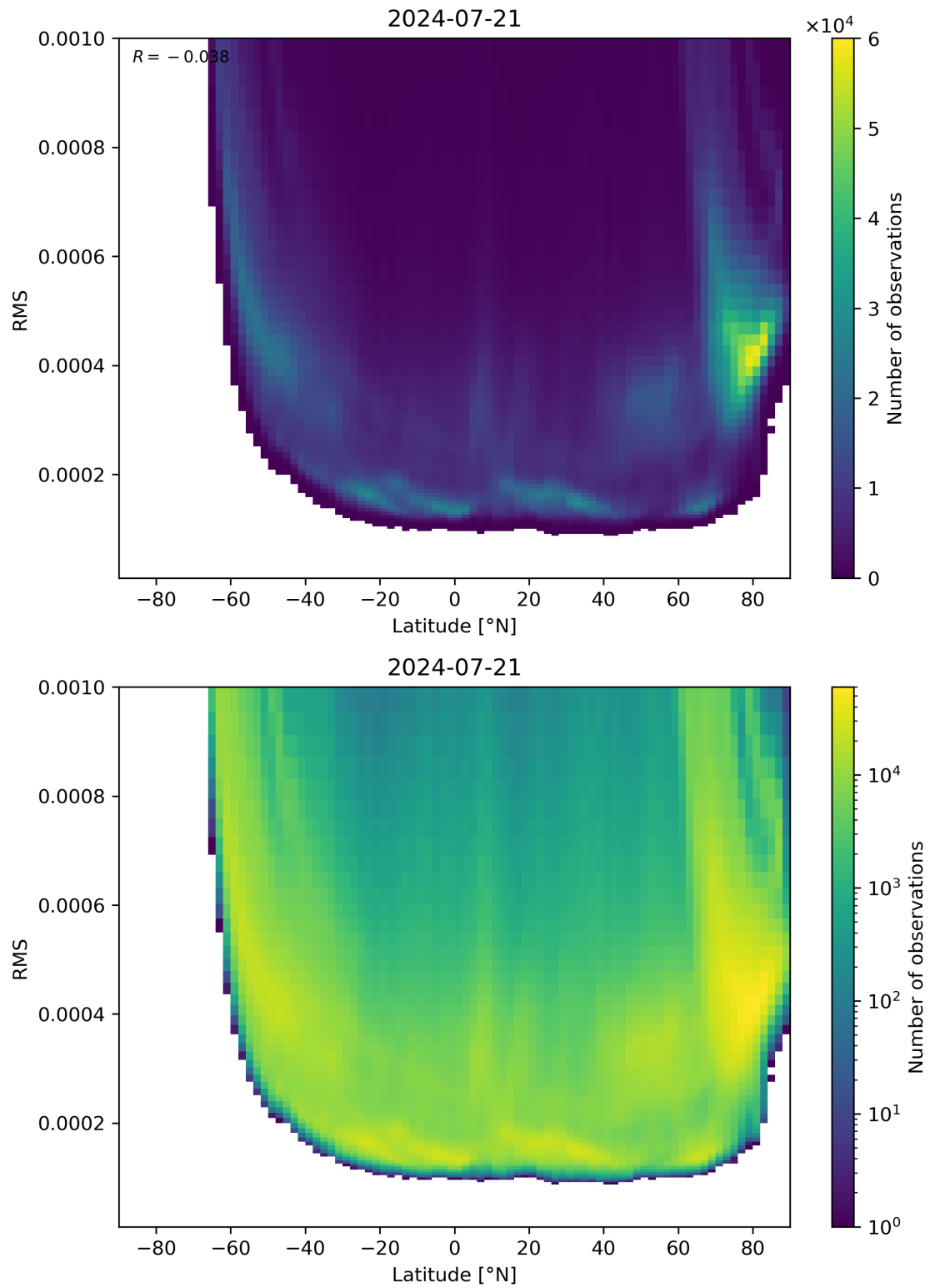
Figure 94: Scatter density plot of “Latitude” against “RMS” for 2024-07-21 to 2024-07-22.
