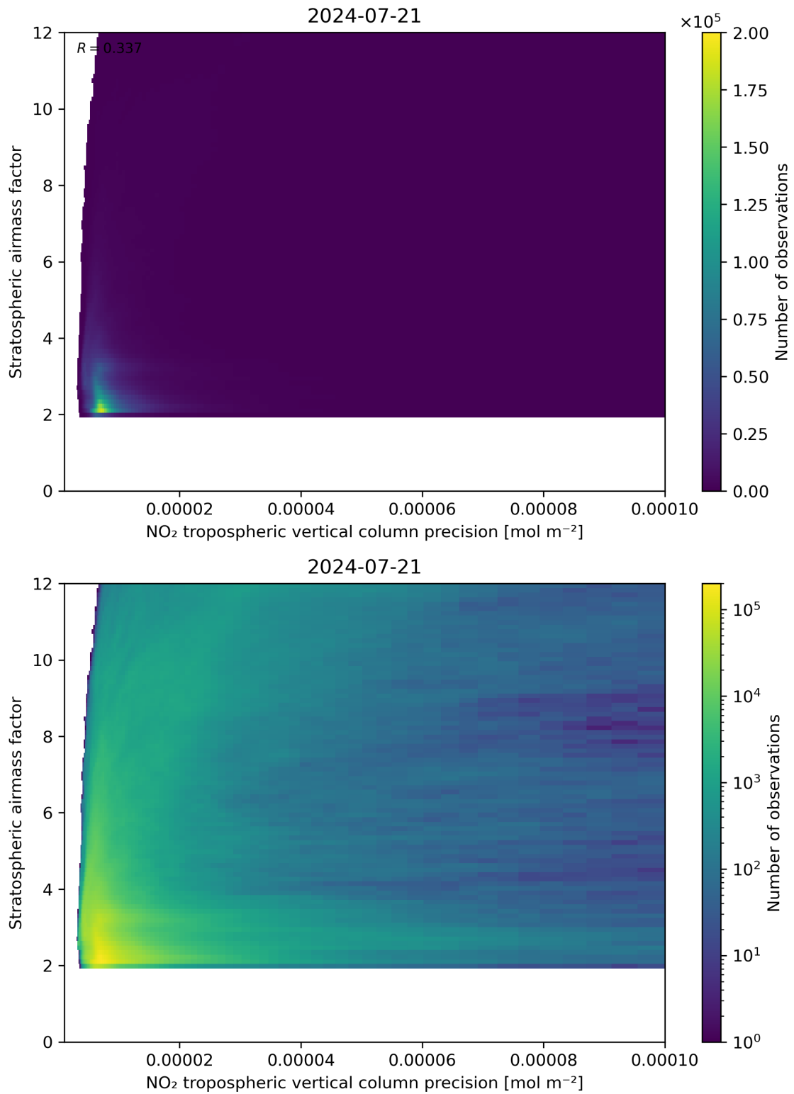
Figure 131: Scatter density plot of “NO 2 tropospheric vertical column precision” against “Stratospheric airmass factor” for 2024-07-21 to 2024-07-22.
