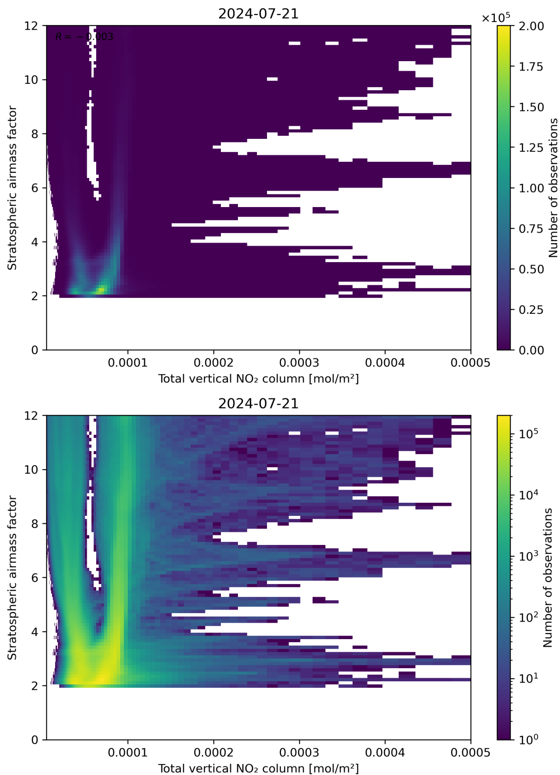
Figure 110: Scatter density plot of “Total vertical NO 2 column” against “Stratospheric airmass factor” for 2024-07-21 to 2024-07-22.
