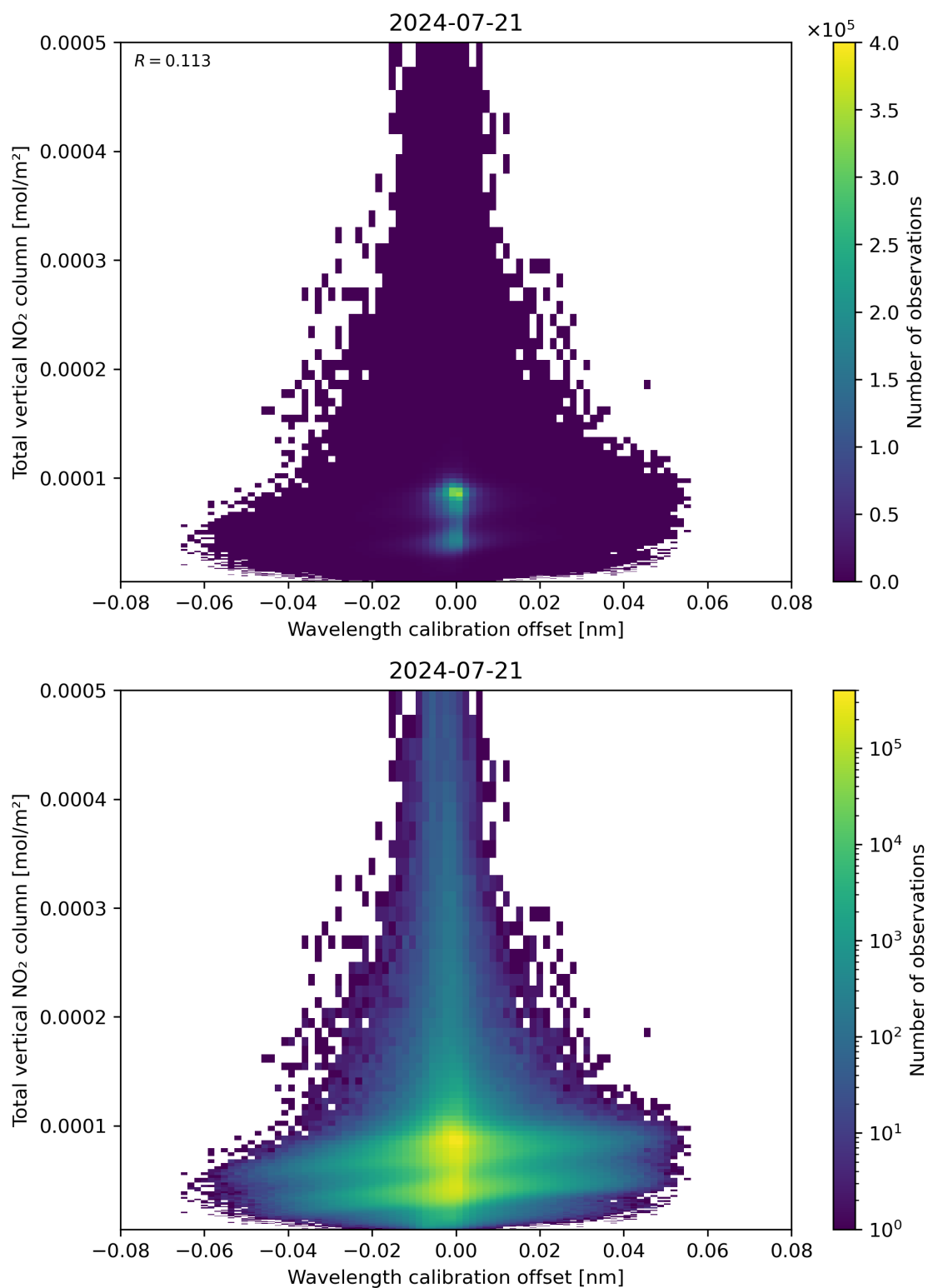
Figure 179: Scatter density plot of “Wavelength calibration offset” against “Total vertical NO 2 column” for 2024-07-21 to 2024-07-22.
