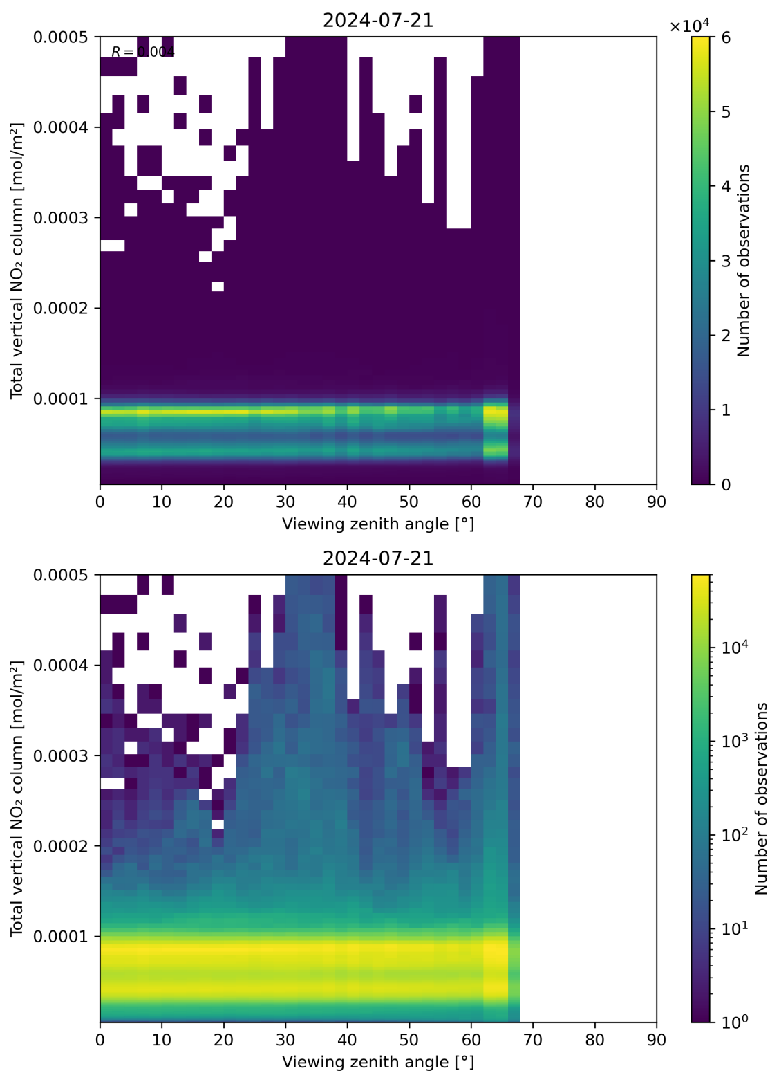
Figure 167: Scatter density plot of “Viewing zenith angle” against “Total vertical NO 2 column” for 2024-07-21 to 2024-07-22.
