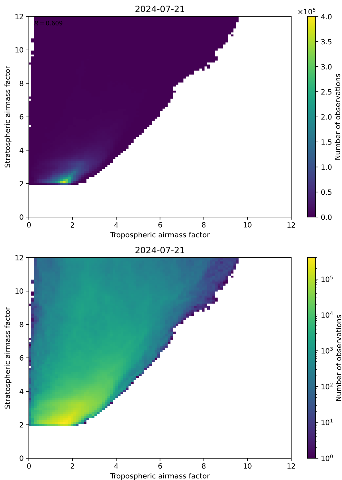
Figure 71: Scatter density plot of “Tropospheric airmass factor” against “Stratospheric airmass factor” for 2024-07-21 to 2024-07-22.
