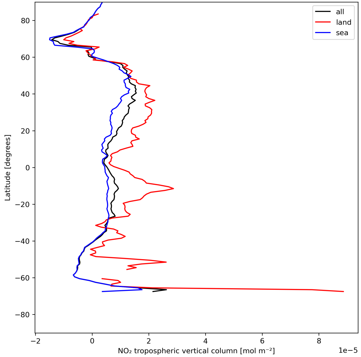
Figure 12: Zonal average of “NO 2 tropospheric vertical column” for 2024-07-21 to 2024-07-22.
