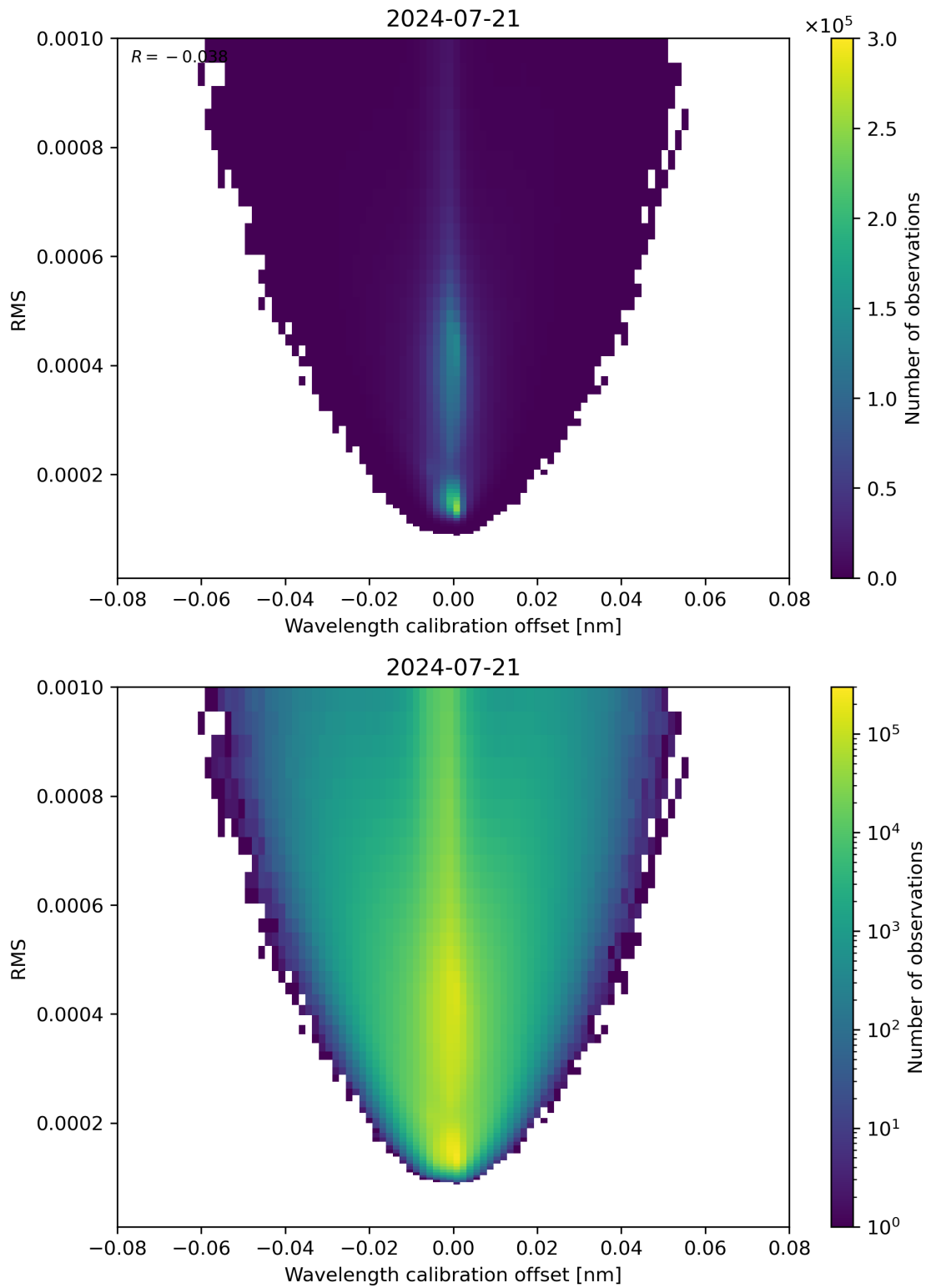
Figure 181: Scatter density plot of “Wavelength calibration offset” against “RMS” for 2024-07-21 to 2024-07-22.
