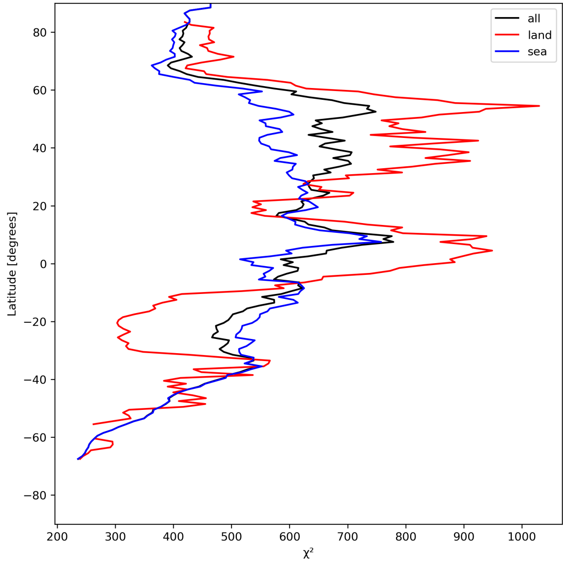
Figure 25: Zonal average of “ \chi^2 ” for 2024-07-21 to 2024-07-22.
