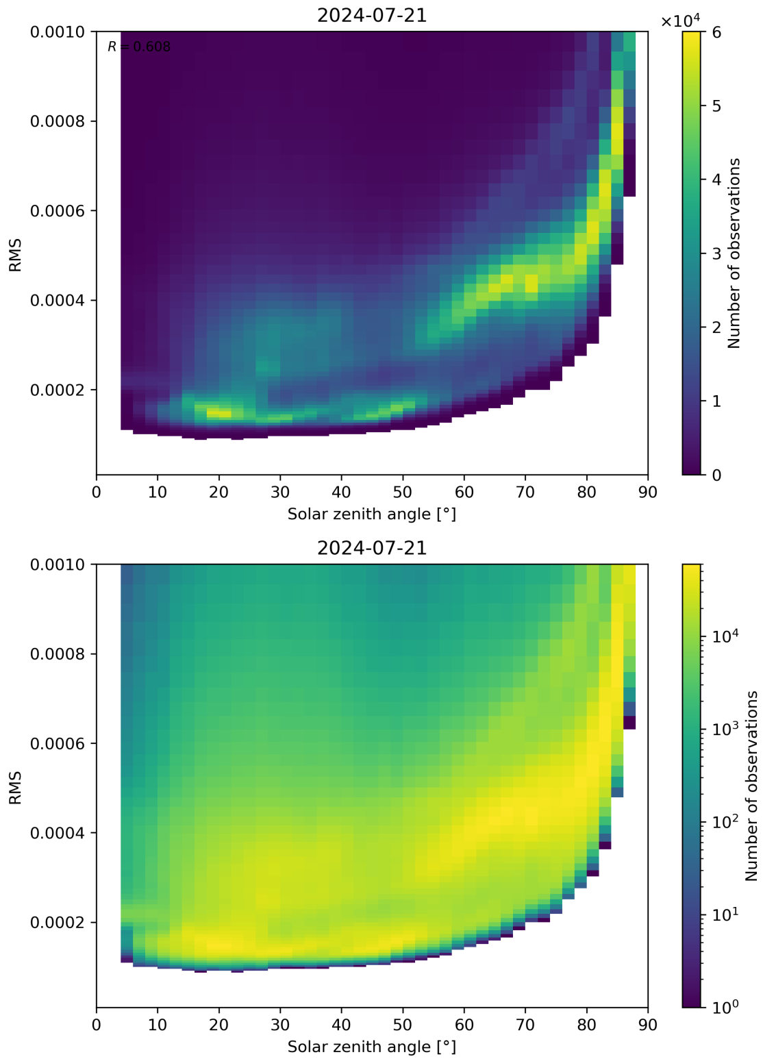
Figure 157: Scatter density plot of “Solar zenith angle” against “RMS” for 2024-07-21 to 2024-07-22.
