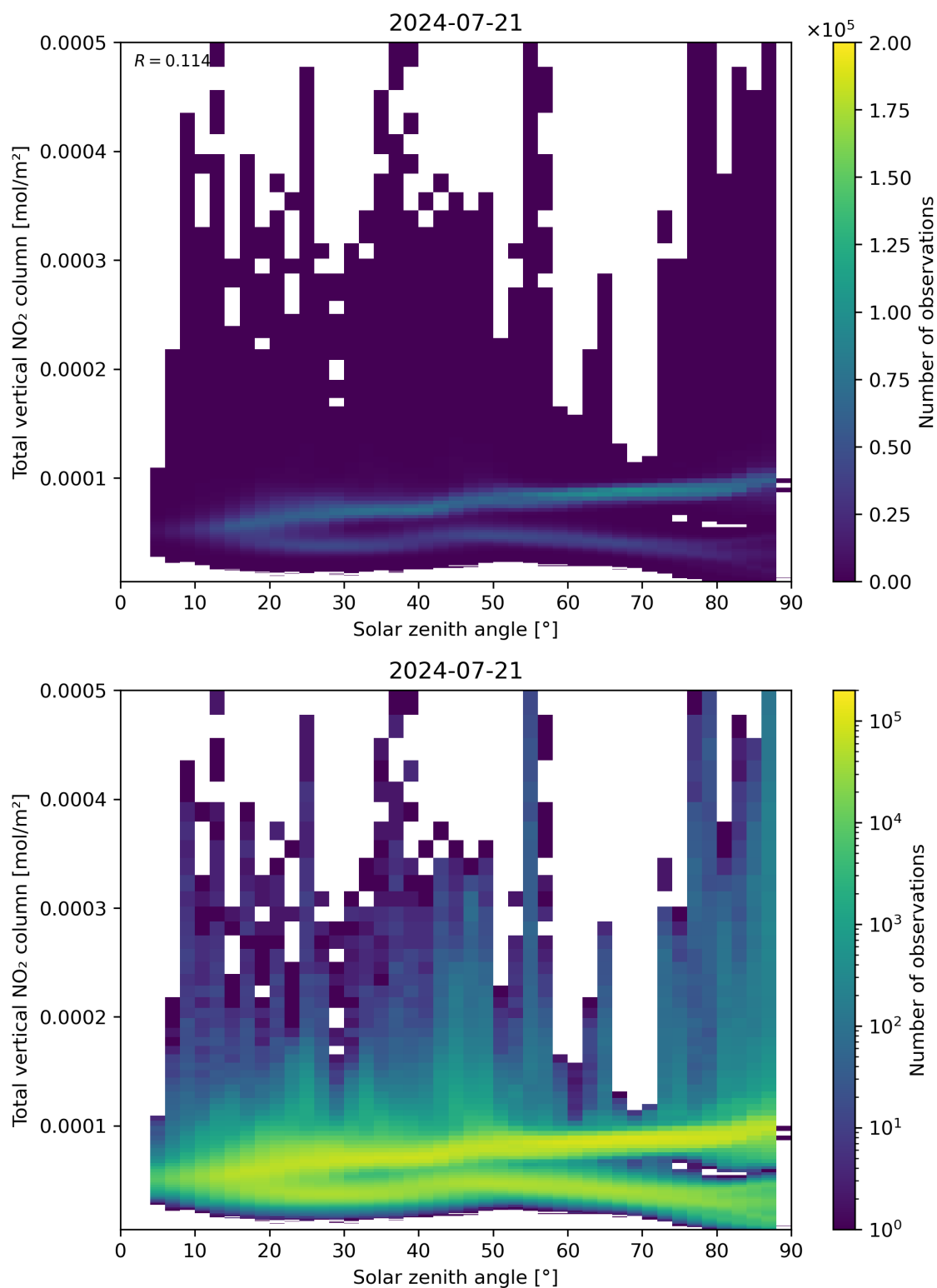
Figure 153: Scatter density plot of “Solar zenith angle” against “Total vertical NO 2 column” for 2024-07-21 to 2024-07-22.
