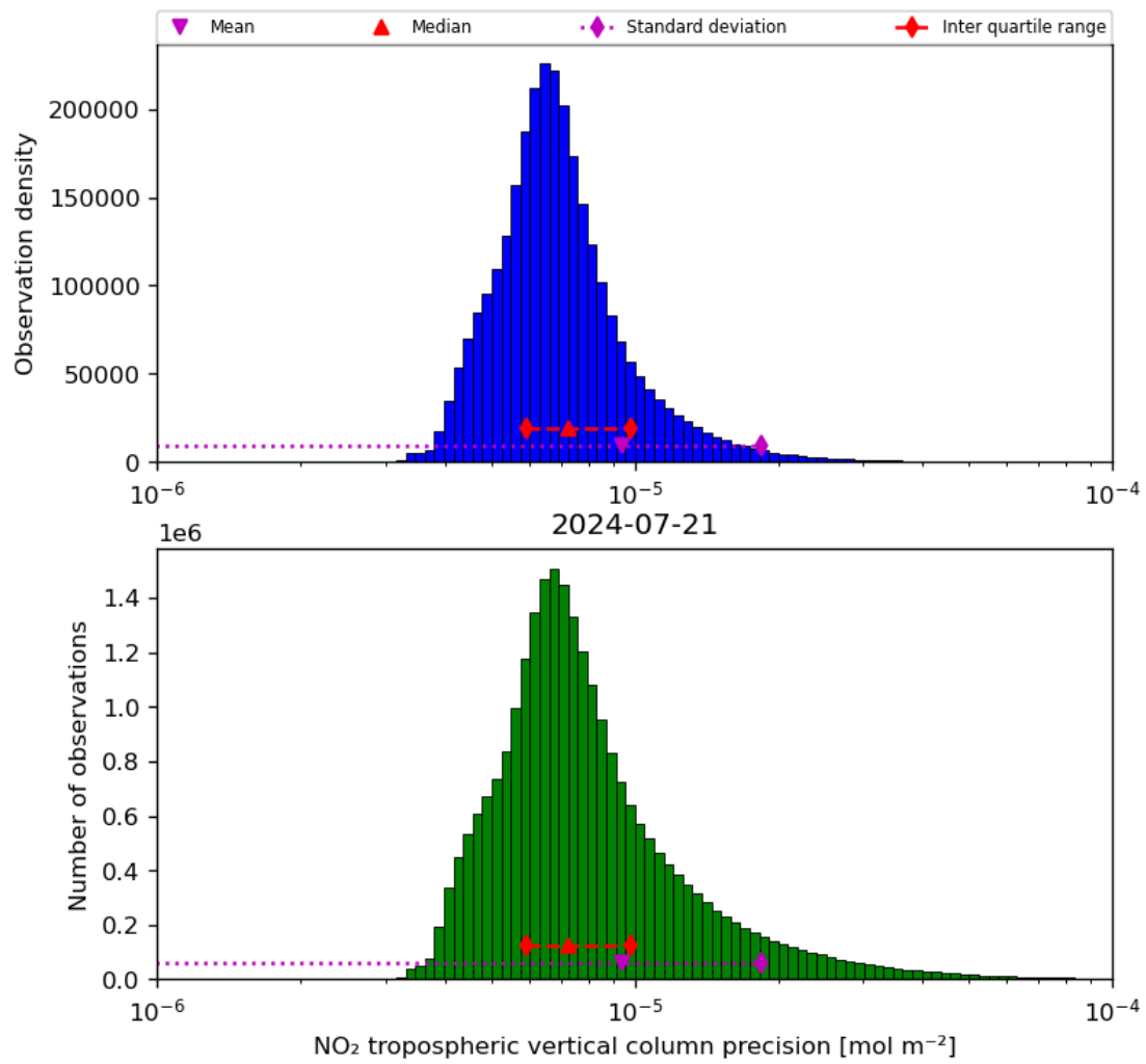
Figure 30: Histogram of “NO 2 tropospheric vertical column precision” for 2024-07-21 to 2024-07-22
