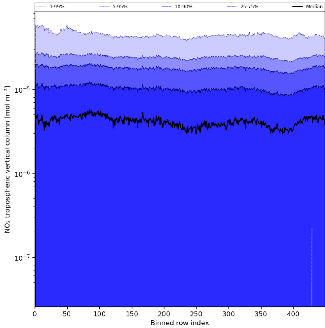
Figure 46: Along track statistics of “NO 2 tropospheric vertical column” for 2024-07-21 to 2024-07-22
