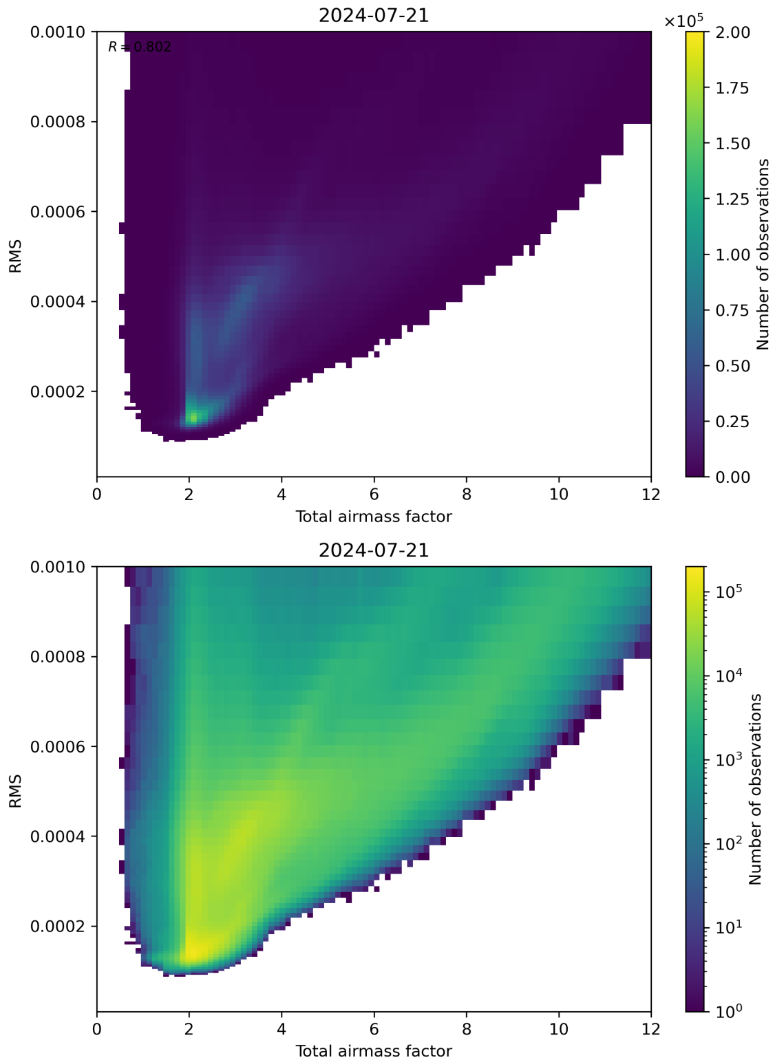
Figure 69: Scatter density plot of “Total airmass factor” against “RMS” for 2024-07-21 to 2024-07-22.
