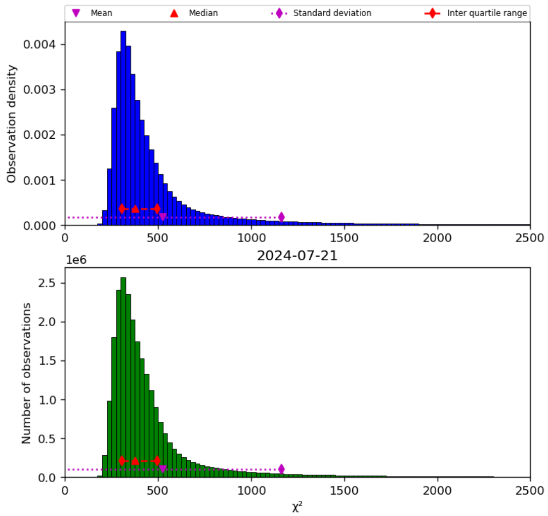
Figure 42: Histogram of “ \chi^2 ” for 2024-07-21 to 2024-07-22
