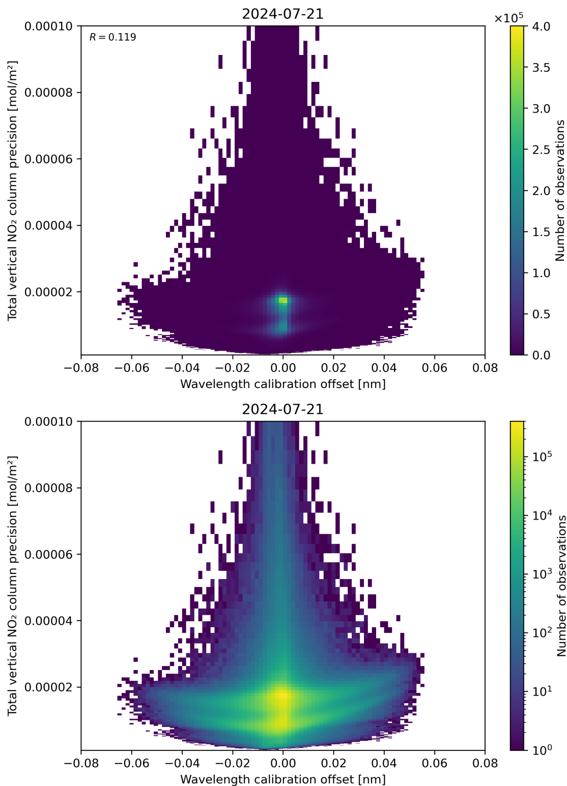
Figure 180: Scatter density plot of “Wavelength calibration offset” against “Total vertical NO 2 column precision” for 2024-07-21 to 2024-07-22.
