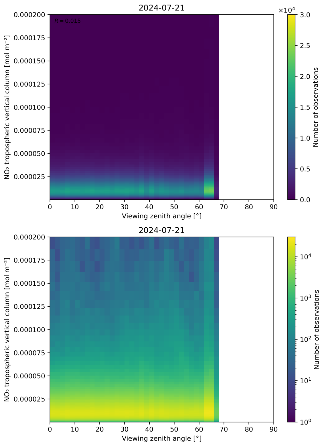
Figure 169: Scatter density plot of “Viewing zenith angle” against “NO 2 tropospheric vertical column” for 2024-07-21 to 2024-07-22.
