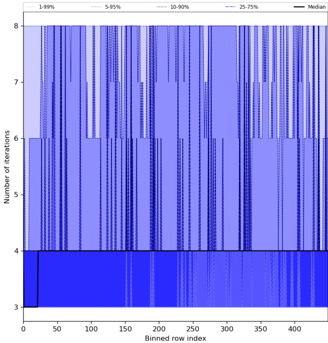
Figure 51: Along track statistics of “Number of iterations” for 2024-07-21 to 2024-07-22
