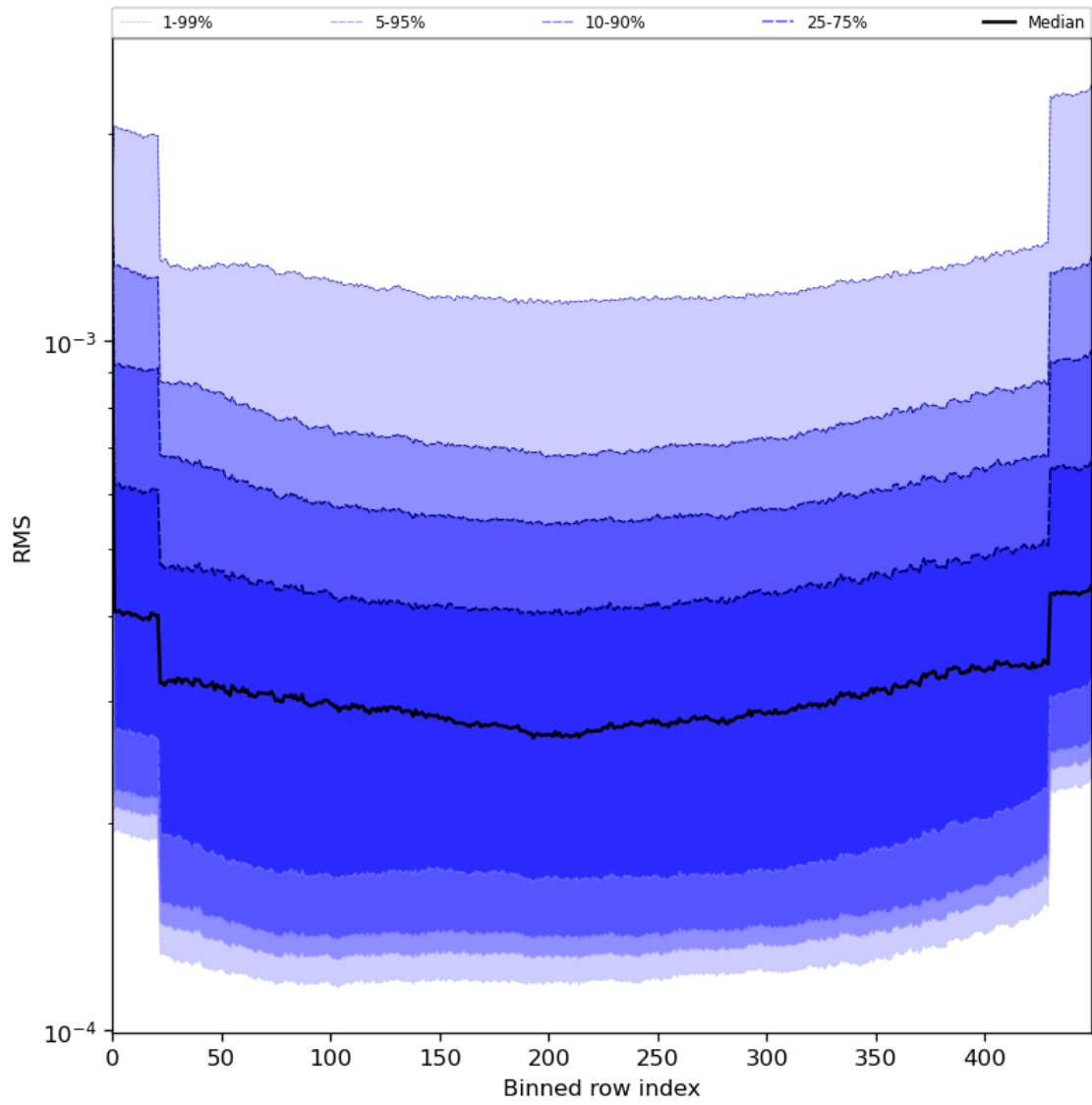
Figure 60: Along track statistics of “RMS” for 2024-07-21 to 2024-07-22
