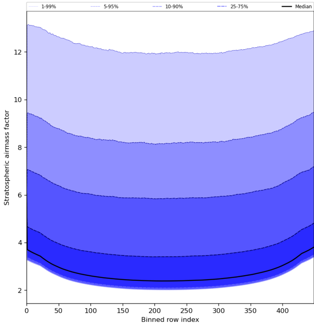
Figure 61: Along track statistics of “Stratospheric airmass factor” for 2024-07-21 to 2024-07-22
