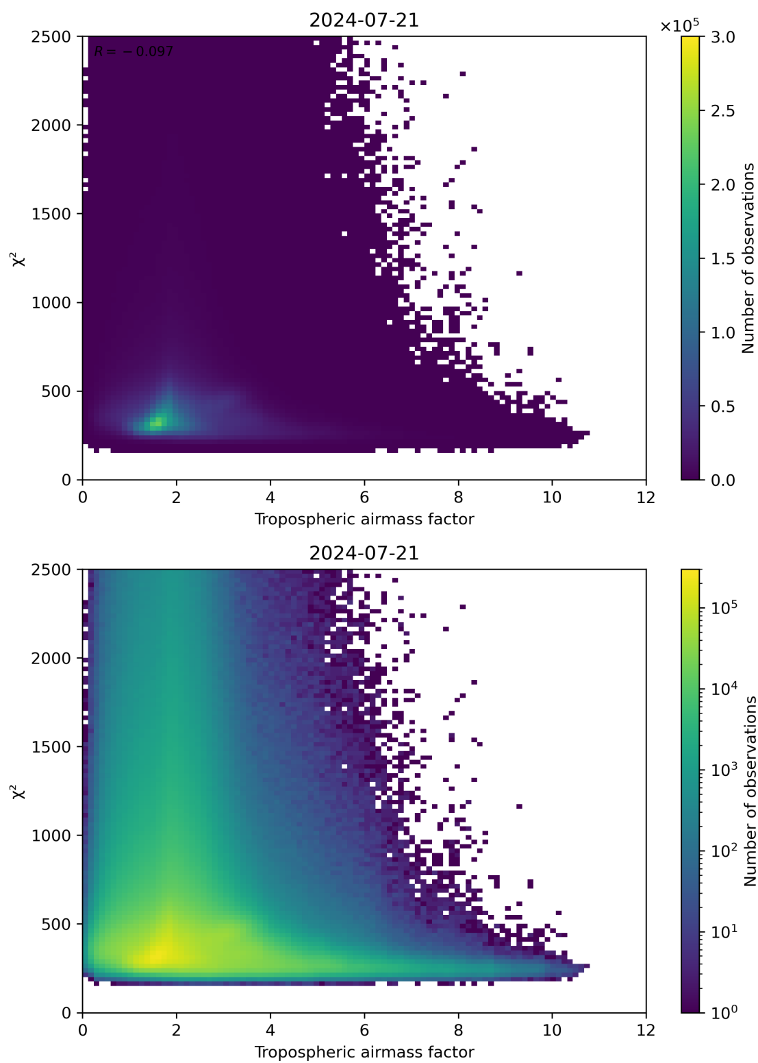
Figure 73: Scatter density plot of “Tropospheric airmass factor” against “ \chi^2 ” for 2024-07-21 to 2024-07-22.
