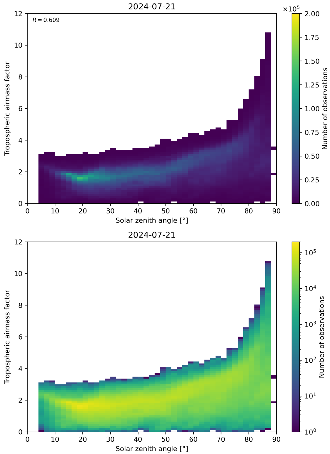
Figure 147: Scatter density plot of “Solar zenith angle” against “Tropospheric airmass factor” for 2024-07-21 to 2024-07-22.
