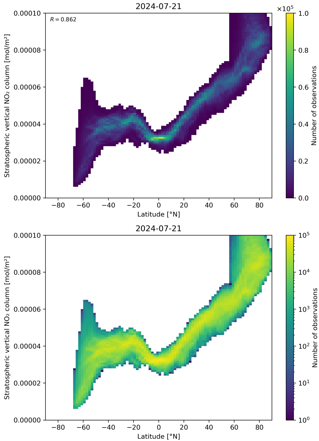
Figure 87: Scatter density plot of “Latitude” against “Stratospheric vertical NO 2 column” for 2024-07-21 to 2024-07-22.
