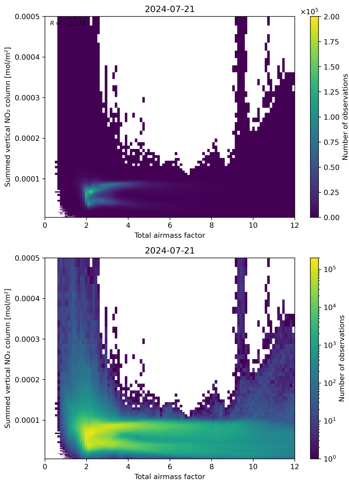
Figure 65: Scatter density plot of “Total airmass factor” against “Summed vertical NO 2 column” for 2024-07-21 to 2024-07-22.
