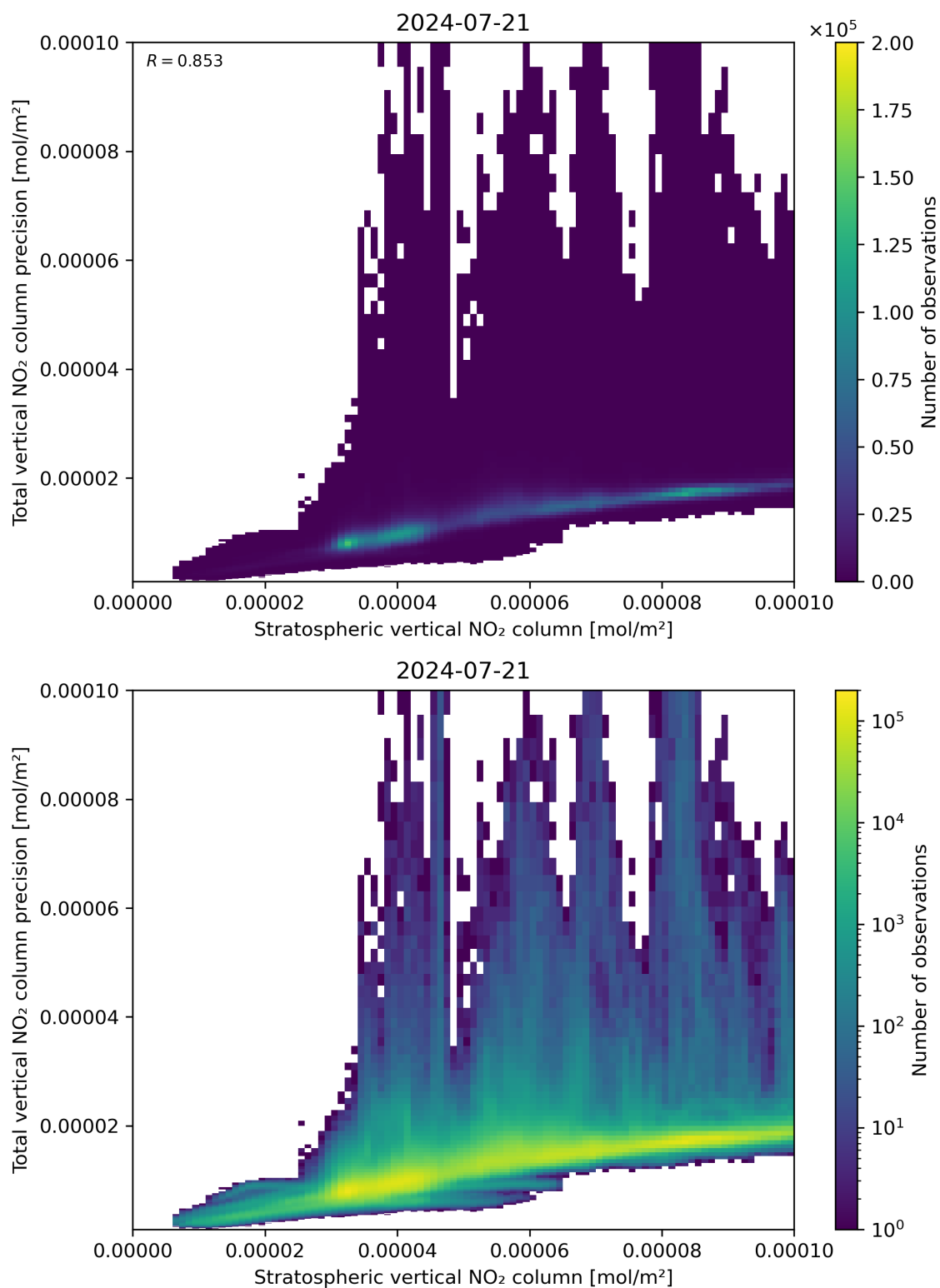
Figure 101: Scatter density plot of “Stratospheric vertical NO 2 column” against “Total vertical NO 2 column precision” for 2024-07-21 to 2024-07-22.
