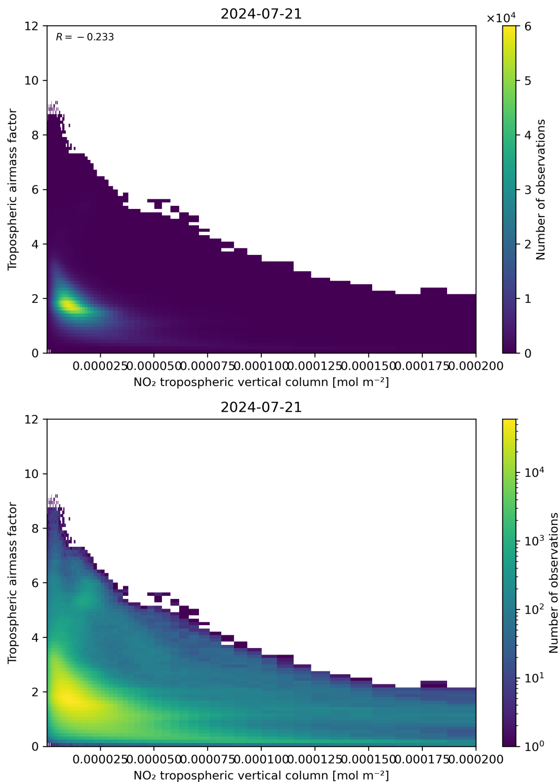
Figure 123: Scatter density plot of “NO 2 tropospheric vertical column” against “Tropospheric air mass factor” for 2024-07-21 to 2024-07-22.
