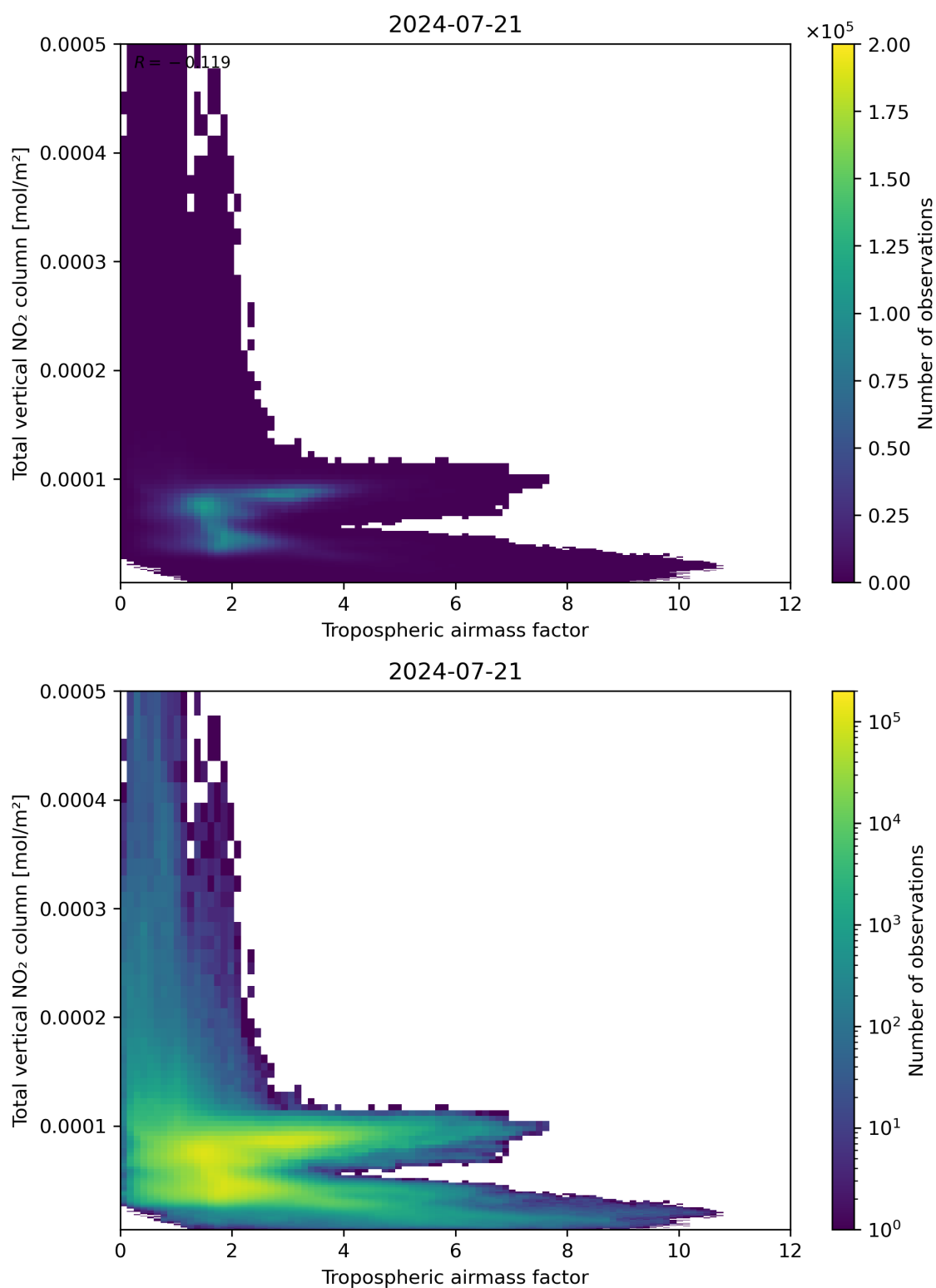
Figure 77: Scatter density plot of “Tropospheric airmass factor” against “Total vertical NO 2 column” for 2024-07-21 to 2024-07-22.
