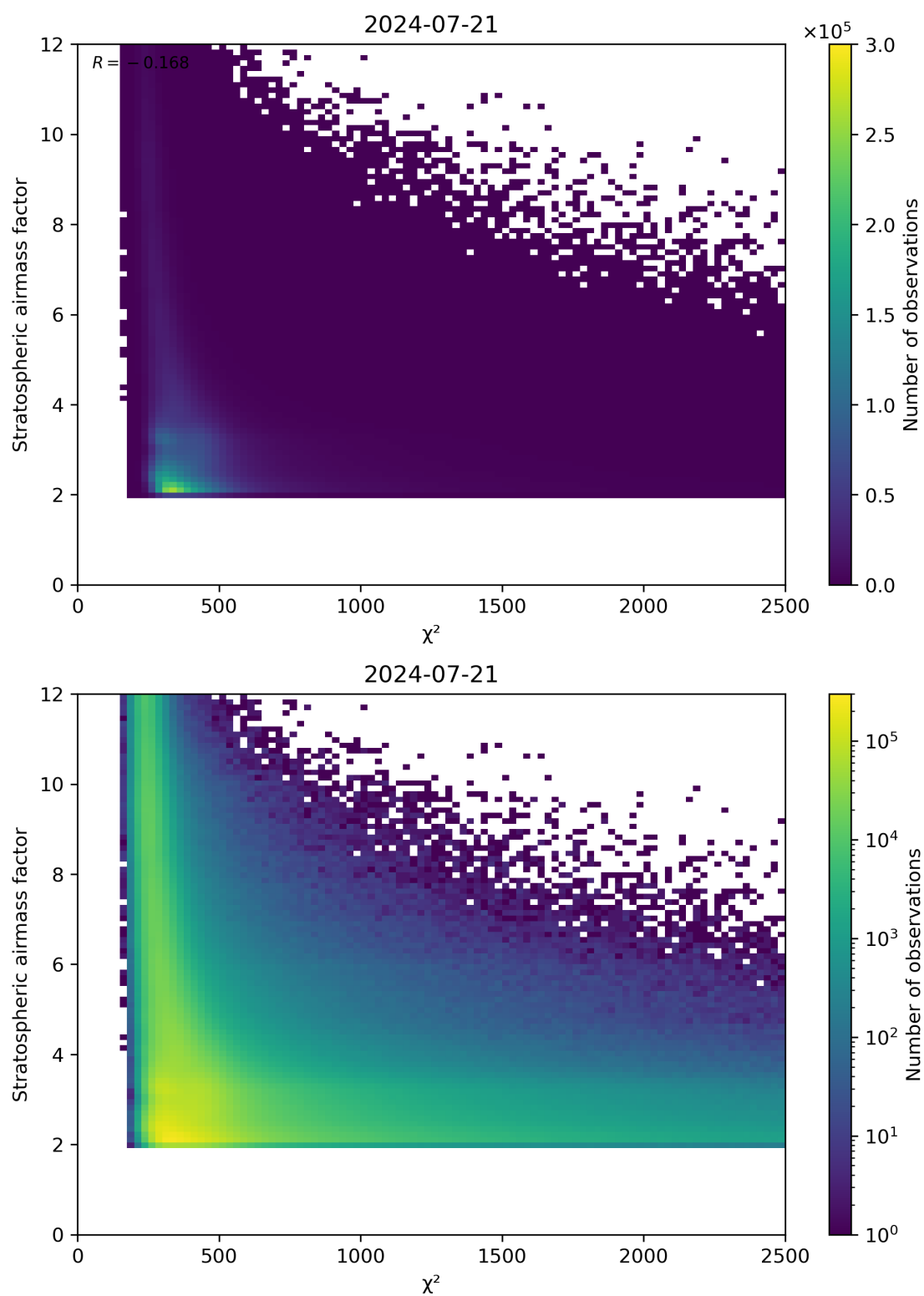
Figure 81: Scatter density plot of “ \chi^2 ” against “Stratospheric airmass factor” for 2024-07-21 to 2024-07-22.
