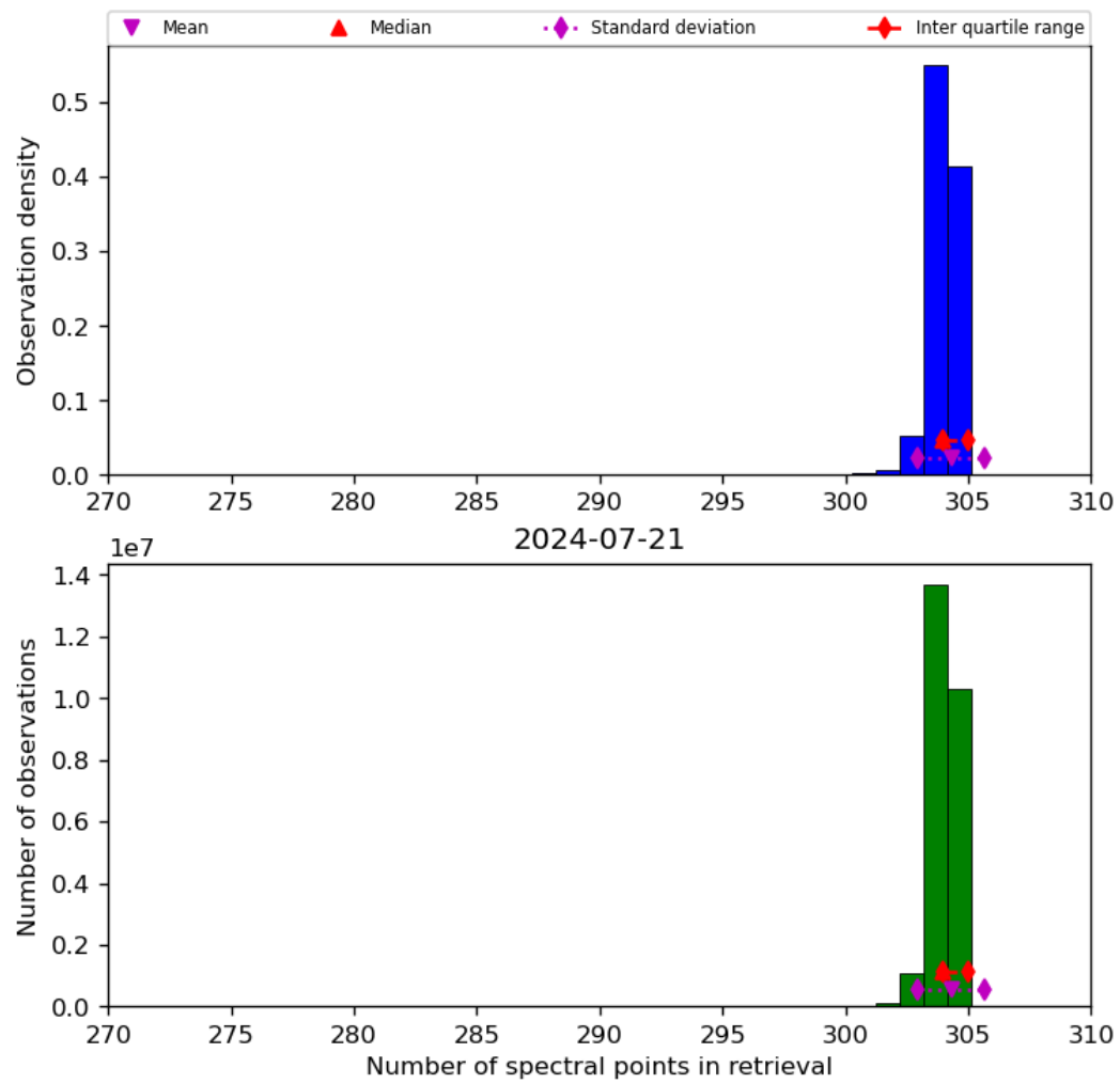
Figure 33: Histogram of “Number of spectral points in retrieval” for 2024-07-21 to 2024-07-22
