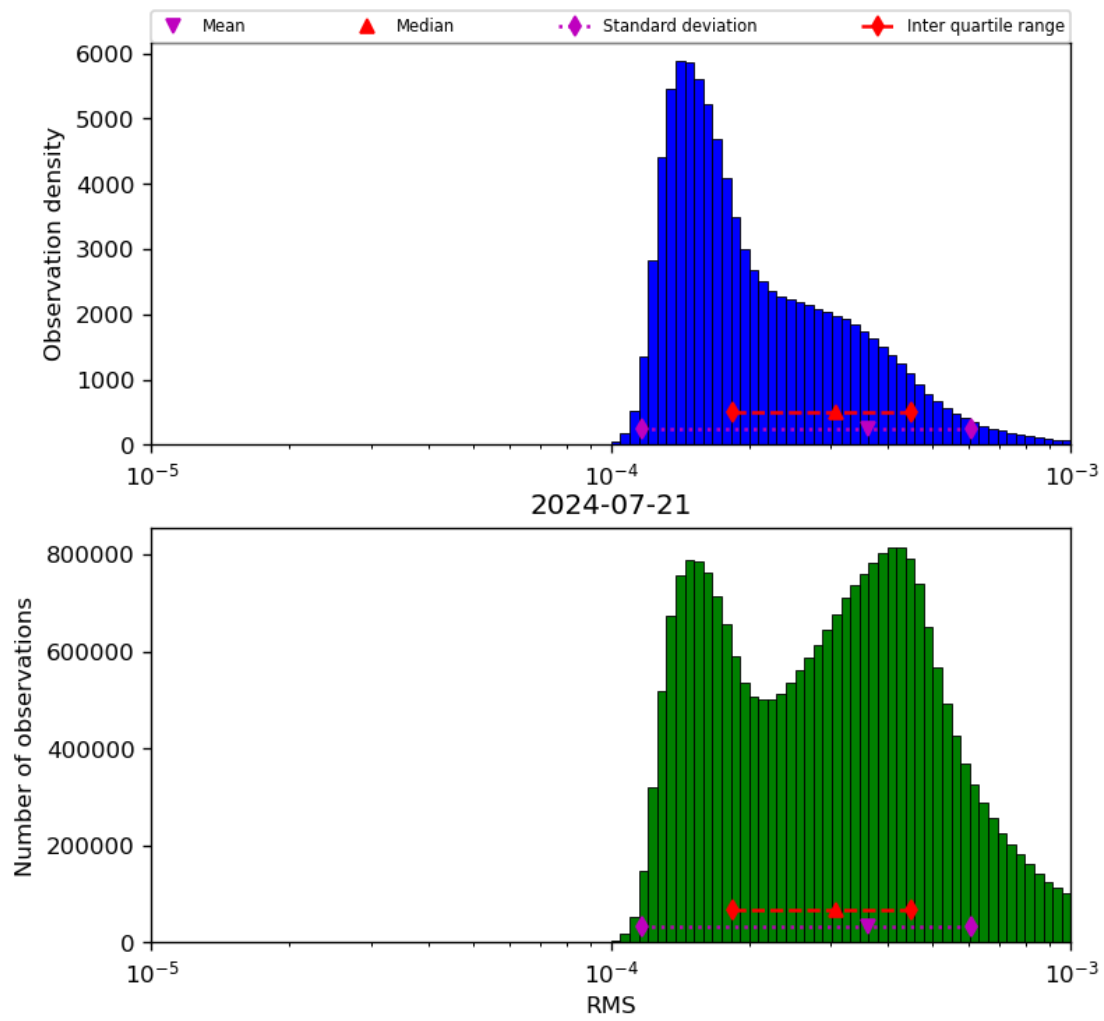
Figure 43: Histogram of “RMS” for 2024-07-21 to 2024-07-22
