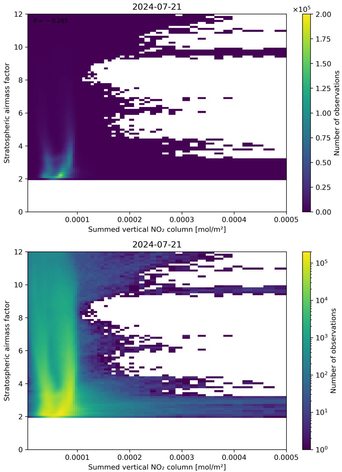
Figure 103: Scatter density plot of “Summed vertical NO 2 column” against “Stratospheric air mass factor” for 2024-07-21 to 2024-07-22.
