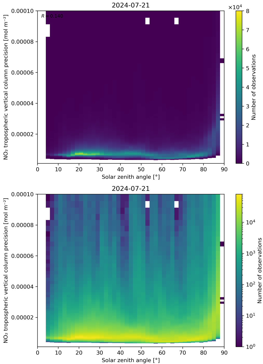
Figure 156: Scatter density plot of “Solar zenith angle” against “NO 2 tropospheric vertical column precision” for 2024-07-21 to 2024-07-22.
