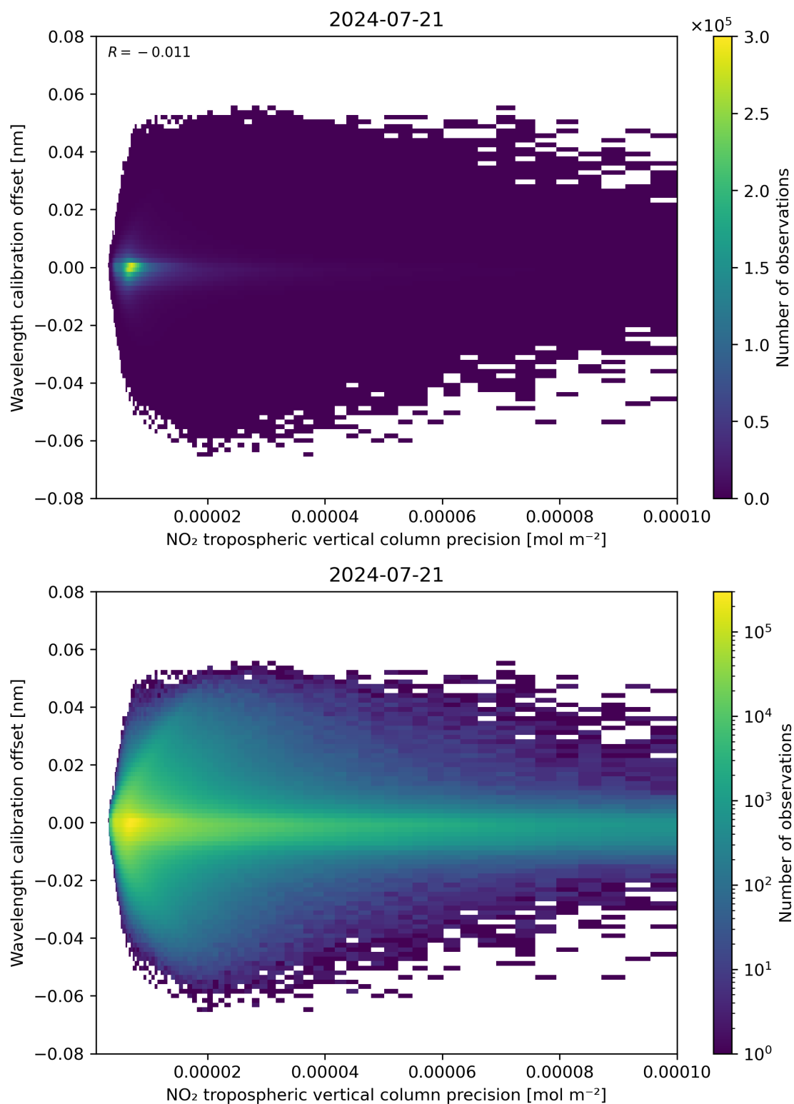
Figure 141: Scatter density plot of “NO 2 tropospheric vertical column precision” against “Wavelength calibration offset” for 2024-07-21 to 2024-07-22.
