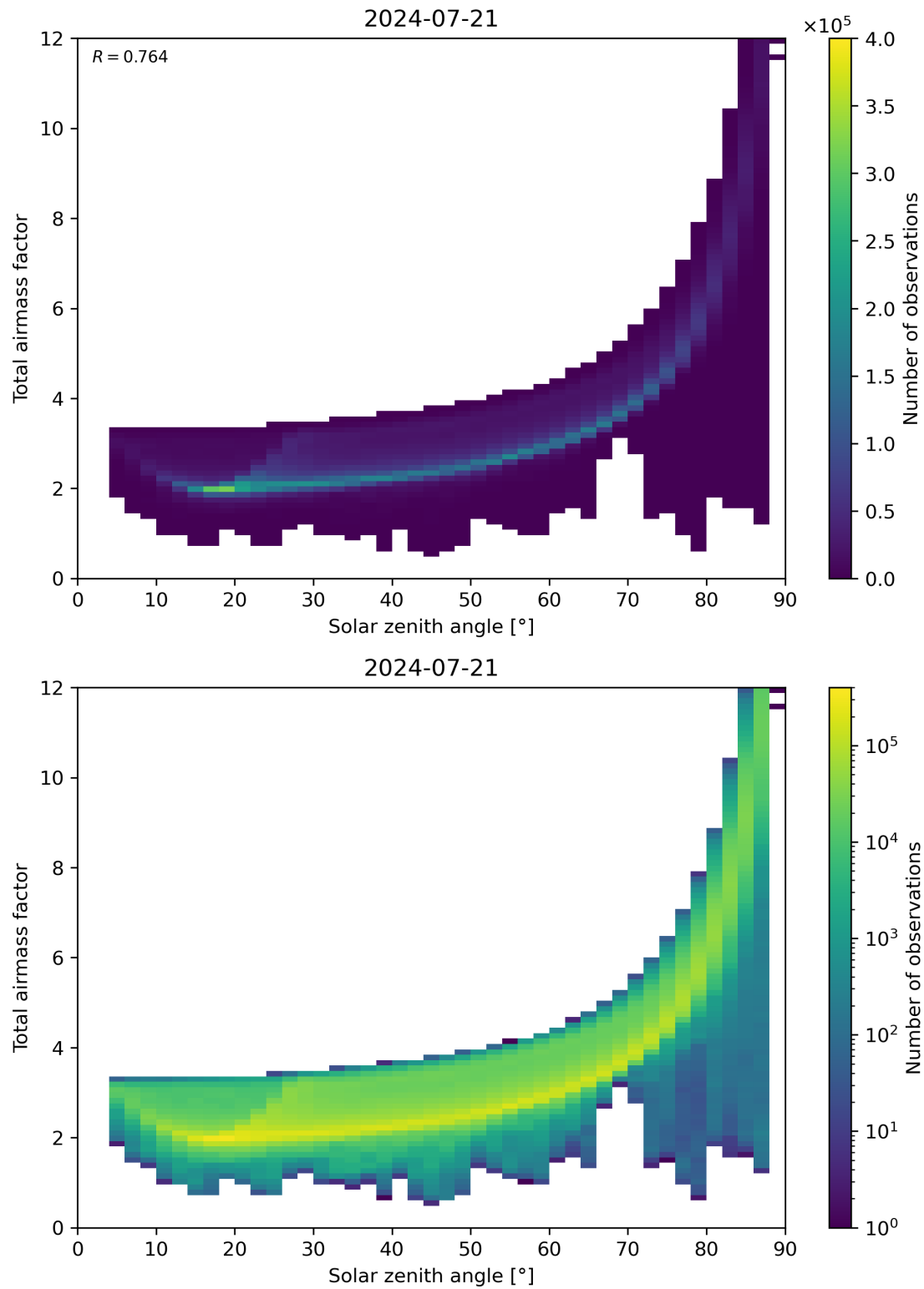
Figure 146: Scatter density plot of “Solar zenith angle” against “Total air mass factor” for 2024-07-21 to 2024-07-22.
