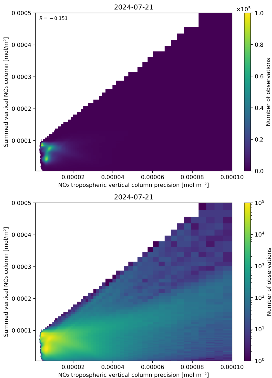
Figure 136: Scatter density plot of “NO 2 tropospheric vertical column precision” against “Summed vertical NO 2 column” for 2024-07-21 to 2024-07-22.
