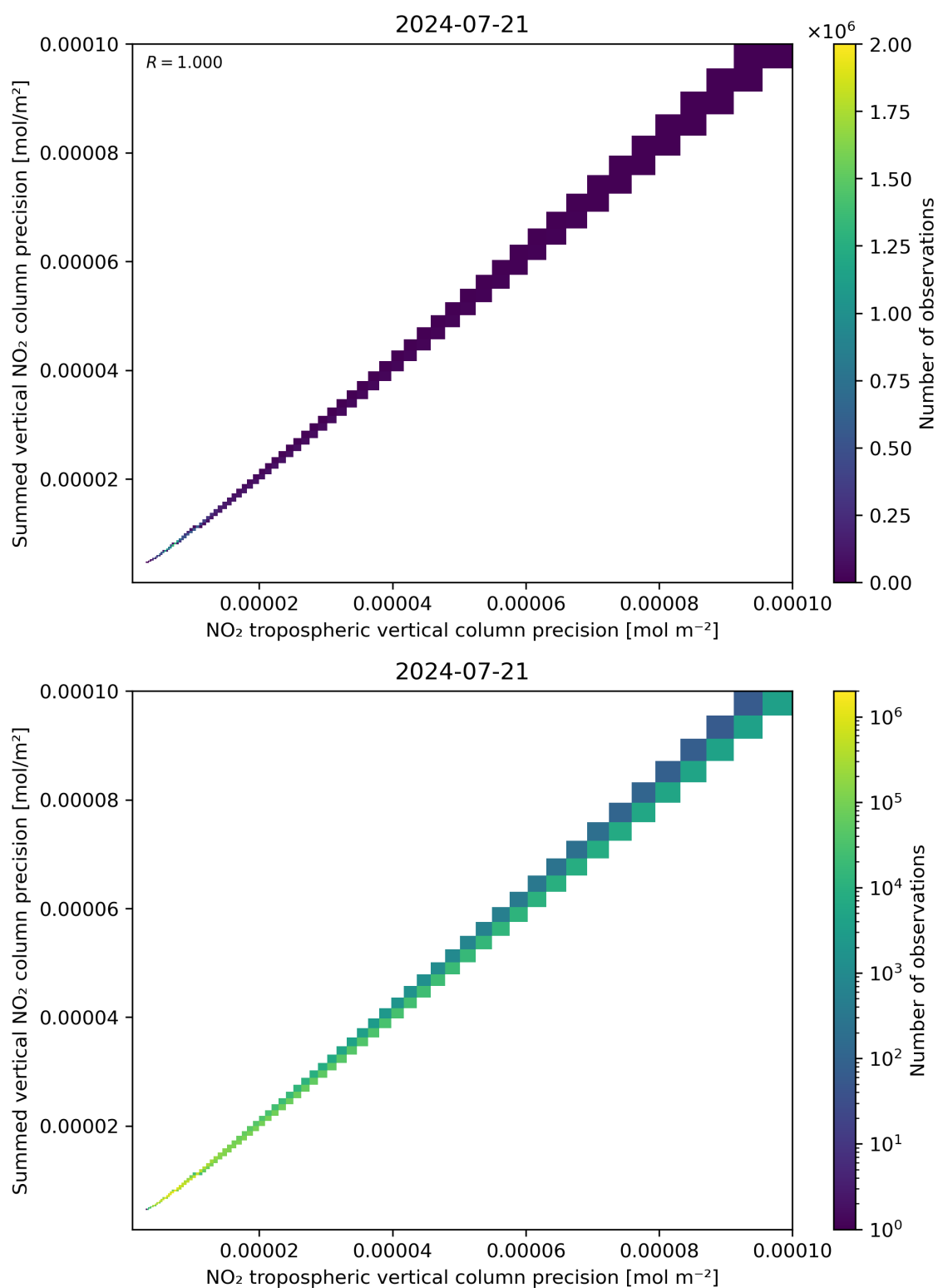
Figure 137: Scatter density plot of “NO 2 tropospheric vertical column precision” against “Summed vertical NO 2 column precision” for 2024-07-21 to 2024-07-22.
