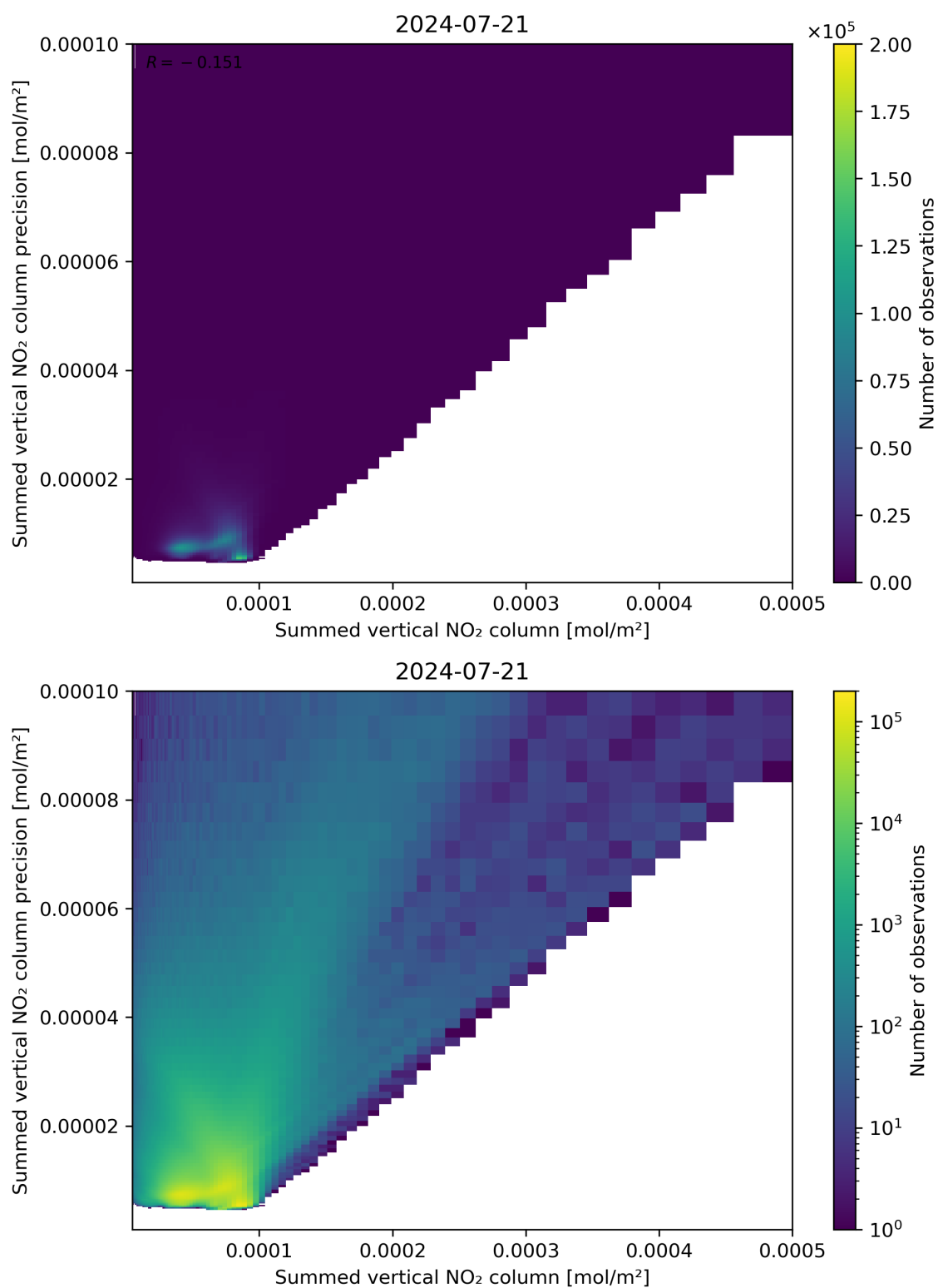
Figure 105: Scatter density plot of “Summed vertical NO 2 column” against “Summed vertical NO 2 column precision” for 2024-07-21 to 2024-07-22.
