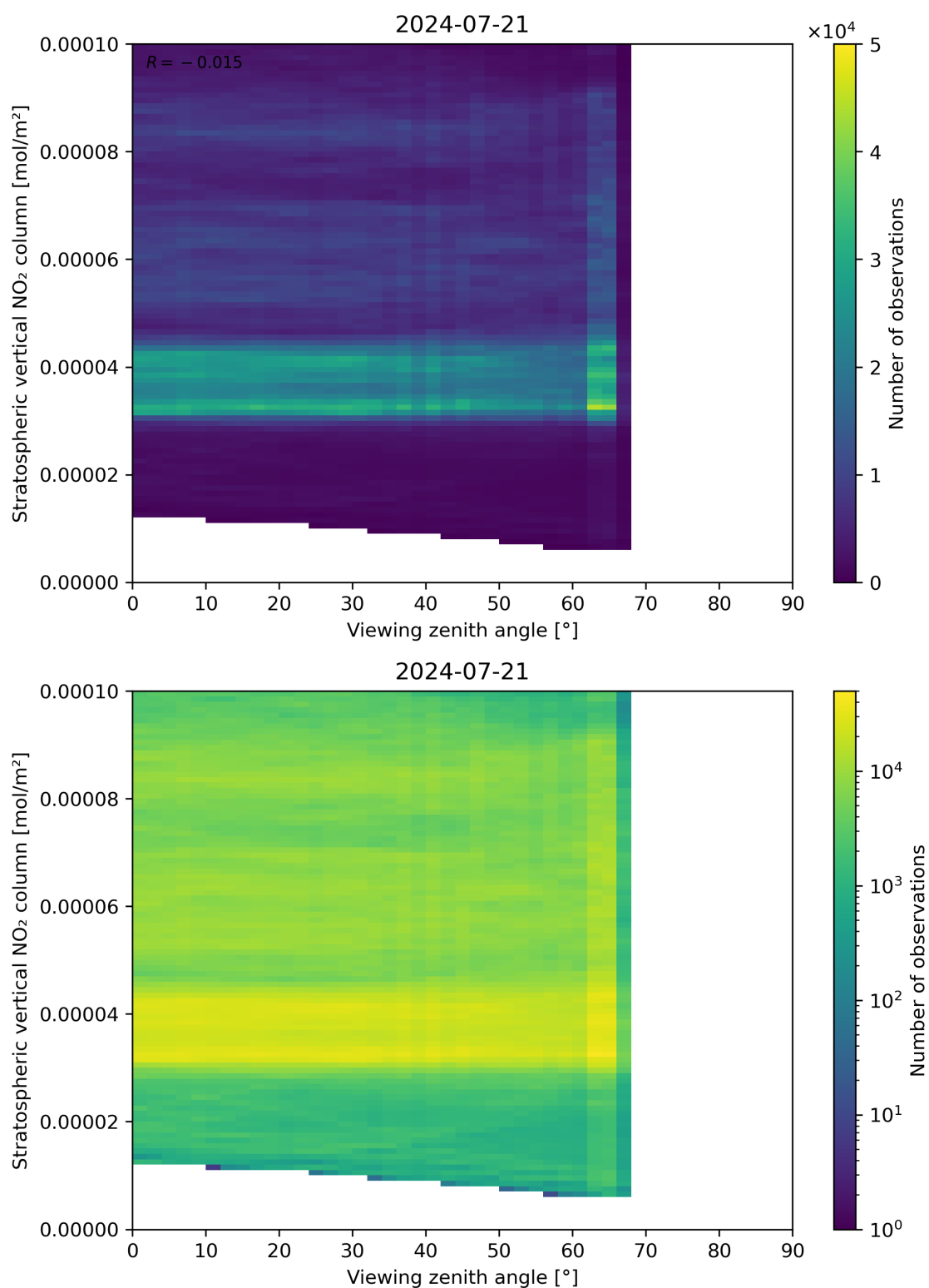
Figure 164: Scatter density plot of “Viewing zenith angle” against “Stratospheric vertical NO 2 column” for 2024-07-21 to 2024-07-22.
