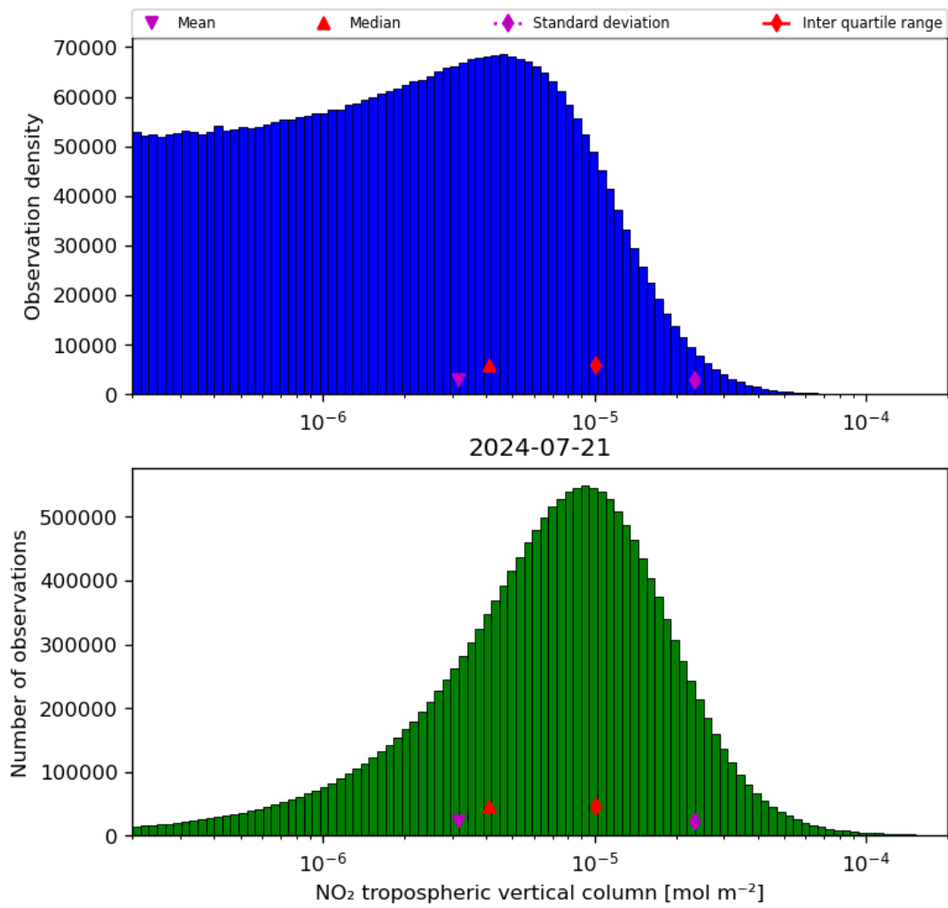
Figure 29: Histogram of “NO 2 tropospheric vertical column” for 2024-07-21 to 2024-07-22
