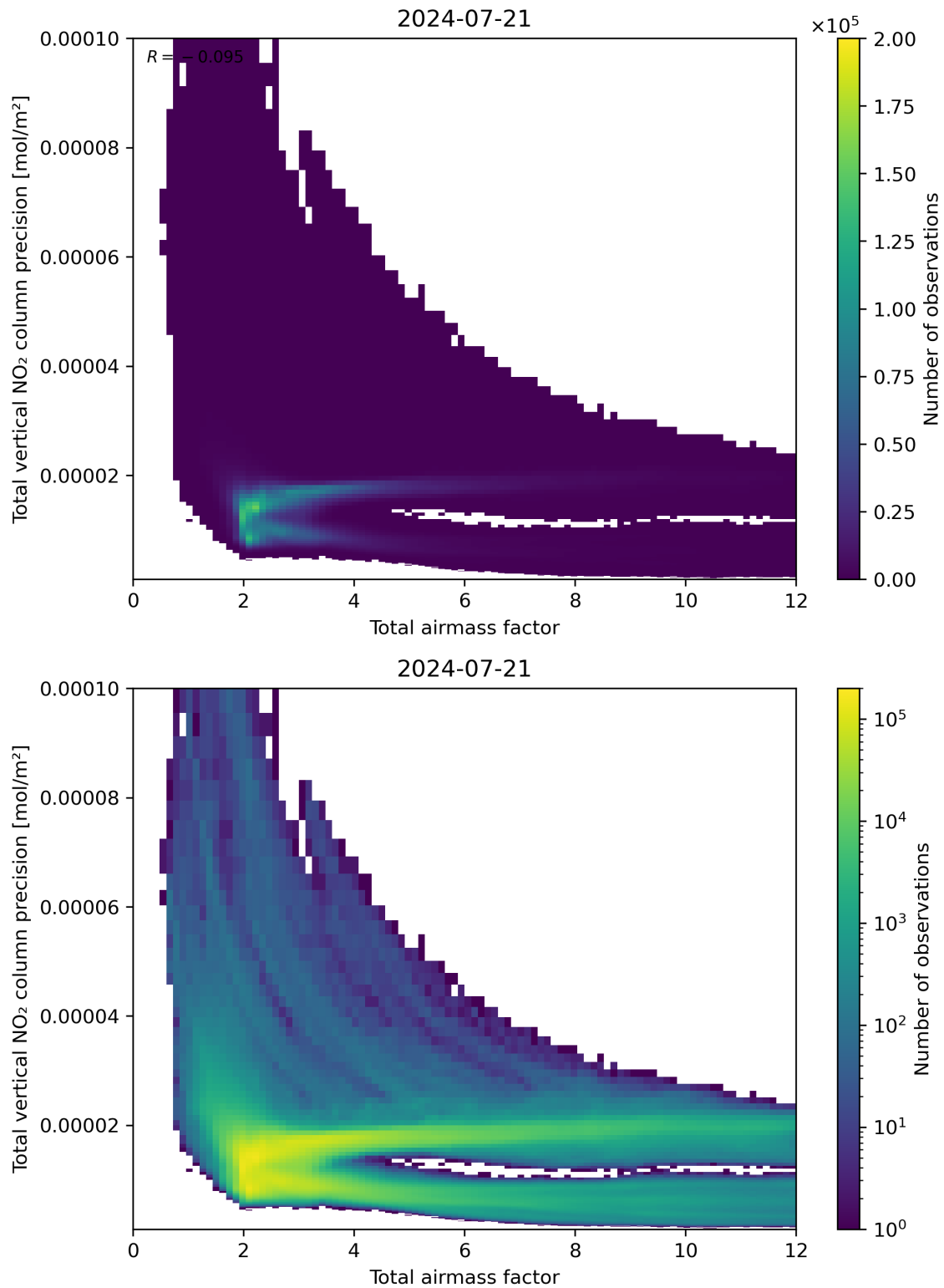
Figure 68: Scatter density plot of “Total airmass factor” against “Total vertical NO 2 column precision” for 2024-07-21 to 2024-07-22.
