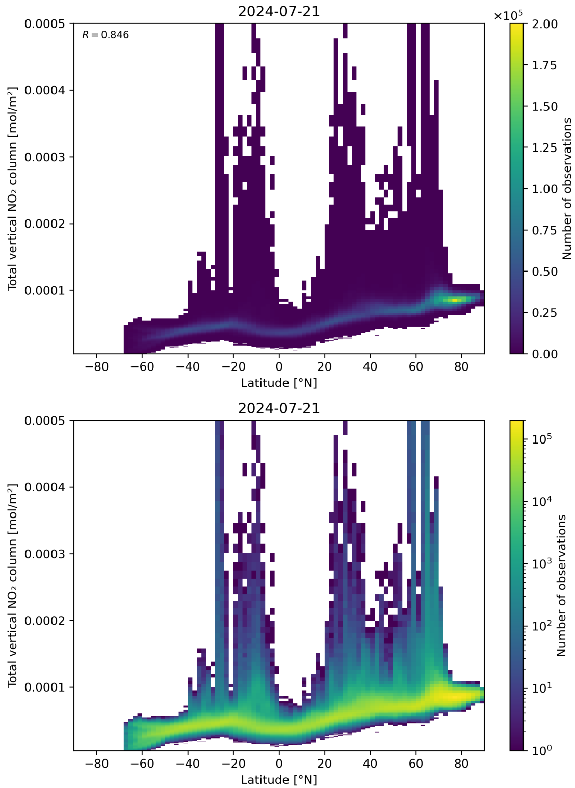
Figure 90: Scatter density plot of “Latitude” against “Total vertical NO 2 column” for 2024-07-21 to 2024-07-22.
