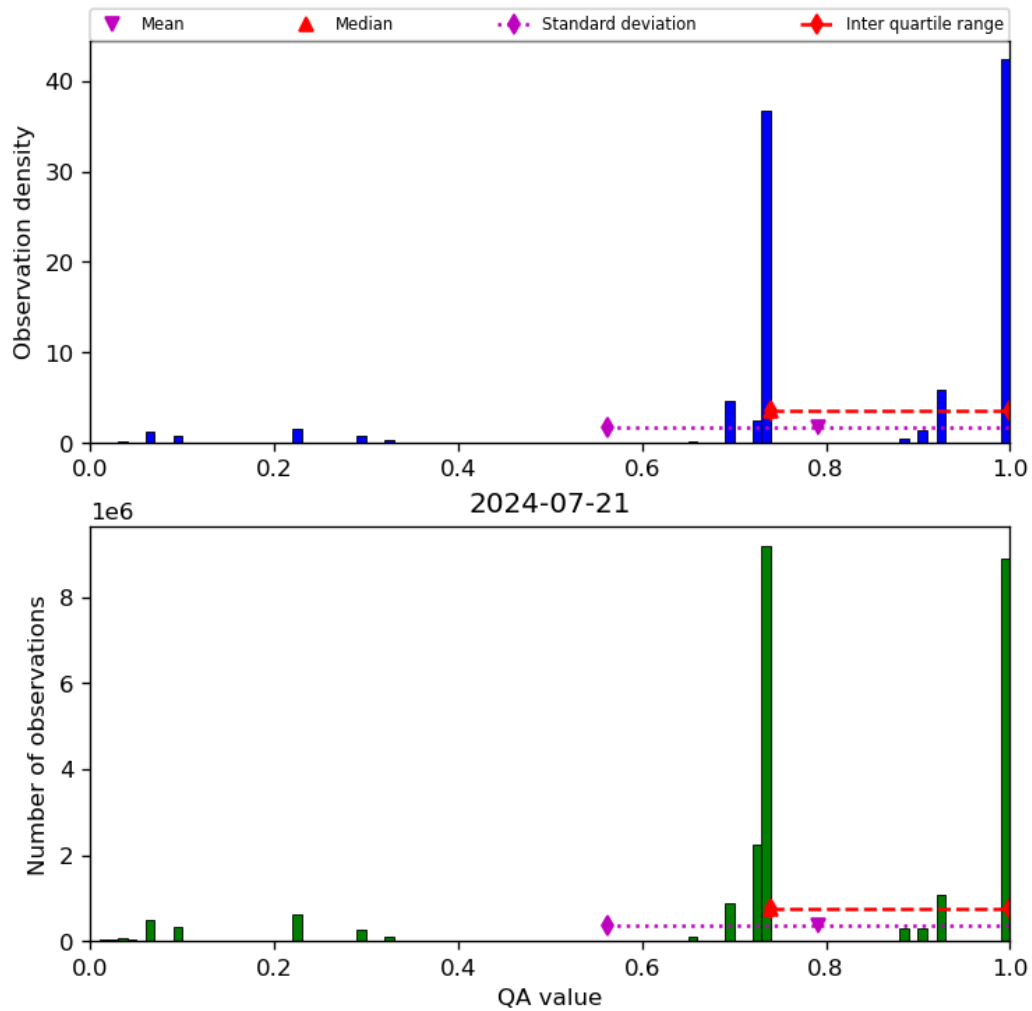
Figure 28: Histogram of “QA value” for 2024-07-21 to 2024-07-22
