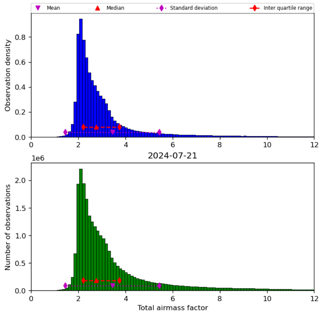
Figure 32: Histogram of “Total airmass factor” for 2024-07-21 to 2024-07-22
