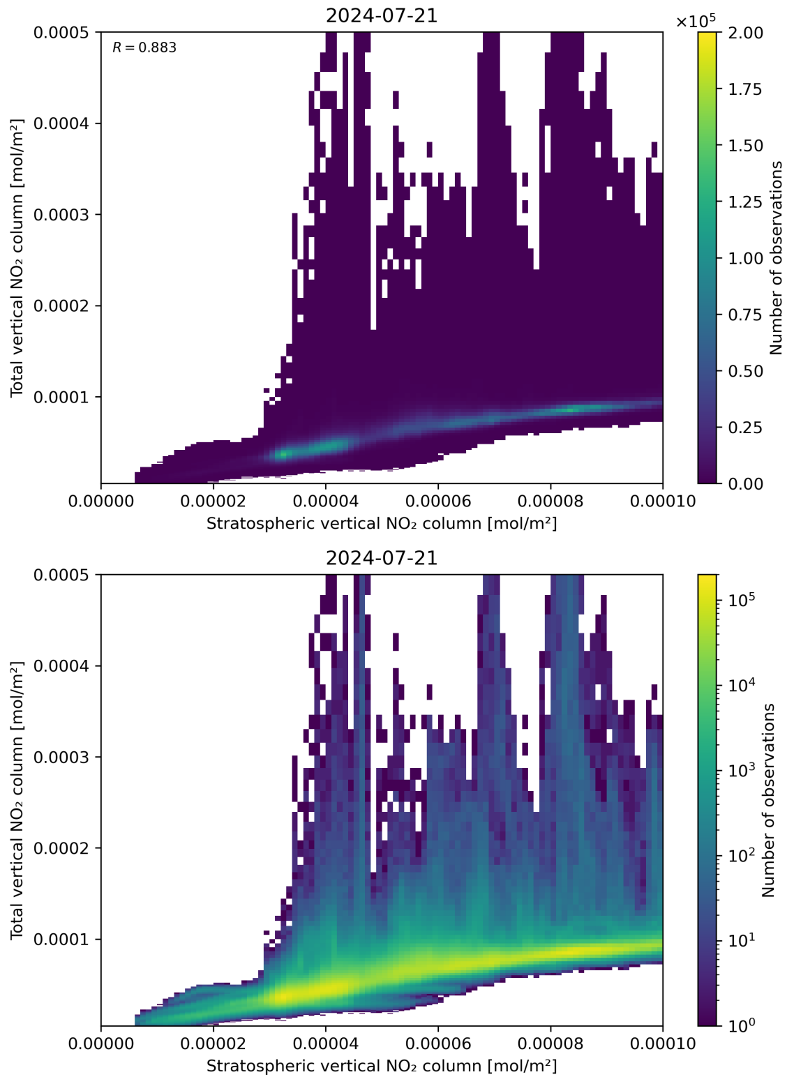
Figure 100: Scatter density plot of “Stratospheric vertical NO 2 column” against “Total vertical NO 2 column” for 2024-07-21 to 2024-07-22.
