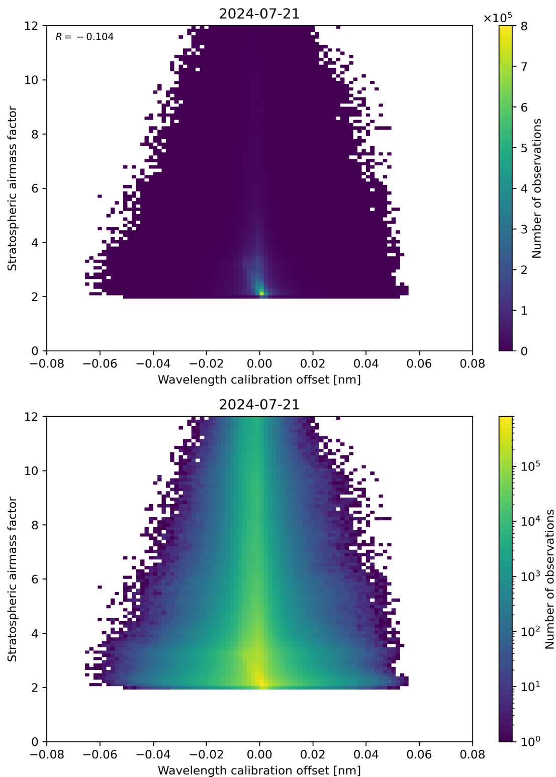
Figure 174: Scatter density plot of “Wavelength calibration offset” against “Stratospheric airmass factor” for 2024-07-21 to 2024-07-22.
