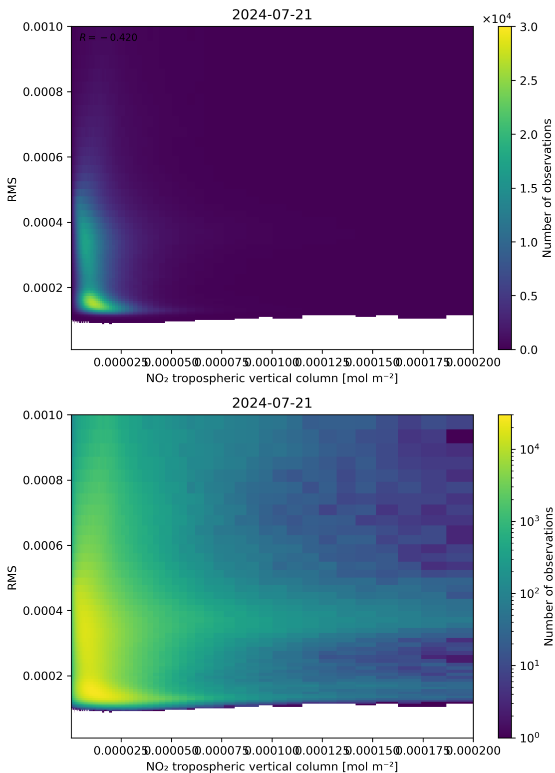
Figure 142: Scatter density plot of “NO 2 tropospheric vertical column” against “RMS” for 2024-07-21 to 2024-07-22.
