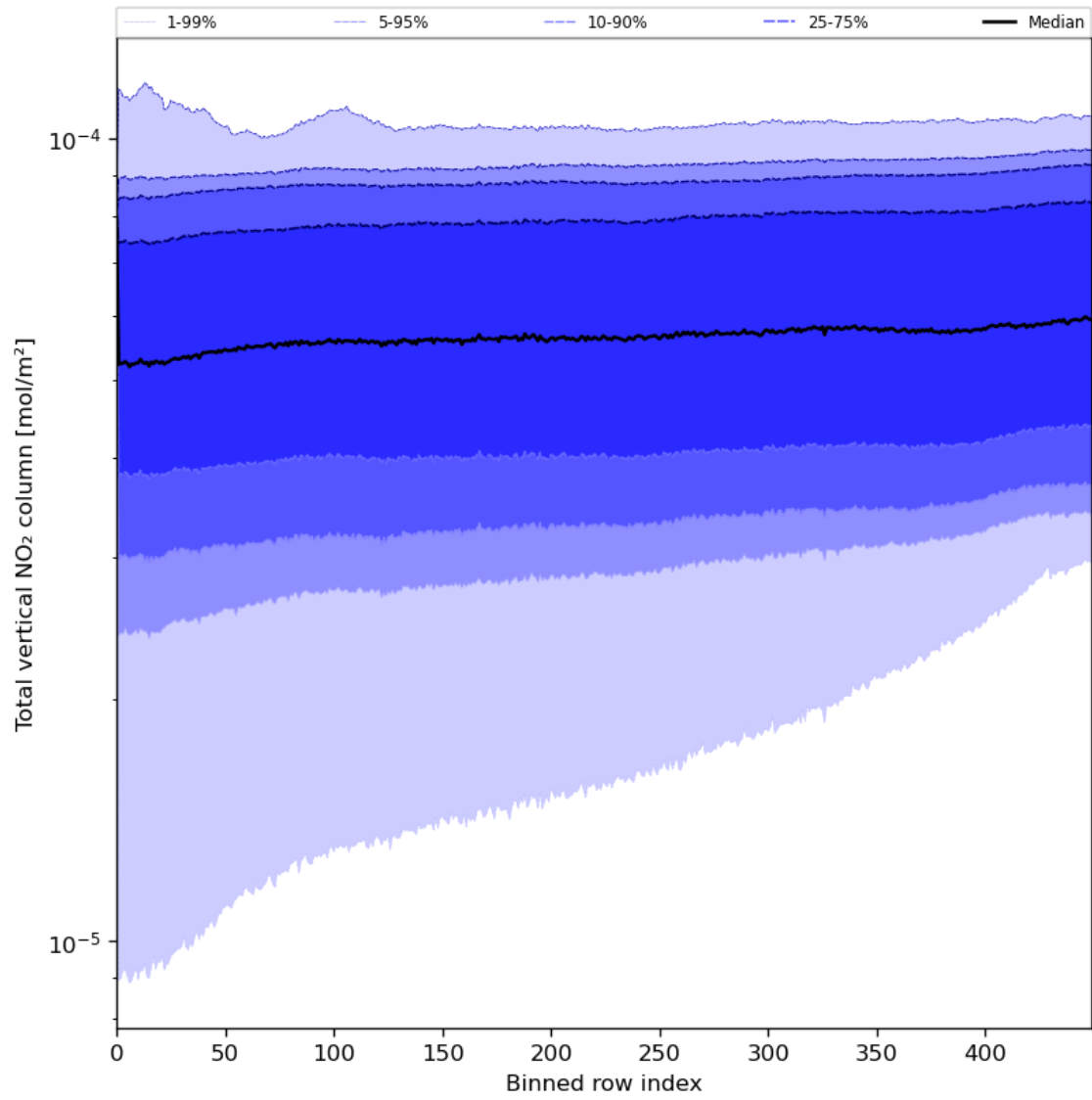
Figure 55: Along track statistics of “Total vertical NO 2 column” for 2024-07-21 to 2024-07-22
