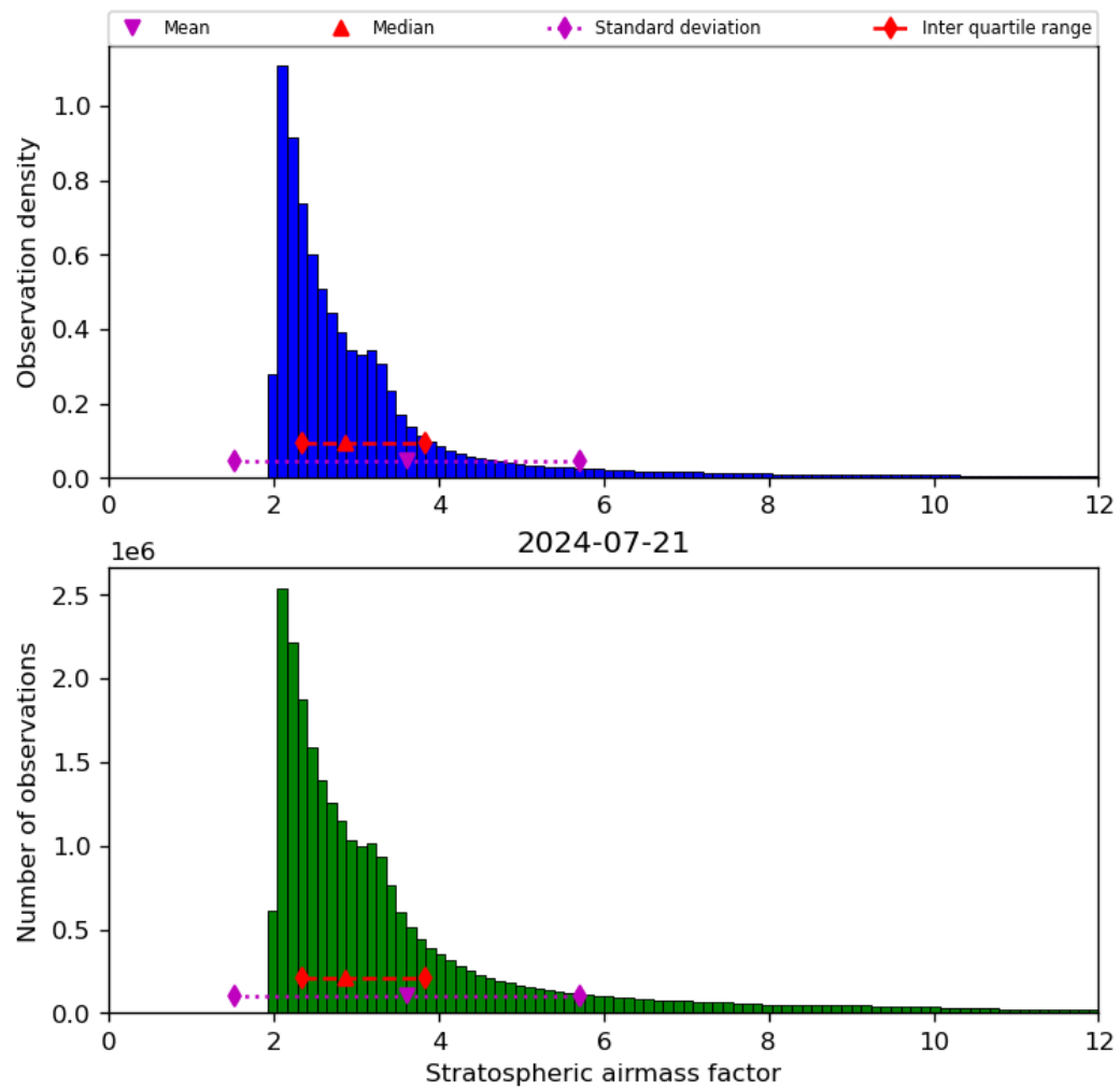
Figure 44: Histogram of “Stratospheric airmass factor” for 2024-07-21 to 2024-07-22
