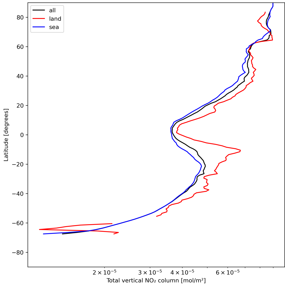
Figure 21: Zonal average of “Total vertical NO 2 column” for 2024-07-21 to 2024-07-22.
