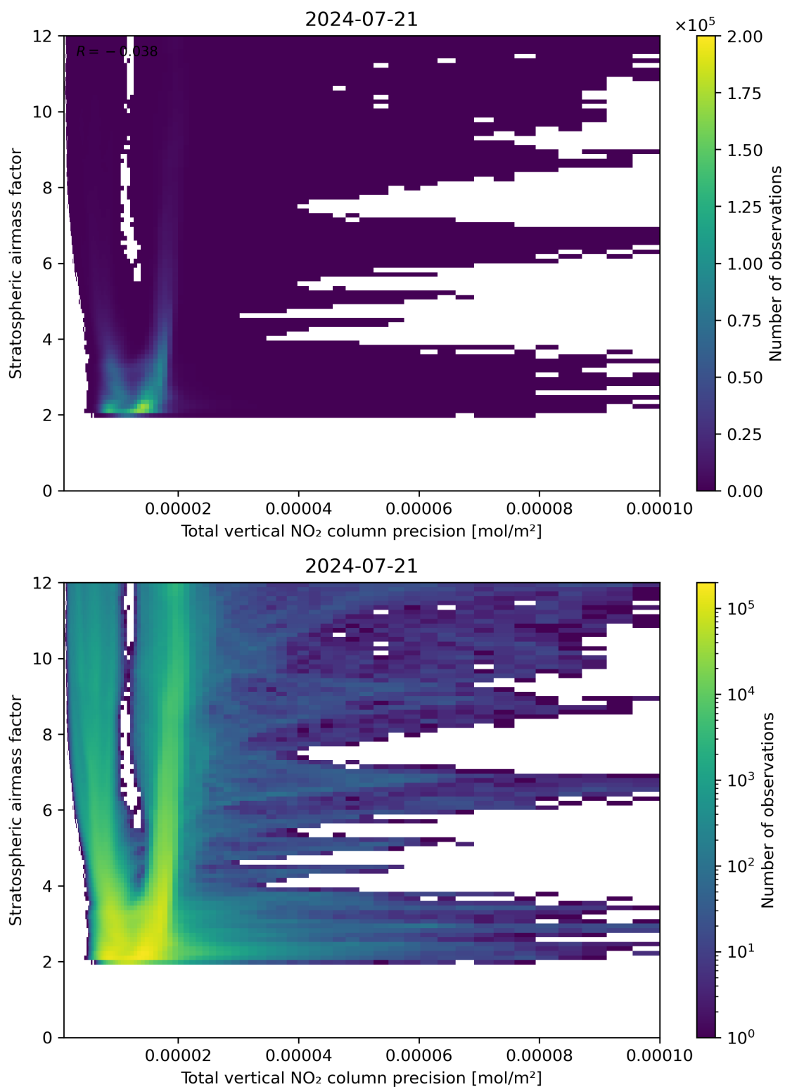
Figure 115: Scatter density plot of “Total vertical NO 2 column precision” against “Stratospheric air mass factor” for 2024-07-21 to 2024-07-22.
