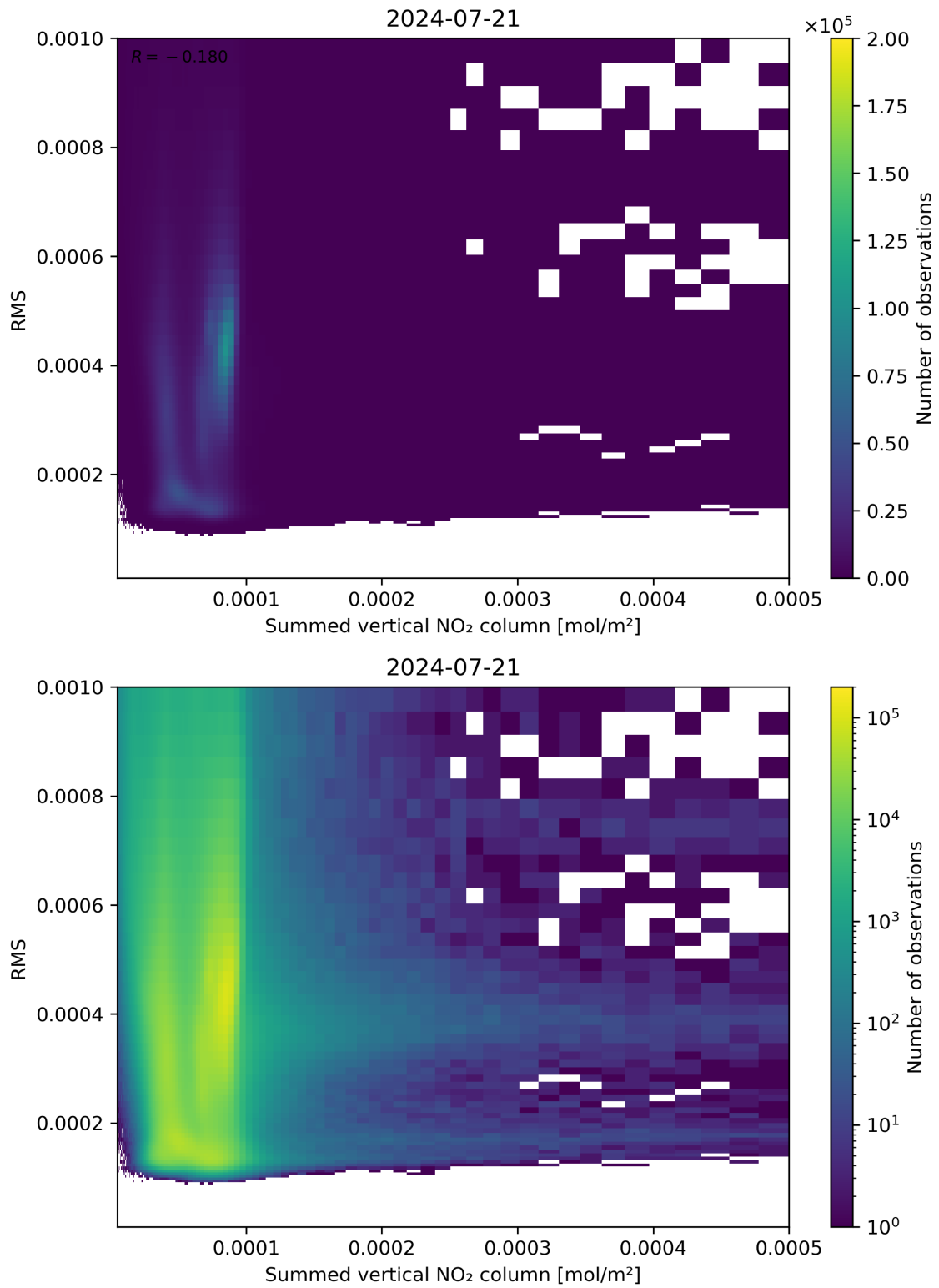
Figure 109: Scatter density plot of “Summed vertical NO 2 column” against “RMS” for 2024-07-21 to 2024-07-22.
