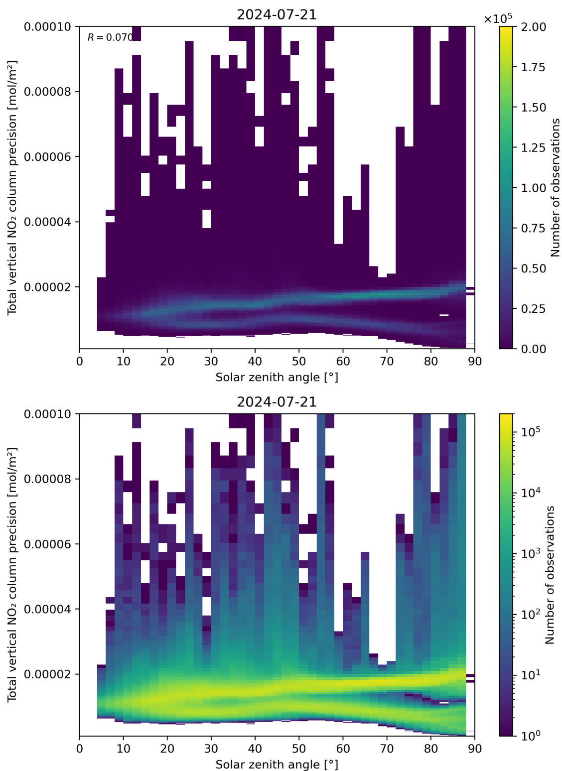
Figure 154: Scatter density plot of “Solar zenith angle” against “Total vertical NO 2 column precision” for 2024-07-21 to 2024-07-22.
