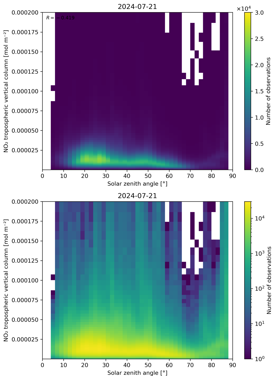
Figure 155: Scatter density plot of “Solar zenith angle” against “NO 2 tropospheric vertical column” for 2024-07-21 to 2024-07-22.
