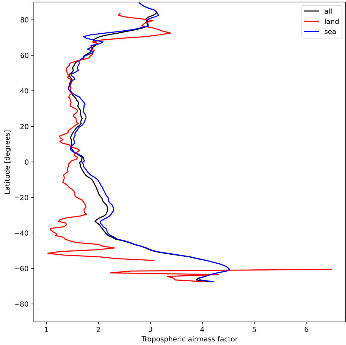
Figure 14: Zonal average of “Tropospheric airmass factor” for 2024-07-21 to 2024-07-22.
