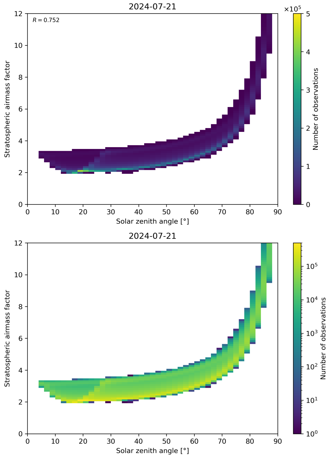
Figure 145: Scatter density plot of “Solar zenith angle” against “Stratospheric airmass factor” for 2024-07-21 to 2024-07-22.
