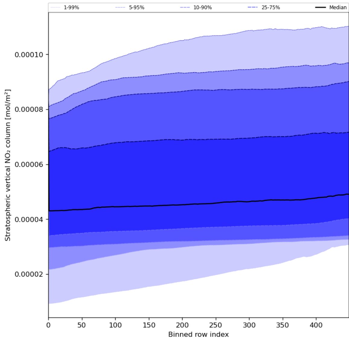
Figure 53: Along track statistics of “Stratospheric vertical NO 2 column” for 2024-07-21 to 2024-07-22
