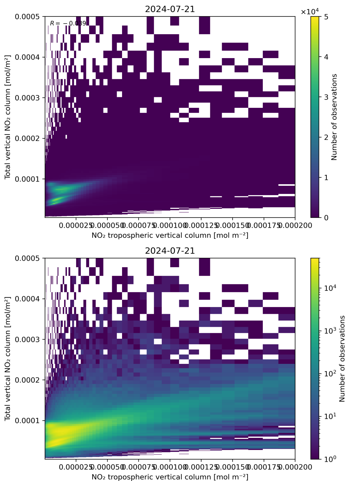
Figure 128: Scatter density plot of “NO 2 tropospheric vertical column” against “Total vertical NO 2 column” for 2024-07-21 to 2024-07-22.
