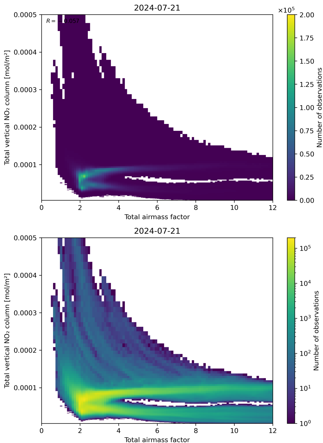
Figure 67: Scatter density plot of “Total airmass factor” against “Total vertical NO 2 column” for 2024-07-21 to 2024-07-22.
