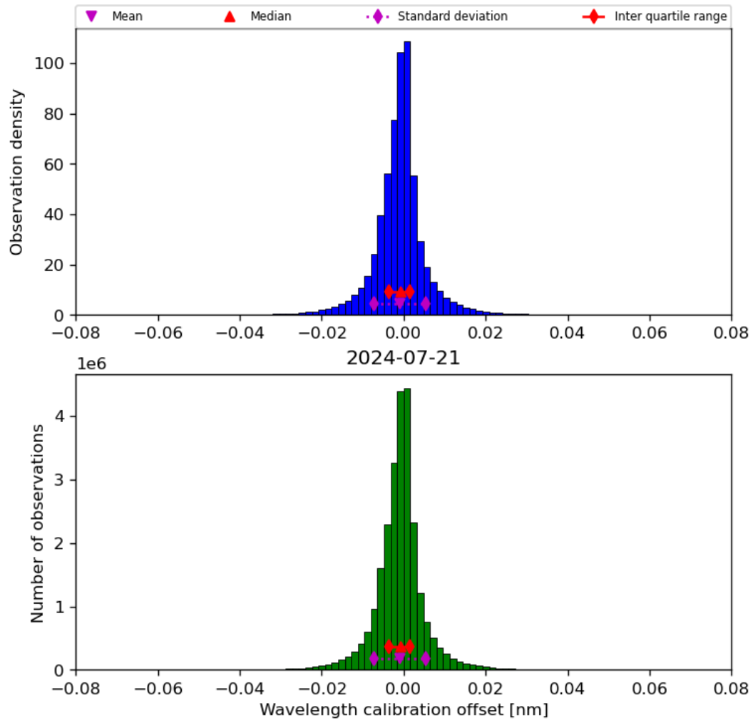
Figure 35: Histogram of “Wavelength calibration offset” for 2024-07-21 to 2024-07-22
