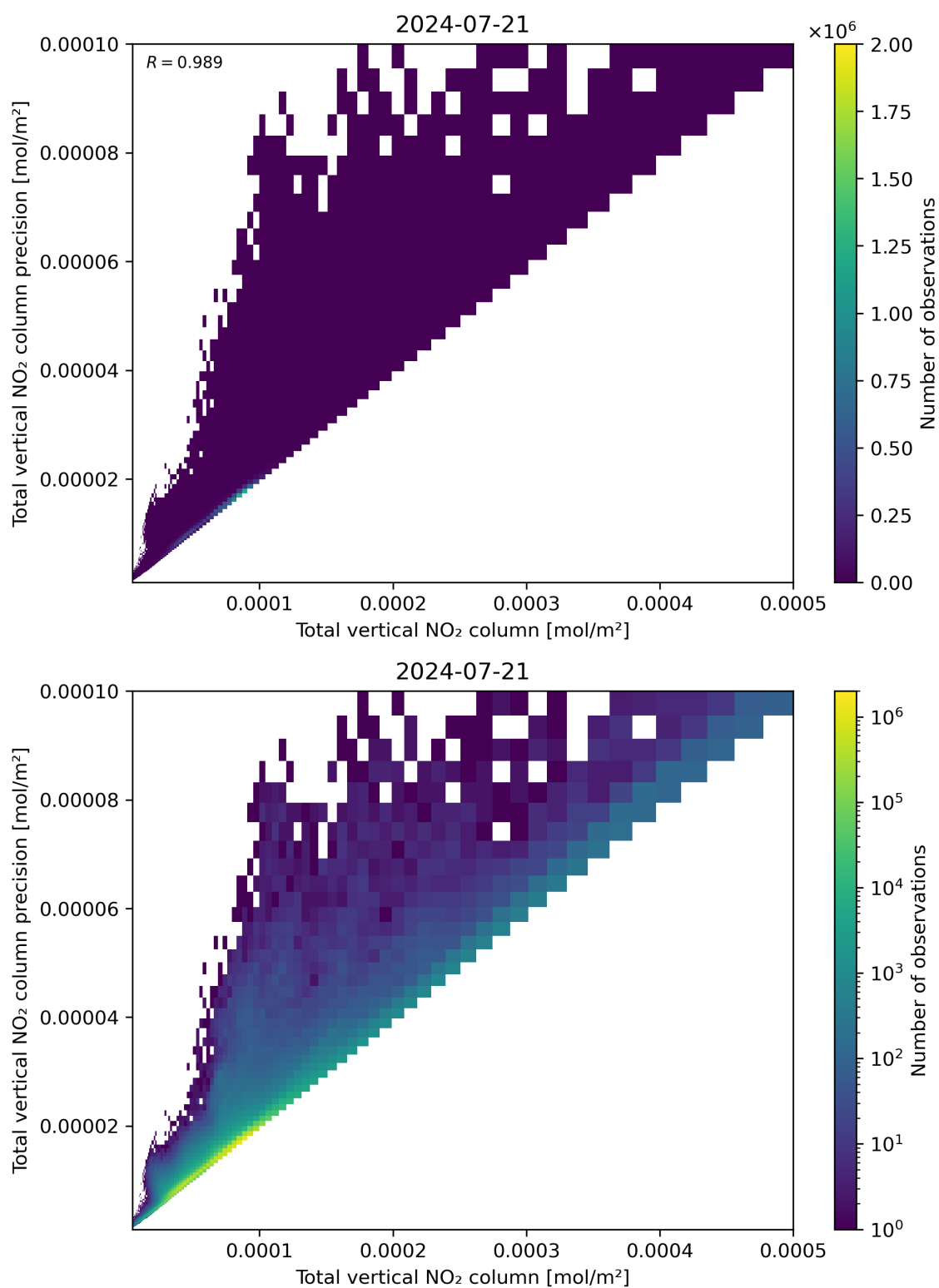
Figure 114: Scatter density plot of “Total vertical NO 2 column” against “Total vertical NO 2 column precision” for 2024-07-21 to 2024-07-22.
