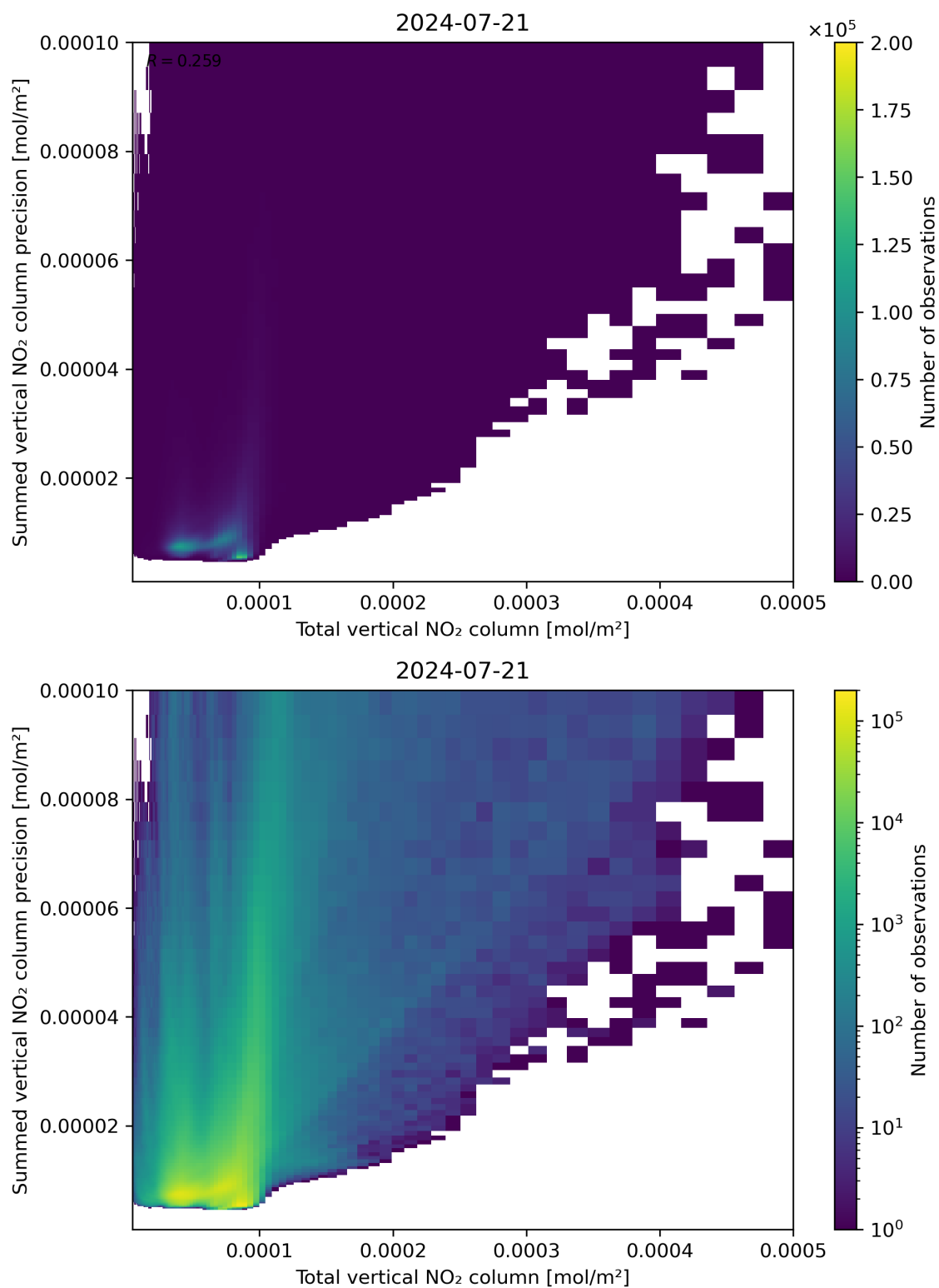
Figure 113: Scatter density plot of “Total vertical NO 2 column” against “Summed vertical NO 2 column precision” for 2024-07-21 to 2024-07-22.
