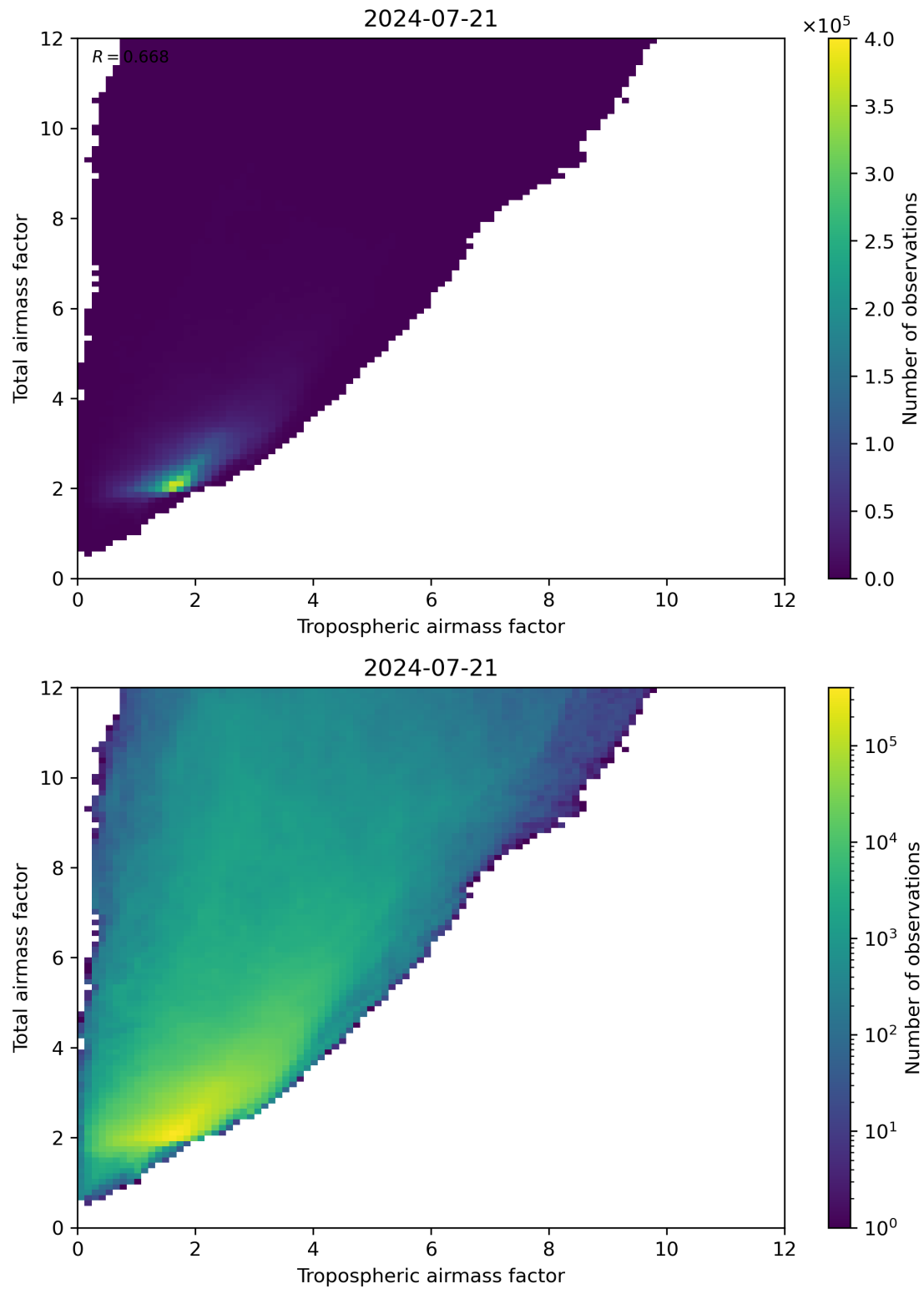
Figure 72: Scatter density plot of “Tropospheric airmass factor” against “Total airmass factor” for 2024-07-21 to 2024-07-22.
