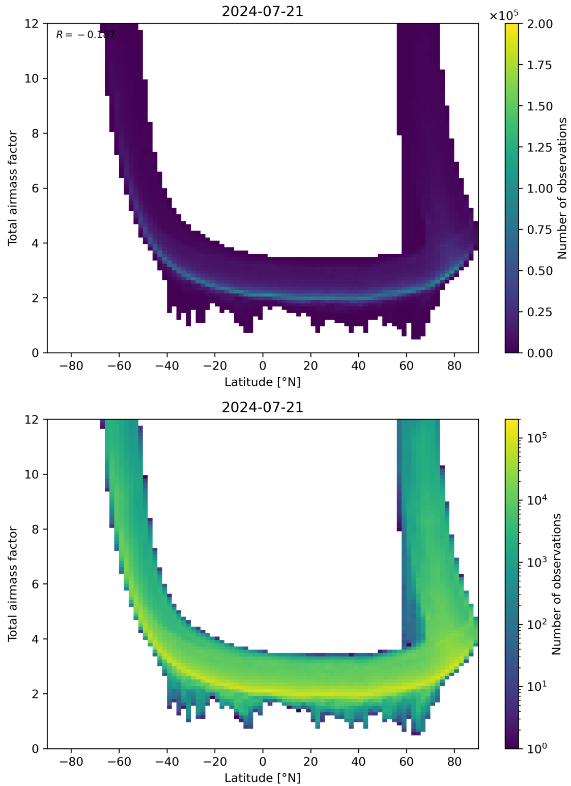
Figure 84: Scatter density plot of “Latitude” against “Total airmass factor” for 2024-07-21 to 2024-07-22.
