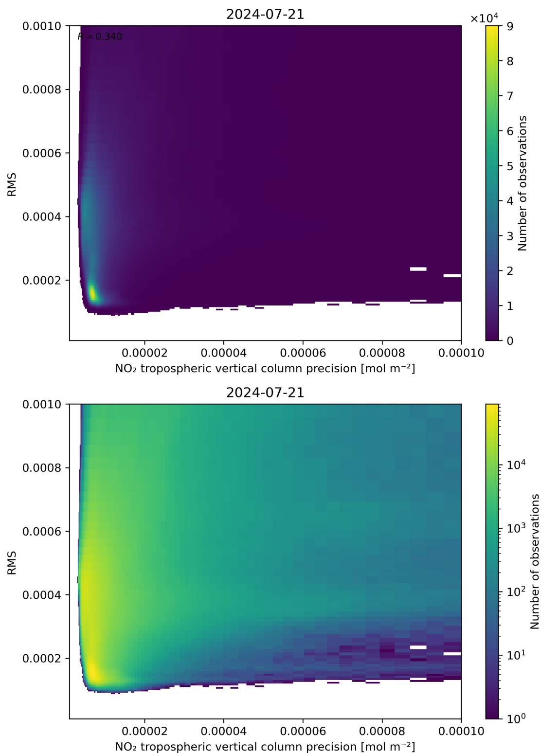
Figure 140: Scatter density plot of “NO 2 tropospheric vertical column precision” against “RMS” for 2024-07-21 to 2024-07-22.
