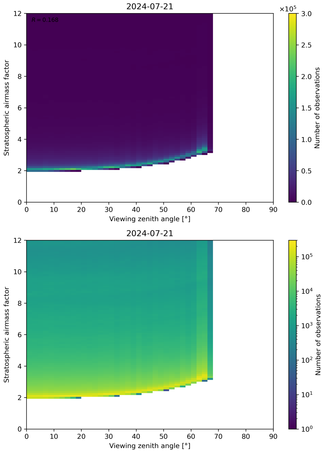
Figure 159: Scatter density plot of “Viewing zenith angle” against “Stratospheric airmass factor” for 2024-07-21 to 2024-07-22.
