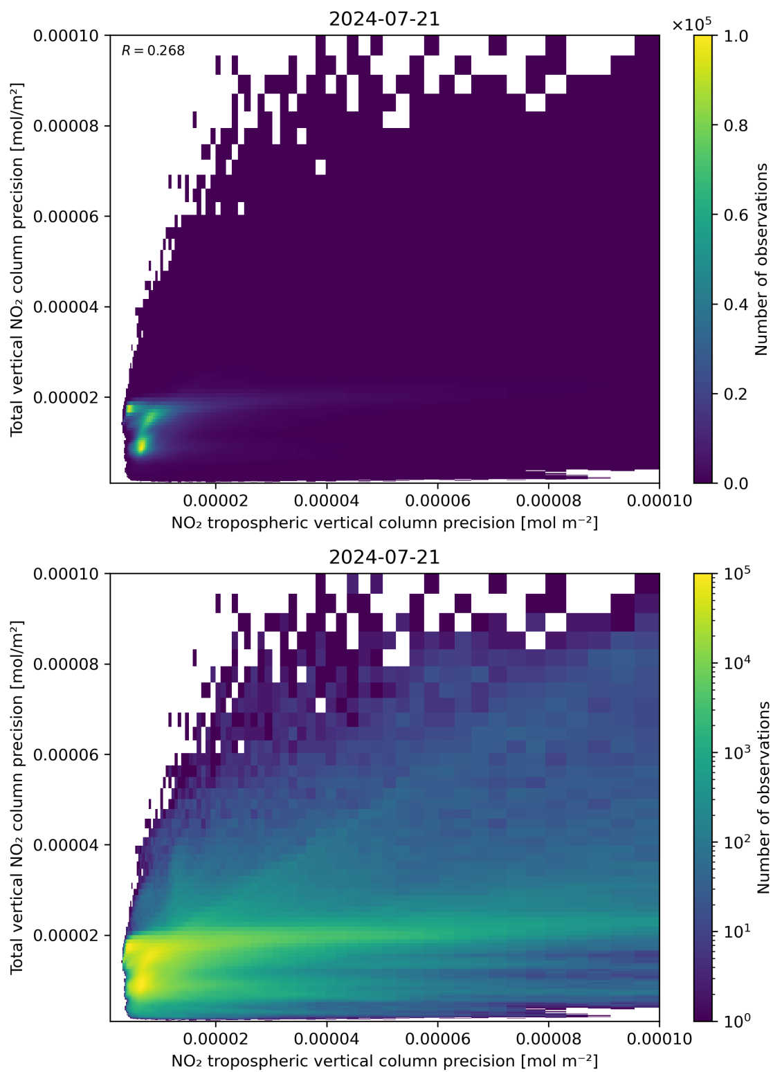
Figure 139: Scatter density plot of “NO 2 tropospheric vertical column precision” against “Total vertical NO 2 column precision” for 2024-07-21 to 2024-07-22.
