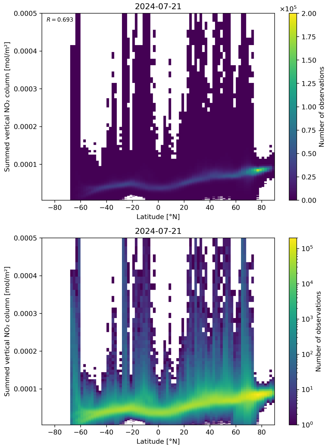
Figure 88: Scatter density plot of “Latitude” against “Summed vertical NO 2 column” for 2024-07-21 to 2024-07-22.
