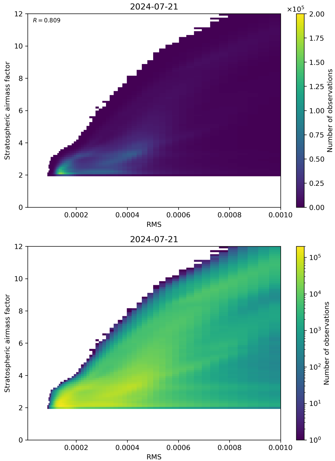
Figure 144: Scatter density plot of “RMS” against “Stratospheric airmass factor” for 2024-07-21 to 2024-07-22.
