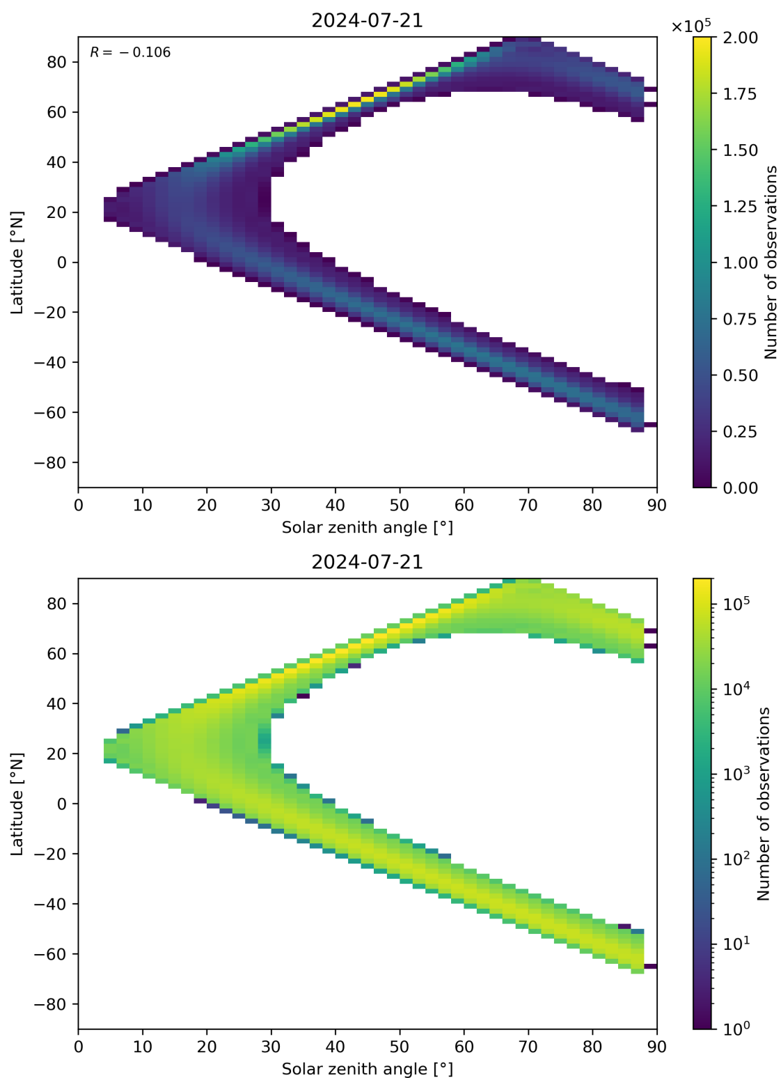
Figure 149: Scatter density plot of “Solar zenith angle” against “Latitude” for 2024-07-21 to 2024-07-22.
