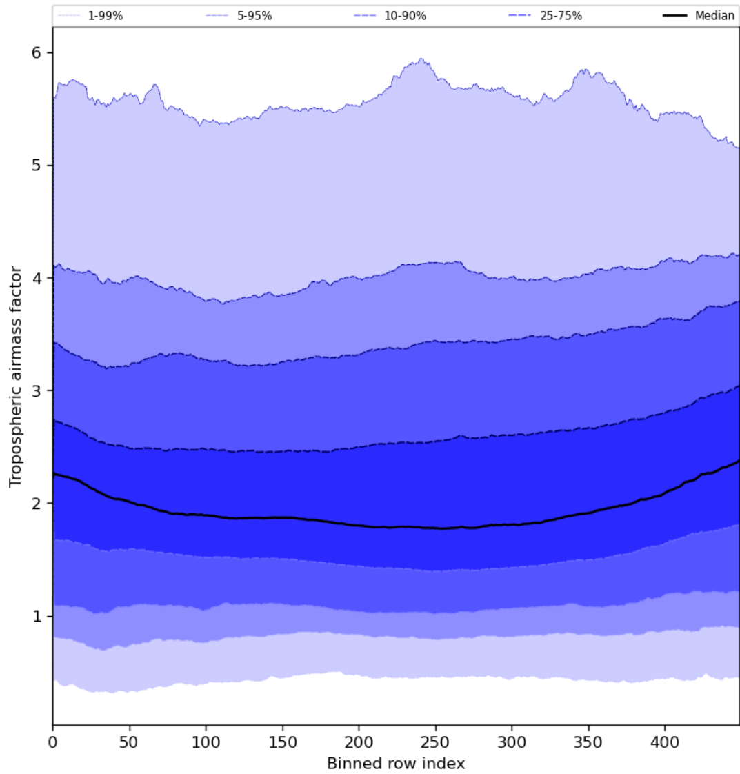
Figure 48: Along track statistics of “Tropospheric airmass factor” for 2024-07-21 to 2024-07-22
