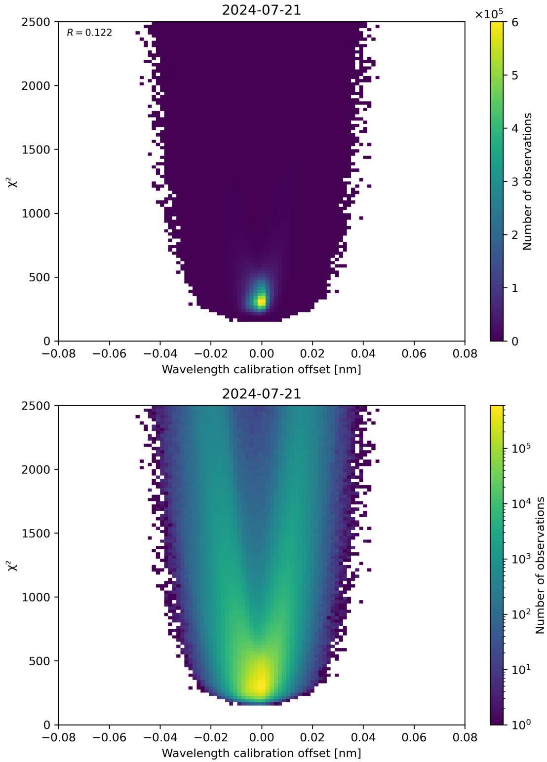
Figure 175: Scatter density plot of “Wavelength calibration offset” against “ \chi^2 ” for 2024-07-21 to 2024-07-22.
