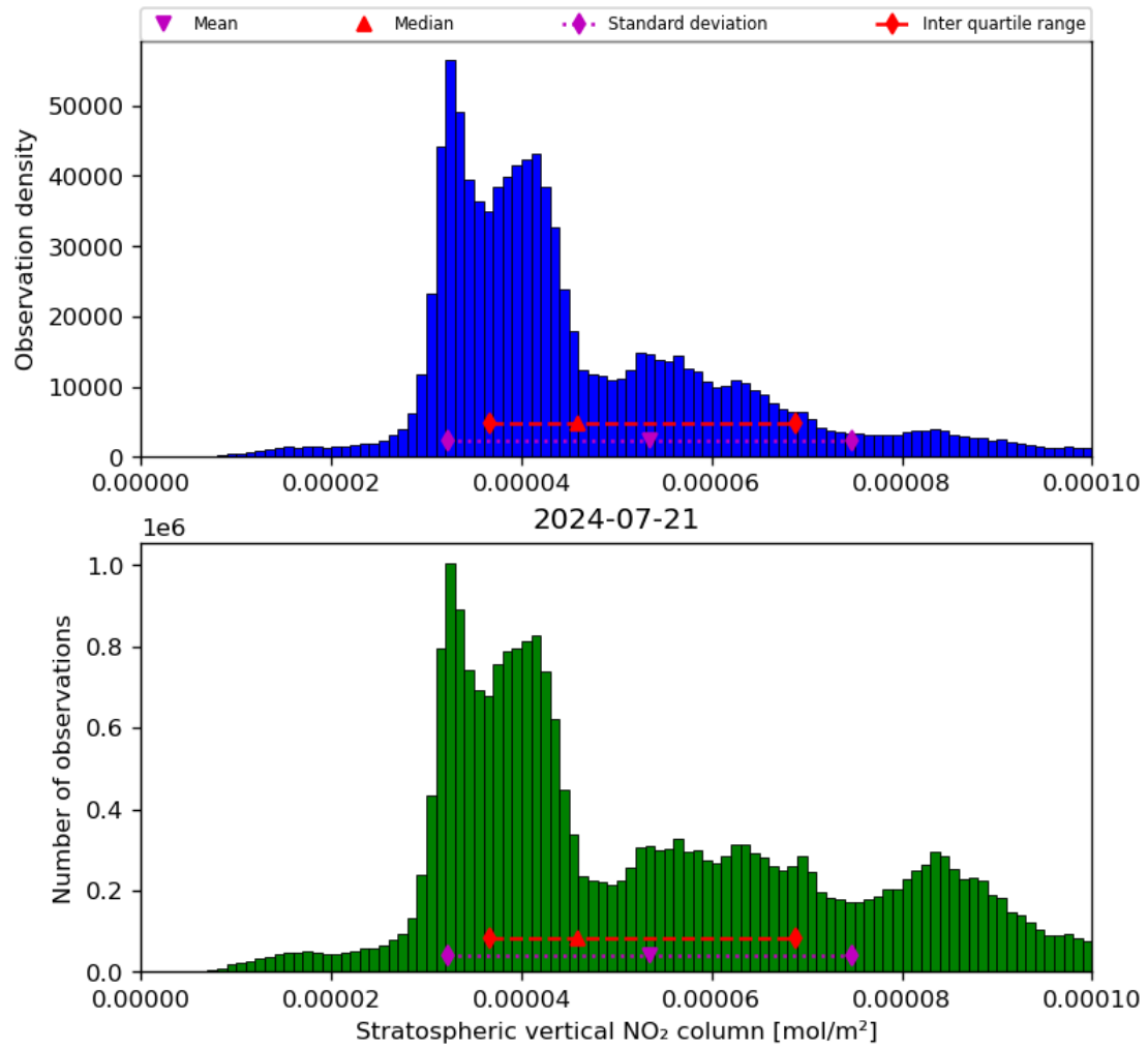
Figure 36: Histogram of “Stratospheric vertical NO 2 column” for 2024-07-21 to 2024-07-22
