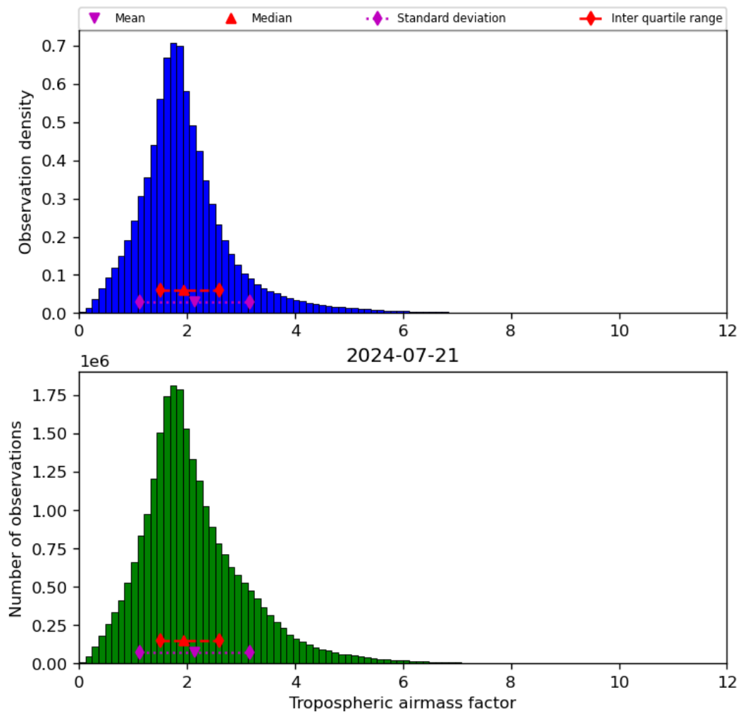
Figure 31: Histogram of “Tropospheric airmass factor” for 2024-07-21 to 2024-07-22
