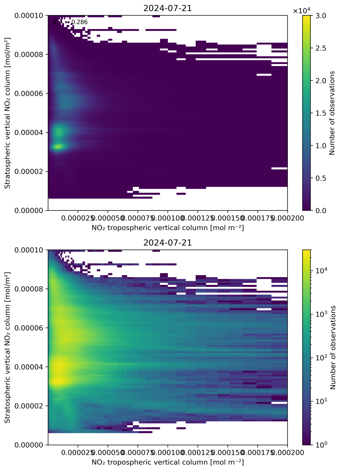
Figure 125: Scatter density plot of “NO 2 tropospheric vertical column” against “Stratospheric vertical NO 2 column” for 2024-07-21 to 2024-07-22.
