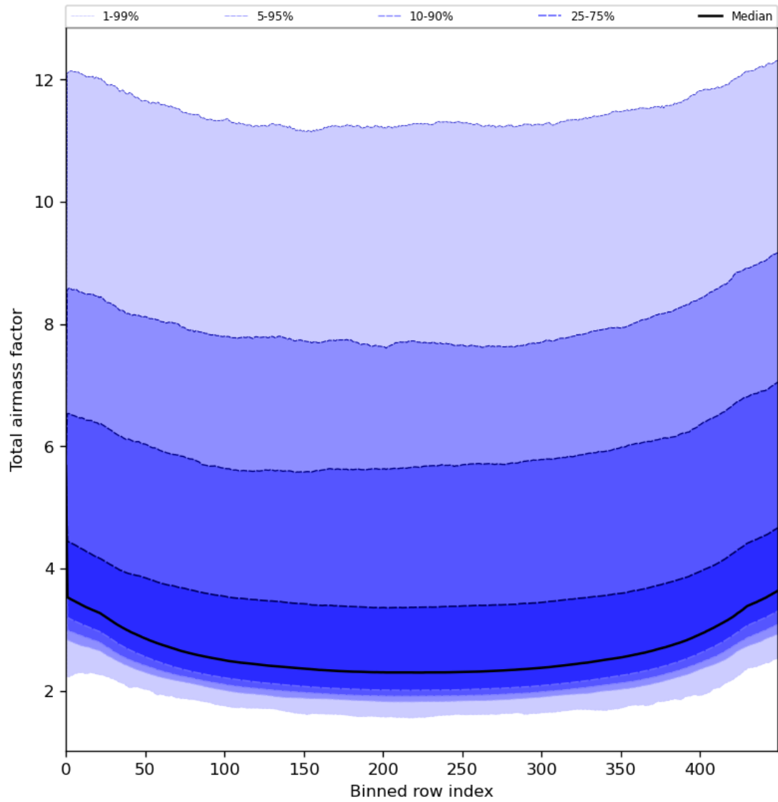
Figure 49: Along track statistics of “Total airmass factor” for 2024-07-21 to 2024-07-22
