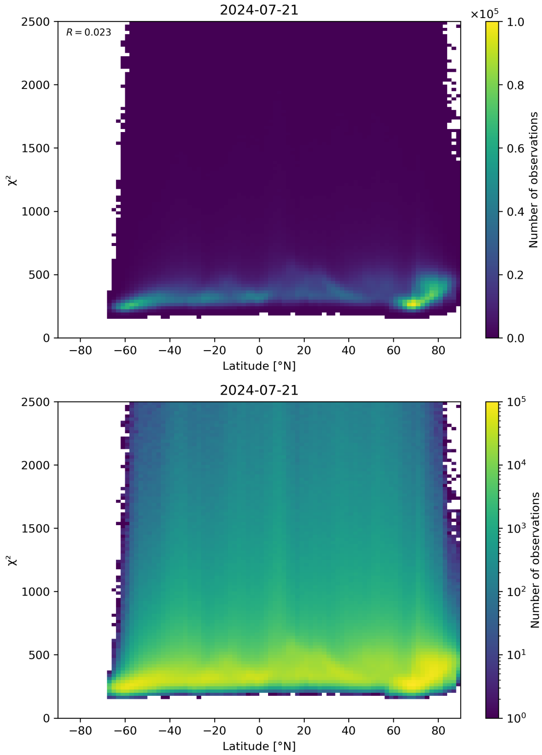
Figure 86: Scatter density plot of “Latitude” against “ \chi^2 ” for 2024-07-21 to 2024-07-22.
