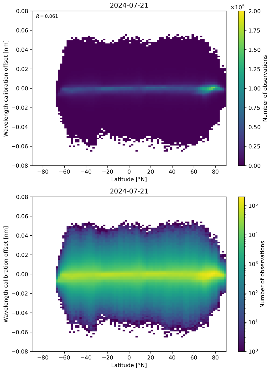
Figure 95: Scatter density plot of “Latitude” against “Wavelength calibration offset” for 2024-07-21 to 2024-07-22.
