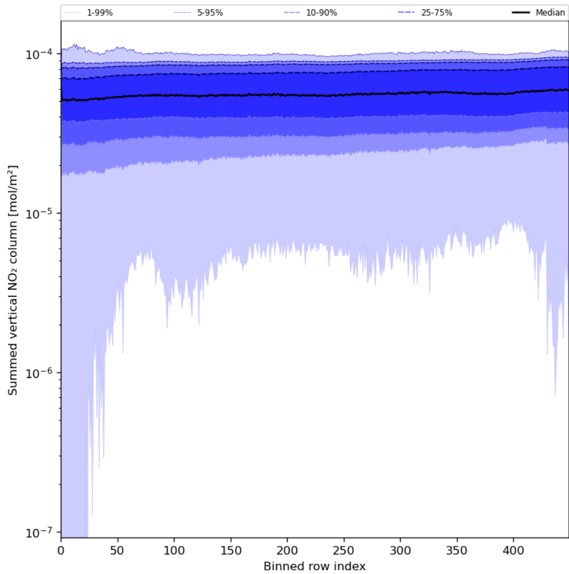
Figure 57: Along track statistics of “Summed vertical NO 2 column” for 2024-07-21 to 2024-07-22
