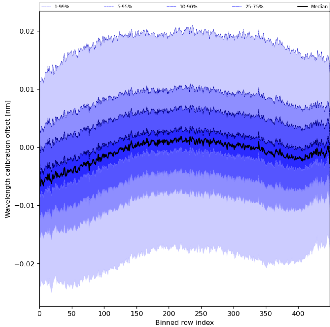
Figure 52: Along track statistics of “Wavelength calibration offset” for 2024-07-21 to 2024-07-22
