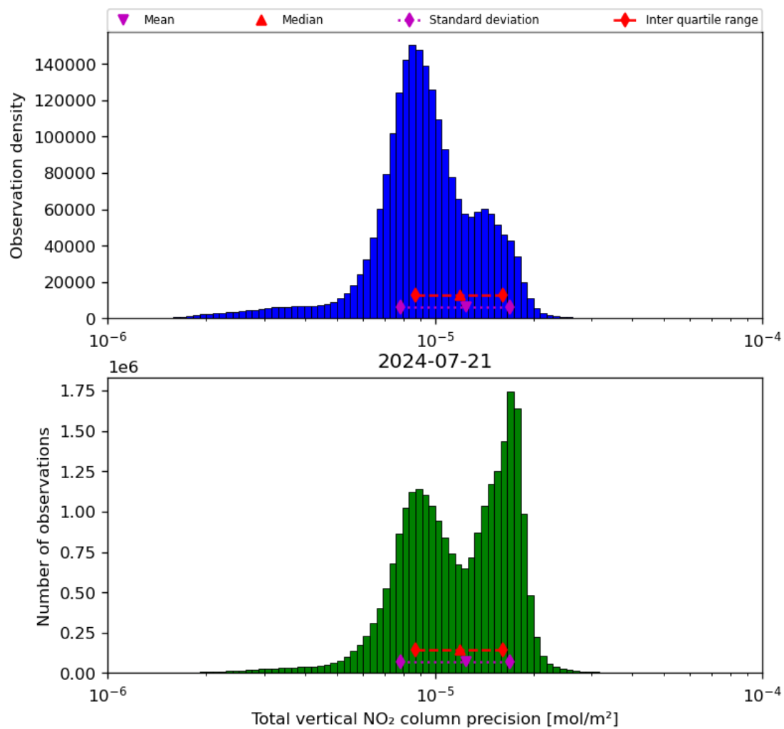
Figure 39: Histogram of “Total vertical NO 2 column precision” for 2024-07-21 to 2024-07-22
