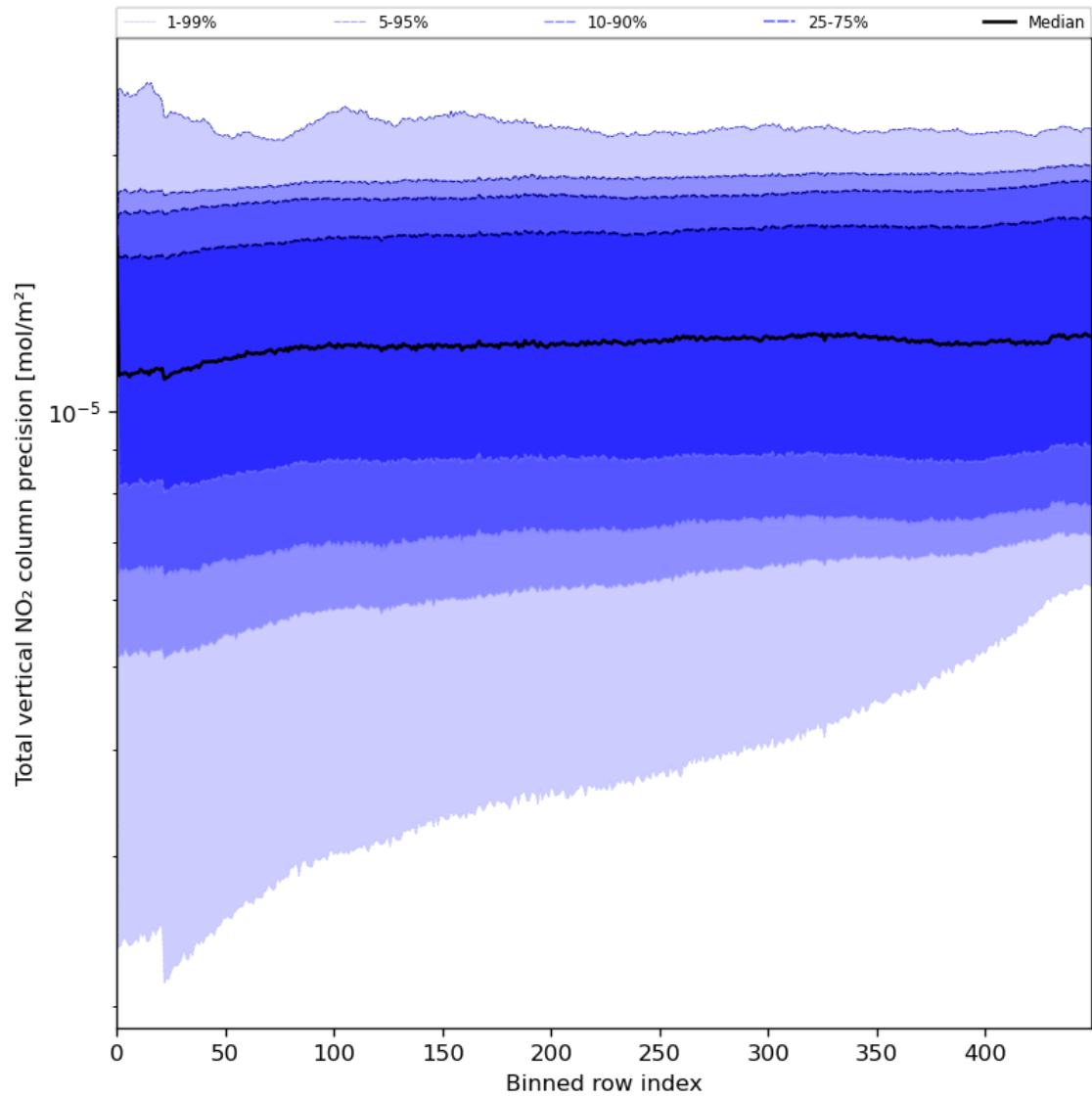
Figure 56: Along track statistics of “Total vertical NO 2 column precision” for 2024-07-21 to 2024-07-22
