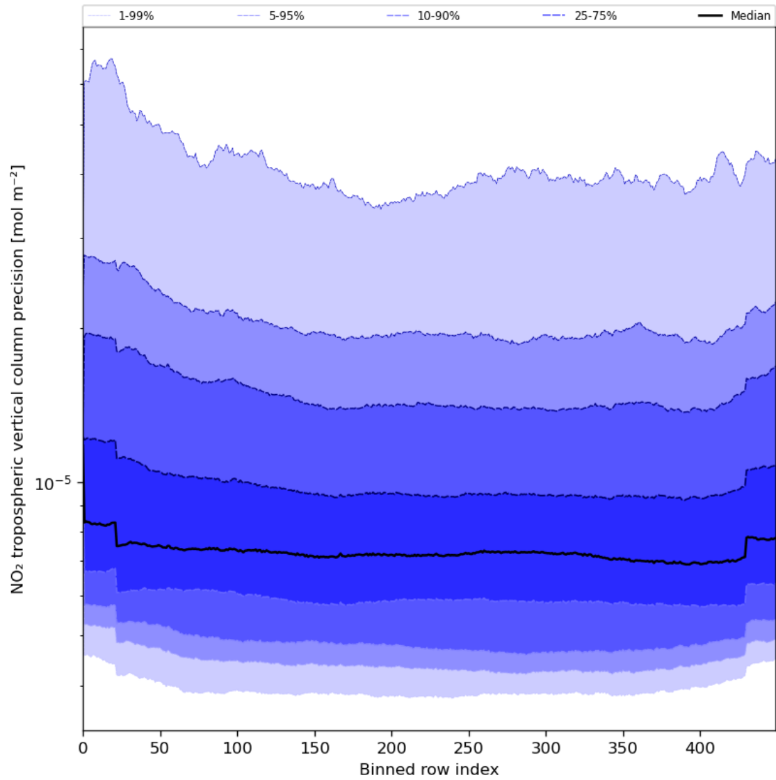
Figure 47: Along track statistics of “NO 2 tropospheric vertical column precision” for 2024-07-21 to 2024-07-22
