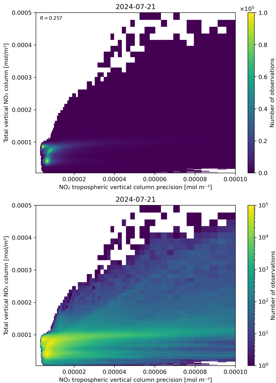
Figure 138: Scatter density plot of “NO 2 tropospheric vertical column precision” against “Total vertical NO 2 column” for 2024-07-21 to 2024-07-22.
