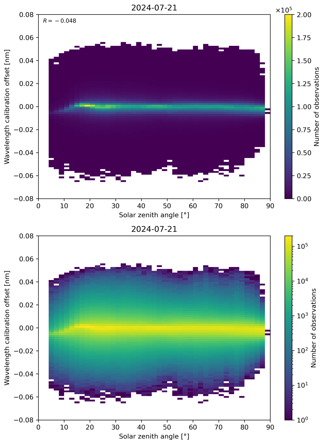
Figure 158: Scatter density plot of “Solar zenith angle” against “Wavelength calibration offset” for 2024-07-21 to 2024-07-22.
