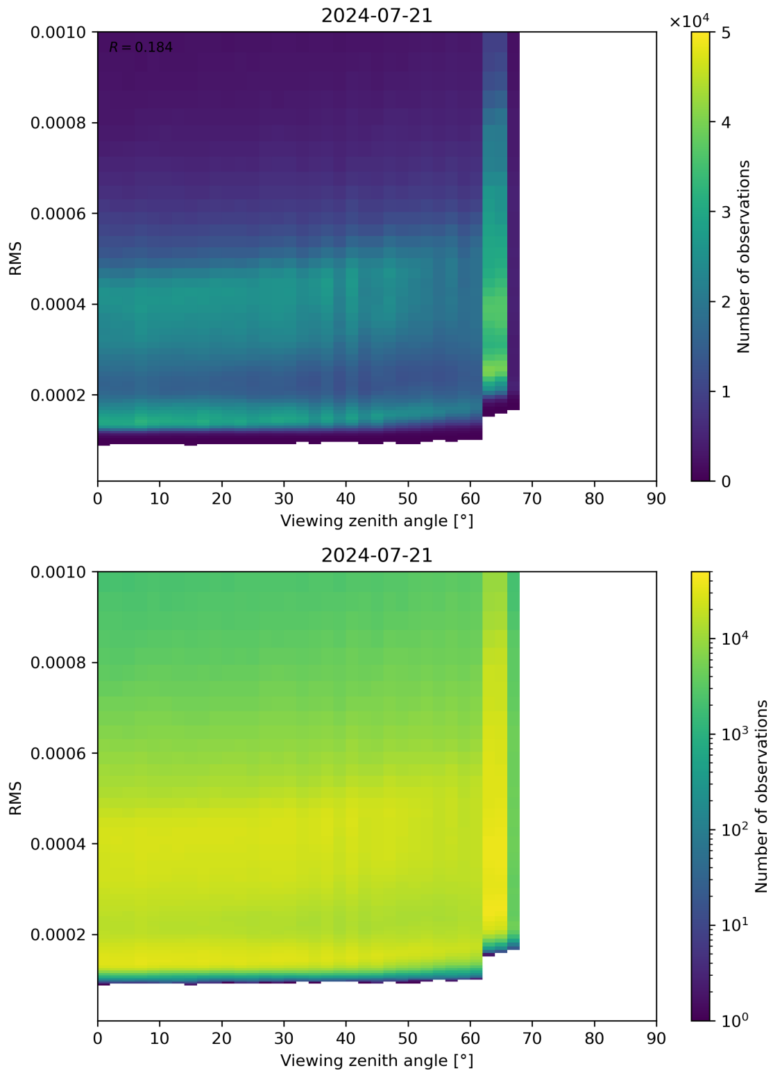
Figure 171: Scatter density plot of “Viewing zenith angle” against “RMS” for 2024-07-21 to 2024-07-22.
