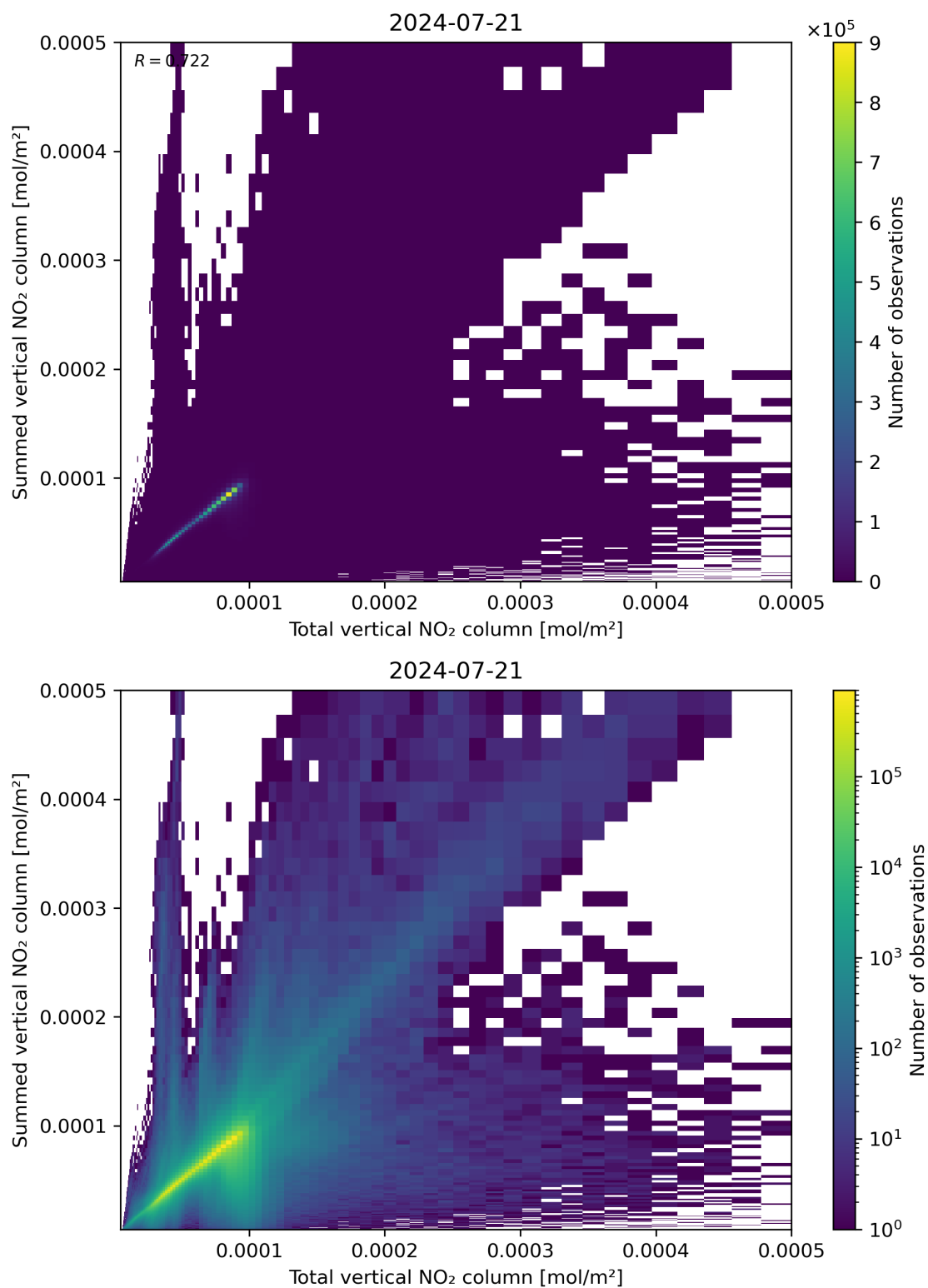
Figure 112: Scatter density plot of “Total vertical NO 2 column” against “Summed vertical NO 2 column” for 2024-07-21 to 2024-07-22.
