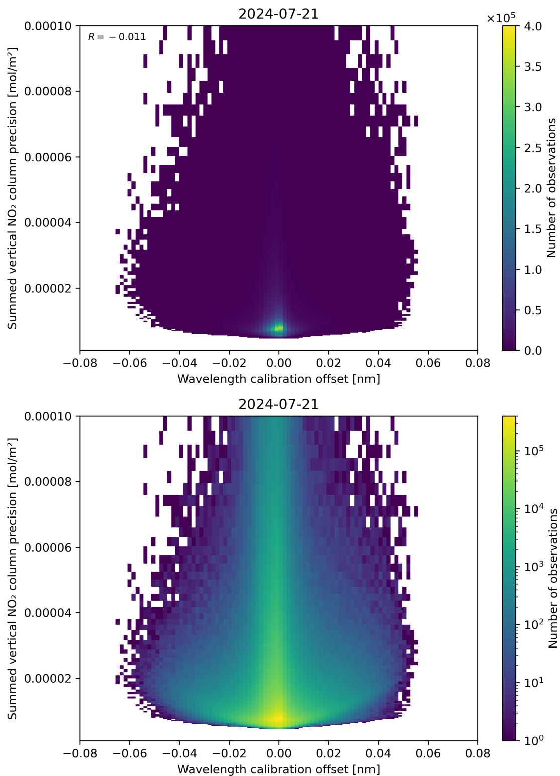
Figure 178: Scatter density plot of “Wavelength calibration offset” against “Summed vertical NO 2 column precision” for 2024-07-21 to 2024-07-22.
