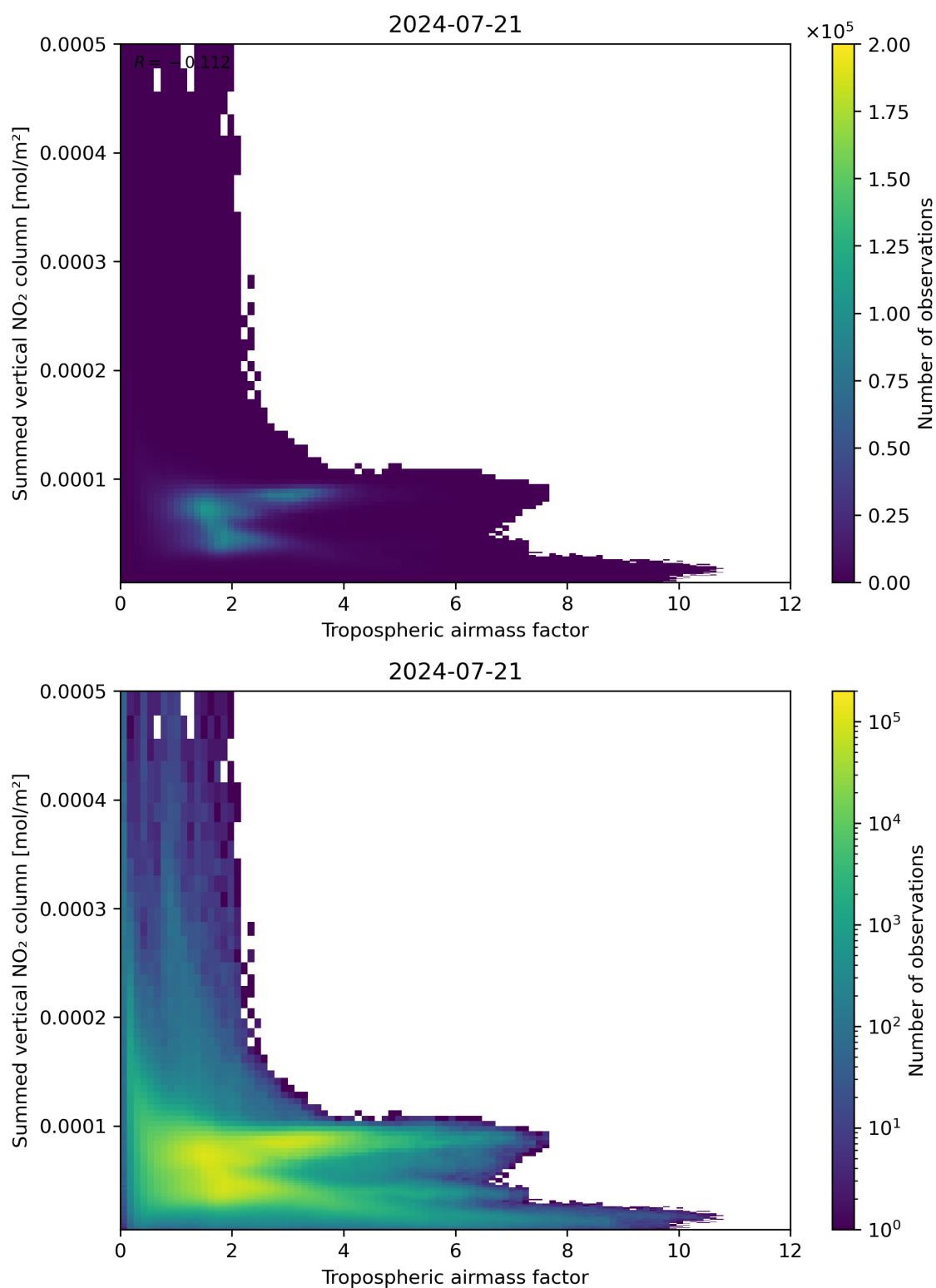
Figure 75: Scatter density plot of “Tropospheric airmass factor” against “Summed vertical NO 2 column” for 2024-07-21 to 2024-07-22.
