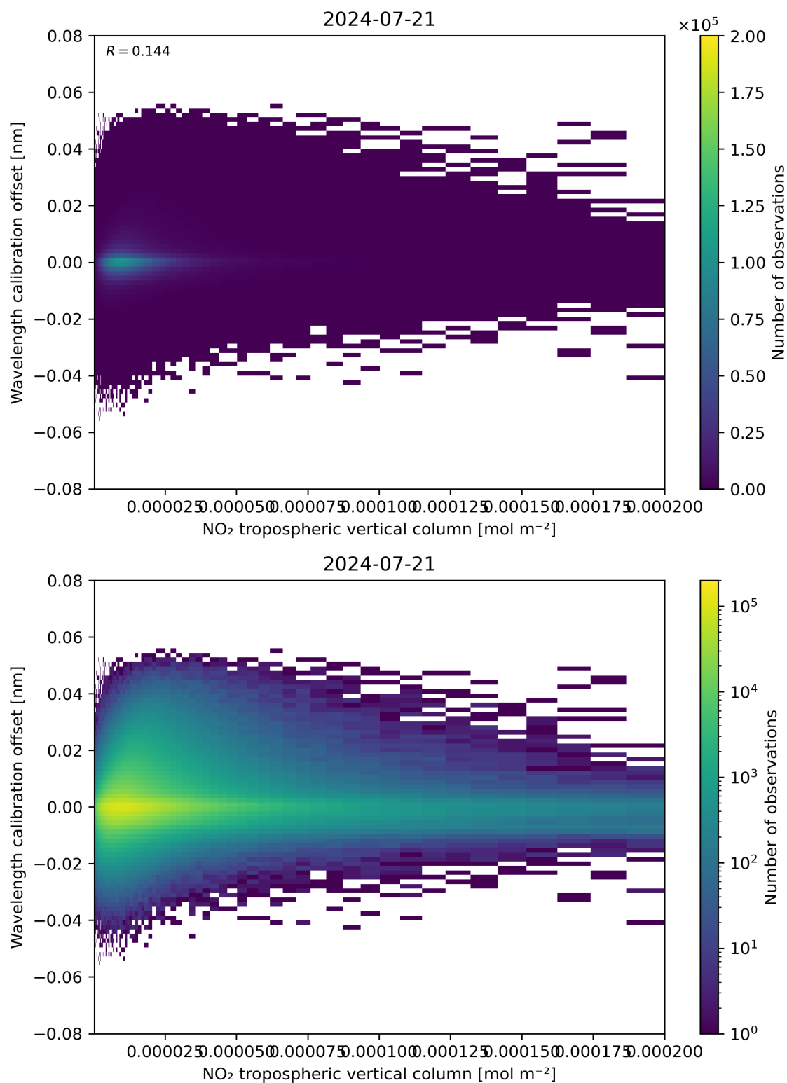
Figure 143: Scatter density plot of “NO 2 tropospheric vertical column” against “Wavelength calibration offset” for 2024-07-21 to 2024-07-22.
