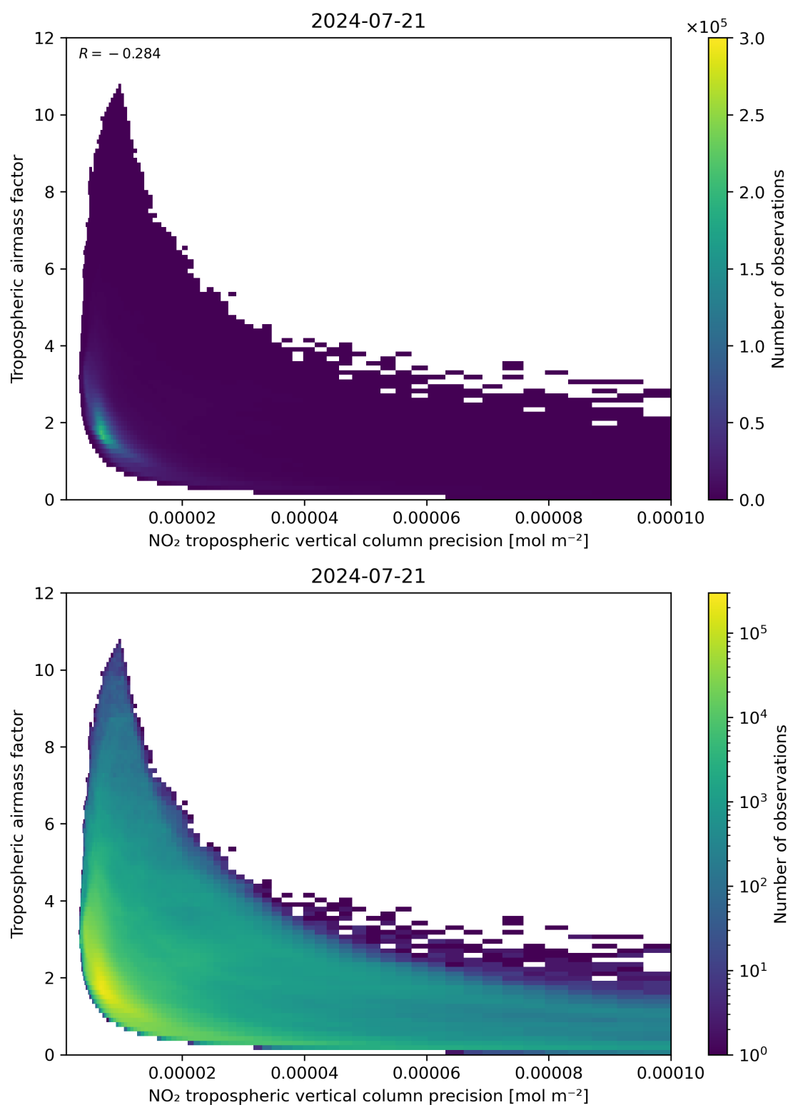
Figure 133: Scatter density plot of “NO 2 tropospheric vertical column precision” against “Tropospheric airmass factor” for 2024-07-21 to 2024-07-22.
