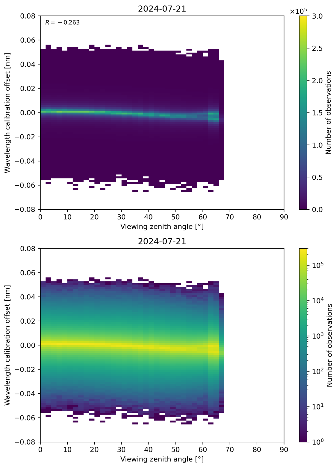
Figure 173: Scatter density plot of “Viewing zenith angle” against “Wavelength calibration offset” for 2024-07-21 to 2024-07-22.
