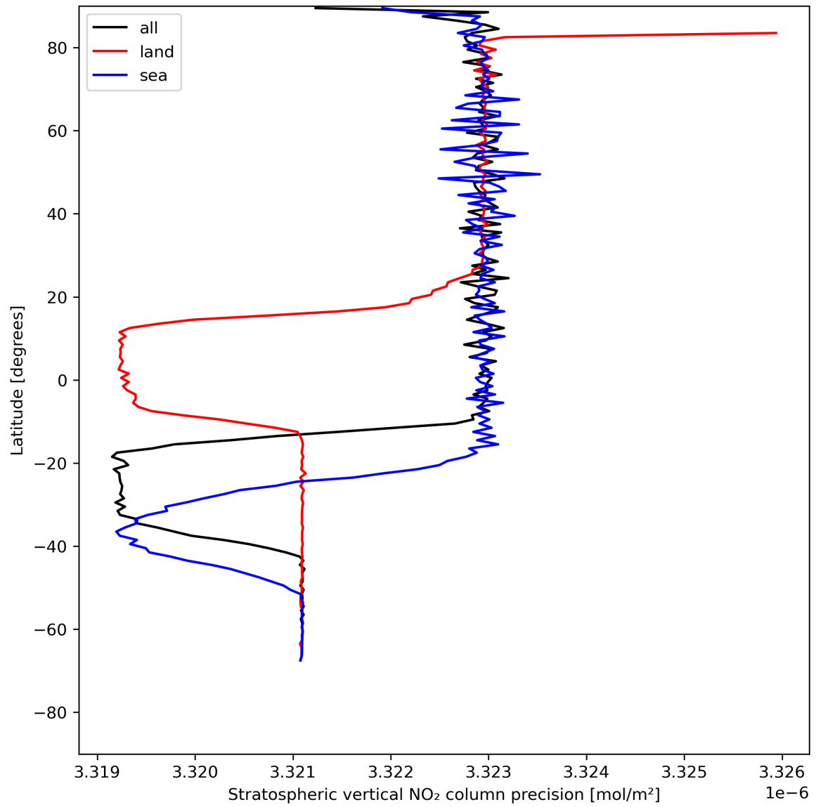
Figure 20: Zonal average of “Stratospheric vertical NO 2 column precision” for 2024-07-21 to 2024-07-22.
