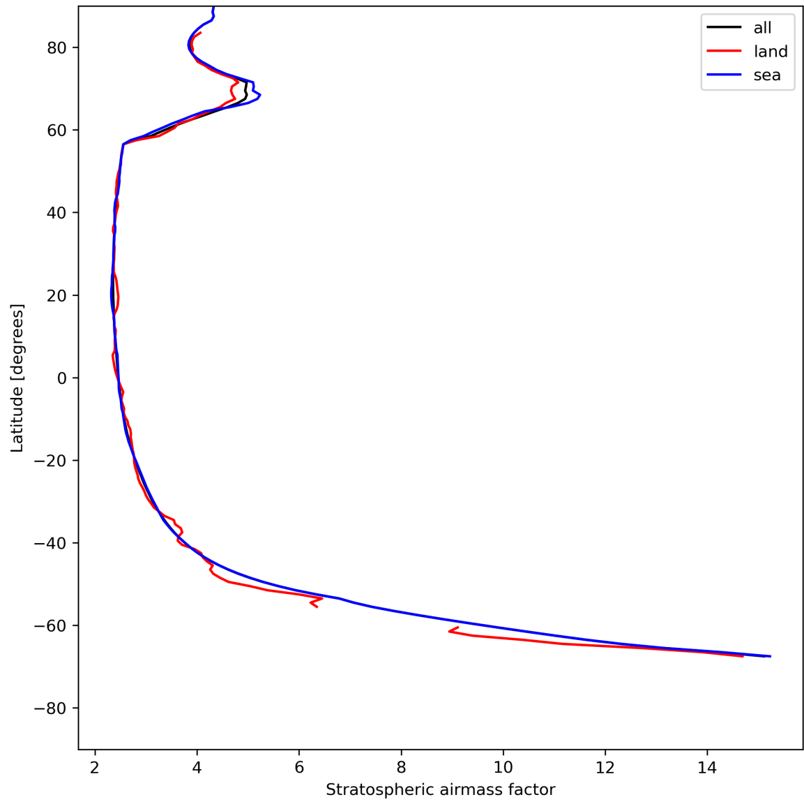
Figure 27: Zonal average of “Stratospheric airmass factor” for 2024-07-21 to 2024-07-22.
