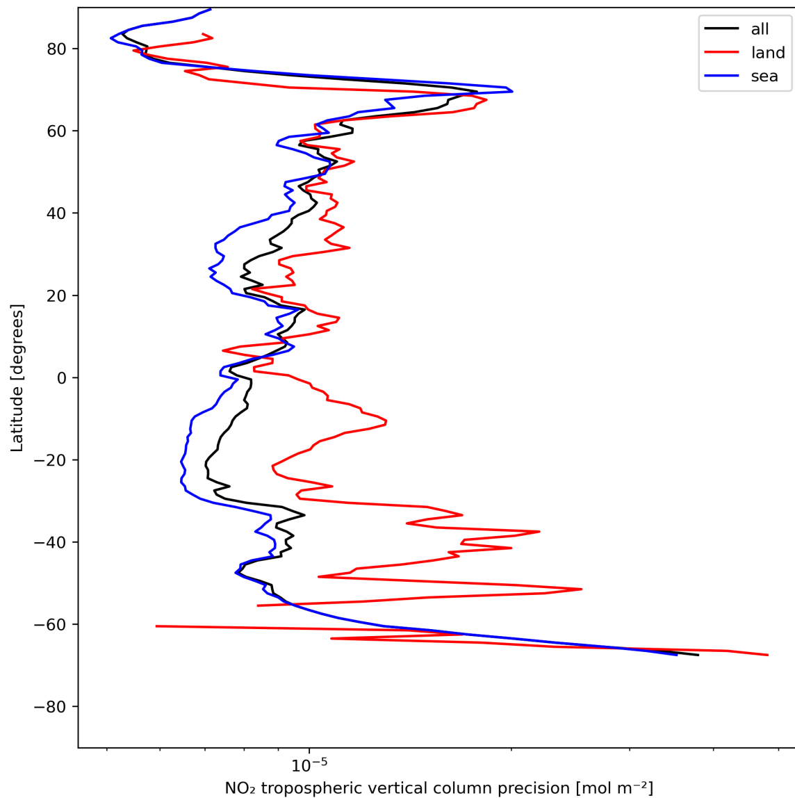
Figure 13: Zonal average of “NO 2 tropospheric vertical column precision” for 2024-07-21 to 2024-07-22.
