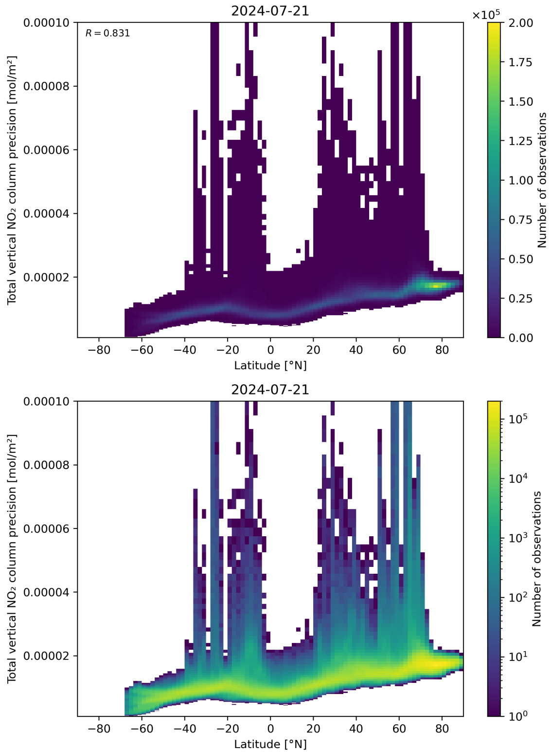
Figure 91: Scatter density plot of “Latitude” against “Total vertical NO 2 column precision” for 2024-07-21 to 2024-07-22.
