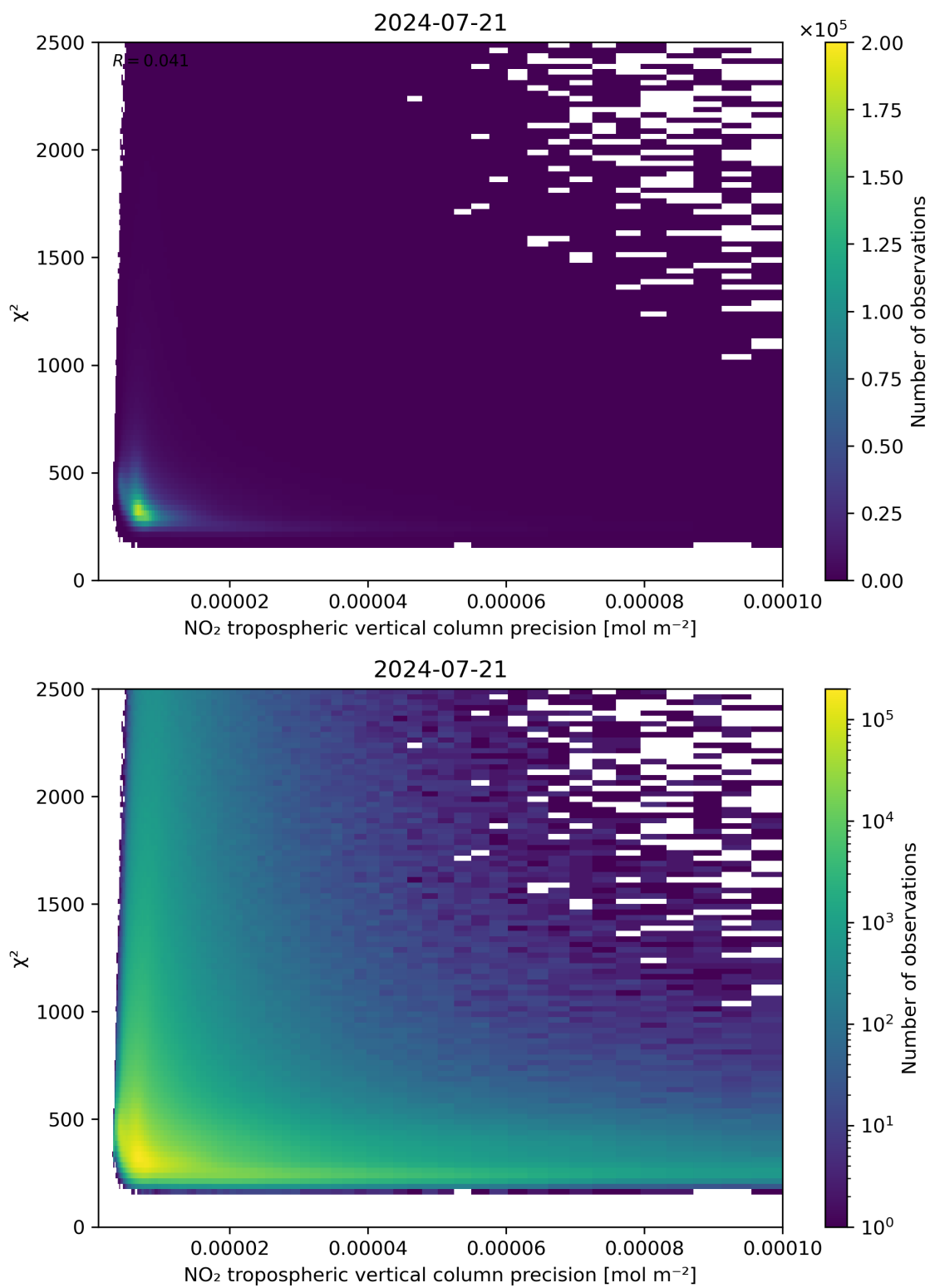
Figure 134: Scatter density plot of “NO 2 tropospheric vertical column precision” against “ \chi^2 ” for 2024-07-21 to 2024-07-22.
