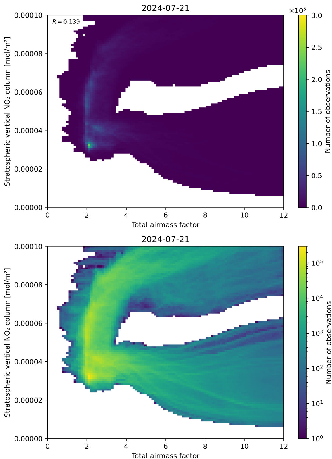
Figure 64: Scatter density plot of “Total airmass factor” against “Stratospheric vertical \text{NO}_2 column” for 2024-07-21 to 2024-07-22.
