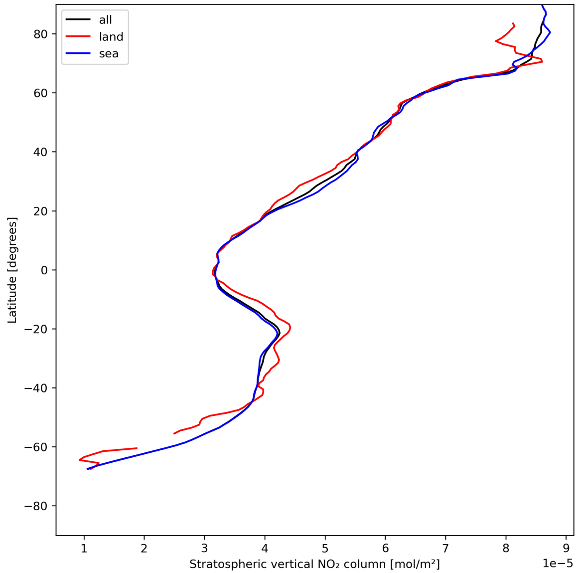
Figure 19: Zonal average of “Stratospheric vertical NO 2 column” for 2024-07-21 to 2024-07-22.
