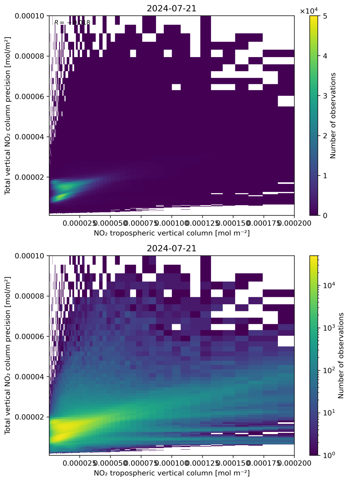
Figure 129: Scatter density plot of “NO 2 tropospheric vertical column” against “Total vertical NO 2 column precision” for 2024-07-21 to 2024-07-22.
