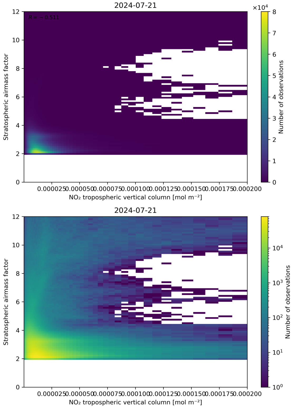
Figure 121: Scatter density plot of “NO 2 tropospheric vertical column” against “Stratospheric air mass factor” for 2024-07-21 to 2024-07-22.
