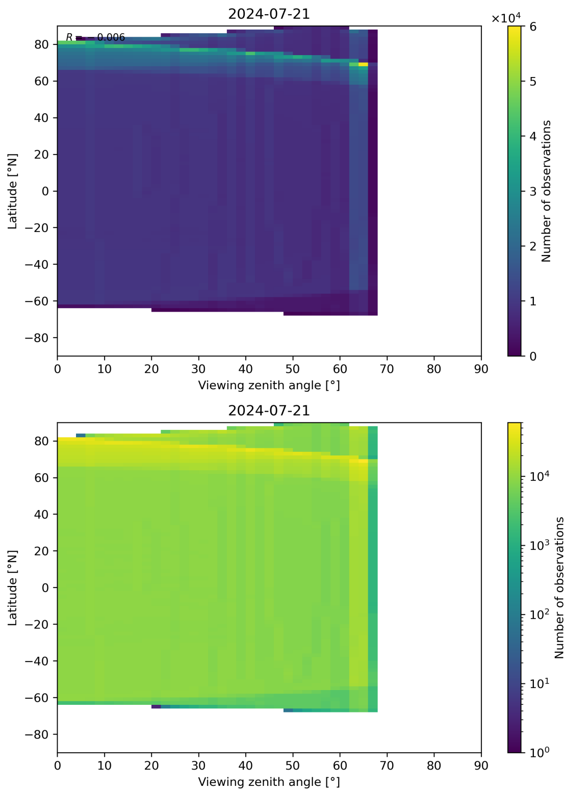
Figure 163: Scatter density plot of “Viewing zenith angle” against “Latitude” for 2024-07-21 to 2024-07-22.
