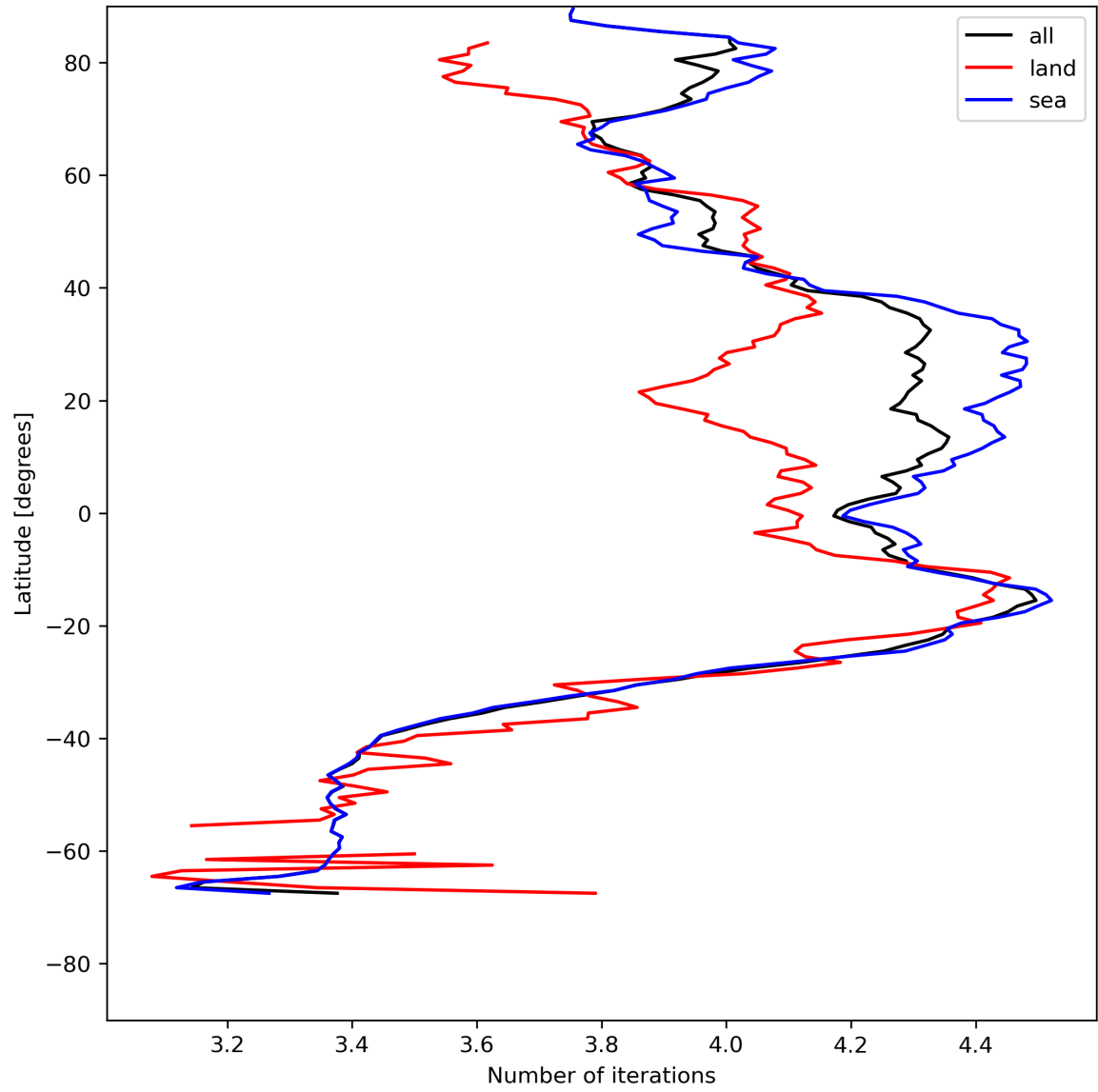
Figure 17: Zonal average of “Number of iterations” for 2024-07-21 to 2024-07-22.
