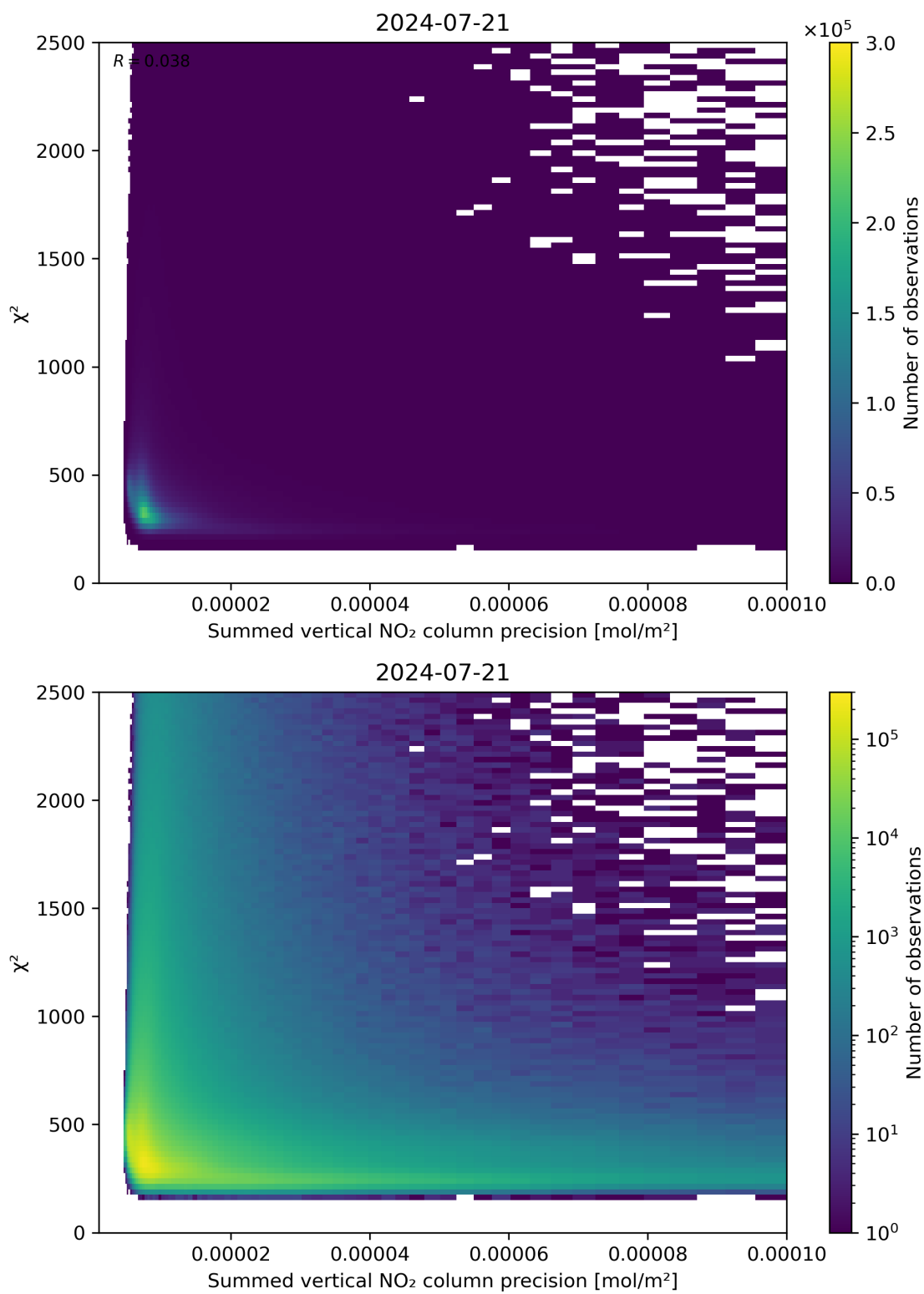
Figure 107: Scatter density plot of “Summed vertical NO 2 column precision” against “ \chi^2 ” for 2024-07-21 to 2024-07-22.
