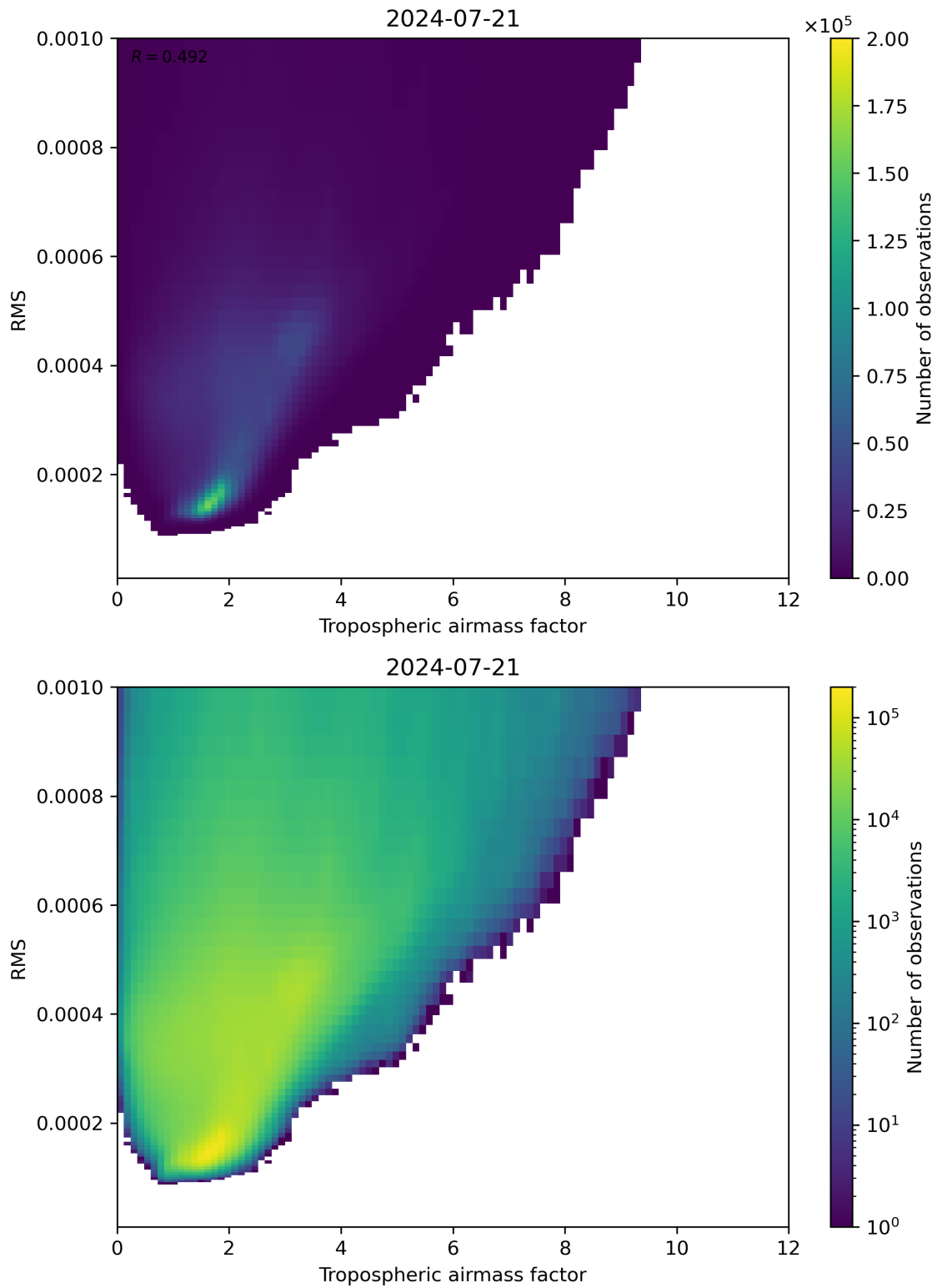
Figure 79: Scatter density plot of “Tropospheric airmass factor” against “RMS” for 2024-07-21 to 2024-07-22.
