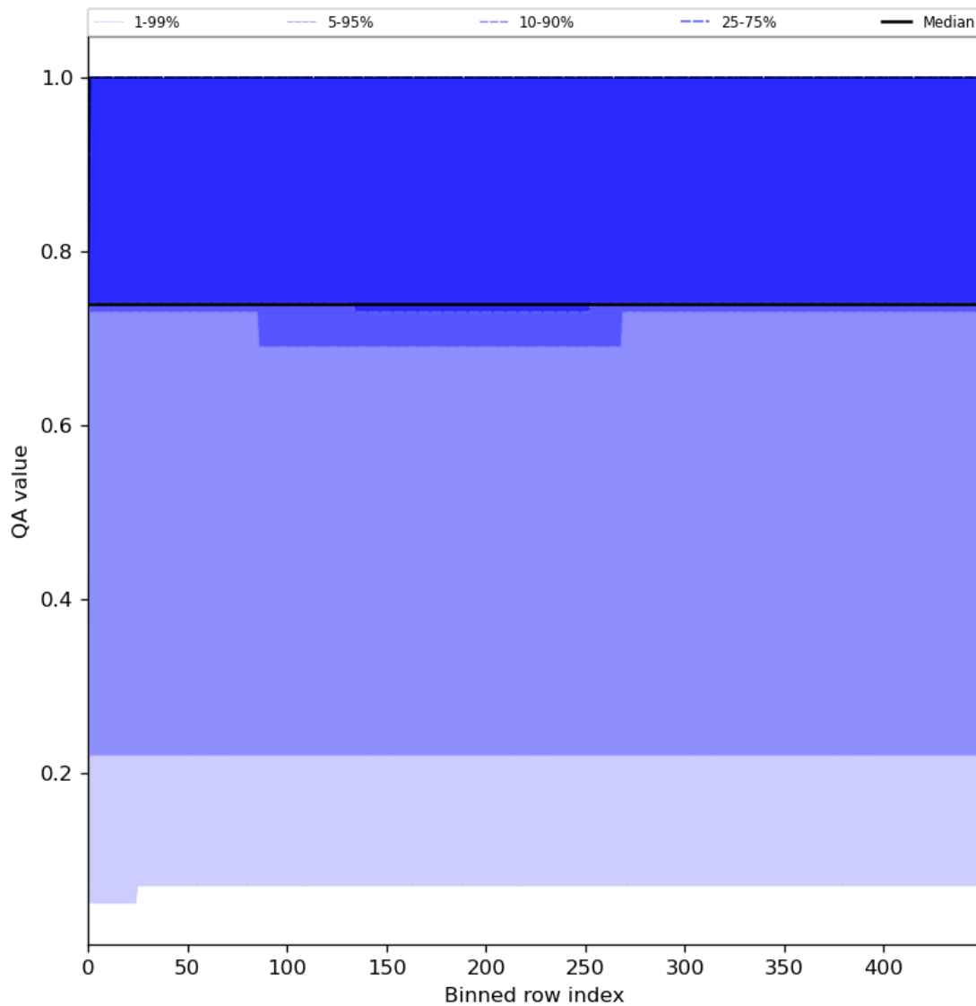
Figure 45: Along track statistics of “QA value” for 2024-07-21 to 2024-07-22
