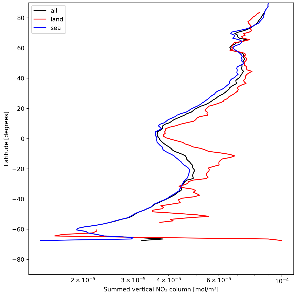
Figure 23: Zonal average of “Summed vertical NO 2 column” for 2024-07-21 to 2024-07-22.
