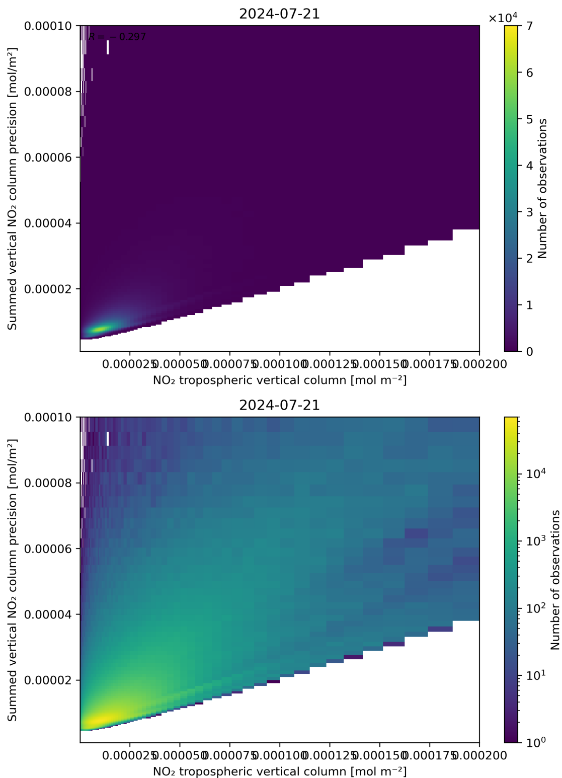
Figure 127: Scatter density plot of “NO 2 tropospheric vertical column” against “Summed vertical NO 2 column precision” for 2024-07-21 to 2024-07-22.
