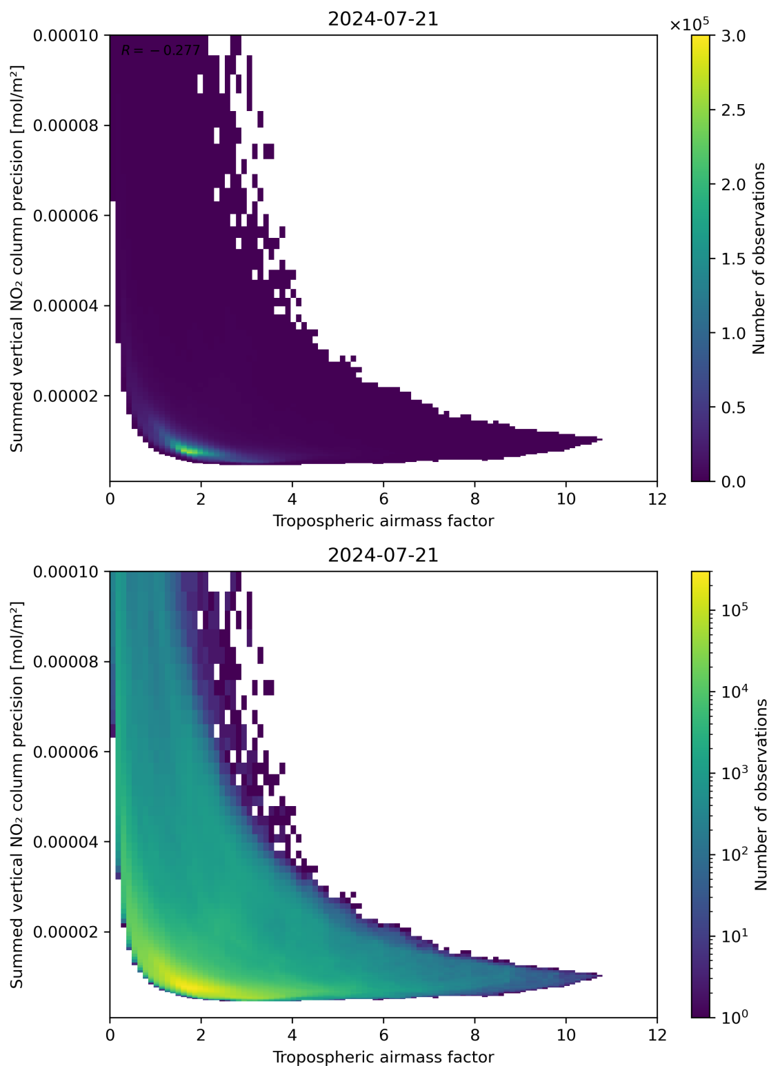
Figure 76: Scatter density plot of “Tropospheric air mass factor” against “Summed vertical NO 2 column precision” for 2024-07-21 to 2024-07-22.
