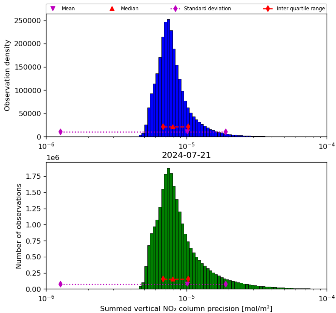
Figure 41: Histogram of “Summed vertical NO 2 column precision” for 2024-07-21 to 2024-07-22
