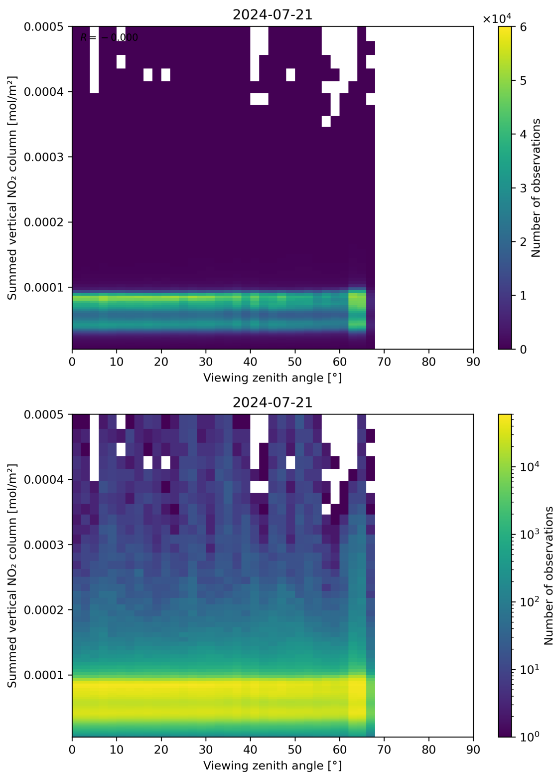
Figure 165: Scatter density plot of “Viewing zenith angle” against “Summed vertical NO 2 column” for 2024-07-21 to 2024-07-22.
