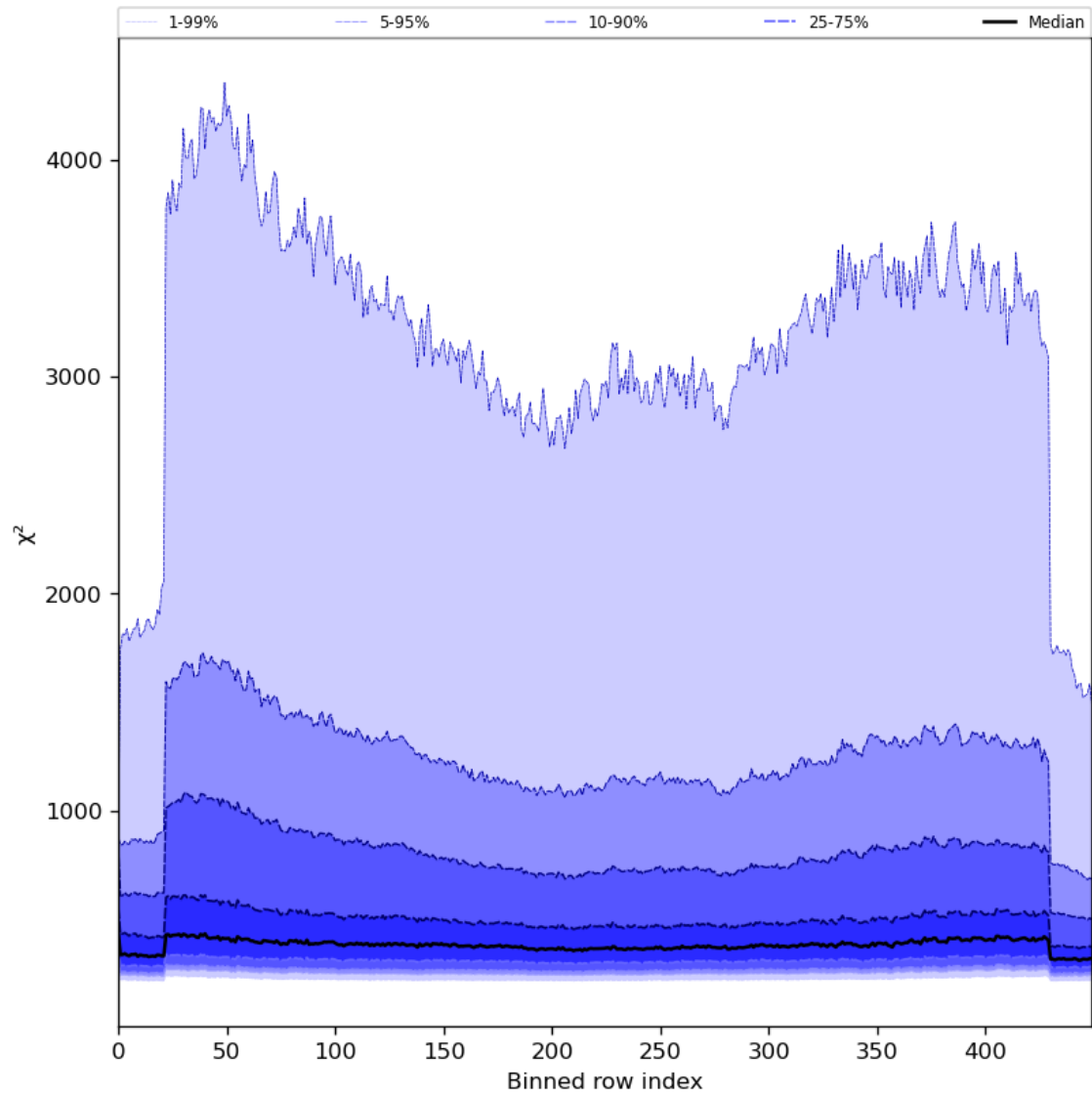
Figure 59: Along track statistics of “ \chi^2 ” for 2024-07-21 to 2024-07-22
