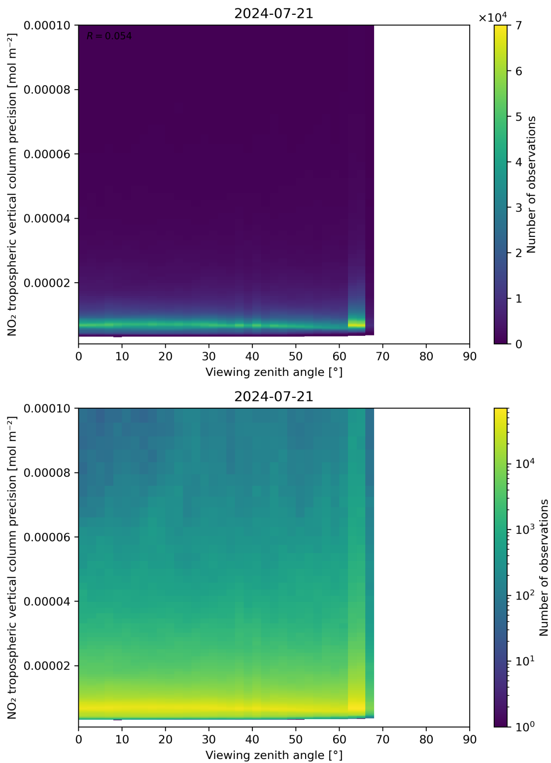
Figure 170: Scatter density plot of “Viewing zenith angle” against “NO 2 tropospheric vertical column precision” for 2024-07-21 to 2024-07-22.
