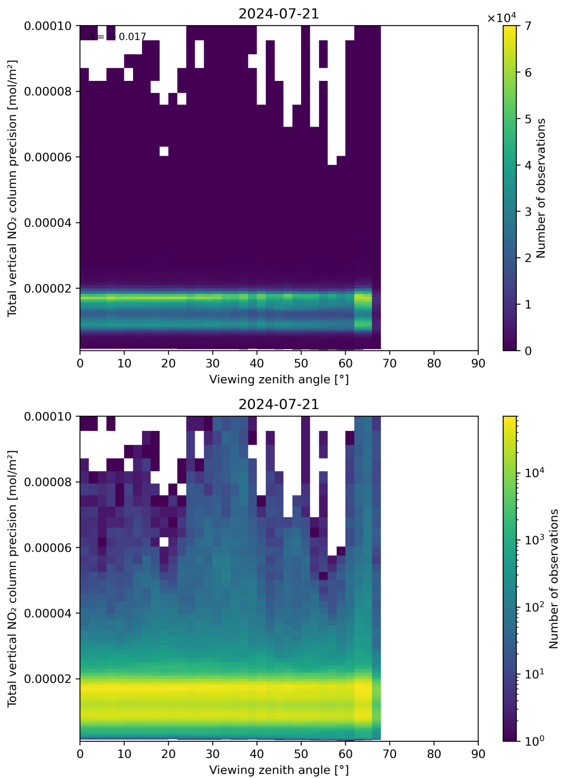
Figure 168: Scatter density plot of “Viewing zenith angle” against “Total vertical NO 2 column precision” for 2024-07-21 to 2024-07-22.
