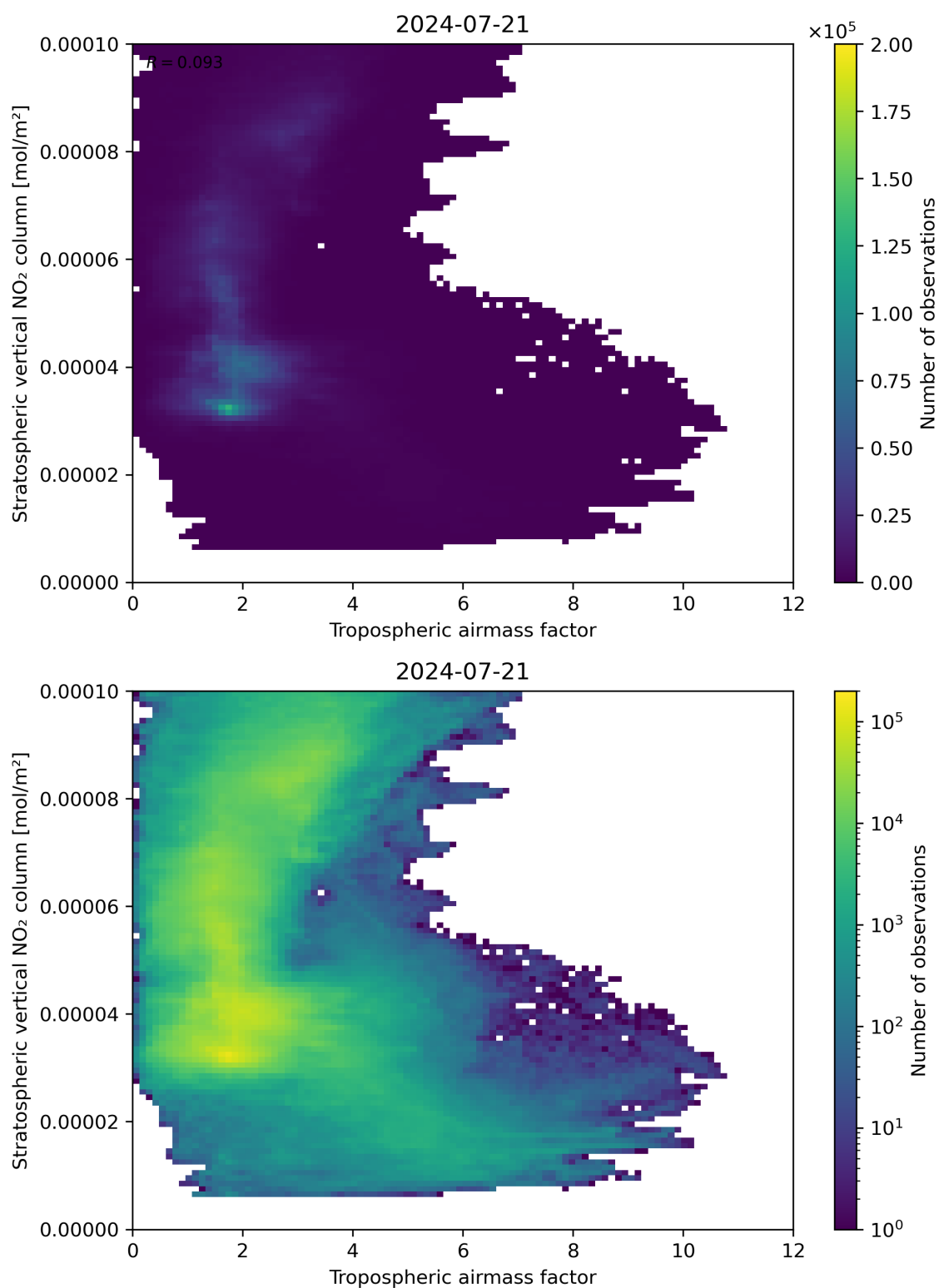
Figure 74: Scatter density plot of “Tropospheric air mass factor” against “Stratospheric vertical NO 2 column” for 2024-07-21 to 2024-07-22.
