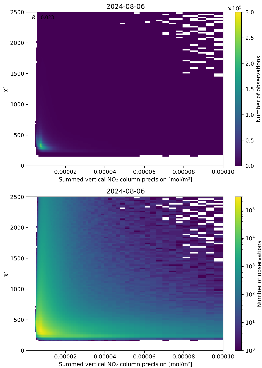
Figure 107: Scatter density plot of “Summed vertical NO 2 column precision” against “ \chi^2 ” for 2024-08-06 to 2024-08-07.
