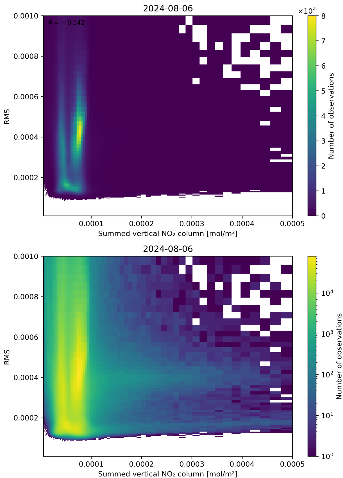
Figure 109: Scatter density plot of “Summed vertical NO 2 column” against “RMS” for 2024-08-06 to 2024-08-07.
