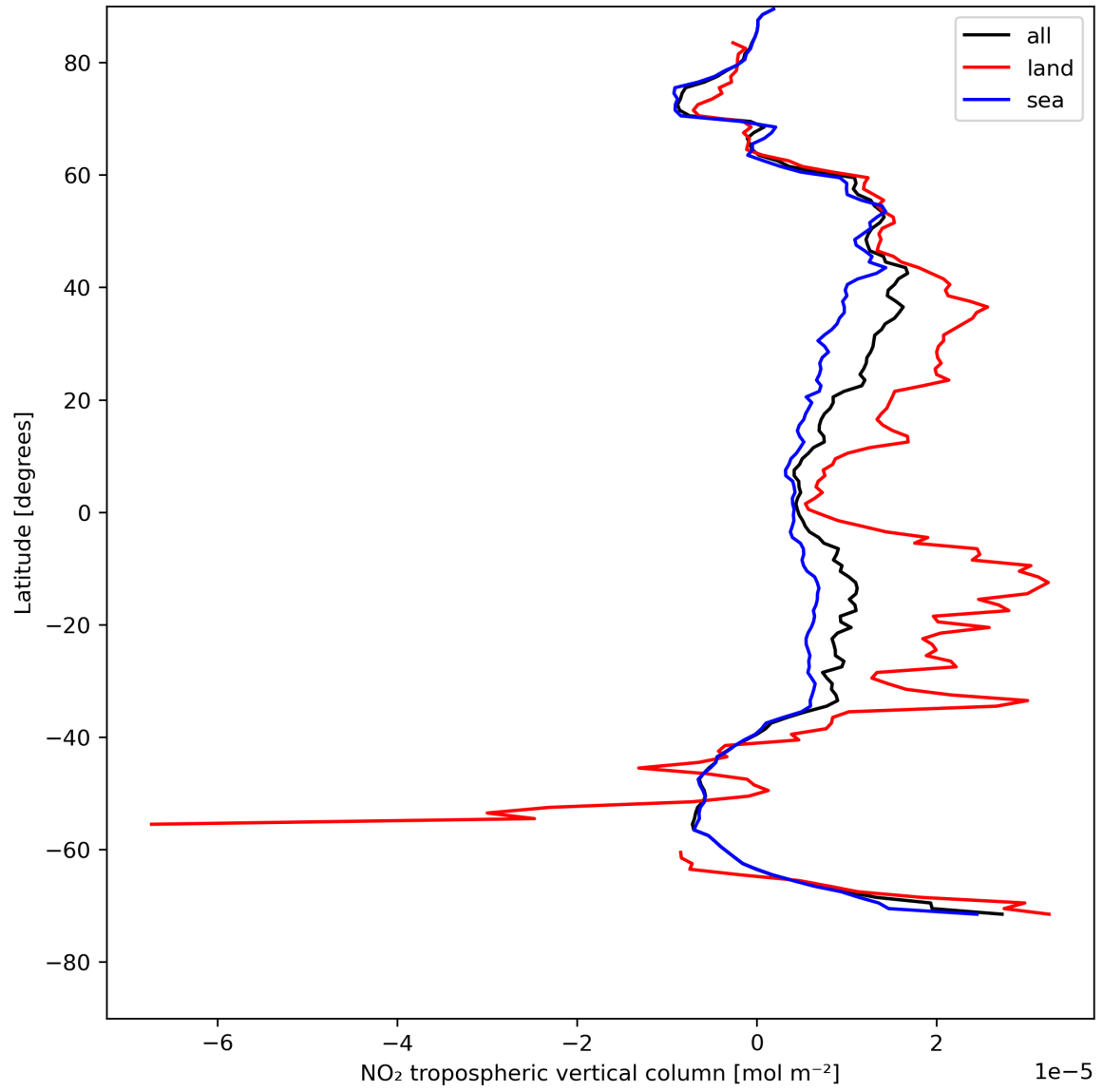
Figure 12: Zonal average of “NO 2 tropospheric vertical column” for 2024-08-06 to 2024-08-07.
