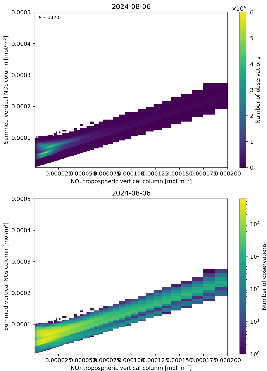
Figure 126: Scatter density plot of “NO 2 tropospheric vertical column” against “Summed vertical NO 2 column” for 2024-08-06 to 2024-08-07.
