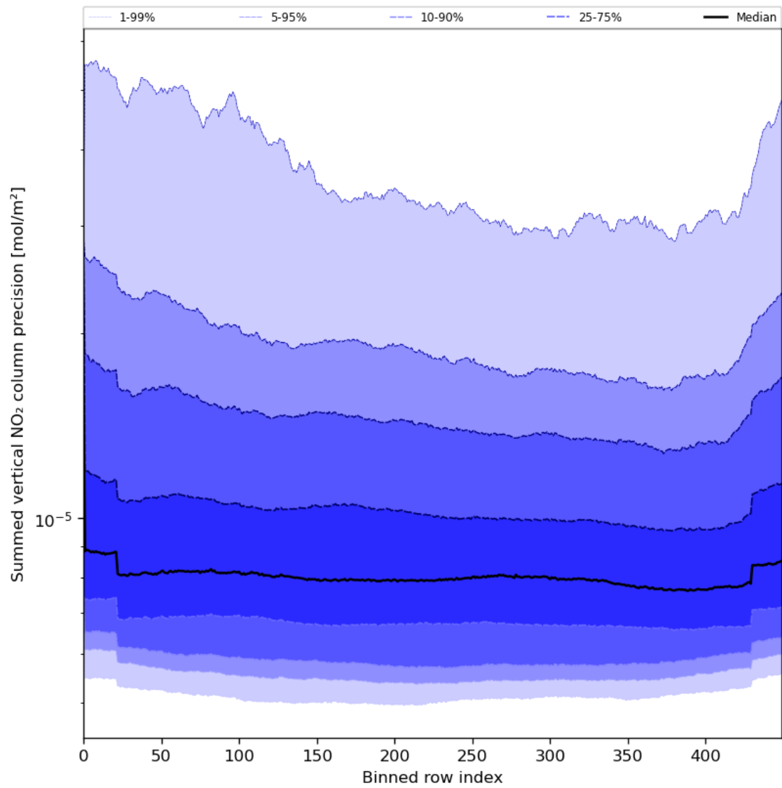
Figure 58: Along track statistics of “Summed vertical NO 2 column precision” for 2024-08-06 to 2024-08-07
