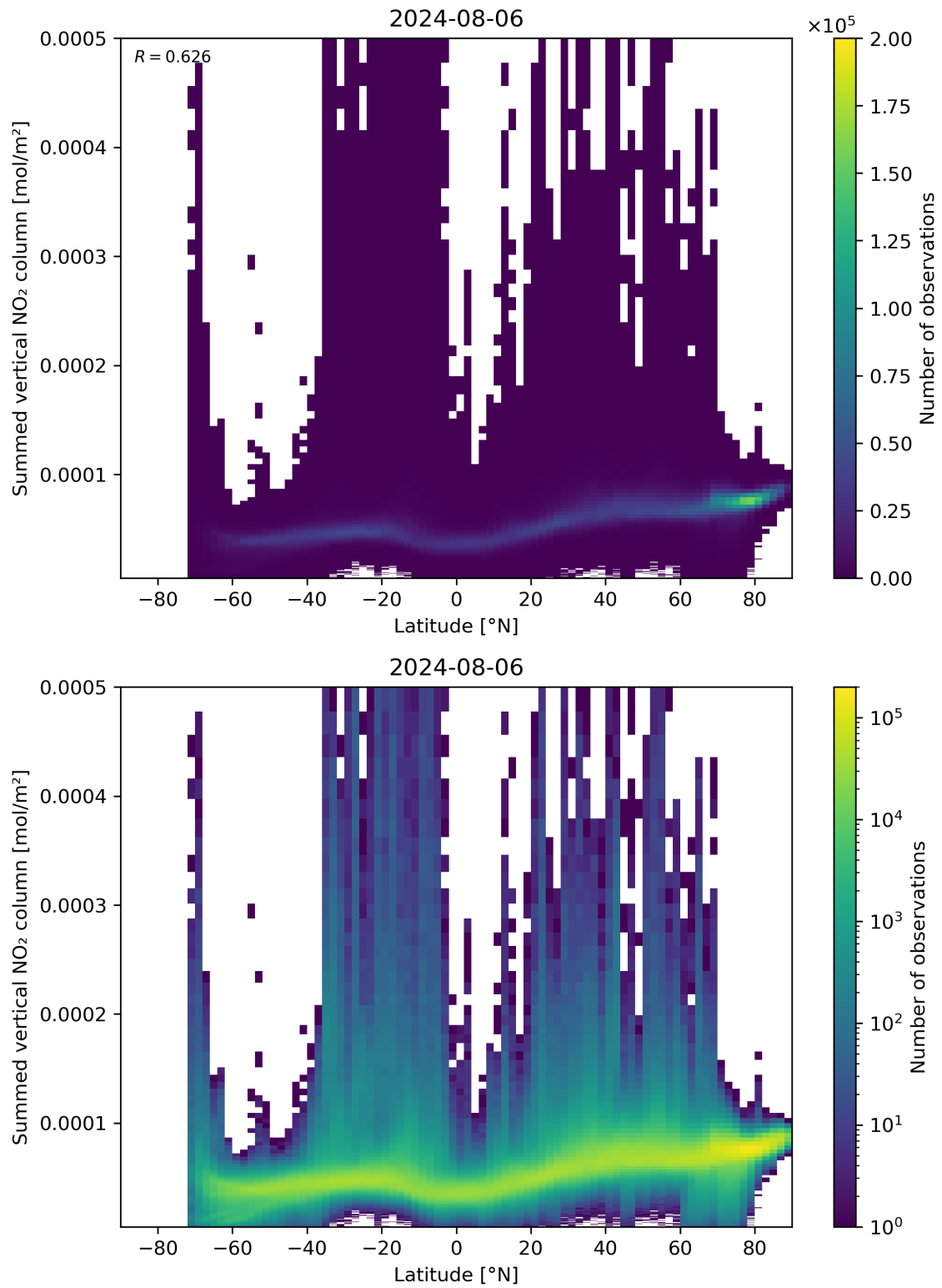
Figure 88: Scatter density plot of “Latitude” against “Summed vertical NO 2 column” for 2024-08-06 to 2024-08-07.
