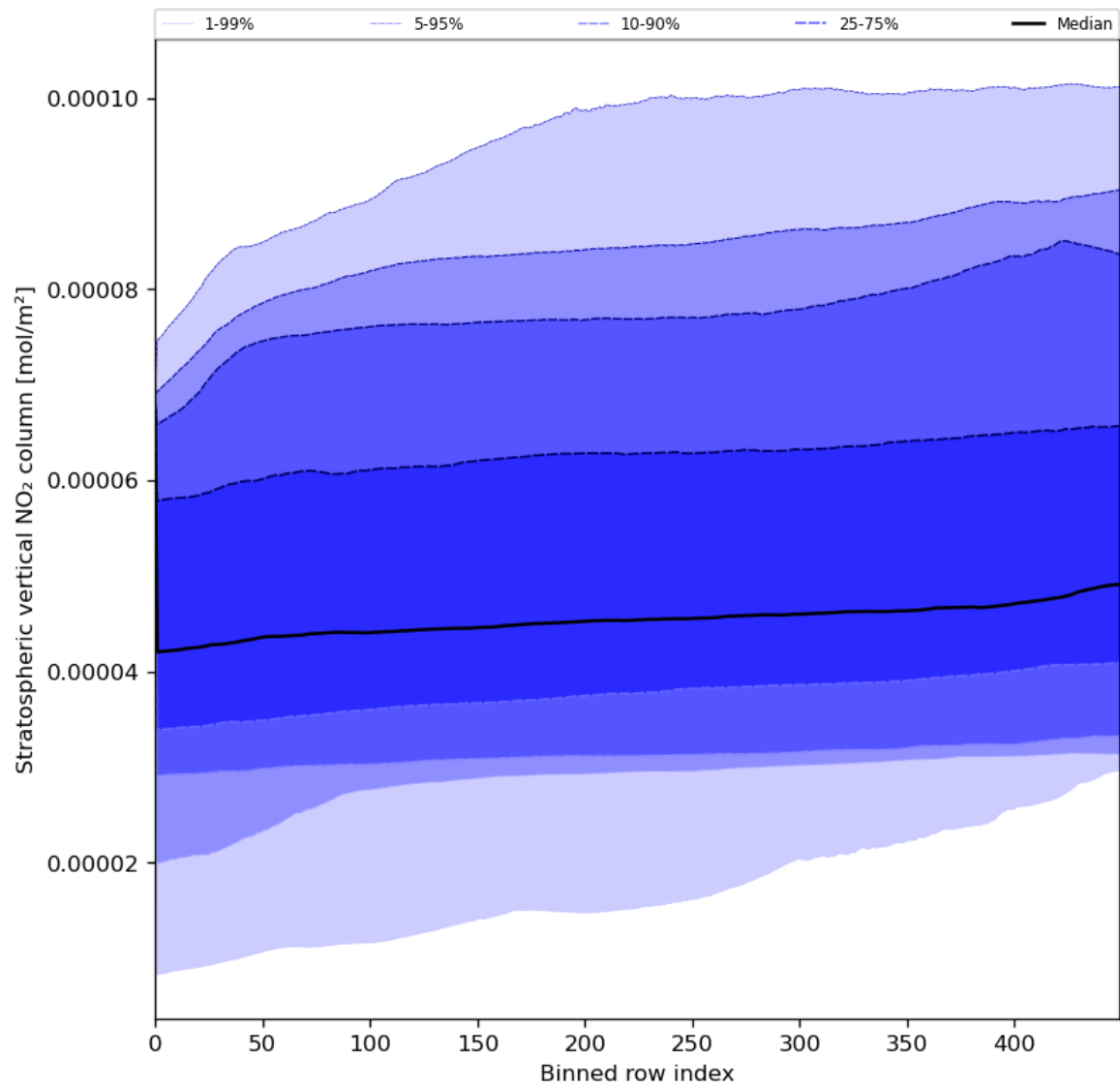
Figure 53: Along track statistics of “Stratospheric vertical NO 2 column” for 2024-08-06 to 2024-08-07
