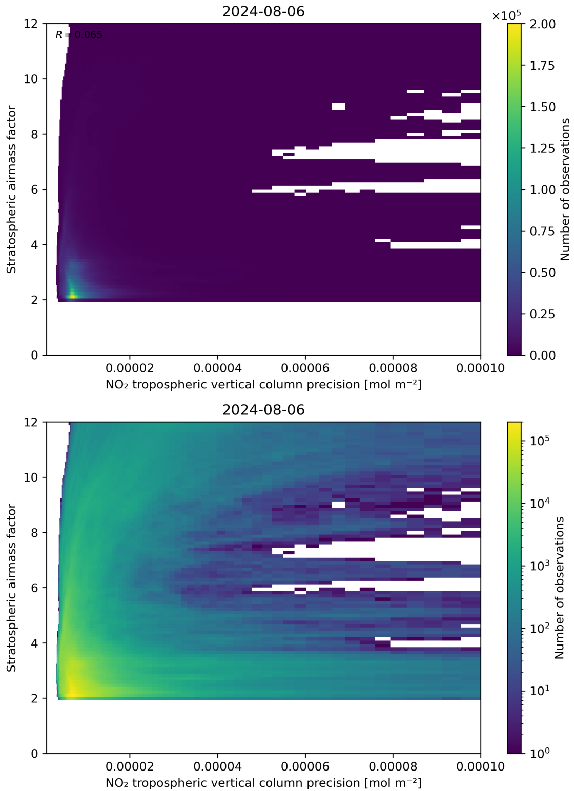
Figure 131: Scatter density plot of “NO 2 tropospheric vertical column precision” against “Stratospheric airmass factor” for 2024-08-06 to 2024-08-07.
