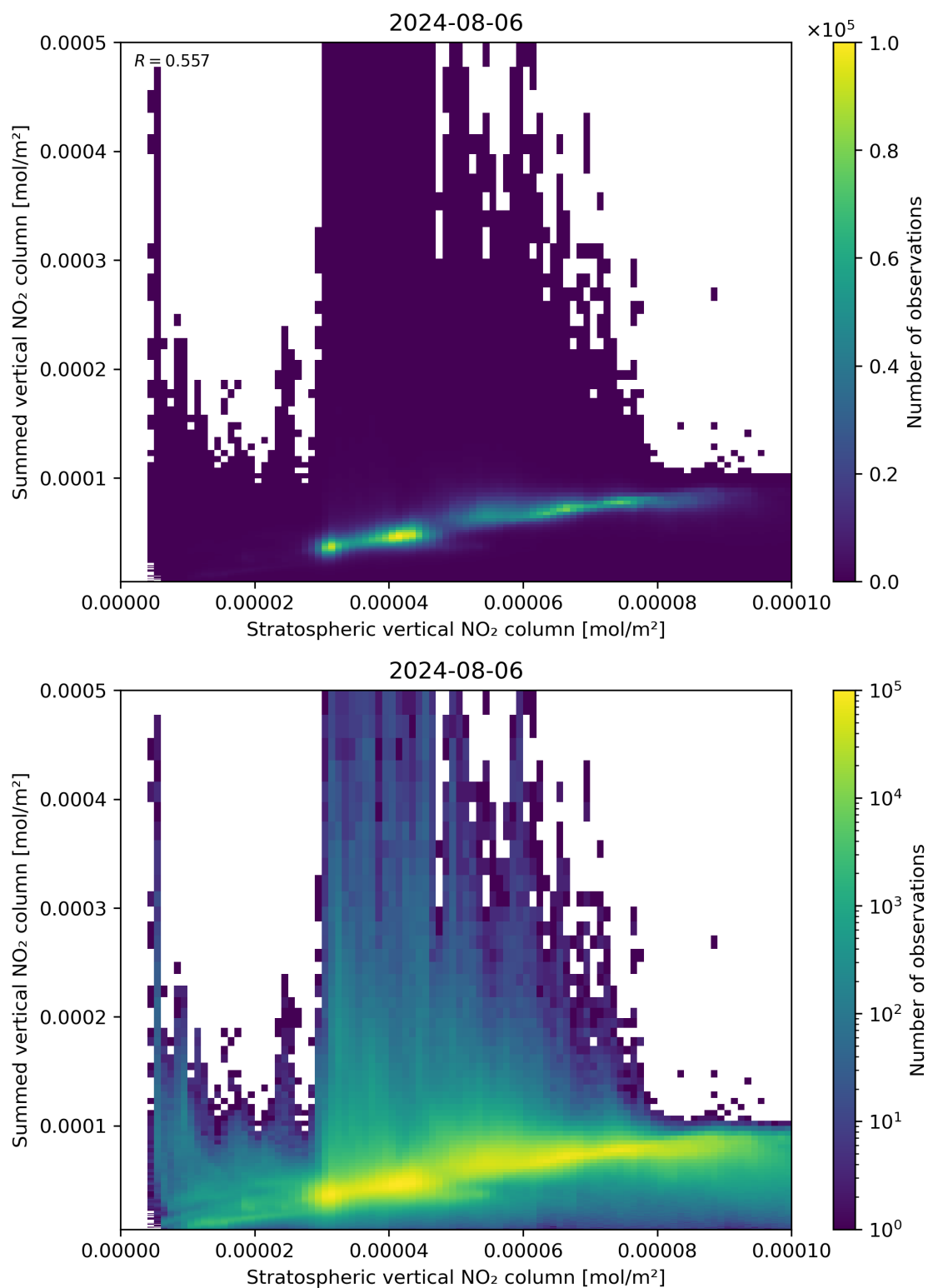
Figure 98: Scatter density plot of “Stratospheric vertical NO 2 column” against “Summed vertical NO 2 column” for 2024-08-06 to 2024-08-07.
