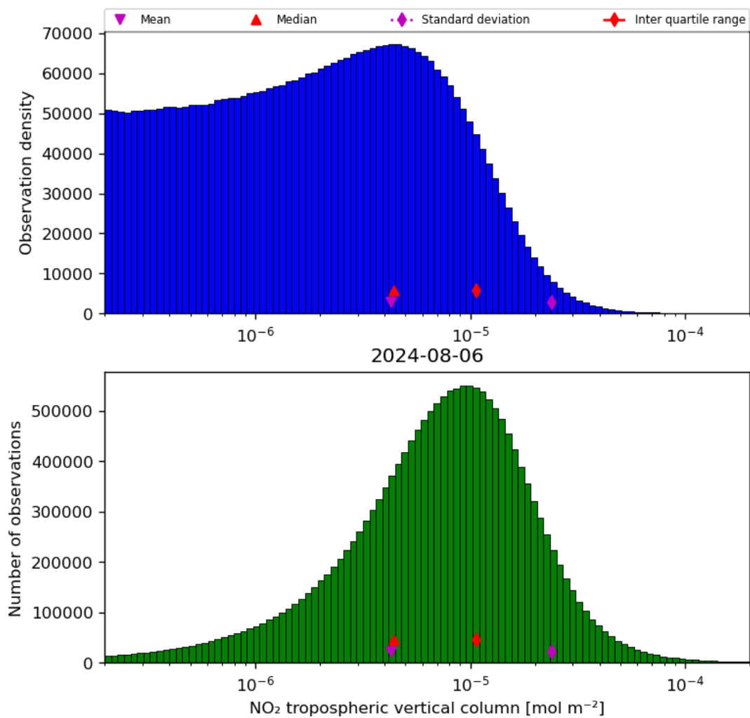
Figure 29: Histogram of “NO 2 tropospheric vertical column” for 2024-08-06 to 2024-08-07
