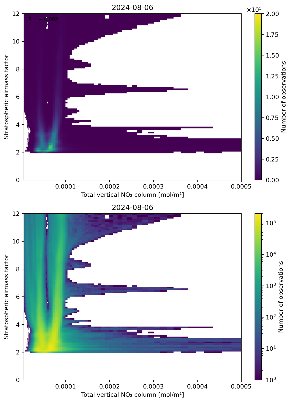
Figure 110: Scatter density plot of “Total vertical NO 2 column” against “Stratospheric airmass factor” for 2024-08-06 to 2024-08-07.
