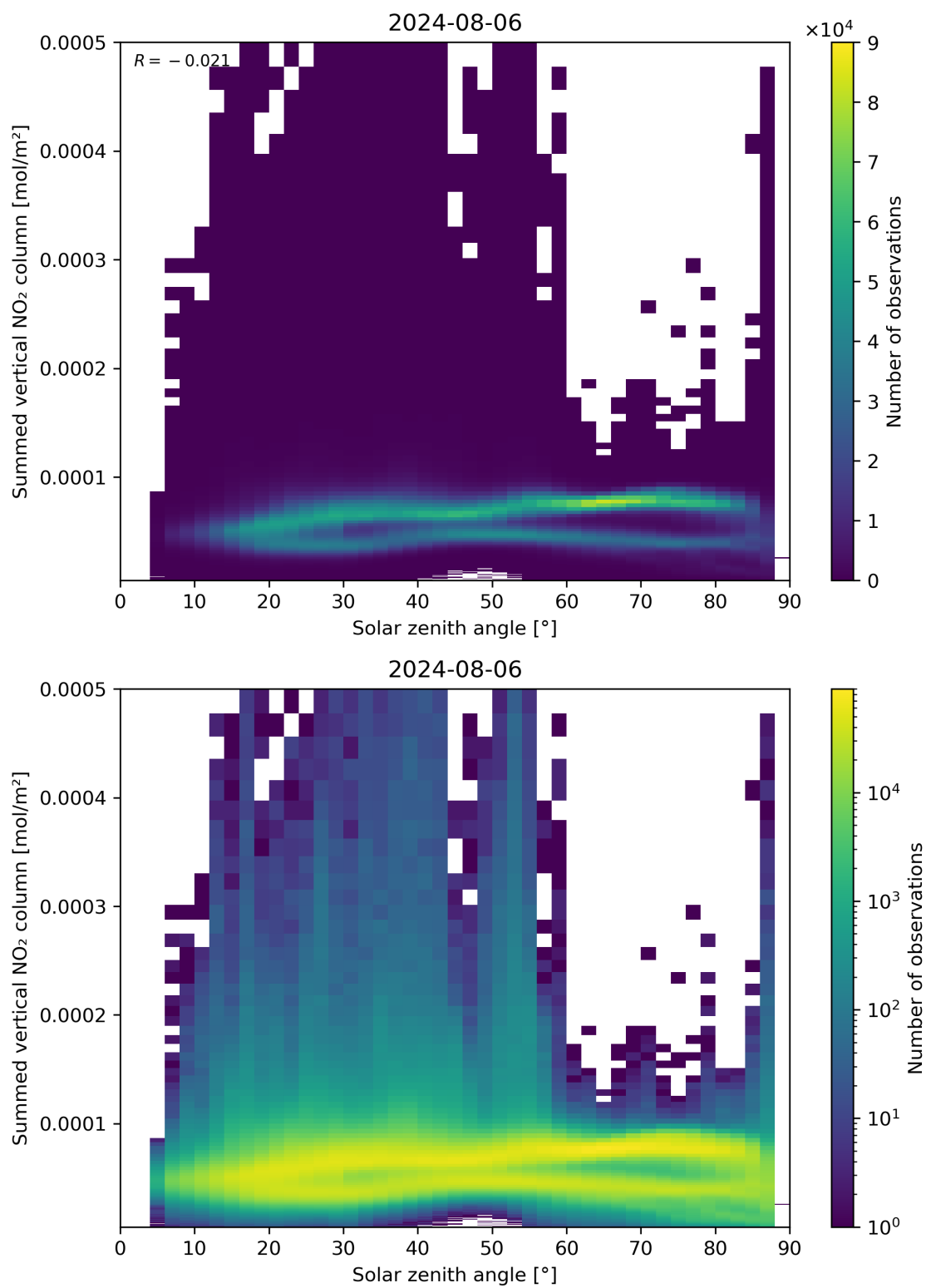
Figure 151: Scatter density plot of “Solar zenith angle” against “Summed vertical NO 2 column” for 2024-08-06 to 2024-08-07.
