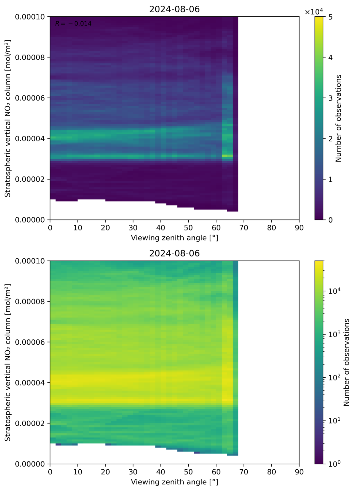
Figure 164: Scatter density plot of “Viewing zenith angle” against “Stratospheric vertical NO 2 column” for 2024-08-06 to 2024-08-07.
