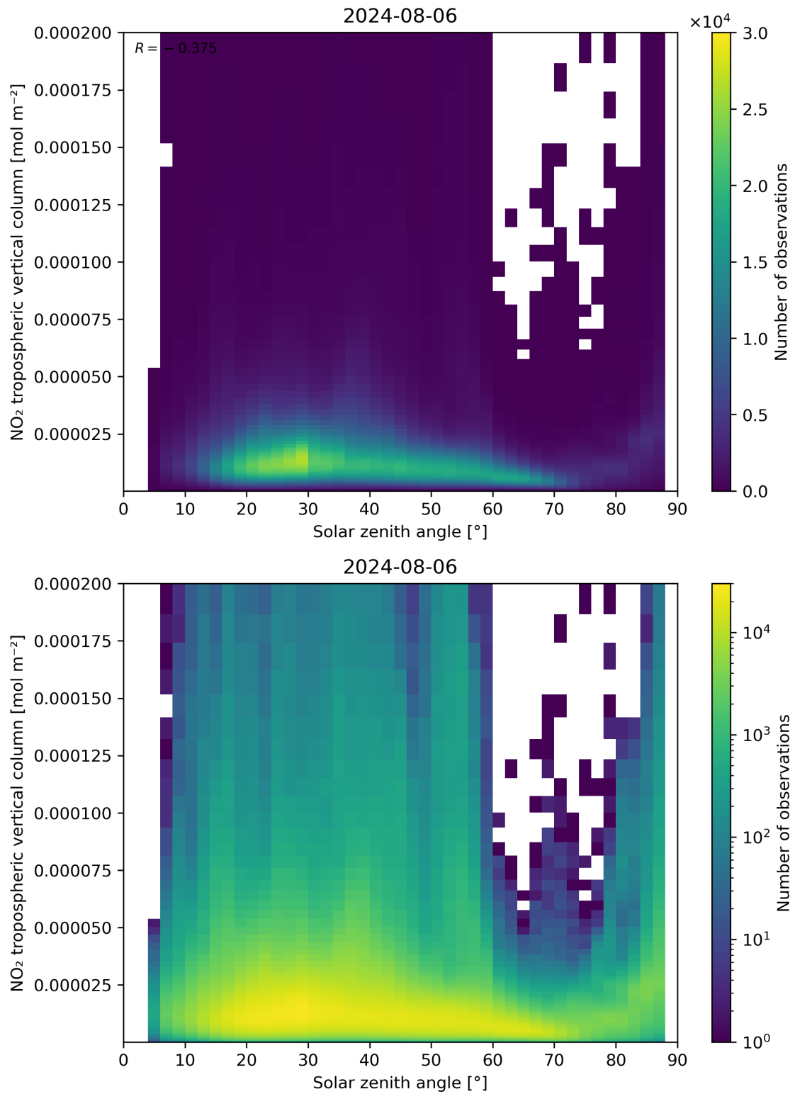
Figure 155: Scatter density plot of “Solar zenith angle” against “NO 2 tropospheric vertical column” for 2024-08-06 to 2024-08-07.
