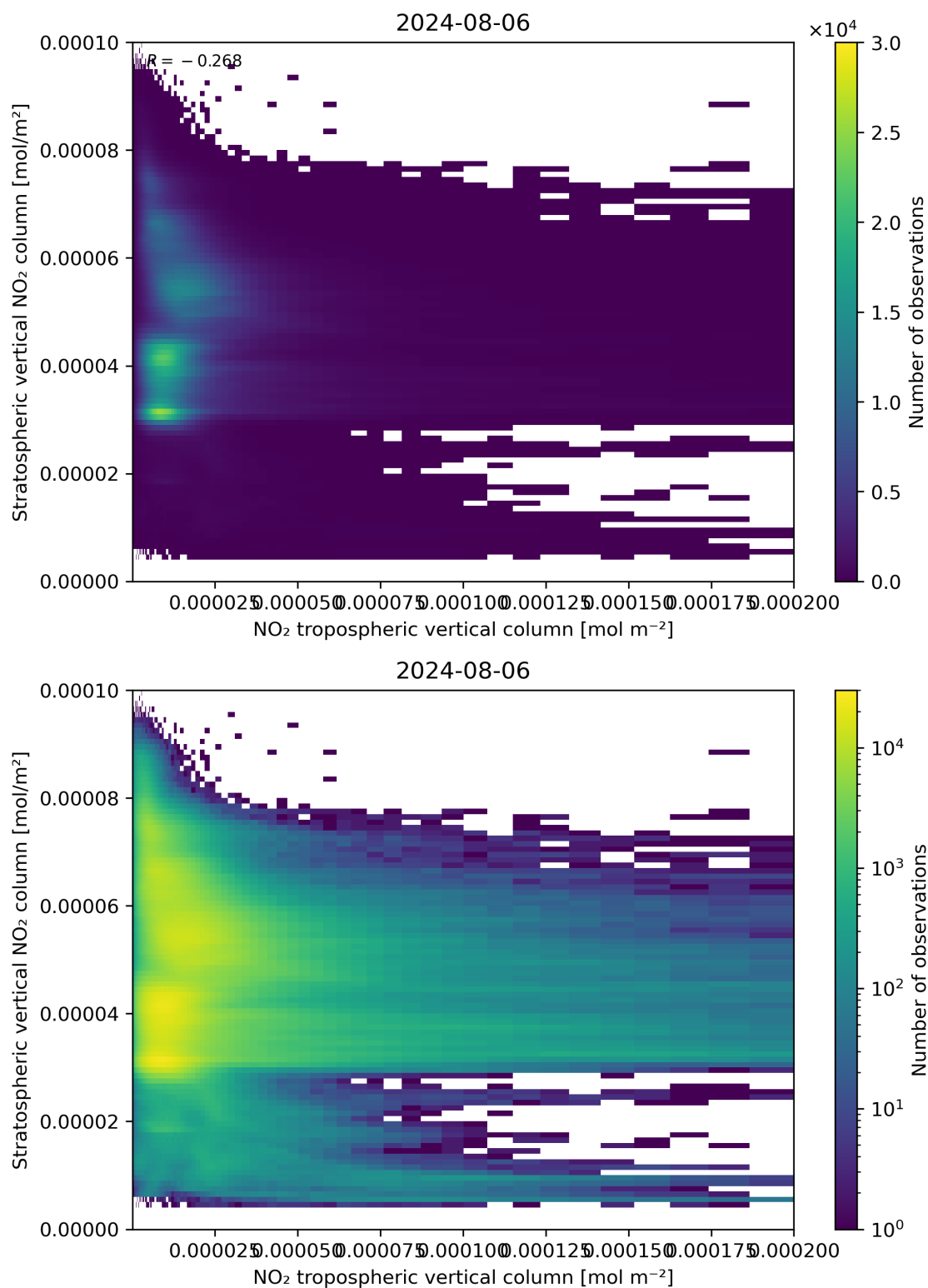
Figure 125: Scatter density plot of “NO 2 tropospheric vertical column” against “Stratospheric vertical NO 2 column” for 2024-08-06 to 2024-08-07.
