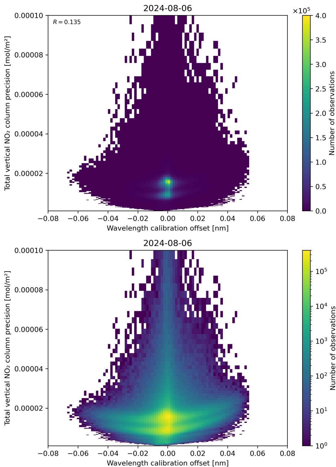
Figure 180: Scatter density plot of “Wavelength calibration offset” against “Total vertical NO 2 column precision” for 2024-08-06 to 2024-08-07.
