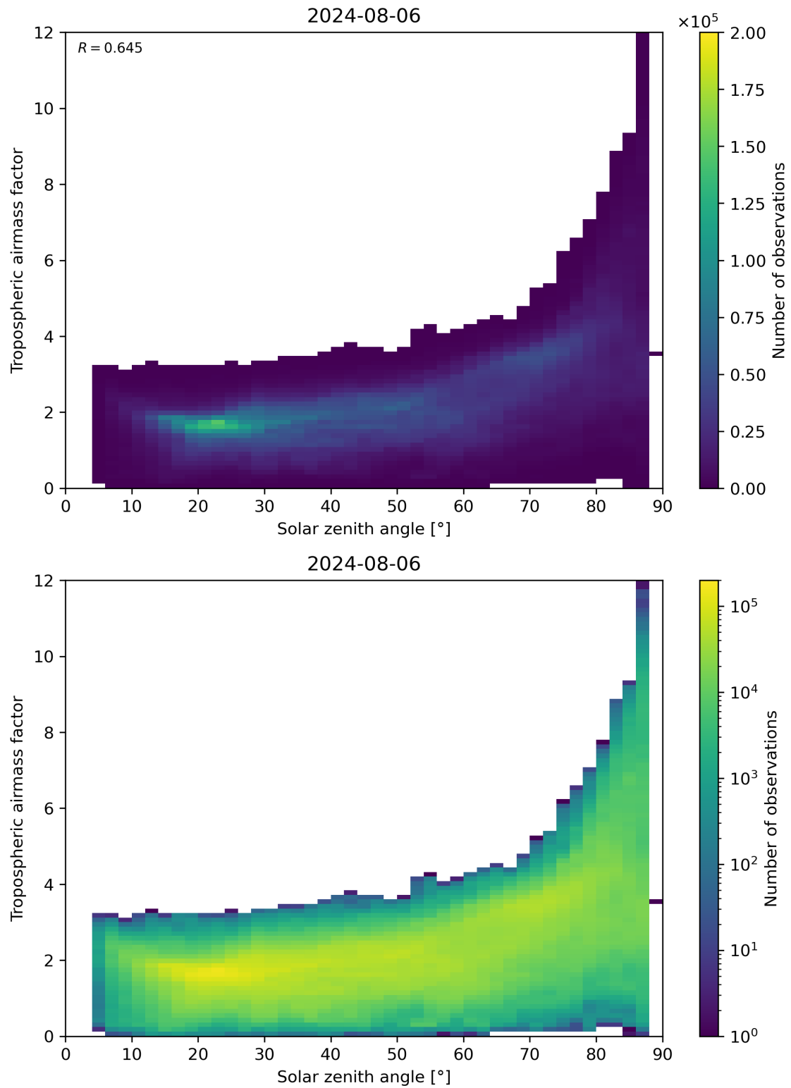
Figure 147: Scatter density plot of “Solar zenith angle” against “Tropospheric airmass factor” for 2024-08-06 to 2024-08-07.
