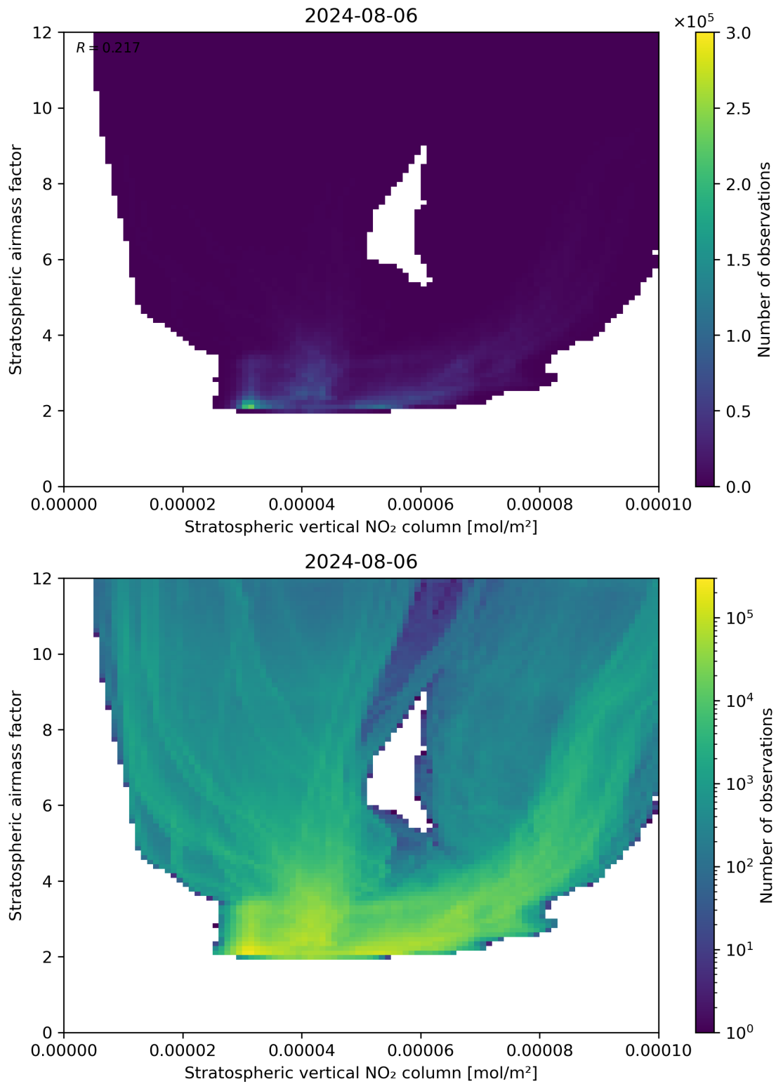
Figure 96: Scatter density plot of “Stratospheric vertical NO 2 column” against “Stratospheric airmass factor” for 2024-08-06 to 2024-08-07.
