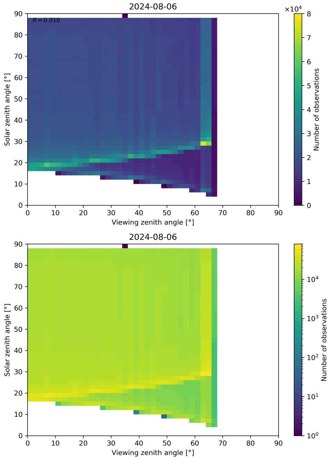
Figure 172: Scatter density plot of “Viewing zenith angle” against “Solar zenith angle” for 2024-08-06 to 2024-08-07.
