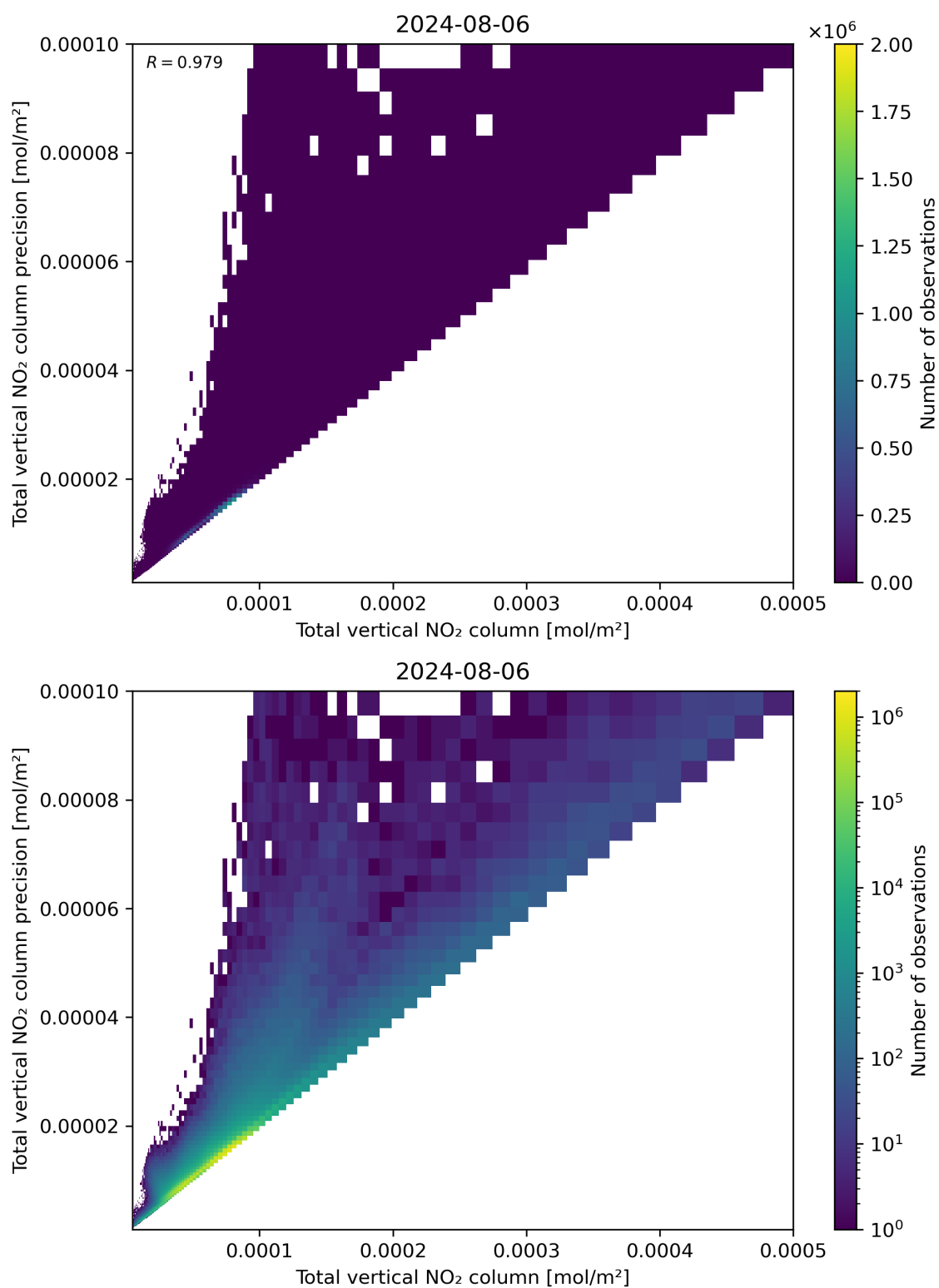
Figure 114: Scatter density plot of “Total vertical NO 2 column” against “Total vertical NO 2 column precision” for 2024-08-06 to 2024-08-07.
