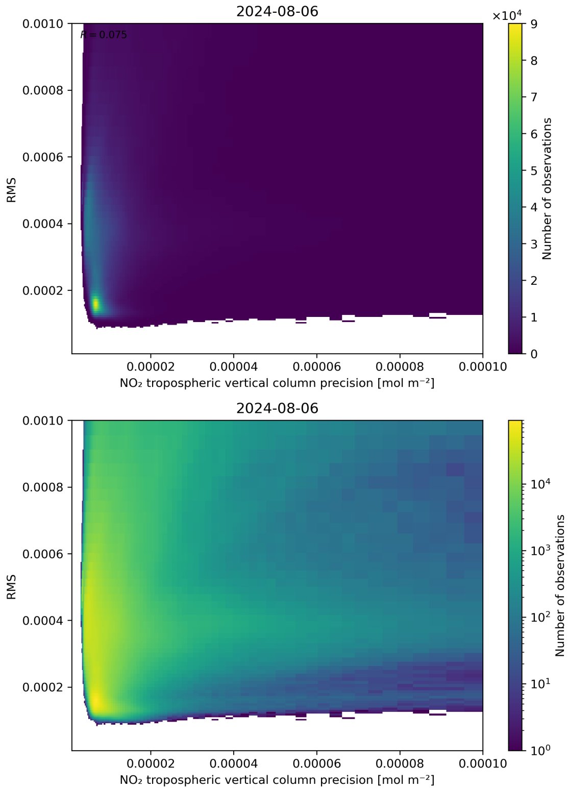
Figure 140: Scatter density plot of “NO 2 tropospheric vertical column precision” against “RMS” for 2024-08-06 to 2024-08-07.
