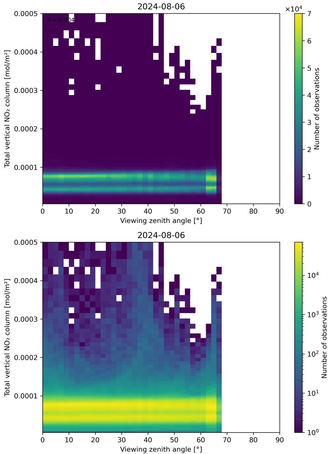
Figure 167: Scatter density plot of “Viewing zenith angle” against “Total vertical NO 2 column” for 2024-08-06 to 2024-08-07.
