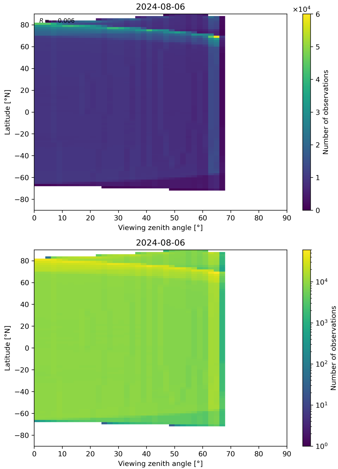
Figure 163: Scatter density plot of “Viewing zenith angle” against “Latitude” for 2024-08-06 to 2024-08-07.
