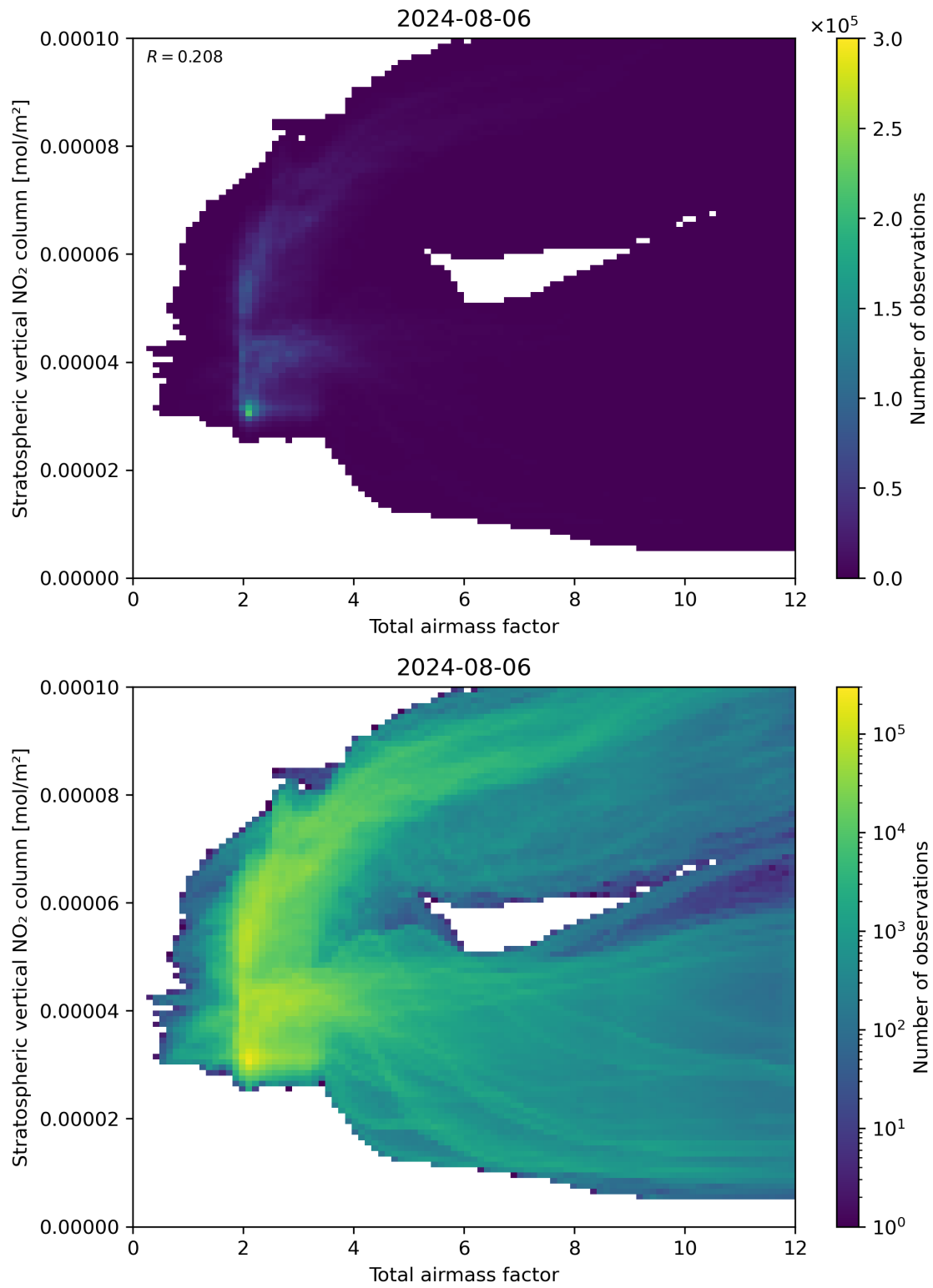
Figure 64: Scatter density plot of “Total airmass factor” against “Stratospheric vertical \text{NO}_2 column” for 2024-08-06 to 2024-08-07.
