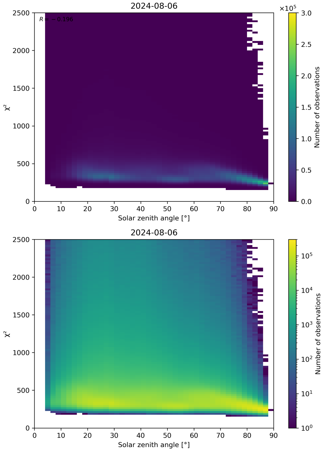
Figure 148: Scatter density plot of “Solar zenith angle” against “ \chi^2 ” for 2024-08-06 to 2024-08-07.
