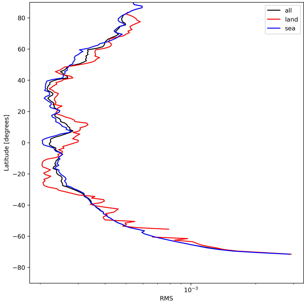
Figure 26: Zonal average of “RMS” for 2024-08-06 to 2024-08-07.
