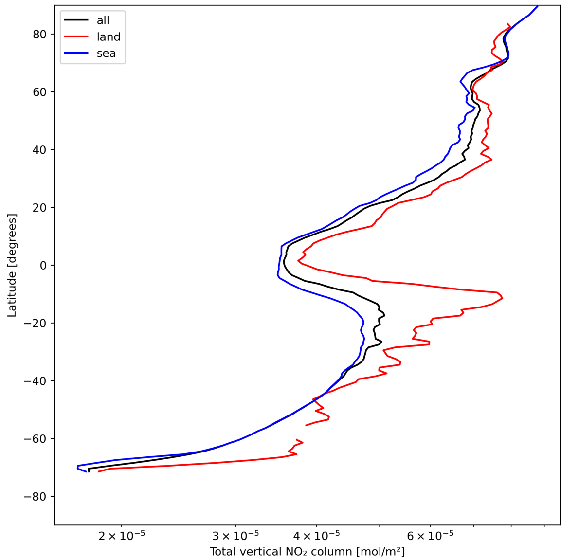
Figure 21: Zonal average of “Total vertical NO 2 column” for 2024-08-06 to 2024-08-07.
