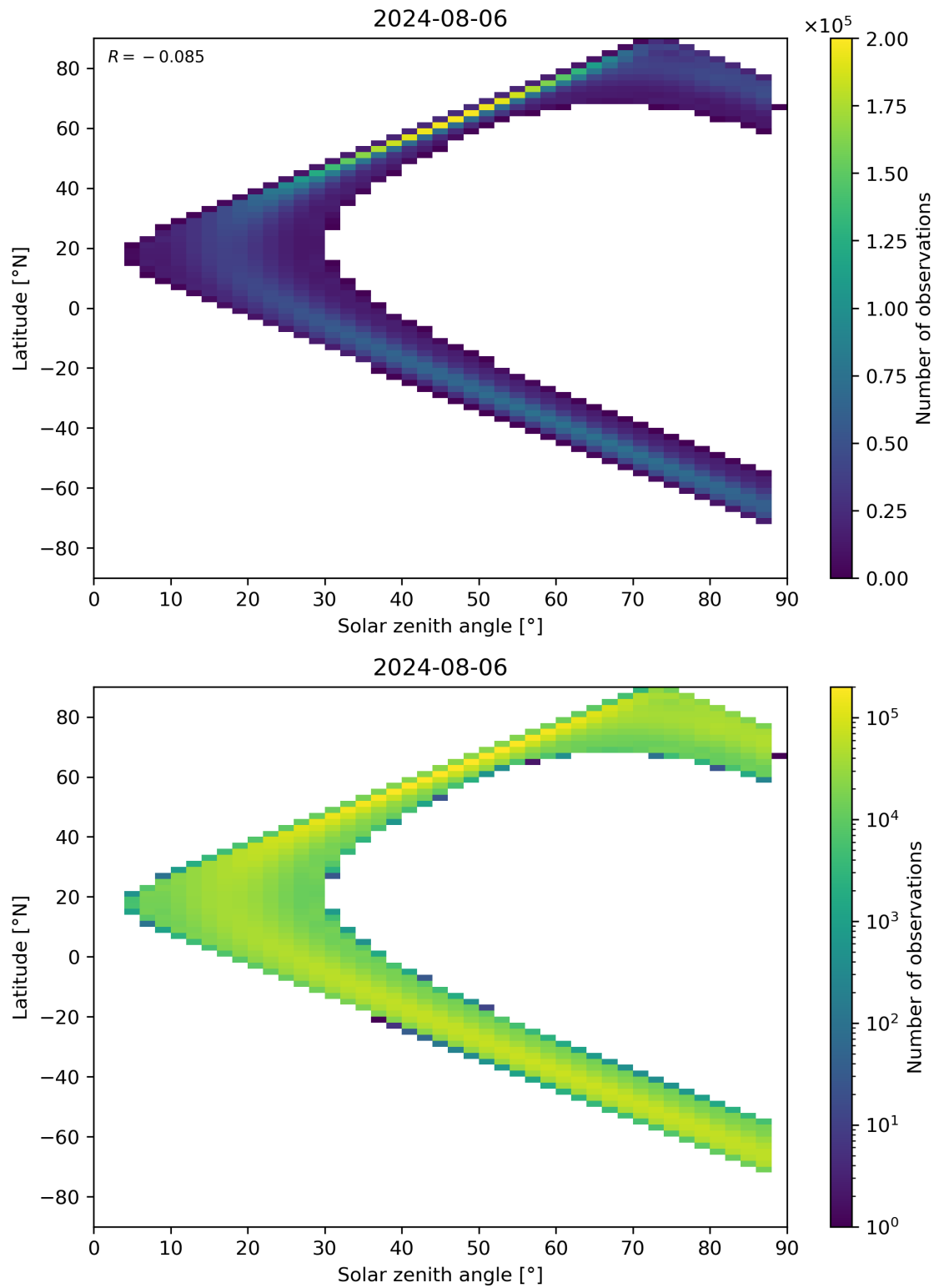
Figure 149: Scatter density plot of “Solar zenith angle” against “Latitude” for 2024-08-06 to 2024-08-07.
