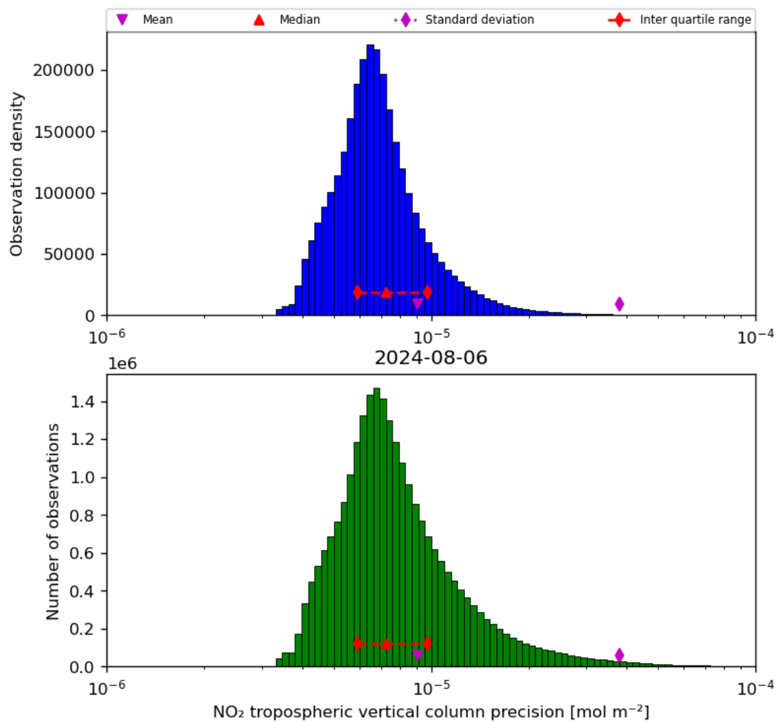
Figure 30: Histogram of "NO 2 tropospheric vertical column precision" for 2024-08-06 to 2024-08-07
