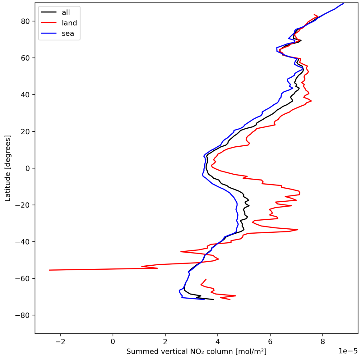
Figure 23: Zonal average of “Summed vertical NO 2 column” for 2024-08-06 to 2024-08-07.
