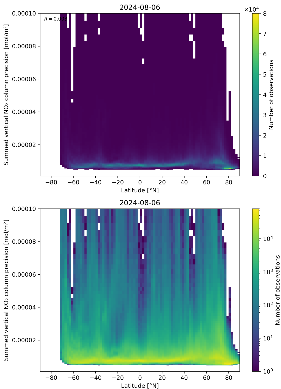
Figure 89: Scatter density plot of “Latitude” against “Summed vertical NO 2 column precision” for 2024-08-06 to 2024-08-07.
