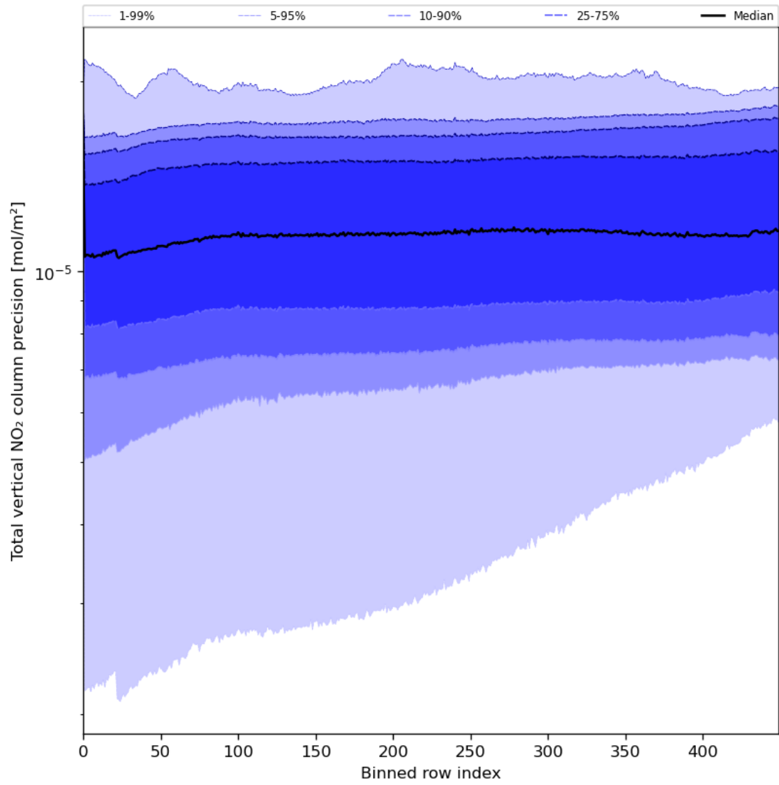
Figure 56: Along track statistics of “Total vertical NO 2 column precision” for 2024-08-06 to 2024-08-07
