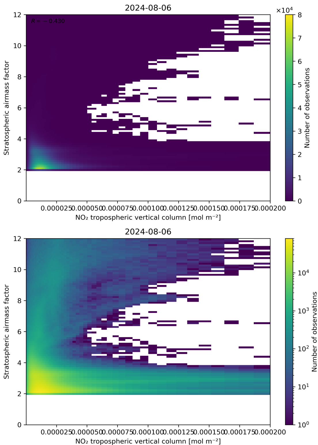
Figure 121: Scatter density plot of “NO 2 tropospheric vertical column” against “Stratospheric air mass factor” for 2024-08-06 to 2024-08-07.
