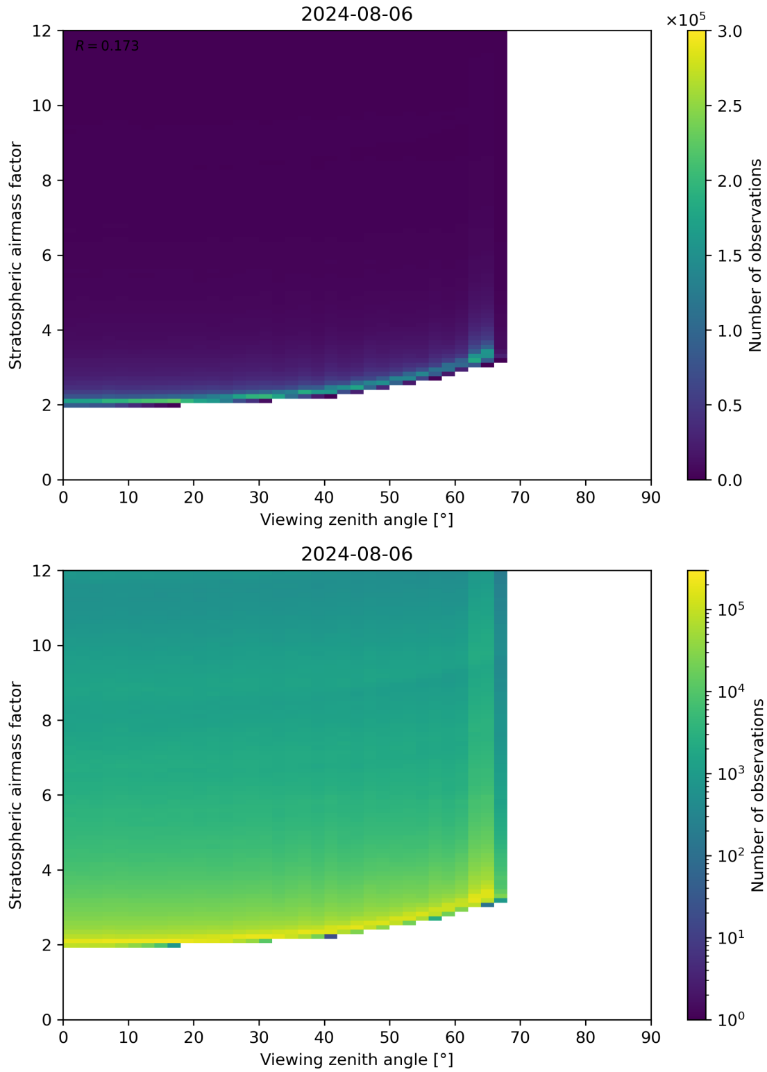
Figure 159: Scatter density plot of “Viewing zenith angle” against “Stratospheric airmass factor” for 2024-08-06 to 2024-08-07.
