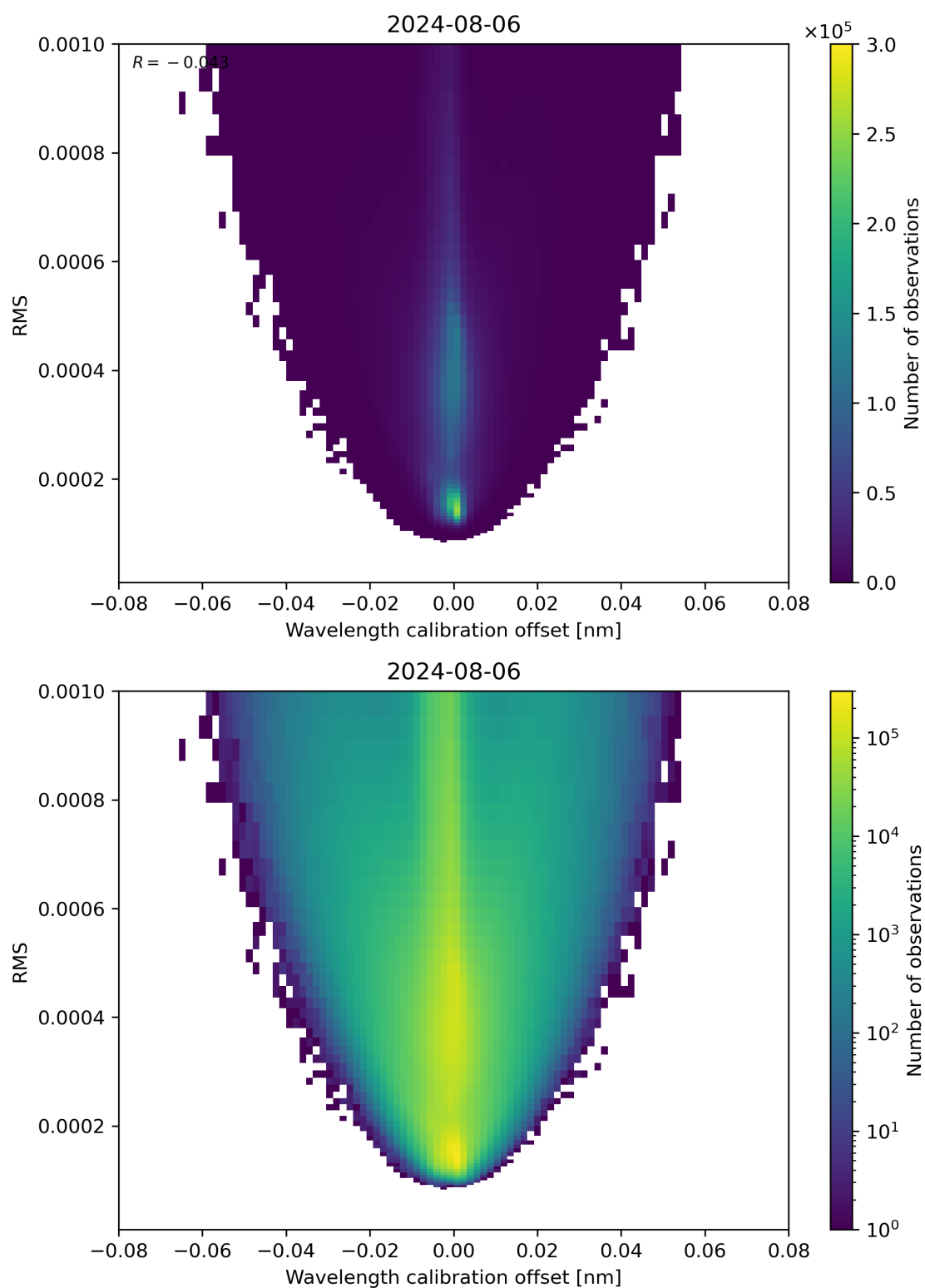
Figure 181: Scatter density plot of “Wavelength calibration offset” against “RMS” for 2024-08-06 to 2024-08-07.
