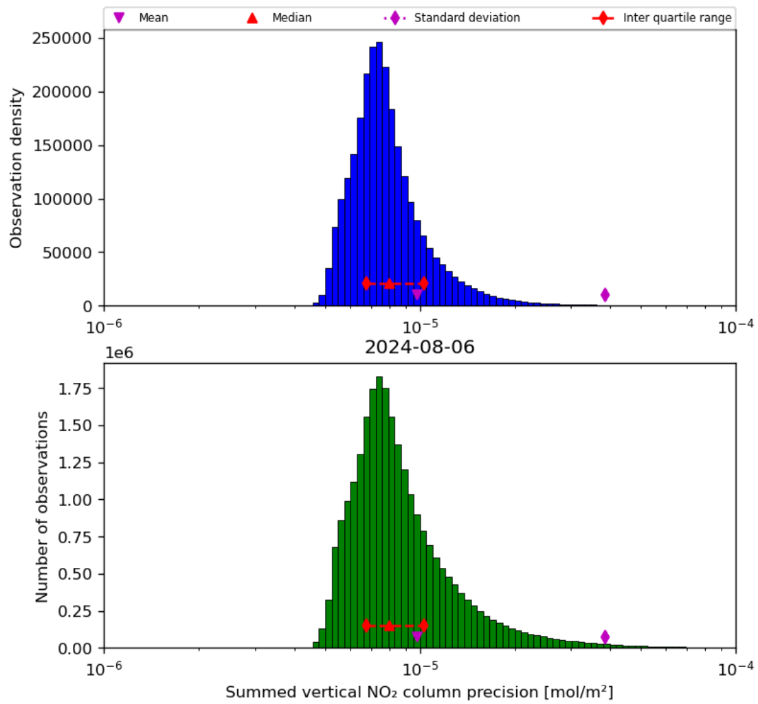
Figure 41: Histogram of “Summed vertical NO 2 column precision” for 2024-08-06 to 2024-08-07
