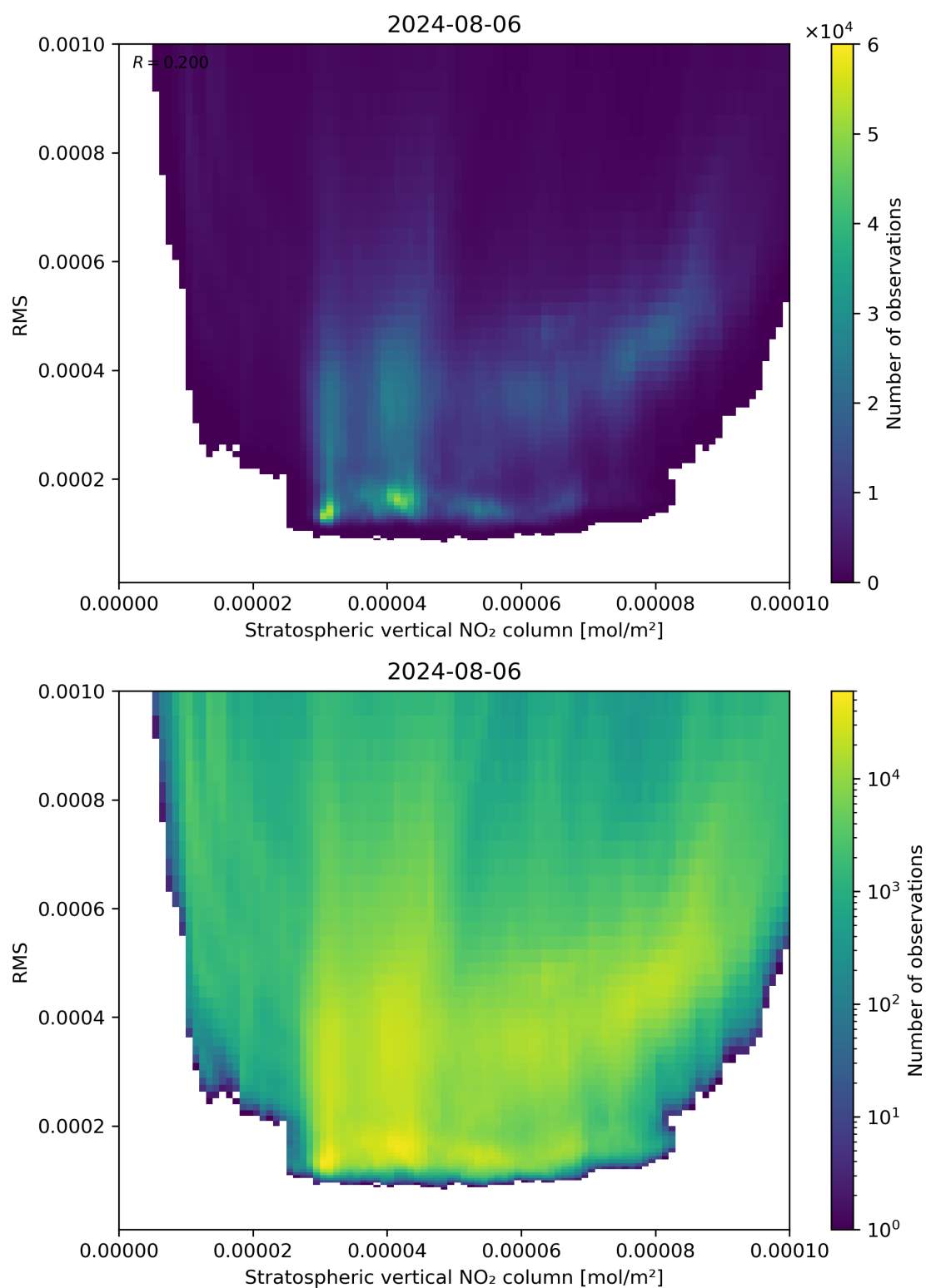
Figure 102: Scatter density plot of “Stratospheric vertical NO 2 column” against “RMS” for 2024-08-06 to 2024-08-07.
