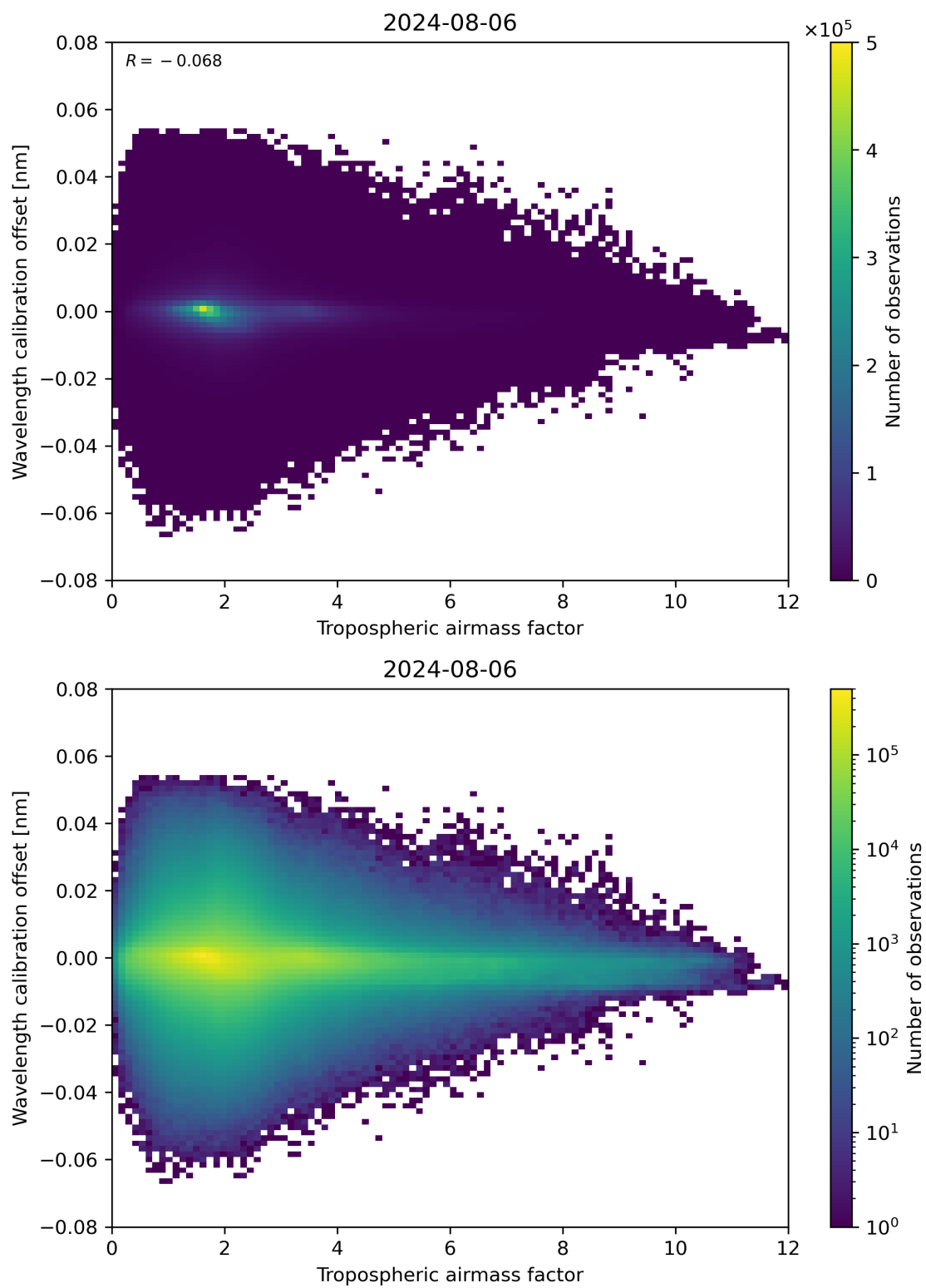
Figure 80: Scatter density plot of “Tropospheric air mass factor” against “Wavelength calibration offset” for 2024-08-06 to 2024-08-07.
