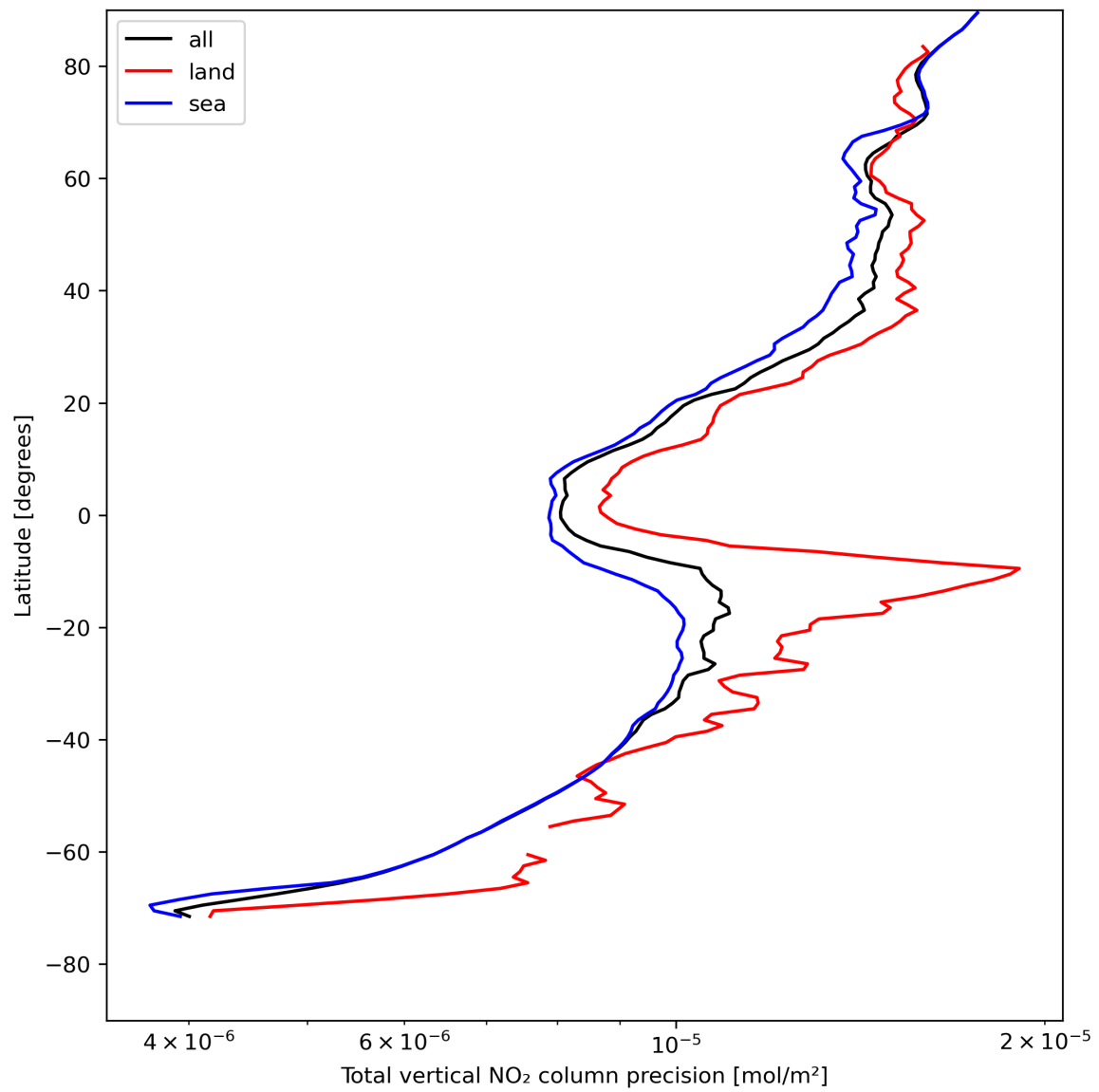
Figure 22: Zonal average of “Total vertical NO 2 column precision” for 2024-08-06 to 2024-08-07.
