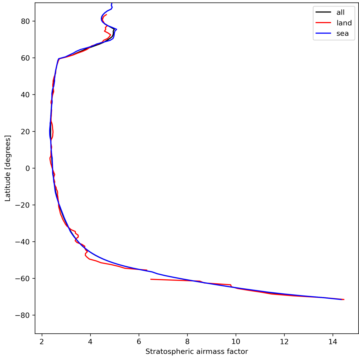
Figure 27: Zonal average of “Stratospheric air mass factor” for 2024-08-06 to 2024-08-07.
