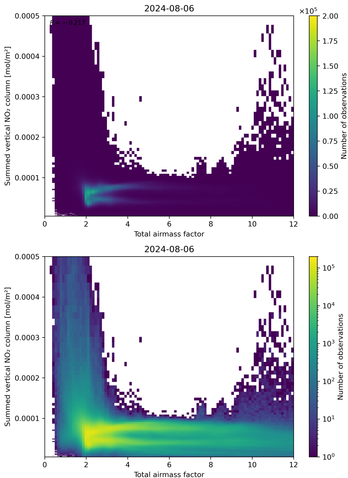
Figure 65: Scatter density plot of “Total airmass factor” against “Summed vertical NO 2 column” for 2024-08-06 to 2024-08-07.
