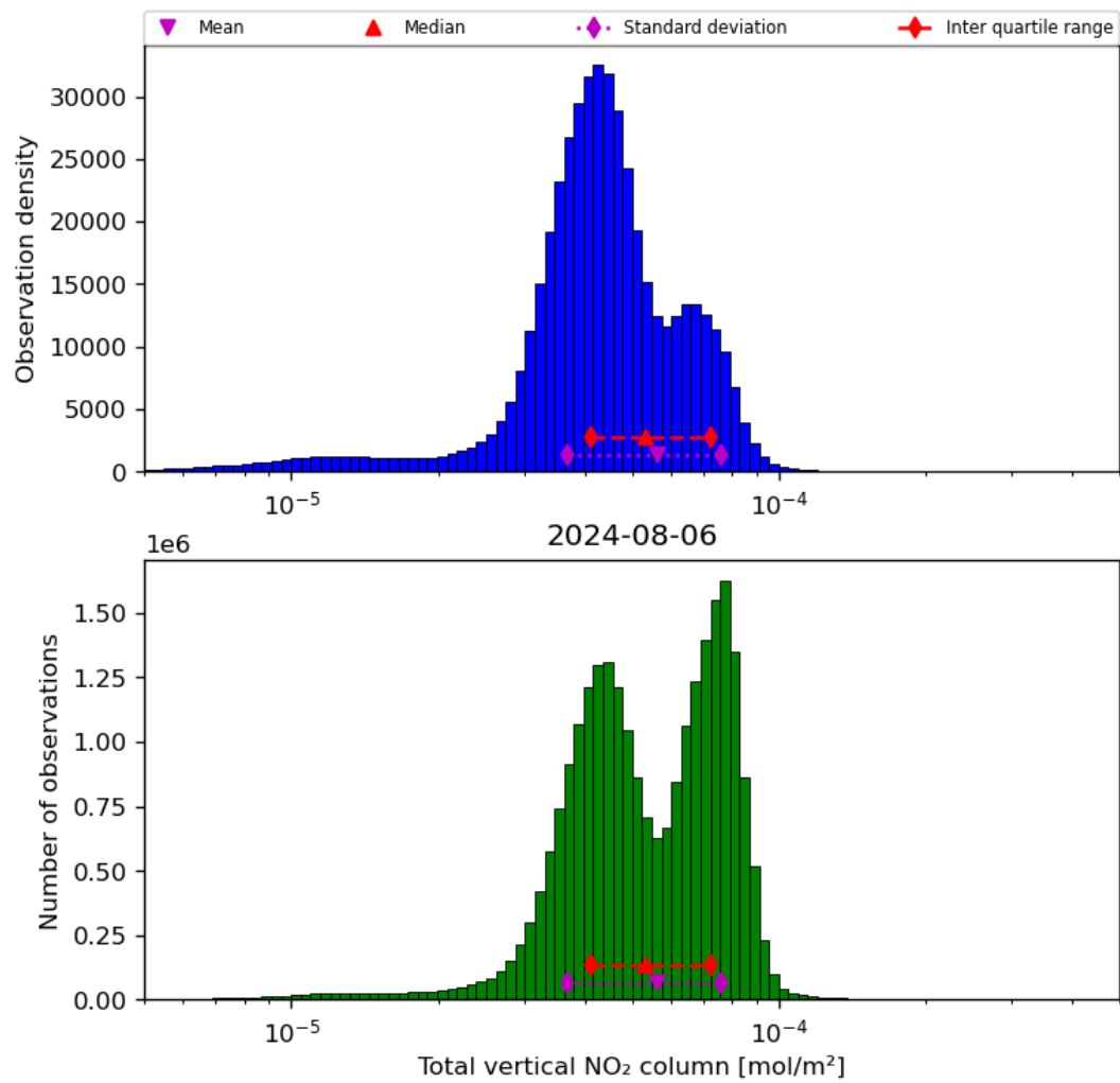
Figure 38: Histogram of “Total vertical NO 2 column” for 2024-08-06 to 2024-08-07
