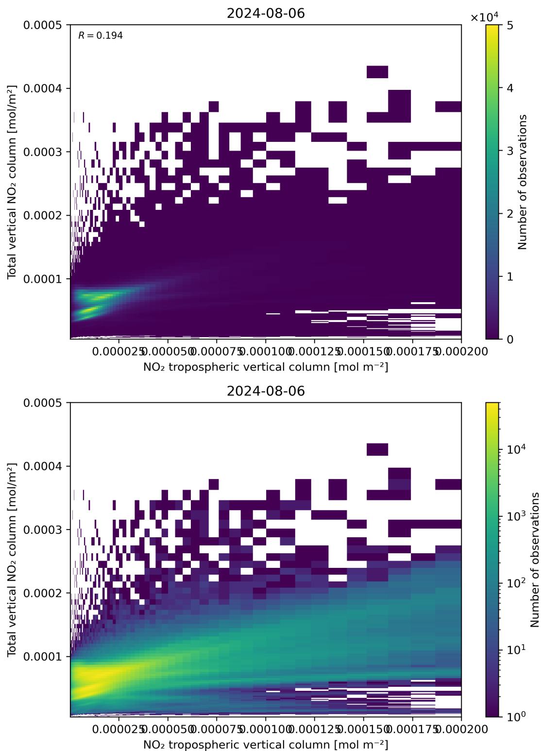
Figure 128: Scatter density plot of “NO 2 tropospheric vertical column” against “Total vertical NO 2 column” for 2024-08-06 to 2024-08-07.
