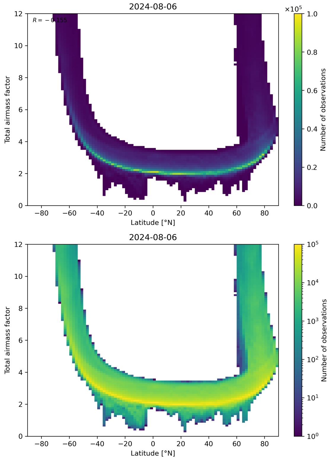
Figure 84: Scatter density plot of “Latitude” against “Total airmass factor” for 2024-08-06 to 2024-08-07.
