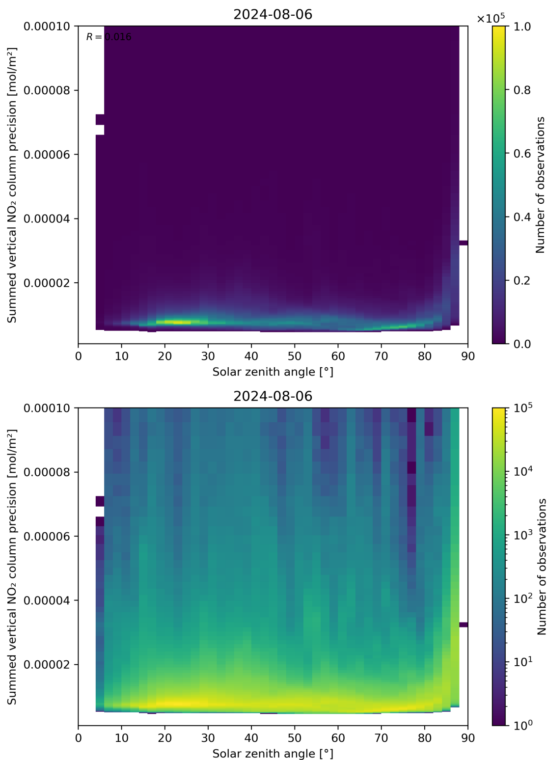
Figure 152: Scatter density plot of “Solar zenith angle” against “Summed vertical NO 2 column precision” for 2024-08-06 to 2024-08-07.
