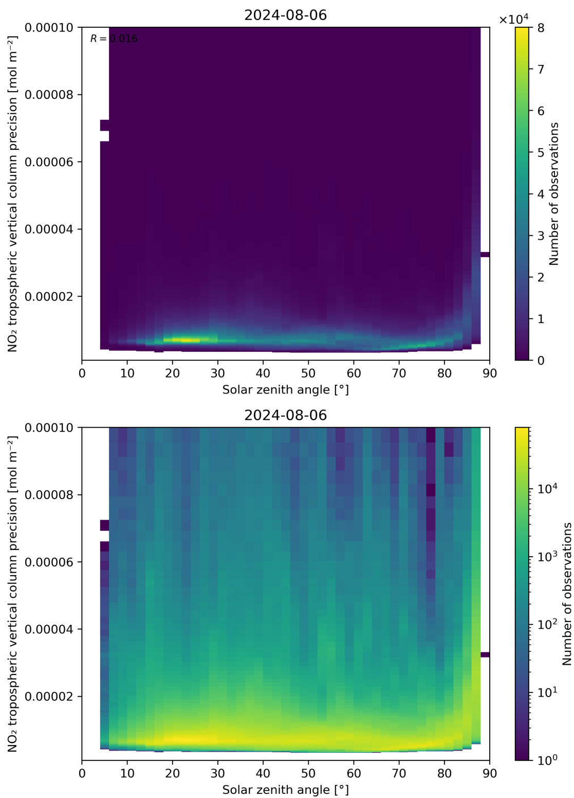
Figure 156: Scatter density plot of “Solar zenith angle” against “NO 2 tropospheric vertical column precision” for 2024-08-06 to 2024-08-07.
