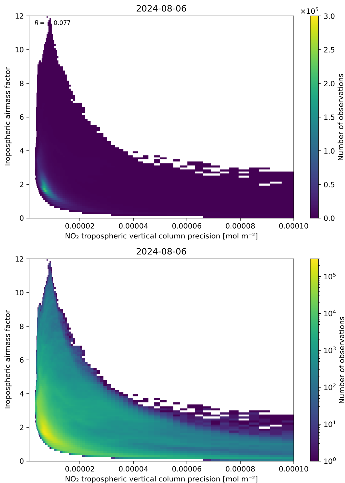
Figure 133: Scatter density plot of “NO 2 tropospheric vertical column precision” against “Tropospheric airmass factor” for 2024-08-06 to 2024-08-07.
