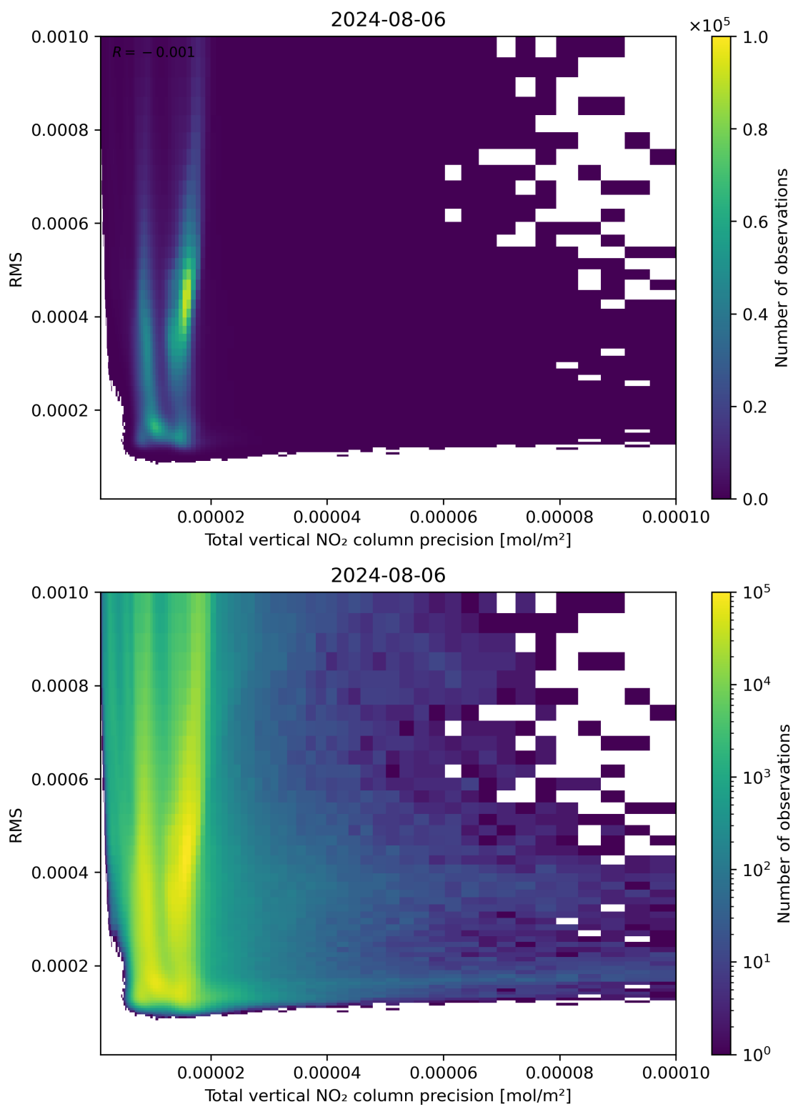
Figure 119: Scatter density plot of “Total vertical NO 2 column precision” against “RMS” for 2024-08-06 to 2024-08-07.
