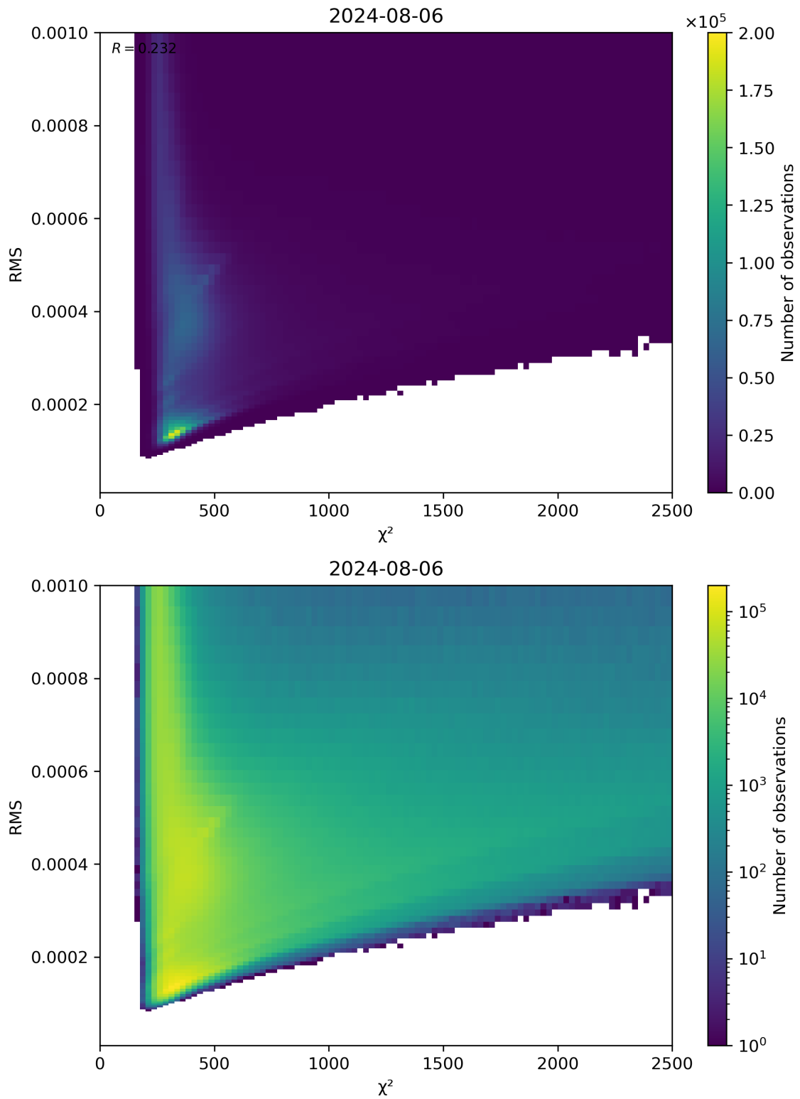
Figure 82: Scatter density plot of “ \chi^2 ” against “RMS” for 2024-08-06 to 2024-08-07.
