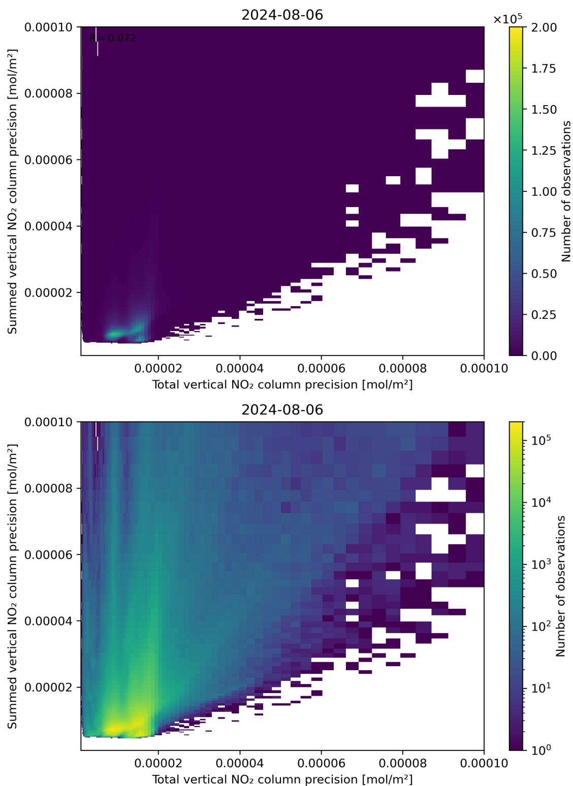
Figure 118: Scatter density plot of “Total vertical NO 2 column precision” against “Summed vertical NO 2 column precision” for 2024-08-06 to 2024-08-07.
