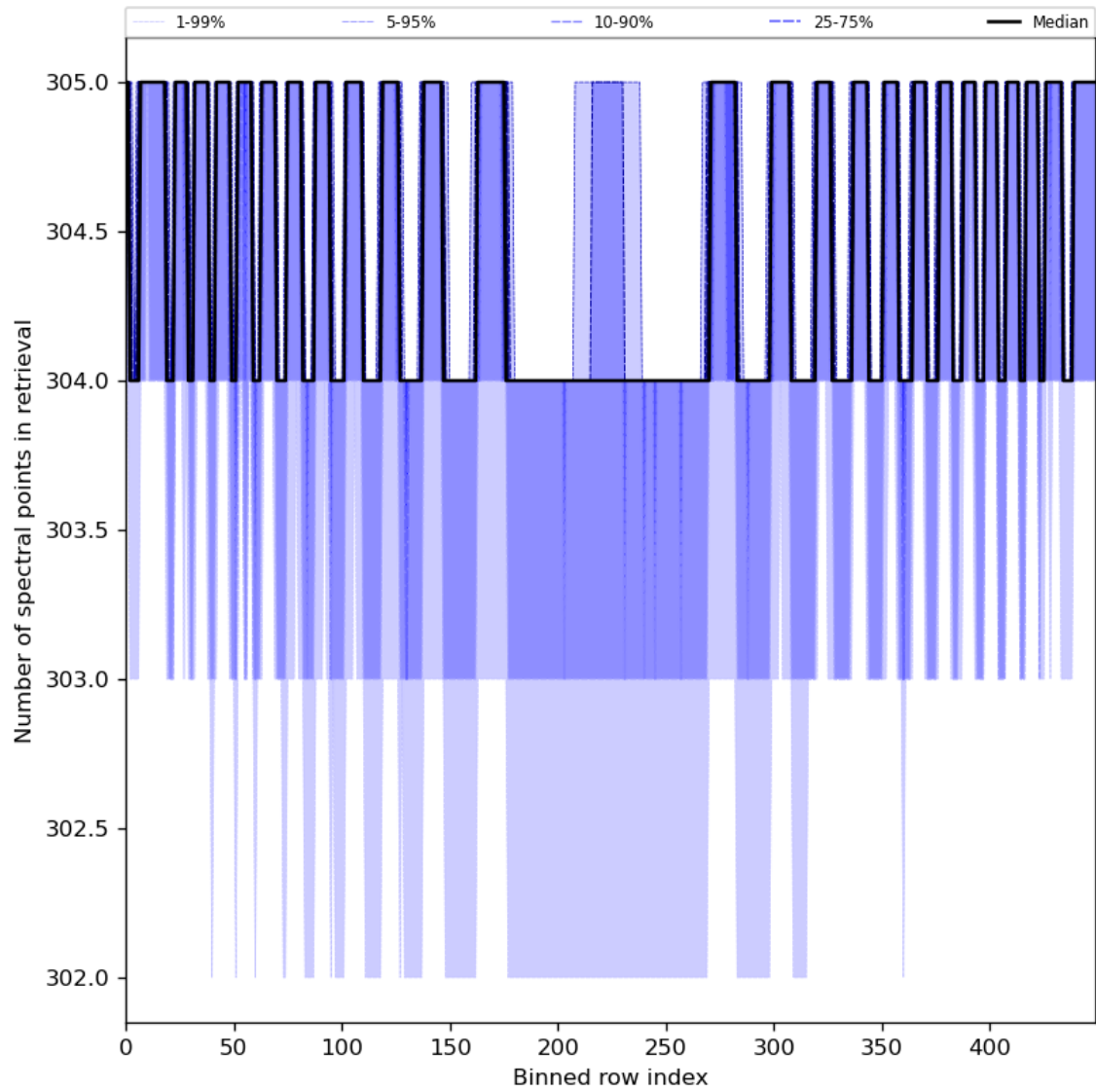
Figure 50: Along track statistics of “Number of spectral points in retrieval” for 2024-08-06 to 2024-08-07
