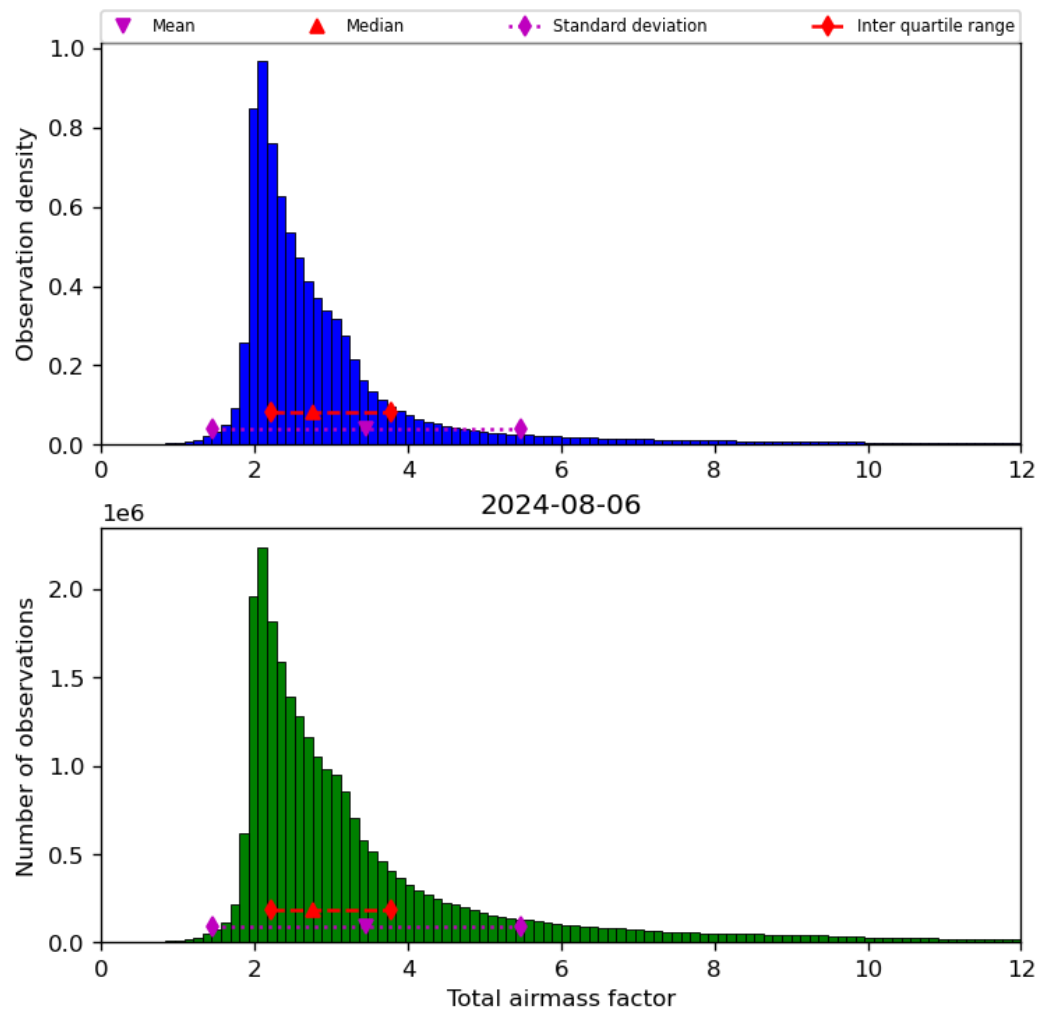
Figure 32: Histogram of “Total airmass factor” for 2024-08-06 to 2024-08-07
