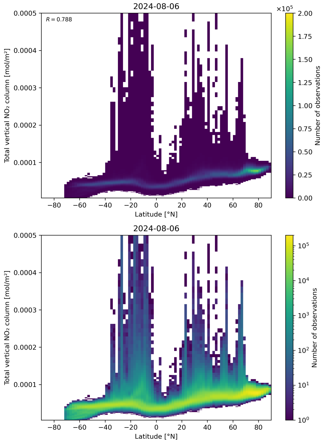
Figure 90: Scatter density plot of “Latitude” against “Total vertical NO 2 column” for 2024-08-06 to 2024-08-07.
