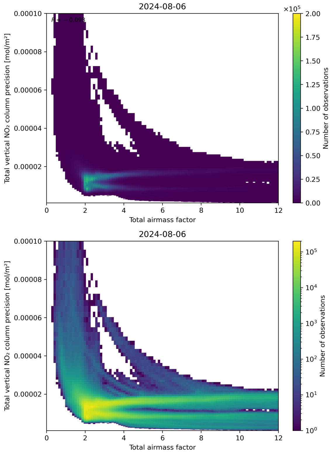
Figure 68: Scatter density plot of “Total airmass factor” against “Total vertical NO 2 column precision” for 2024-08-06 to 2024-08-07.
