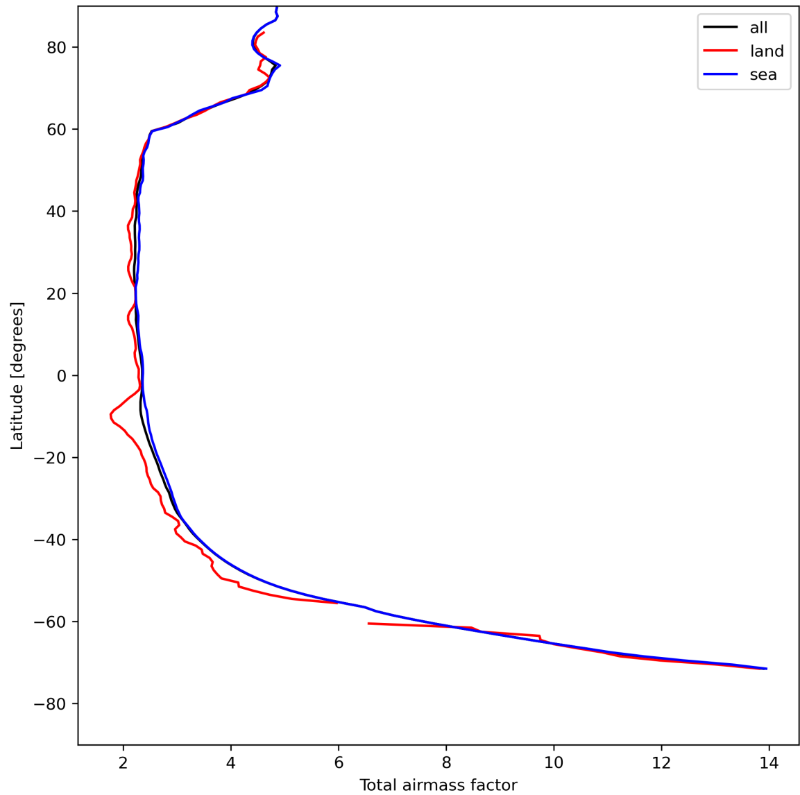
Figure 15: Zonal average of “Total airmass factor” for 2024-08-06 to 2024-08-07.
