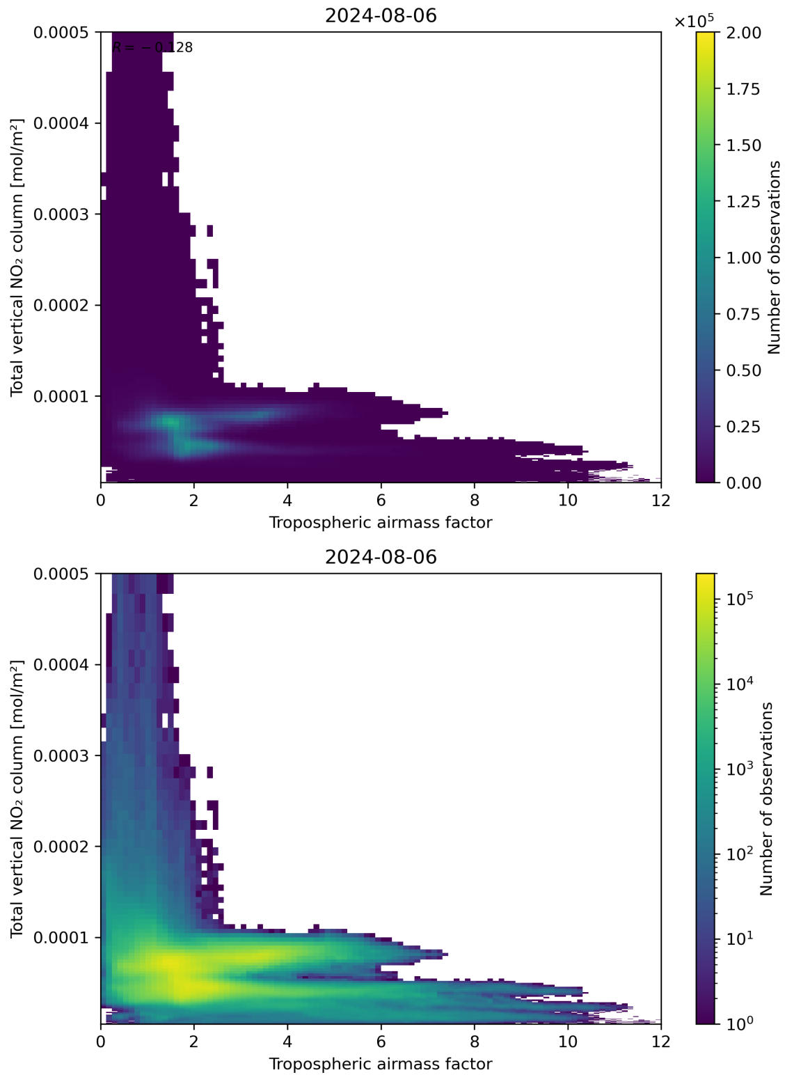
Figure 77: Scatter density plot of “Tropospheric airmass factor” against “Total vertical NO 2 column” for 2024-08-06 to 2024-08-07.
