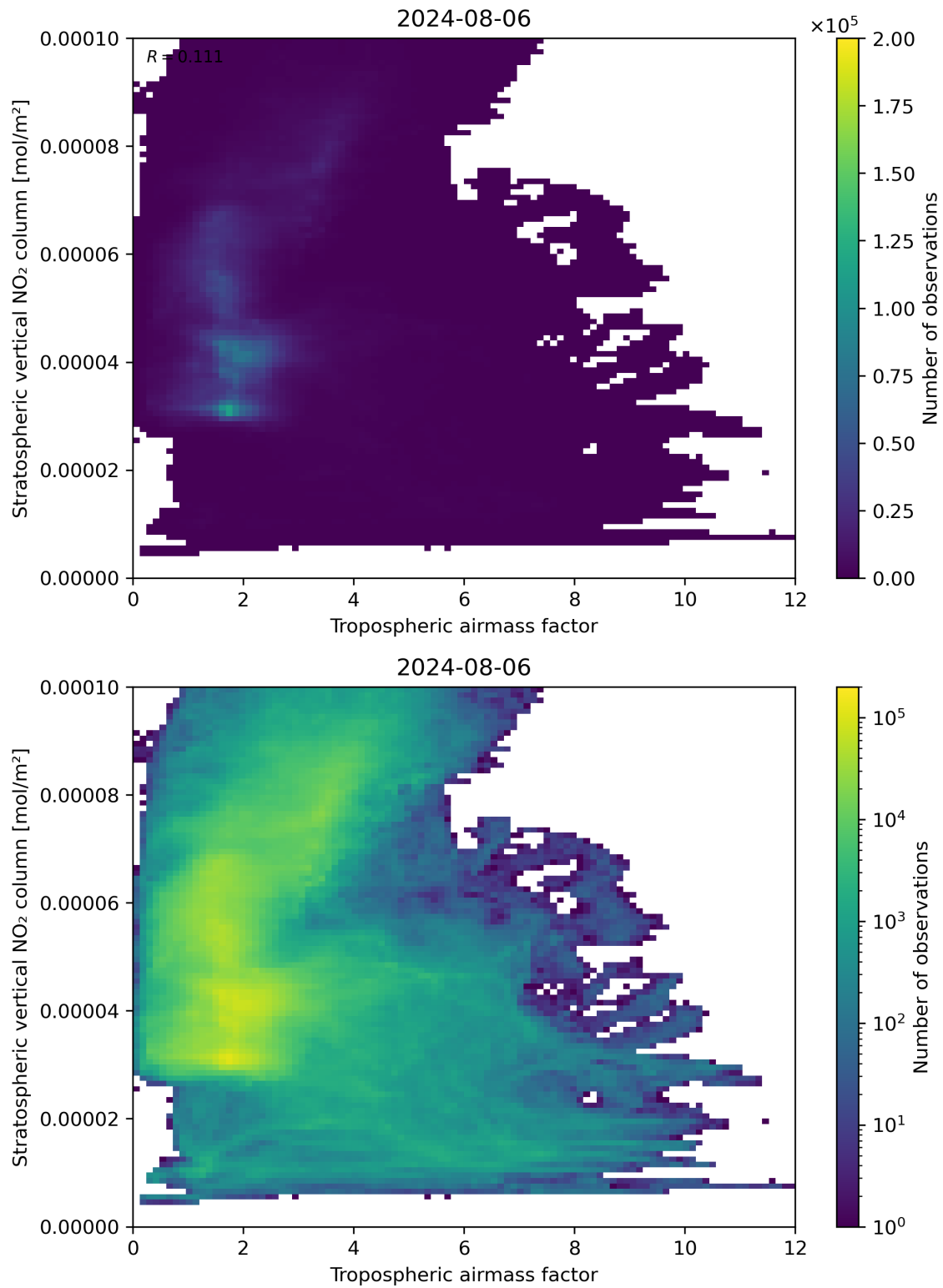
Figure 74: Scatter density plot of “Tropospheric air mass factor” against “Stratospheric vertical NO 2 column” for 2024-08-06 to 2024-08-07.
