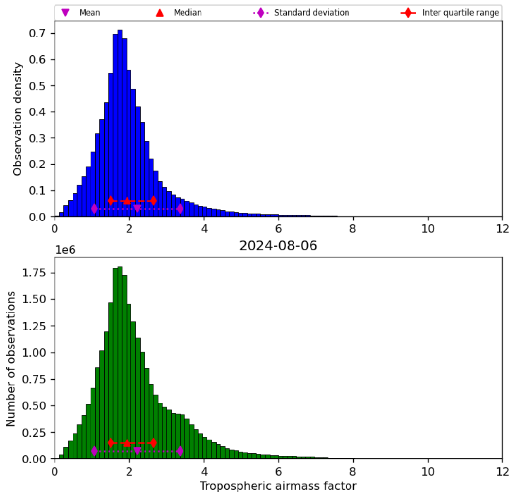
Figure 31: Histogram of “Tropospheric airmass factor” for 2024-08-06 to 2024-08-07
