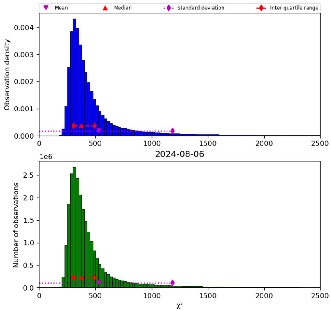
Figure 42: Histogram of " \chi^2 " for 2024-08-06 to 2024-08-07
