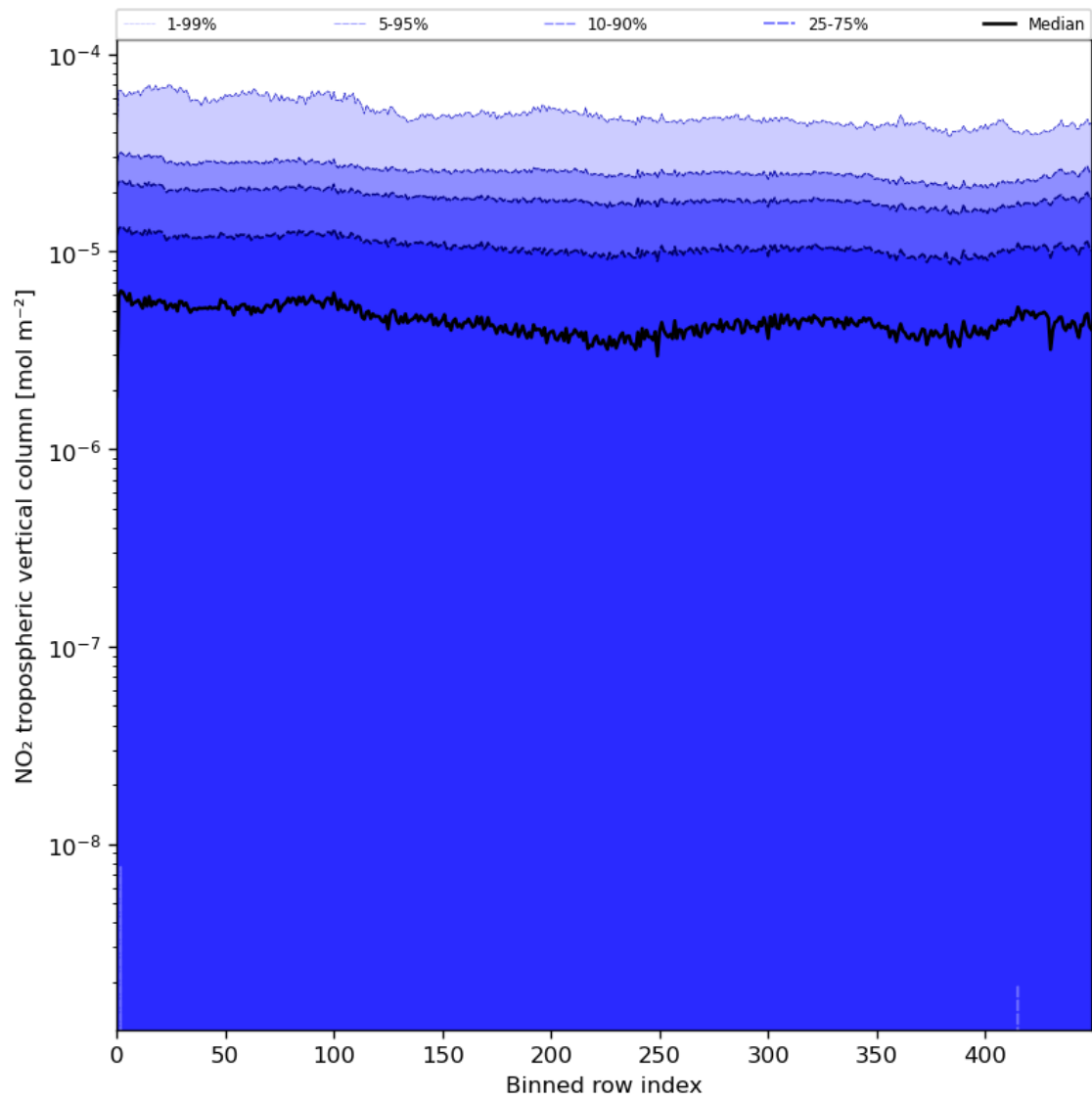
Figure 46: Along track statistics of “NO 2 tropospheric vertical column” for 2024-08-06 to 2024-08-07
