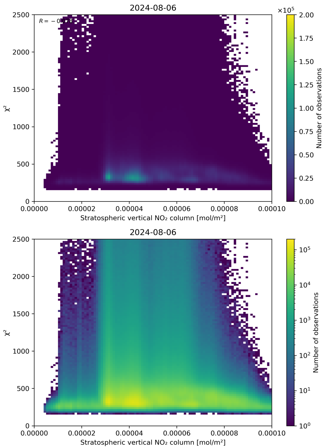
Figure 97: Scatter density plot of “Stratospheric vertical NO 2 column” against “ \chi^2 ” for 2024-08-06 to 2024-08-07.
