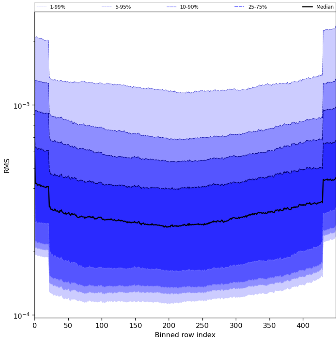
Figure 60: Along track statistics of “RMS” for 2024-08-06 to 2024-08-07
