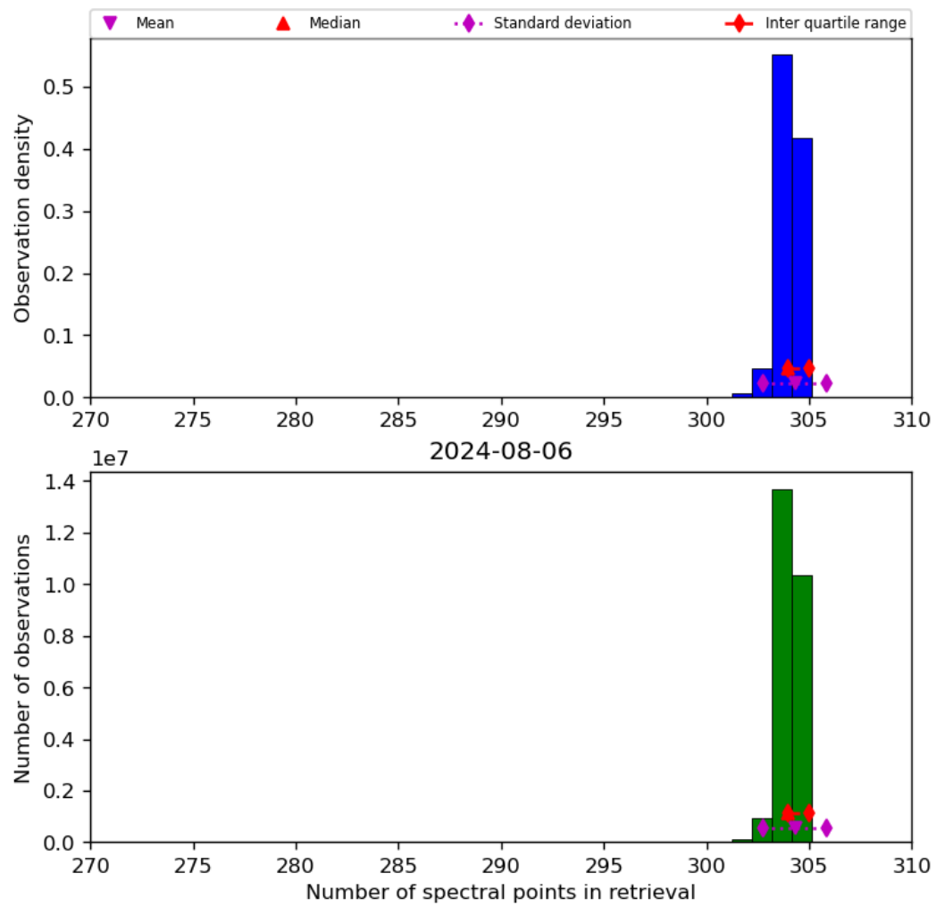
Figure 33: Histogram of “Number of spectral points in retrieval” for 2024-08-06 to 2024-08-07
