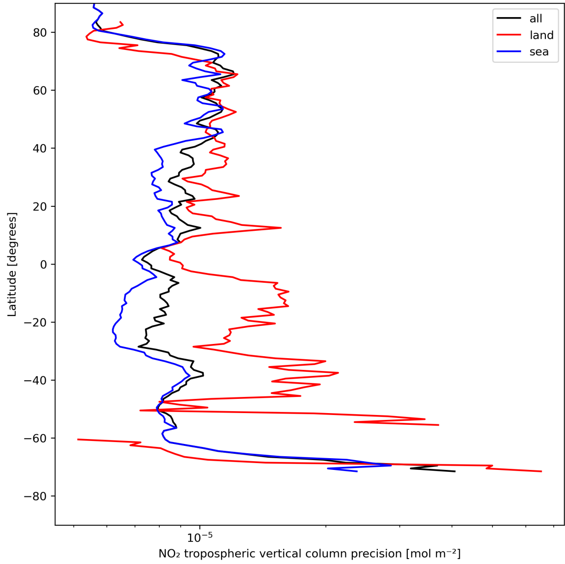
Figure 13: Zonal average of “NO 2 tropospheric vertical column precision” for 2024-08-06 to 2024-08-07.
