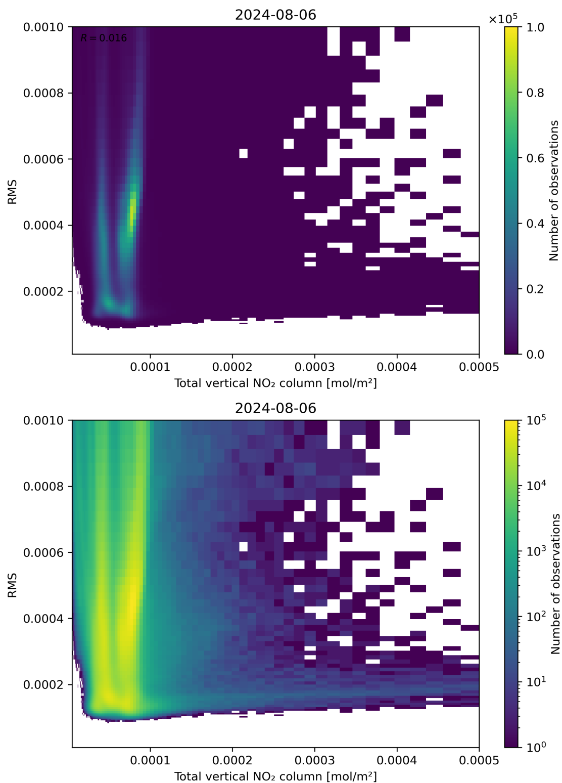
Figure 120: Scatter density plot of “Total vertical NO 2 column” against “RMS” for 2024-08-06 to 2024-08-07.
