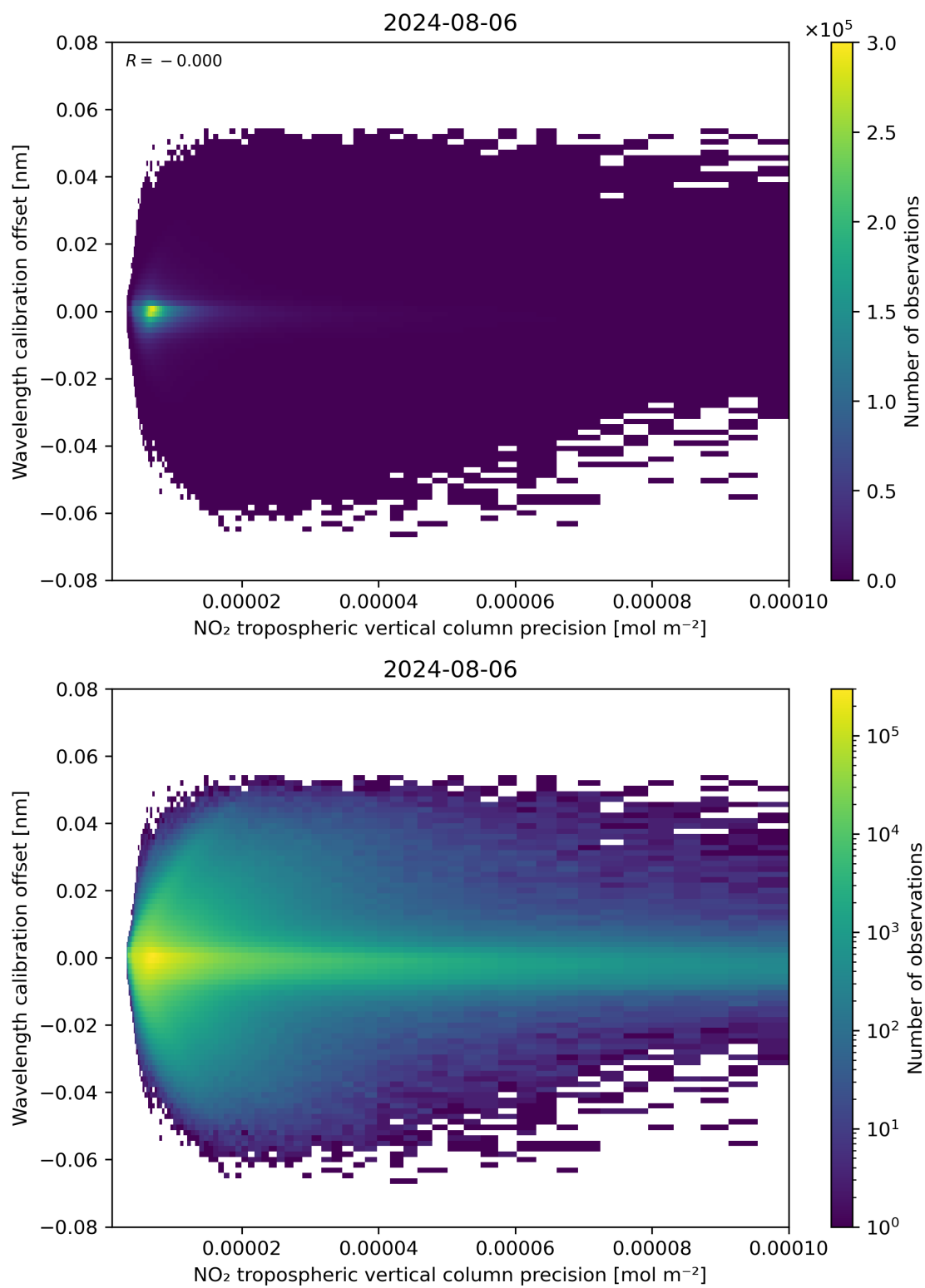
Figure 141: Scatter density plot of “NO 2 tropospheric vertical column precision” against “Wavelength calibration offset” for 2024-08-06 to 2024-08-07.
