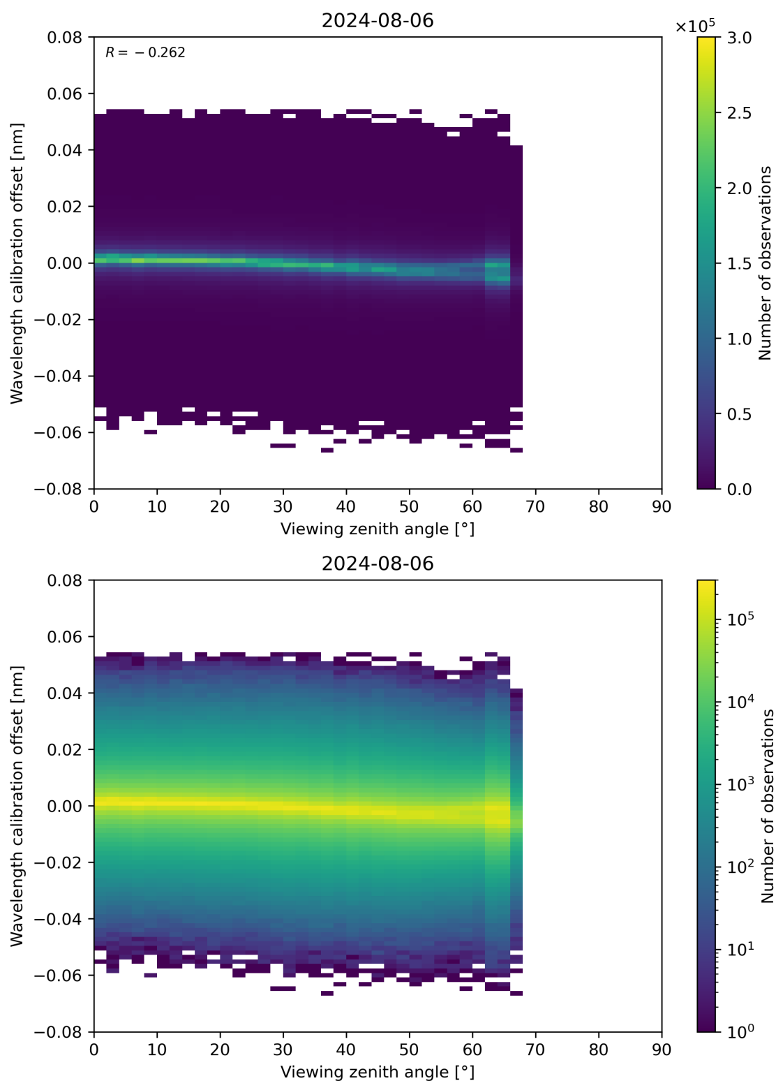
Figure 173: Scatter density plot of “Viewing zenith angle” against “Wavelength calibration offset” for 2024-08-06 to 2024-08-07.
