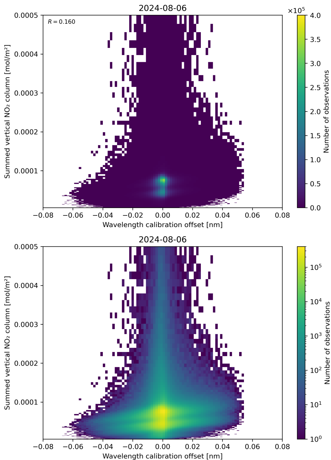
Figure 177: Scatter density plot of “Wavelength calibration offset” against “Summed vertical NO 2 column” for 2024-08-06 to 2024-08-07.
