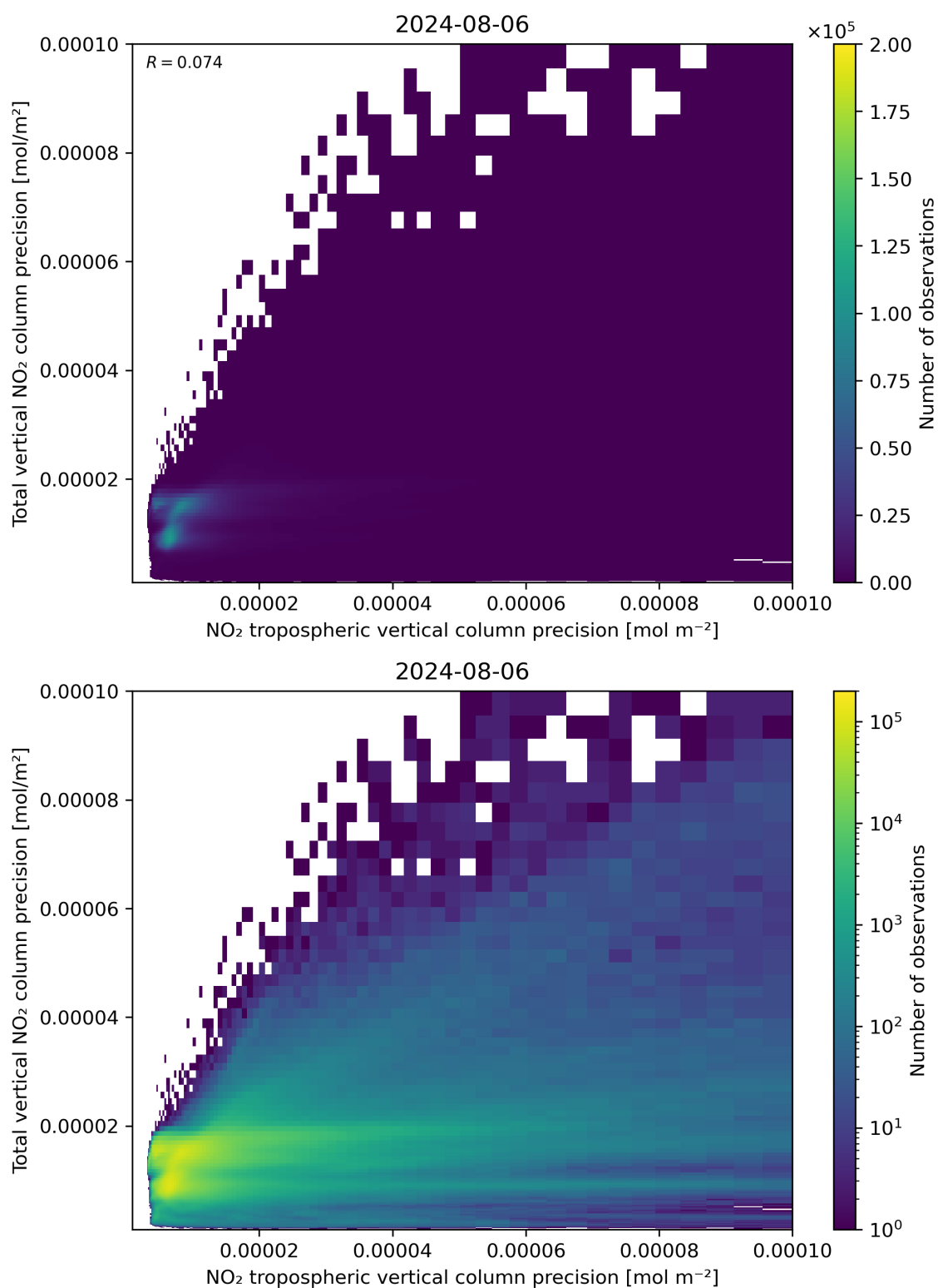
Figure 139: Scatter density plot of “NO 2 tropospheric vertical column precision” against “Total vertical NO 2 column precision” for 2024-08-06 to 2024-08-07.
