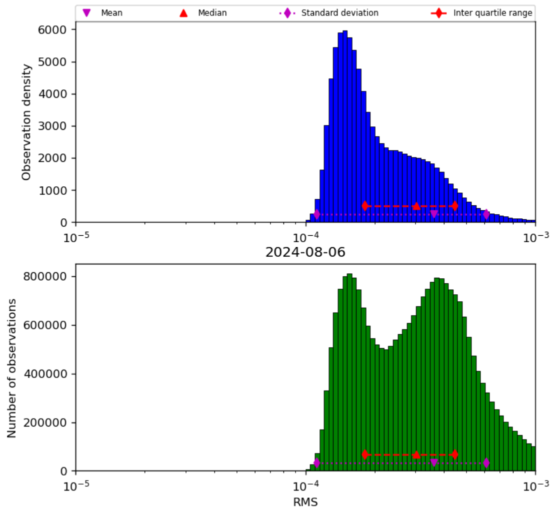
Figure 43: Histogram of “RMS” for 2024-08-06 to 2024-08-07
