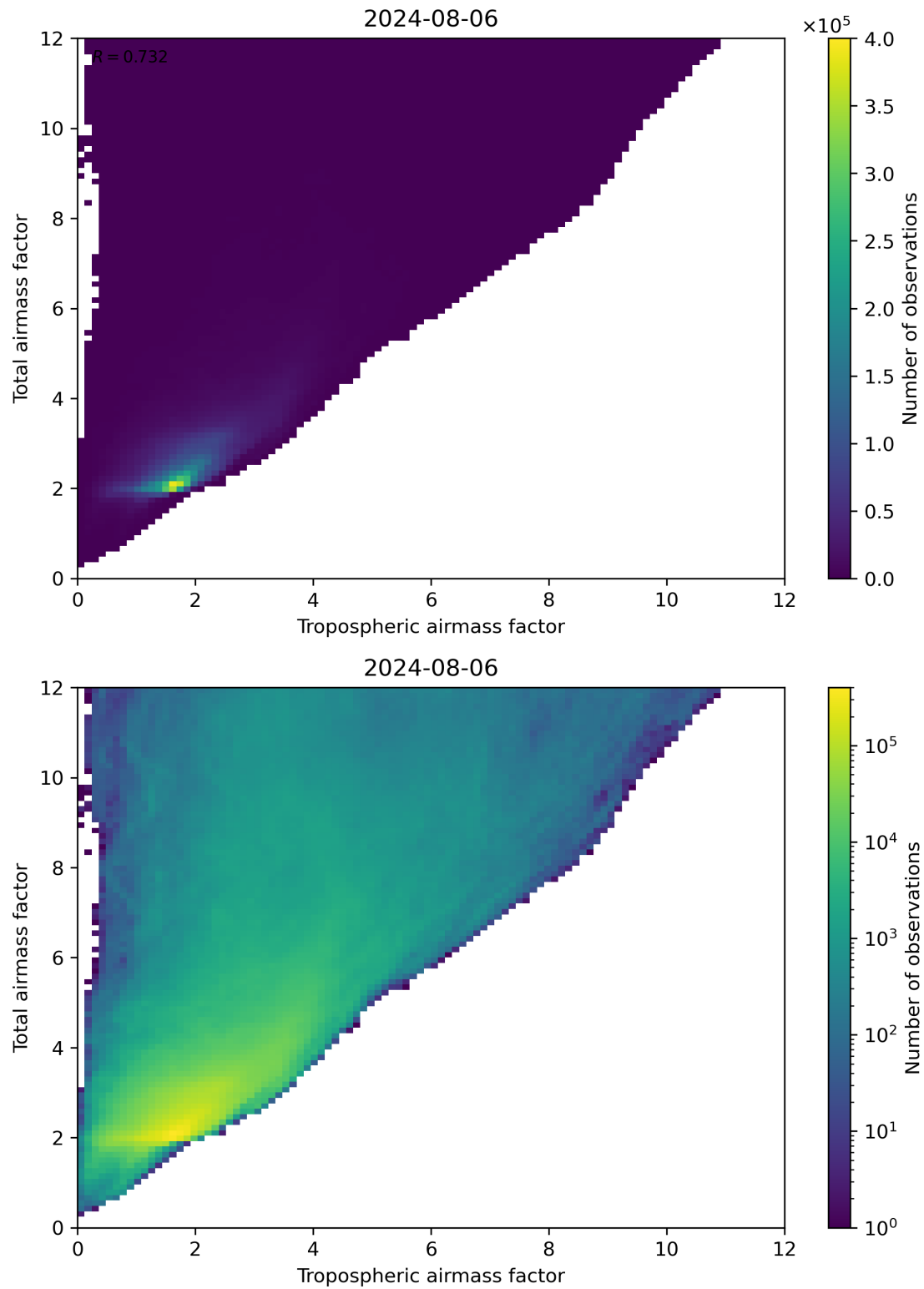
Figure 72: Scatter density plot of “Tropospheric airmass factor” against “Total airmass factor” for 2024-08-06 to 2024-08-07.
