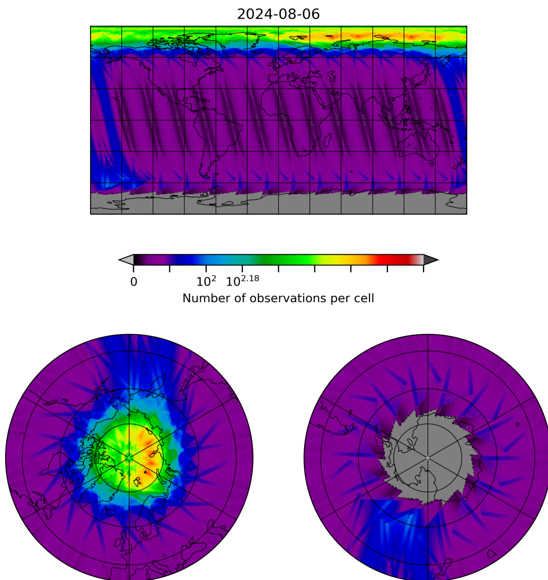
Figure 10: Map of the number of observations for 2024-08-06 to 2024-08-07
