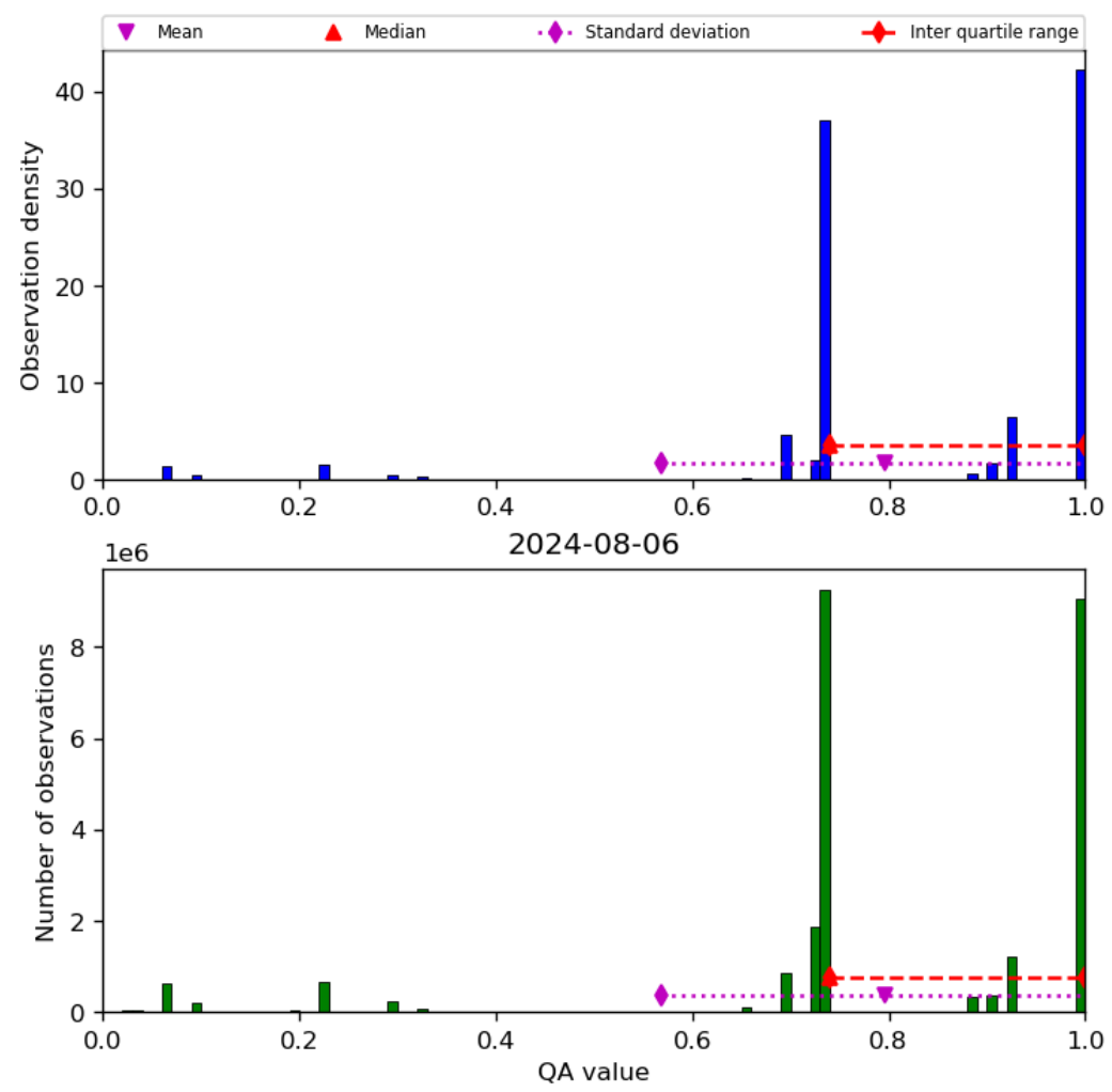
Figure 28: Histogram of “QA value” for 2024-08-06 to 2024-08-07
