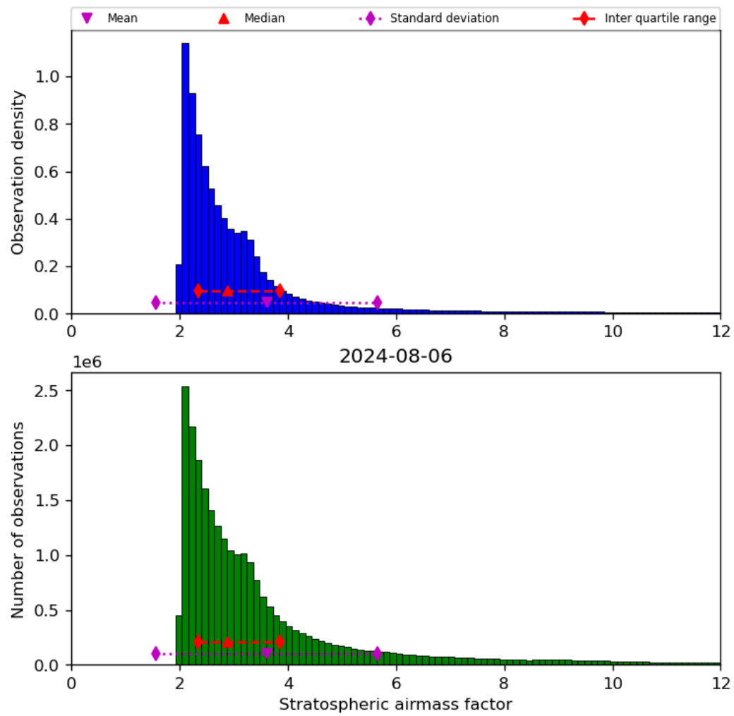
Figure 44: Histogram of “Stratospheric airmass factor” for 2024-08-06 to 2024-08-07
