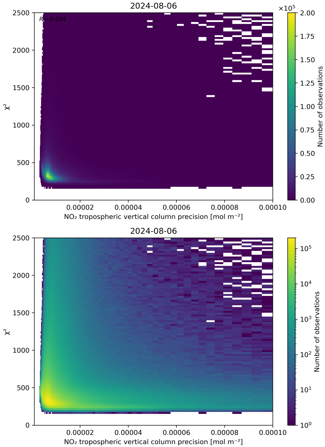
Figure 134: Scatter density plot of “NO 2 tropospheric vertical column precision” against “ \chi^2 ” for 2024-08-06 to 2024-08-07.
