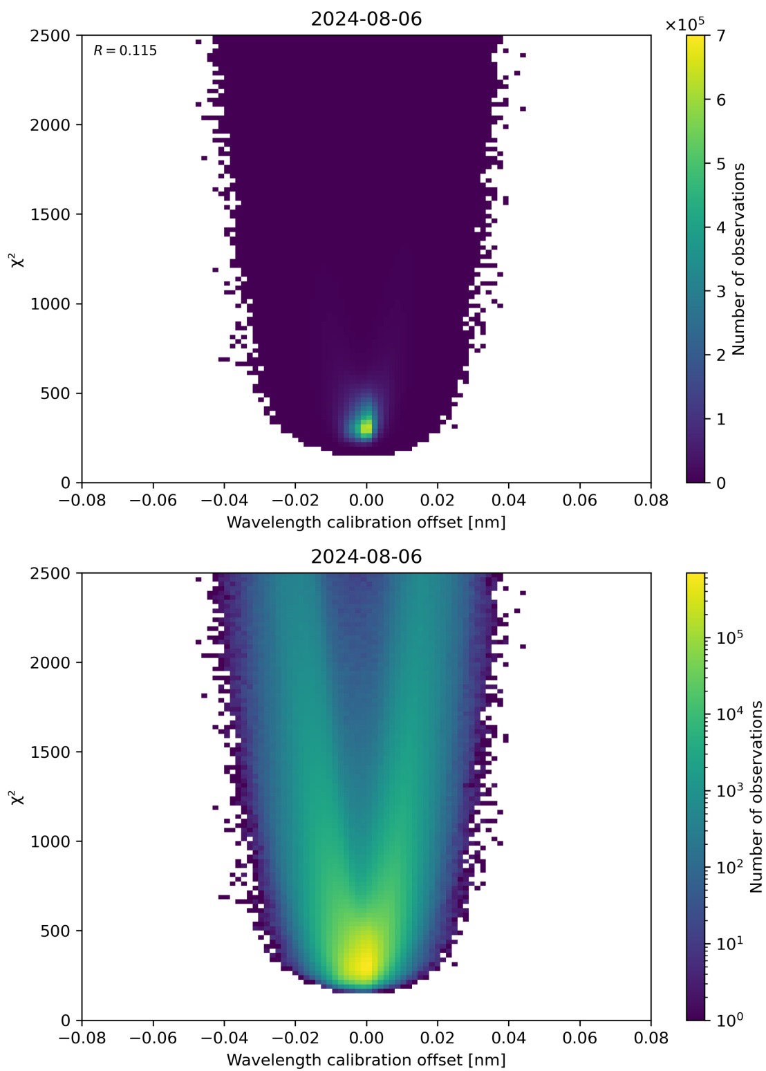
Figure 175: Scatter density plot of “Wavelength calibration offset” against “ \chi^2 ” for 2024-08-06 to 2024-08-07.
