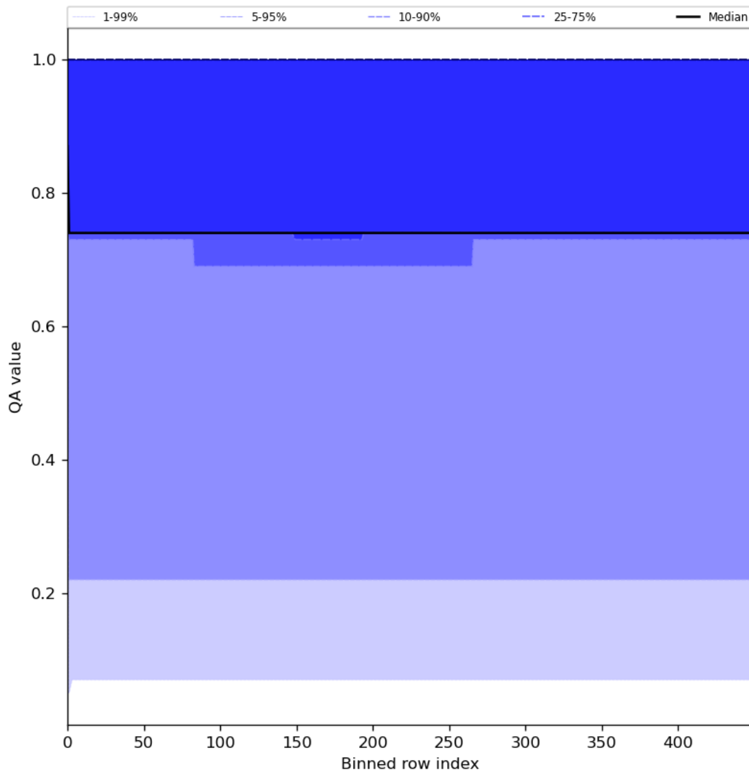
Figure 45: Along track statistics of “QA value” for 2024-08-06 to 2024-08-07
