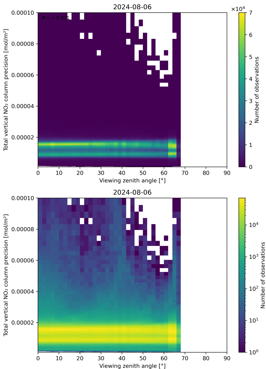
Figure 168: Scatter density plot of “Viewing zenith angle” against “Total vertical NO 2 column precision” for 2024-08-06 to 2024-08-07.
