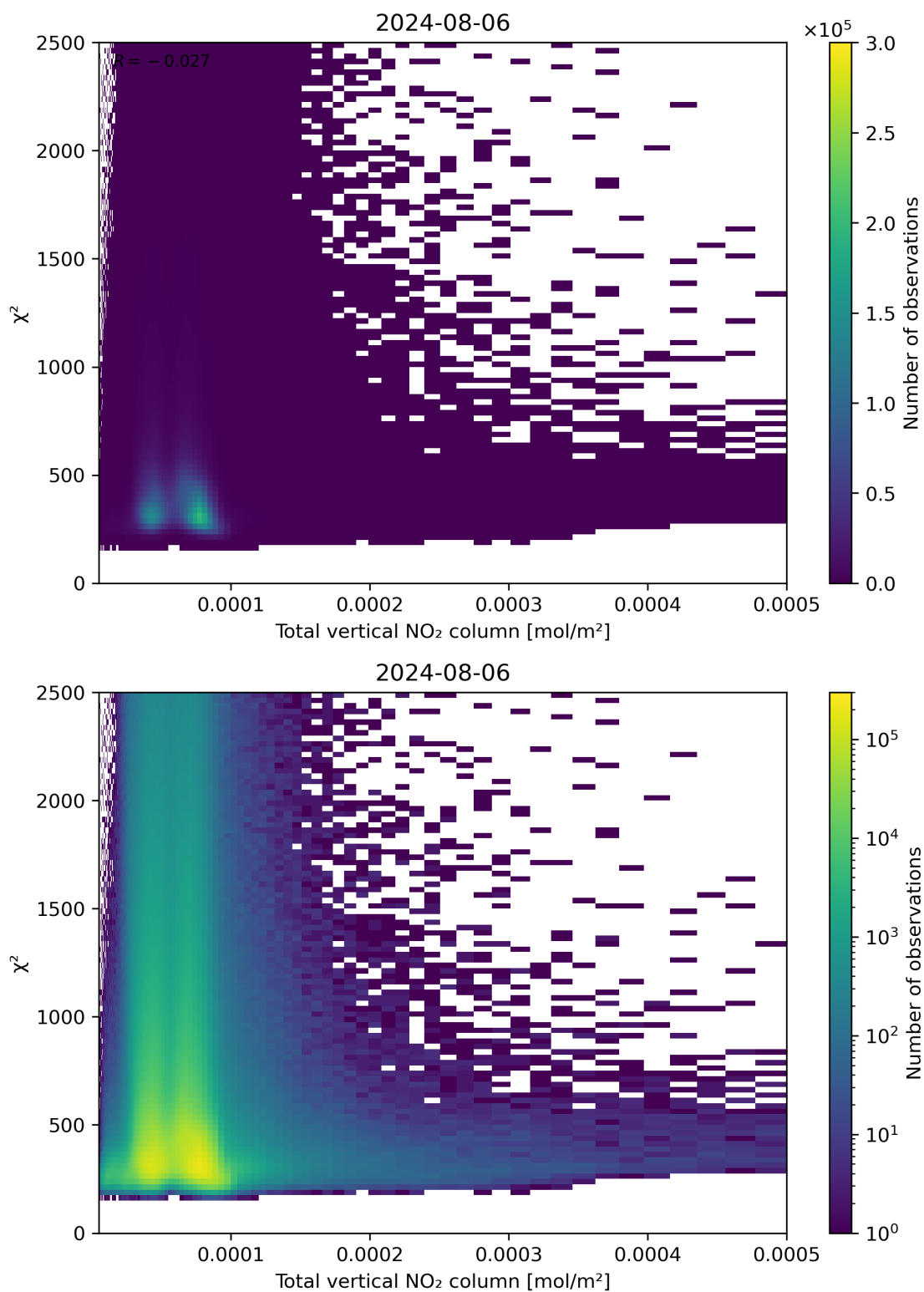
Figure 111: Scatter density plot of “Total vertical NO 2 column” against “ \chi^2 ” for 2024-08-06 to 2024-08-07.
