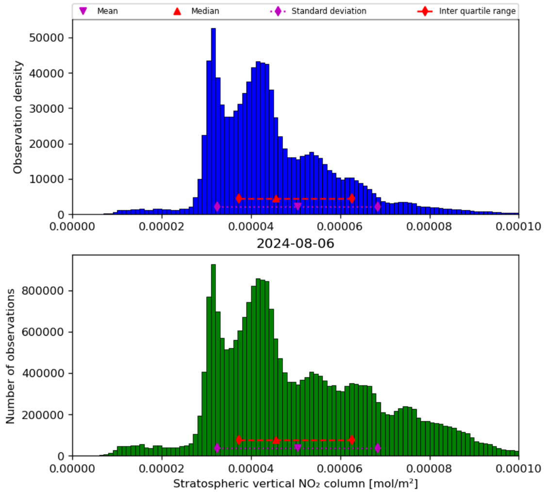
Figure 36: Histogram of “Stratospheric vertical NO 2 column” for 2024-08-06 to 2024-08-07
