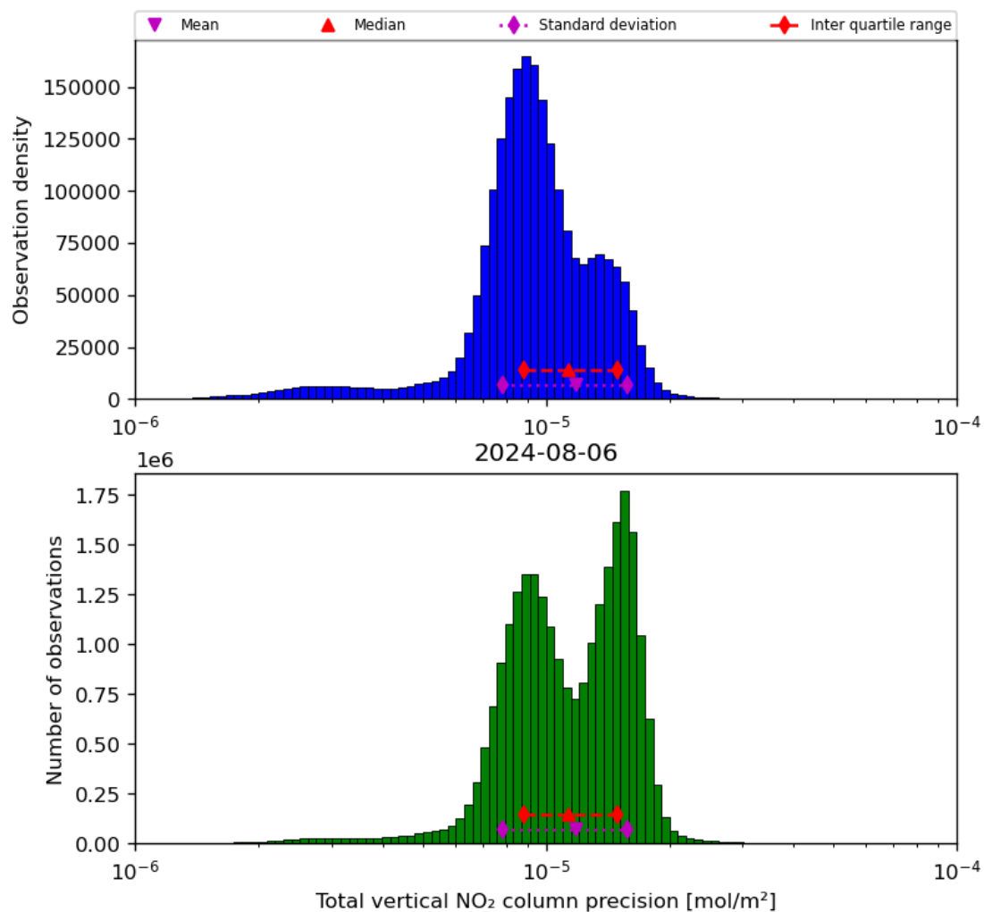
Figure 39: Histogram of “Total vertical NO 2 column precision” for 2024-08-06 to 2024-08-07
