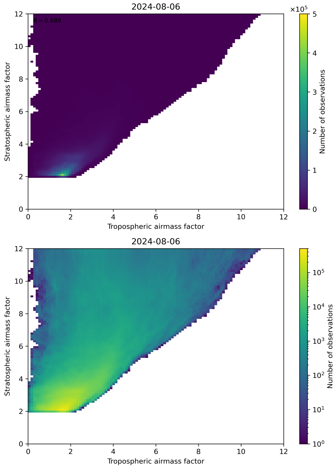
Figure 71: Scatter density plot of “Tropospheric airmass factor” against “Stratospheric airmass factor” for 2024-08-06 to 2024-08-07.
