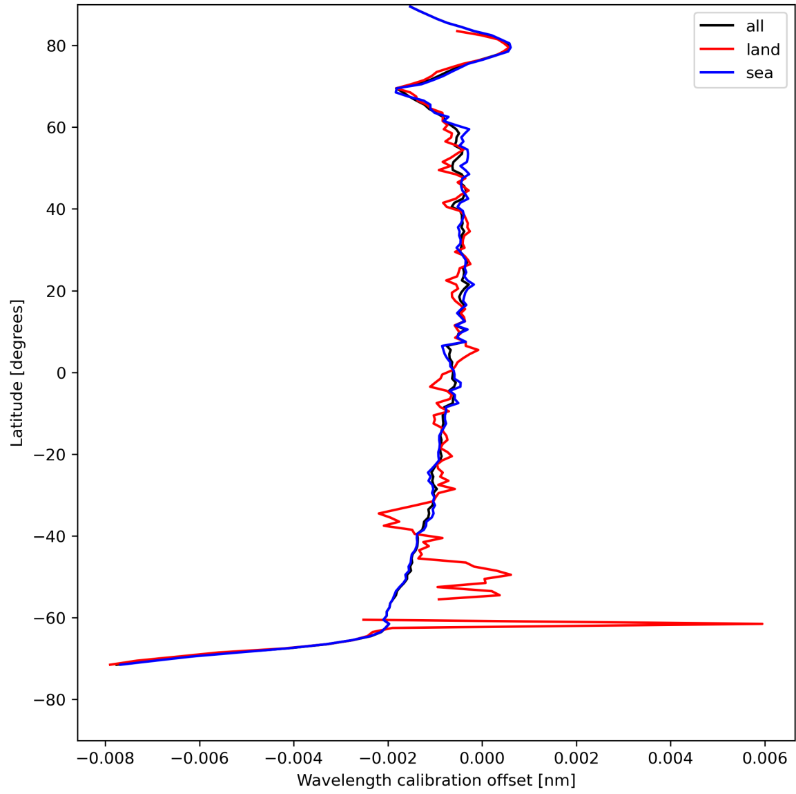
Figure 18: Zonal average of “Wavelength calibration offset” for 2024-08-06 to 2024-08-07.
