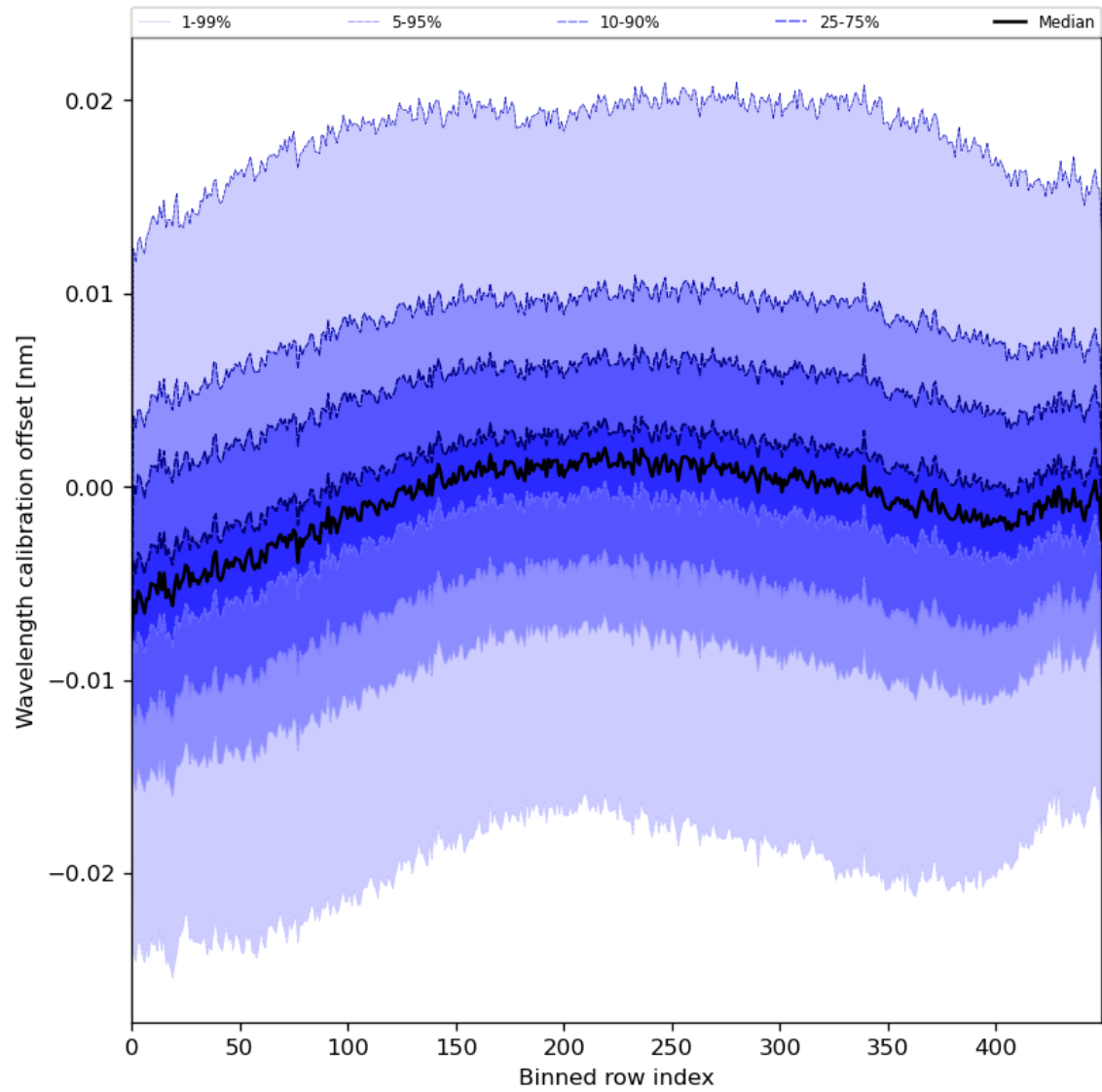
Figure 52: Along track statistics of “Wavelength calibration offset” for 2024-08-06 to 2024-08-07
