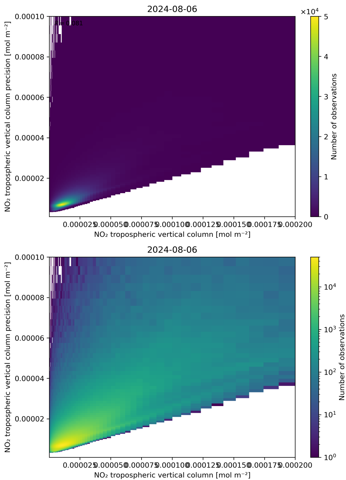
Figure 130: Scatter density plot of “NO 2 tropospheric vertical column” against “NO 2 tropospheric vertical column precision” for 2024-08-06 to 2024-08-07.
