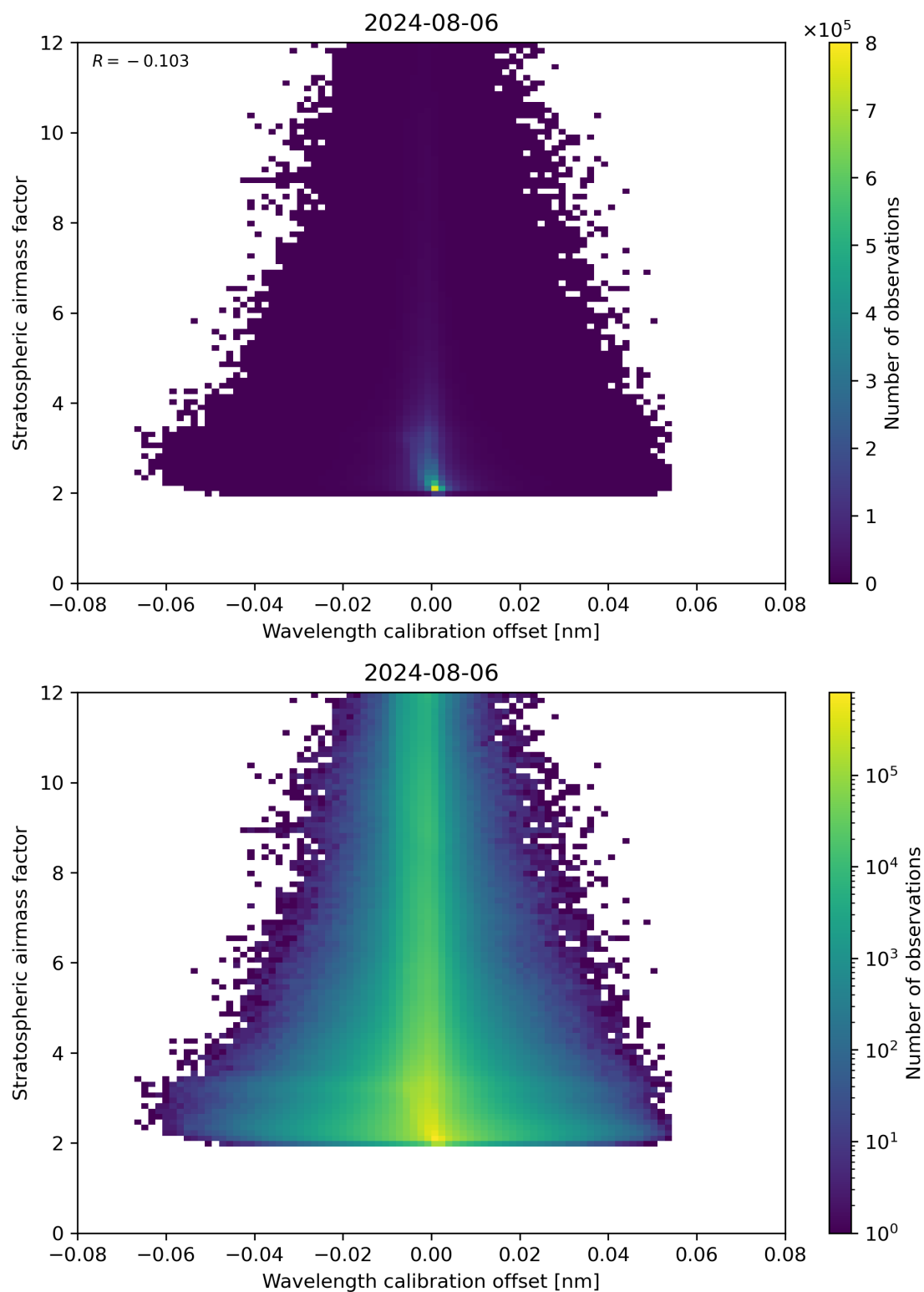
Figure 174: Scatter density plot of “Wavelength calibration offset” against “Stratospheric airmass factor” for 2024-08-06 to 2024-08-07.
