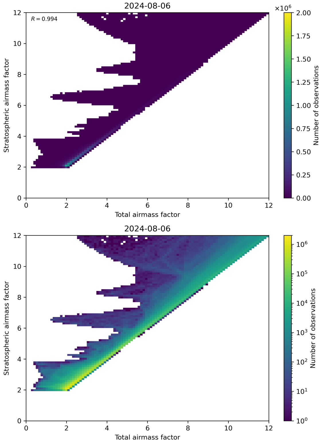
Figure 62: Scatter density plot of “Total airmass factor” against “Stratospheric airmass factor” for 2024-08-06 to 2024-08-07.
