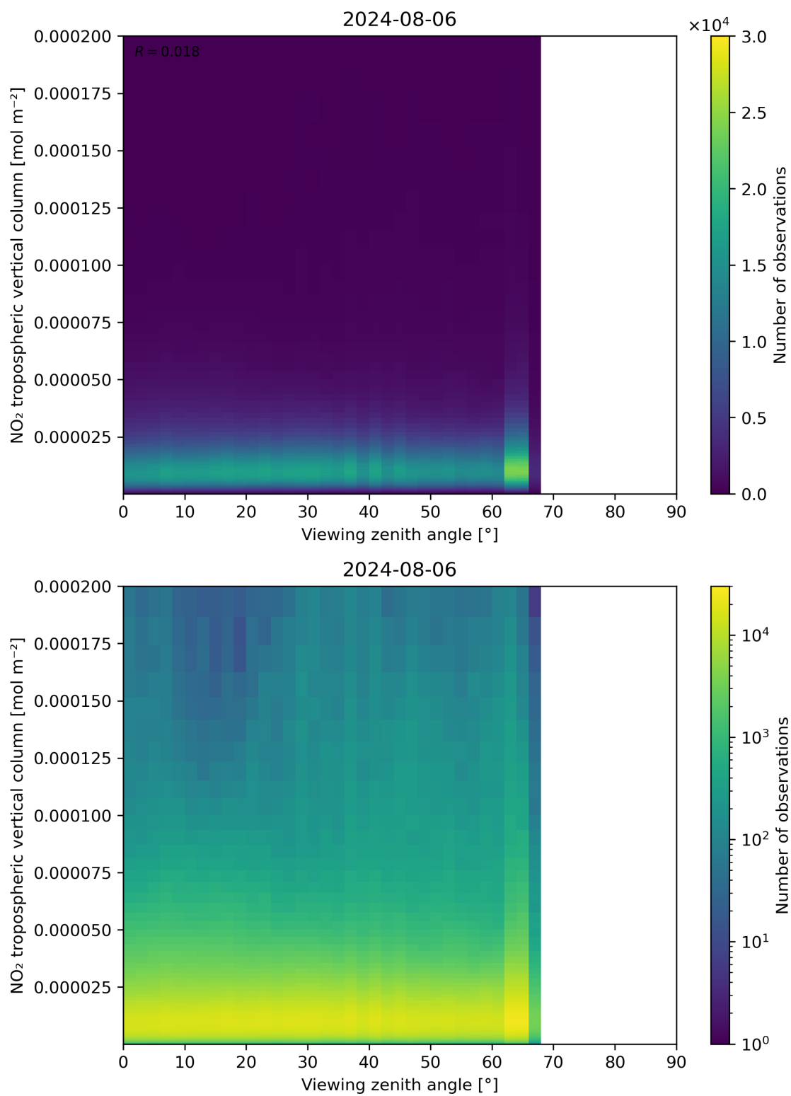
Figure 169: Scatter density plot of “Viewing zenith angle” against “NO 2 tropospheric vertical column” for 2024-08-06 to 2024-08-07.
