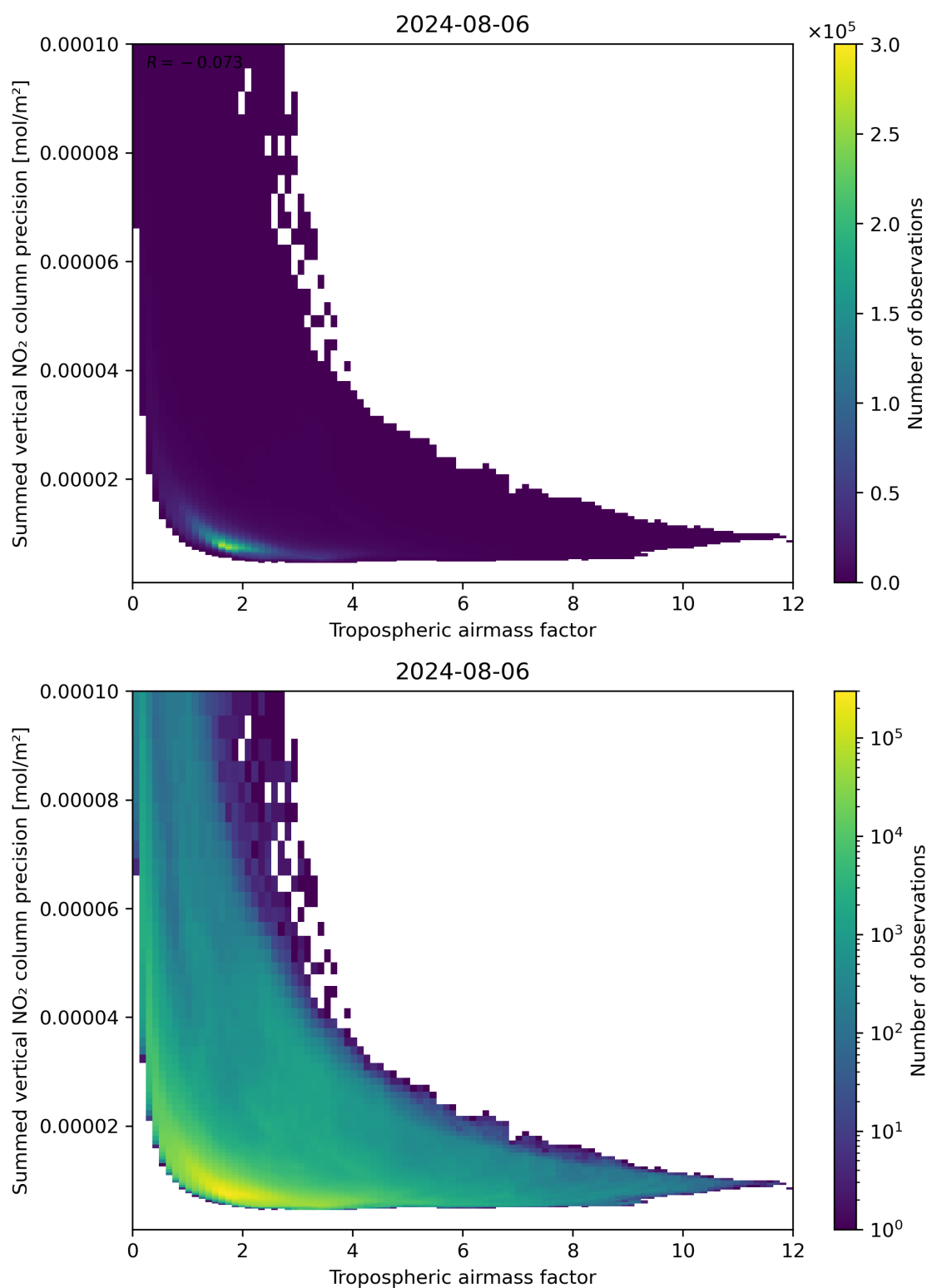
Figure 76: Scatter density plot of “Tropospheric air mass factor” against “Summed vertical NO 2 column precision” for 2024-08-06 to 2024-08-07.
