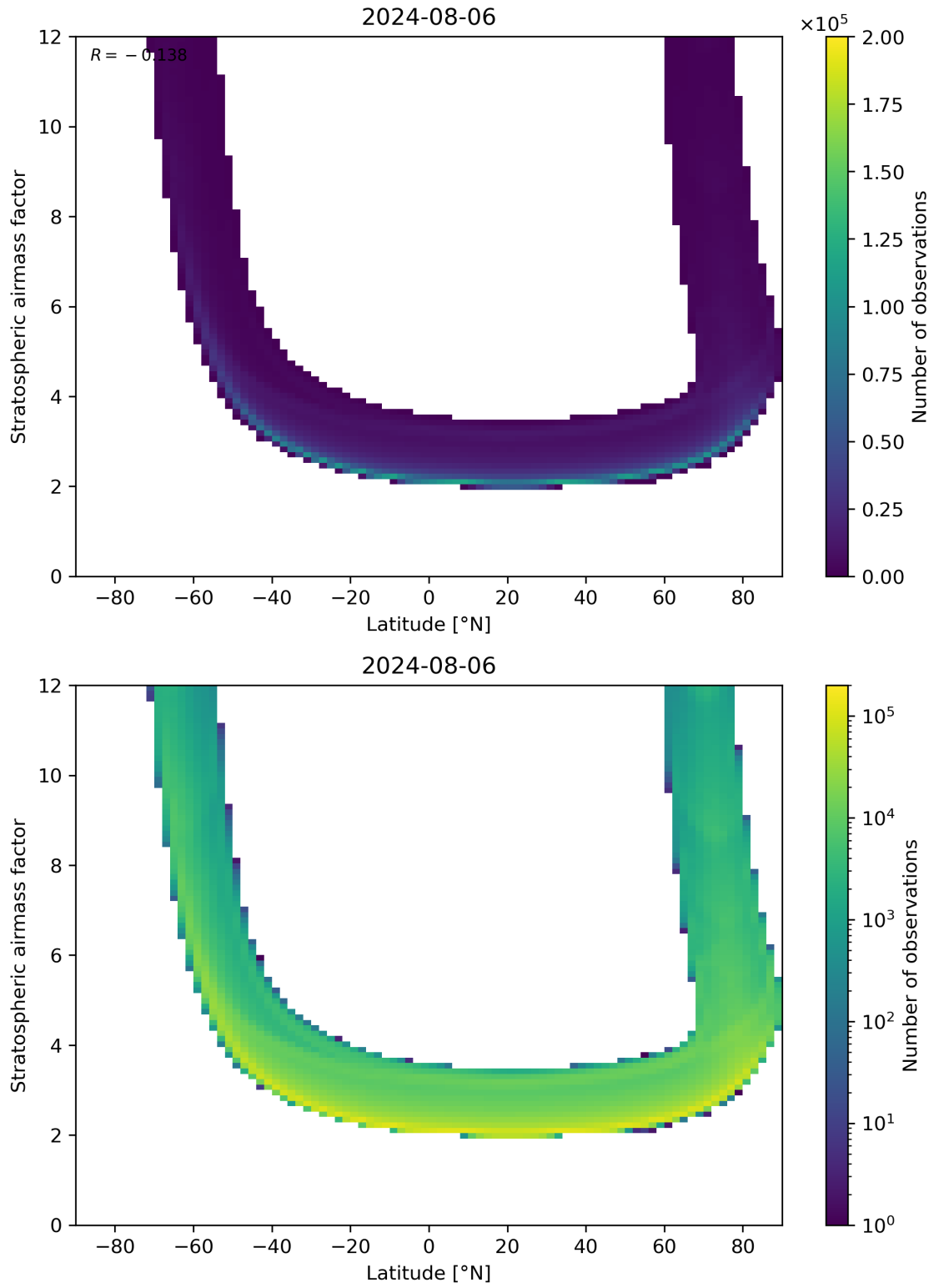
Figure 83: Scatter density plot of “Latitude” against “Stratospheric air mass factor” for 2024-08-06 to 2024-08-07.
