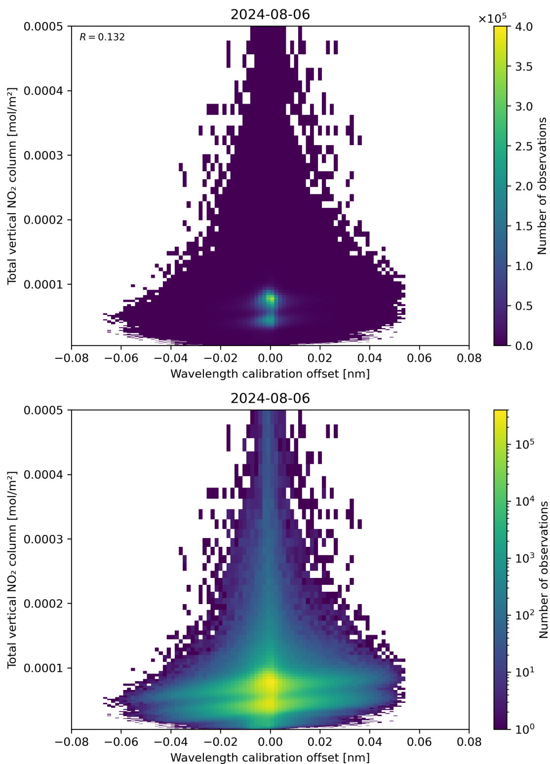
Figure 179: Scatter density plot of “Wavelength calibration offset” against “Total vertical NO 2 column” for 2024-08-06 to 2024-08-07.
