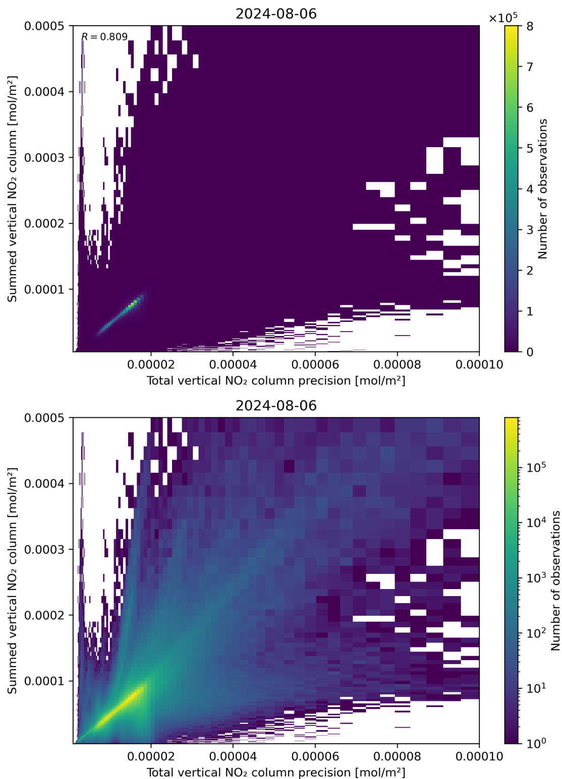
Figure 117: Scatter density plot of “Total vertical NO 2 column precision” against “Summed vertical NO 2 column” for 2024-08-06 to 2024-08-07.
