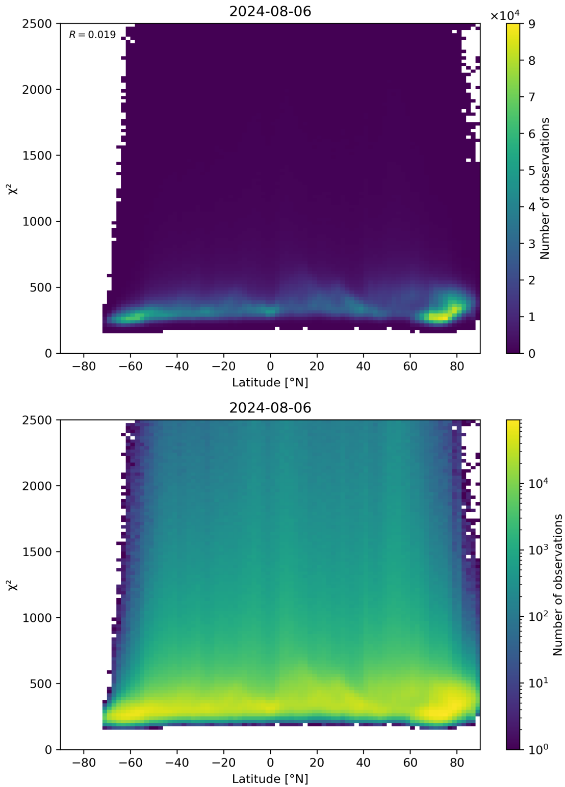
Figure 86: Scatter density plot of “Latitude” against “ \chi^2 ” for 2024-08-06 to 2024-08-07.
