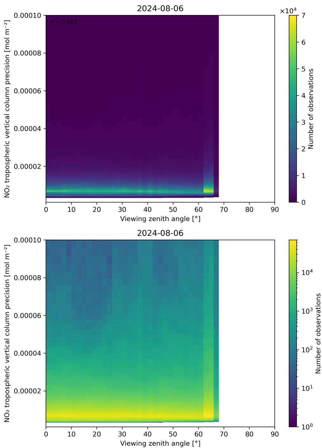
Figure 170: Scatter density plot of “Viewing zenith angle” against “NO 2 tropospheric vertical column precision” for 2024-08-06 to 2024-08-07.
