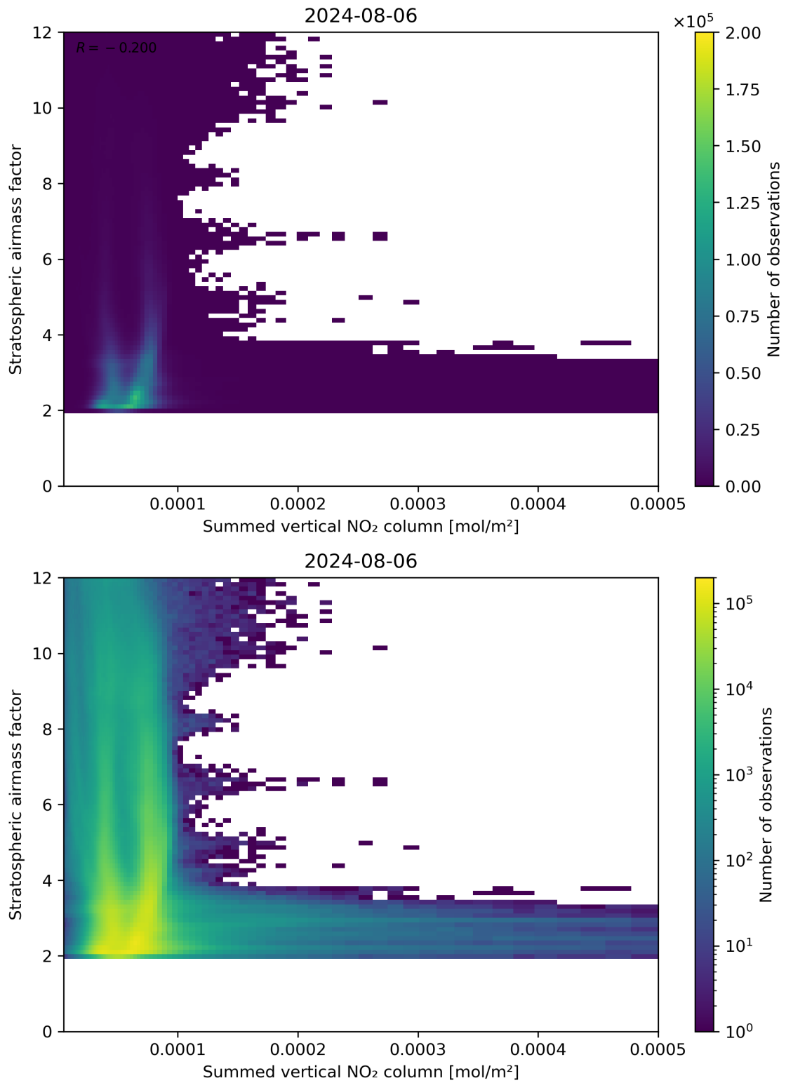
Figure 103: Scatter density plot of “Summed vertical NO 2 column” against “Stratospheric air mass factor” for 2024-08-06 to 2024-08-07.
