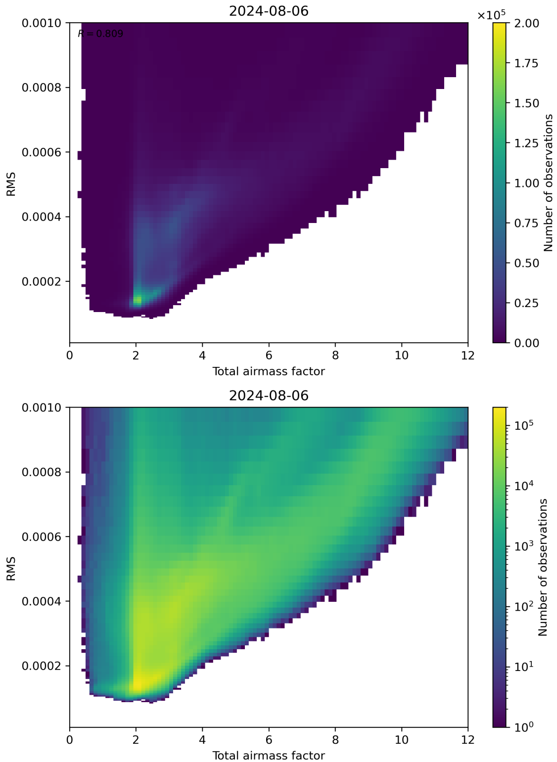
Figure 69: Scatter density plot of “Total airmass factor” against “RMS” for 2024-08-06 to 2024-08-07.
