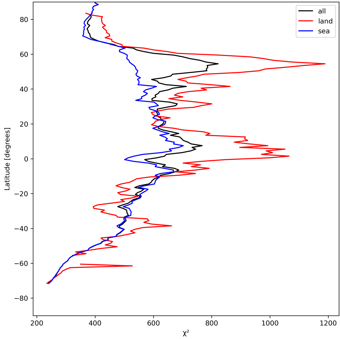
Figure 25: Zonal average of “ \chi^2 ” for 2024-08-06 to 2024-08-07.
