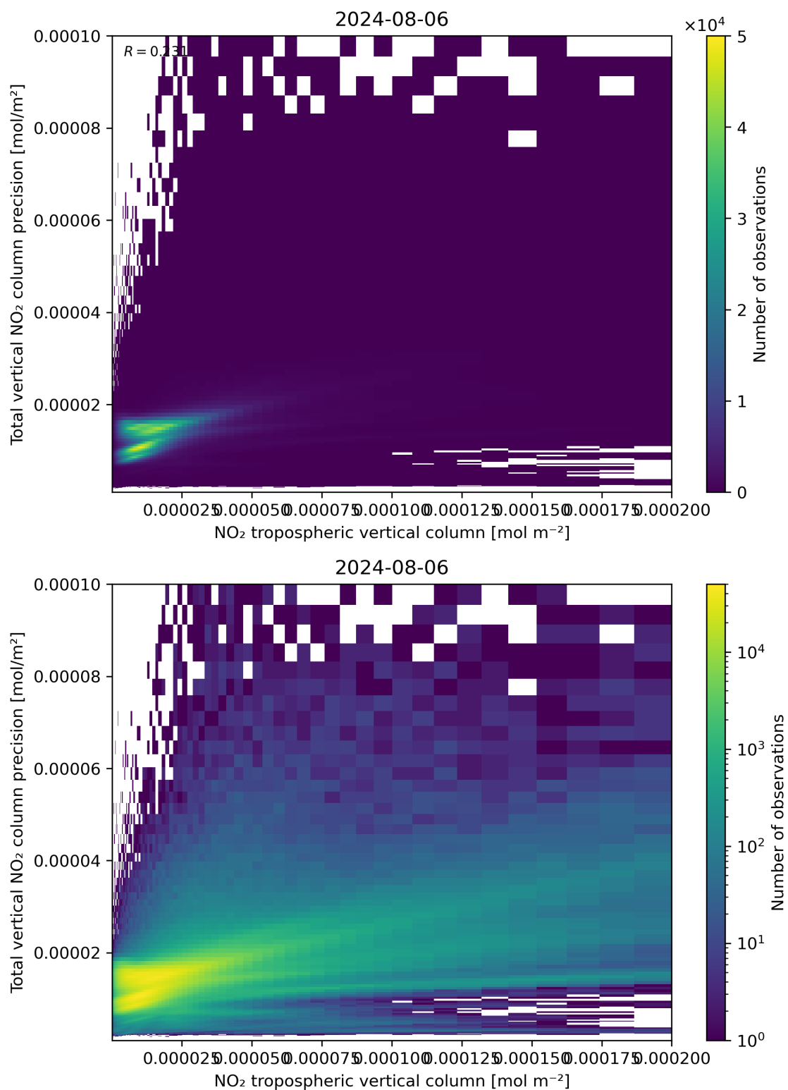
Figure 129: Scatter density plot of “NO 2 tropospheric vertical column” against “Total vertical NO 2 column precision” for 2024-08-06 to 2024-08-07.
