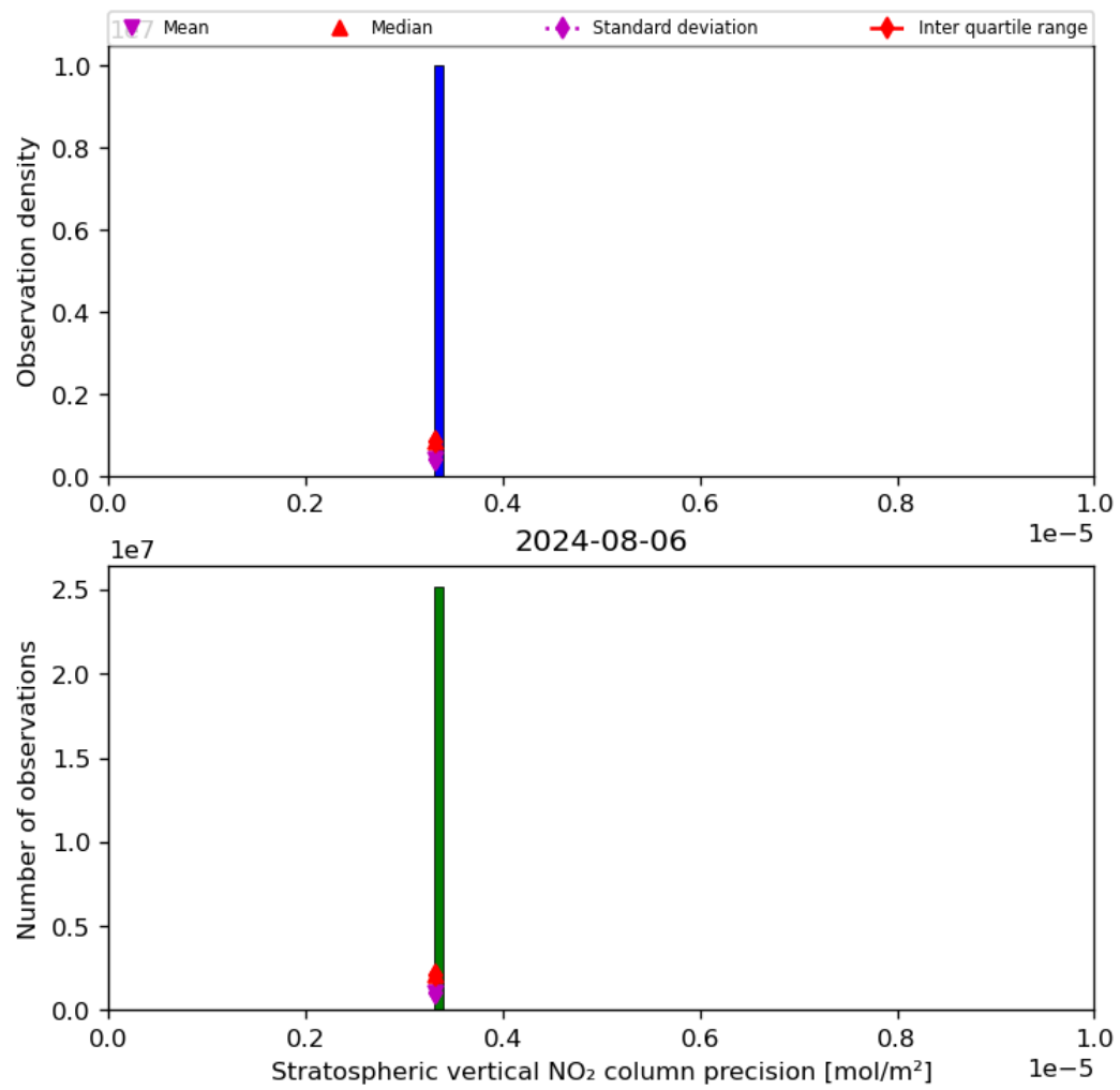
Figure 37: Histogram of “Stratospheric vertical NO 2 column precision” for 2024-08-06 to 2024-08-07
