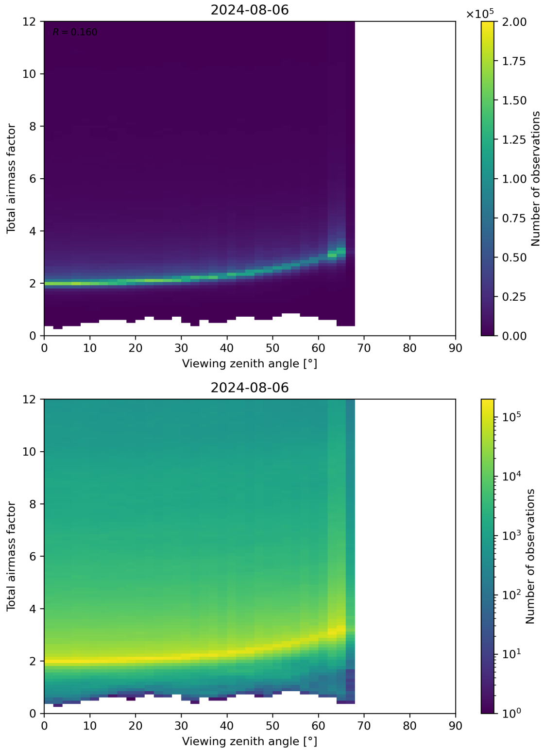
Figure 160: Scatter density plot of “Viewing zenith angle” against “Total airmass factor” for 2024-08-06 to 2024-08-07.
