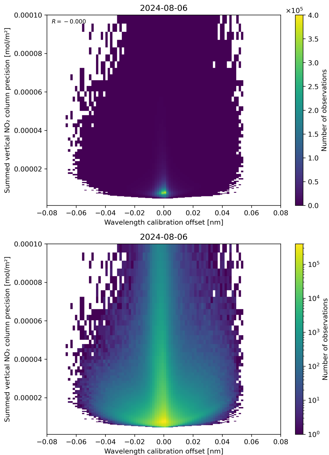
Figure 178: Scatter density plot of “Wavelength calibration offset” against “Summed vertical NO 2 column precision” for 2024-08-06 to 2024-08-07.
