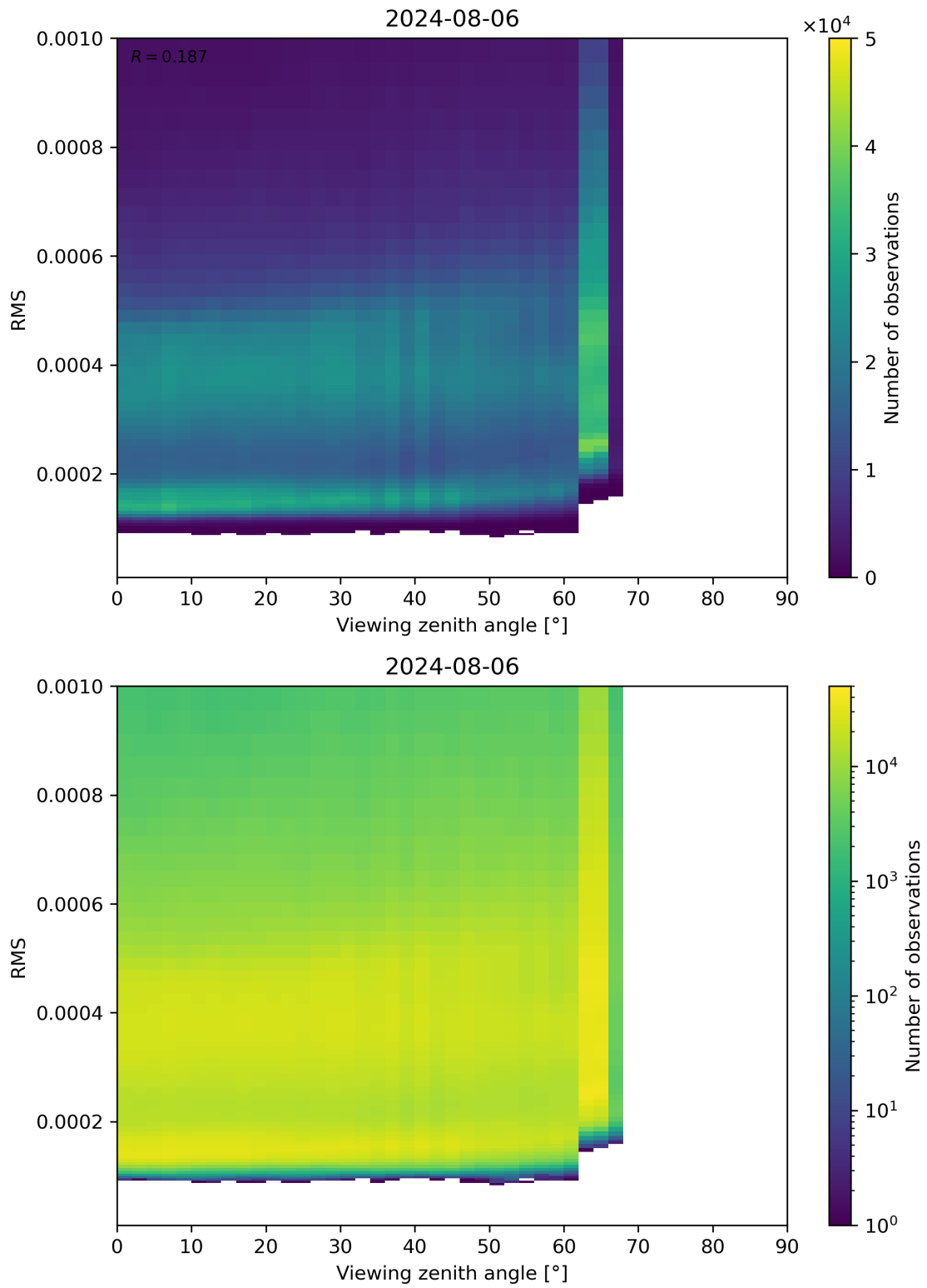
Figure 171: Scatter density plot of “Viewing zenith angle” against “RMS” for 2024-08-06 to 2024-08-07.
