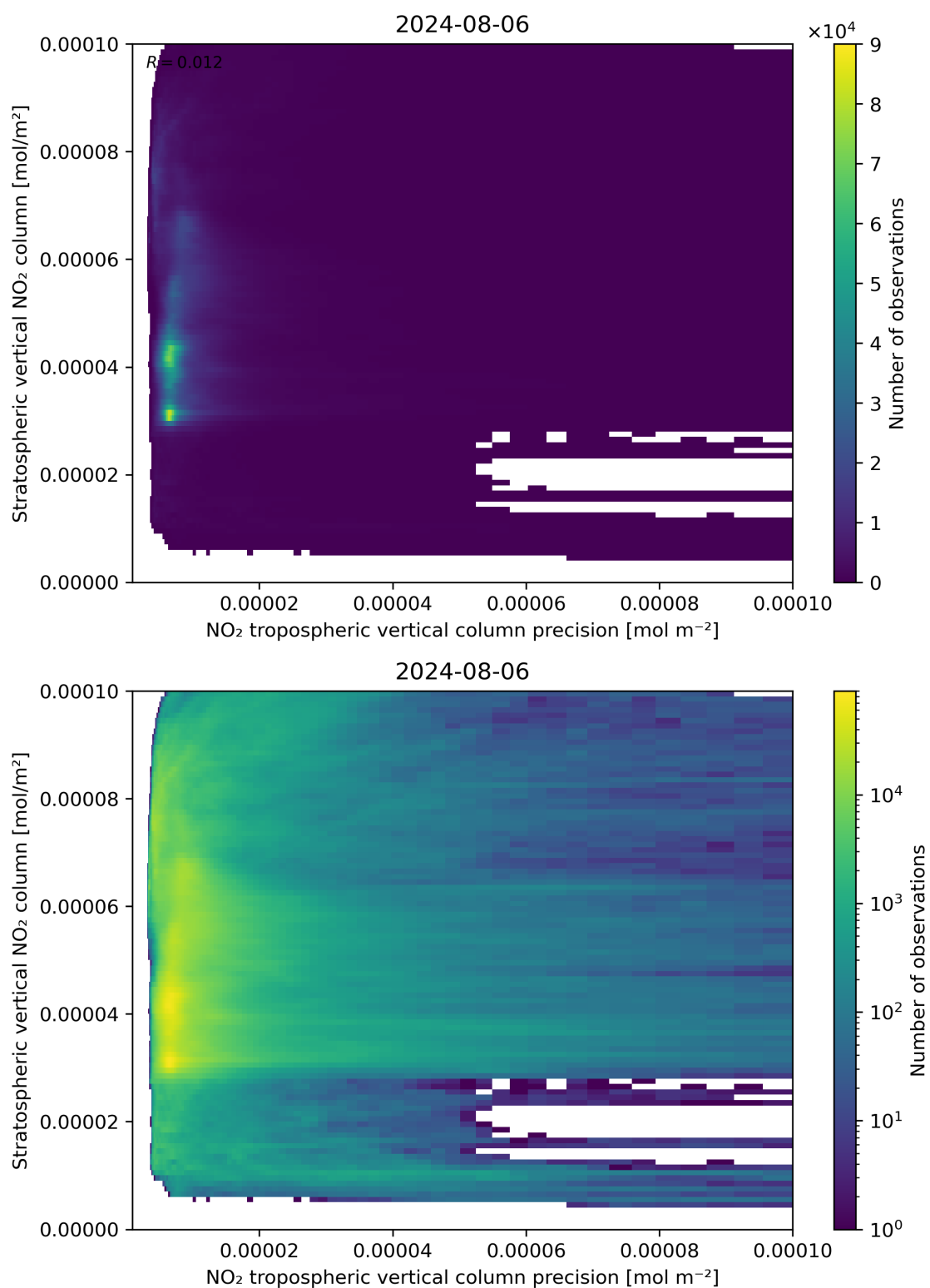
Figure 135: Scatter density plot of “NO 2 tropospheric vertical column precision” against “Stratospheric vertical NO 2 column” for 2024-08-06 to 2024-08-07.
