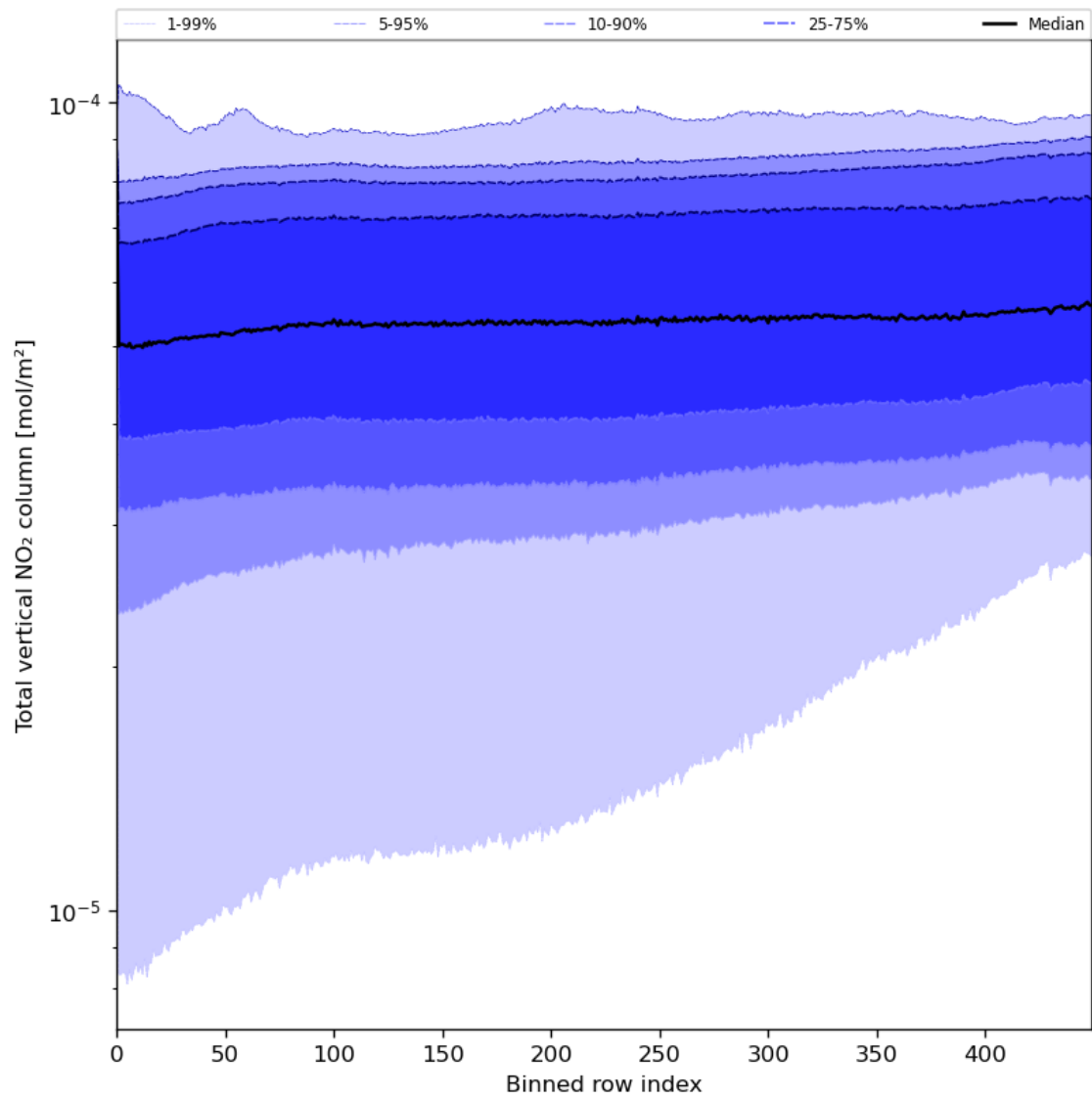
Figure 55: Along track statistics of "Total vertical NO 2 column" for 2024-08-06 to 2024-08-07
