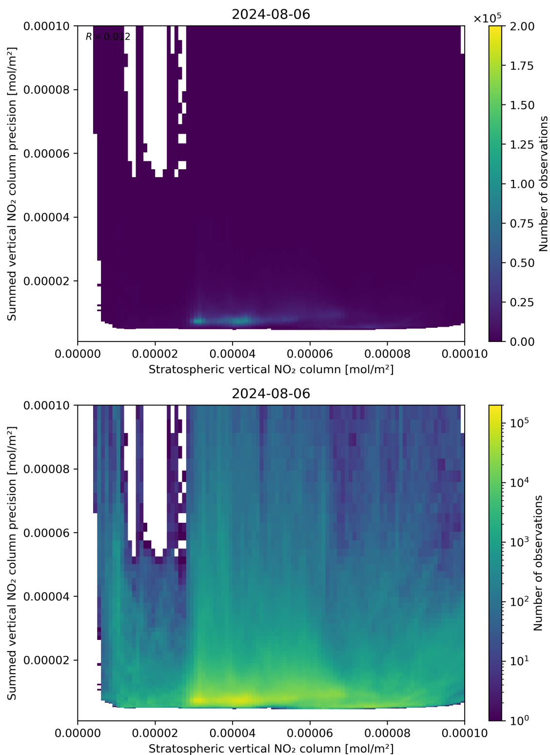
Figure 99: Scatter density plot of “Stratospheric vertical NO 2 column” against “Summed vertical NO 2 column precision” for 2024-08-06 to 2024-08-07.
