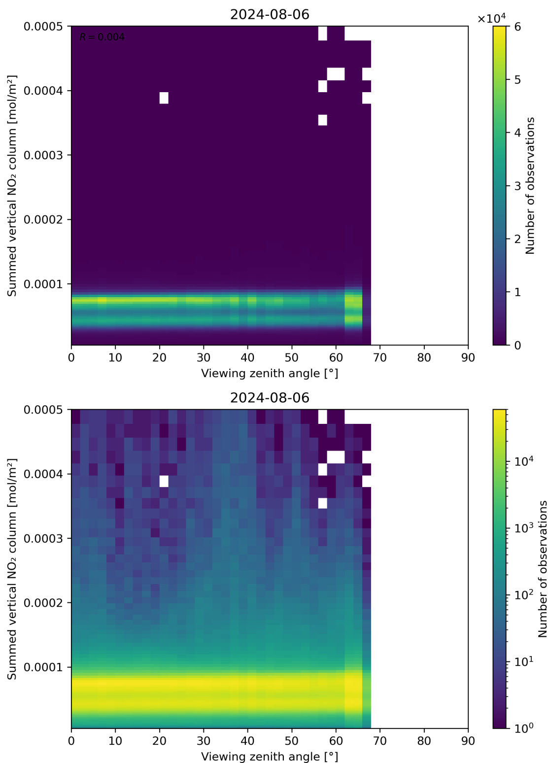
Figure 165: Scatter density plot of “Viewing zenith angle” against “Summed vertical NO 2 column” for 2024-08-06 to 2024-08-07.
