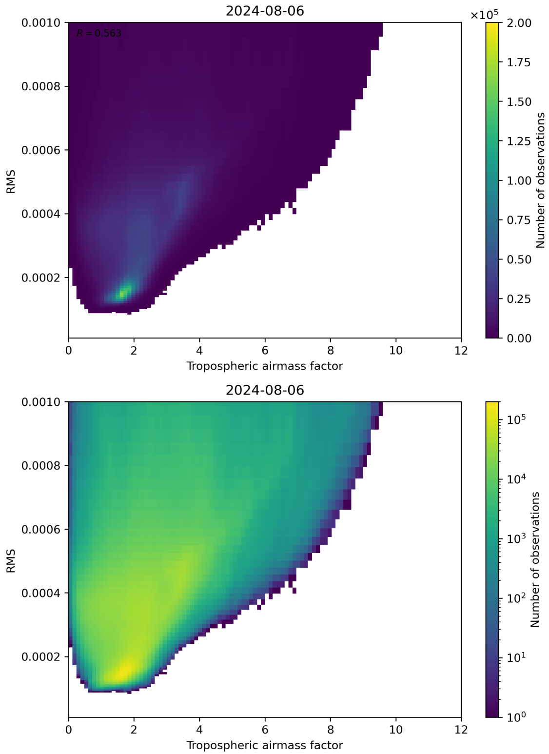
Figure 79: Scatter density plot of “Tropospheric airmass factor” against “RMS” for 2024-08-06 to 2024-08-07.
