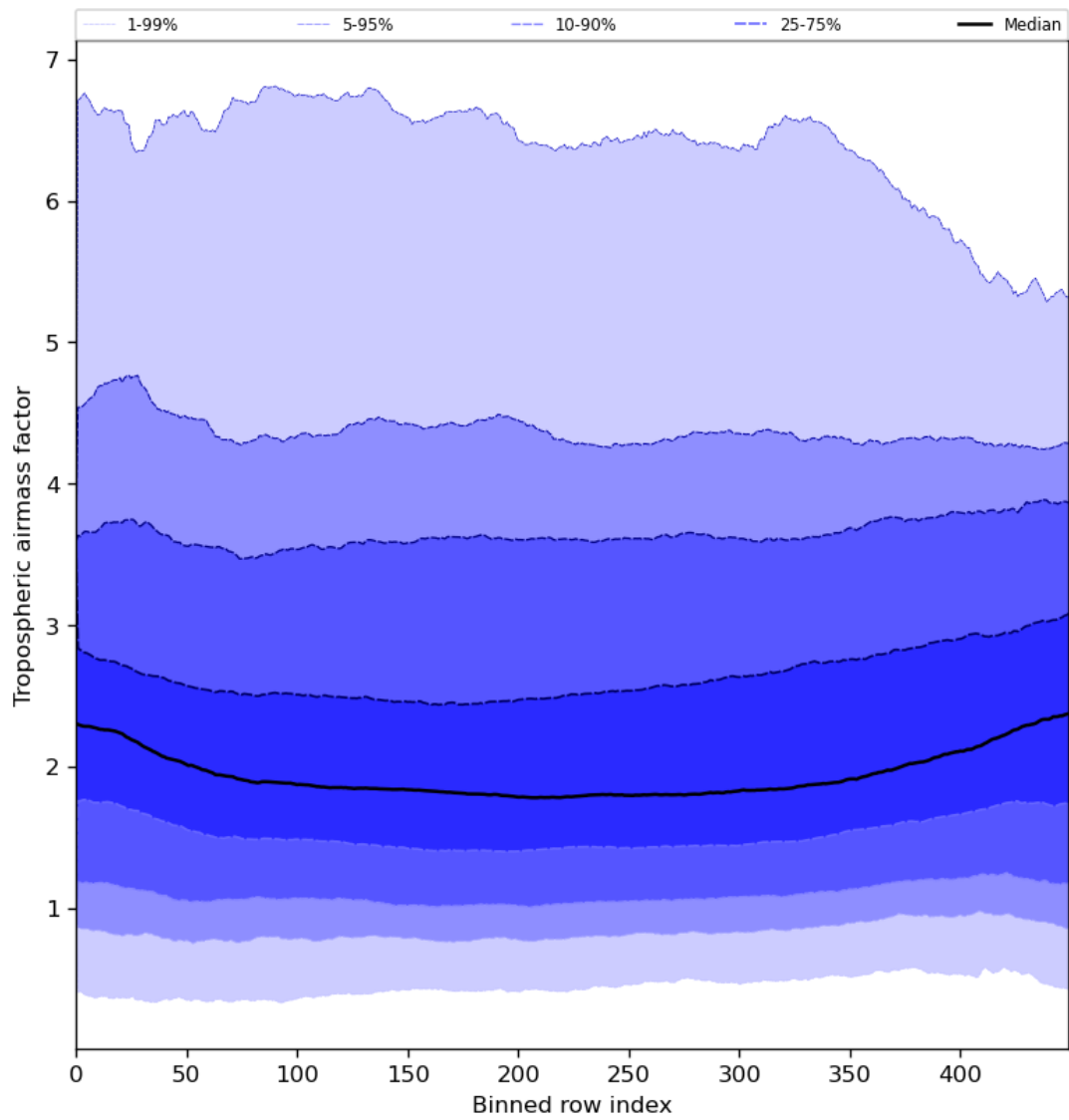
Figure 48: Along track statistics of “Tropospheric airmass factor” for 2024-08-06 to 2024-08-07
