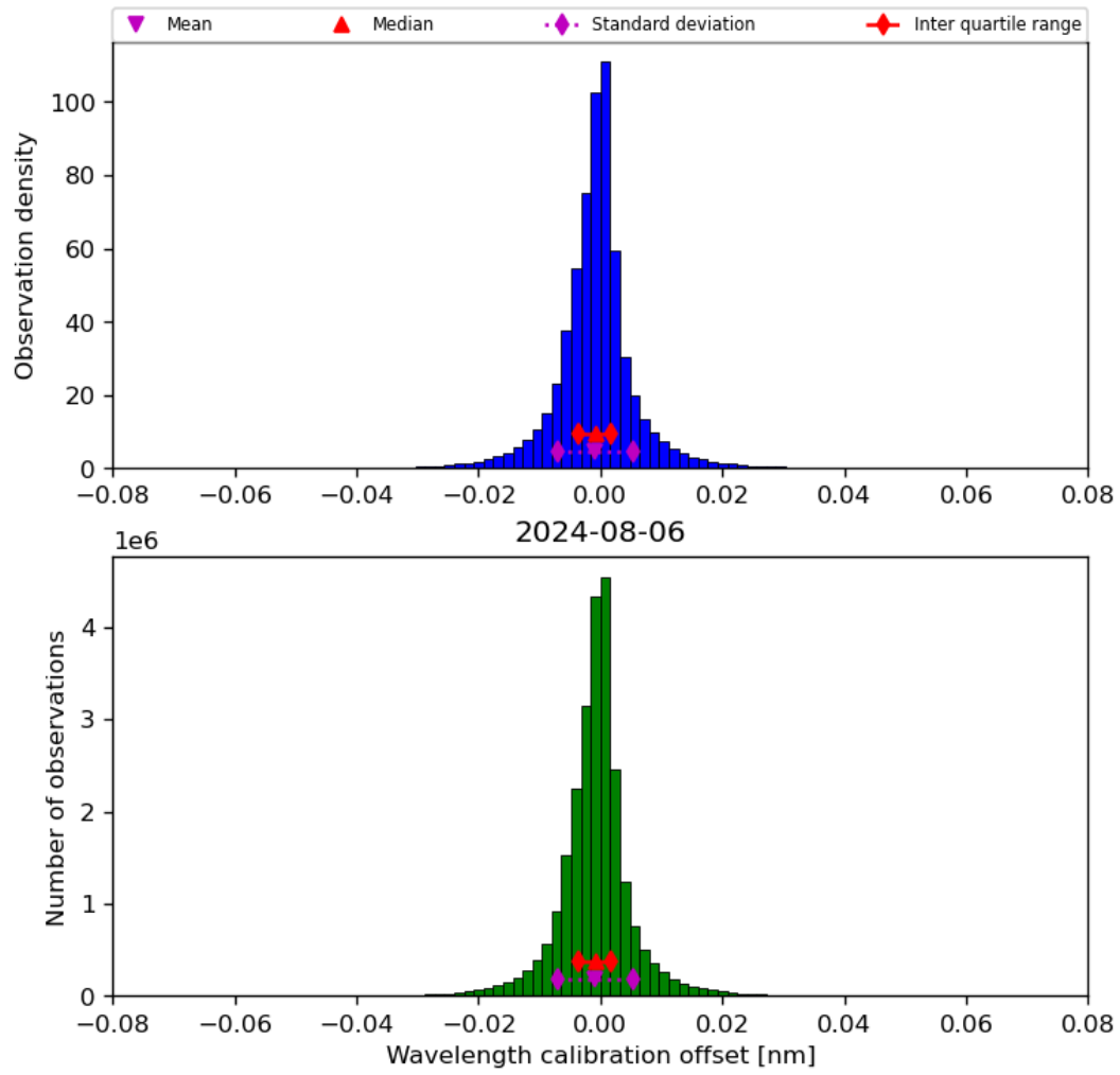
Figure 35: Histogram of “Wavelength calibration offset” for 2024-08-06 to 2024-08-07
