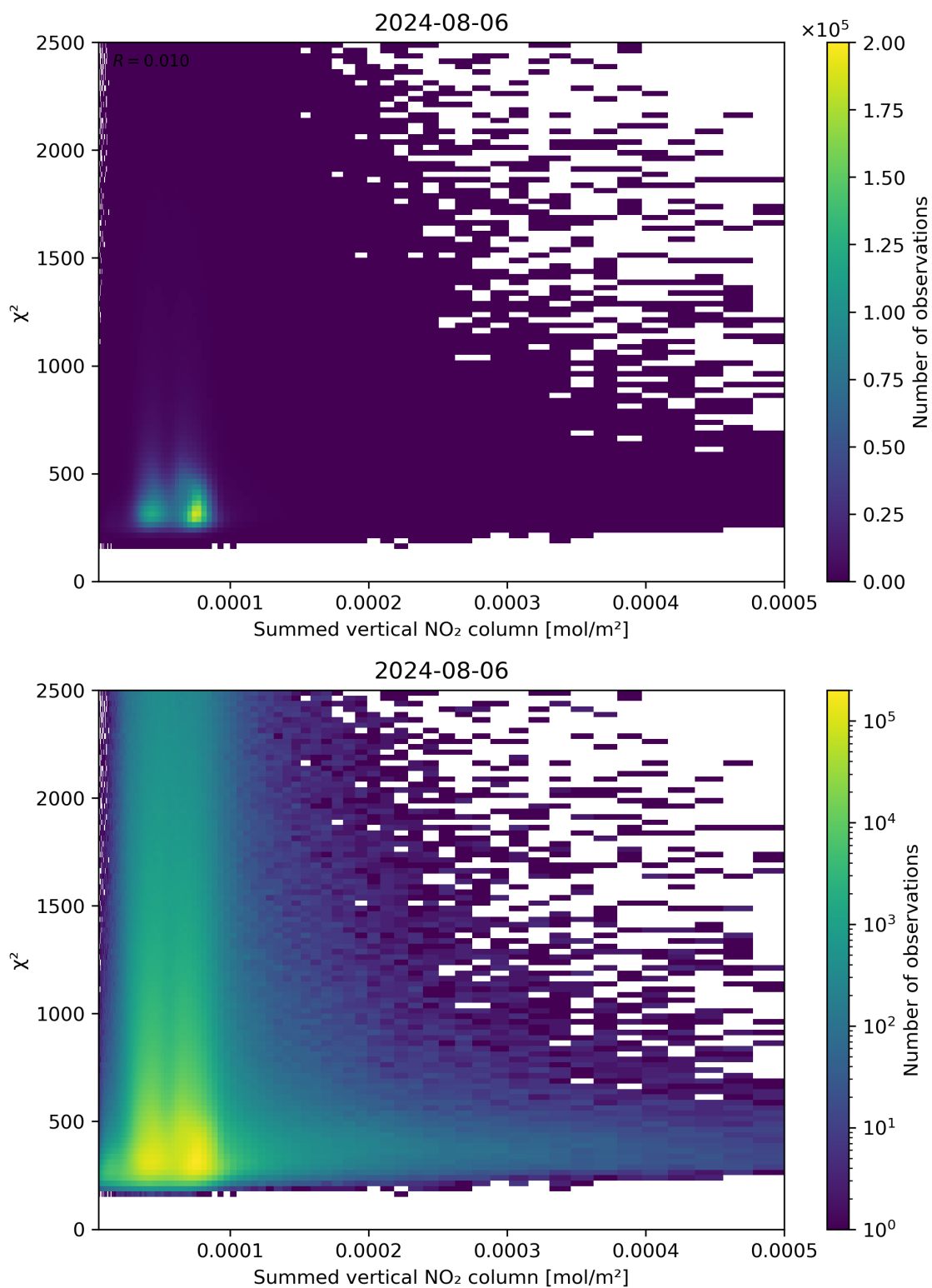
Figure 104: Scatter density plot of “Summed vertical NO 2 column” against “ \chi^2 ” for 2024-08-06 to 2024-08-07.
