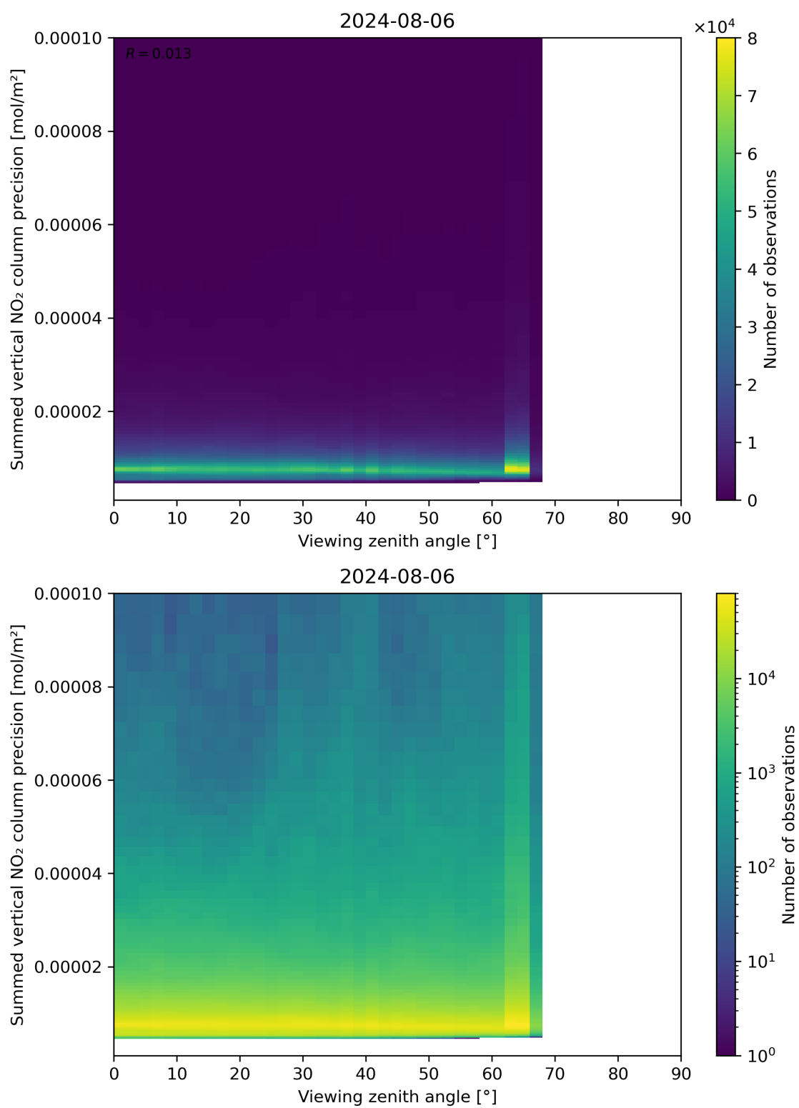
Figure 166: Scatter density plot of “Viewing zenith angle” against “Summed vertical NO 2 column precision” for 2024-08-06 to 2024-08-07.
