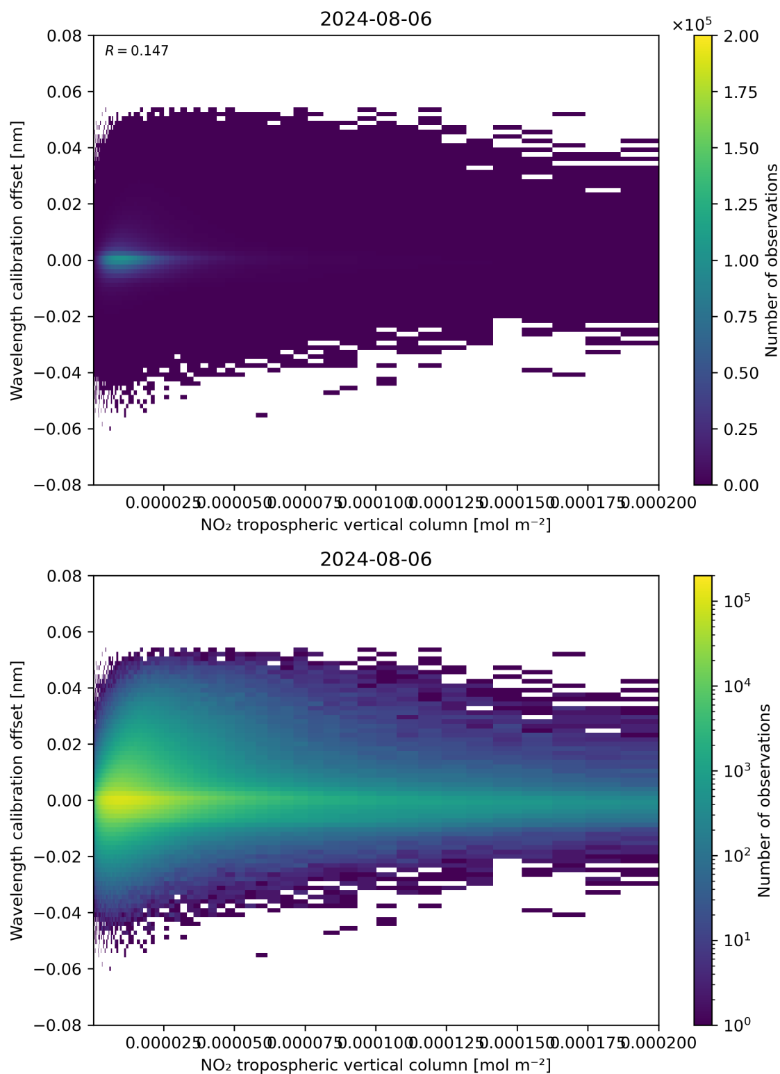
Figure 143: Scatter density plot of “NO 2 tropospheric vertical column” against “Wavelength calibration offset” for 2024-08-06 to 2024-08-07.
