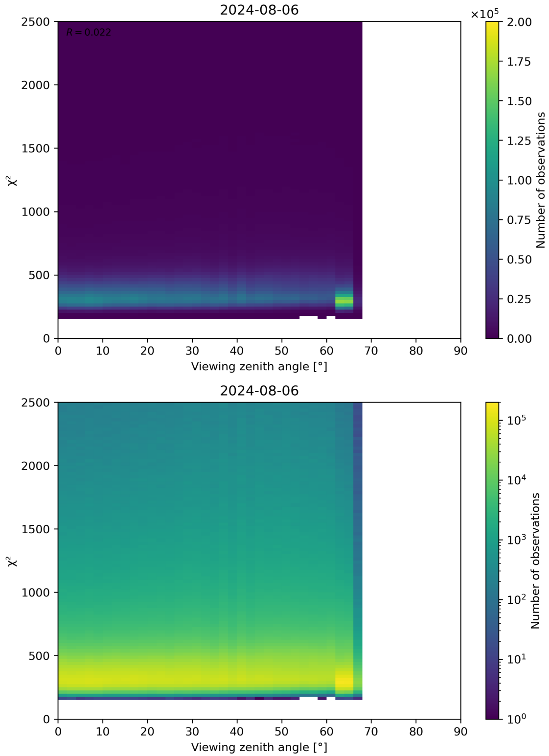
Figure 162: Scatter density plot of “Viewing zenith angle” against “ \chi^2 ” for 2024-08-06 to 2024-08-07.
