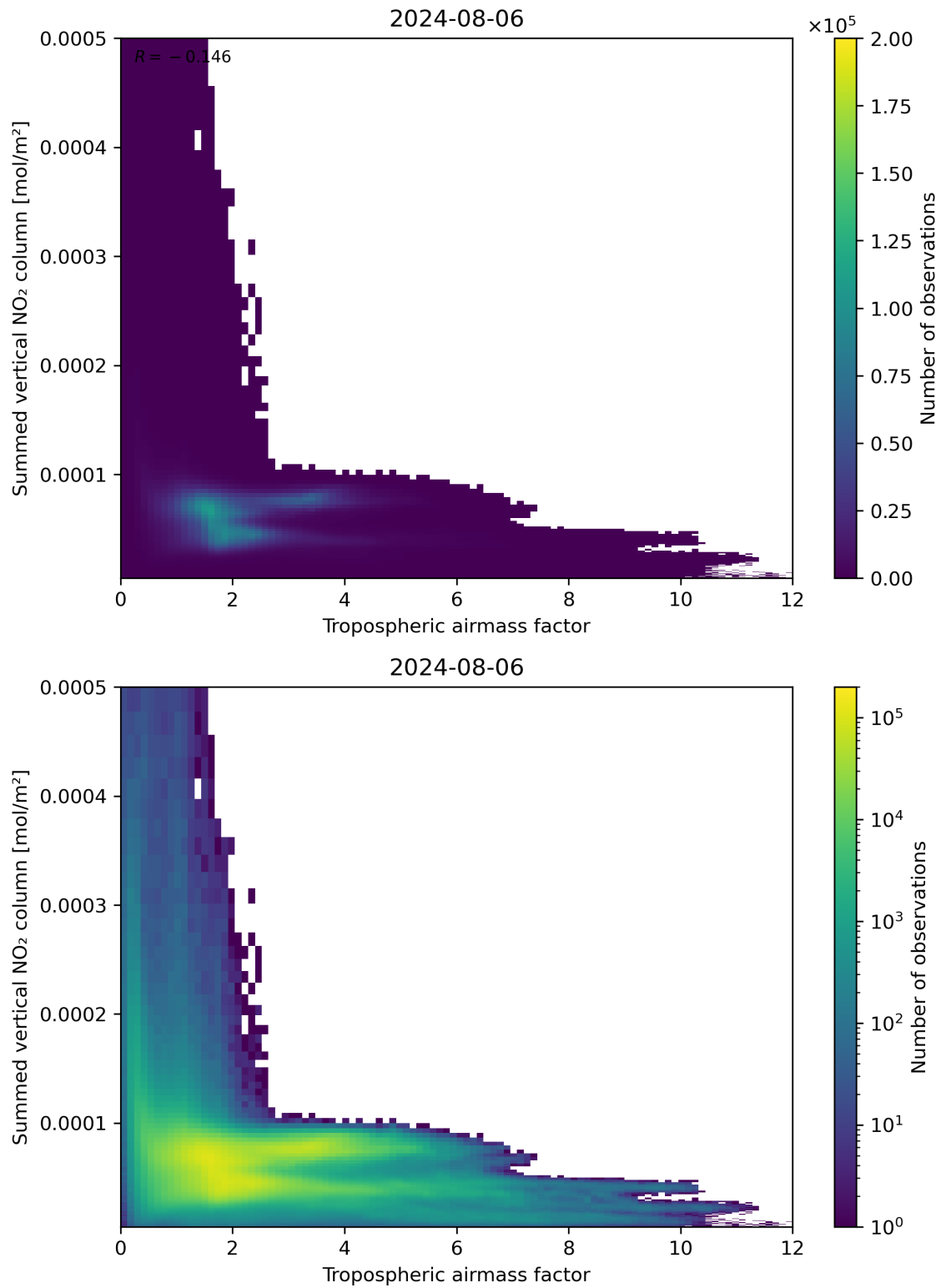
Figure 75: Scatter density plot of “Tropospheric airmass factor” against “Summed vertical NO 2 column” for 2024-08-06 to 2024-08-07.
