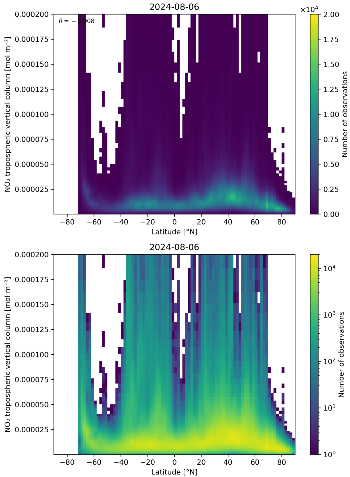
Figure 92: Scatter density plot of “Latitude” against “NO 2 tropospheric vertical column” for 2024-08-06 to 2024-08-07.
