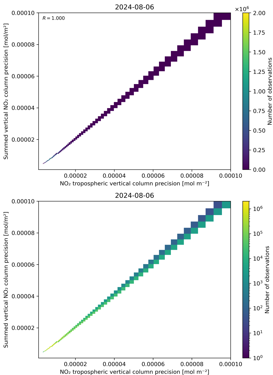
Figure 137: Scatter density plot of “NO 2 tropospheric vertical column precision” against “Summed vertical NO 2 column precision” for 2024-08-06 to 2024-08-07.
