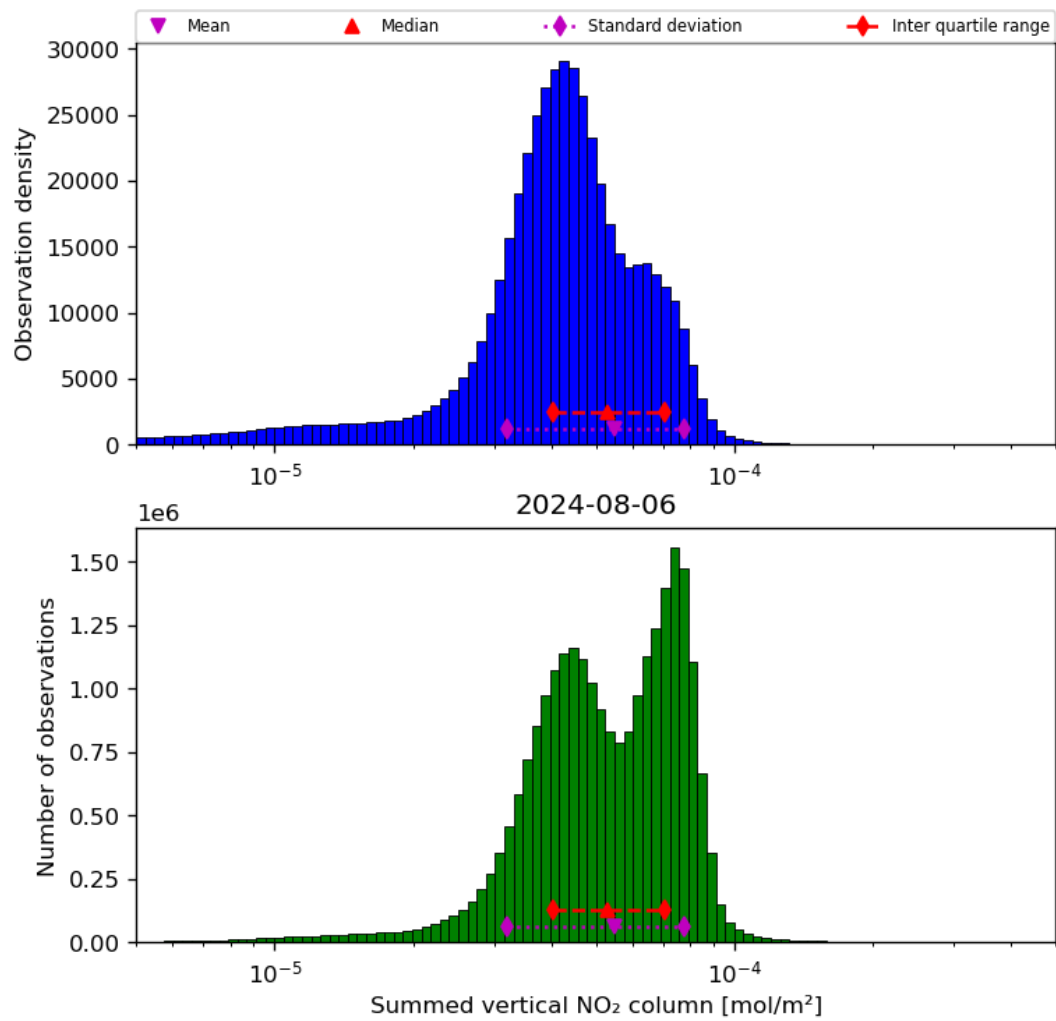
Figure 40: Histogram of “Summed vertical NO 2 column” for 2024-08-06 to 2024-08-07
