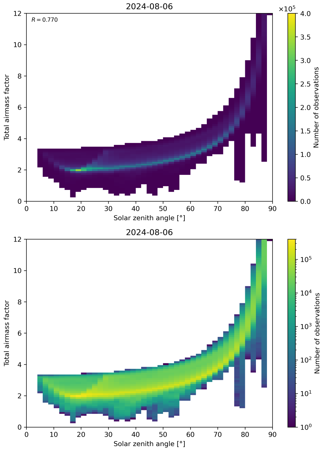
Figure 146: Scatter density plot of “Solar zenith angle” against “Total air mass factor” for 2024-08-06 to 2024-08-07.
