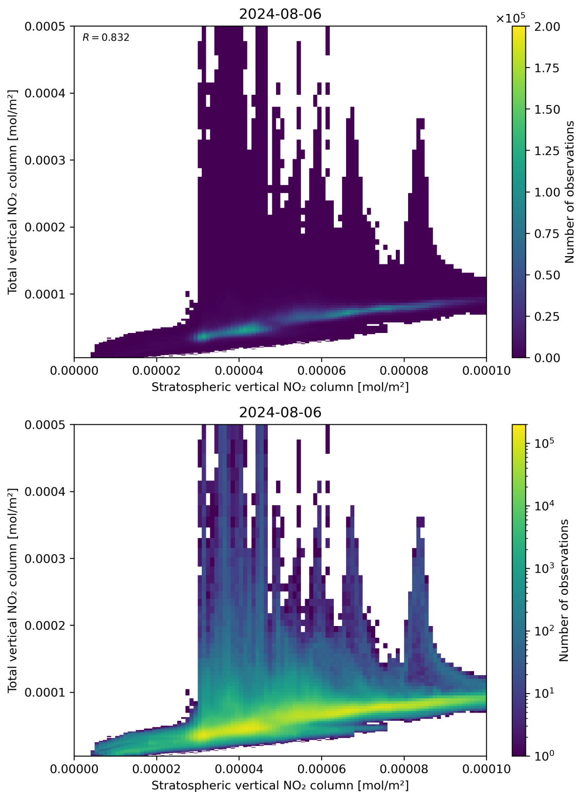
Figure 100: Scatter density plot of “Stratospheric vertical NO 2 column” against “Total vertical NO 2 column” for 2024-08-06 to 2024-08-07.
