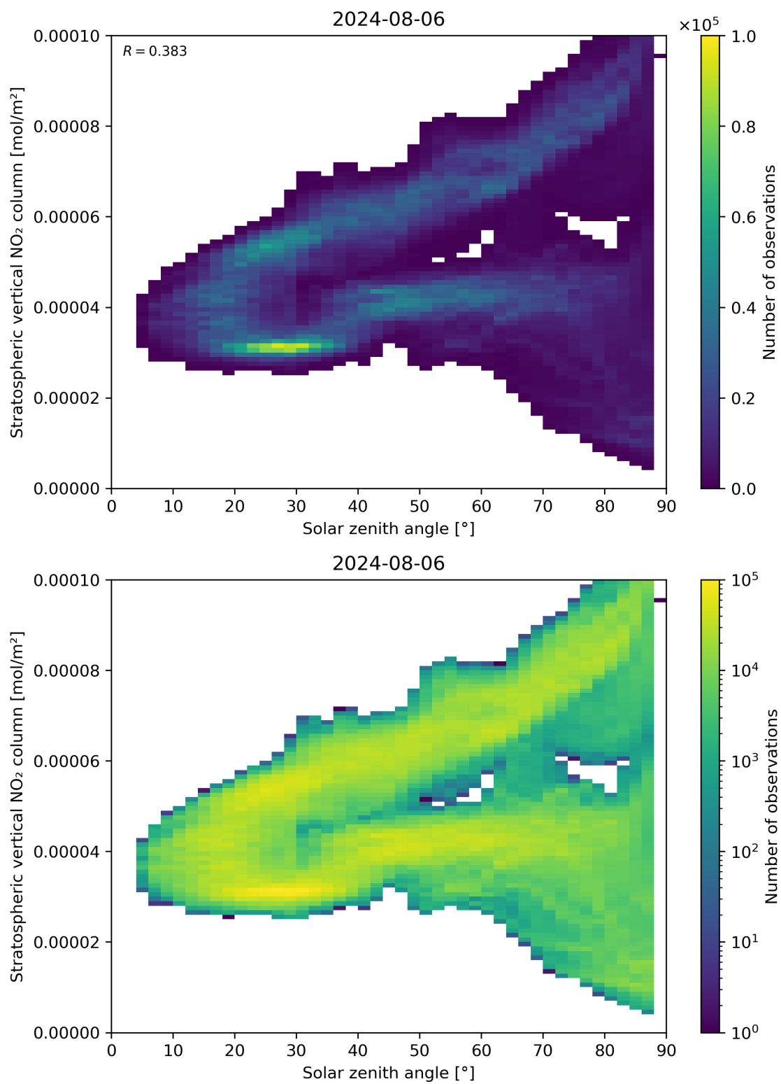
Figure 150: Scatter density plot of “Solar zenith angle” against “Stratospheric vertical NO 2 column” for 2024-08-06 to 2024-08-07.
