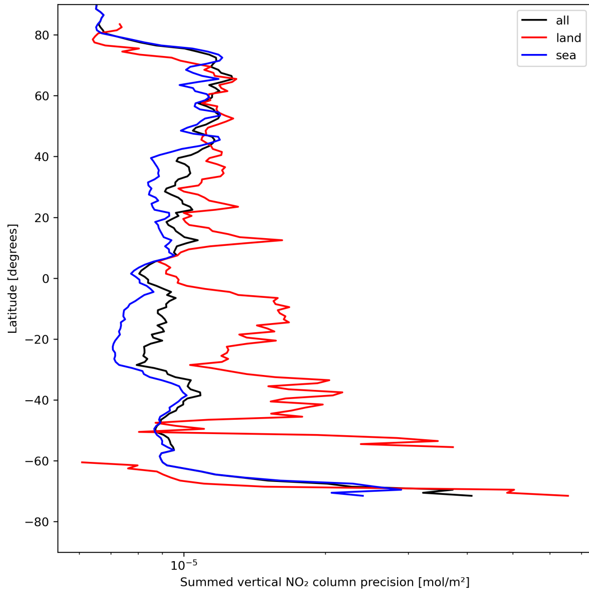
Figure 24: Zonal average of “Summed vertical NO 2 column precision” for 2024-08-06 to 2024-08-07.
