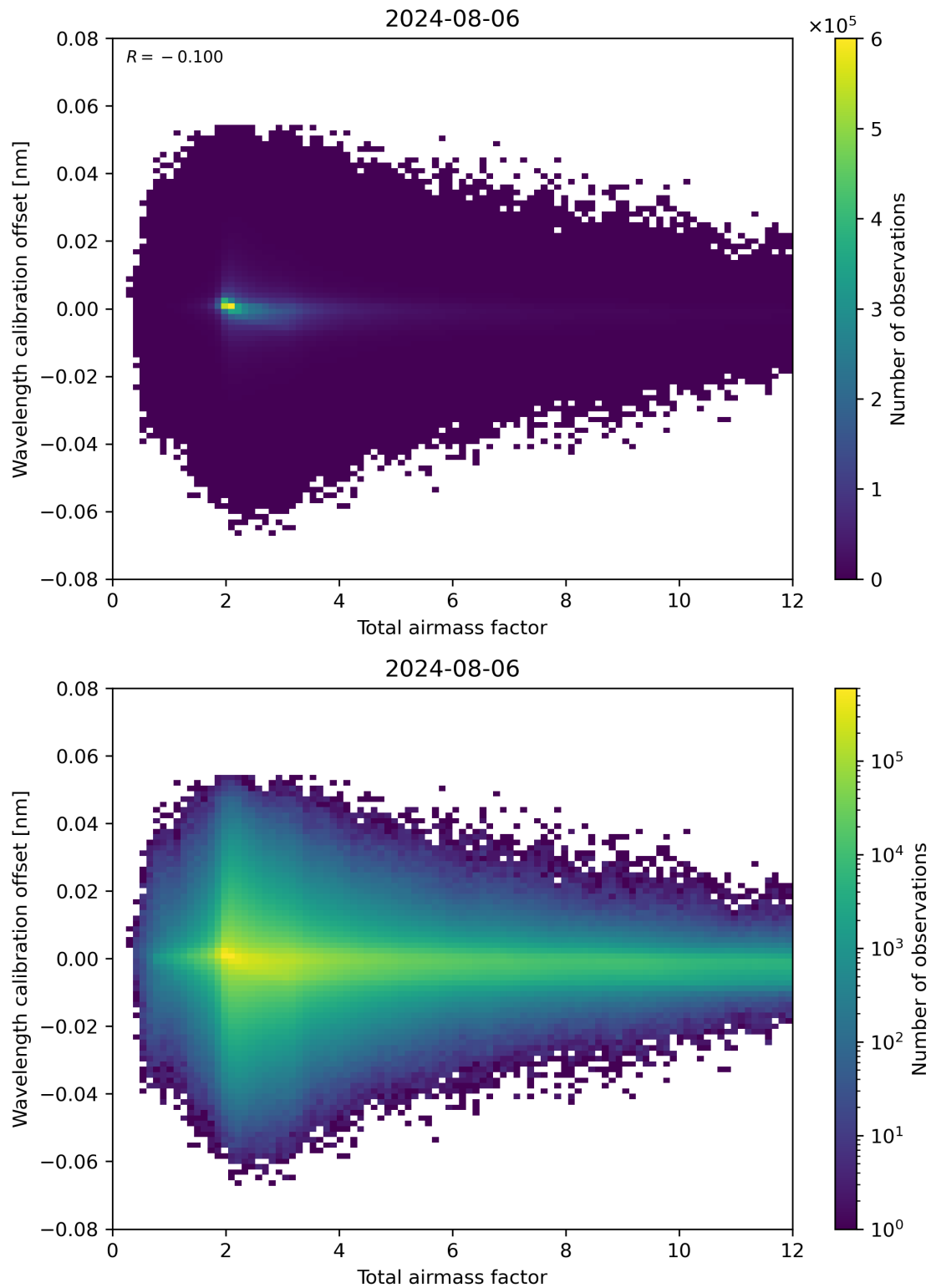
Figure 70: Scatter density plot of “Total airmass factor” against “Wavelength calibration offset” for 2024-08-06 to 2024-08-07.
