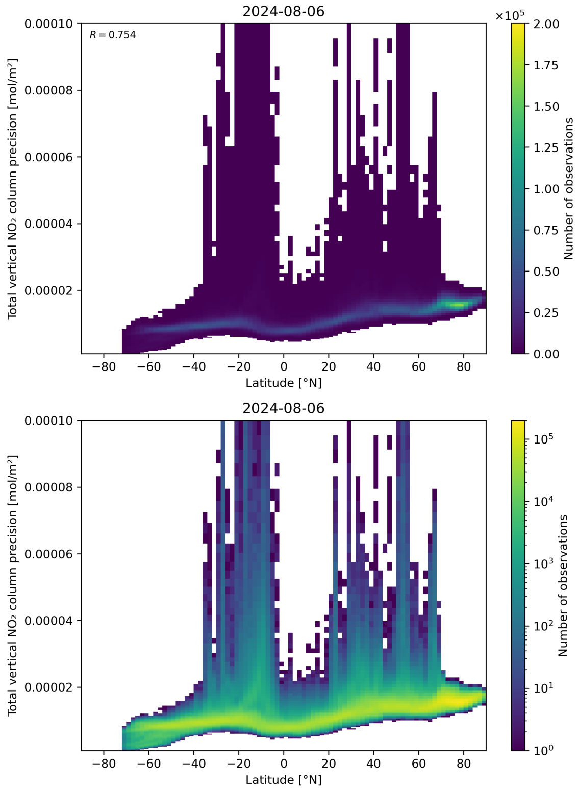
Figure 91: Scatter density plot of “Latitude” against “Total vertical NO 2 column precision” for 2024-08-06 to 2024-08-07.
