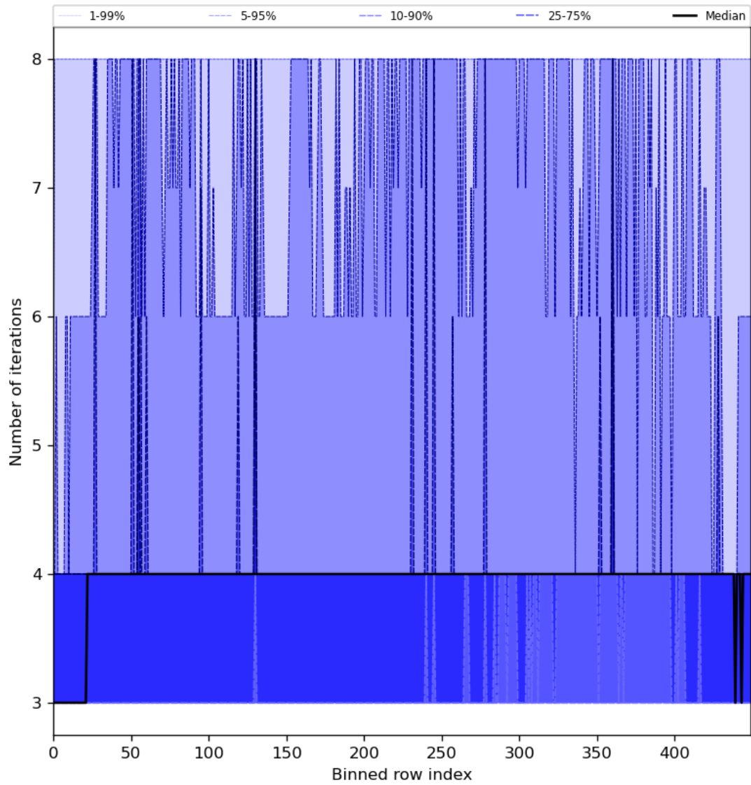
Figure 51: Along track statistics of “Number of iterations” for 2024-08-06 to 2024-08-07
