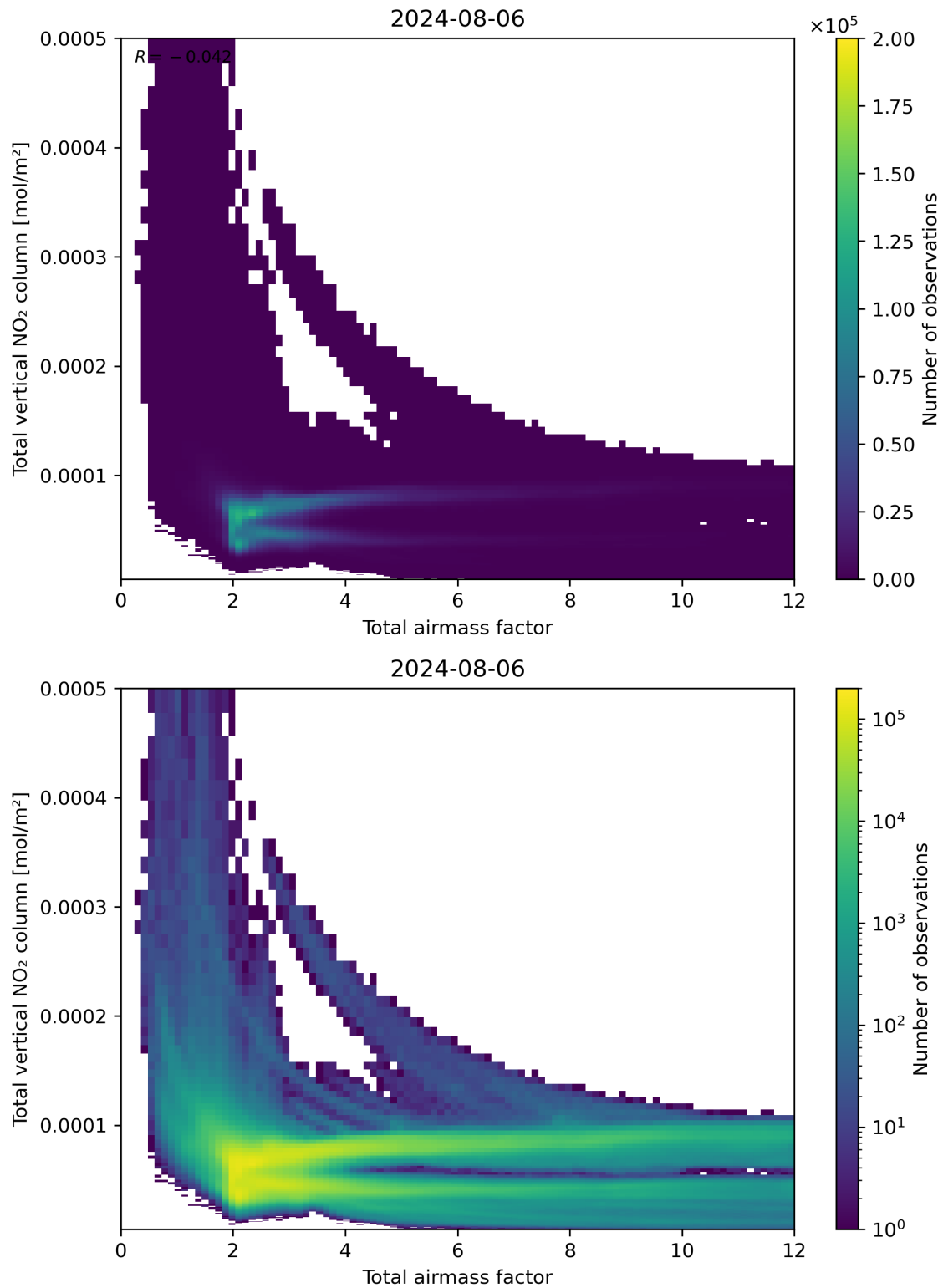
Figure 67: Scatter density plot of “Total airmass factor” against “Total vertical NO 2 column” for 2024-08-06 to 2024-08-07.
