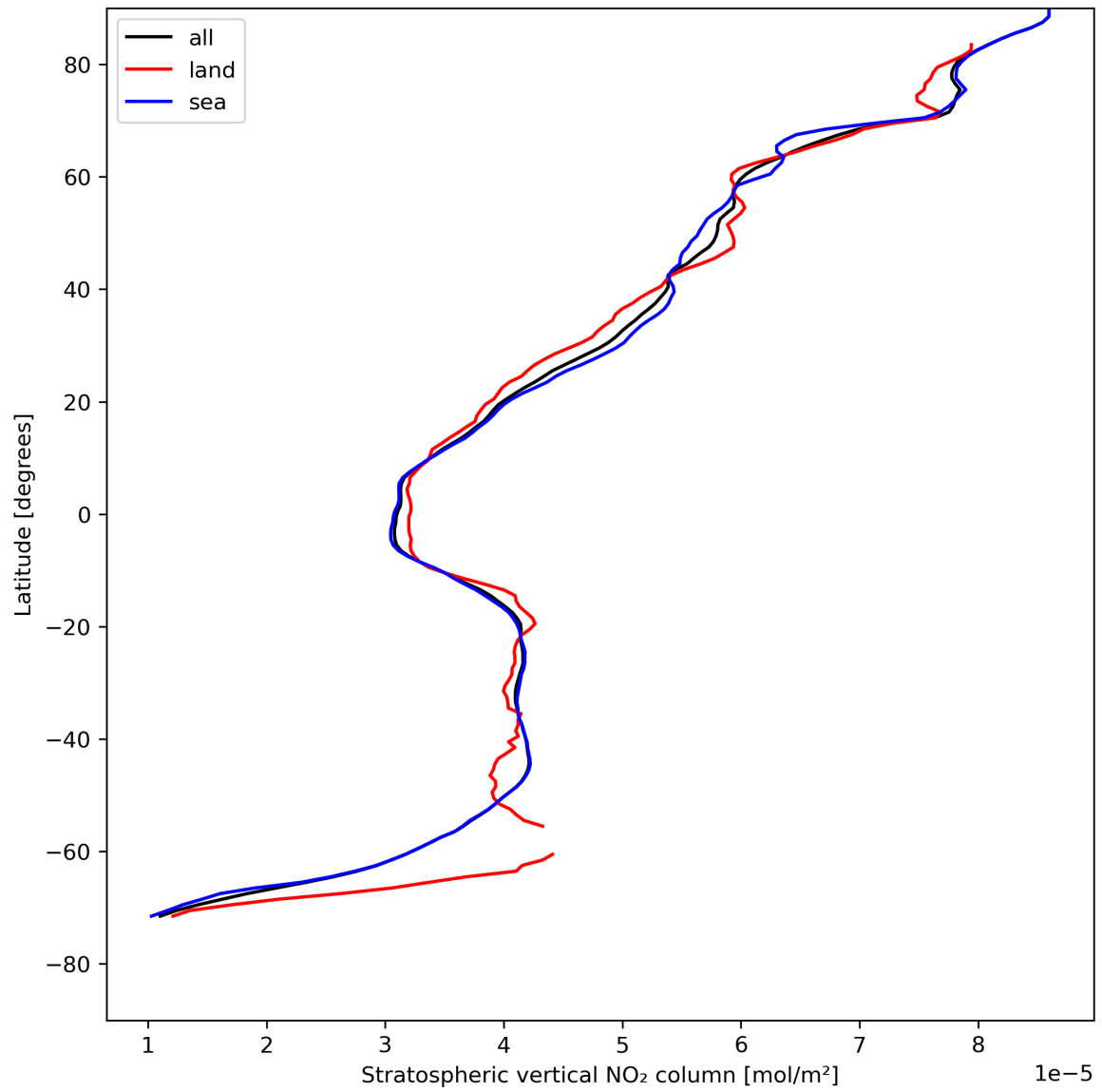
Figure 19: Zonal average of “Stratospheric vertical NO 2 column” for 2024-08-06 to 2024-08-07.
