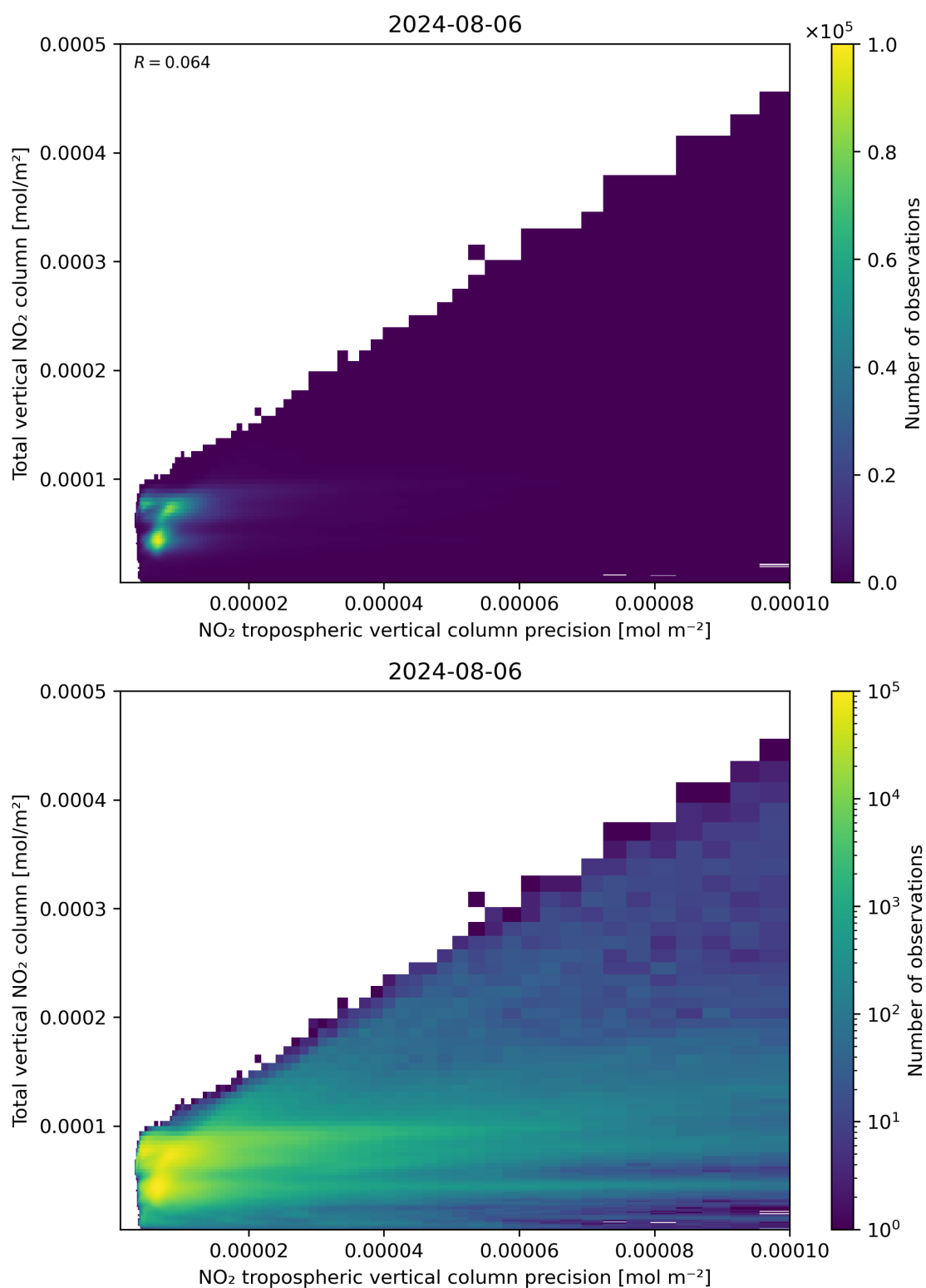
Figure 138: Scatter density plot of “NO 2 tropospheric vertical column precision” against “Total vertical NO 2 column” for 2024-08-06 to 2024-08-07.
