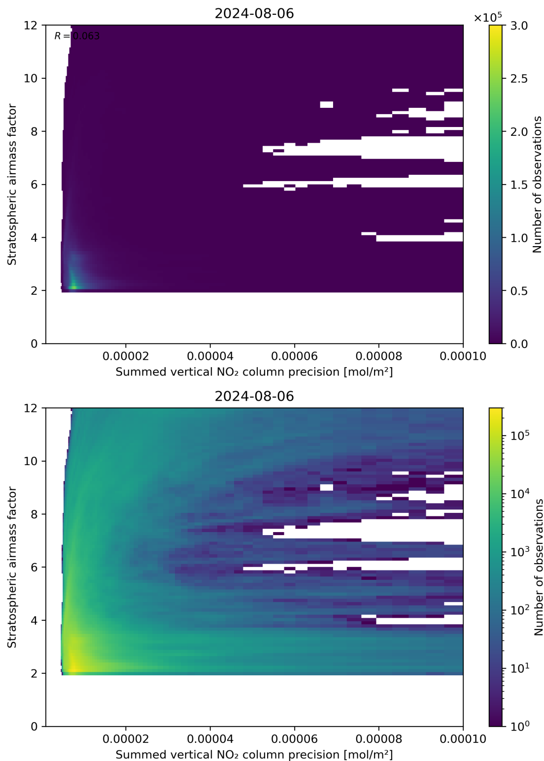
Figure 106: Scatter density plot of “Summed vertical NO 2 column precision” against “Stratospheric airmass factor” for 2024-08-06 to 2024-08-07.
