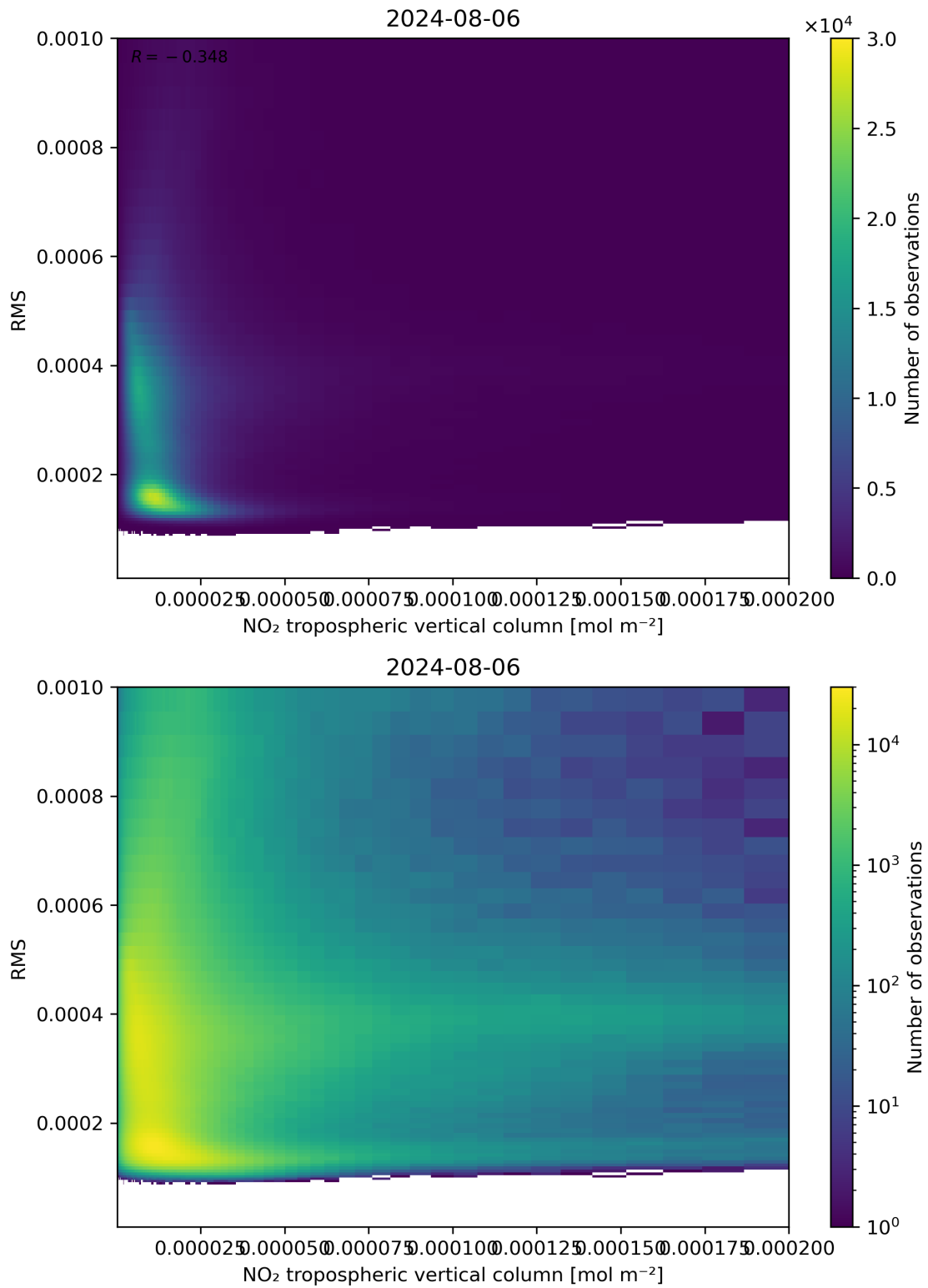
Figure 142: Scatter density plot of “NO 2 tropospheric vertical column” against “RMS” for 2024-08-06 to 2024-08-07.
