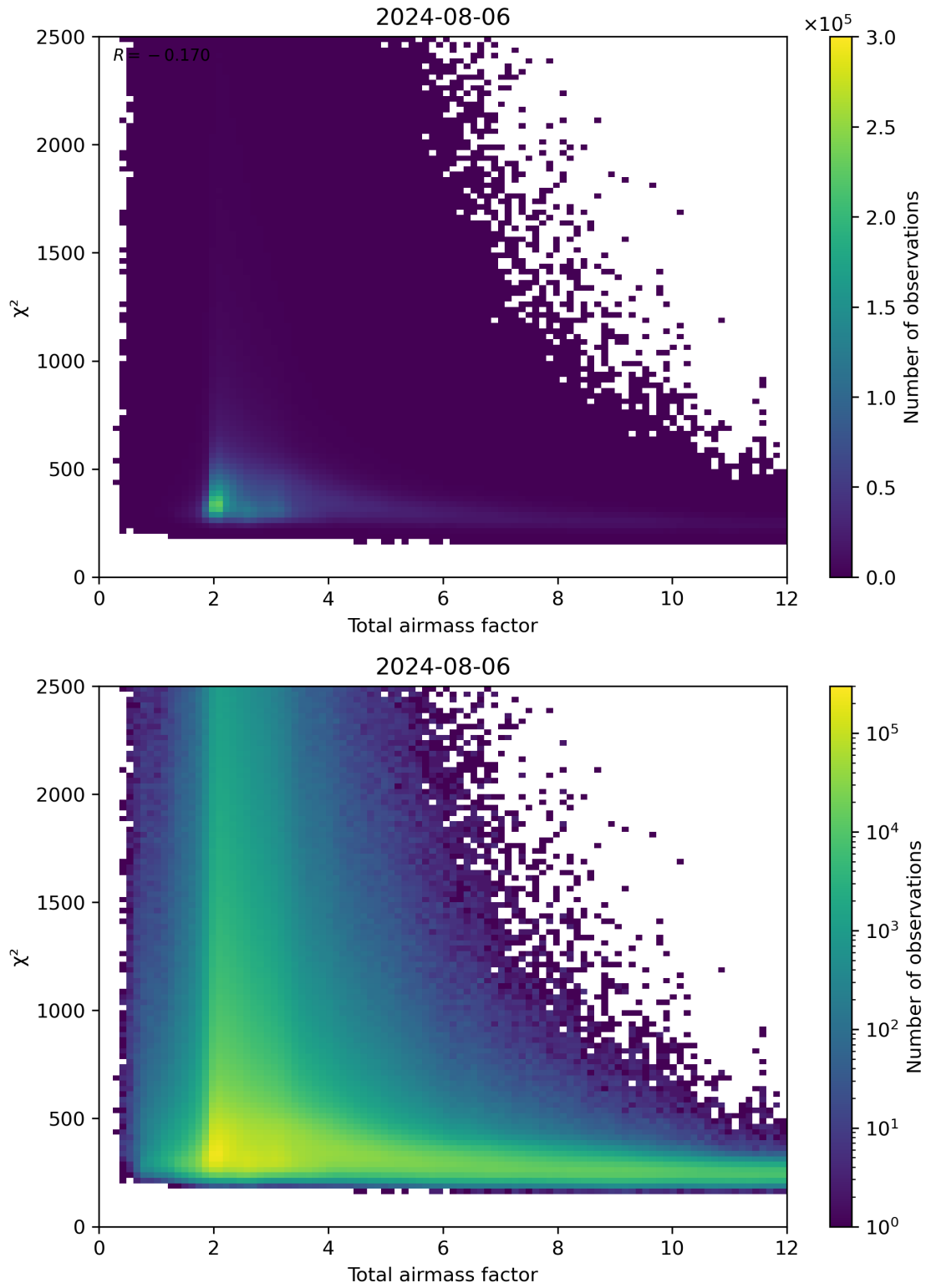
Figure 63: Scatter density plot of “Total airmass factor” against “ \chi^2 ” for 2024-08-06 to 2024-08-07.
