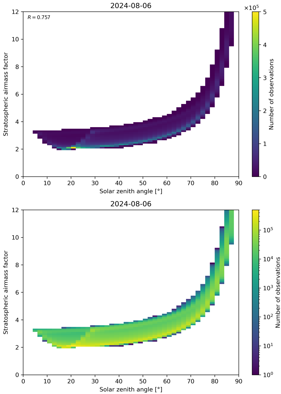
Figure 145: Scatter density plot of “Solar zenith angle” against “Stratospheric airmass factor” for 2024-08-06 to 2024-08-07.
