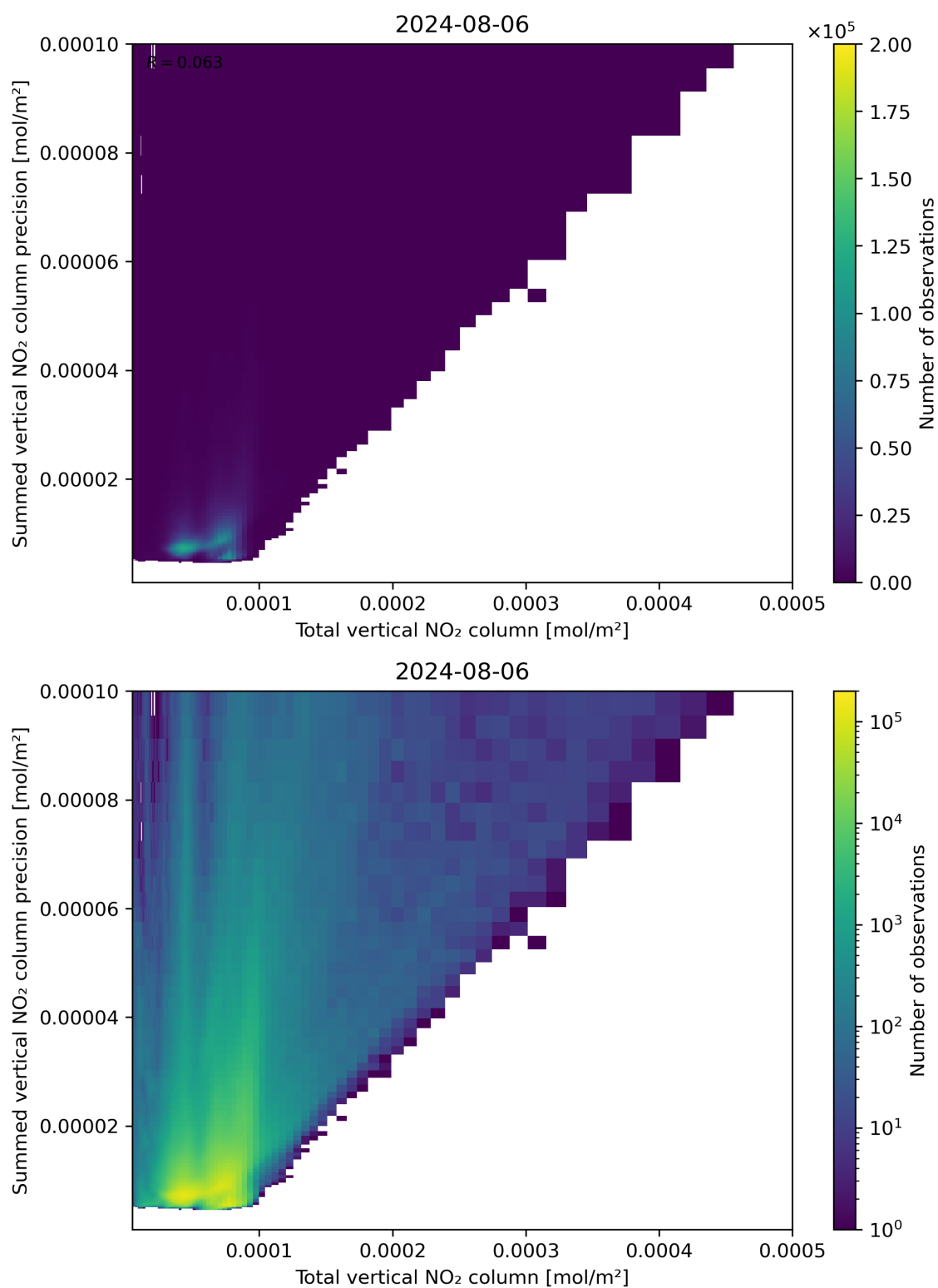
Figure 113: Scatter density plot of “Total vertical NO 2 column” against “Summed vertical NO 2 column precision” for 2024-08-06 to 2024-08-07.
