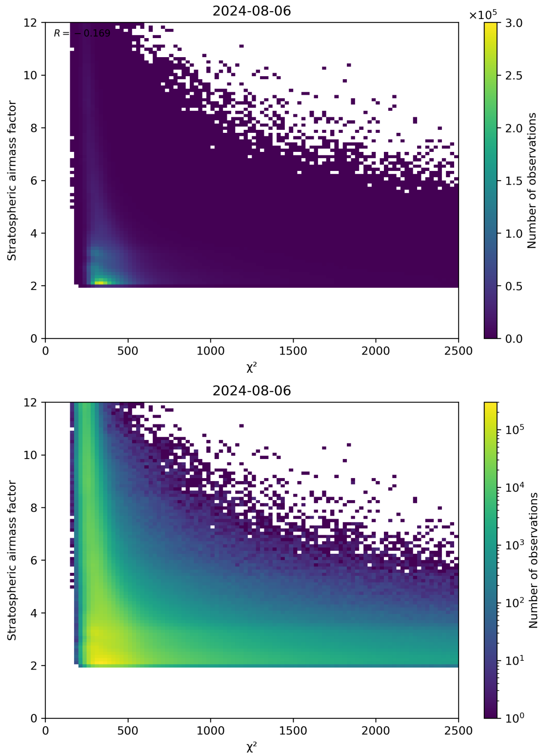
Figure 81: Scatter density plot of “ \chi^2 ” against “Stratospheric airmass factor” for 2024-08-06 to 2024-08-07.
