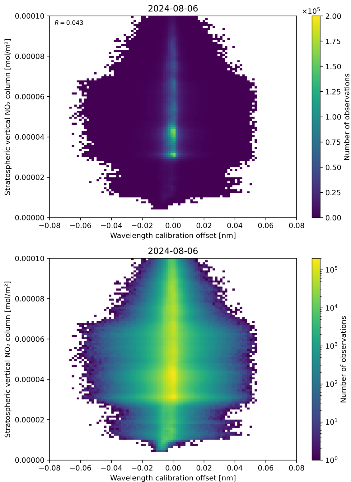
Figure 176: Scatter density plot of “Wavelength calibration offset” against “Stratospheric vertical NO 2 column” for 2024-08-06 to 2024-08-07.
