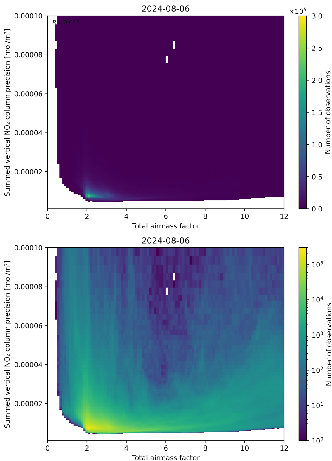
Figure 66: Scatter density plot of “Total airmass factor” against “Summed vertical NO 2 column precision” for 2024-08-06 to 2024-08-07.
