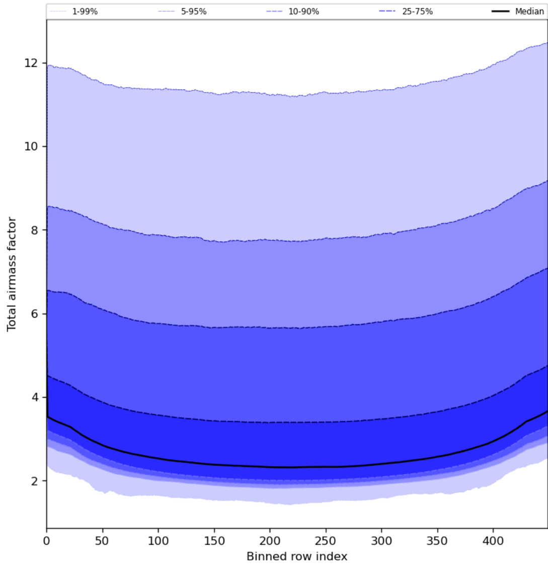
Figure 49: Along track statistics of “Total airmass factor” for 2024-08-06 to 2024-08-07
