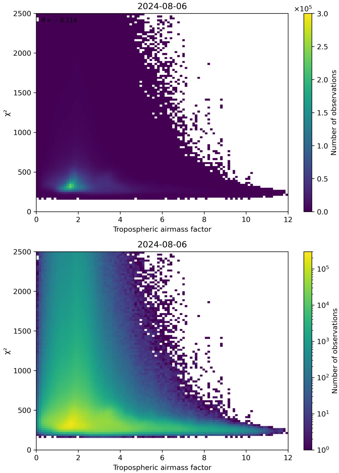
Figure 73: Scatter density plot of “Tropospheric airmass factor” against “ \chi^2 ” for 2024-08-06 to 2024-08-07.
