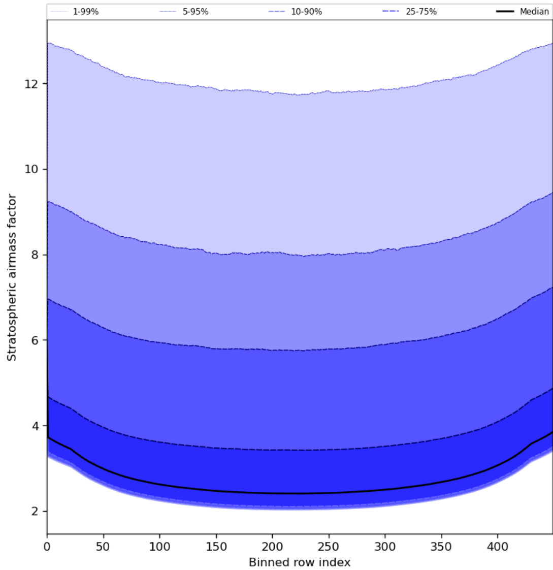
Figure 61: Along track statistics of “Stratospheric airmass factor” for 2024-08-06 to 2024-08-07
