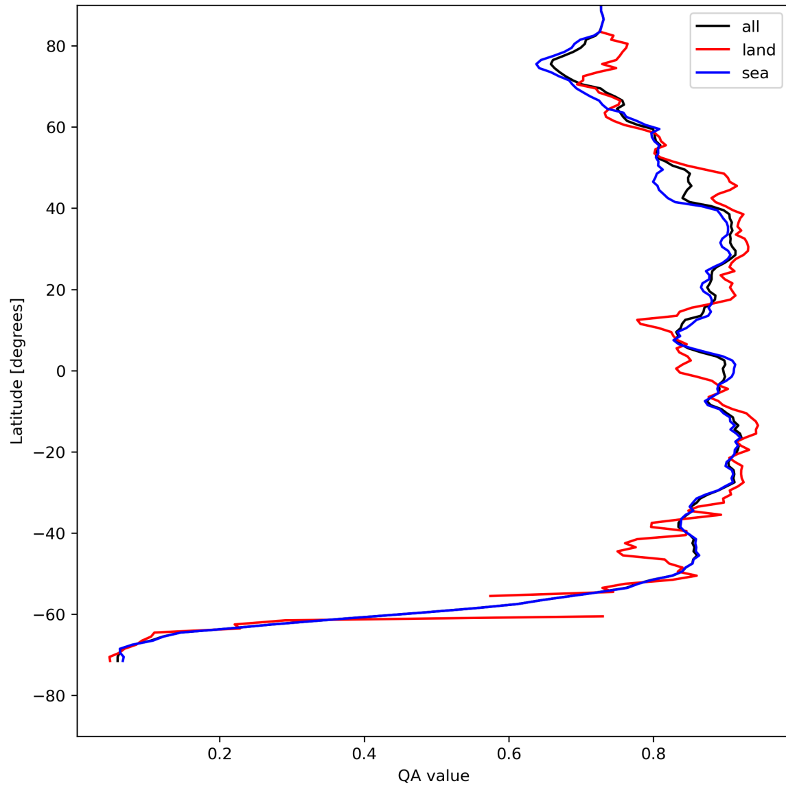
Figure 11: Zonal average of “QA value” for 2024-08-06 to 2024-08-07.
