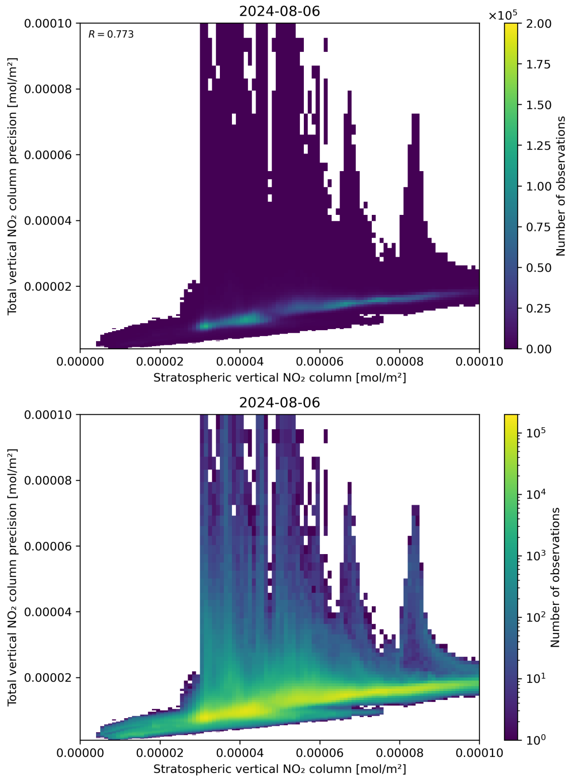
Figure 101: Scatter density plot of “Stratospheric vertical NO 2 column” against “Total vertical NO 2 column precision” for 2024-08-06 to 2024-08-07.
