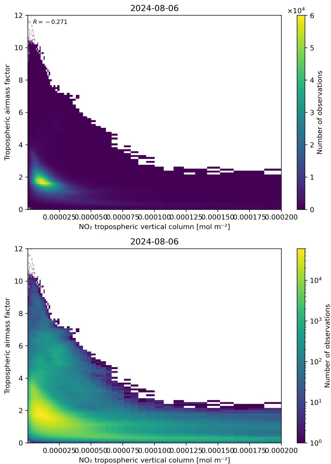
Figure 123: Scatter density plot of “NO 2 tropospheric vertical column” against “Tropospheric air mass factor” for 2024-08-06 to 2024-08-07.
