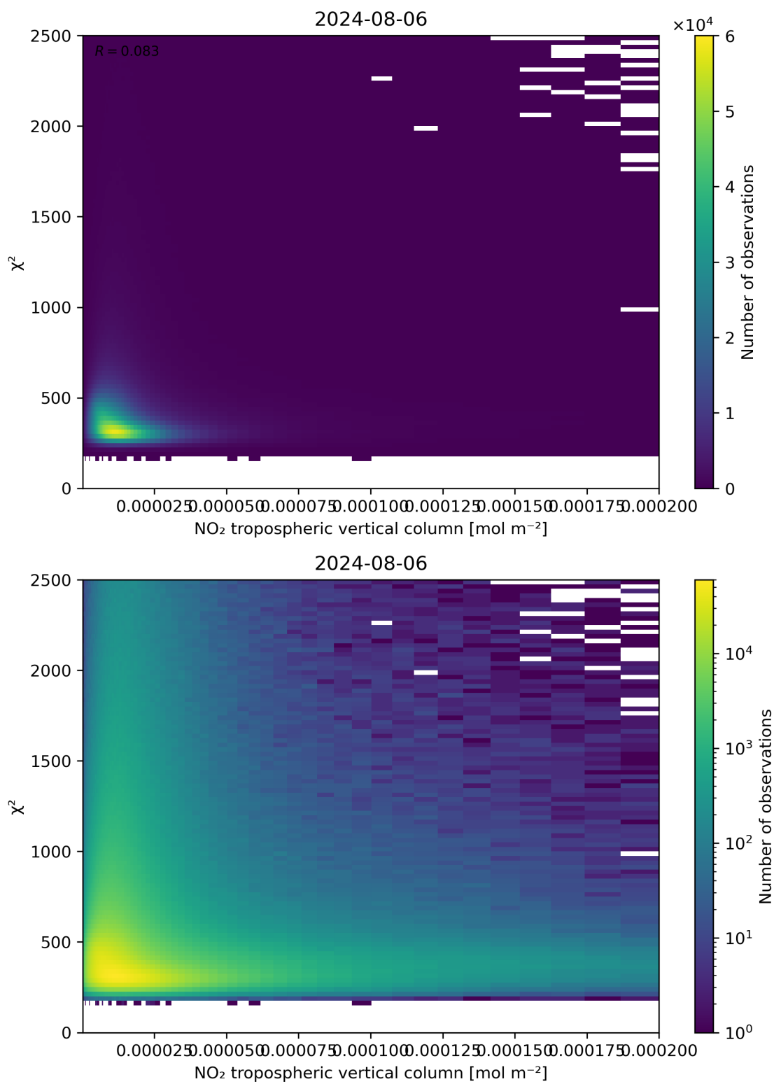
Figure 124: Scatter density plot of “NO 2 tropospheric vertical column” against “ \chi^2 ” for 2024-08-06 to 2024-08-07.
