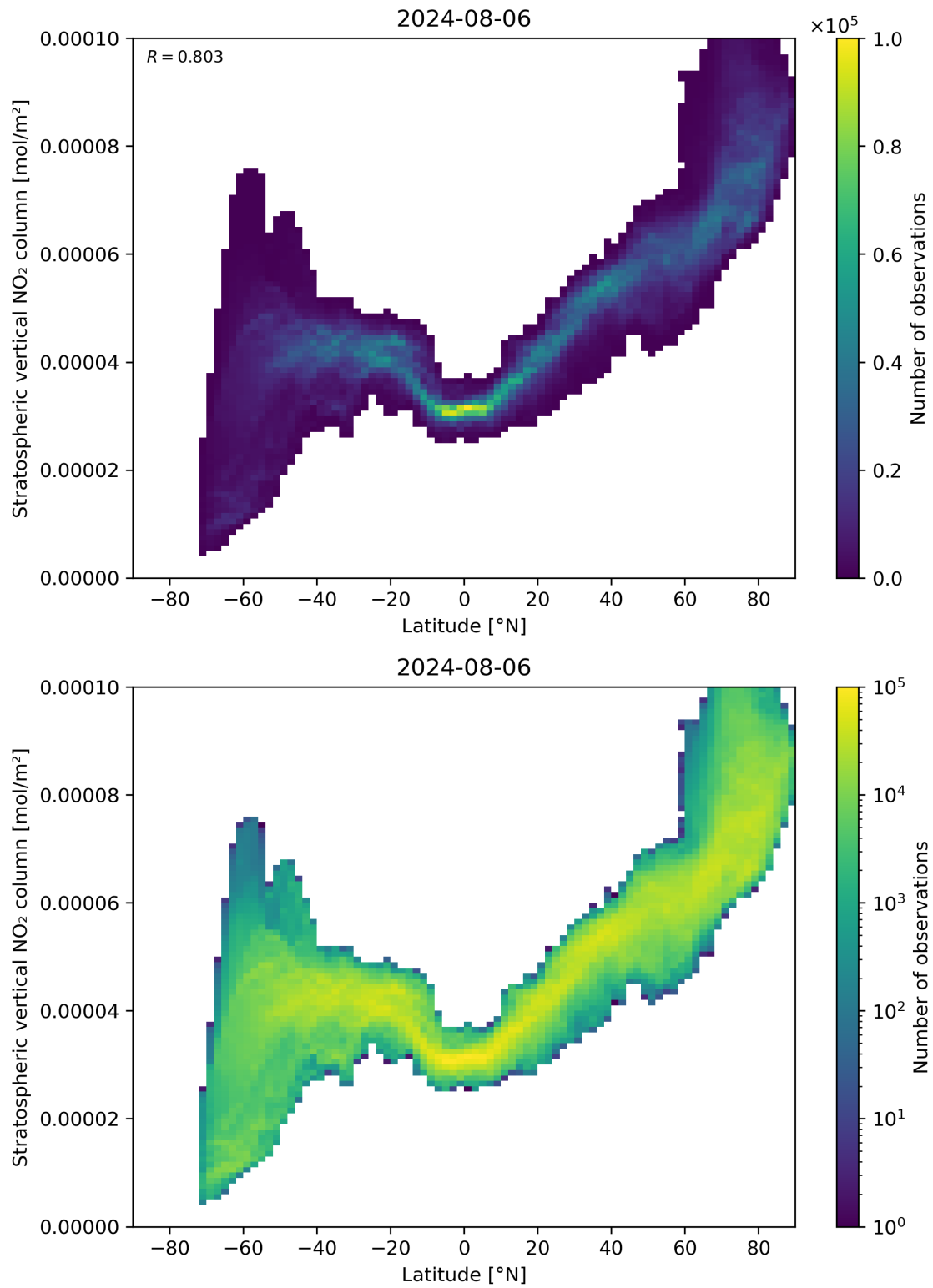
Figure 87: Scatter density plot of “Latitude” against “Stratospheric vertical \text{NO}_2 column” for 2024-08-06 to 2024-08-07.
