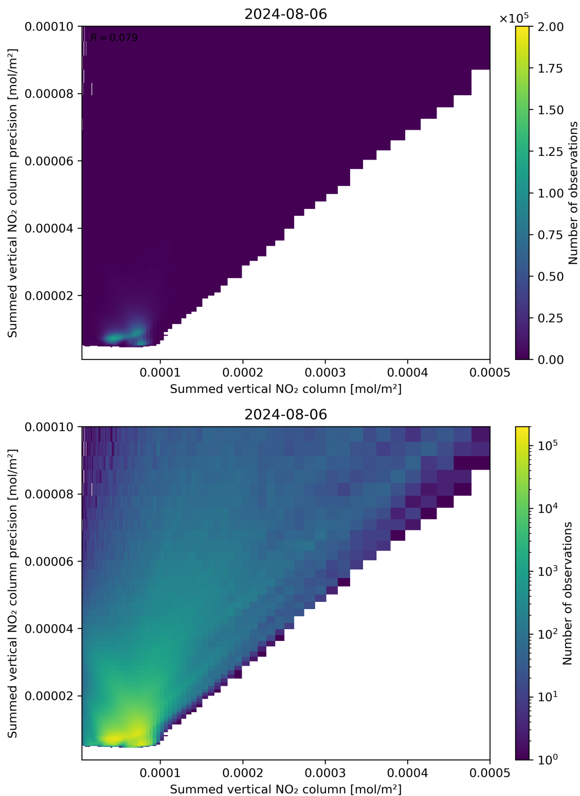
Figure 105: Scatter density plot of “Summed vertical NO 2 column” against “Summed vertical NO 2 column precision” for 2024-08-06 to 2024-08-07.
