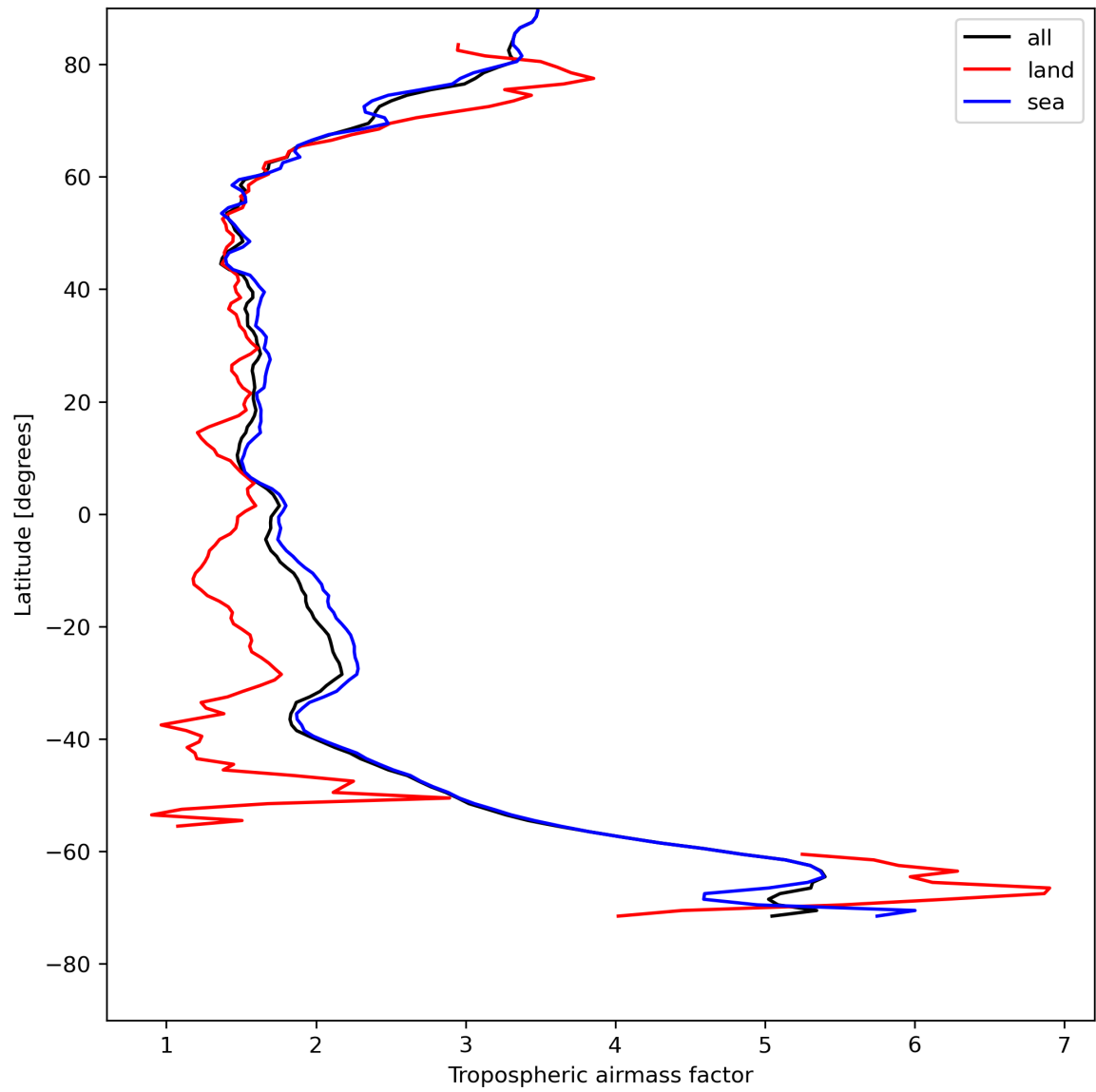
Figure 14: Zonal average of “Tropospheric airmass factor” for 2024-08-06 to 2024-08-07.
