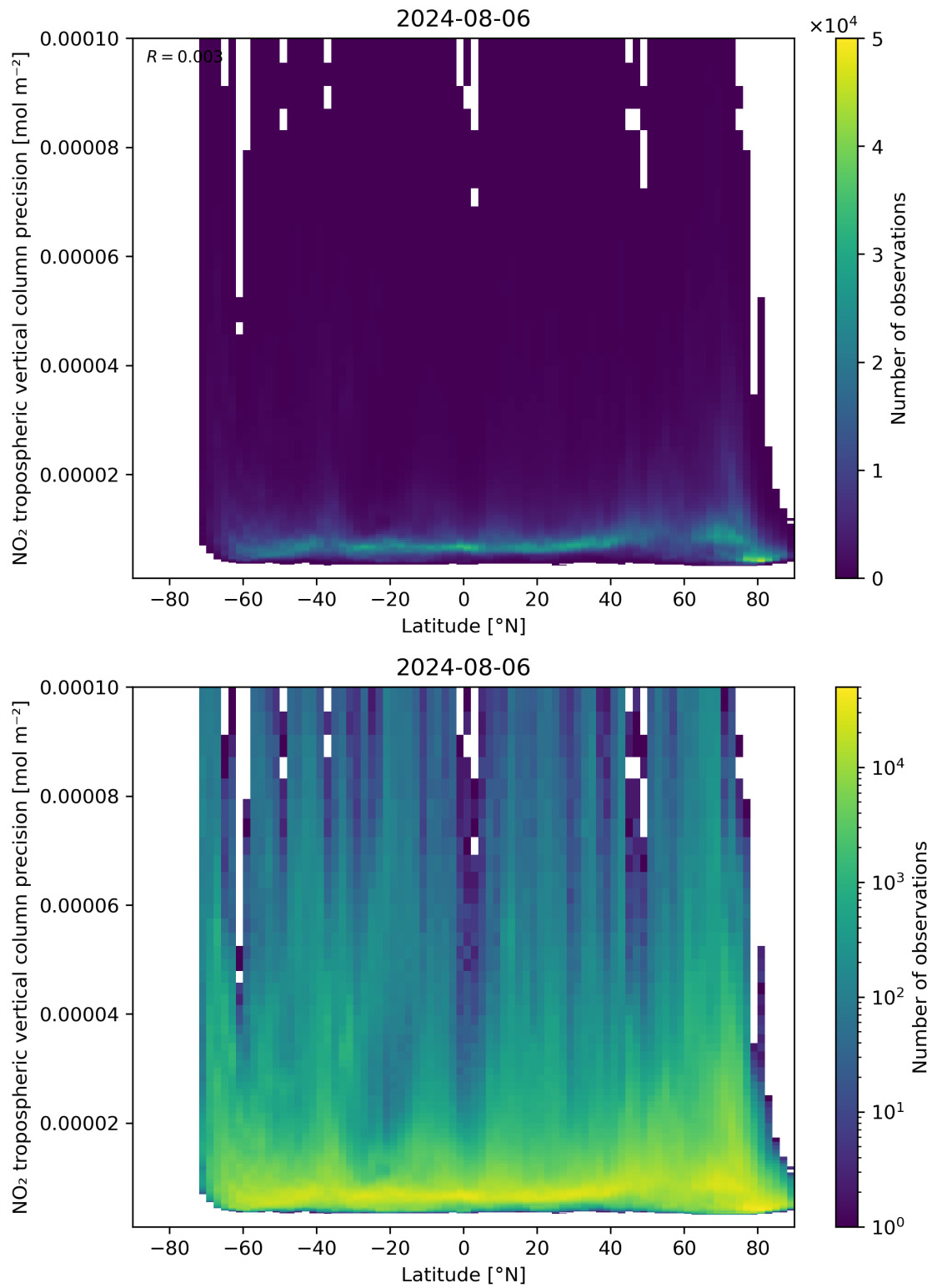
Figure 93: Scatter density plot of “Latitude” against “NO 2 tropospheric vertical column precision” for 2024-08-06 to 2024-08-07.
