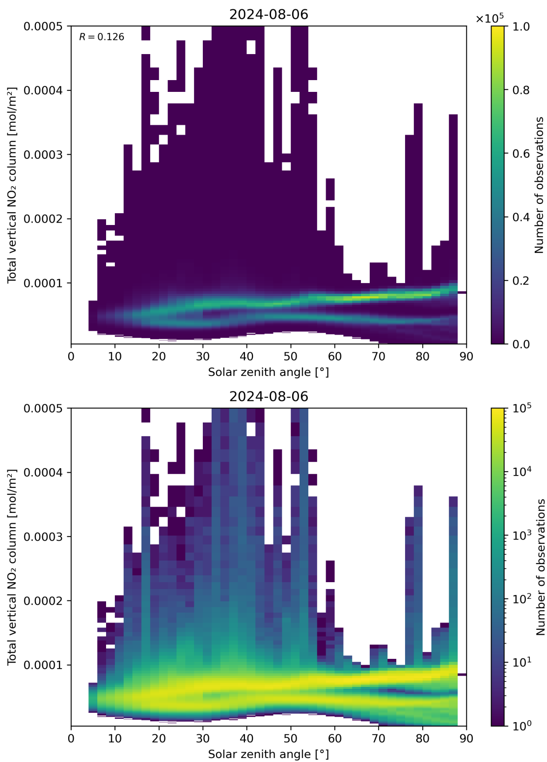
Figure 153: Scatter density plot of “Solar zenith angle” against “Total vertical NO 2 column” for 2024-08-06 to 2024-08-07.
