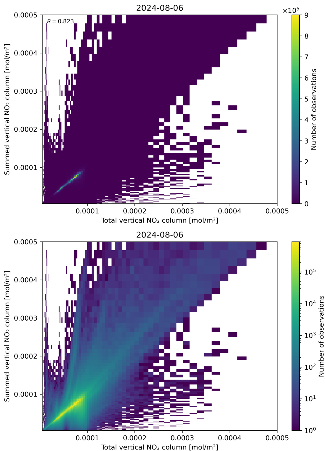
Figure 112: Scatter density plot of “Total vertical NO 2 column” against “Summed vertical NO 2 column” for 2024-08-06 to 2024-08-07.
