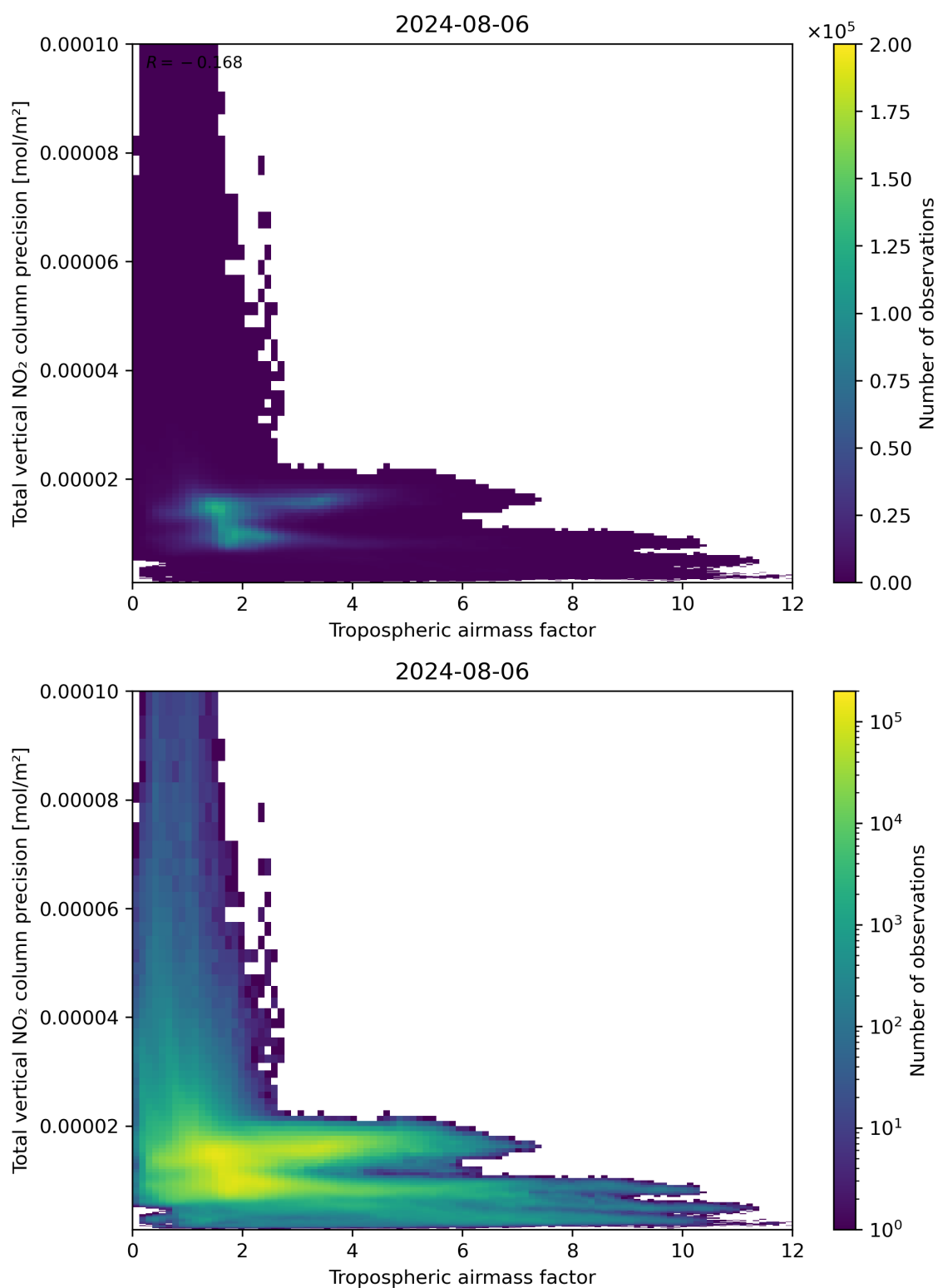
Figure 78: Scatter density plot of “Tropospheric air mass factor” against “Total vertical NO 2 column precision” for 2024-08-06 to 2024-08-07.
