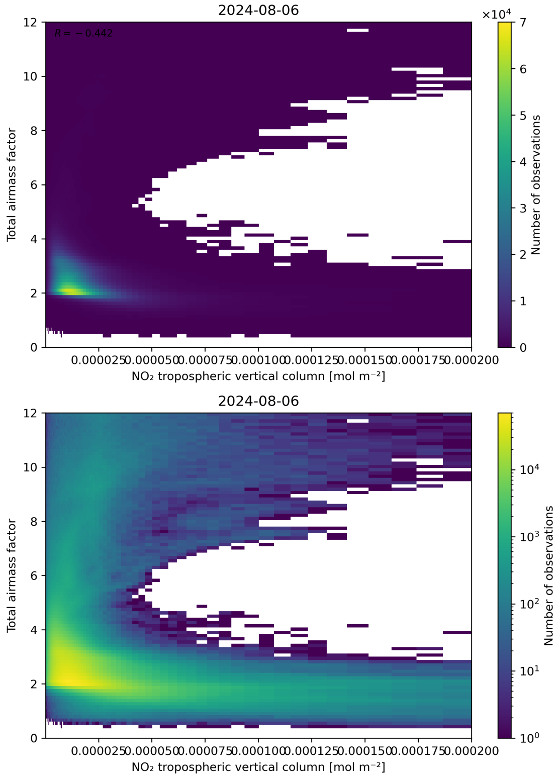
Figure 122: Scatter density plot of “NO 2 tropospheric vertical column” against “Total airmass factor” for 2024-08-06 to 2024-08-07.
