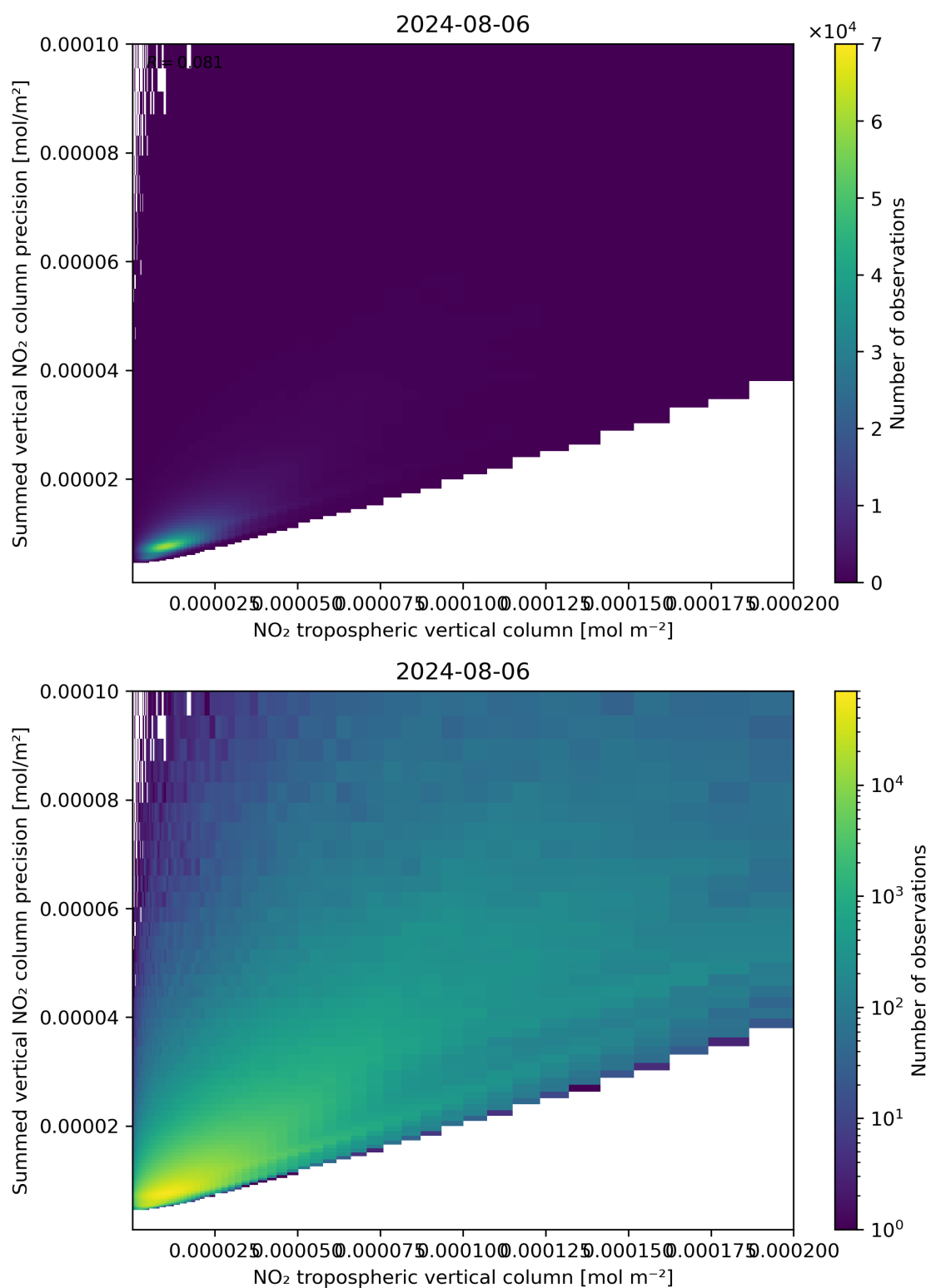
Figure 127: Scatter density plot of “NO 2 tropospheric vertical column” against “Summed vertical NO 2 column precision” for 2024-08-06 to 2024-08-07.
