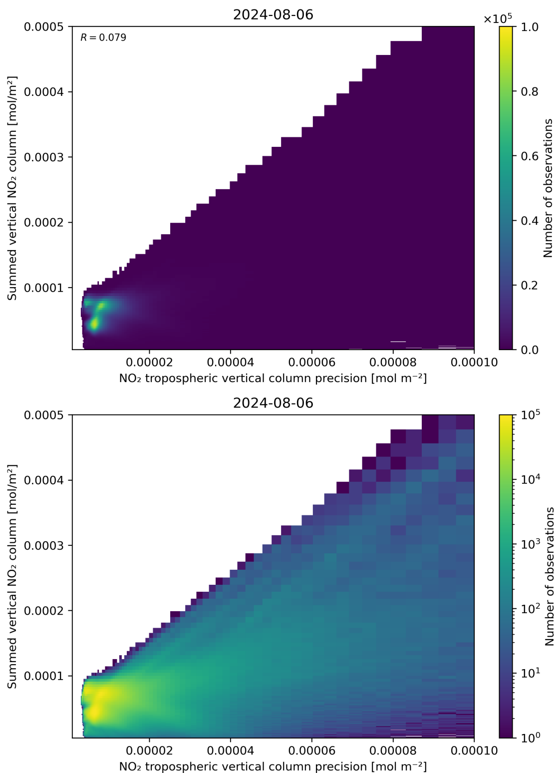
Figure 136: Scatter density plot of “NO 2 tropospheric vertical column precision” against “Summed vertical NO 2 column” for 2024-08-06 to 2024-08-07.
