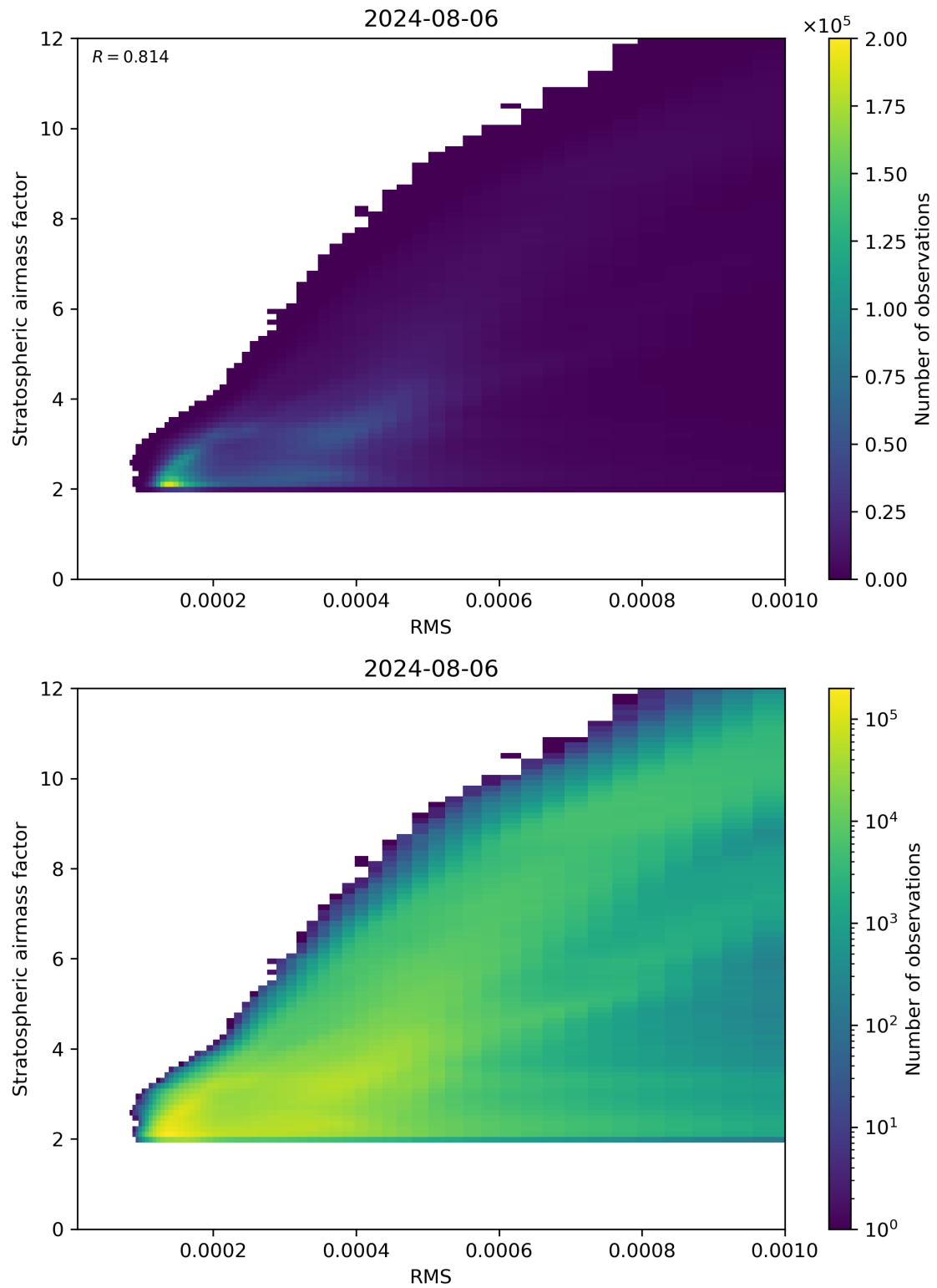
Figure 144: Scatter density plot of “RMS” against “Stratospheric airmass factor” for 2024-08-06 to 2024-08-07.
