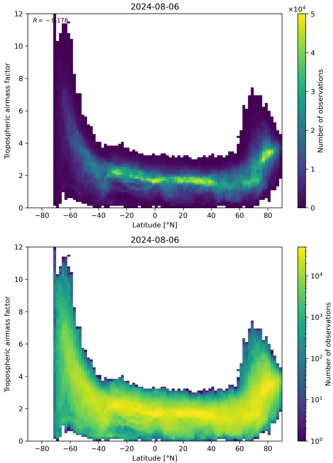
Figure 85: Scatter density plot of “Latitude” against “Tropospheric air mass factor” for 2024-08-06 to 2024-08-07.
