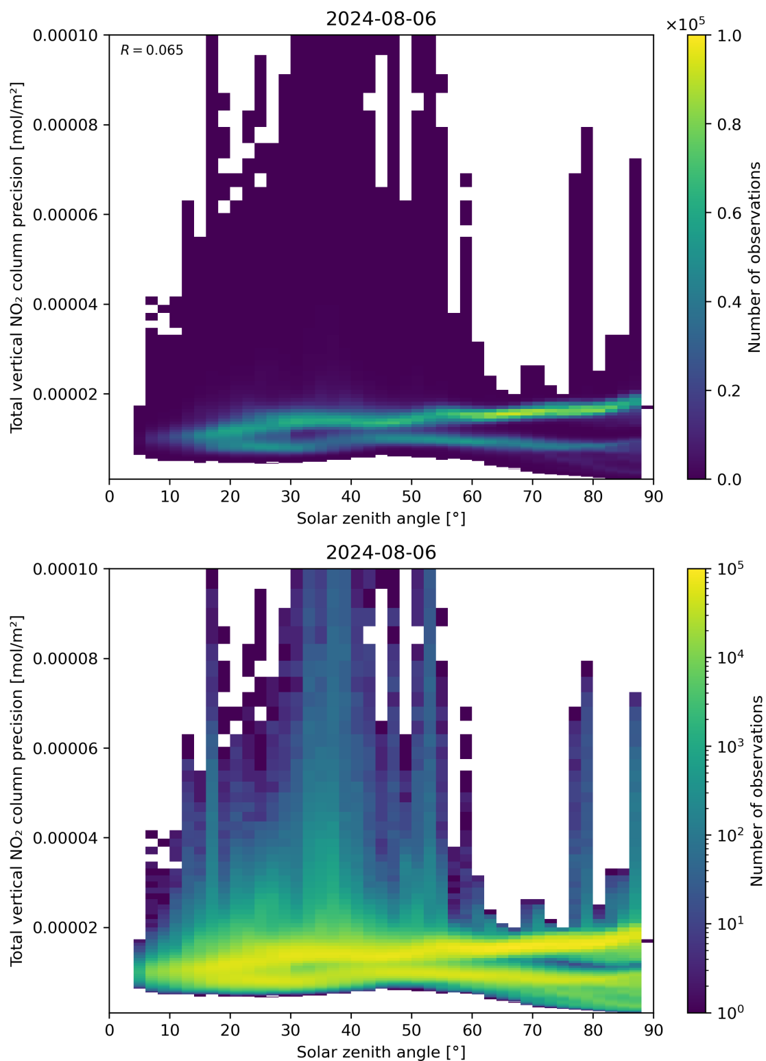
Figure 154: Scatter density plot of “Solar zenith angle” against “Total vertical NO 2 column precision” for 2024-08-06 to 2024-08-07.
