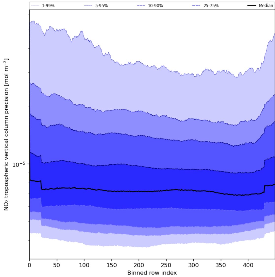
Figure 47: Along track statistics of “NO 2 tropospheric vertical column precision” for 2024-08-06 to 2024-08-07
