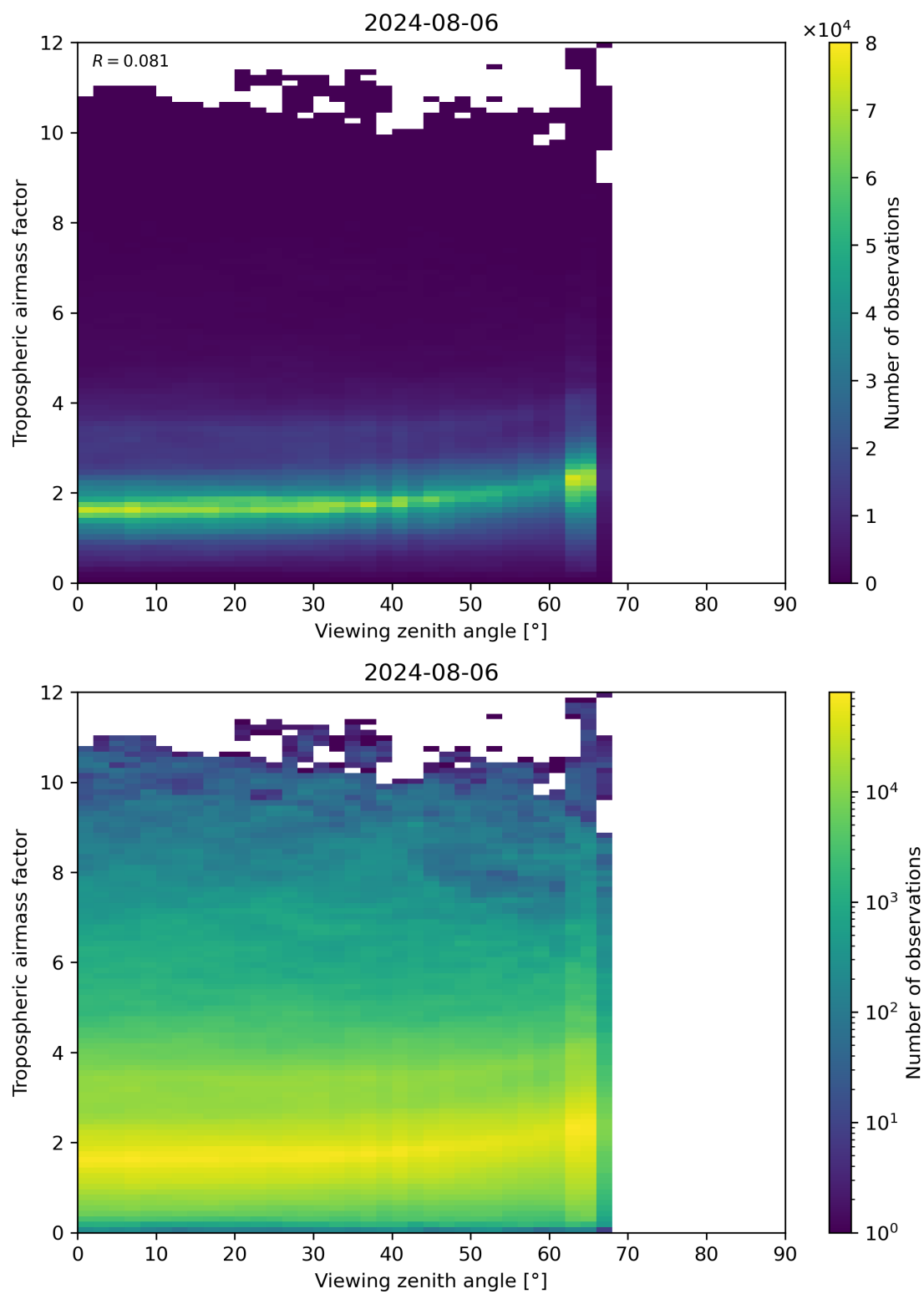
Figure 161: Scatter density plot of “Viewing zenith angle” against “Tropospheric airmass factor” for 2024-08-06 to 2024-08-07.
