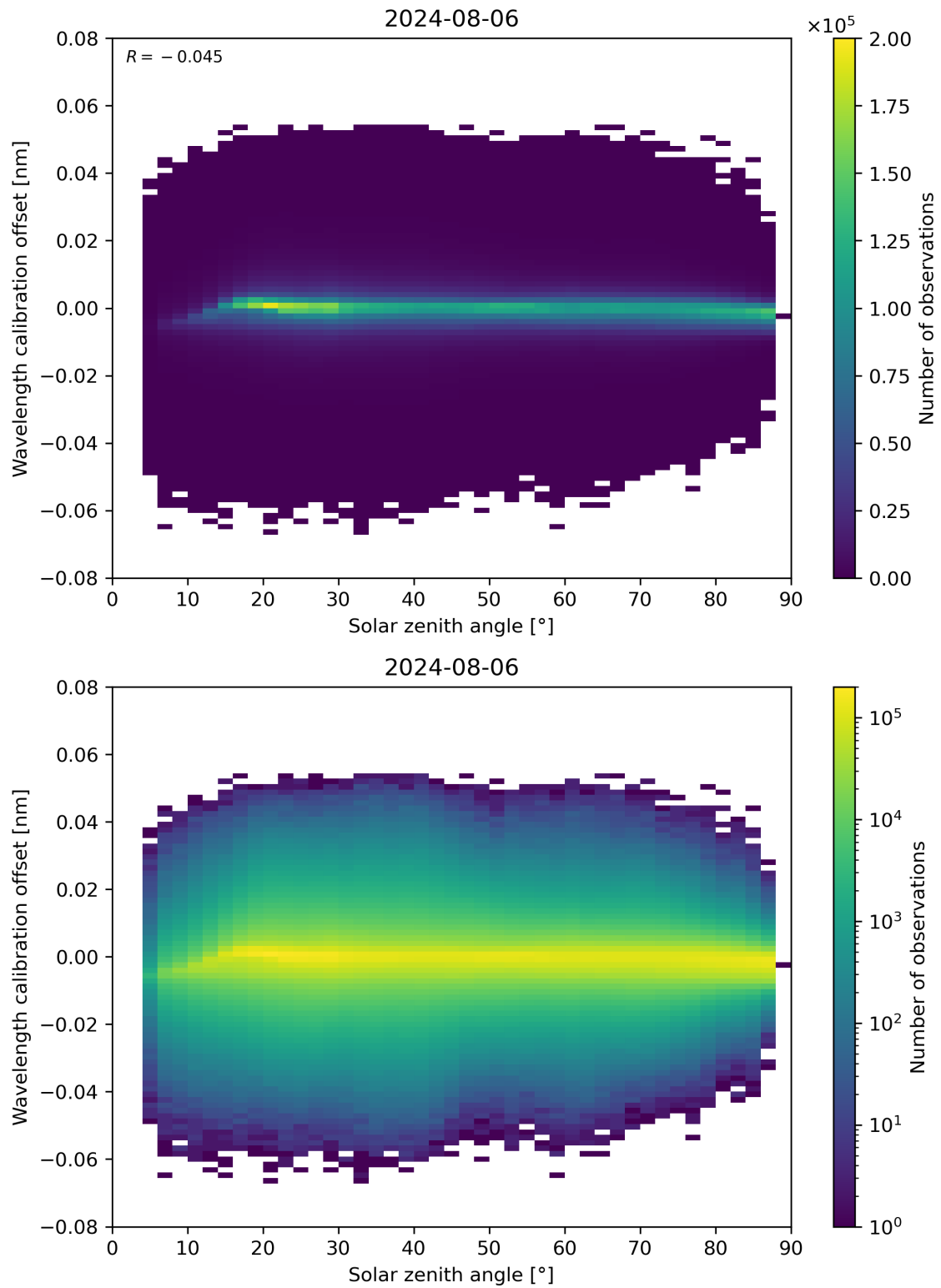
Figure 158: Scatter density plot of “Solar zenith angle” against “Wavelength calibration offset” for 2024-08-06 to 2024-08-07.
