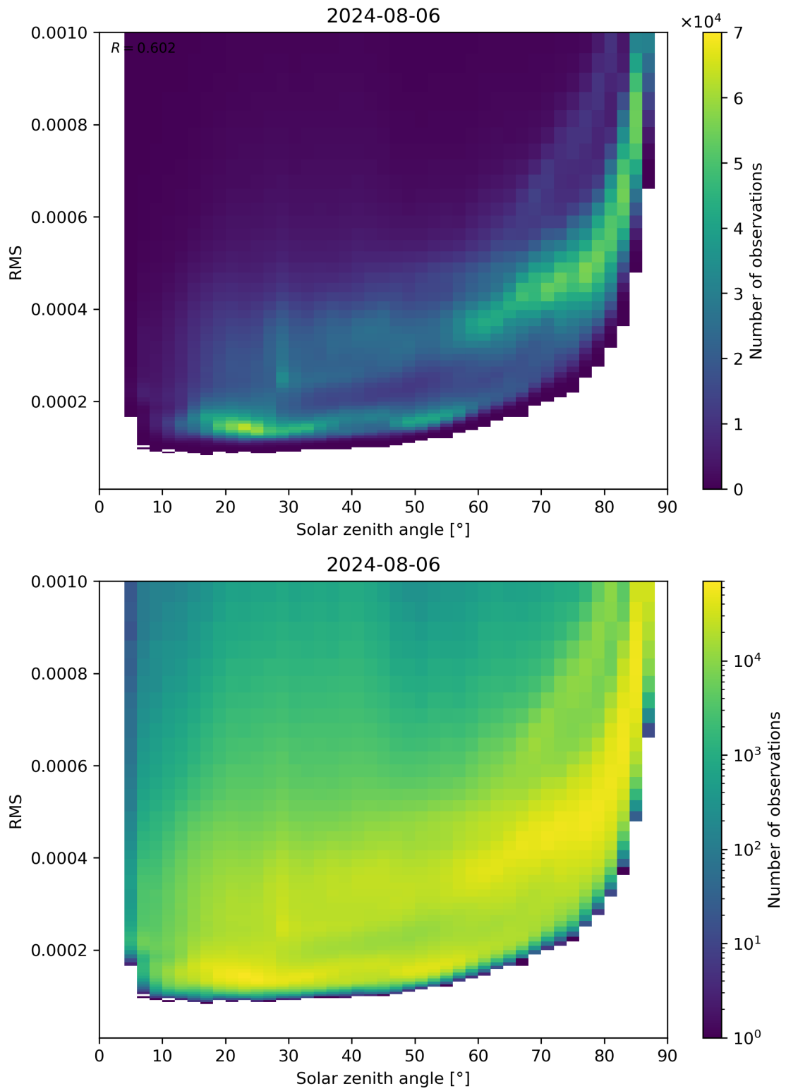
Figure 157: Scatter density plot of “Solar zenith angle” against “RMS” for 2024-08-06 to 2024-08-07.
