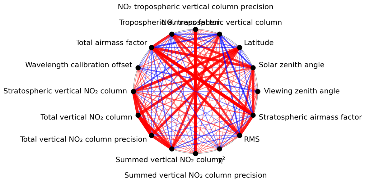
Figure 1: Map of correlation graph for 2024-08-06 to 2024-08-07.
