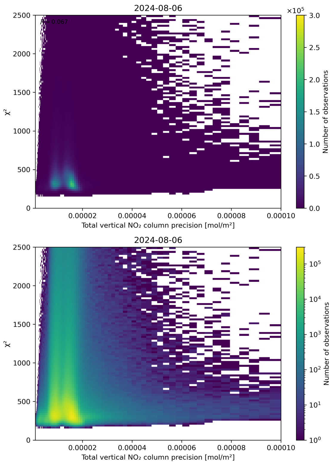
Figure 116: Scatter density plot of “Total vertical NO 2 column precision” against “ \chi^2 ” for 2024-08-06 to 2024-08-07.
