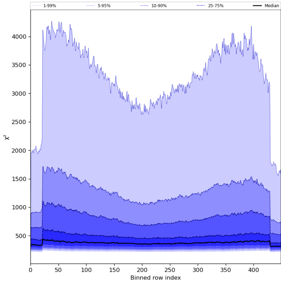
Figure 59: Along track statistics of “ \chi^2 ” for 2024-08-06 to 2024-08-07
