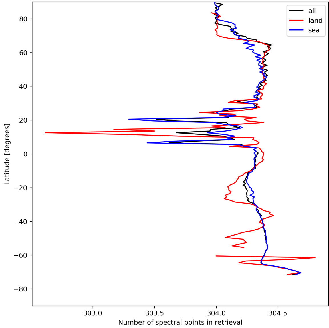
Figure 16: Zonal average of “Number of spectral points in retrieval” for 2024-08-06 to 2024-08-07.
