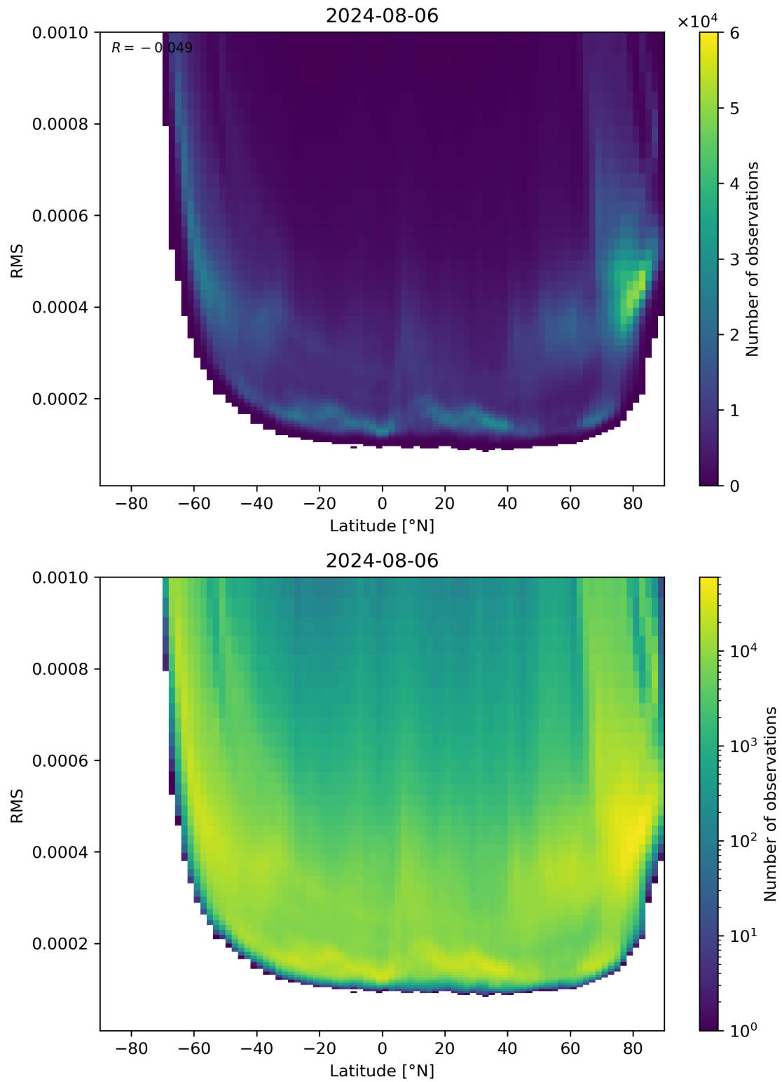
Figure 94: Scatter density plot of “Latitude” against “RMS” for 2024-08-06 to 2024-08-07.
