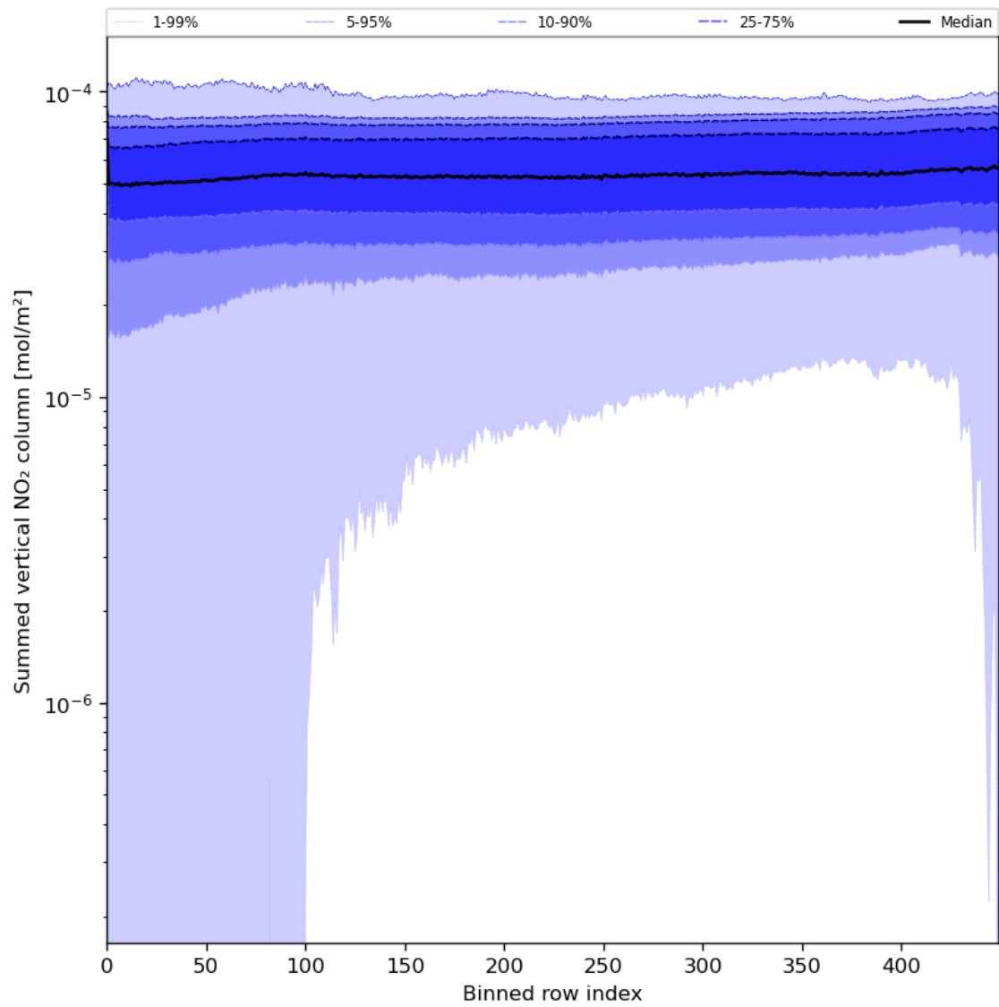
Figure 57: Along track statistics of “Summed vertical NO 2 column” for 2024-08-06 to 2024-08-07
