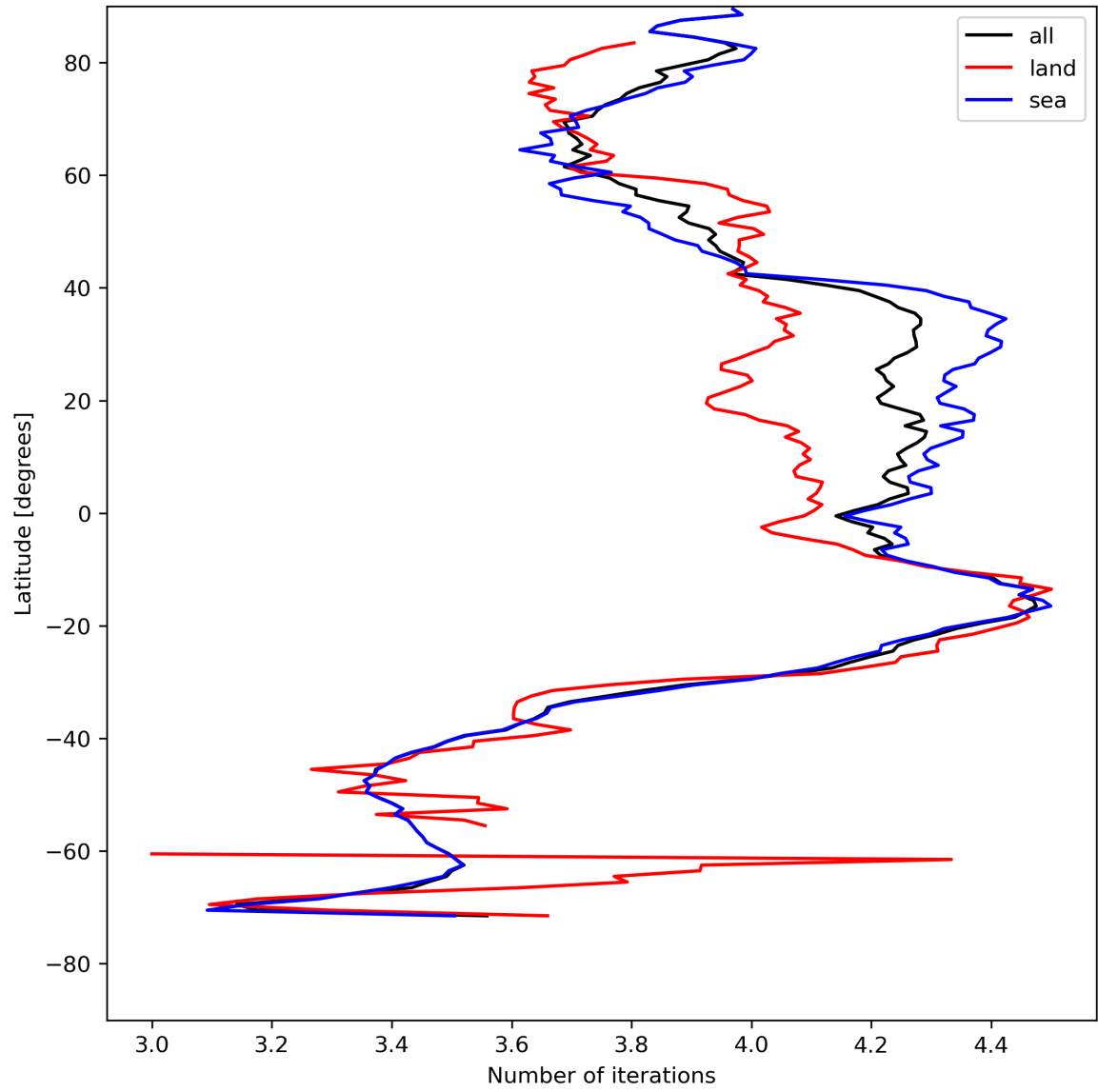
Figure 17: Zonal average of “Number of iterations” for 2024-08-06 to 2024-08-07.
