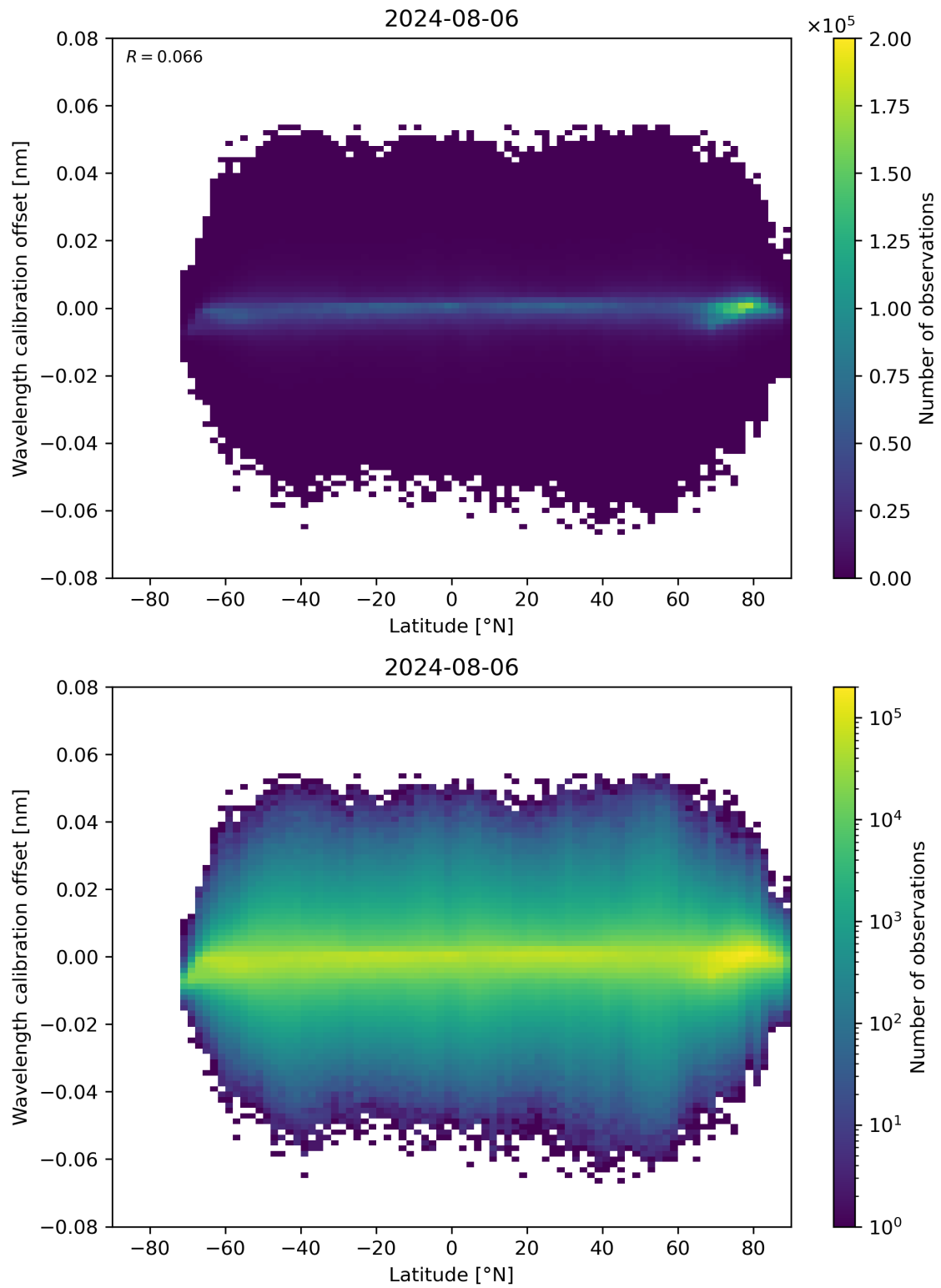
Figure 95: Scatter density plot of “Latitude” against “Wavelength calibration offset” for 2024-08-06 to 2024-08-07.
