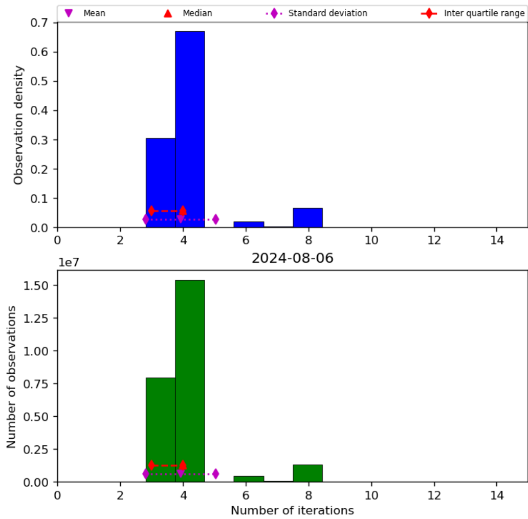
Figure 34: Histogram of “Number of iterations” for 2024-08-06 to 2024-08-07
