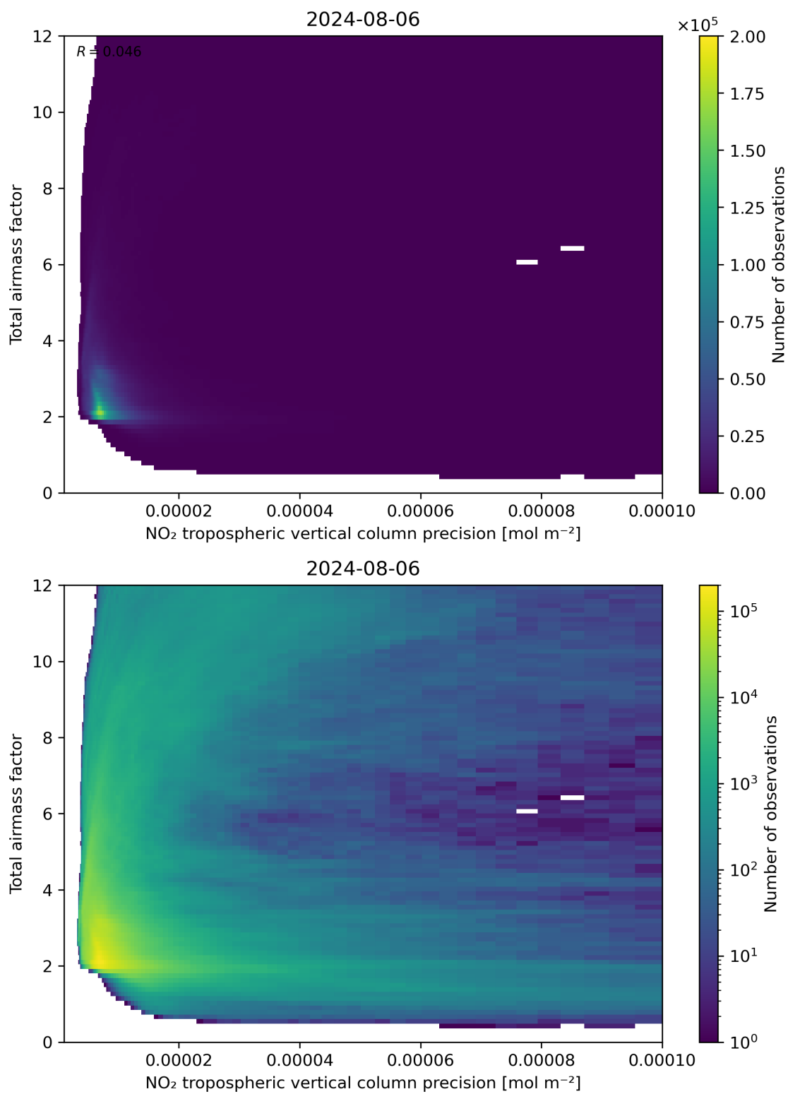
Figure 132: Scatter density plot of “NO 2 tropospheric vertical column precision” against “Total air mass factor” for 2024-08-06 to 2024-08-07.
