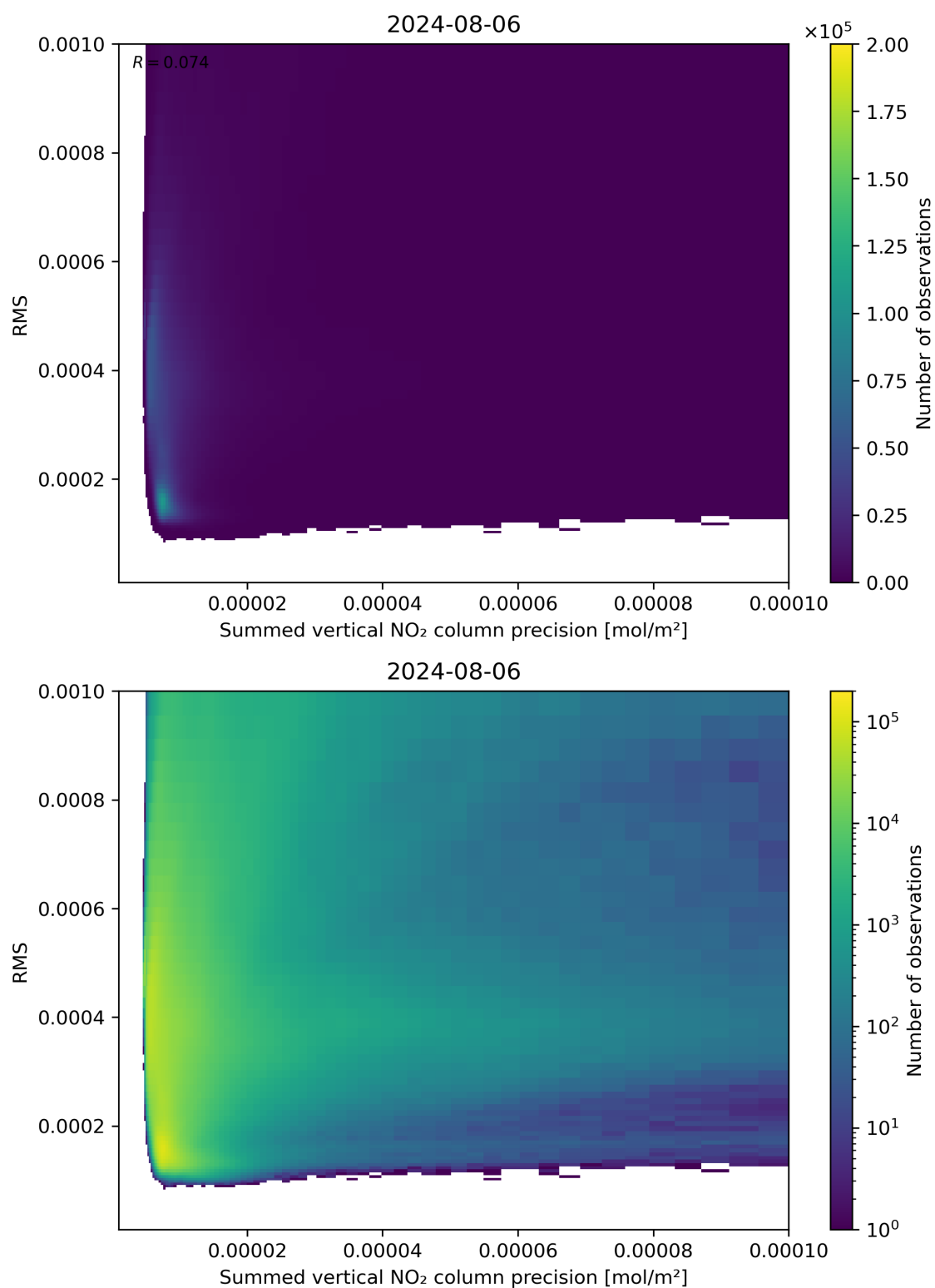
Figure 108: Scatter density plot of “Summed vertical NO 2 column precision” against “RMS” for 2024-08-06 to 2024-08-07.
