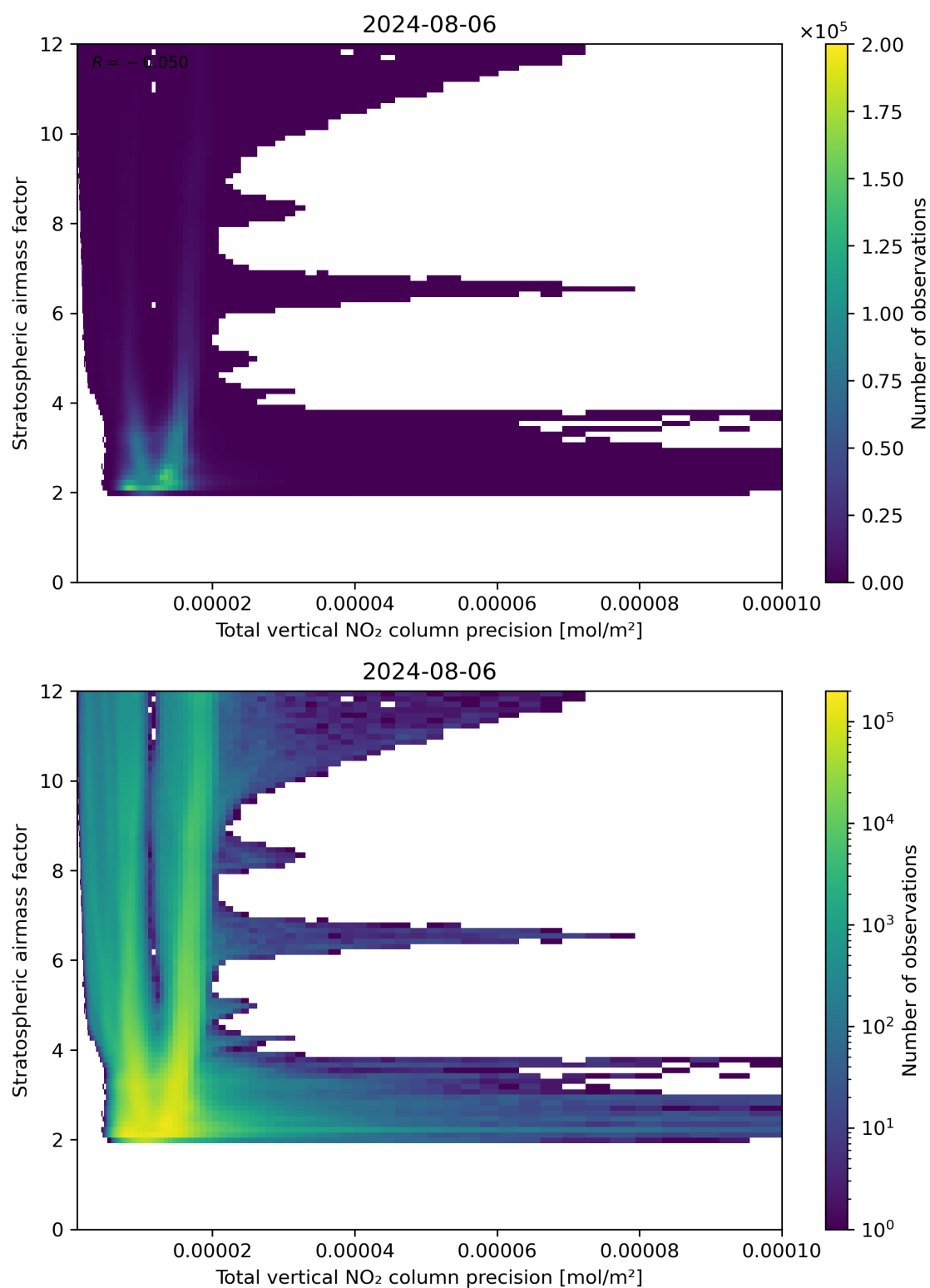
Figure 115: Scatter density plot of “Total vertical NO 2 column precision” against “Stratospheric air mass factor” for 2024-08-06 to 2024-08-07.
