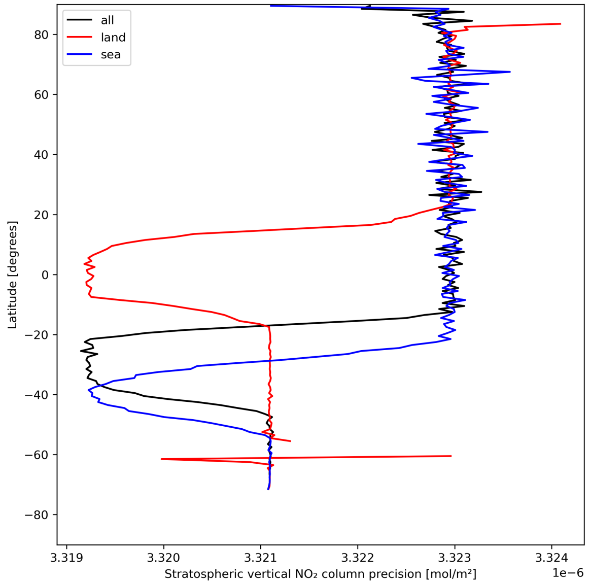
Figure 20: Zonal average of “Stratospheric vertical NO 2 column precision” for 2024-08-06 to 2024-08-07.
