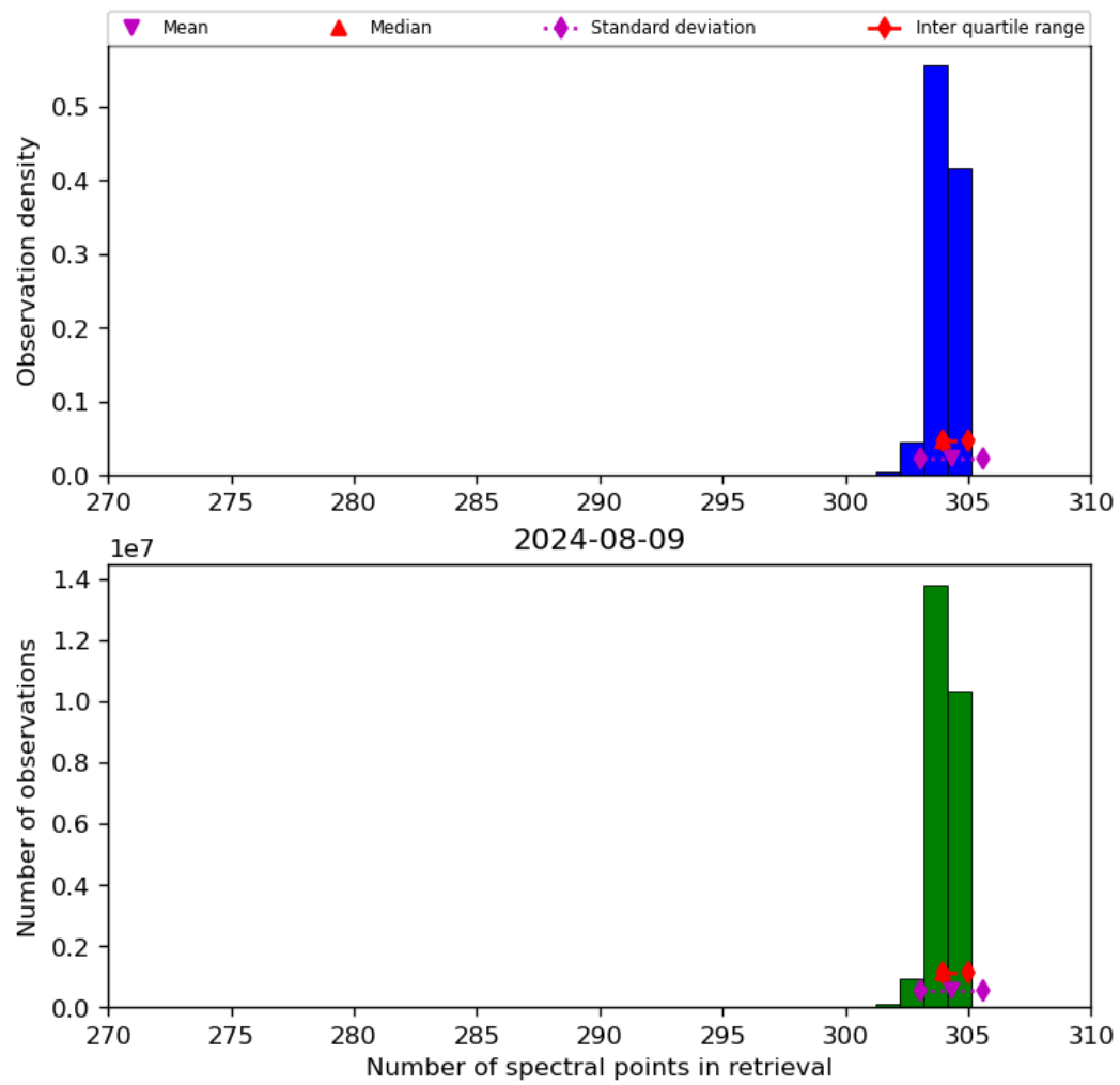
Figure 33: Histogram of “Number of spectral points in retrieval” for 2024-08-08 to 2024-08-10
