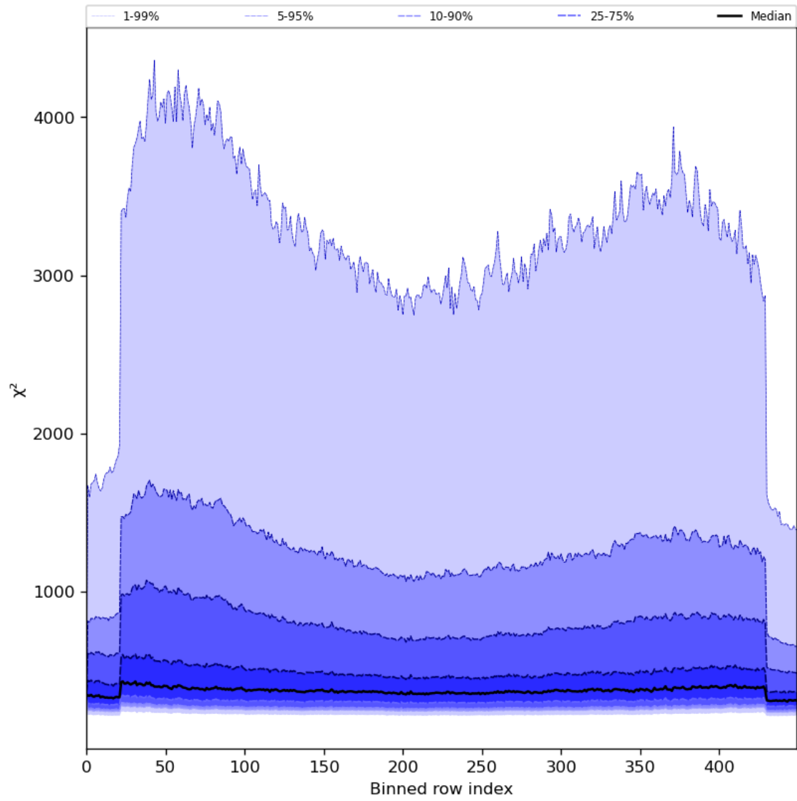
Figure 59: Along track statistics of “ \chi^2 ” for 2024-08-08 to 2024-08-10
