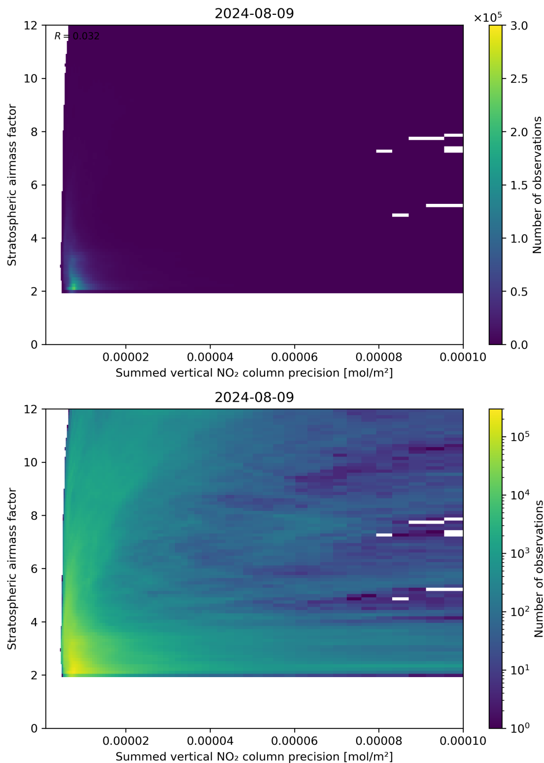
Figure 106: Scatter density plot of “Summed vertical NO 2 column precision” against “Stratospheric airmass factor” for 2024-08-08 to 2024-08-10.
