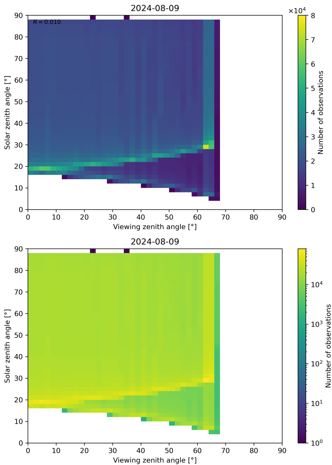
Figure 172: Scatter density plot of “Viewing zenith angle” against “Solar zenith angle” for 2024-08-08 to 2024-08-10.
