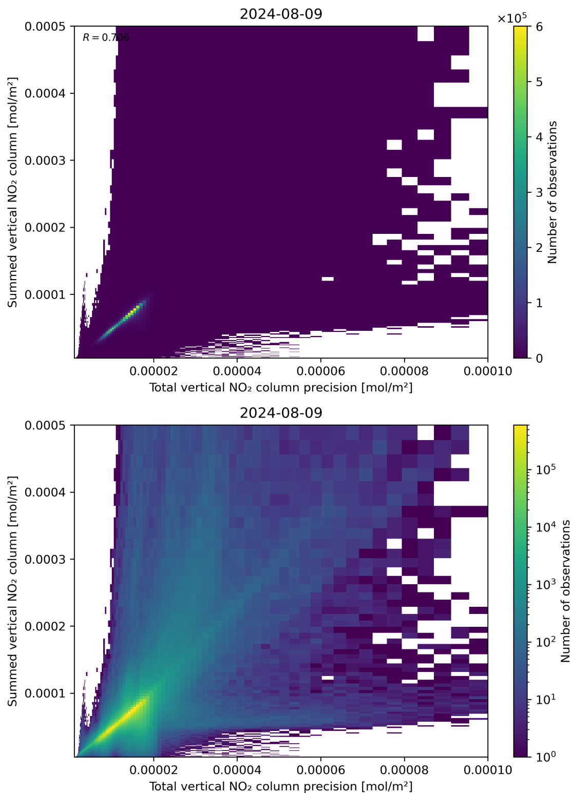
Figure 117: Scatter density plot of “Total vertical NO 2 column precision” against “Summed vertical NO 2 column” for 2024-08-08 to 2024-08-10.
