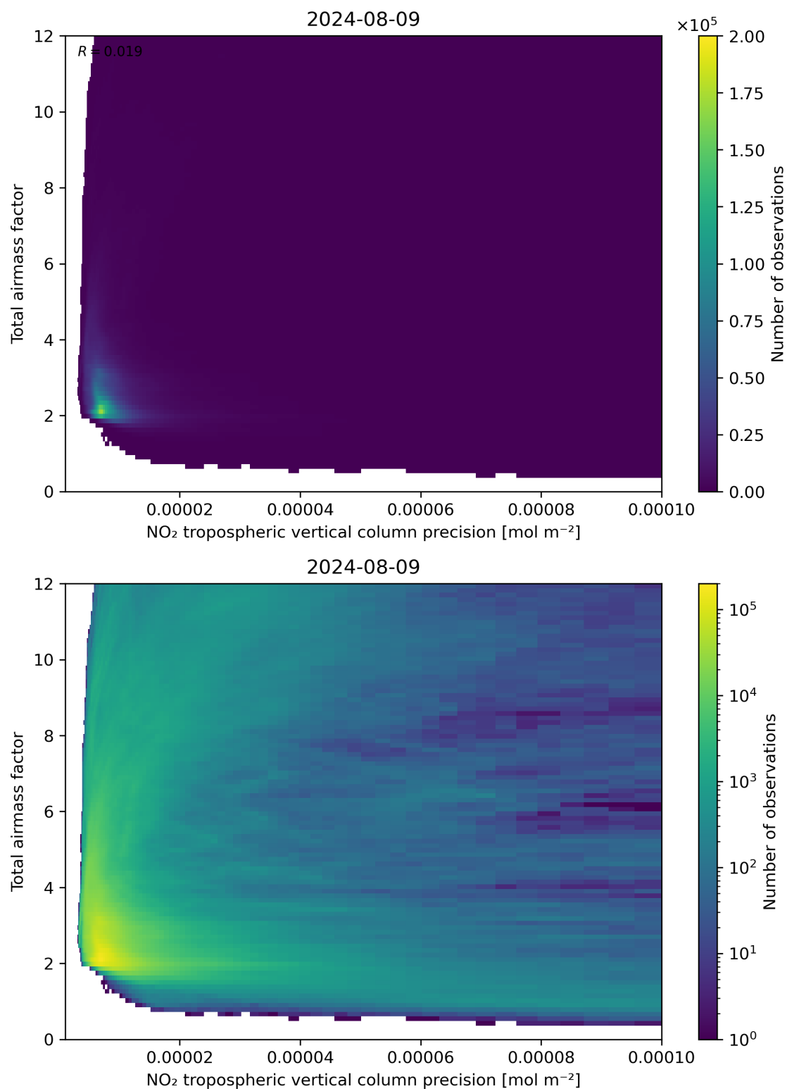
Figure 132: Scatter density plot of “NO 2 tropospheric vertical column precision” against “Total air mass factor” for 2024-08-08 to 2024-08-10.
