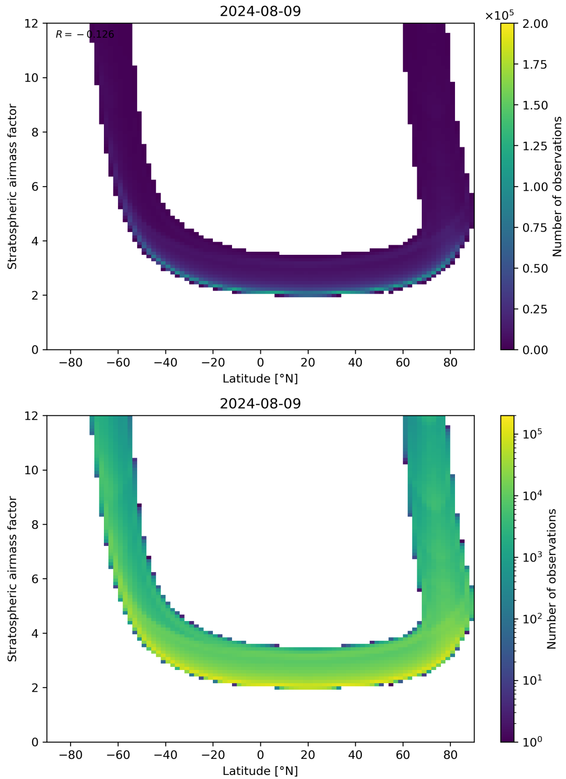
Figure 83: Scatter density plot of “Latitude” against “Stratospheric air mass factor” for 2024-08-08 to 2024-08-10.
