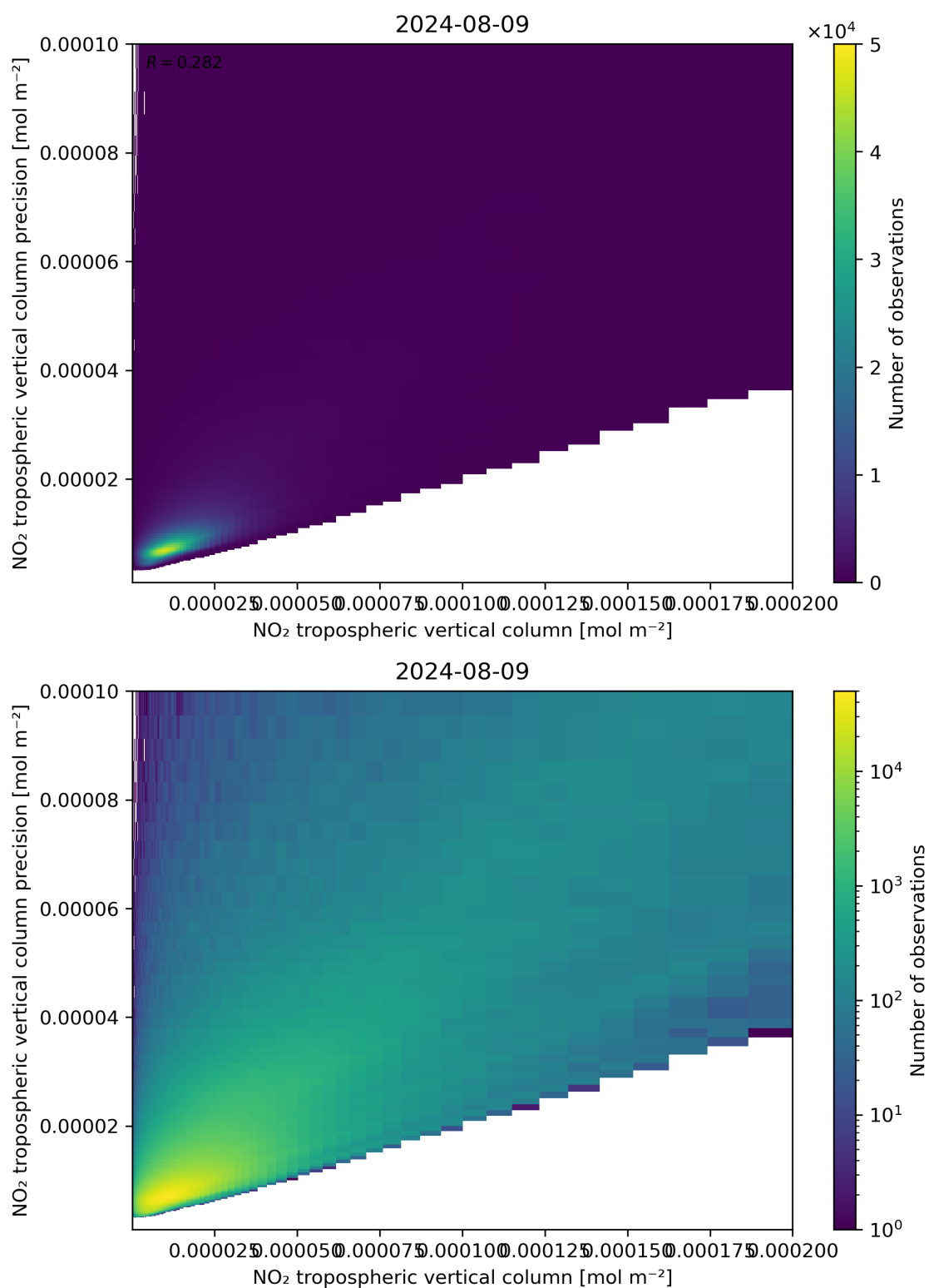
Figure 130: Scatter density plot of “NO 2 tropospheric vertical column” against “NO 2 tropospheric vertical column precision” for 2024-08-08 to 2024-08-10.
