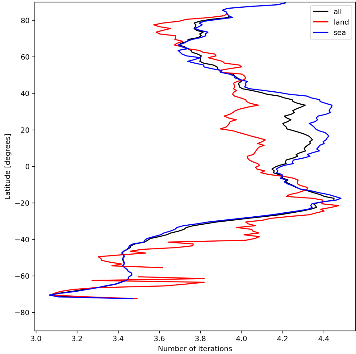
Figure 17: Zonal average of “Number of iterations” for 2024-08-08 to 2024-08-10.
