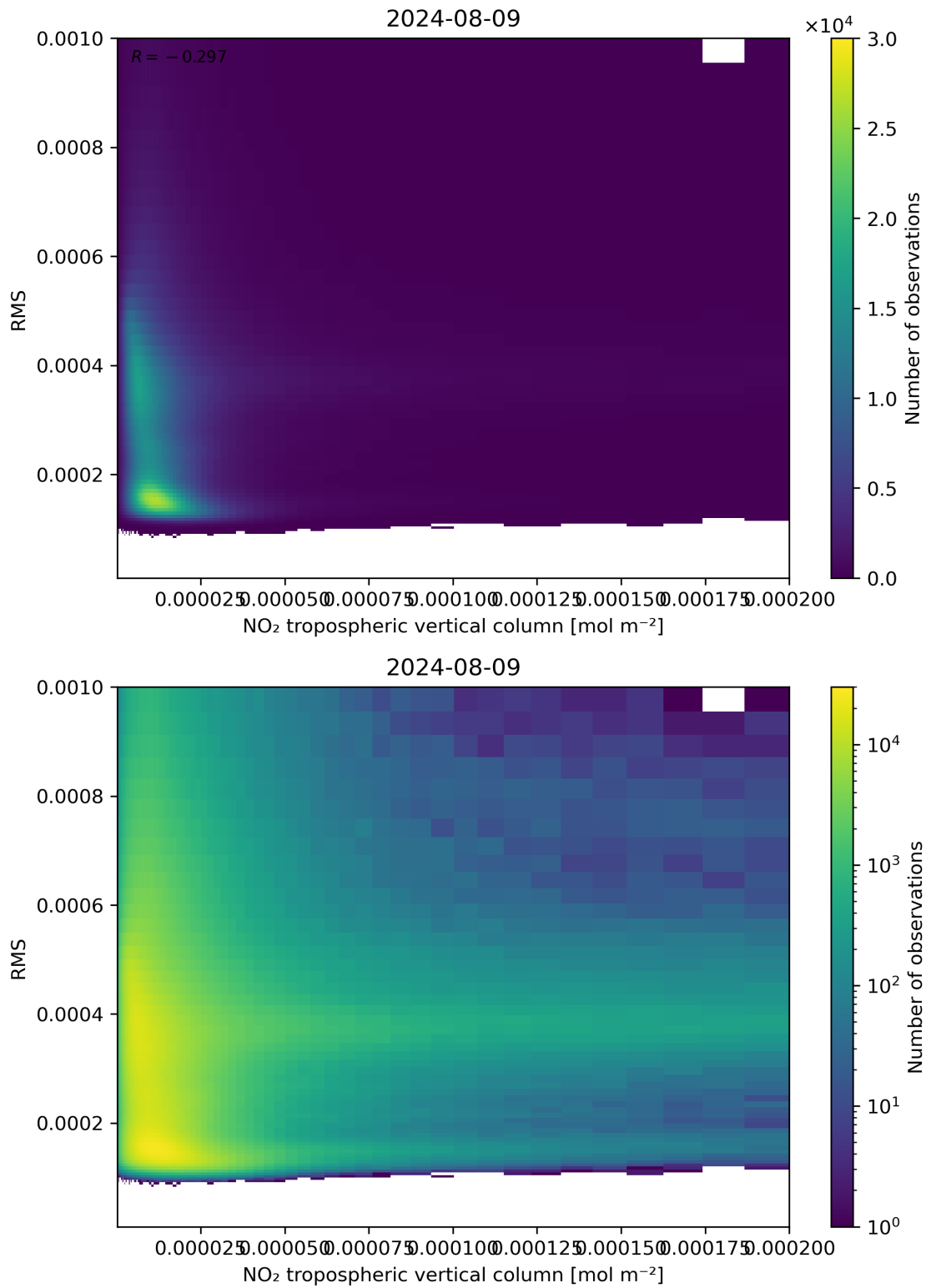
Figure 142: Scatter density plot of “NO 2 tropospheric vertical column” against “RMS” for 2024-08-08 to 2024-08-10.
