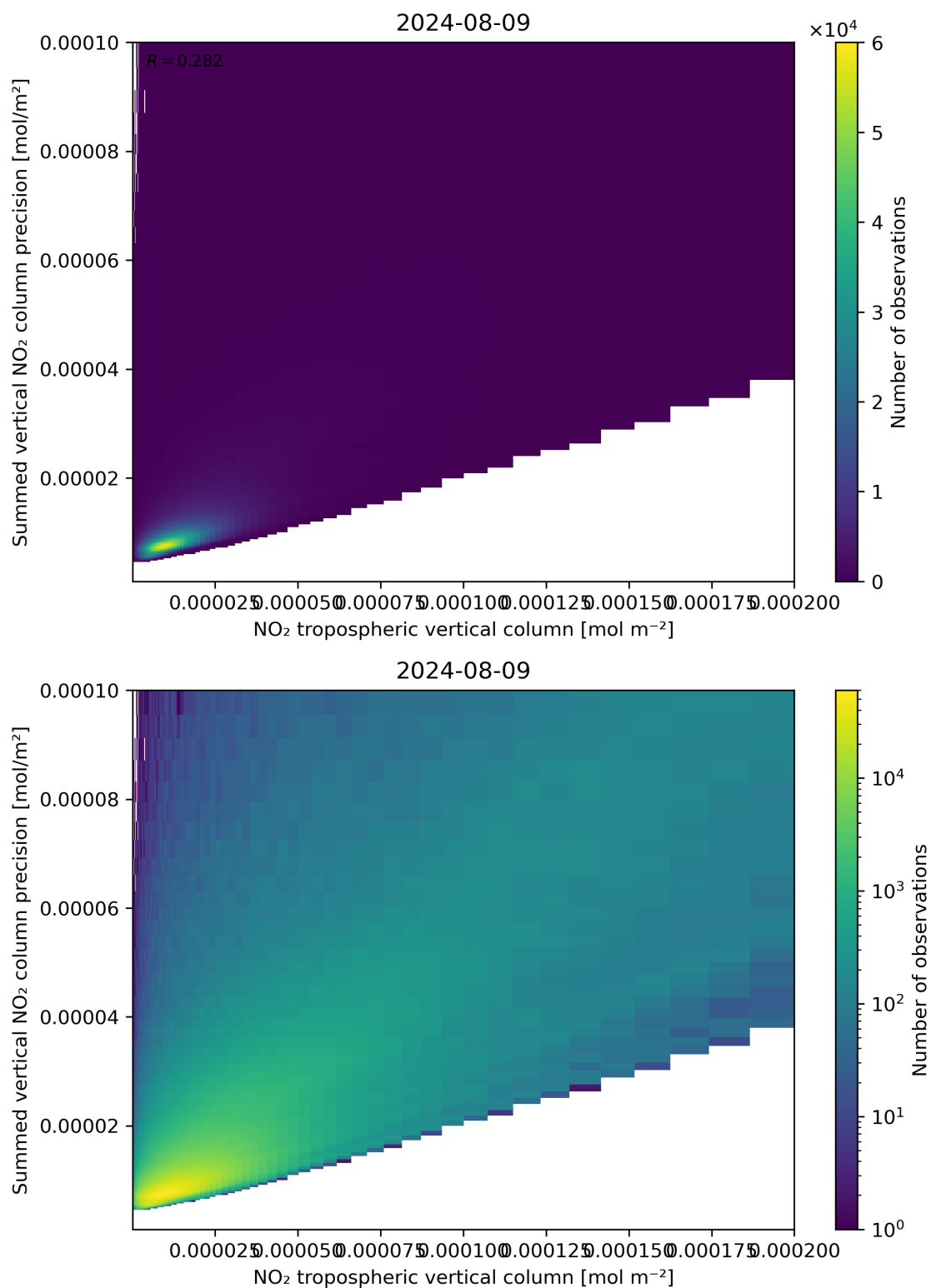
Figure 127: Scatter density plot of “NO 2 tropospheric vertical column” against “Summed vertical NO 2 column precision” for 2024-08-08 to 2024-08-10.
