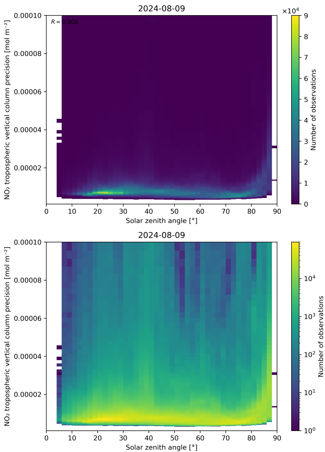
Figure 156: Scatter density plot of “Solar zenith angle” against “NO 2 tropospheric vertical column precision” for 2024-08-08 to 2024-08-10.
