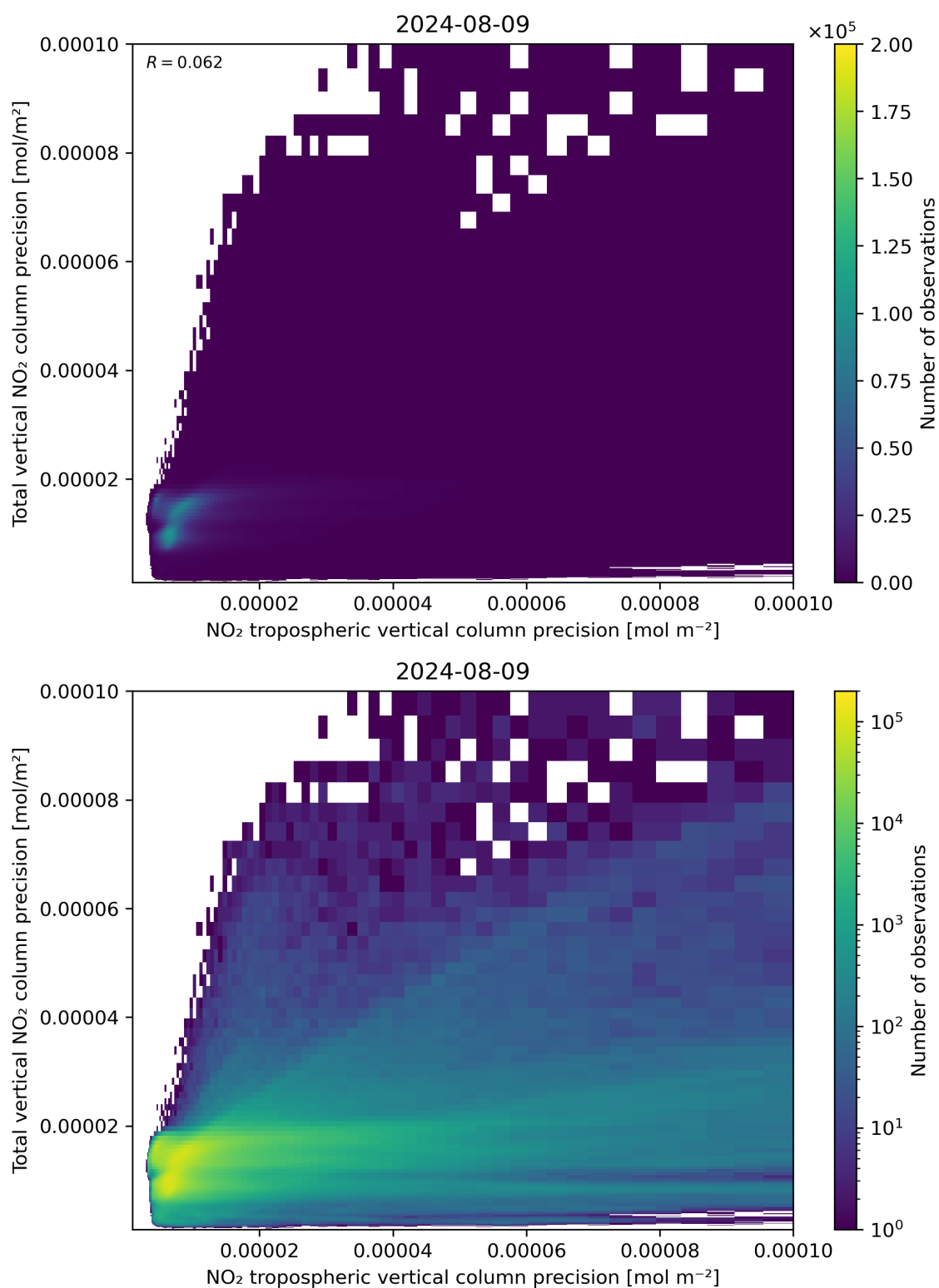
Figure 139: Scatter density plot of “NO 2 tropospheric vertical column precision” against “Total vertical NO 2 column precision” for 2024-08-08 to 2024-08-10.
