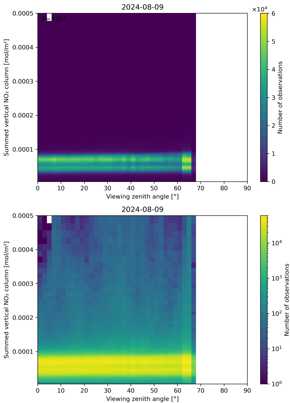
Figure 165: Scatter density plot of “Viewing zenith angle” against “Summed vertical NO 2 column” for 2024-08-08 to 2024-08-10.
