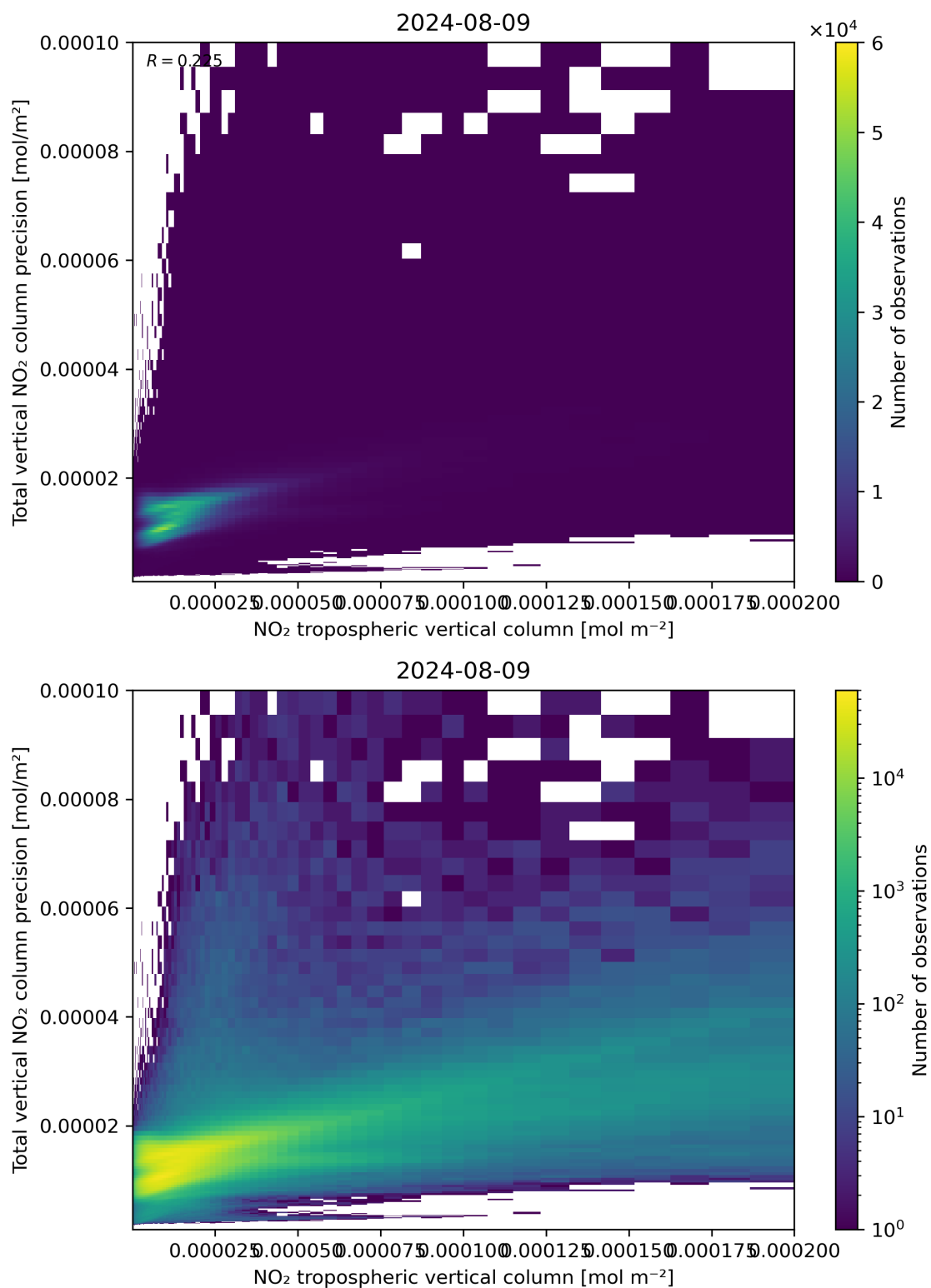
Figure 129: Scatter density plot of “NO 2 tropospheric vertical column” against “Total vertical NO 2 column precision” for 2024-08-08 to 2024-08-10.
