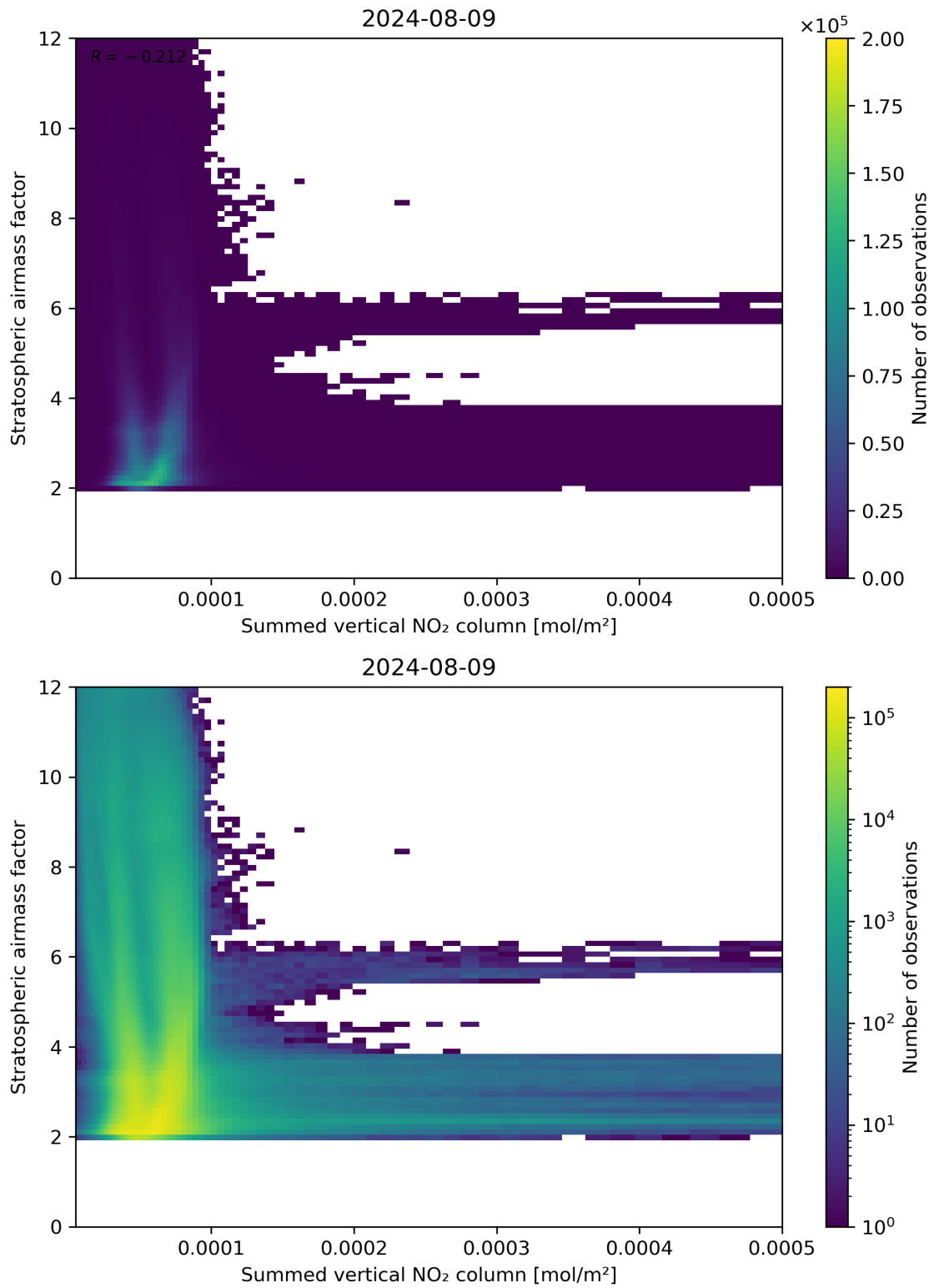
Figure 103: Scatter density plot of “Summed vertical NO 2 column” against “Stratospheric air mass factor” for 2024-08-08 to 2024-08-10.
