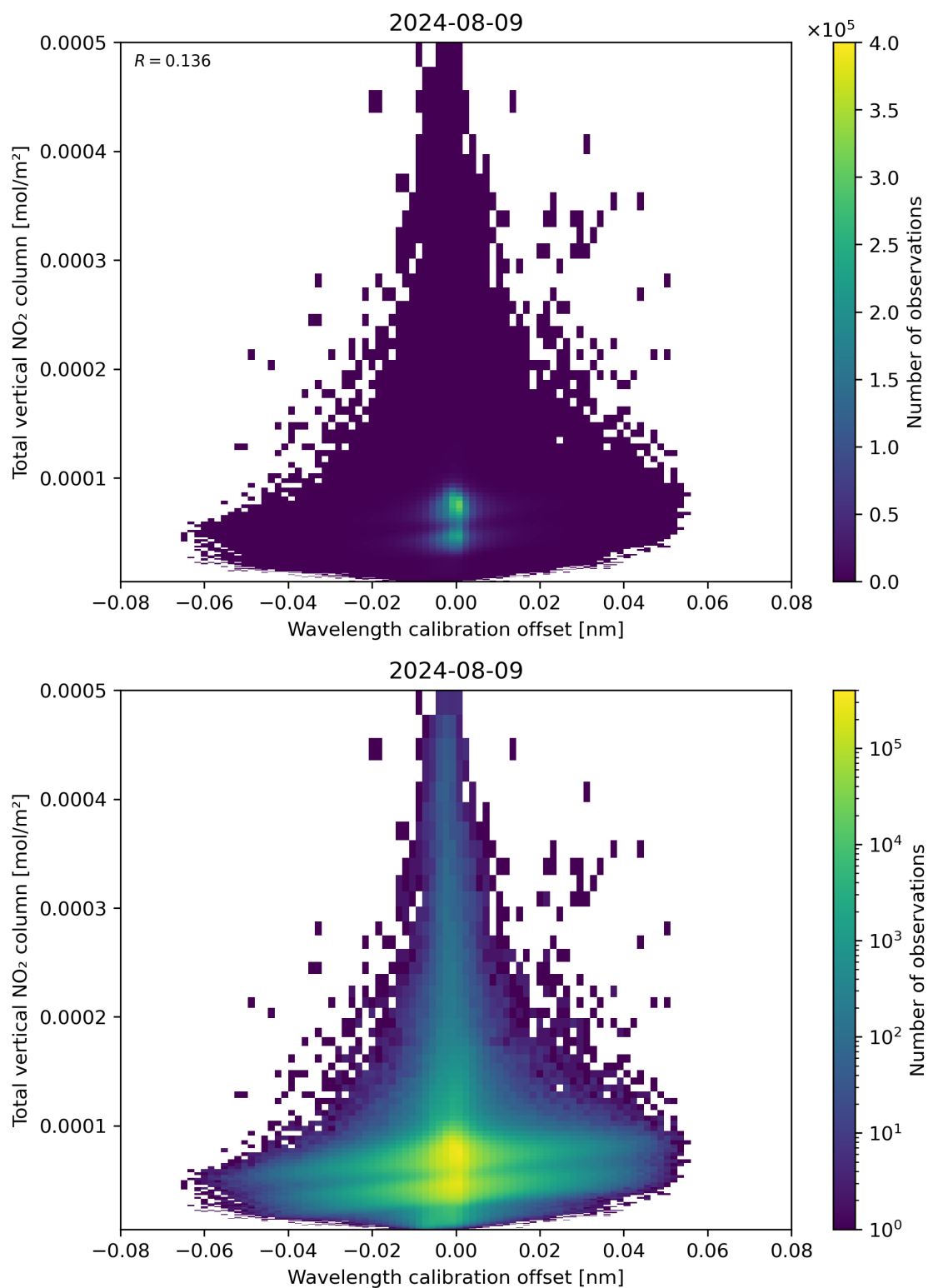
Figure 179: Scatter density plot of “Wavelength calibration offset” against “Total vertical NO 2 column” for 2024-08-08 to 2024-08-10.
