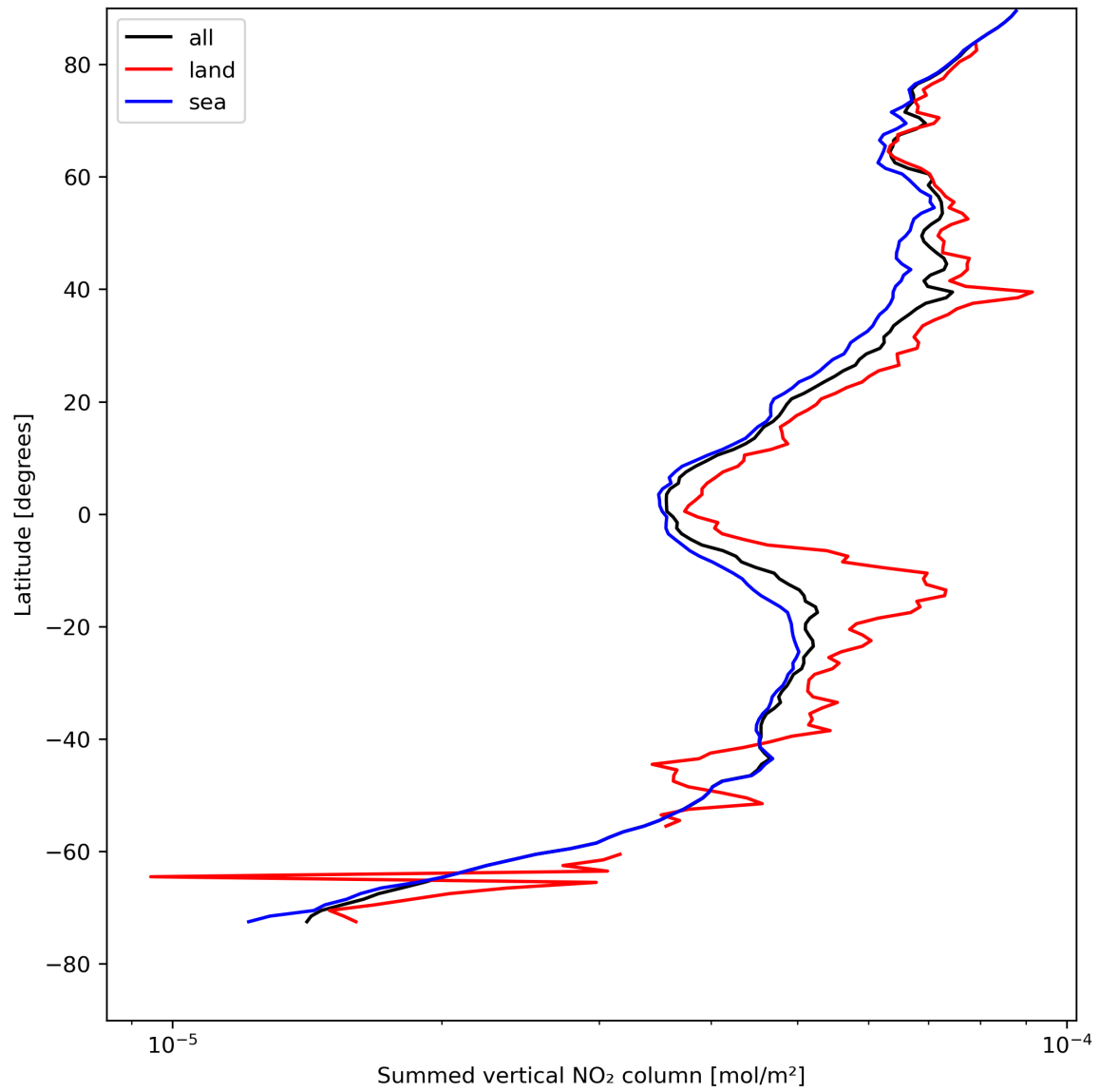
Figure 23: Zonal average of “Summed vertical NO 2 column” for 2024-08-08 to 2024-08-10.
