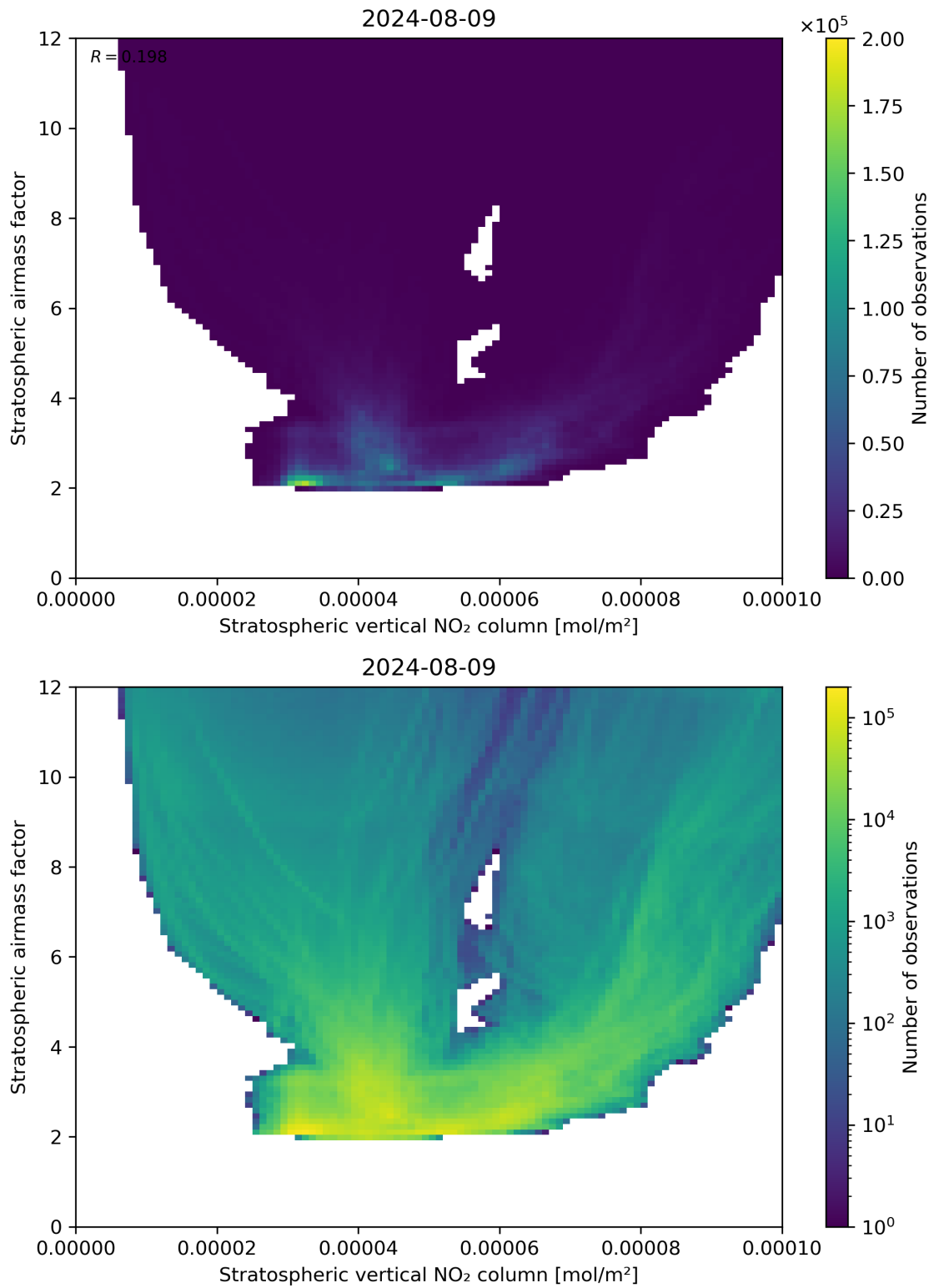
Figure 96: Scatter density plot of “Stratospheric vertical NO 2 column” against “Stratospheric airmass factor” for 2024-08-08 to 2024-08-10.
