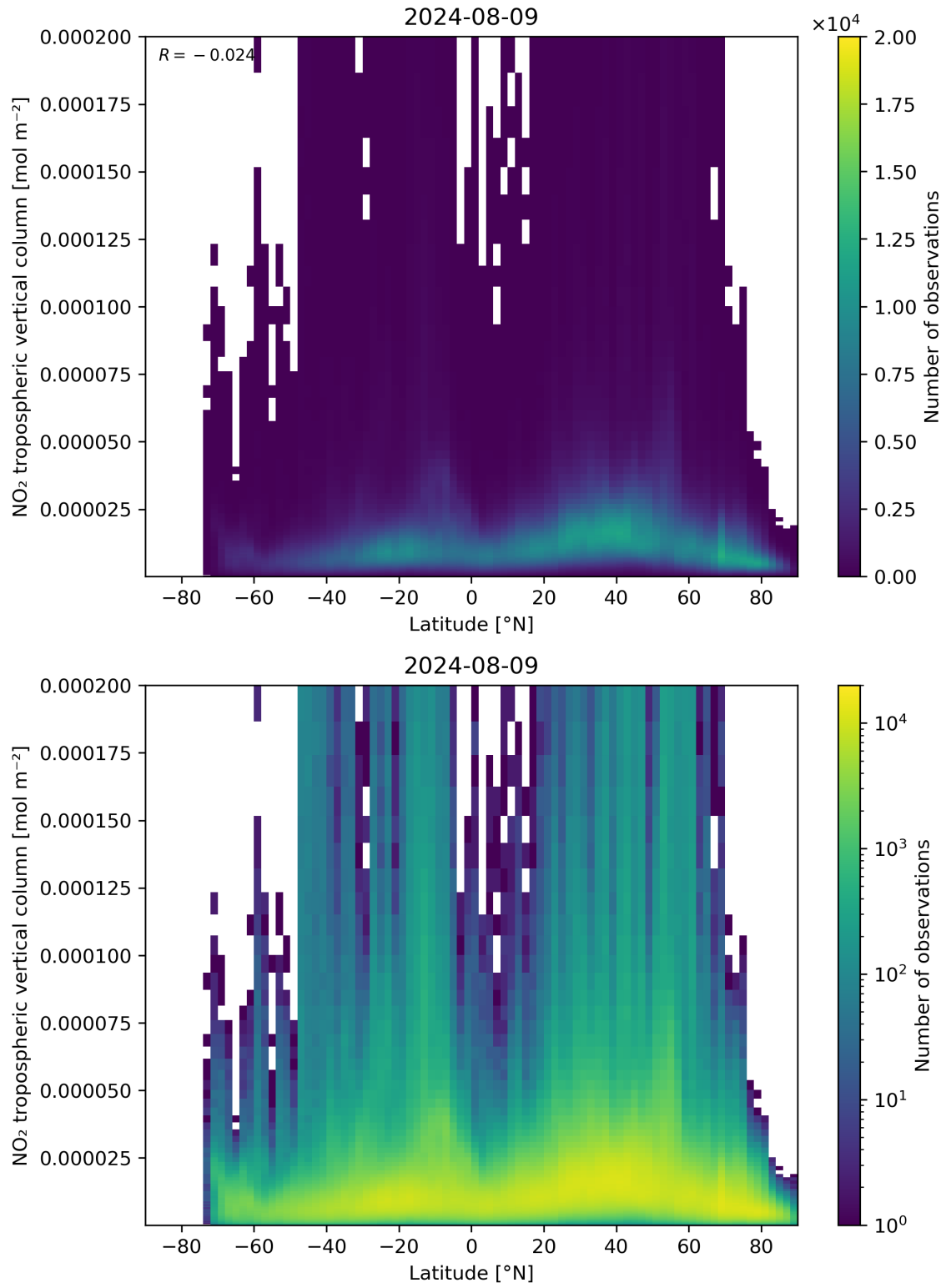
Figure 92: Scatter density plot of “Latitude” against “NO 2 tropospheric vertical column” for 2024-08-08 to 2024-08-10.
