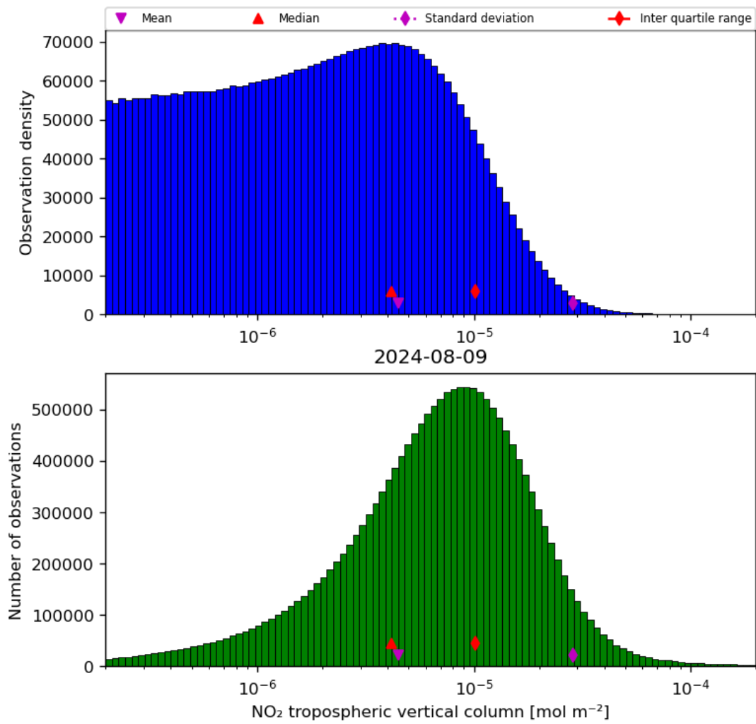
Figure 29: Histogram of “NO 2 tropospheric vertical column” for 2024-08-08 to 2024-08-10
