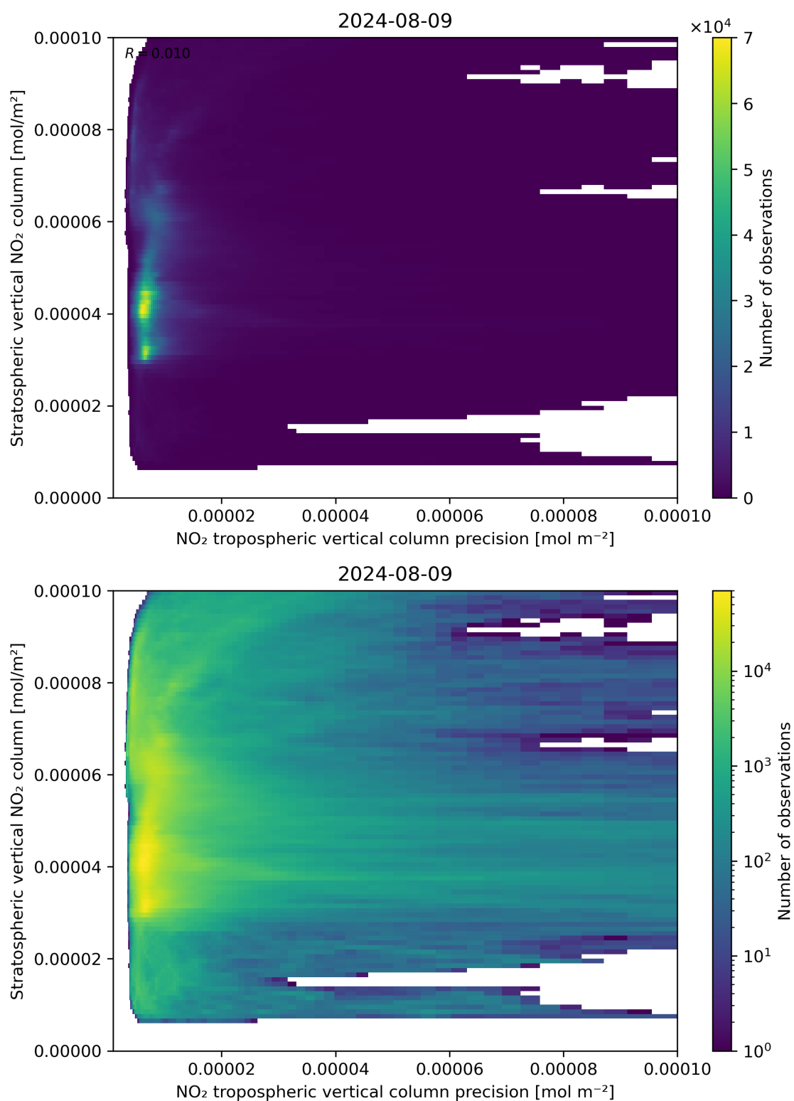
Figure 135: Scatter density plot of “NO 2 tropospheric vertical column precision” against “Stratospheric vertical NO 2 column” for 2024-08-08 to 2024-08-10.
