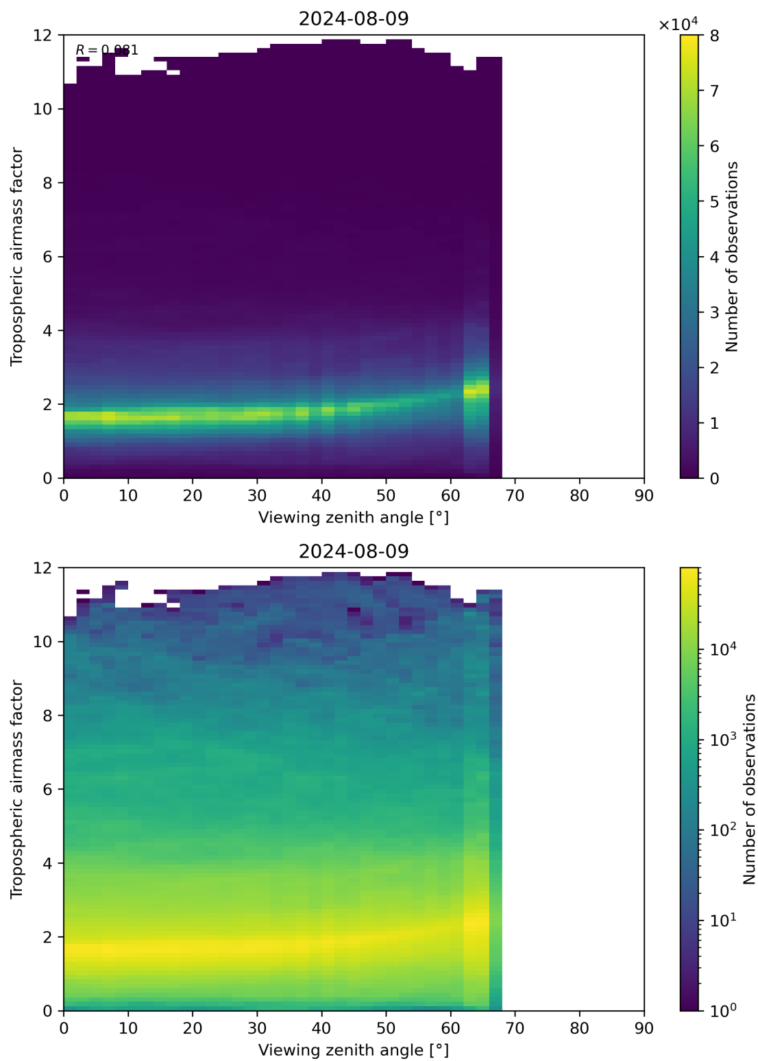
Figure 161: Scatter density plot of “Viewing zenith angle” against “Tropospheric airmass factor” for 2024-08-08 to 2024-08-10.
