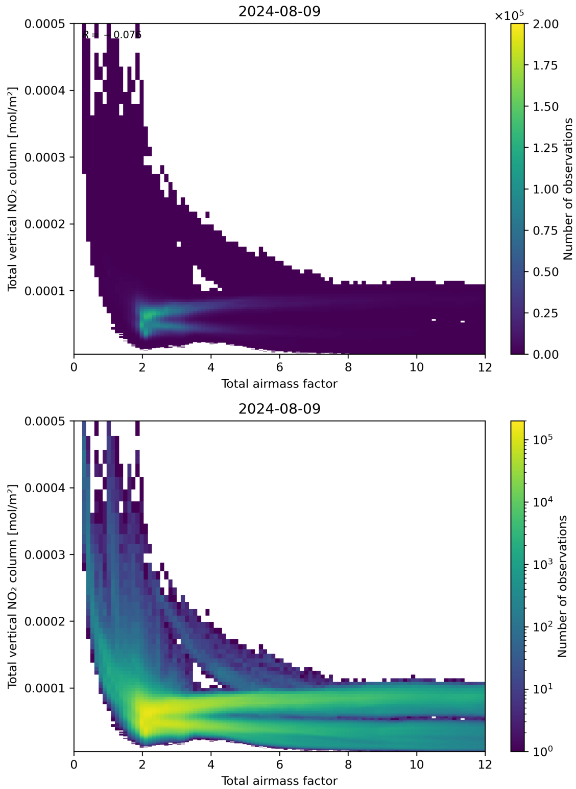
Figure 67: Scatter density plot of “Total airmass factor” against “Total vertical NO 2 column” for 2024-08-08 to 2024-08-10.
