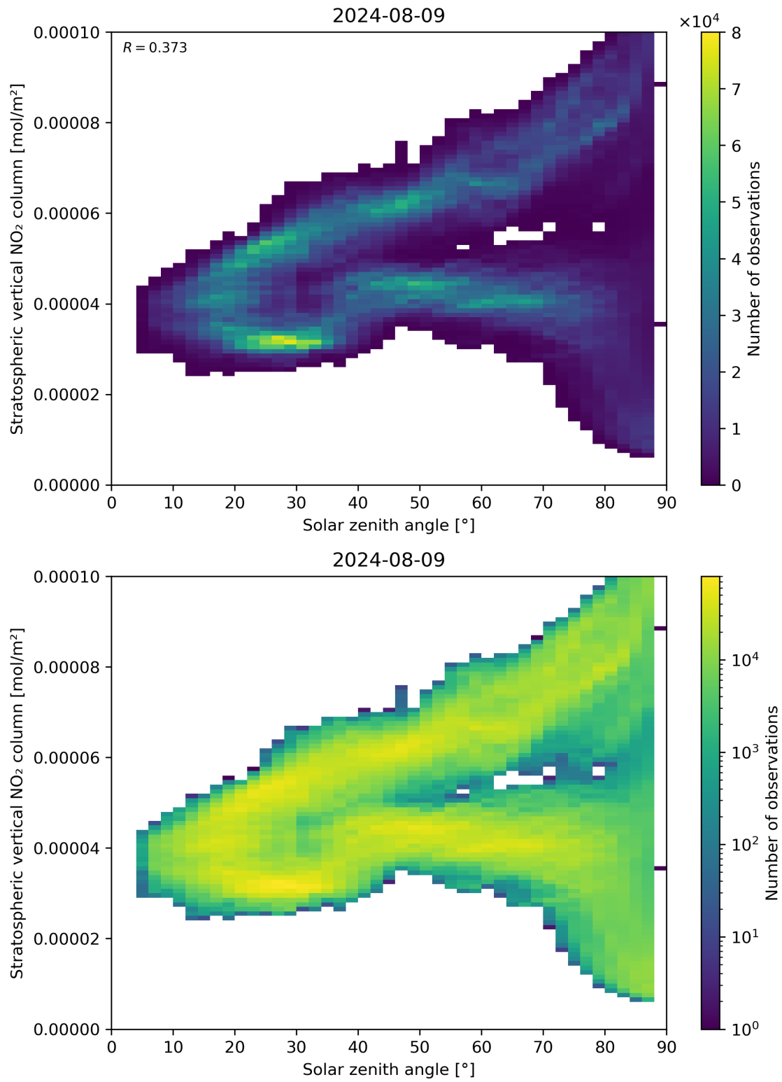
Figure 150: Scatter density plot of “Solar zenith angle” against “Stratospheric vertical NO 2 column” for 2024-08-08 to 2024-08-10.
