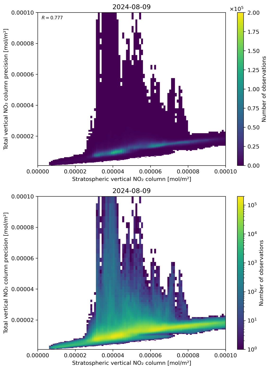
Figure 101: Scatter density plot of “Stratospheric vertical NO 2 column” against “Total vertical NO 2 column precision” for 2024-08-08 to 2024-08-10.
