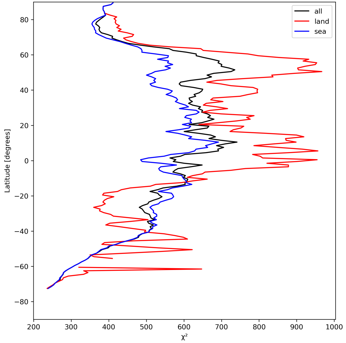
Figure 25: Zonal average of “ \chi^2 ” for 2024-08-08 to 2024-08-10.
