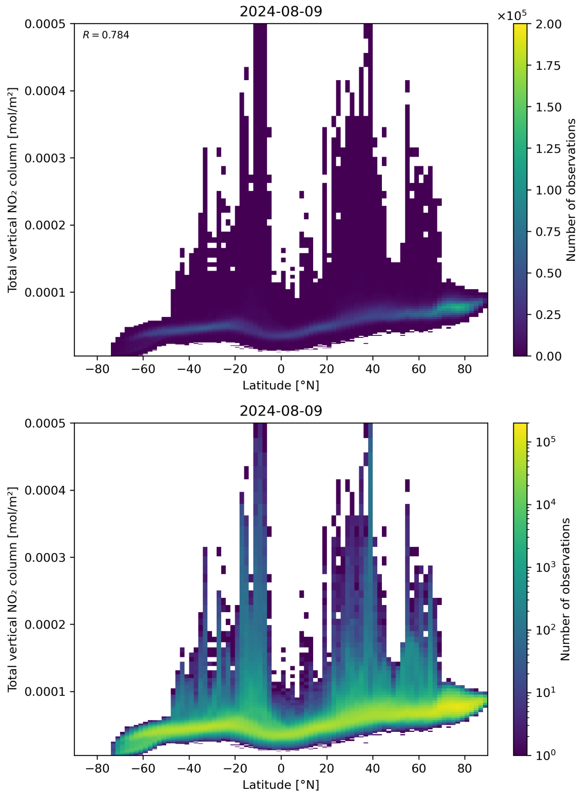
Figure 90: Scatter density plot of “Latitude” against “Total vertical NO 2 column” for 2024-08-08 to 2024-08-10.
