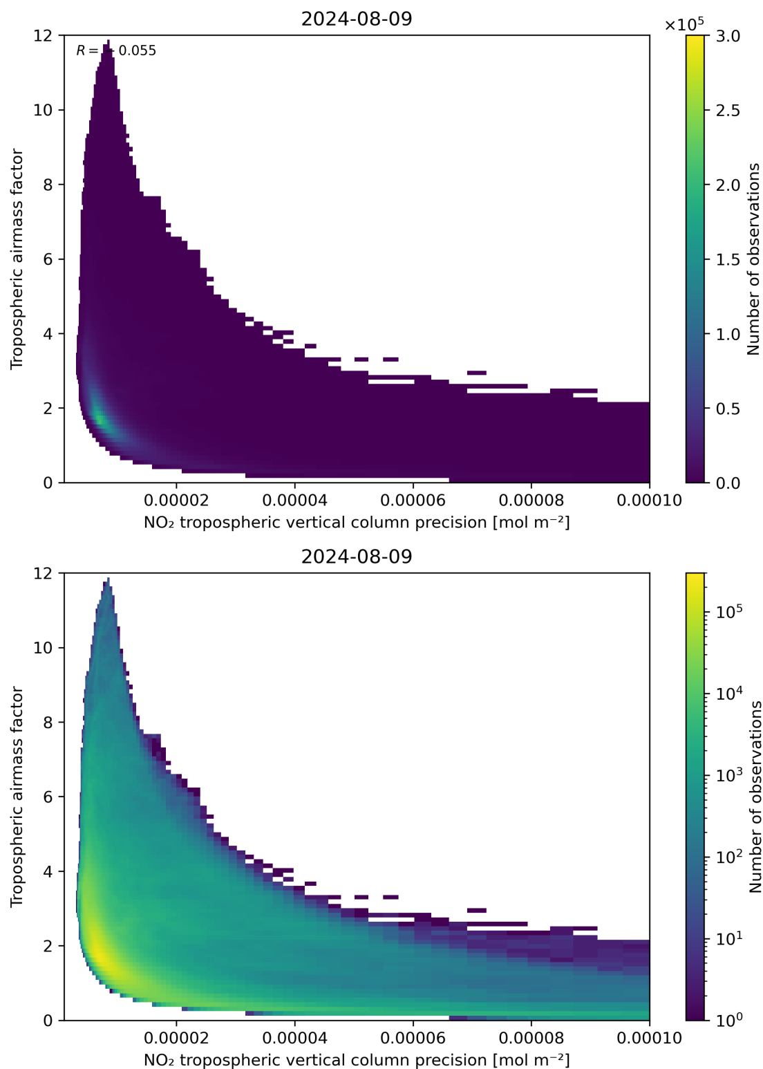
Figure 133: Scatter density plot of “NO 2 tropospheric vertical column precision” against “Tropospheric airmass factor” for 2024-08-08 to 2024-08-10.
