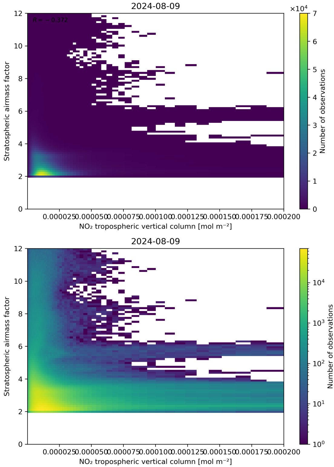
Figure 121: Scatter density plot of “NO 2 tropospheric vertical column” against “Stratospheric air mass factor” for 2024-08-08 to 2024-08-10.
