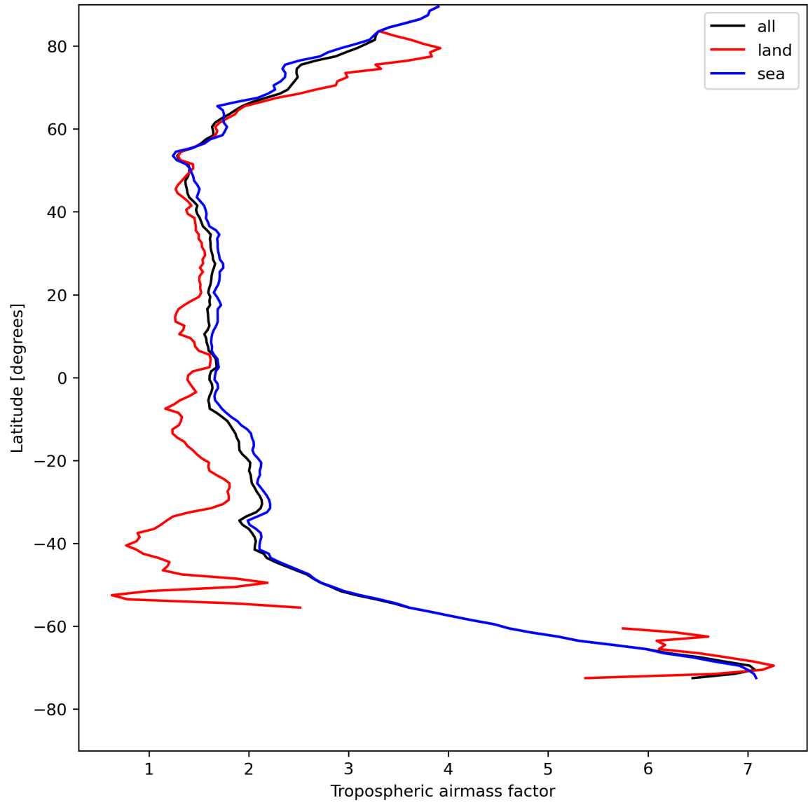
Figure 14: Zonal average of “Tropospheric airmass factor” for 2024-08-08 to 2024-08-10.
