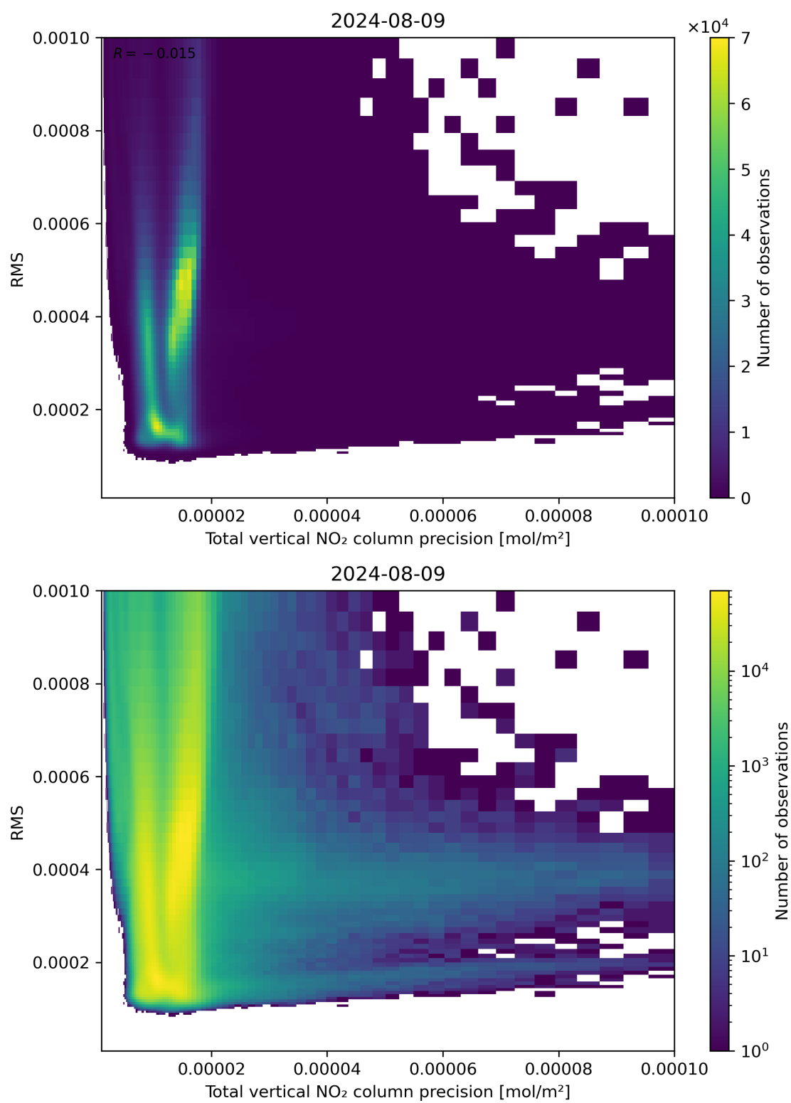
Figure 119: Scatter density plot of “Total vertical NO 2 column precision” against “RMS” for 2024-08-08 to 2024-08-10.
