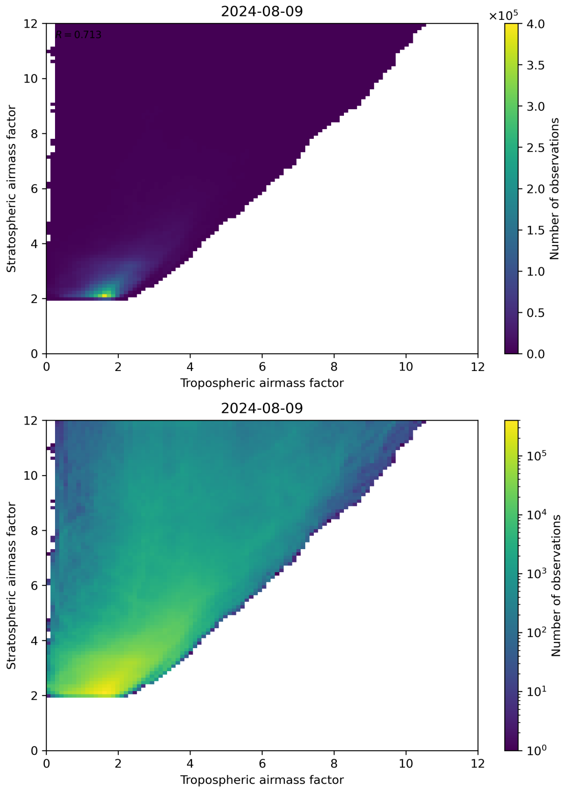
Figure 71: Scatter density plot of “Tropospheric airmass factor” against “Stratospheric airmass factor” for 2024-08-08 to 2024-08-10.
