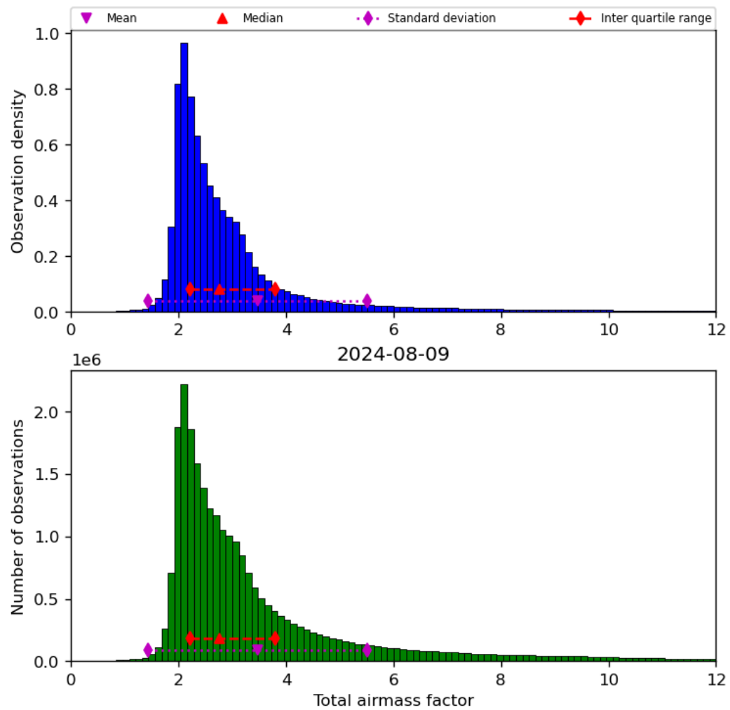
Figure 32: Histogram of “Total airmass factor” for 2024-08-08 to 2024-08-10
