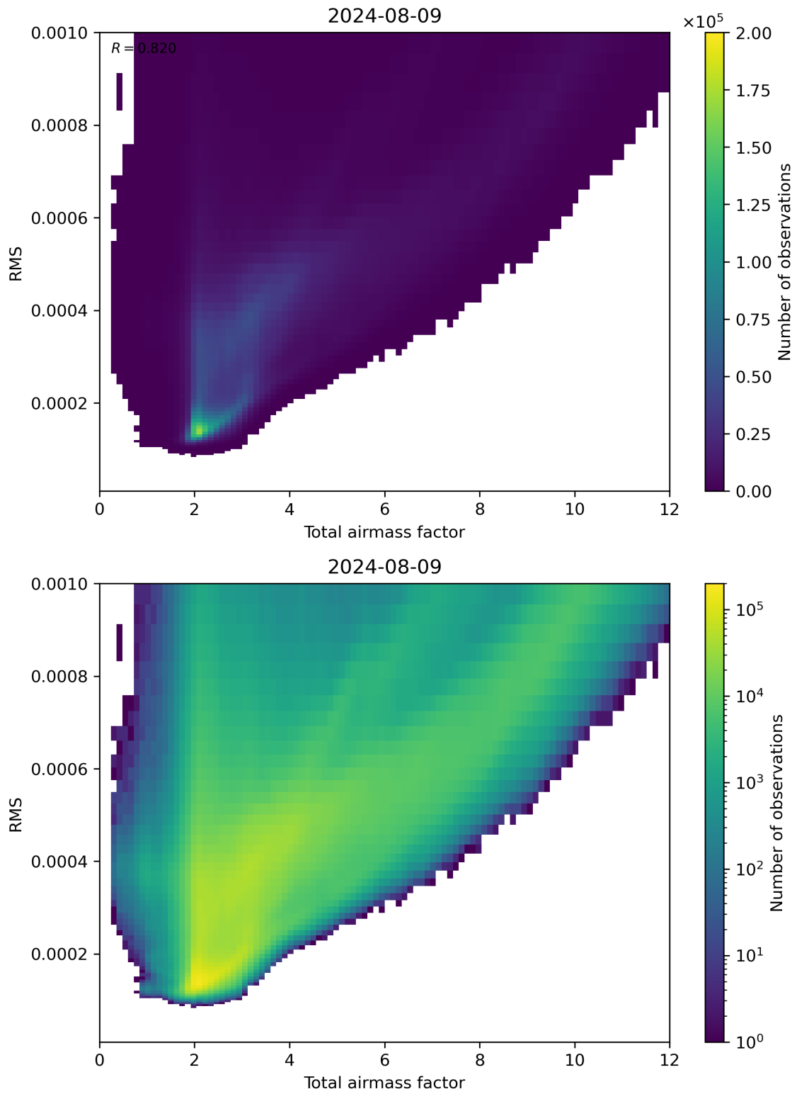
Figure 69: Scatter density plot of “Total airmass factor” against “RMS” for 2024-08-08 to 2024-08-10.
