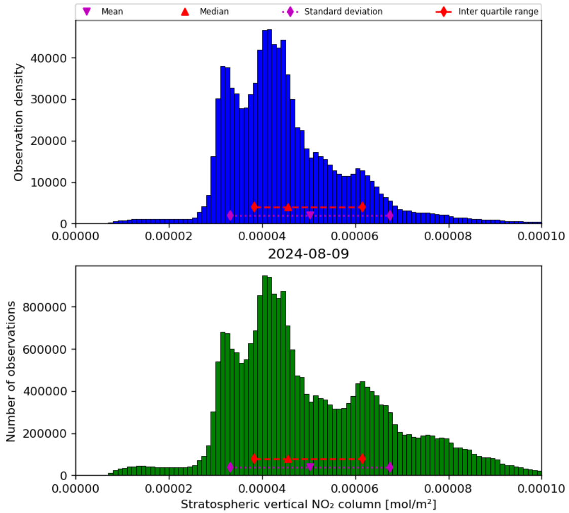
Figure 36: Histogram of “Stratospheric vertical NO 2 column” for 2024-08-08 to 2024-08-10
