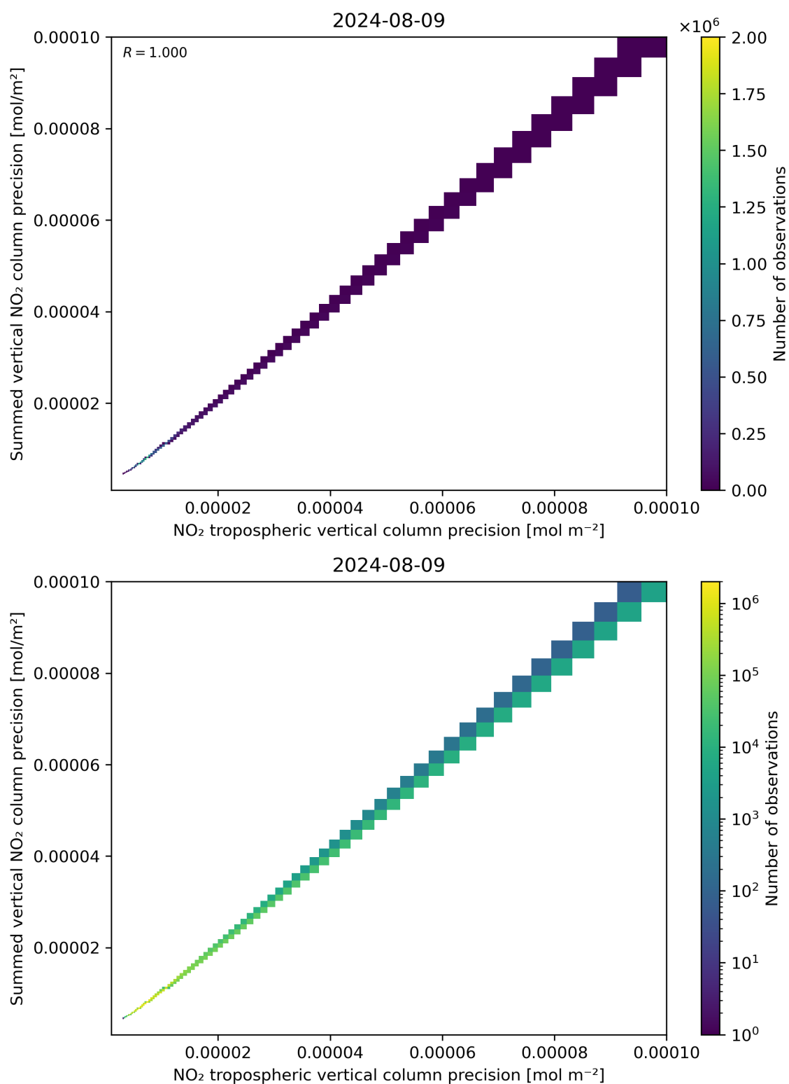
Figure 137: Scatter density plot of “NO 2 tropospheric vertical column precision” against “Summed vertical NO 2 column precision” for 2024-08-08 to 2024-08-10.
