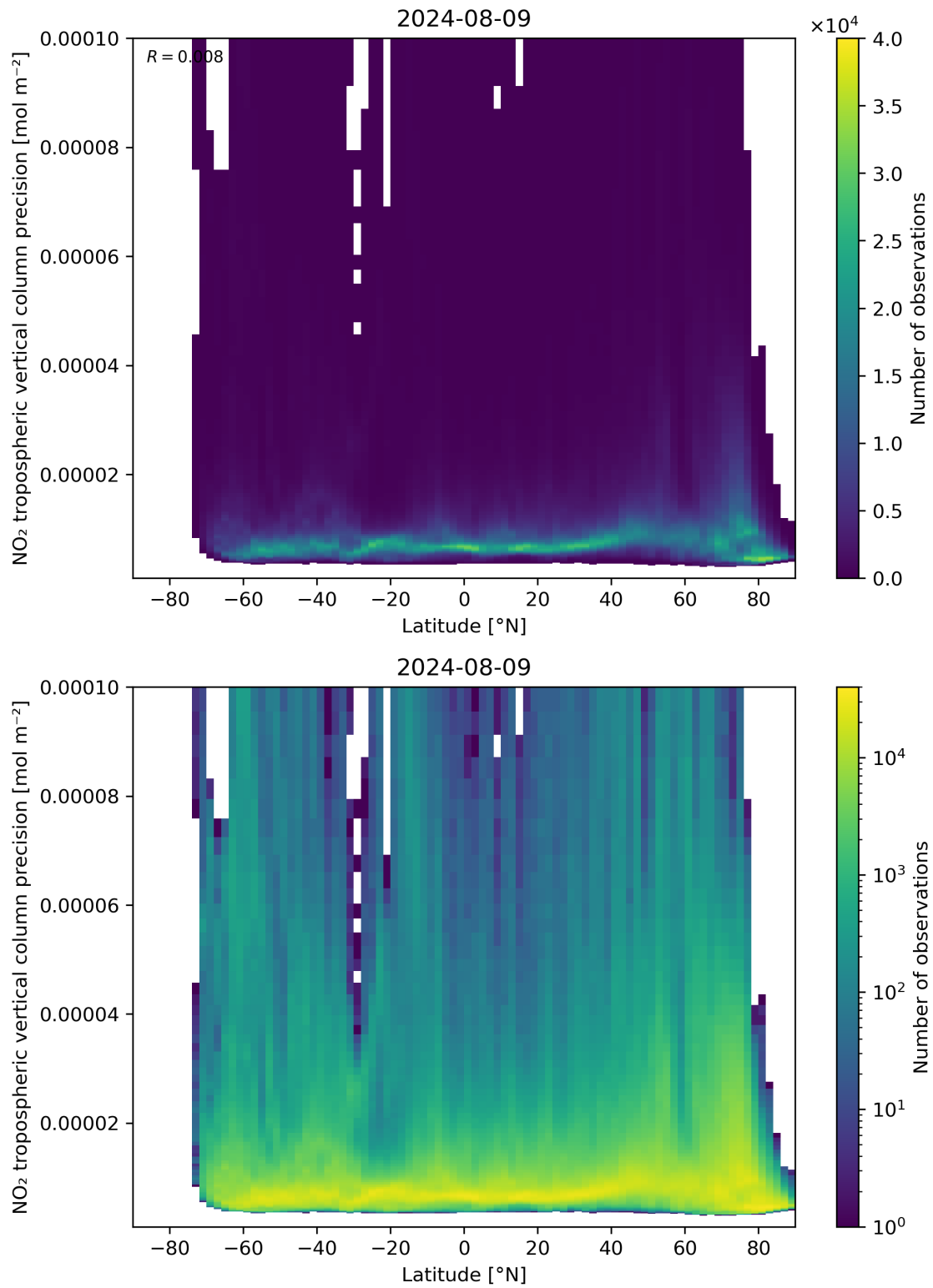
Figure 93: Scatter density plot of “Latitude” against “NO 2 tropospheric vertical column precision” for 2024-08-08 to 2024-08-10.
