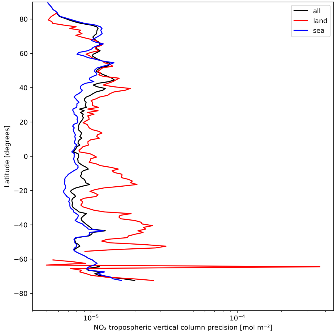
Figure 13: Zonal average of “NO 2 tropospheric vertical column precision” for 2024-08-08 to 2024-08-10.
