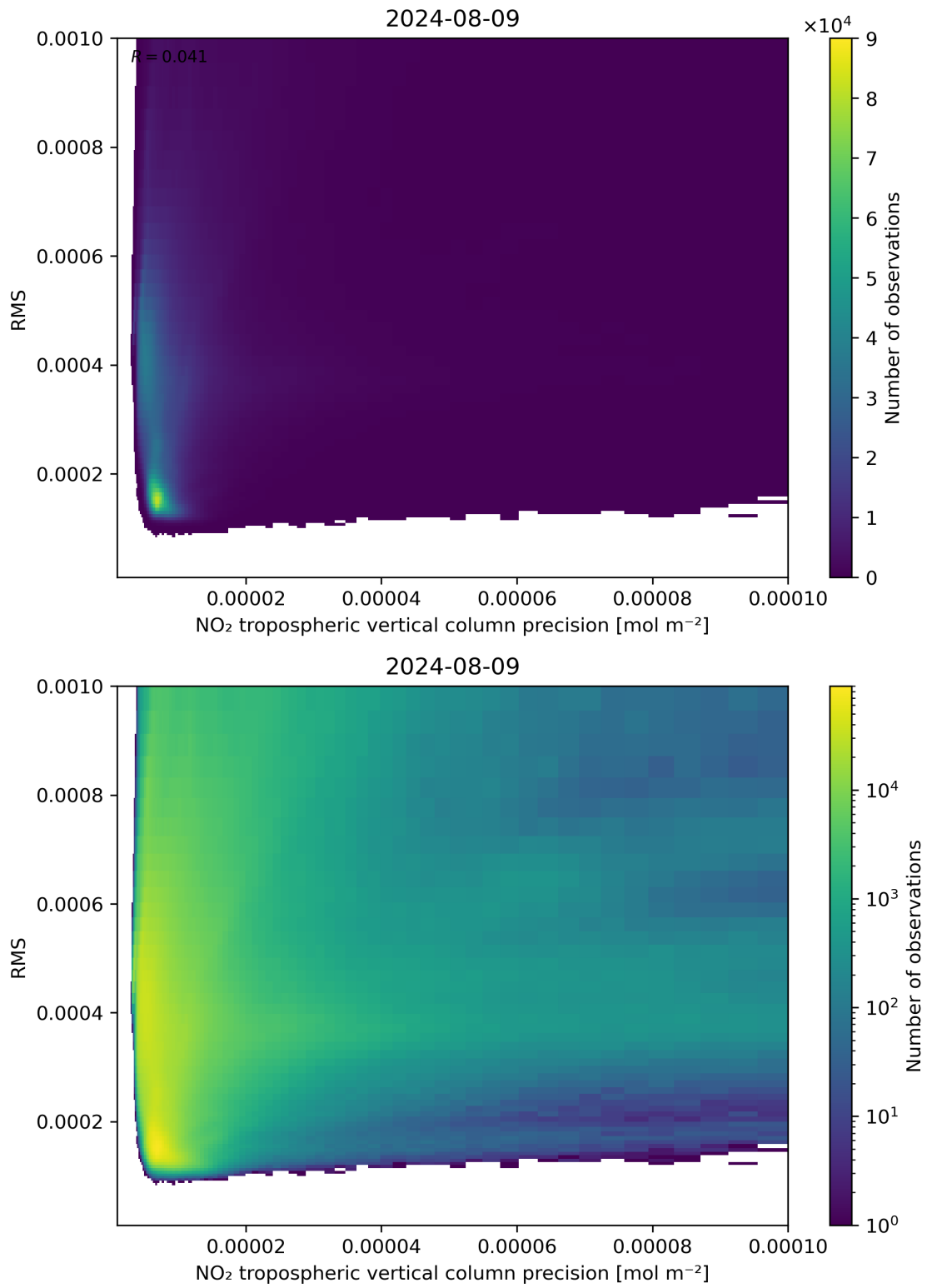
Figure 140: Scatter density plot of “NO 2 tropospheric vertical column precision” against “RMS” for 2024-08-08 to 2024-08-10.
