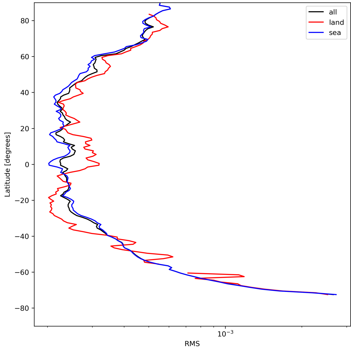
Figure 26: Zonal average of “RMS” for 2024-08-08 to 2024-08-10.
