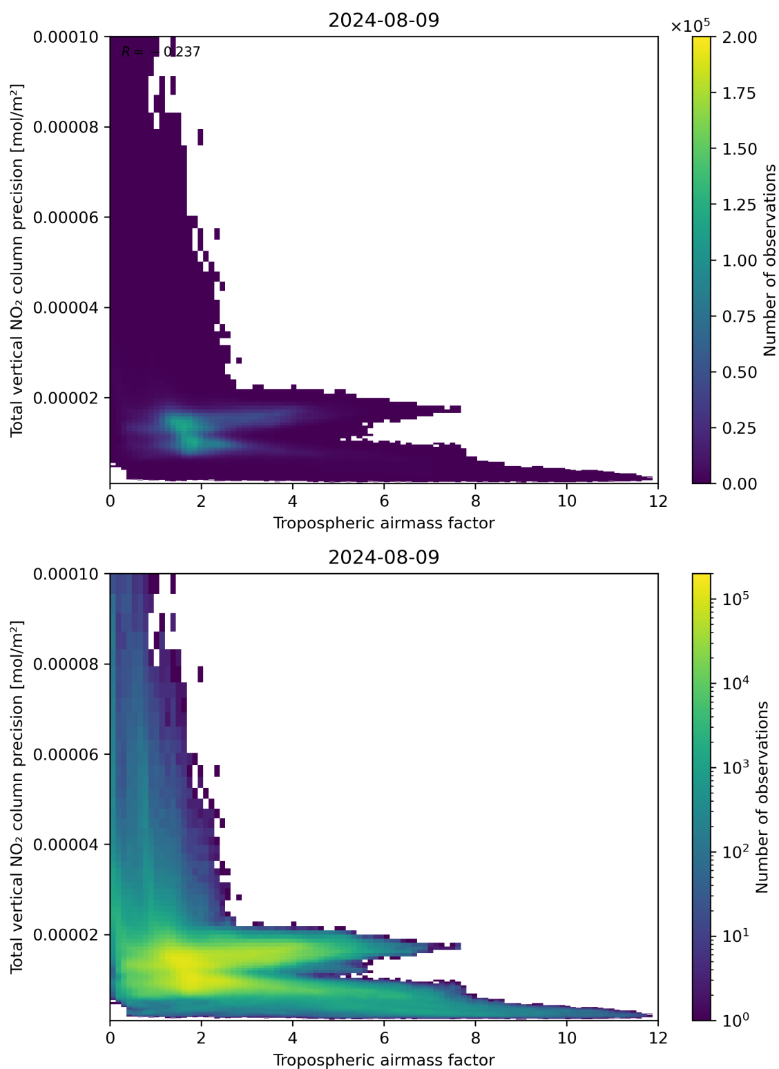
Figure 78: Scatter density plot of “Tropospheric air mass factor” against “Total vertical NO 2 column precision” for 2024-08-08 to 2024-08-10.
