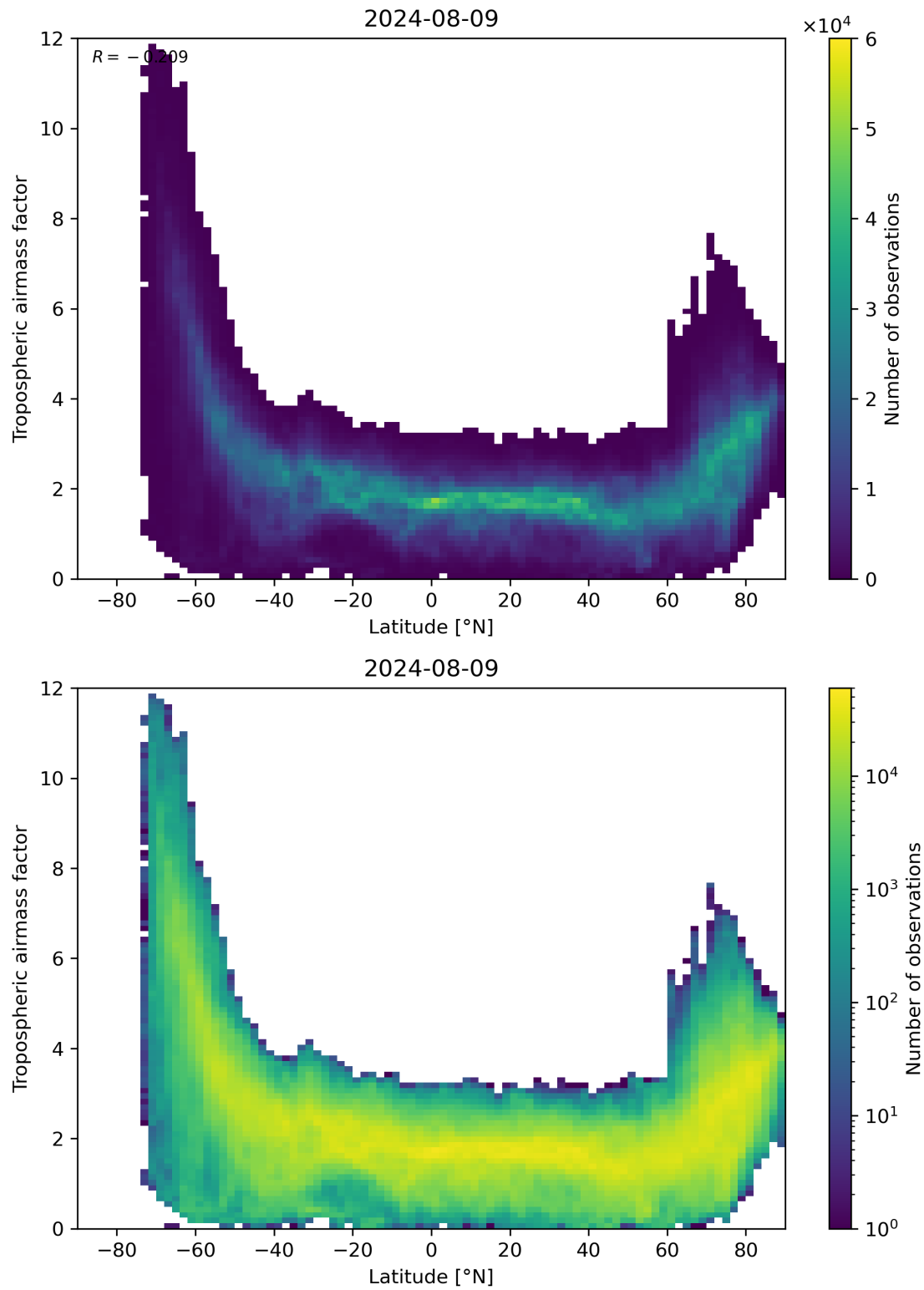
Figure 85: Scatter density plot of “Latitude” against “Tropospheric airmass factor” for 2024-08-08 to 2024-08-10.
