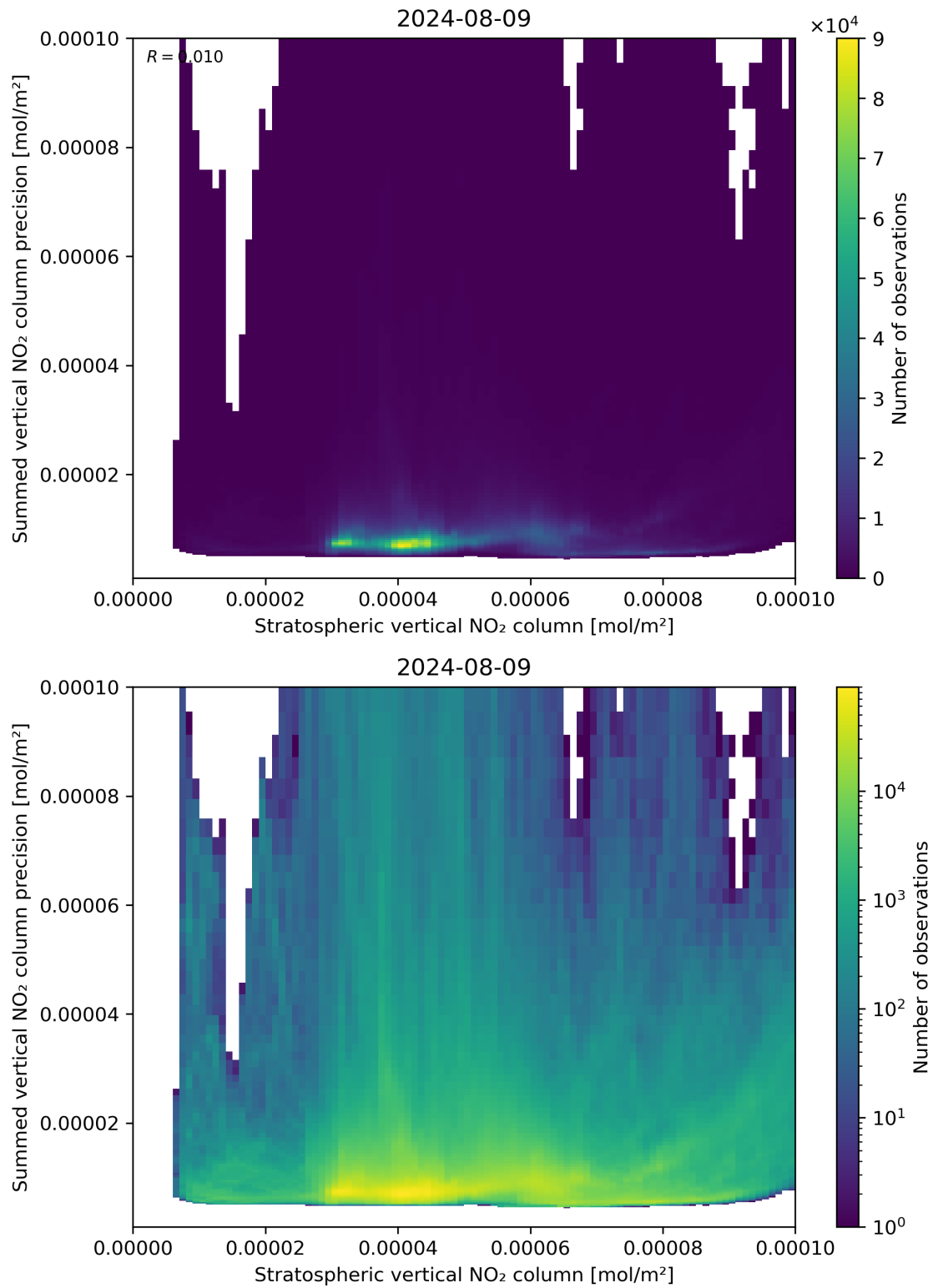
Figure 99: Scatter density plot of “Stratospheric vertical NO 2 column” against “Summed vertical NO 2 column precision” for 2024-08-08 to 2024-08-10.
