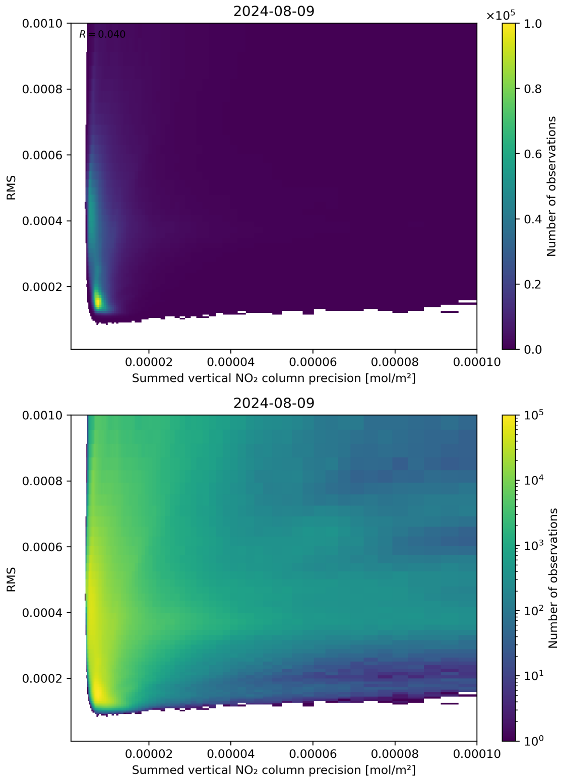
Figure 108: Scatter density plot of “Summed vertical NO 2 column precision” against “RMS” for 2024-08-08 to 2024-08-10.
