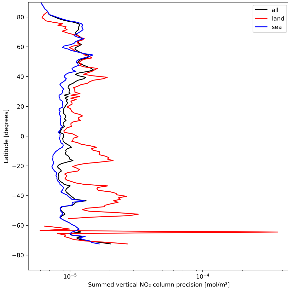
Figure 24: Zonal average of “Summed vertical NO 2 column precision” for 2024-08-08 to 2024-08-10.
