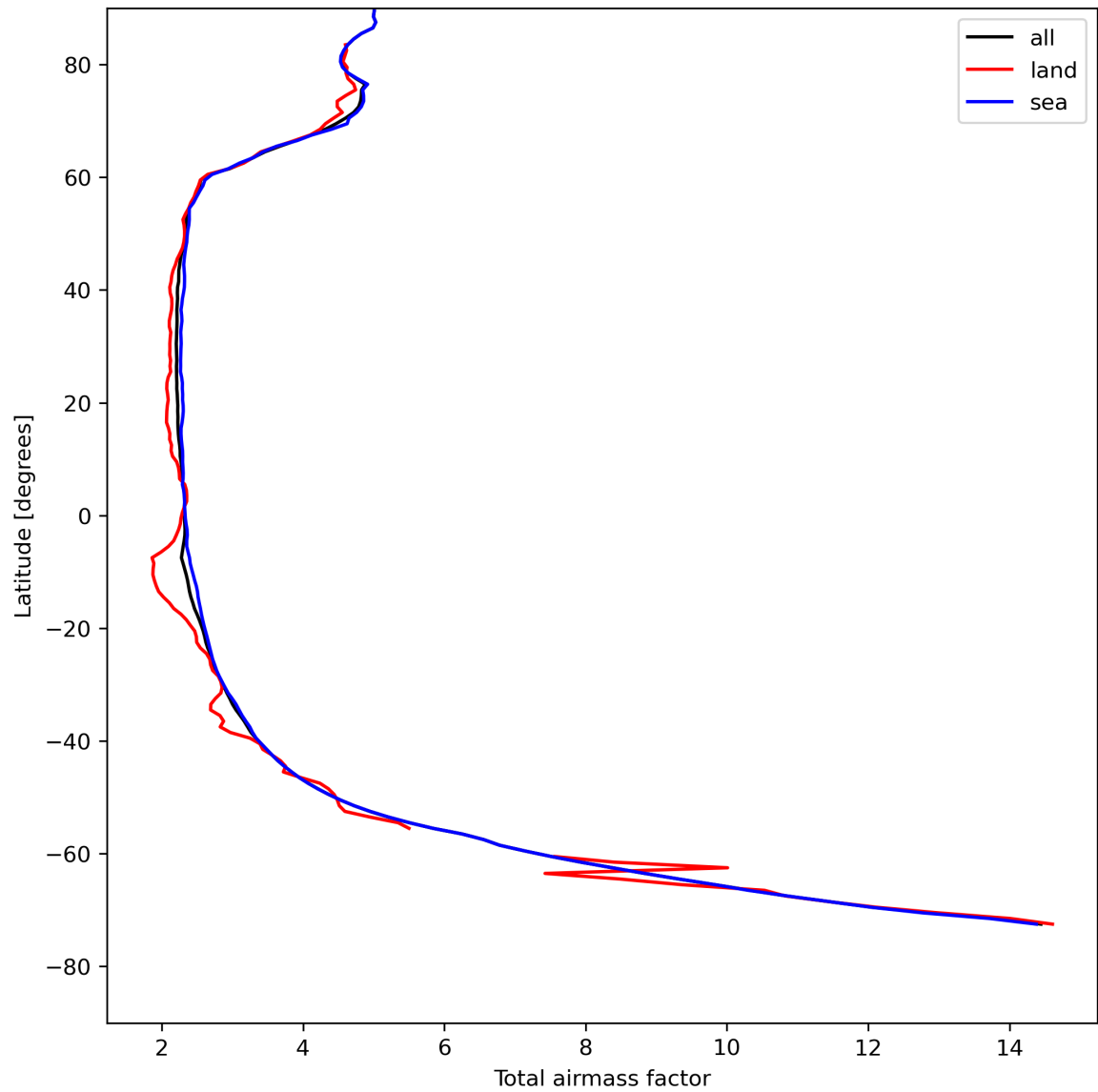
Figure 15: Zonal average of “Total airmass factor” for 2024-08-08 to 2024-08-10.
