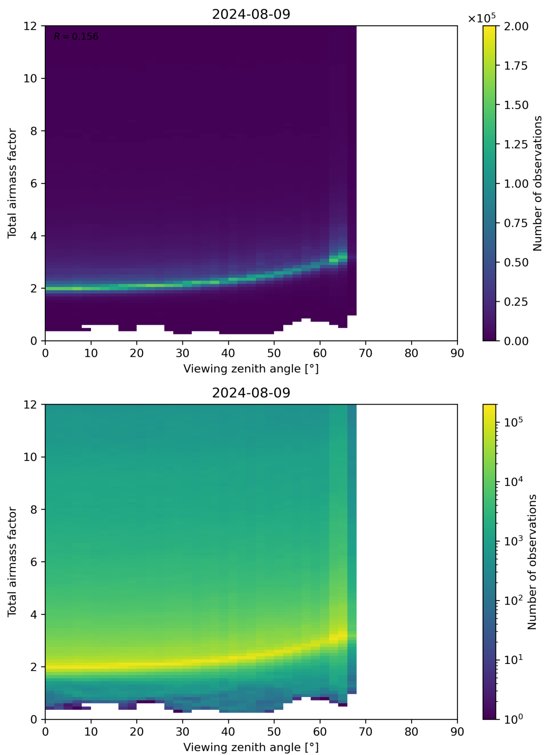
Figure 160: Scatter density plot of “Viewing zenith angle” against “Total airmass factor” for 2024-08-08 to 2024-08-10.
