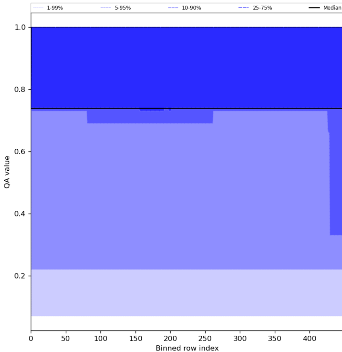
Figure 45: Along track statistics of “QA value” for 2024-08-08 to 2024-08-10
