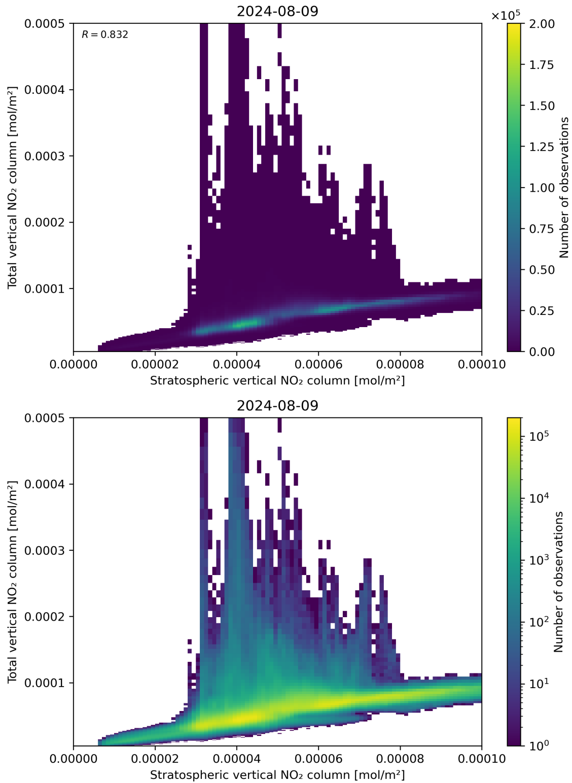
Figure 100: Scatter density plot of “Stratospheric vertical NO 2 column” against “Total vertical NO 2 column” for 2024-08-08 to 2024-08-10.
