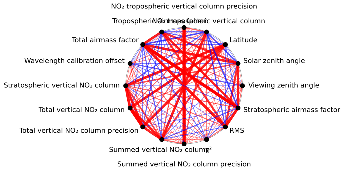
Figure 1: Map of correlation graph for 2024-08-08 to 2024-08-10.
