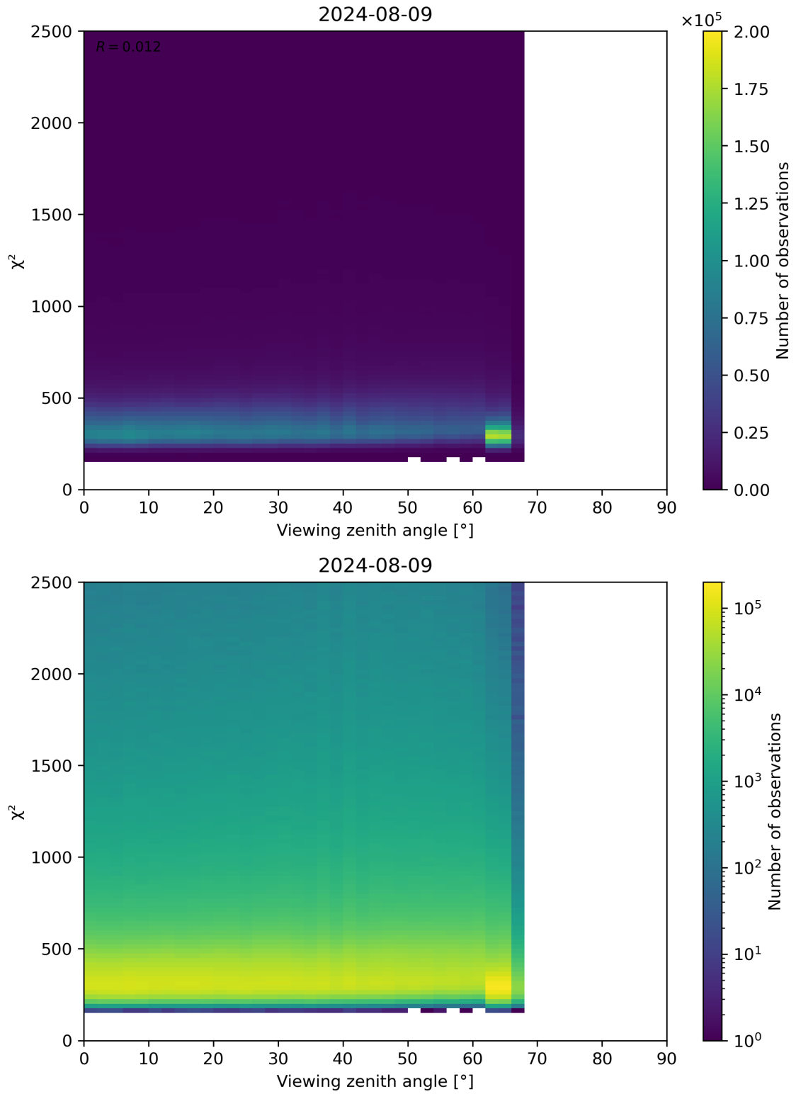
Figure 162: Scatter density plot of “Viewing zenith angle” against “ \chi^2 ” for 2024-08-08 to 2024-08-10.
