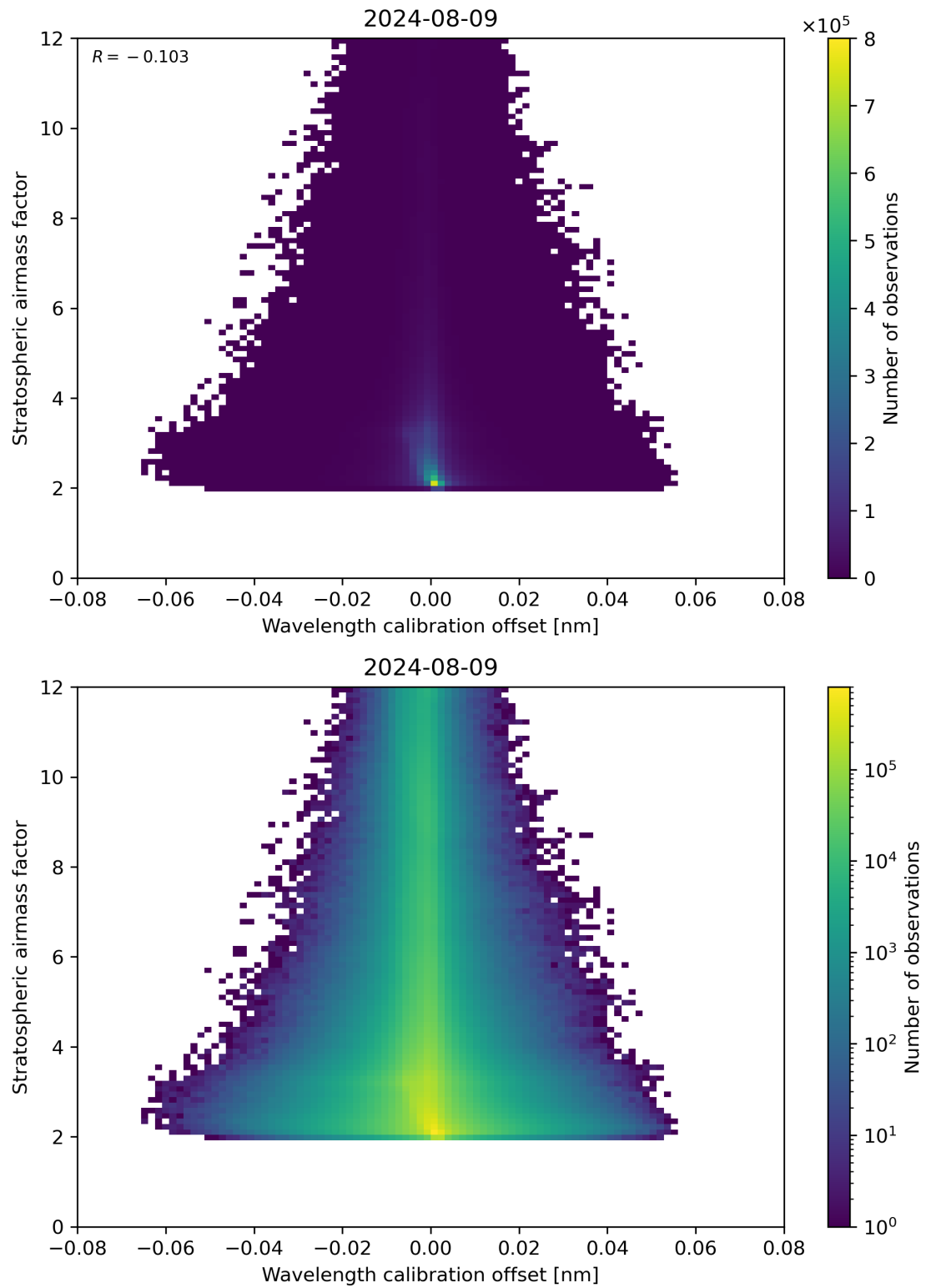
Figure 174: Scatter density plot of “Wavelength calibration offset” against “Stratospheric airmass factor” for 2024-08-08 to 2024-08-10.
