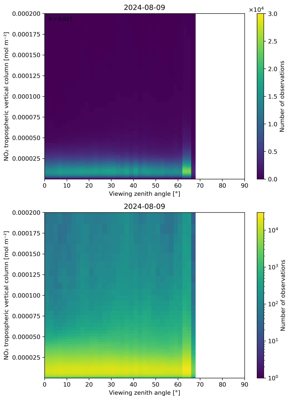
Figure 169: Scatter density plot of “Viewing zenith angle” against “NO 2 tropospheric vertical column” for 2024-08-08 to 2024-08-10.
