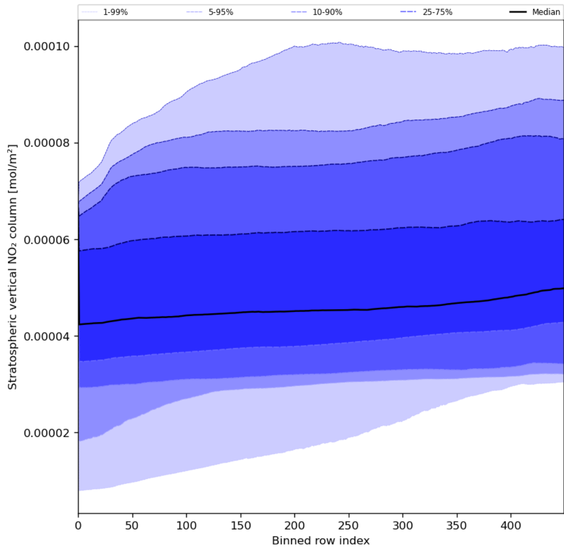
Figure 53: Along track statistics of “Stratospheric vertical NO 2 column” for 2024-08-08 to 2024-08-10
