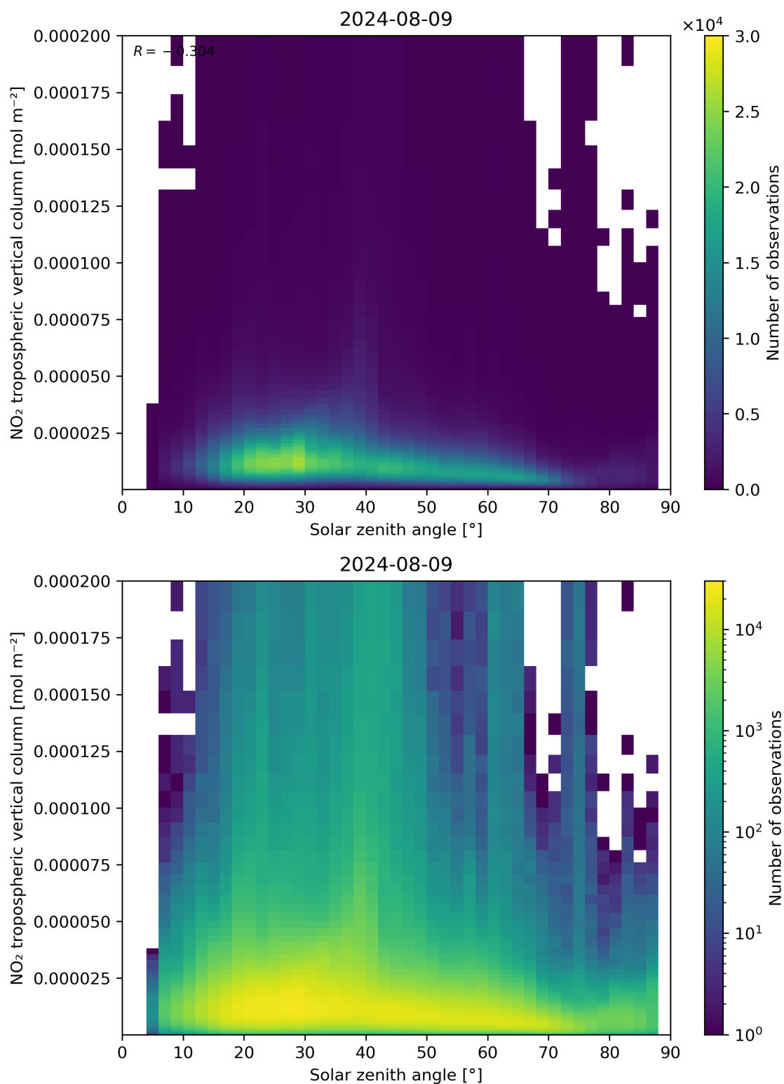
Figure 155: Scatter density plot of “Solar zenith angle” against “NO 2 tropospheric vertical column” for 2024-08-08 to 2024-08-10.
