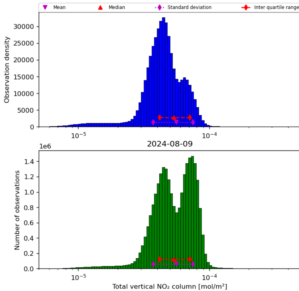
Figure 38: Histogram of “Total vertical NO 2 column” for 2024-08-08 to 2024-08-10
