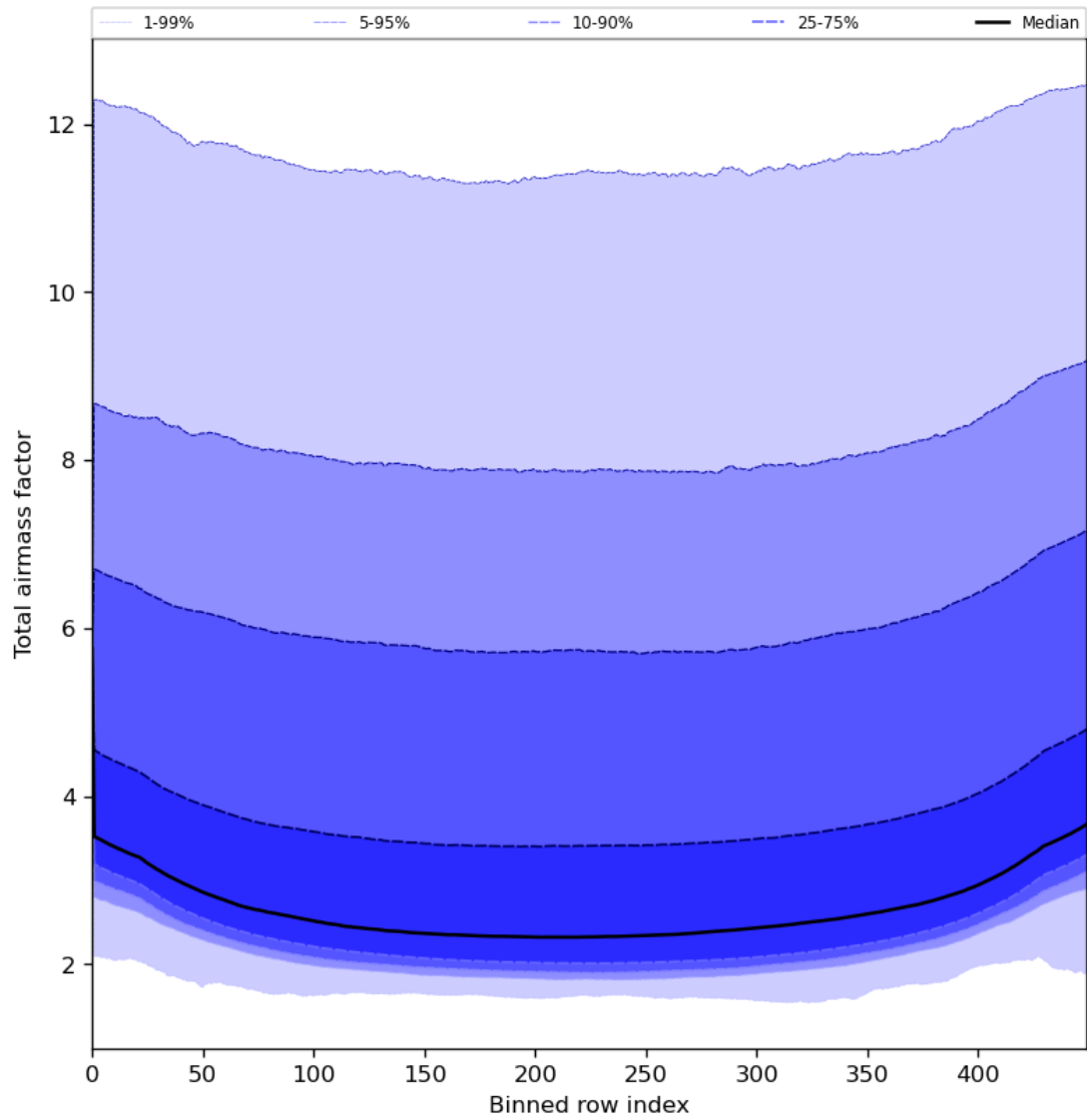
Figure 49: Along track statistics of “Total airmass factor” for 2024-08-08 to 2024-08-10
