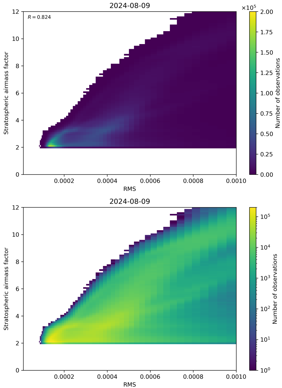
Figure 144: Scatter density plot of “RMS” against “Stratospheric airmass factor” for 2024-08-08 to 2024-08-10.
