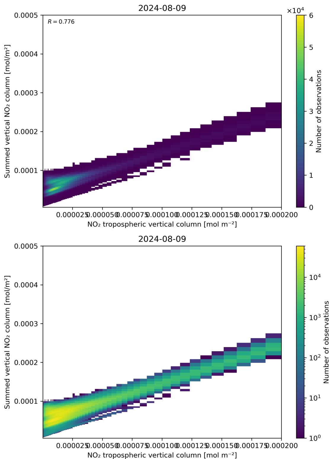
Figure 126: Scatter density plot of “NO 2 tropospheric vertical column” against “Summed vertical NO 2 column” for 2024-08-08 to 2024-08-10.
