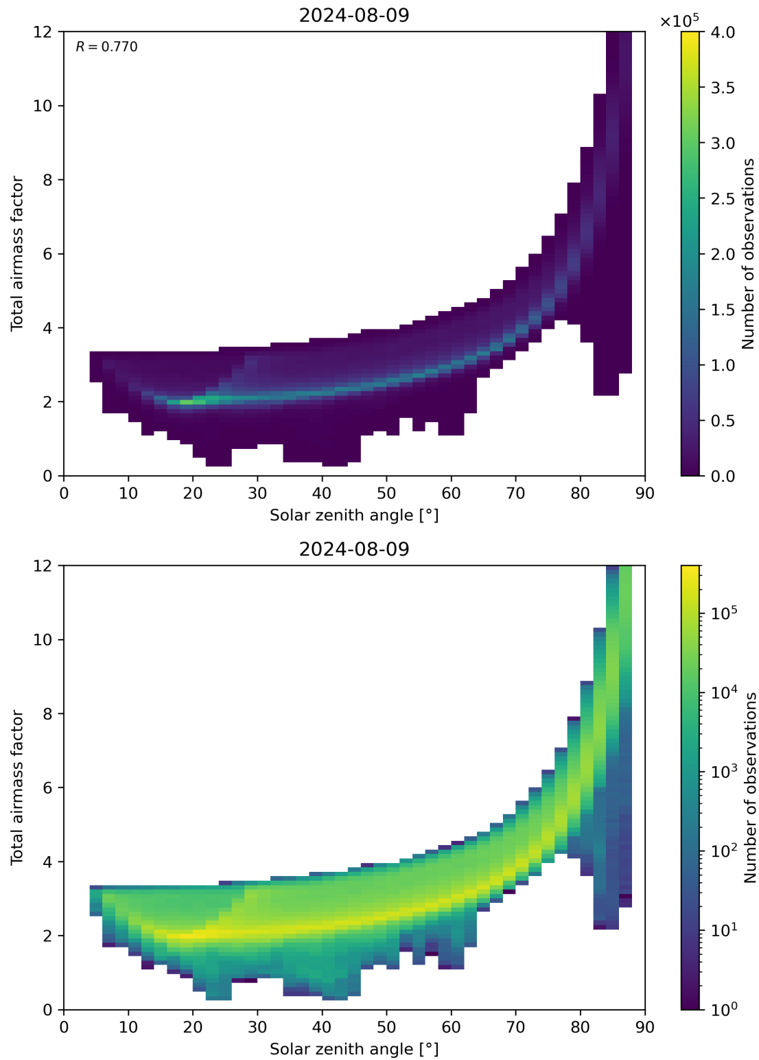
Figure 146: Scatter density plot of “Solar zenith angle” against “Total air mass factor” for 2024-08-08 to 2024-08-10.
