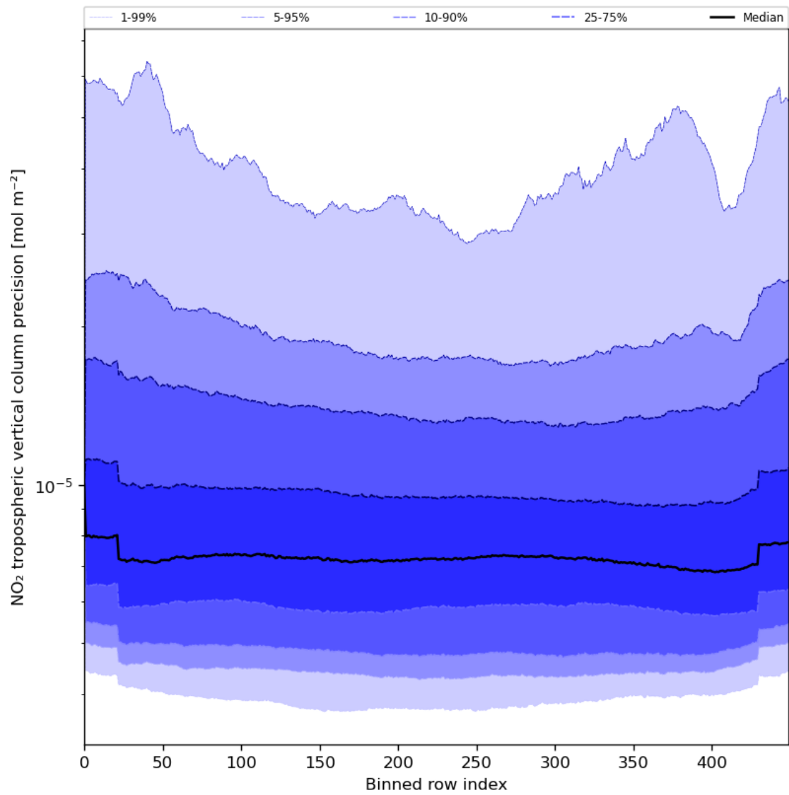
Figure 47: Along track statistics of “NO 2 tropospheric vertical column precision” for 2024-08-08 to 2024-08-10
