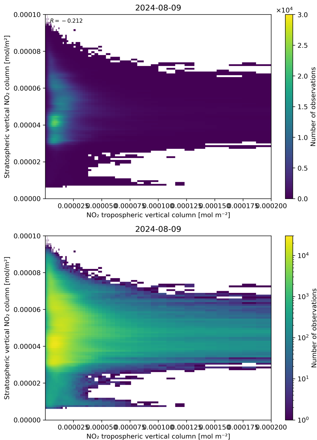
Figure 125: Scatter density plot of “NO 2 tropospheric vertical column” against “Stratospheric vertical NO 2 column” for 2024-08-08 to 2024-08-10.
