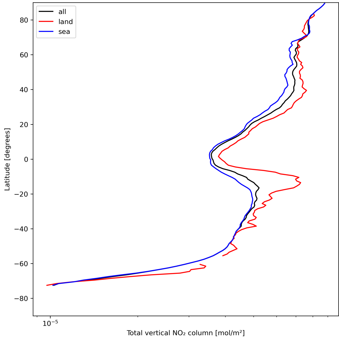
Figure 21: Zonal average of “Total vertical NO 2 column” for 2024-08-08 to 2024-08-10.
