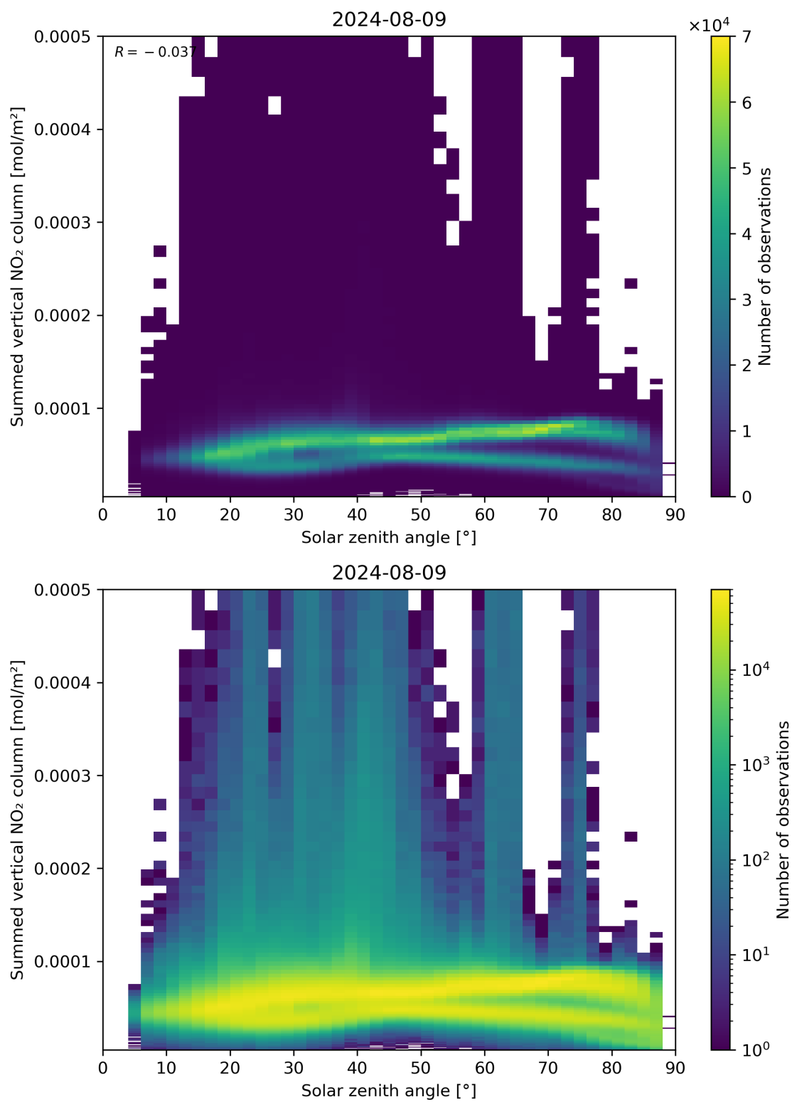
Figure 151: Scatter density plot of “Solar zenith angle” against “Summed vertical NO 2 column” for 2024-08-08 to 2024-08-10.
