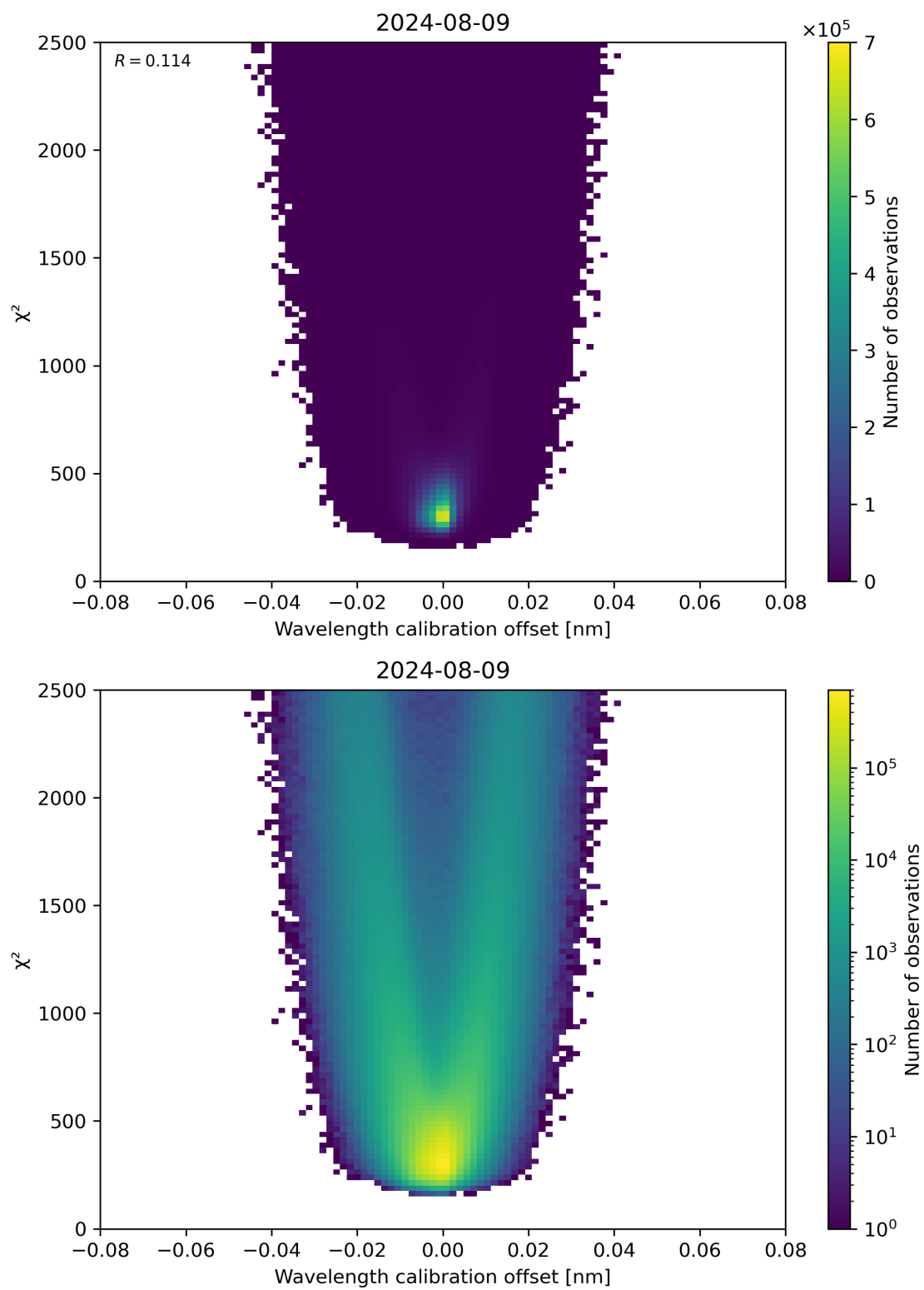
Figure 175: Scatter density plot of “Wavelength calibration offset” against “ \chi^2 ” for 2024-08-08 to 2024-08-10.
