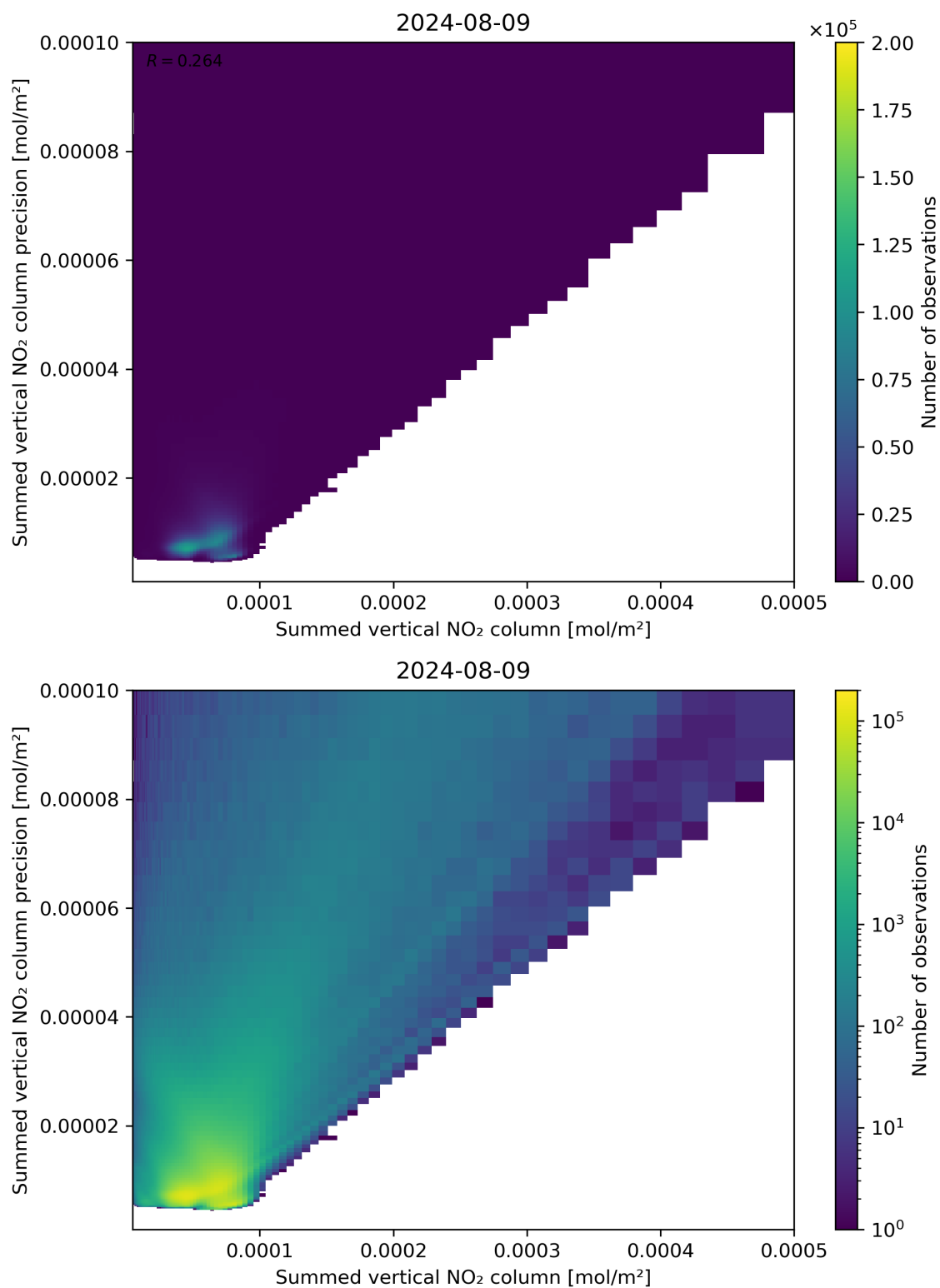
Figure 105: Scatter density plot of “Summed vertical NO 2 column” against “Summed vertical NO 2 column precision” for 2024-08-08 to 2024-08-10.
