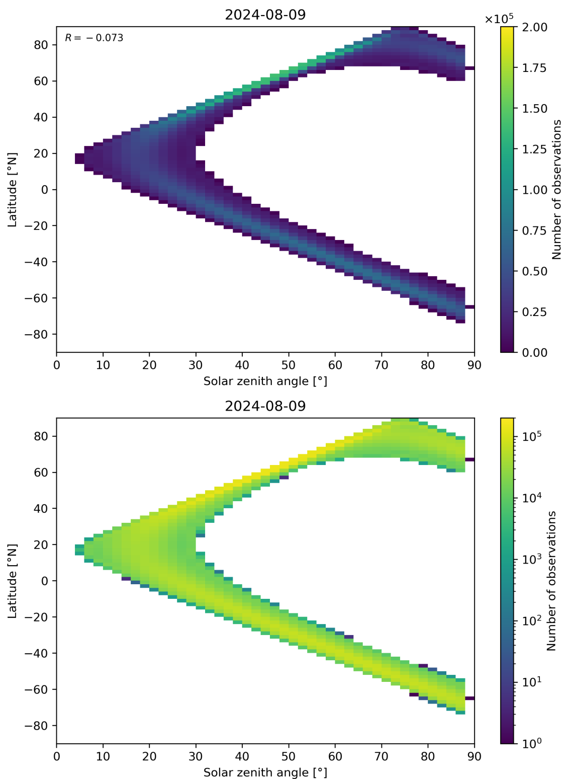
Figure 149: Scatter density plot of “Solar zenith angle” against “Latitude” for 2024-08-08 to 2024-08-10.
