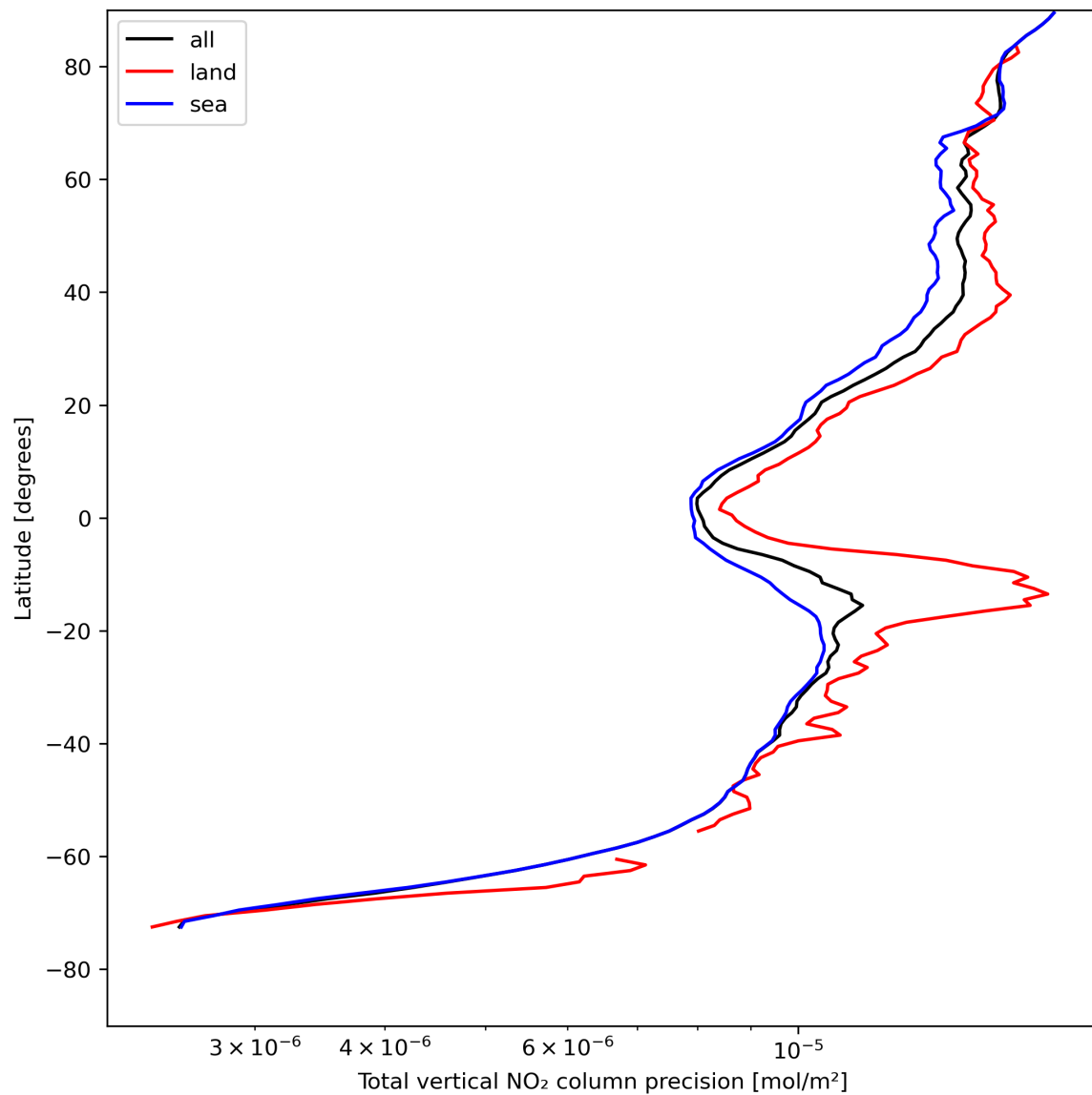
Figure 22: Zonal average of “Total vertical NO 2 column precision” for 2024-08-08 to 2024-08-10.
