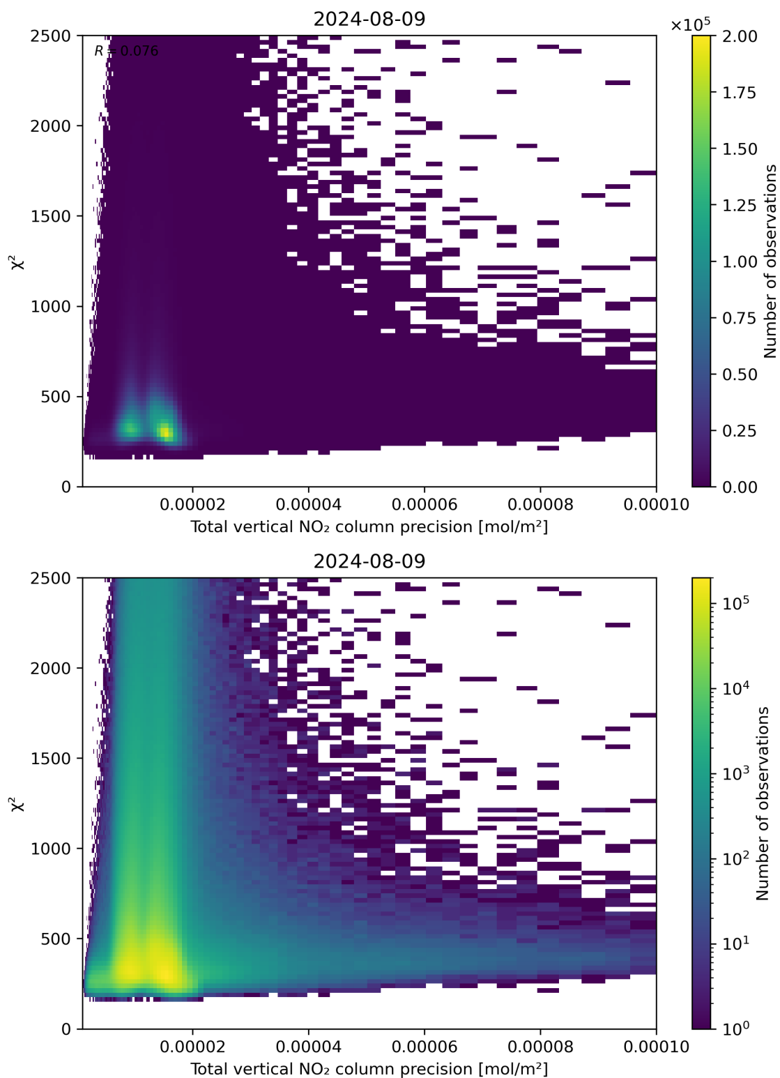
Figure 116: Scatter density plot of “Total vertical NO 2 column precision” against “ \chi^2 ” for 2024-08-08 to 2024-08-10.
