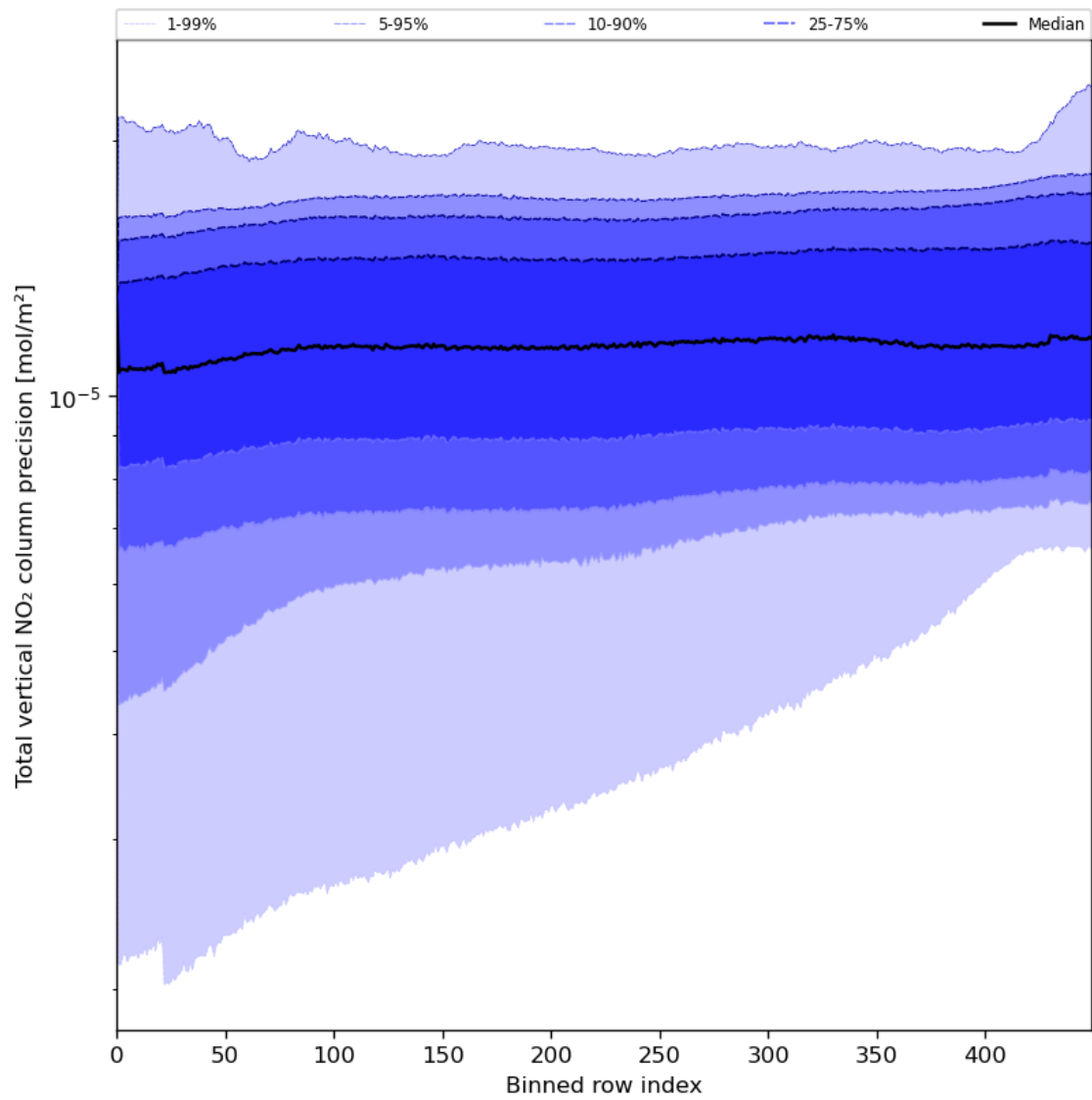
Figure 56: Along track statistics of “Total vertical NO 2 column precision” for 2024-08-08 to 2024-08-10
