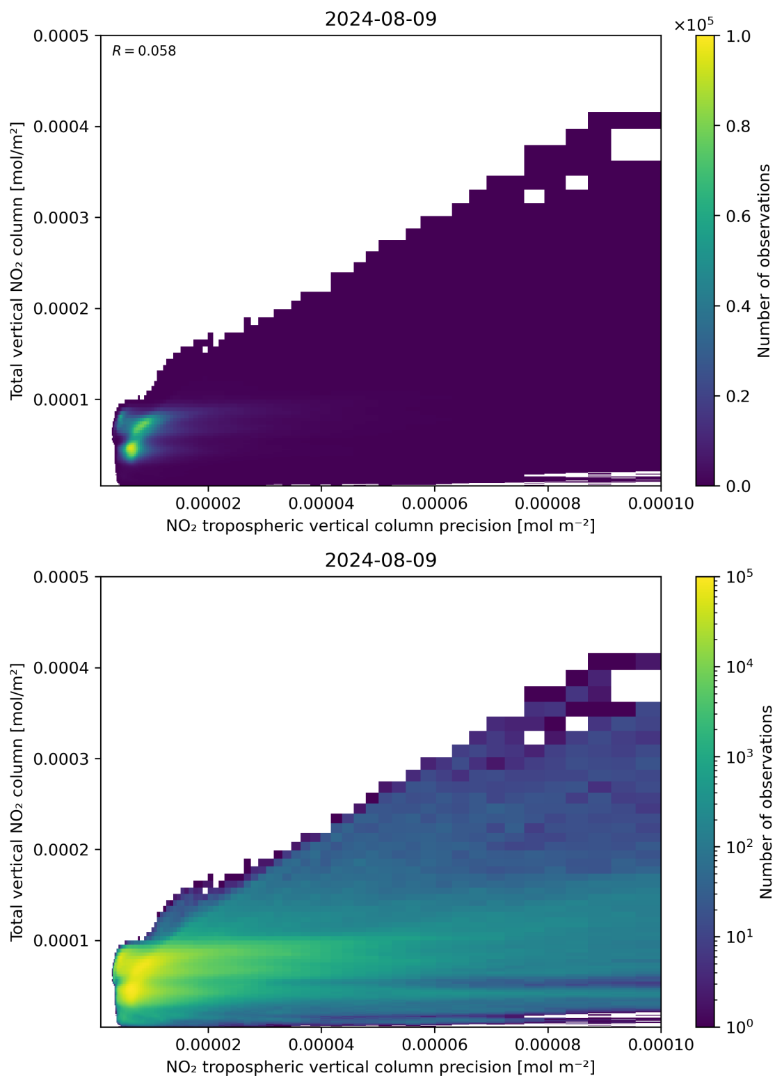
Figure 138: Scatter density plot of “NO 2 tropospheric vertical column precision” against “Total vertical NO 2 column” for 2024-08-08 to 2024-08-10.
