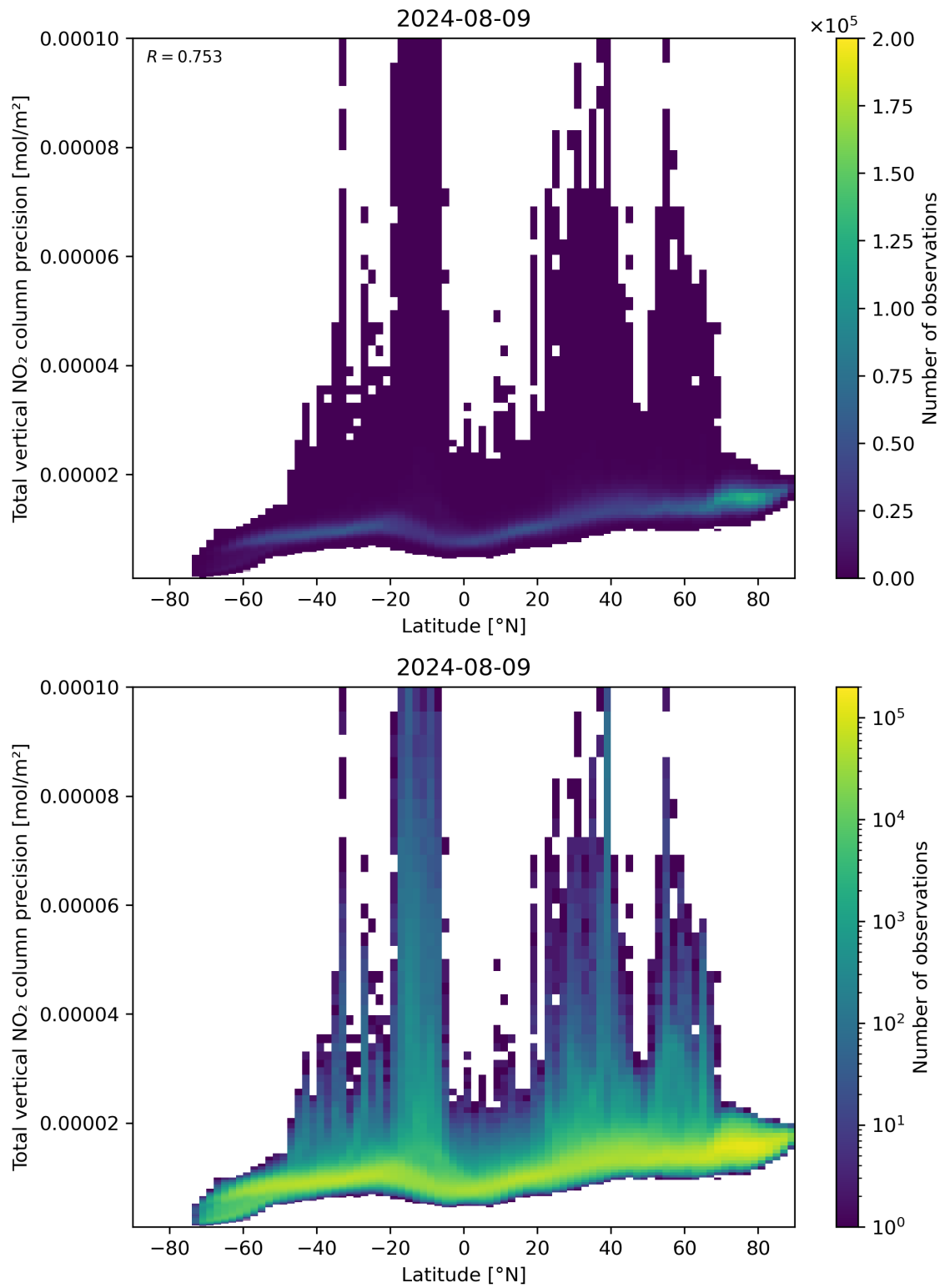
Figure 91: Scatter density plot of “Latitude” against “Total vertical NO 2 column precision” for 2024-08-08 to 2024-08-10.
