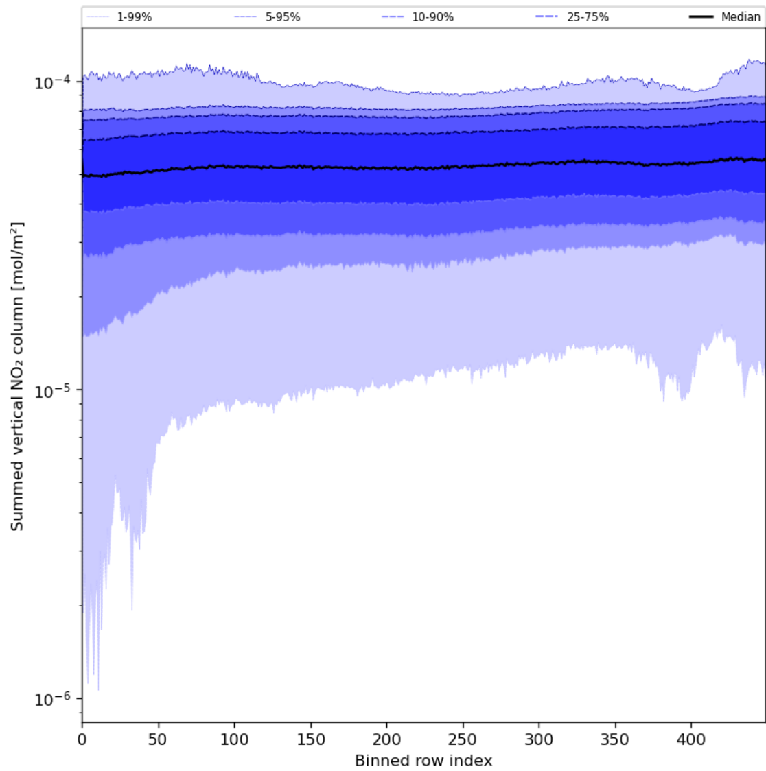
Figure 57: Along track statistics of “Summed vertical NO 2 column” for 2024-08-08 to 2024-08-10
