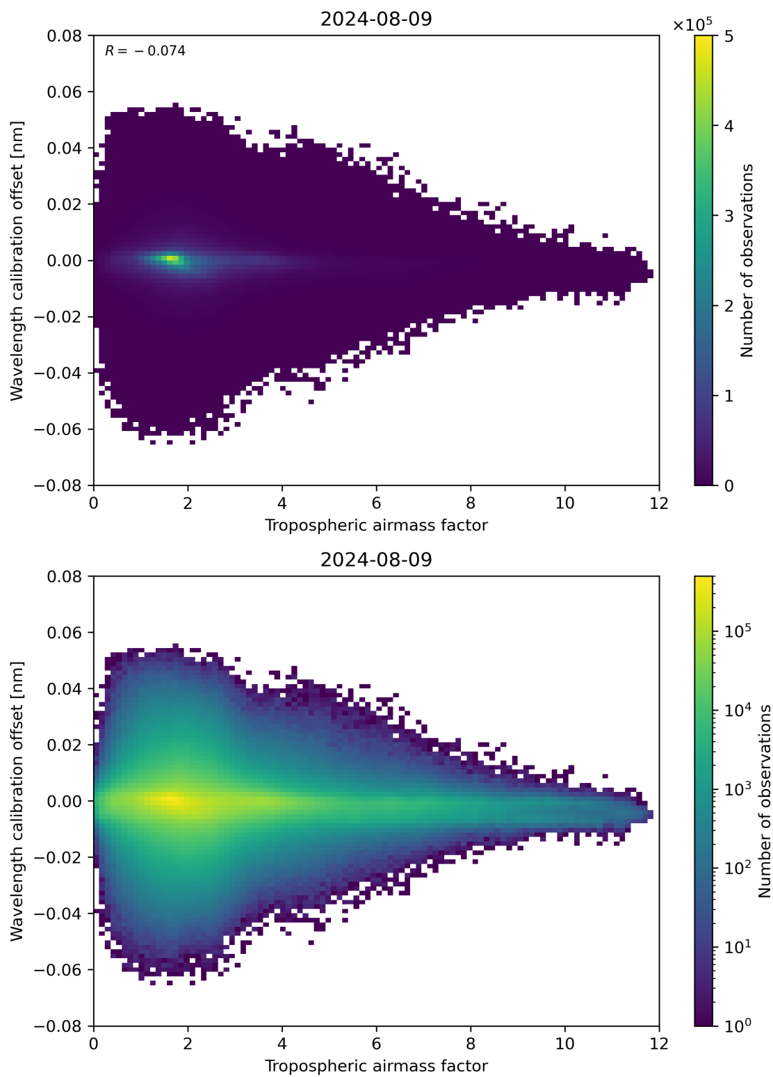
Figure 80: Scatter density plot of “Tropospheric air mass factor” against “Wavelength calibration offset” for 2024-08-08 to 2024-08-10.
