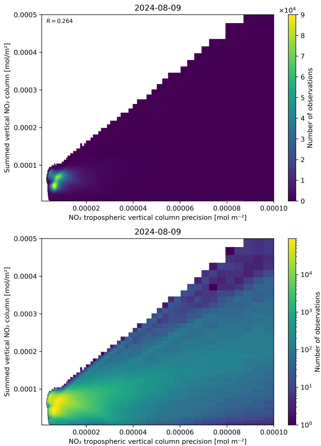
Figure 136: Scatter density plot of “NO 2 tropospheric vertical column precision” against “Summed vertical NO 2 column” for 2024-08-08 to 2024-08-10.
