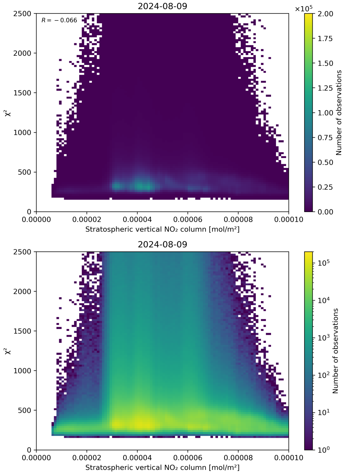
Figure 97: Scatter density plot of “Stratospheric vertical NO 2 column” against “ \chi^2 ” for 2024-08-08 to 2024-08-10.
