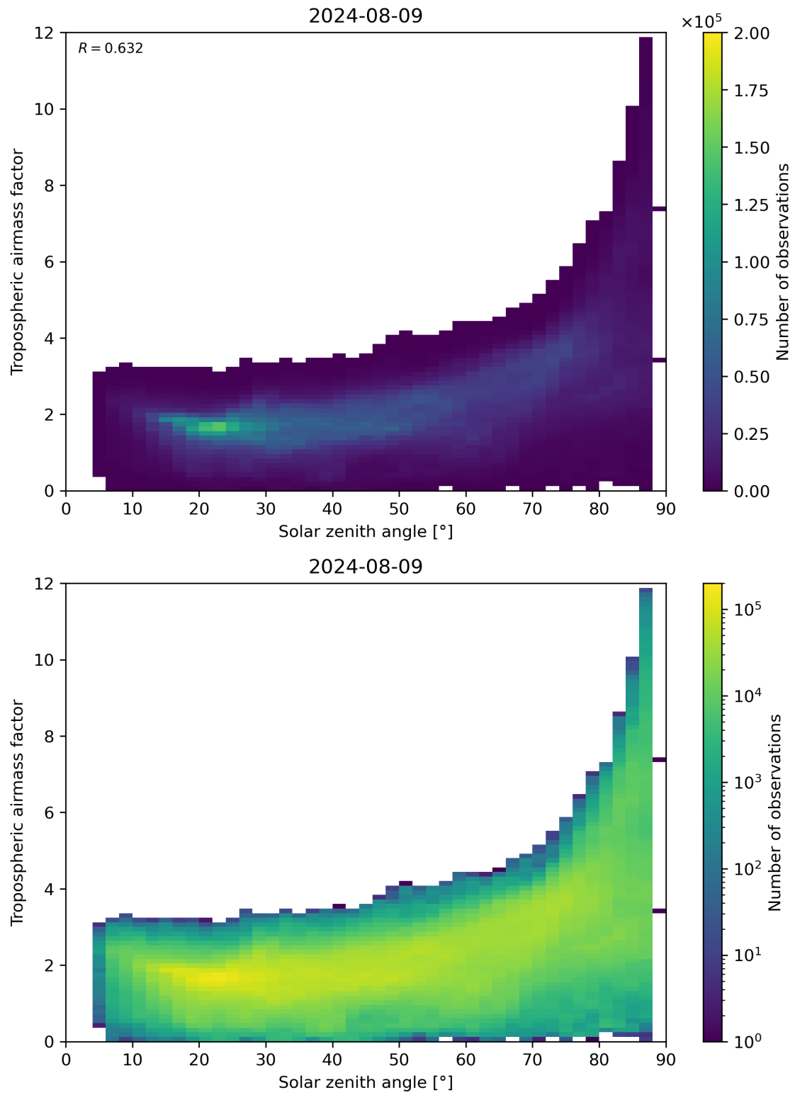
Figure 147: Scatter density plot of “Solar zenith angle” against “Tropospheric airmass factor” for 2024-08-08 to 2024-08-10.
