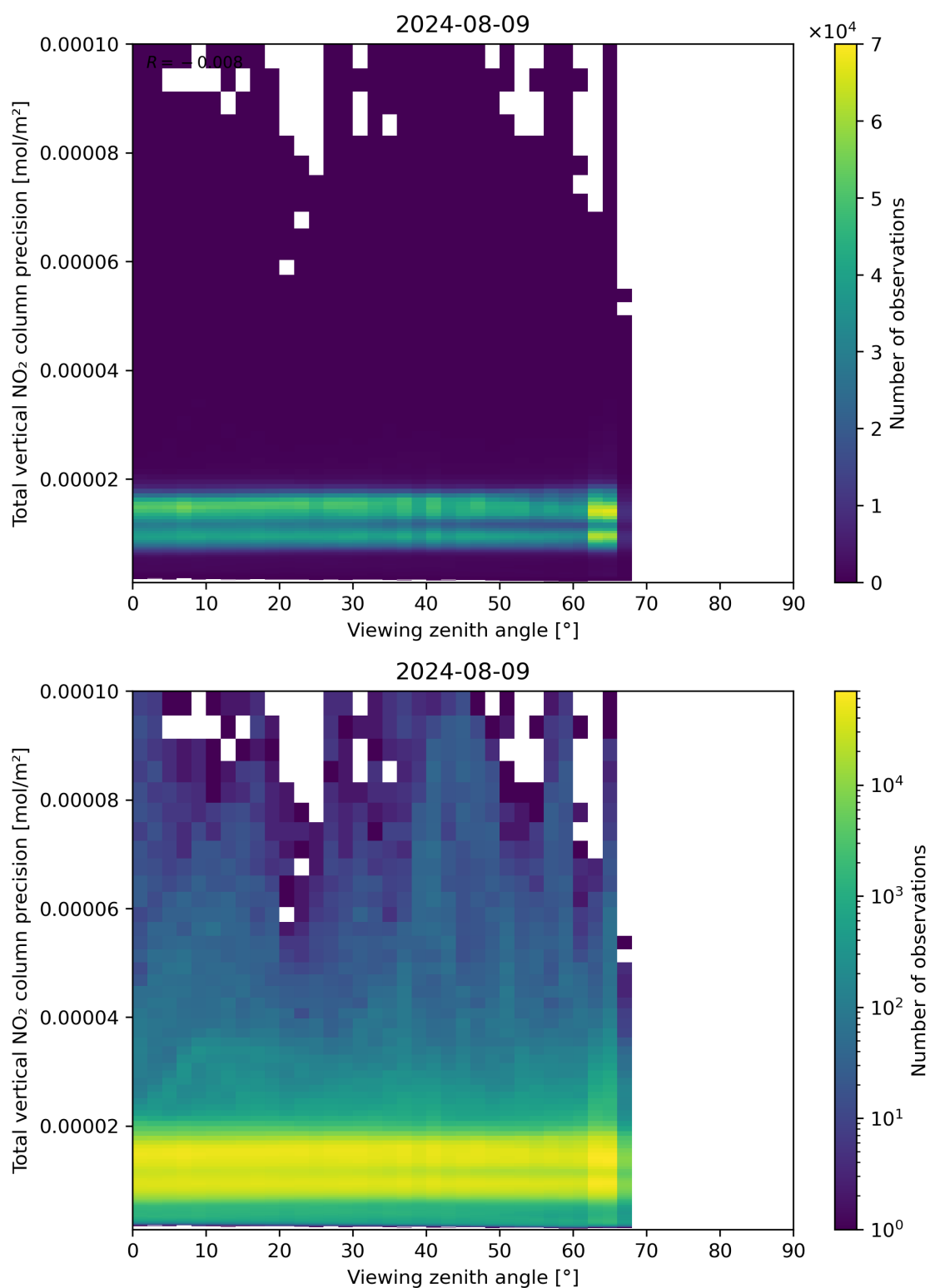
Figure 168: Scatter density plot of “Viewing zenith angle” against “Total vertical NO 2 column precision” for 2024-08-08 to 2024-08-10.
