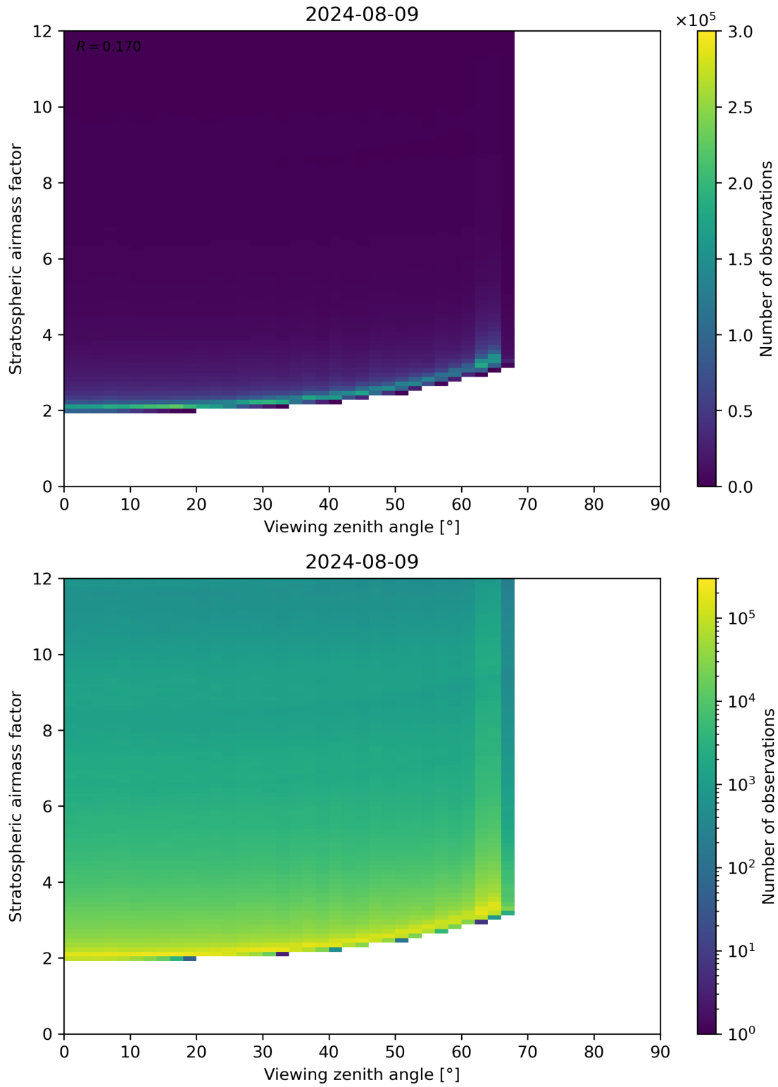
Figure 159: Scatter density plot of “Viewing zenith angle” against “Stratospheric airmass factor” for 2024-08-08 to 2024-08-10.
