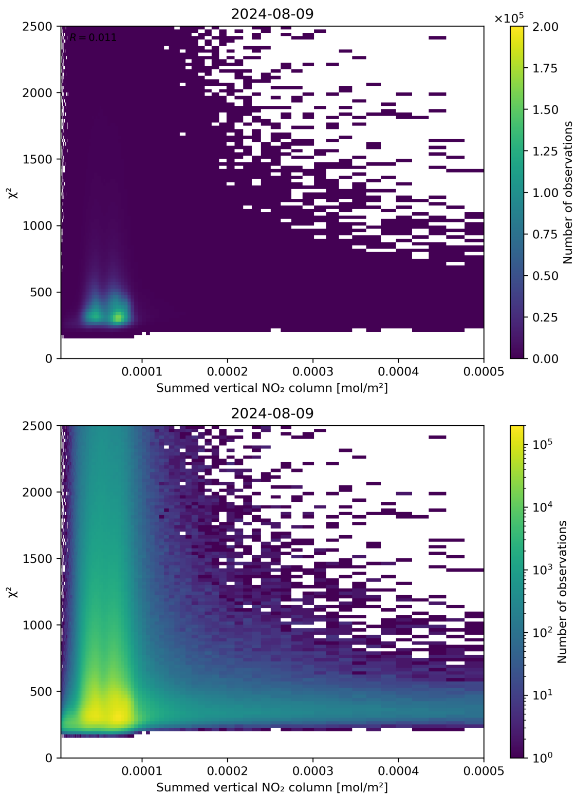
Figure 104: Scatter density plot of “Summed vertical NO 2 column” against “ \chi^2 ” for 2024-08-08 to 2024-08-10.
