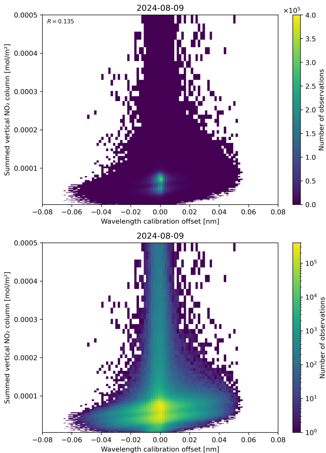
Figure 177: Scatter density plot of “Wavelength calibration offset” against “Summed vertical NO 2 column” for 2024-08-08 to 2024-08-10.
