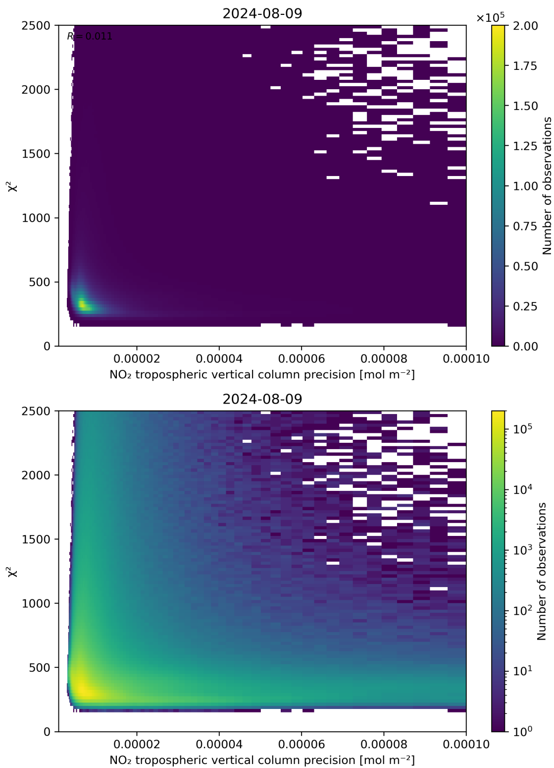
Figure 134: Scatter density plot of “NO 2 tropospheric vertical column precision” against “ \chi^2 ” for 2024-08-08 to 2024-08-10.
