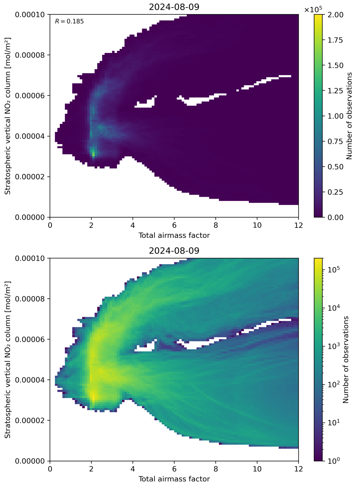
Figure 64: Scatter density plot of “Total airmass factor” against “Stratospheric vertical NO 2 column” for 2024-08-08 to 2024-08-10.
