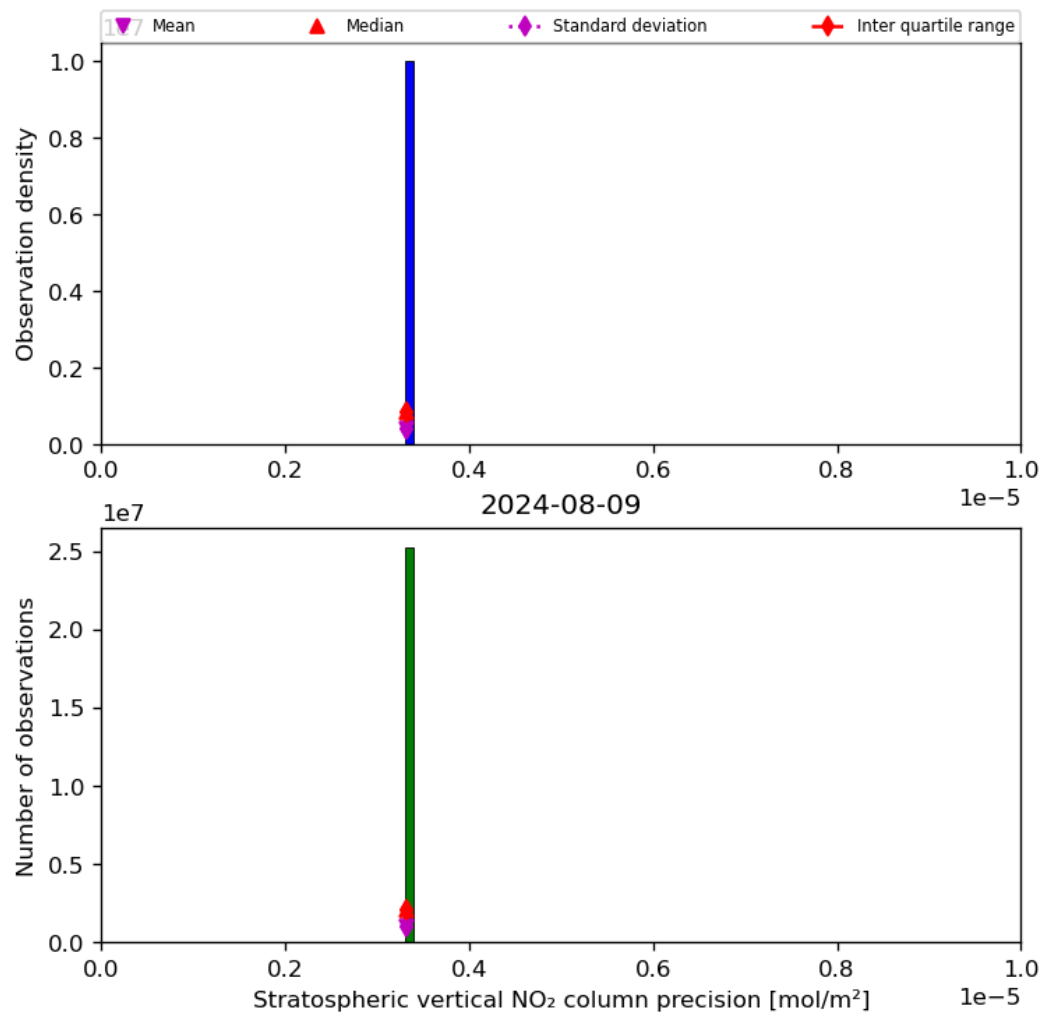
Figure 37: Histogram of “Stratospheric vertical NO 2 column precision” for 2024-08-08 to 2024-08-10
