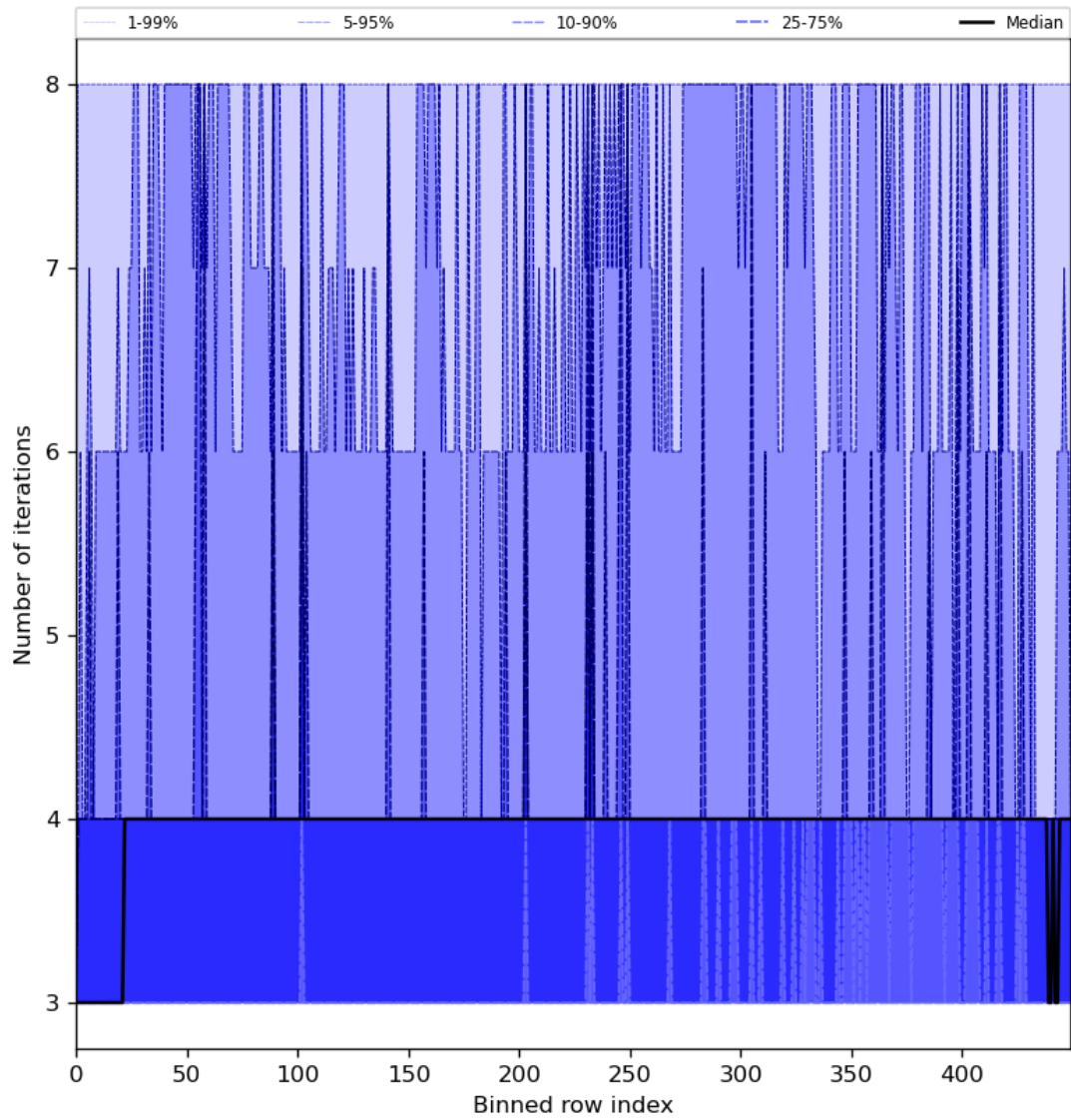
Figure 51: Along track statistics of “Number of iterations” for 2024-08-08 to 2024-08-10
