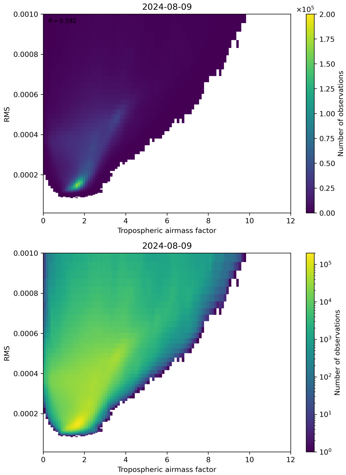
Figure 79: Scatter density plot of “Tropospheric airmass factor” against “RMS” for 2024-08-08 to 2024-08-10.
