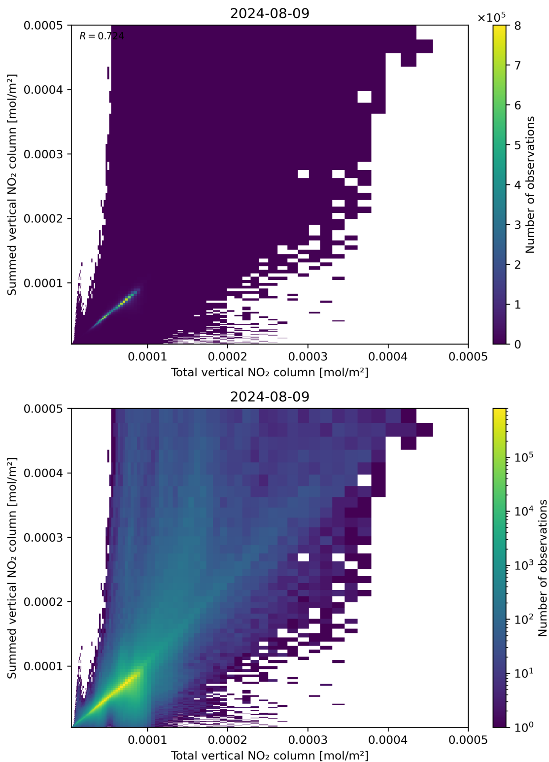
Figure 112: Scatter density plot of “Total vertical NO 2 column” against “Summed vertical NO 2 column” for 2024-08-08 to 2024-08-10.
