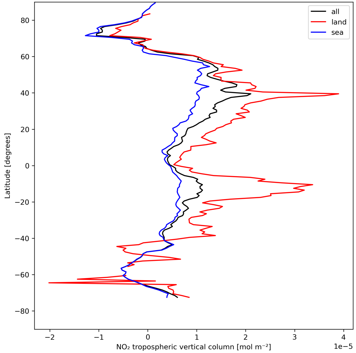
Figure 12: Zonal average of “NO 2 tropospheric vertical column” for 2024-08-08 to 2024-08-10.
