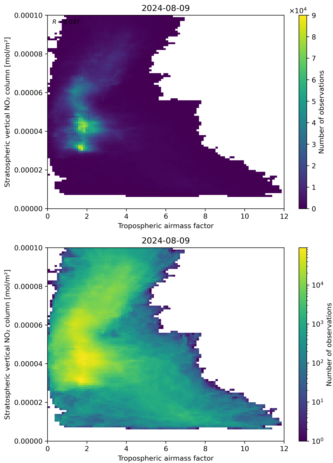
Figure 74: Scatter density plot of “Tropospheric air mass factor” against “Stratospheric vertical NO 2 column” for 2024-08-08 to 2024-08-10.
