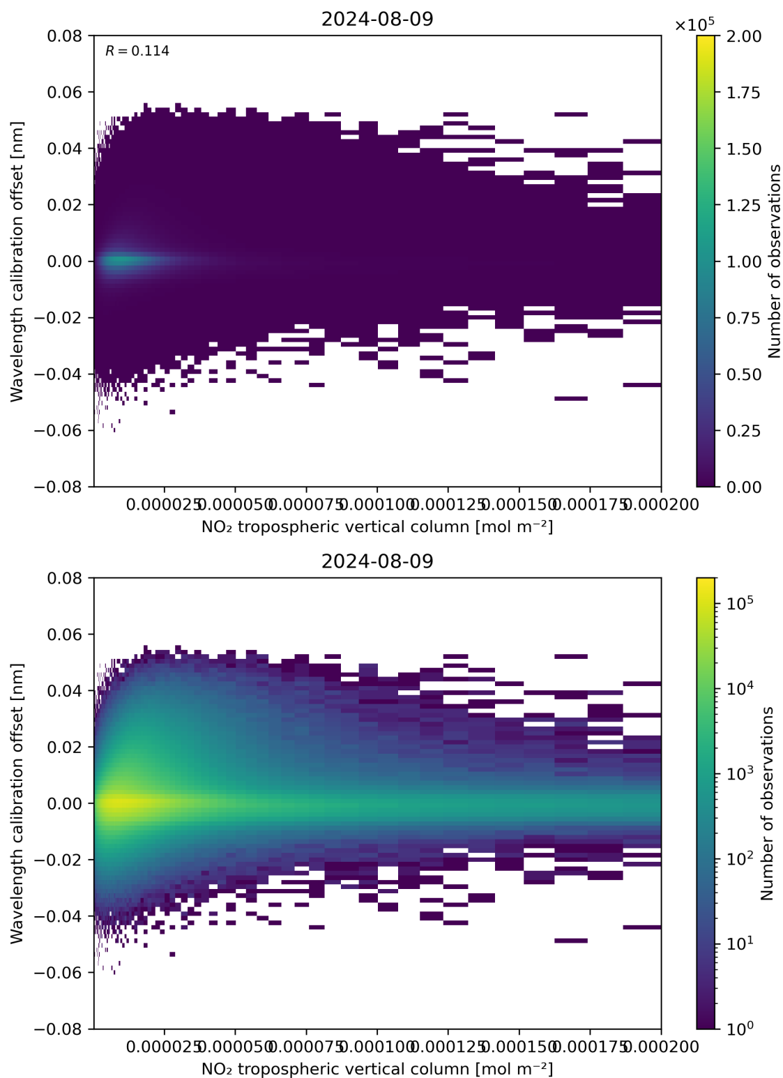
Figure 143: Scatter density plot of “NO 2 tropospheric vertical column” against “Wavelength calibration offset” for 2024-08-08 to 2024-08-10.
