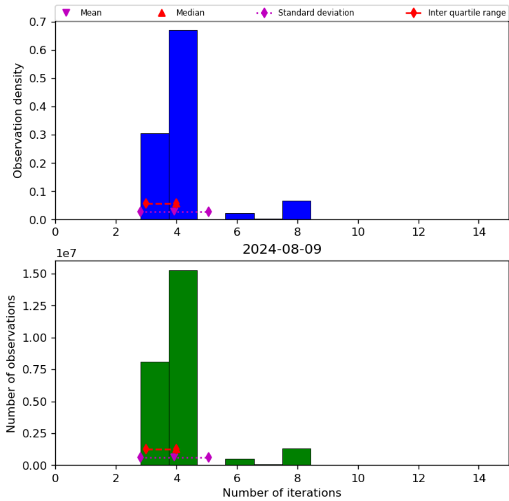
Figure 34: Histogram of “Number of iterations” for 2024-08-08 to 2024-08-10
