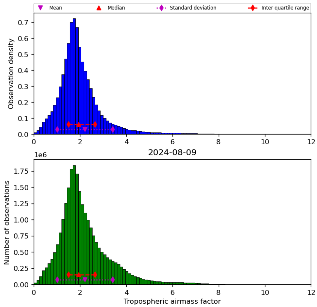
Figure 31: Histogram of “Tropospheric airmass factor” for 2024-08-08 to 2024-08-10
