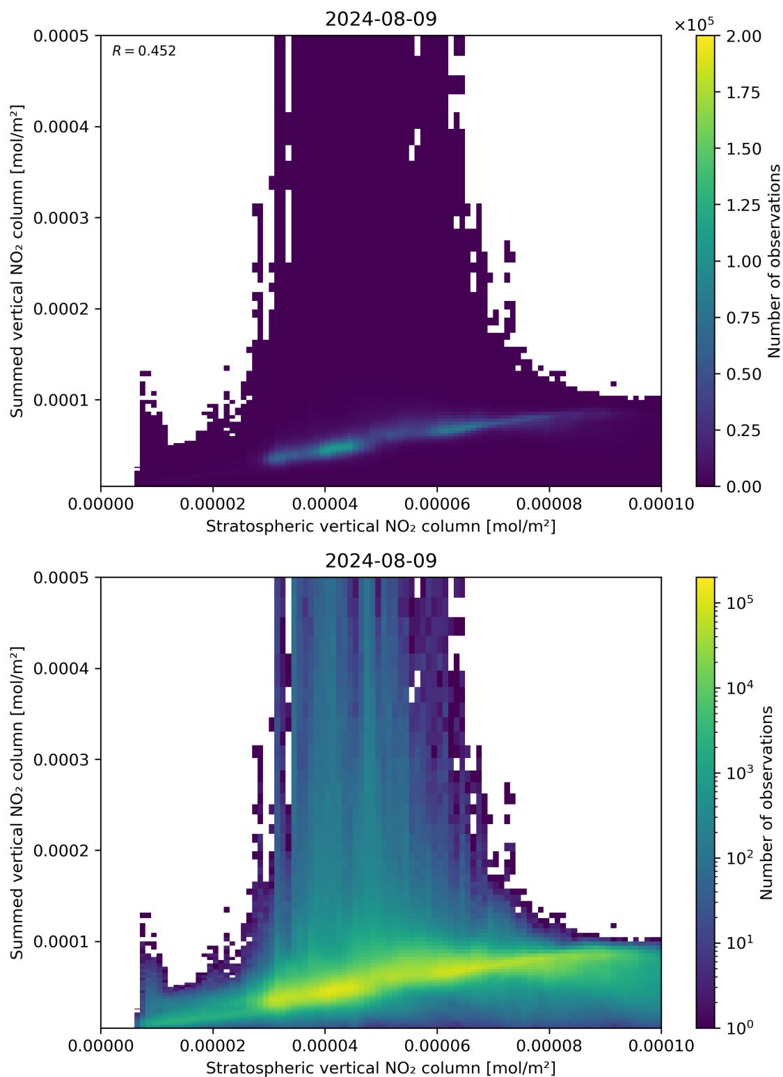
Figure 98: Scatter density plot of “Stratospheric vertical NO 2 column” against “Summed vertical NO 2 column” for 2024-08-08 to 2024-08-10.
