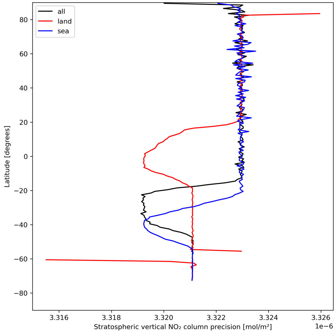
Figure 20: Zonal average of “Stratospheric vertical NO 2 column precision” for 2024-08-08 to 2024-08-10.
