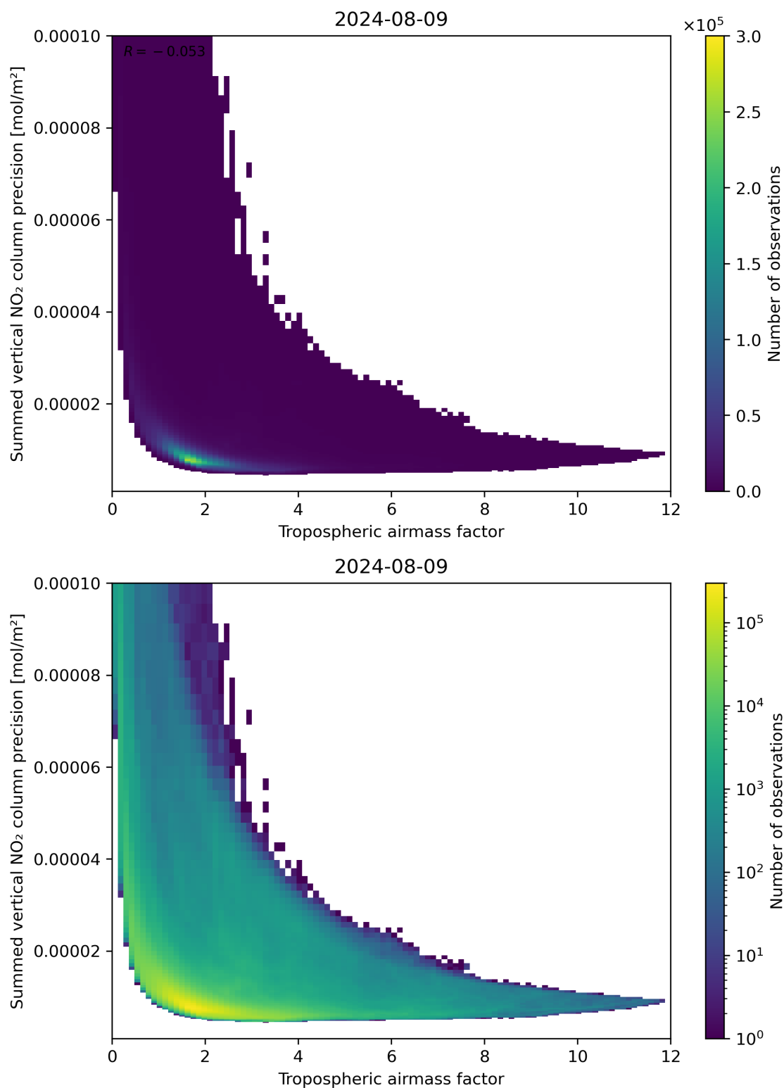
Figure 76: Scatter density plot of “Tropospheric air mass factor” against “Summed vertical NO 2 column precision” for 2024-08-08 to 2024-08-10.
