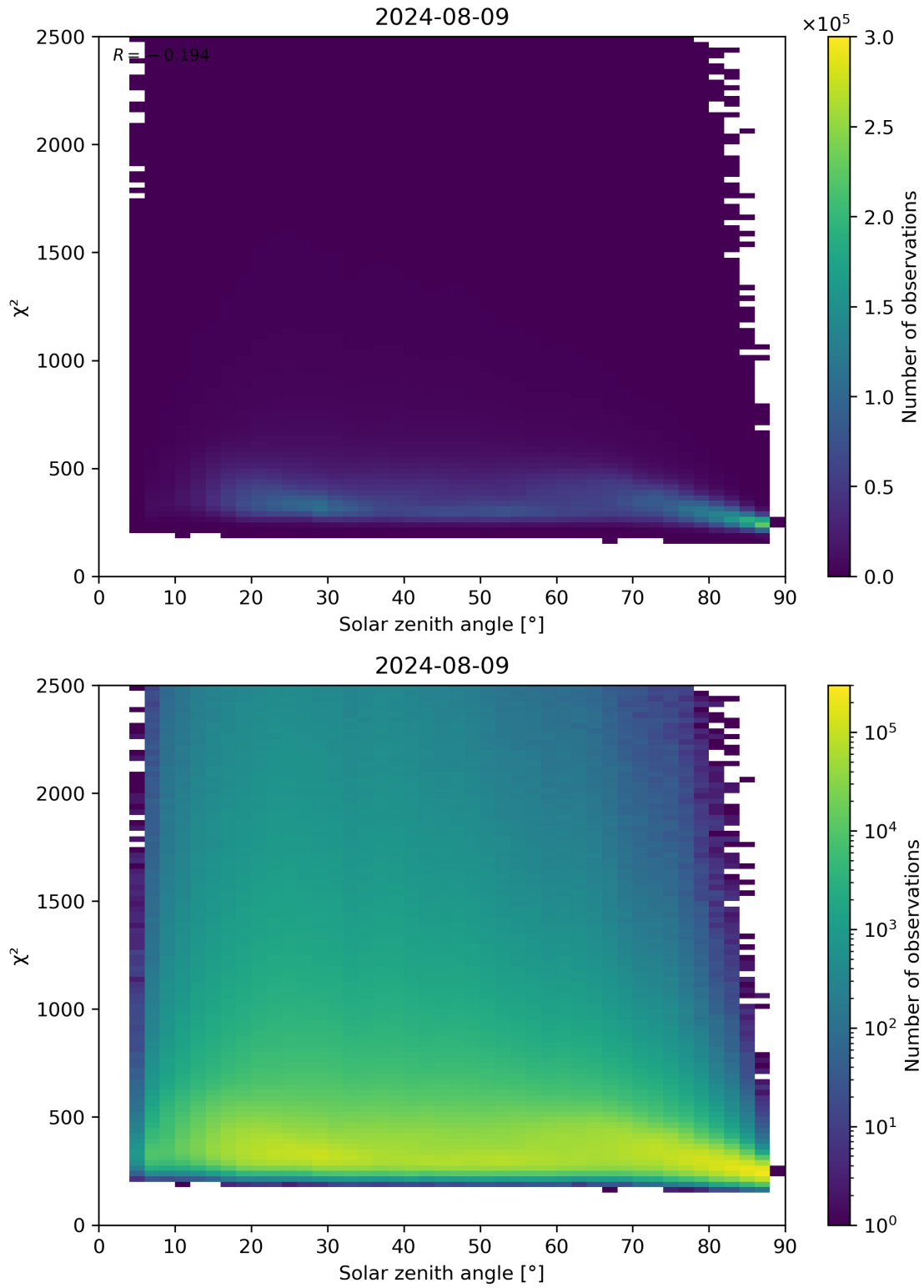
Figure 148: Scatter density plot of “Solar zenith angle” against “ \chi^2 ” for 2024-08-08 to 2024-08-10.
