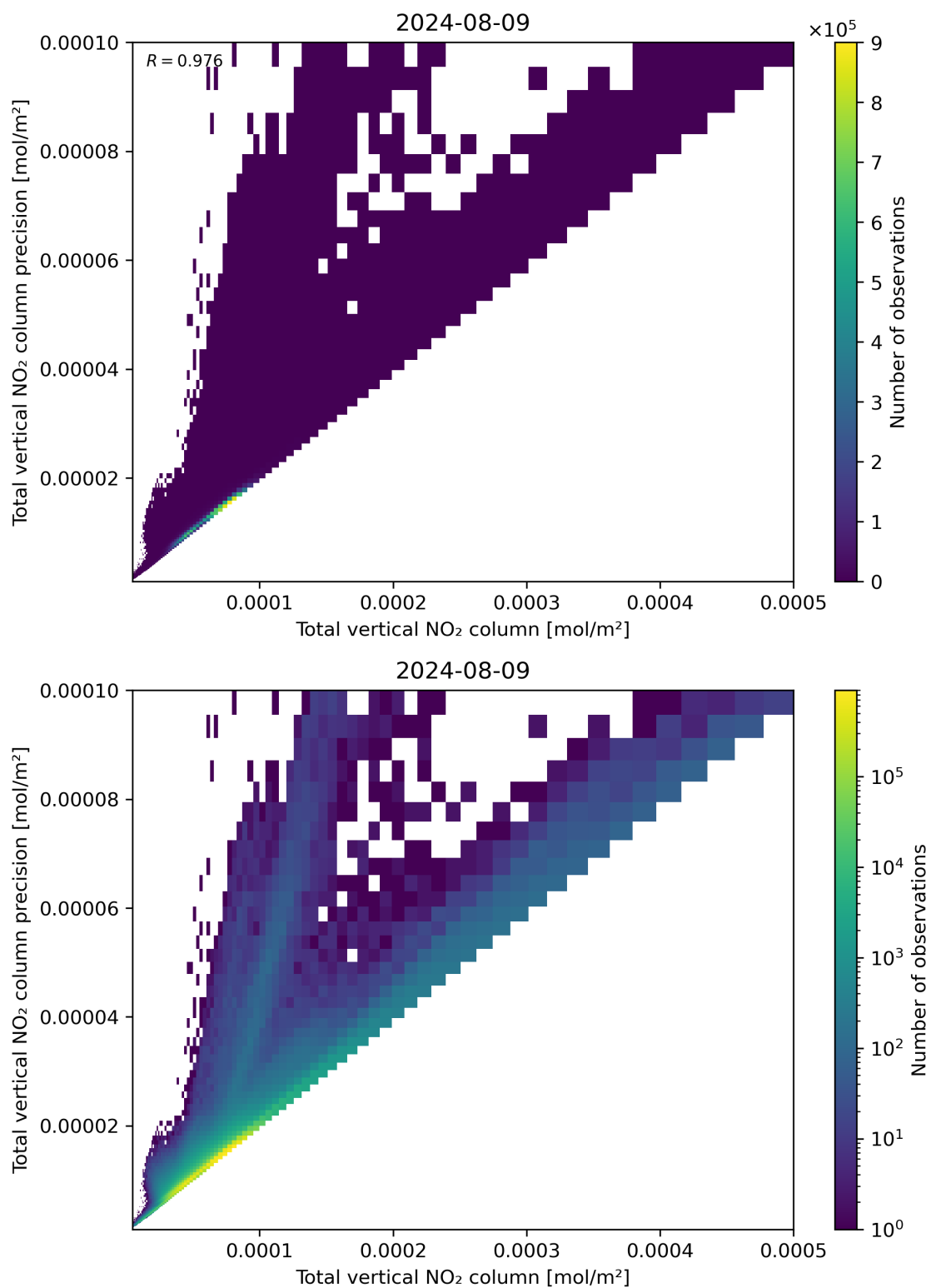
Figure 114: Scatter density plot of “Total vertical NO 2 column” against “Total vertical NO 2 column precision” for 2024-08-08 to 2024-08-10.
