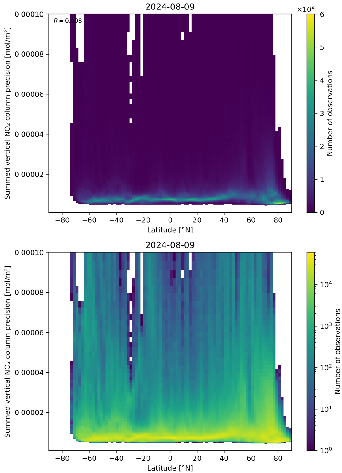
Figure 89: Scatter density plot of “Latitude” against “Summed vertical NO 2 column precision” for 2024-08-08 to 2024-08-10.
