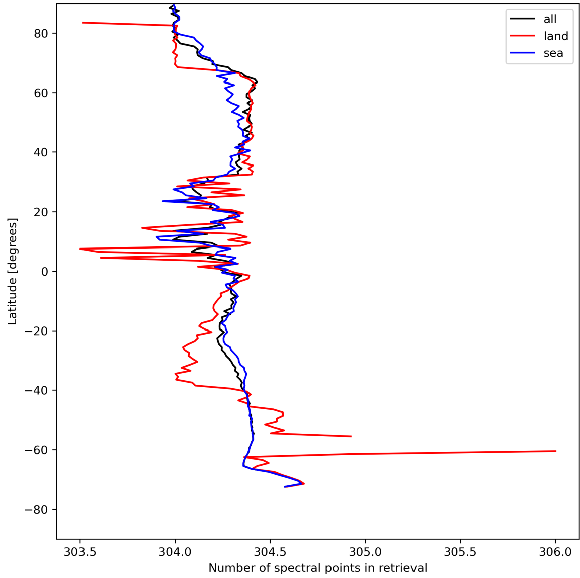
Figure 16: Zonal average of “Number of spectral points in retrieval” for 2024-08-08 to 2024-08-10.
