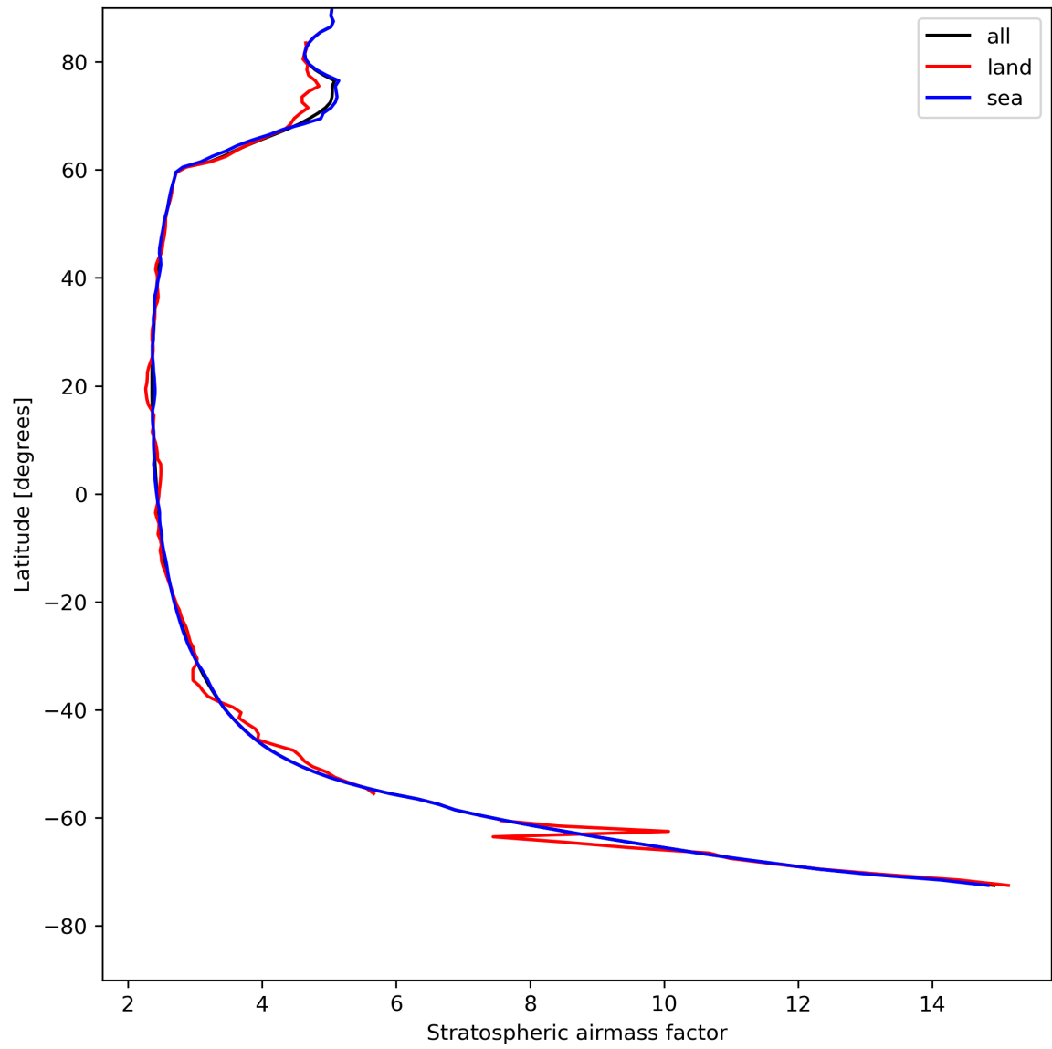
Figure 27: Zonal average of “Stratospheric airmass factor” for 2024-08-08 to 2024-08-10.
