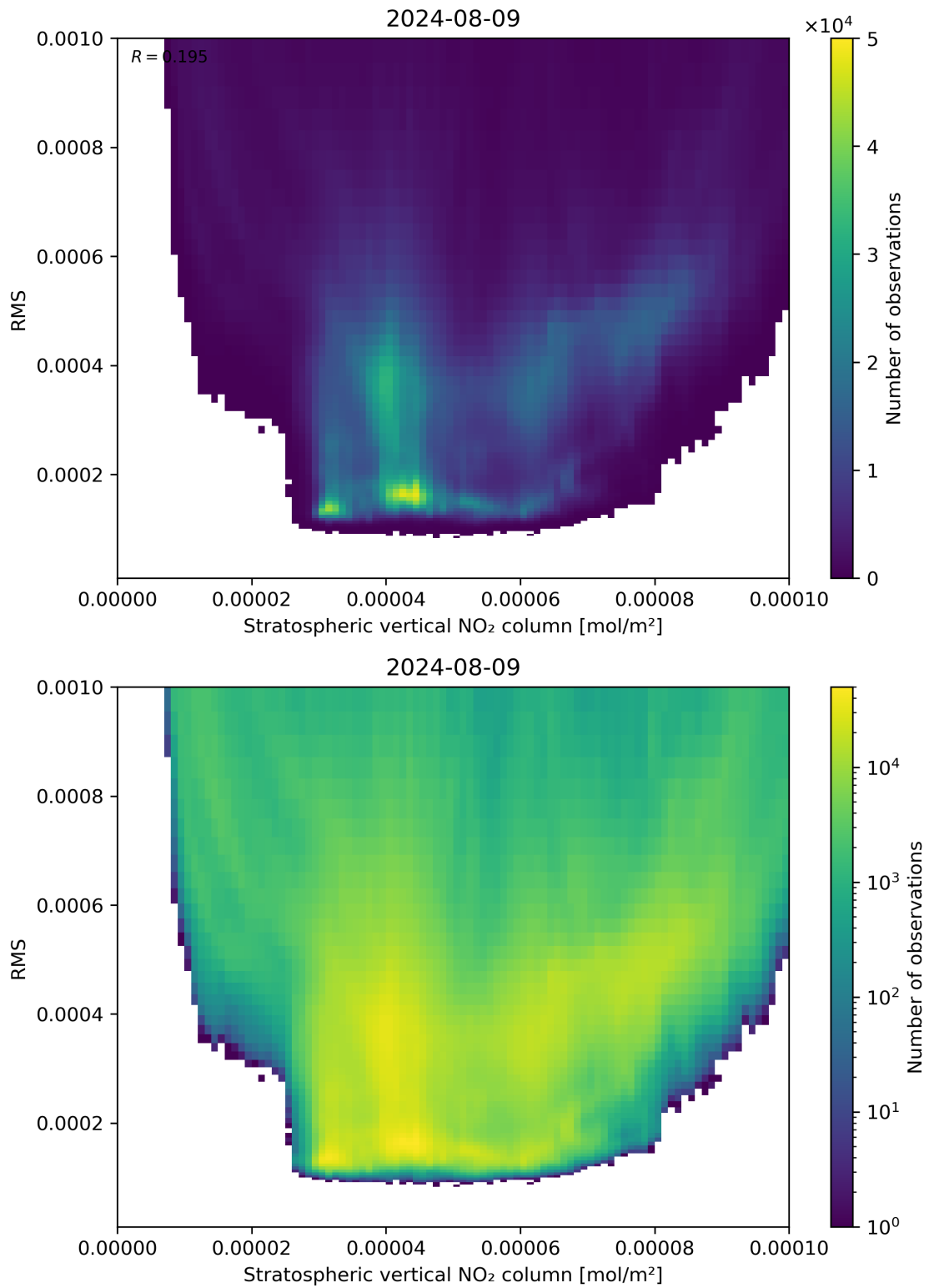
Figure 102: Scatter density plot of “Stratospheric vertical NO 2 column” against “RMS” for 2024-08-08 to 2024-08-10.
