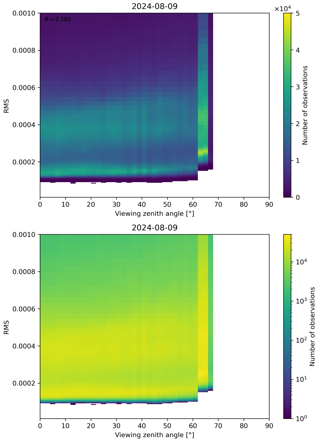
Figure 171: Scatter density plot of “Viewing zenith angle” against “RMS” for 2024-08-08 to 2024-08-10.
