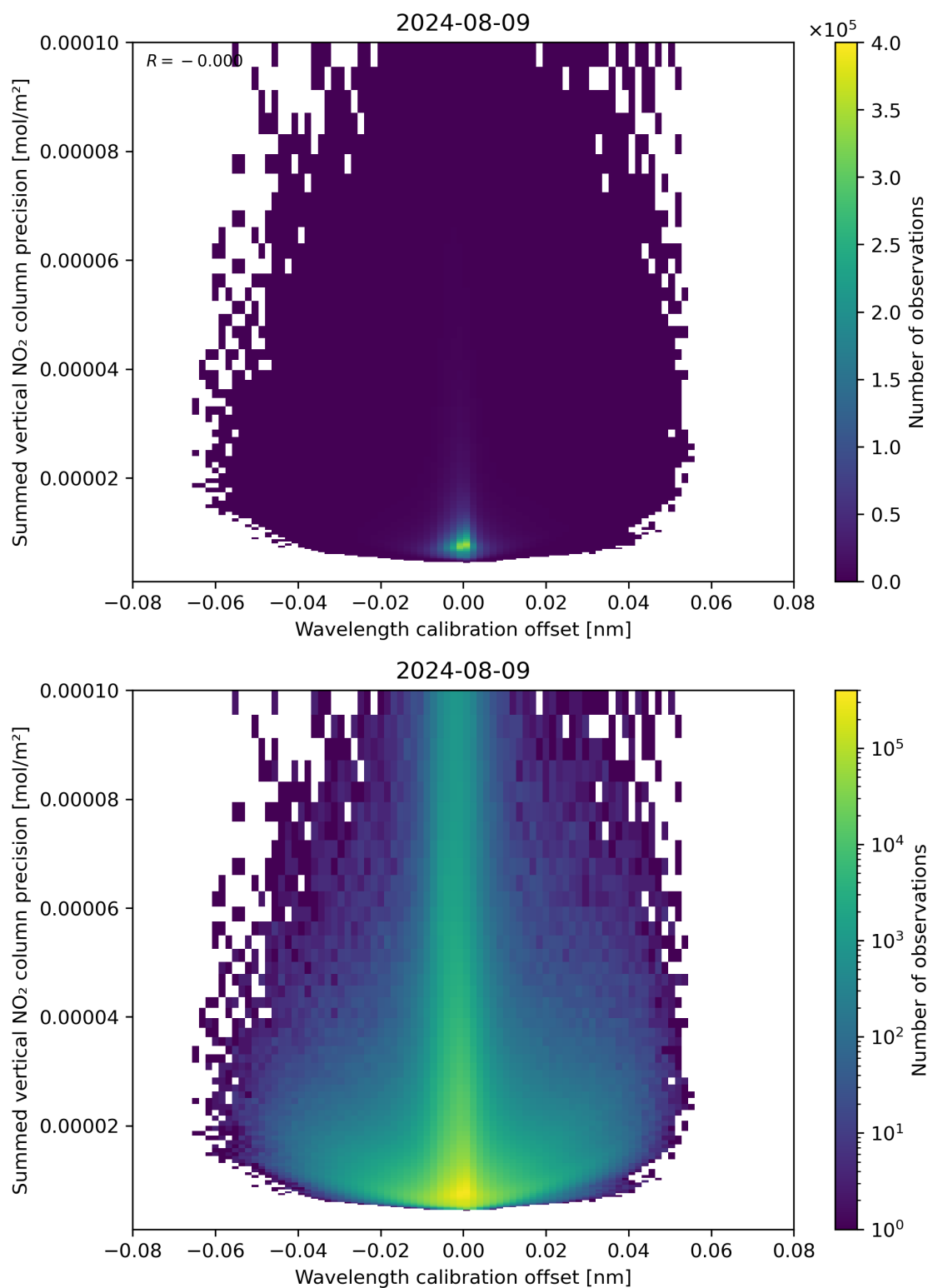
Figure 178: Scatter density plot of “Wavelength calibration offset” against “Summed vertical NO 2 column precision” for 2024-08-08 to 2024-08-10.
