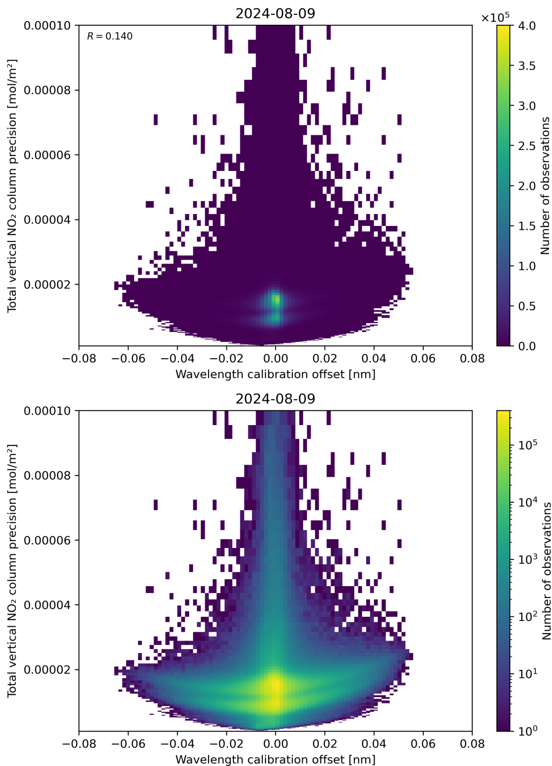
Figure 180: Scatter density plot of “Wavelength calibration offset” against “Total vertical NO 2 column precision” for 2024-08-08 to 2024-08-10.
