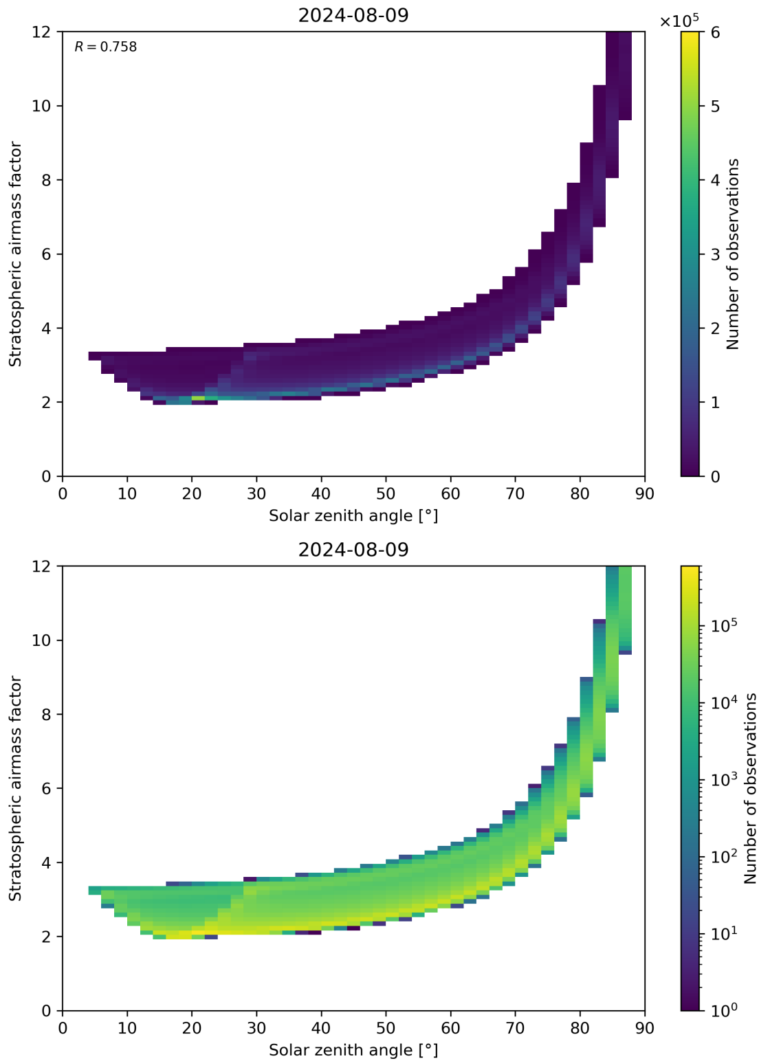
Figure 145: Scatter density plot of “Solar zenith angle” against “Stratospheric airmass factor” for 2024-08-08 to 2024-08-10.
