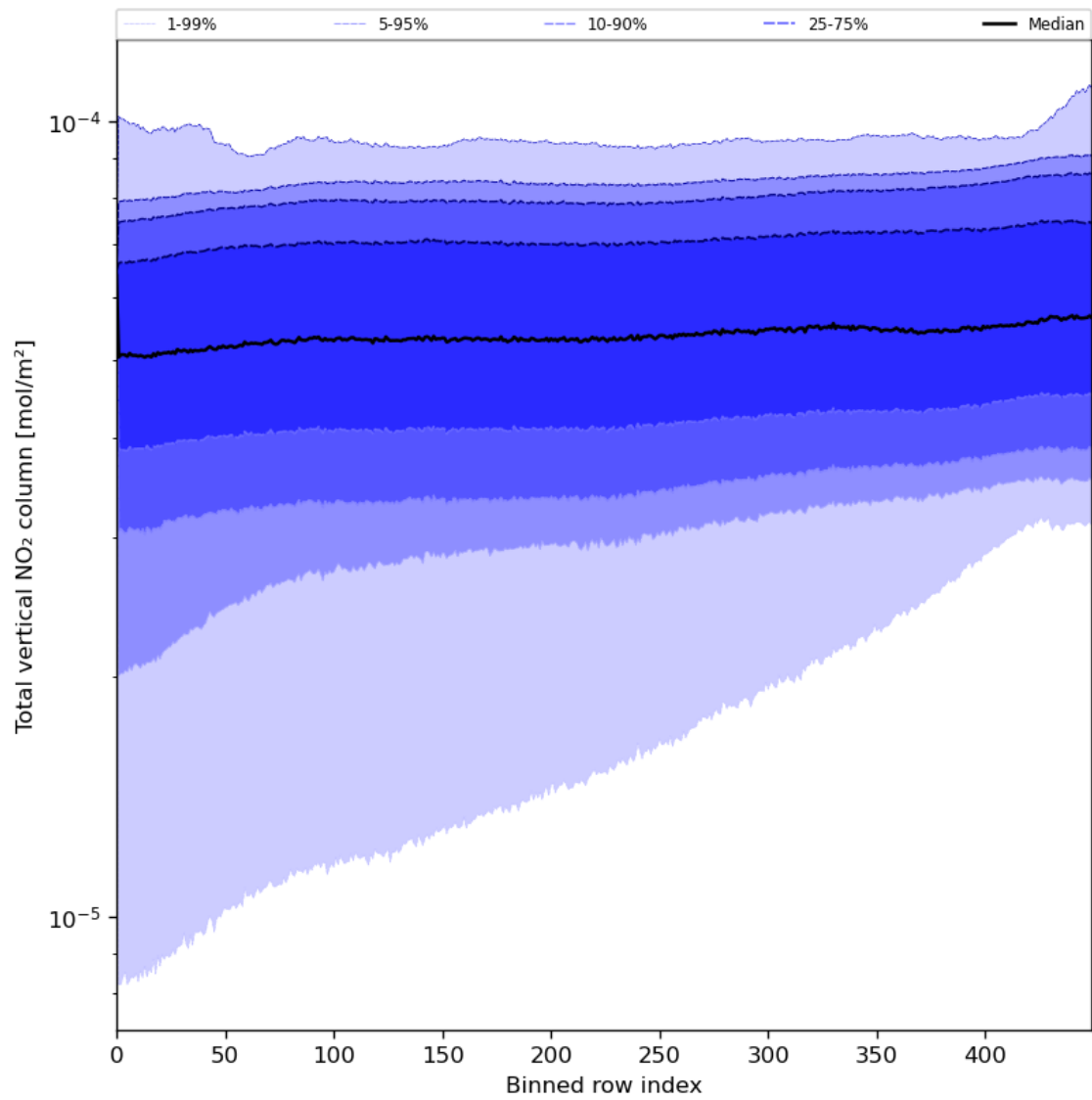
Figure 55: Along track statistics of “Total vertical NO 2 column” for 2024-08-08 to 2024-08-10
