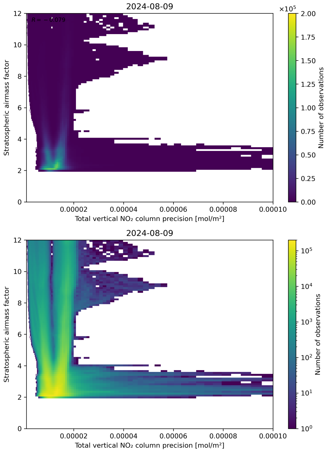
Figure 115: Scatter density plot of “Total vertical NO 2 column precision” against “Stratospheric air mass factor” for 2024-08-08 to 2024-08-10.
