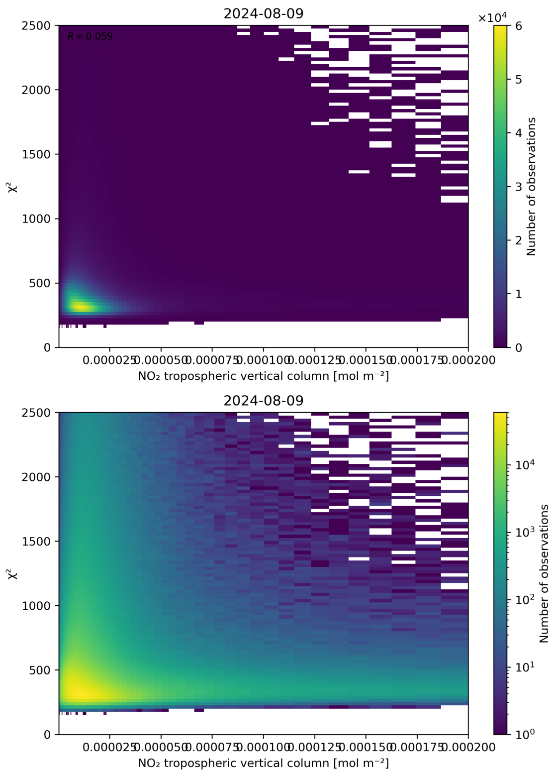
Figure 124: Scatter density plot of “NO 2 tropospheric vertical column” against “ \chi^2 ” for 2024-08-08 to 2024-08-10.
