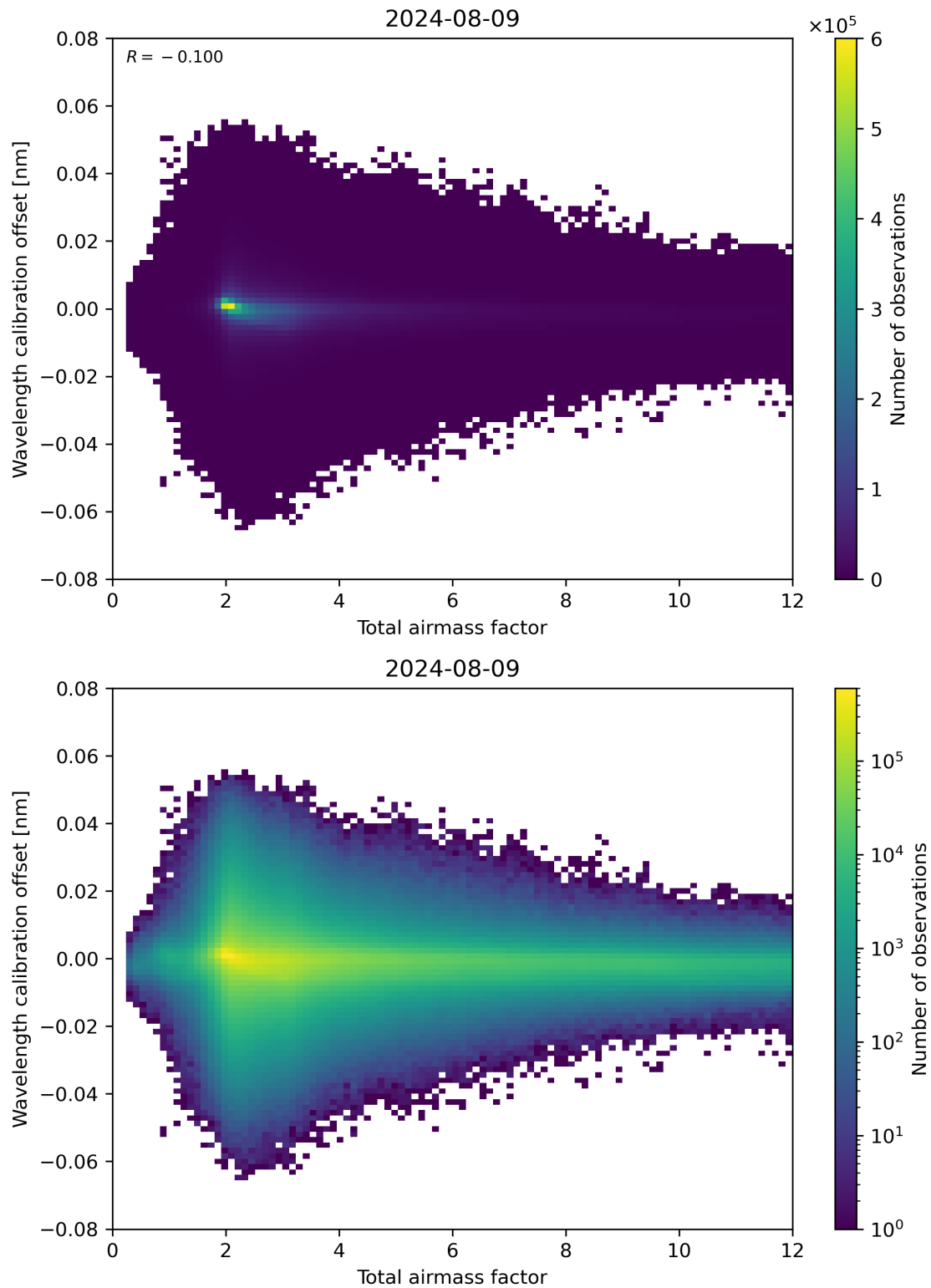
Figure 70: Scatter density plot of “Total airmass factor” against “Wavelength calibration offset” for 2024-08-08 to 2024-08-10.
