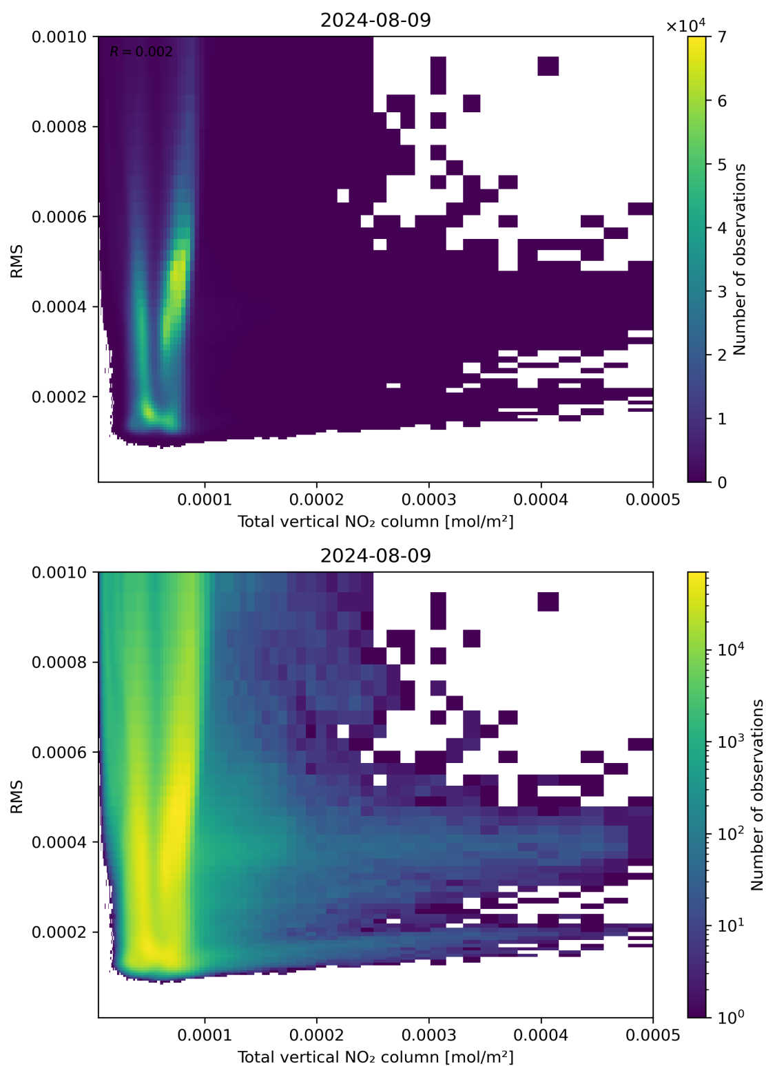
Figure 120: Scatter density plot of “Total vertical NO 2 column” against “RMS” for 2024-08-08 to 2024-08-10.
