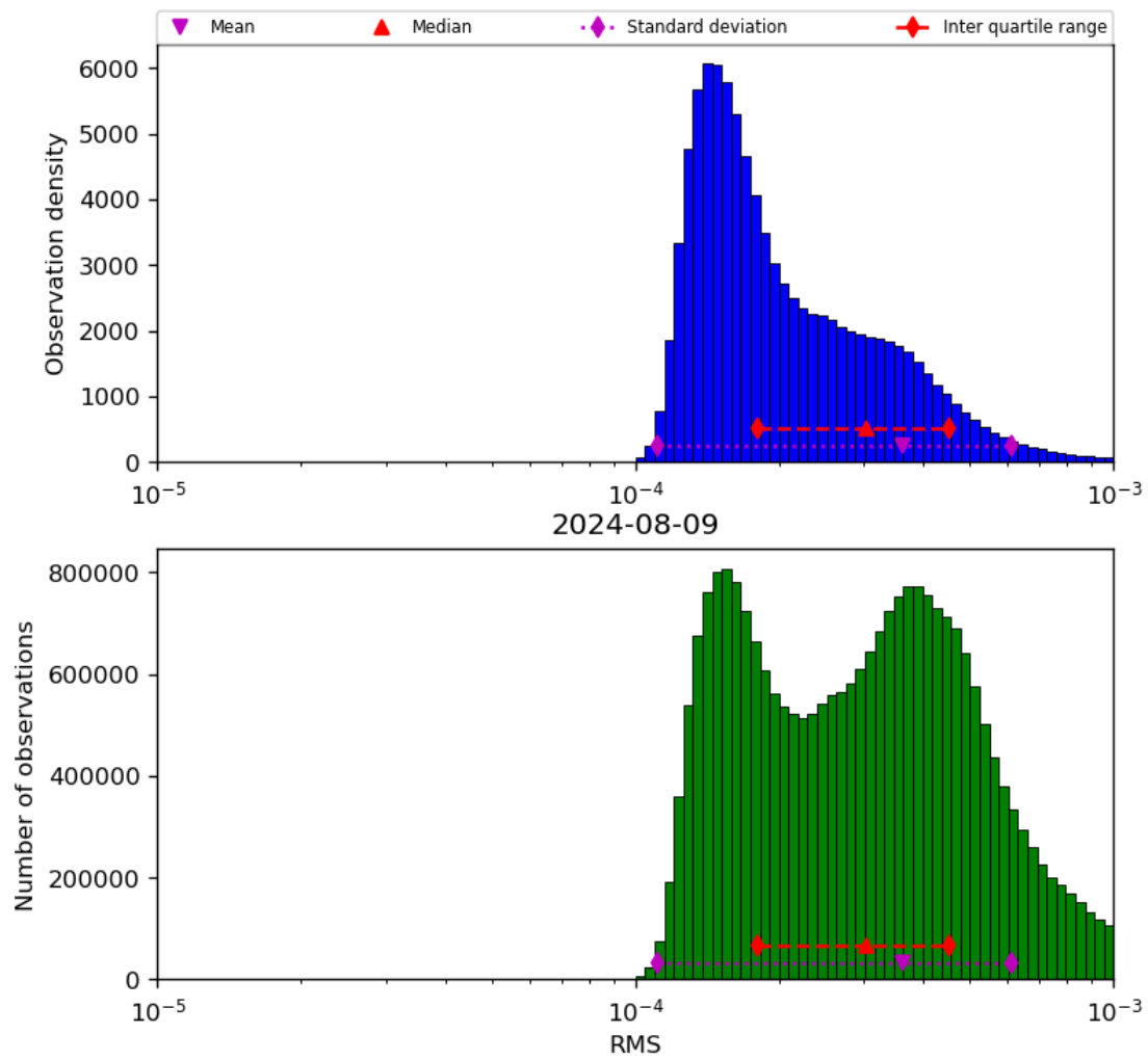
Figure 43: Histogram of “RMS” for 2024-08-08 to 2024-08-10
