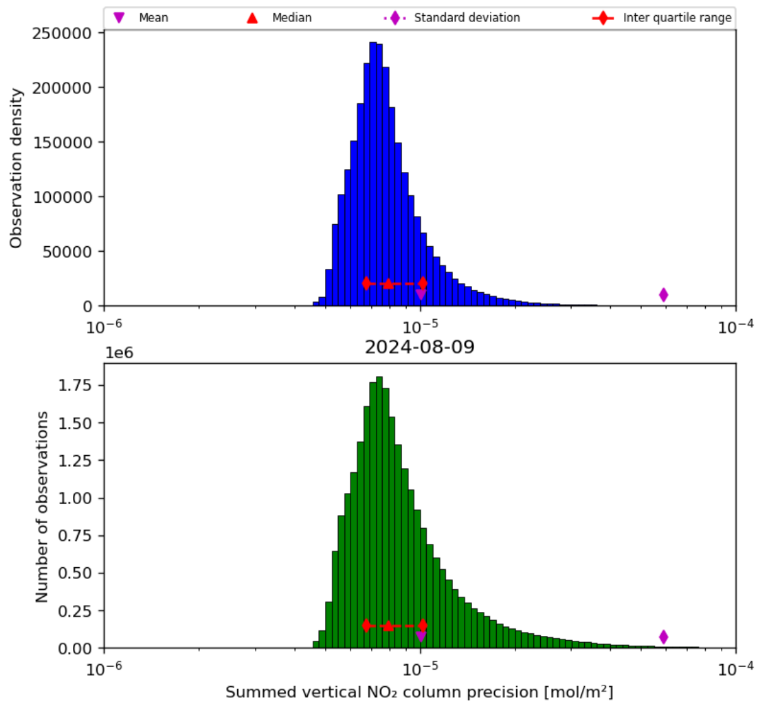
Figure 41: Histogram of “Summed vertical NO 2 column precision” for 2024-08-08 to 2024-08-10
