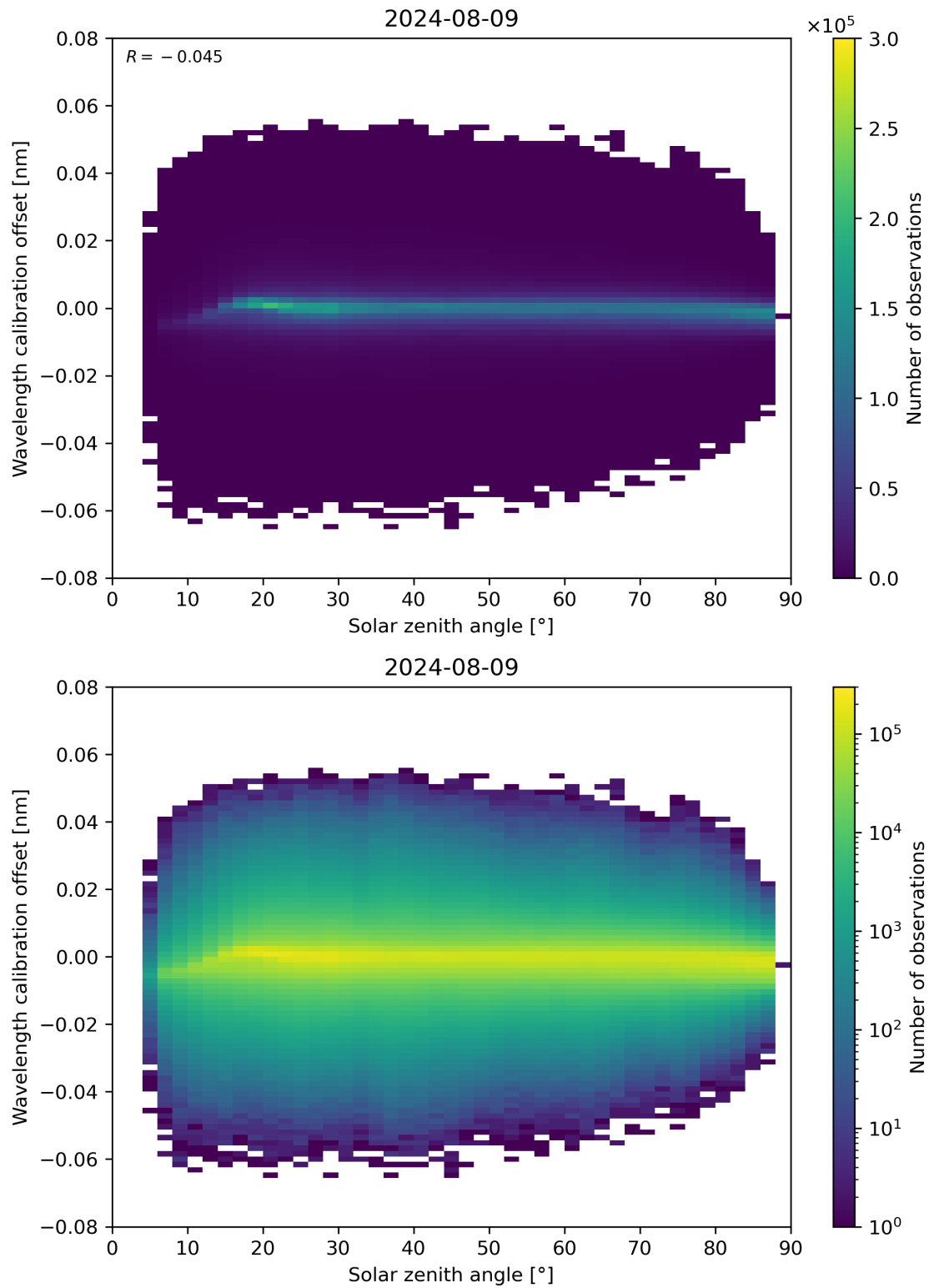
Figure 158: Scatter density plot of “Solar zenith angle” against “Wavelength calibration offset” for 2024-08-08 to 2024-08-10.
