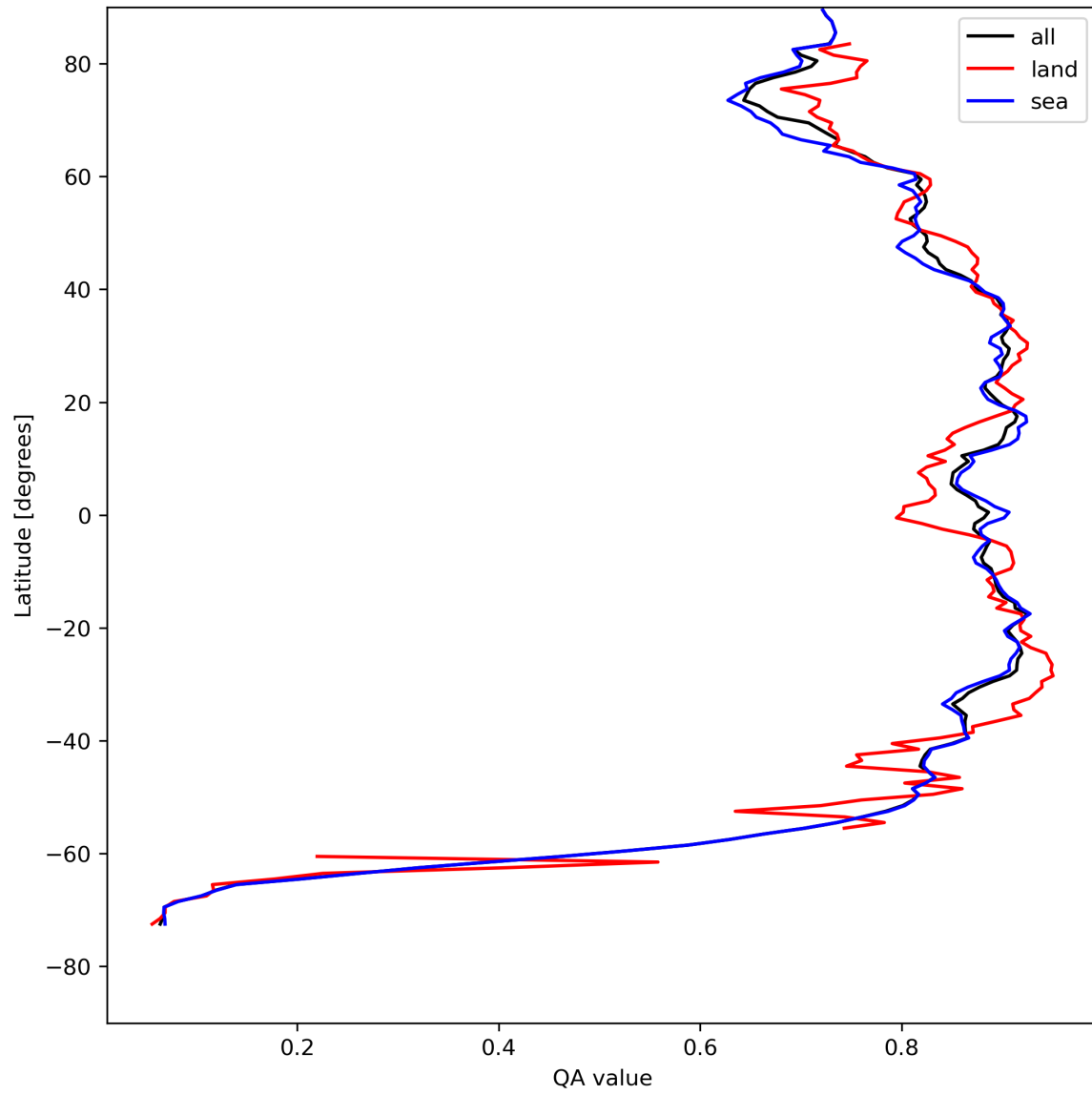
Figure 11: Zonal average of “QA value” for 2024-08-08 to 2024-08-10.
