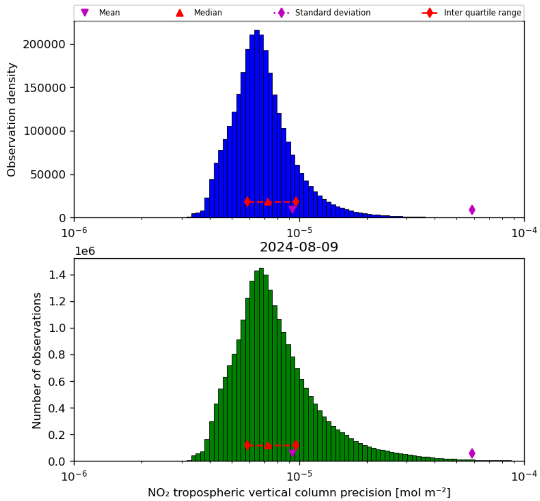
Figure 30: Histogram of “NO 2 tropospheric vertical column precision” for 2024-08-08 to 2024-08-10
