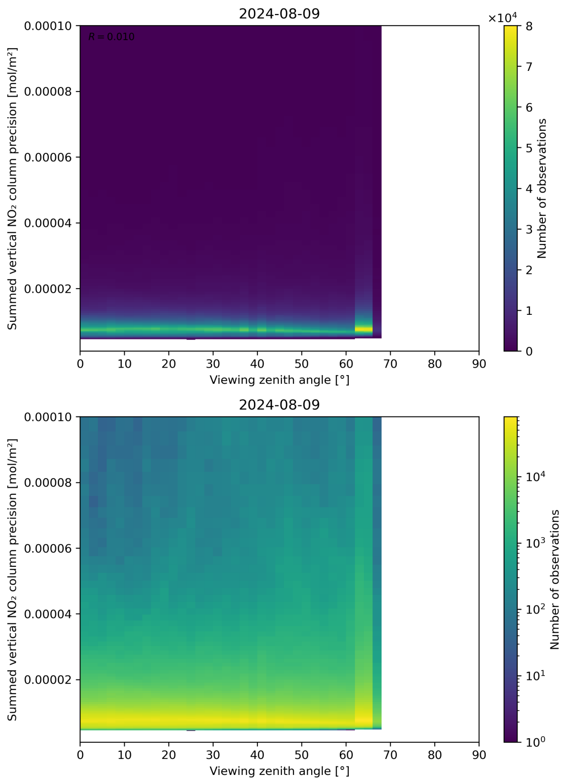
Figure 166: Scatter density plot of “Viewing zenith angle” against “Summed vertical NO 2 column precision” for 2024-08-08 to 2024-08-10.
