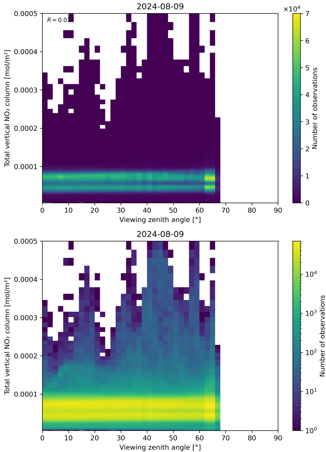
Figure 167: Scatter density plot of “Viewing zenith angle” against “Total vertical NO 2 column” for 2024-08-08 to 2024-08-10.
