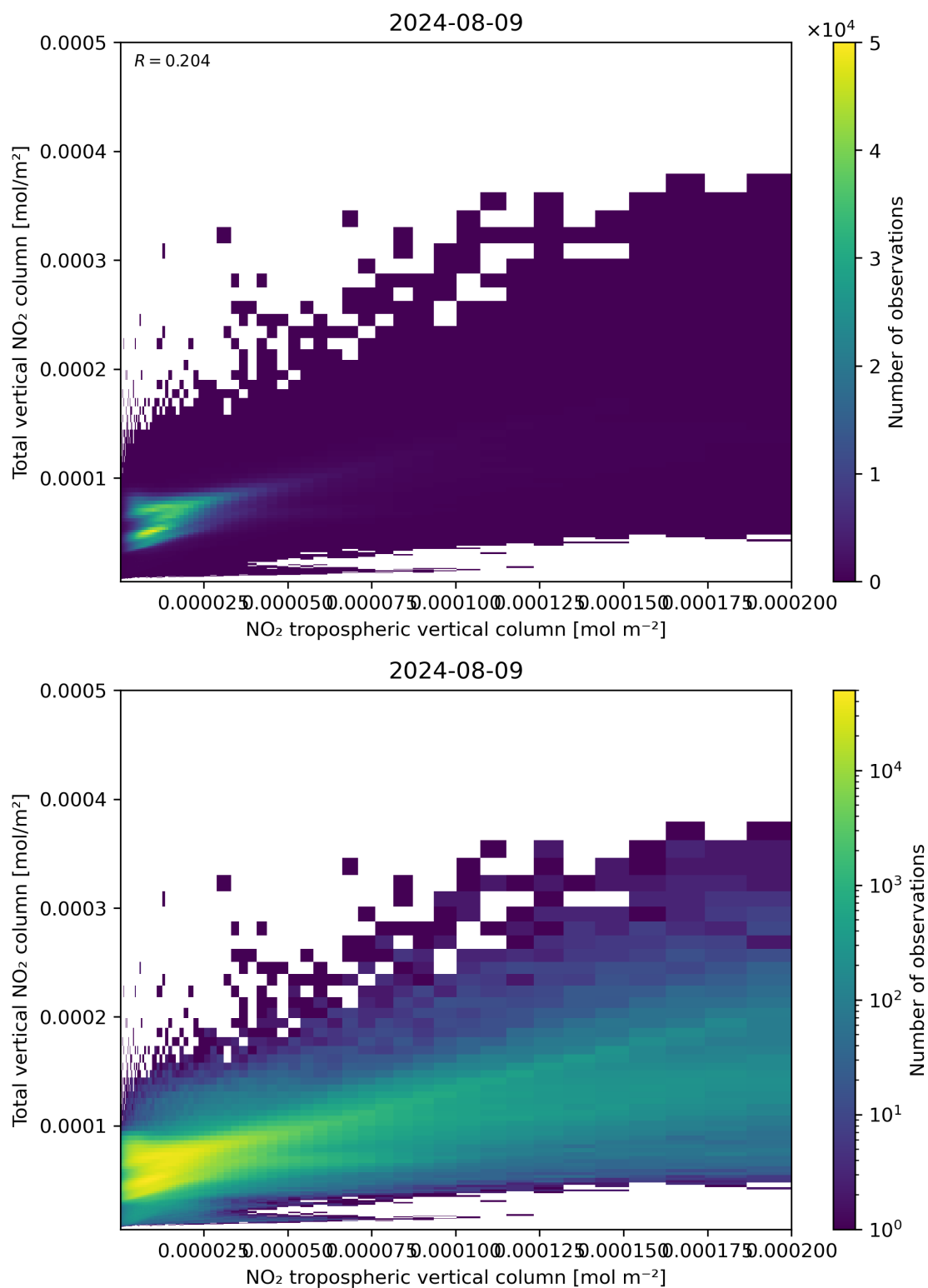
Figure 128: Scatter density plot of “NO 2 tropospheric vertical column” against “Total vertical NO 2 column” for 2024-08-08 to 2024-08-10.
