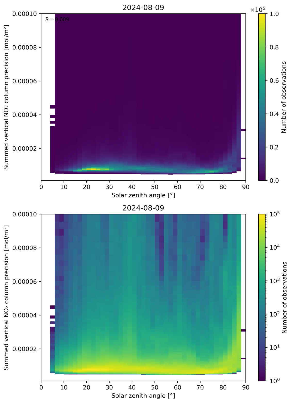
Figure 152: Scatter density plot of “Solar zenith angle” against “Summed vertical NO 2 column precision” for 2024-08-08 to 2024-08-10.
