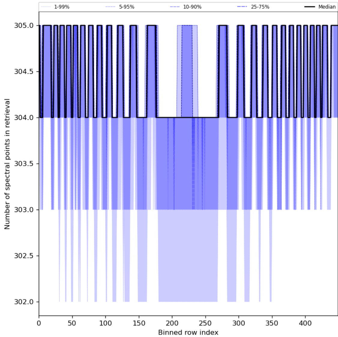
Figure 50: Along track statistics of “Number of spectral points in retrieval” for 2024-08-08 to 2024-08-10
