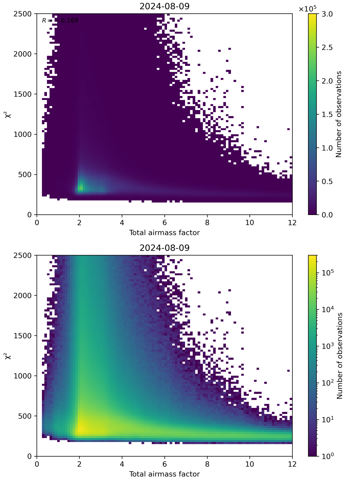
Figure 63: Scatter density plot of “Total airmass factor” against “ \chi^2 ” for 2024-08-08 to 2024-08-10.
