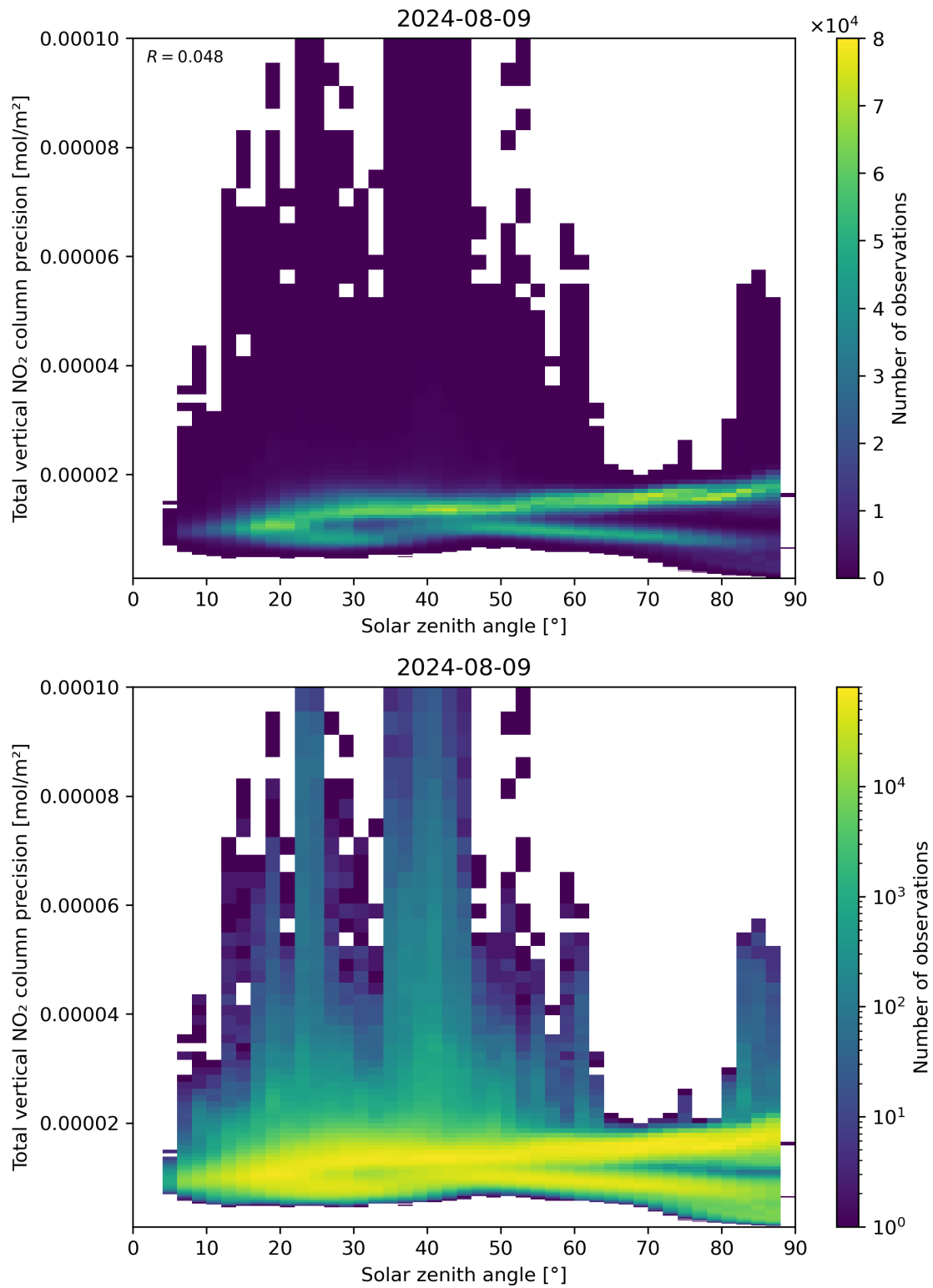
Figure 154: Scatter density plot of “Solar zenith angle” against “Total vertical NO 2 column precision” for 2024-08-08 to 2024-08-10.
