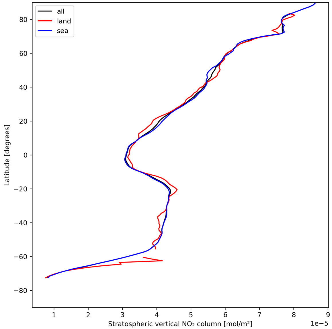
Figure 19: Zonal average of “Stratospheric vertical NO 2 column” for 2024-08-08 to 2024-08-10.
