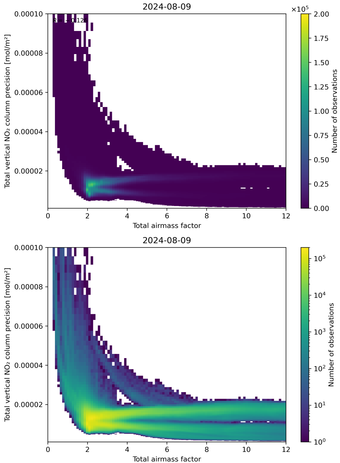
Figure 68: Scatter density plot of “Total airmass factor” against “Total vertical NO 2 column precision” for 2024-08-08 to 2024-08-10.
