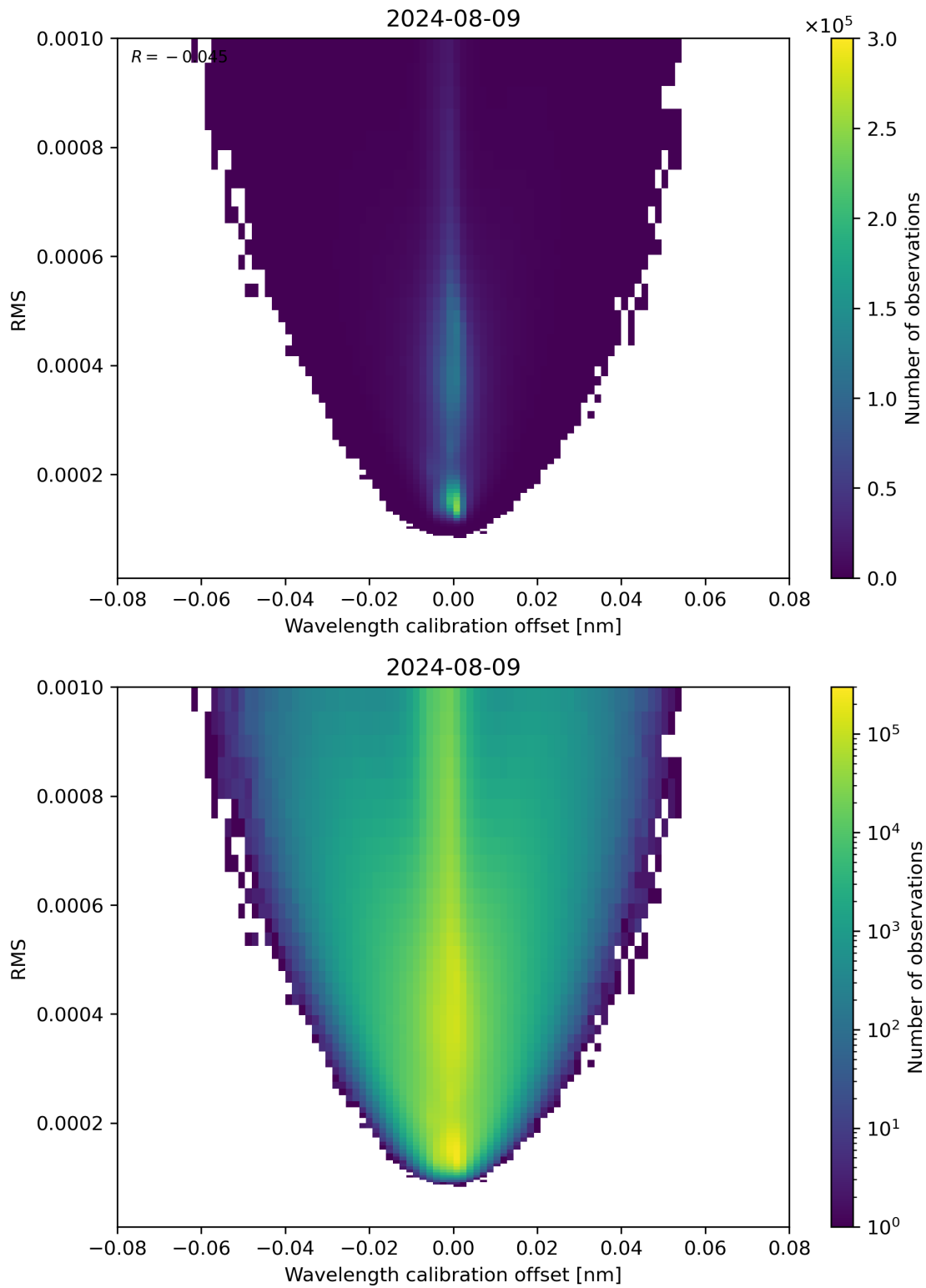
Figure 181: Scatter density plot of “Wavelength calibration offset” against “RMS” for 2024-08-08 to 2024-08-10.
