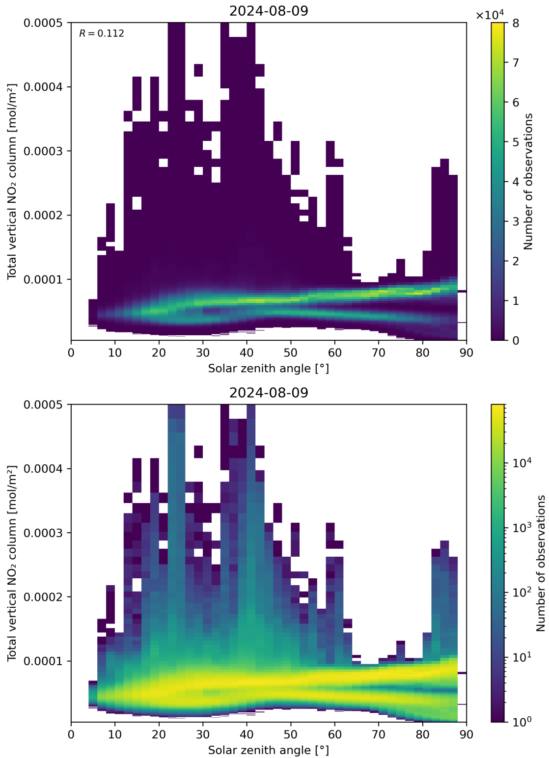
Figure 153: Scatter density plot of “Solar zenith angle” against “Total vertical NO 2 column” for 2024-08-08 to 2024-08-10.
