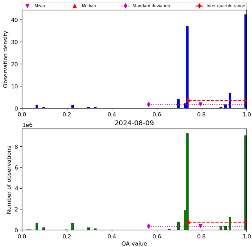
Figure 28: Histogram of “QA value” for 2024-08-08 to 2024-08-10
