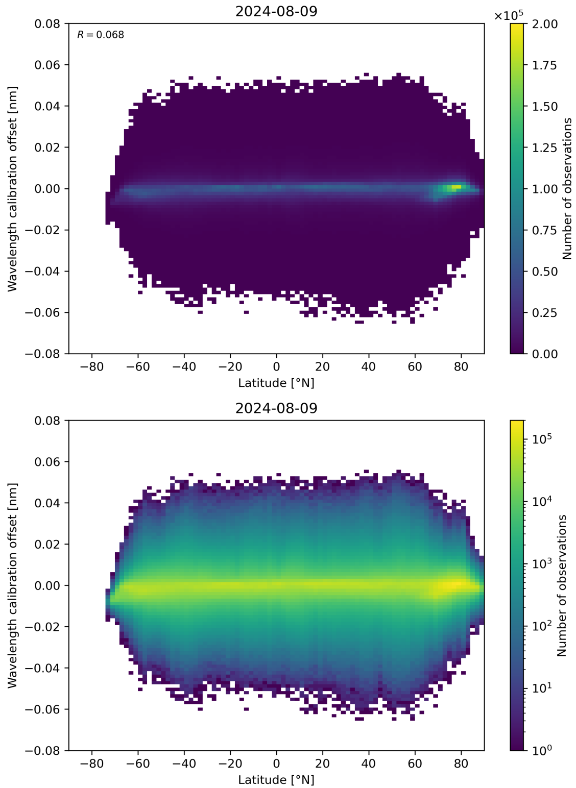
Figure 95: Scatter density plot of “Latitude” against “Wavelength calibration offset” for 2024-08-08 to 2024-08-10.
