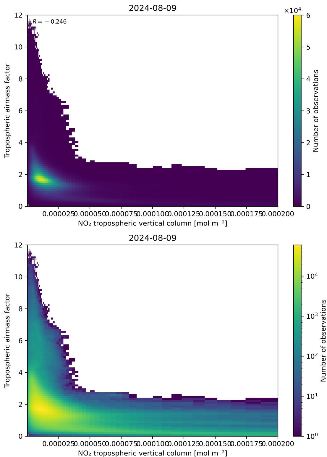
Figure 123: Scatter density plot of “NO 2 tropospheric vertical column” against “Tropospheric air mass factor” for 2024-08-08 to 2024-08-10.
