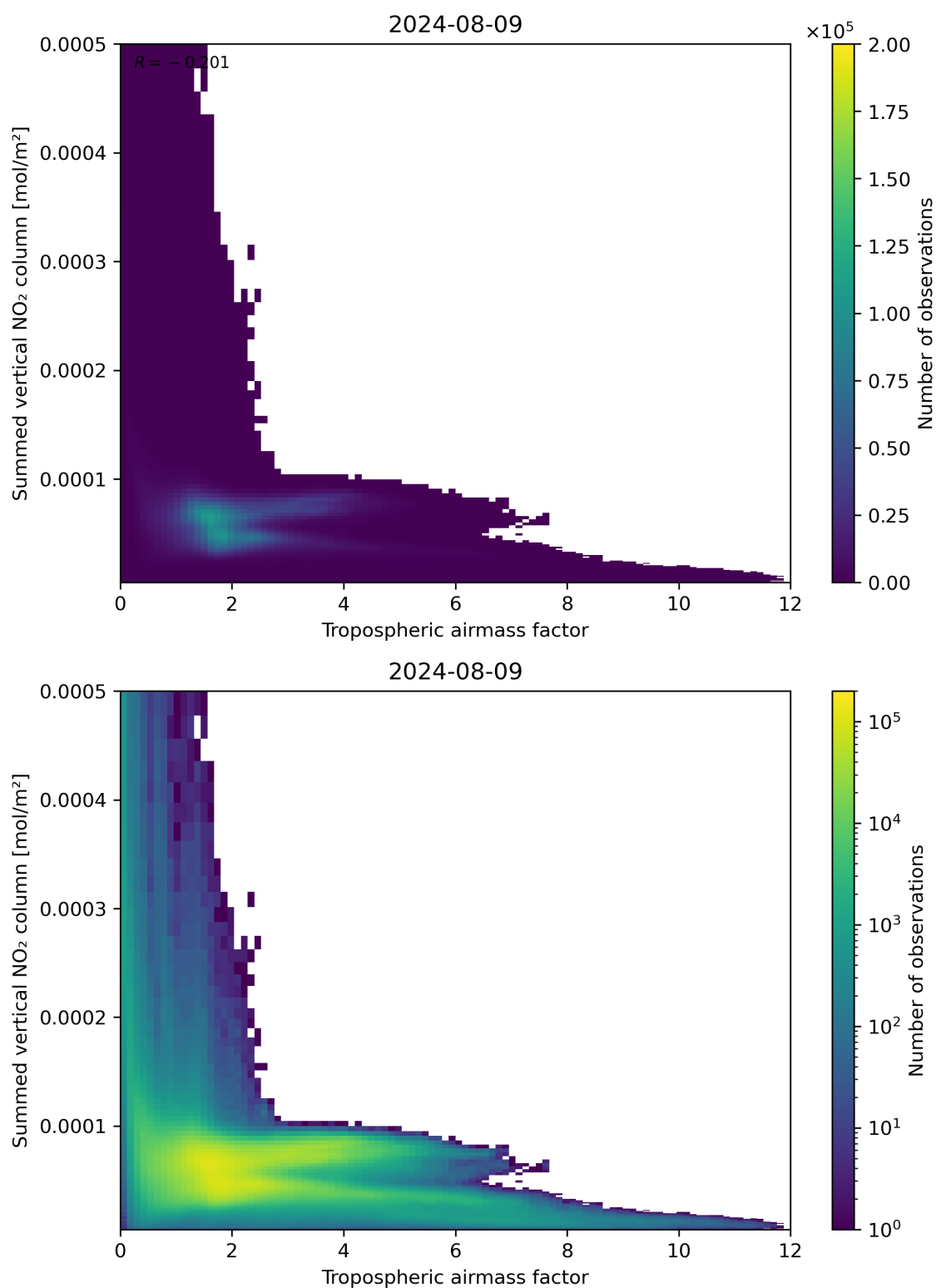
Figure 75: Scatter density plot of “Tropospheric airmass factor” against “Summed vertical NO 2 column” for 2024-08-08 to 2024-08-10.
