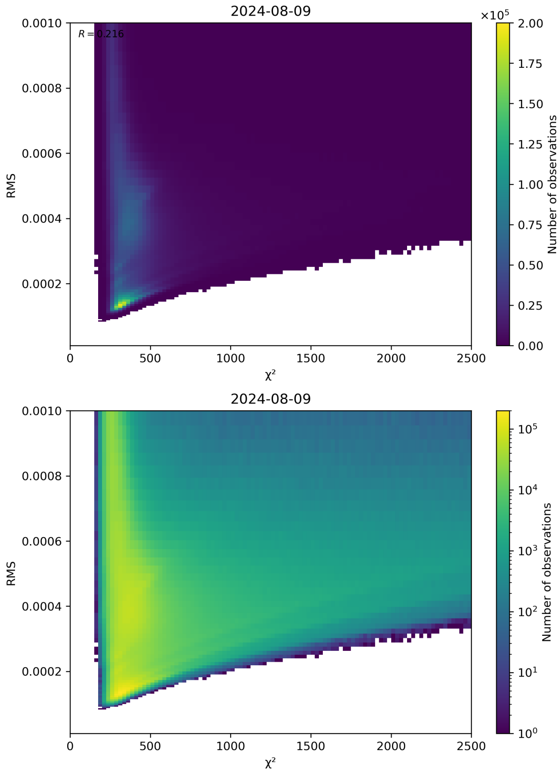
Figure 82: Scatter density plot of “ \chi^2 ” against “RMS” for 2024-08-08 to 2024-08-10.
