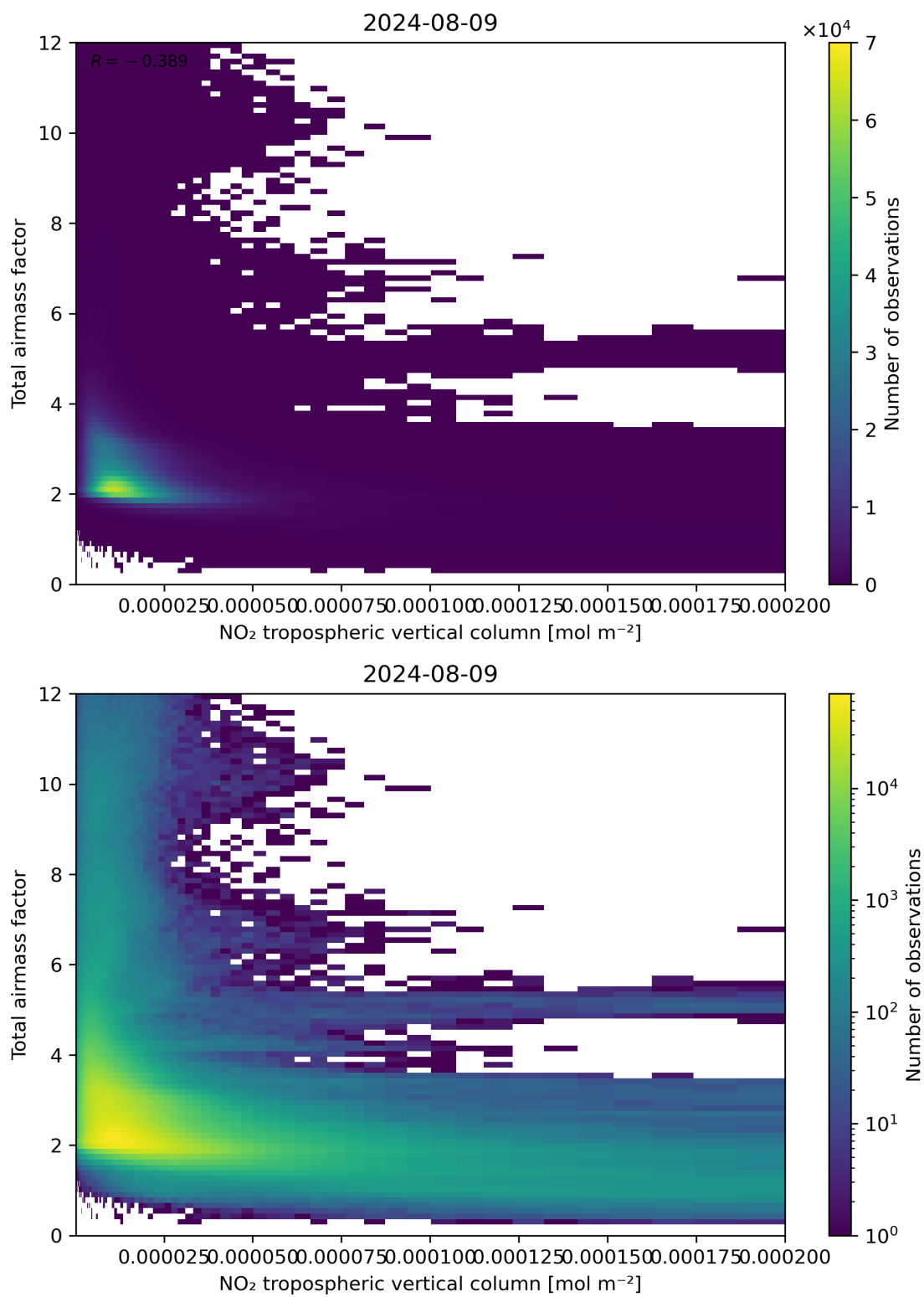
Figure 122: Scatter density plot of “NO 2 tropospheric vertical column” against “Total air mass factor” for 2024-08-08 to 2024-08-10.
