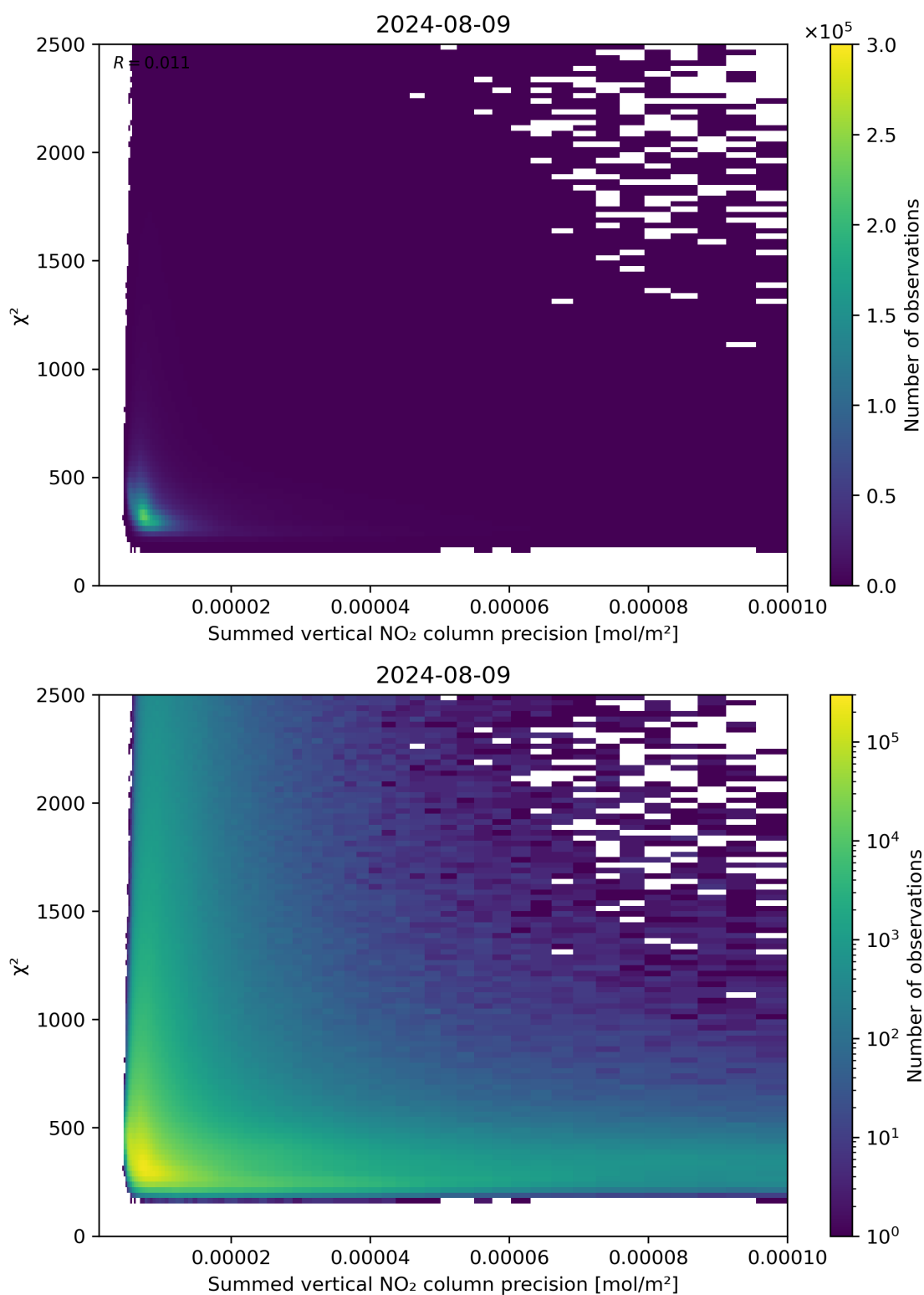
Figure 107: Scatter density plot of “Summed vertical NO 2 column precision” against “ \chi^2 ” for 2024-08-08 to 2024-08-10.
