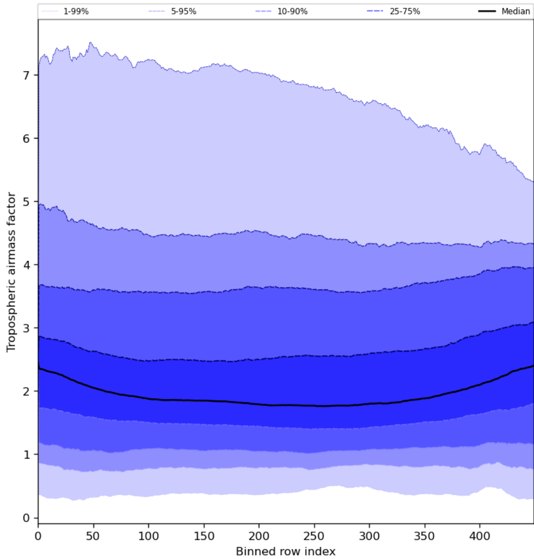
Figure 48: Along track statistics of “Tropospheric air mass factor” for 2024-08-08 to 2024-08-10
