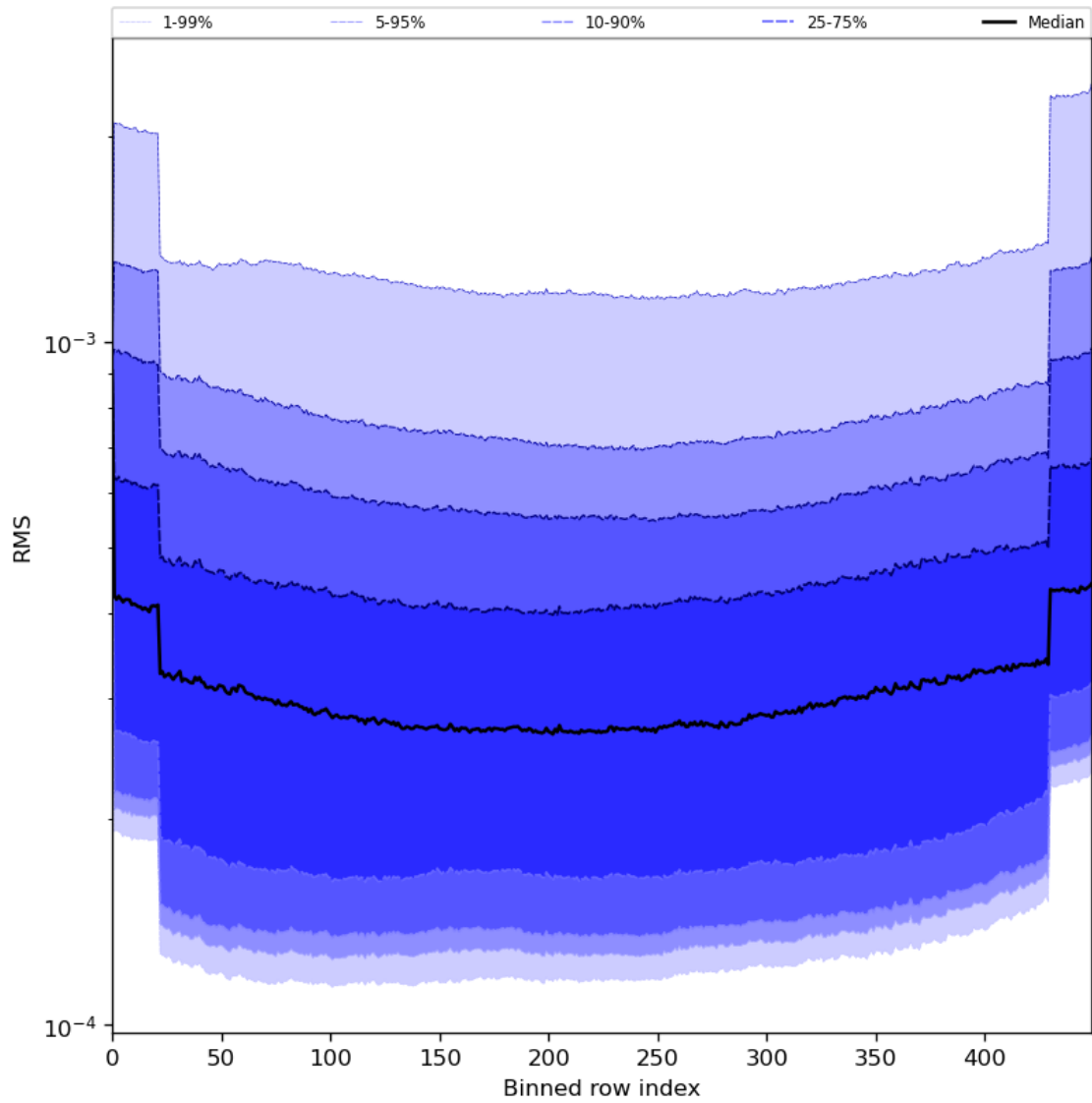
Figure 60: Along track statistics of “RMS” for 2024-08-08 to 2024-08-10
