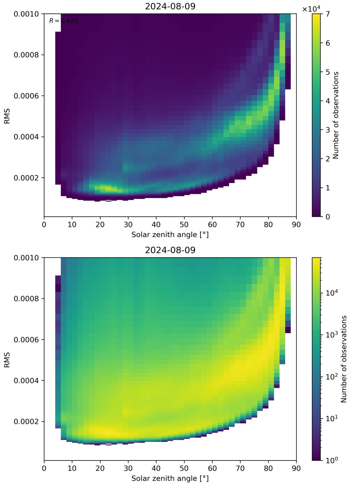
Figure 157: Scatter density plot of “Solar zenith angle” against “RMS” for 2024-08-08 to 2024-08-10.
