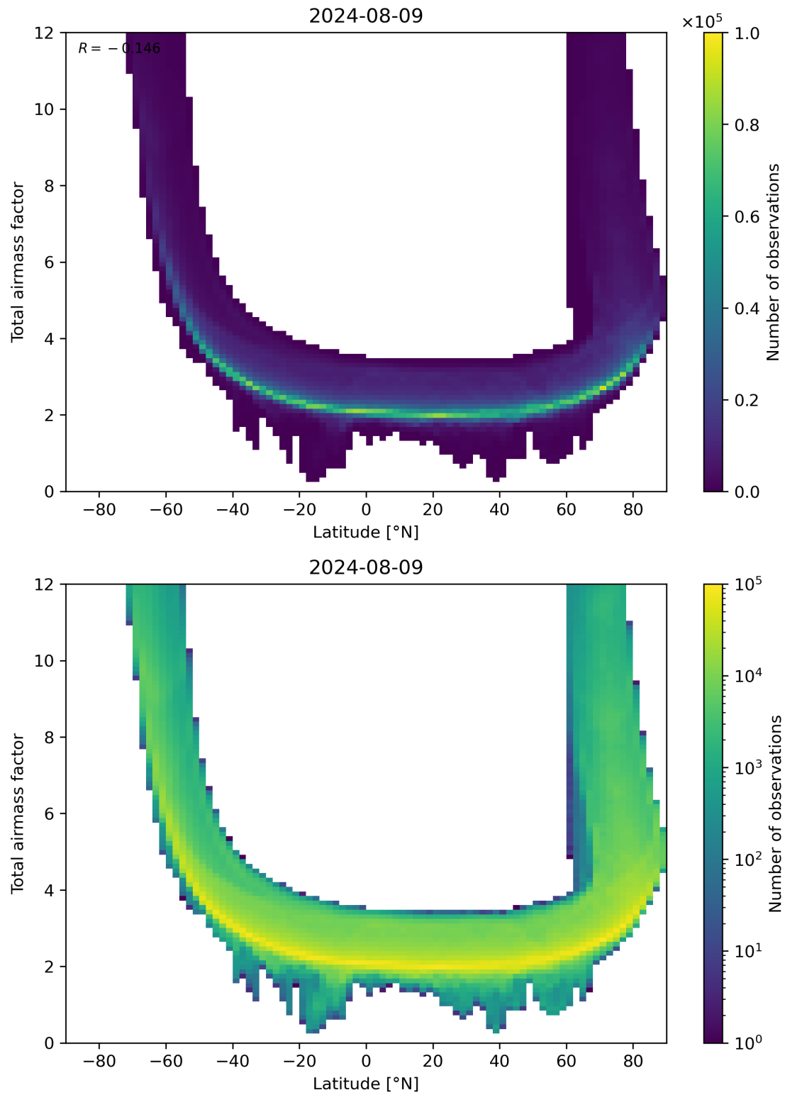
Figure 84: Scatter density plot of “Latitude” against “Total airmass factor” for 2024-08-08 to 2024-08-10.
