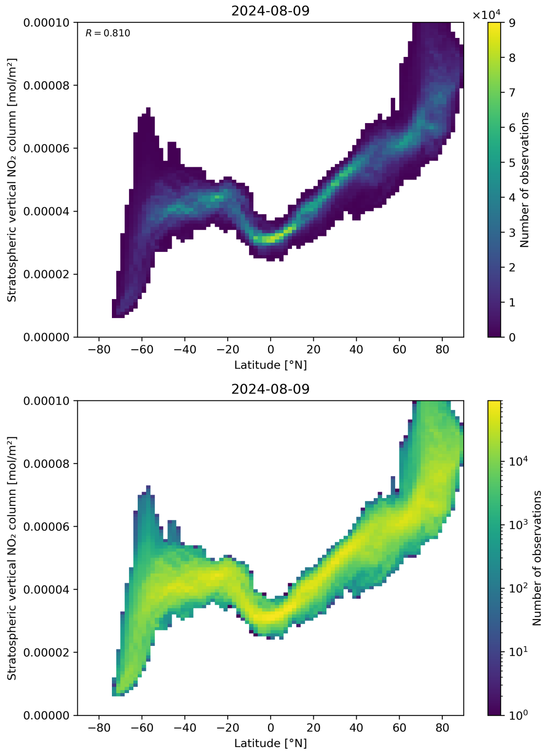
Figure 87: Scatter density plot of “Latitude” against “Stratospheric vertical \text{NO}_2 column” for 2024-08-08 to 2024-08-10.
