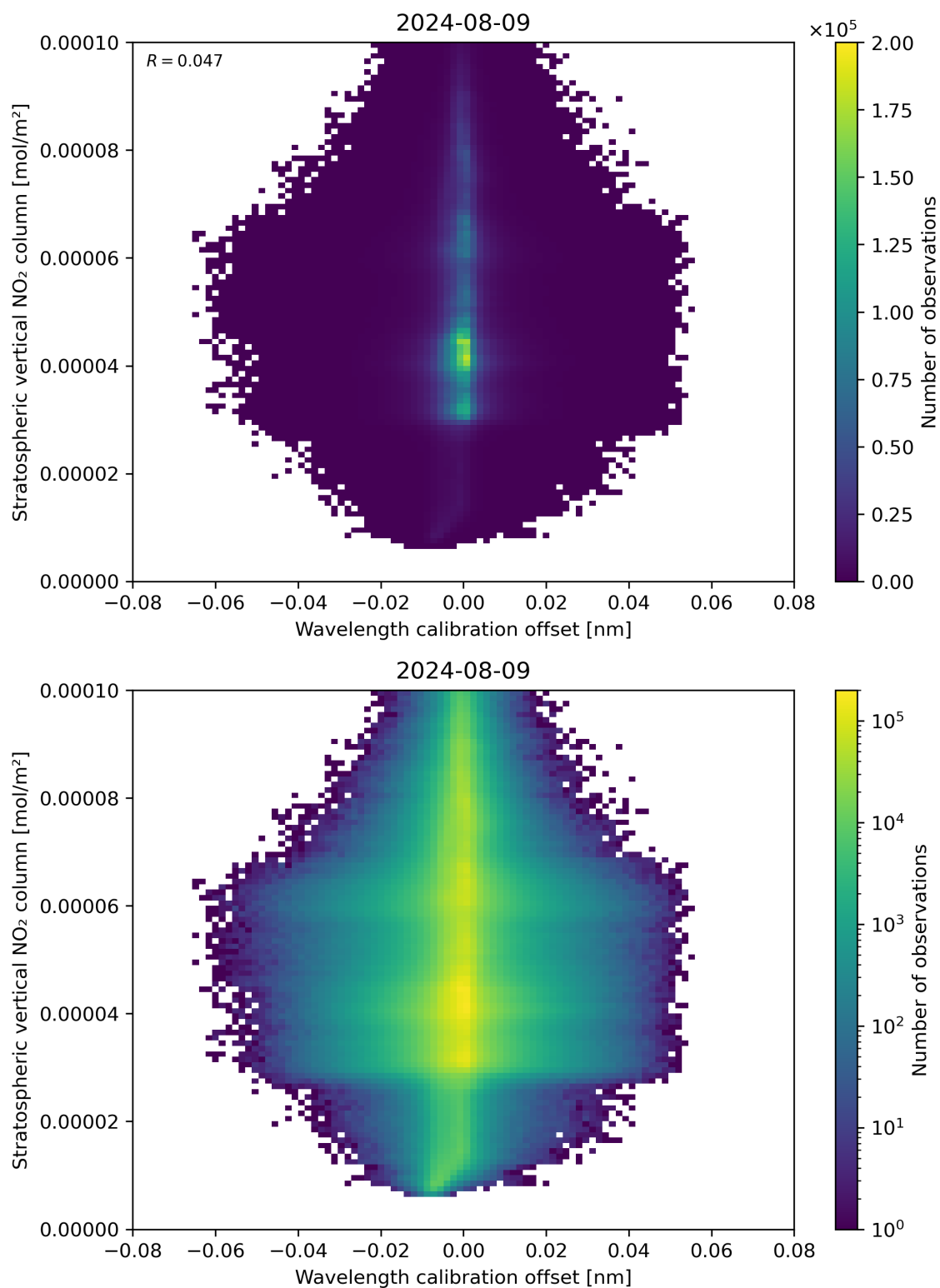
Figure 176: Scatter density plot of “Wavelength calibration offset” against “Stratospheric vertical NO 2 column” for 2024-08-08 to 2024-08-10.
