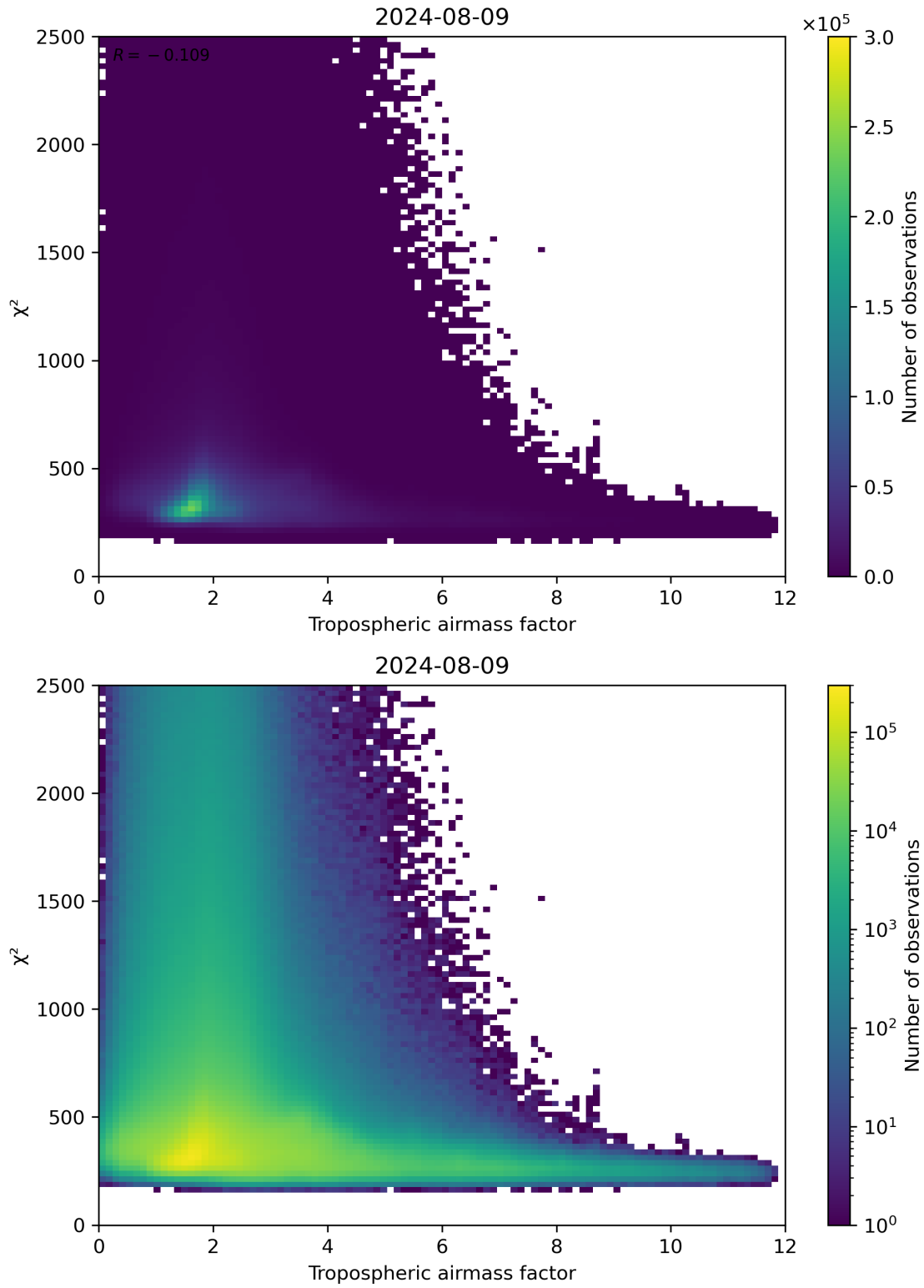
Figure 73: Scatter density plot of “Tropospheric airmass factor” against “ \chi^2 ” for 2024-08-08 to 2024-08-10.
