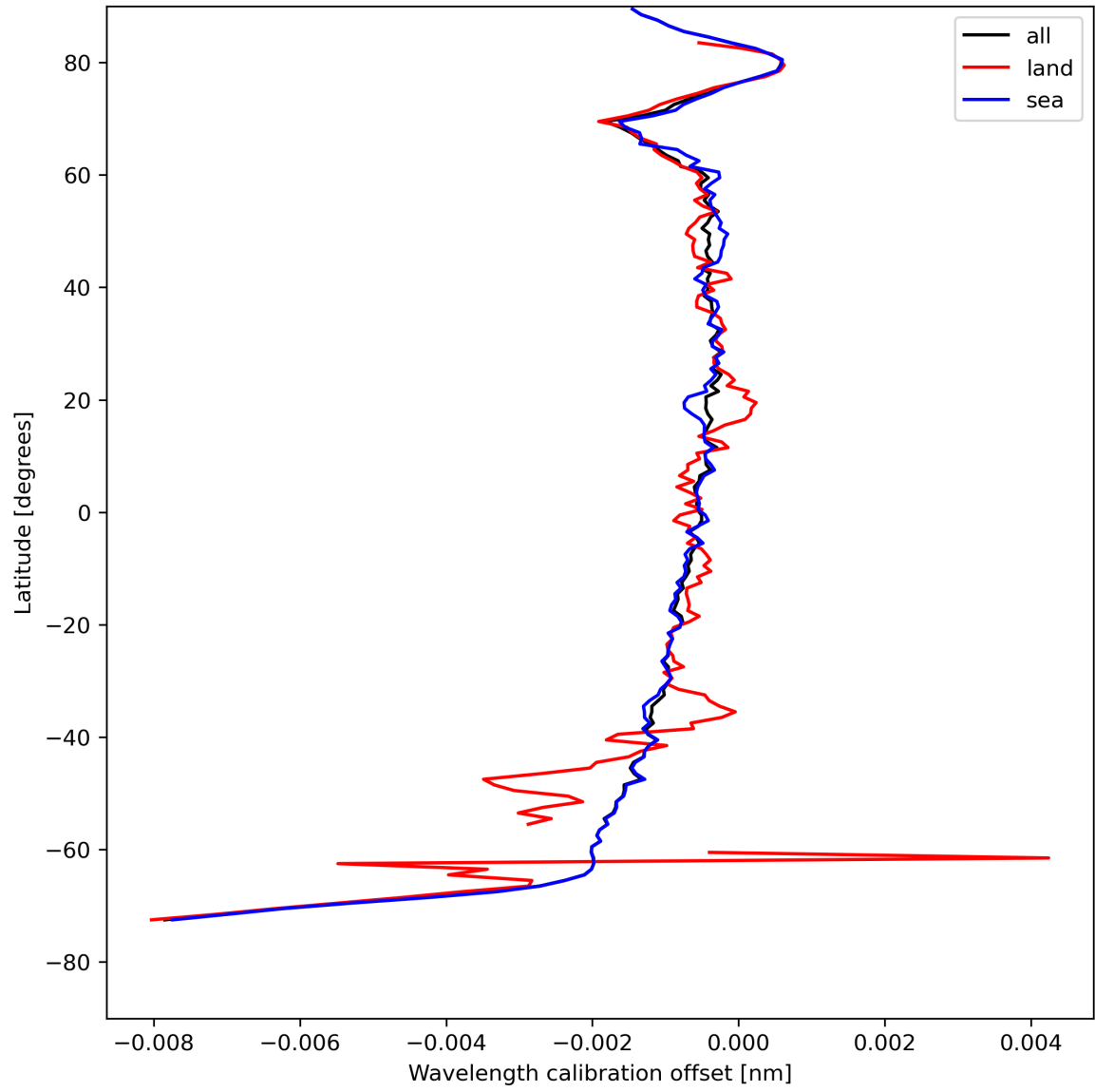
Figure 18: Zonal average of “Wavelength calibration offset” for 2024-08-08 to 2024-08-10.
