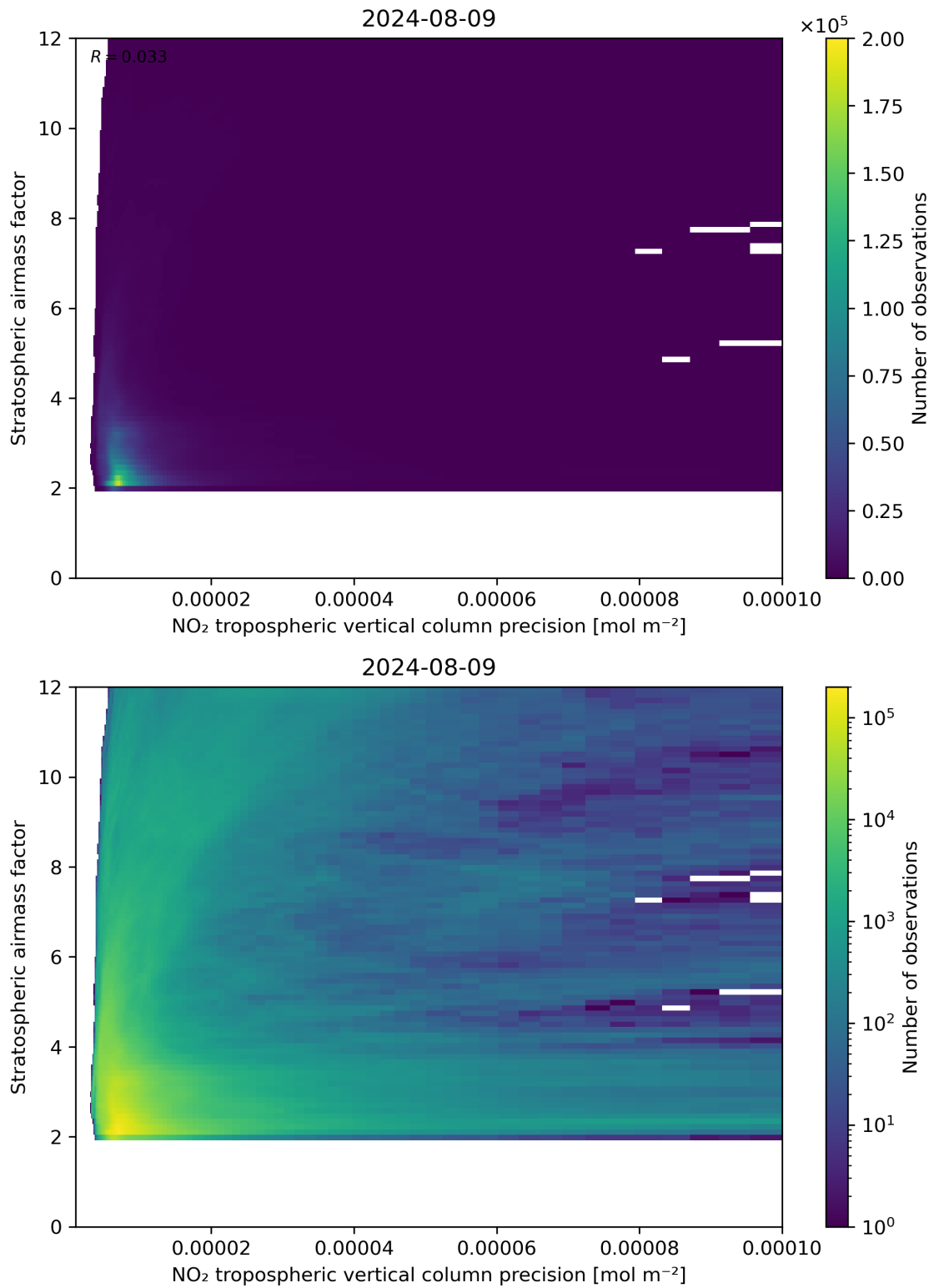
Figure 131: Scatter density plot of “NO 2 tropospheric vertical column precision” against “Stratospheric airmass factor” for 2024-08-08 to 2024-08-10.
