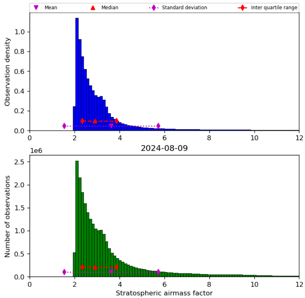
Figure 44: Histogram of “Stratospheric airmass factor” for 2024-08-08 to 2024-08-10
