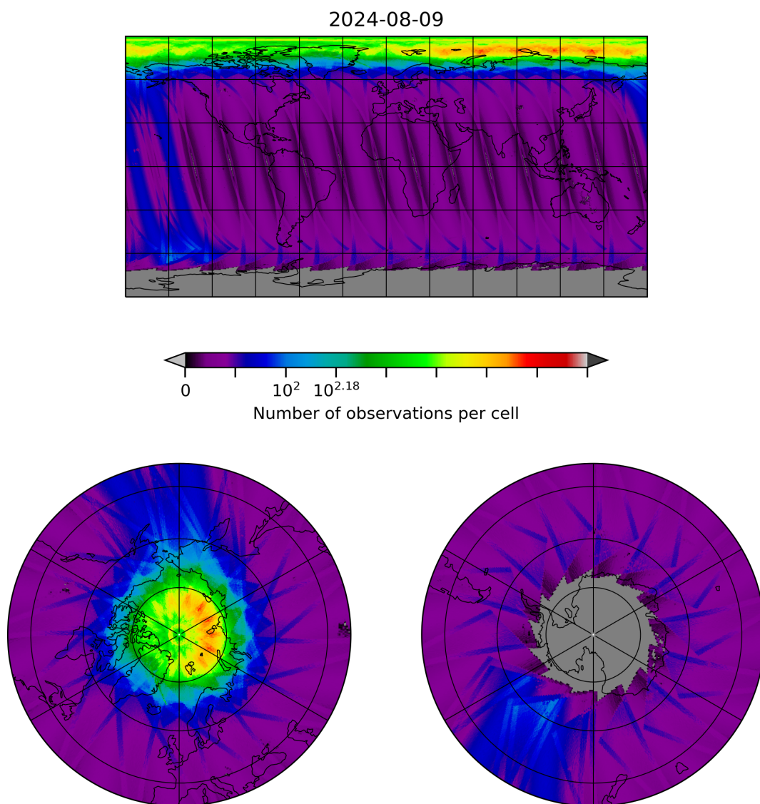
Figure 10: Map of the number of observations for 2024-08-08 to 2024-08-10
