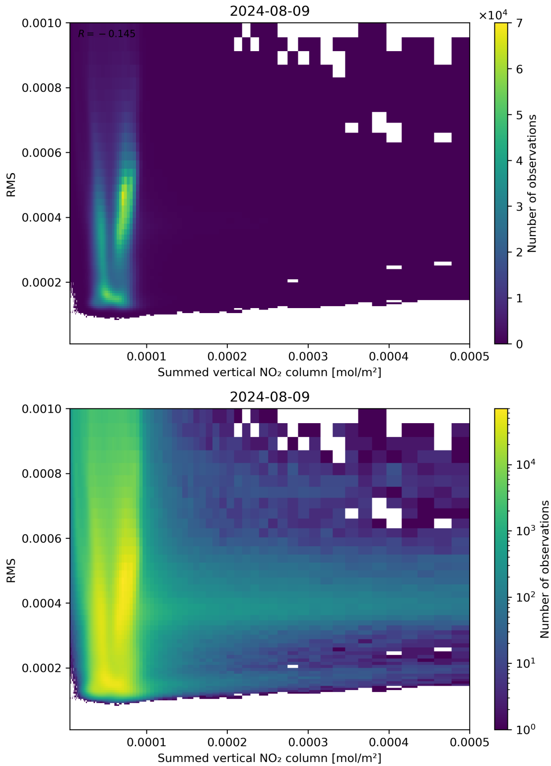
Figure 109: Scatter density plot of “Summed vertical NO 2 column” against “RMS” for 2024-08-08 to 2024-08-10.
