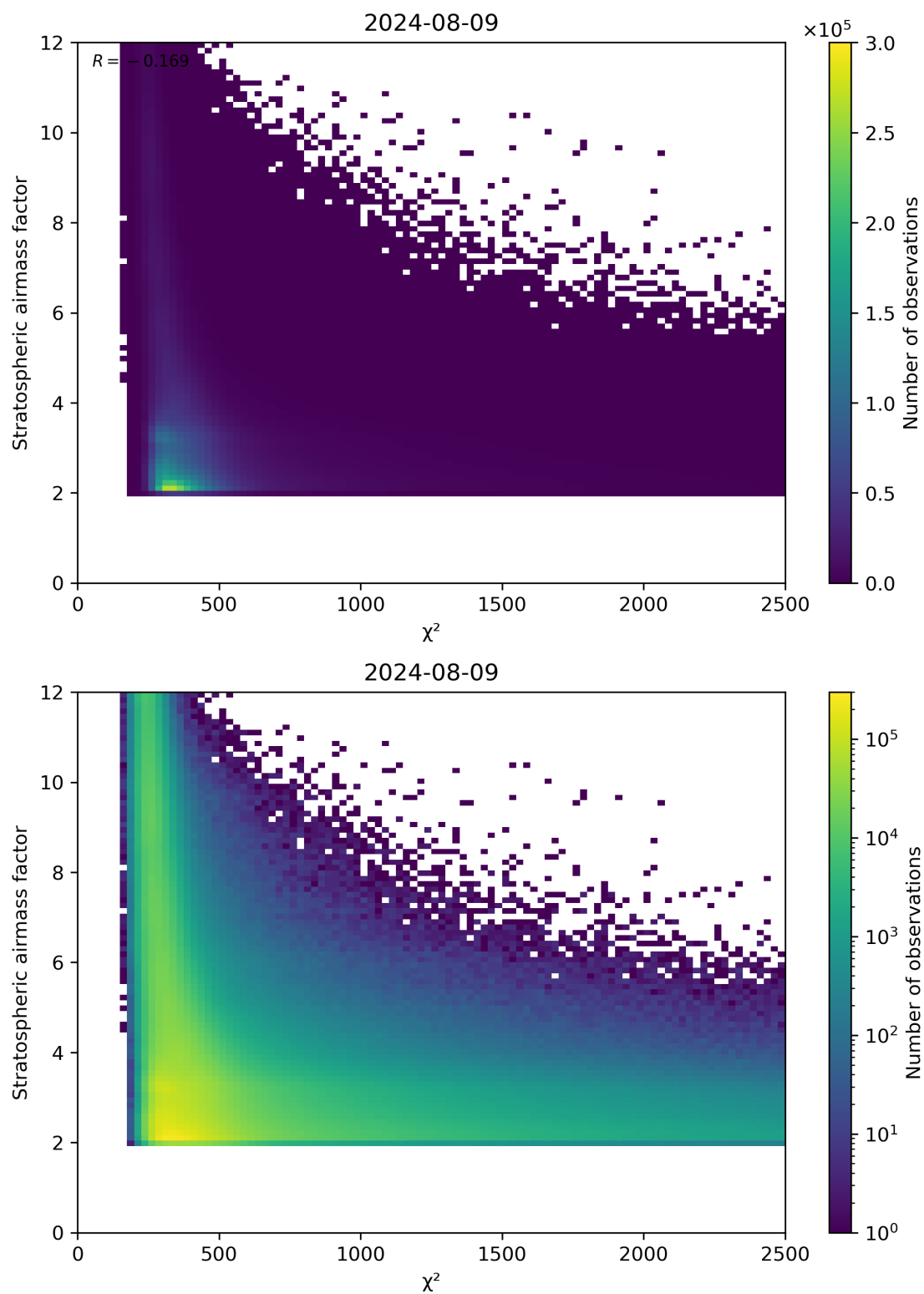
Figure 81: Scatter density plot of “ \chi^2 ” against “Stratospheric airmass factor” for 2024-08-08 to 2024-08-10.
