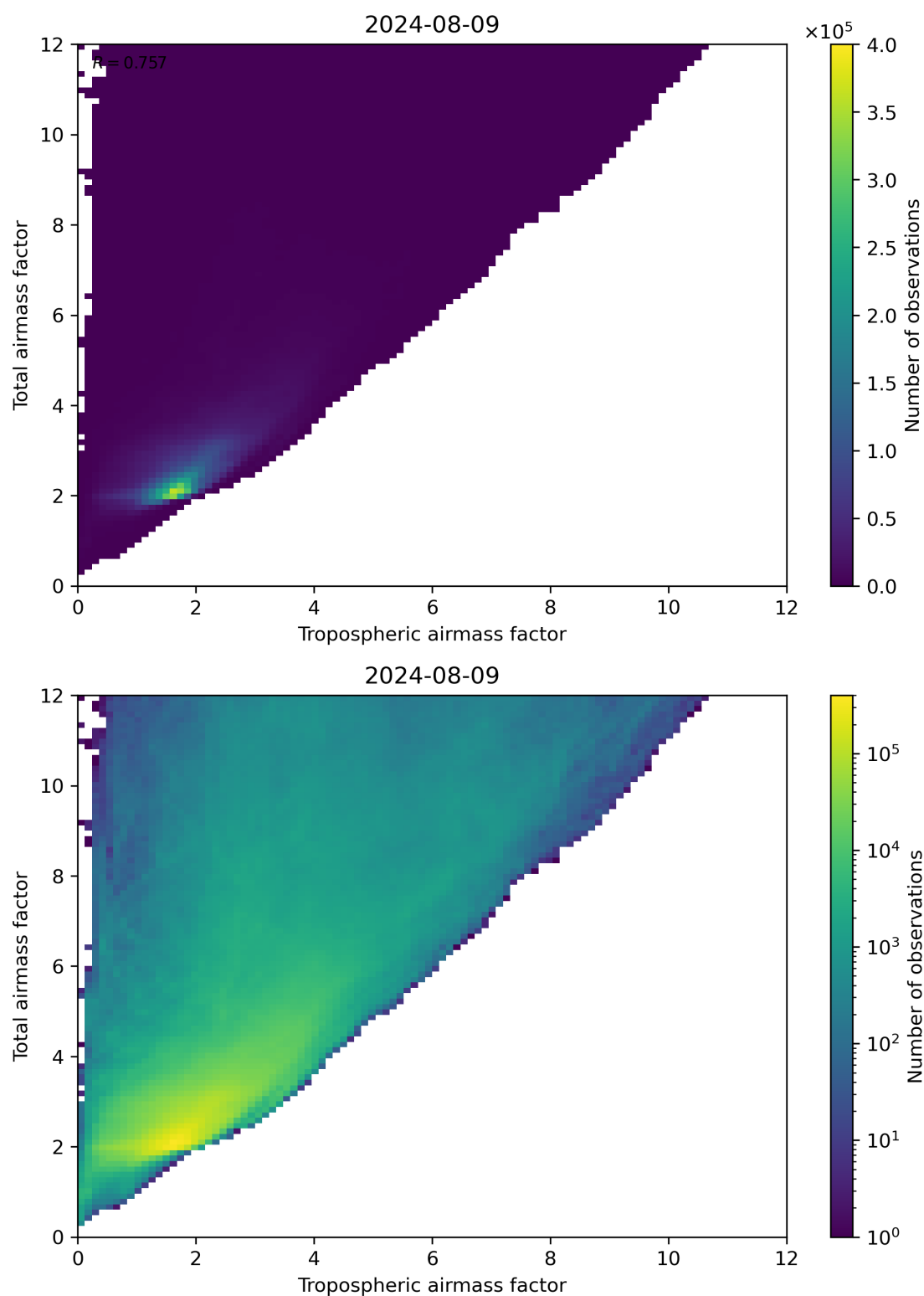
Figure 72: Scatter density plot of “Tropospheric airmass factor” against “Total airmass factor” for 2024-08-08 to 2024-08-10.
