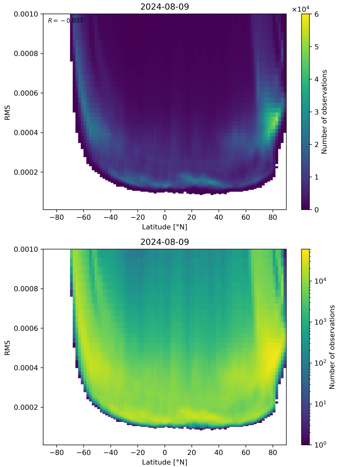
Figure 94: Scatter density plot of “Latitude” against “RMS” for 2024-08-08 to 2024-08-10.
