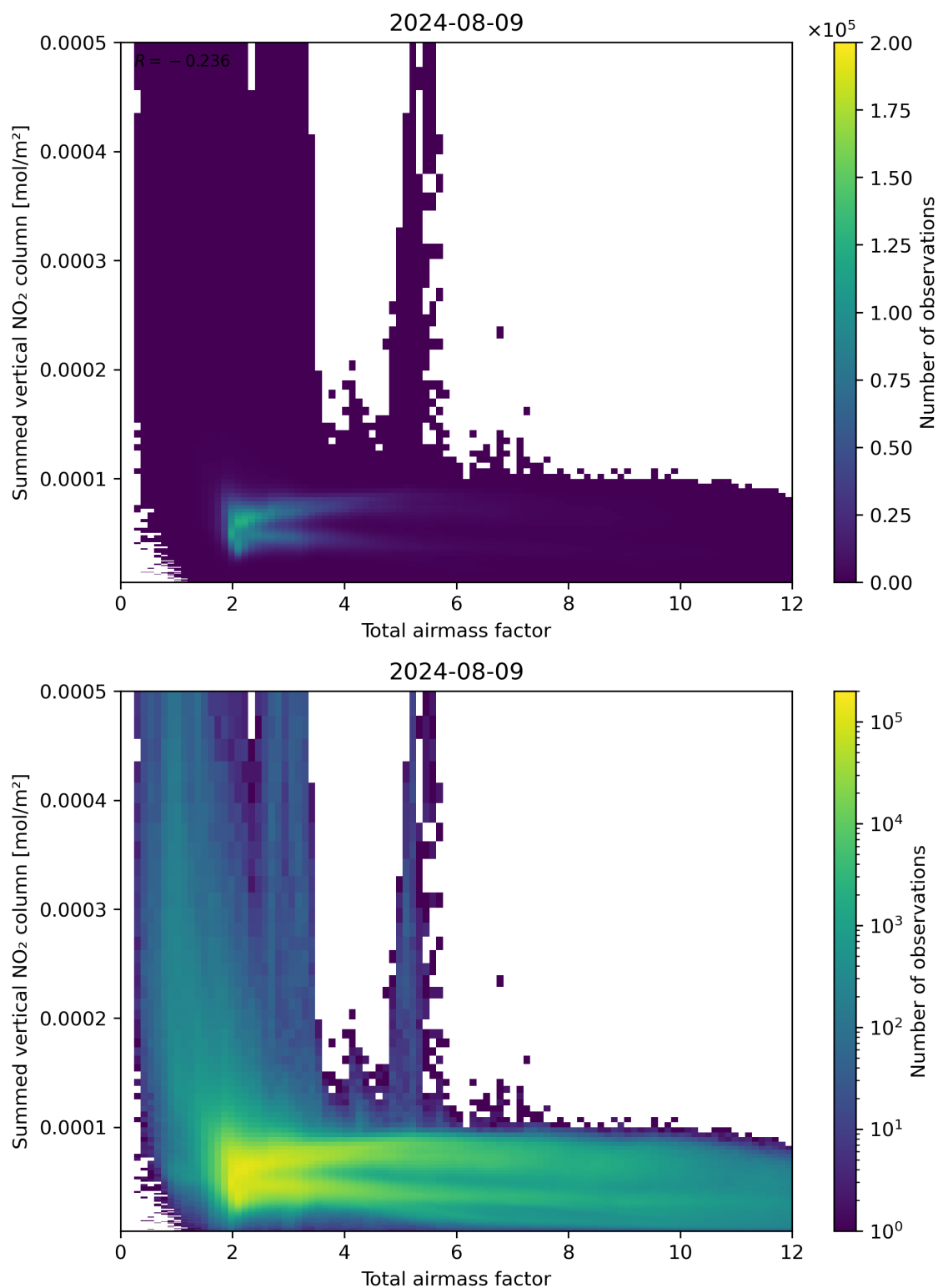
Figure 65: Scatter density plot of “Total airmass factor” against “Summed vertical NO 2 column” for 2024-08-08 to 2024-08-10.
