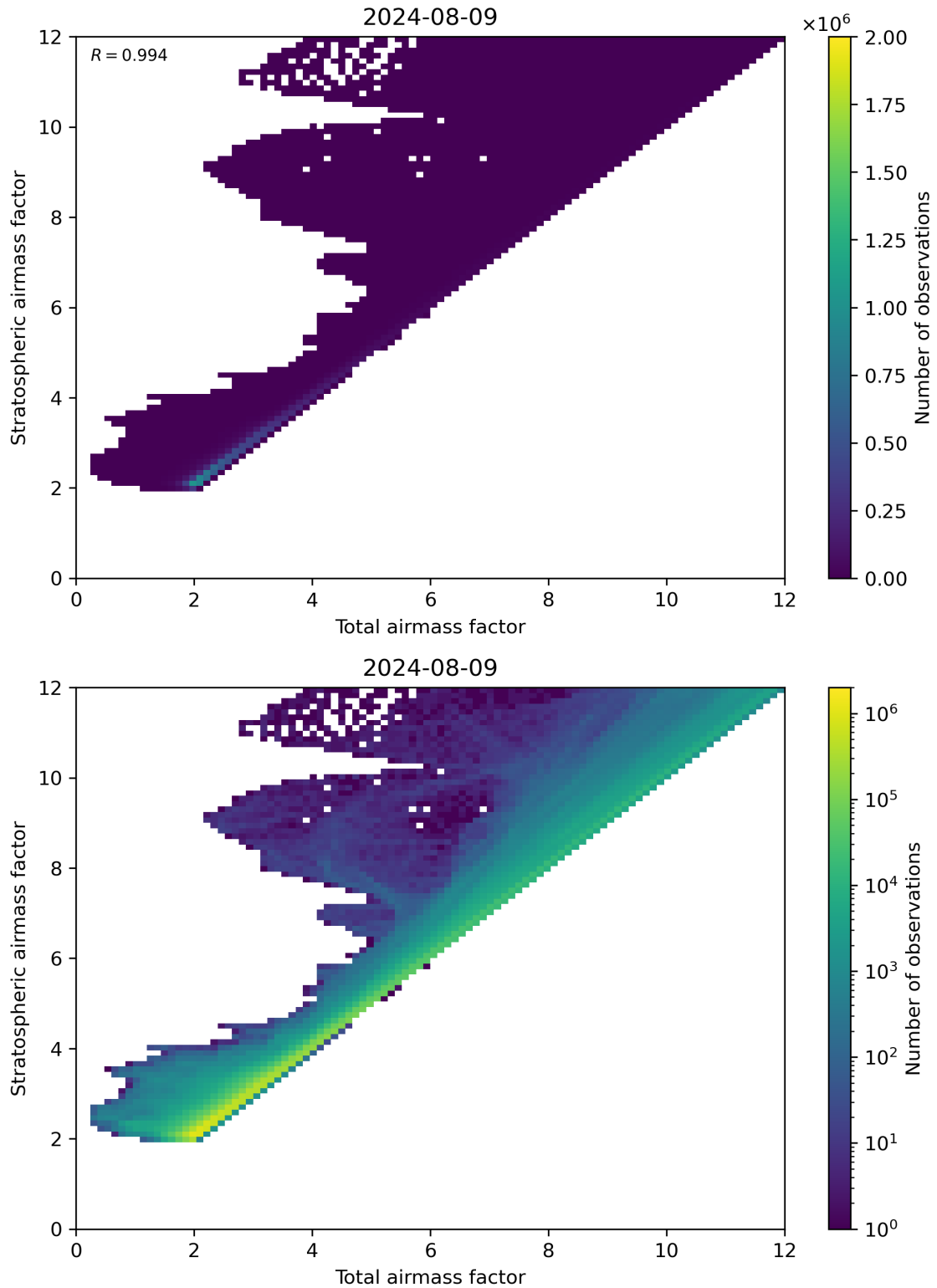
Figure 62: Scatter density plot of “Total airmass factor” against “Stratospheric airmass factor” for 2024-08-08 to 2024-08-10.
