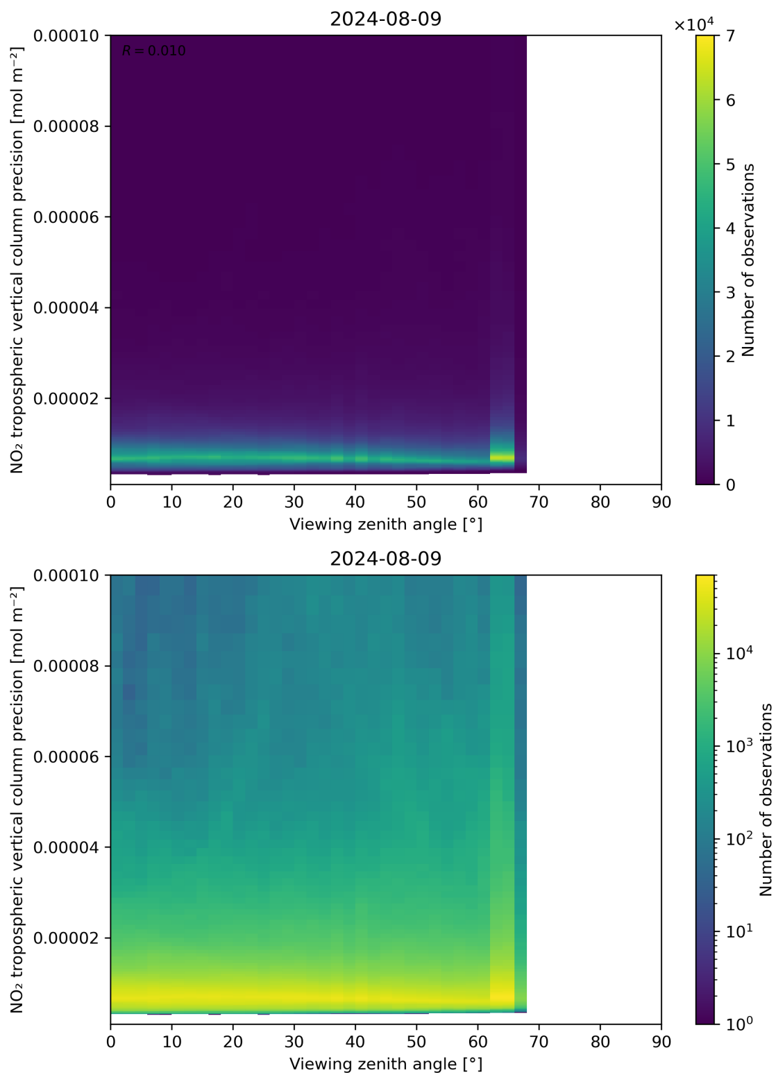
Figure 170: Scatter density plot of “Viewing zenith angle” against “NO 2 tropospheric vertical column precision” for 2024-08-08 to 2024-08-10.
