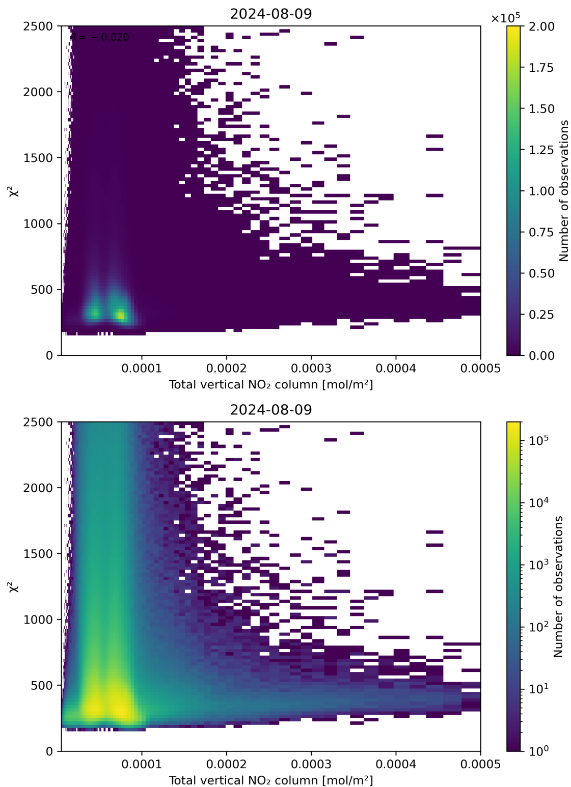
Figure 111: Scatter density plot of “Total vertical NO 2 column” against “ \chi^2 ” for 2024-08-08 to 2024-08-10.
