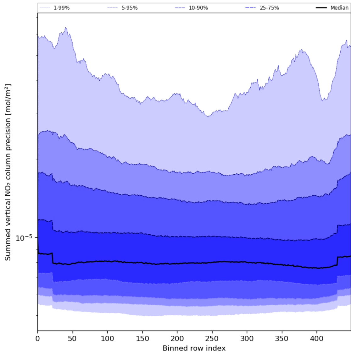
Figure 58: Along track statistics of “Summed vertical NO 2 column precision” for 2024-08-08 to 2024-08-10
