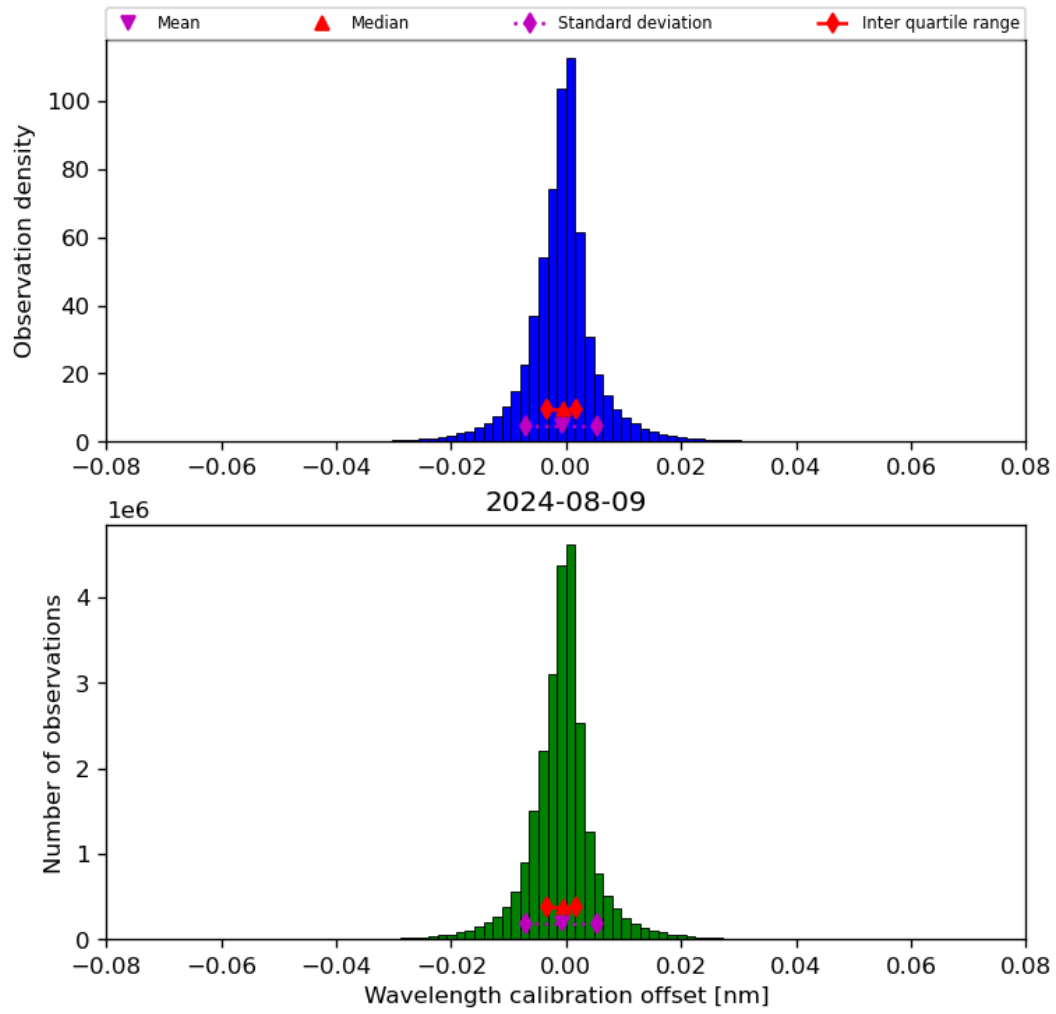
Figure 35: Histogram of “Wavelength calibration offset” for 2024-08-08 to 2024-08-10
