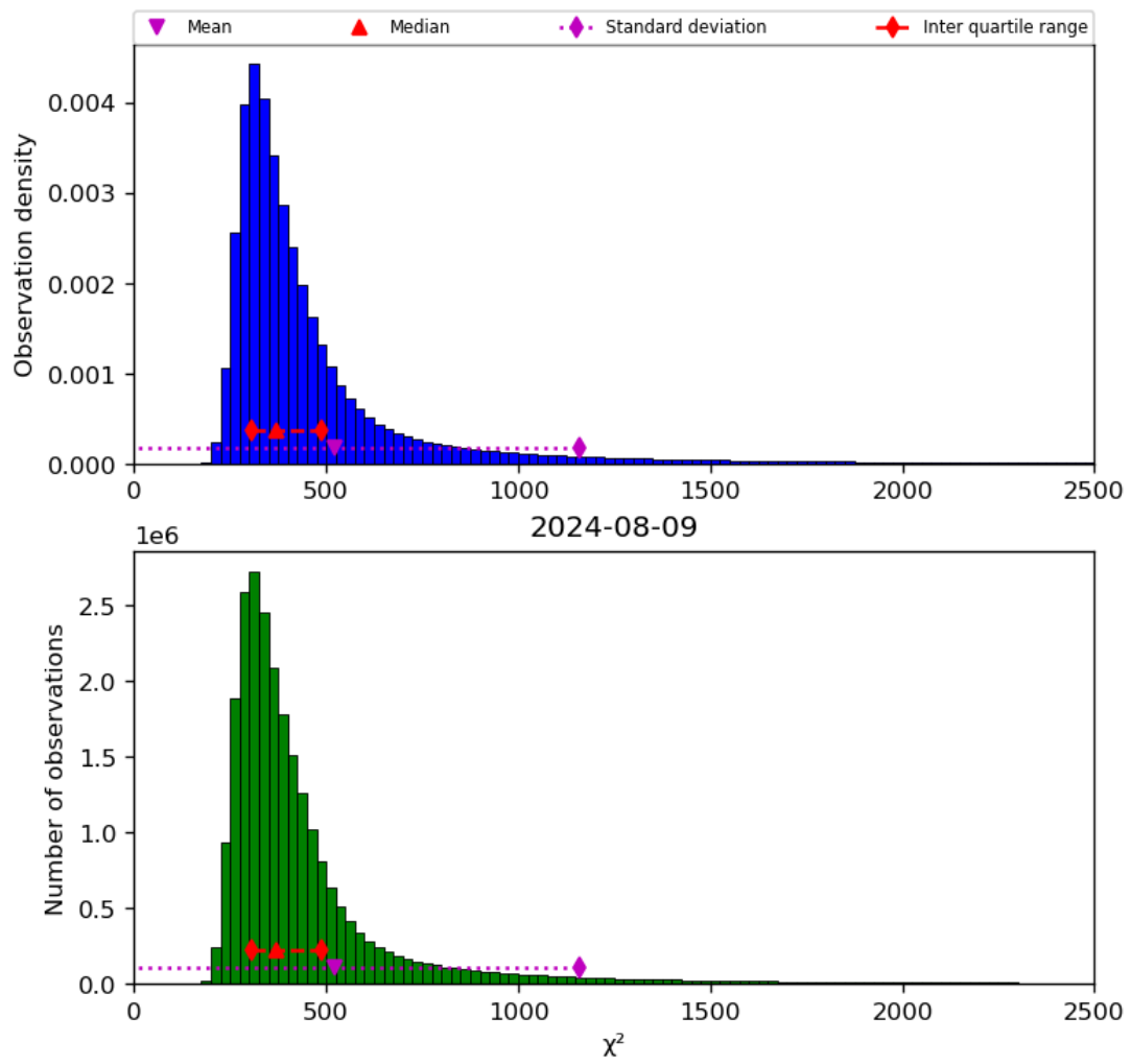
Figure 42: Histogram of “ \chi^2 ” for 2024-08-08 to 2024-08-10
