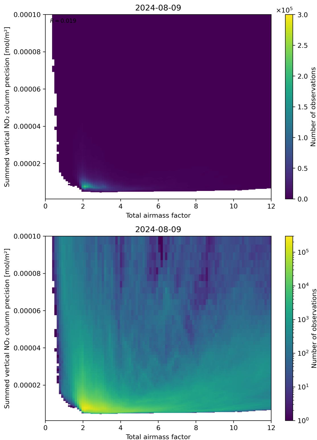
Figure 66: Scatter density plot of “Total airmass factor” against “Summed vertical NO 2 column precision” for 2024-08-08 to 2024-08-10.
