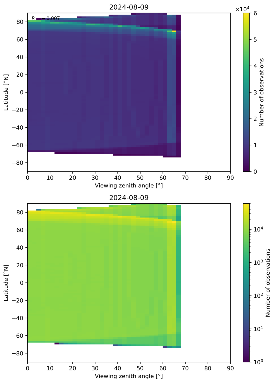
Figure 163: Scatter density plot of “Viewing zenith angle” against “Latitude” for 2024-08-08 to 2024-08-10.
