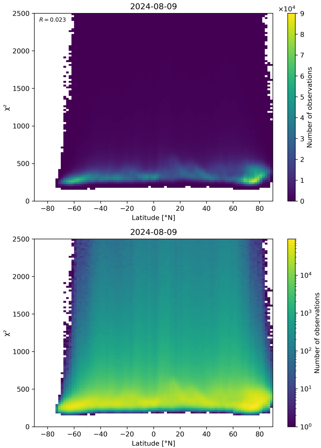
Figure 86: Scatter density plot of “Latitude” against “ \chi^2 ” for 2024-08-08 to 2024-08-10.
