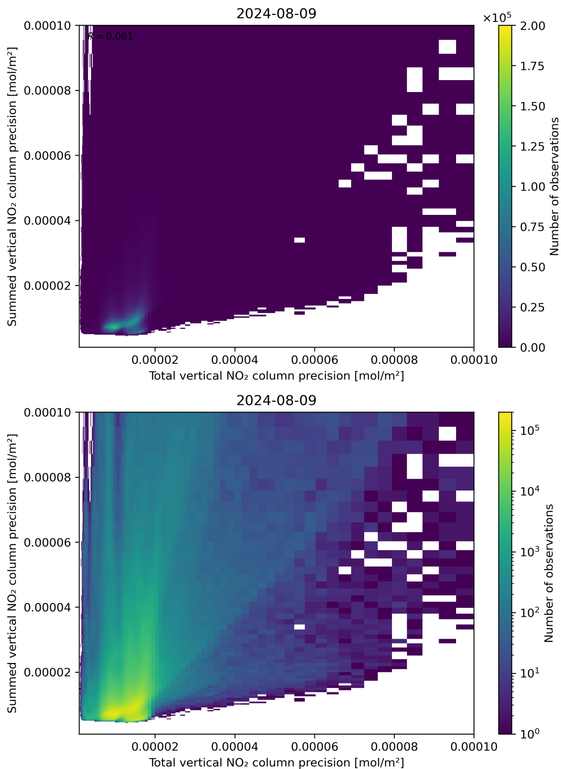
Figure 118: Scatter density plot of “Total vertical NO 2 column precision” against “Summed vertical NO 2 column precision” for 2024-08-08 to 2024-08-10.
