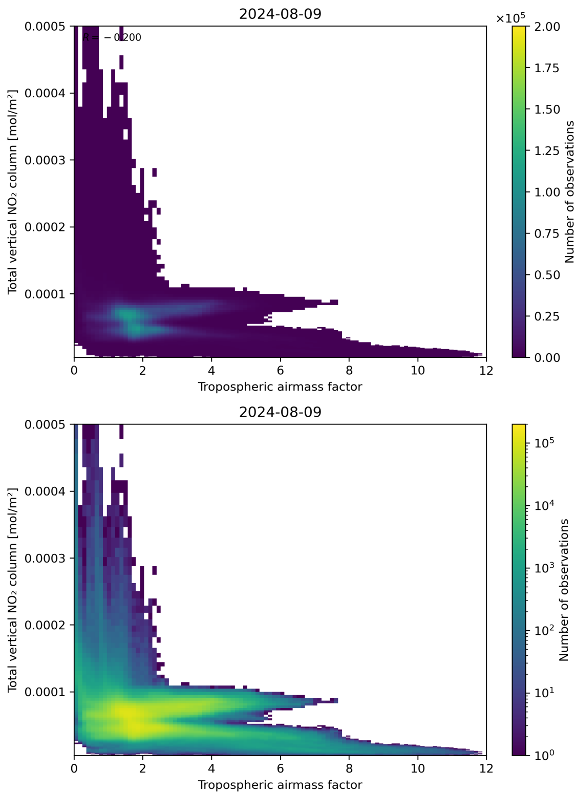
Figure 77: Scatter density plot of “Tropospheric airmass factor” against “Total vertical NO 2 column” for 2024-08-08 to 2024-08-10.
