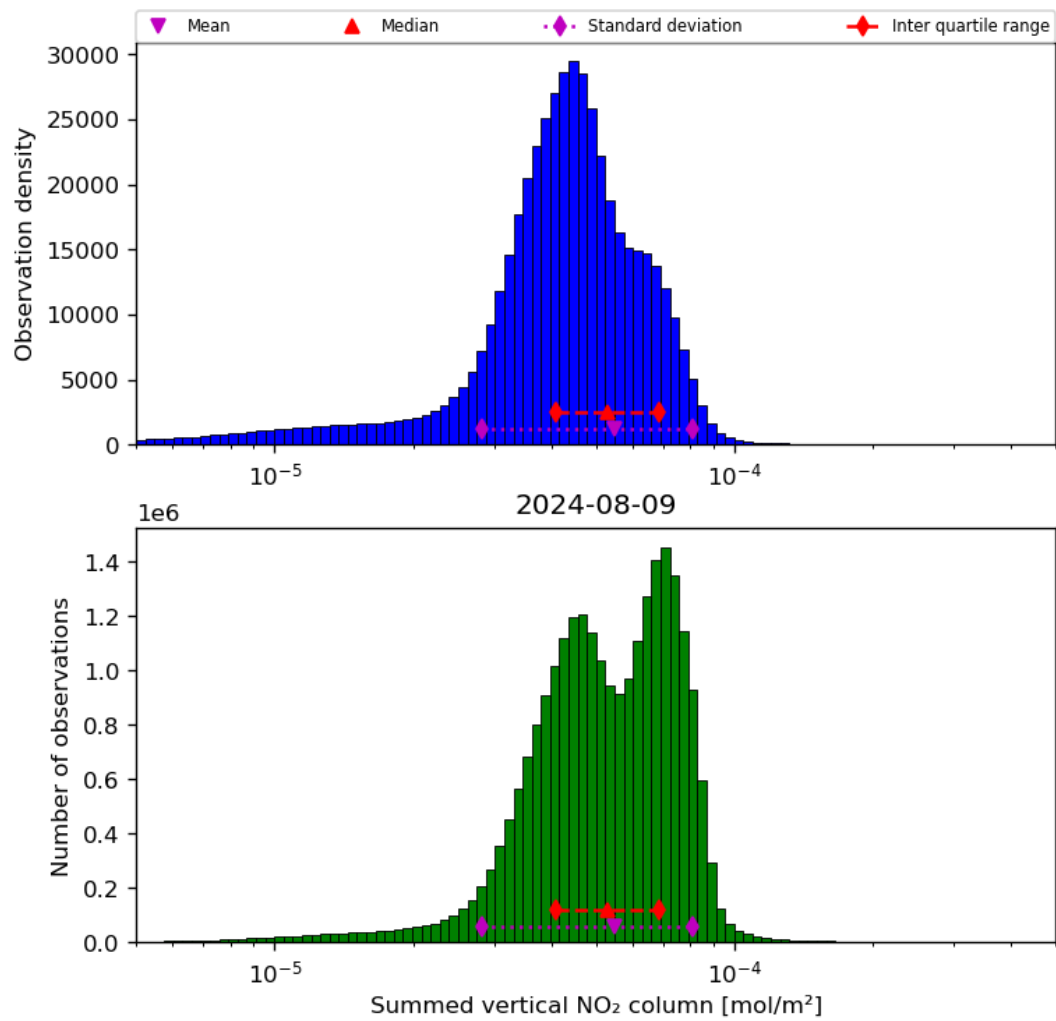
Figure 40: Histogram of “Summed vertical NO 2 column” for 2024-08-08 to 2024-08-10
