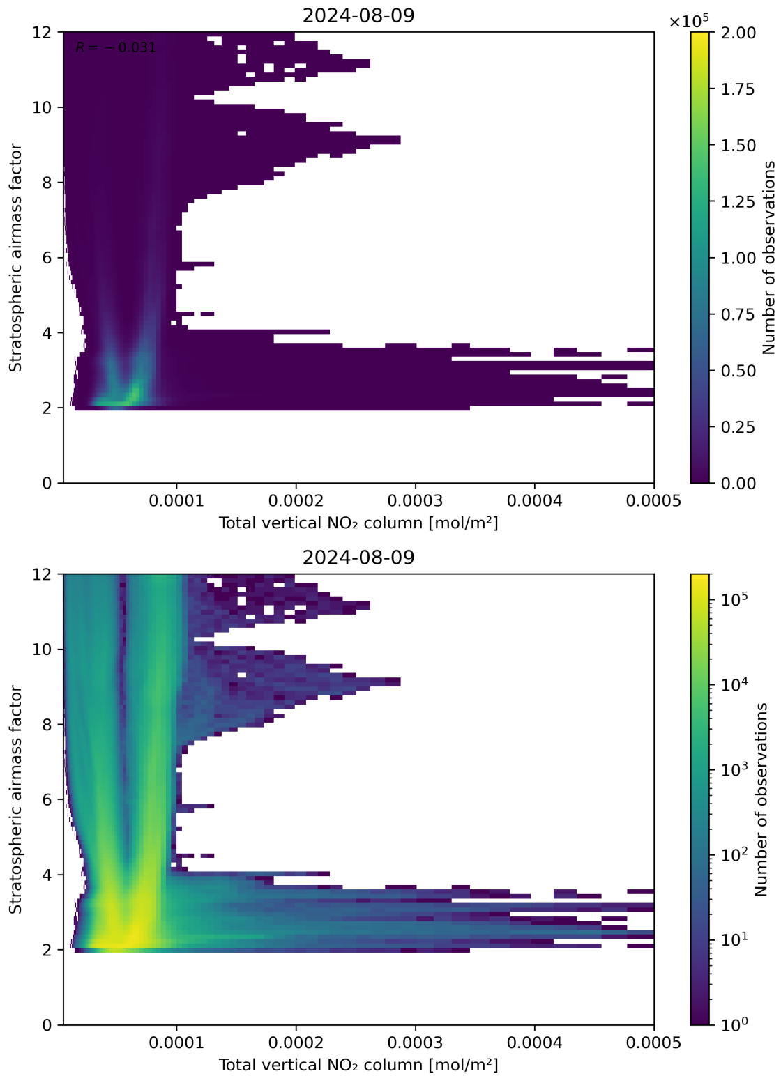
Figure 110: Scatter density plot of “Total vertical NO 2 column” against “Stratospheric airmass factor” for 2024-08-08 to 2024-08-10.
