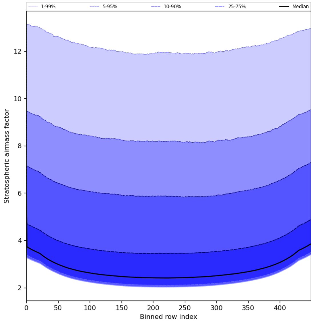
Figure 61: Along track statistics of “Stratospheric airmass factor” for 2024-08-08 to 2024-08-10
