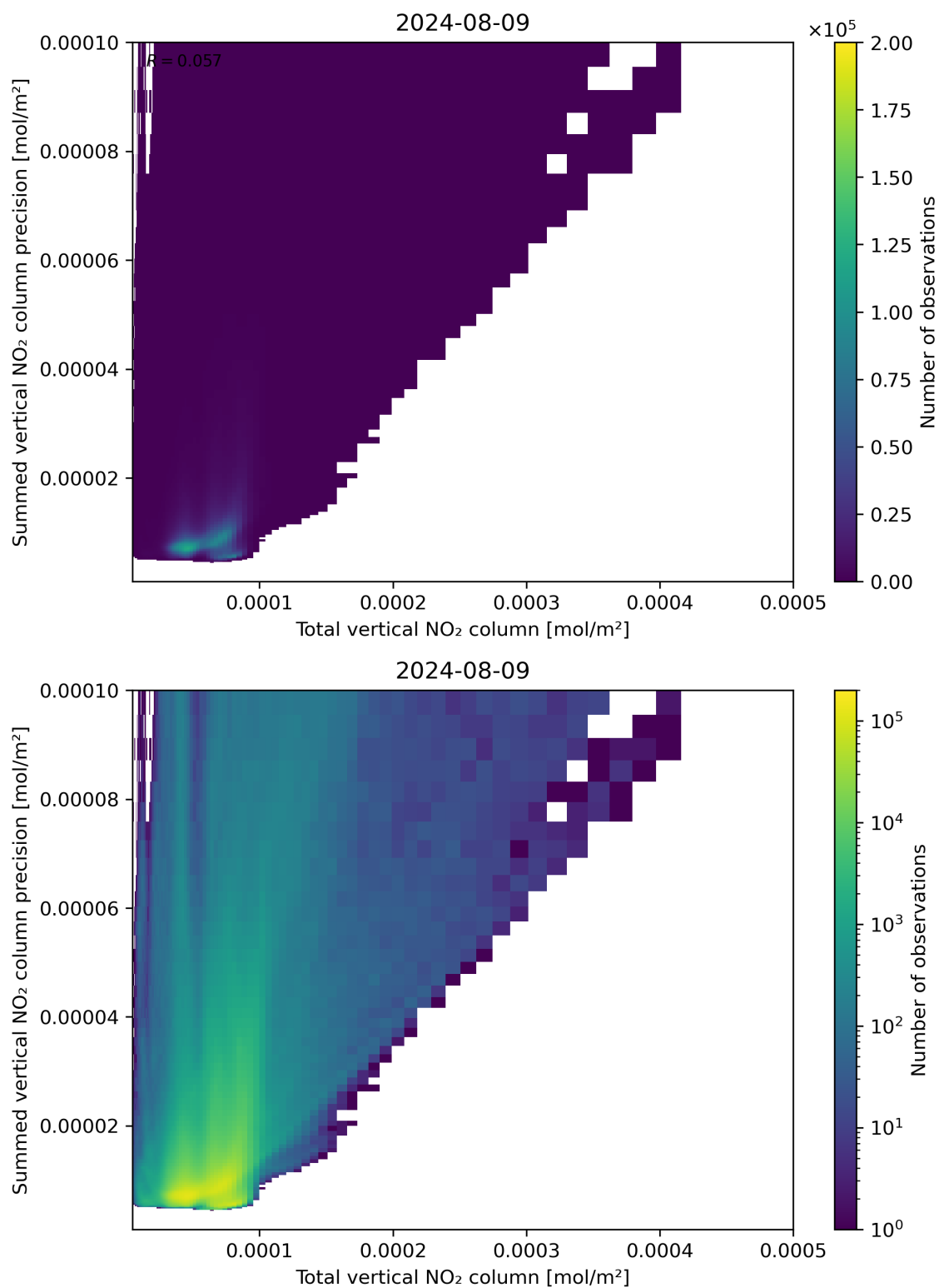
Figure 113: Scatter density plot of “Total vertical NO 2 column” against “Summed vertical NO 2 column precision” for 2024-08-08 to 2024-08-10.
