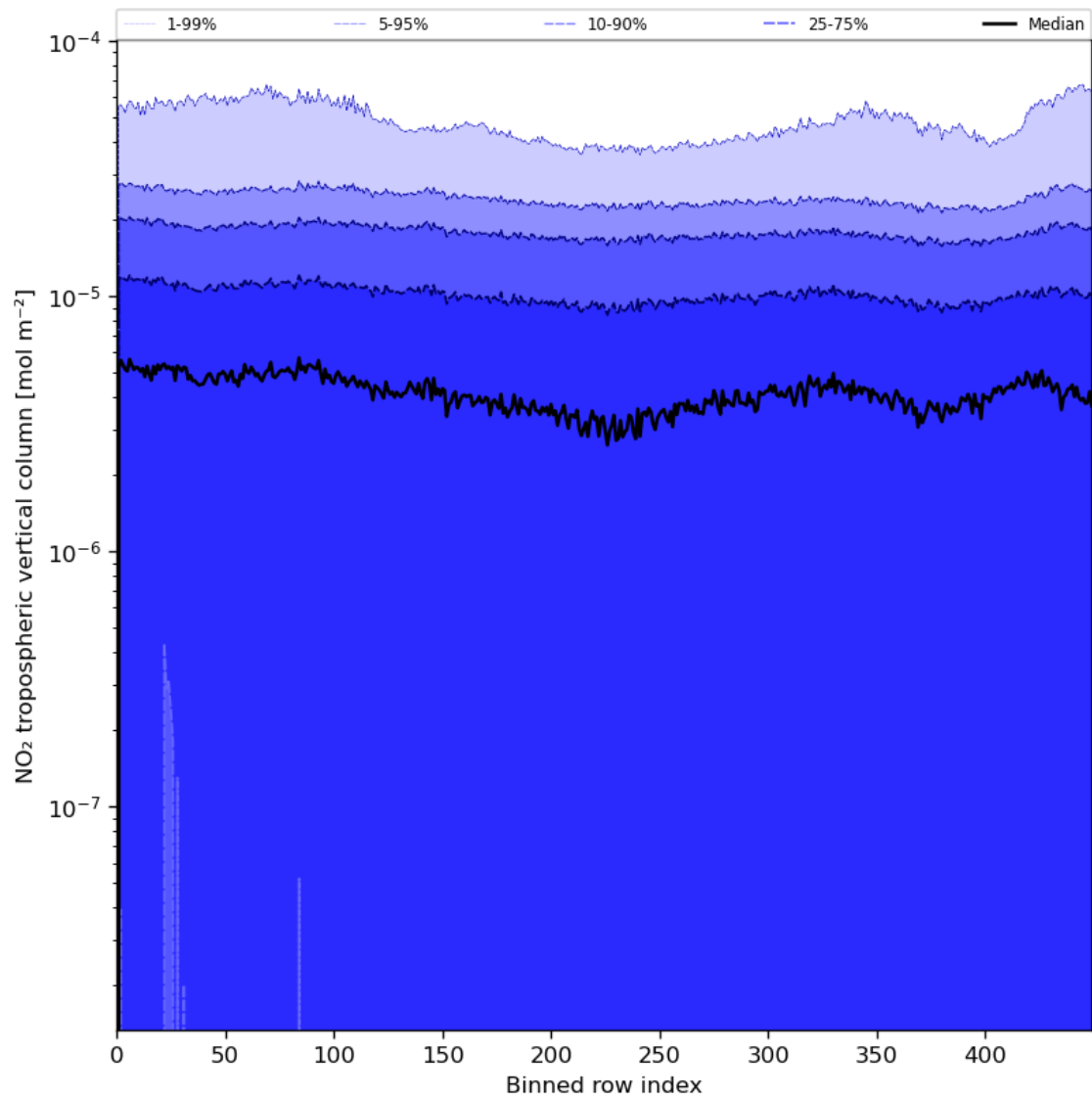
Figure 46: Along track statistics of “NO 2 tropospheric vertical column” for 2024-08-08 to 2024-08-10
