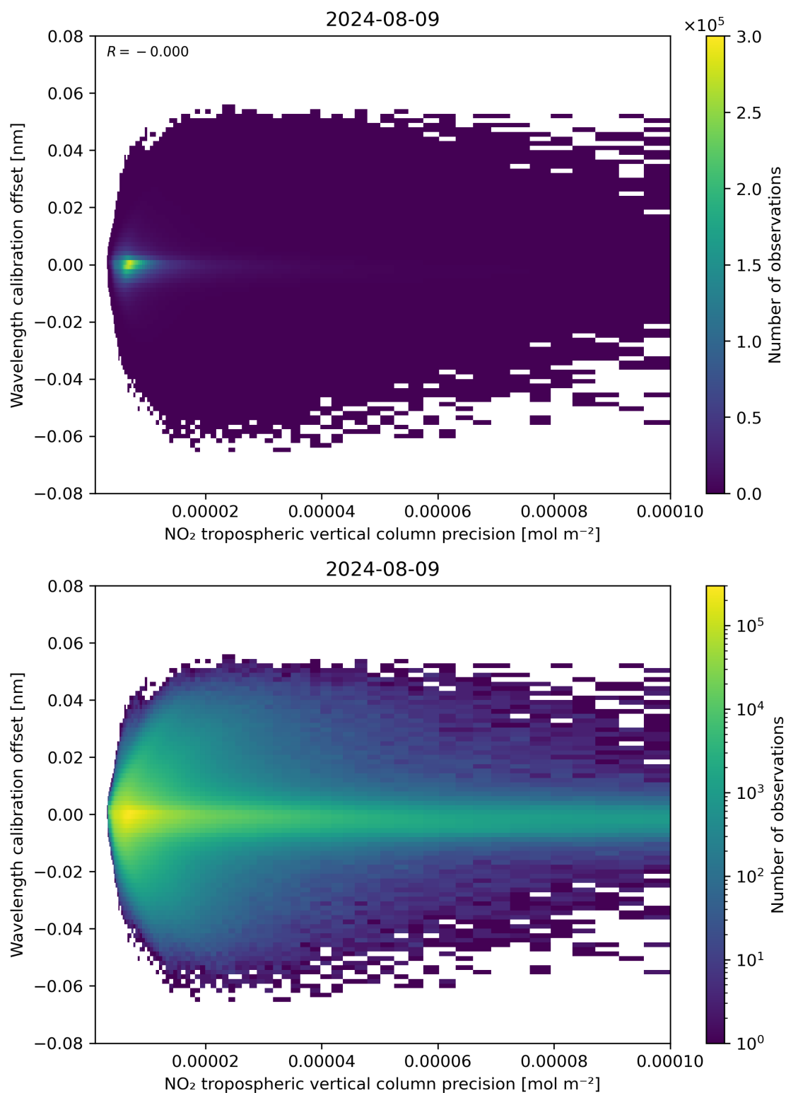
Figure 141: Scatter density plot of “NO 2 tropospheric vertical column precision” against “Wavelength calibration offset” for 2024-08-08 to 2024-08-10.
