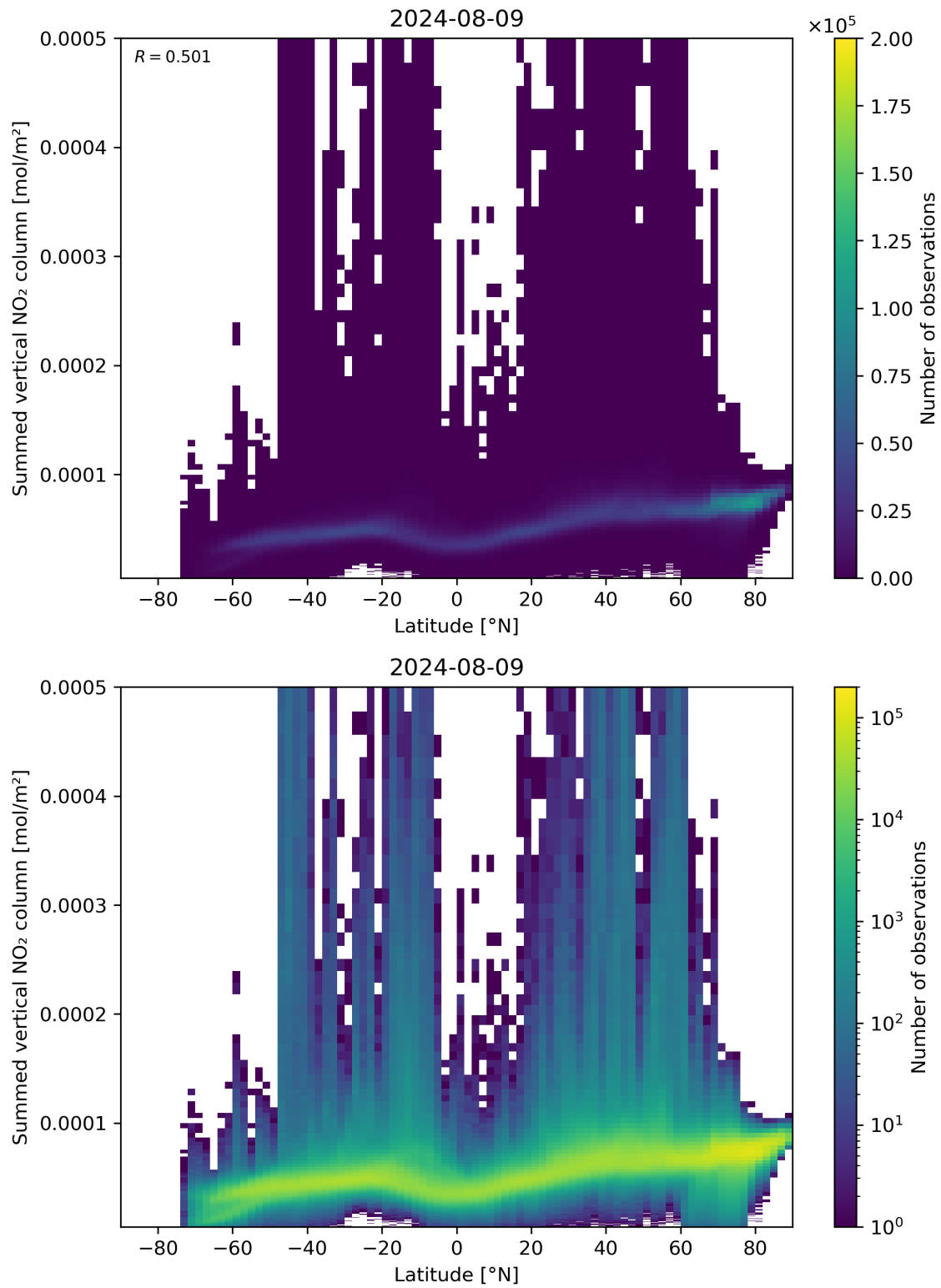
Figure 88: Scatter density plot of “Latitude” against “Summed vertical NO 2 column” for 2024-08-08 to 2024-08-10.
