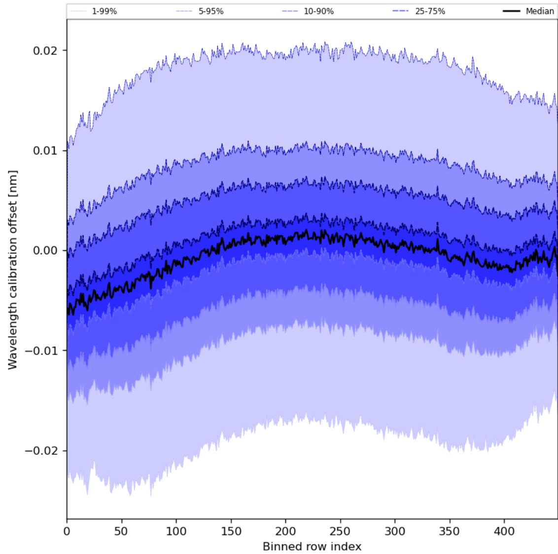
Figure 52: Along track statistics of “Wavelength calibration offset” for 2024-08-08 to 2024-08-10
