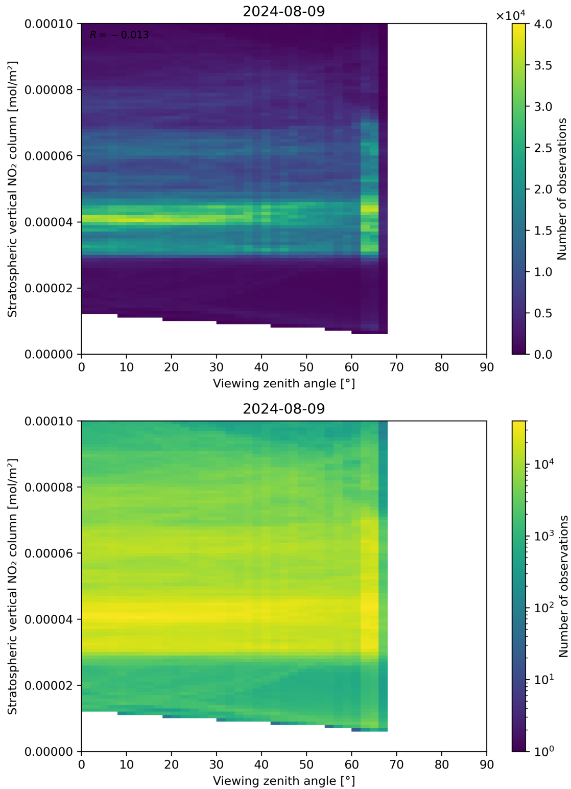
Figure 164: Scatter density plot of “Viewing zenith angle” against “Stratospheric vertical NO 2 column” for 2024-08-08 to 2024-08-10.
