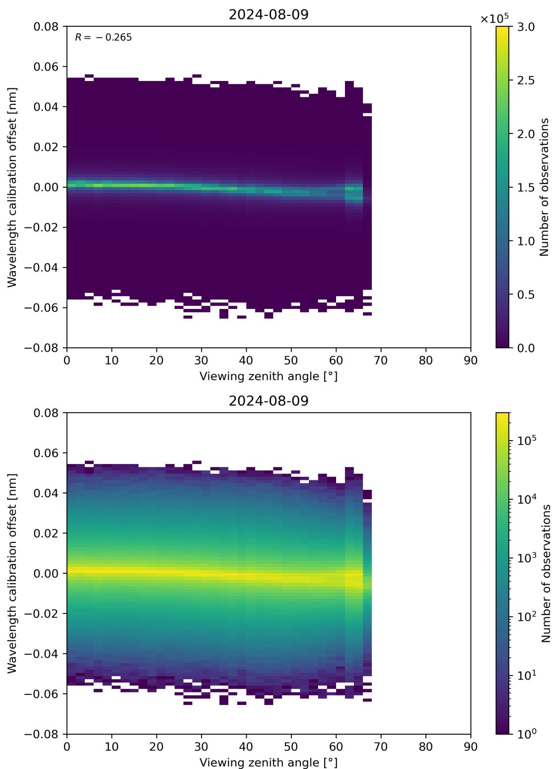
Figure 173: Scatter density plot of “Viewing zenith angle” against “Wavelength calibration offset” for 2024-08-08 to 2024-08-10.
