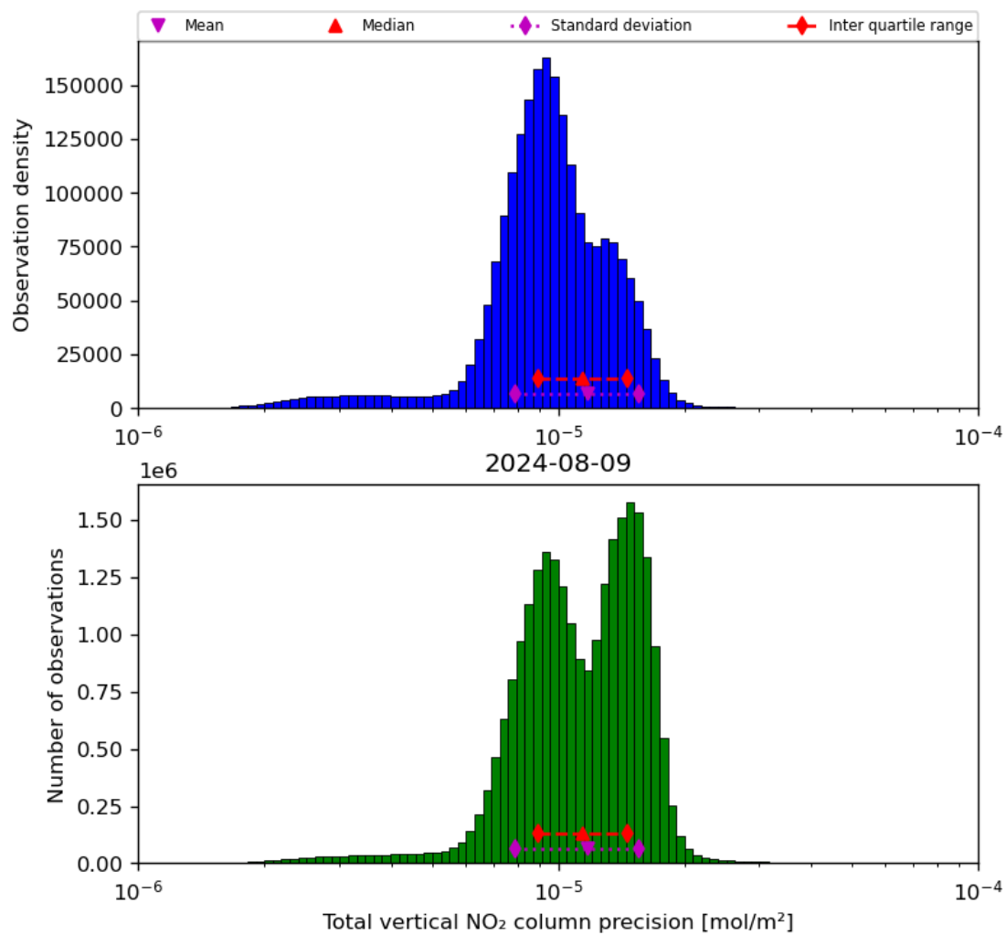
Figure 39: Histogram of "Total vertical NO 2 column precision" for 2024-08-08 to 2024-08-10
