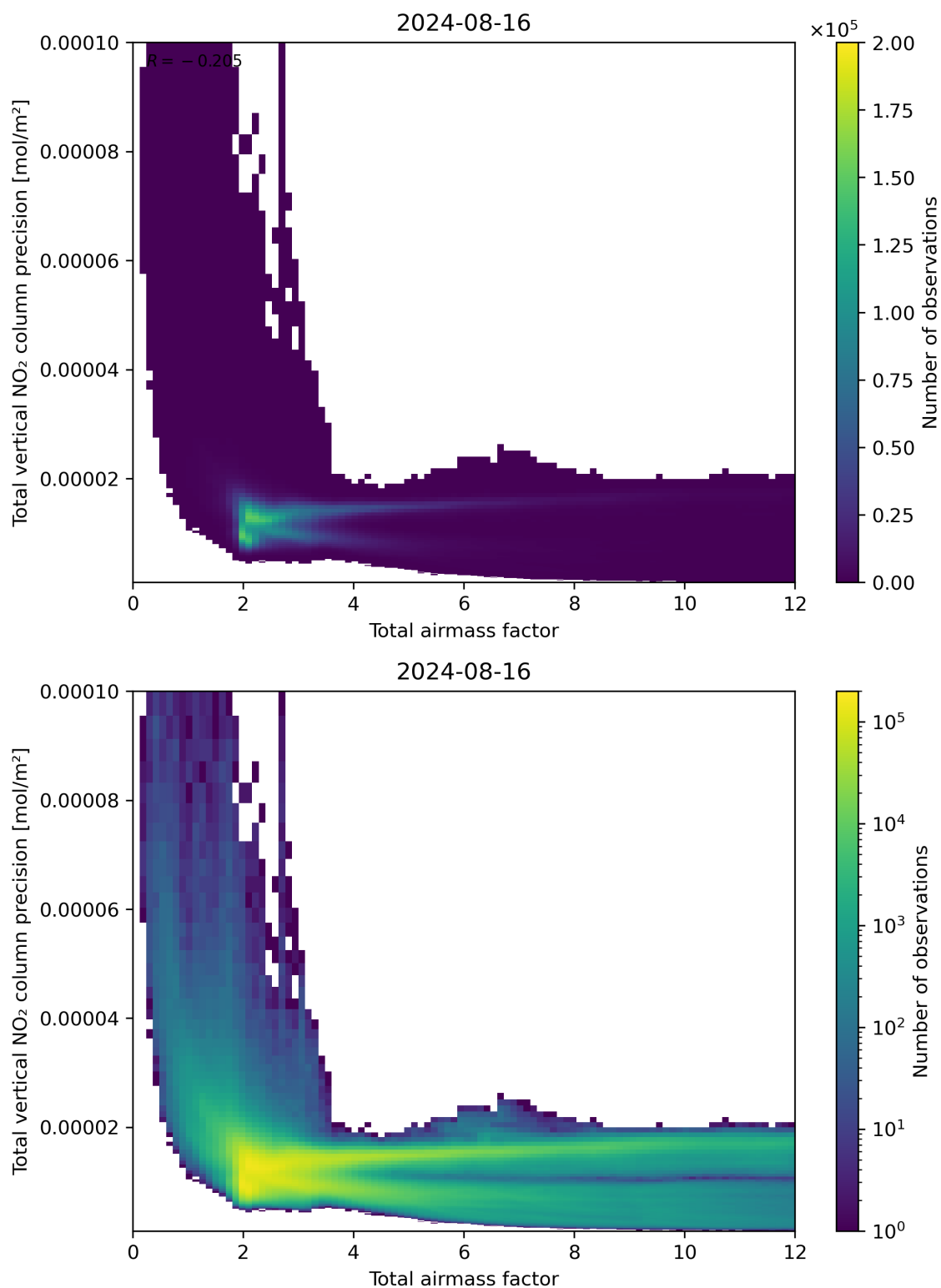
Figure 68: Scatter density plot of “Total airmass factor” against “Total vertical NO 2 column precision” for 2024-08-16 to 2024-08-17.
