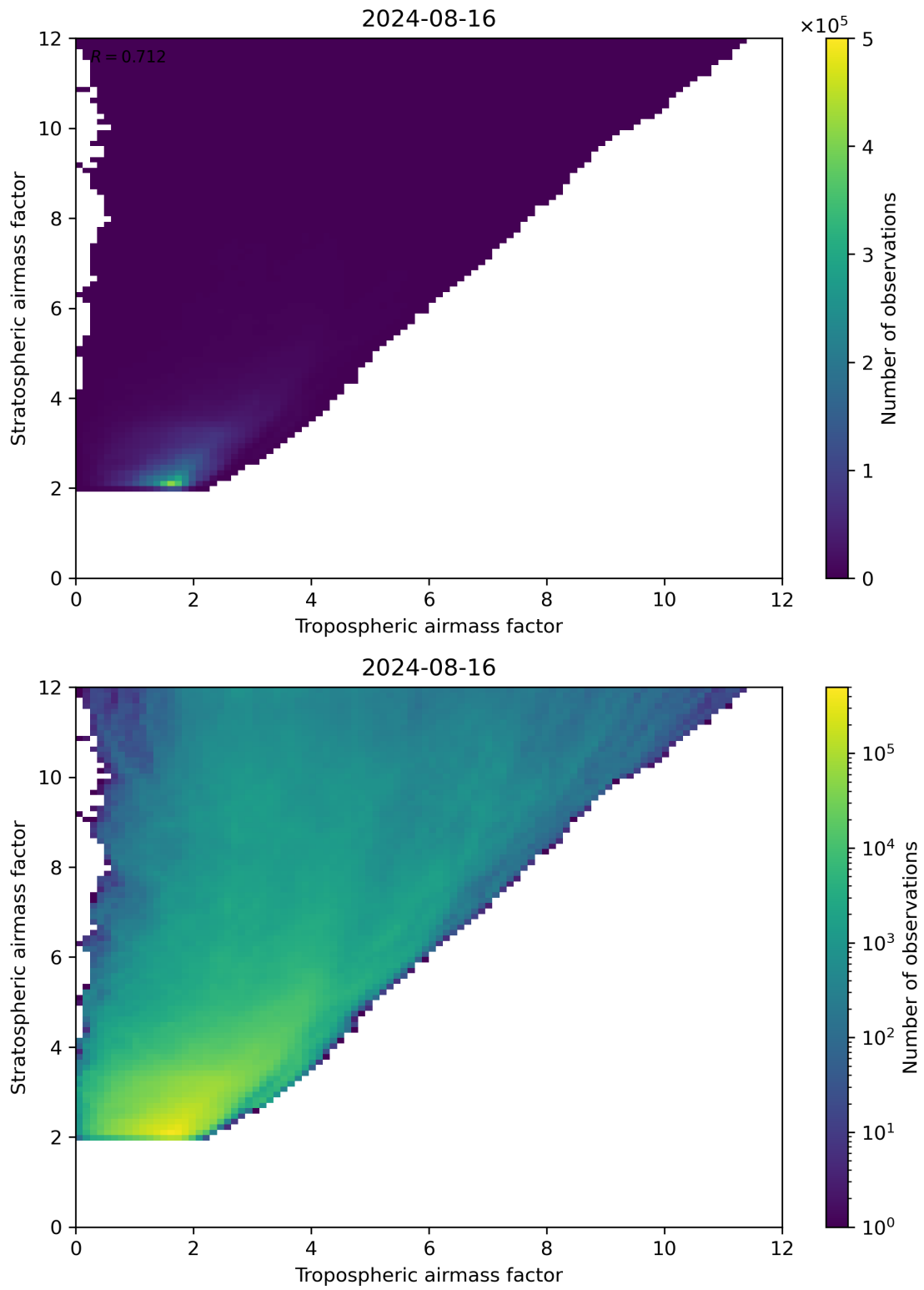
Figure 71: Scatter density plot of “Tropospheric airmass factor” against “Stratospheric airmass factor” for 2024-08-16 to 2024-08-17.
