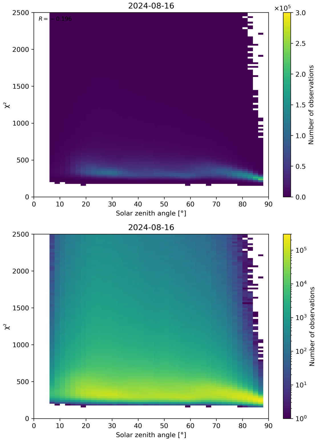
Figure 148: Scatter density plot of “Solar zenith angle” against “ \chi^2 ” for 2024-08-16 to 2024-08-17.
