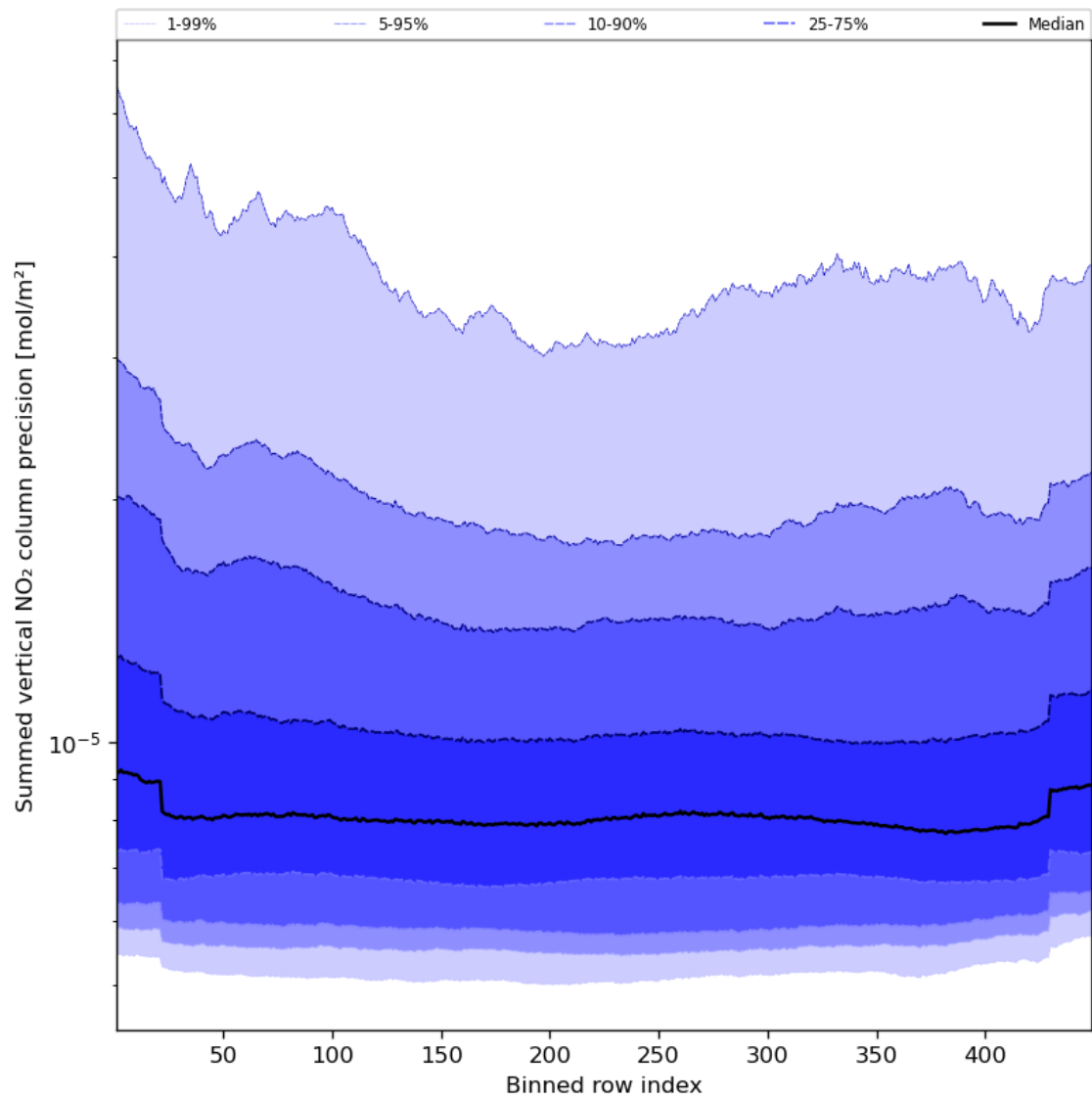
Figure 58: Along track statistics of “Summed vertical NO 2 column precision” for 2024-08-16 to 2024-08-17
