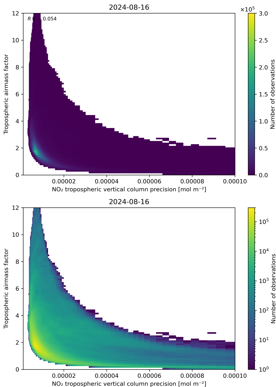
Figure 133: Scatter density plot of “NO 2 tropospheric vertical column precision” against “Tropospheric airmass factor” for 2024-08-16 to 2024-08-17.
