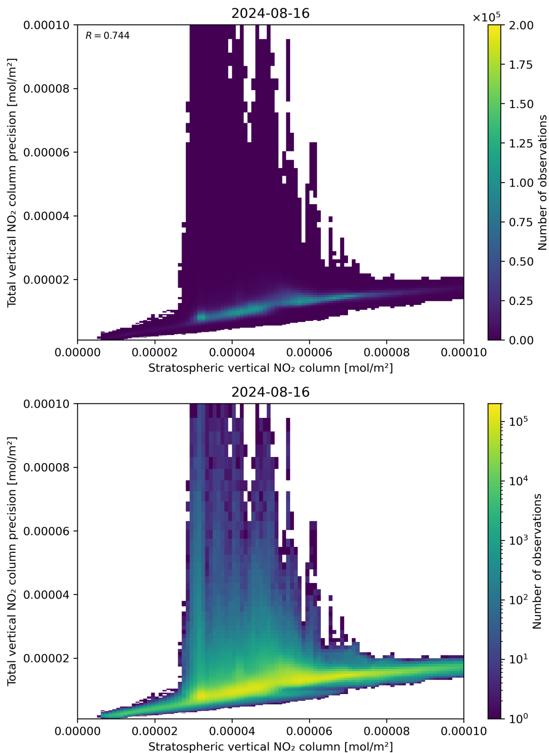
Figure 101: Scatter density plot of “Stratospheric vertical NO 2 column” against “Total vertical NO 2 column precision” for 2024-08-16 to 2024-08-17.
