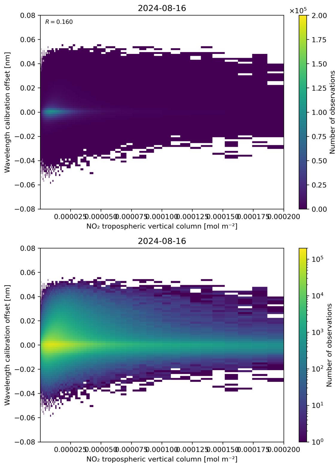
Figure 143: Scatter density plot of “NO 2 tropospheric vertical column” against “Wavelength calibration offset” for 2024-08-16 to 2024-08-17.
