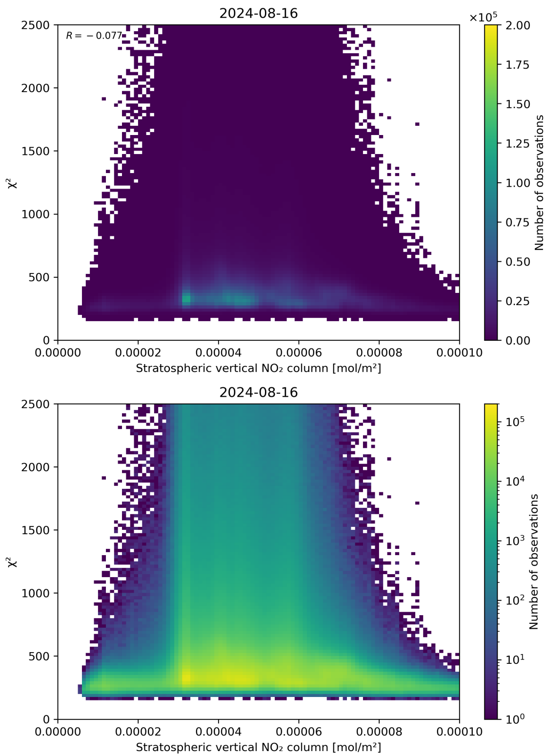
Figure 97: Scatter density plot of “Stratospheric vertical NO 2 column” against “ \chi^2 ” for 2024-08-16 to 2024-08-17.
