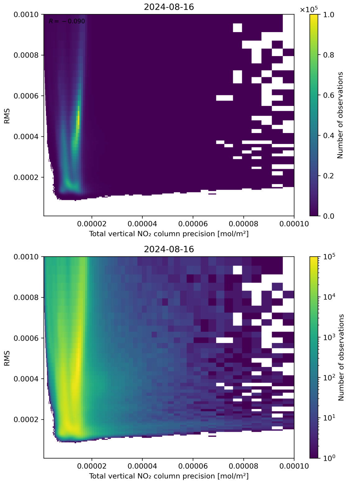
Figure 119: Scatter density plot of “Total vertical NO 2 column precision” against “RMS” for 2024-08-16 to 2024-08-17.
