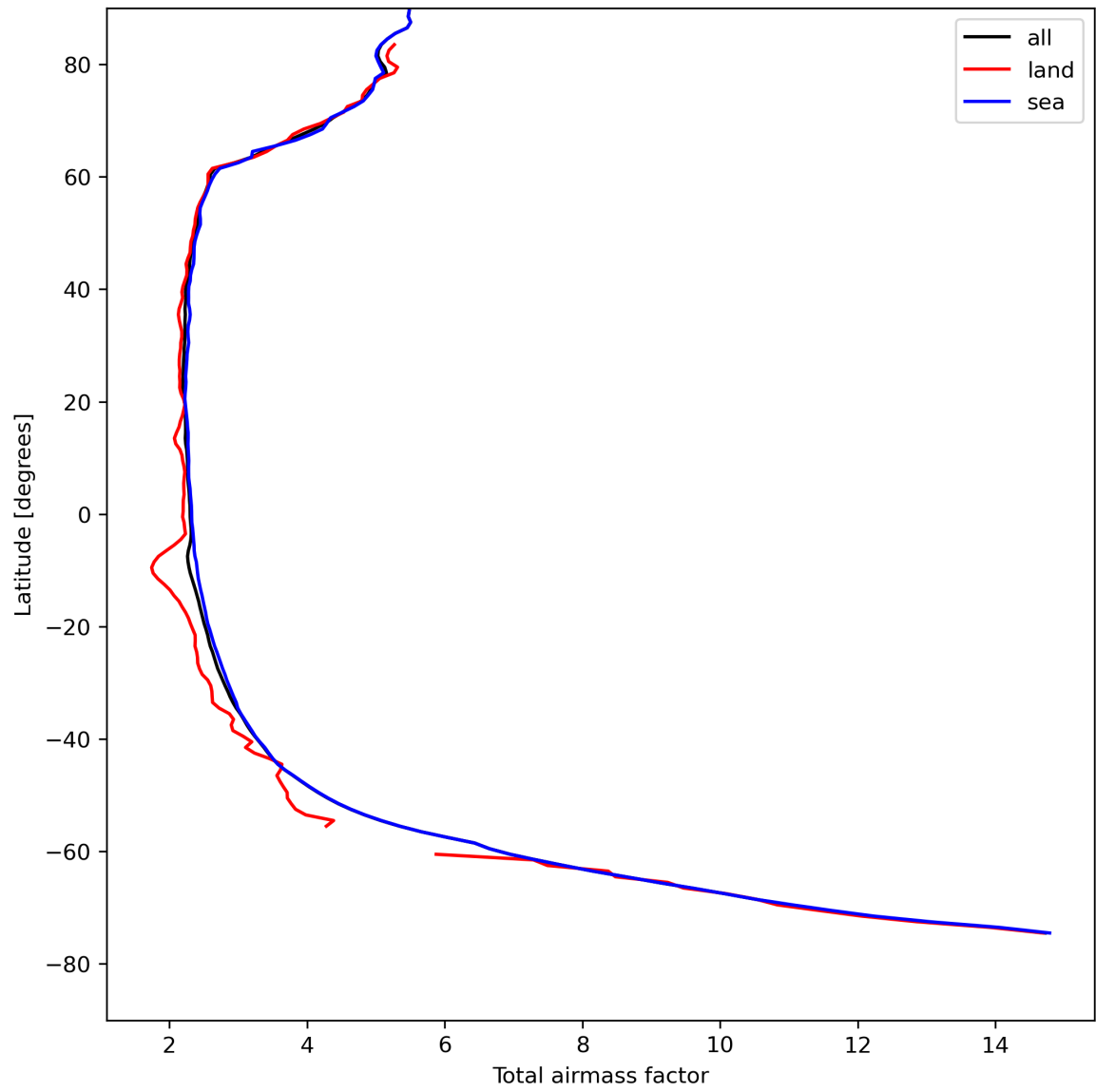
Figure 15: Zonal average of “Total airmass factor” for 2024-08-16 to 2024-08-17.
