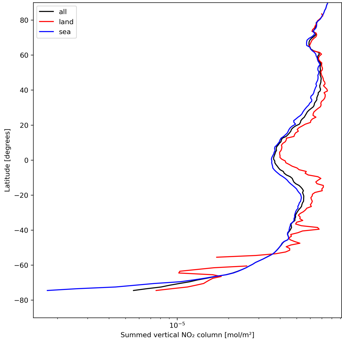
Figure 23: Zonal average of “Summed vertical NO 2 column” for 2024-08-16 to 2024-08-17.
