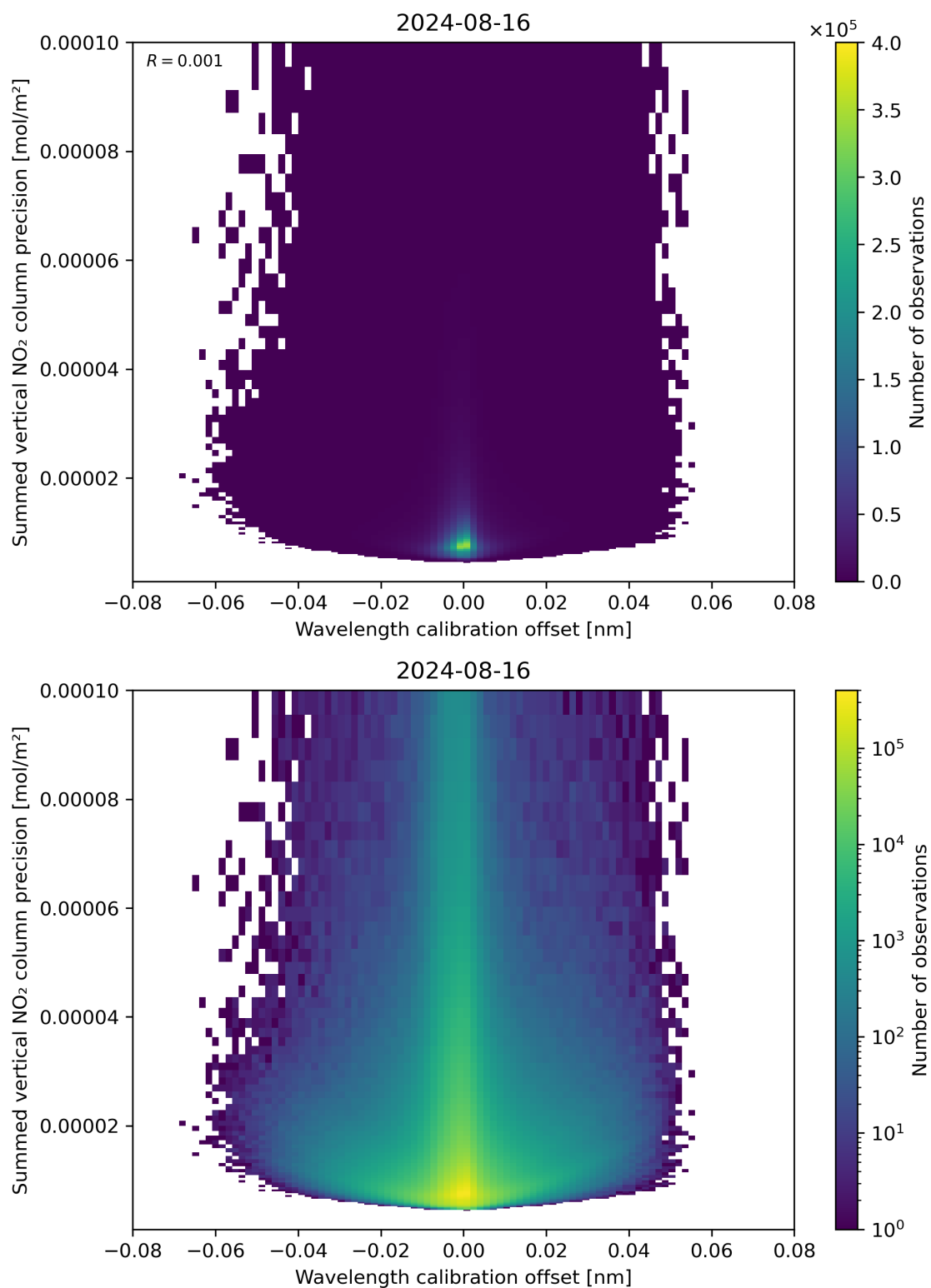
Figure 178: Scatter density plot of “Wavelength calibration offset” against “Summed vertical NO 2 column precision” for 2024-08-16 to 2024-08-17.
