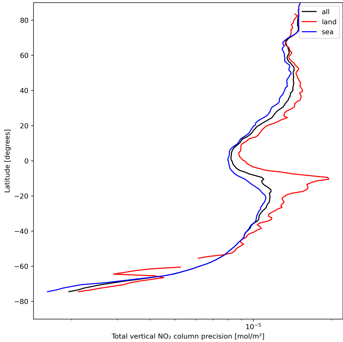
Figure 22: Zonal average of “Total vertical NO 2 column precision” for 2024-08-16 to 2024-08-17.
