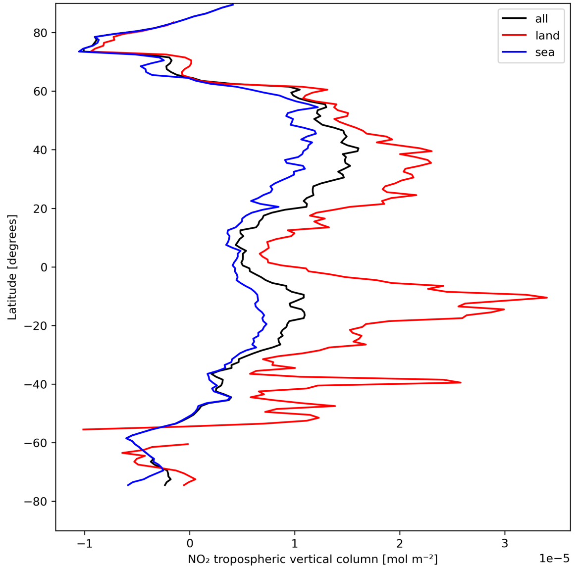
Figure 12: Zonal average of “NO 2 tropospheric vertical column” for 2024-08-16 to 2024-08-17.
