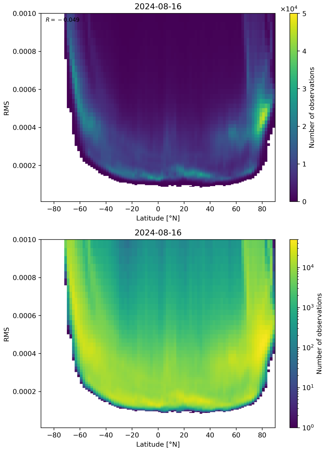
Figure 94: Scatter density plot of “Latitude” against “RMS” for 2024-08-16 to 2024-08-17.
