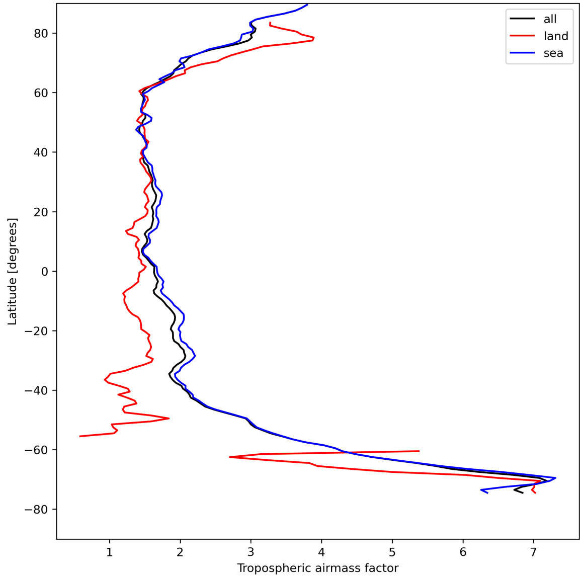
Figure 14: Zonal average of “Tropospheric air mass factor” for 2024-08-16 to 2024-08-17.
