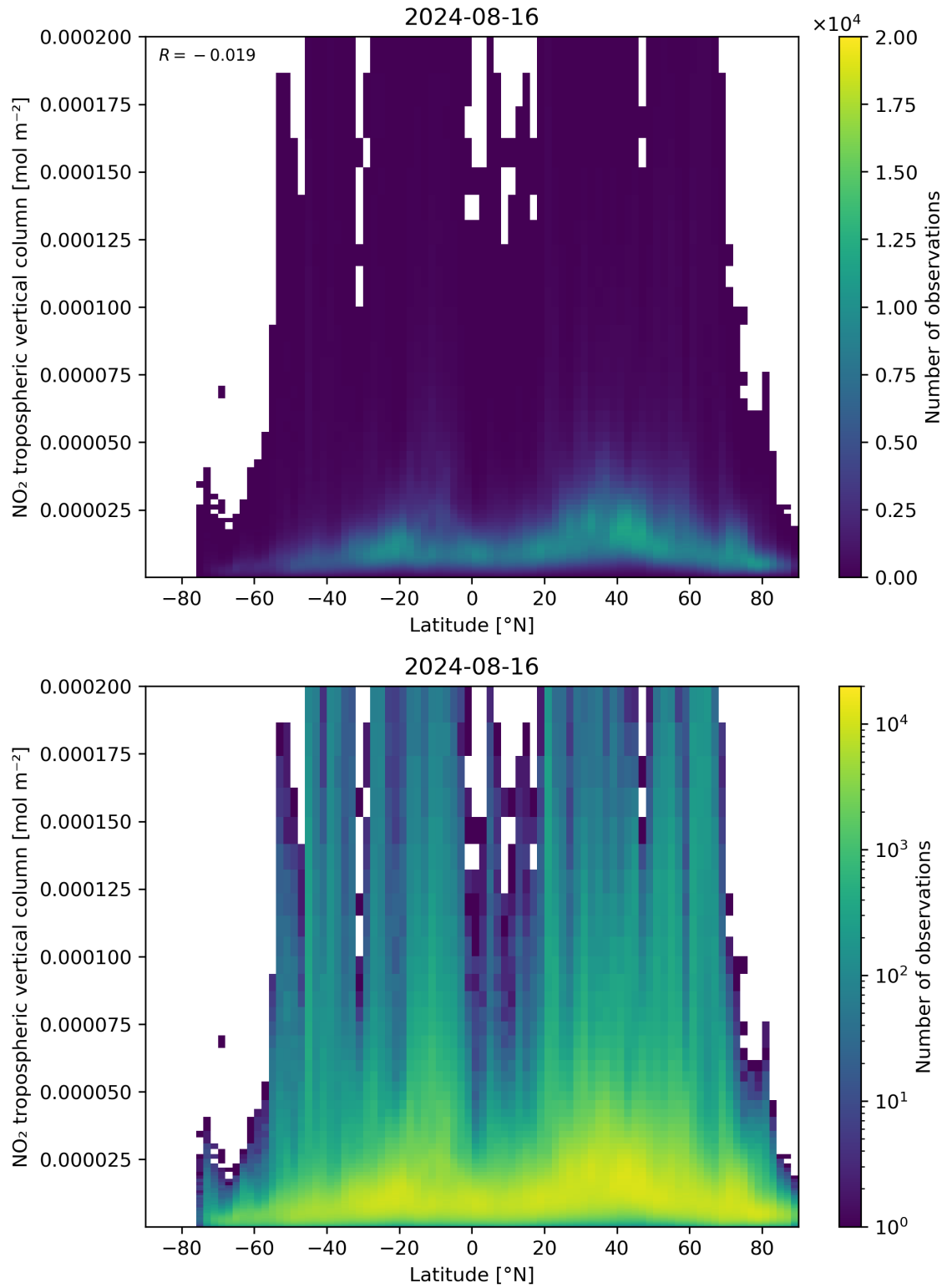
Figure 92: Scatter density plot of “Latitude” against “NO 2 tropospheric vertical column” for 2024-08-16 to 2024-08-17.
