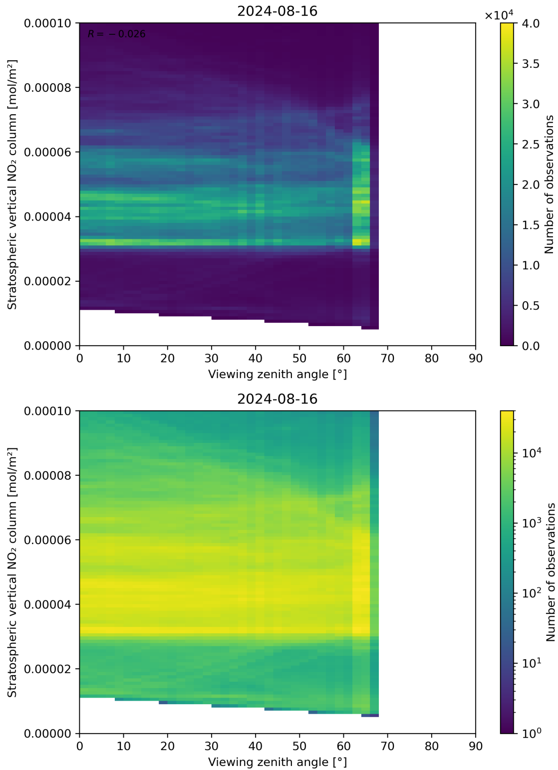
Figure 164: Scatter density plot of “Viewing zenith angle” against “Stratospheric vertical NO 2 column” for 2024-08-16 to 2024-08-17.
