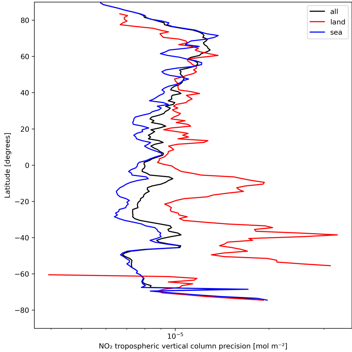
Figure 13: Zonal average of “NO 2 tropospheric vertical column precision” for 2024-08-16 to 2024-08-17.
