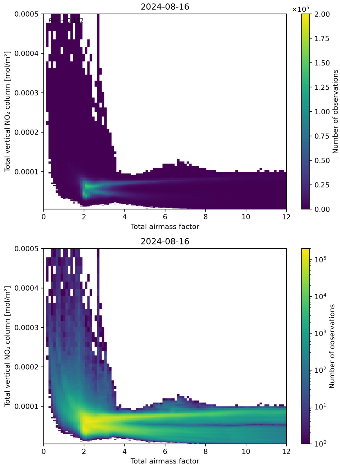
Figure 67: Scatter density plot of “Total airmass factor” against “Total vertical NO 2 column” for 2024-08-16 to 2024-08-17.
