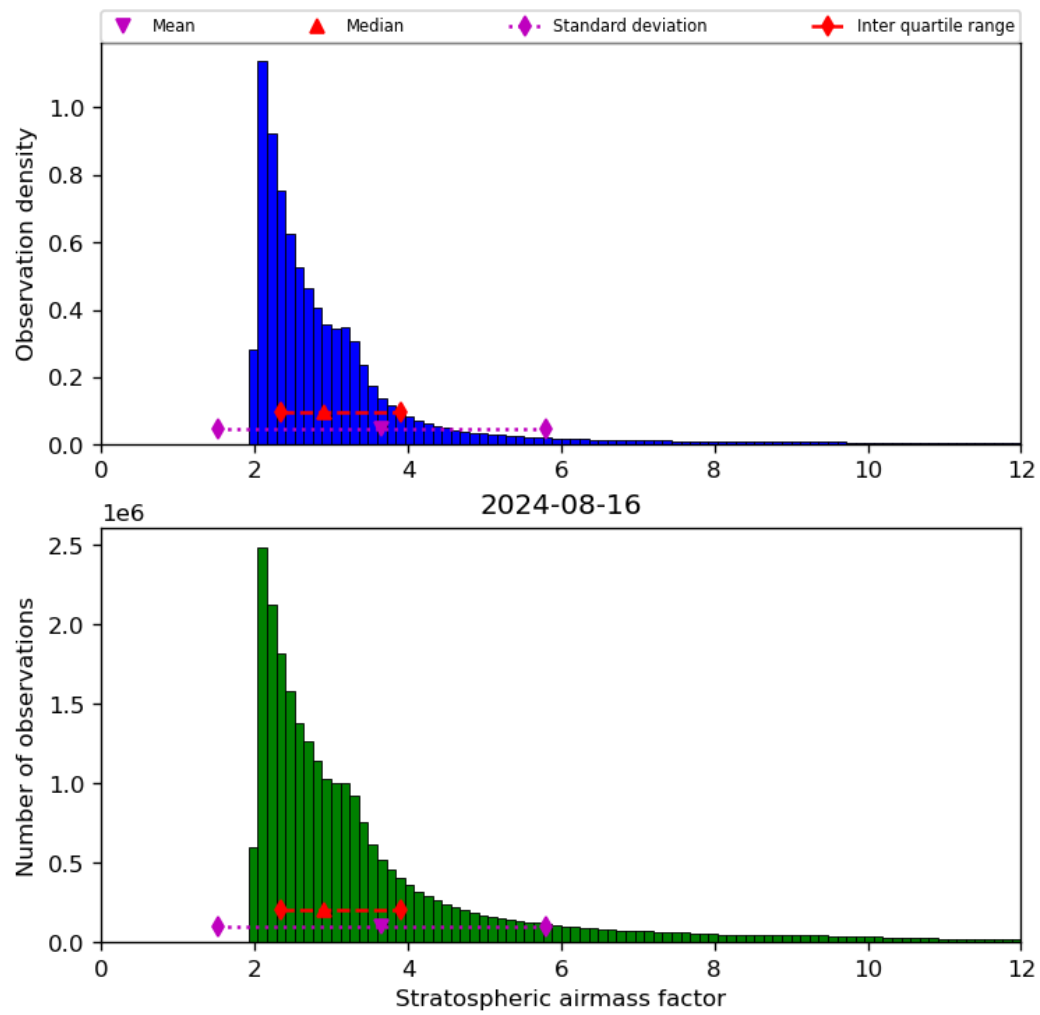
Figure 44: Histogram of “Stratospheric airmass factor” for 2024-08-16 to 2024-08-17
