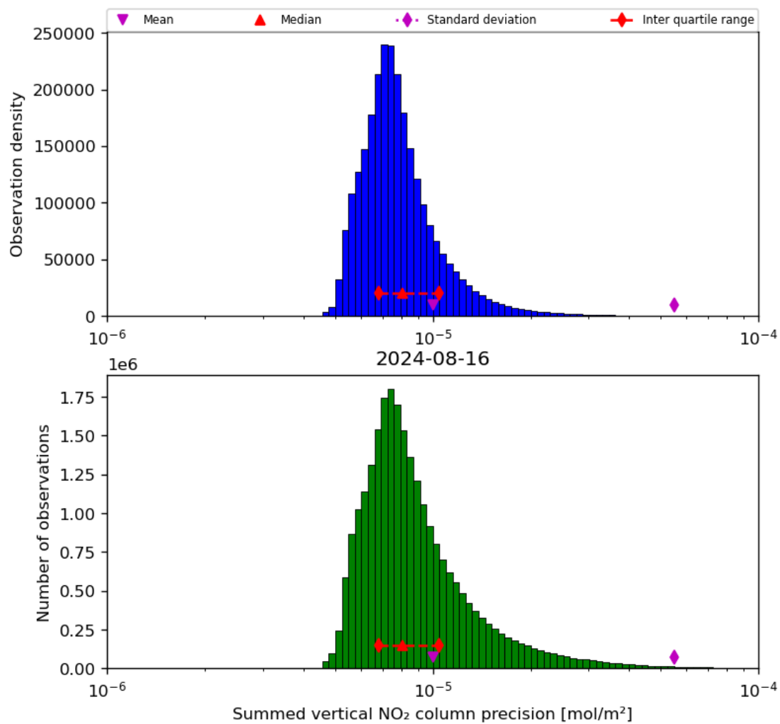
Figure 41: Histogram of “Summed vertical NO 2 column precision” for 2024-08-16 to 2024-08-17
