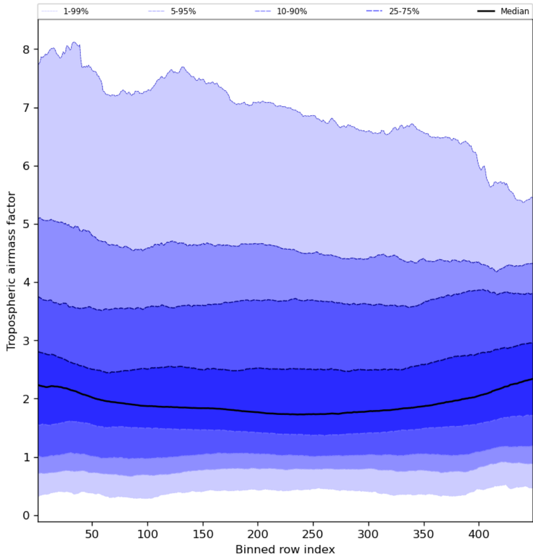
Figure 48: Along track statistics of “Tropospheric air mass factor” for 2024-08-16 to 2024-08-17
