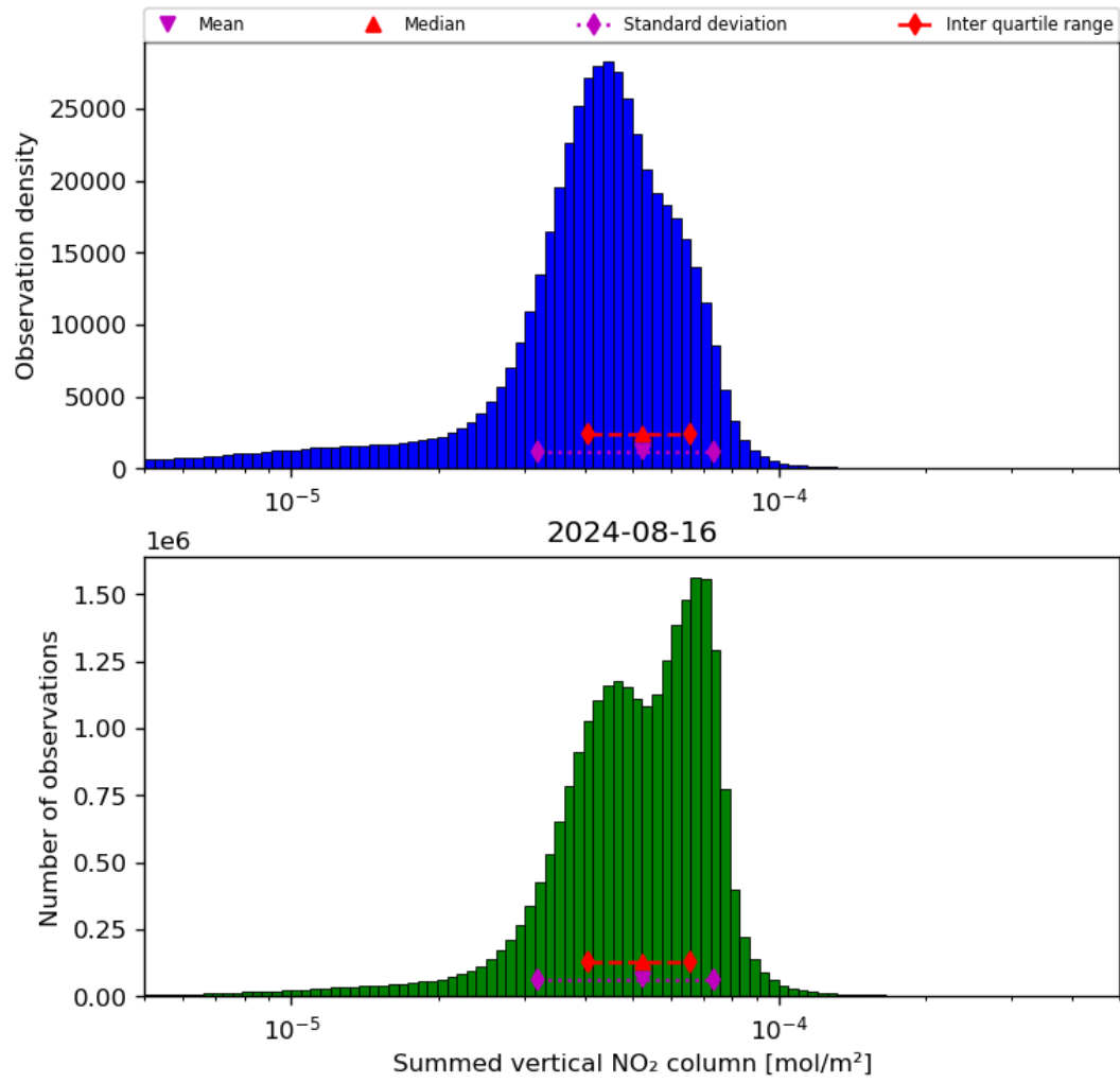
Figure 40: Histogram of “Summed vertical NO 2 column” for 2024-08-16 to 2024-08-17
