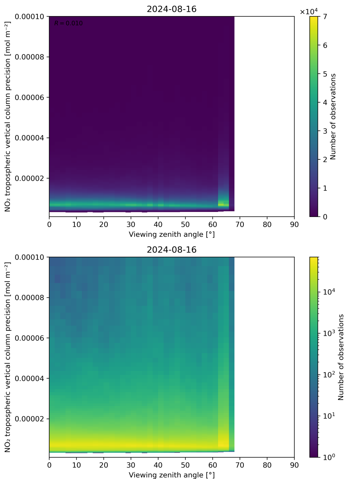
Figure 170: Scatter density plot of “Viewing zenith angle” against “NO 2 tropospheric vertical column precision” for 2024-08-16 to 2024-08-17.
