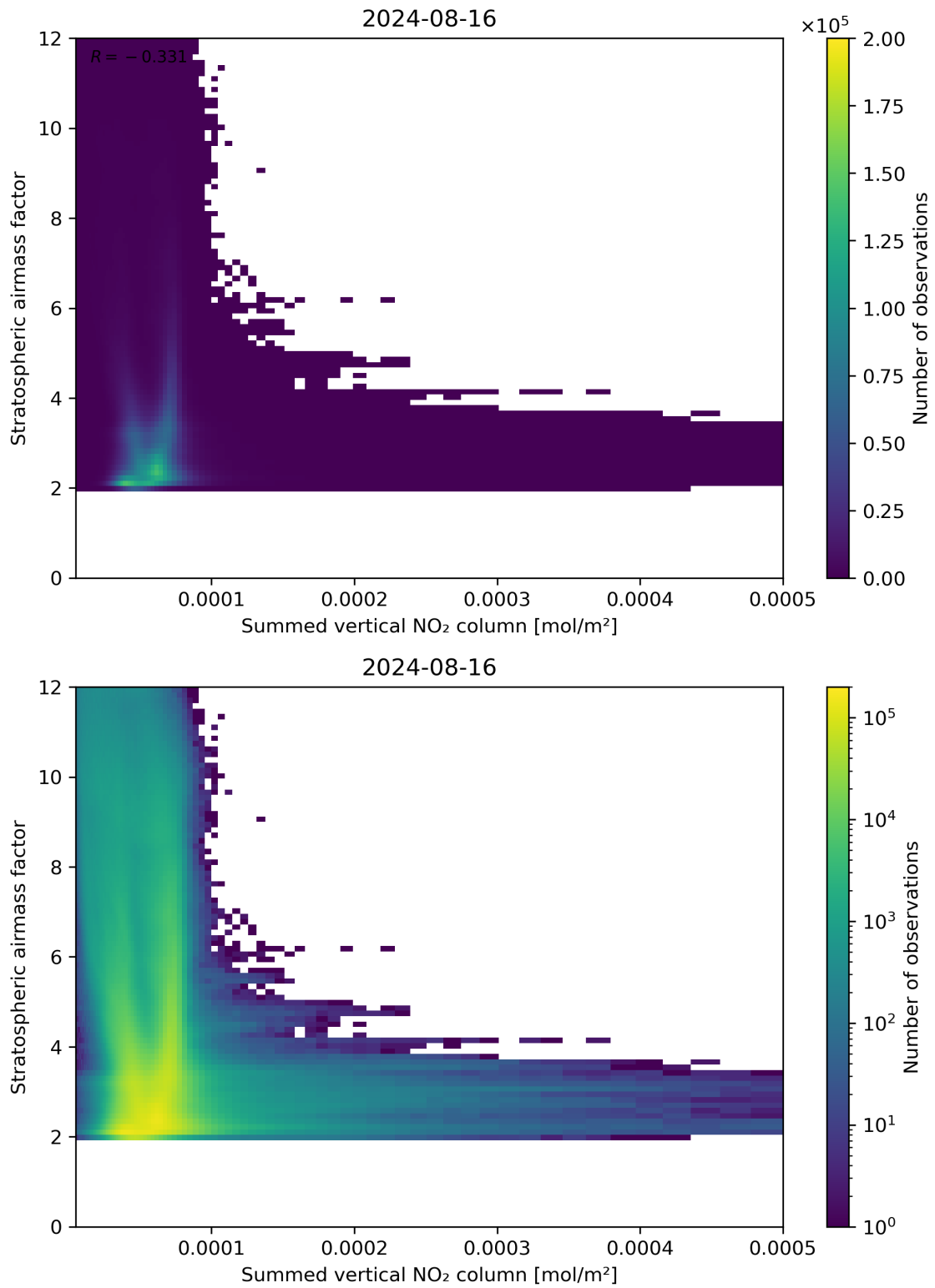
Figure 103: Scatter density plot of “Summed vertical NO 2 column” against “Stratospheric air mass factor” for 2024-08-16 to 2024-08-17.
