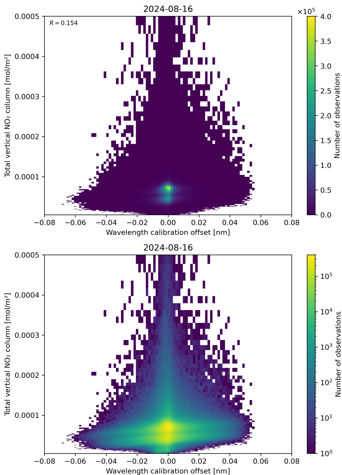
Figure 179: Scatter density plot of “Wavelength calibration offset” against “Total vertical NO 2 column” for 2024-08-16 to 2024-08-17.
