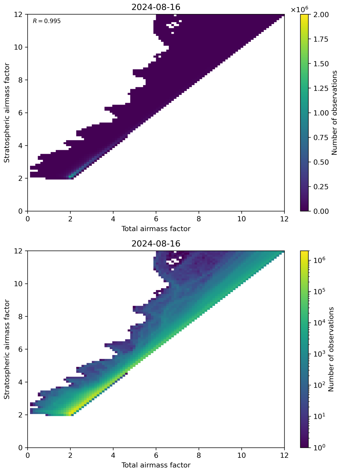
Figure 62: Scatter density plot of “Total airmass factor” against “Stratospheric airmass factor” for 2024-08-16 to 2024-08-17.
