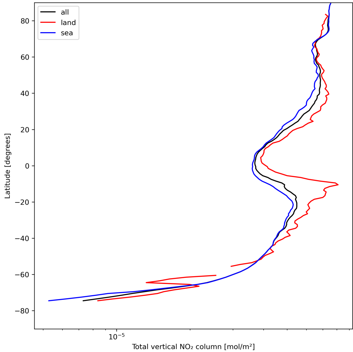
Figure 21: Zonal average of “Total vertical NO 2 column” for 2024-08-16 to 2024-08-17.
