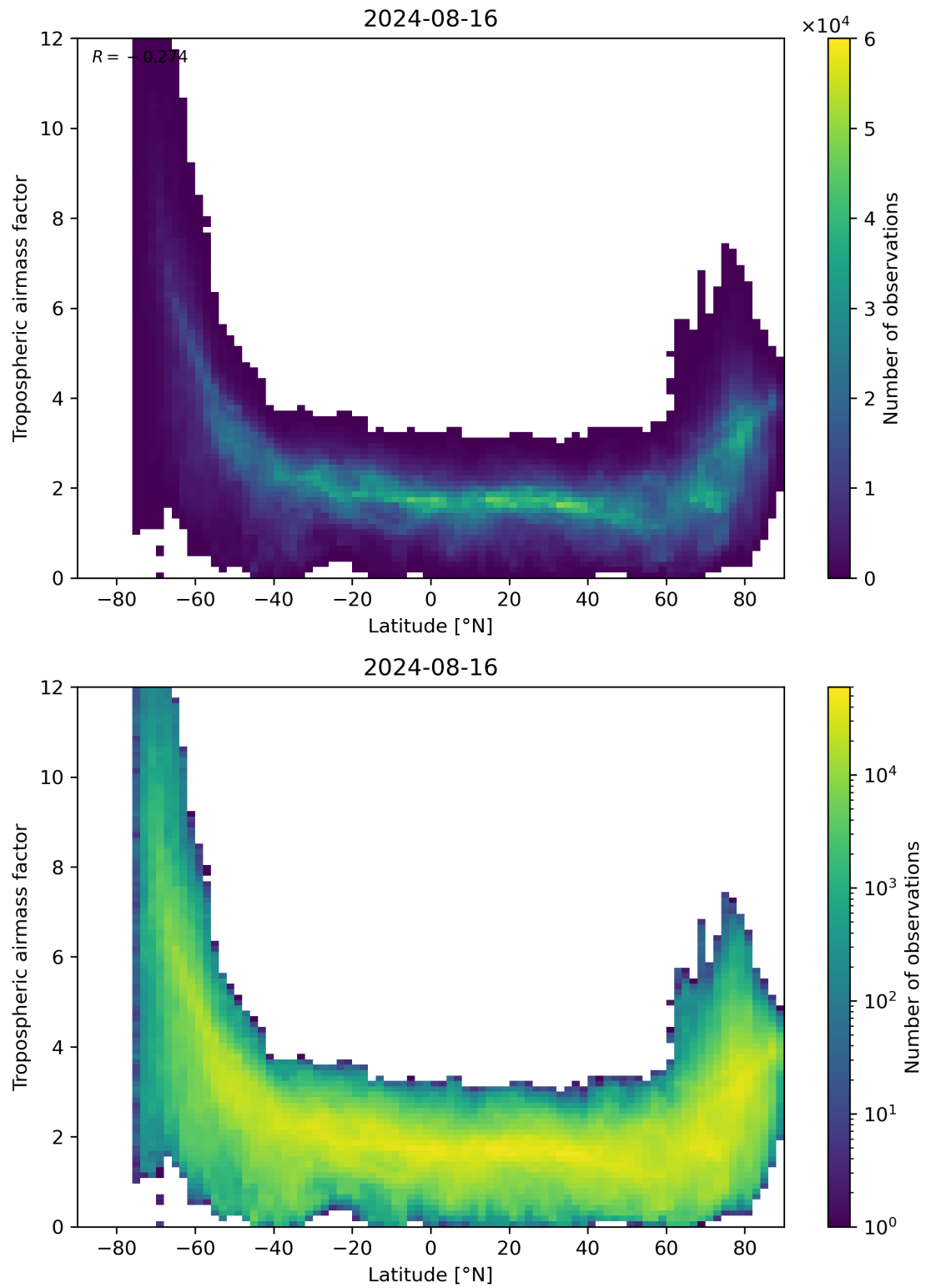
Figure 85: Scatter density plot of “Latitude” against “Tropospheric airmass factor” for 2024-08-16 to 2024-08-17.
