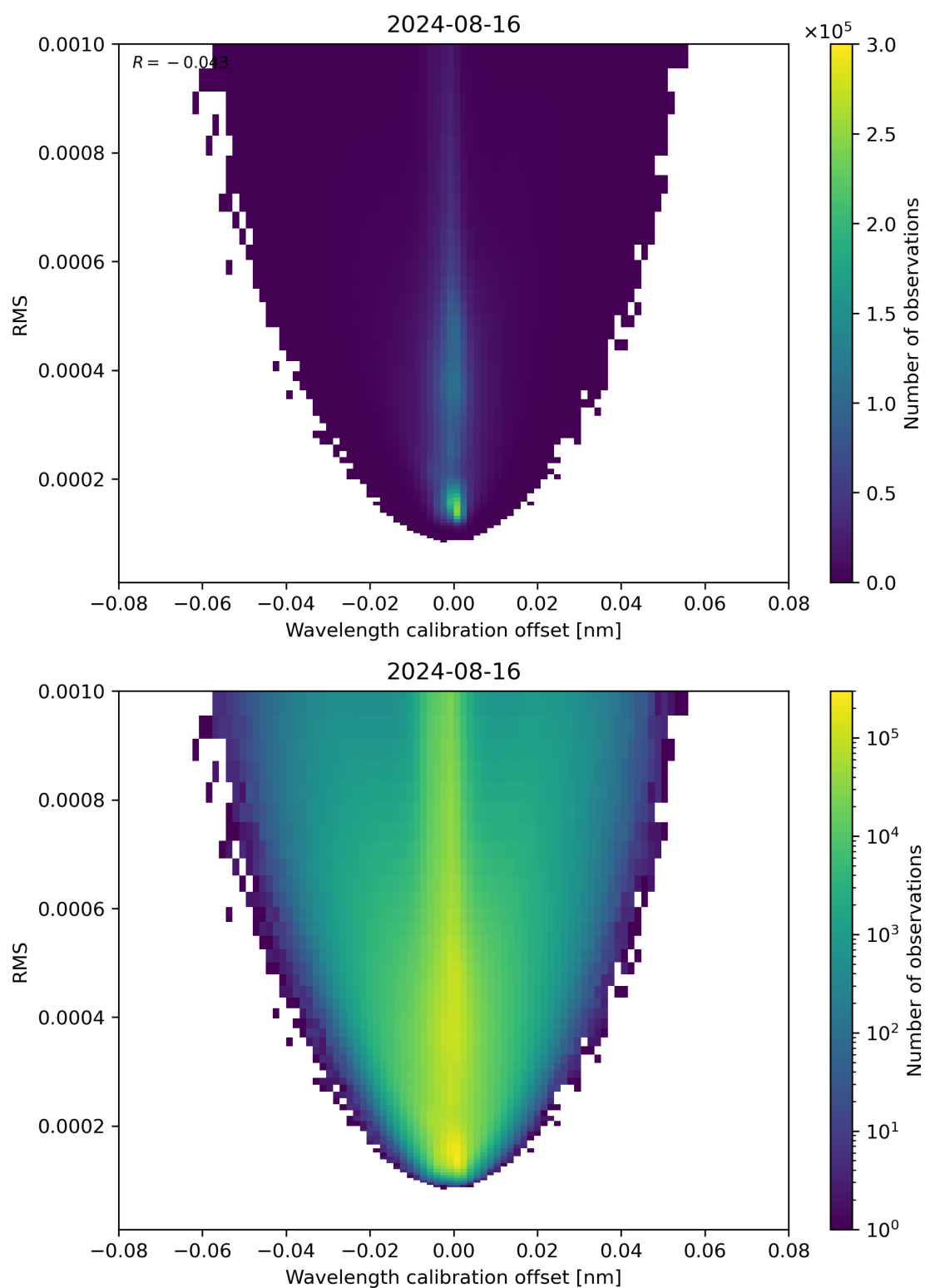
Figure 181: Scatter density plot of “Wavelength calibration offset” against “RMS” for 2024-08-16 to 2024-08-17.
