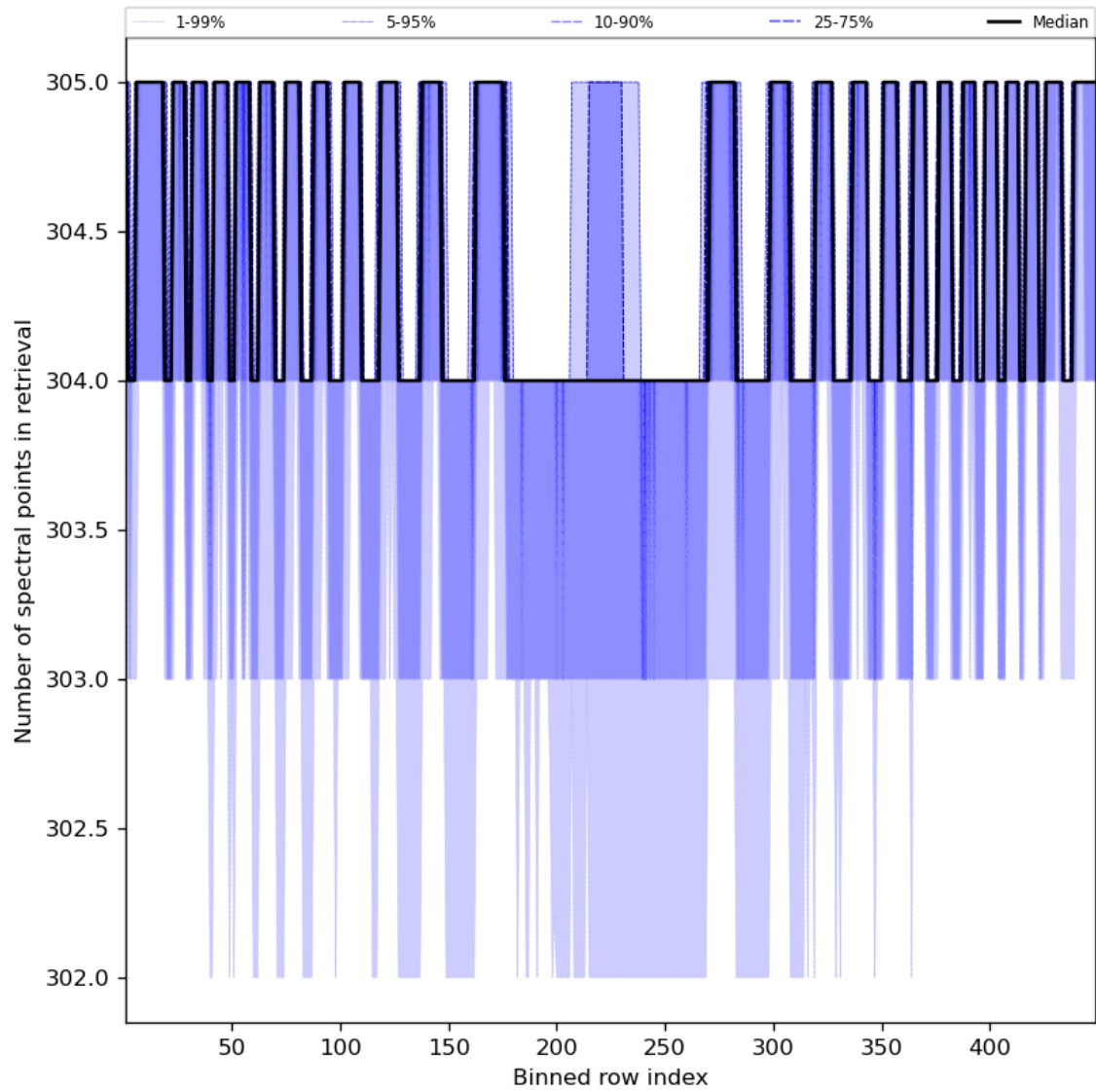
Figure 50: Along track statistics of “Number of spectral points in retrieval” for 2024-08-16 to 2024-08-17
