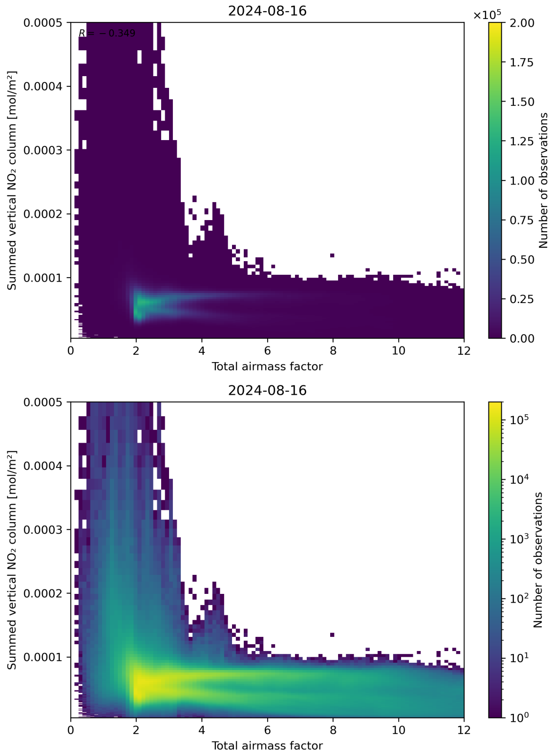
Figure 65: Scatter density plot of “Total airmass factor” against “Summed vertical NO 2 column” for 2024-08-16 to 2024-08-17.
