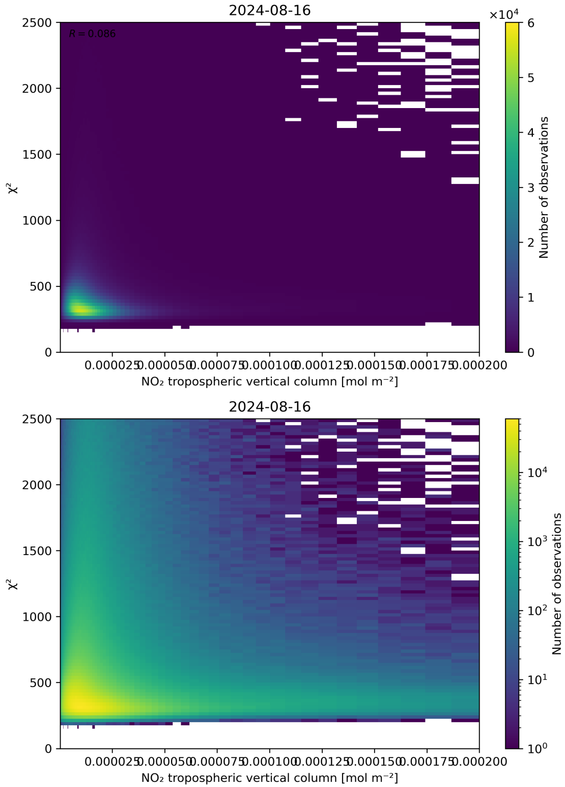
Figure 124: Scatter density plot of “NO 2 tropospheric vertical column” against “ \chi^2 ” for 2024-08-16 to 2024-08-17.
