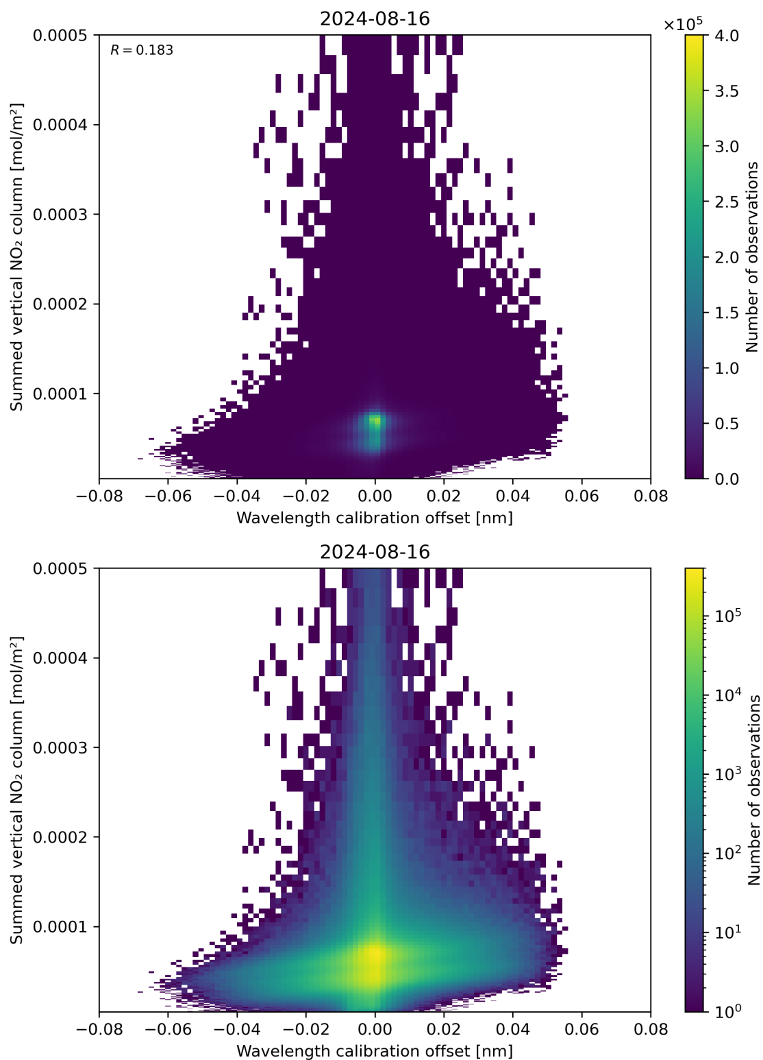
Figure 177: Scatter density plot of “Wavelength calibration offset” against “Summed vertical NO 2 column” for 2024-08-16 to 2024-08-17.
