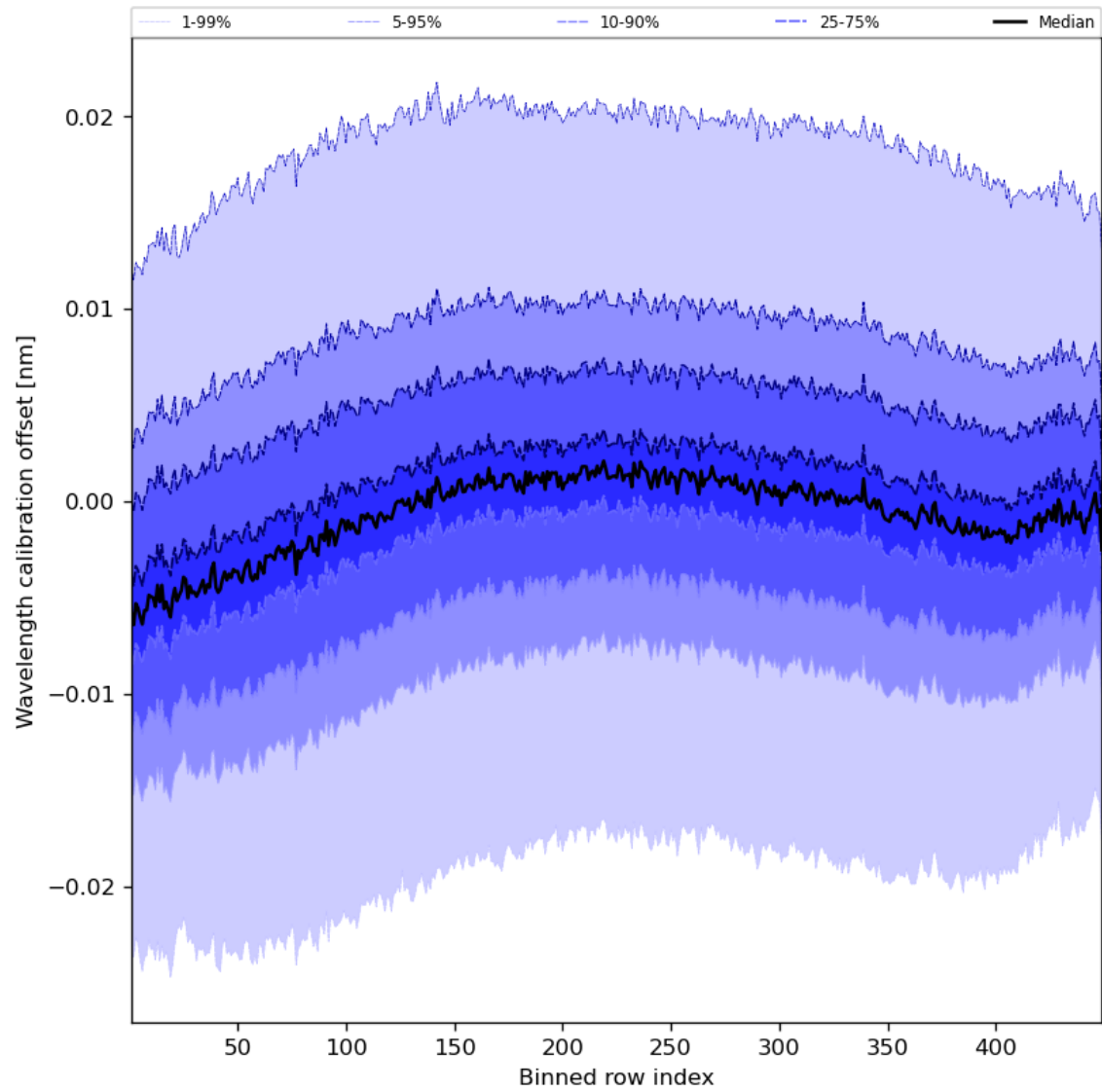
Figure 52: Along track statistics of “Wavelength calibration offset” for 2024-08-16 to 2024-08-17
