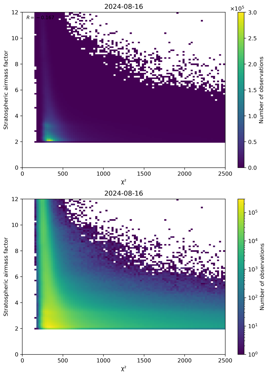
Figure 81: Scatter density plot of “ \chi^2 ” against “Stratospheric airmass factor” for 2024-08-16 to 2024-08-17.
