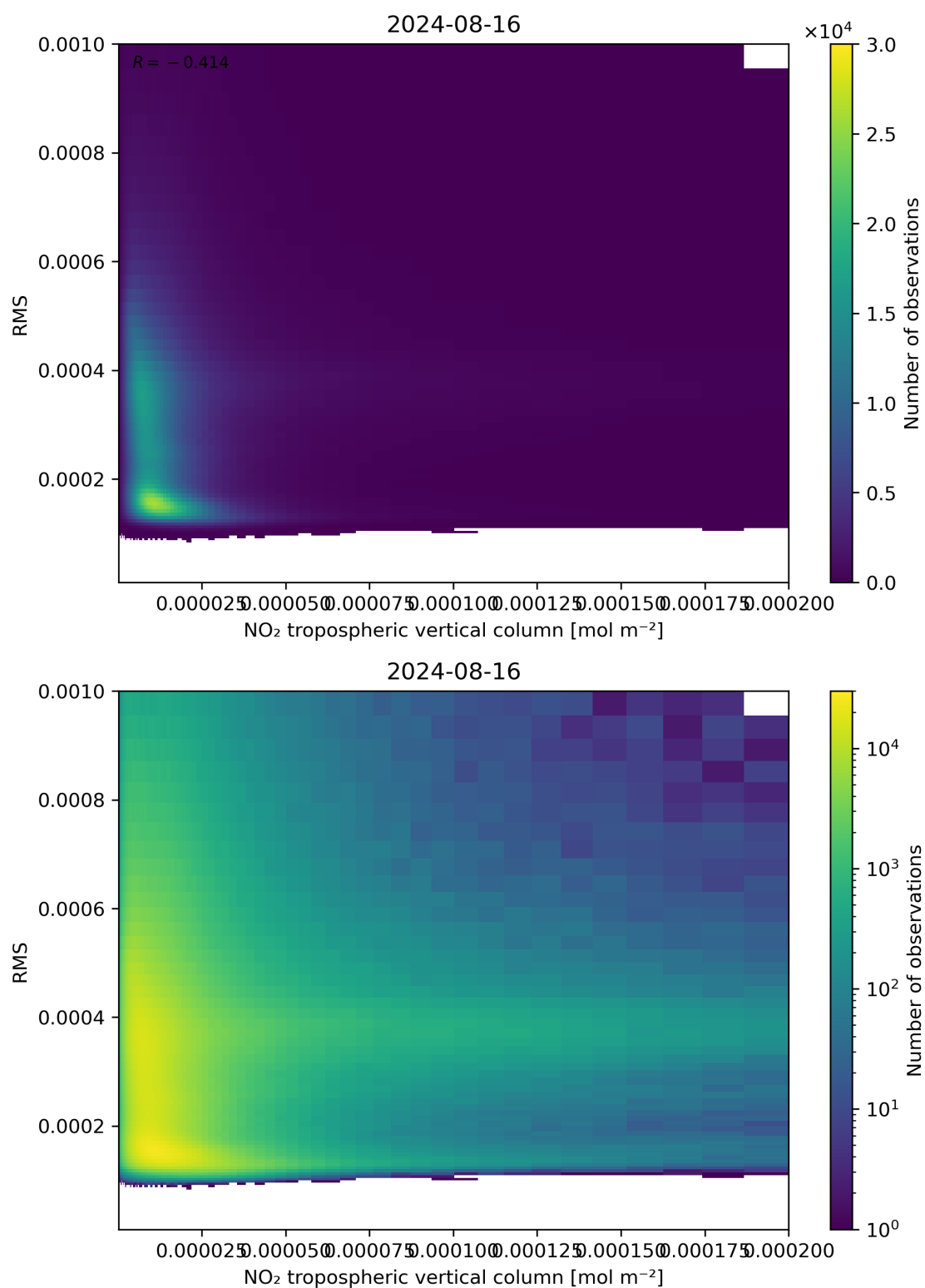
Figure 142: Scatter density plot of “NO 2 tropospheric vertical column” against “RMS” for 2024-08-16 to 2024-08-17.
