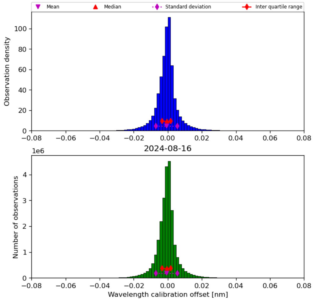
Figure 35: Histogram of “Wavelength calibration offset” for 2024-08-16 to 2024-08-17
