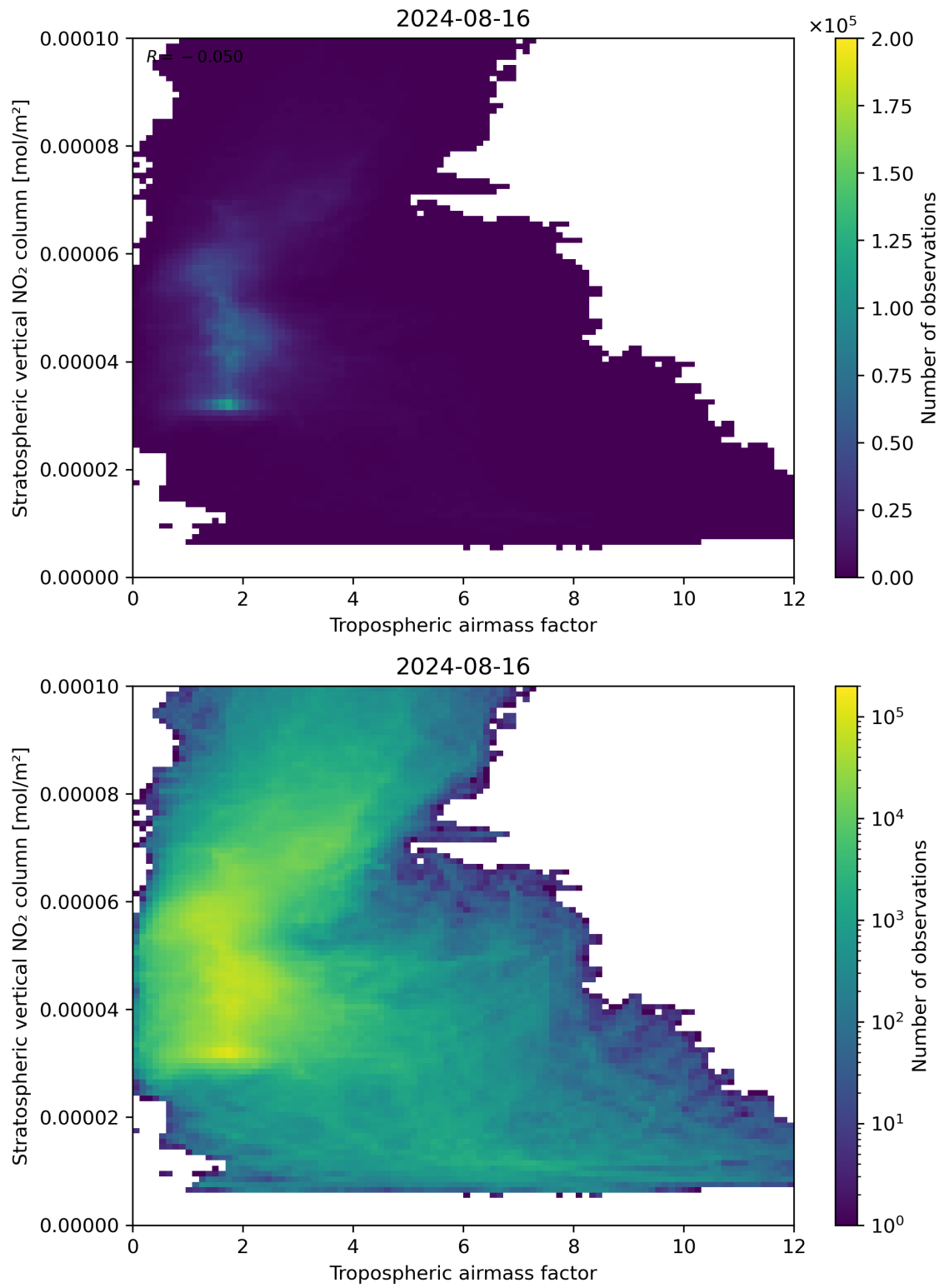
Figure 74: Scatter density plot of “Tropospheric air mass factor” against “Stratospheric vertical NO 2 column” for 2024-08-16 to 2024-08-17.
