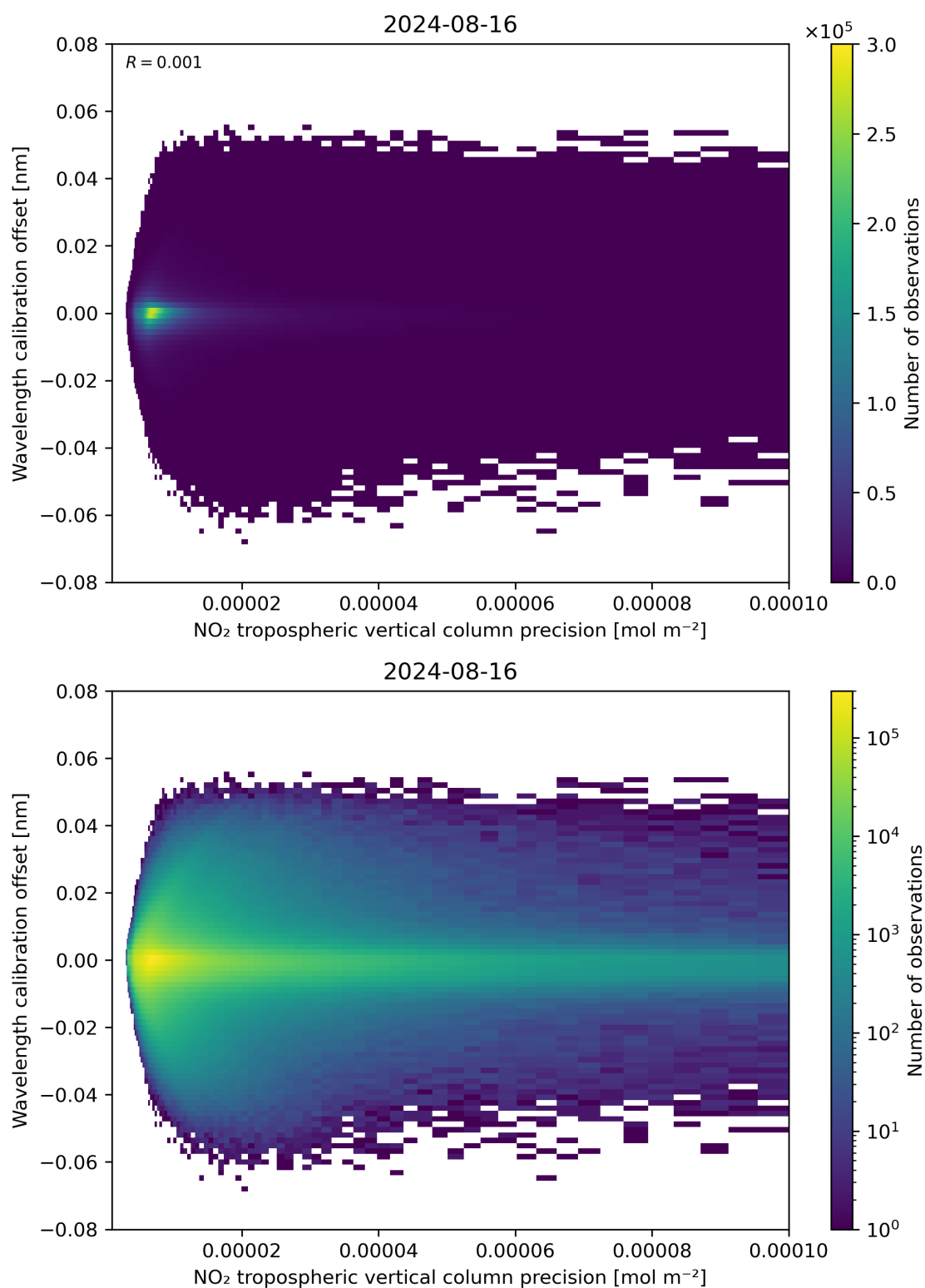
Figure 141: Scatter density plot of “NO 2 tropospheric vertical column precision” against “Wavelength calibration offset” for 2024-08-16 to 2024-08-17.
