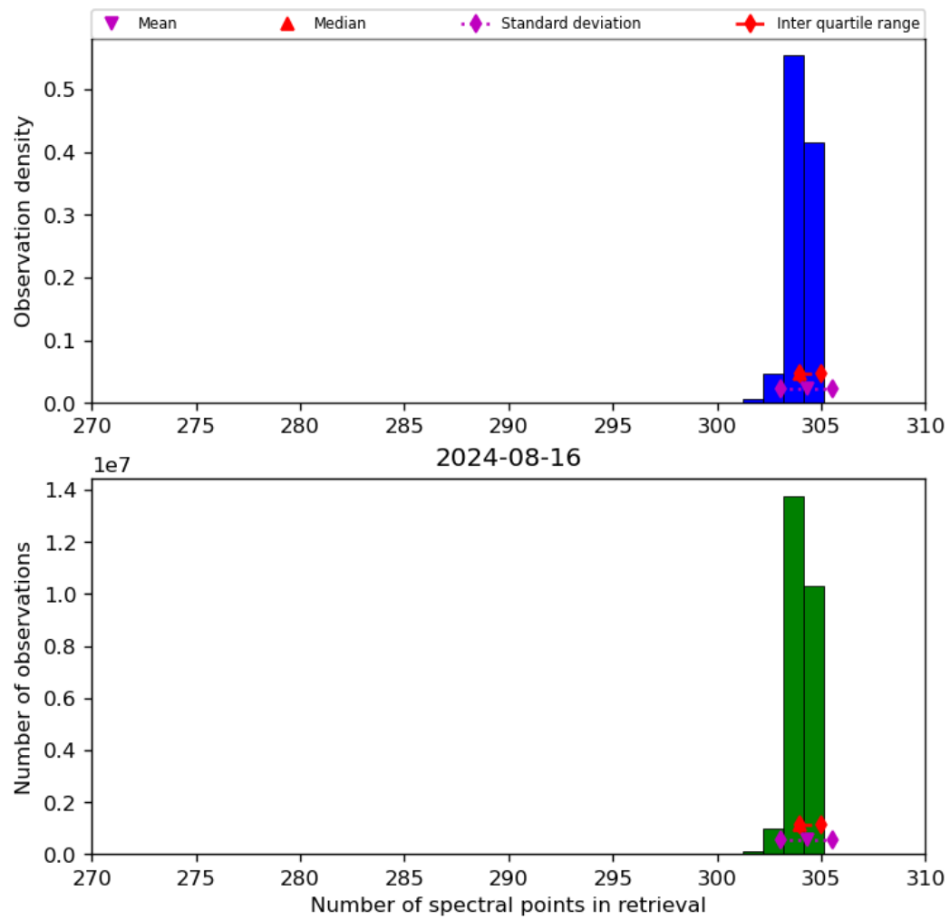
Figure 33: Histogram of “Number of spectral points in retrieval” for 2024-08-16 to 2024-08-17
