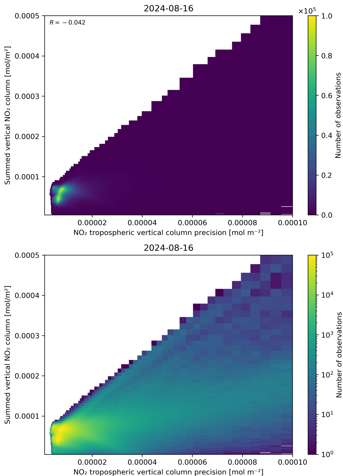
Figure 136: Scatter density plot of “NO 2 tropospheric vertical column precision” against “Summed vertical NO 2 column” for 2024-08-16 to 2024-08-17.
