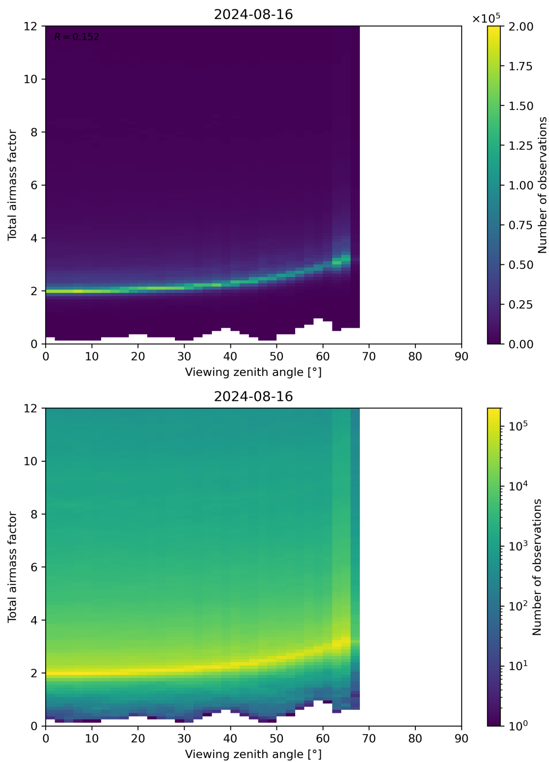
Figure 160: Scatter density plot of “Viewing zenith angle” against “Total airmass factor” for 2024-08-16 to 2024-08-17.
