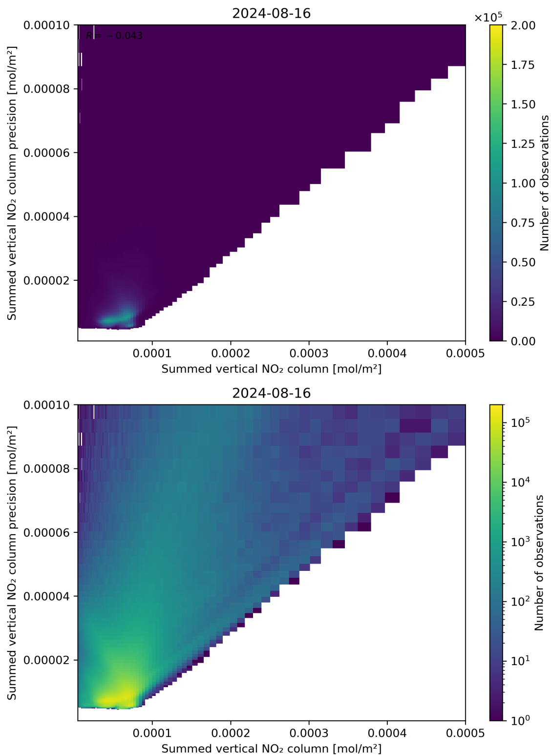
Figure 105: Scatter density plot of “Summed vertical NO 2 column” against “Summed vertical NO 2 column precision” for 2024-08-16 to 2024-08-17.
