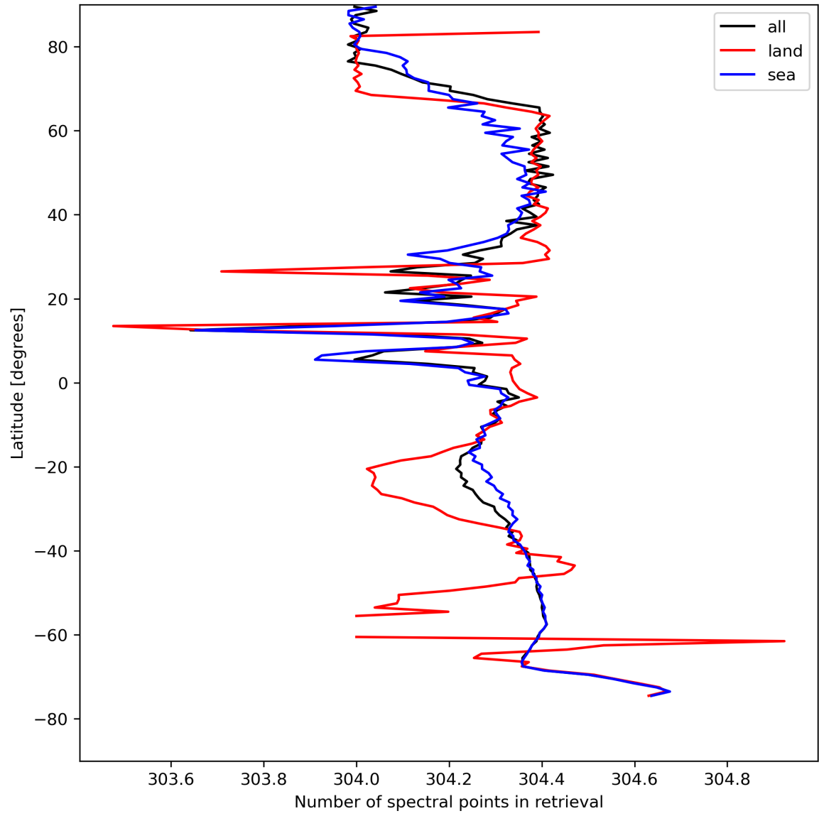
Figure 16: Zonal average of “Number of spectral points in retrieval” for 2024-08-16 to 2024-08-17.
