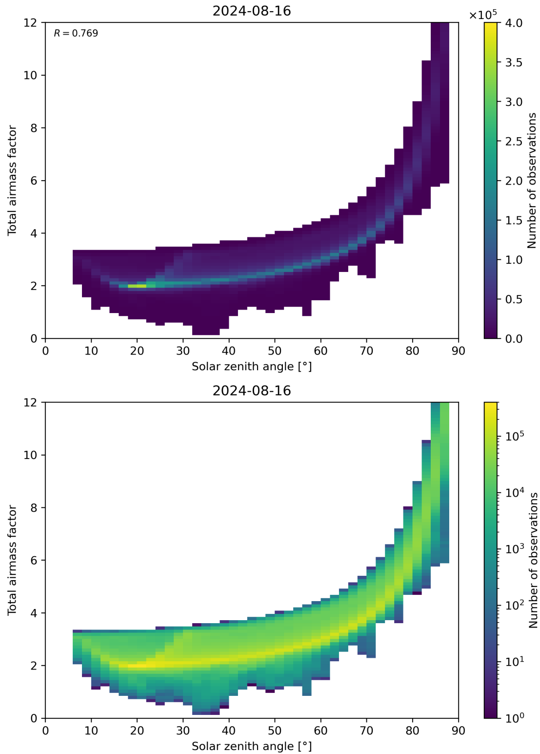
Figure 146: Scatter density plot of “Solar zenith angle” against “Total air mass factor” for 2024-08-16 to 2024-08-17.
