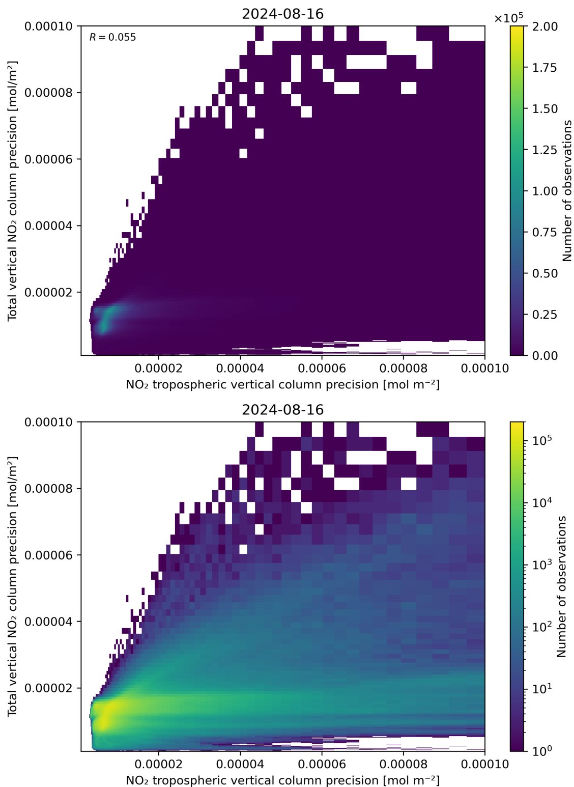
Figure 139: Scatter density plot of “NO 2 tropospheric vertical column precision” against “Total vertical NO 2 column precision” for 2024-08-16 to 2024-08-17.
