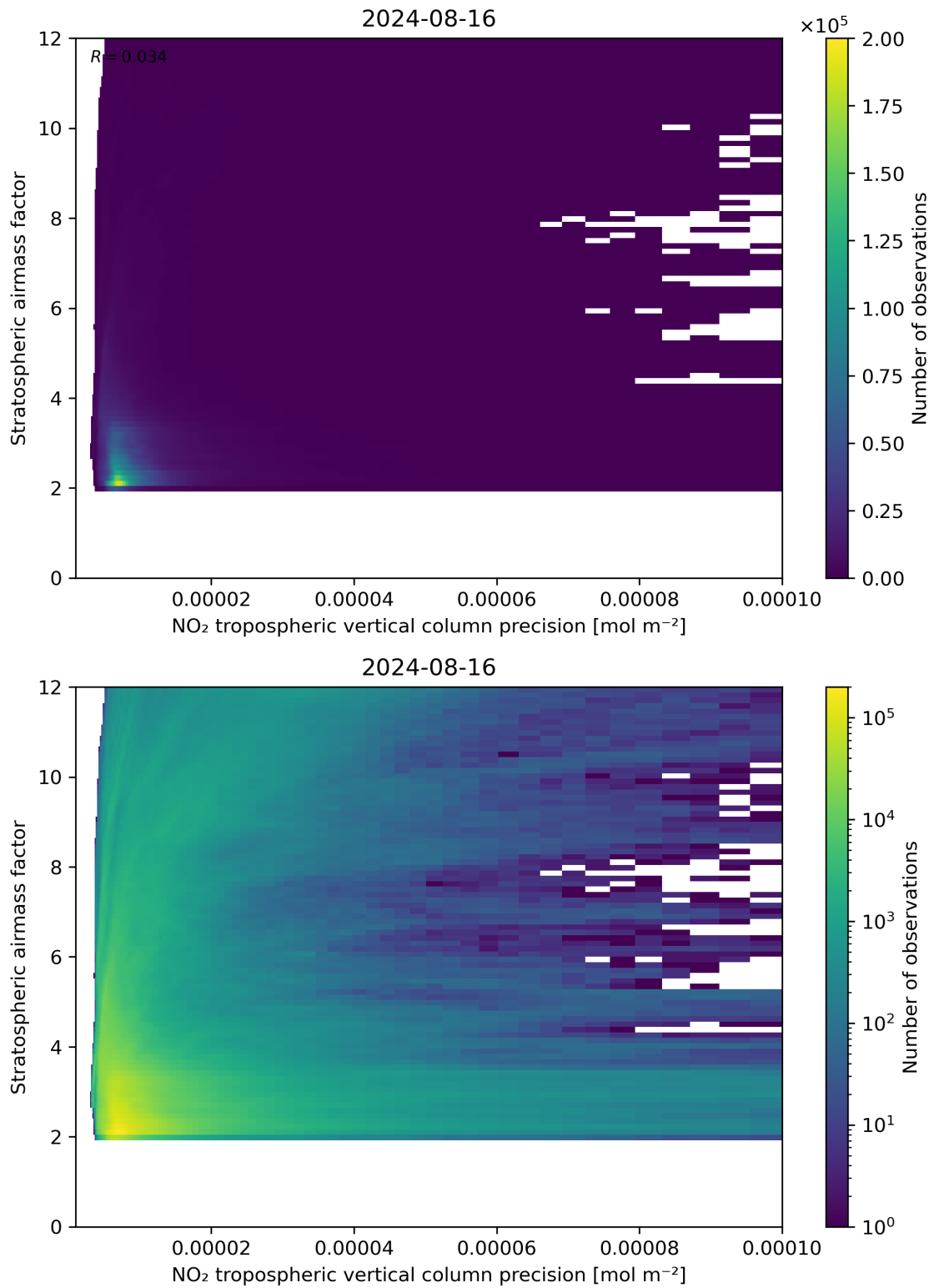
Figure 131: Scatter density plot of “NO 2 tropospheric vertical column precision” against “Stratospheric airmass factor” for 2024-08-16 to 2024-08-17.
