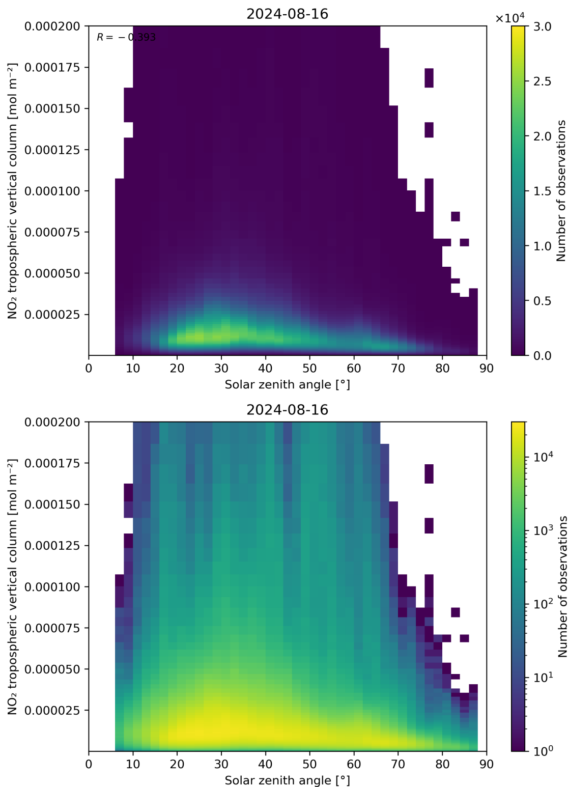
Figure 155: Scatter density plot of “Solar zenith angle” against “NO 2 tropospheric vertical column” for 2024-08-16 to 2024-08-17.
