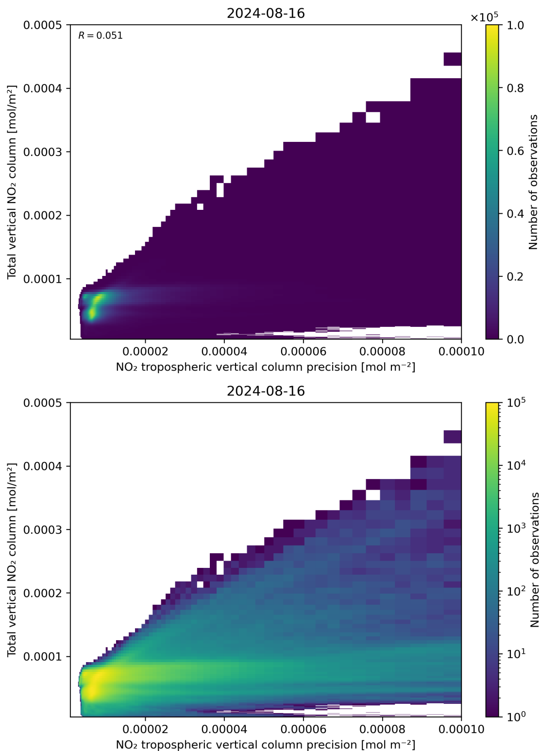
Figure 138: Scatter density plot of “NO 2 tropospheric vertical column precision” against “Total vertical NO 2 column” for 2024-08-16 to 2024-08-17.
