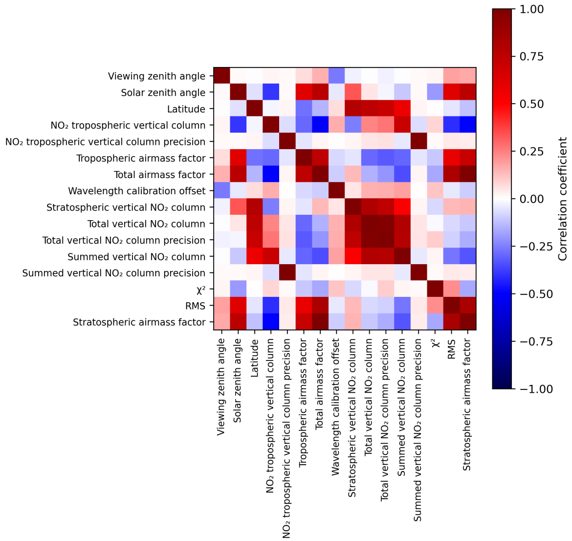
Figure 2: Map of correlation matrix for 2024-08-16 to 2024-08-17.
