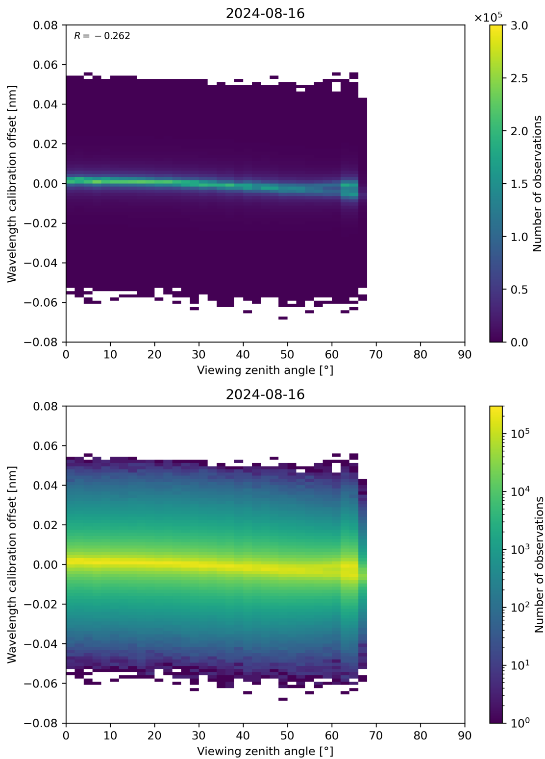
Figure 173: Scatter density plot of “Viewing zenith angle” against “Wavelength calibration offset” for 2024-08-16 to 2024-08-17.
