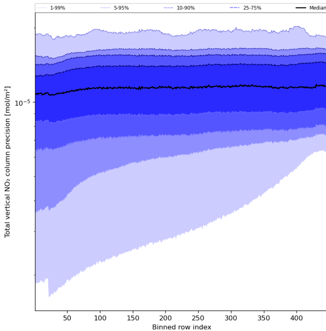
Figure 56: Along track statistics of “Total vertical NO 2 column precision” for 2024-08-16 to 2024-08-17
