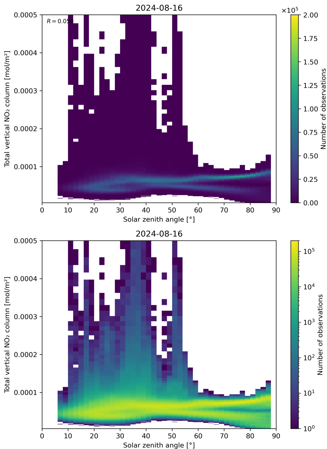
Figure 153: Scatter density plot of “Solar zenith angle” against “Total vertical NO 2 column” for 2024-08-16 to 2024-08-17.
