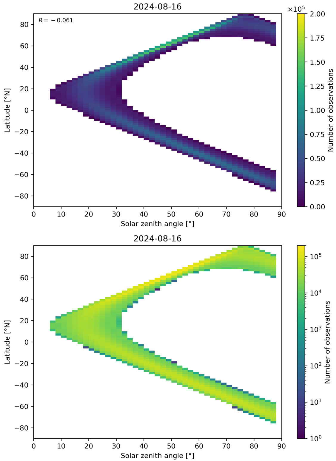
Figure 149: Scatter density plot of “Solar zenith angle” against “Latitude” for 2024-08-16 to 2024-08-17.
