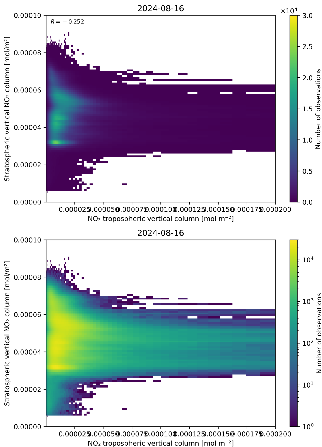
Figure 125: Scatter density plot of “NO 2 tropospheric vertical column” against “Stratospheric vertical NO 2 column” for 2024-08-16 to 2024-08-17.
