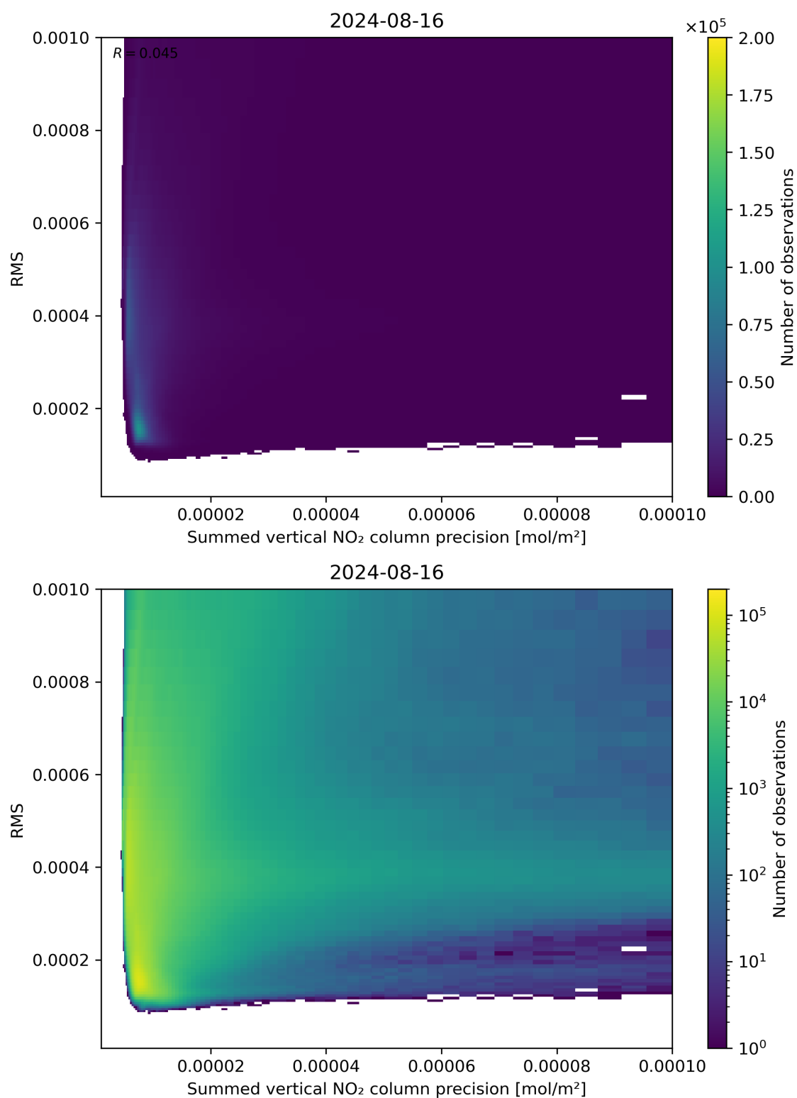
Figure 108: Scatter density plot of “Summed vertical NO 2 column precision” against “RMS” for 2024-08-16 to 2024-08-17.
