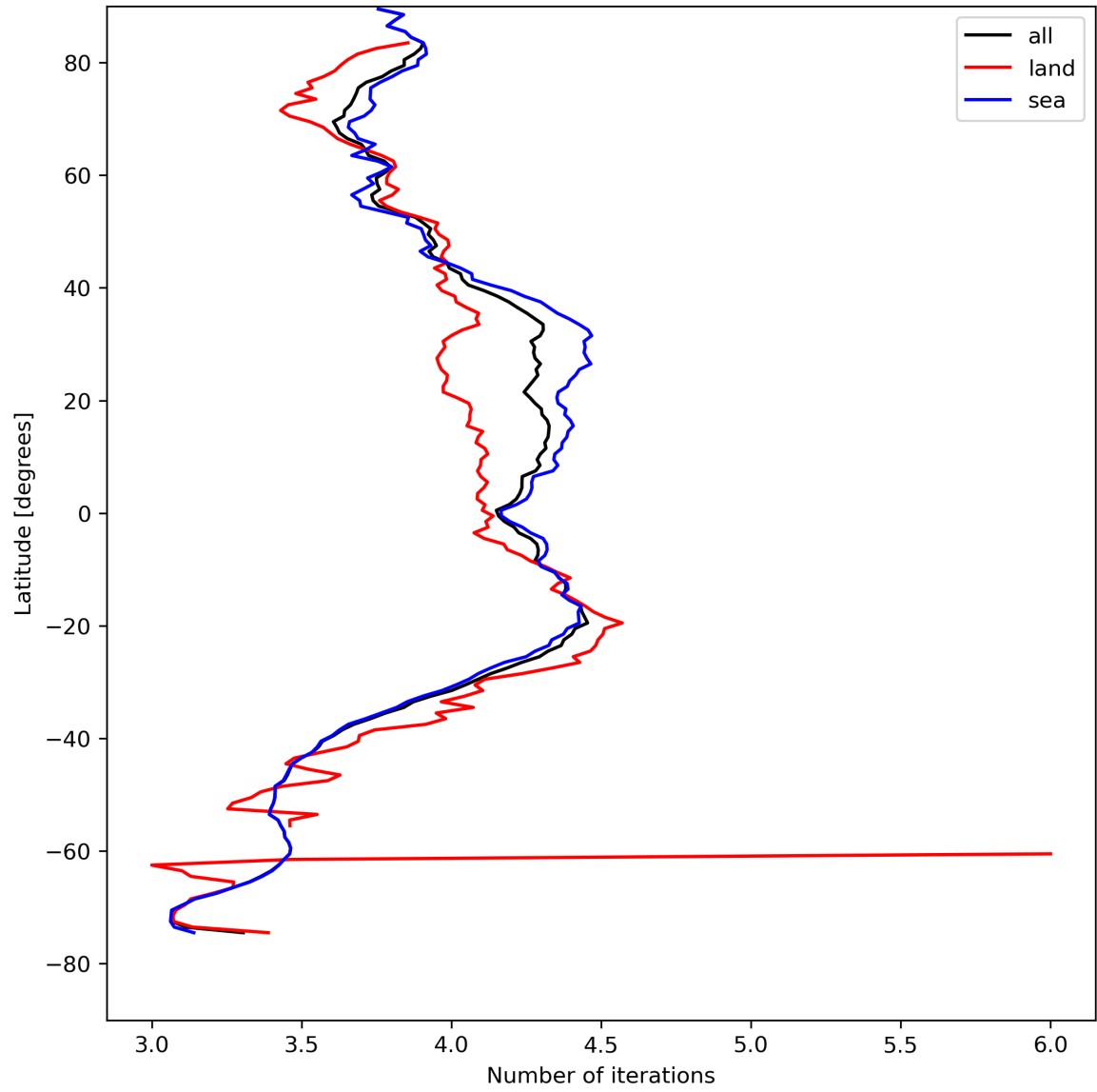
Figure 17: Zonal average of “Number of iterations” for 2024-08-16 to 2024-08-17.
