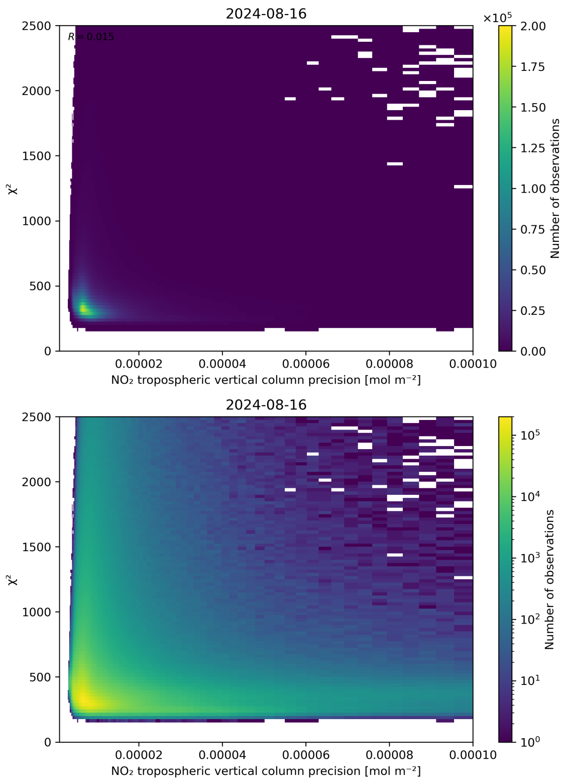
Figure 134: Scatter density plot of “NO 2 tropospheric vertical column precision” against “ \chi^2 ” for 2024-08-16 to 2024-08-17.
