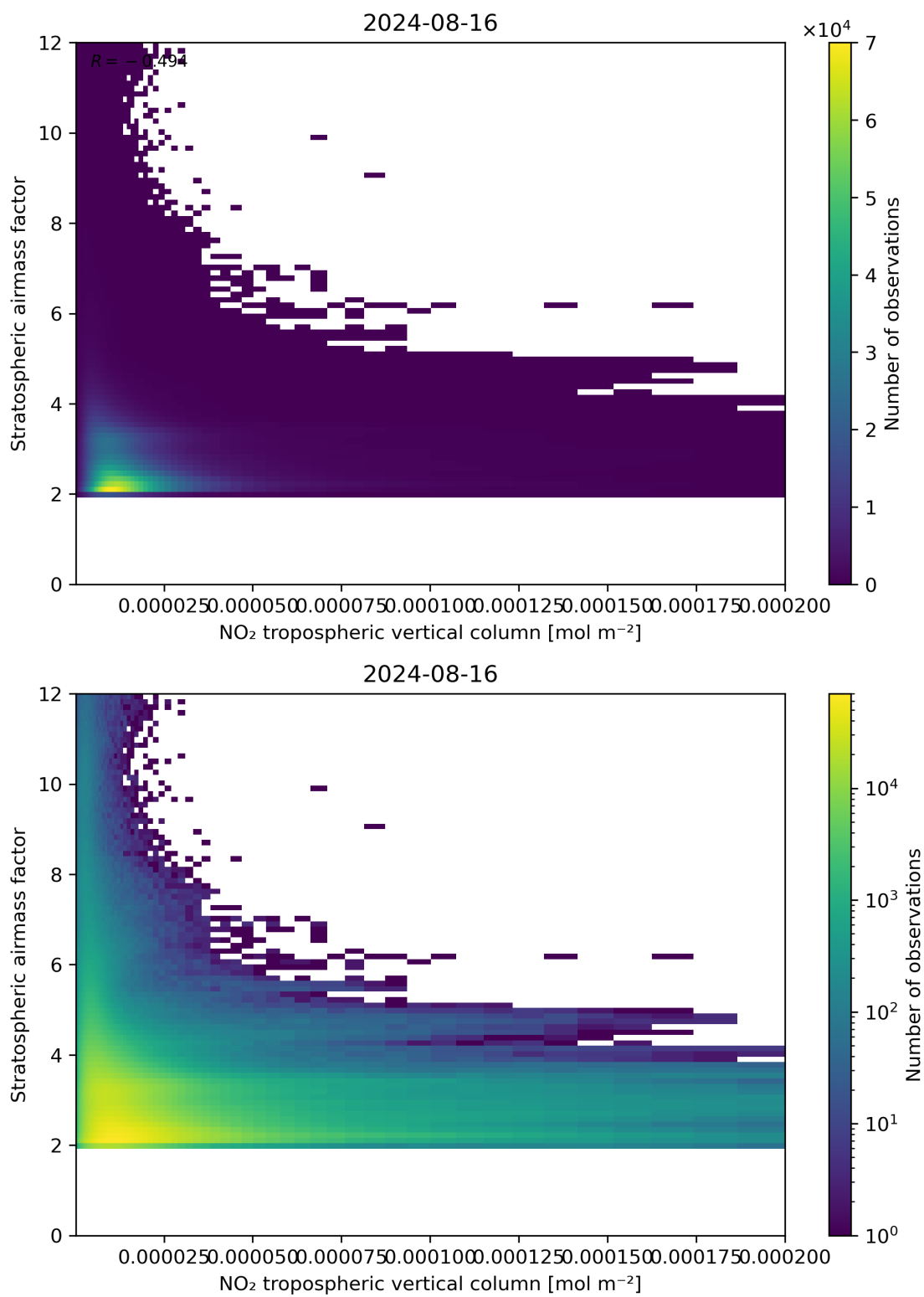
Figure 121: Scatter density plot of “NO 2 tropospheric vertical column” against “Stratospheric air mass factor” for 2024-08-16 to 2024-08-17.
