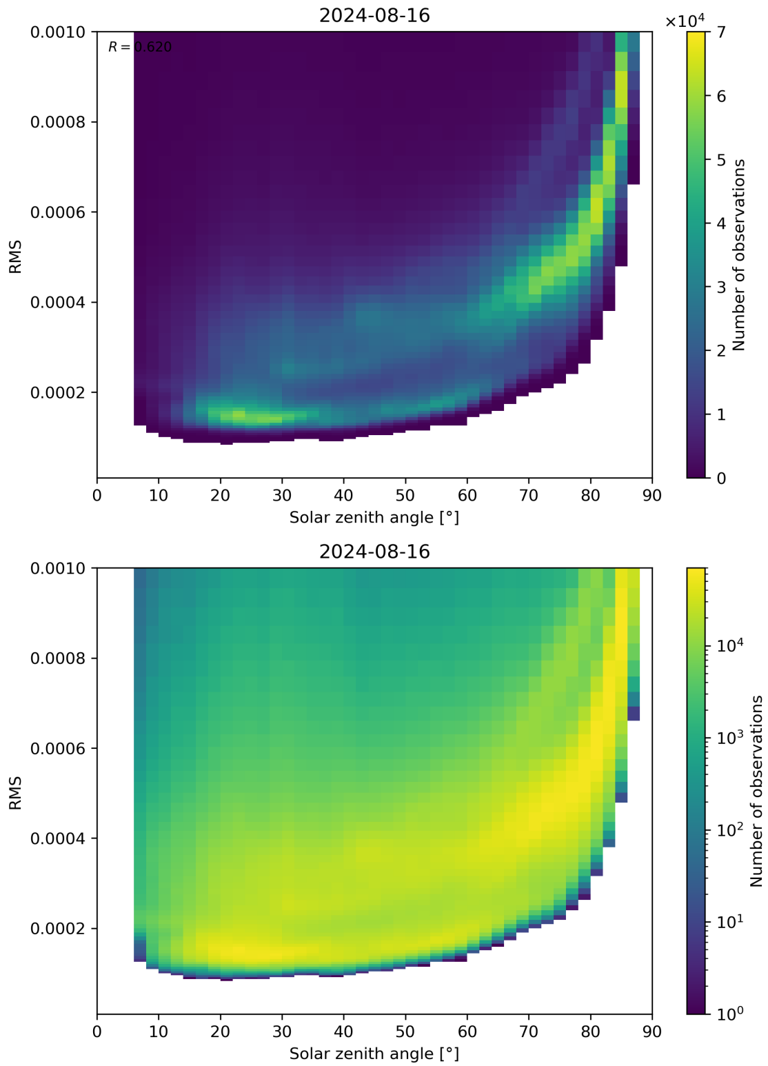
Figure 157: Scatter density plot of “Solar zenith angle” against “RMS” for 2024-08-16 to 2024-08-17.
