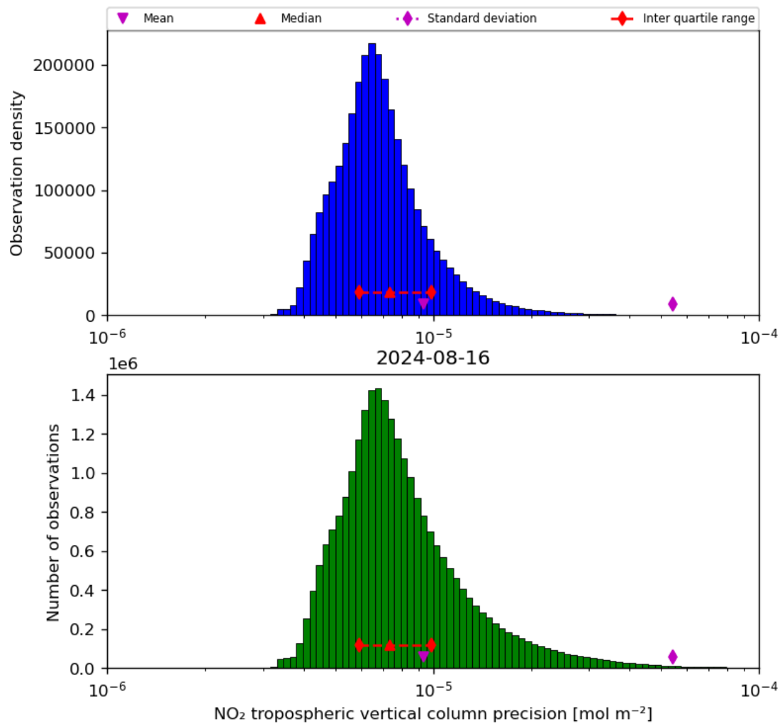
Figure 30: Histogram of “NO 2 tropospheric vertical column precision” for 2024-08-16 to 2024-08-17
