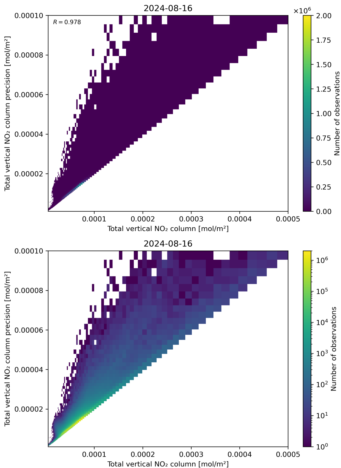
Figure 114: Scatter density plot of “Total vertical NO 2 column” against “Total vertical NO 2 column precision” for 2024-08-16 to 2024-08-17.
