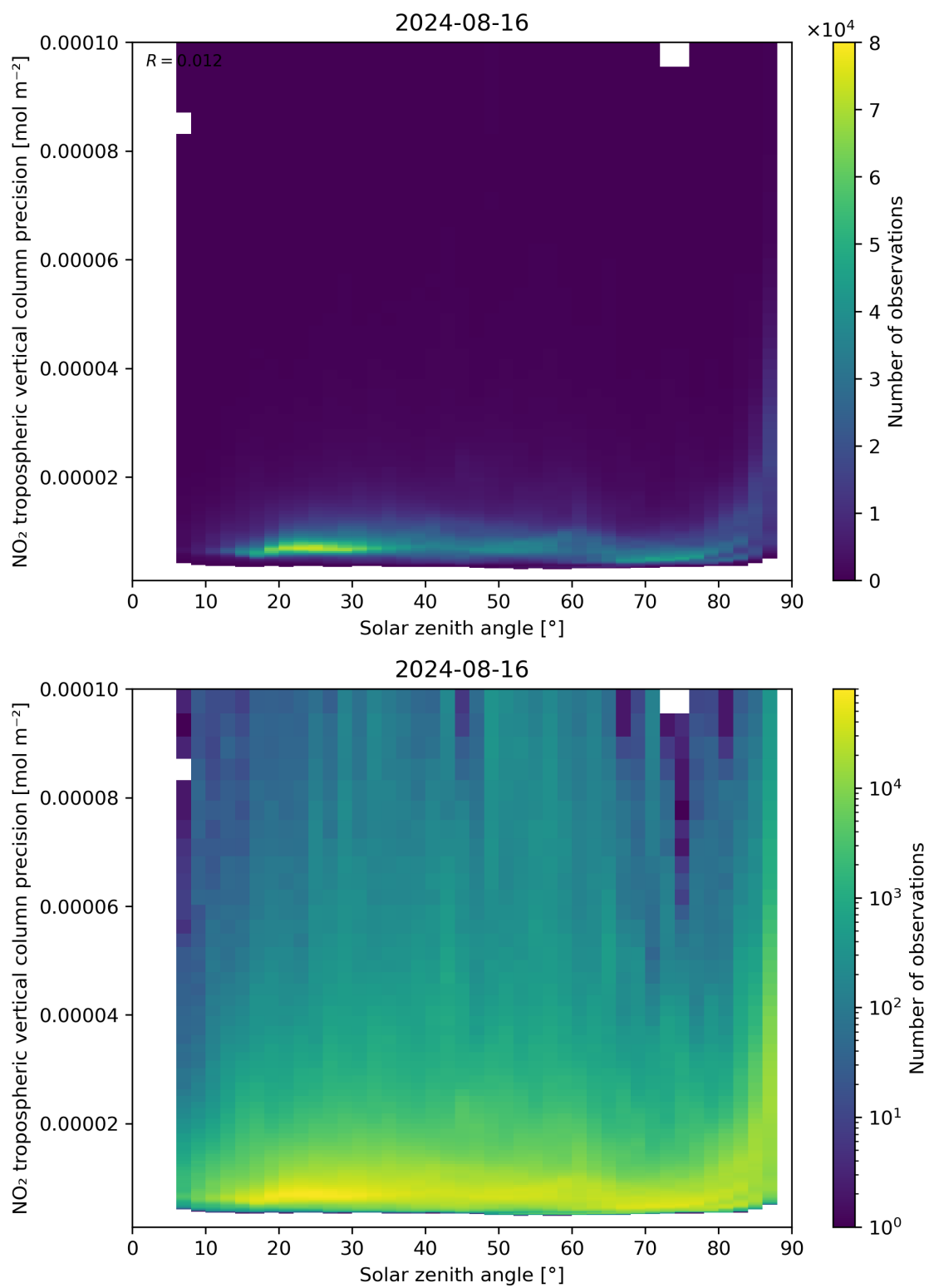
Figure 156: Scatter density plot of “Solar zenith angle” against “NO 2 tropospheric vertical column precision” for 2024-08-16 to 2024-08-17.
