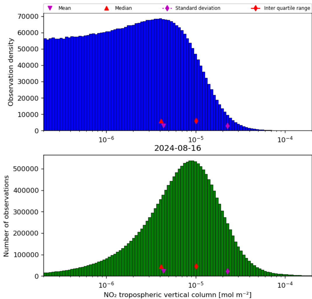
Figure 29: Histogram of “NO 2 tropospheric vertical column” for 2024-08-16 to 2024-08-17
