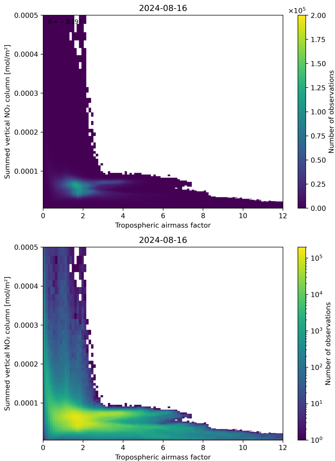
Figure 75: Scatter density plot of “Tropospheric airmass factor” against “Summed vertical NO 2 column” for 2024-08-16 to 2024-08-17.
