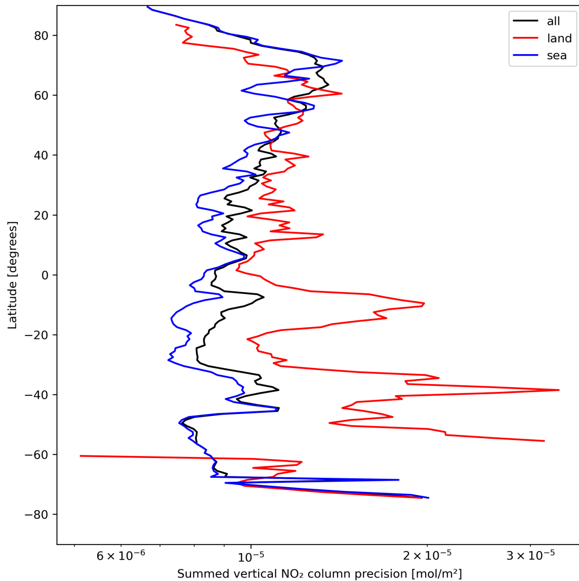
Figure 24: Zonal average of “Summed vertical NO 2 column precision” for 2024-08-16 to 2024-08-17.
