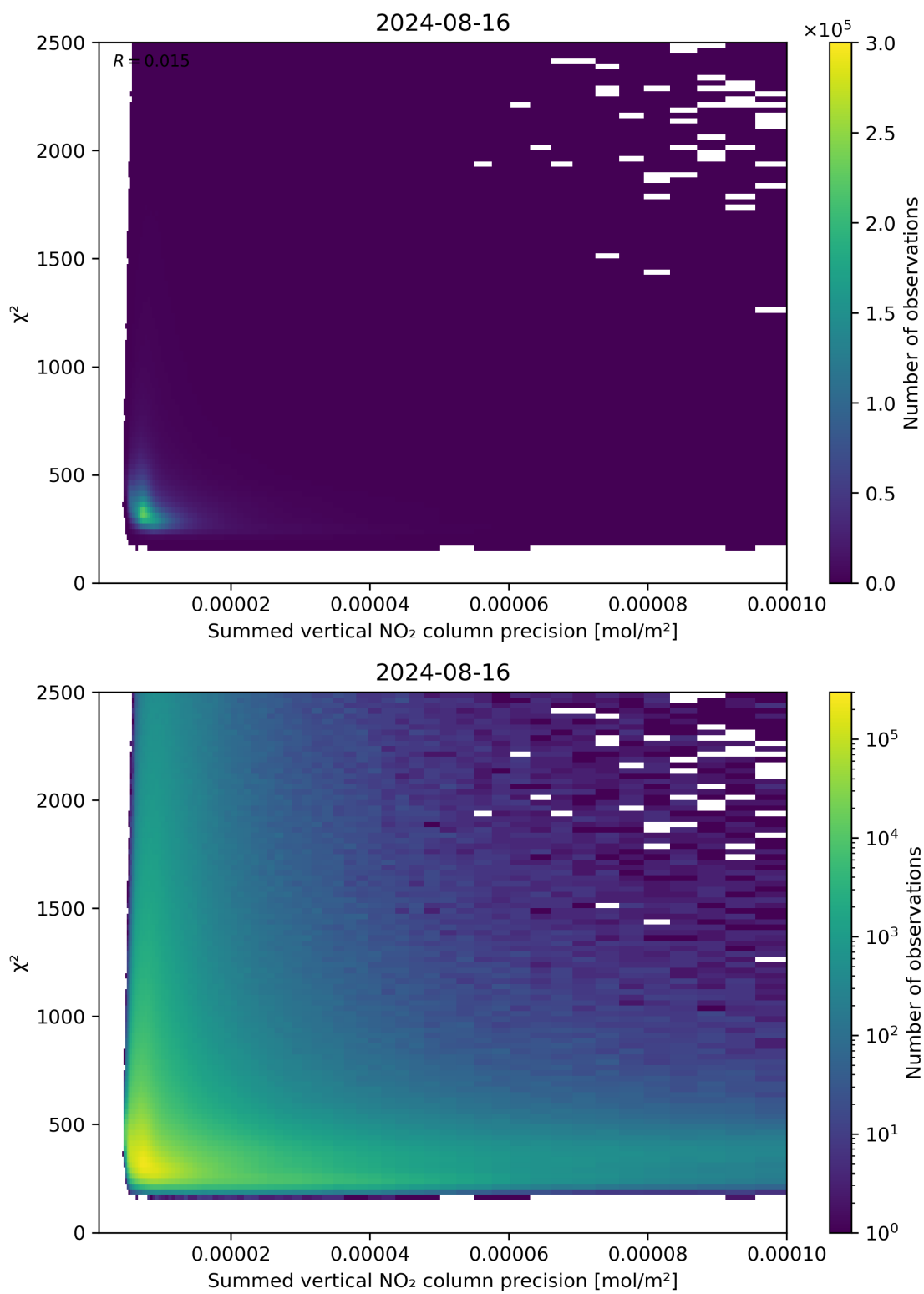
Figure 107: Scatter density plot of “Summed vertical NO 2 column precision” against “ \chi^2 ” for 2024-08-16 to 2024-08-17.
