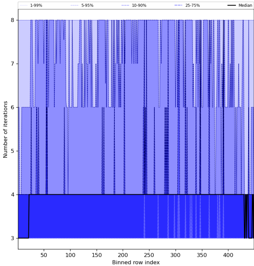
Figure 51: Along track statistics of “Number of iterations” for 2024-08-16 to 2024-08-17
