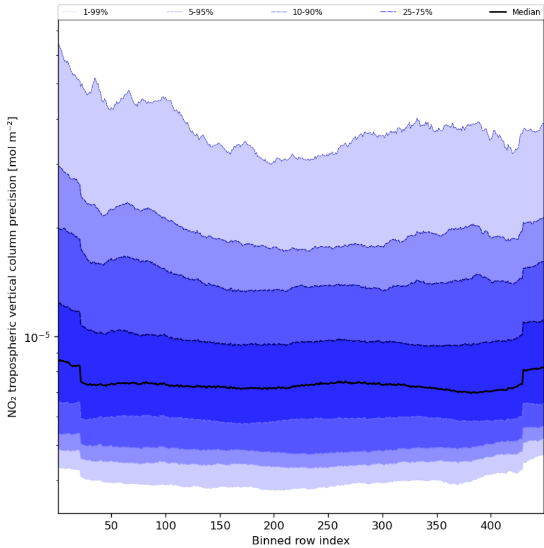
Figure 47: Along track statistics of “NO 2 tropospheric vertical column precision” for 2024-08-16 to 2024-08-17
