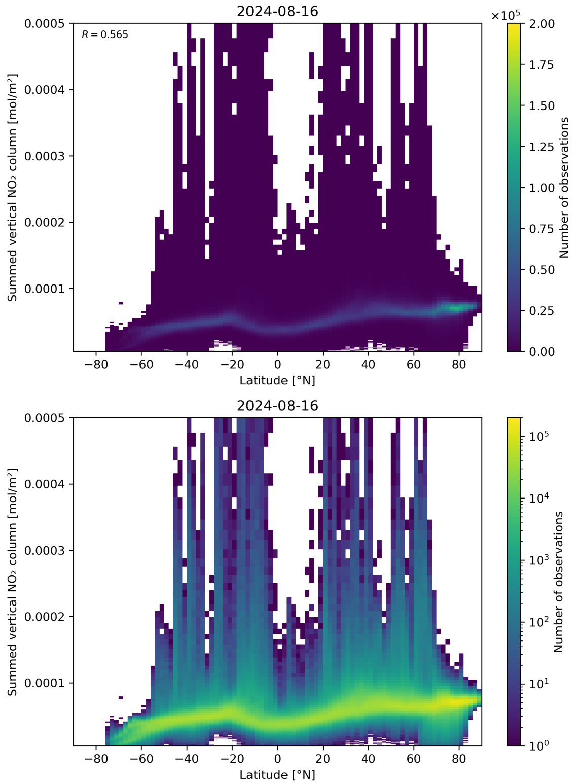
Figure 88: Scatter density plot of “Latitude” against “Summed vertical NO 2 column” for 2024-08-16 to 2024-08-17.
