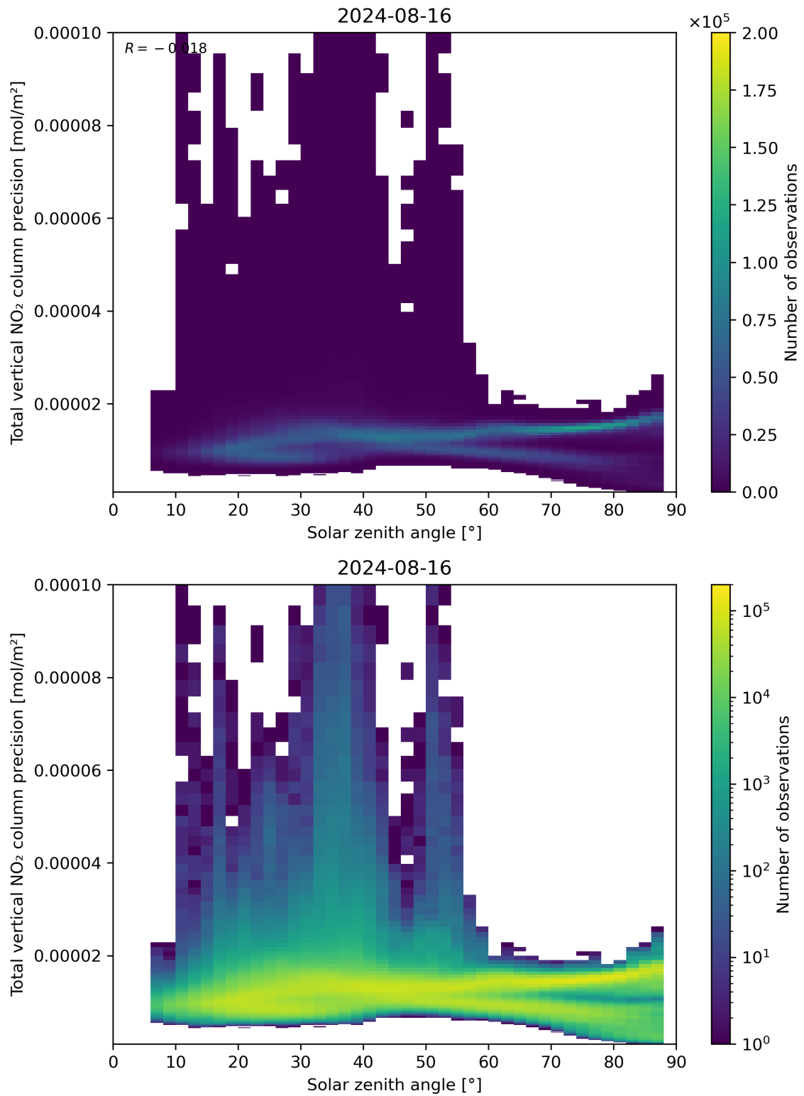
Figure 154: Scatter density plot of “Solar zenith angle” against “Total vertical NO 2 column precision” for 2024-08-16 to 2024-08-17.
