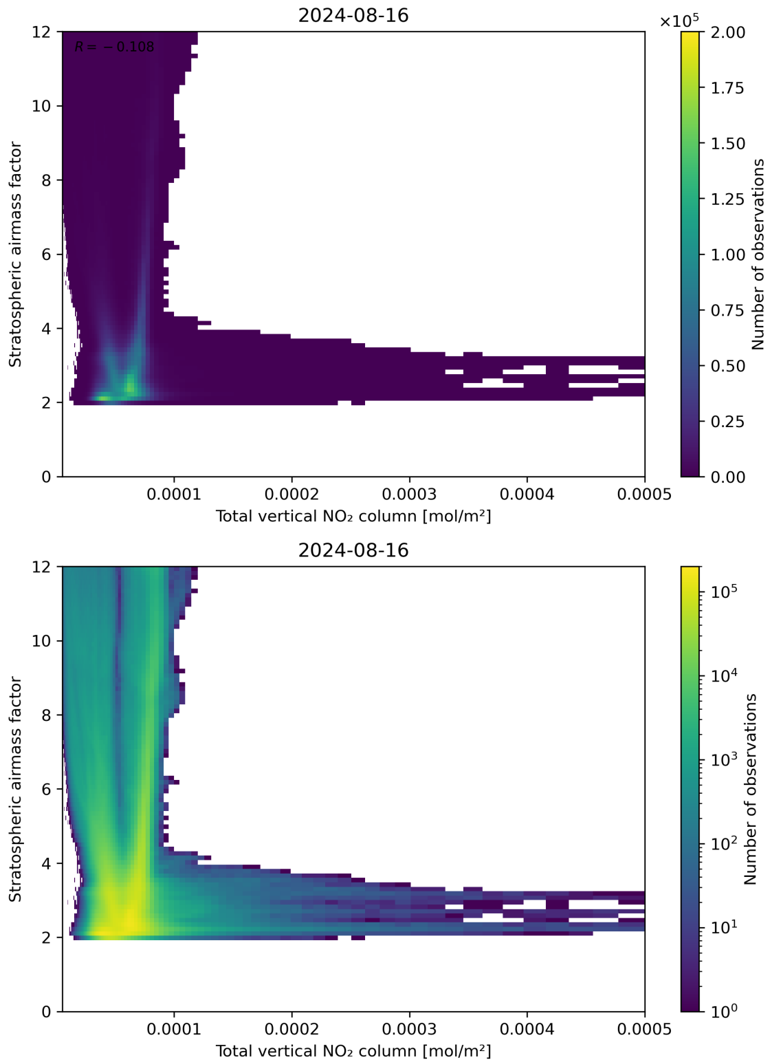
Figure 110: Scatter density plot of “Total vertical NO 2 column” against “Stratospheric airmass factor” for 2024-08-16 to 2024-08-17.
