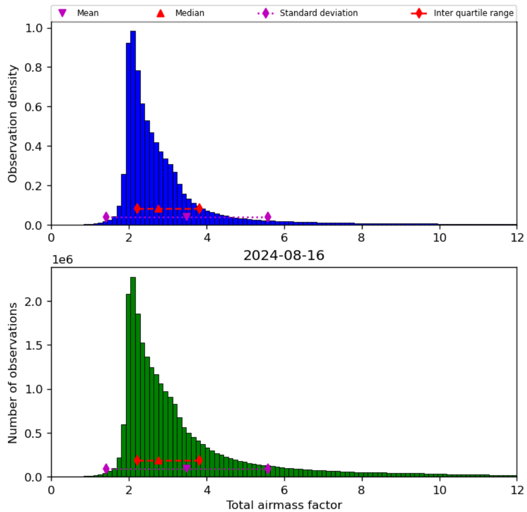
Figure 32: Histogram of “Total airmass factor” for 2024-08-16 to 2024-08-17
