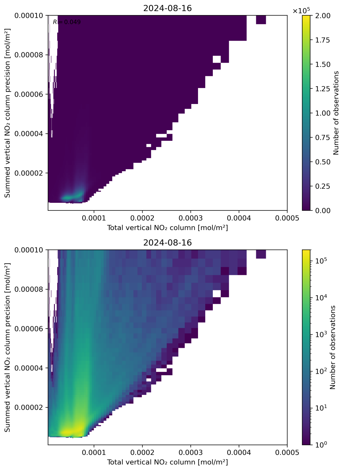
Figure 113: Scatter density plot of “Total vertical NO 2 column” against “Summed vertical NO 2 column precision” for 2024-08-16 to 2024-08-17.
