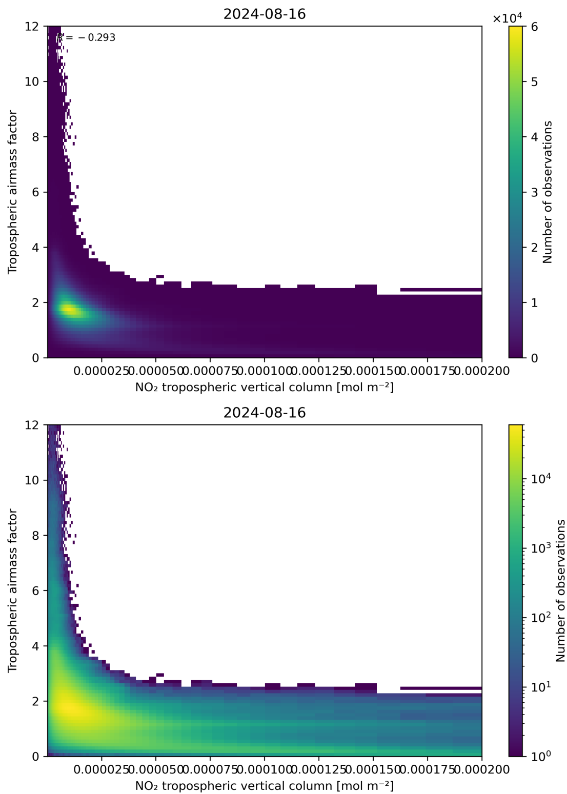
Figure 123: Scatter density plot of “NO 2 tropospheric vertical column” against “Tropospheric air mass factor” for 2024-08-16 to 2024-08-17.
