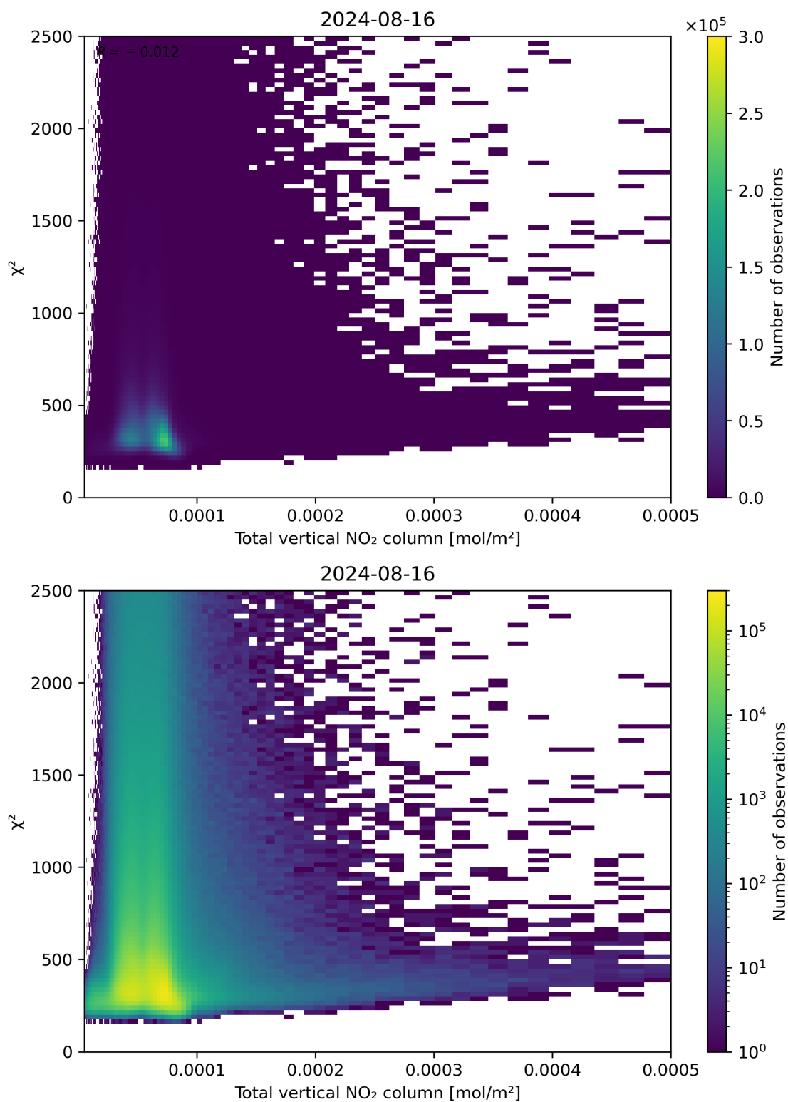
Figure 111: Scatter density plot of “Total vertical NO 2 column” against “ \chi^2 ” for 2024-08-16 to 2024-08-17.
