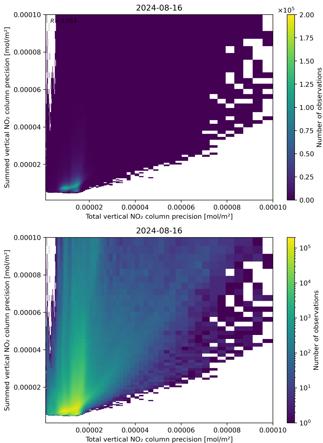
Figure 118: Scatter density plot of “Total vertical NO 2 column precision” against “Summed vertical NO 2 column precision” for 2024-08-16 to 2024-08-17.
