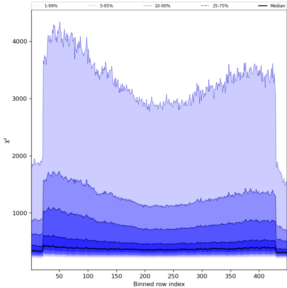
Figure 59: Along track statistics of “ \chi^2 ” for 2024-08-16 to 2024-08-17
