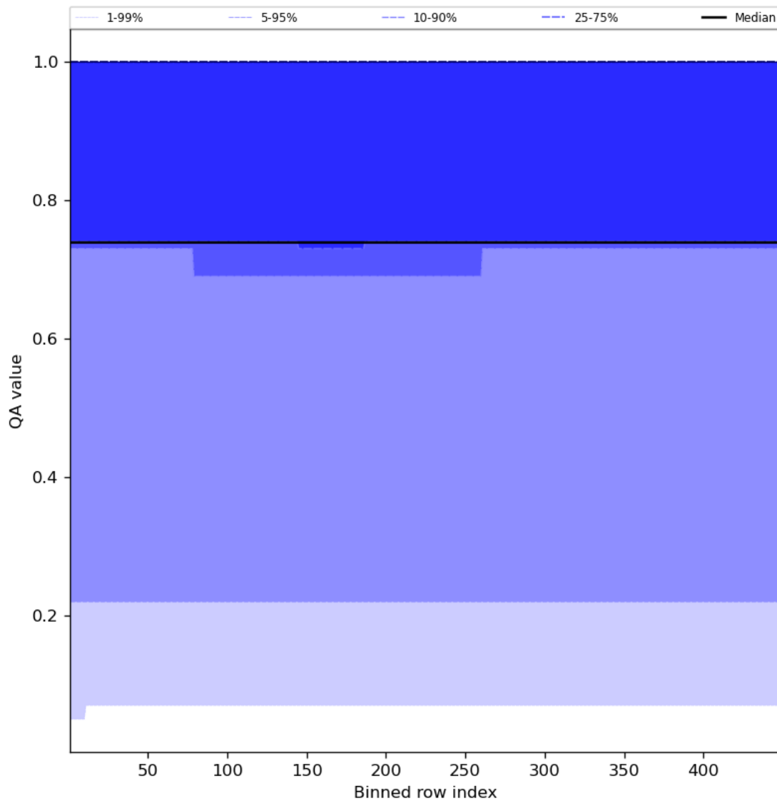
Figure 45: Along track statistics of “QA value” for 2024-08-16 to 2024-08-17
