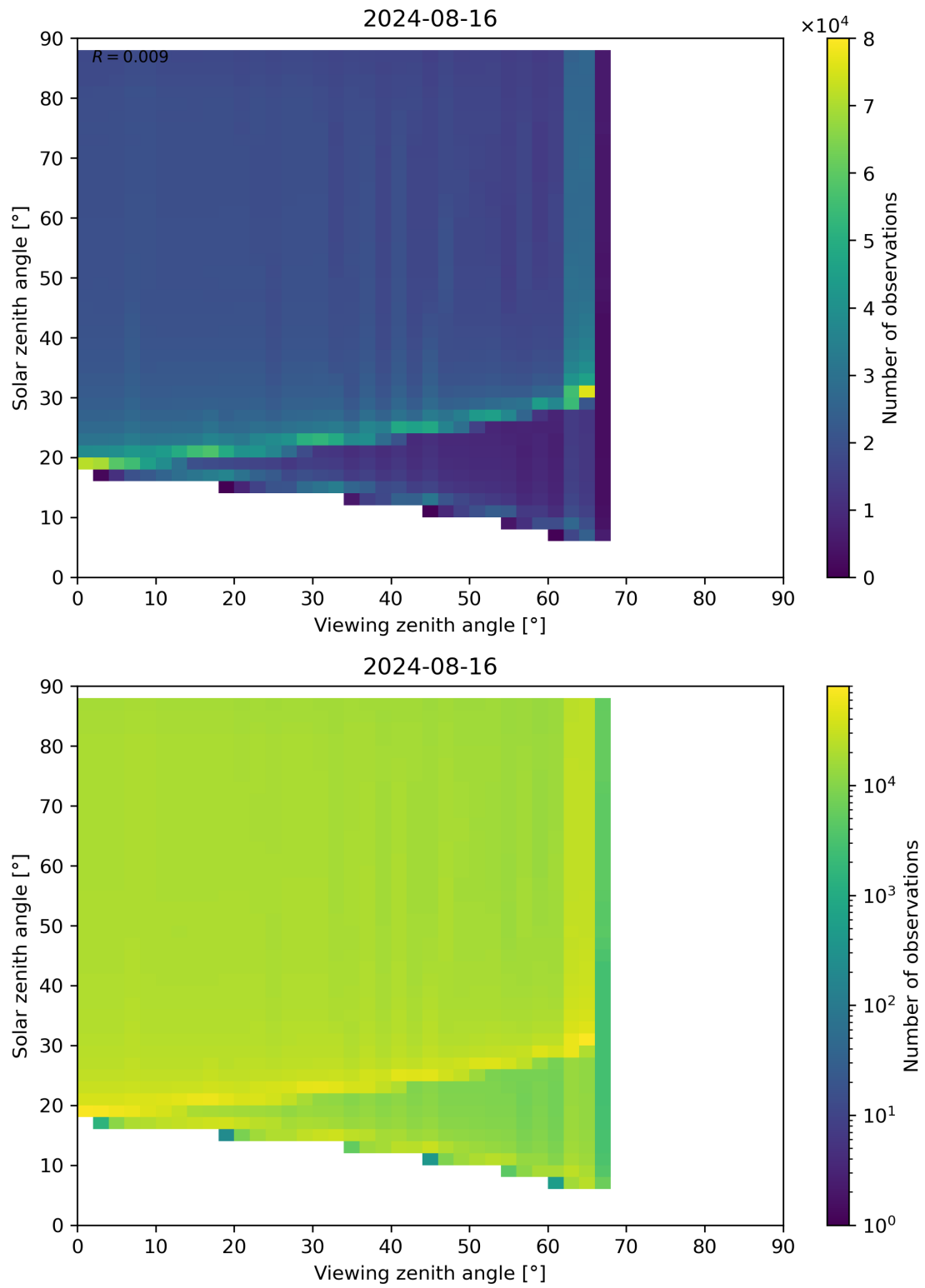
Figure 172: Scatter density plot of “Viewing zenith angle” against “Solar zenith angle” for 2024-08-16 to 2024-08-17.
