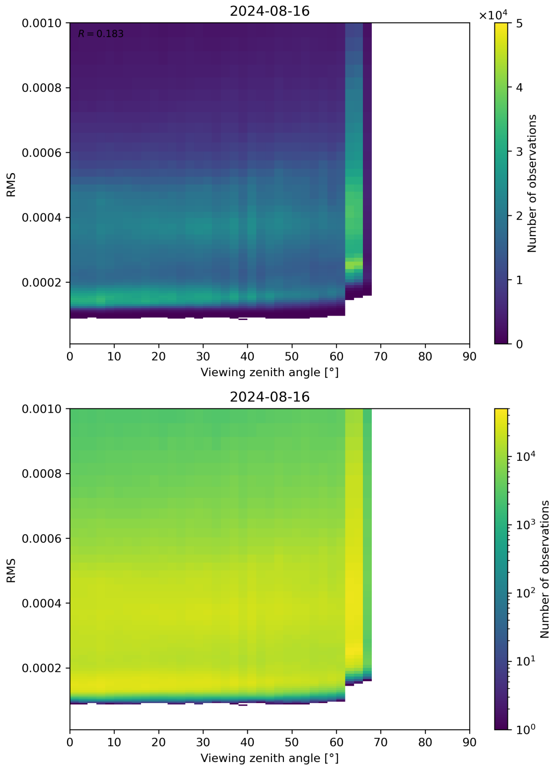
Figure 171: Scatter density plot of “Viewing zenith angle” against “RMS” for 2024-08-16 to 2024-08-17.
