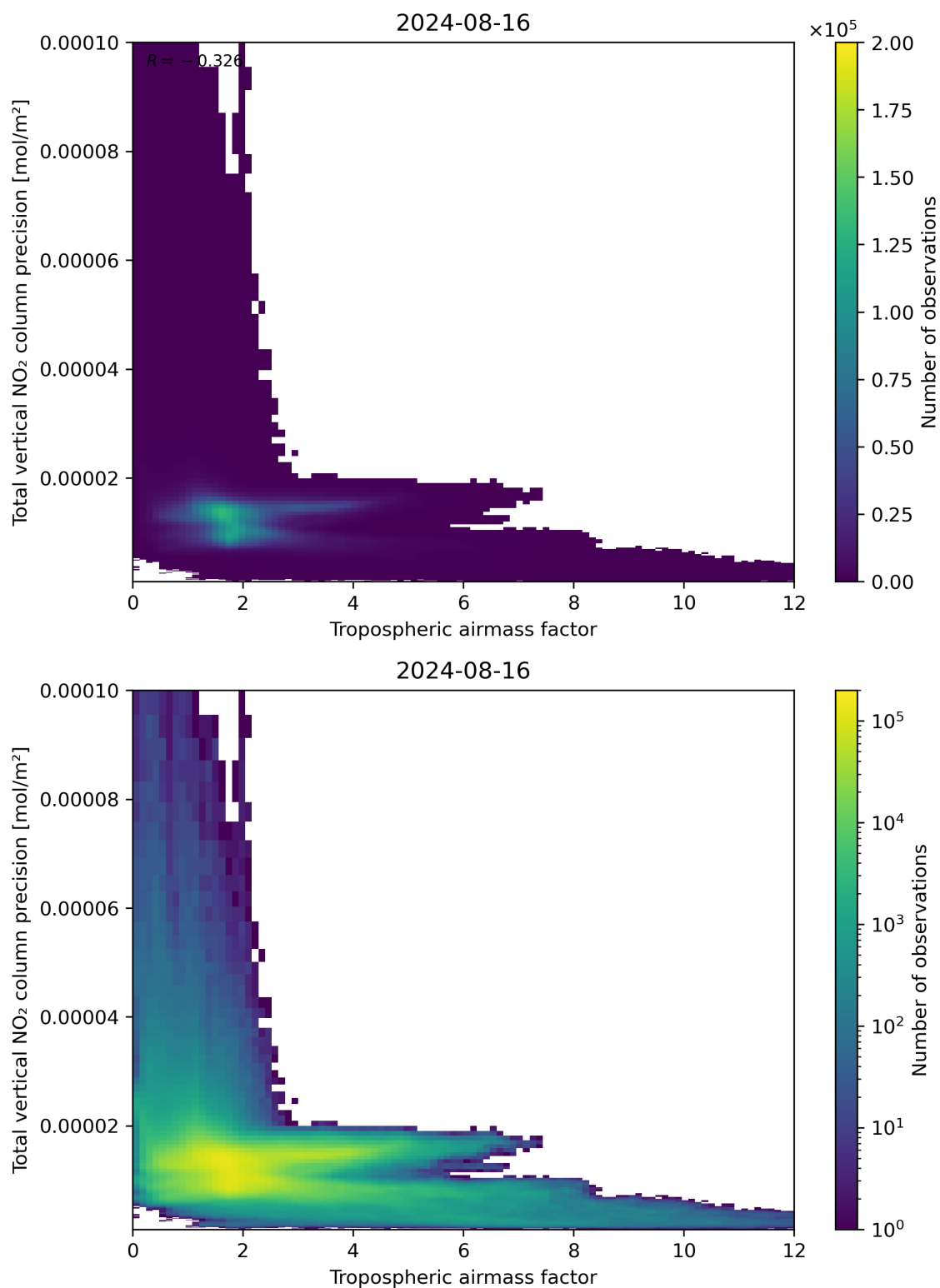
Figure 78: Scatter density plot of “Tropospheric air mass factor” against “Total vertical NO 2 column precision” for 2024-08-16 to 2024-08-17.
