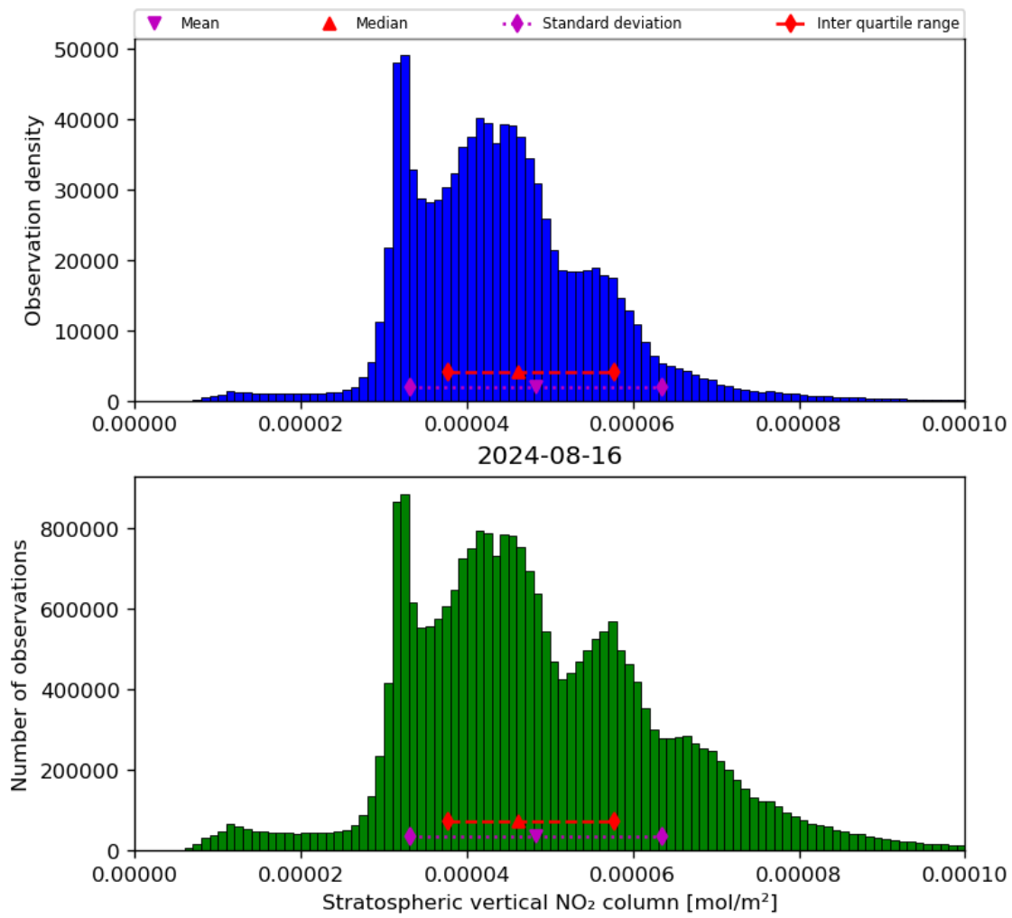
Figure 36: Histogram of “Stratospheric vertical NO 2 column” for 2024-08-16 to 2024-08-17
