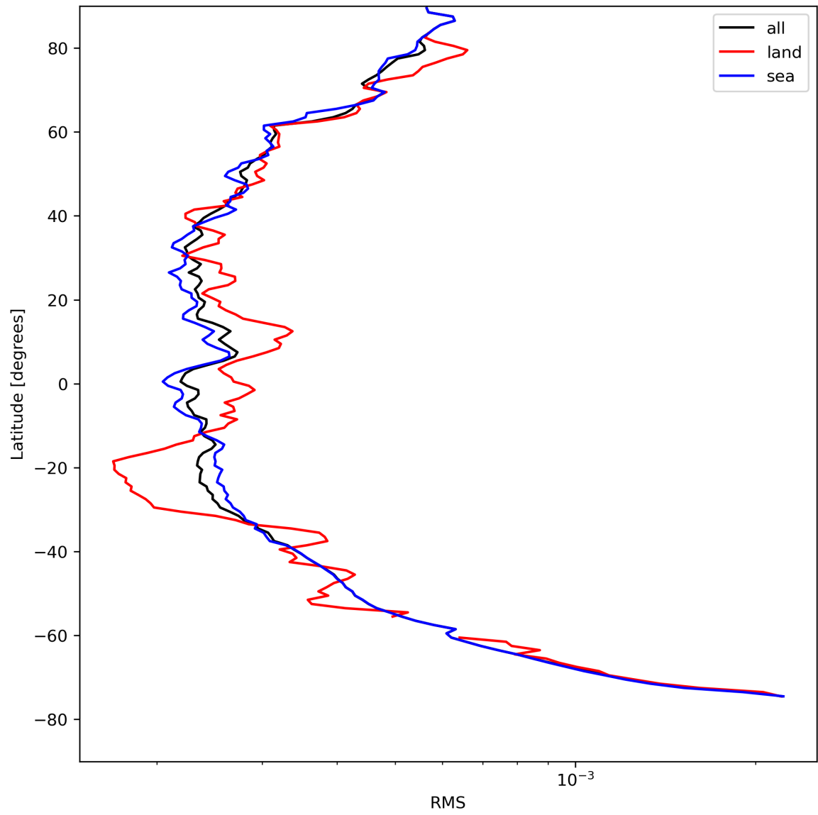
Figure 26: Zonal average of “RMS” for 2024-08-16 to 2024-08-17.
