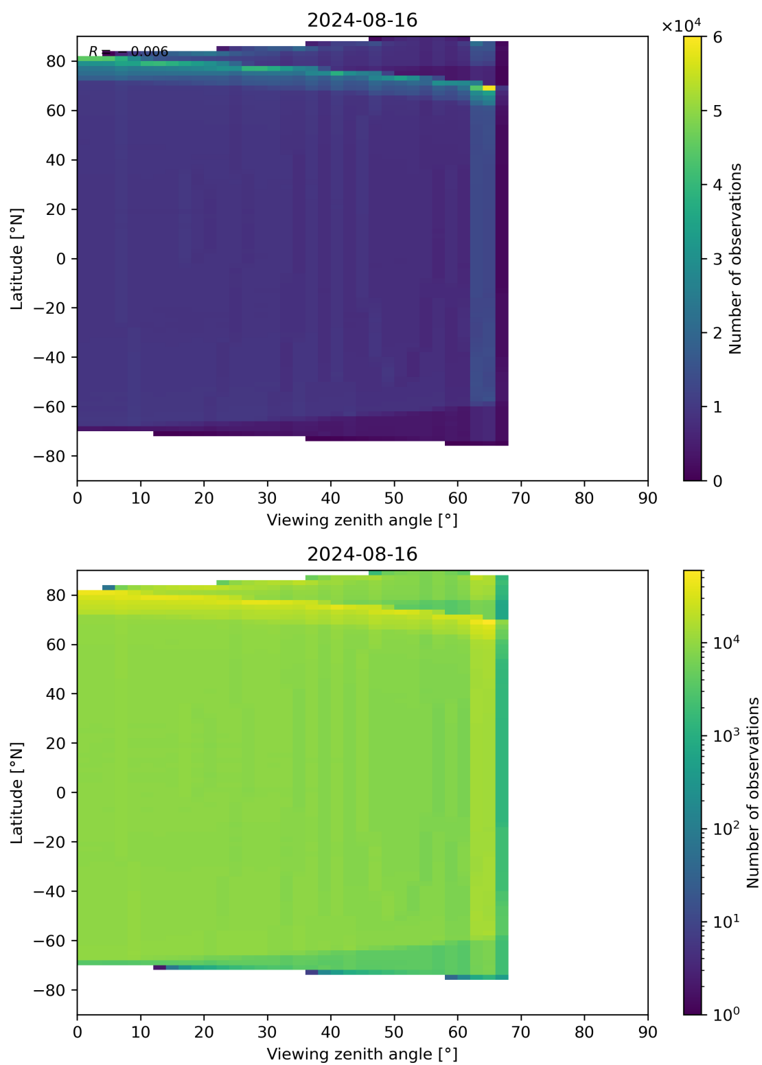
Figure 163: Scatter density plot of “Viewing zenith angle” against “Latitude” for 2024-08-16 to 2024-08-17.
