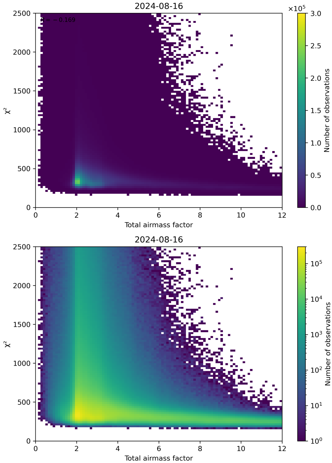
Figure 63: Scatter density plot of “Total airmass factor” against “ \chi^2 ” for 2024-08-16 to 2024-08-17.
