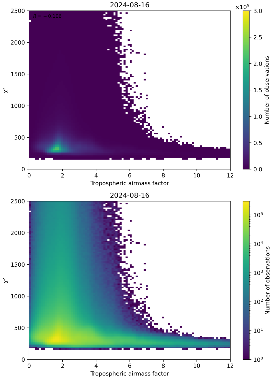
Figure 73: Scatter density plot of “Tropospheric airmass factor” against “ \chi^2 ” for 2024-08-16 to 2024-08-17.
