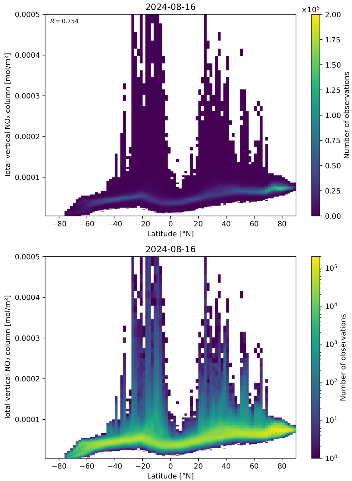
Figure 90: Scatter density plot of “Latitude” against “Total vertical NO 2 column” for 2024-08-16 to 2024-08-17.
