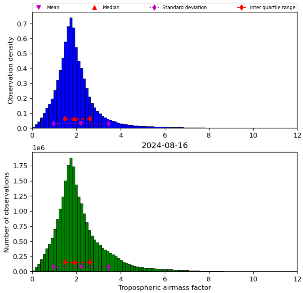
Figure 31: Histogram of “Tropospheric airmass factor” for 2024-08-16 to 2024-08-17
