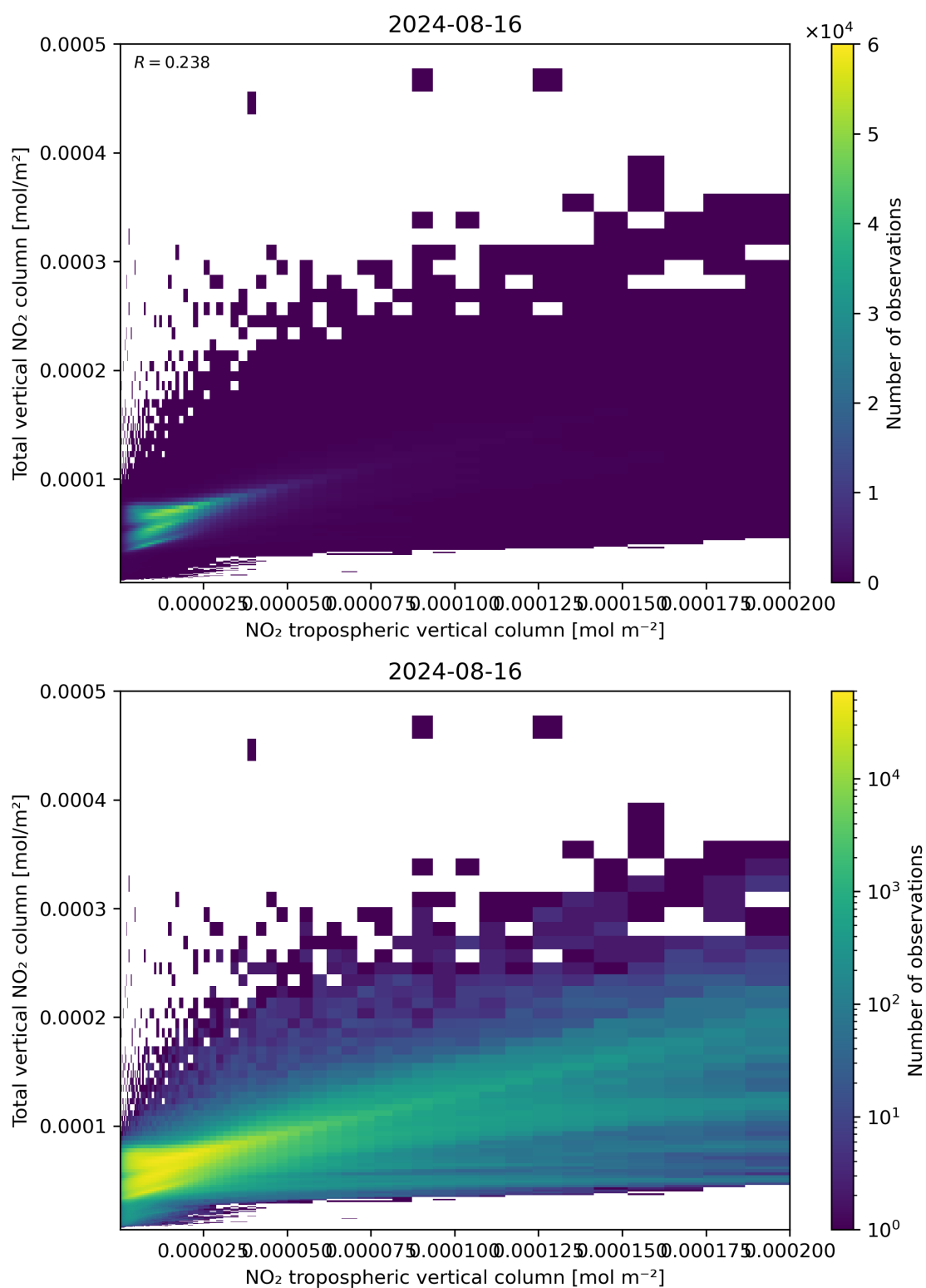
Figure 128: Scatter density plot of “NO 2 tropospheric vertical column” against “Total vertical NO 2 column” for 2024-08-16 to 2024-08-17.
