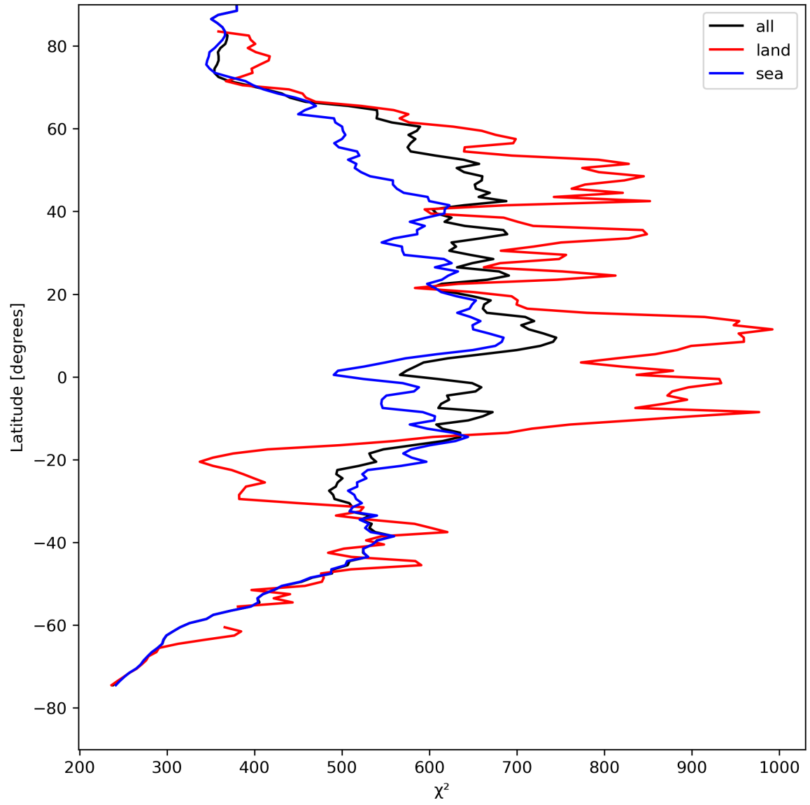
Figure 25: Zonal average of “ \chi^2 ” for 2024-08-16 to 2024-08-17.
