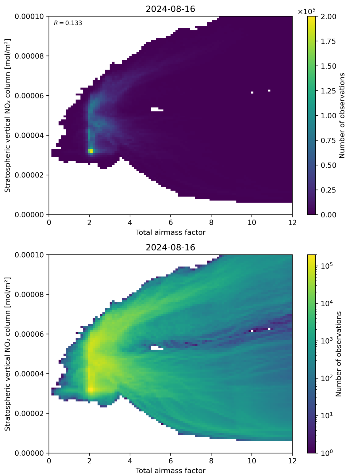
Figure 64: Scatter density plot of “Total airmass factor” against “Stratospheric vertical NO 2 column” for 2024-08-16 to 2024-08-17.
