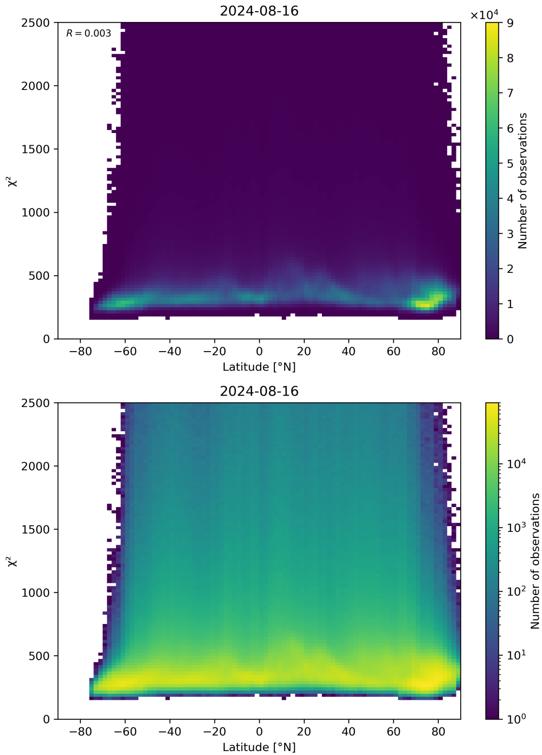
Figure 86: Scatter density plot of “Latitude” against “ \chi^2 ” for 2024-08-16 to 2024-08-17.
