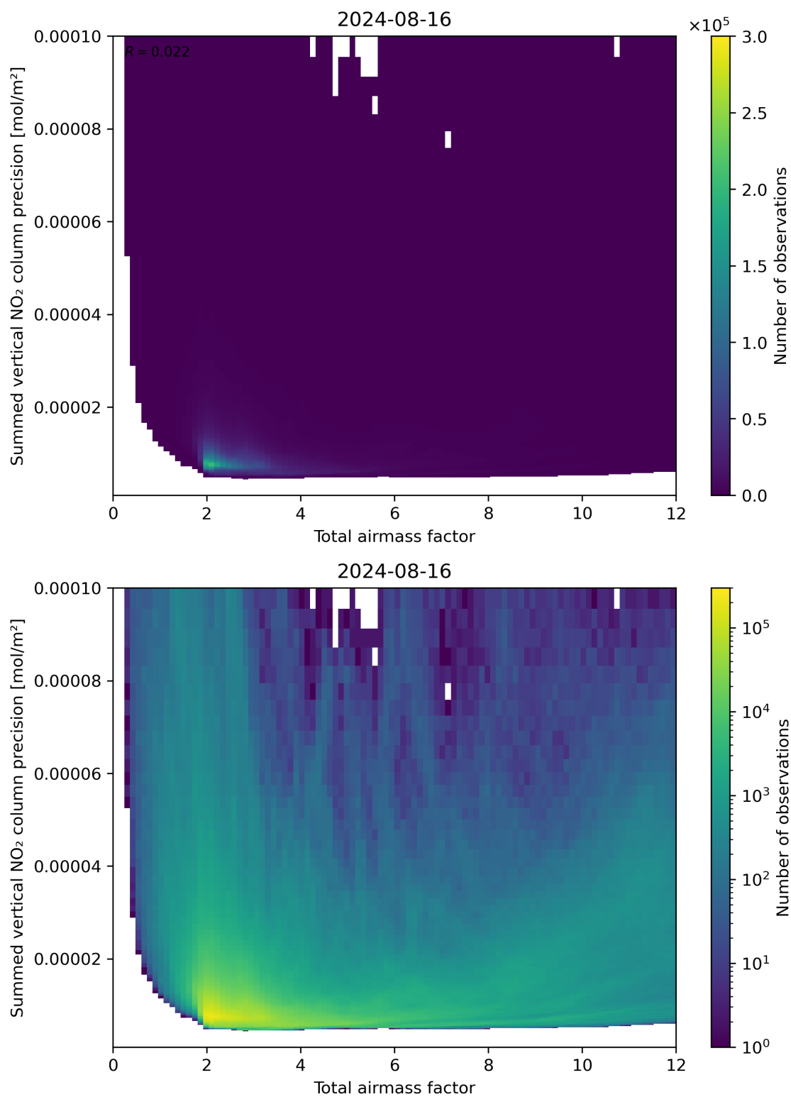
Figure 66: Scatter density plot of “Total airmass factor” against “Summed vertical NO 2 column precision” for 2024-08-16 to 2024-08-17.
