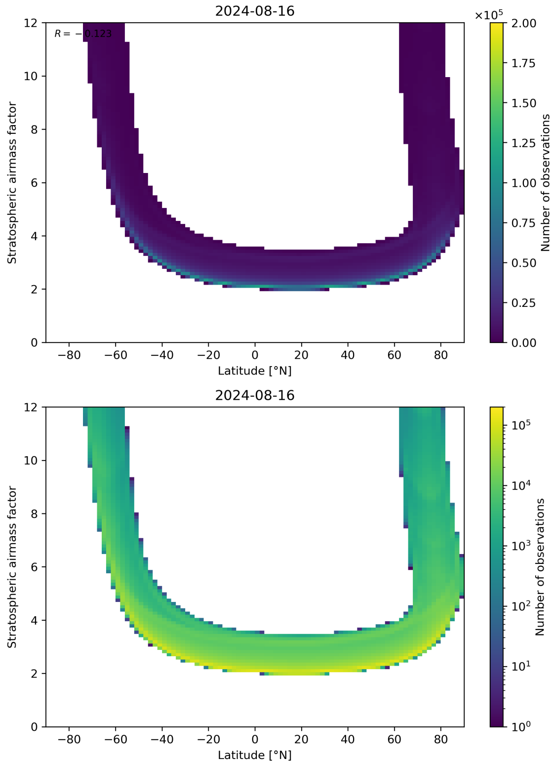
Figure 83: Scatter density plot of “Latitude” against “Stratospheric air mass factor” for 2024-08-16 to 2024-08-17.
