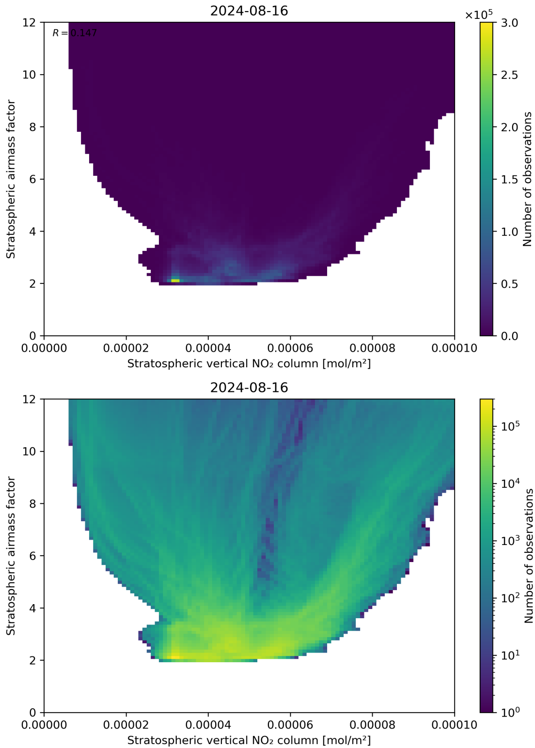
Figure 96: Scatter density plot of “Stratospheric vertical NO 2 column” against “Stratospheric airmass factor” for 2024-08-16 to 2024-08-17.
