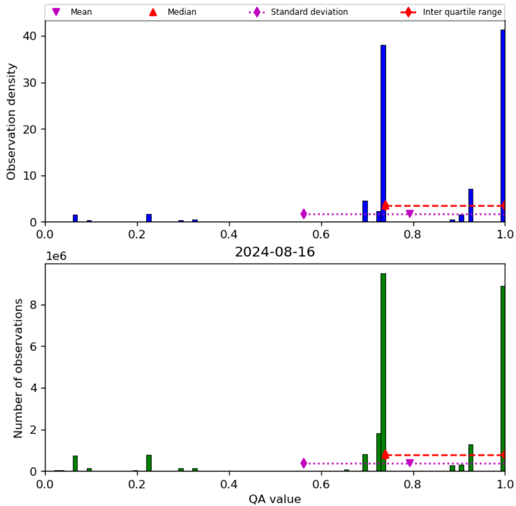
Figure 28: Histogram of “QA value” for 2024-08-16 to 2024-08-17
