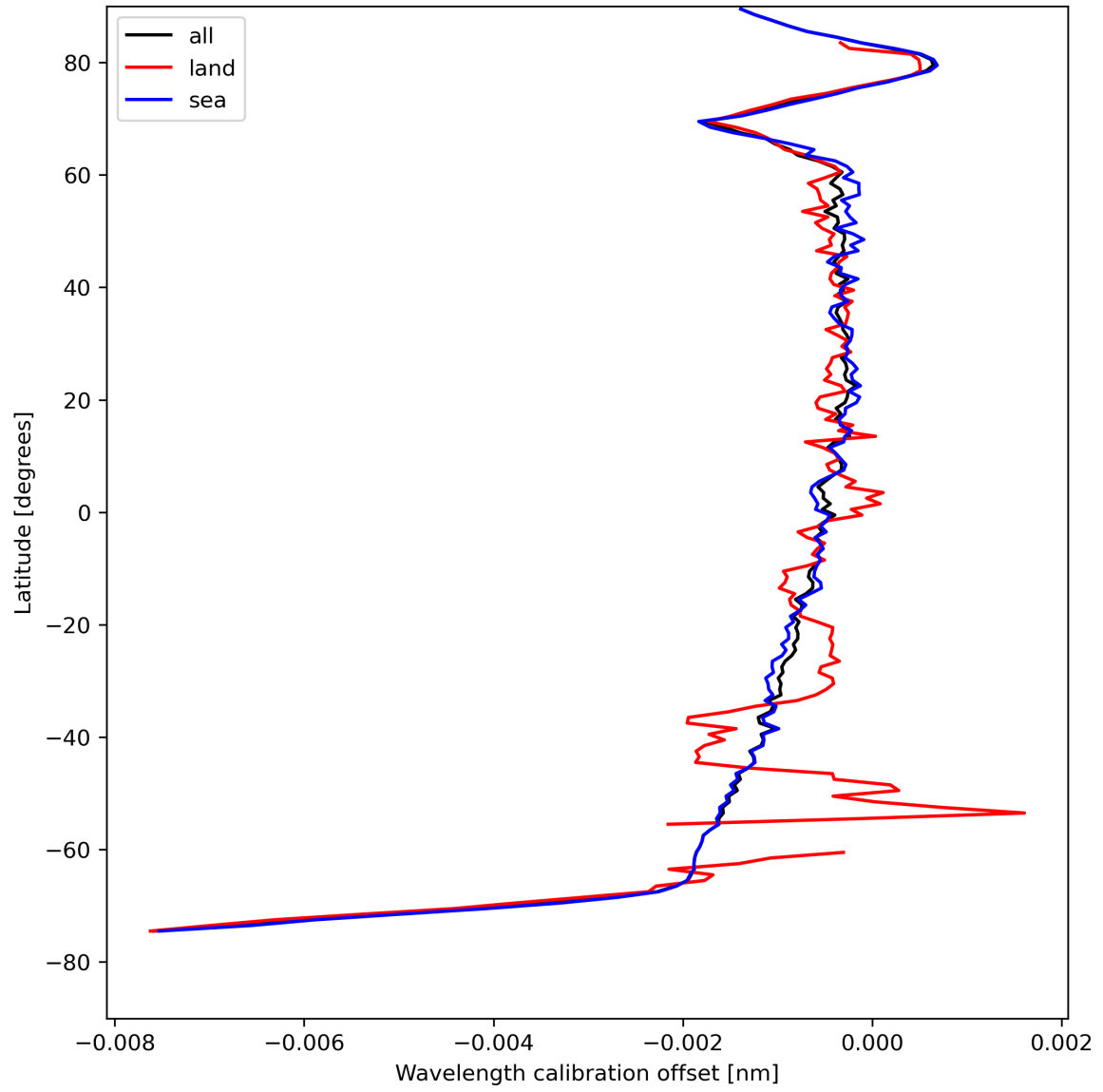
Figure 18: Zonal average of “Wavelength calibration offset” for 2024-08-16 to 2024-08-17.
