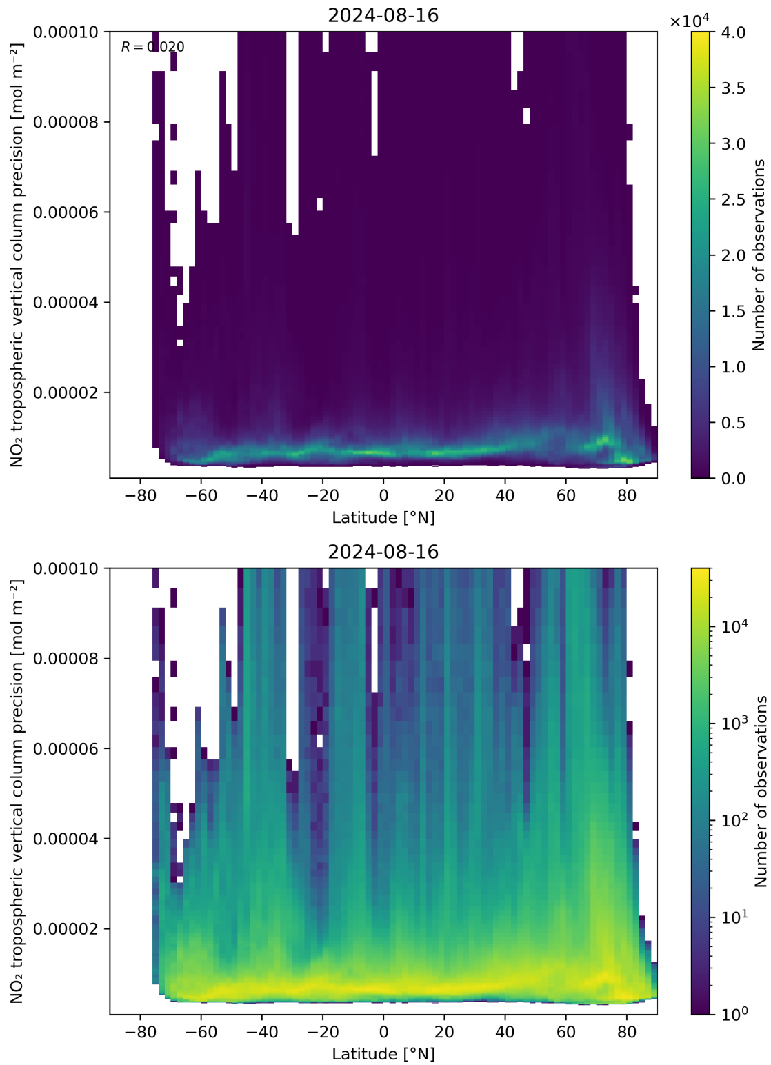
Figure 93: Scatter density plot of “Latitude” against “NO 2 tropospheric vertical column precision” for 2024-08-16 to 2024-08-17.
