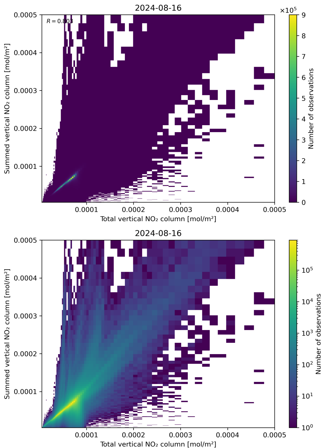
Figure 112: Scatter density plot of “Total vertical NO 2 column” against “Summed vertical NO 2 column” for 2024-08-16 to 2024-08-17.
