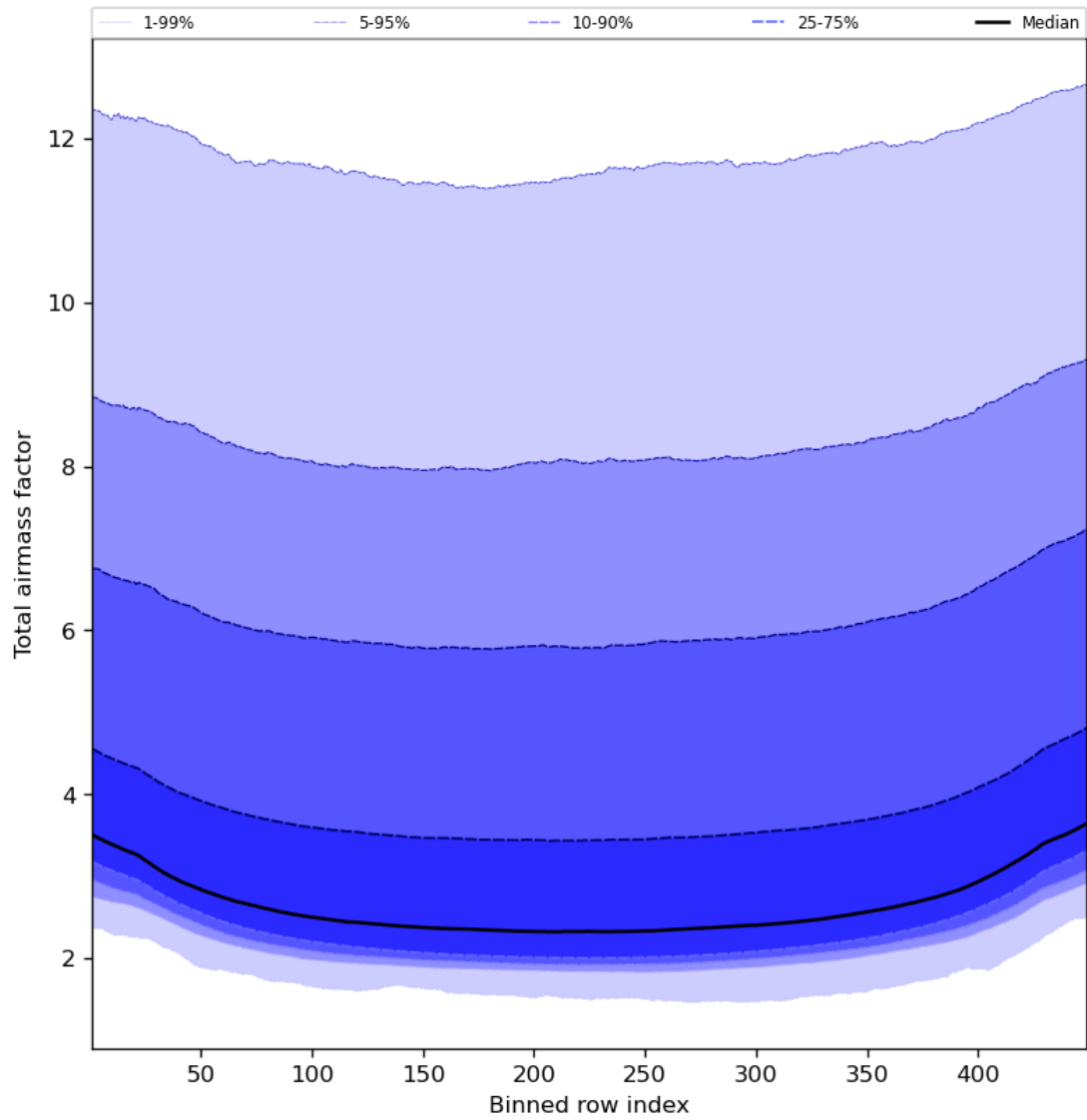
Figure 49: Along track statistics of “Total airmass factor” for 2024-08-16 to 2024-08-17
