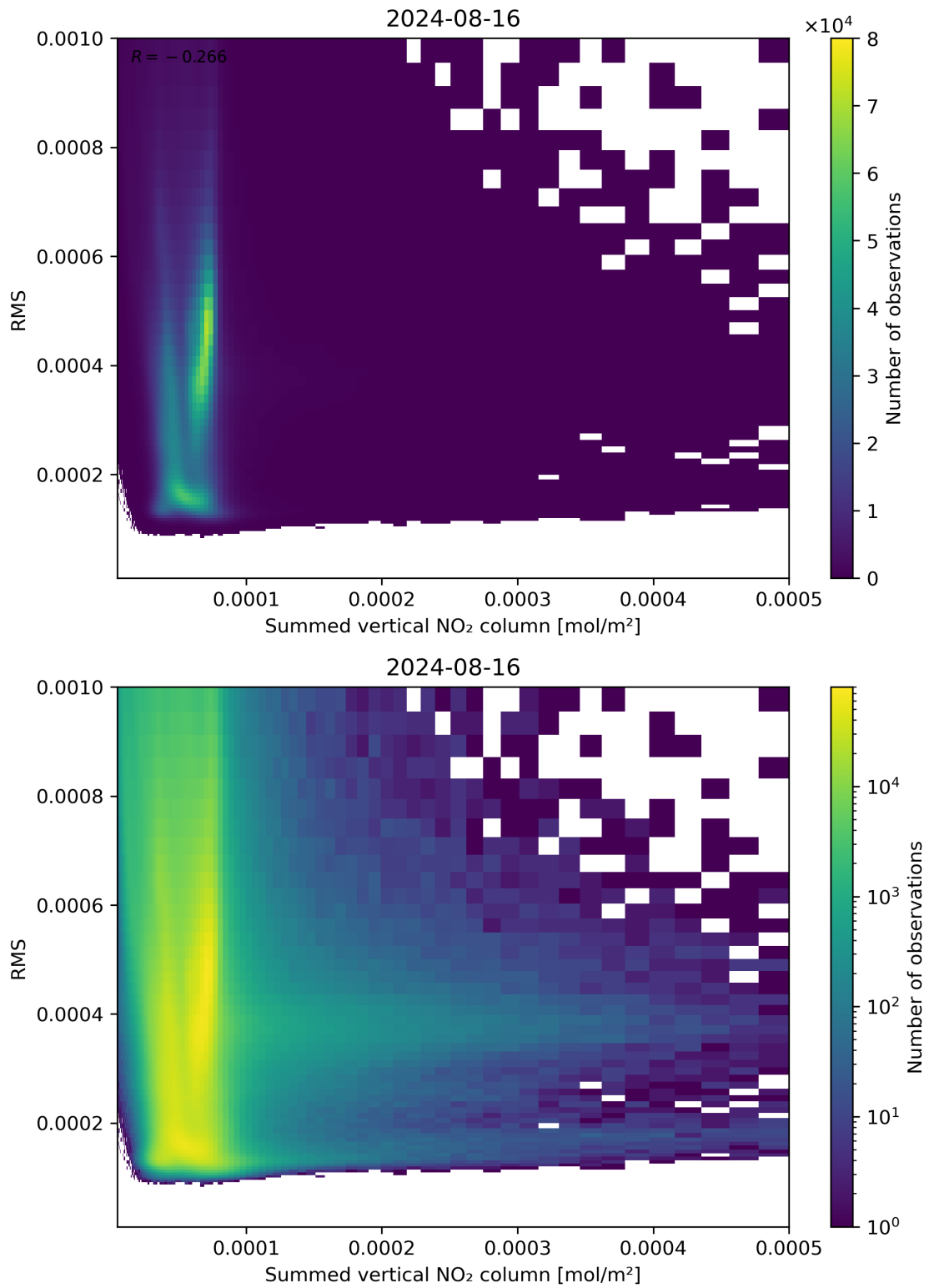
Figure 109: Scatter density plot of “Summed vertical NO 2 column” against “RMS” for 2024-08-16 to 2024-08-17.
