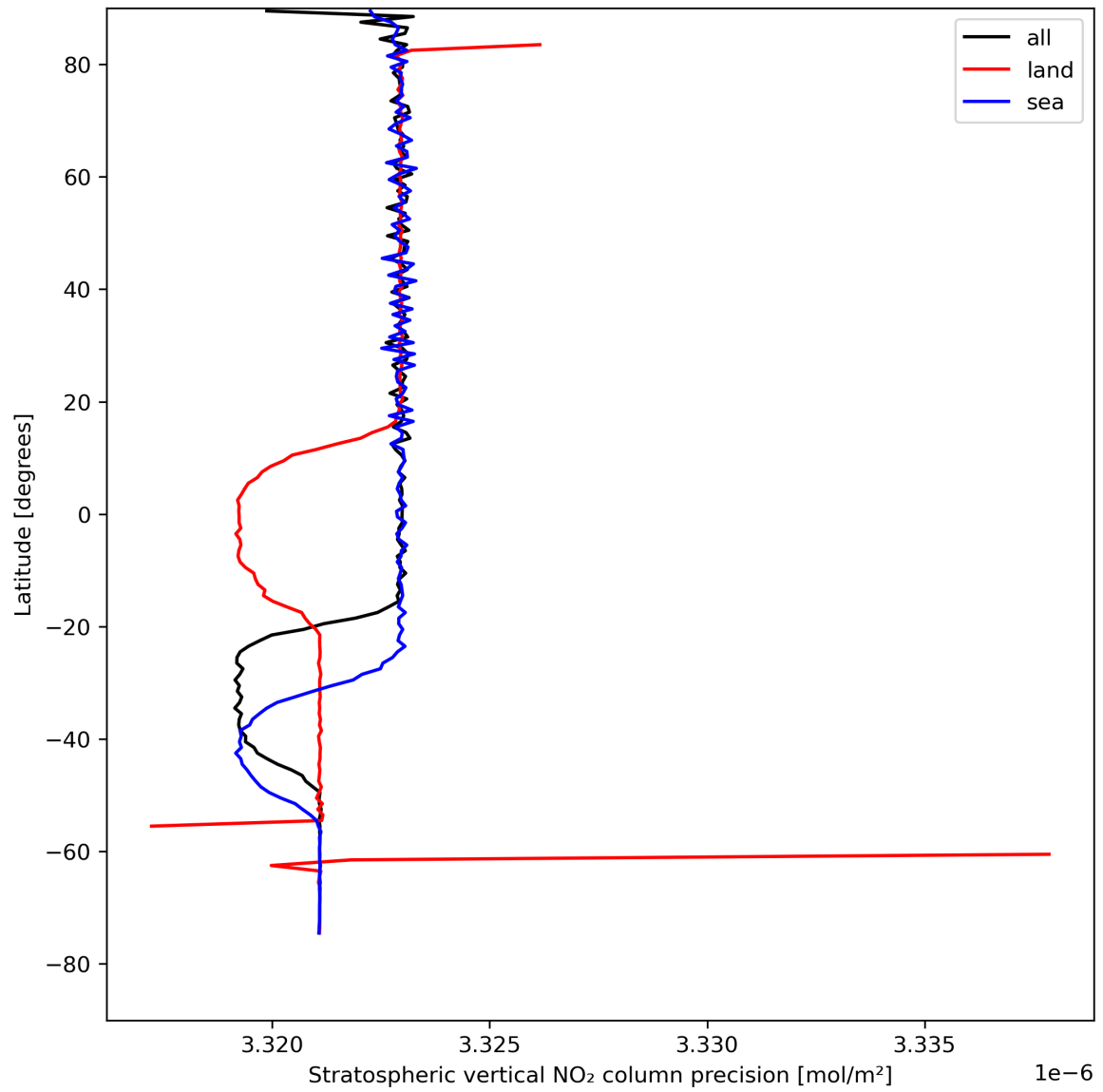
Figure 20: Zonal average of “Stratospheric vertical NO 2 column precision” for 2024-08-16 to 2024-08-17.
