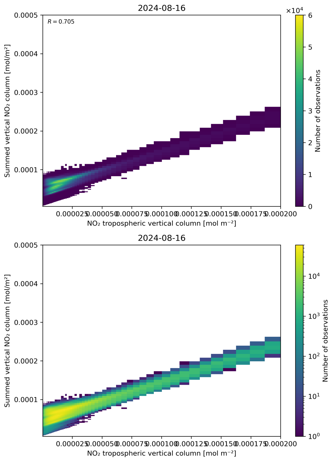
Figure 126: Scatter density plot of “NO 2 tropospheric vertical column” against “Summed vertical NO 2 column” for 2024-08-16 to 2024-08-17.
