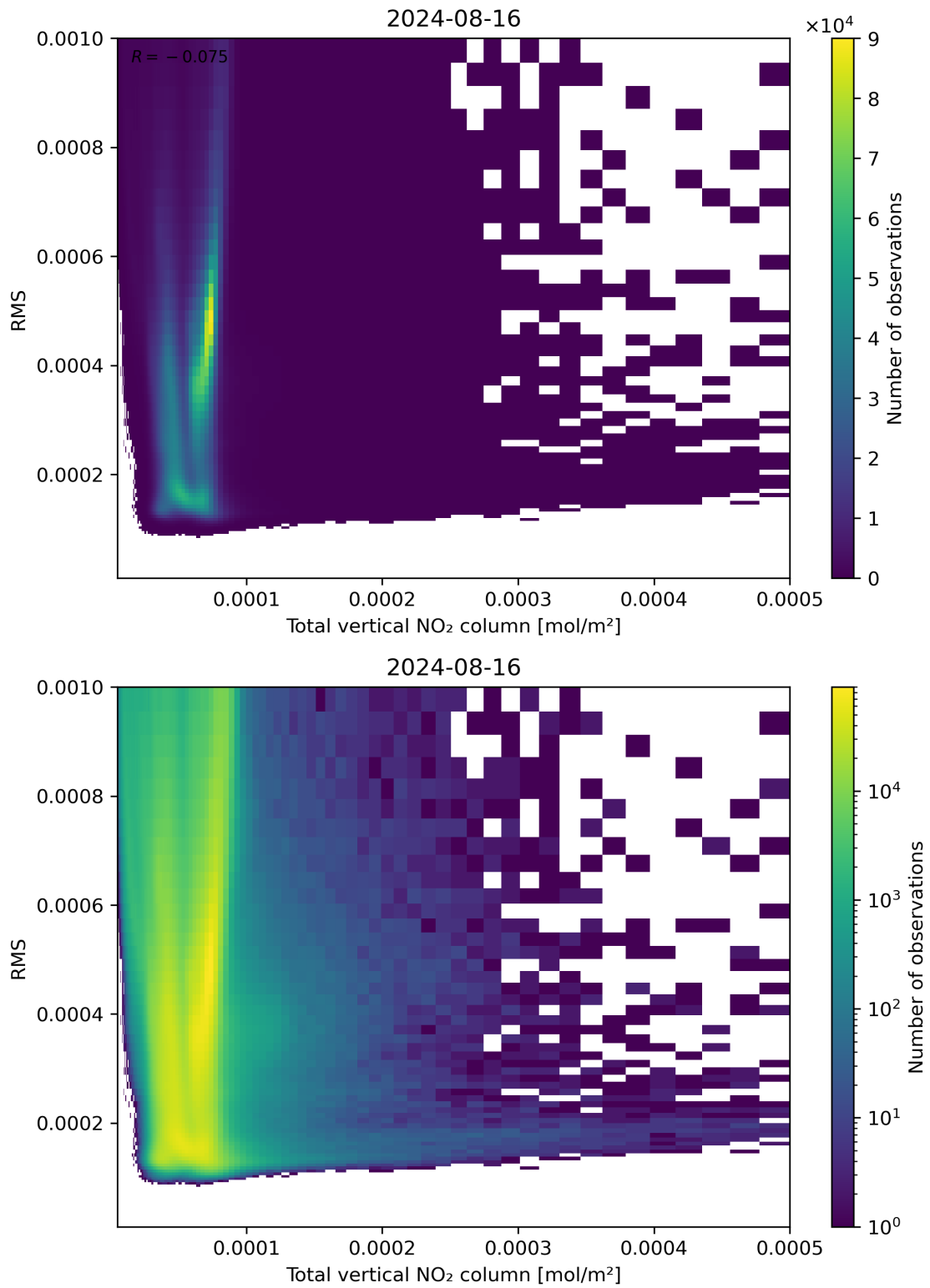
Figure 120: Scatter density plot of “Total vertical NO 2 column” against “RMS” for 2024-08-16 to 2024-08-17.
