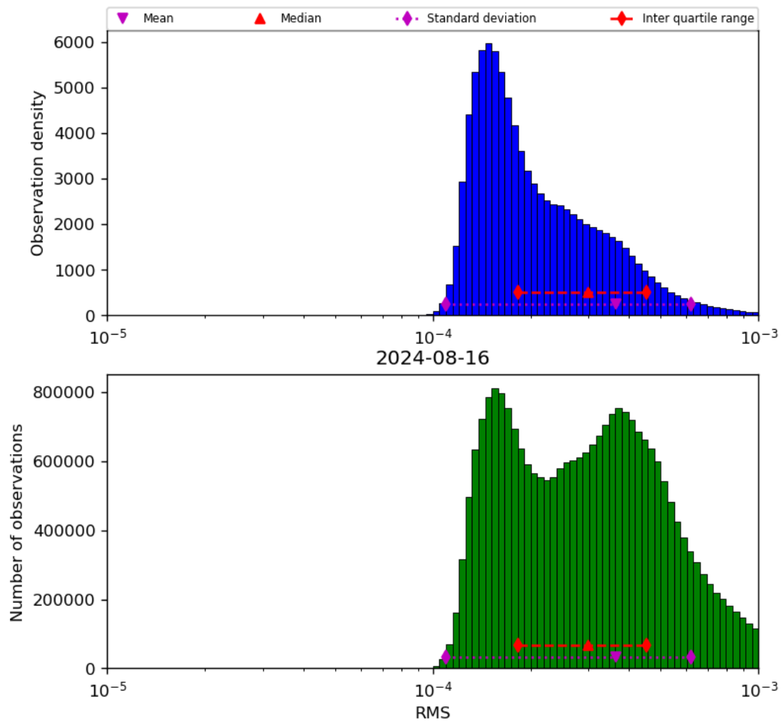
Figure 43: Histogram of “RMS” for 2024-08-16 to 2024-08-17
