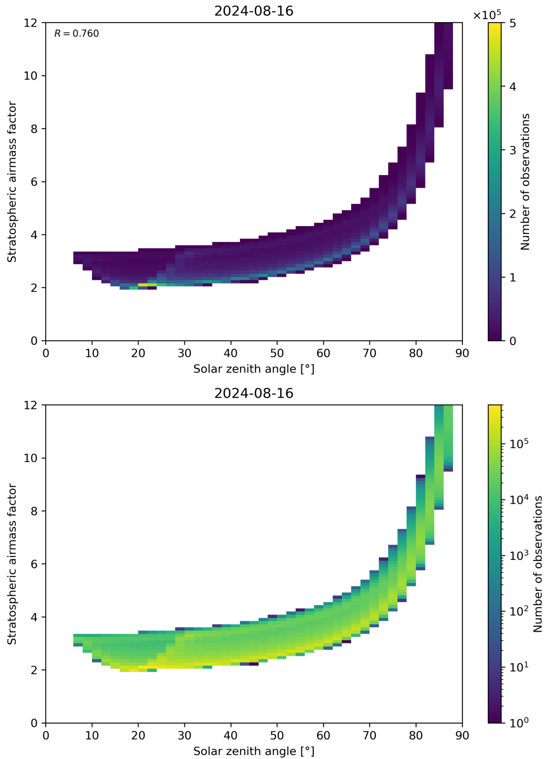
Figure 145: Scatter density plot of “Solar zenith angle” against “Stratospheric airmass factor” for 2024-08-16 to 2024-08-17.
