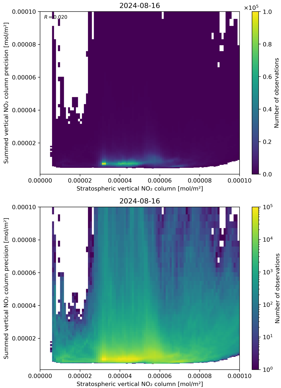
Figure 99: Scatter density plot of “Stratospheric vertical NO 2 column” against “Summed vertical NO 2 column precision” for 2024-08-16 to 2024-08-17.
