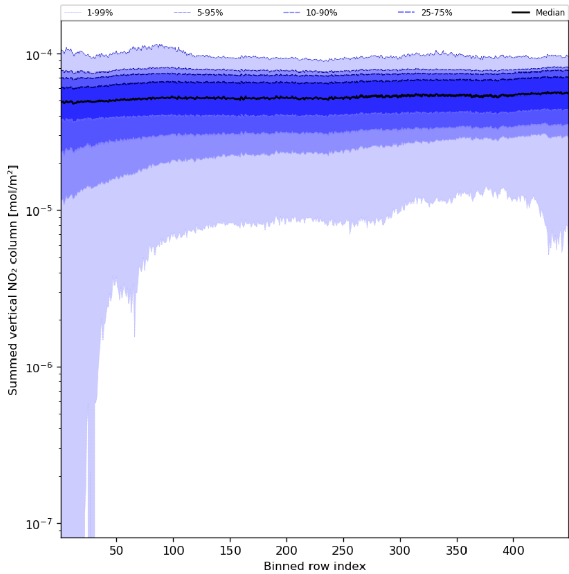
Figure 57: Along track statistics of “Summed vertical NO 2 column” for 2024-08-16 to 2024-08-17
