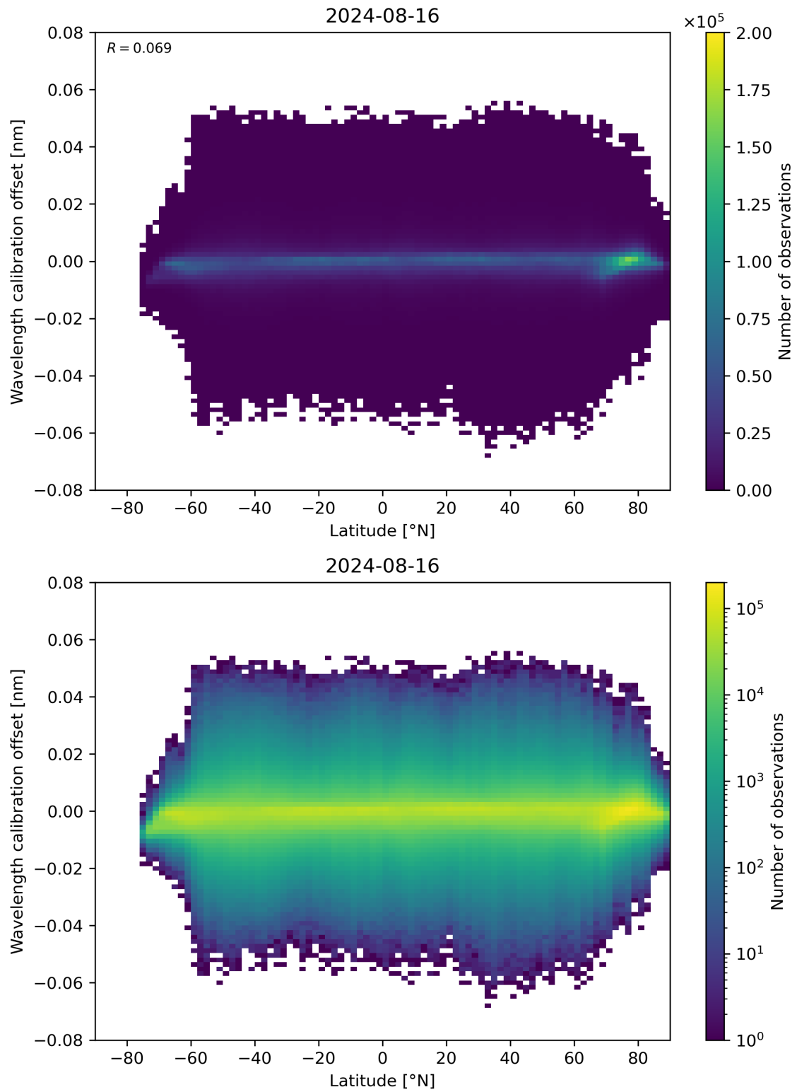
Figure 95: Scatter density plot of “Latitude” against “Wavelength calibration offset” for 2024-08-16 to 2024-08-17.
