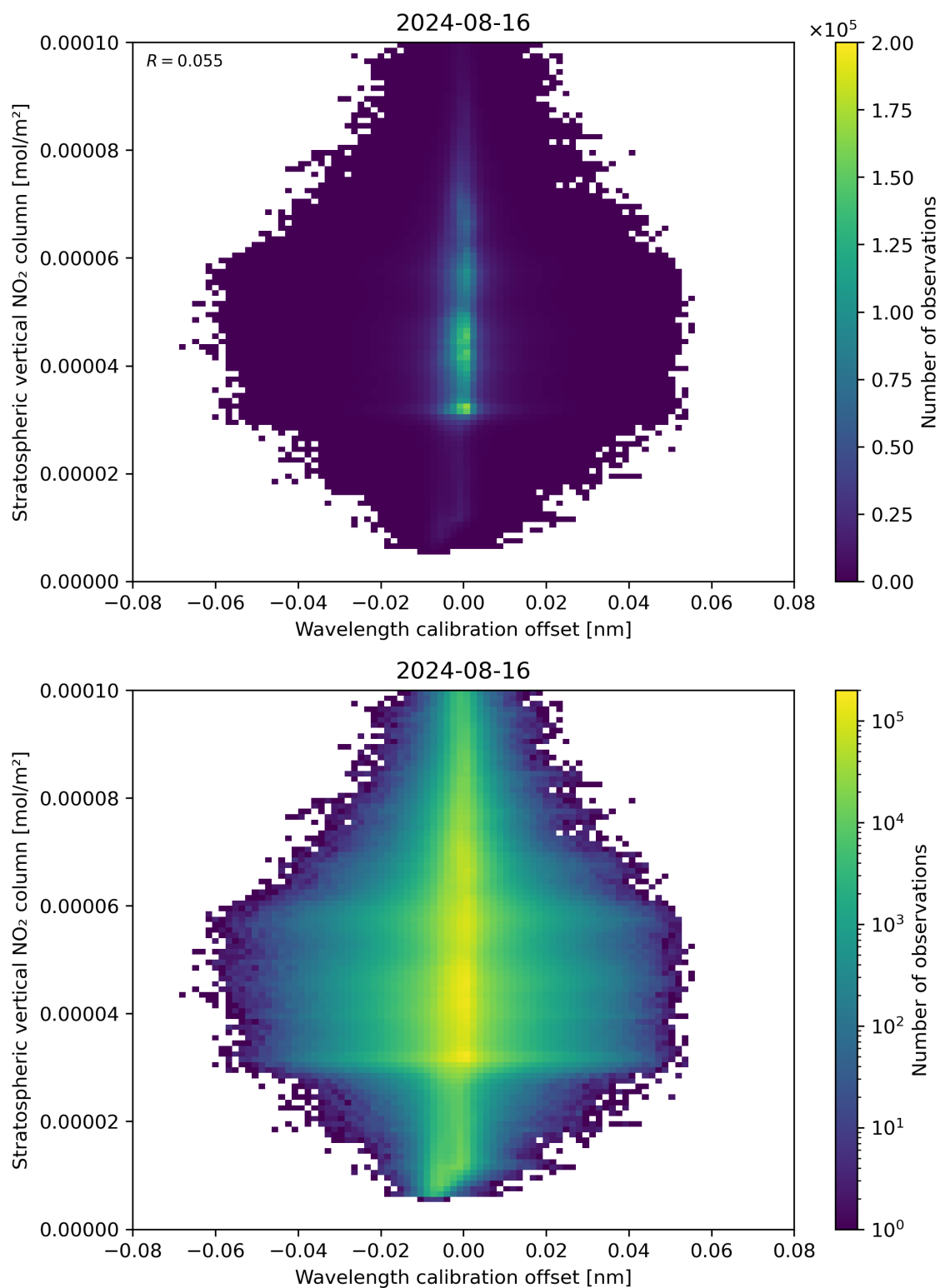
Figure 176: Scatter density plot of “Wavelength calibration offset” against “Stratospheric vertical NO 2 column” for 2024-08-16 to 2024-08-17.
