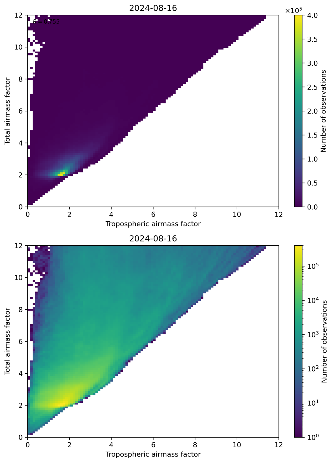
Figure 72: Scatter density plot of “Tropospheric airmass factor” against “Total airmass factor” for 2024-08-16 to 2024-08-17.
