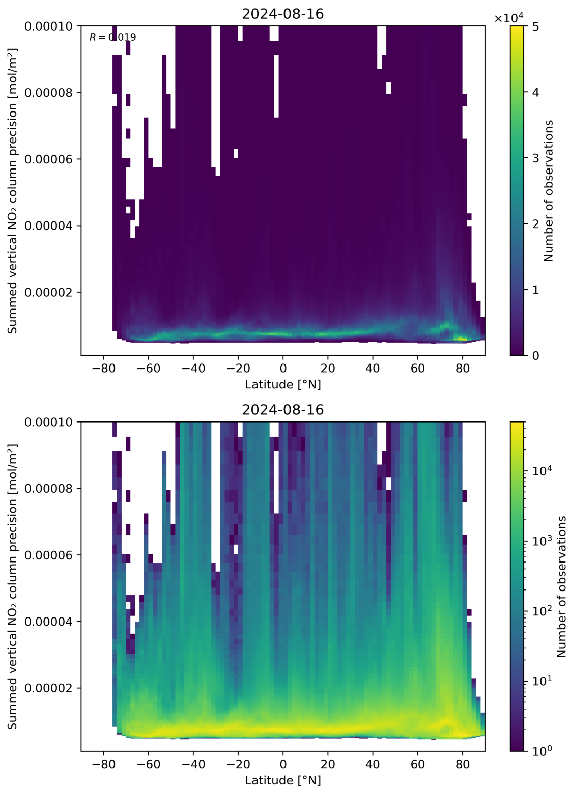
Figure 89: Scatter density plot of “Latitude” against “Summed vertical NO 2 column precision” for 2024-08-16 to 2024-08-17.
