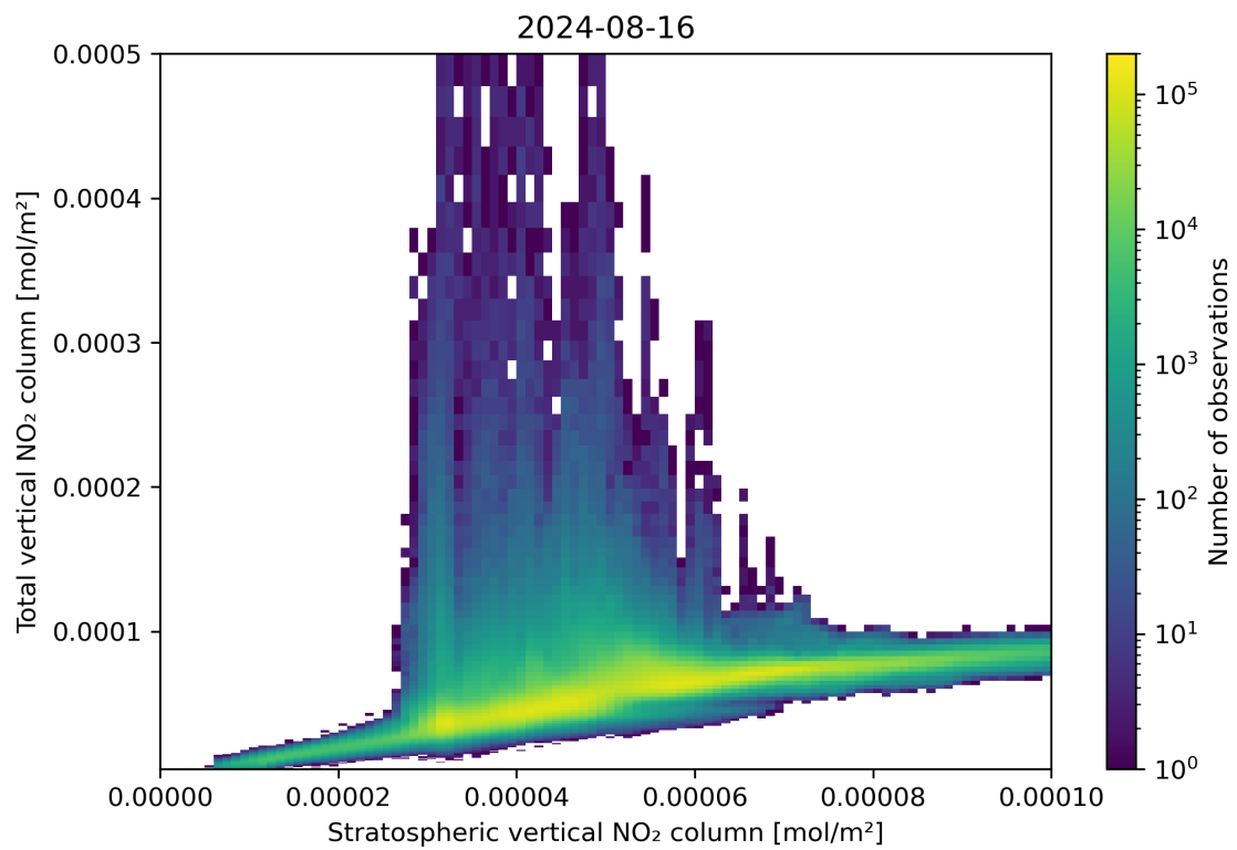
Figure 100: Scatter density plot of “Stratospheric vertical NO 2 column” against “Total vertical NO 2 column” for 2024-08-16 to 2024-08-17.
