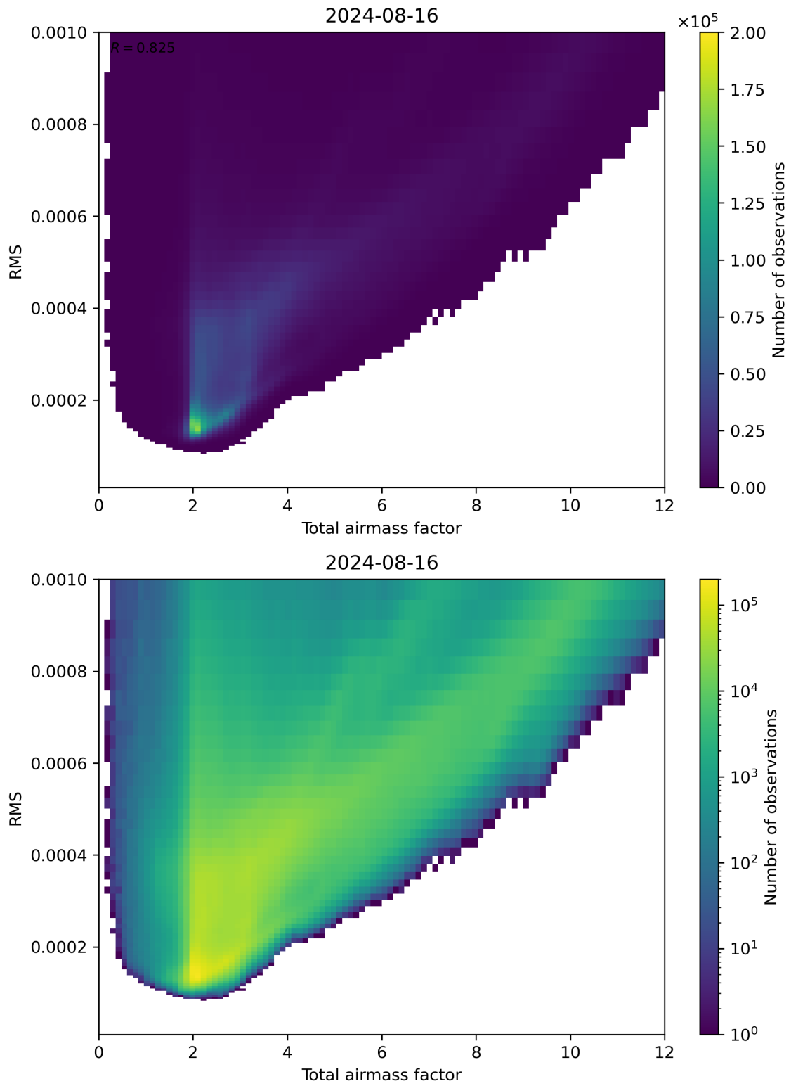
Figure 69: Scatter density plot of “Total airmass factor” against “RMS” for 2024-08-16 to 2024-08-17.
