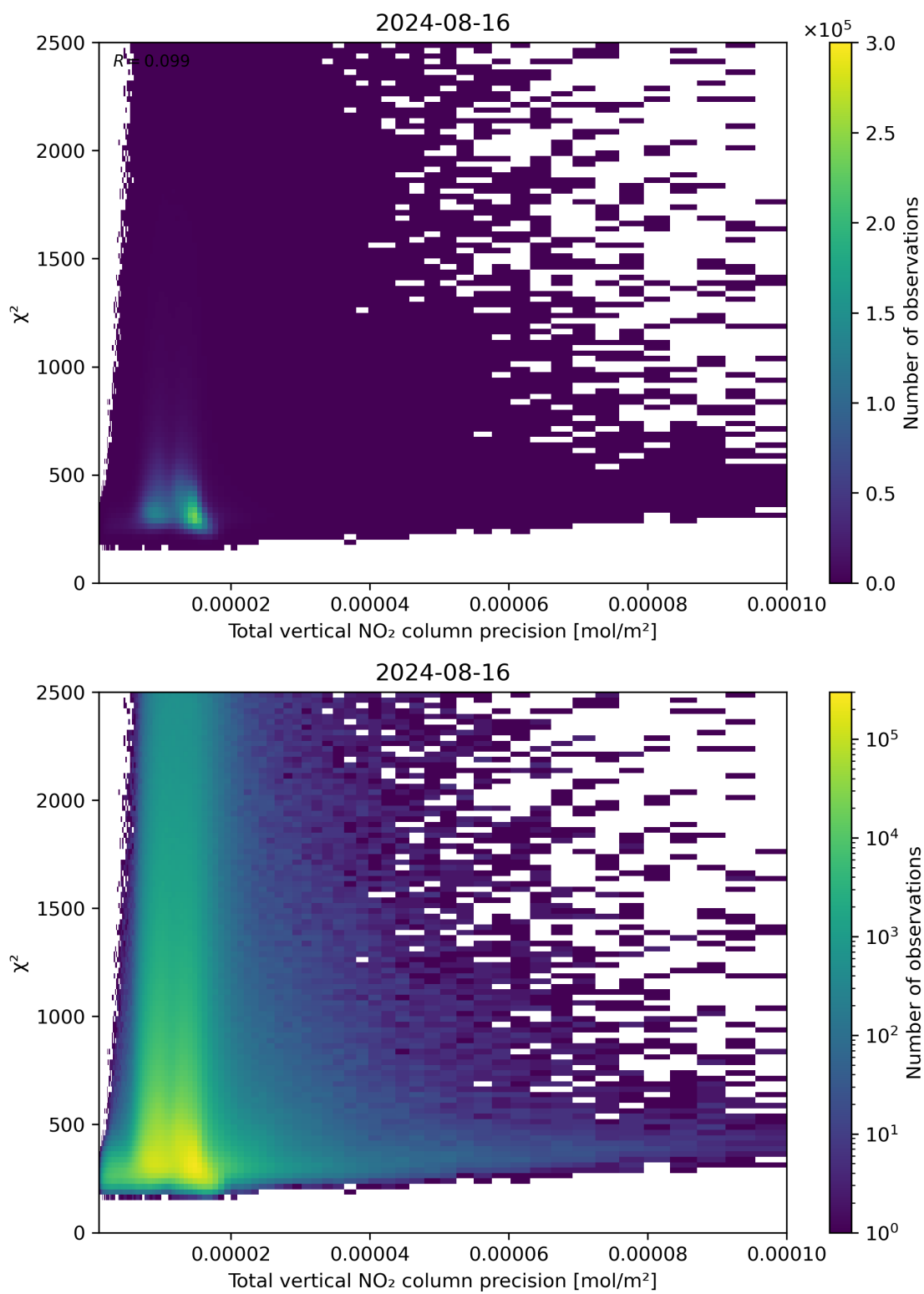
Figure 116: Scatter density plot of “Total vertical NO 2 column precision” against “ \chi^2 ” for 2024-08-16 to 2024-08-17.
