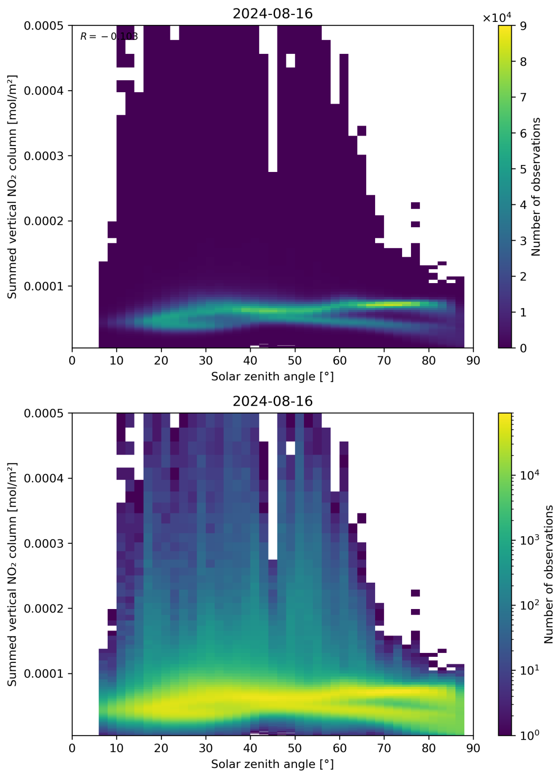
Figure 151: Scatter density plot of “Solar zenith angle” against “Summed vertical NO 2 column” for 2024-08-16 to 2024-08-17.
