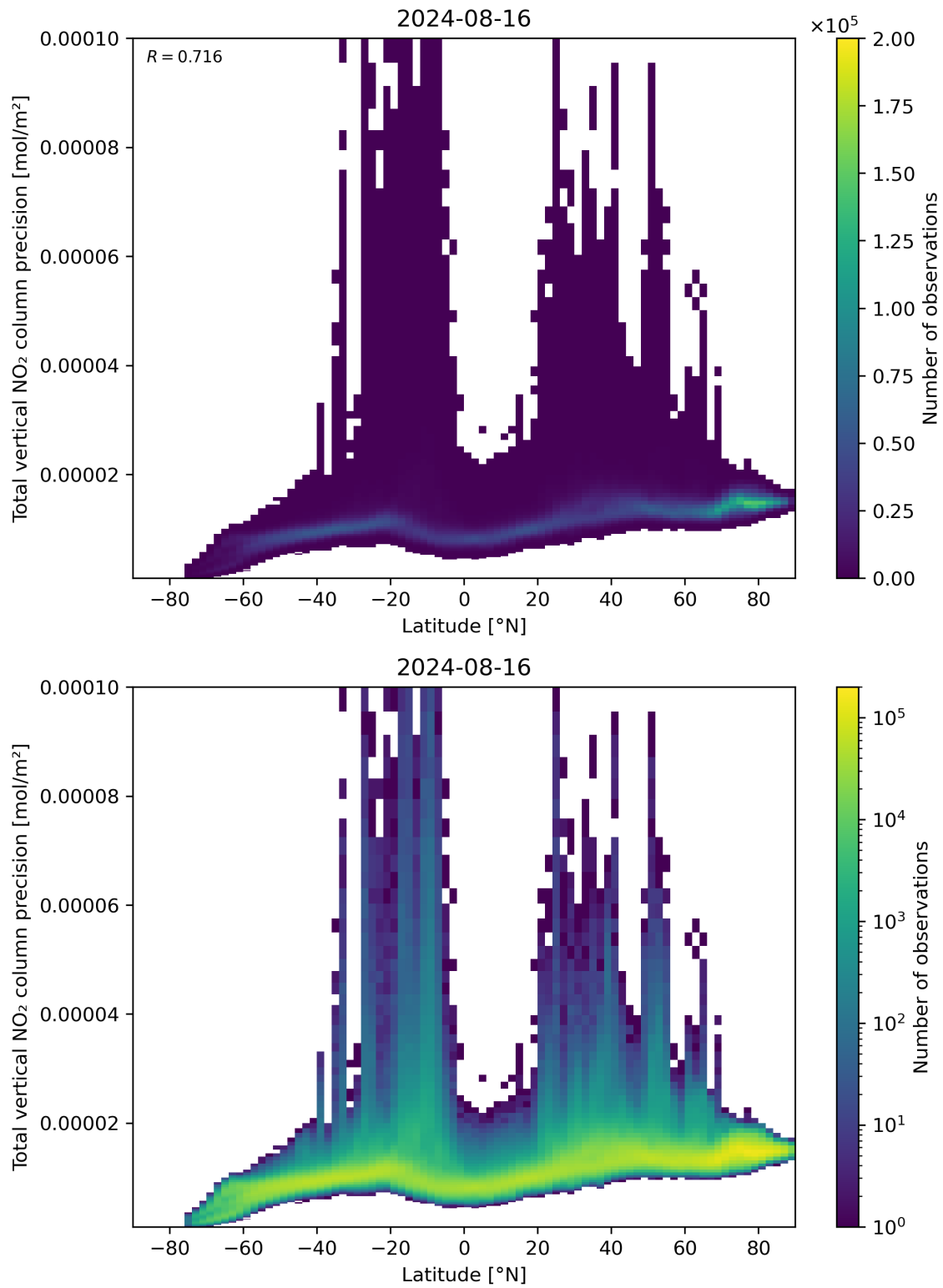
Figure 91: Scatter density plot of “Latitude” against “Total vertical NO 2 column precision” for 2024-08-16 to 2024-08-17.
