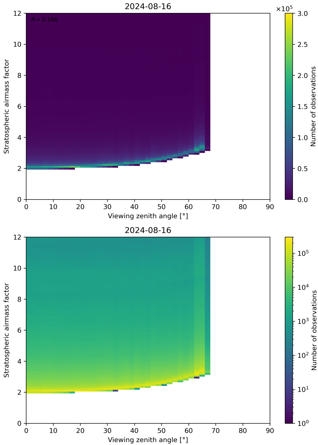
Figure 159: Scatter density plot of “Viewing zenith angle” against “Stratospheric airmass factor” for 2024-08-16 to 2024-08-17.
