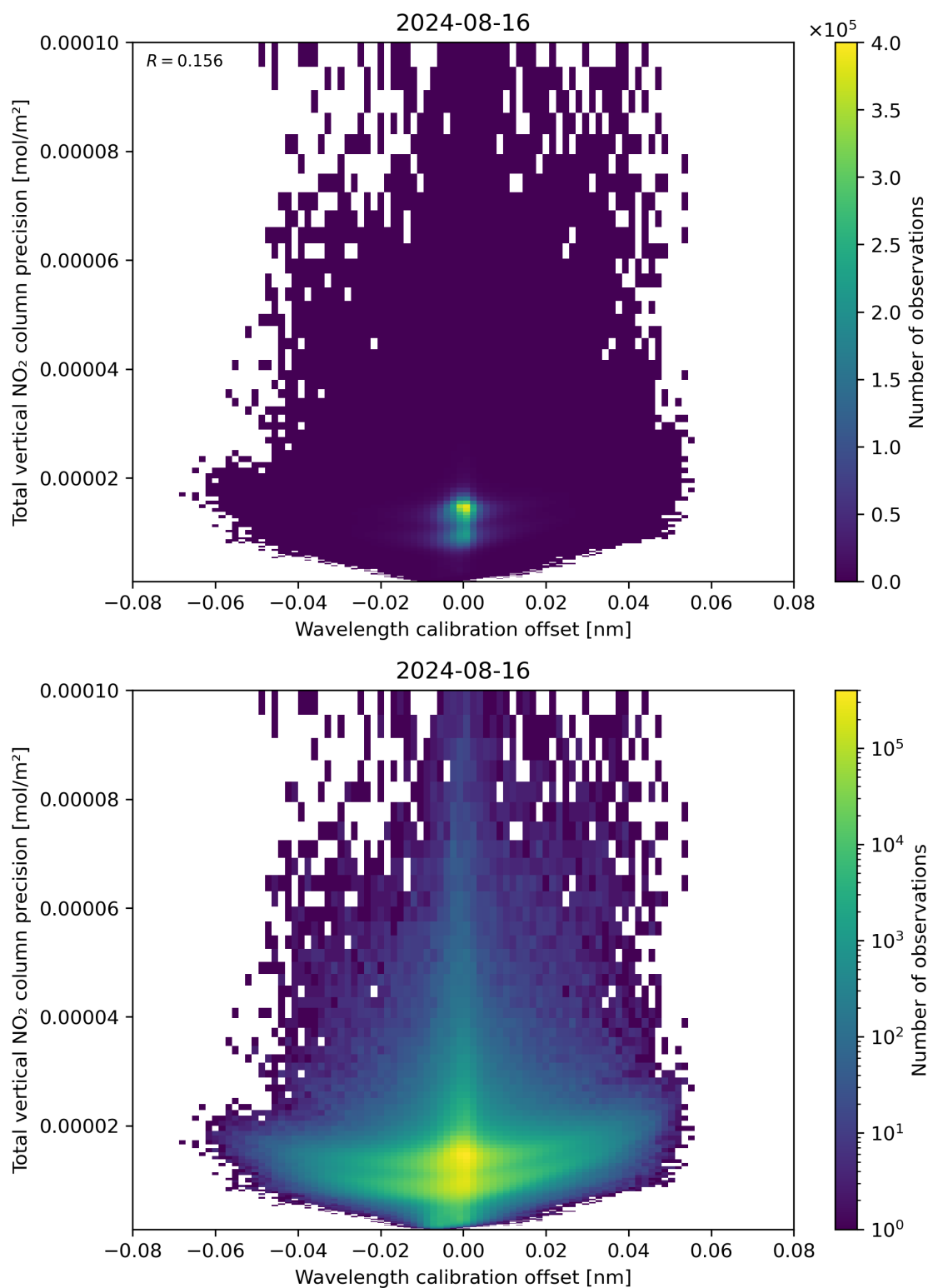
Figure 180: Scatter density plot of “Wavelength calibration offset” against “Total vertical NO 2 column precision” for 2024-08-16 to 2024-08-17.
