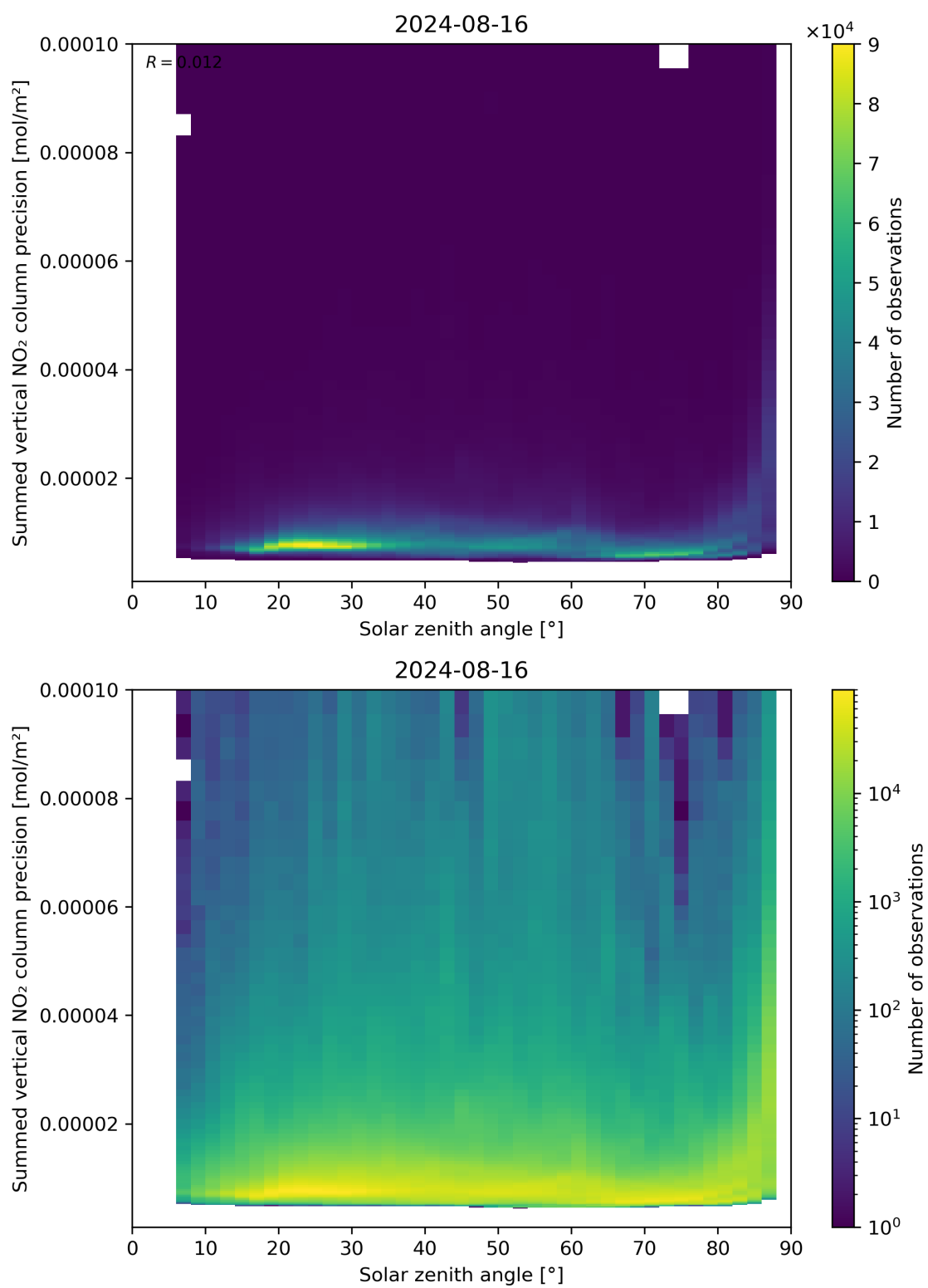
Figure 152: Scatter density plot of “Solar zenith angle” against “Summed vertical NO 2 column precision” for 2024-08-16 to 2024-08-17.
