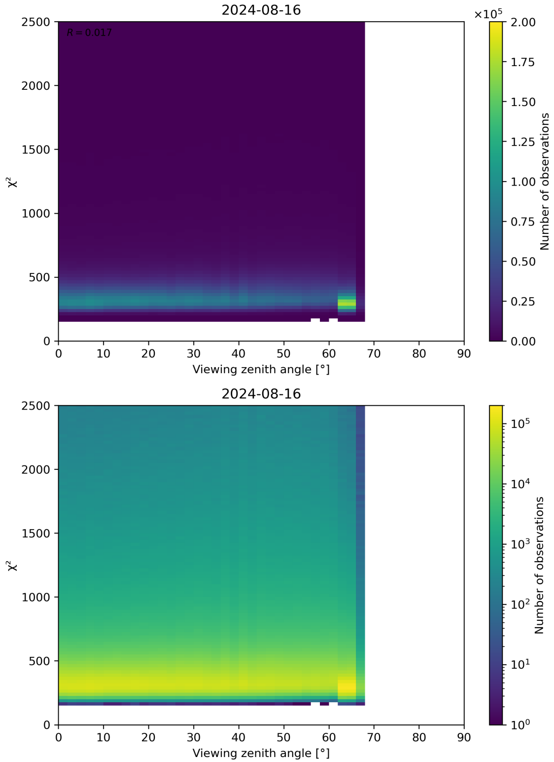
Figure 162: Scatter density plot of “Viewing zenith angle” against “ \chi^2 ” for 2024-08-16 to 2024-08-17.
