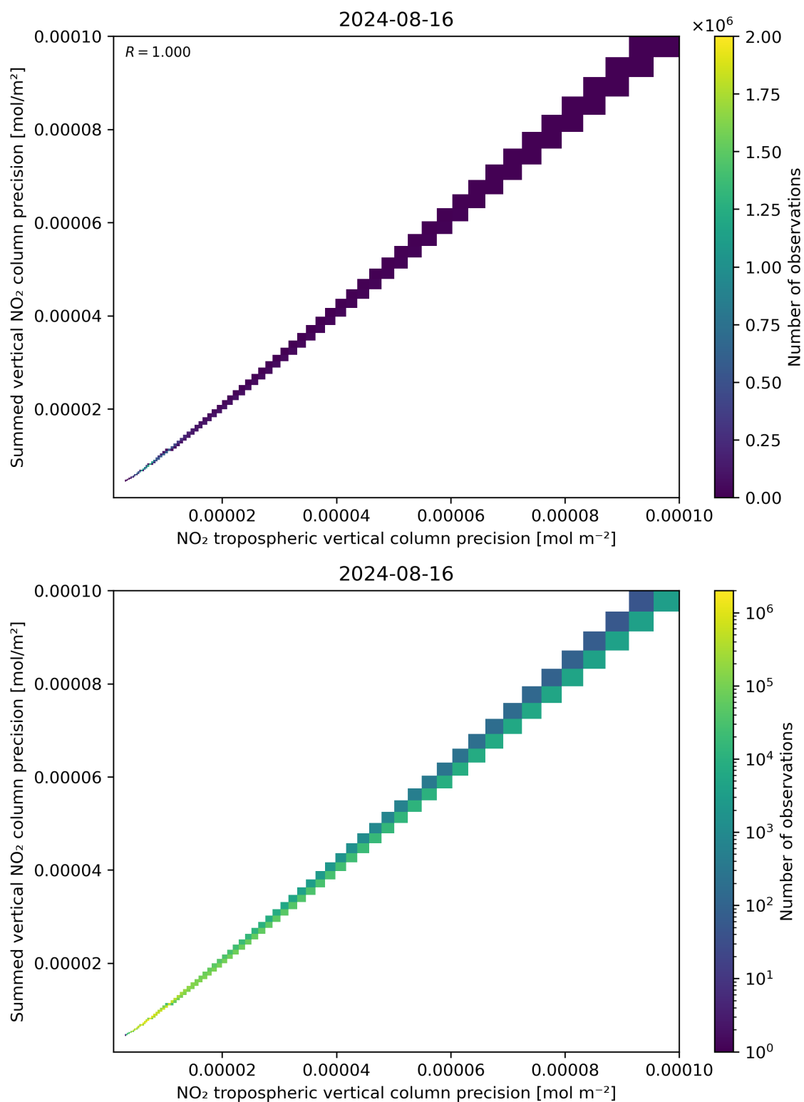
Figure 137: Scatter density plot of “NO 2 tropospheric vertical column precision” against “Summed vertical NO 2 column precision” for 2024-08-16 to 2024-08-17.
