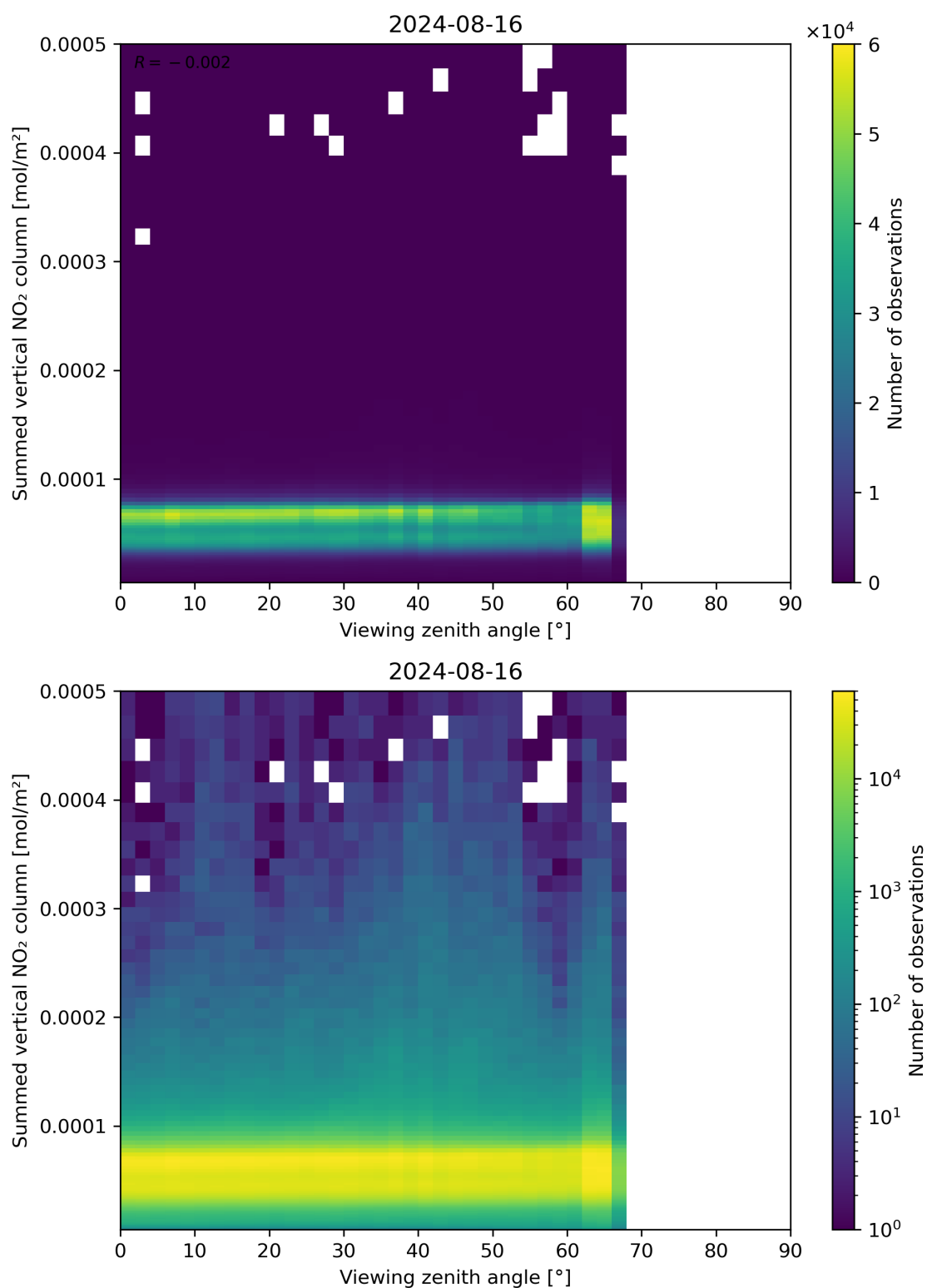
Figure 165: Scatter density plot of “Viewing zenith angle” against “Summed vertical NO 2 column” for 2024-08-16 to 2024-08-17.
