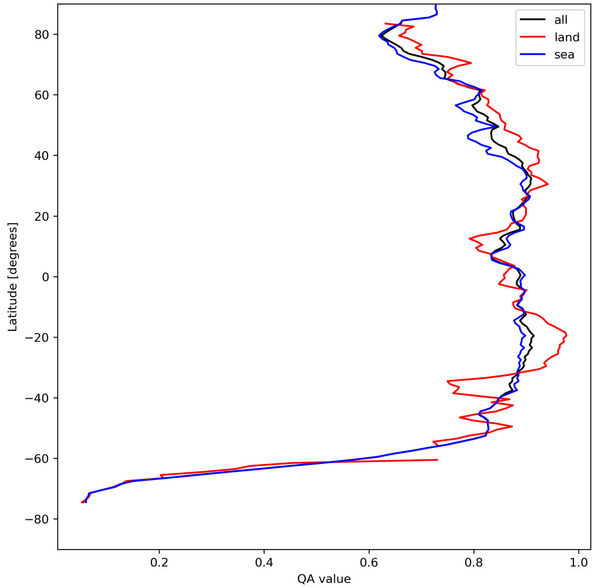
Figure 11: Zonal average of “QA value” for 2024-08-16 to 2024-08-17.
