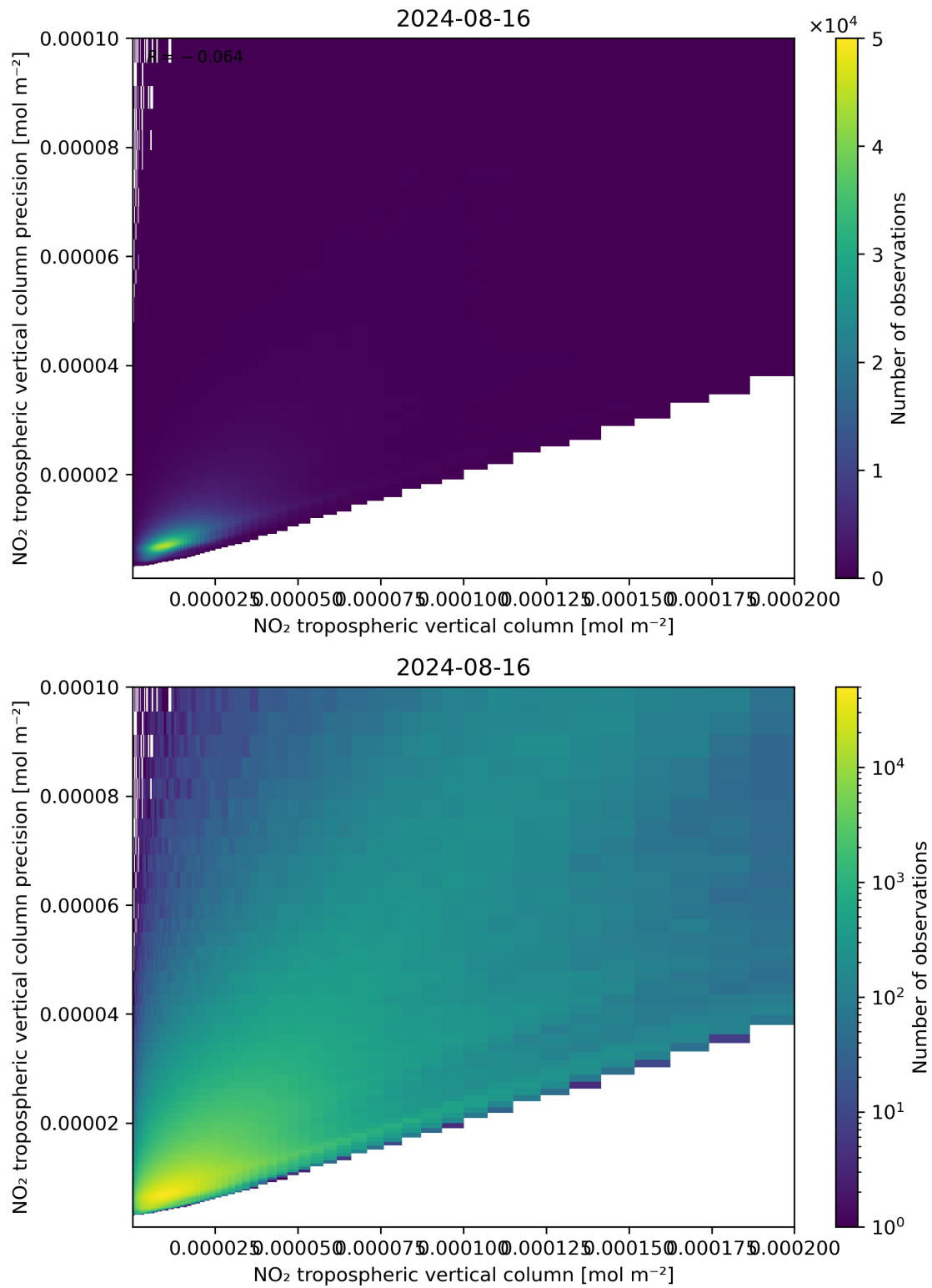
Figure 130: Scatter density plot of “NO 2 tropospheric vertical column” against “NO 2 tropospheric vertical column precision” for 2024-08-16 to 2024-08-17.
