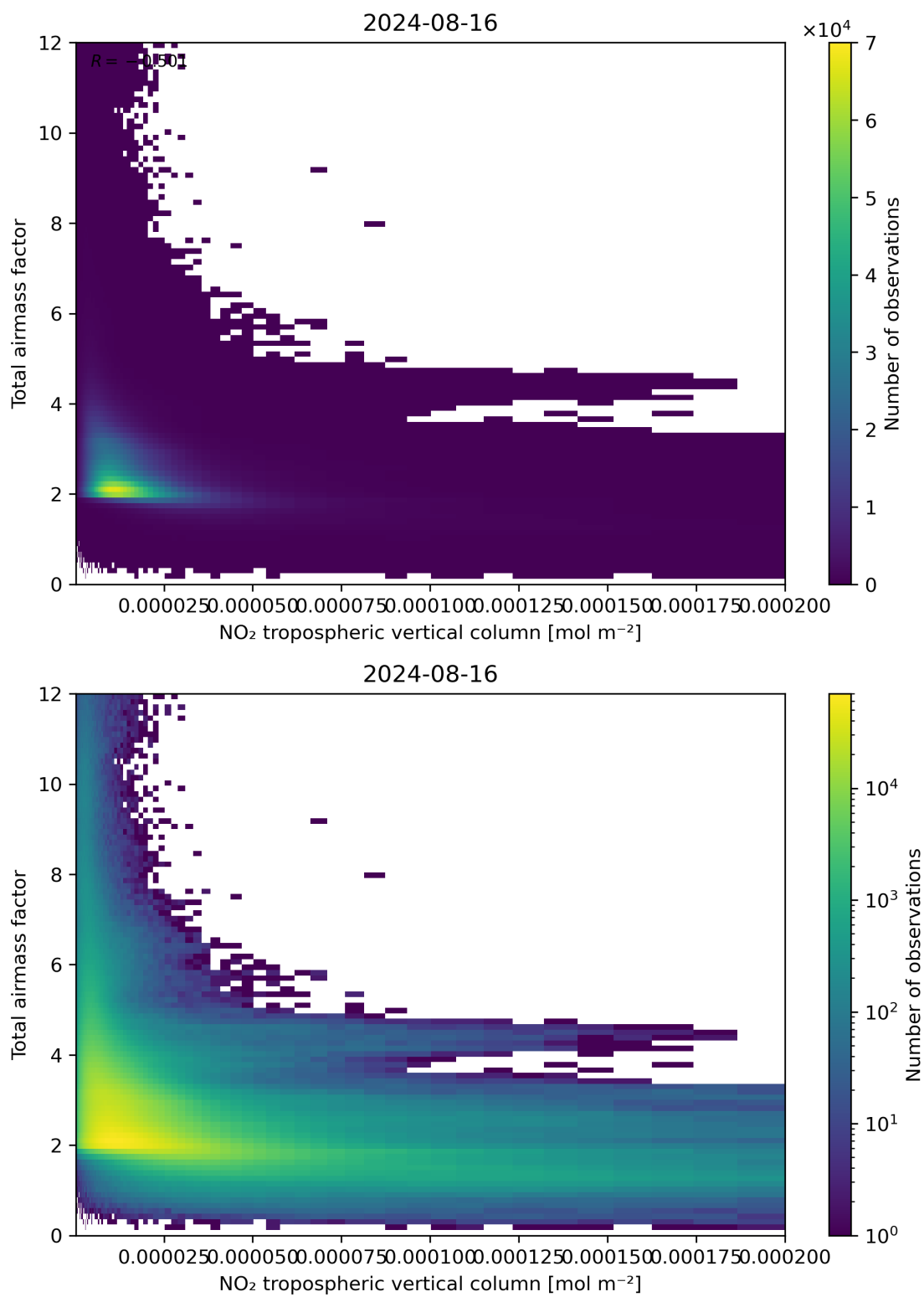
Figure 122: Scatter density plot of “NO 2 tropospheric vertical column” against “Total airmass factor” for 2024-08-16 to 2024-08-17.
