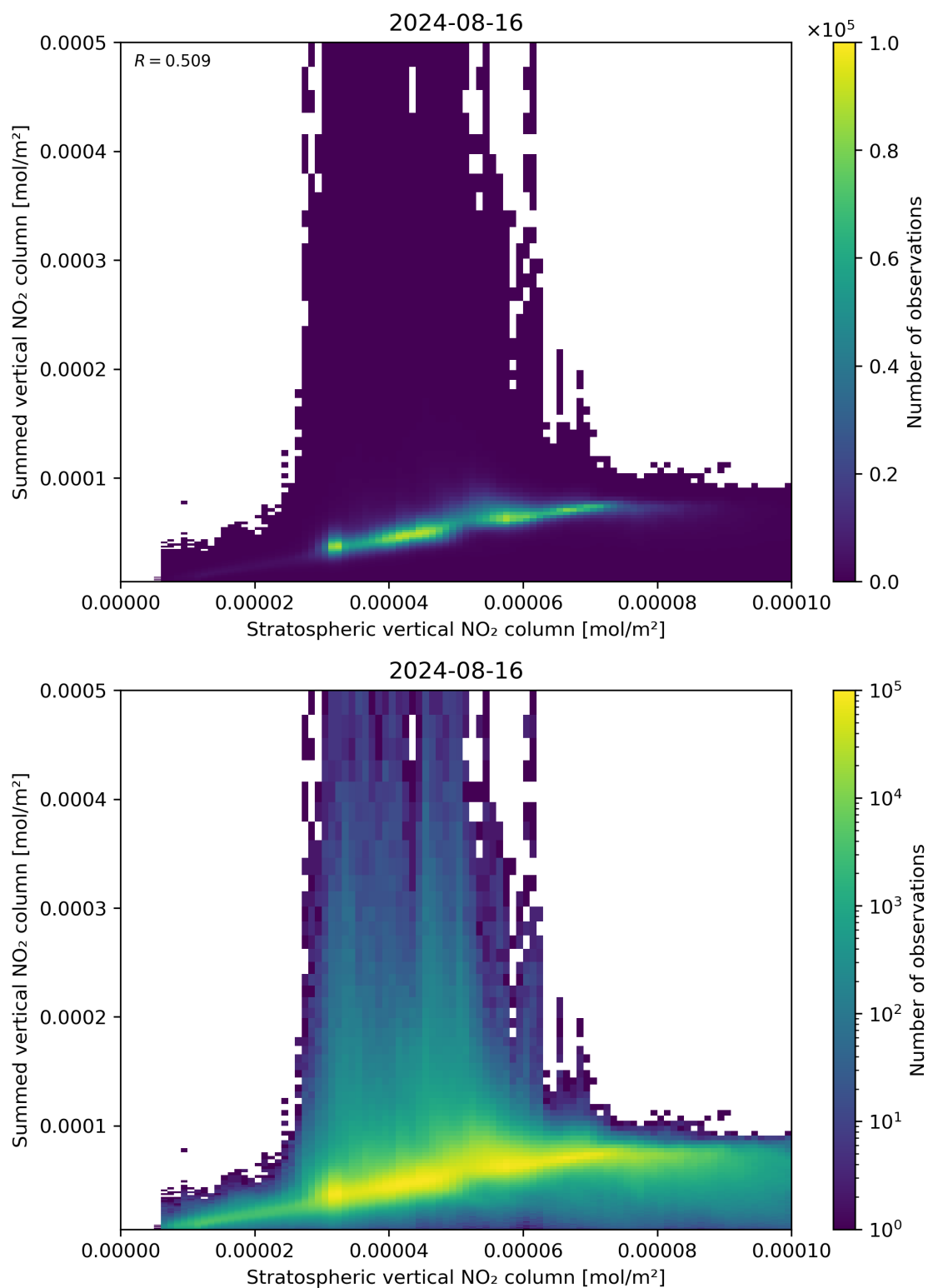
Figure 98: Scatter density plot of “Stratospheric vertical NO 2 column” against “Summed vertical NO 2 column” for 2024-08-16 to 2024-08-17.
