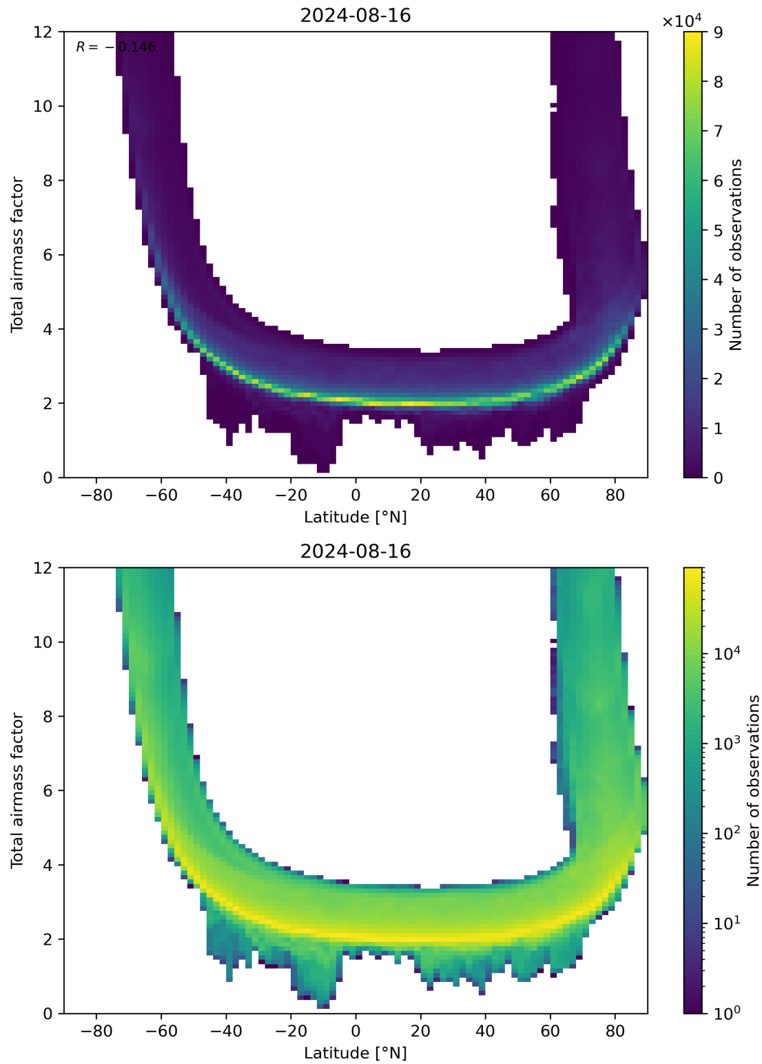
Figure 84: Scatter density plot of “Latitude” against “Total airmass factor” for 2024-08-16 to 2024-08-17.
