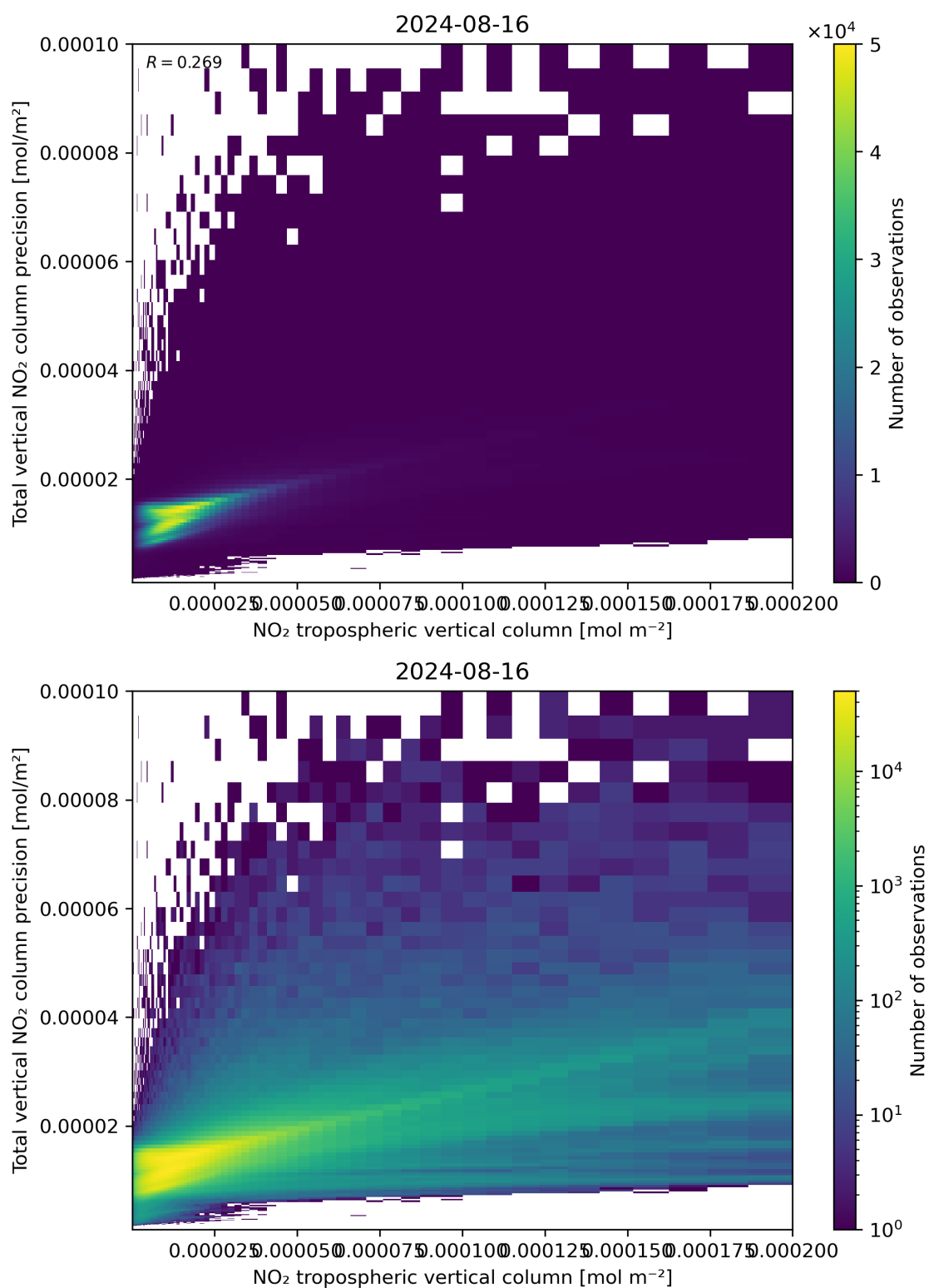
Figure 129: Scatter density plot of “NO 2 tropospheric vertical column” against “Total vertical NO 2 column precision” for 2024-08-16 to 2024-08-17.
