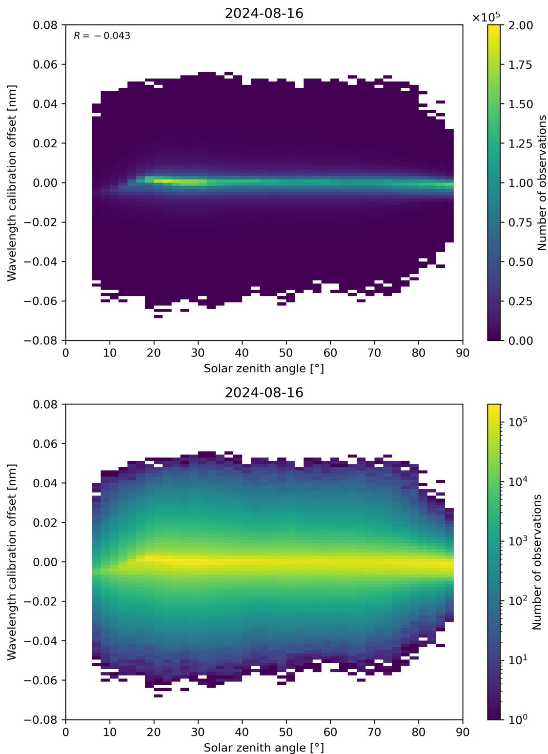
Figure 158: Scatter density plot of “Solar zenith angle” against “Wavelength calibration offset” for 2024-08-16 to 2024-08-17.
