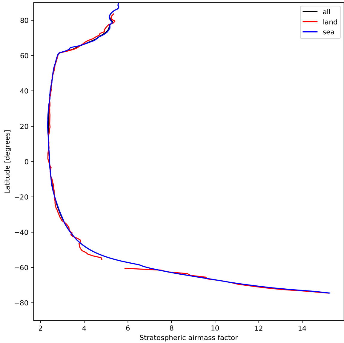
Figure 27: Zonal average of “Stratospheric airmass factor” for 2024-08-16 to 2024-08-17.
