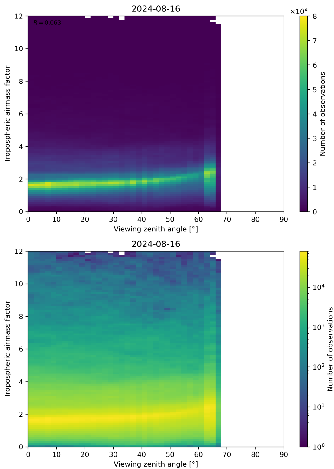
Figure 161: Scatter density plot of “Viewing zenith angle” against “Tropospheric airmass factor” for 2024-08-16 to 2024-08-17.
