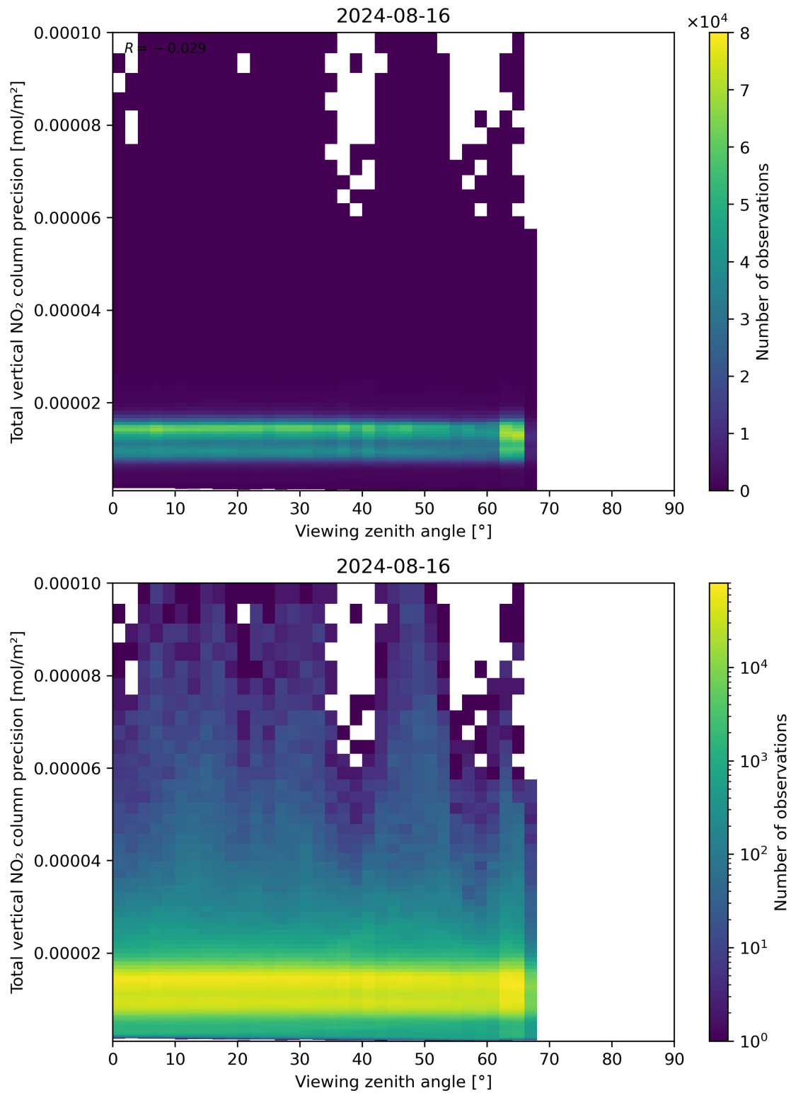
Figure 168: Scatter density plot of “Viewing zenith angle” against “Total vertical NO 2 column precision” for 2024-08-16 to 2024-08-17.
