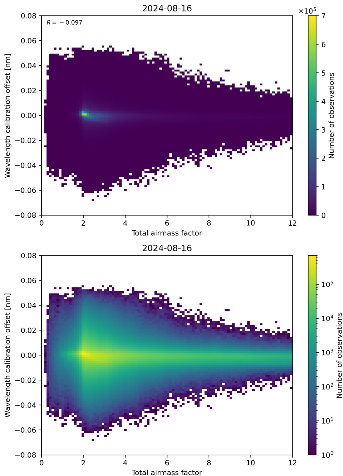
Figure 70: Scatter density plot of “Total airmass factor” against “Wavelength calibration offset” for 2024-08-16 to 2024-08-17.
