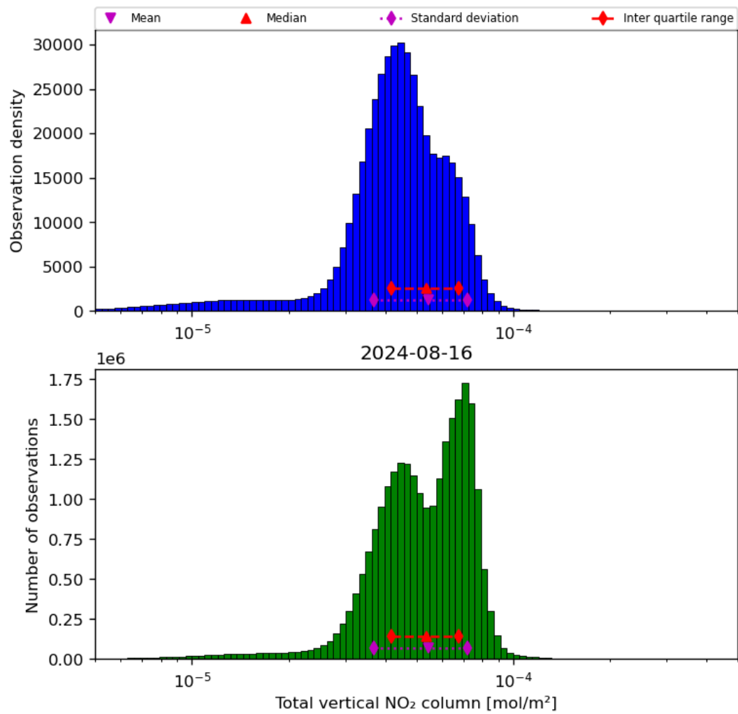
Figure 38: Histogram of “Total vertical NO 2 column” for 2024-08-16 to 2024-08-17
