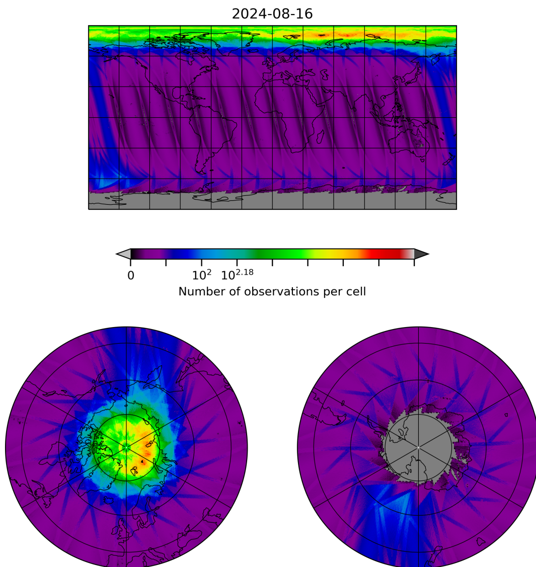
Figure 10: Map of the number of observations for 2024-08-16 to 2024-08-17
