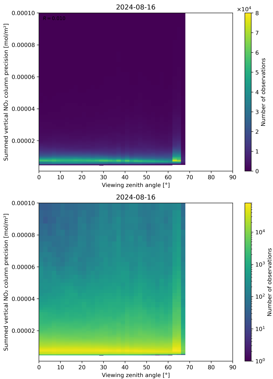
Figure 166: Scatter density plot of “Viewing zenith angle” against “Summed vertical NO 2 column precision” for 2024-08-16 to 2024-08-17.
