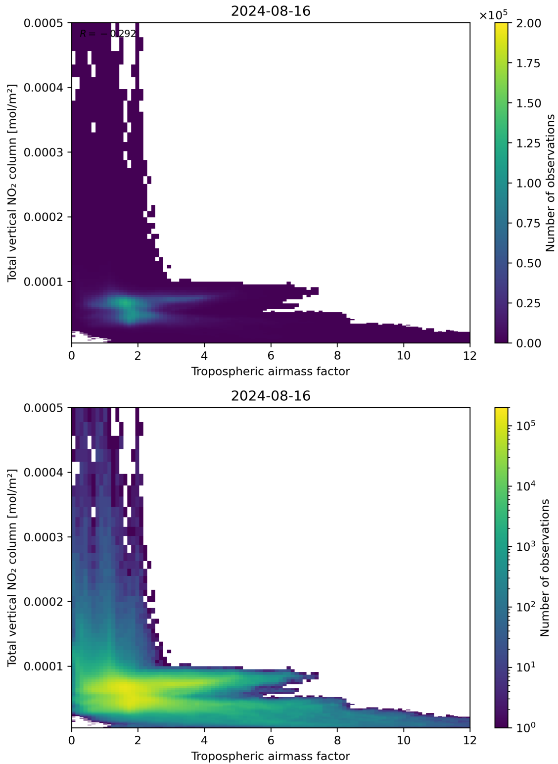
Figure 77: Scatter density plot of “Tropospheric airmass factor” against “Total vertical NO 2 column” for 2024-08-16 to 2024-08-17.
