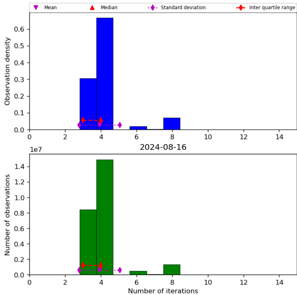
Figure 34: Histogram of “Number of iterations” for 2024-08-16 to 2024-08-17
