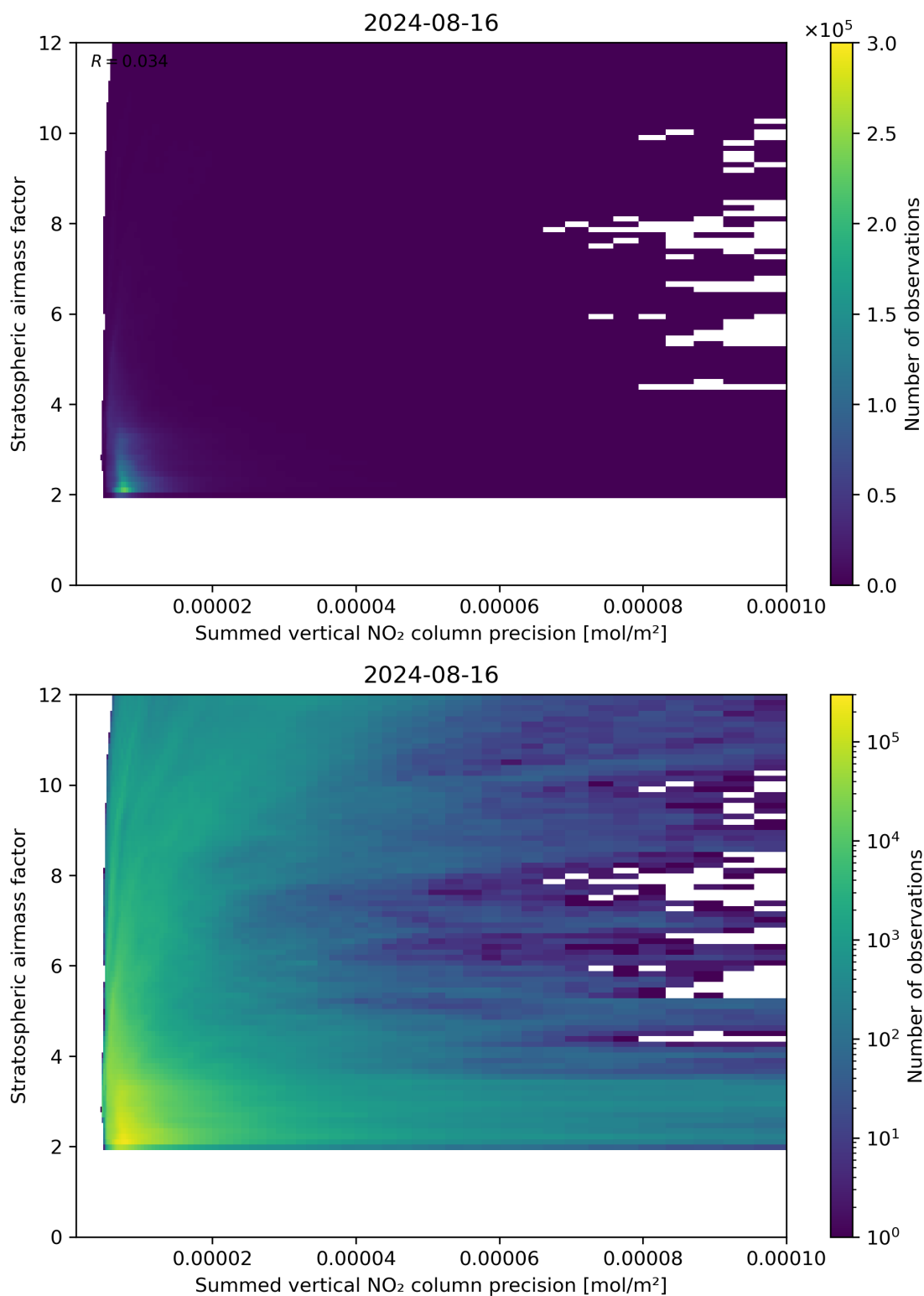
Figure 106: Scatter density plot of “Summed vertical NO 2 column precision” against “Stratospheric airmass factor” for 2024-08-16 to 2024-08-17.
