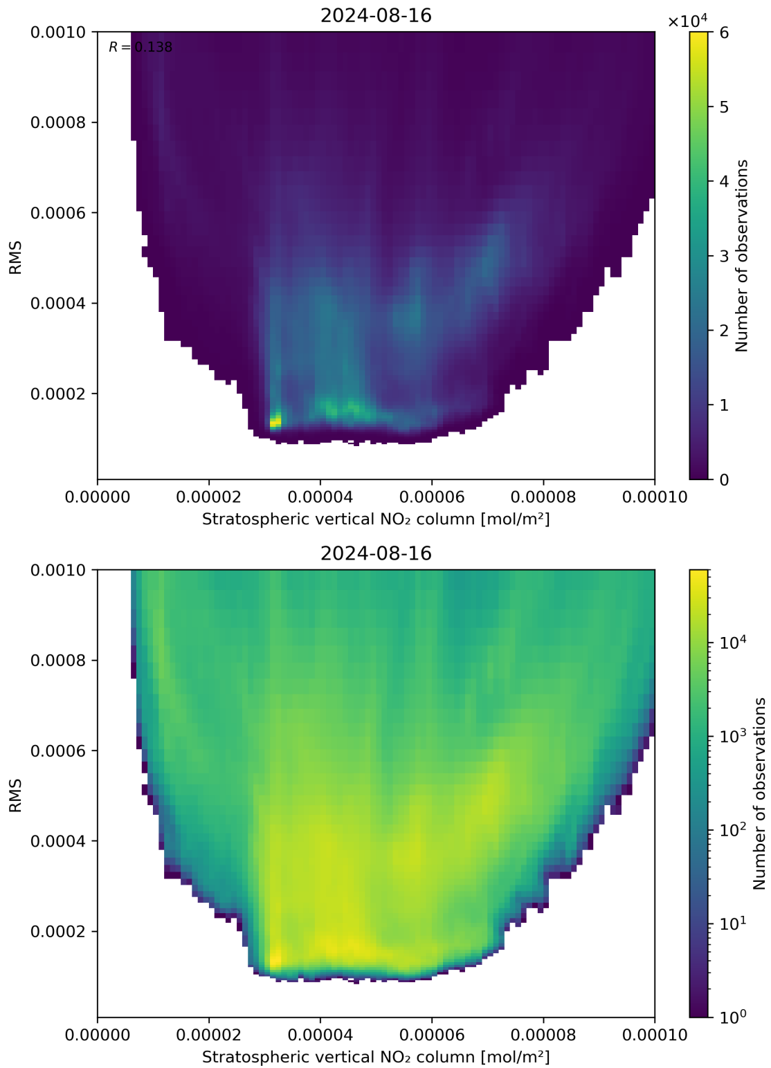
Figure 102: Scatter density plot of “Stratospheric vertical NO 2 column” against “RMS” for 2024-08-16 to 2024-08-17.
