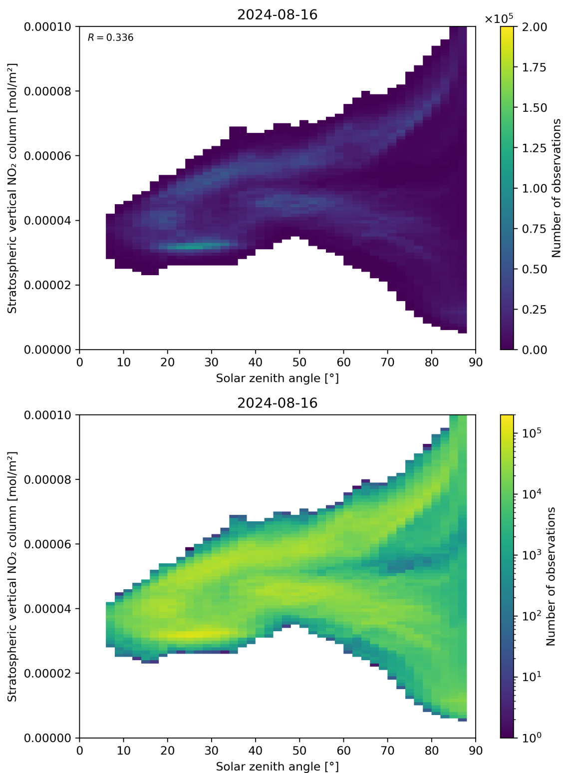
Figure 150: Scatter density plot of “Solar zenith angle” against “Stratospheric vertical NO 2 column” for 2024-08-16 to 2024-08-17.
