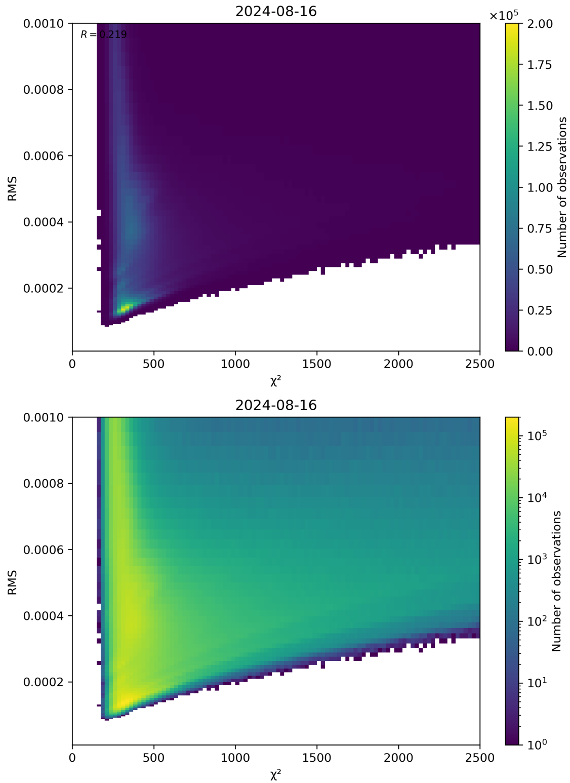
Figure 82: Scatter density plot of “ \chi^2 ” against “RMS” for 2024-08-16 to 2024-08-17.
