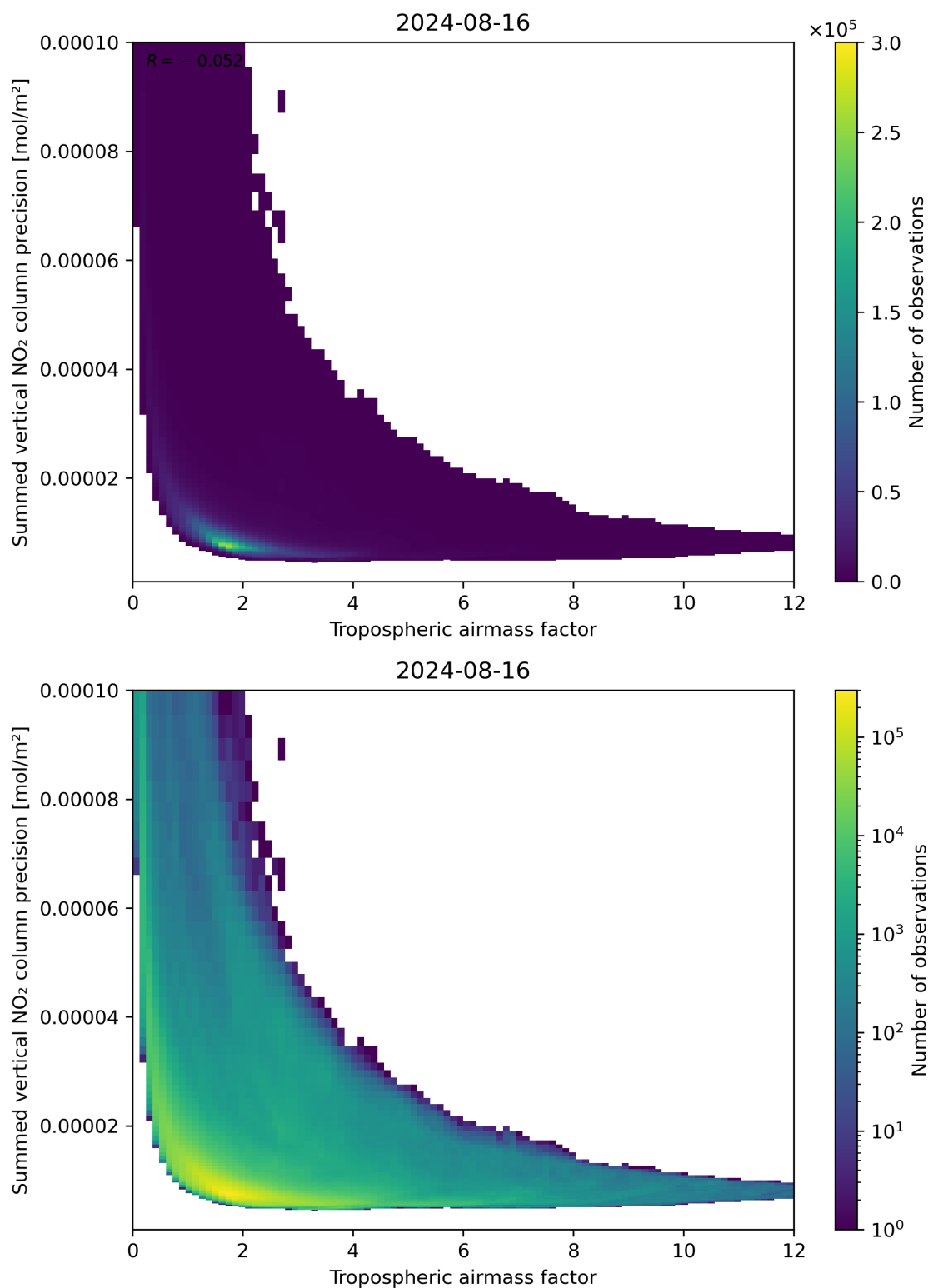
Figure 76: Scatter density plot of “Tropospheric air mass factor” against “Summed vertical NO 2 column precision” for 2024-08-16 to 2024-08-17.
