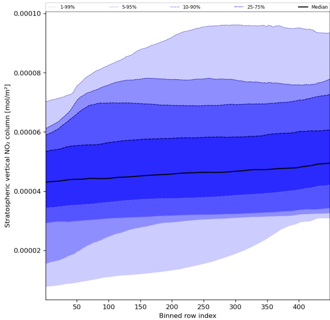
Figure 53: Along track statistics of “Stratospheric vertical NO 2 column” for 2024-08-16 to 2024-08-17
