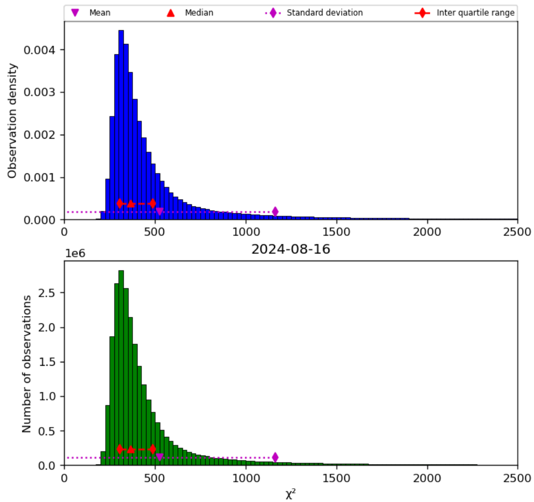
Figure 42: Histogram of " \chi^2 " for 2024-08-16 to 2024-08-17
