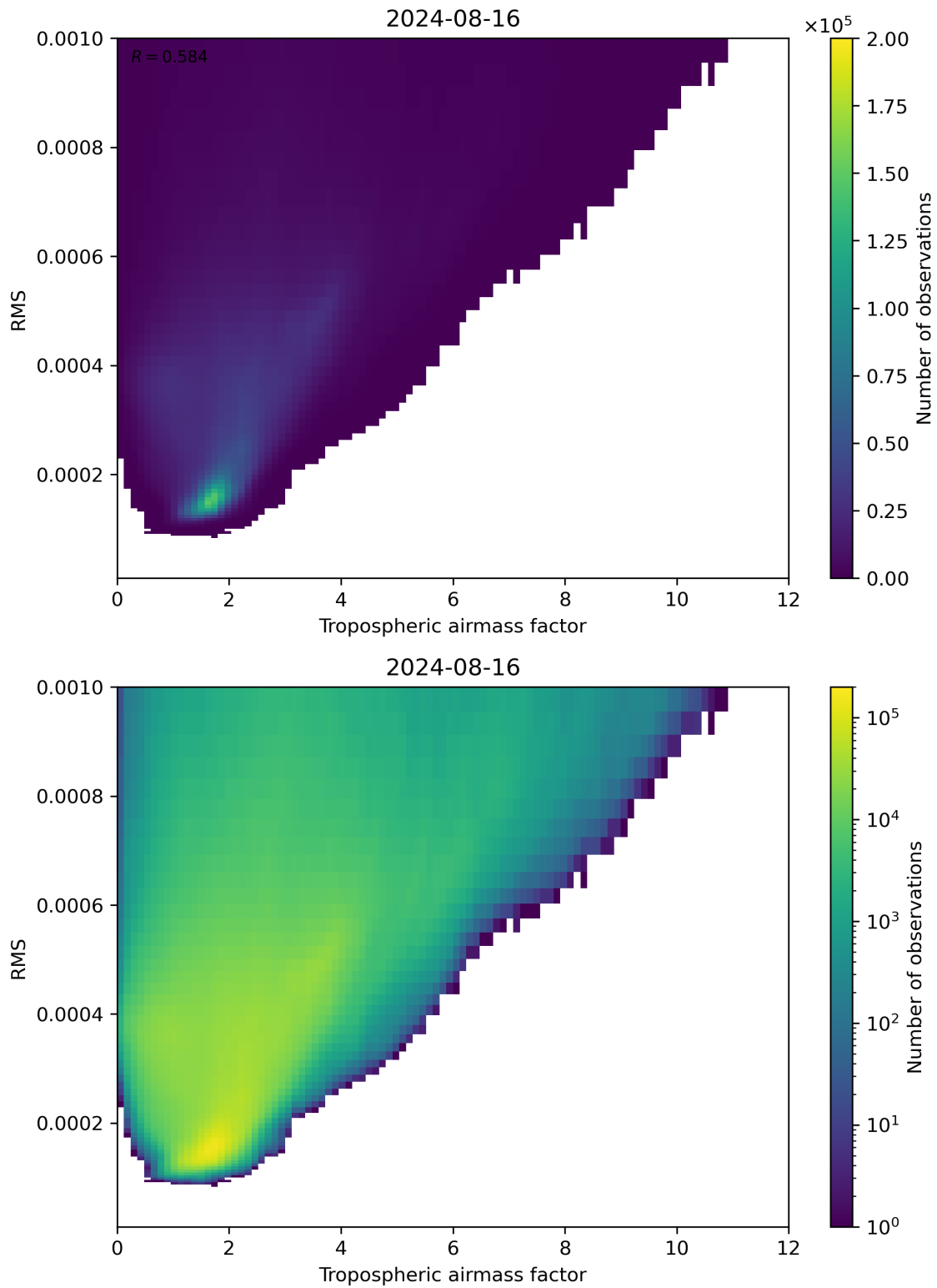
Figure 79: Scatter density plot of “Tropospheric airmass factor” against “RMS” for 2024-08-16 to 2024-08-17.
