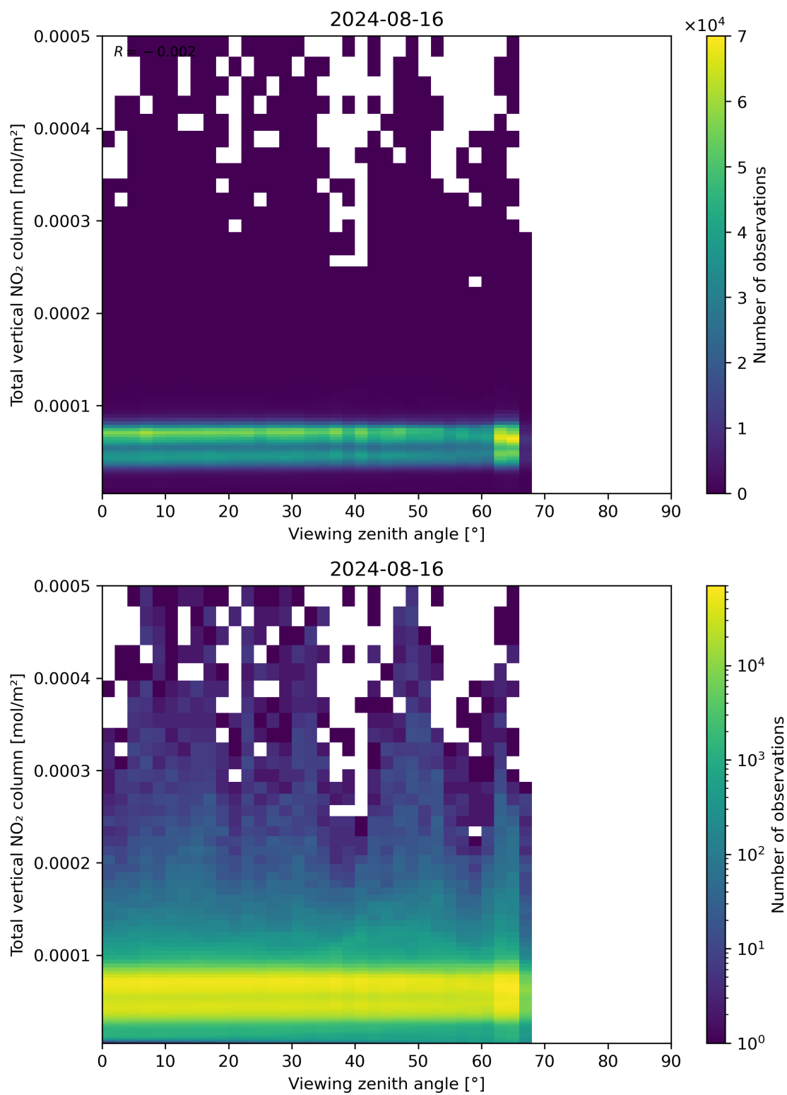
Figure 167: Scatter density plot of “Viewing zenith angle” against “Total vertical NO 2 column” for 2024-08-16 to 2024-08-17.
