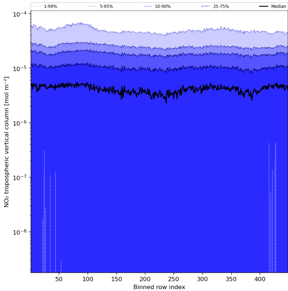
Figure 46: Along track statistics of “NO 2 tropospheric vertical column” for 2024-08-16 to 2024-08-17
