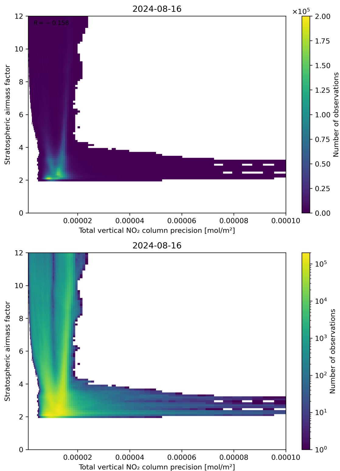
Figure 115: Scatter density plot of “Total vertical NO 2 column precision” against “Stratospheric air mass factor” for 2024-08-16 to 2024-08-17.
