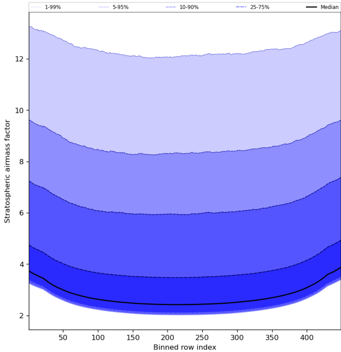
Figure 61: Along track statistics of “Stratospheric airmass factor” for 2024-08-16 to 2024-08-17
