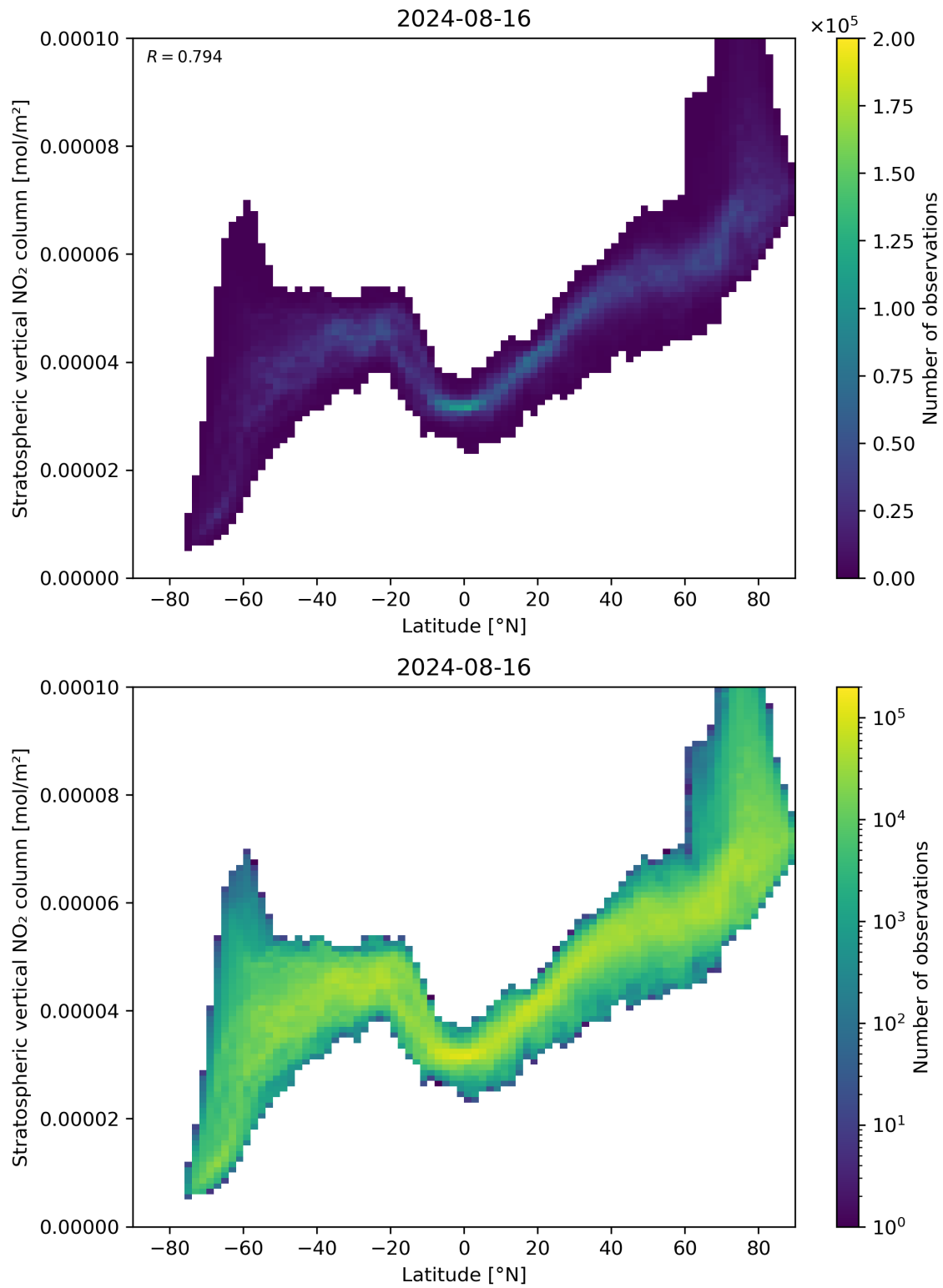
Figure 87: Scatter density plot of “Latitude” against “Stratospheric vertical NO 2 column” for 2024-08-16 to 2024-08-17.
