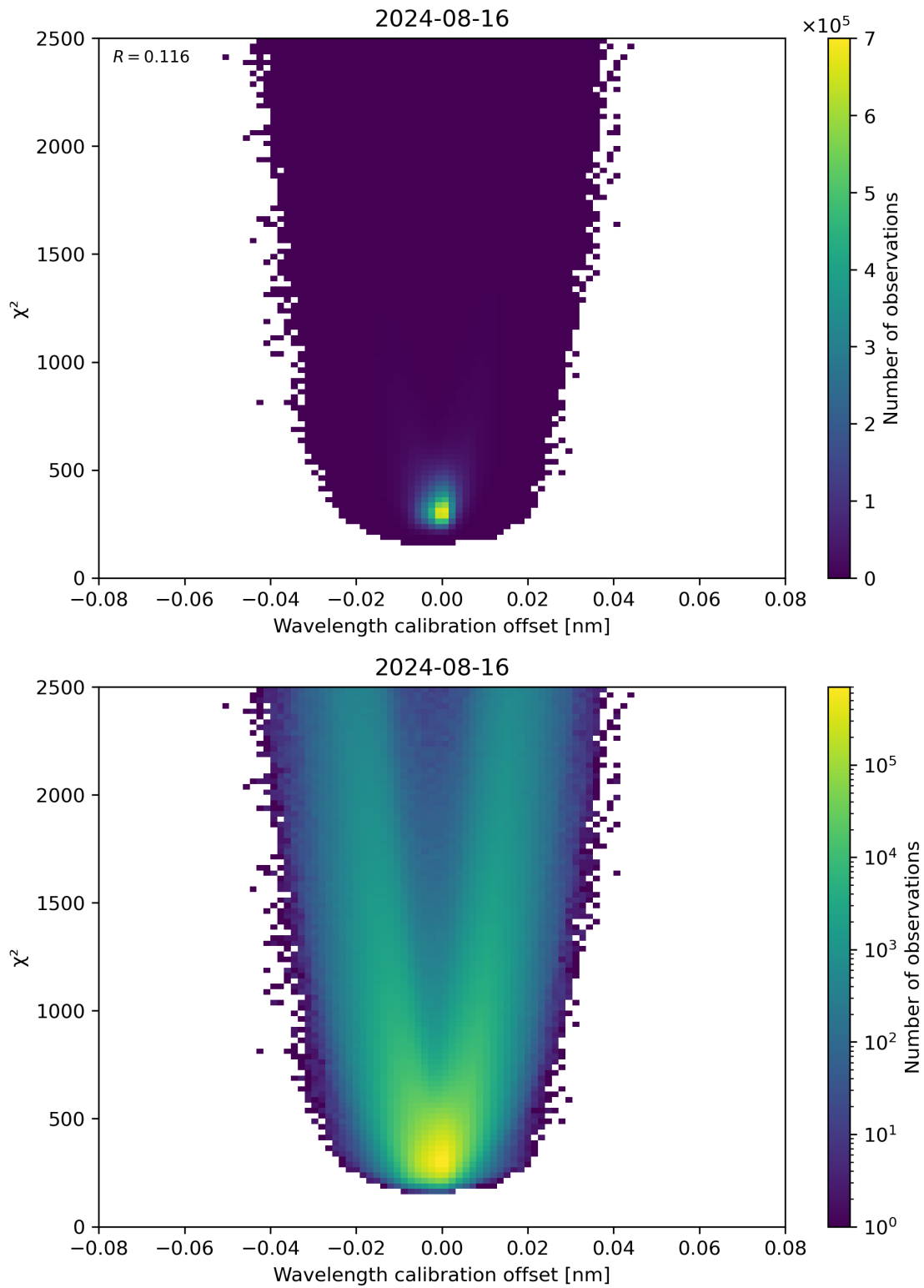
Figure 175: Scatter density plot of “Wavelength calibration offset” against “ \chi^2 ” for 2024-08-16 to 2024-08-17.
