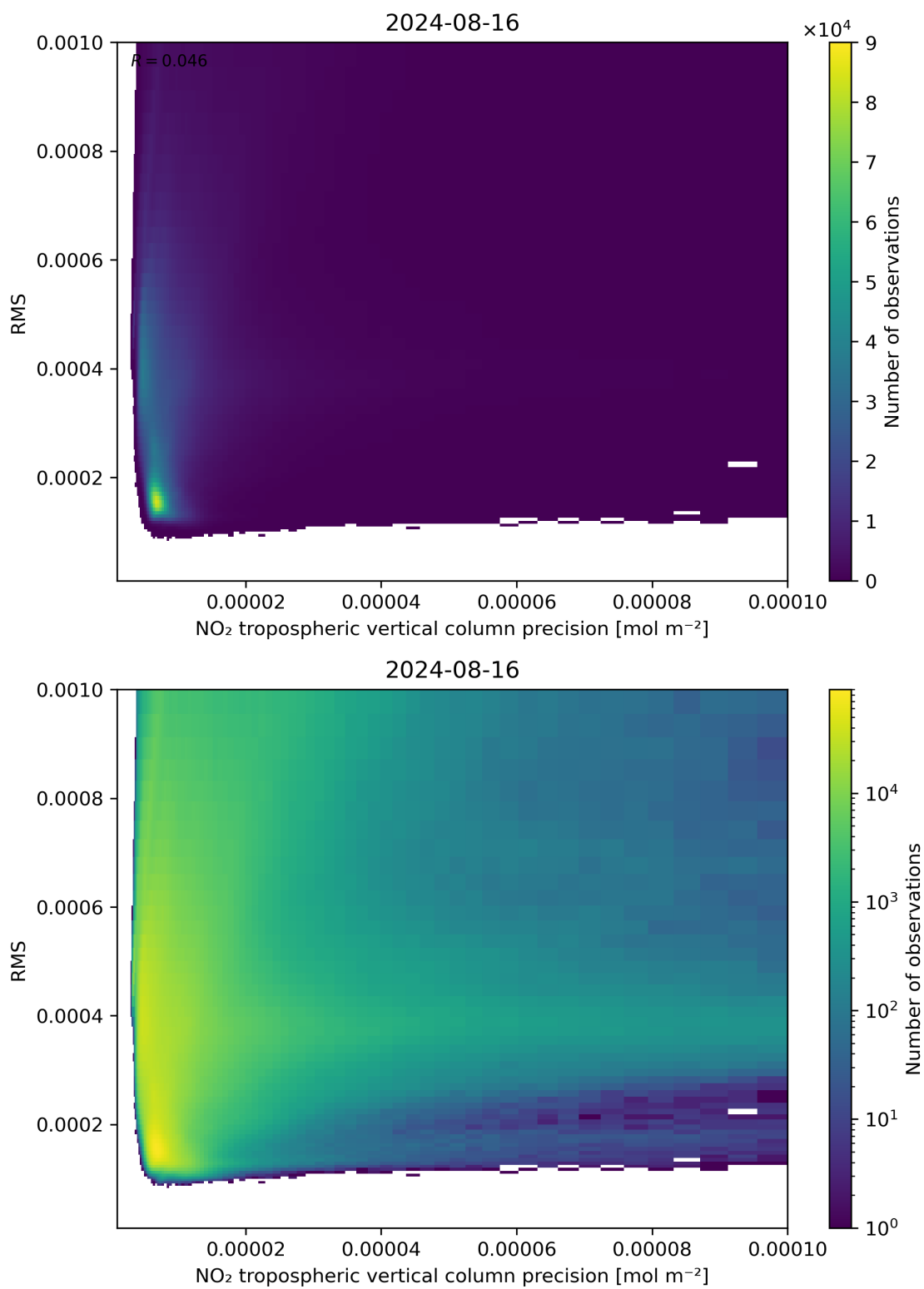
Figure 140: Scatter density plot of “NO 2 tropospheric vertical column precision” against “RMS” for 2024-08-16 to 2024-08-17.
