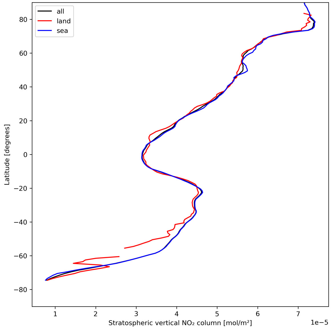
Figure 19: Zonal average of “Stratospheric vertical NO 2 column” for 2024-08-16 to 2024-08-17.
