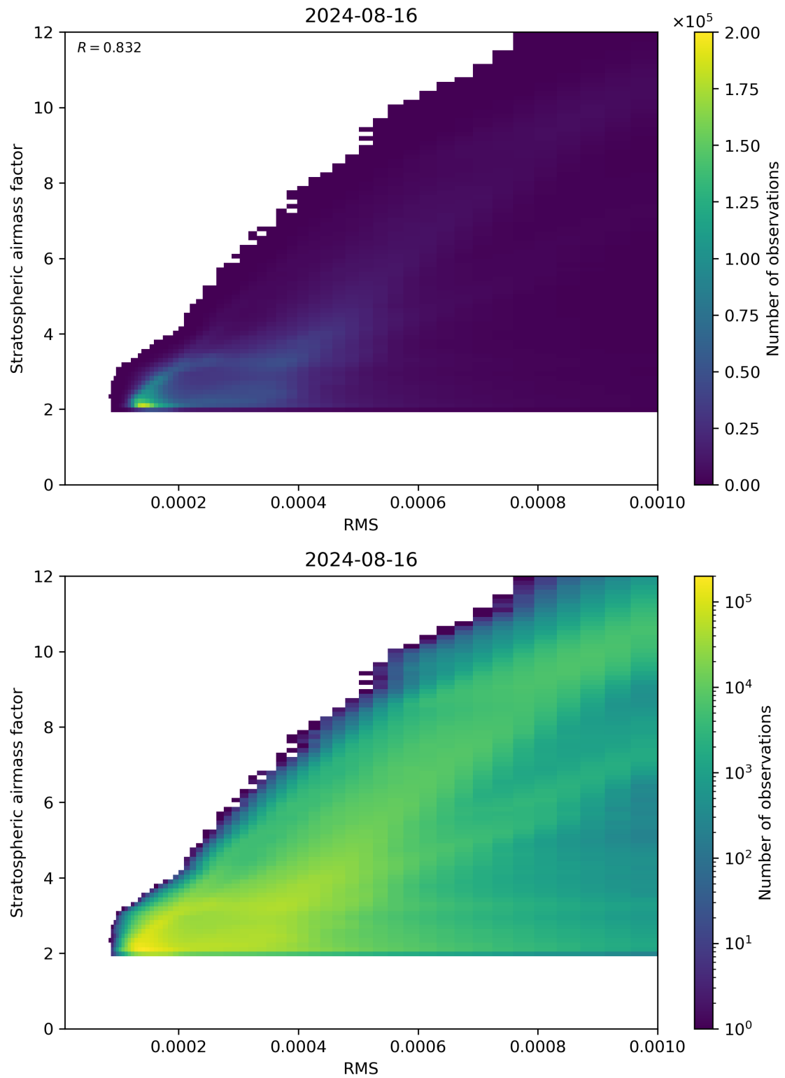
Figure 144: Scatter density plot of “RMS” against “Stratospheric airmass factor” for 2024-08-16 to 2024-08-17.
