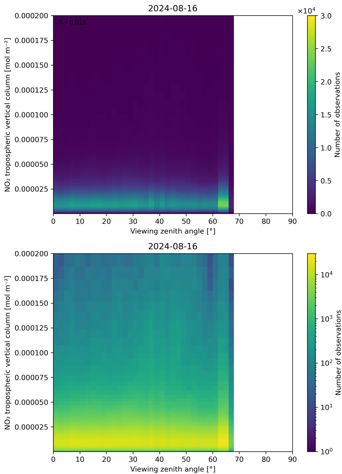
Figure 169: Scatter density plot of “Viewing zenith angle” against “NO 2 tropospheric vertical column” for 2024-08-16 to 2024-08-17.
