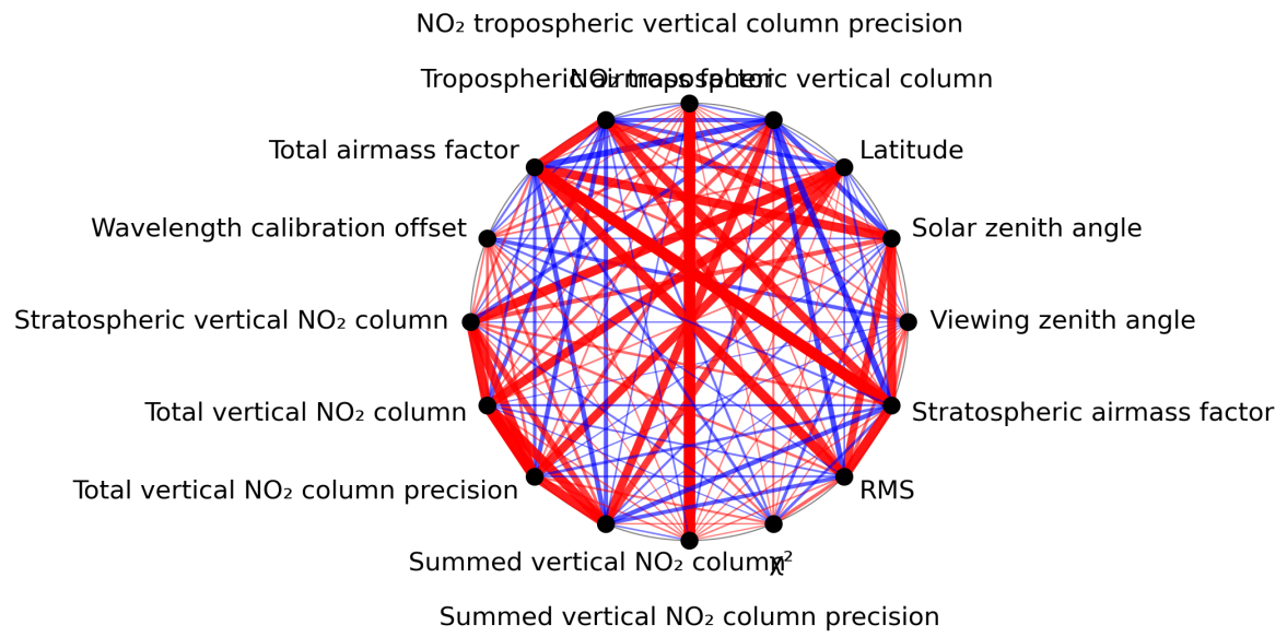
Figure 1: Map of correlation graph for 2024-08-16 to 2024-08-17.
