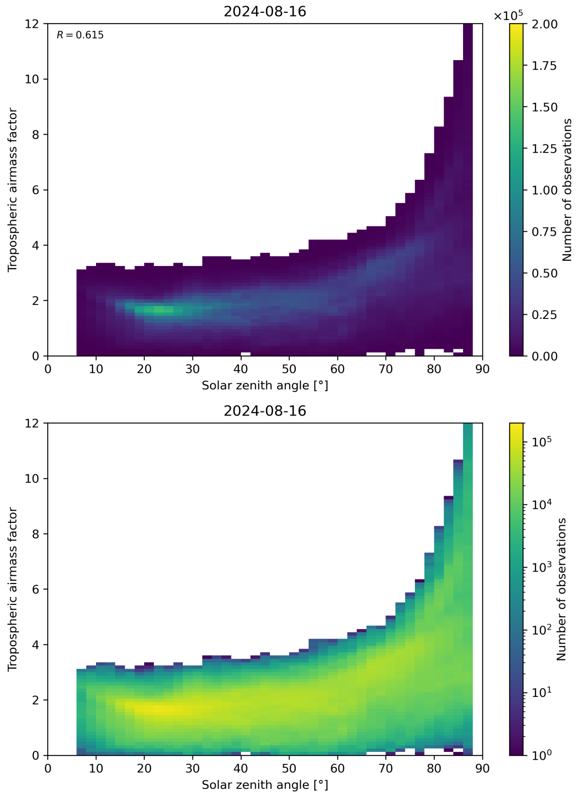
Figure 147: Scatter density plot of “Solar zenith angle” against “Tropospheric airmass factor” for 2024-08-16 to 2024-08-17.
