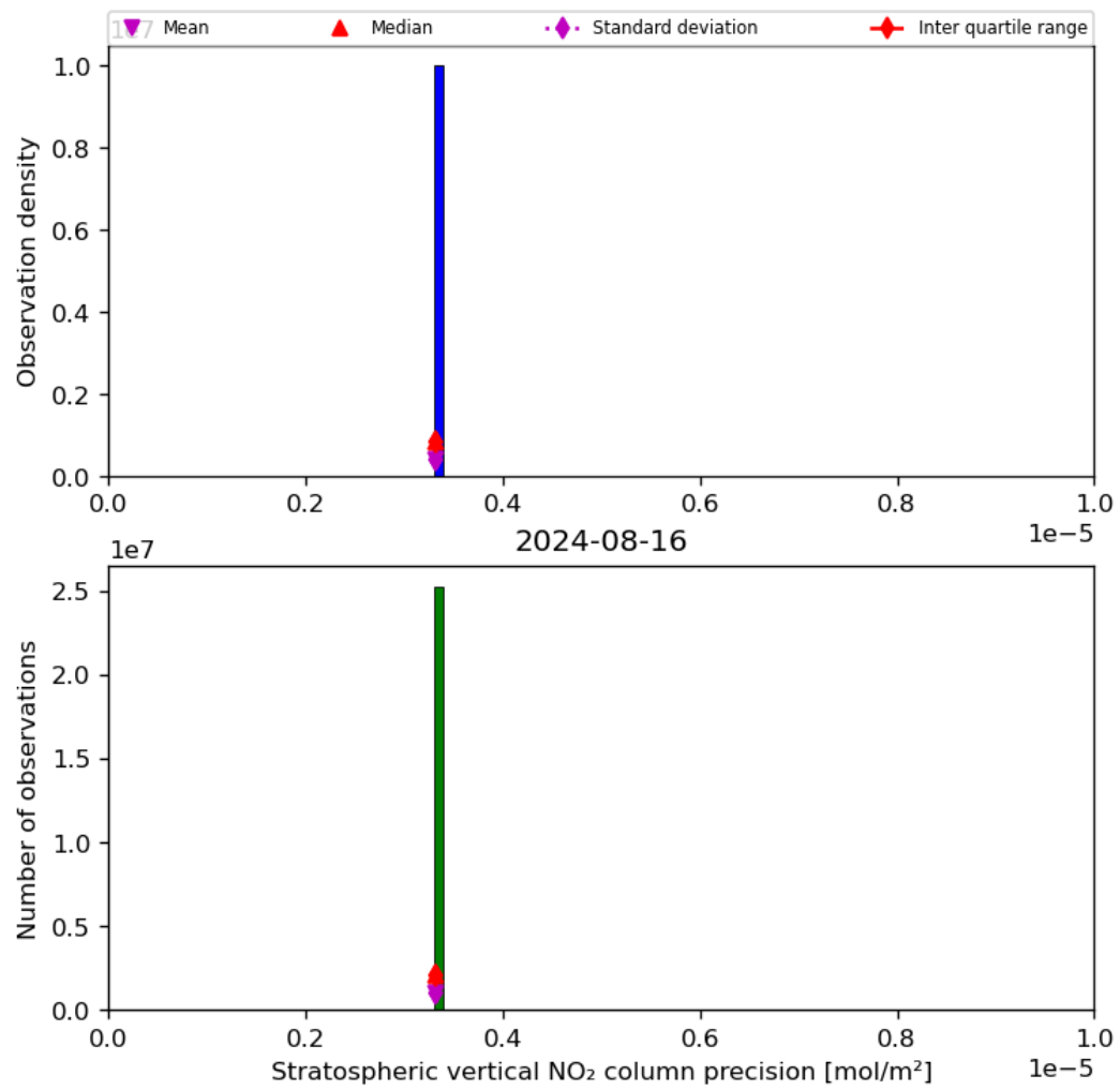
Figure 37: Histogram of “Stratospheric vertical NO 2 column precision” for 2024-08-16 to 2024-08-17
