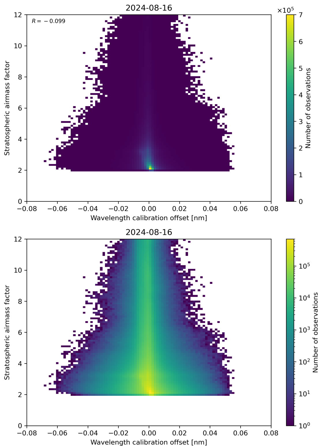
Figure 174: Scatter density plot of “Wavelength calibration offset” against “Stratospheric air mass factor” for 2024-08-16 to 2024-08-17.
