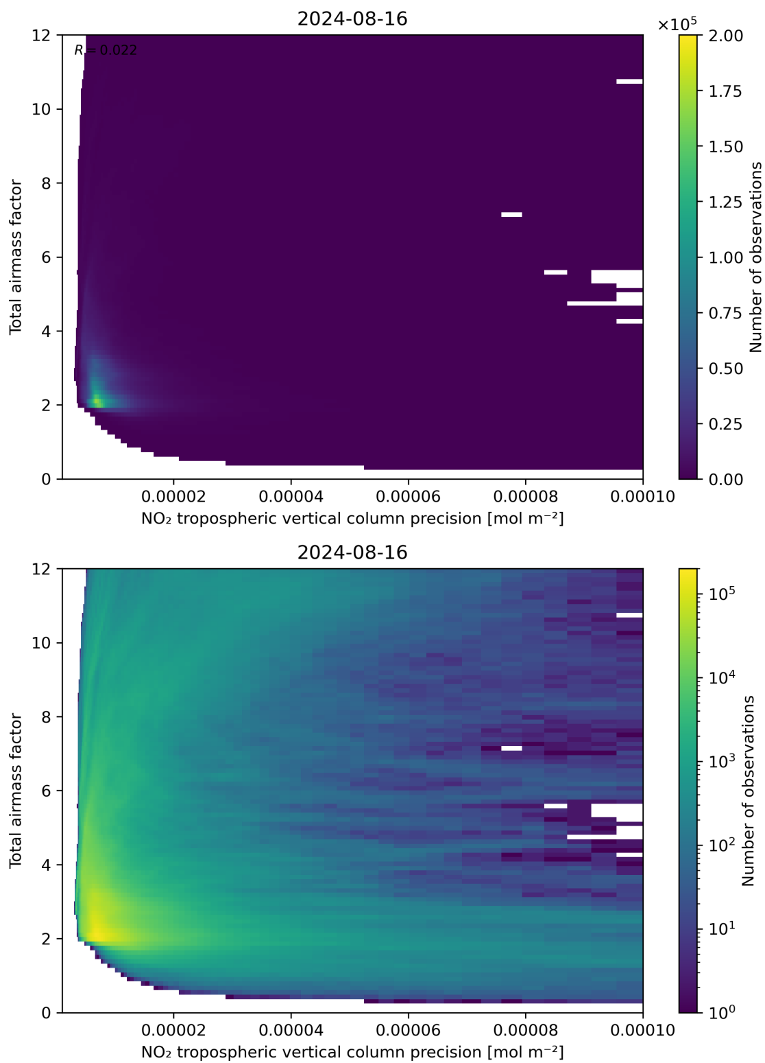
Figure 132: Scatter density plot of “NO 2 tropospheric vertical column precision” against “Total air mass factor” for 2024-08-16 to 2024-08-17.
