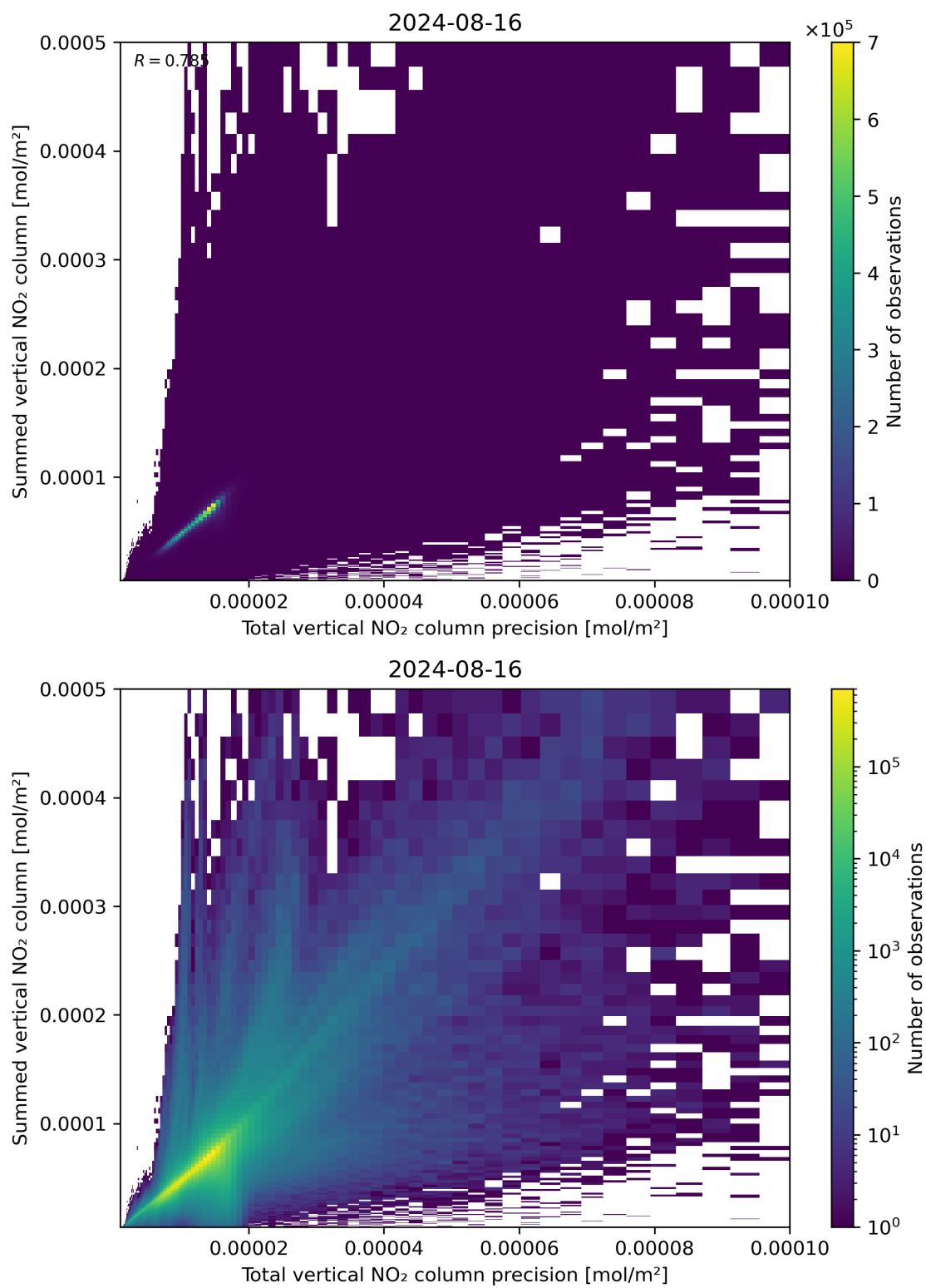
Figure 117: Scatter density plot of “Total vertical NO 2 column precision” against “Summed vertical NO 2 column” for 2024-08-16 to 2024-08-17.
