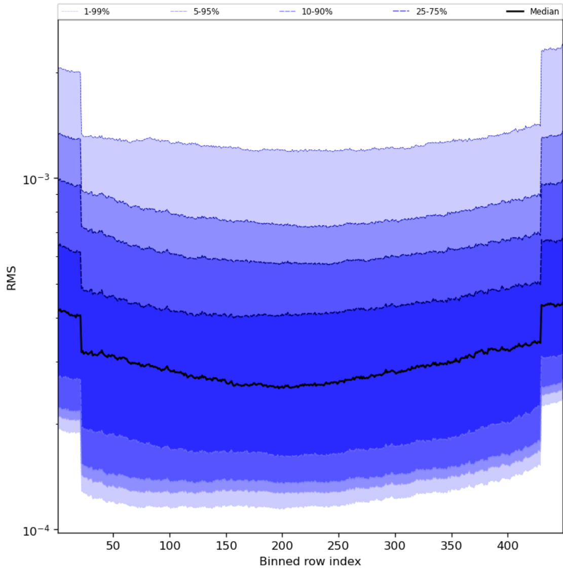
Figure 60: Along track statistics of “RMS” for 2024-08-16 to 2024-08-17
