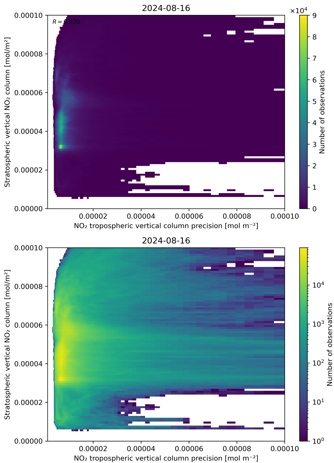
Figure 135: Scatter density plot of “NO 2 tropospheric vertical column precision” against “Stratospheric vertical NO 2 column” for 2024-08-16 to 2024-08-17.
