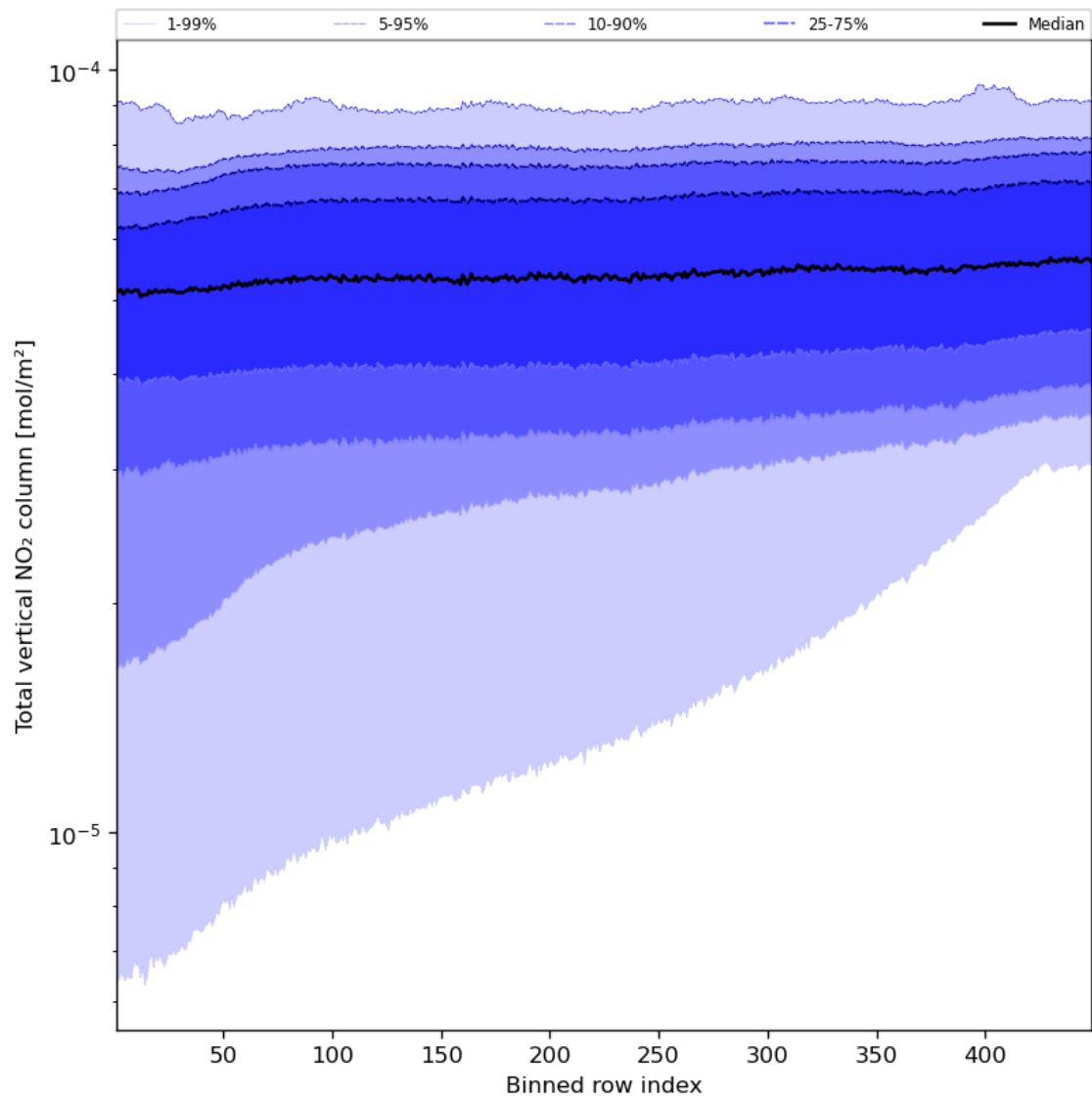
Figure 55: Along track statistics of “Total vertical NO 2 column” for 2024-08-16 to 2024-08-17
