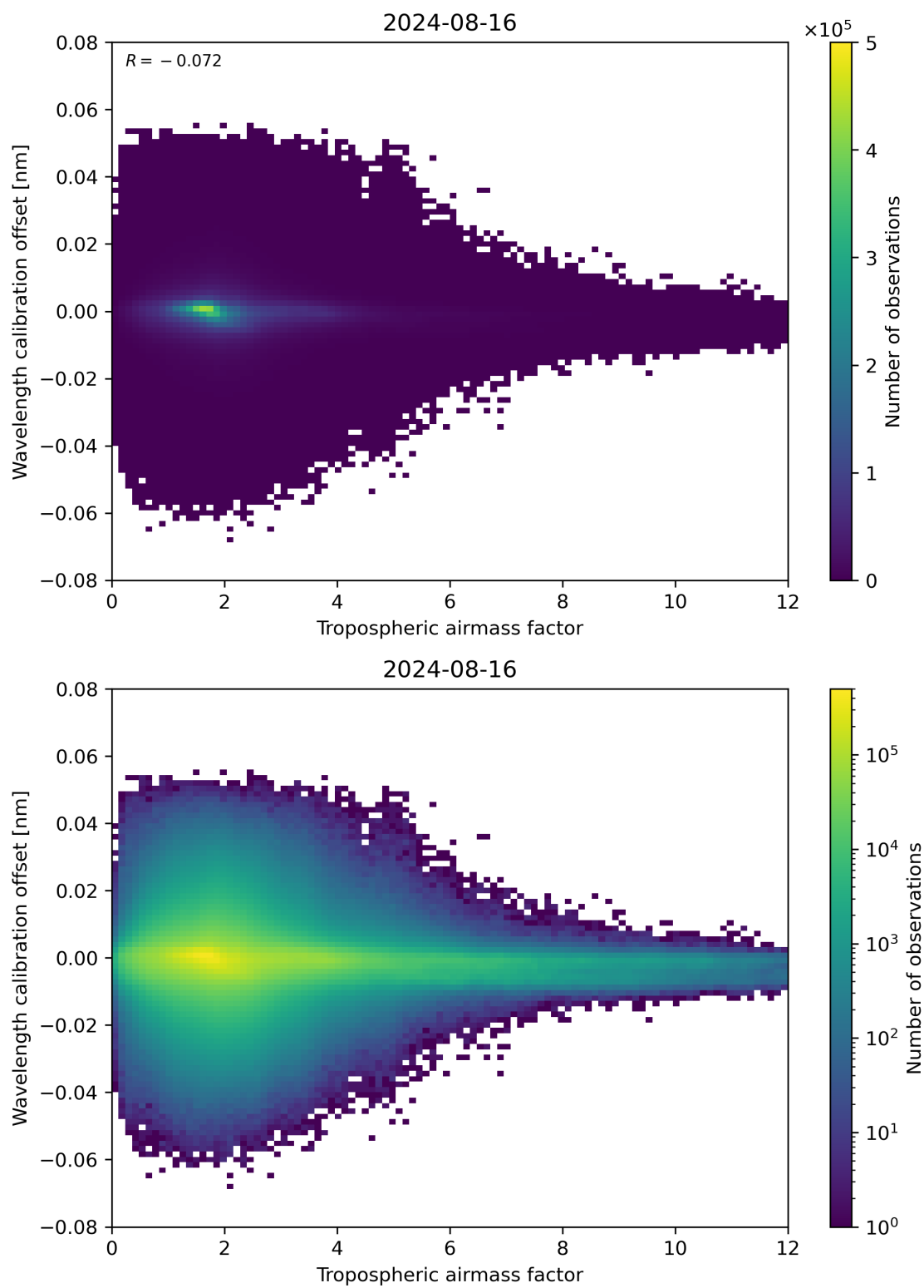
Figure 80: Scatter density plot of “Tropospheric airmass factor” against “Wavelength calibration offset” for 2024-08-16 to 2024-08-17.
