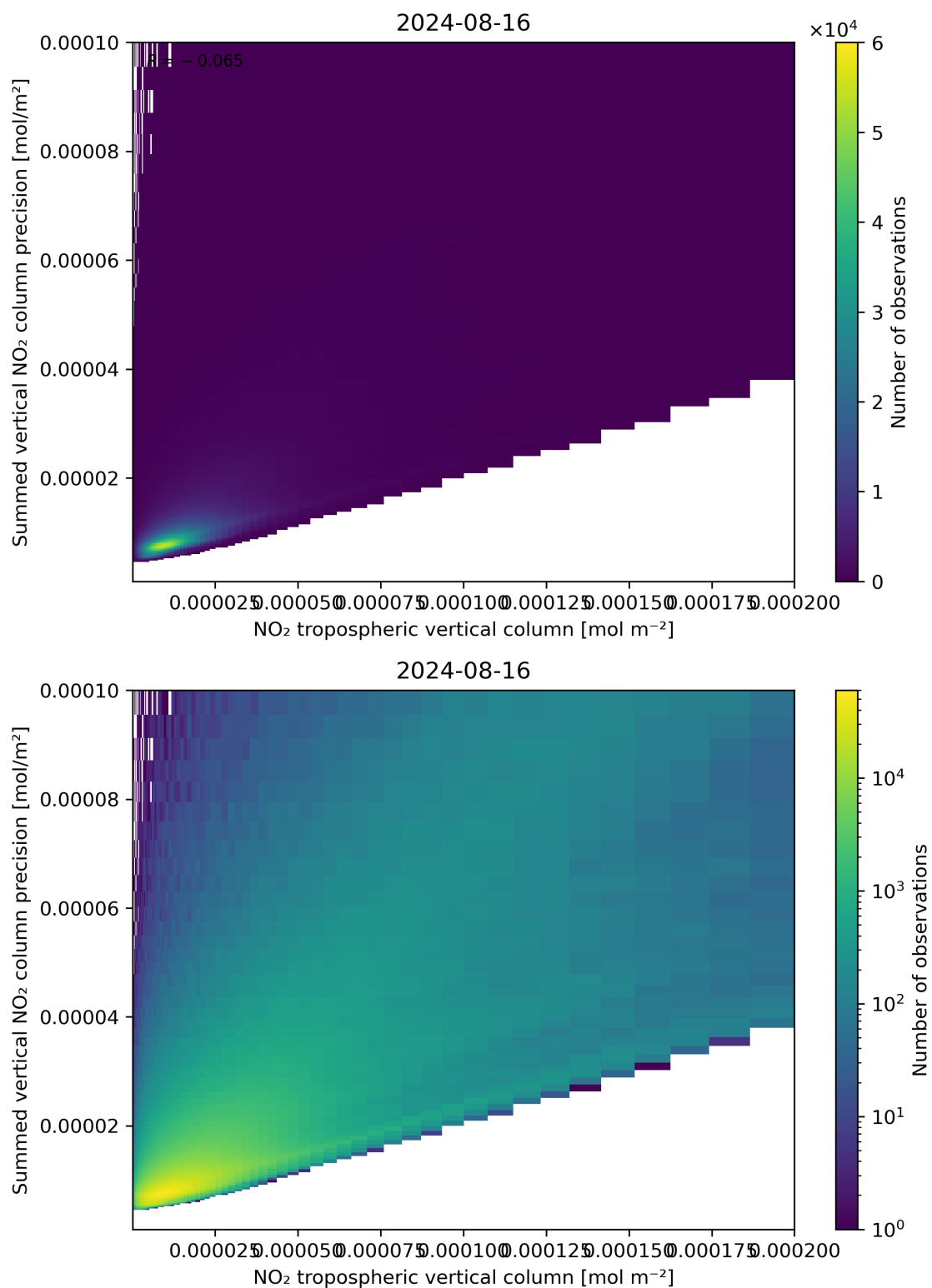
Figure 127: Scatter density plot of “NO 2 tropospheric vertical column” against “Summed vertical NO 2 column precision” for 2024-08-16 to 2024-08-17.
