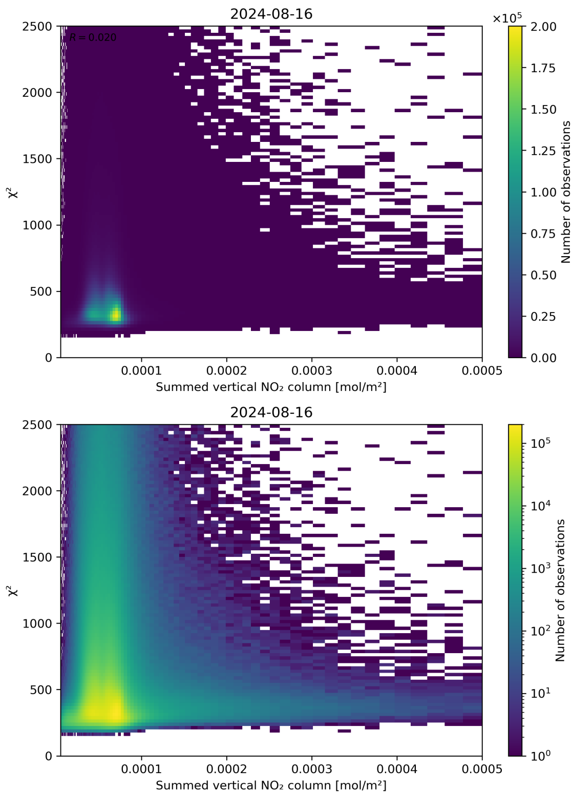
Figure 104: Scatter density plot of “Summed vertical NO 2 column” against “ \chi^2 ” for 2024-08-16 to 2024-08-17.
