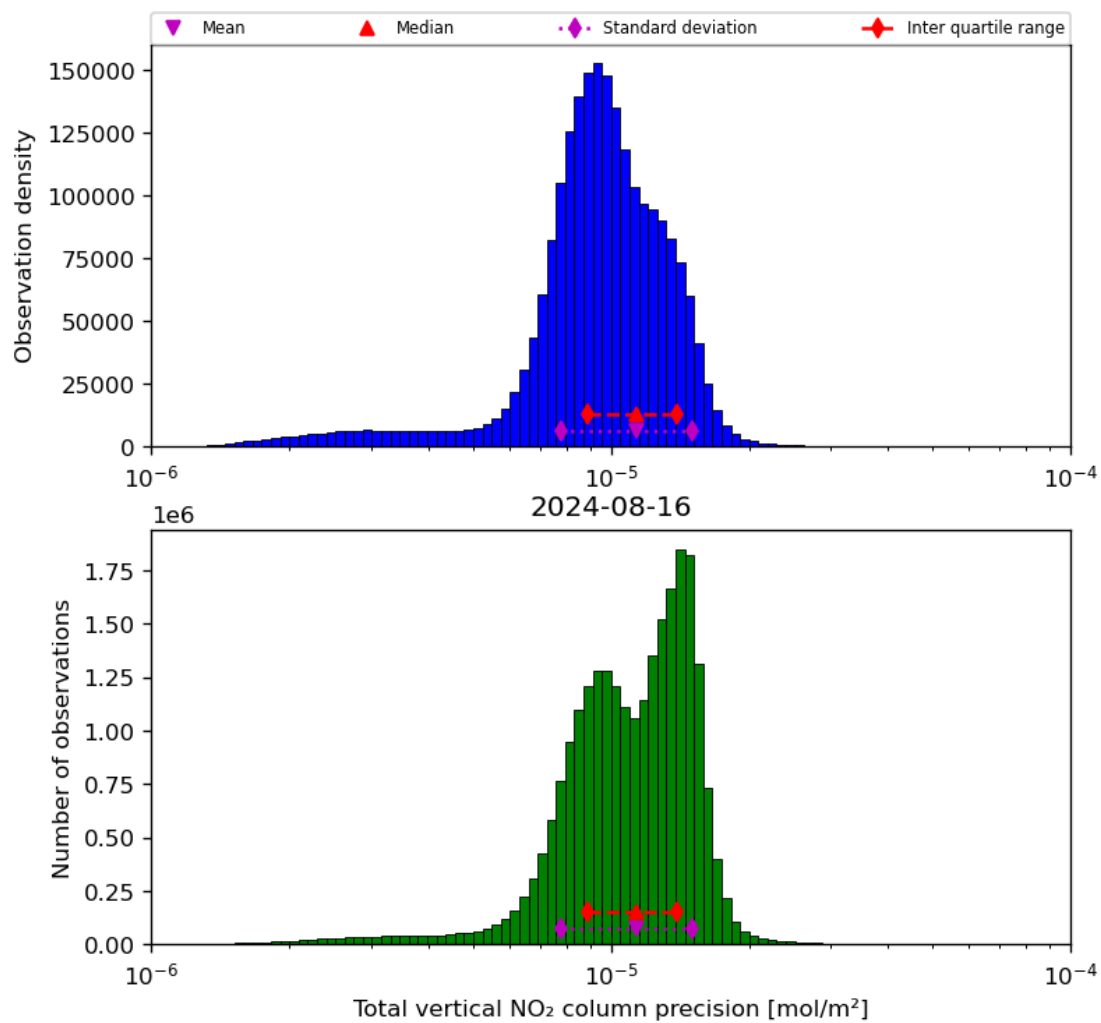
Figure 39: Histogram of “Total vertical NO 2 column precision” for 2024-08-16 to 2024-08-17
