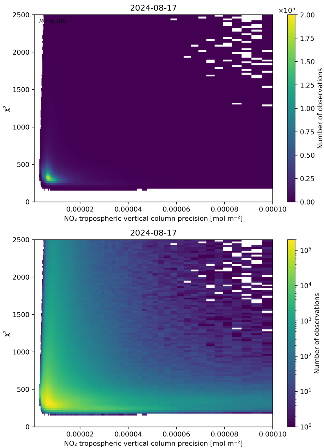
Figure 134: Scatter density plot of “NO 2 tropospheric vertical column precision” against “ \chi^2 ” for 2024-08-16 to 2024-08-18.
