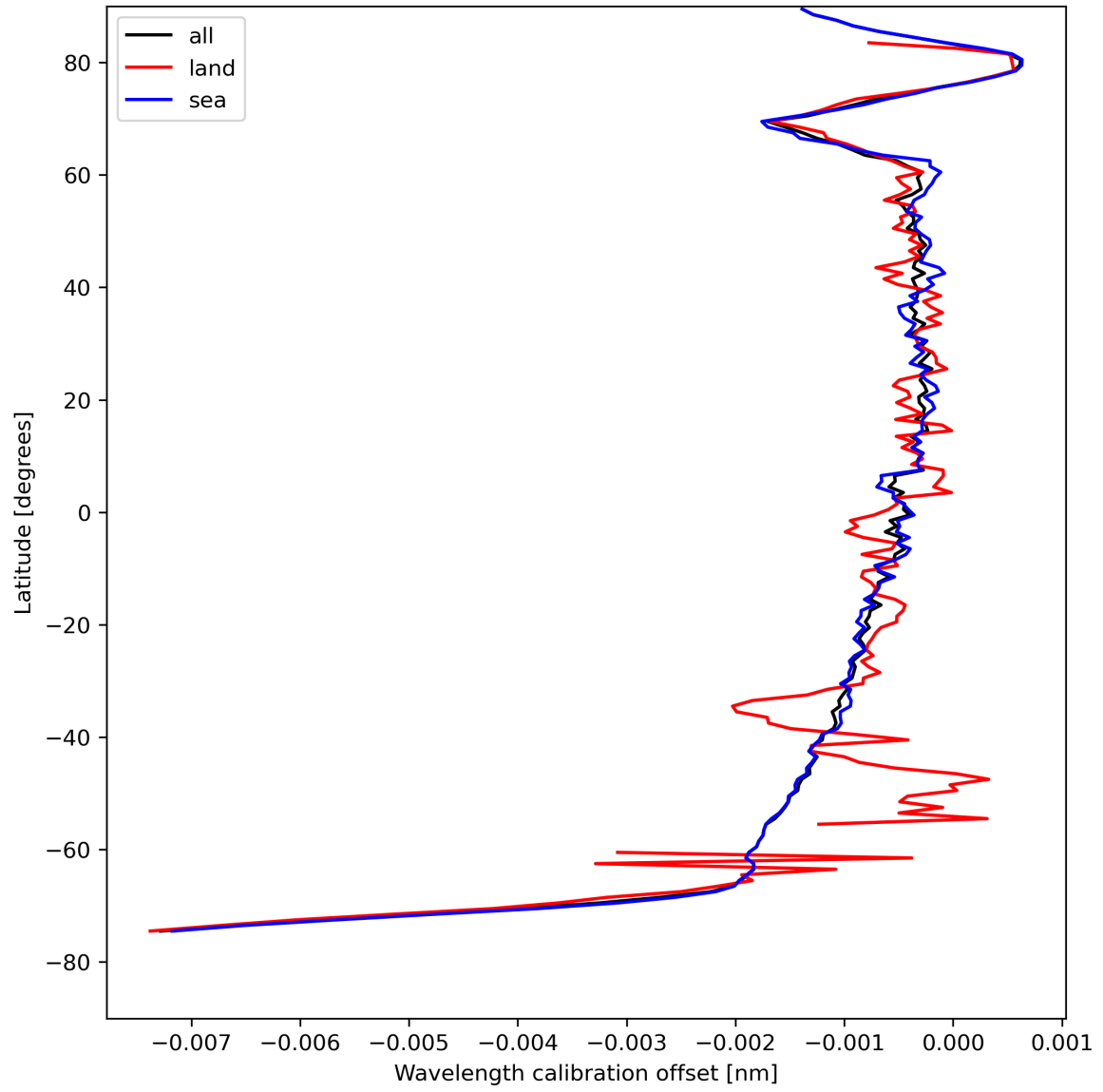
Figure 18: Zonal average of “Wavelength calibration offset” for 2024-08-16 to 2024-08-18.
