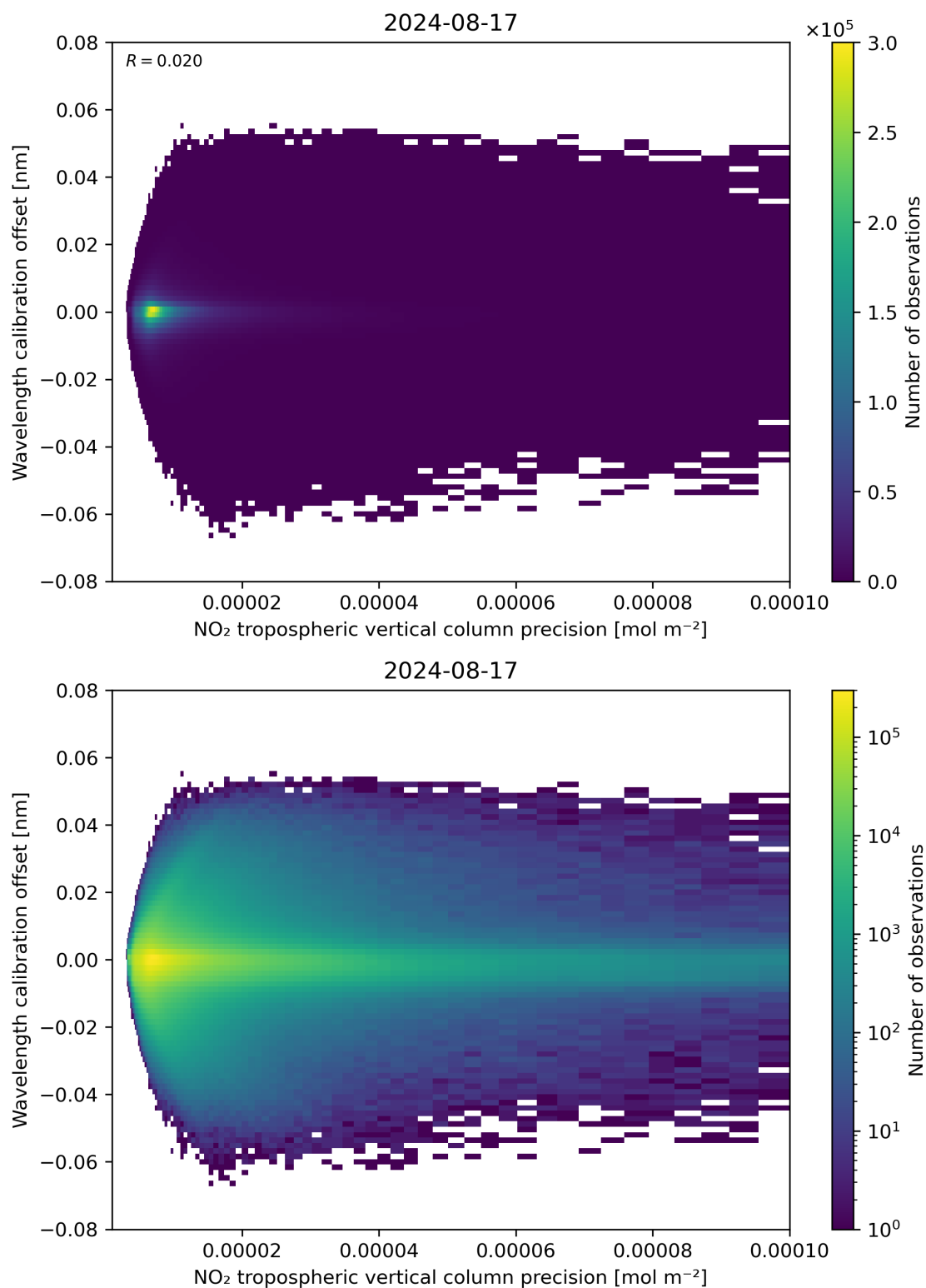
Figure 141: Scatter density plot of “NO 2 tropospheric vertical column precision” against “Wavelength calibration offset” for 2024-08-16 to 2024-08-18.
