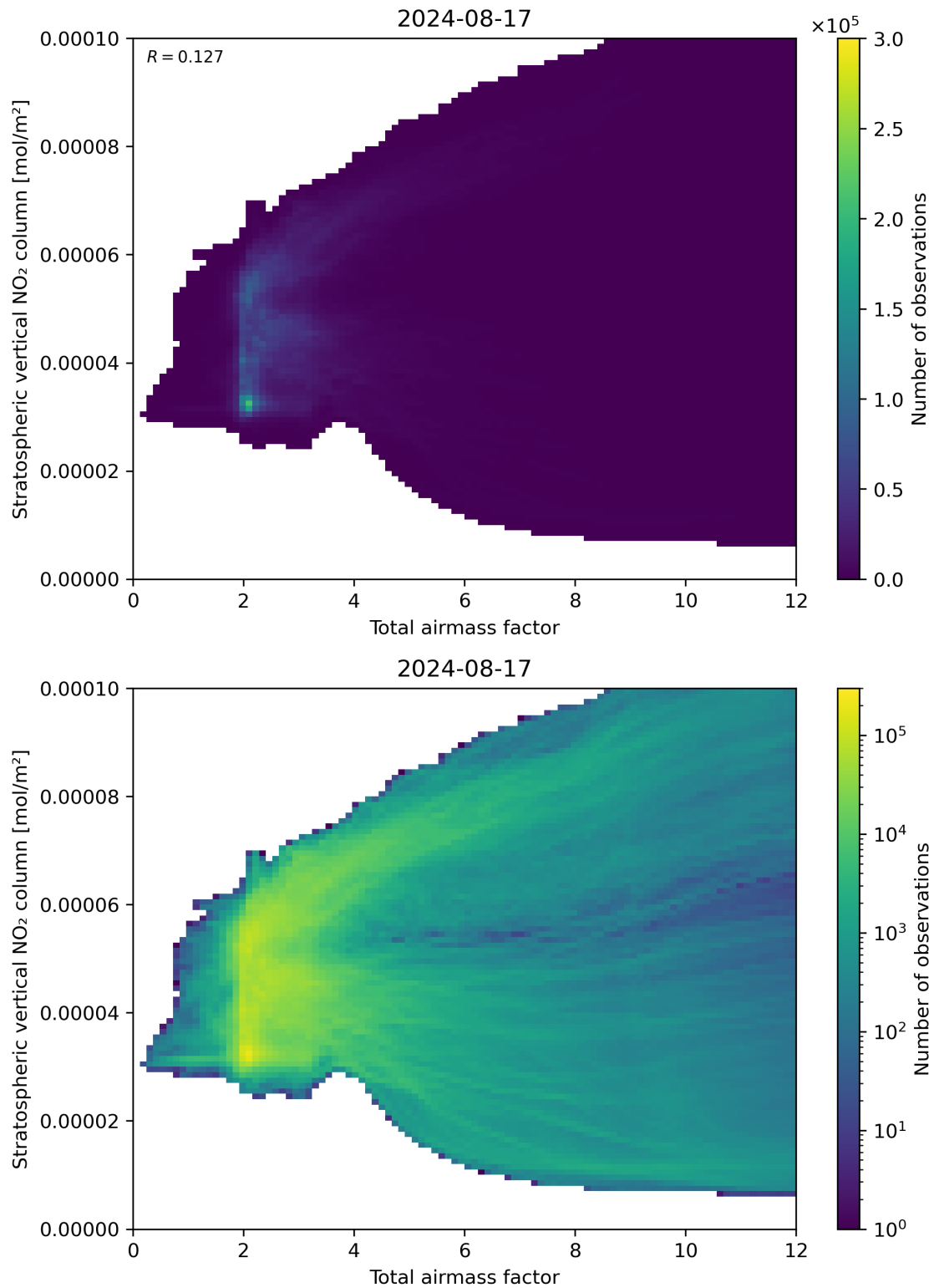
Figure 64: Scatter density plot of “Total airmass factor” against “Stratospheric vertical NO 2 column” for 2024-08-16 to 2024-08-18.
