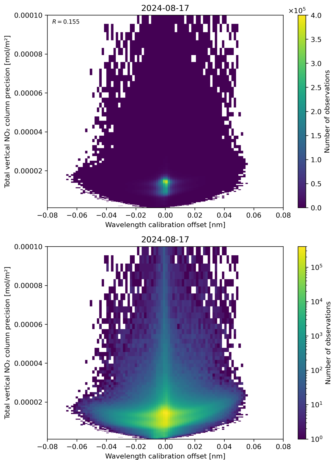
Figure 180: Scatter density plot of “Wavelength calibration offset” against “Total vertical NO 2 column precision” for 2024-08-16 to 2024-08-18.
