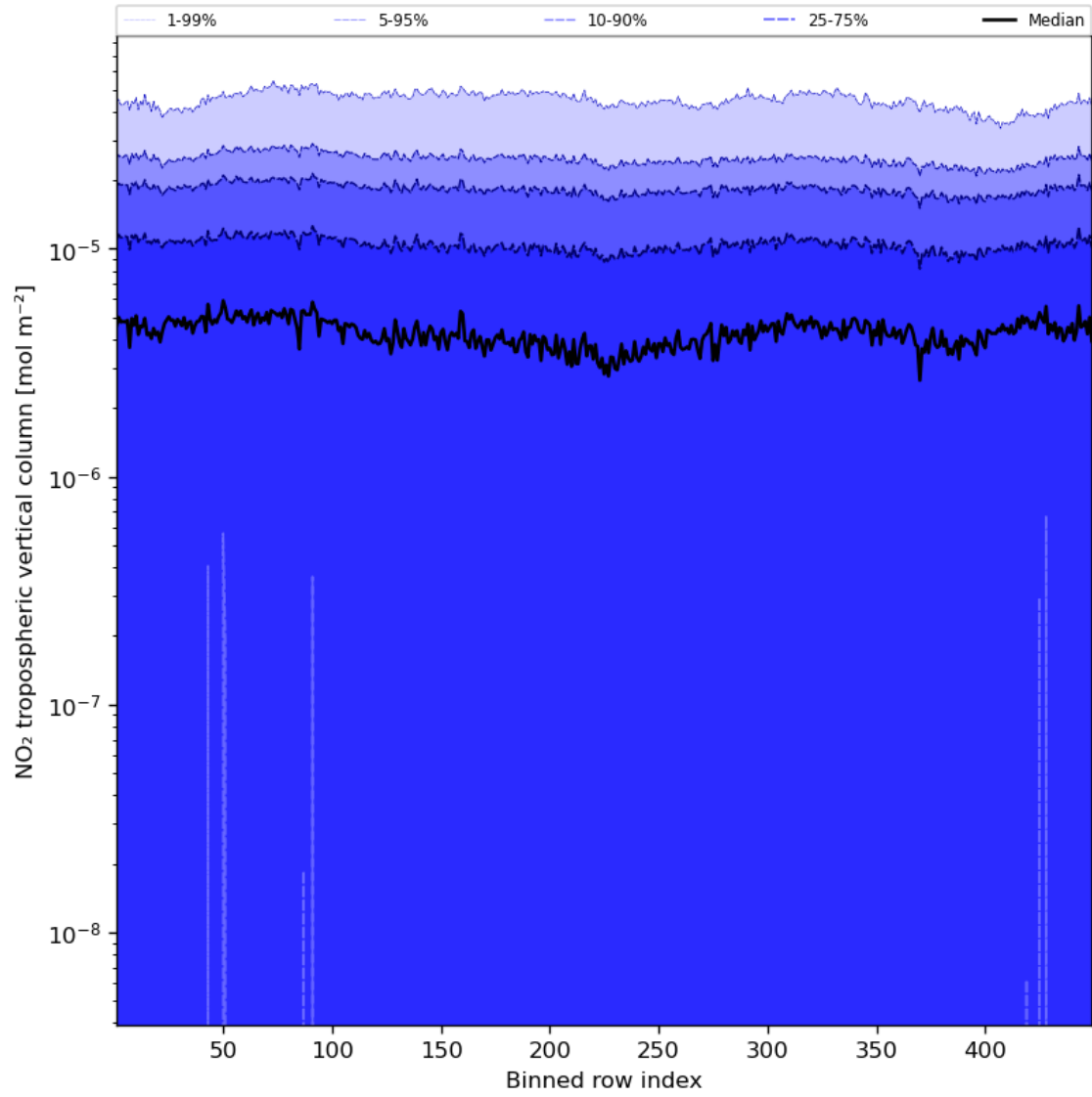
Figure 46: Along track statistics of "NO 2 tropospheric vertical column" for 2024-08-16 to 2024-08-18
