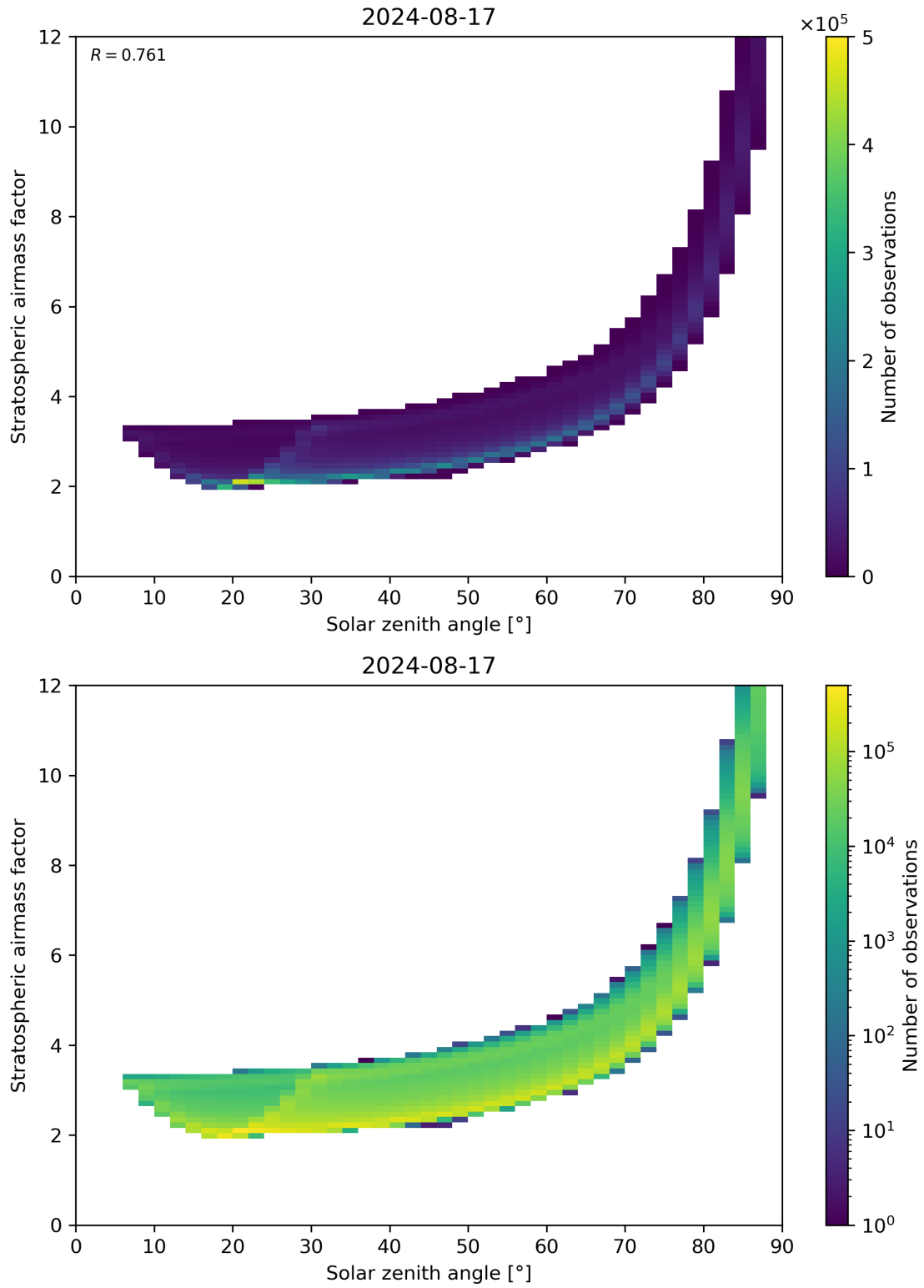
Figure 145: Scatter density plot of “Solar zenith angle” against “Stratospheric airmass factor” for 2024-08-16 to 2024-08-18.
