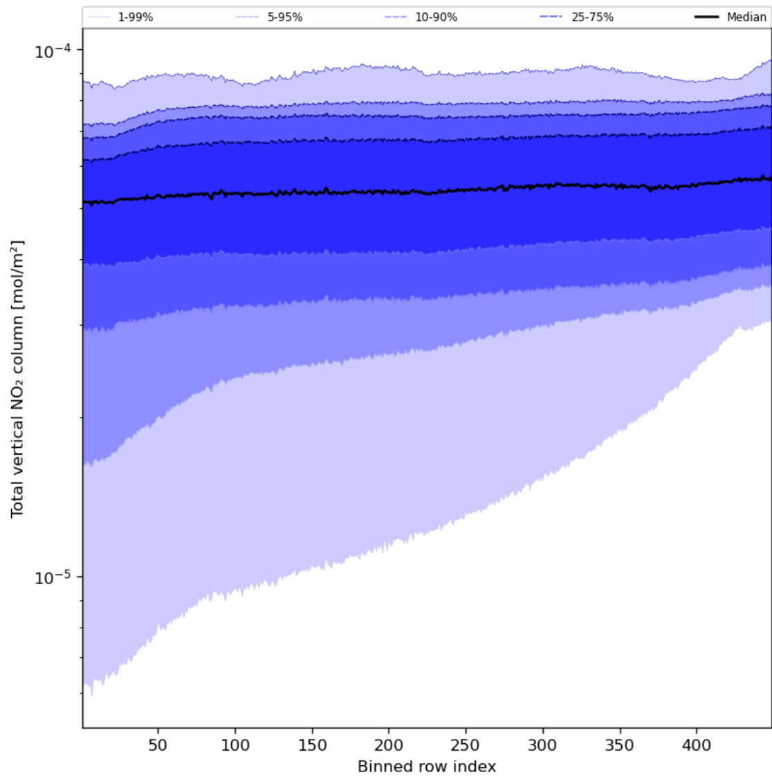
Figure 55: Along track statistics of “Total vertical NO 2 column” for 2024-08-16 to 2024-08-18
