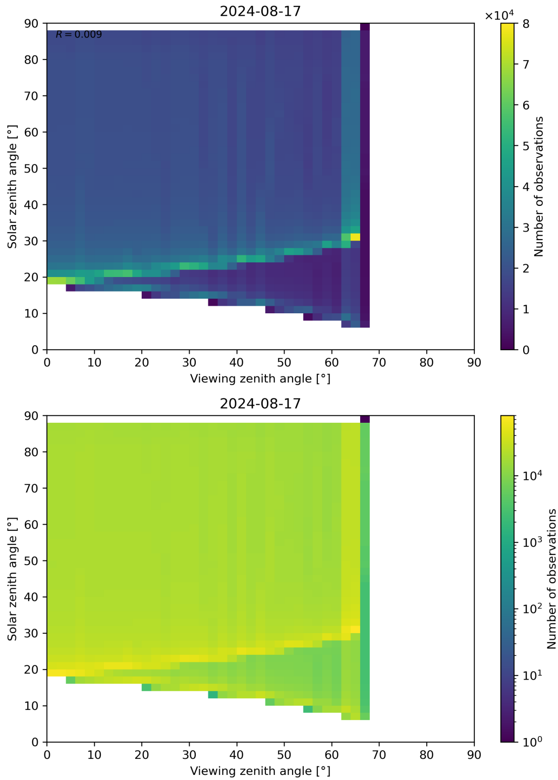
Figure 172: Scatter density plot of “Viewing zenith angle” against “Solar zenith angle” for 2024-08-16 to 2024-08-18.
