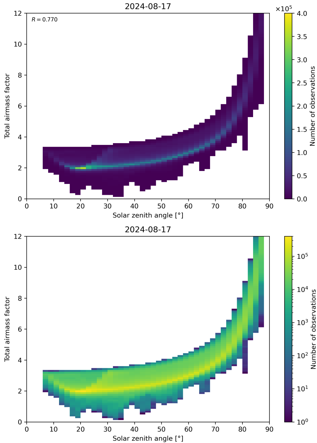
Figure 146: Scatter density plot of “Solar zenith angle” against “Total air mass factor” for 2024-08-16 to 2024-08-18.
