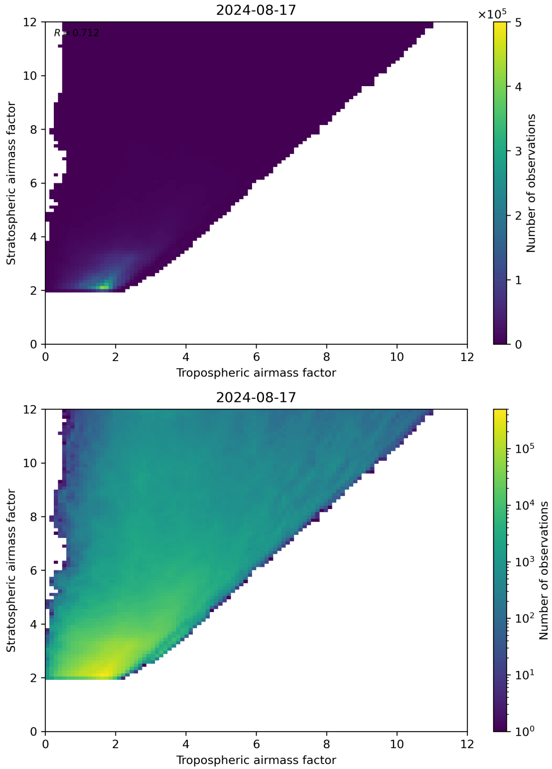
Figure 71: Scatter density plot of “Tropospheric airmass factor” against “Stratospheric airmass factor” for 2024-08-16 to 2024-08-18.
