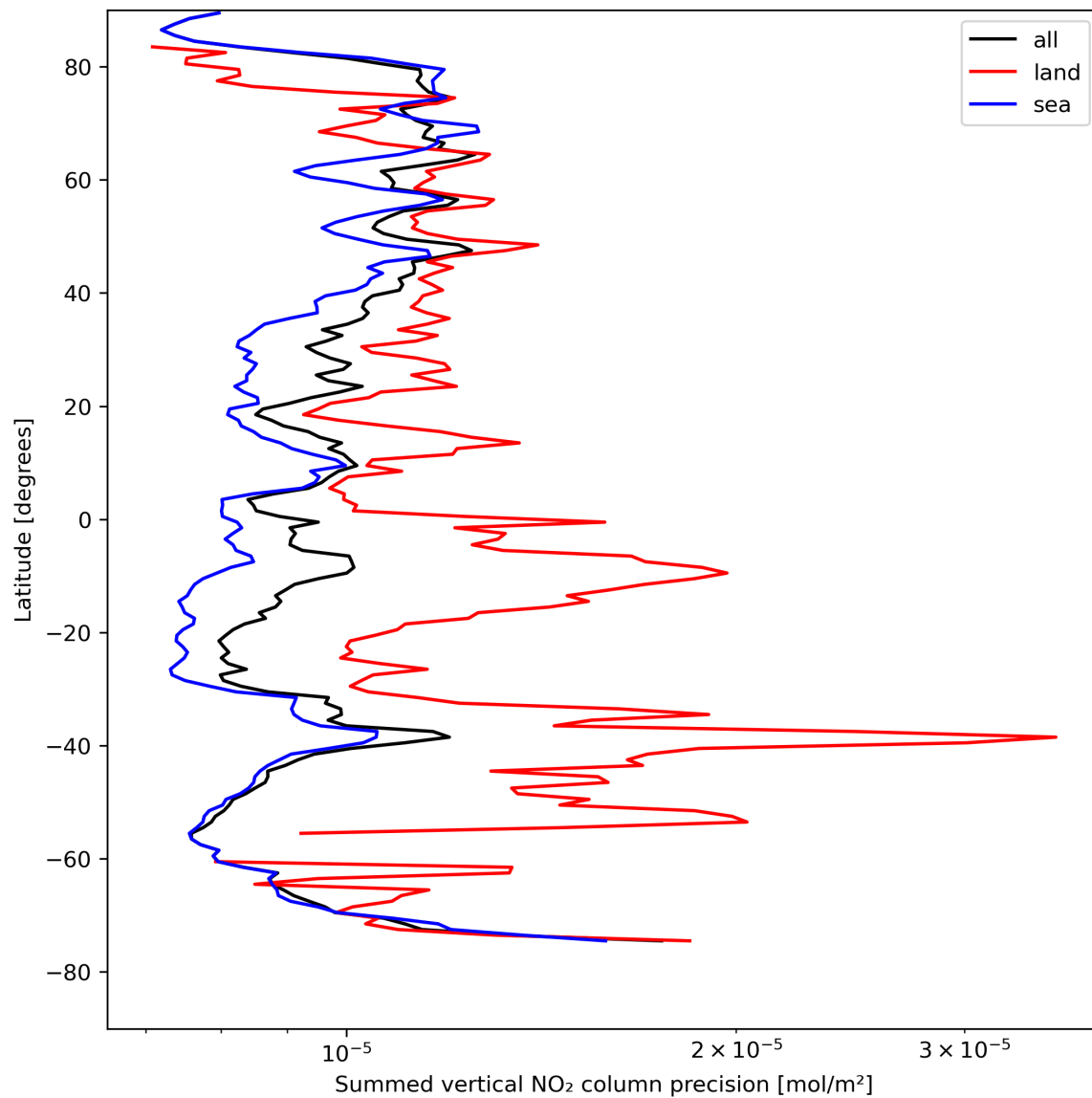
Figure 24: Zonal average of “Summed vertical NO 2 column precision” for 2024-08-16 to 2024-08-18.
