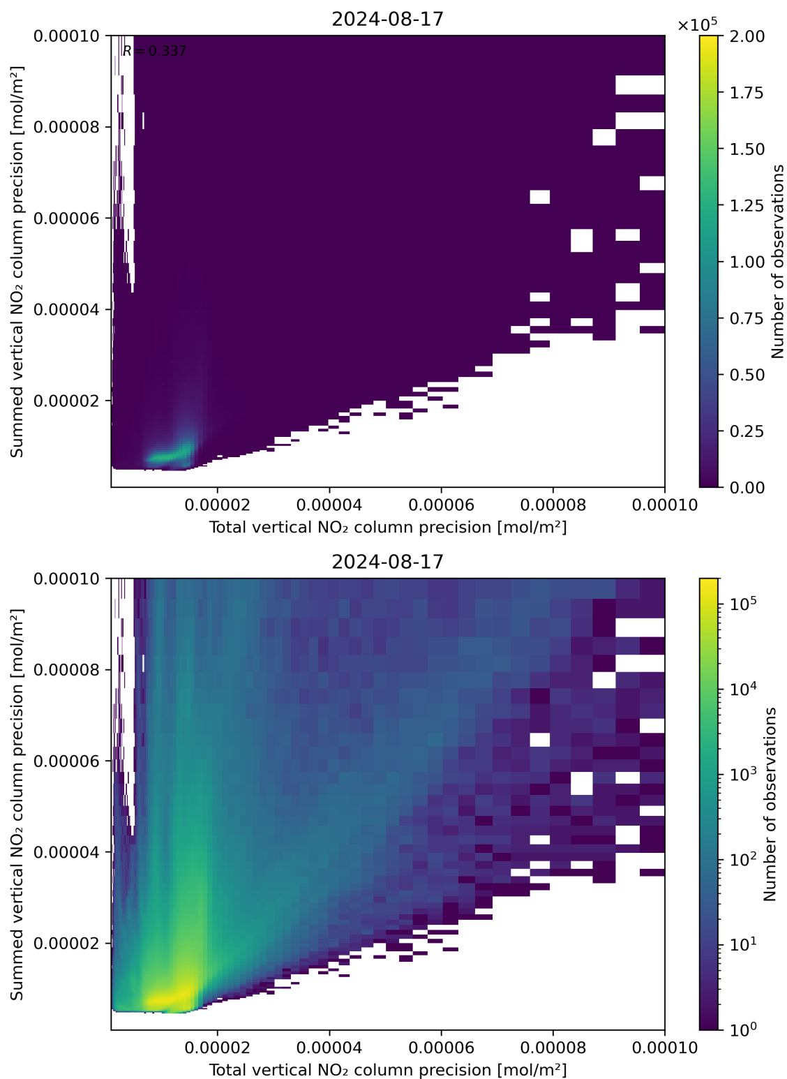
Figure 118: Scatter density plot of “Total vertical NO 2 column precision” against “Summed vertical NO 2 column precision” for 2024-08-16 to 2024-08-18.
