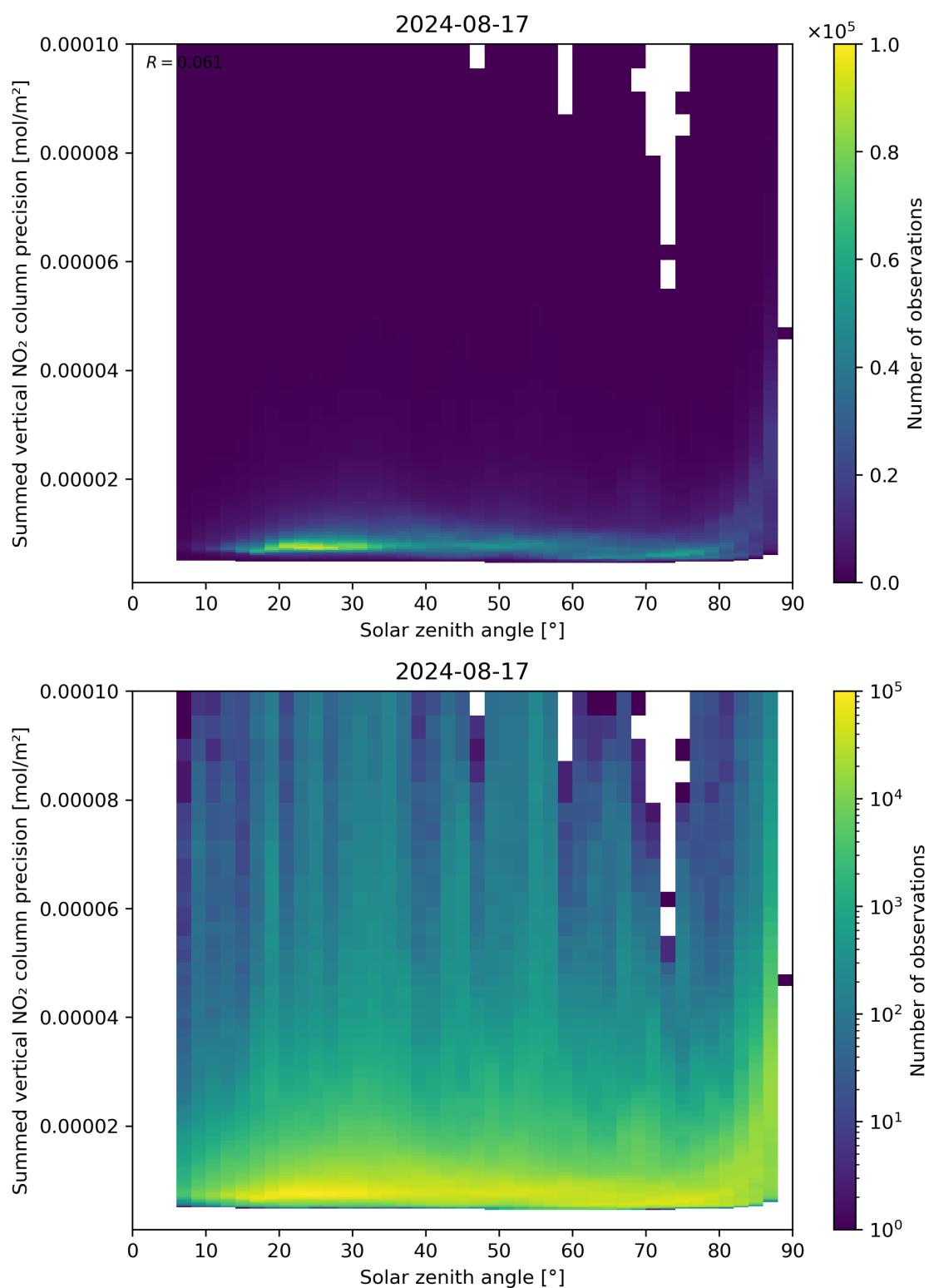
Figure 152: Scatter density plot of “Solar zenith angle” against “Summed vertical NO 2 column precision” for 2024-08-16 to 2024-08-18.
