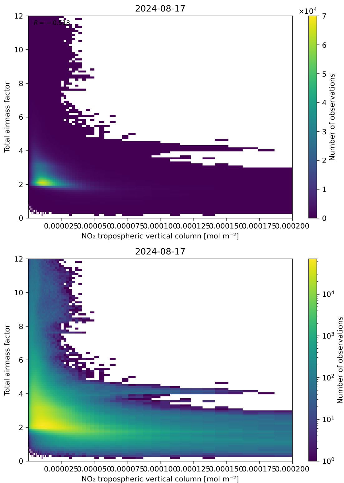
Figure 122: Scatter density plot of “NO 2 tropospheric vertical column” against “Total air mass factor” for 2024-08-16 to 2024-08-18.
