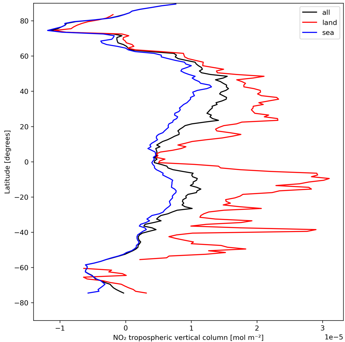
Figure 12: Zonal average of “NO 2 tropospheric vertical column” for 2024-08-16 to 2024-08-18.
