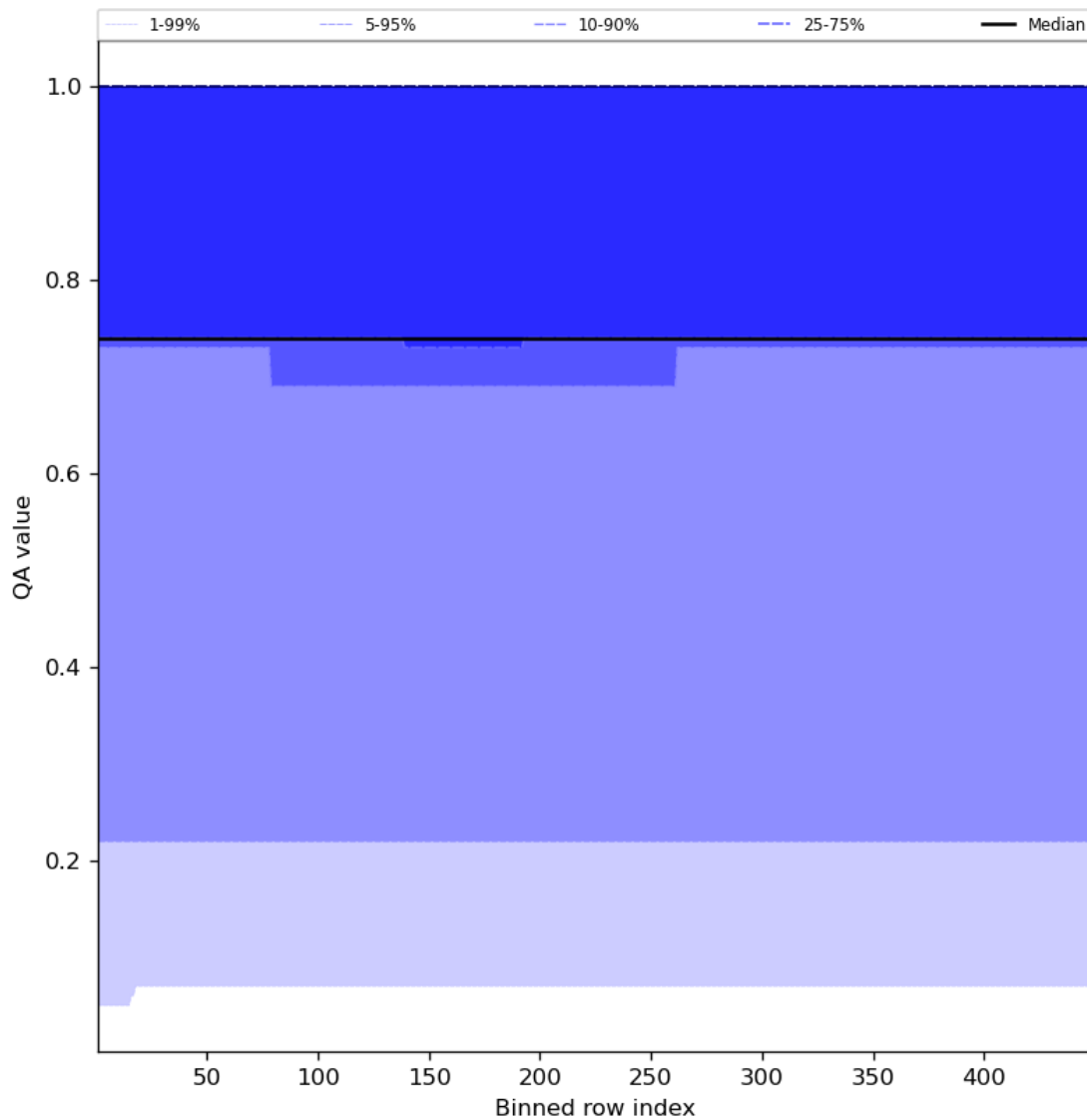
Figure 45: Along track statistics of “QA value” for 2024-08-16 to 2024-08-18
