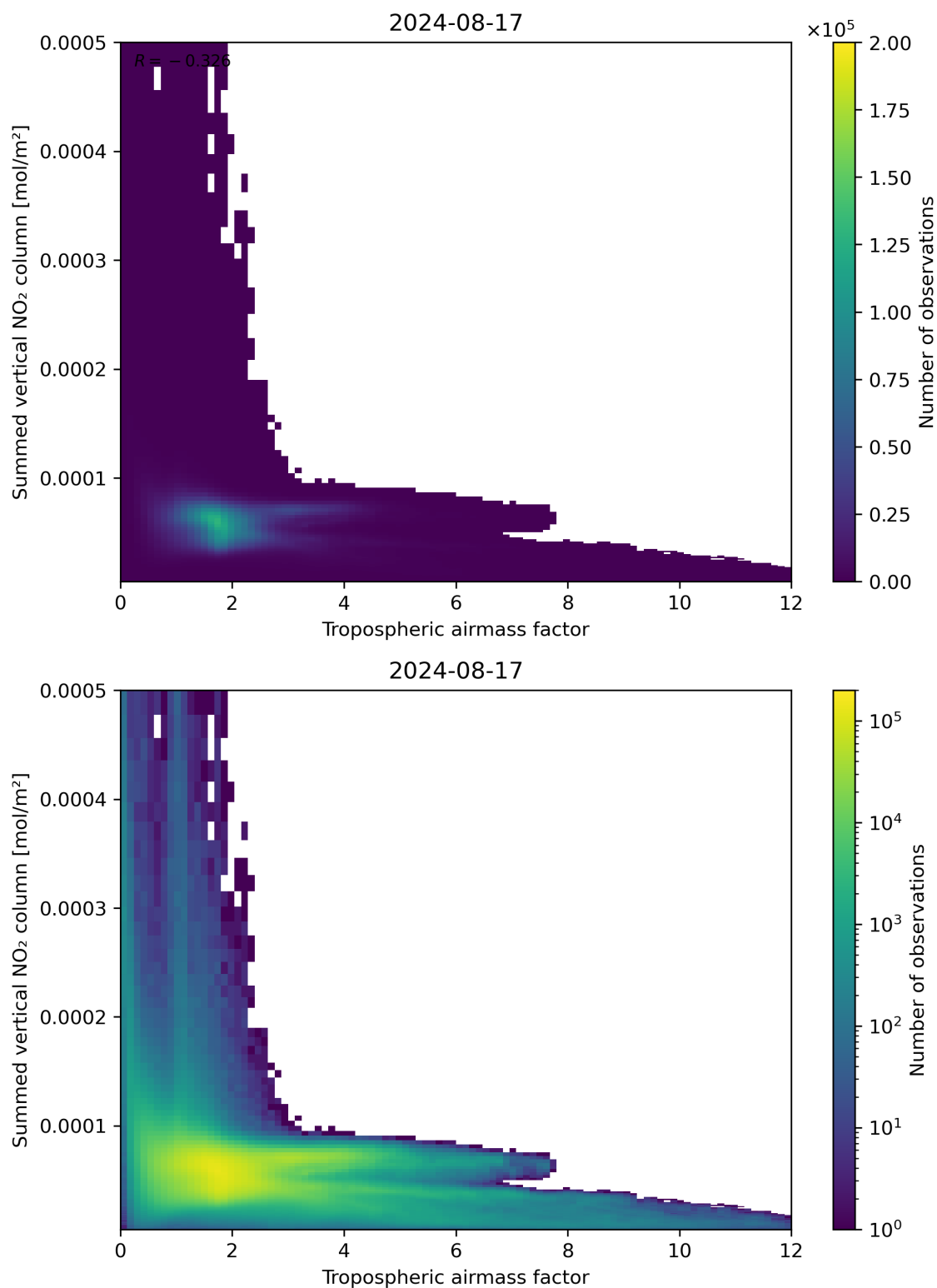
Figure 75: Scatter density plot of “Tropospheric airmass factor” against “Summed vertical NO 2 column” for 2024-08-16 to 2024-08-18.
