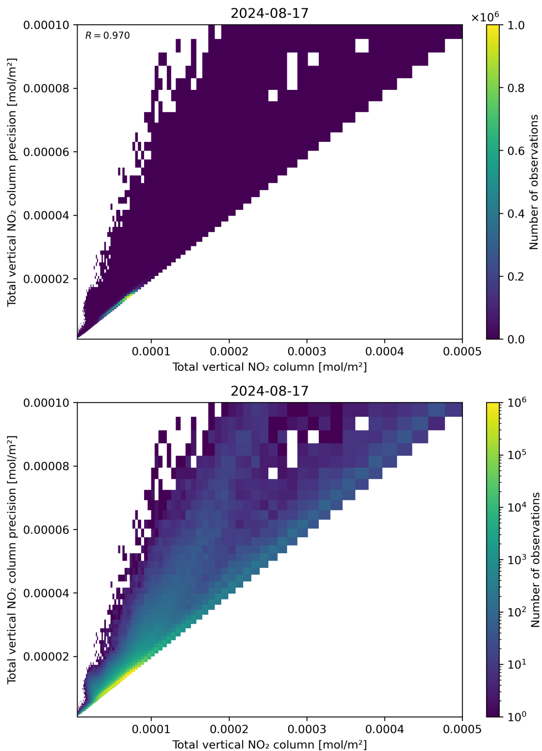
Figure 114: Scatter density plot of “Total vertical NO 2 column” against “Total vertical NO 2 column precision” for 2024-08-16 to 2024-08-18.
