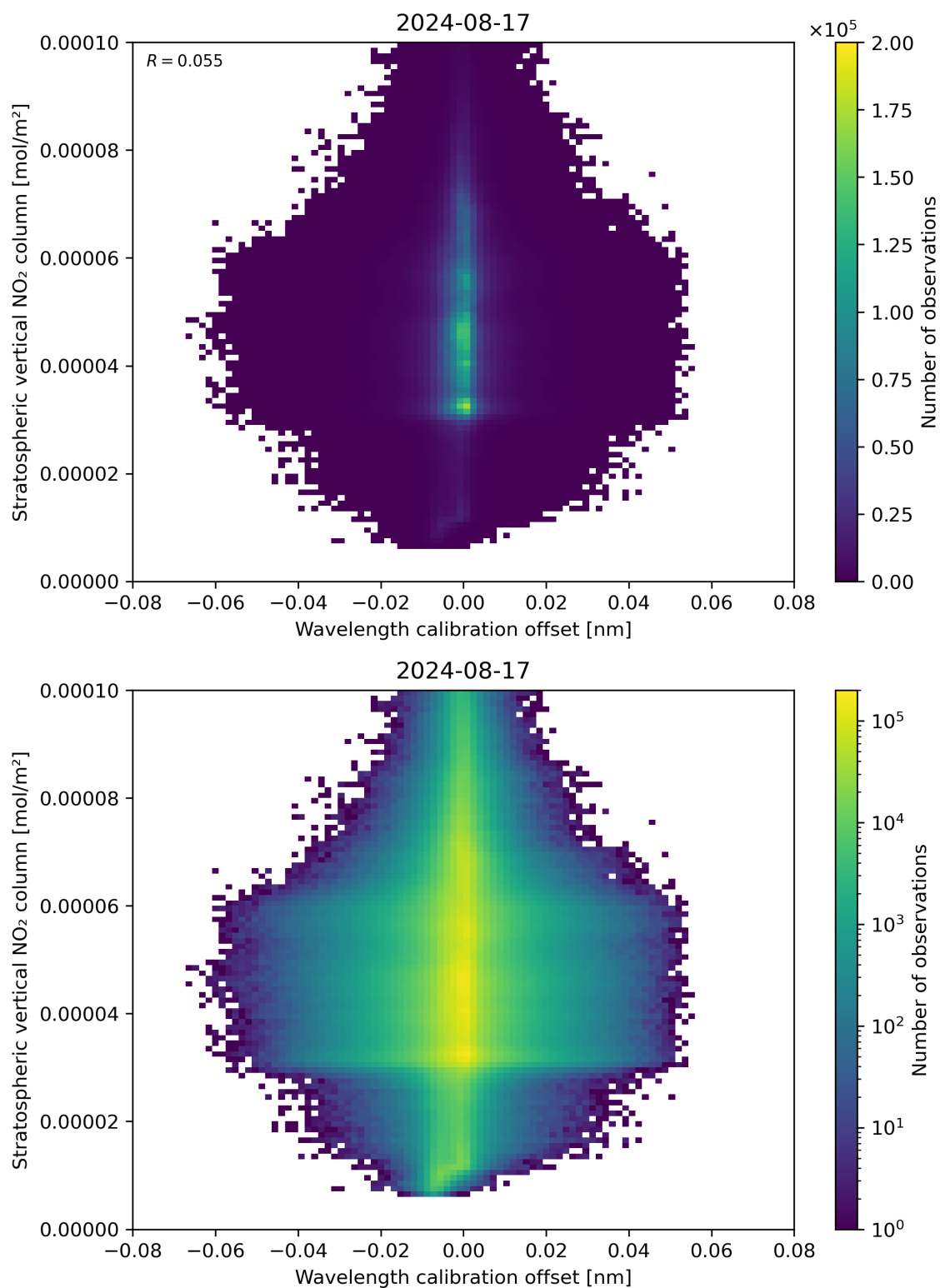
Figure 176: Scatter density plot of “Wavelength calibration offset” against “Stratospheric vertical NO 2 column” for 2024-08-16 to 2024-08-18.
