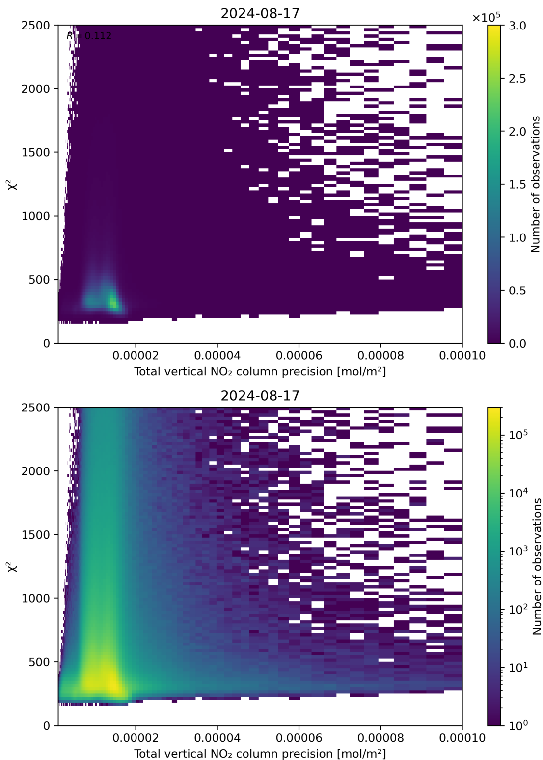
Figure 116: Scatter density plot of “Total vertical NO 2 column precision” against “ \chi^2 ” for 2024-08-16 to 2024-08-18.
