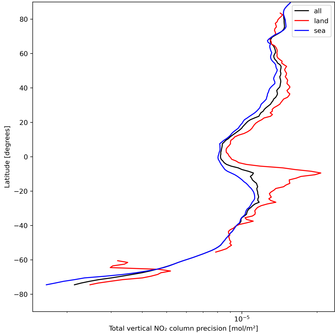
Figure 22: Zonal average of “Total vertical NO 2 column precision” for 2024-08-16 to 2024-08-18.
