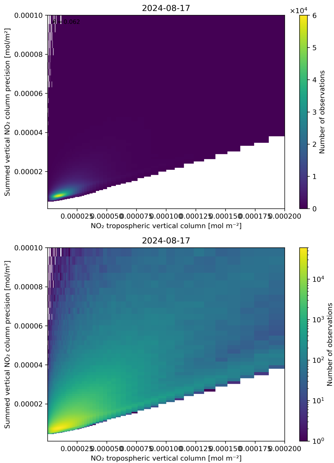
Figure 127: Scatter density plot of “NO 2 tropospheric vertical column” against “Summed vertical NO 2 column precision” for 2024-08-16 to 2024-08-18.
