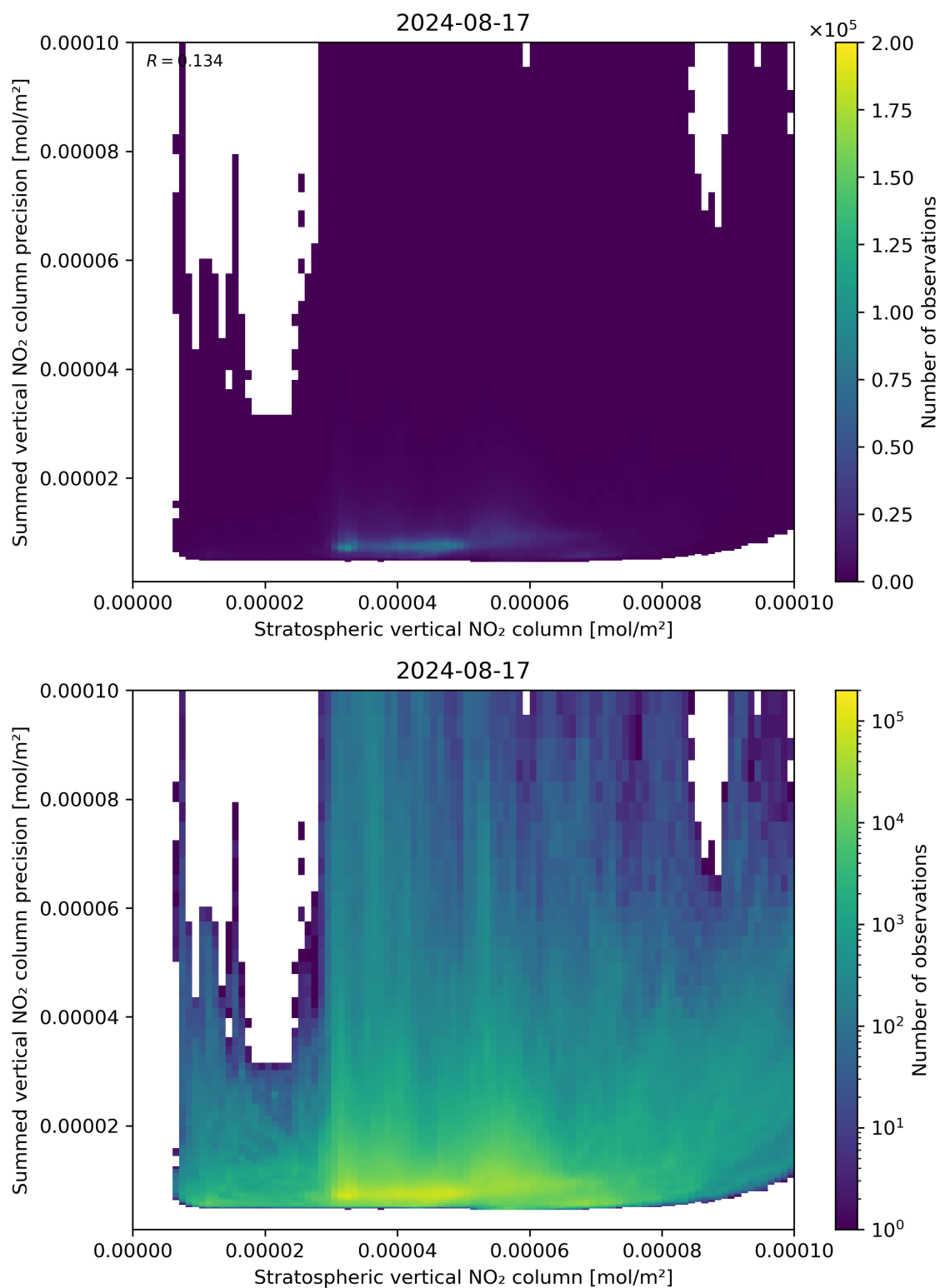
Figure 99: Scatter density plot of “Stratospheric vertical NO 2 column” against “Summed vertical NO 2 column precision” for 2024-08-16 to 2024-08-18.
