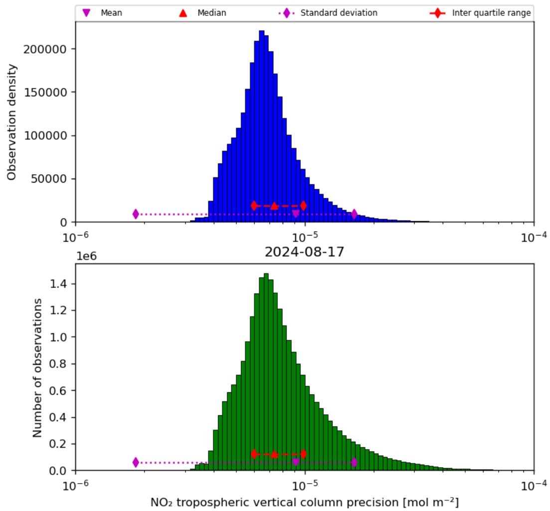
Figure 30: Histogram of “NO 2 tropospheric vertical column precision” for 2024-08-16 to 2024-08-18
