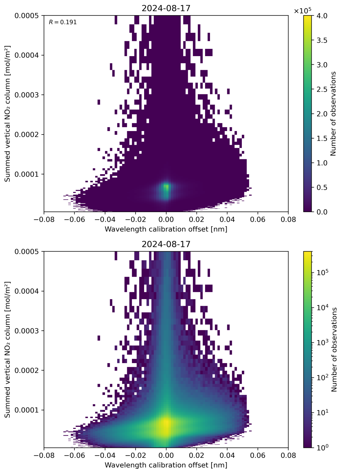
Figure 177: Scatter density plot of “Wavelength calibration offset” against “Summed vertical NO 2 column” for 2024-08-16 to 2024-08-18.
