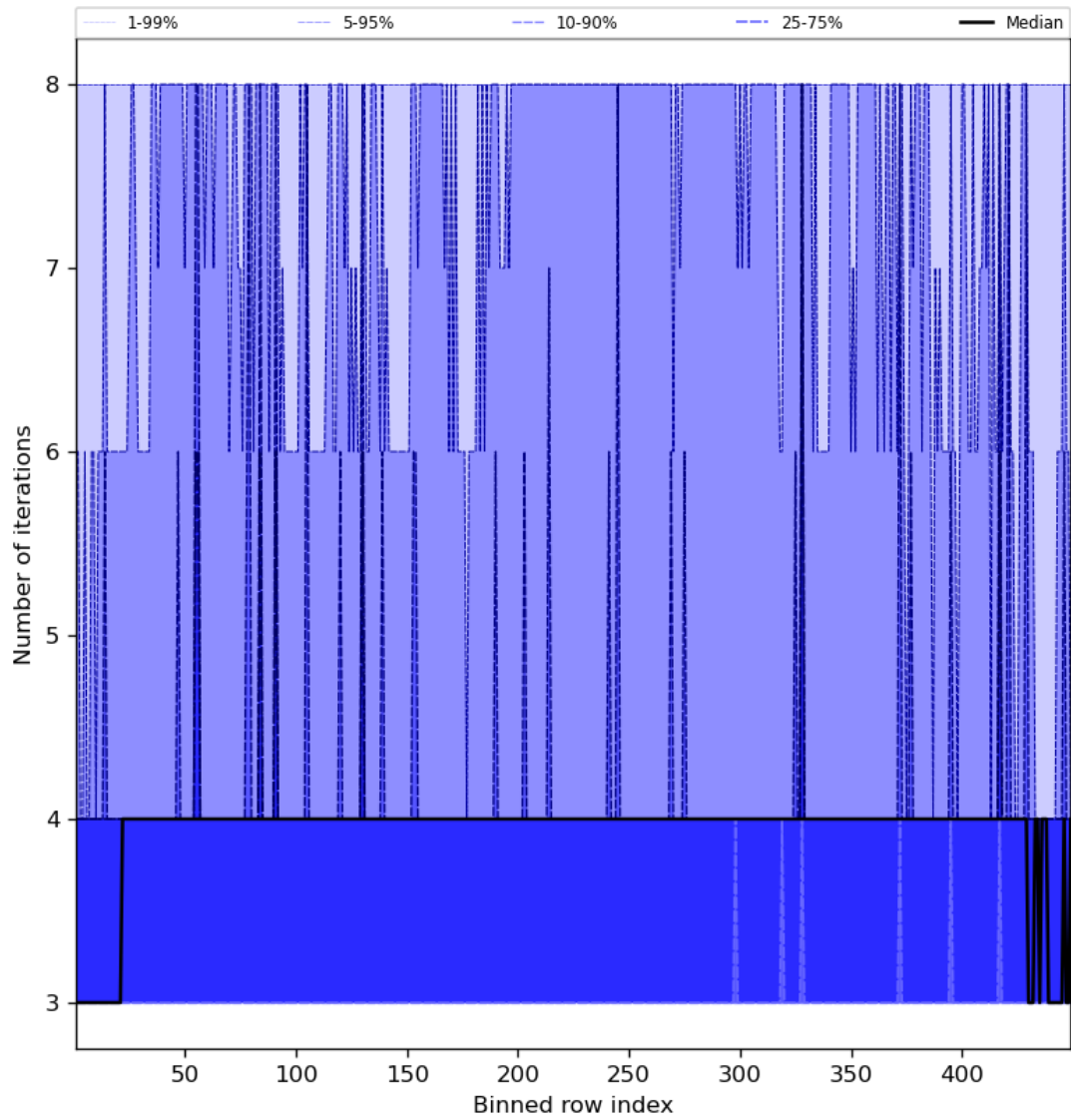
Figure 51: Along track statistics of “Number of iterations” for 2024-08-16 to 2024-08-18
