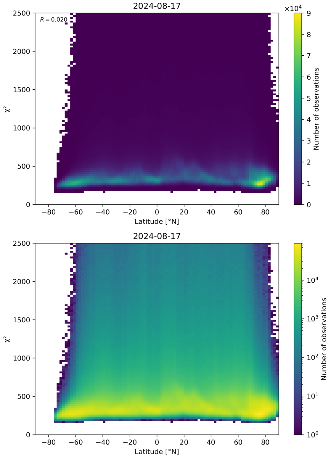
Figure 86: Scatter density plot of “Latitude” against “ \chi^2 ” for 2024-08-16 to 2024-08-18.
