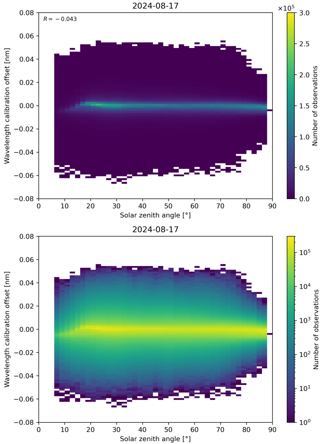
Figure 158: Scatter density plot of “Solar zenith angle” against “Wavelength calibration offset” for 2024-08-16 to 2024-08-18.
