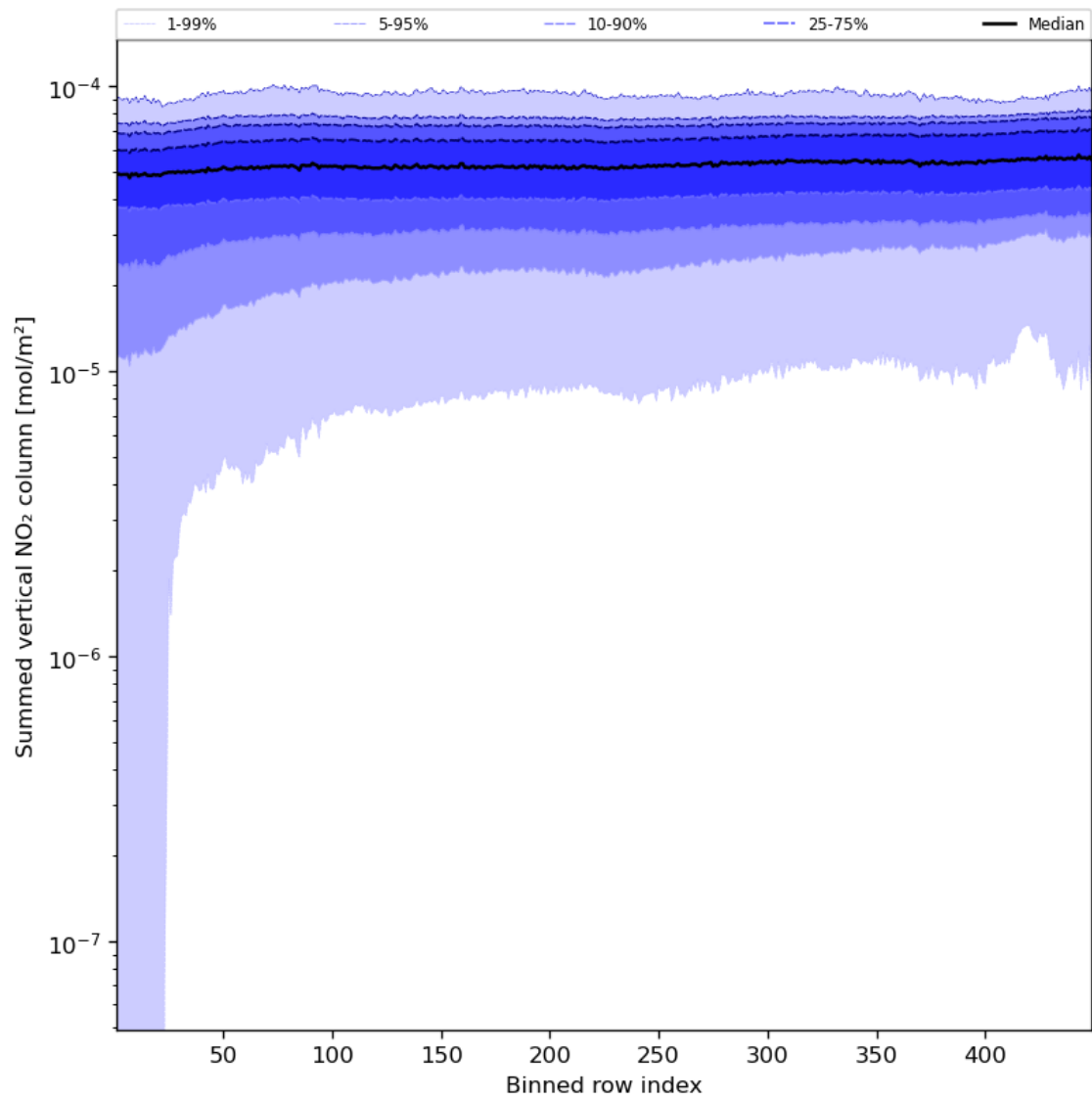
Figure 57: Along track statistics of “Summed vertical NO 2 column” for 2024-08-16 to 2024-08-18
