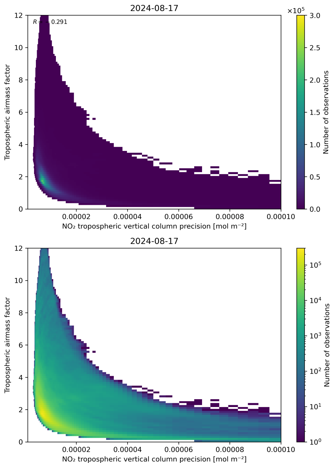
Figure 133: Scatter density plot of “NO 2 tropospheric vertical column precision” against “Tropospheric airmass factor” for 2024-08-16 to 2024-08-18.
