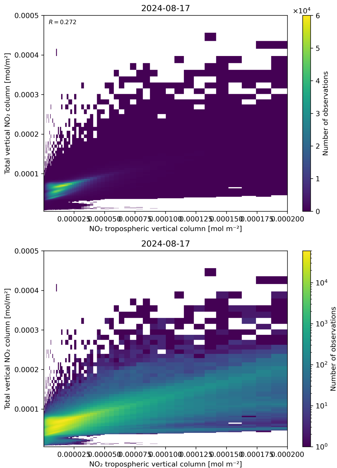
Figure 128: Scatter density plot of “NO 2 tropospheric vertical column” against “Total vertical NO 2 column” for 2024-08-16 to 2024-08-18.
