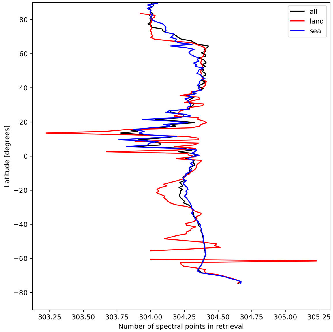
Figure 16: Zonal average of “Number of spectral points in retrieval” for 2024-08-16 to 2024-08-18.
