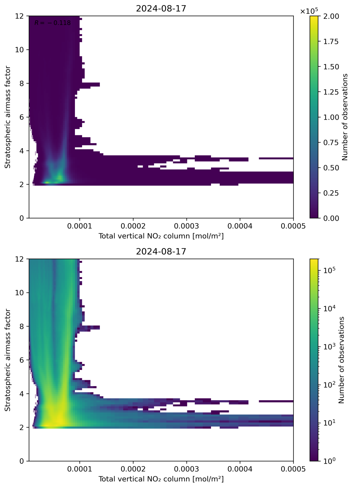
Figure 110: Scatter density plot of “Total vertical NO 2 column” against “Stratospheric airmass factor” for 2024-08-16 to 2024-08-18.
