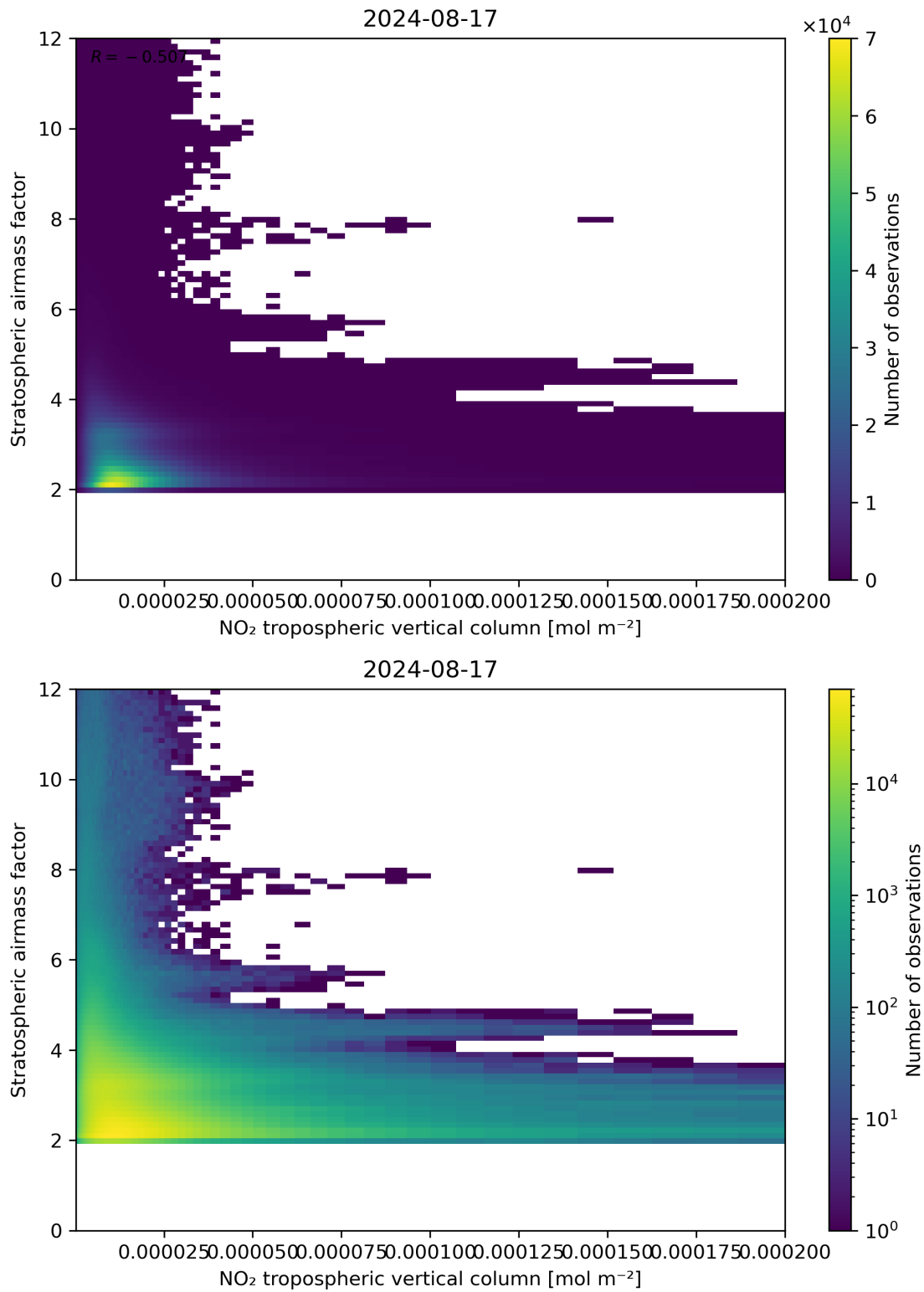
Figure 121: Scatter density plot of “NO 2 tropospheric vertical column” against “Stratospheric air mass factor” for 2024-08-16 to 2024-08-18.
