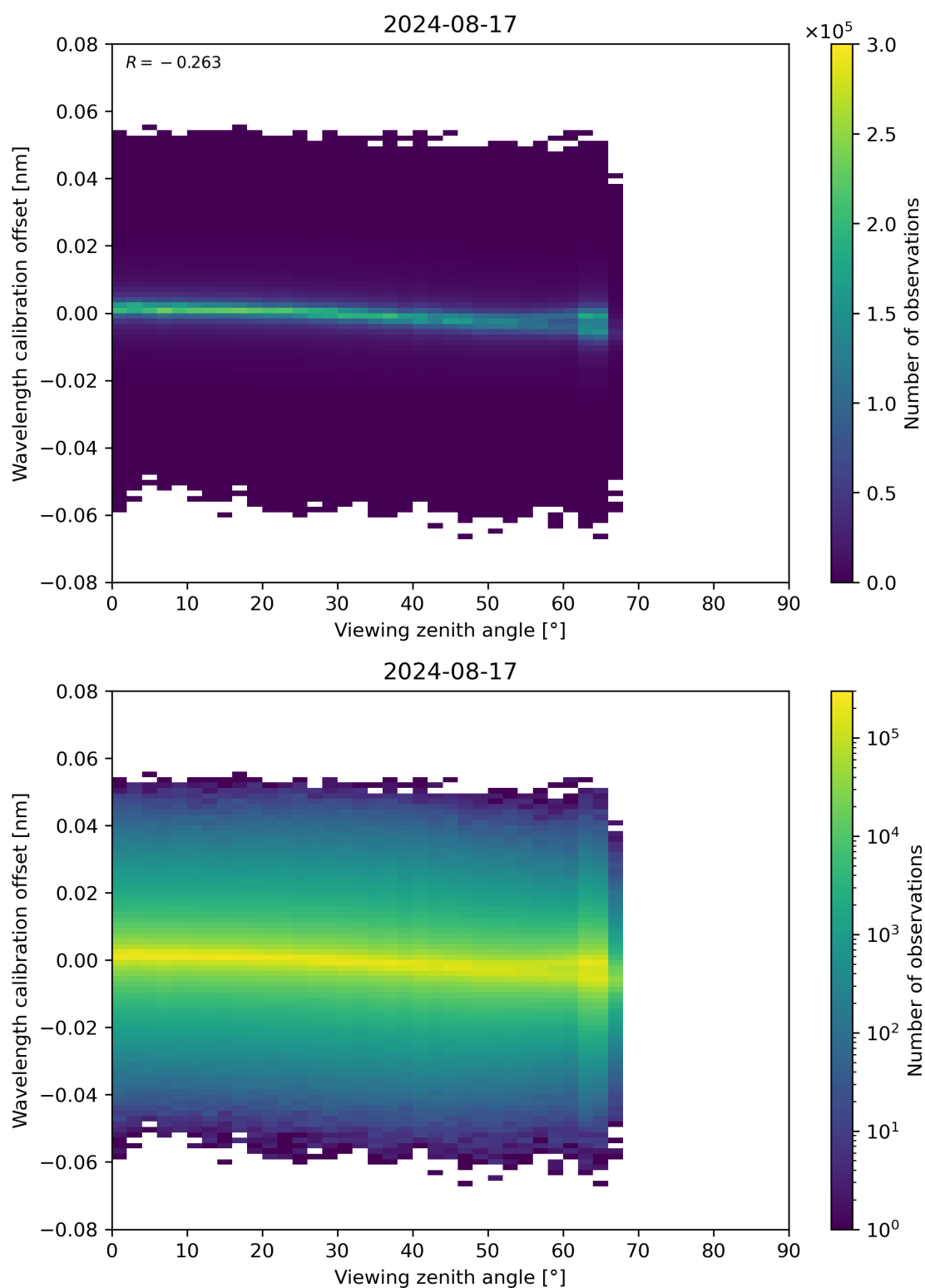
Figure 173: Scatter density plot of “Viewing zenith angle” against “Wavelength calibration offset” for 2024-08-16 to 2024-08-18.
