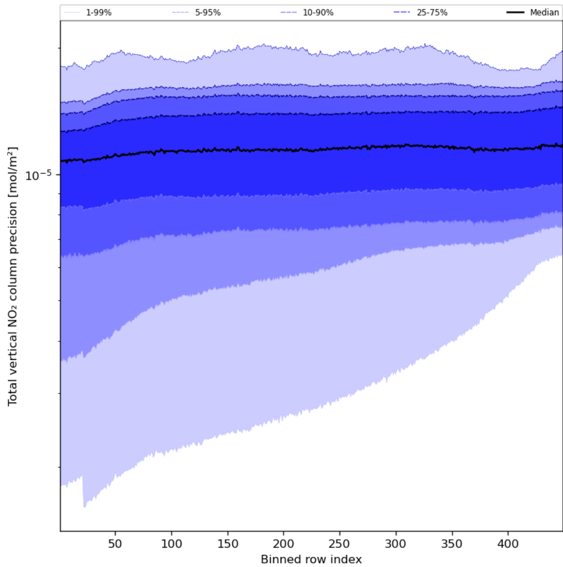
Figure 56: Along track statistics of “Total vertical NO 2 column precision” for 2024-08-16 to 2024-08-18
