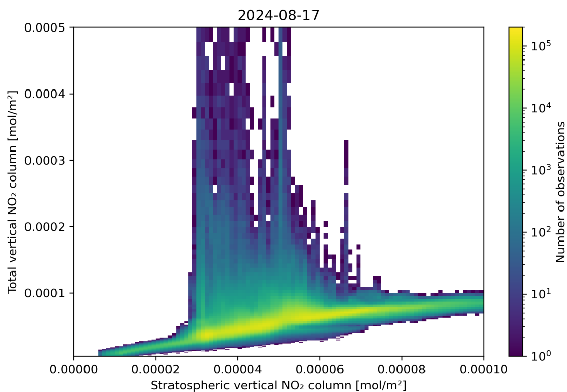
Figure 100: Scatter density plot of “Stratospheric vertical NO 2 column” against “Total vertical NO 2 column” for 2024-08-16 to 2024-08-18.
