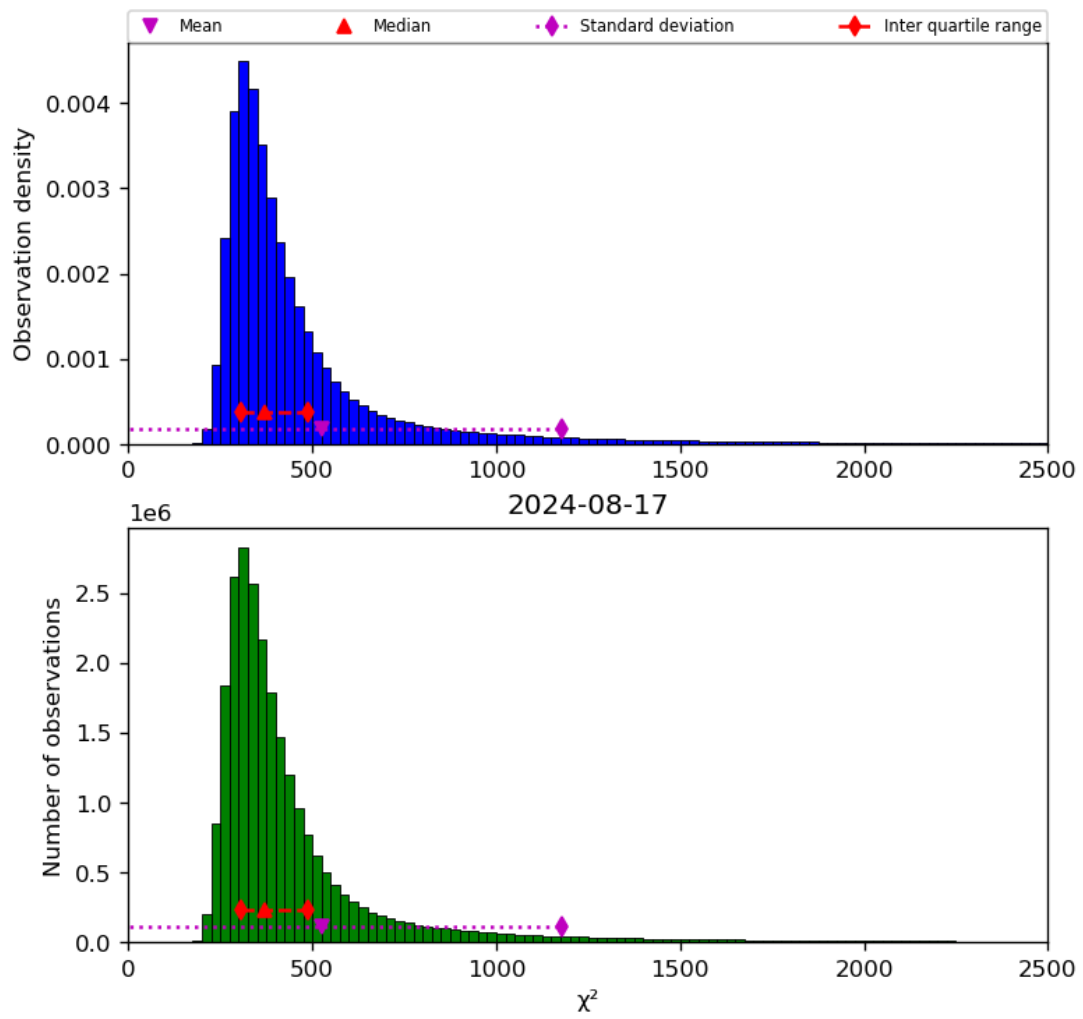
Figure 42: Histogram of “ \chi^2 ” for 2024-08-16 to 2024-08-18
