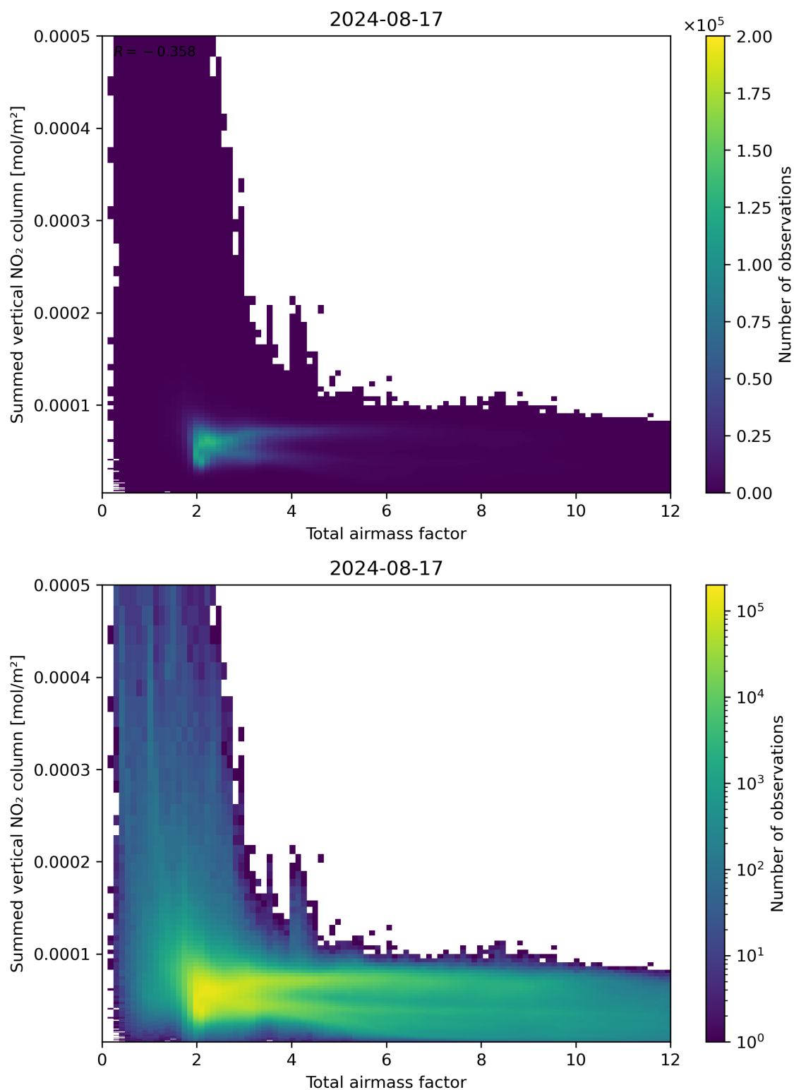
Figure 65: Scatter density plot of “Total airmass factor” against “Summed vertical NO 2 column” for 2024-08-16 to 2024-08-18.
