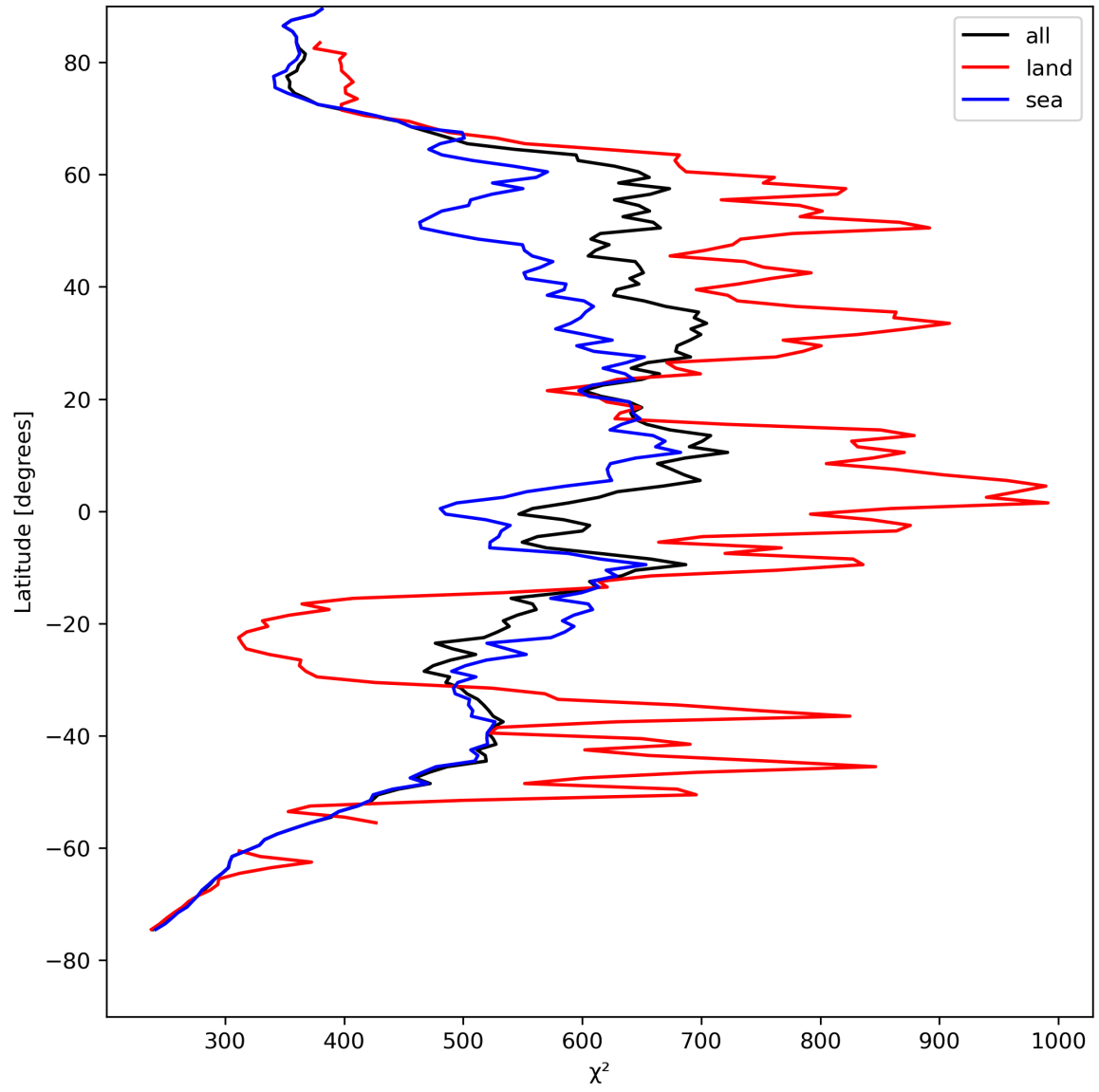
Figure 25: Zonal average of “ \chi^2 ” for 2024-08-16 to 2024-08-18.
