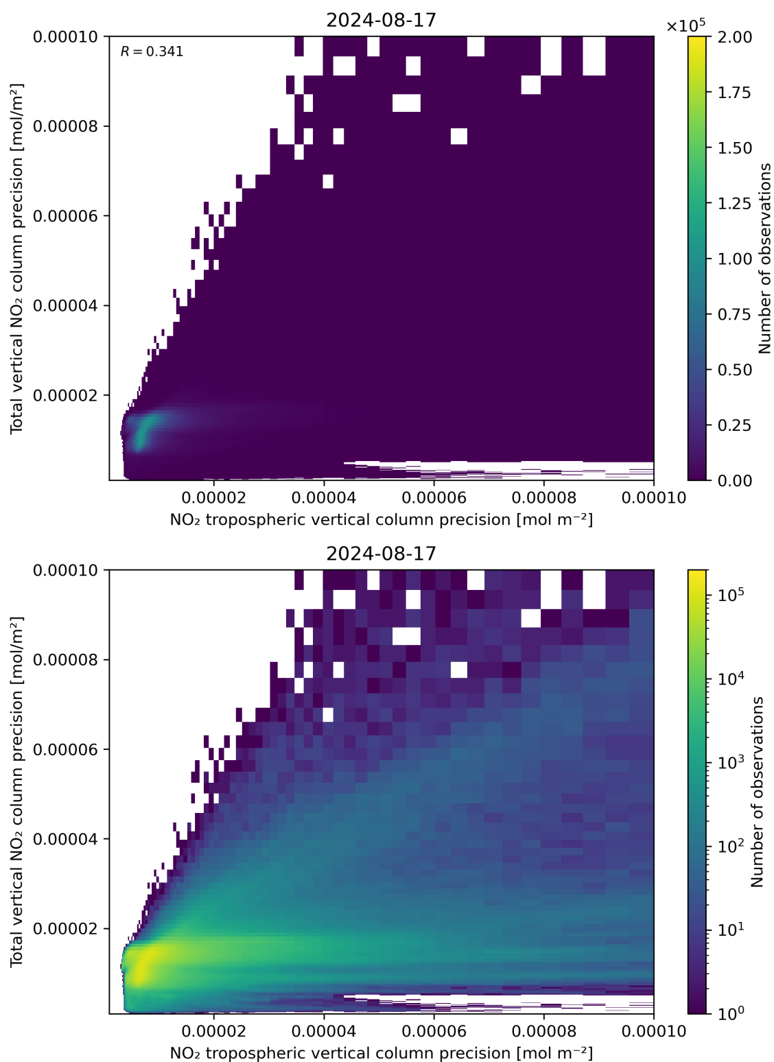
Figure 139: Scatter density plot of “NO 2 tropospheric vertical column precision” against “Total vertical NO 2 column precision” for 2024-08-16 to 2024-08-18.
