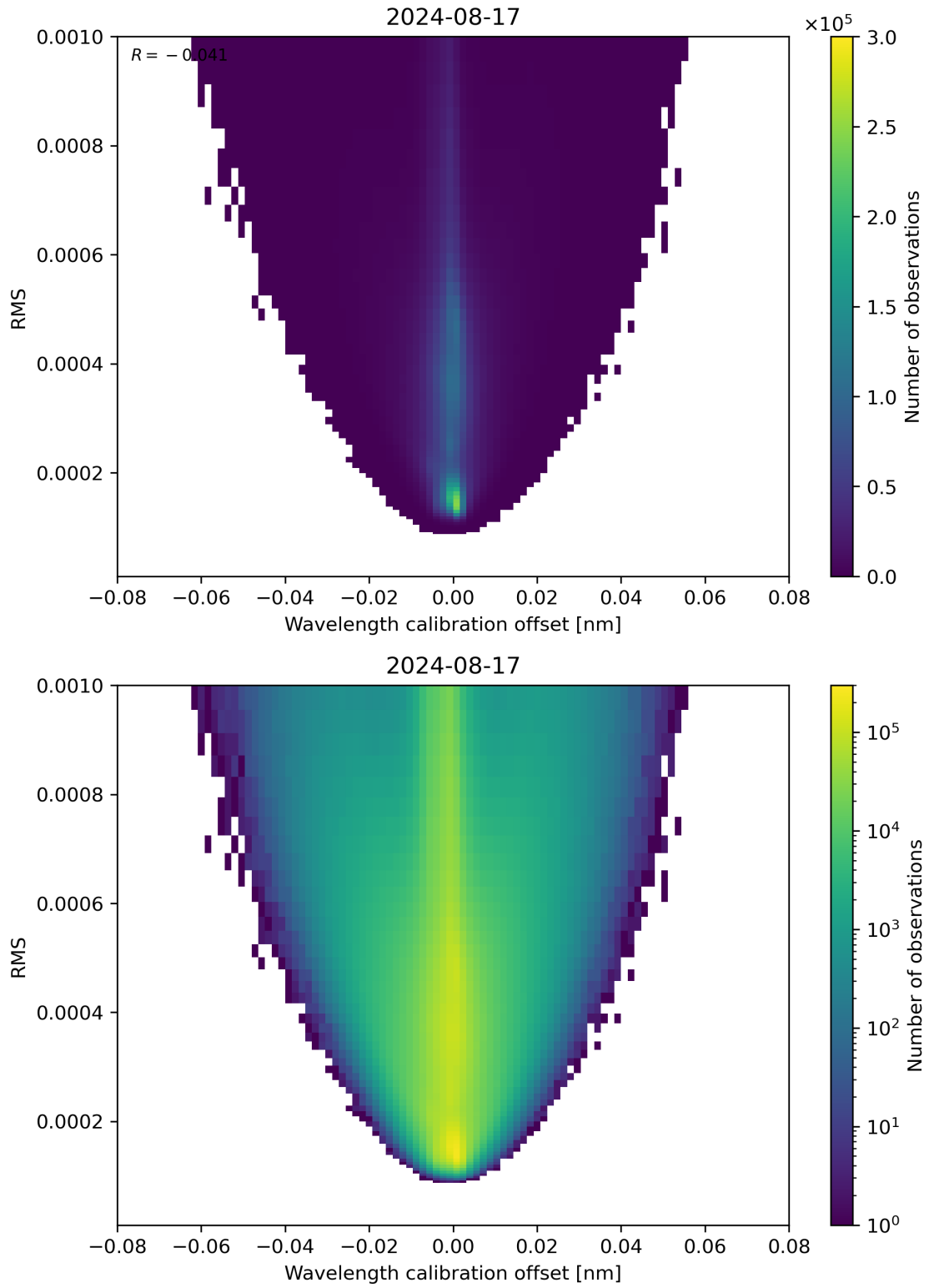
Figure 181: Scatter density plot of “Wavelength calibration offset” against “RMS” for 2024-08-16 to 2024-08-18.
