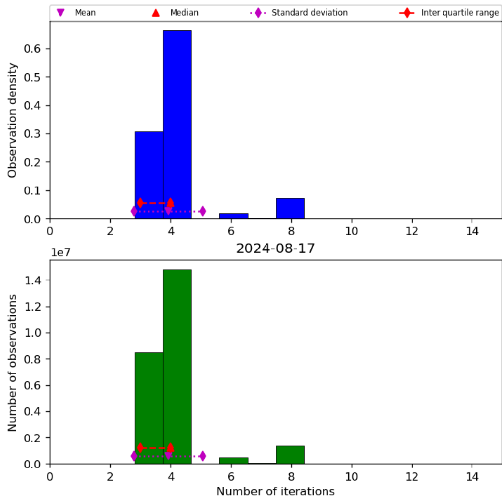
Figure 34: Histogram of “Number of iterations” for 2024-08-16 to 2024-08-18
