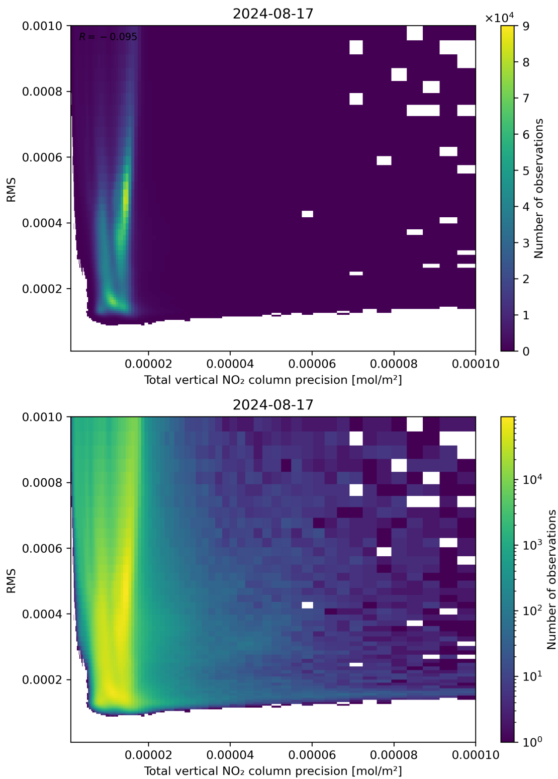
Figure 119: Scatter density plot of “Total vertical NO 2 column precision” against “RMS” for 2024-08-16 to 2024-08-18.
