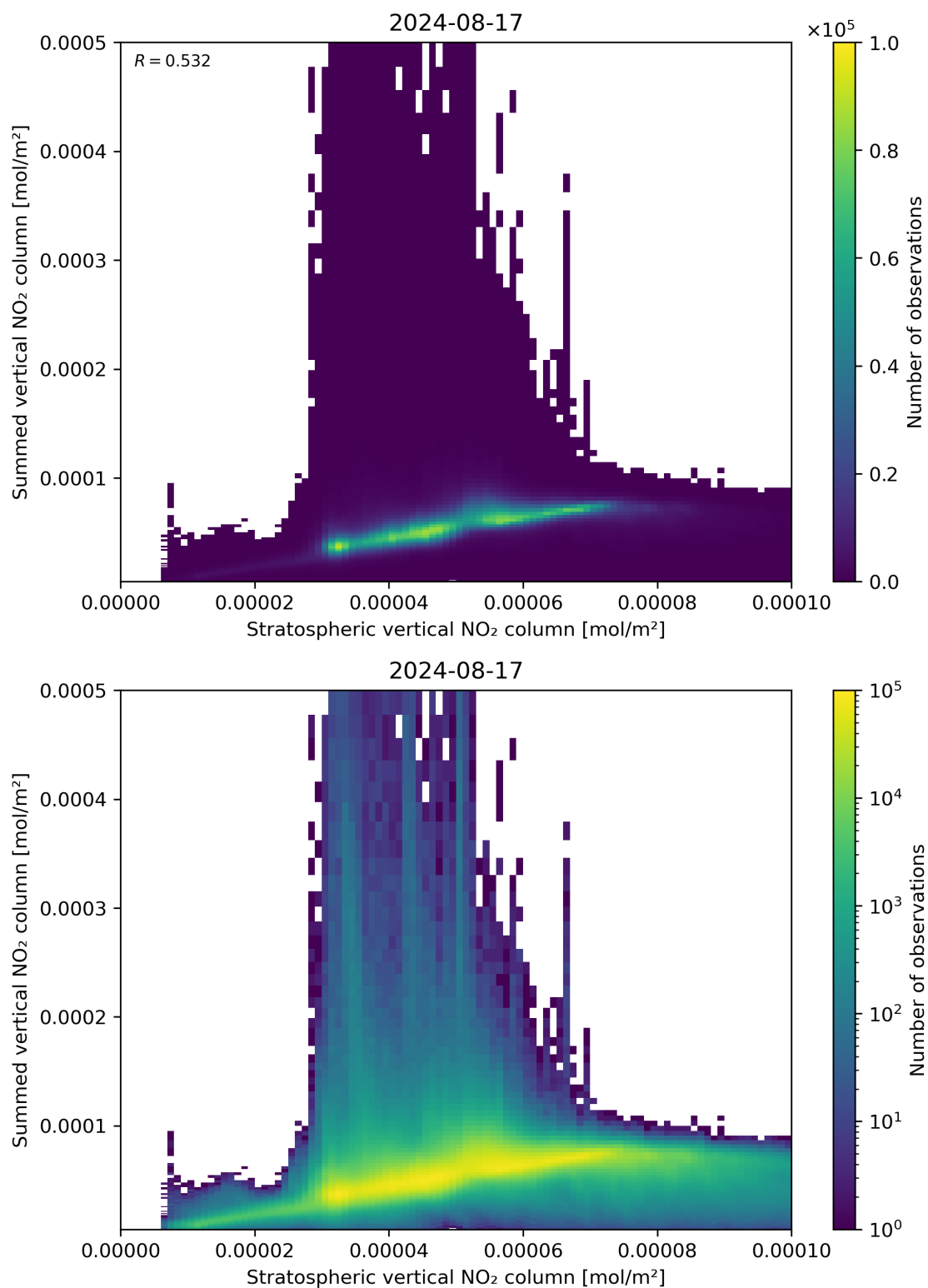
Figure 98: Scatter density plot of “Stratospheric vertical NO 2 column” against “Summed vertical NO 2 column” for 2024-08-16 to 2024-08-18.
