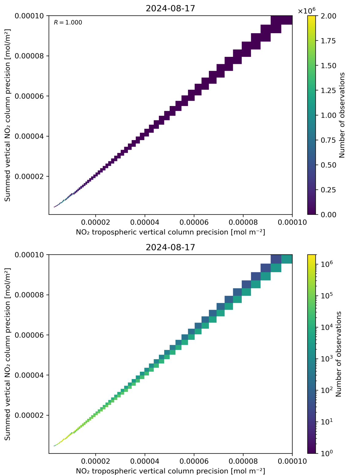
Figure 137: Scatter density plot of “NO 2 tropospheric vertical column precision” against “Summed vertical NO 2 column precision” for 2024-08-16 to 2024-08-18.
