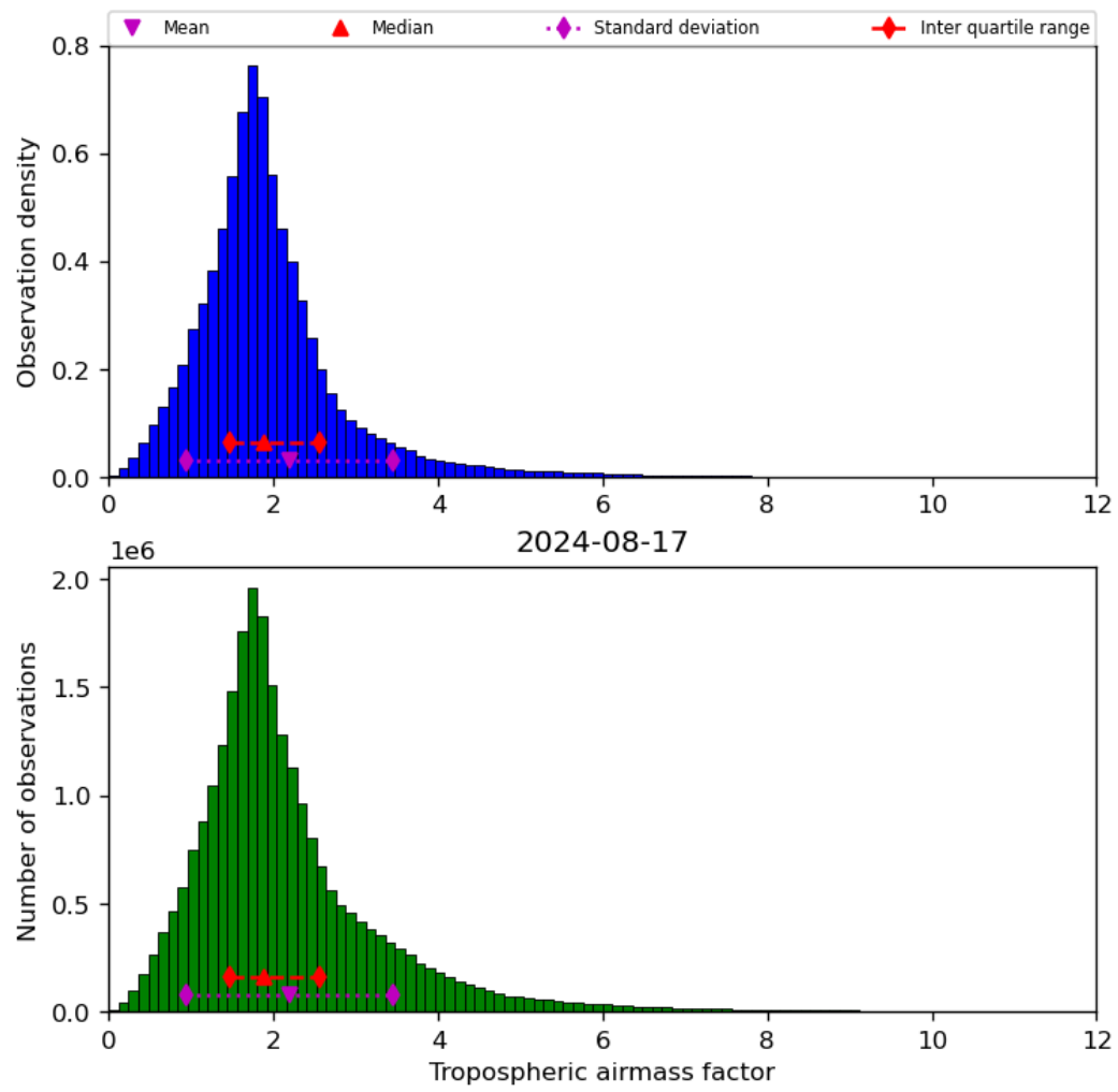
Figure 31: Histogram of “Tropospheric airmass factor” for 2024-08-16 to 2024-08-18
