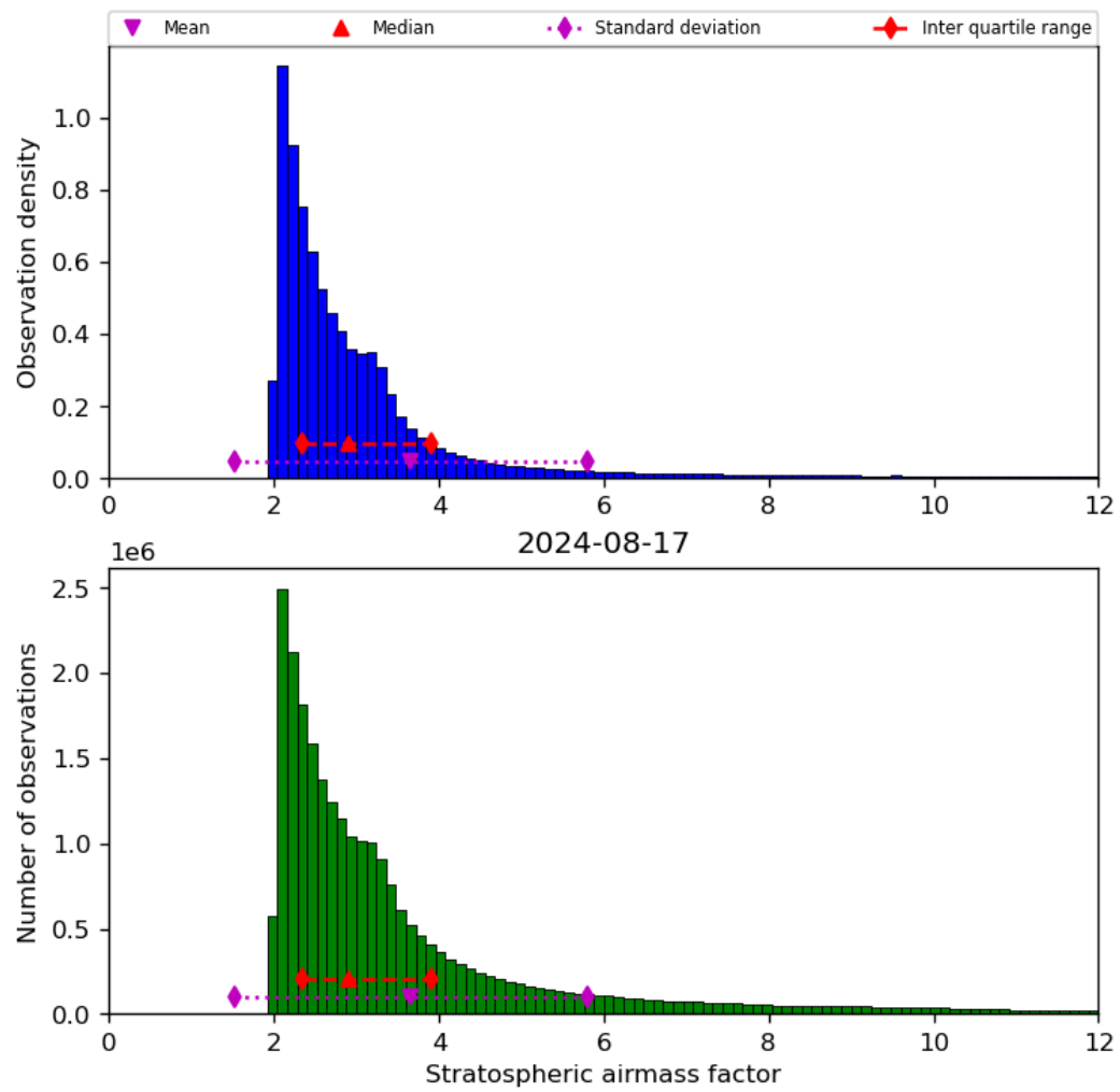
Figure 44: Histogram of “Stratospheric airmass factor” for 2024-08-16 to 2024-08-18
