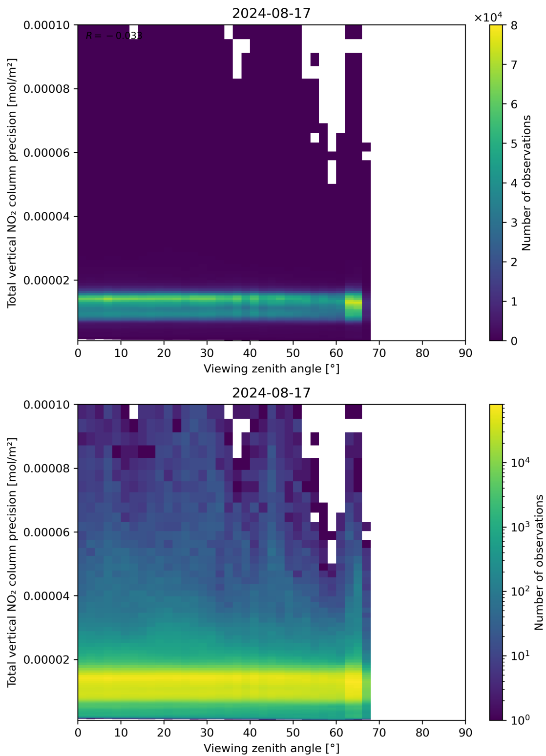
Figure 168: Scatter density plot of “Viewing zenith angle” against “Total vertical NO 2 column precision” for 2024-08-16 to 2024-08-18.
