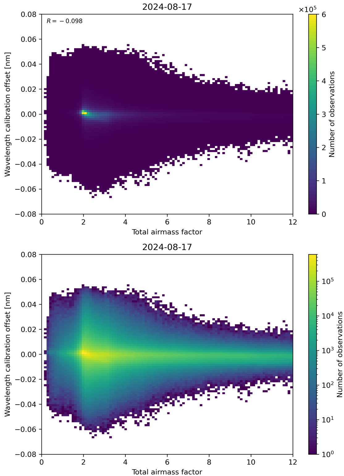
Figure 70: Scatter density plot of “Total airmass factor” against “Wavelength calibration offset” for 2024-08-16 to 2024-08-18.
