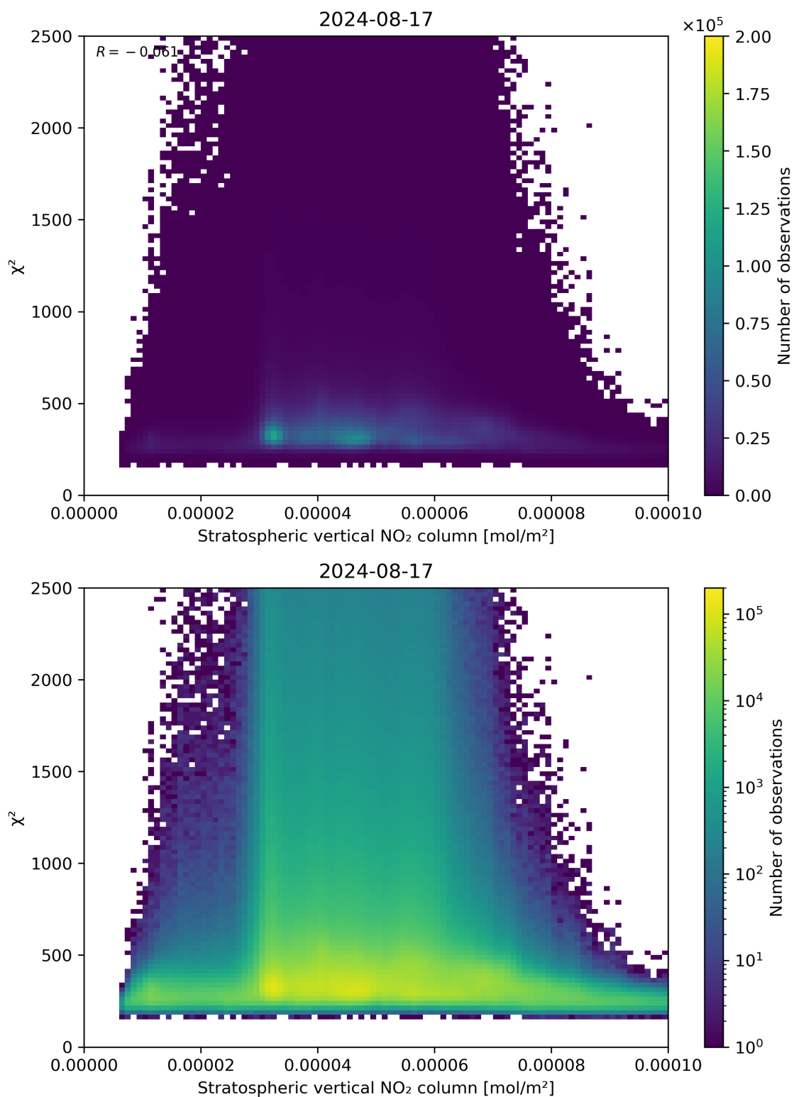
Figure 97: Scatter density plot of “Stratospheric vertical NO 2 column” against “ \chi^2 ” for 2024-08-16 to 2024-08-18.
