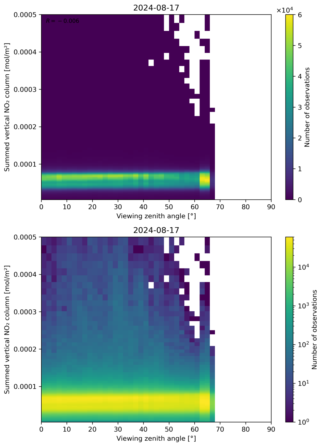
Figure 165: Scatter density plot of “Viewing zenith angle” against “Summed vertical NO 2 column” for 2024-08-16 to 2024-08-18.
