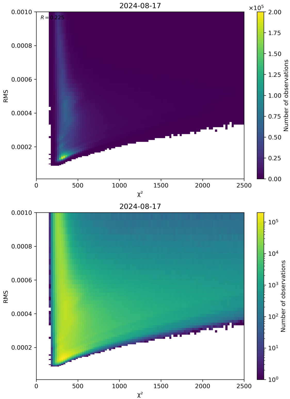
Figure 82: Scatter density plot of “ \chi^2 ” against “RMS” for 2024-08-16 to 2024-08-18.
