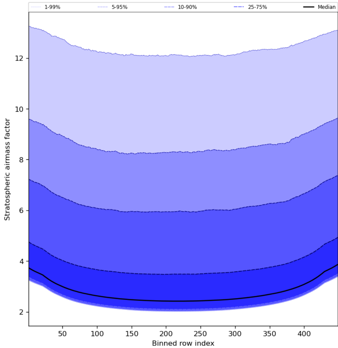
Figure 61: Along track statistics of “Stratospheric airmass factor” for 2024-08-16 to 2024-08-18
