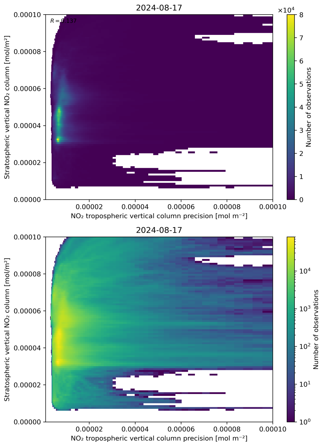
Figure 135: Scatter density plot of “NO 2 tropospheric vertical column precision” against “Stratospheric vertical NO 2 column” for 2024-08-16 to 2024-08-18.
