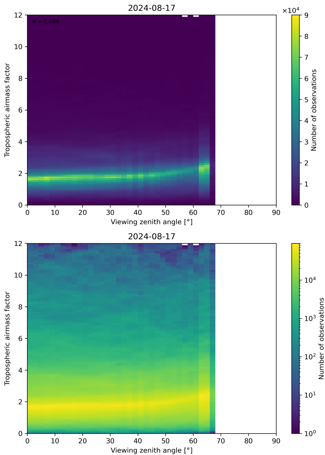
Figure 161: Scatter density plot of “Viewing zenith angle” against “Tropospheric airmass factor” for 2024-08-16 to 2024-08-18.
