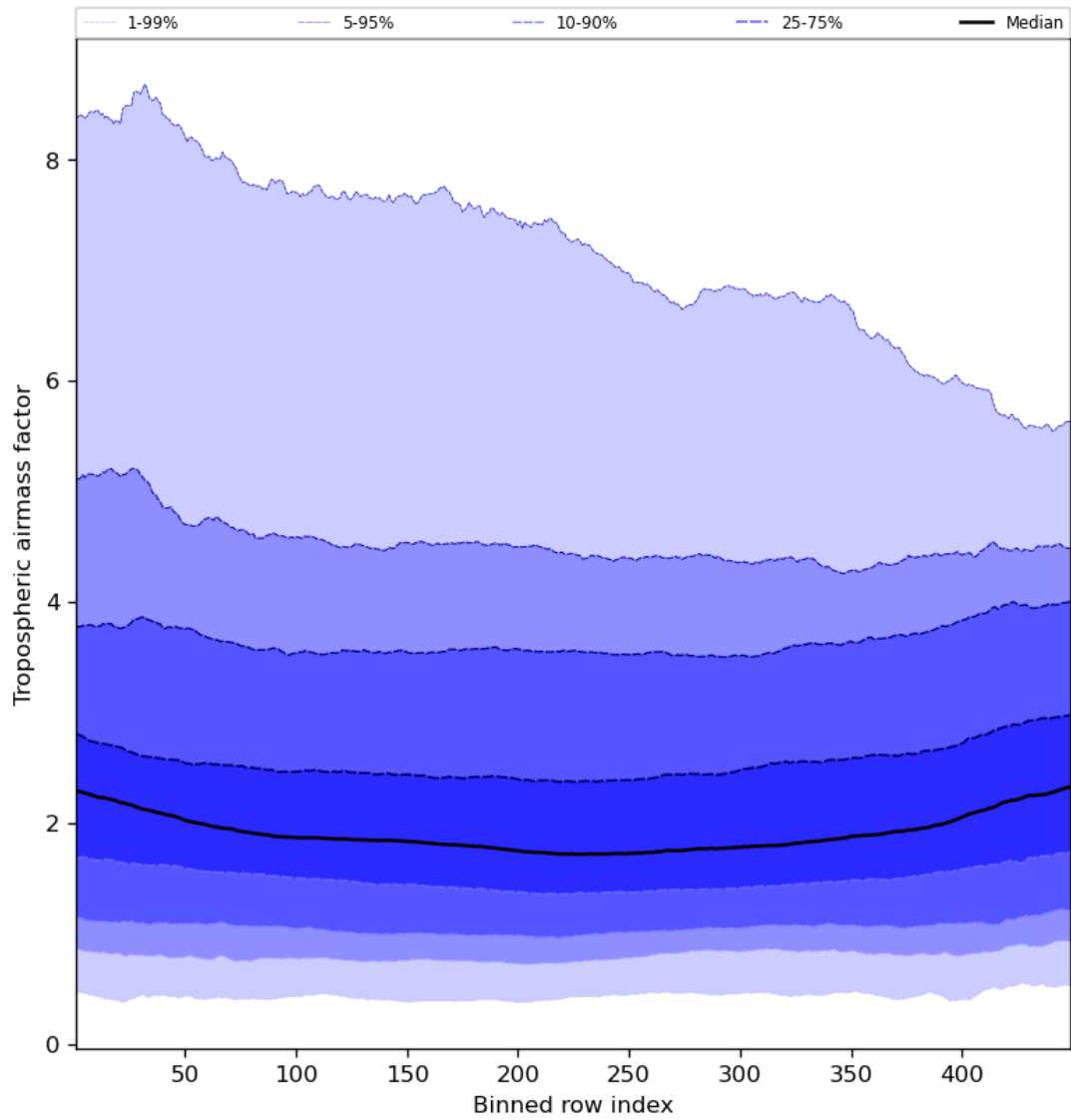
Figure 48: Along track statistics of “Tropospheric airmass factor” for 2024-08-16 to 2024-08-18
