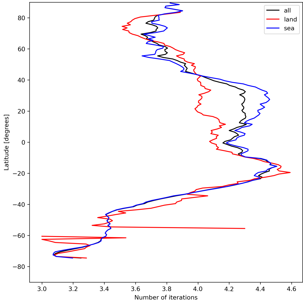
Figure 17: Zonal average of “Number of iterations” for 2024-08-16 to 2024-08-18.
