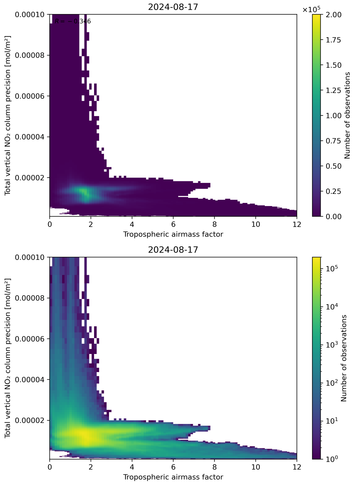
Figure 78: Scatter density plot of “Tropospheric air mass factor” against “Total vertical NO 2 column precision” for 2024-08-16 to 2024-08-18.
