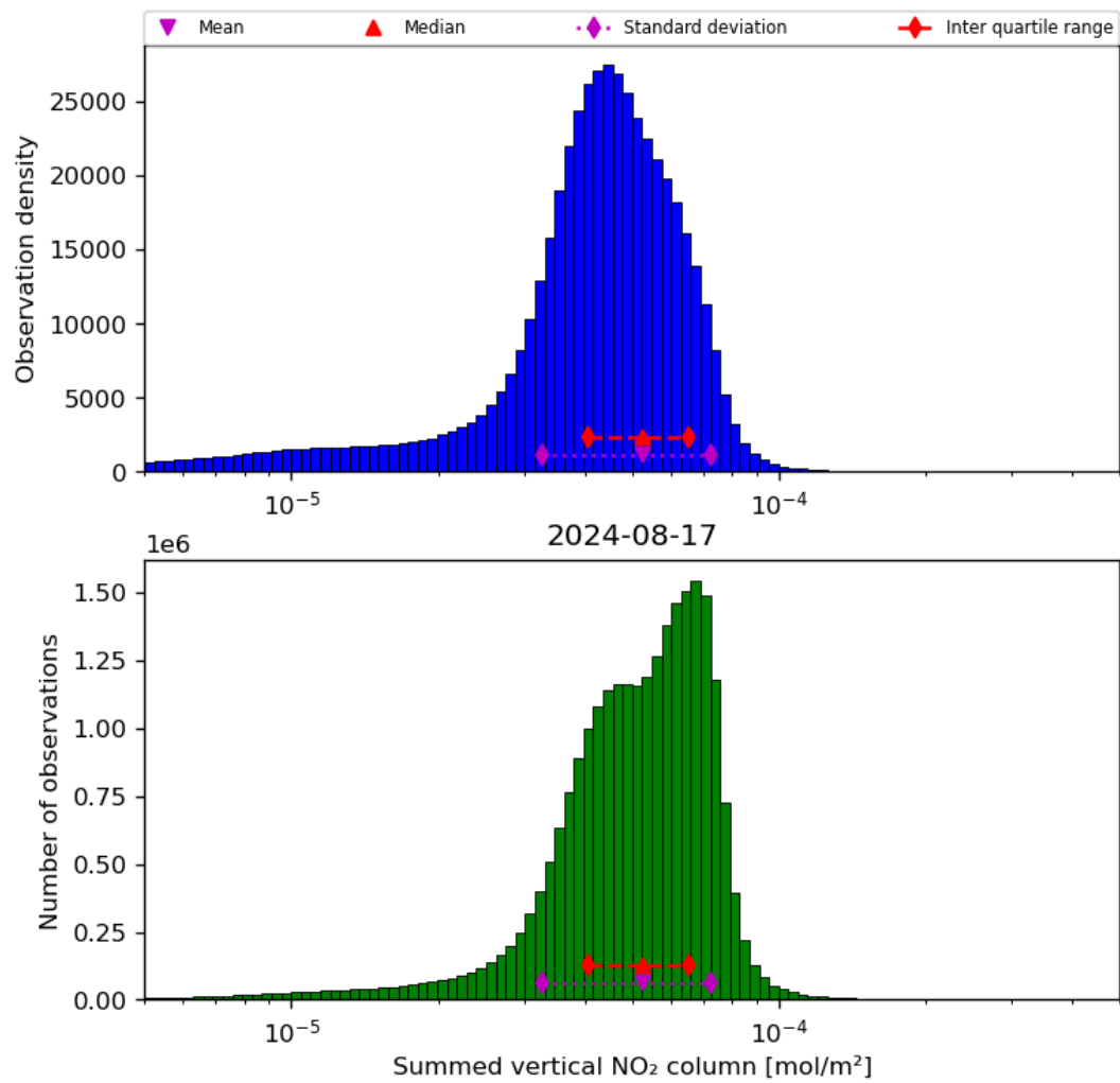
Figure 40: Histogram of “Summed vertical NO 2 column” for 2024-08-16 to 2024-08-18
