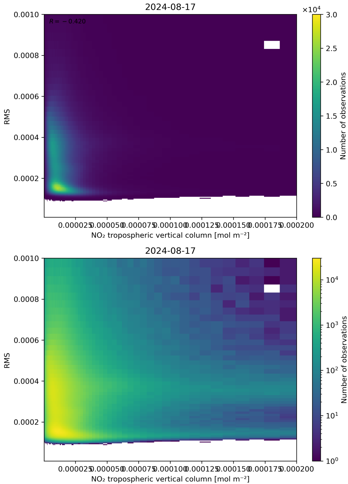
Figure 142: Scatter density plot of “NO 2 tropospheric vertical column” against “RMS” for 2024-08-16 to 2024-08-18.
