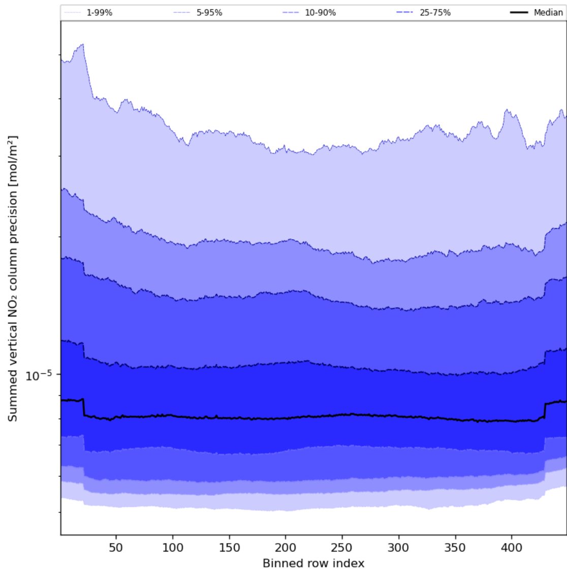
Figure 58: Along track statistics of “Summed vertical NO 2 column precision” for 2024-08-16 to 2024-08-18
