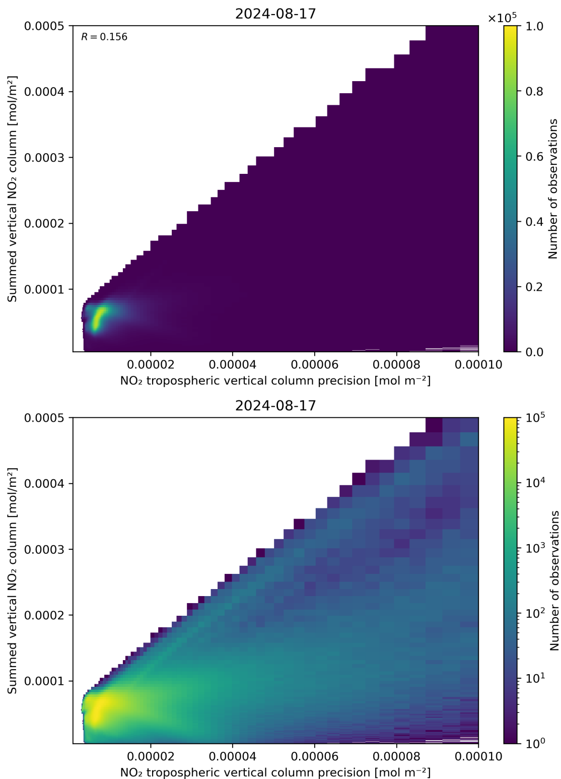
Figure 136: Scatter density plot of “NO 2 tropospheric vertical column precision” against “Summed vertical NO 2 column” for 2024-08-16 to 2024-08-18.
