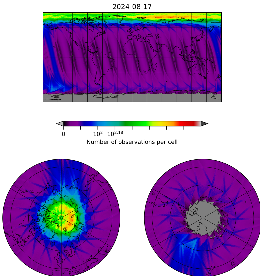
Figure 10: Map of the number of observations for 2024-08-16 to 2024-08-18
