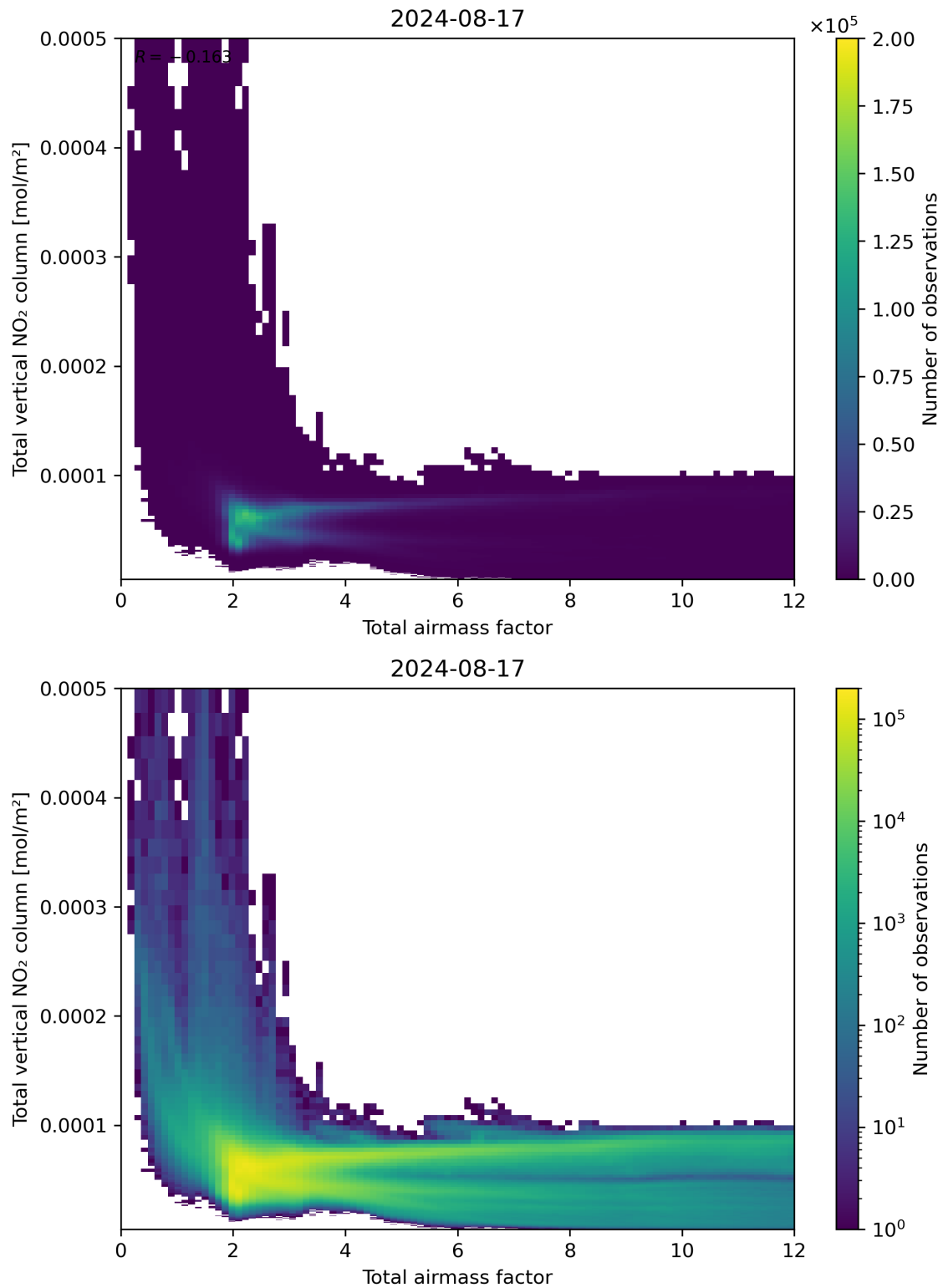
Figure 67: Scatter density plot of “Total airmass factor” against “Total vertical NO 2 column” for 2024-08-16 to 2024-08-18.
