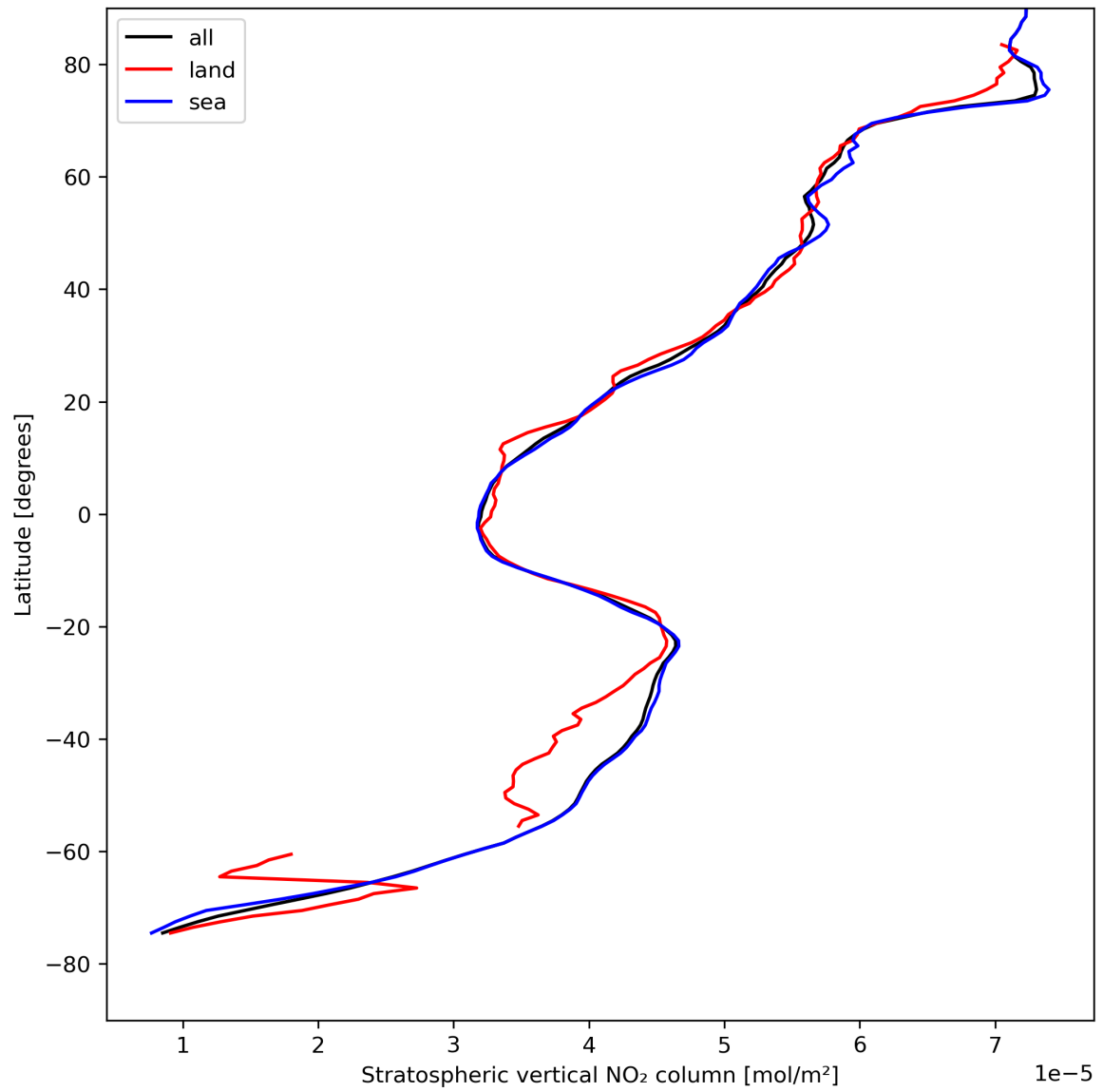
Figure 19: Zonal average of “Stratospheric vertical NO 2 column” for 2024-08-16 to 2024-08-18.
