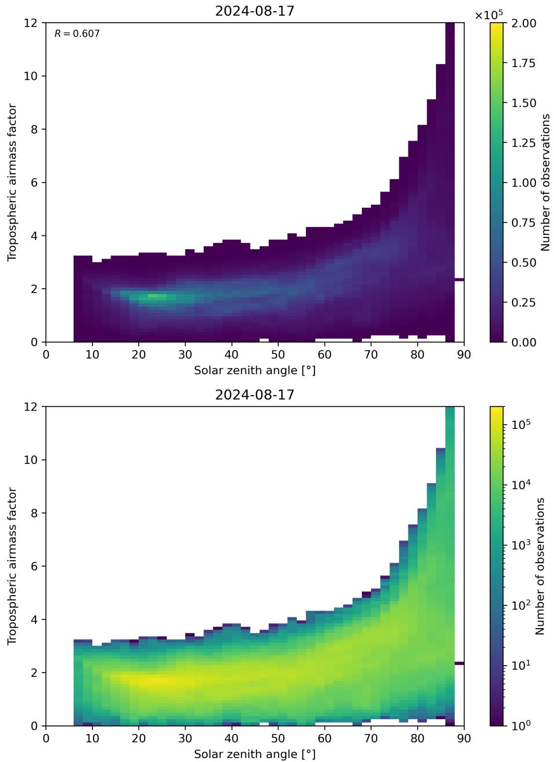
Figure 147: Scatter density plot of “Solar zenith angle” against “Tropospheric airmass factor” for 2024-08-16 to 2024-08-18.
