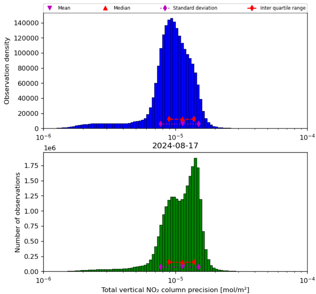
Figure 39: Histogram of “Total vertical NO 2 column precision” for 2024-08-16 to 2024-08-18
