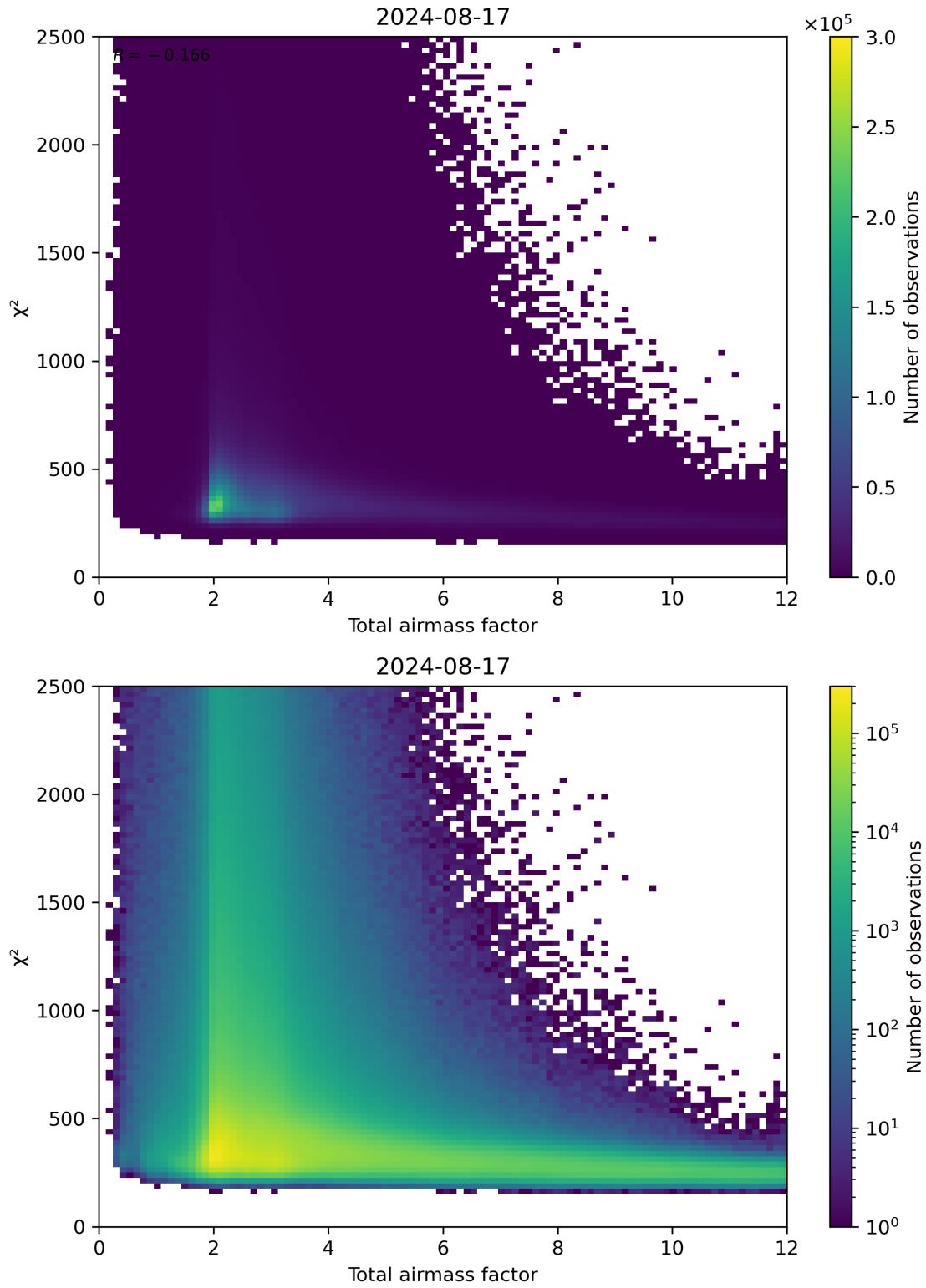
Figure 63: Scatter density plot of “Total airmass factor” against “ \chi^2 ” for 2024-08-16 to 2024-08-18.
