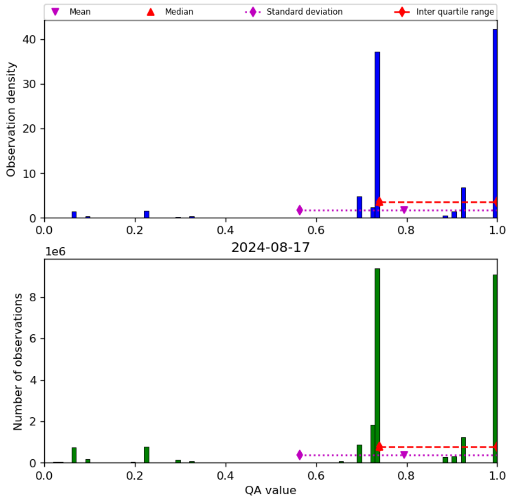
Figure 28: Histogram of “QA value” for 2024-08-16 to 2024-08-18
