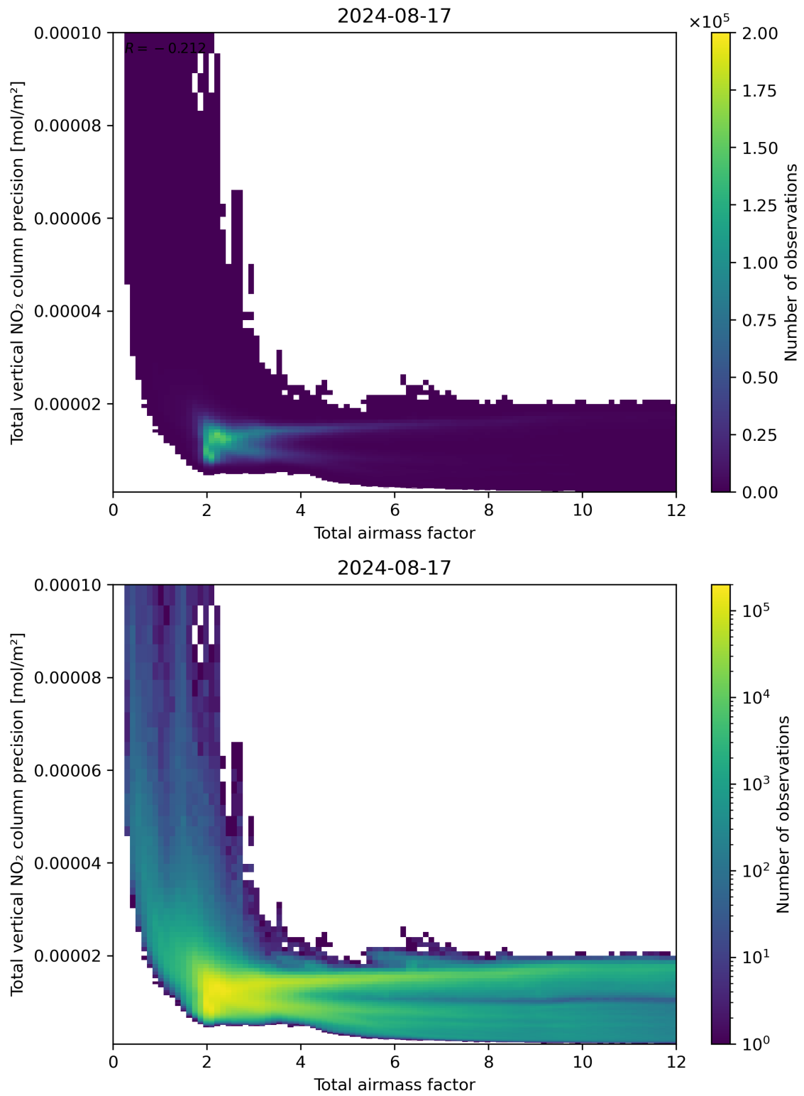
Figure 68: Scatter density plot of “Total airmass factor” against “Total vertical NO 2 column precision” for 2024-08-16 to 2024-08-18.
