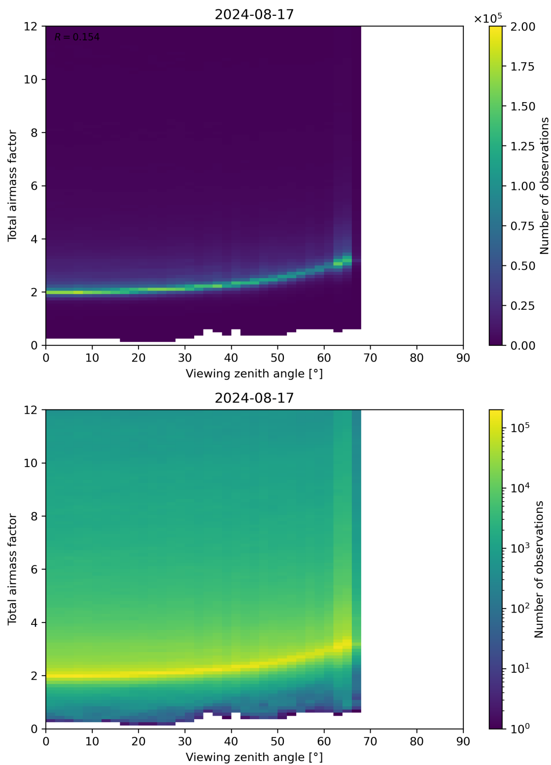
Figure 160: Scatter density plot of “Viewing zenith angle” against “Total airmass factor” for 2024-08-16 to 2024-08-18.
