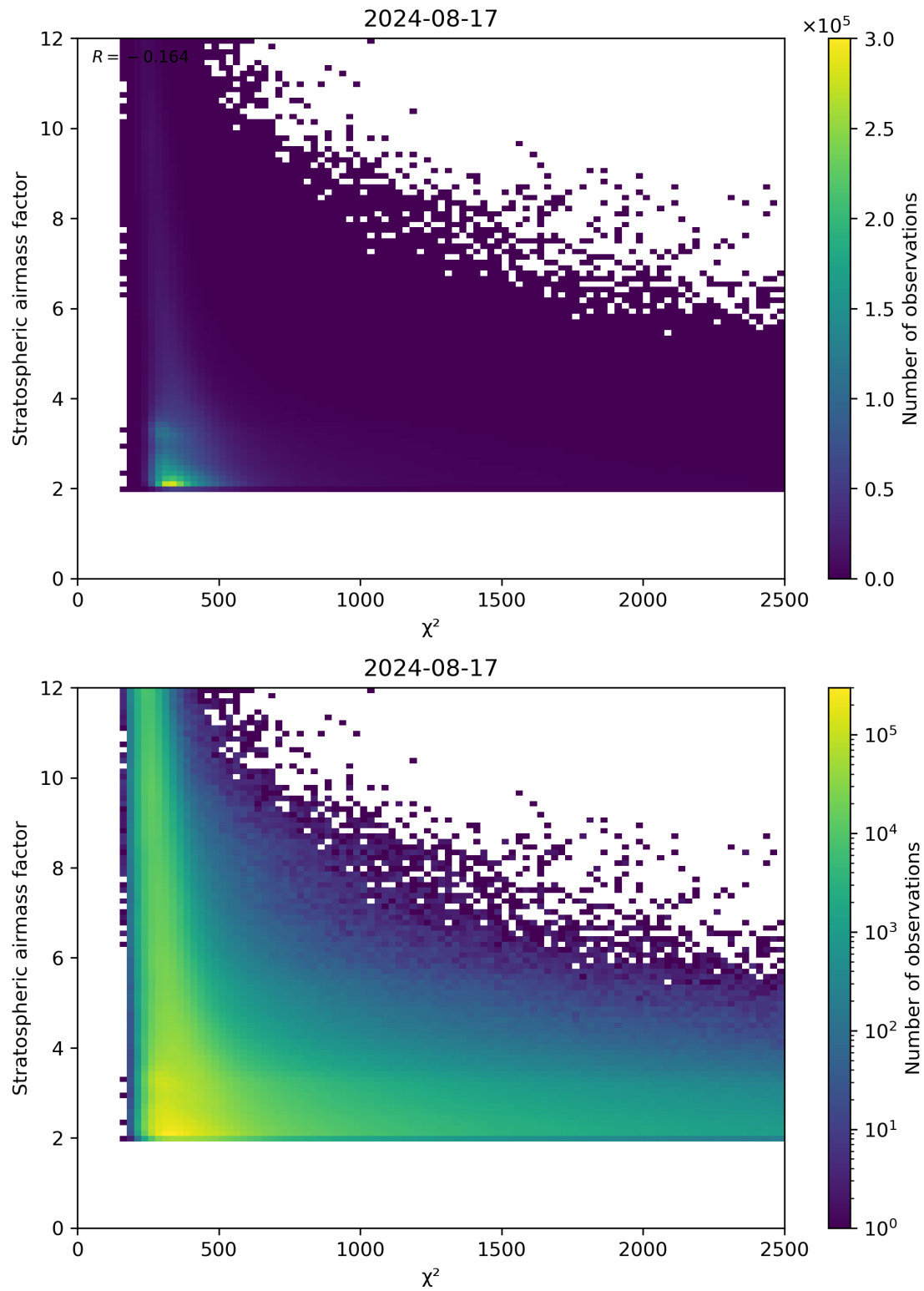
Figure 81: Scatter density plot of “ \chi^2 ” against “Stratospheric air mass factor” for 2024-08-16 to 2024-08-18.
