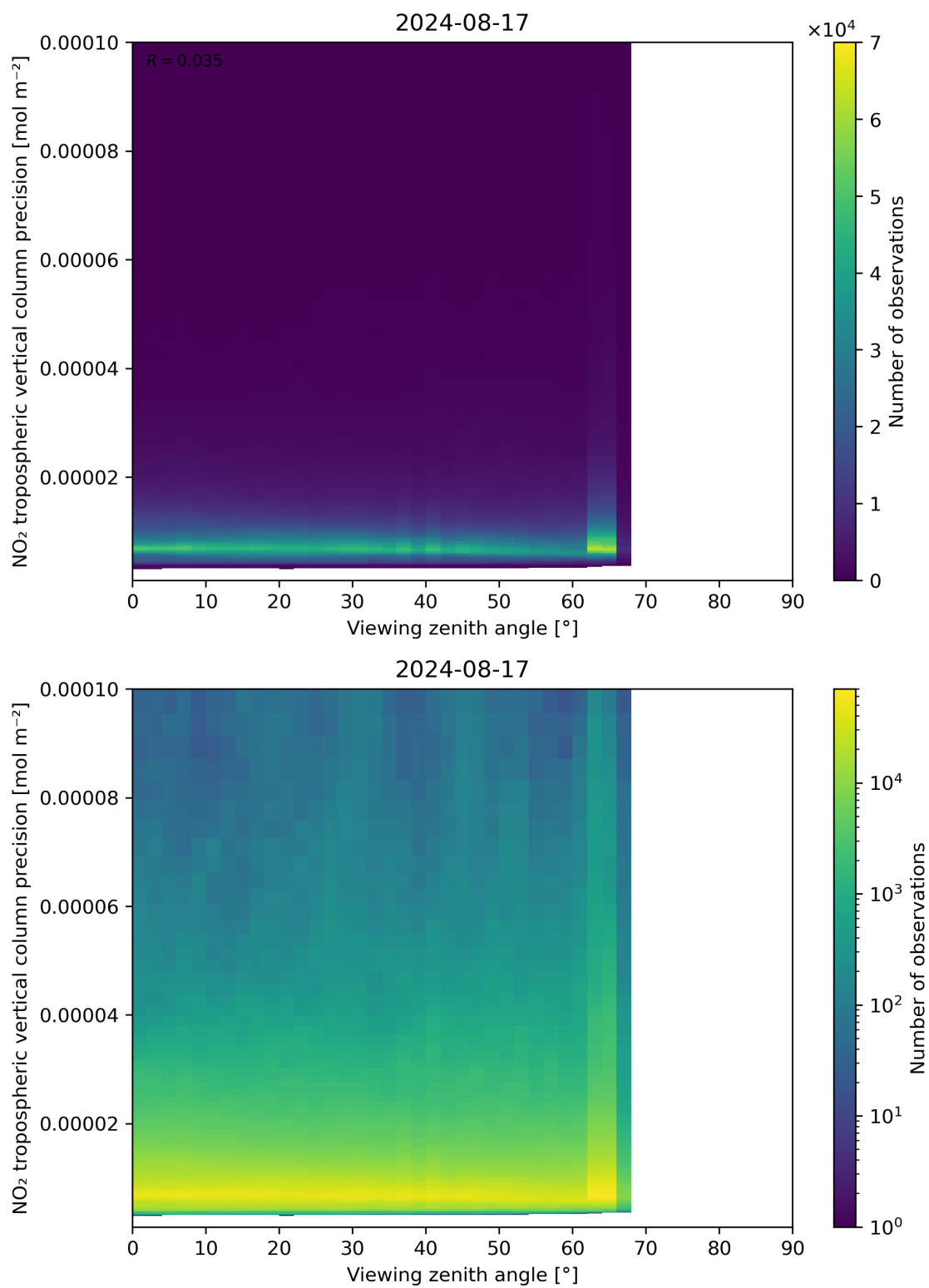
Figure 170: Scatter density plot of “Viewing zenith angle” against “NO 2 tropospheric vertical column precision” for 2024-08-16 to 2024-08-18.
