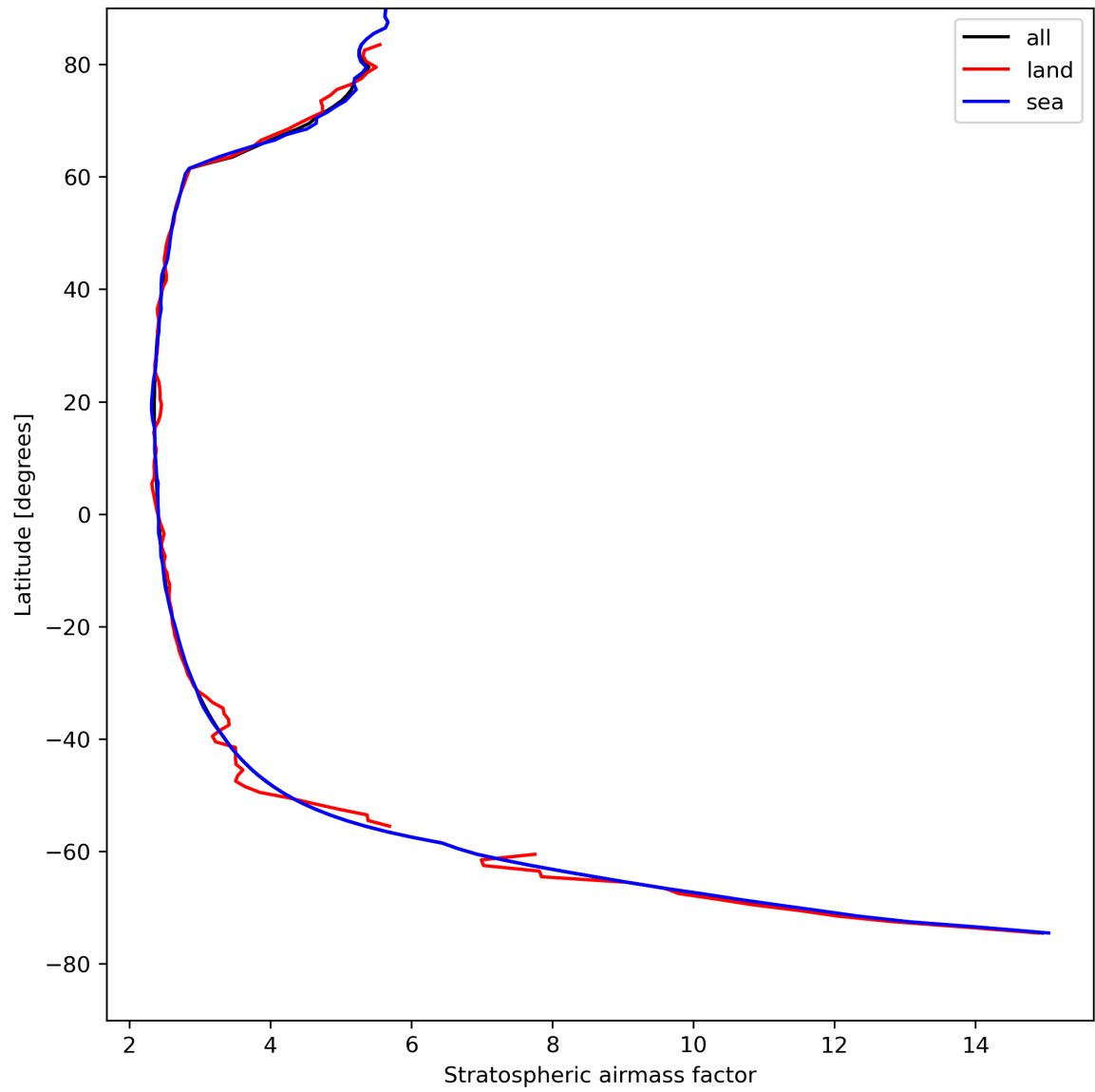
Figure 27: Zonal average of “Stratospheric air mass factor” for 2024-08-16 to 2024-08-18.
