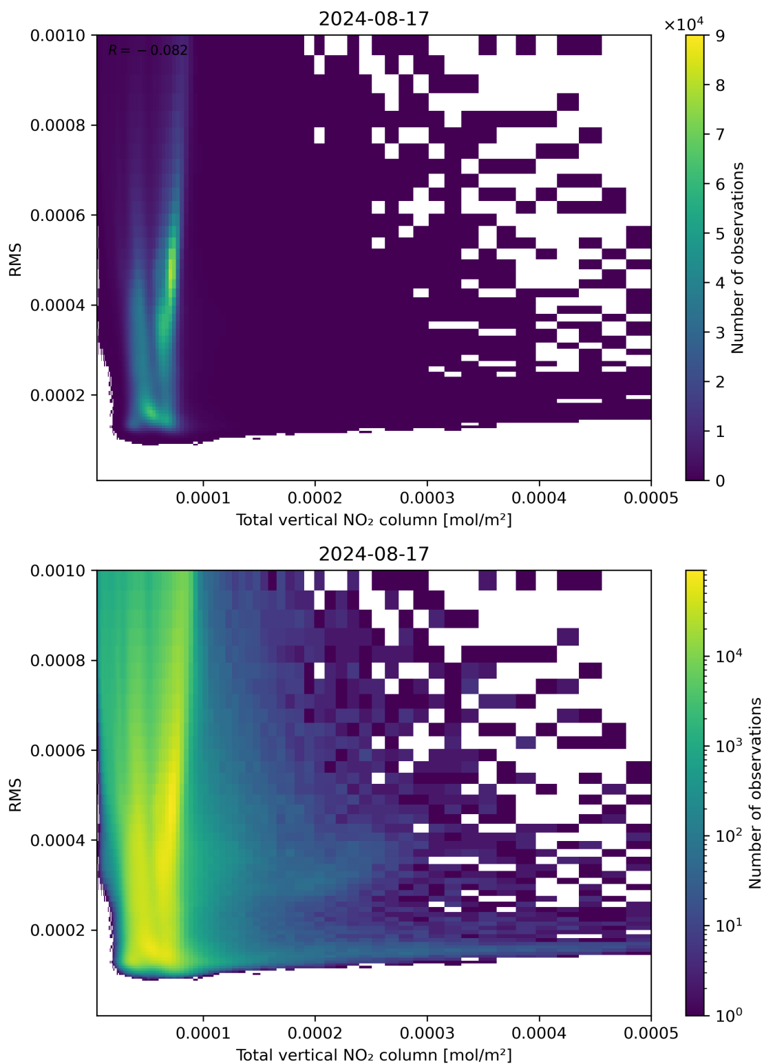
Figure 120: Scatter density plot of “Total vertical NO 2 column” against “RMS” for 2024-08-16 to 2024-08-18.
