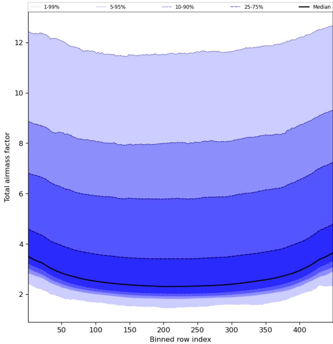
Figure 49: Along track statistics of “Total airmass factor” for 2024-08-16 to 2024-08-18
