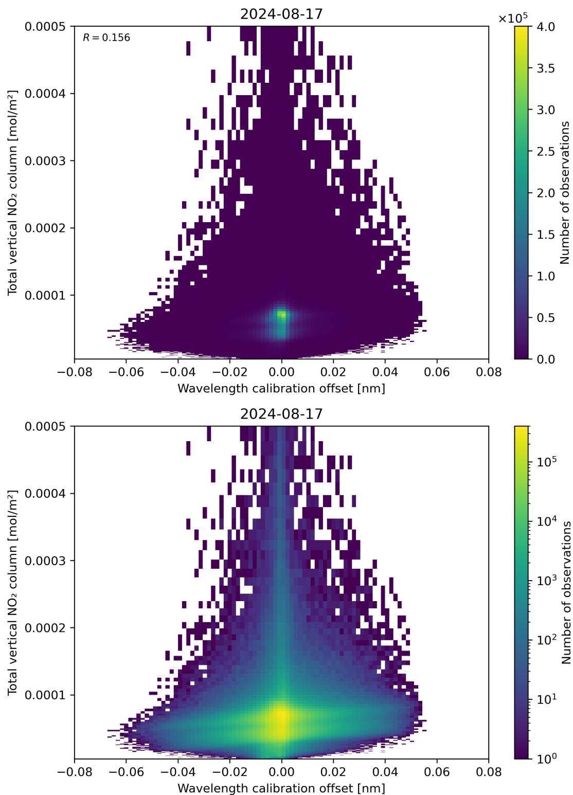
Figure 179: Scatter density plot of “Wavelength calibration offset” against “Total vertical NO 2 column” for 2024-08-16 to 2024-08-18.
