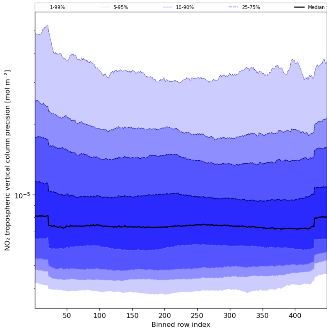
Figure 47: Along track statistics of “NO 2 tropospheric vertical column precision” for 2024-08-16 to 2024-08-18
