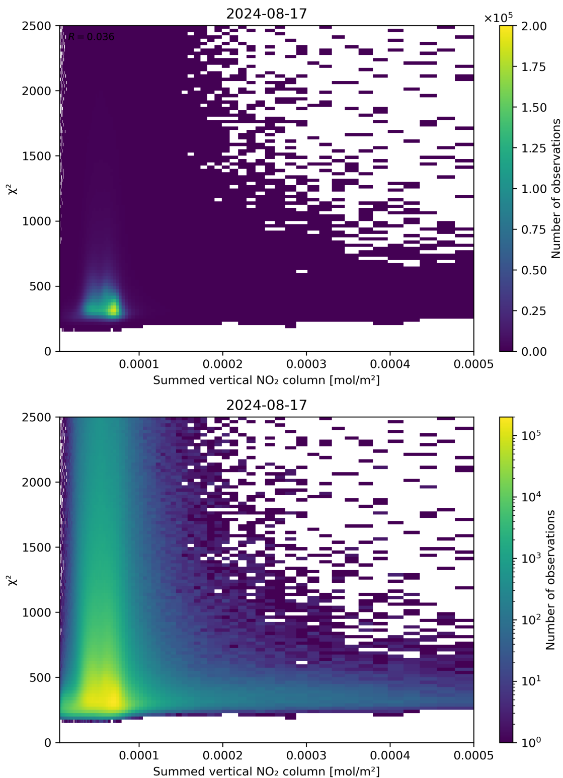
Figure 104: Scatter density plot of “Summed vertical NO 2 column” against “ \chi^2 ” for 2024-08-16 to 2024-08-18.
