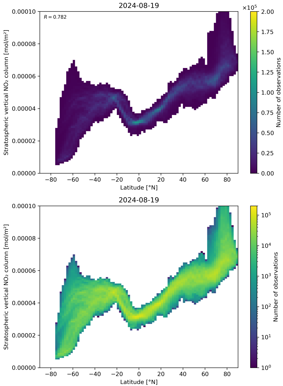
Figure 87: Scatter density plot of “Latitude” against “Stratospheric vertical NO 2 column” for 2024-08-18 to 2024-08-20.
