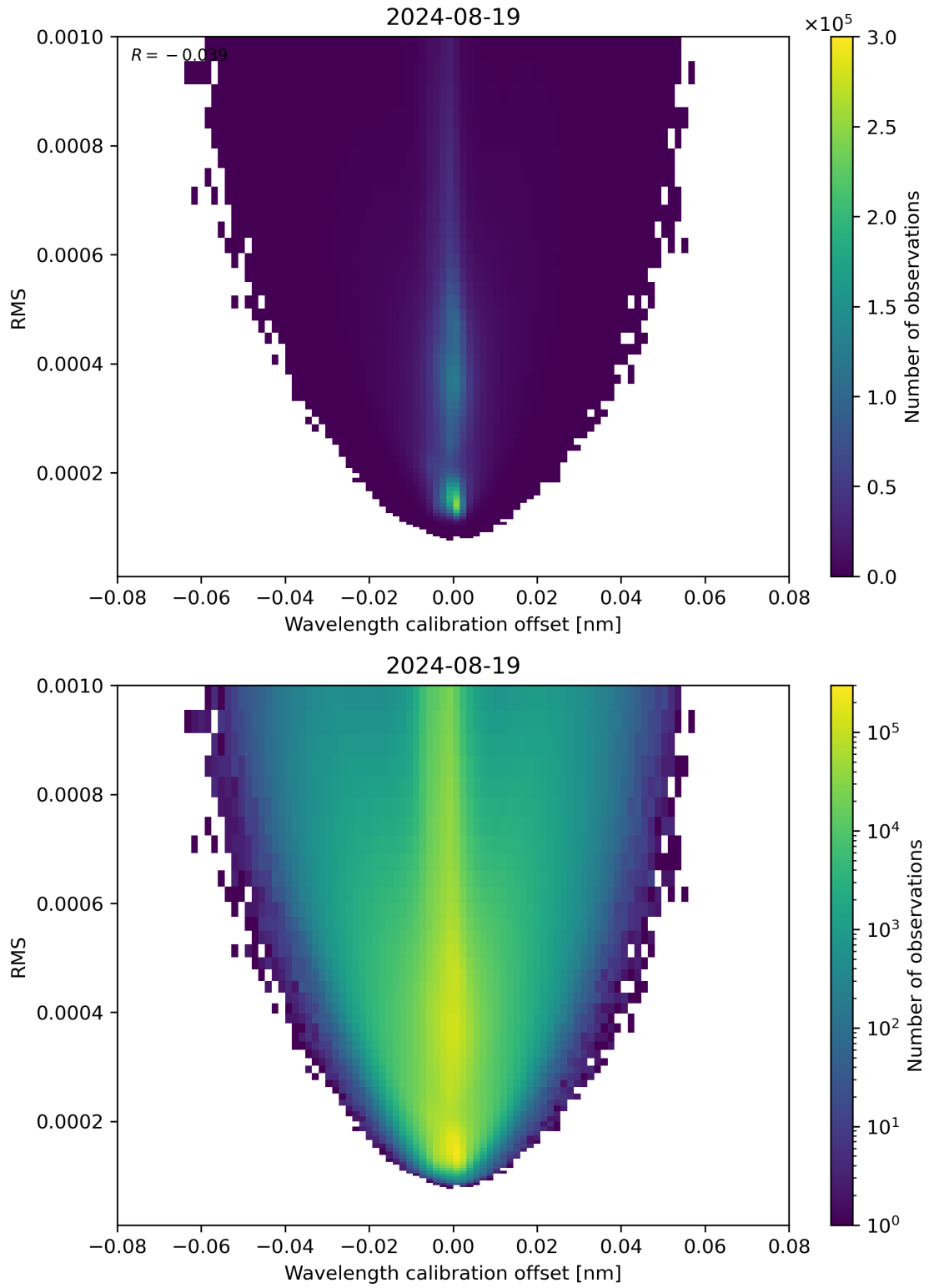
Figure 181: Scatter density plot of “Wavelength calibration offset” against “RMS” for 2024-08-18 to 2024-08-20.
