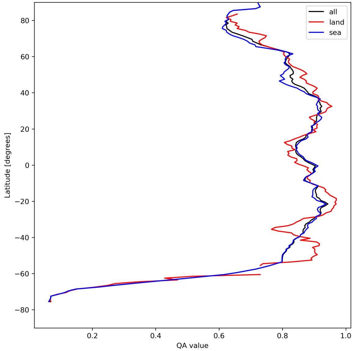
Figure 11: Zonal average of “QA value” for 2024-08-18 to 2024-08-20.
