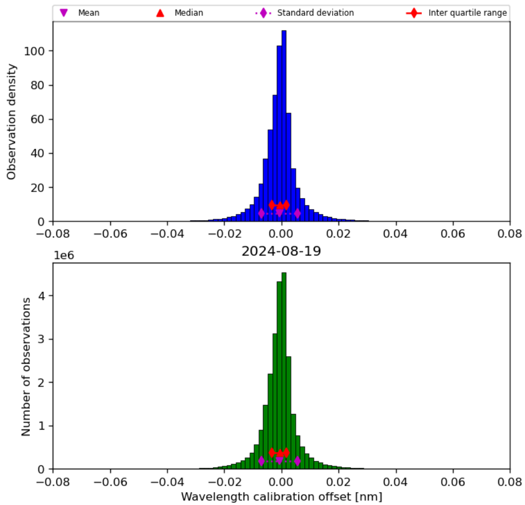
Figure 35: Histogram of “Wavelength calibration offset” for 2024-08-18 to 2024-08-20
