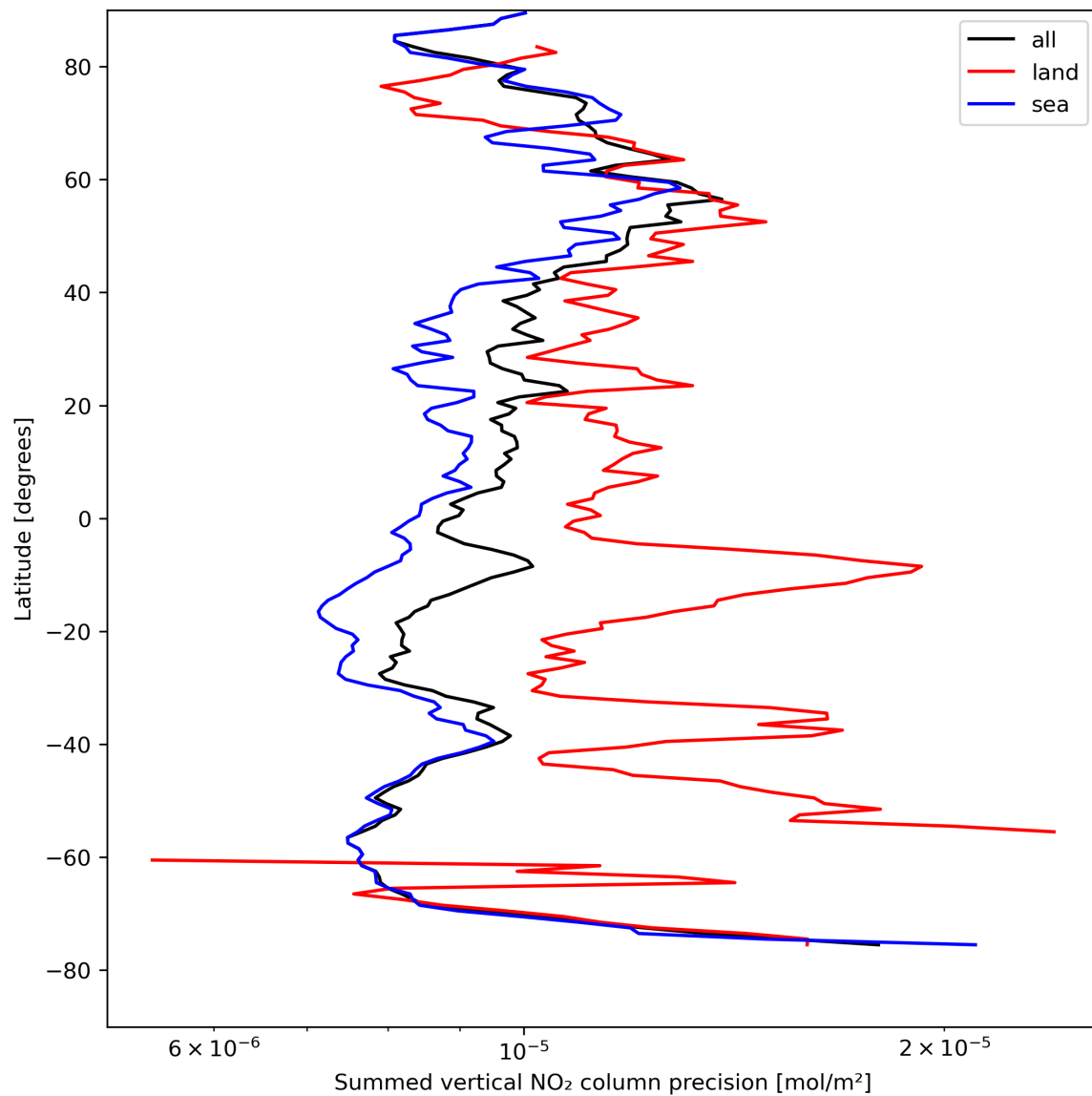
Figure 24: Zonal average of “Summed vertical NO 2 column precision” for 2024-08-18 to 2024-08-20.
