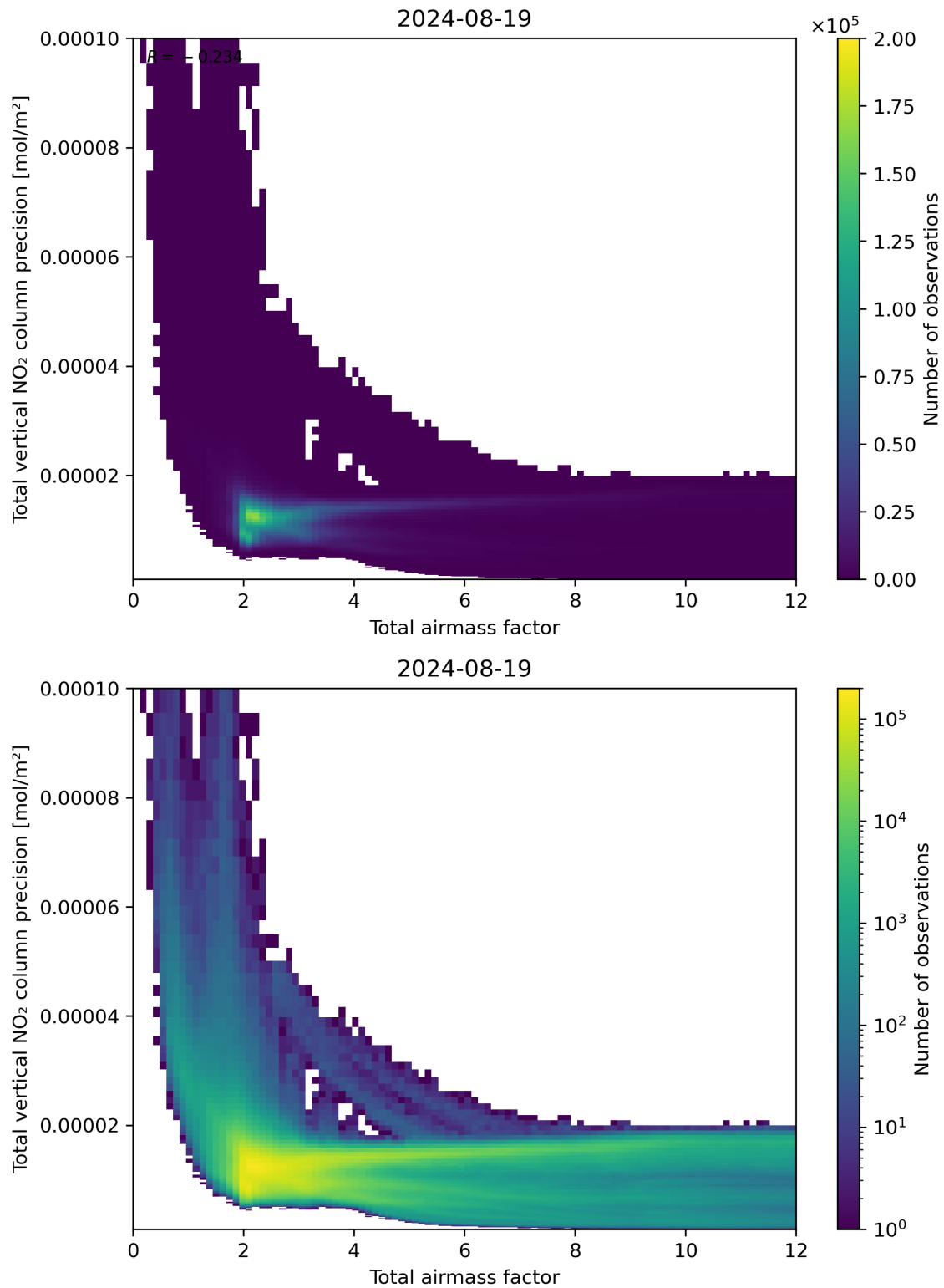
Figure 68: Scatter density plot of “Total airmass factor” against “Total vertical NO 2 column precision” for 2024-08-18 to 2024-08-20.
