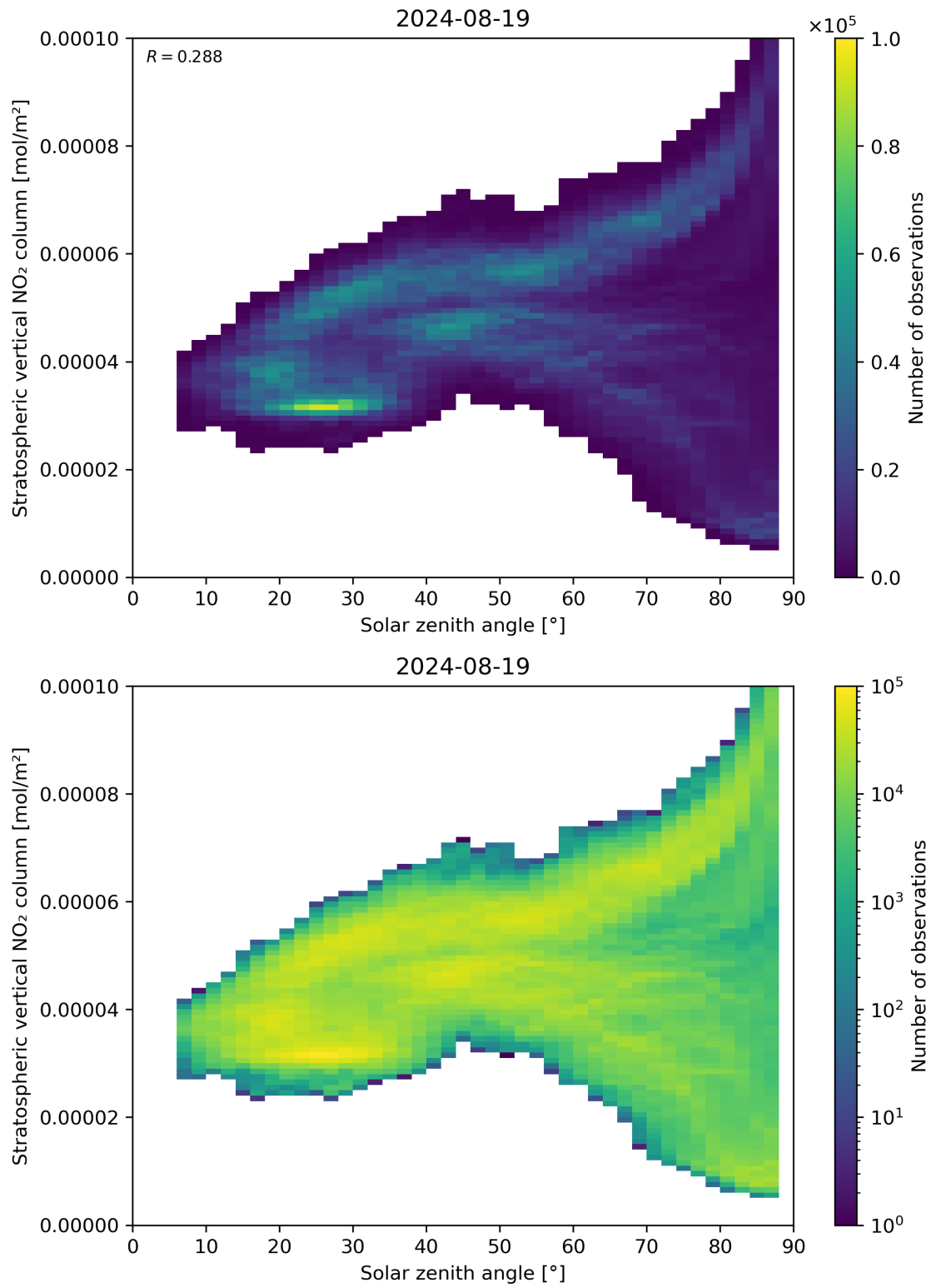
Figure 150: Scatter density plot of “Solar zenith angle” against “Stratospheric vertical NO 2 column” for 2024-08-18 to 2024-08-20.
