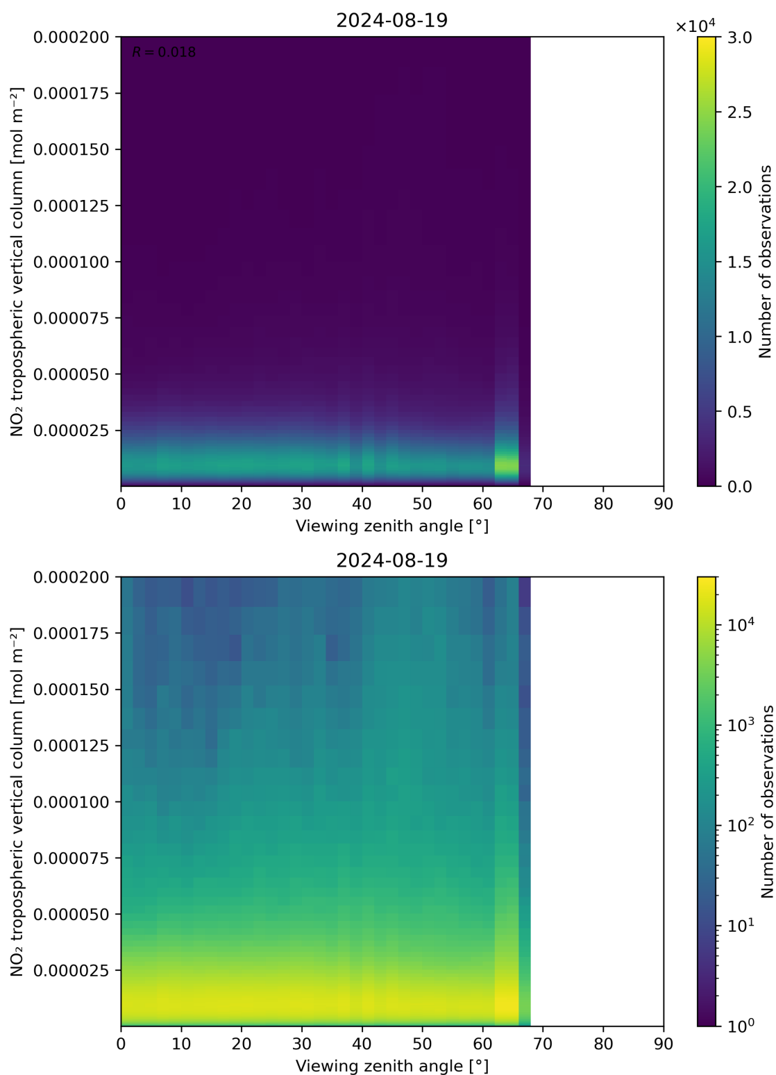
Figure 169: Scatter density plot of “Viewing zenith angle” against “NO 2 tropospheric vertical column” for 2024-08-18 to 2024-08-20.
