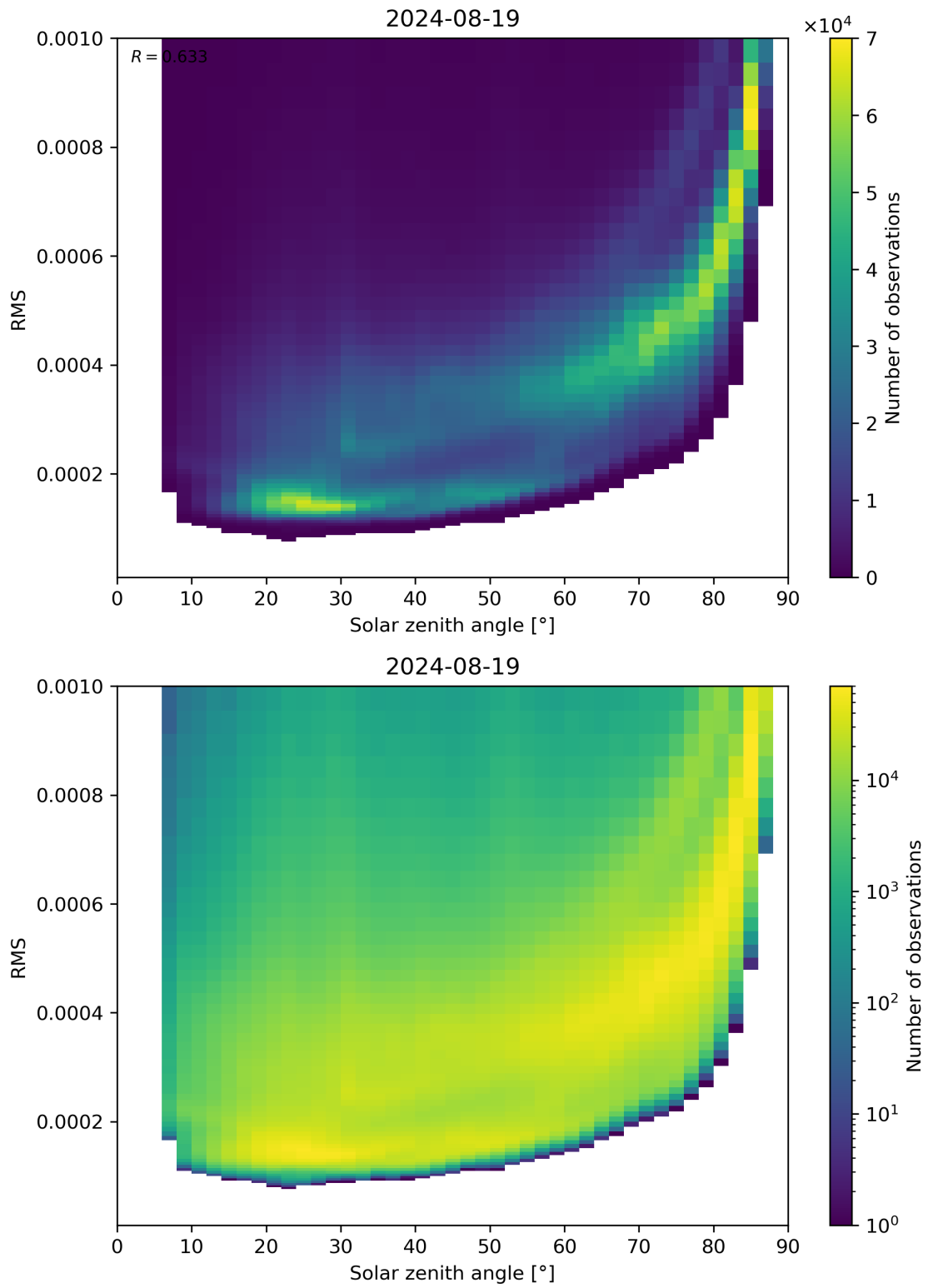
Figure 157: Scatter density plot of “Solar zenith angle” against “RMS” for 2024-08-18 to 2024-08-20.
