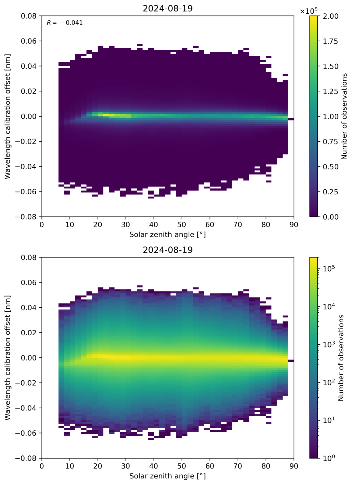
Figure 158: Scatter density plot of “Solar zenith angle” against “Wavelength calibration offset” for 2024-08-18 to 2024-08-20.
