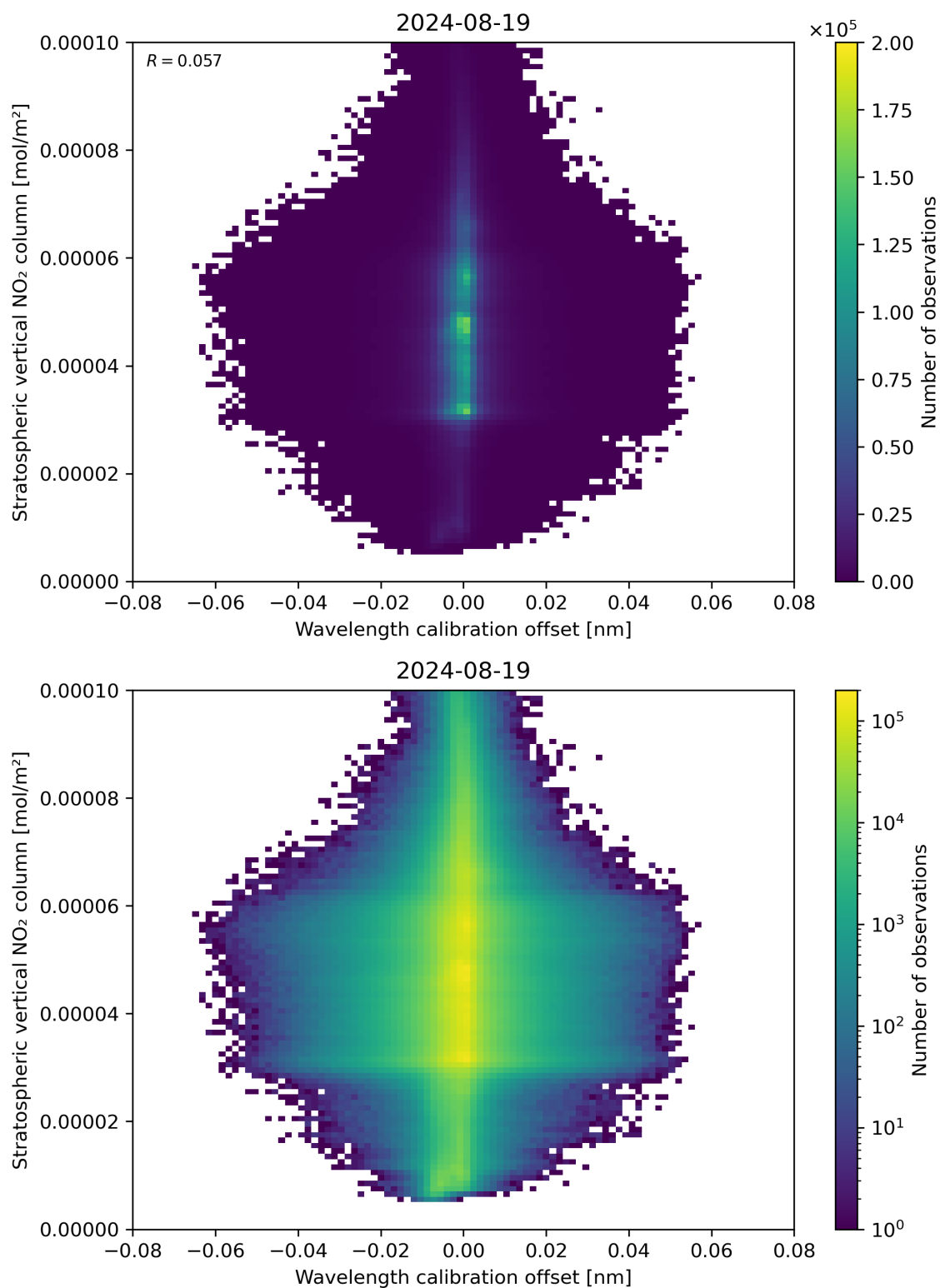
Figure 176: Scatter density plot of “Wavelength calibration offset” against “Stratospheric vertical NO 2 column” for 2024-08-18 to 2024-08-20.
