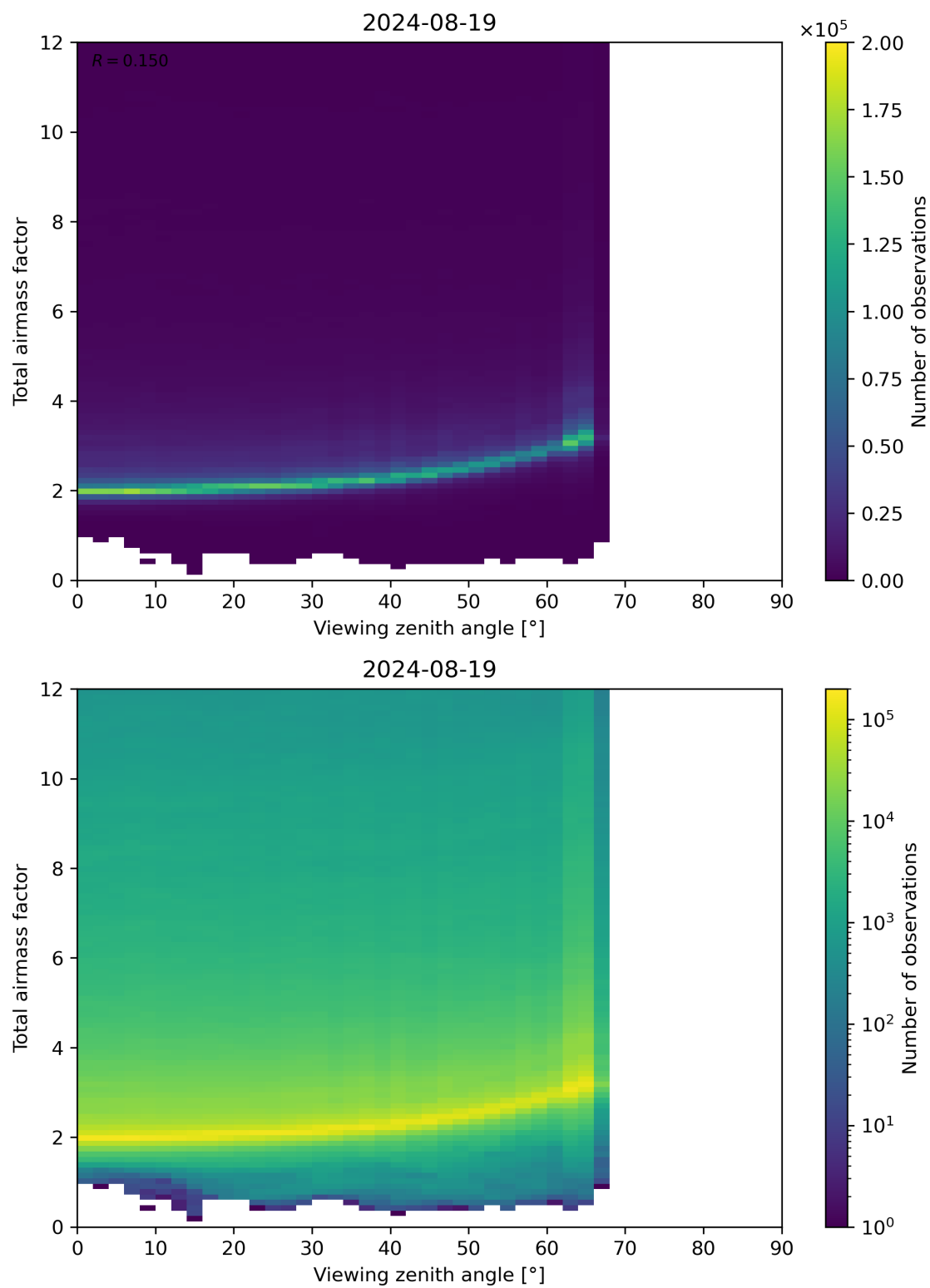
Figure 160: Scatter density plot of “Viewing zenith angle” against “Total airmass factor” for 2024-08-18 to 2024-08-20.
