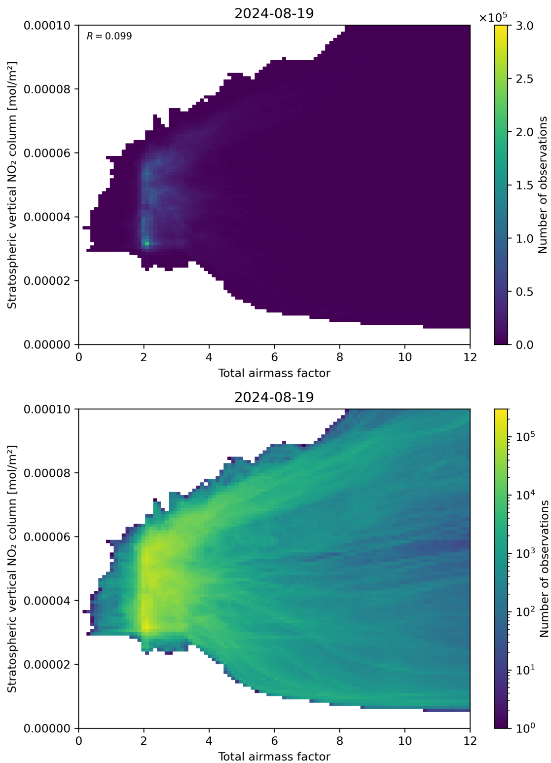
Figure 64: Scatter density plot of “Total airmass factor” against “Stratospheric vertical \text{NO}_2 column” for 2024-08-18 to 2024-08-20.
