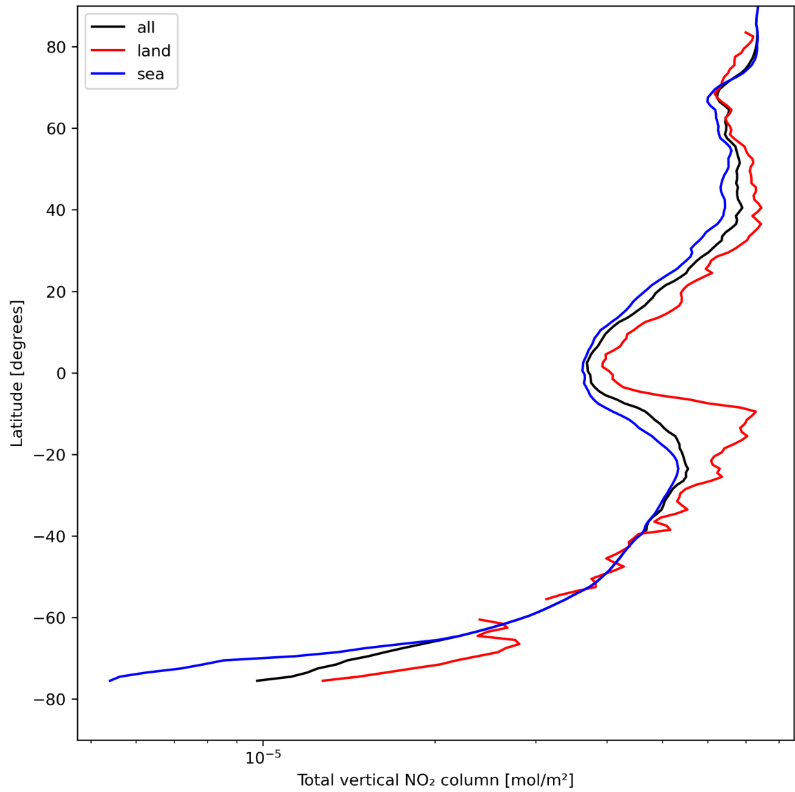
Figure 21: Zonal average of “Total vertical NO 2 column” for 2024-08-18 to 2024-08-20.
