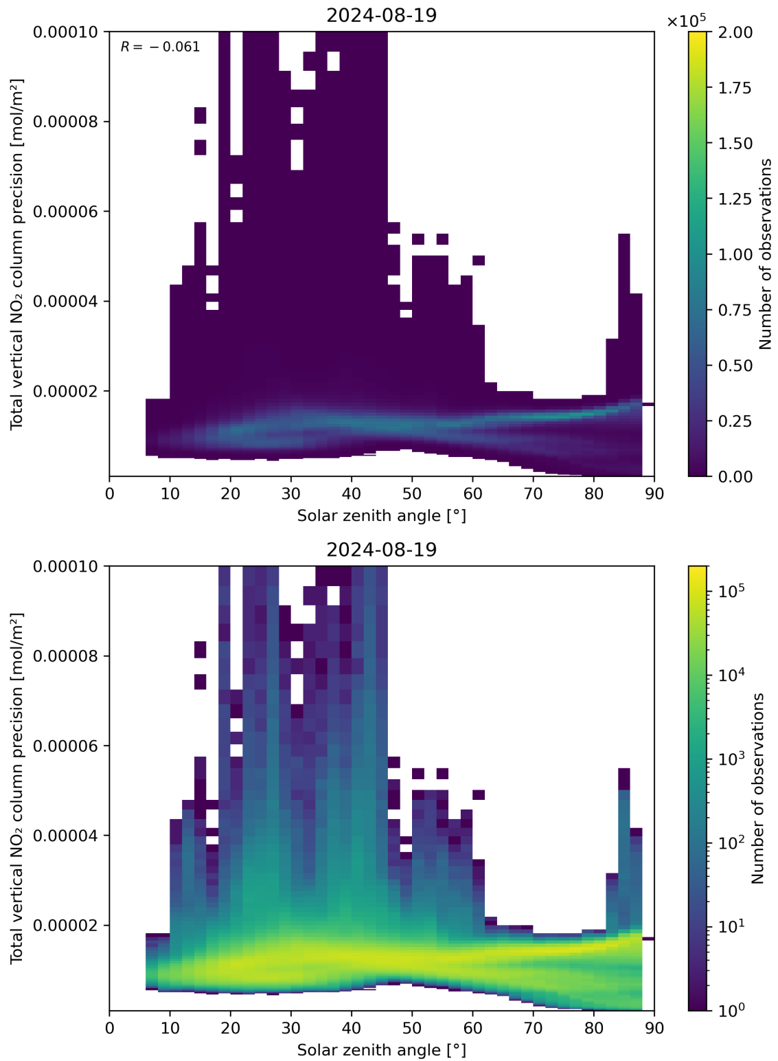
Figure 154: Scatter density plot of “Solar zenith angle” against “Total vertical NO 2 column precision” for 2024-08-18 to 2024-08-20.
