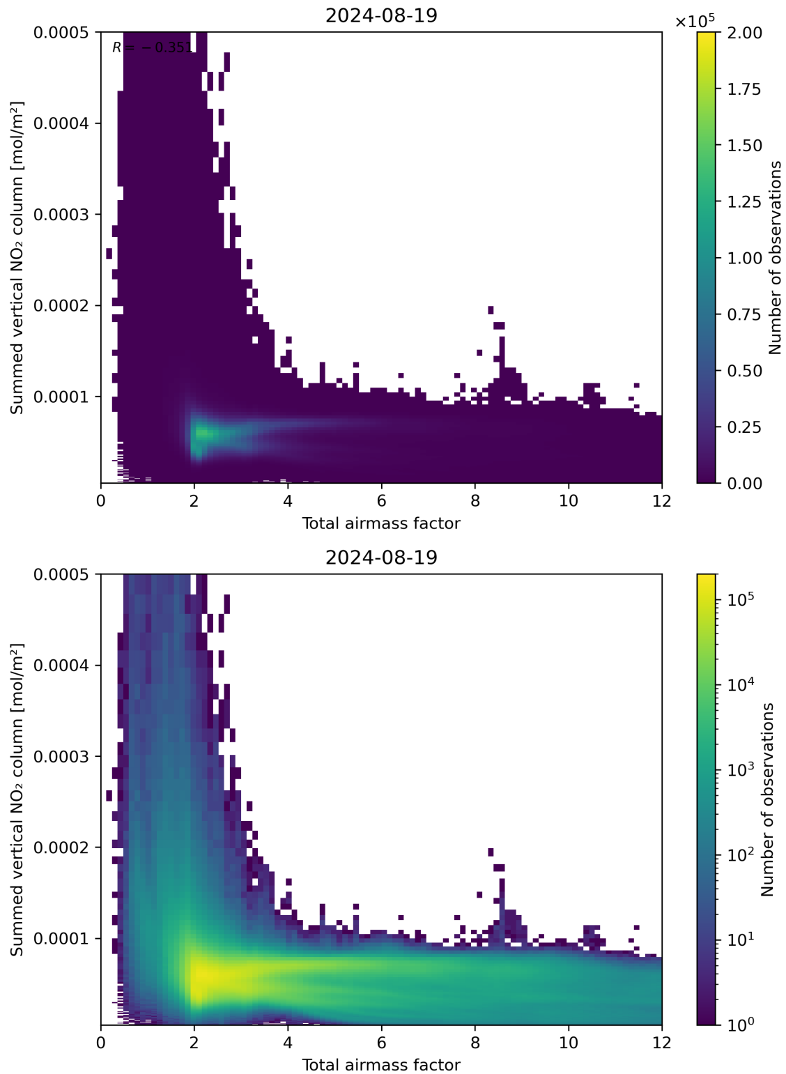
Figure 65: Scatter density plot of “Total airmass factor” against “Summed vertical NO 2 column” for 2024-08-18 to 2024-08-20.
