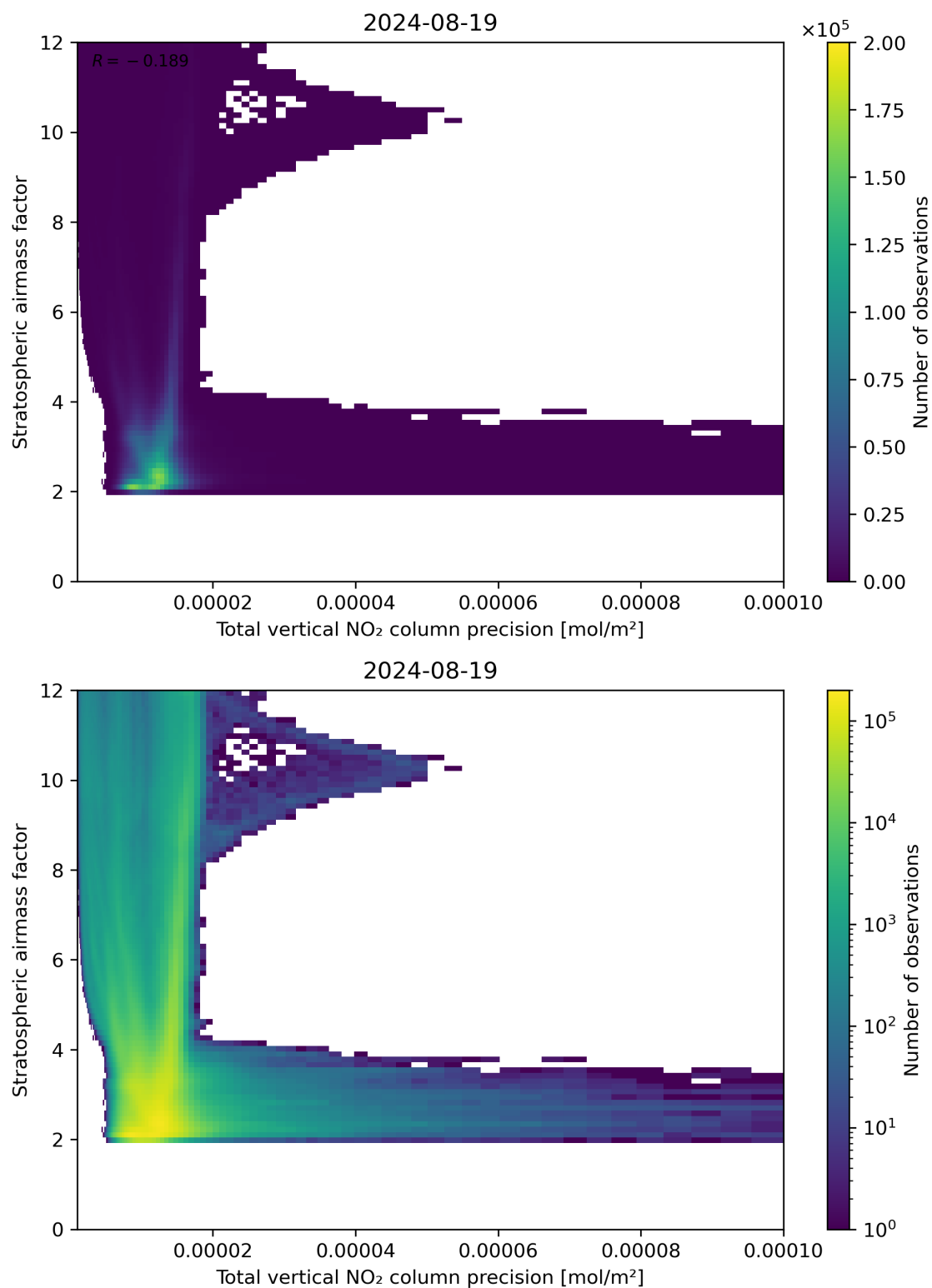
Figure 115: Scatter density plot of “Total vertical NO 2 column precision” against “Stratospheric air mass factor” for 2024-08-18 to 2024-08-20.
