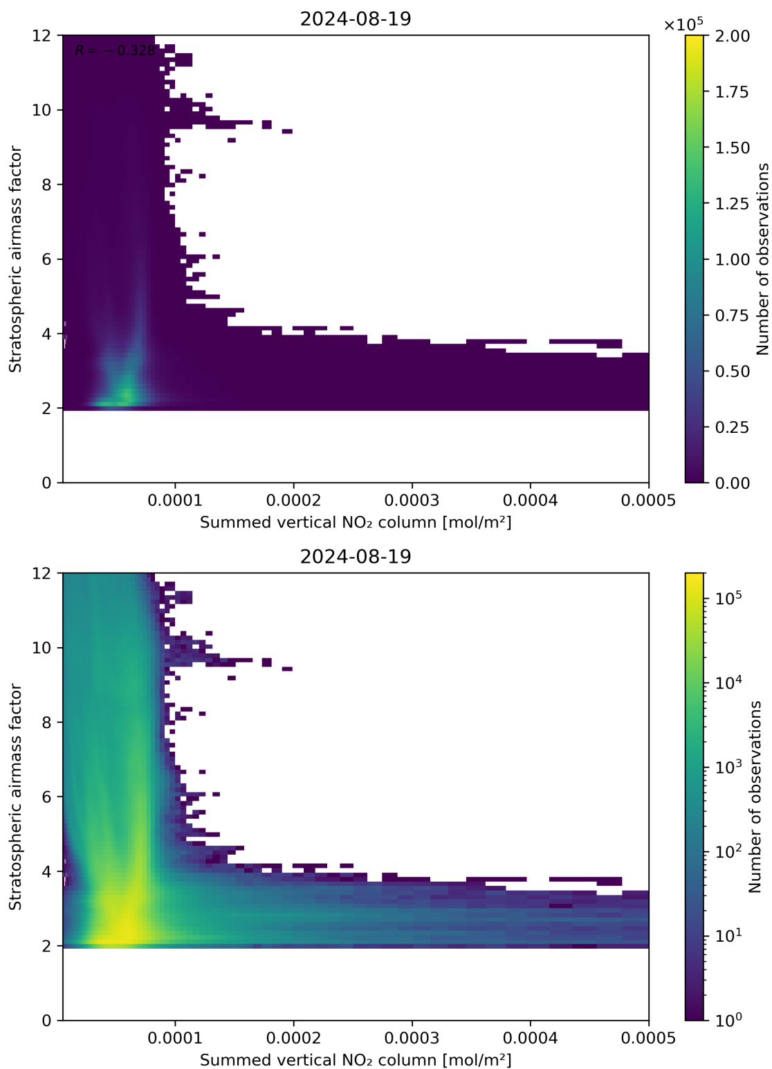
Figure 103: Scatter density plot of “Summed vertical NO 2 column” against “Stratospheric airmass factor” for 2024-08-18 to 2024-08-20.
