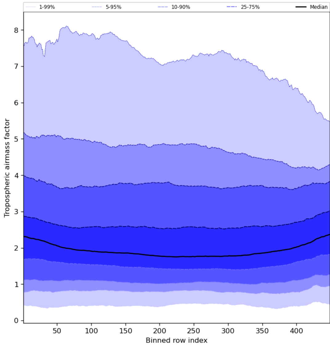
Figure 48: Along track statistics of “Tropospheric airmass factor” for 2024-08-18 to 2024-08-20
