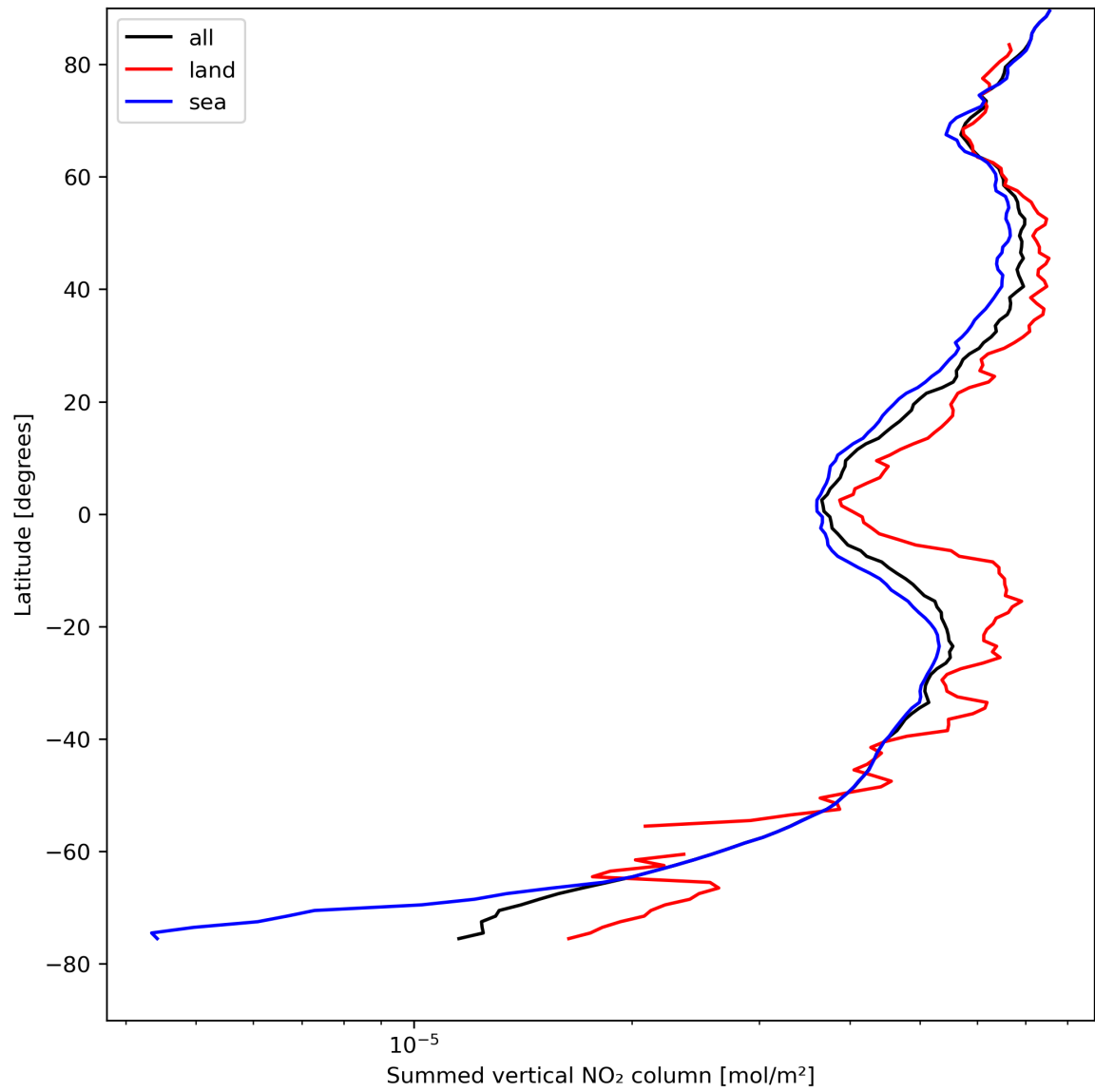
Figure 23: Zonal average of “Summed vertical NO 2 column” for 2024-08-18 to 2024-08-20.
