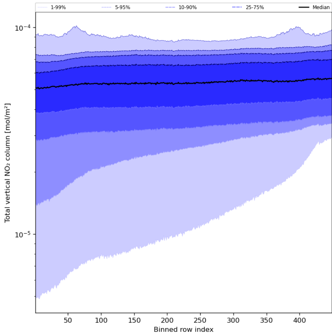
Figure 55: Along track statistics of “Total vertical NO 2 column” for 2024-08-18 to 2024-08-20
