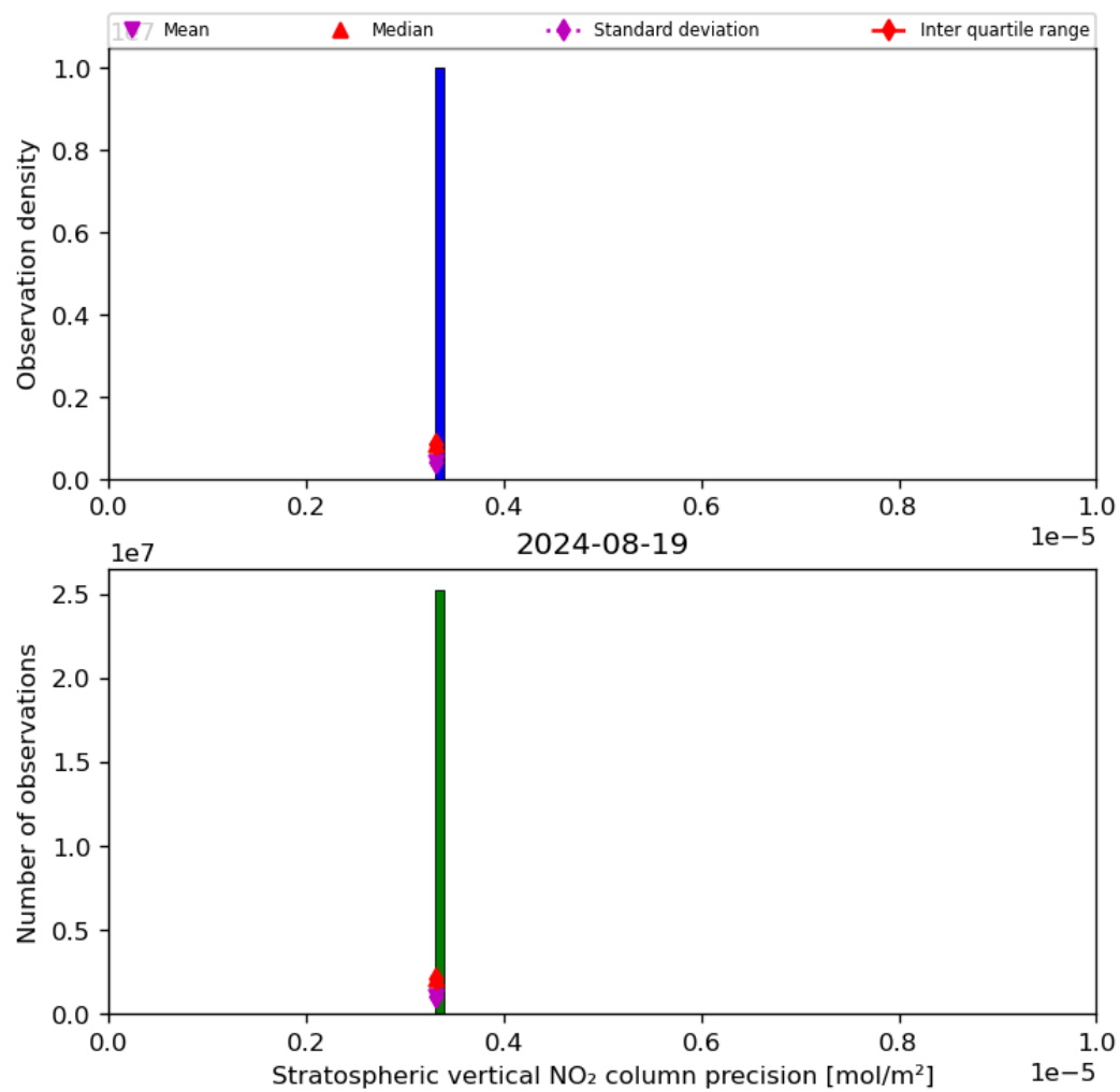
Figure 37: Histogram of “Stratospheric vertical NO 2 column precision” for 2024-08-18 to 2024-08-20
