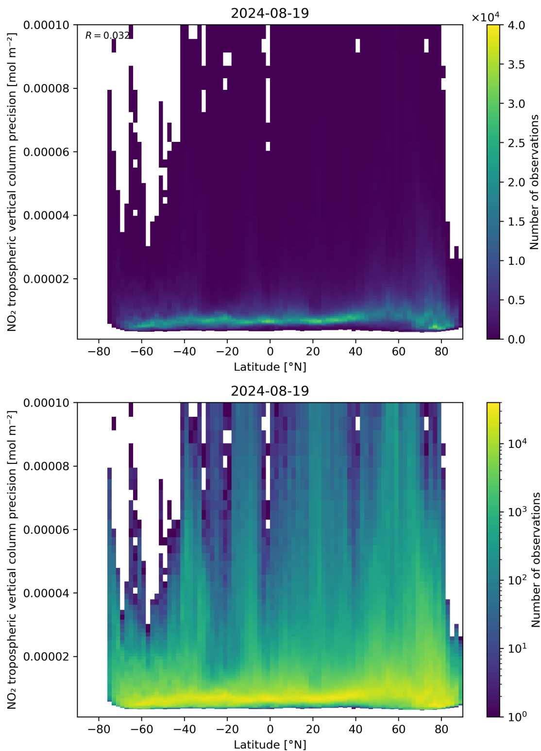
Figure 93: Scatter density plot of “Latitude” against “NO 2 tropospheric vertical column precision” for 2024-08-18 to 2024-08-20.
