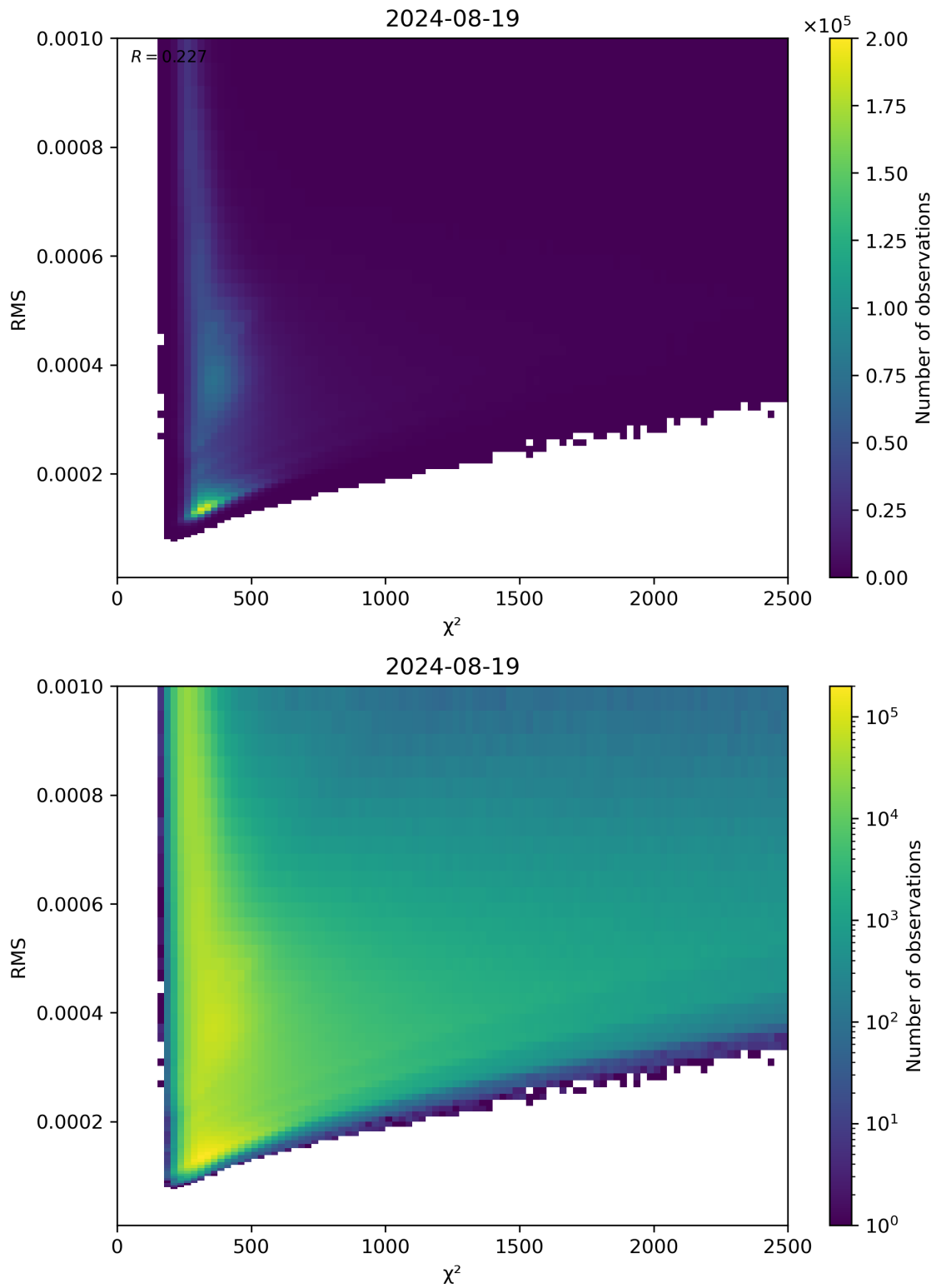
Figure 82: Scatter density plot of “ \chi^2 ” against “RMS” for 2024-08-18 to 2024-08-20.
