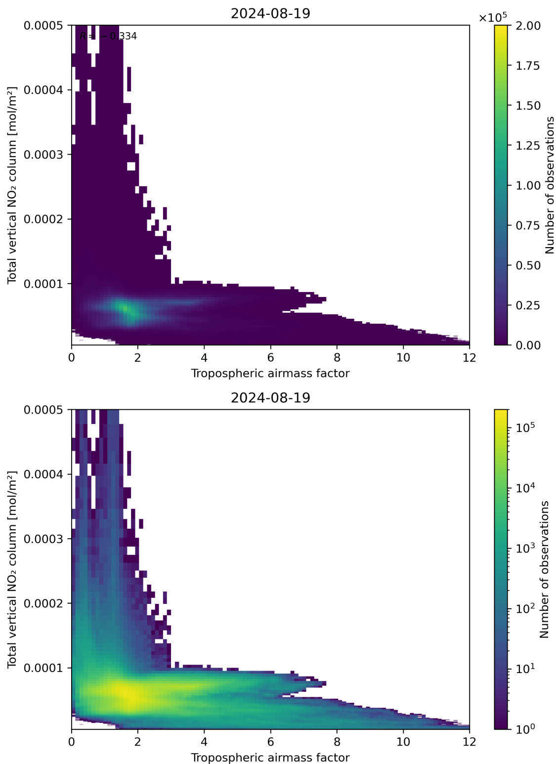
Figure 77: Scatter density plot of “Tropospheric airmass factor” against “Total vertical NO 2 column” for 2024-08-18 to 2024-08-20.
