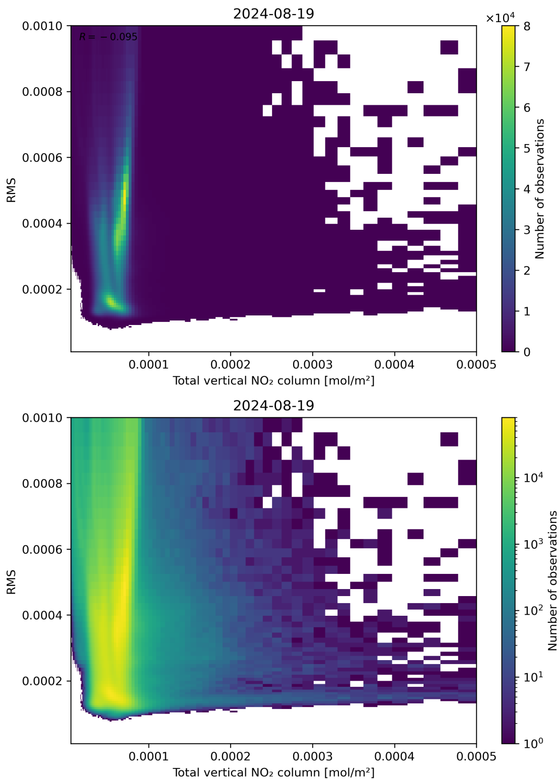
Figure 120: Scatter density plot of “Total vertical NO 2 column” against “RMS” for 2024-08-18 to 2024-08-20.
