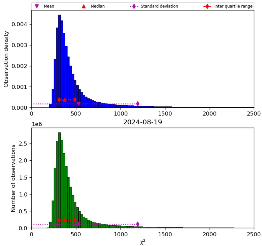
Figure 42: Histogram of " \chi^2 " for 2024-08-18 to 2024-08-20
