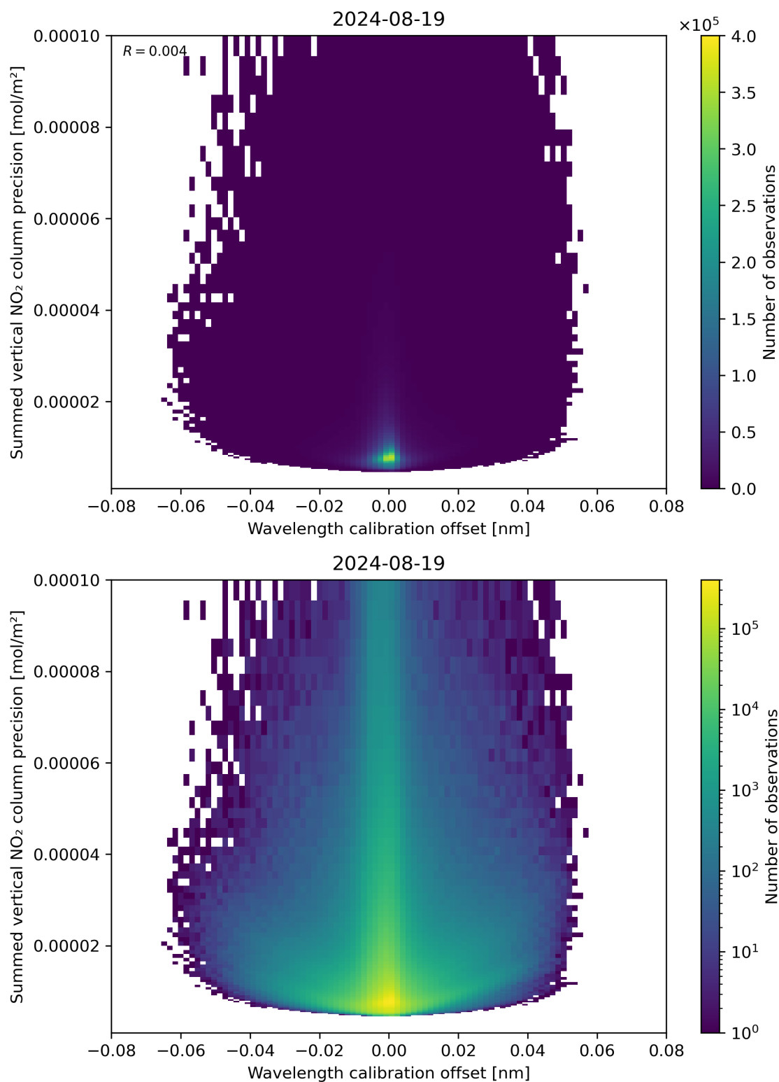
Figure 178: Scatter density plot of “Wavelength calibration offset” against “Summed vertical NO 2 column precision” for 2024-08-18 to 2024-08-20.
