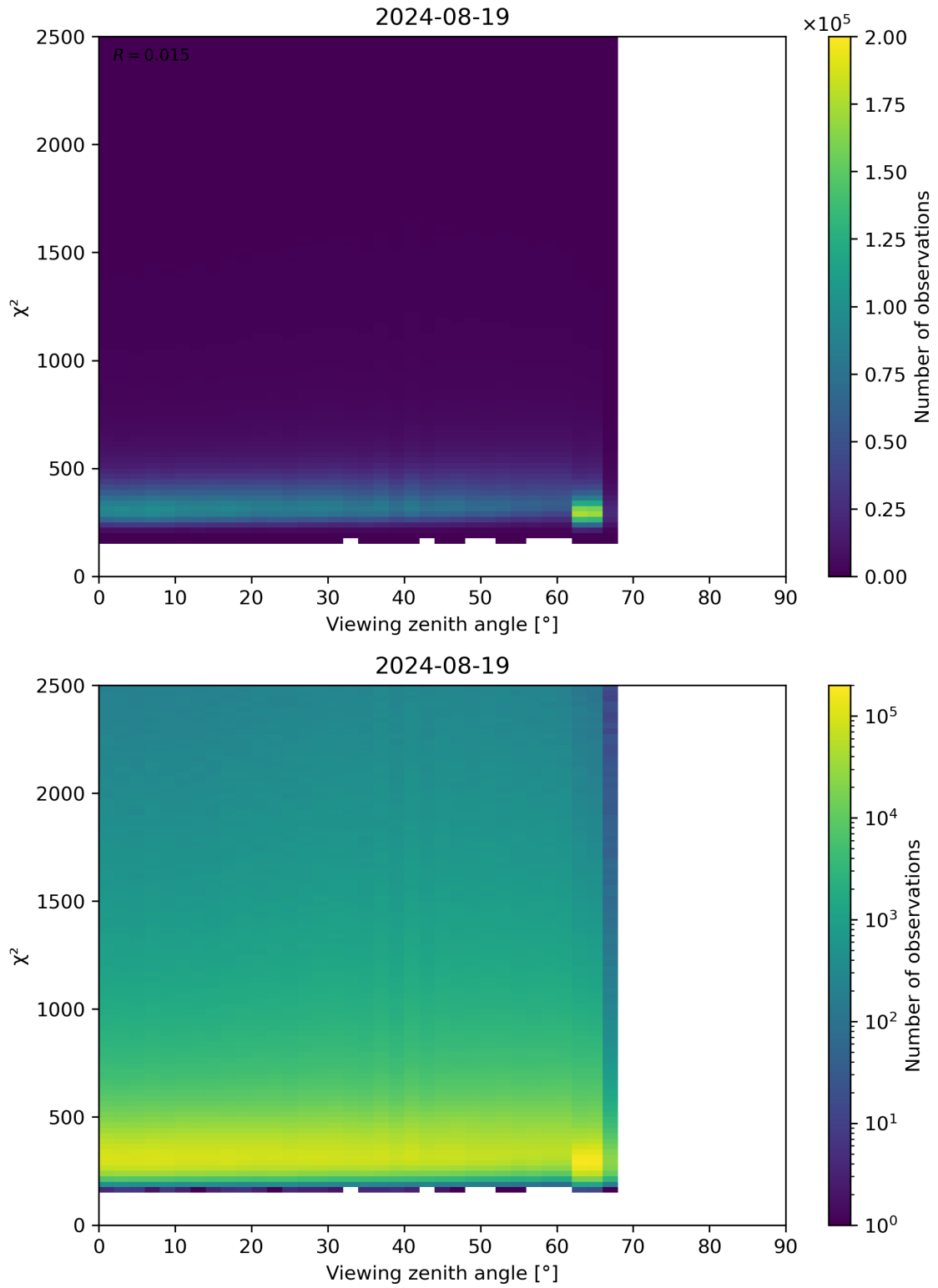
Figure 162: Scatter density plot of “Viewing zenith angle” against “ \chi^2 ” for 2024-08-18 to 2024-08-20.
