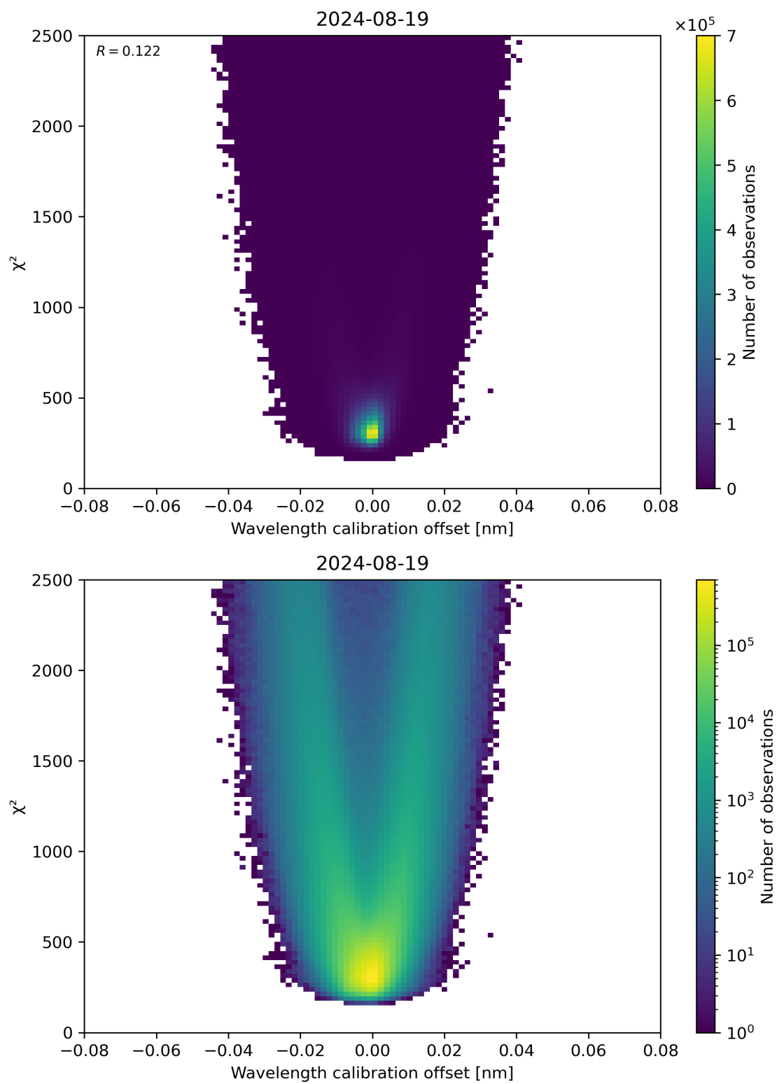
Figure 175: Scatter density plot of “Wavelength calibration offset” against “ \chi^2 ” for 2024-08-18 to 2024-08-20.
