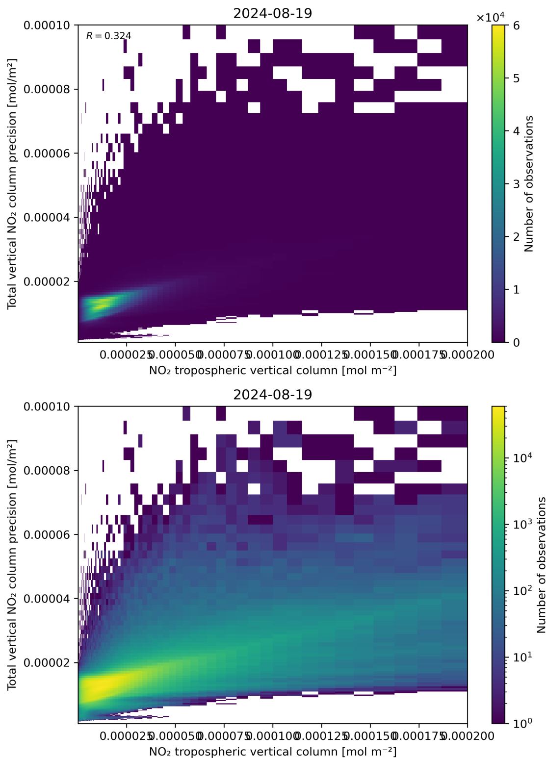
Figure 129: Scatter density plot of “NO 2 tropospheric vertical column” against “Total vertical NO 2 column precision” for 2024-08-18 to 2024-08-20.
