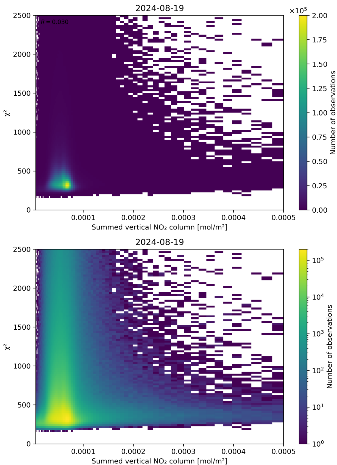
Figure 104: Scatter density plot of “Summed vertical NO 2 column” against “ \chi^2 ” for 2024-08-18 to 2024-08-20.
