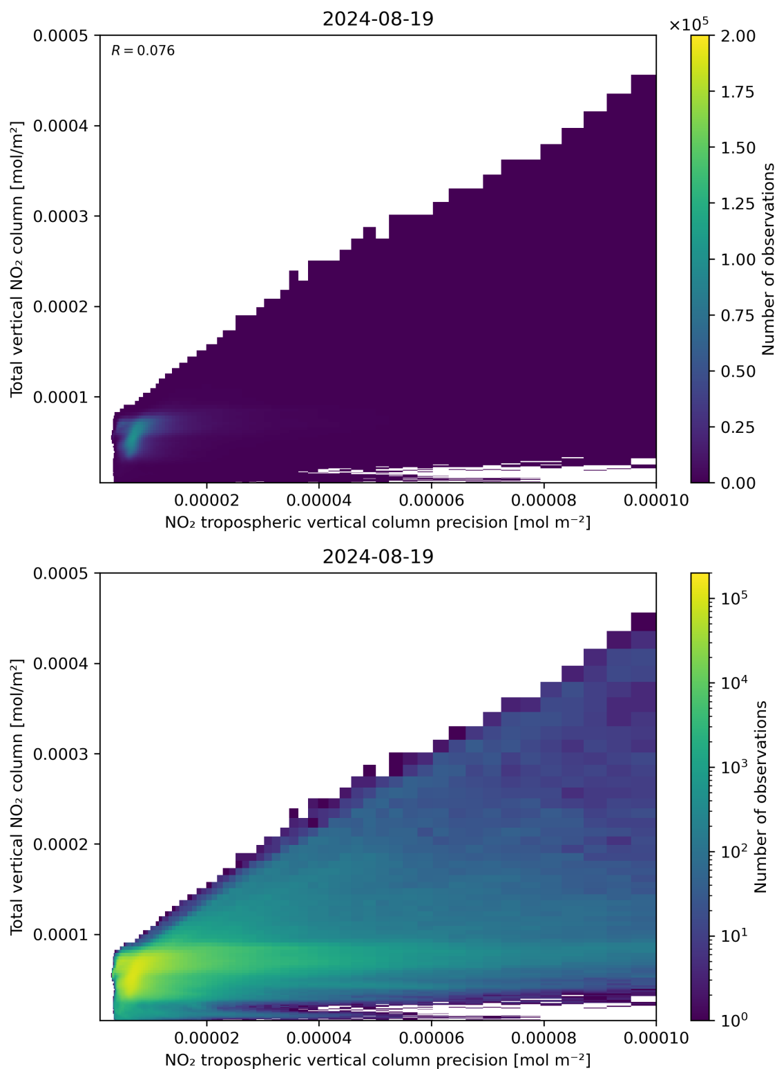
Figure 138: Scatter density plot of “NO 2 tropospheric vertical column precision” against “Total vertical NO 2 column” for 2024-08-18 to 2024-08-20.
