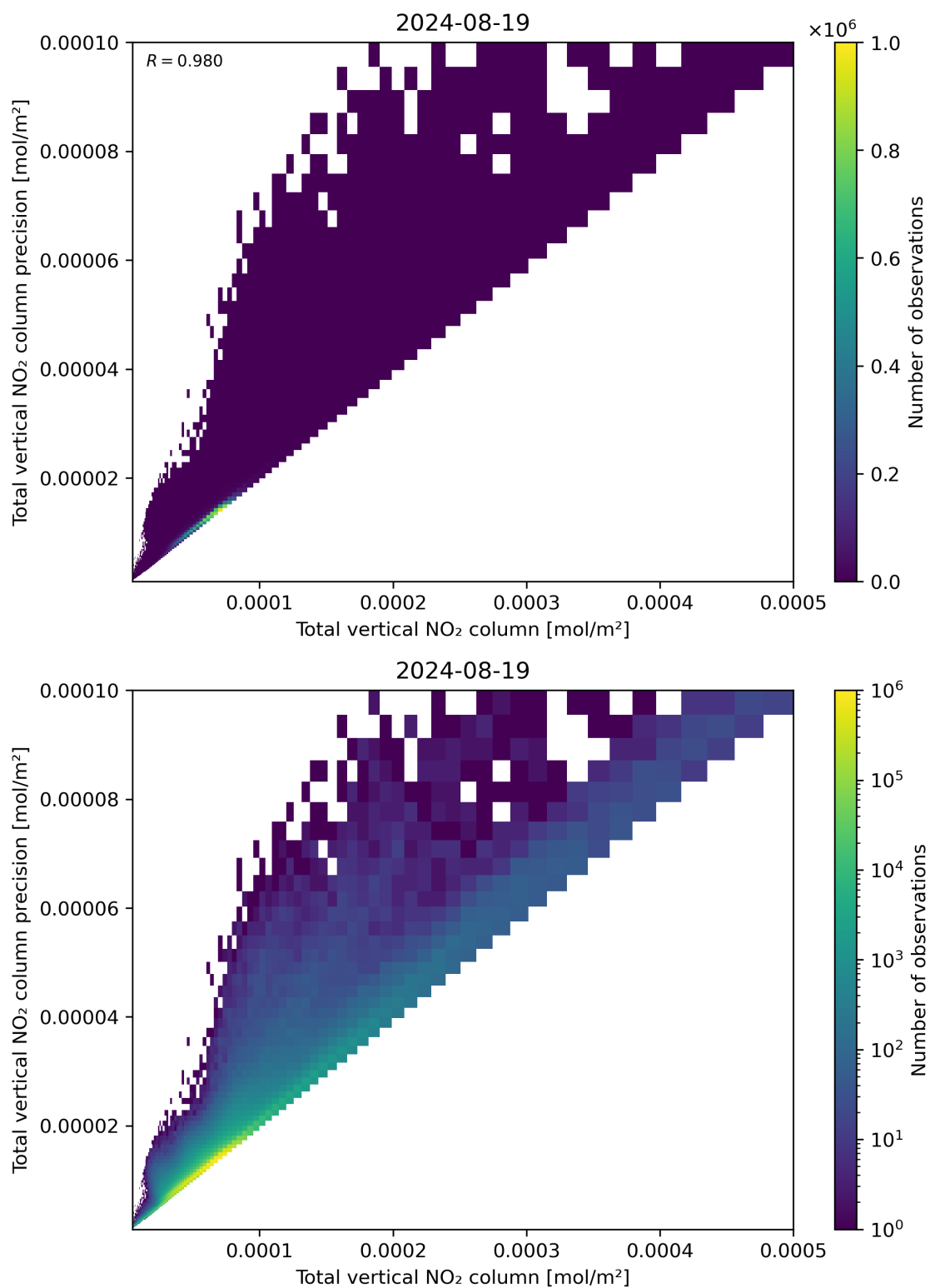
Figure 114: Scatter density plot of “Total vertical NO 2 column” against “Total vertical NO 2 column precision” for 2024-08-18 to 2024-08-20.
