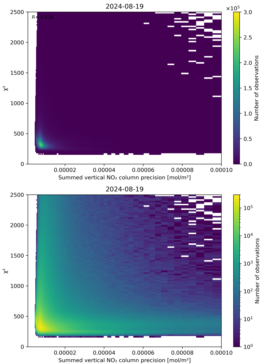
Figure 107: Scatter density plot of “Summed vertical NO 2 column precision” against “ \chi^2 ” for 2024-08-18 to 2024-08-20.
