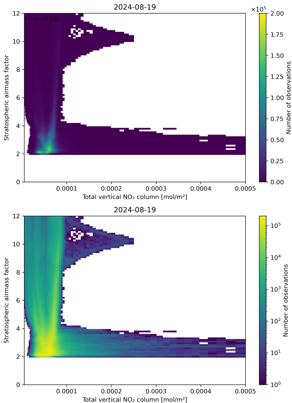
Figure 110: Scatter density plot of “Total vertical NO 2 column” against “Stratospheric airmass factor” for 2024-08-18 to 2024-08-20.
