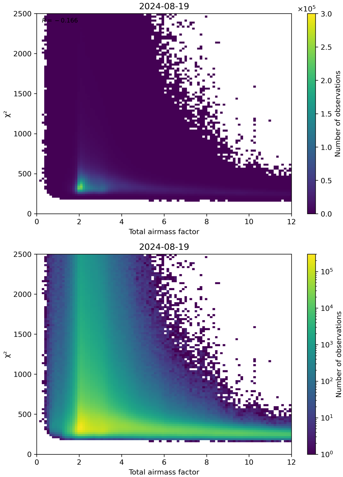
Figure 63: Scatter density plot of “Total airmass factor” against “ \chi^2 ” for 2024-08-18 to 2024-08-20.
