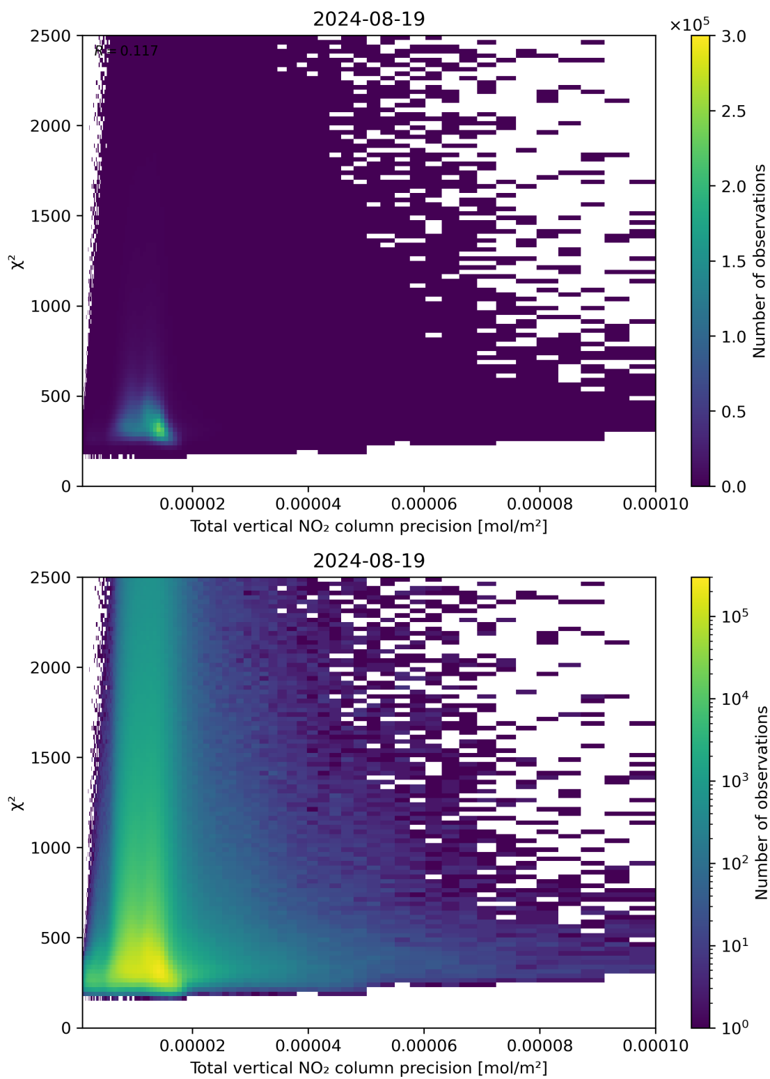
Figure 116: Scatter density plot of “Total vertical NO 2 column precision” against “ \chi^2 ” for 2024-08-18 to 2024-08-20.
