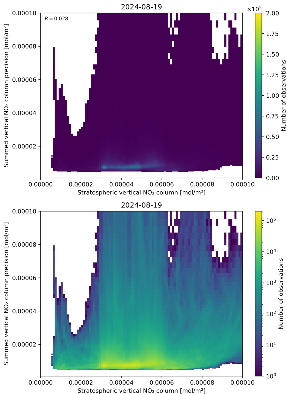
Figure 99: Scatter density plot of “Stratospheric vertical NO 2 column” against “Summed vertical NO 2 column precision” for 2024-08-18 to 2024-08-20.
