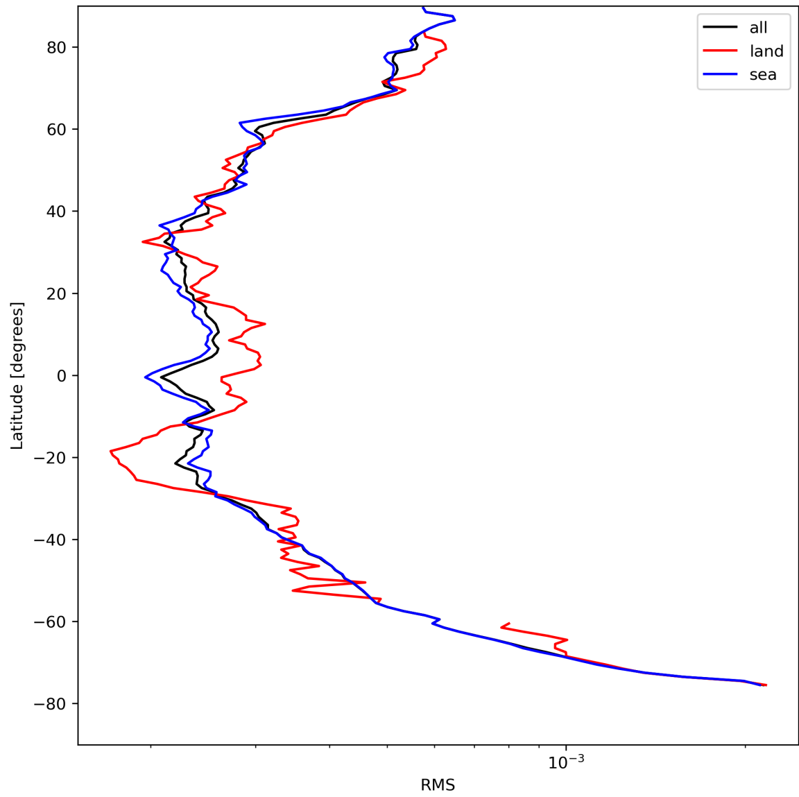
Figure 26: Zonal average of “RMS” for 2024-08-18 to 2024-08-20.
