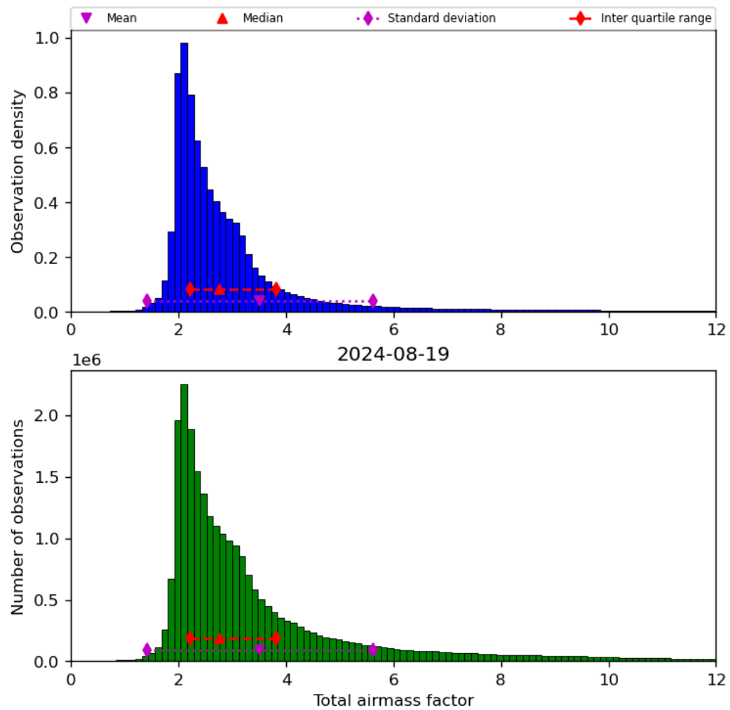
Figure 32: Histogram of “Total airmass factor” for 2024-08-18 to 2024-08-20
