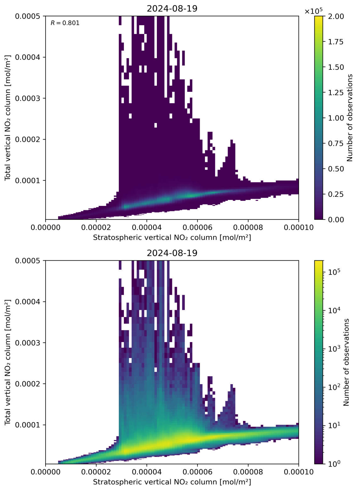
Figure 100: Scatter density plot of “Stratospheric vertical NO 2 column” against “Total vertical NO 2 column” for 2024-08-18 to 2024-08-20.
