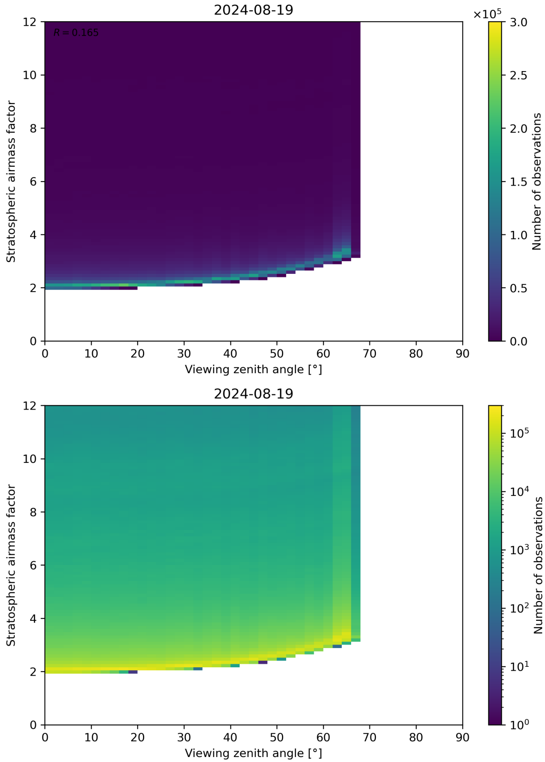
Figure 159: Scatter density plot of “Viewing zenith angle” against “Stratospheric airmass factor” for 2024-08-18 to 2024-08-20.
