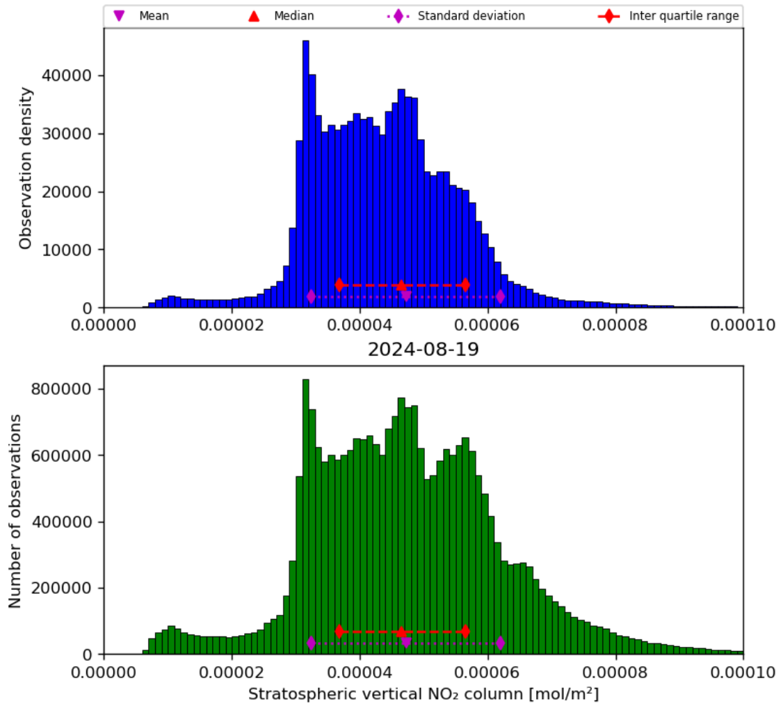
Figure 36: Histogram of “Stratospheric vertical NO 2 column” for 2024-08-18 to 2024-08-20
