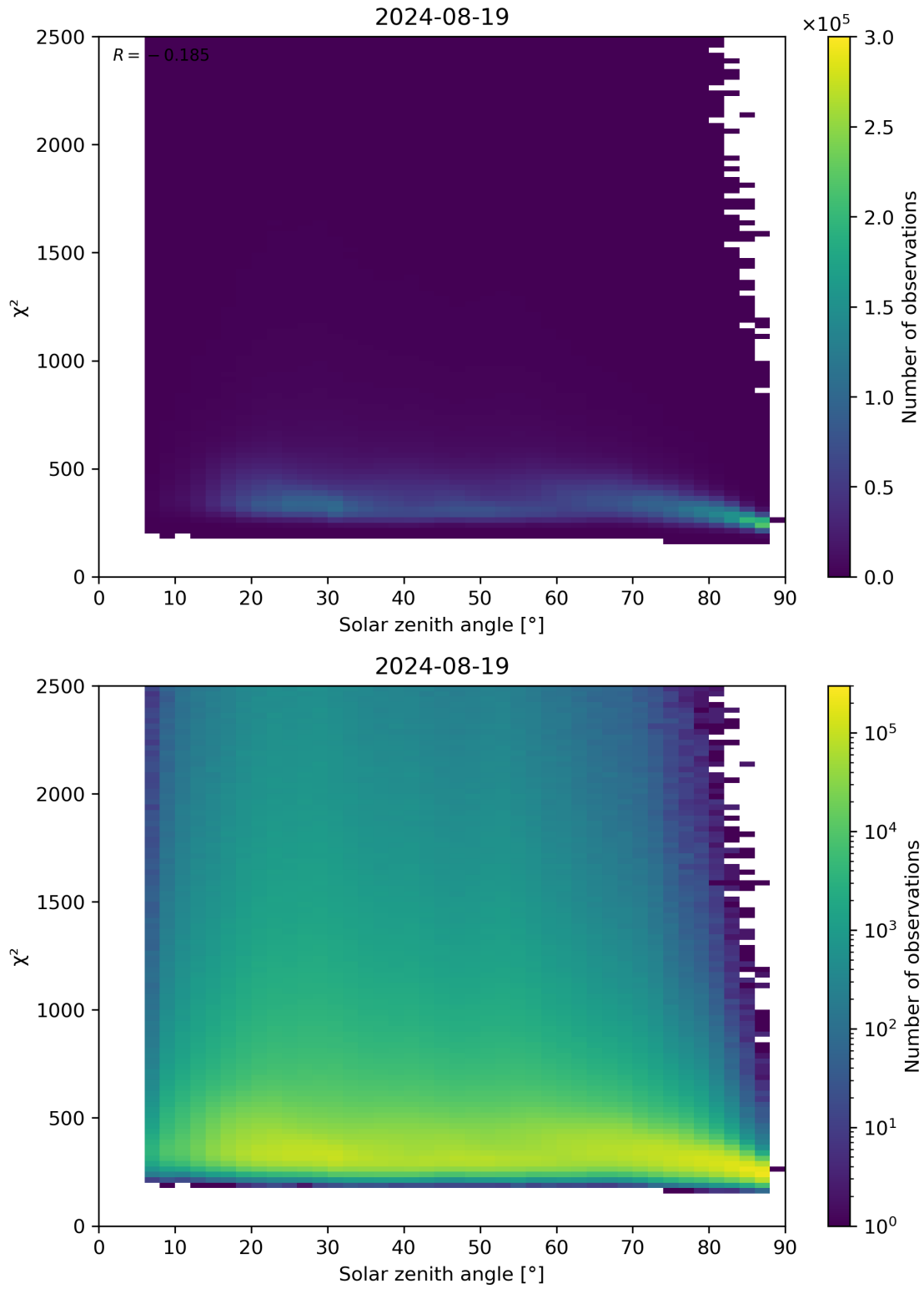
Figure 148: Scatter density plot of “Solar zenith angle” against “ \chi^2 ” for 2024-08-18 to 2024-08-20.
