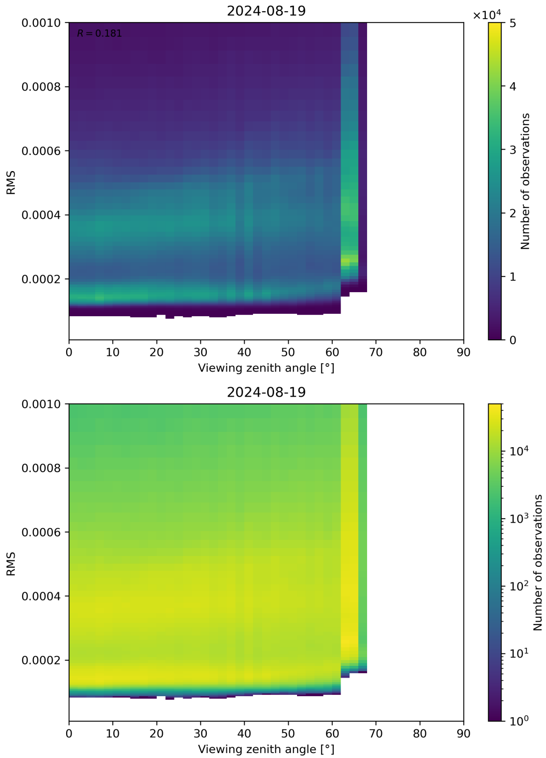
Figure 171: Scatter density plot of “Viewing zenith angle” against “RMS” for 2024-08-18 to 2024-08-20.
