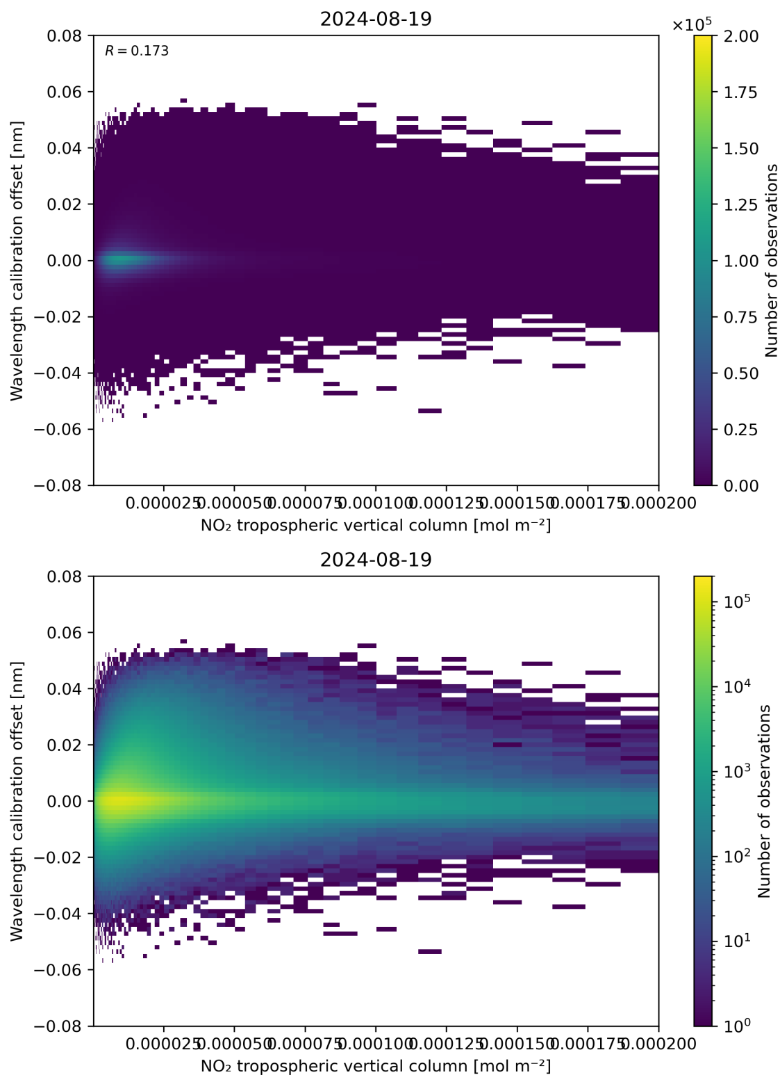
Figure 143: Scatter density plot of “NO 2 tropospheric vertical column” against “Wavelength calibration offset” for 2024-08-18 to 2024-08-20.
