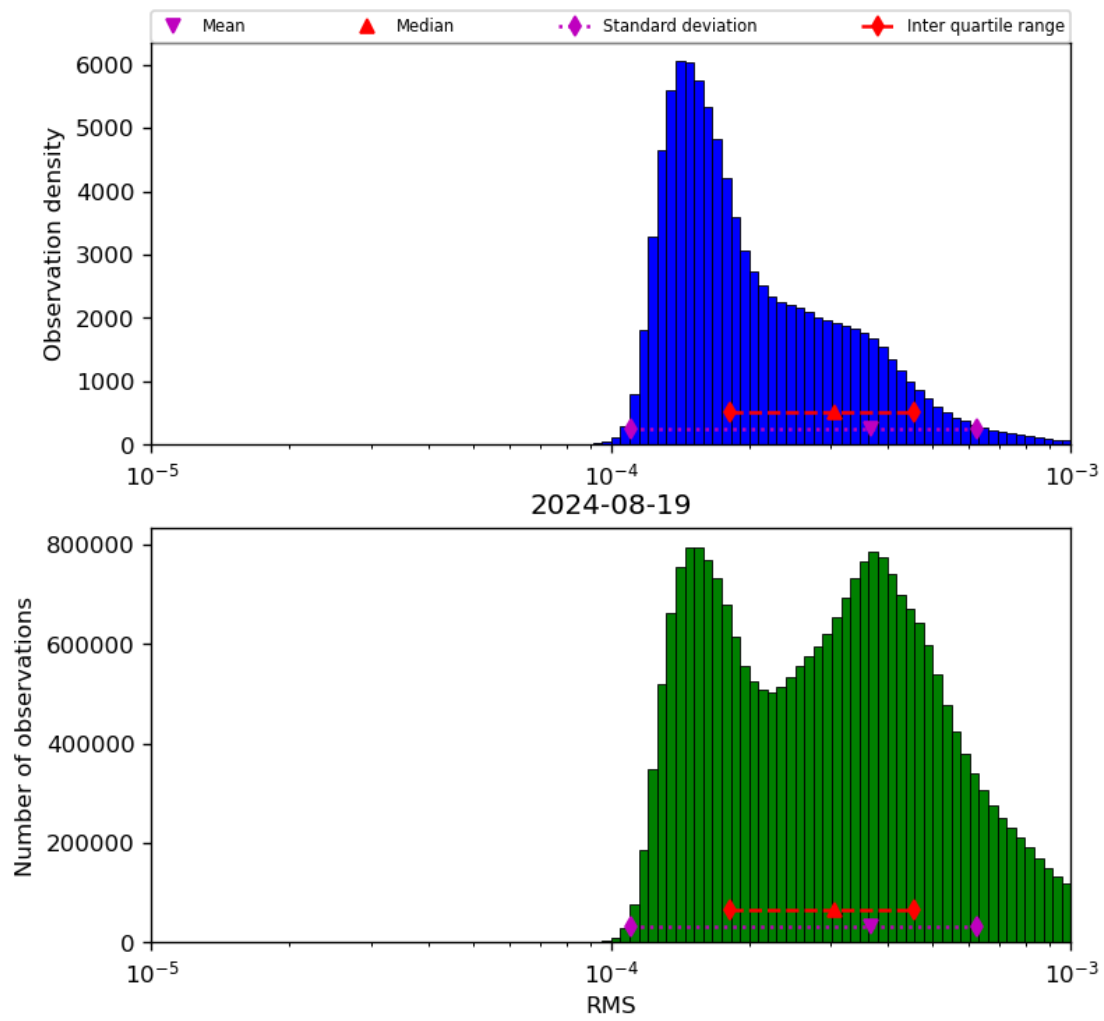
Figure 43: Histogram of “RMS” for 2024-08-18 to 2024-08-20
