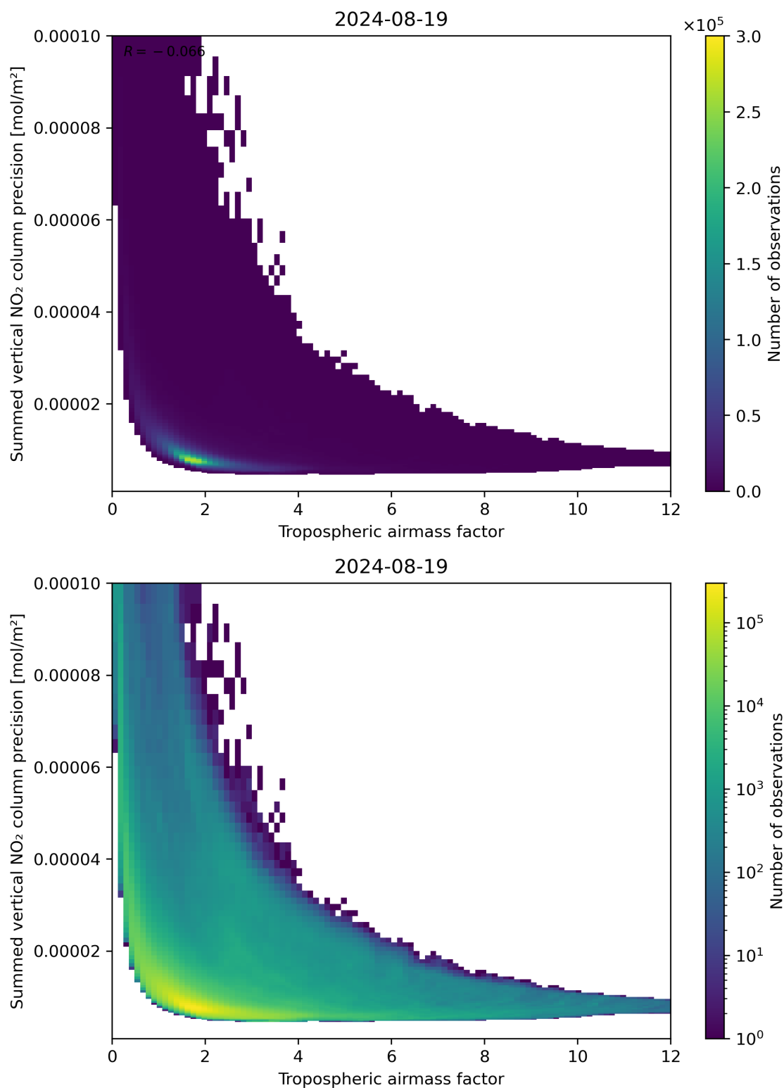
Figure 76: Scatter density plot of “Tropospheric air mass factor” against “Summed vertical NO 2 column precision” for 2024-08-18 to 2024-08-20.
