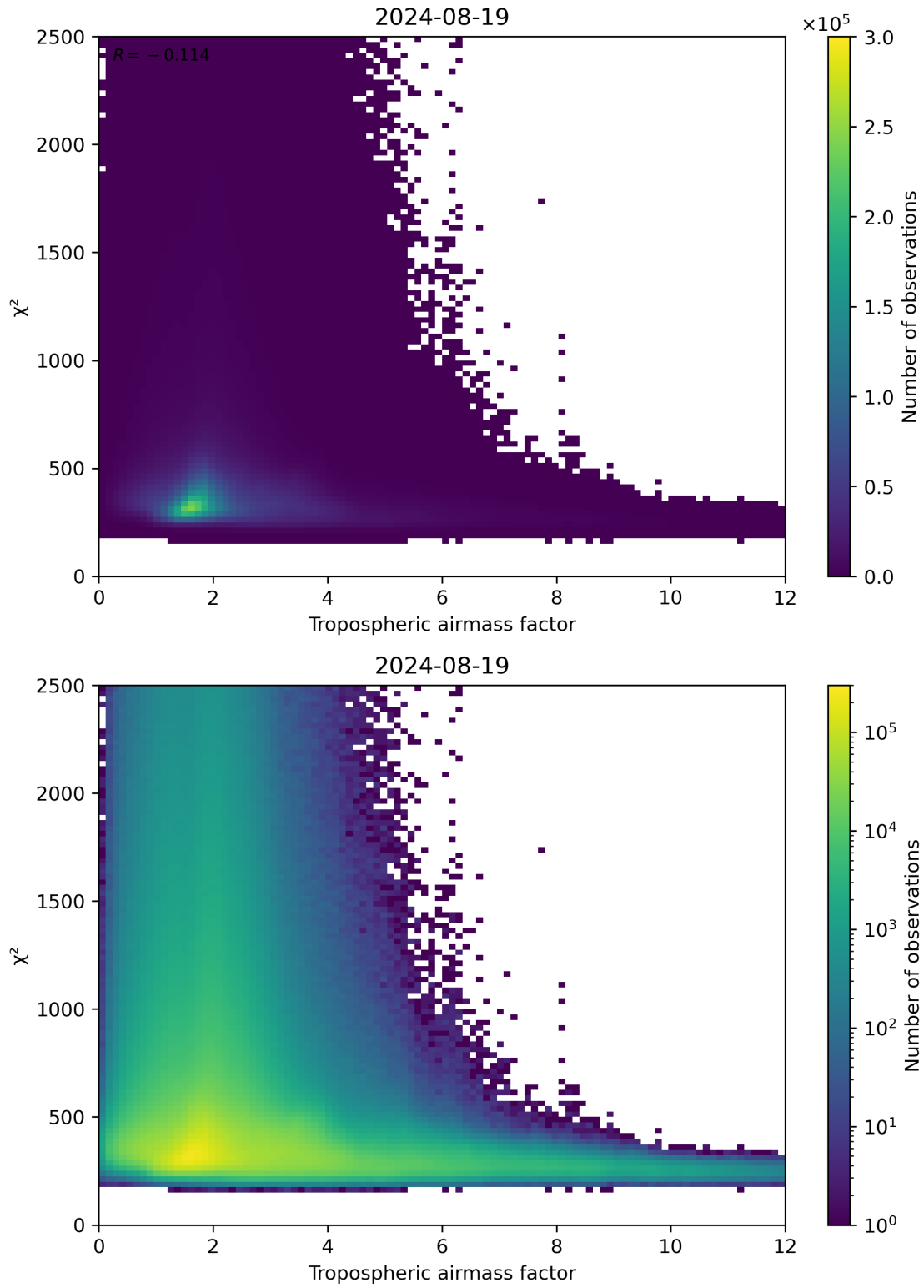
Figure 73: Scatter density plot of “Tropospheric airmass factor” against “ \chi^2 ” for 2024-08-18 to 2024-08-20.
