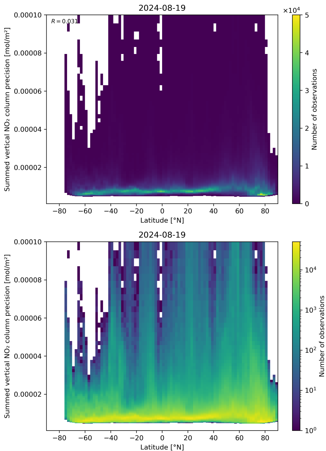
Figure 89: Scatter density plot of “Latitude” against “Summed vertical NO 2 column precision” for 2024-08-18 to 2024-08-20.
