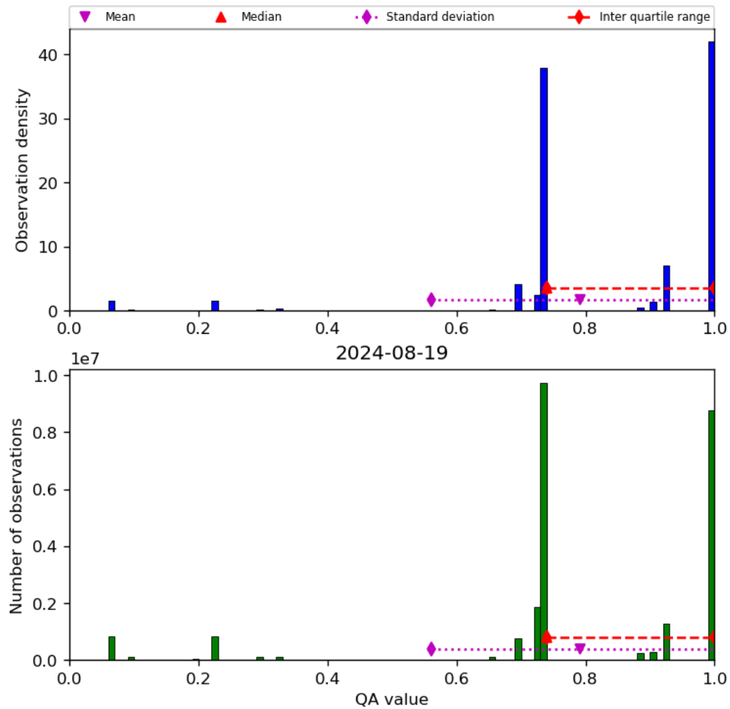
Figure 28: Histogram of “QA value” for 2024-08-18 to 2024-08-20
