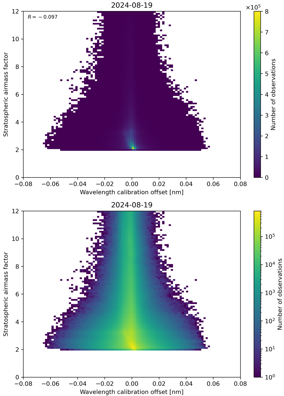
Figure 174: Scatter density plot of “Wavelength calibration offset” against “Stratospheric airmass factor” for 2024-08-18 to 2024-08-20.
