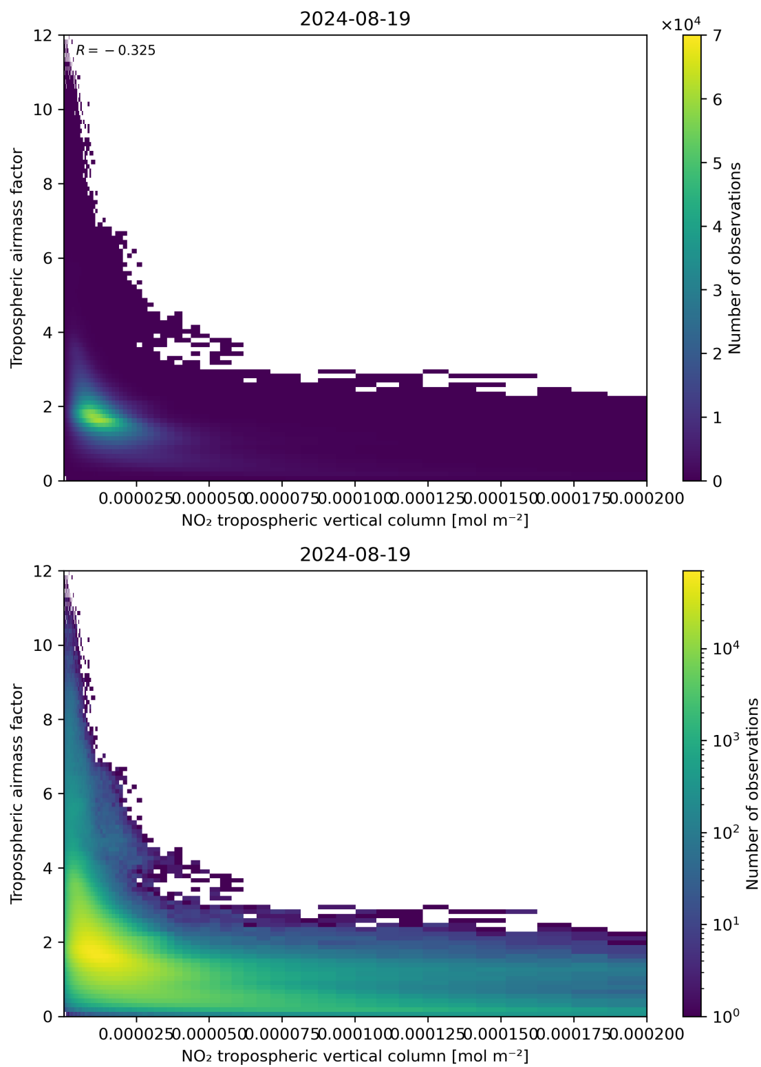
Figure 123: Scatter density plot of “NO 2 tropospheric vertical column” against “Tropospheric air mass factor” for 2024-08-18 to 2024-08-20.
