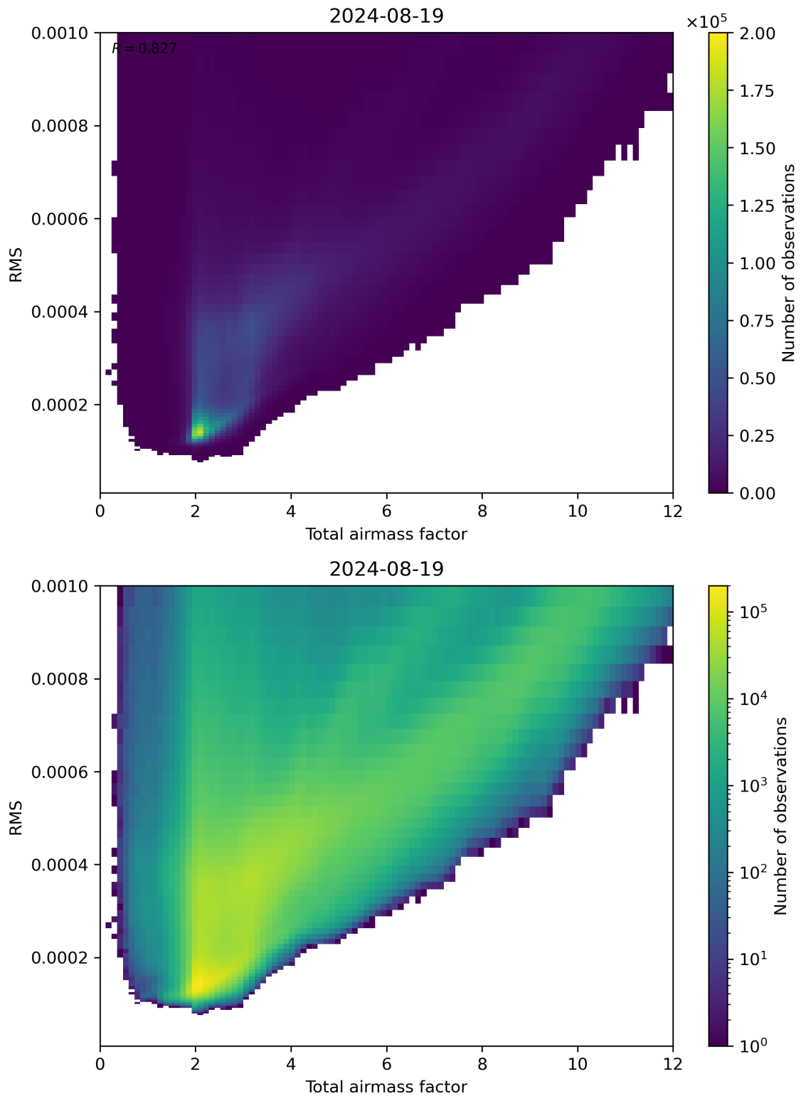
Figure 69: Scatter density plot of “Total airmass factor” against “RMS” for 2024-08-18 to 2024-08-20.
