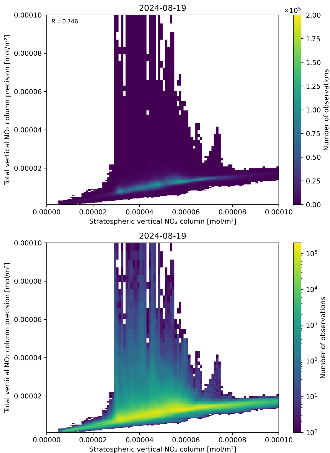
Figure 101: Scatter density plot of “Stratospheric vertical NO 2 column” against “Total vertical NO 2 column precision” for 2024-08-18 to 2024-08-20.
