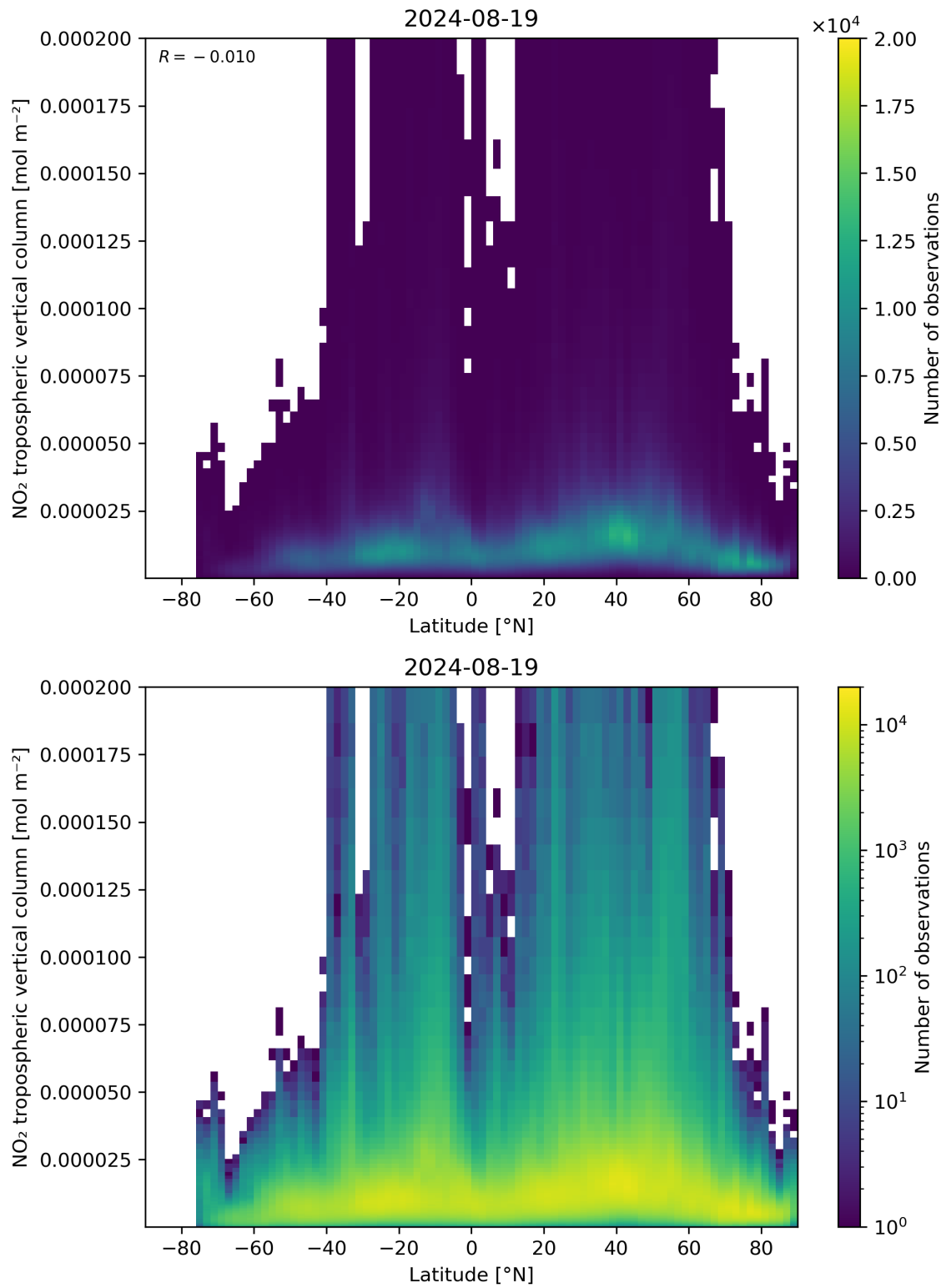
Figure 92: Scatter density plot of “Latitude” against “NO 2 tropospheric vertical column” for 2024-08-18 to 2024-08-20.
