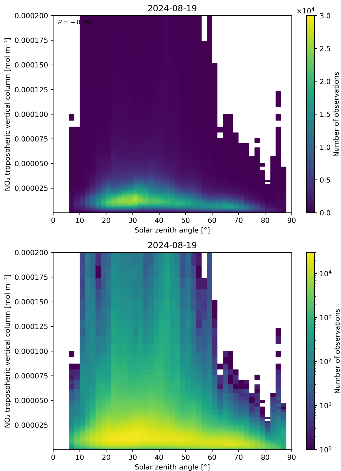
Figure 155: Scatter density plot of “Solar zenith angle” against “NO 2 tropospheric vertical column” for 2024-08-18 to 2024-08-20.
