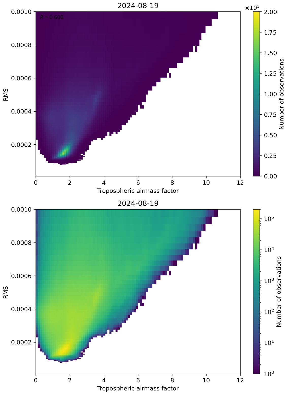
Figure 79: Scatter density plot of “Tropospheric airmass factor” against “RMS” for 2024-08-18 to 2024-08-20.
