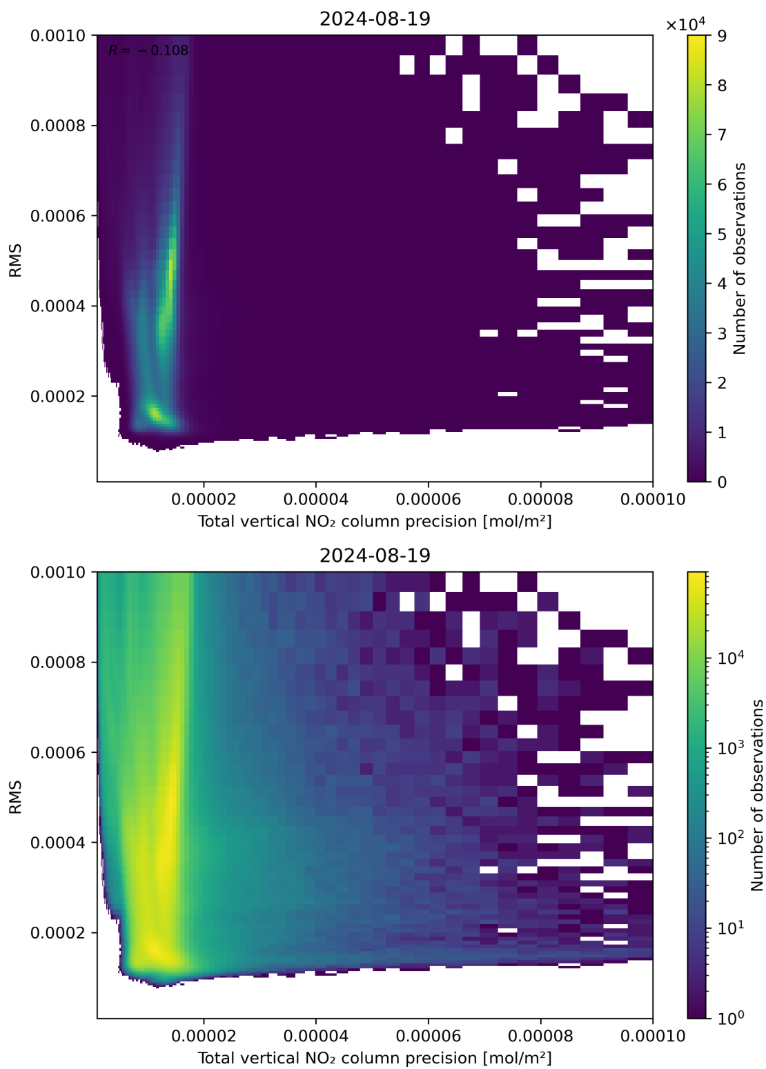
Figure 119: Scatter density plot of “Total vertical NO 2 column precision” against “RMS” for 2024-08-18 to 2024-08-20.
