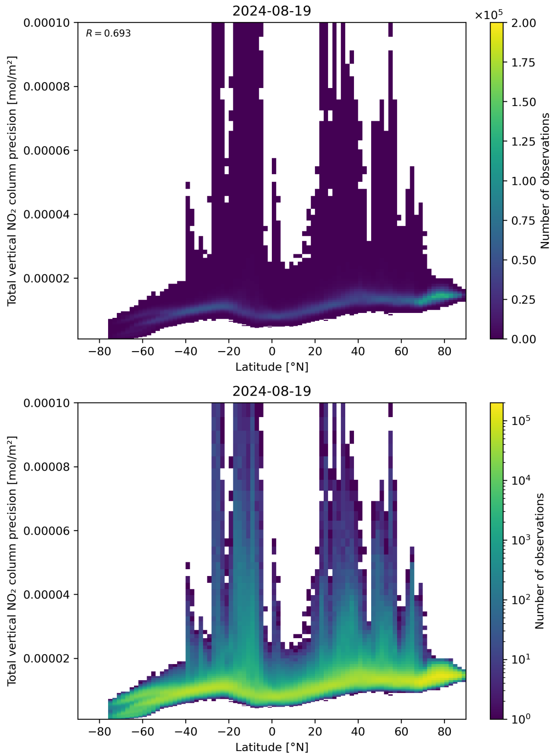
Figure 91: Scatter density plot of “Latitude” against “Total vertical NO 2 column precision” for 2024-08-18 to 2024-08-20.
