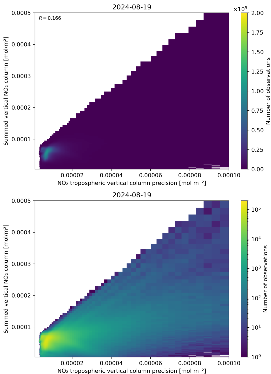
Figure 136: Scatter density plot of “NO 2 tropospheric vertical column precision” against “Summed vertical NO 2 column” for 2024-08-18 to 2024-08-20.
