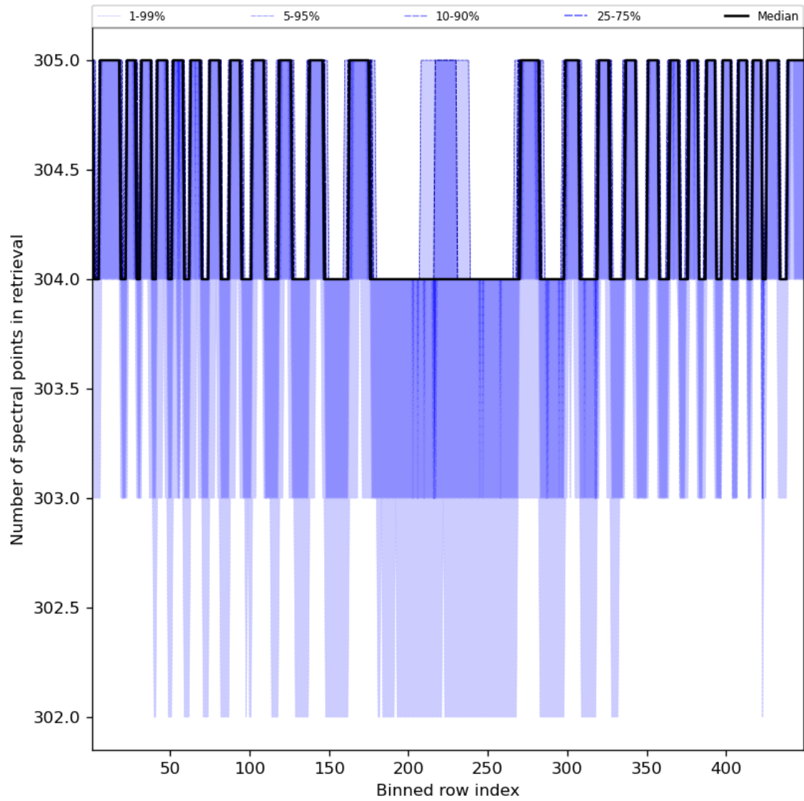
Figure 50: Along track statistics of “Number of spectral points in retrieval” for 2024-08-18 to 2024-08-20
