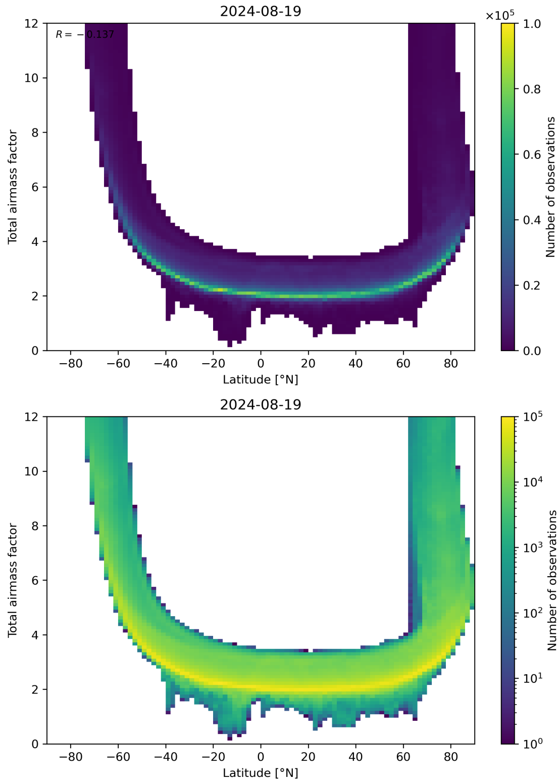
Figure 84: Scatter density plot of “Latitude” against “Total airmass factor” for 2024-08-18 to 2024-08-20.
