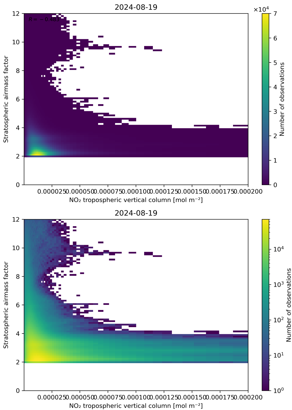
Figure 121: Scatter density plot of “NO 2 tropospheric vertical column” against “Stratospheric air mass factor” for 2024-08-18 to 2024-08-20.
