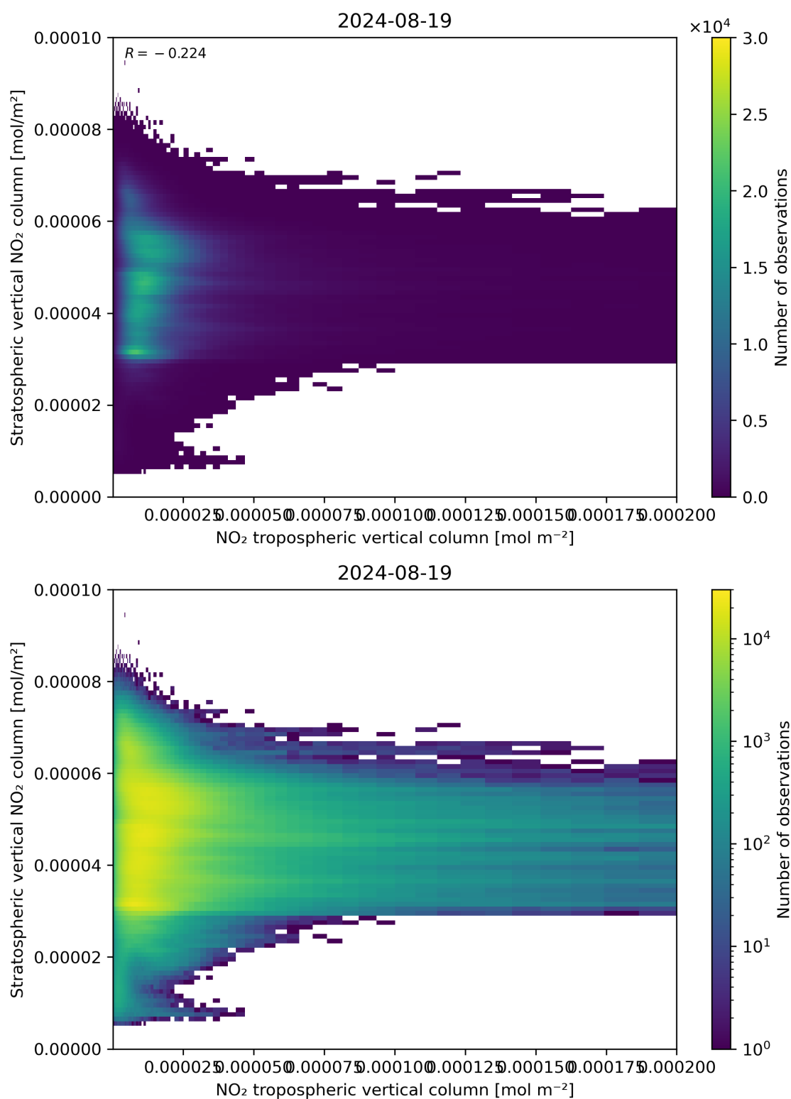
Figure 125: Scatter density plot of “NO 2 tropospheric vertical column” against “Stratospheric vertical NO 2 column” for 2024-08-18 to 2024-08-20.
