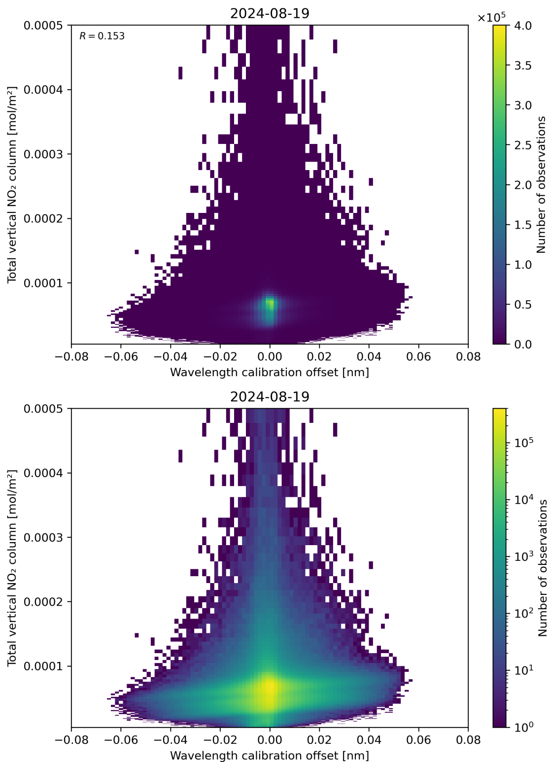
Figure 179: Scatter density plot of “Wavelength calibration offset” against “Total vertical NO 2 column” for 2024-08-18 to 2024-08-20.
