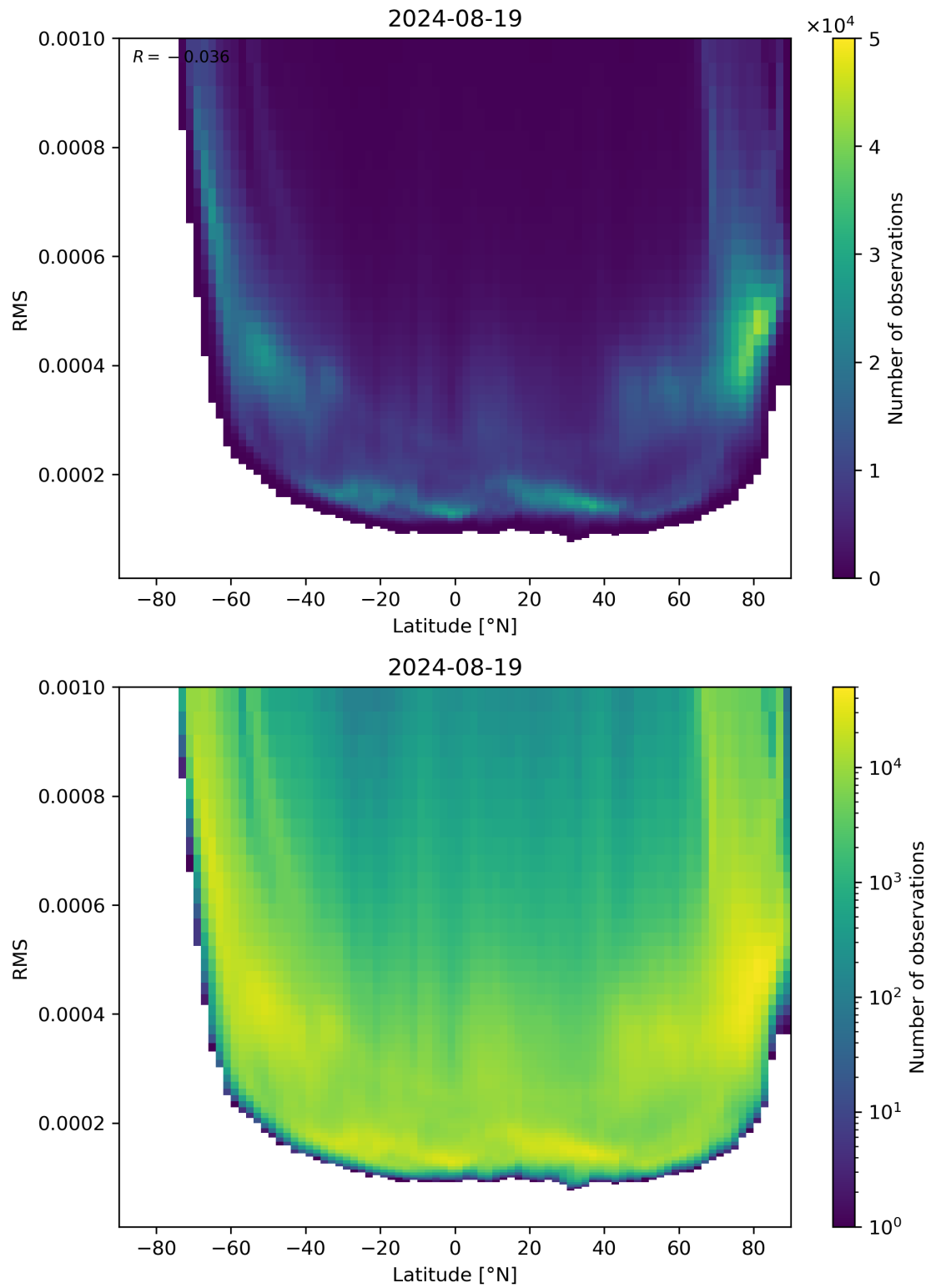
Figure 94: Scatter density plot of “Latitude” against “RMS” for 2024-08-18 to 2024-08-20.
