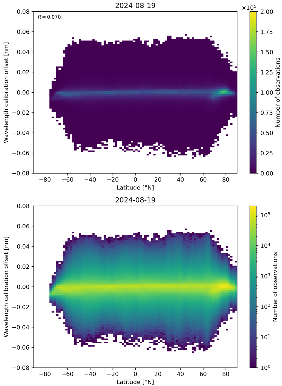
Figure 95: Scatter density plot of “Latitude” against “Wavelength calibration offset” for 2024-08-18 to 2024-08-20.
