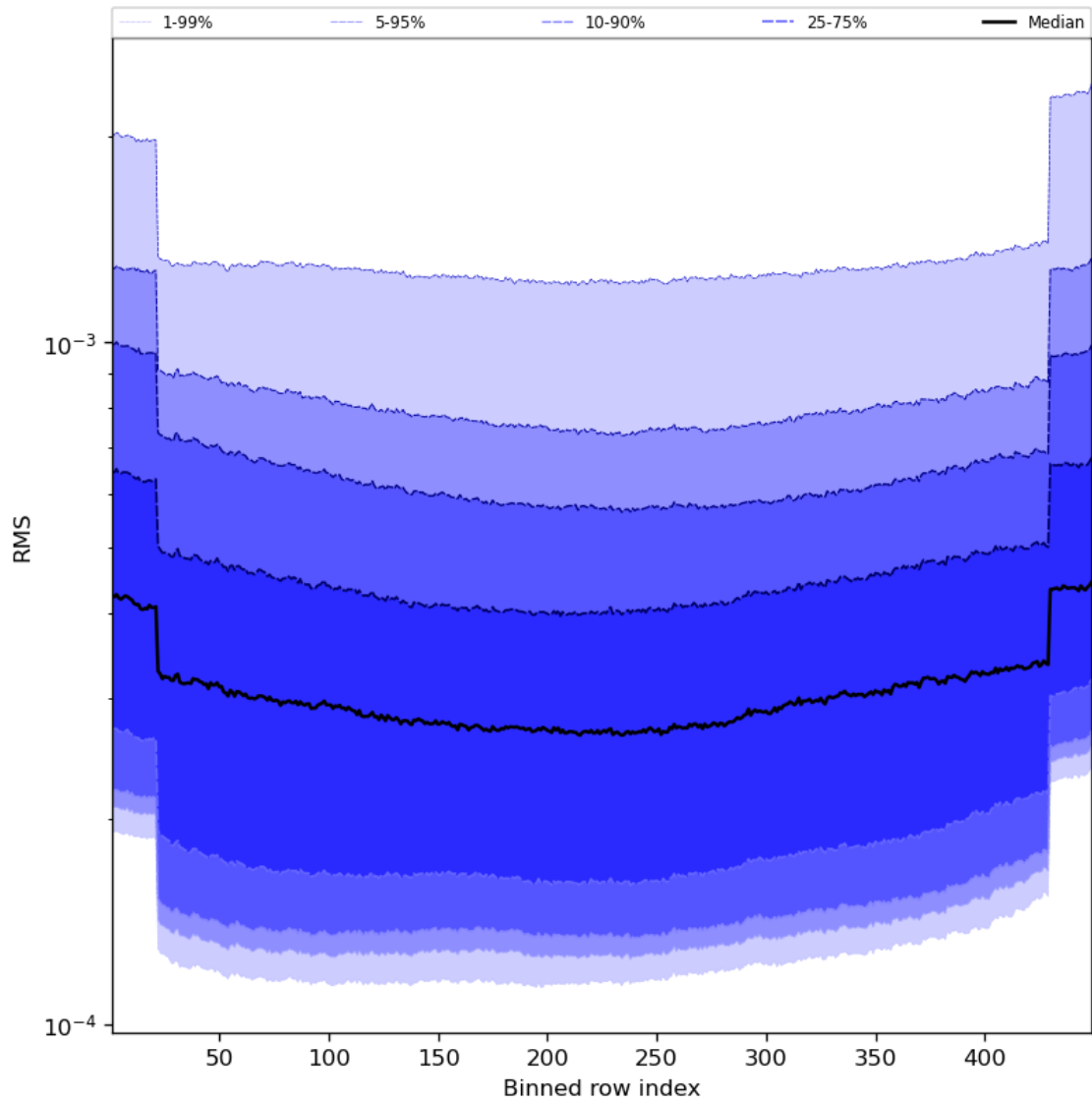
Figure 60: Along track statistics of “RMS” for 2024-08-18 to 2024-08-20
