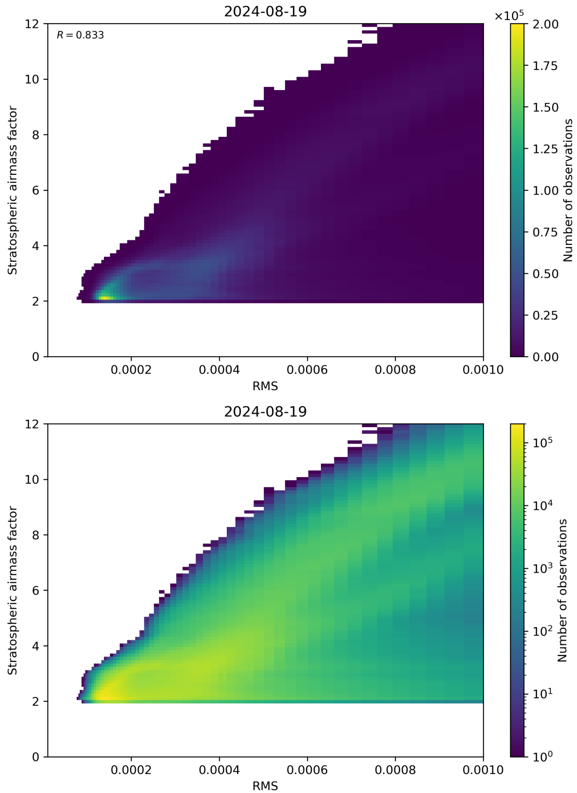
Figure 144: Scatter density plot of “RMS” against “Stratospheric airmass factor” for 2024-08-18 to 2024-08-20.
