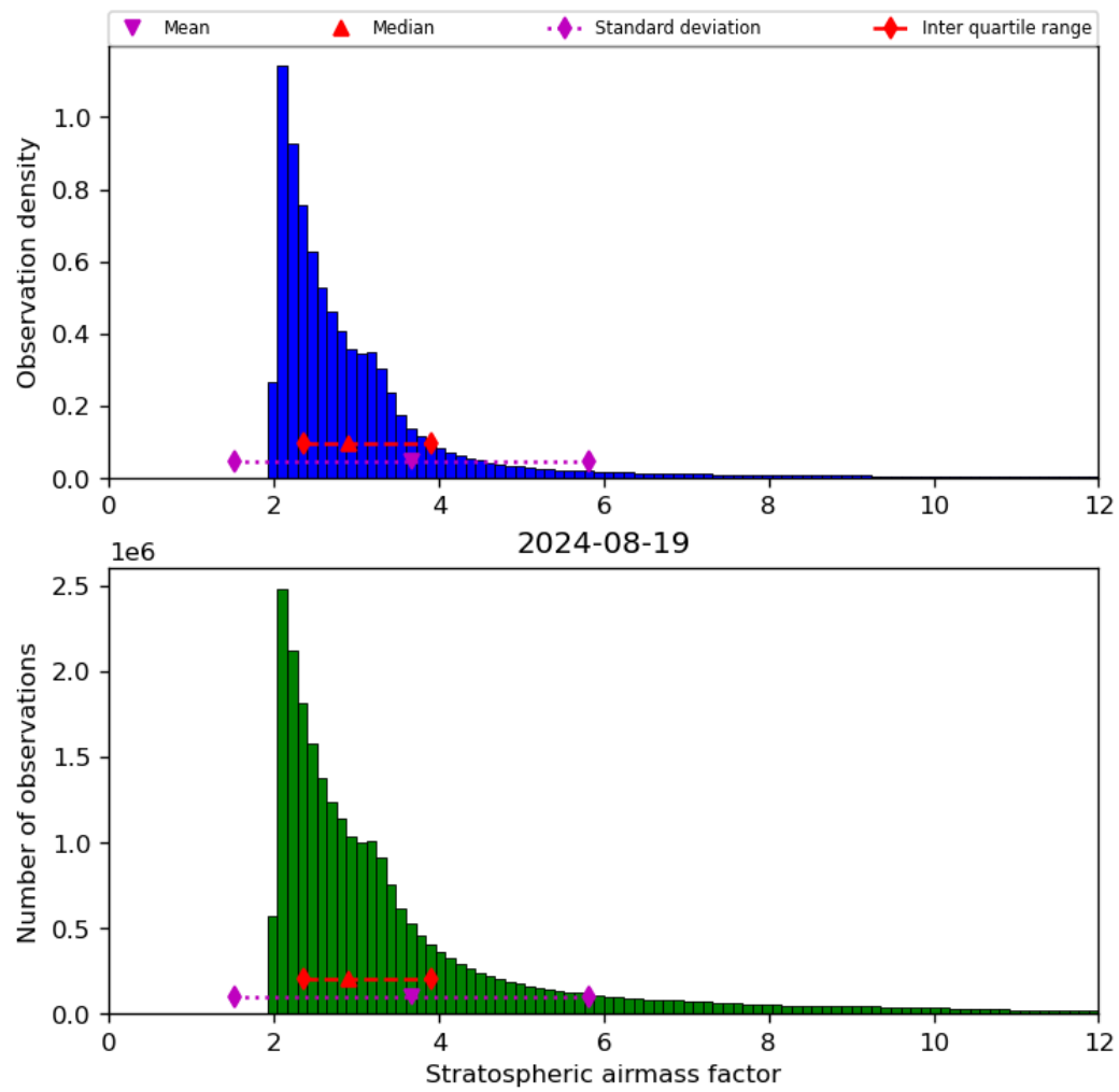
Figure 44: Histogram of “Stratospheric airmass factor” for 2024-08-18 to 2024-08-20
