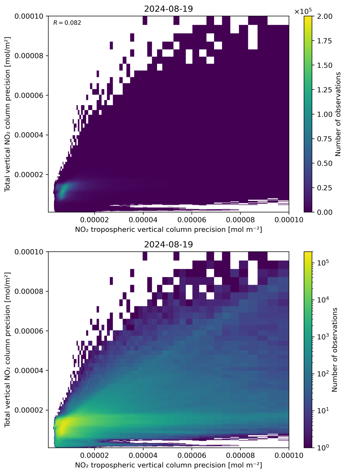
Figure 139: Scatter density plot of “NO 2 tropospheric vertical column precision” against “Total vertical NO 2 column precision” for 2024-08-18 to 2024-08-20.
