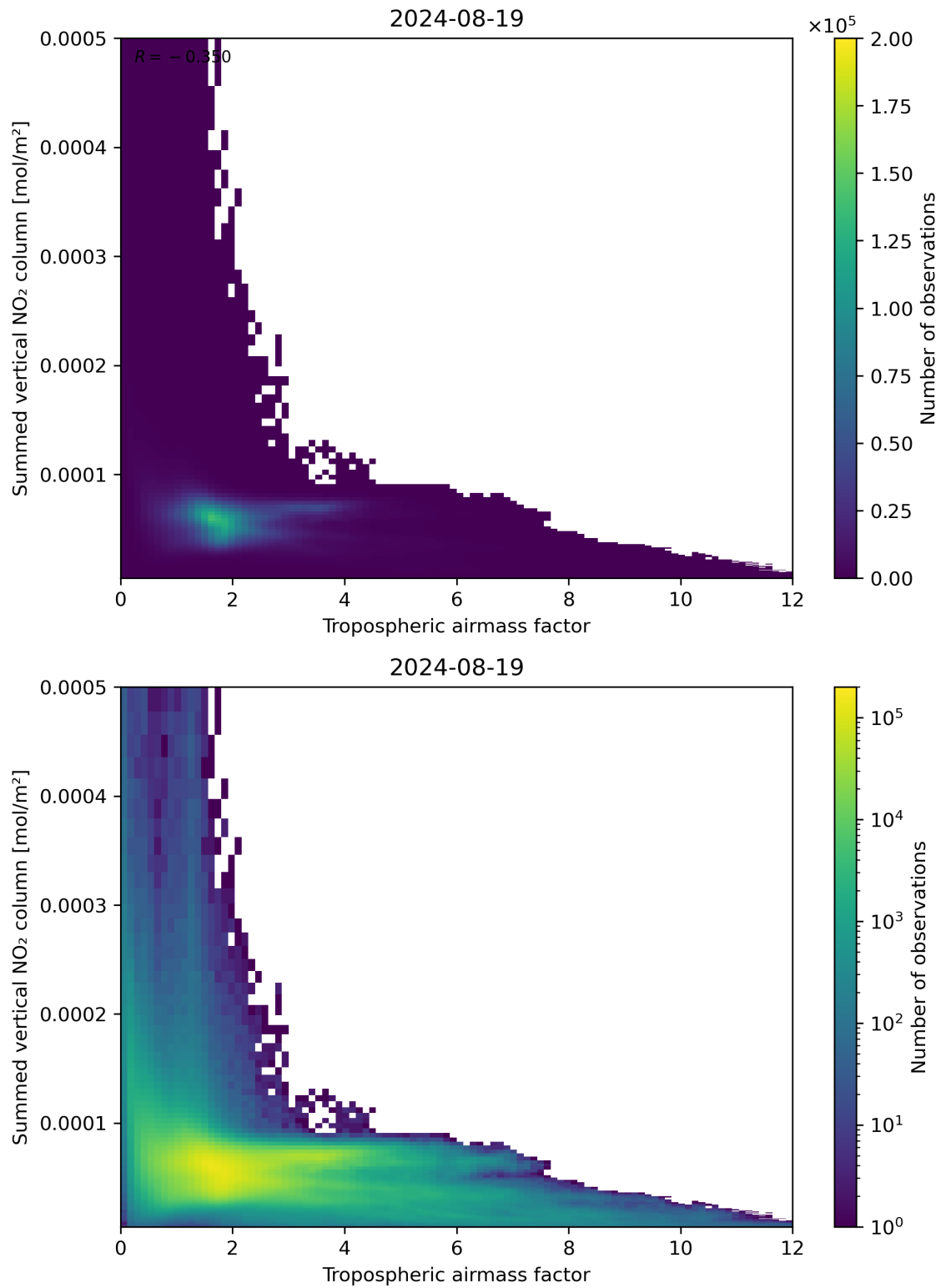
Figure 75: Scatter density plot of “Tropospheric air mass factor” against “Summed vertical NO 2 column” for 2024-08-18 to 2024-08-20.
