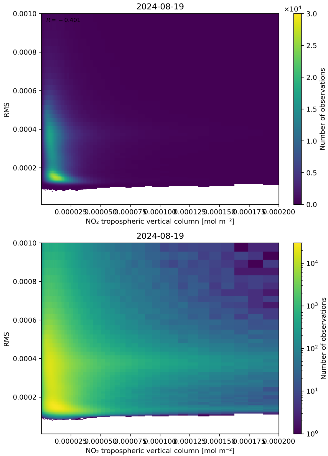
Figure 142: Scatter density plot of “NO 2 tropospheric vertical column” against “RMS” for 2024-08-18 to 2024-08-20.
