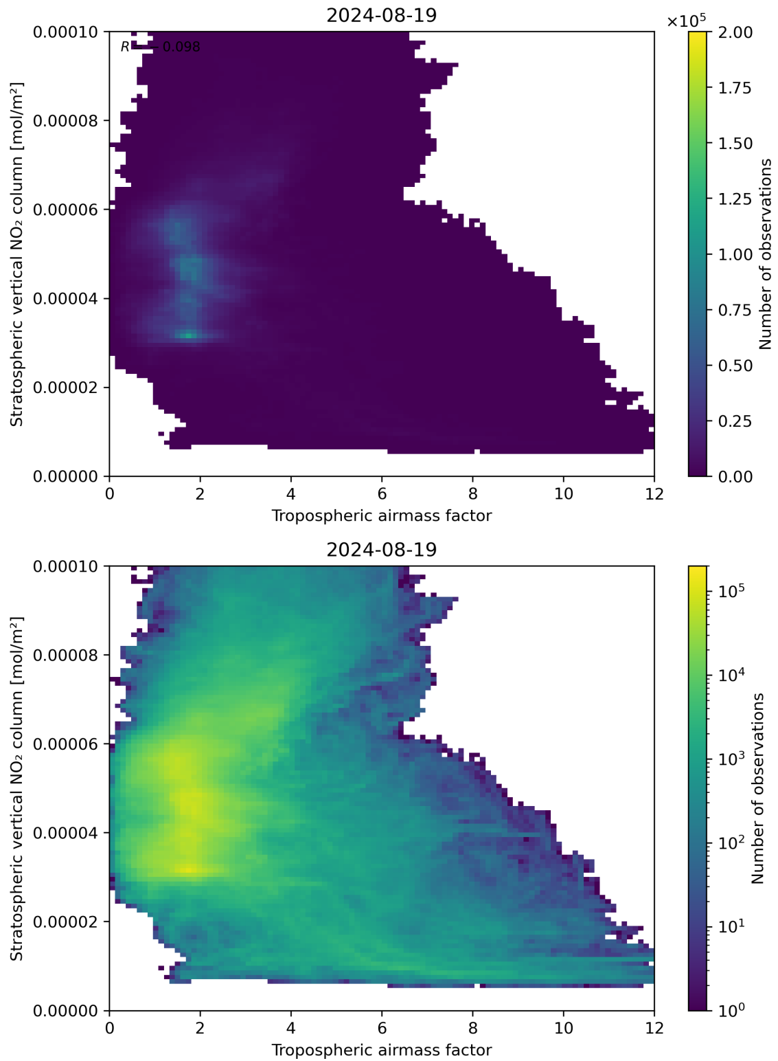
Figure 74: Scatter density plot of “Tropospheric air mass factor” against “Stratospheric vertical NO 2 column” for 2024-08-18 to 2024-08-20.
