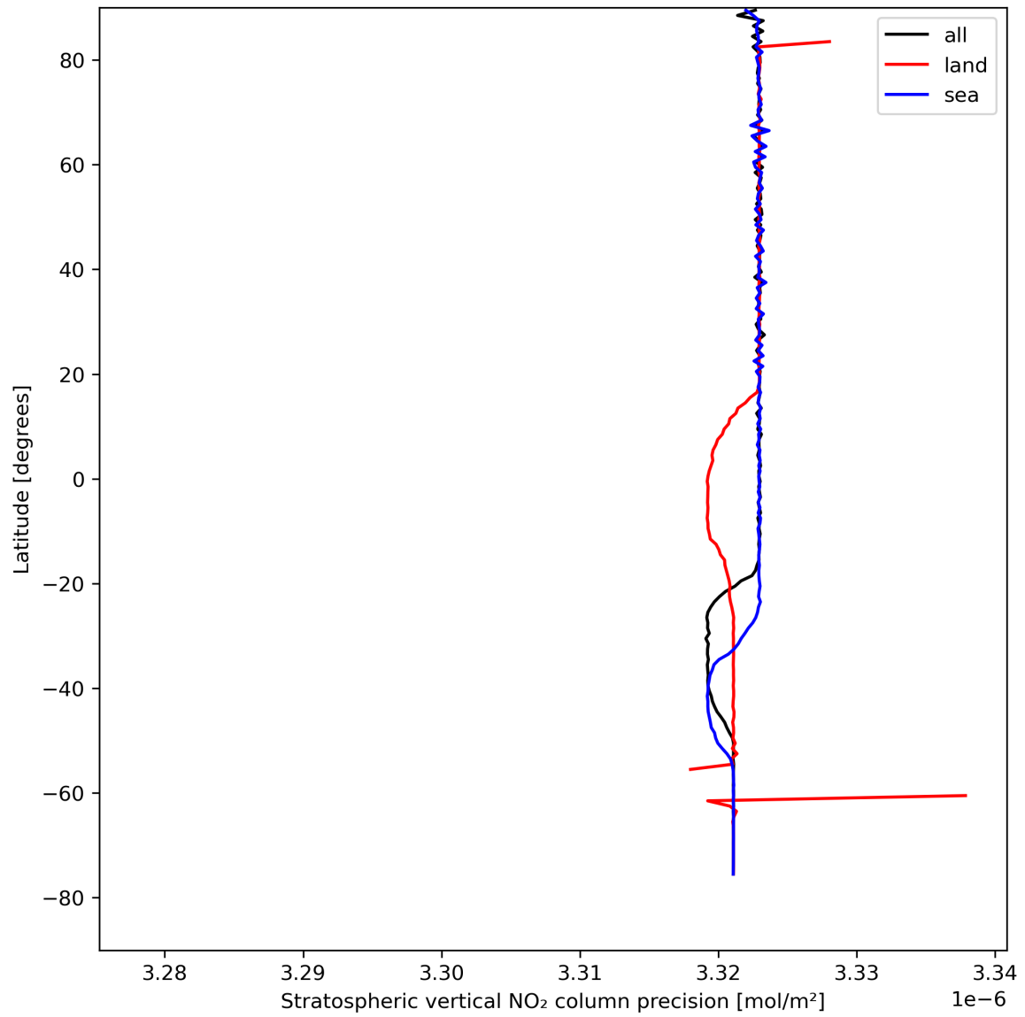
Figure 20: Zonal average of "Stratospheric vertical NO 2 column precision" for 2024-08-18 to 2024-08-20.
