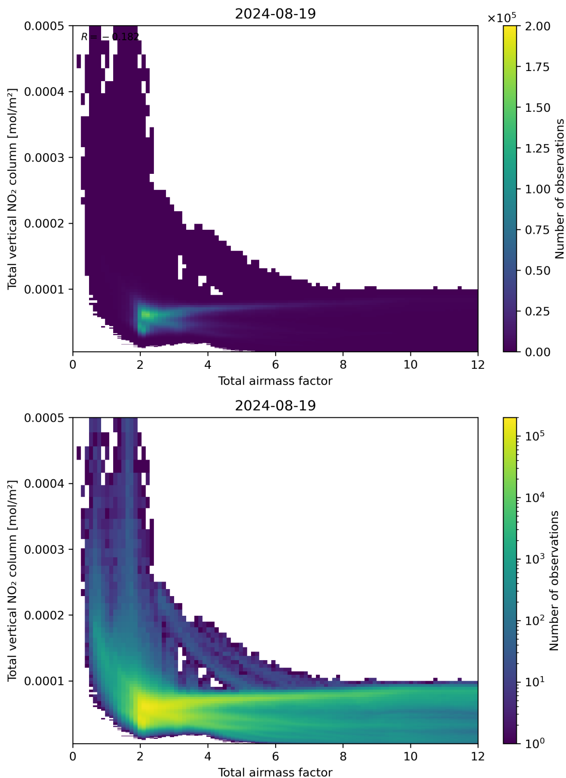
Figure 67: Scatter density plot of “Total airmass factor” against “Total vertical NO 2 column” for 2024-08-18 to 2024-08-20.
