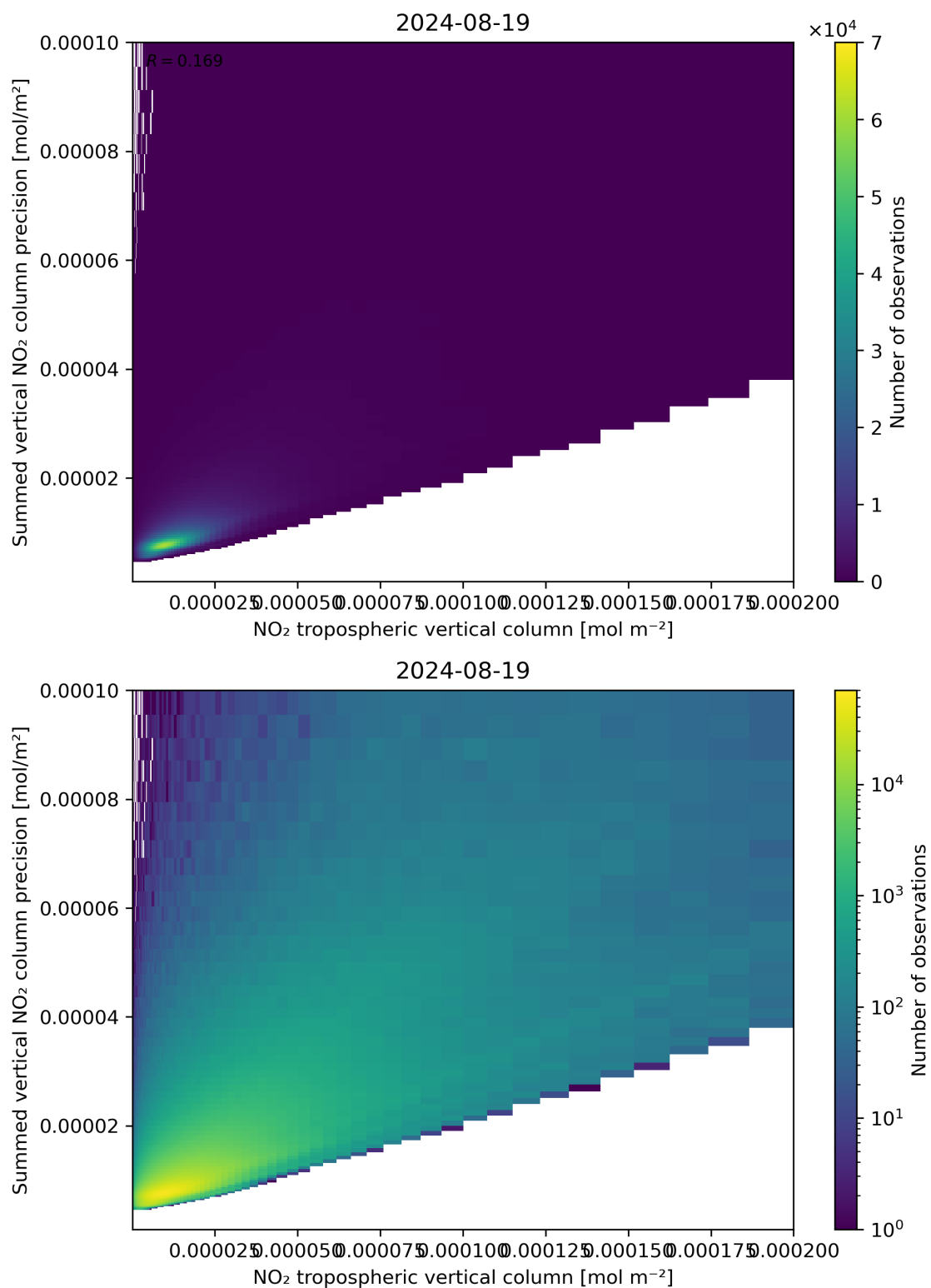
Figure 127: Scatter density plot of “NO 2 tropospheric vertical column” against “Summed vertical NO 2 column precision” for 2024-08-18 to 2024-08-20.
