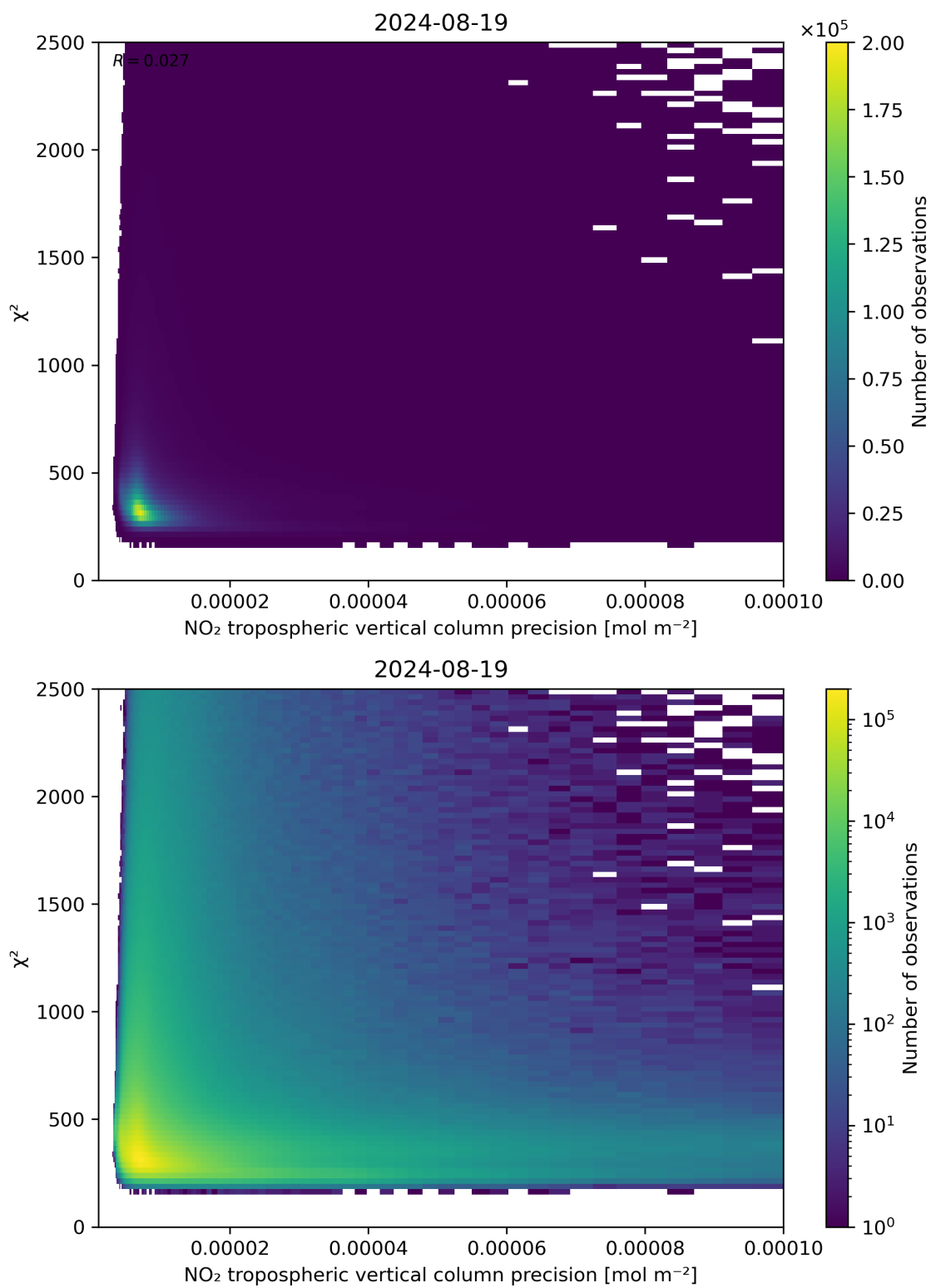
Figure 134: Scatter density plot of “NO 2 tropospheric vertical column precision” against “ \chi^2 ” for 2024-08-18 to 2024-08-20.
