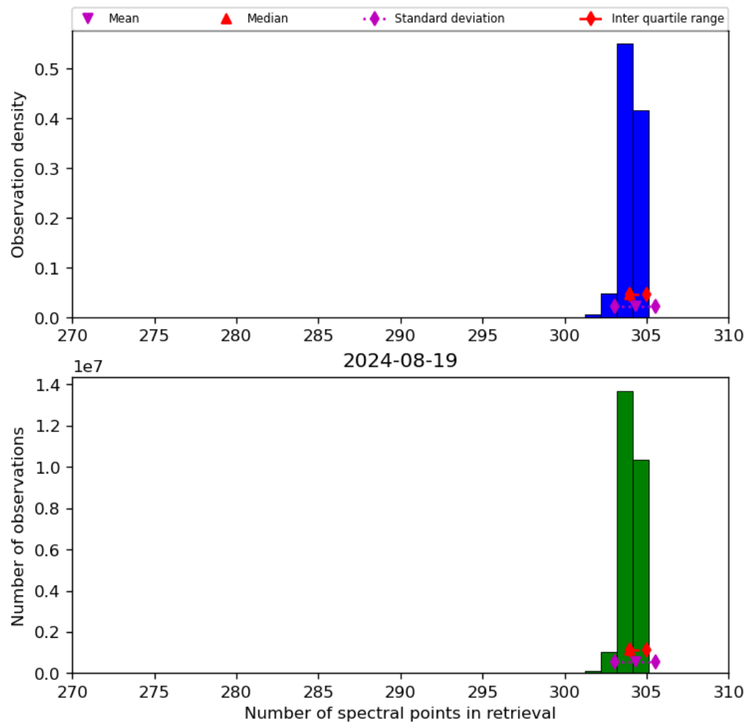
Figure 33: Histogram of “Number of spectral points in retrieval” for 2024-08-18 to 2024-08-20
