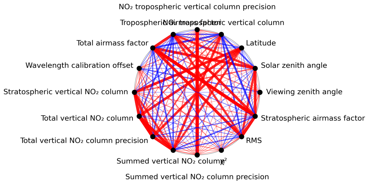
Figure 1: Map of correlation graph for 2024-08-18 to 2024-08-20.
