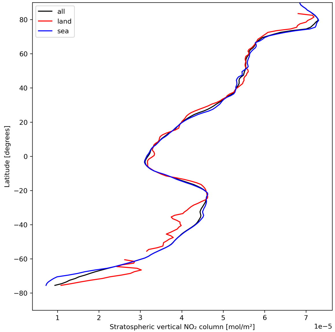
Figure 19: Zonal average of “Stratospheric vertical NO 2 column” for 2024-08-18 to 2024-08-20.
