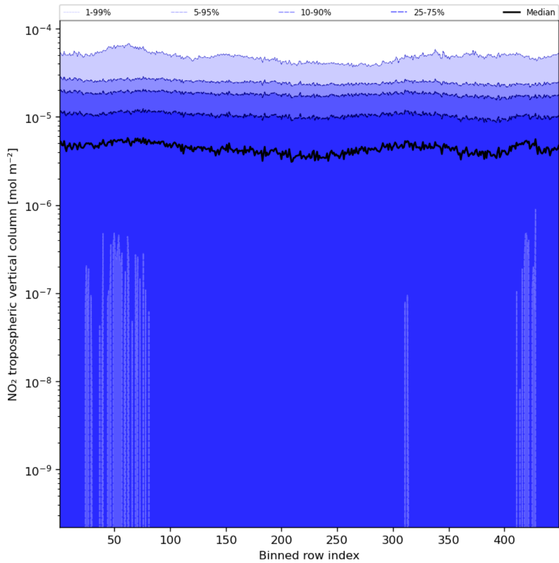
Figure 46: Along track statistics of “NO 2 tropospheric vertical column” for 2024-08-18 to 2024-08-20
