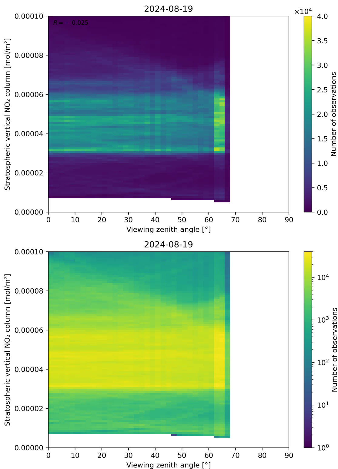
Figure 164: Scatter density plot of “Viewing zenith angle” against “Stratospheric vertical NO 2 column” for 2024-08-18 to 2024-08-20.
