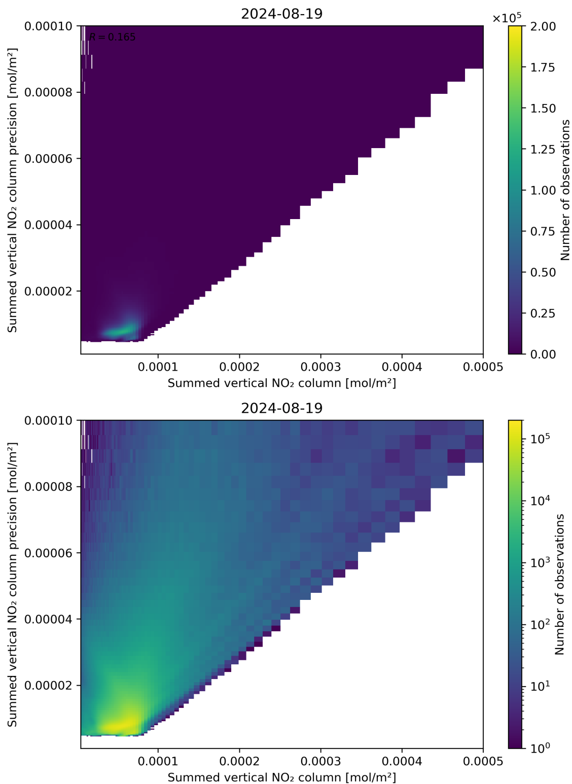
Figure 105: Scatter density plot of “Summed vertical NO 2 column” against “Summed vertical NO 2 column precision” for 2024-08-18 to 2024-08-20.
