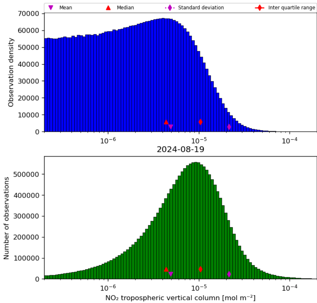
Figure 29: Histogram of “NO 2 tropospheric vertical column” for 2024-08-18 to 2024-08-20
