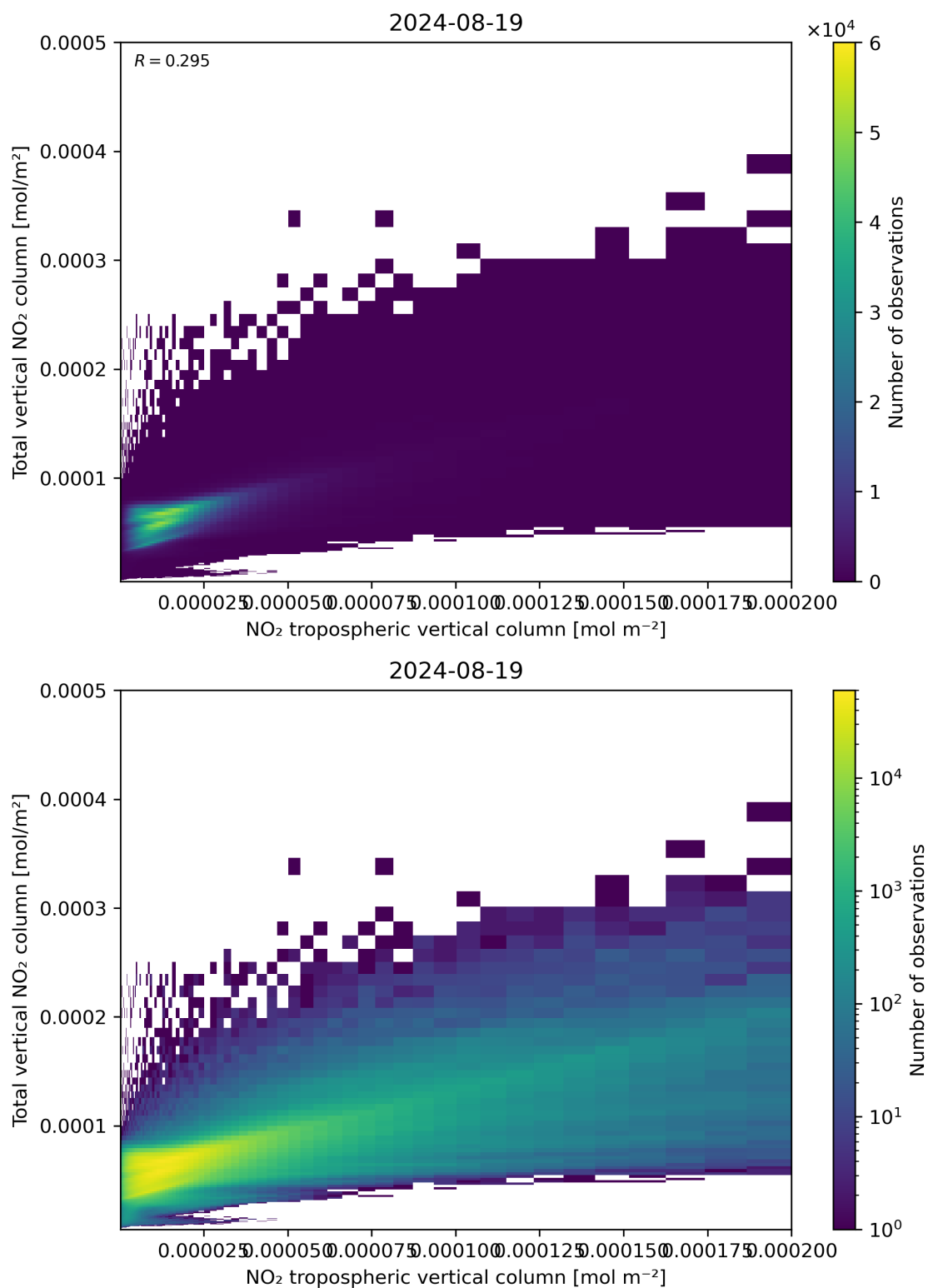
Figure 128: Scatter density plot of “NO 2 tropospheric vertical column” against “Total vertical NO 2 column” for 2024-08-18 to 2024-08-20.
