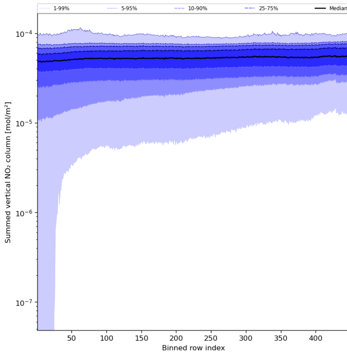
Figure 57: Along track statistics of “Summed vertical NO 2 column” for 2024-08-18 to 2024-08-20
