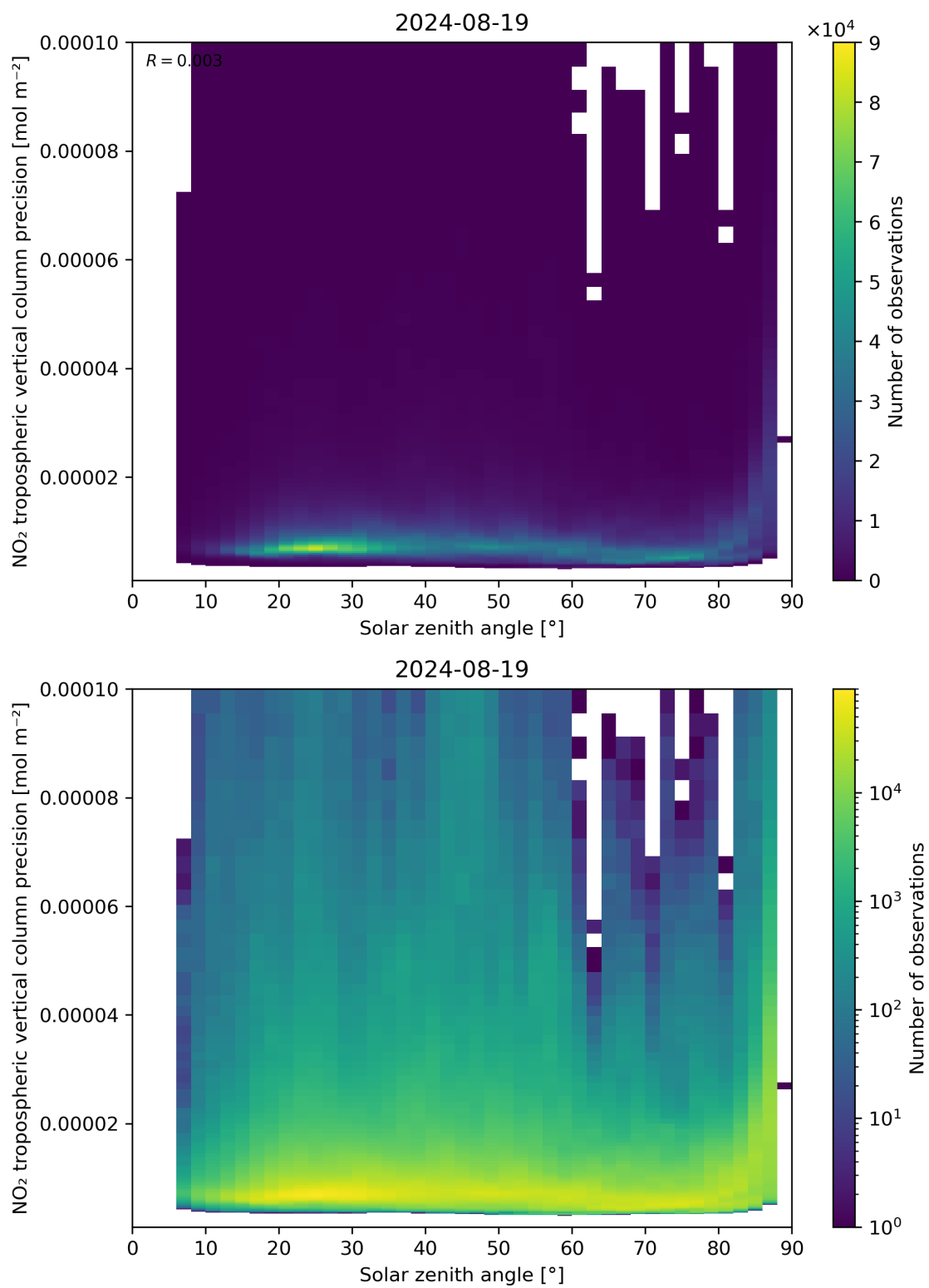
Figure 156: Scatter density plot of “Solar zenith angle” against “NO 2 tropospheric vertical column precision” for 2024-08-18 to 2024-08-20.
