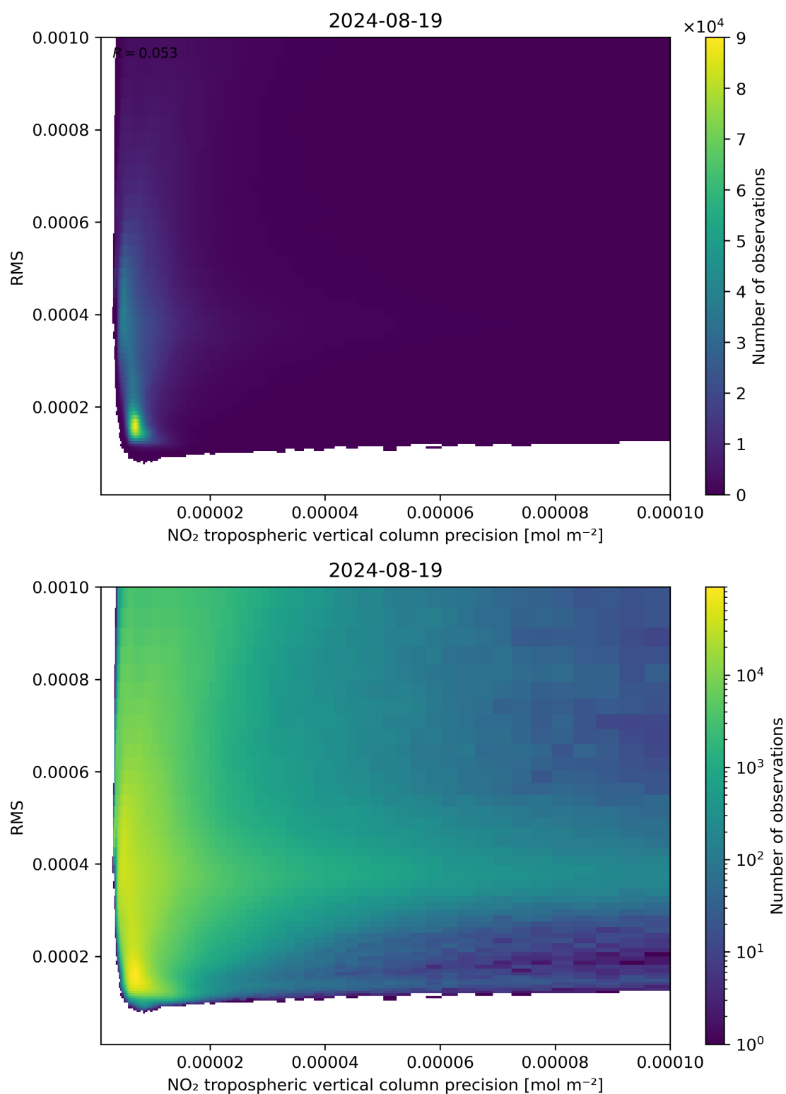
Figure 140: Scatter density plot of “NO 2 tropospheric vertical column precision” against “RMS” for 2024-08-18 to 2024-08-20.
