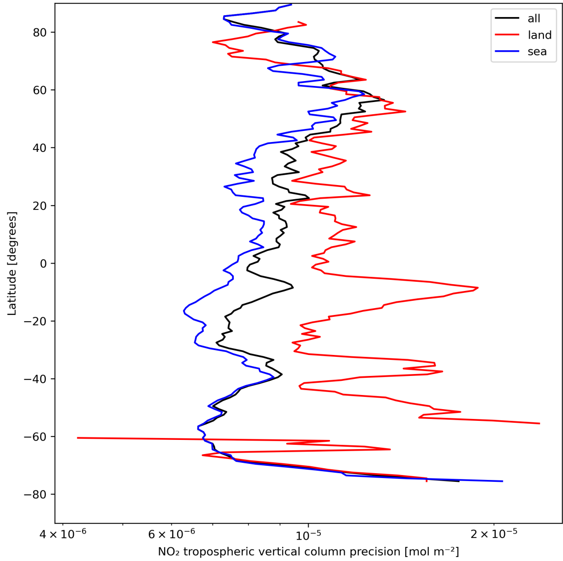
Figure 13: Zonal average of “NO 2 tropospheric vertical column precision” for 2024-08-18 to 2024-08-20.
