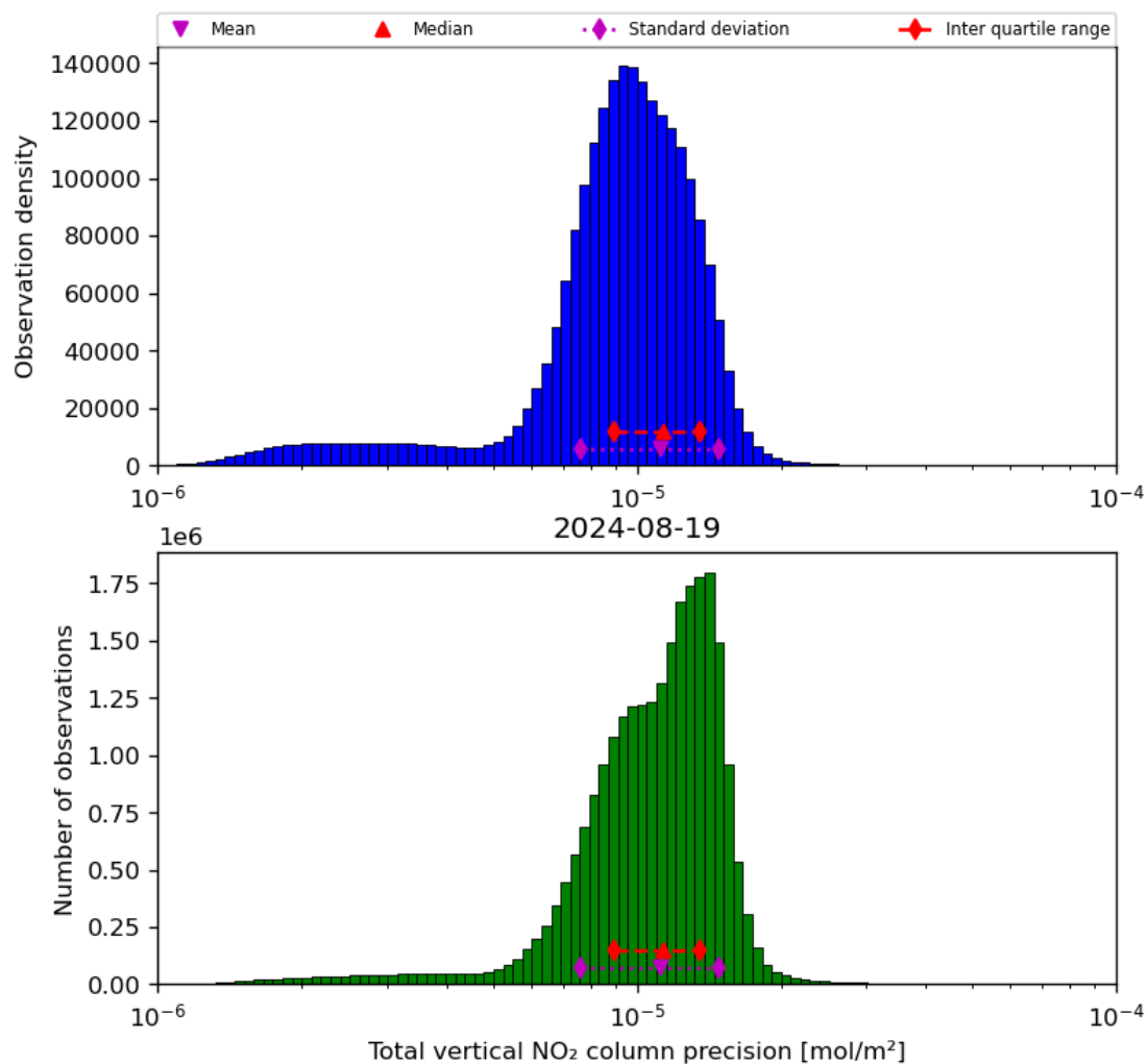
Figure 39: Histogram of “Total vertical NO 2 column precision” for 2024-08-18 to 2024-08-20
