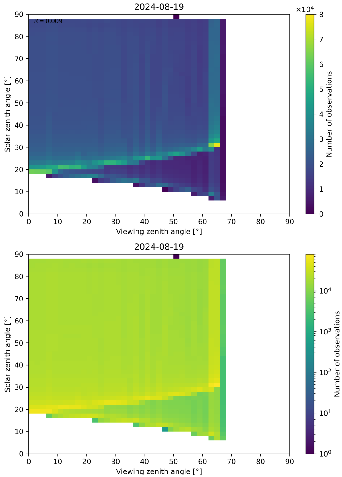
Figure 172: Scatter density plot of “Viewing zenith angle” against “Solar zenith angle” for 2024-08-18 to 2024-08-20.
