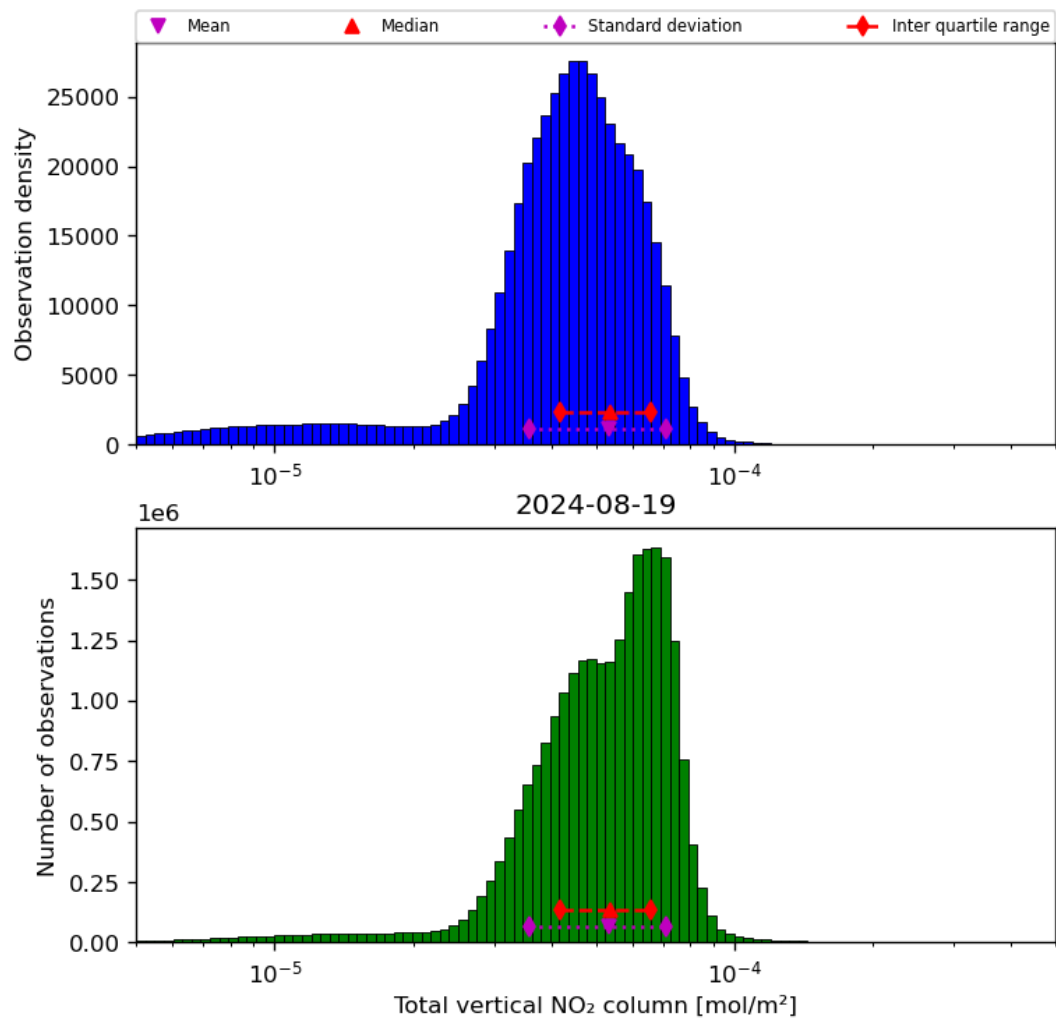
Figure 38: Histogram of “Total vertical NO 2 column” for 2024-08-18 to 2024-08-20
