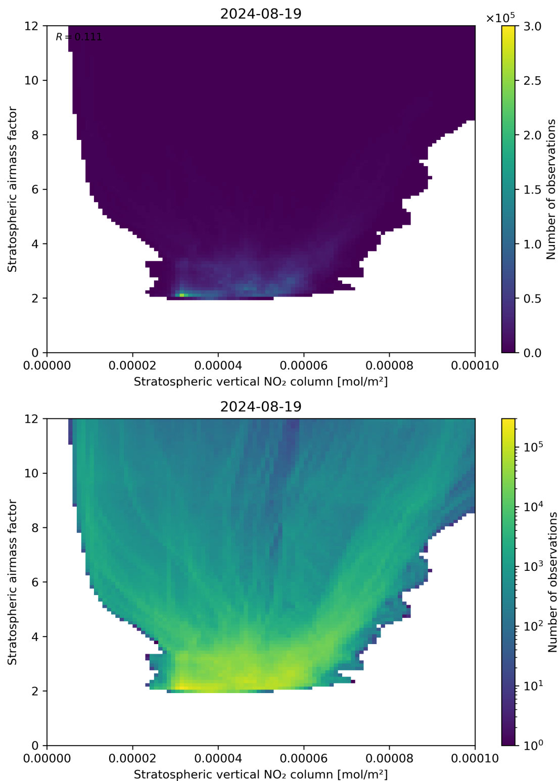
Figure 96: Scatter density plot of “Stratospheric vertical NO 2 column” against “Stratospheric airmass factor” for 2024-08-18 to 2024-08-20.
