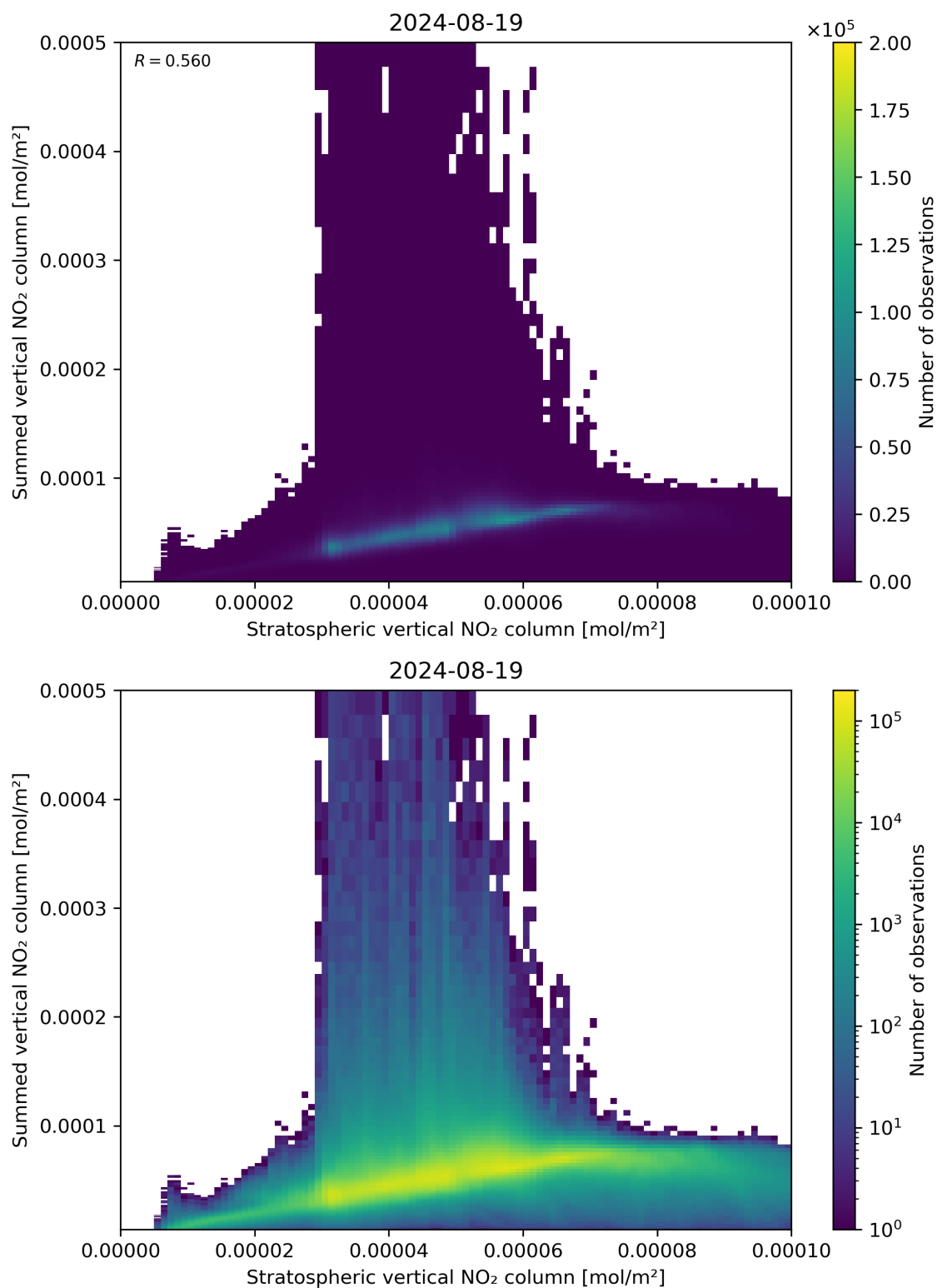
Figure 98: Scatter density plot of “Stratospheric vertical NO 2 column” against “Summed vertical NO 2 column” for 2024-08-18 to 2024-08-20.
