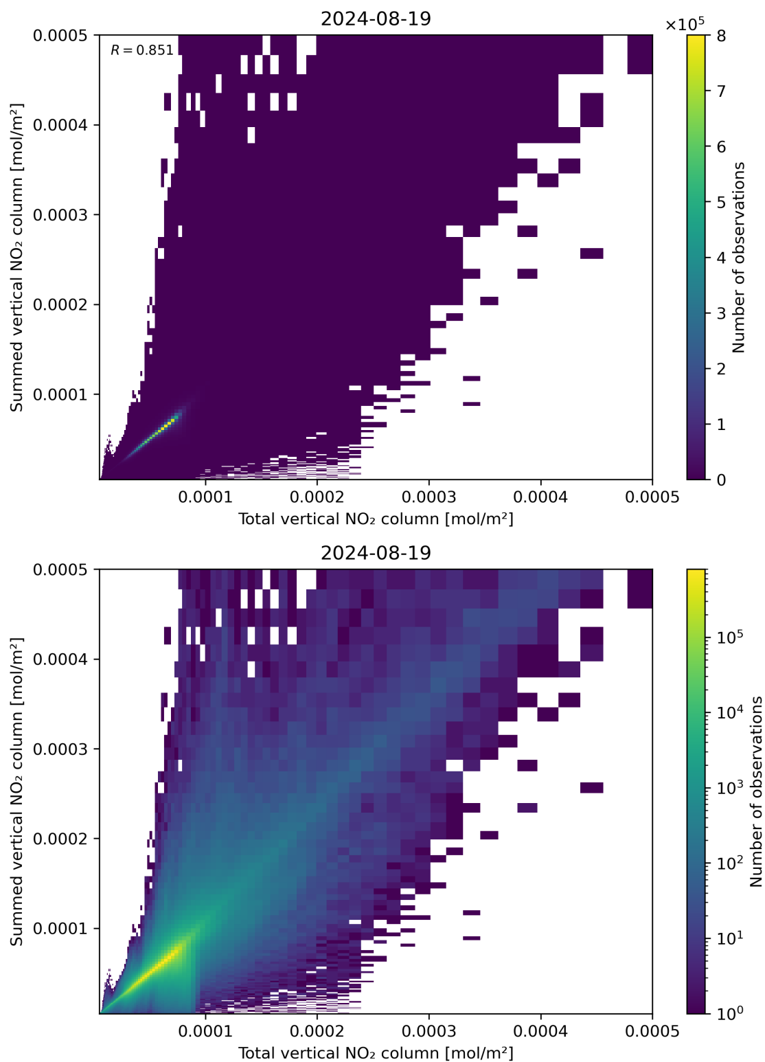
Figure 112: Scatter density plot of “Total vertical NO 2 column” against “Summed vertical NO 2 column” for 2024-08-18 to 2024-08-20.
