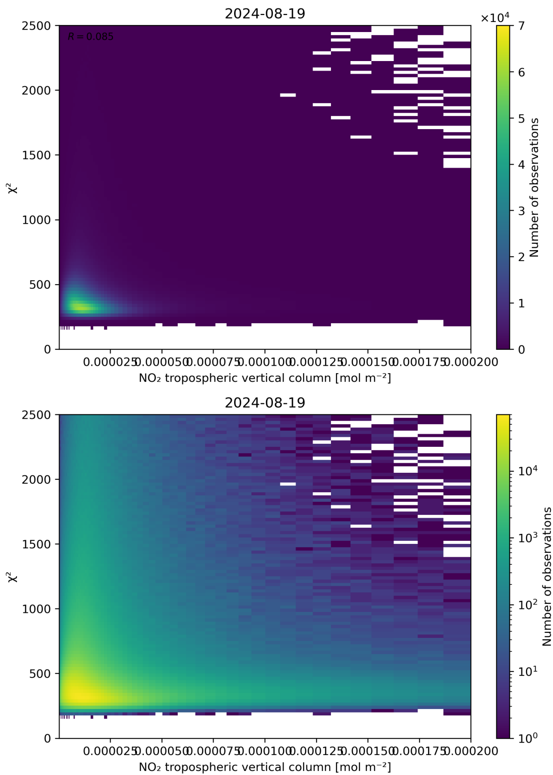
Figure 124: Scatter density plot of “NO 2 tropospheric vertical column” against “ \chi^2 ” for 2024-08-18 to 2024-08-20.
