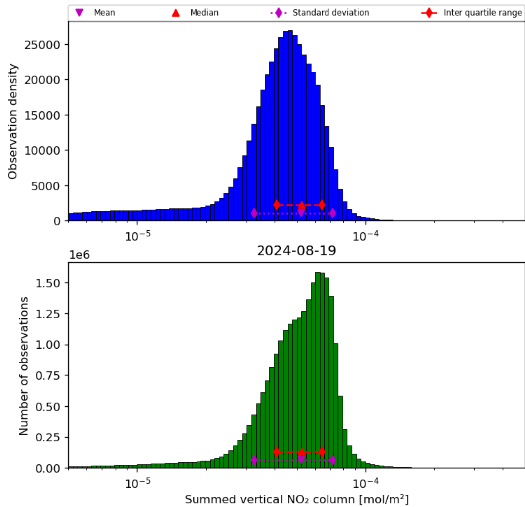
Figure 40: Histogram of “Summed vertical NO 2 column” for 2024-08-18 to 2024-08-20
