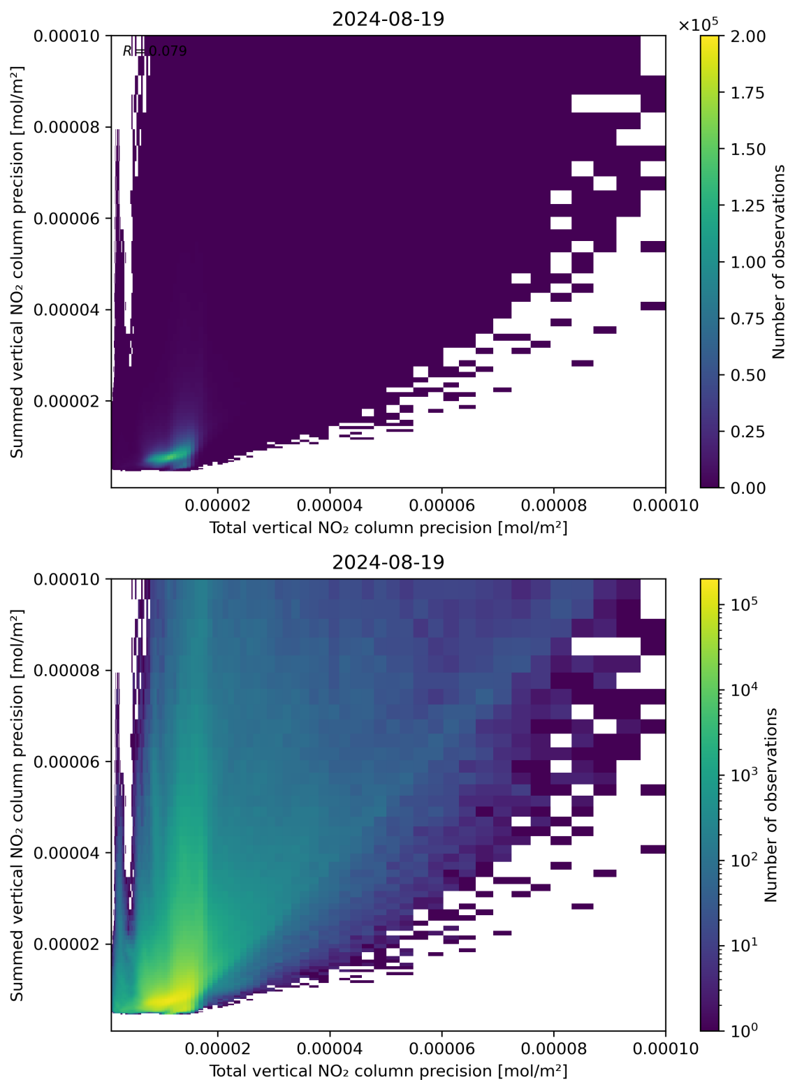
Figure 118: Scatter density plot of “Total vertical NO 2 column precision” against “Summed vertical NO 2 column precision” for 2024-08-18 to 2024-08-20.
