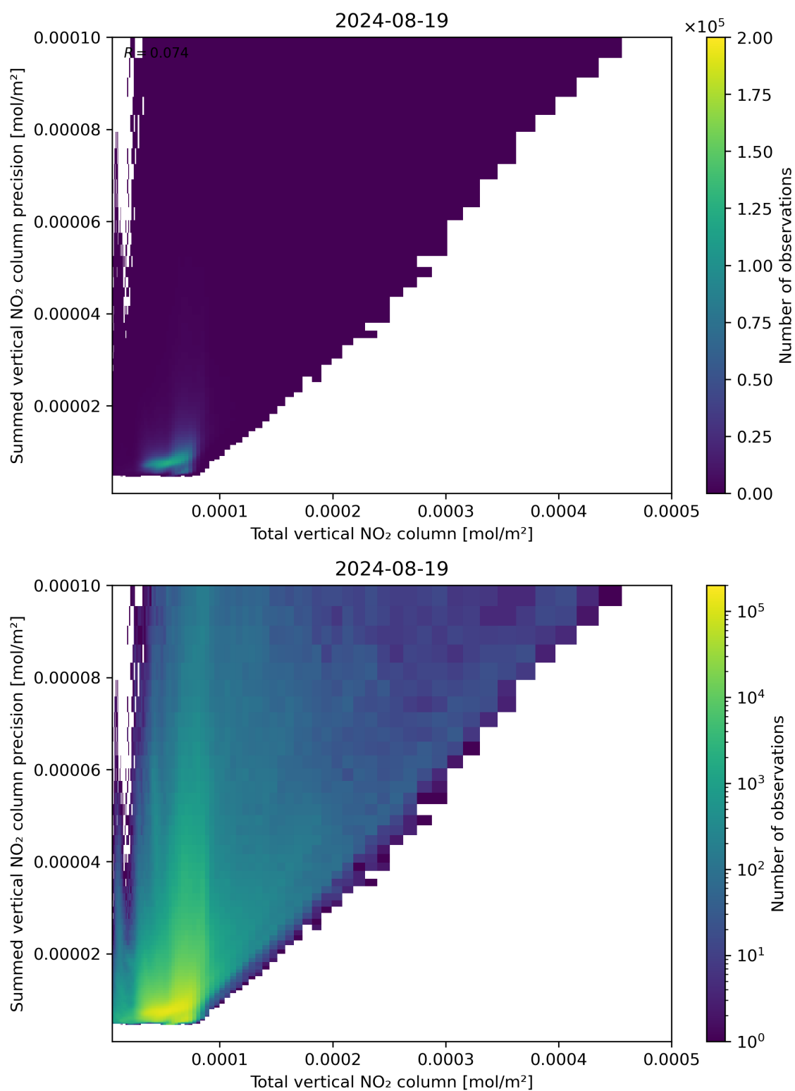
Figure 113: Scatter density plot of “Total vertical NO 2 column” against “Summed vertical NO 2 column precision” for 2024-08-18 to 2024-08-20.
