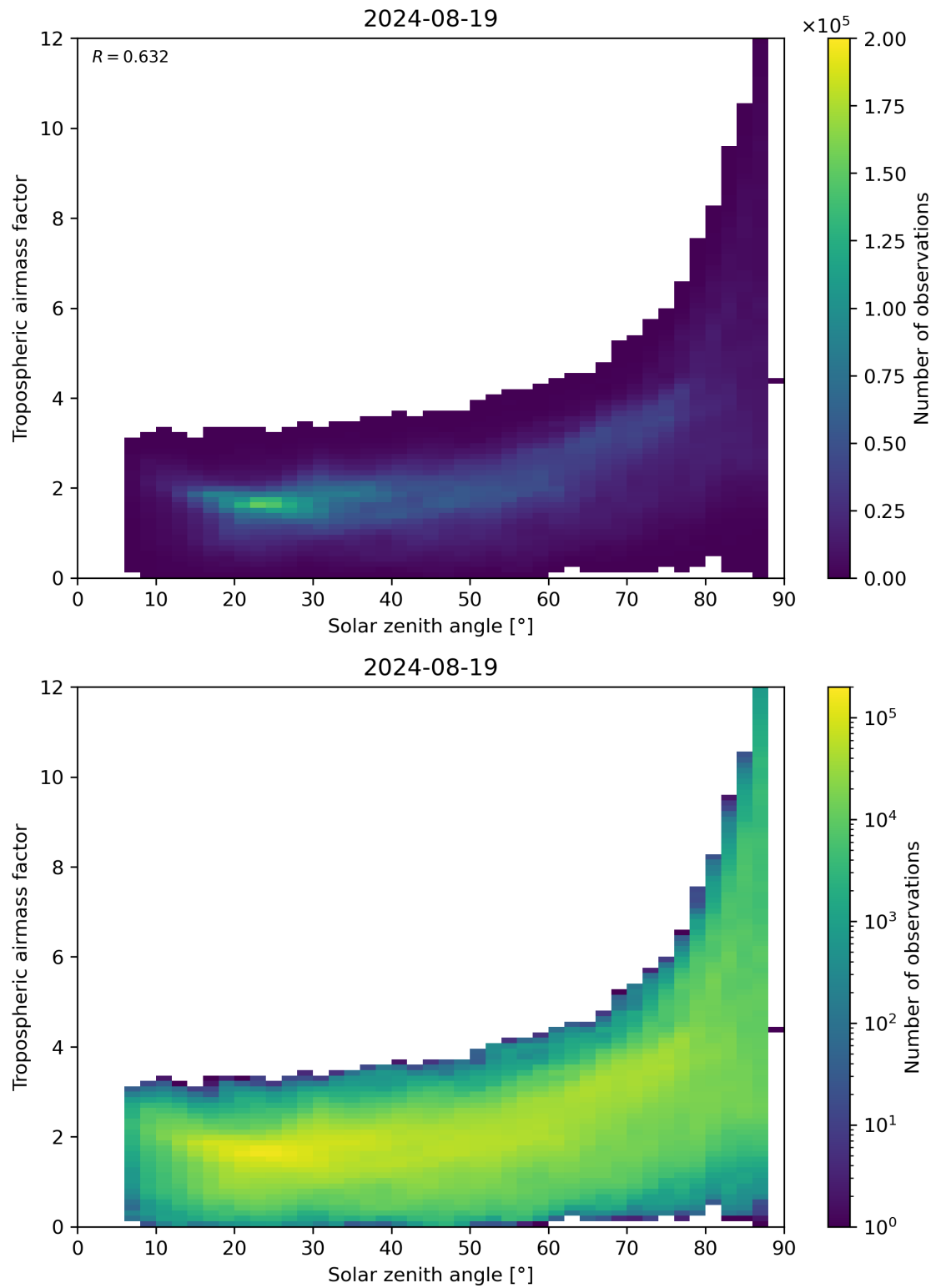
Figure 147: Scatter density plot of “Solar zenith angle” against “Tropospheric airmass factor” for 2024-08-18 to 2024-08-20.
