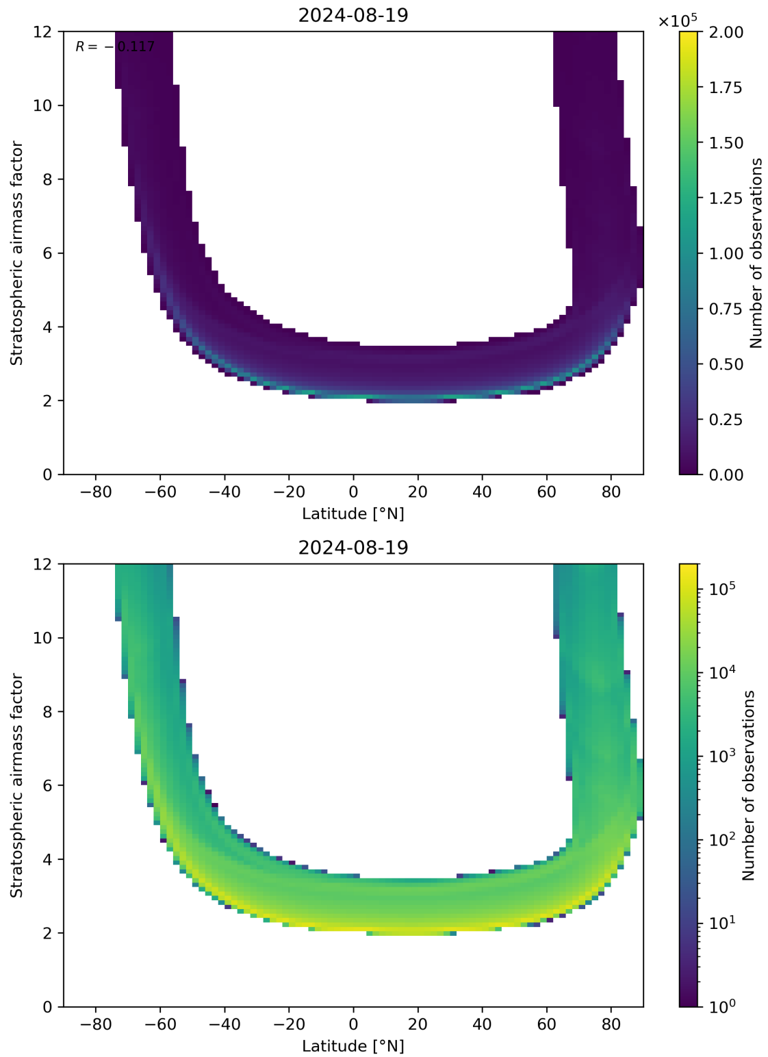
Figure 83: Scatter density plot of “Latitude” against “Stratospheric air mass factor” for 2024-08-18 to 2024-08-20.
