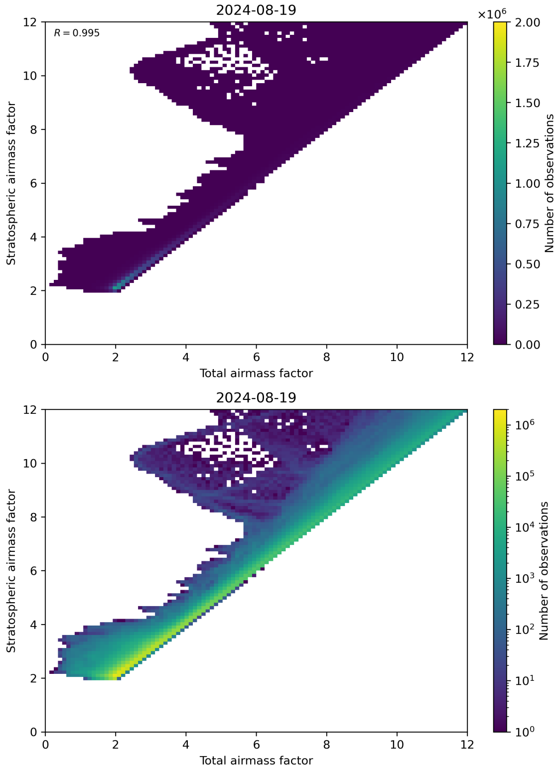
Figure 62: Scatter density plot of “Total airmass factor” against “Stratospheric airmass factor” for 2024-08-18 to 2024-08-20.
