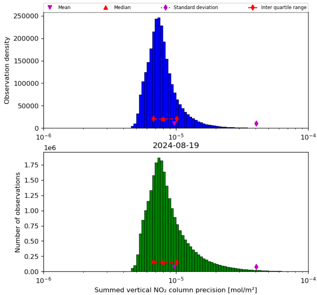
Figure 41: Histogram of "Summed vertical NO 2 column precision" for 2024-08-18 to 2024-08-20
