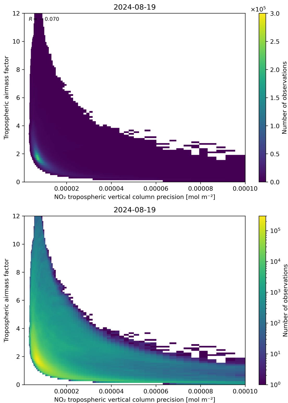
Figure 133: Scatter density plot of “NO 2 tropospheric vertical column precision” against “Tropospheric airmass factor” for 2024-08-18 to 2024-08-20.
