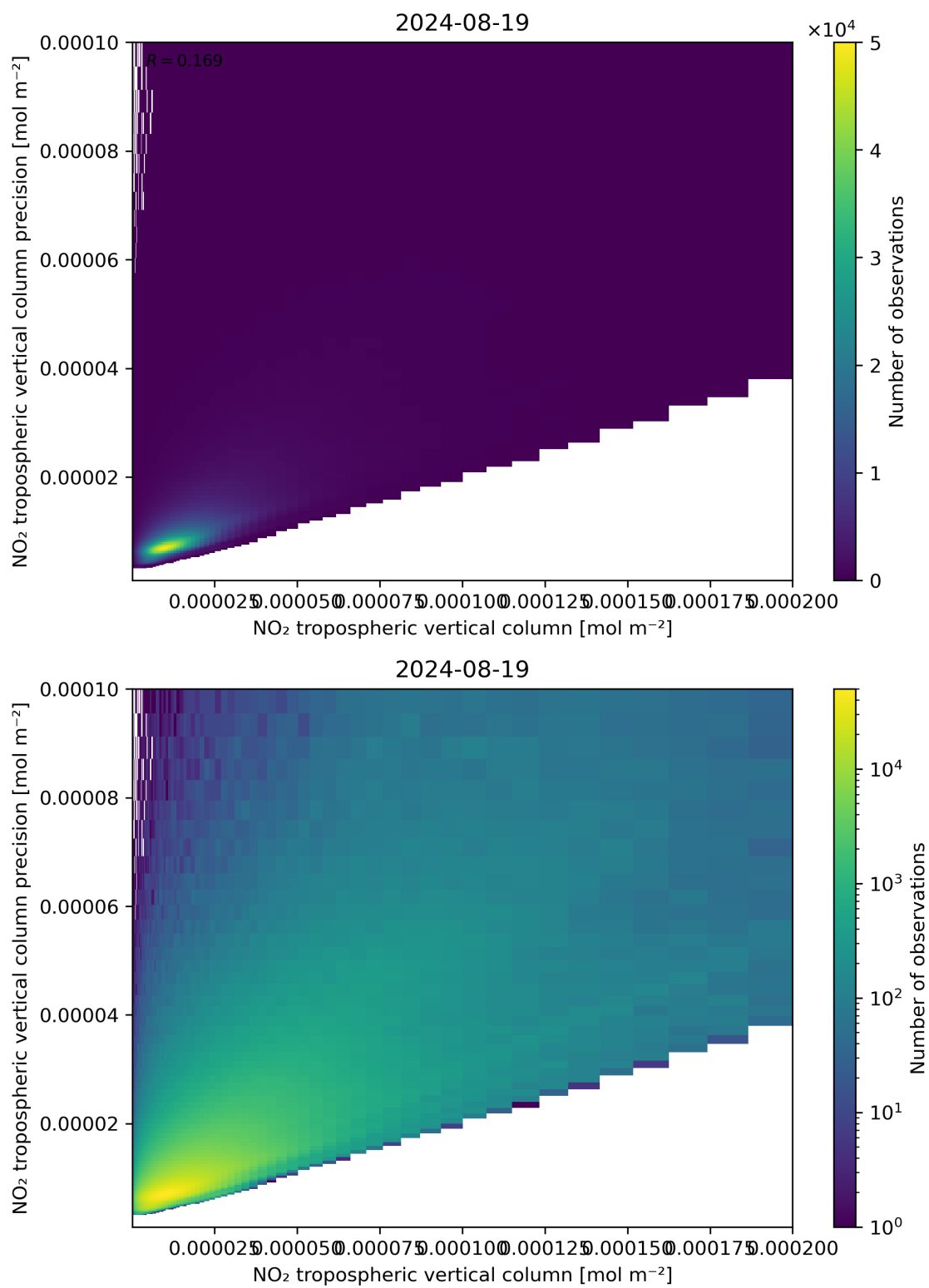
Figure 130: Scatter density plot of “NO 2 tropospheric vertical column” against “NO 2 tropospheric vertical column precision” for 2024-08-18 to 2024-08-20.
