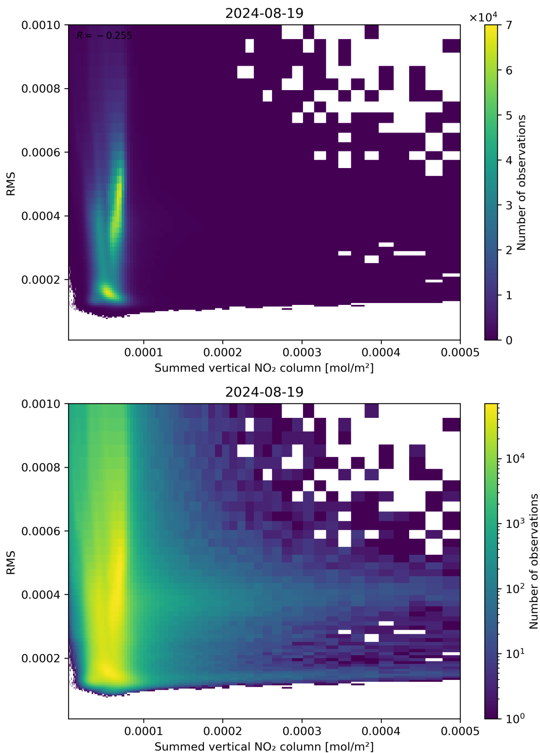
Figure 109: Scatter density plot of “Summed vertical NO 2 column” against “RMS” for 2024-08-18 to 2024-08-20.
