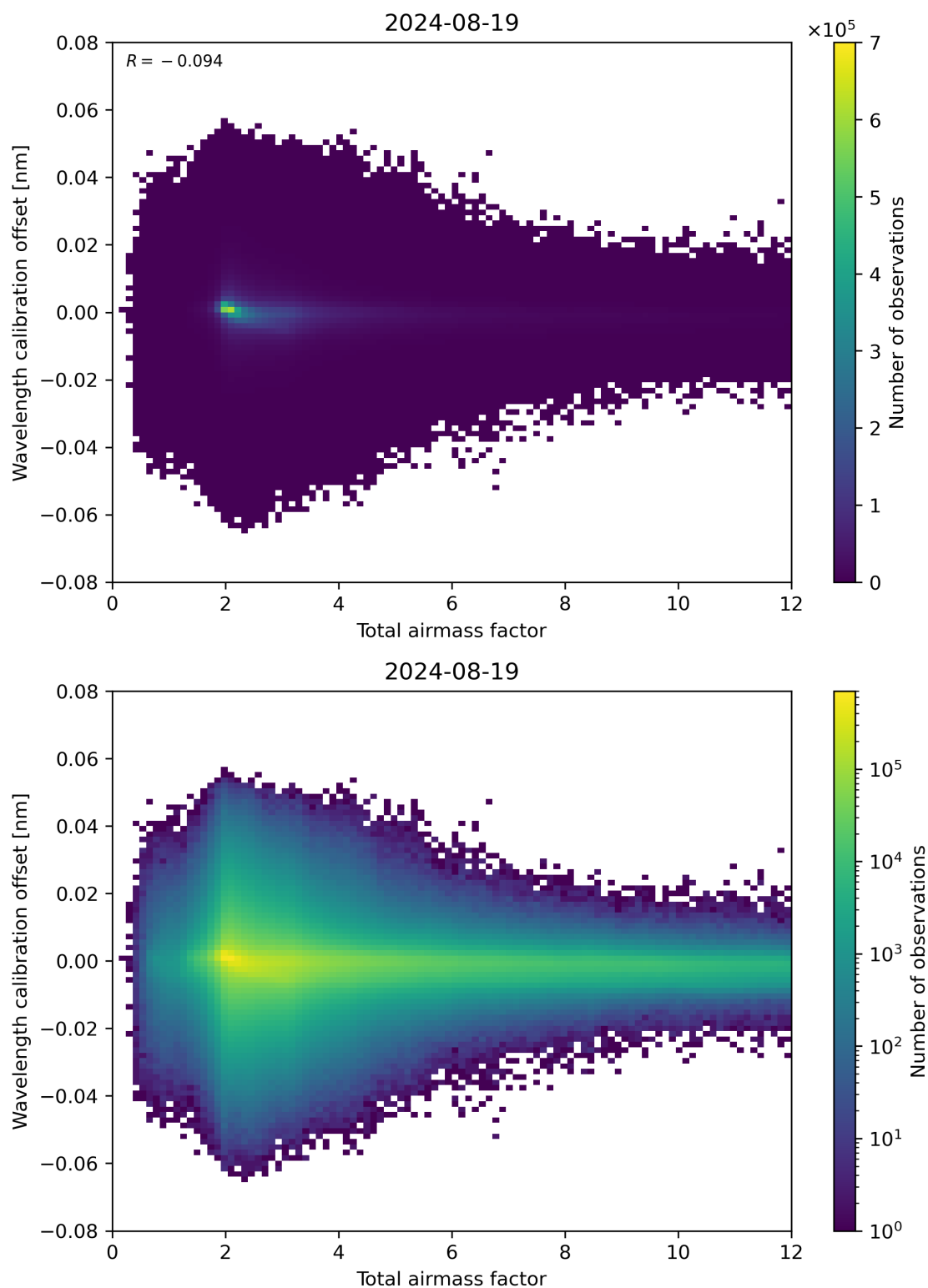
Figure 70: Scatter density plot of “Total airmass factor” against “Wavelength calibration offset” for 2024-08-18 to 2024-08-20.
