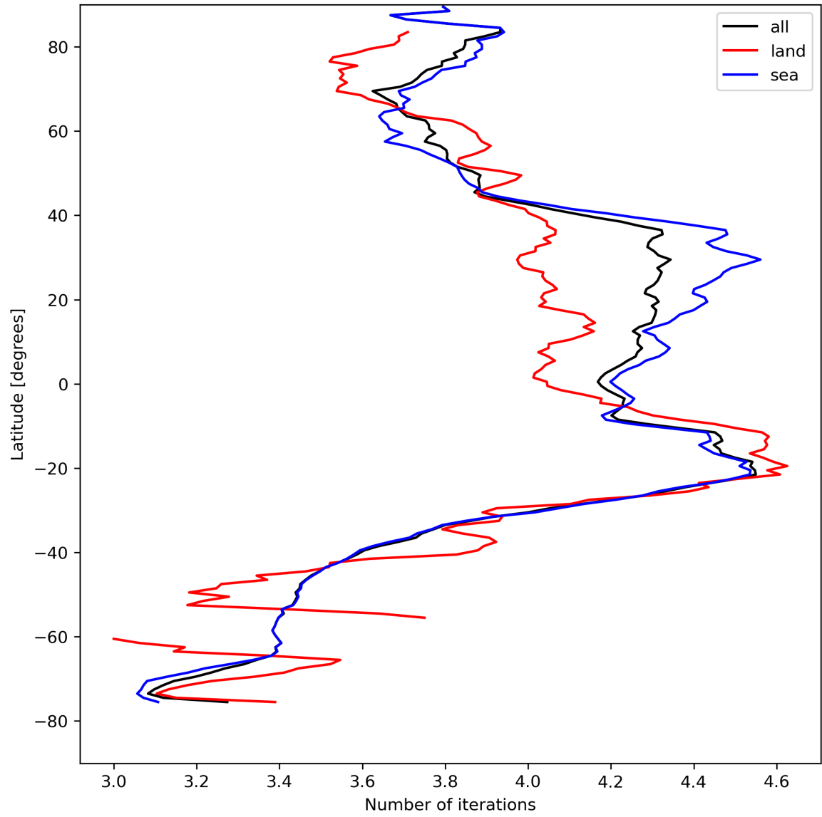
Figure 17: Zonal average of “Number of iterations” for 2024-08-18 to 2024-08-20.
