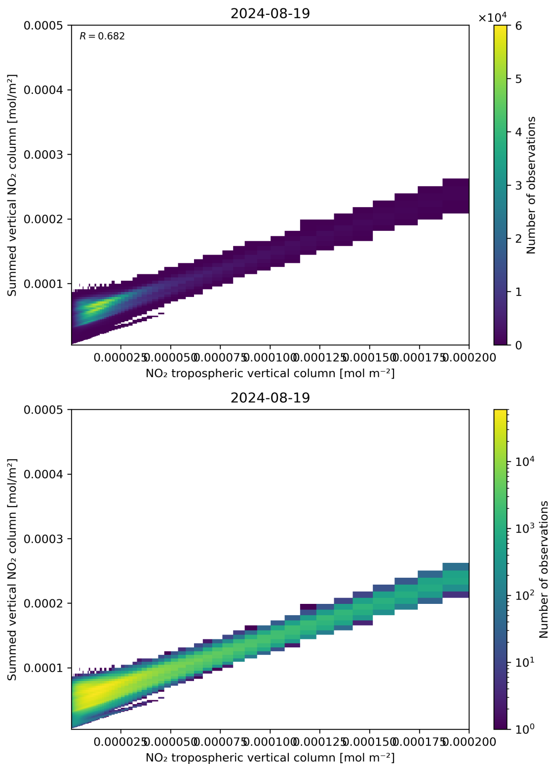
Figure 126: Scatter density plot of “NO 2 tropospheric vertical column” against “Summed vertical NO 2 column” for 2024-08-18 to 2024-08-20.
