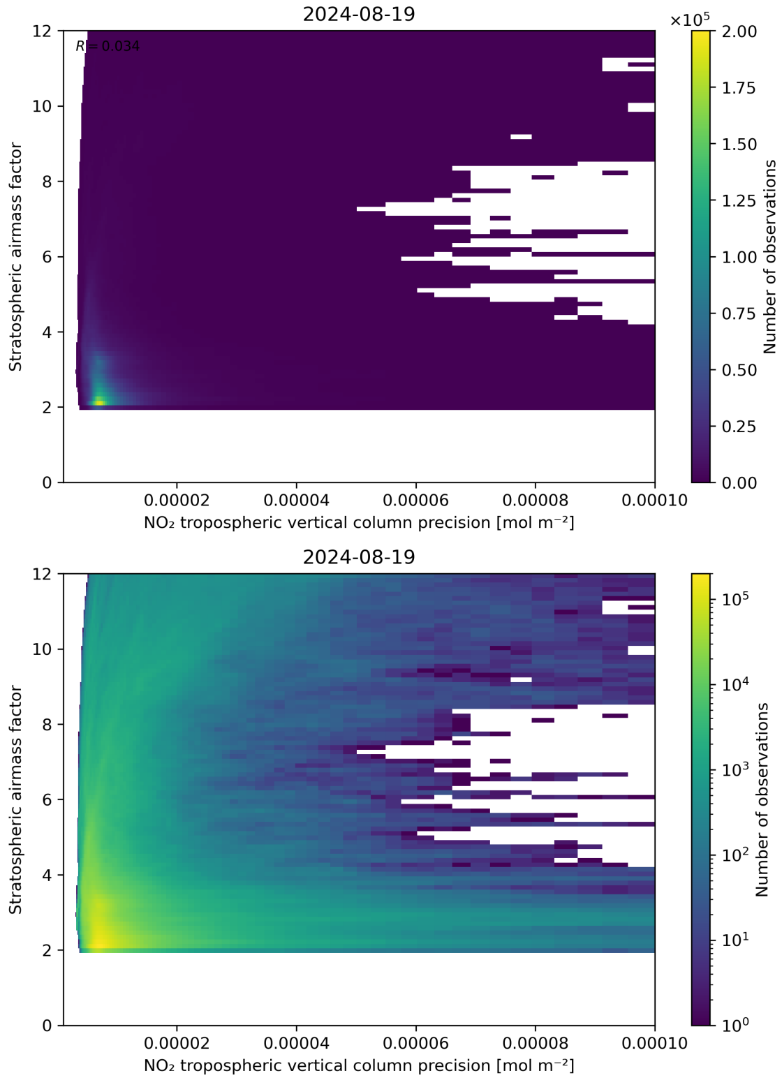
Figure 131: Scatter density plot of “NO 2 tropospheric vertical column precision” against “Stratospheric airmass factor” for 2024-08-18 to 2024-08-20.
