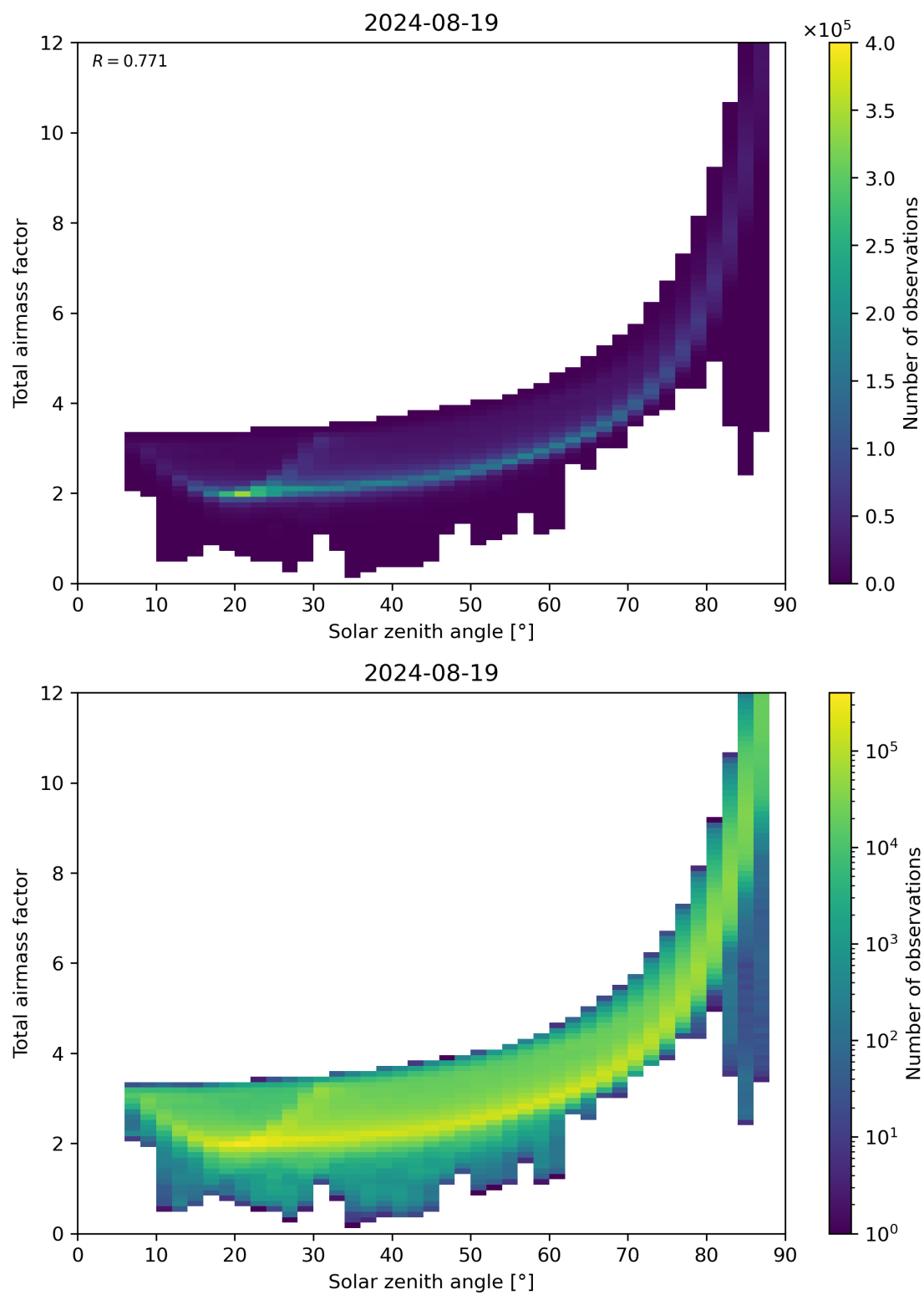
Figure 146: Scatter density plot of “Solar zenith angle” against “Total air mass factor” for 2024-08-18 to 2024-08-20.
