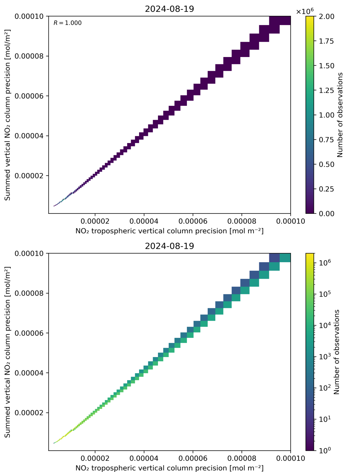
Figure 137: Scatter density plot of “NO 2 tropospheric vertical column precision” against “Summed vertical NO 2 column precision” for 2024-08-18 to 2024-08-20.
