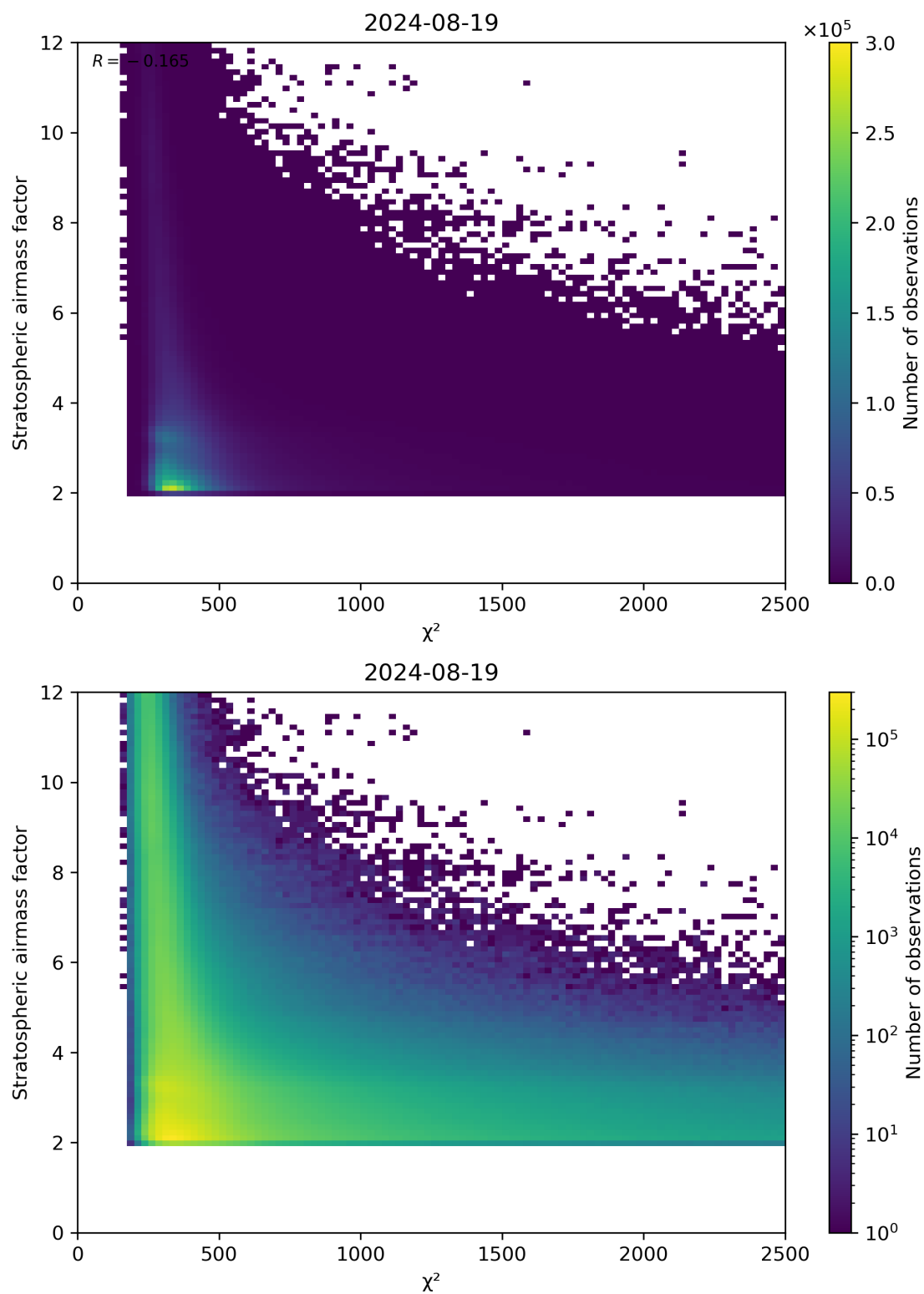
Figure 81: Scatter density plot of “ \chi^2 ” against “Stratospheric airmass factor” for 2024-08-18 to 2024-08-20.
