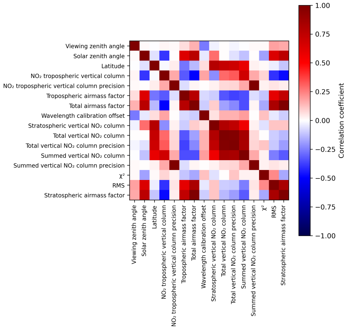
Figure 2: Map of correlation matrix for 2024-08-18 to 2024-08-20.
