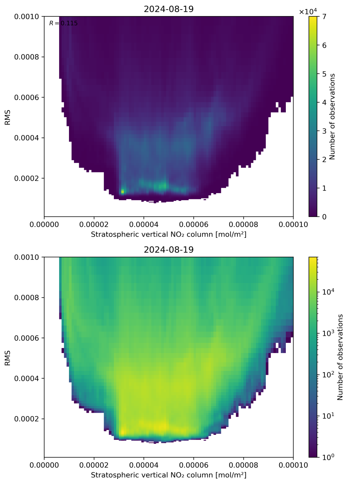
Figure 102: Scatter density plot of “Stratospheric vertical NO 2 column” against “RMS” for 2024-08-18 to 2024-08-20.
