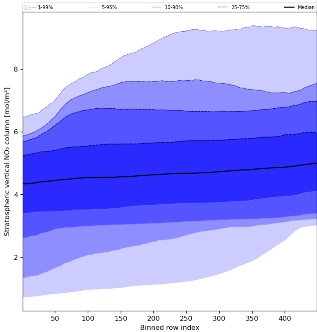
Figure 53: Along track statistics of “Stratospheric vertical NO 2 column” for 2024-08-18 to 2024-08-20
