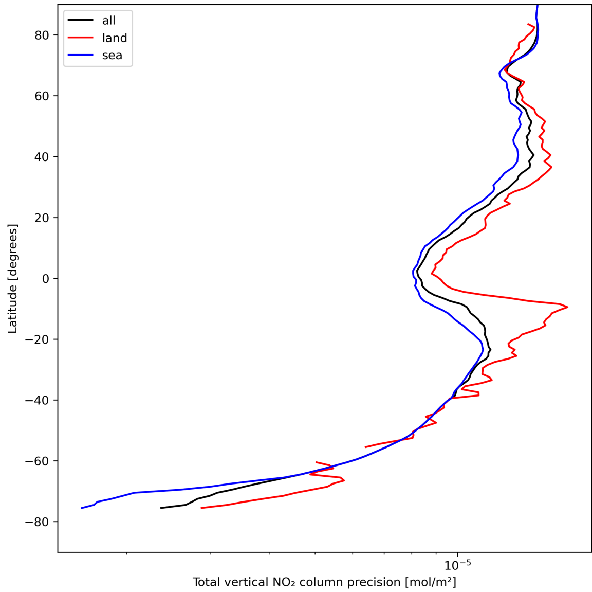
Figure 22: Zonal average of “Total vertical NO 2 column precision” for 2024-08-18 to 2024-08-20.
