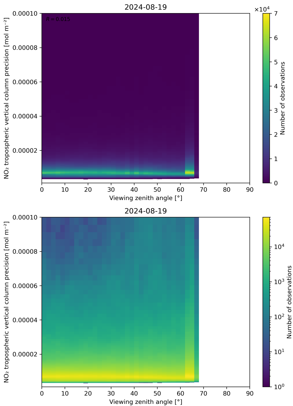
Figure 170: Scatter density plot of “Viewing zenith angle” against “NO 2 tropospheric vertical column precision” for 2024-08-18 to 2024-08-20.
