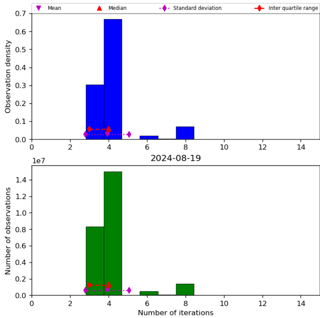
Figure 34: Histogram of “Number of iterations” for 2024-08-18 to 2024-08-20
