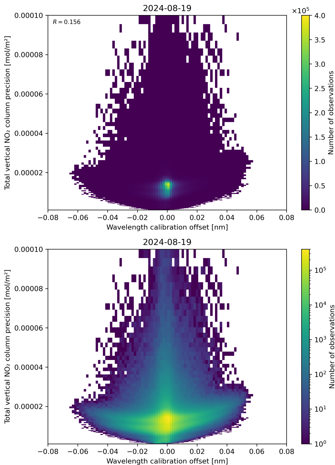
Figure 180: Scatter density plot of “Wavelength calibration offset” against “Total vertical NO 2 column precision” for 2024-08-18 to 2024-08-20.
