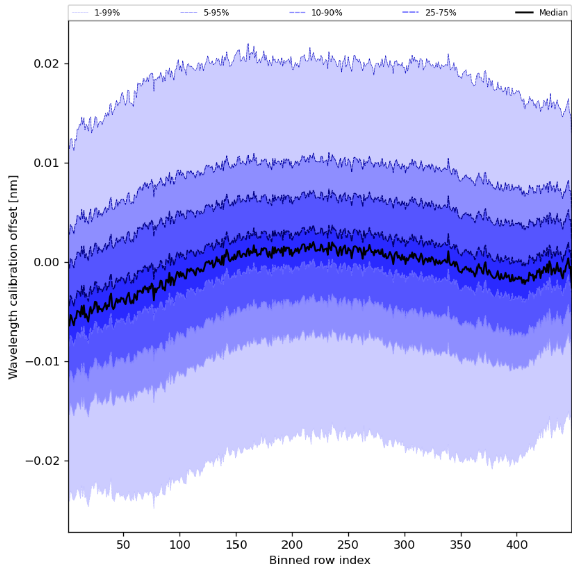
Figure 52: Along track statistics of “Wavelength calibration offset” for 2024-08-18 to 2024-08-20
