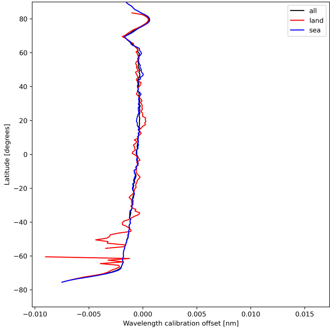
Figure 18: Zonal average of “Wavelength calibration offset” for 2024-08-18 to 2024-08-20.
