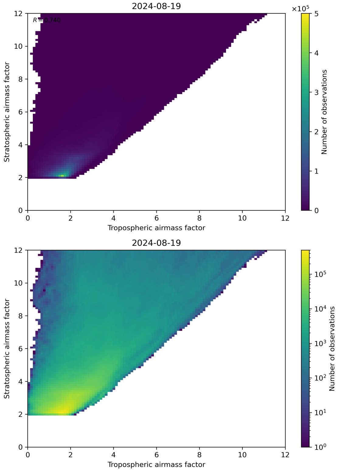
Figure 71: Scatter density plot of “Tropospheric airmass factor” against “Stratospheric airmass factor” for 2024-08-18 to 2024-08-20.
