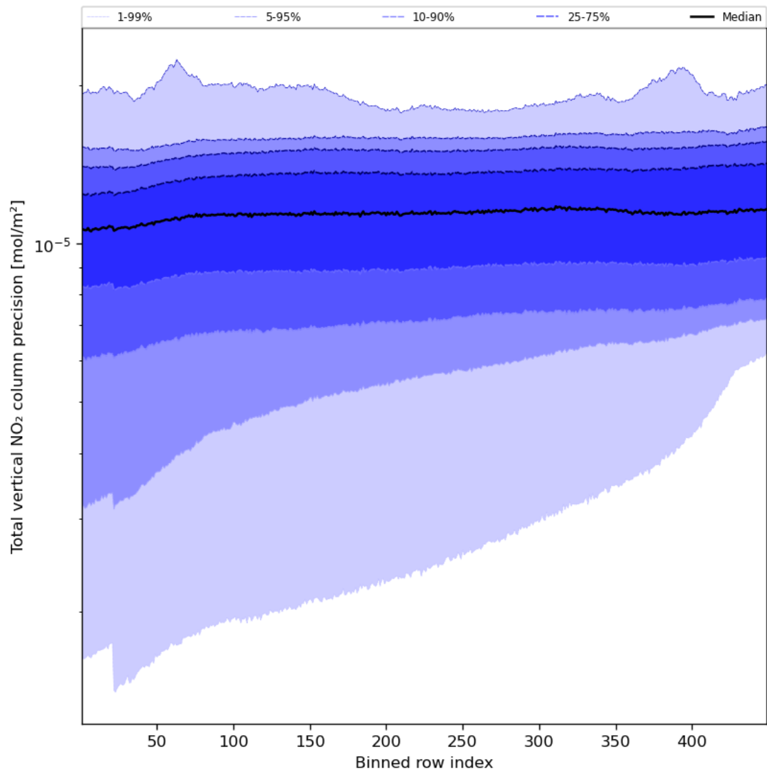
Figure 56: Along track statistics of “Total vertical NO 2 column precision” for 2024-08-18 to 2024-08-20
