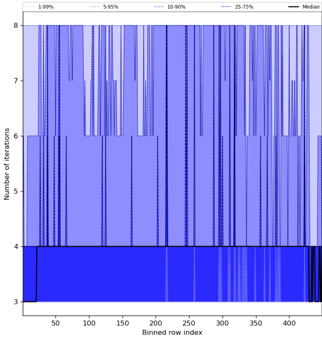
Figure 51: Along track statistics of “Number of iterations” for 2024-08-18 to 2024-08-20
