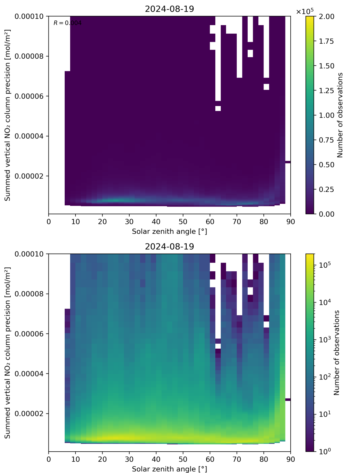
Figure 152: Scatter density plot of “Solar zenith angle” against “Summed vertical NO 2 column precision” for 2024-08-18 to 2024-08-20.
