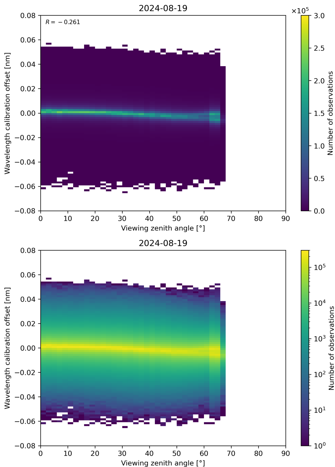
Figure 173: Scatter density plot of “Viewing zenith angle” against “Wavelength calibration offset” for 2024-08-18 to 2024-08-20.
