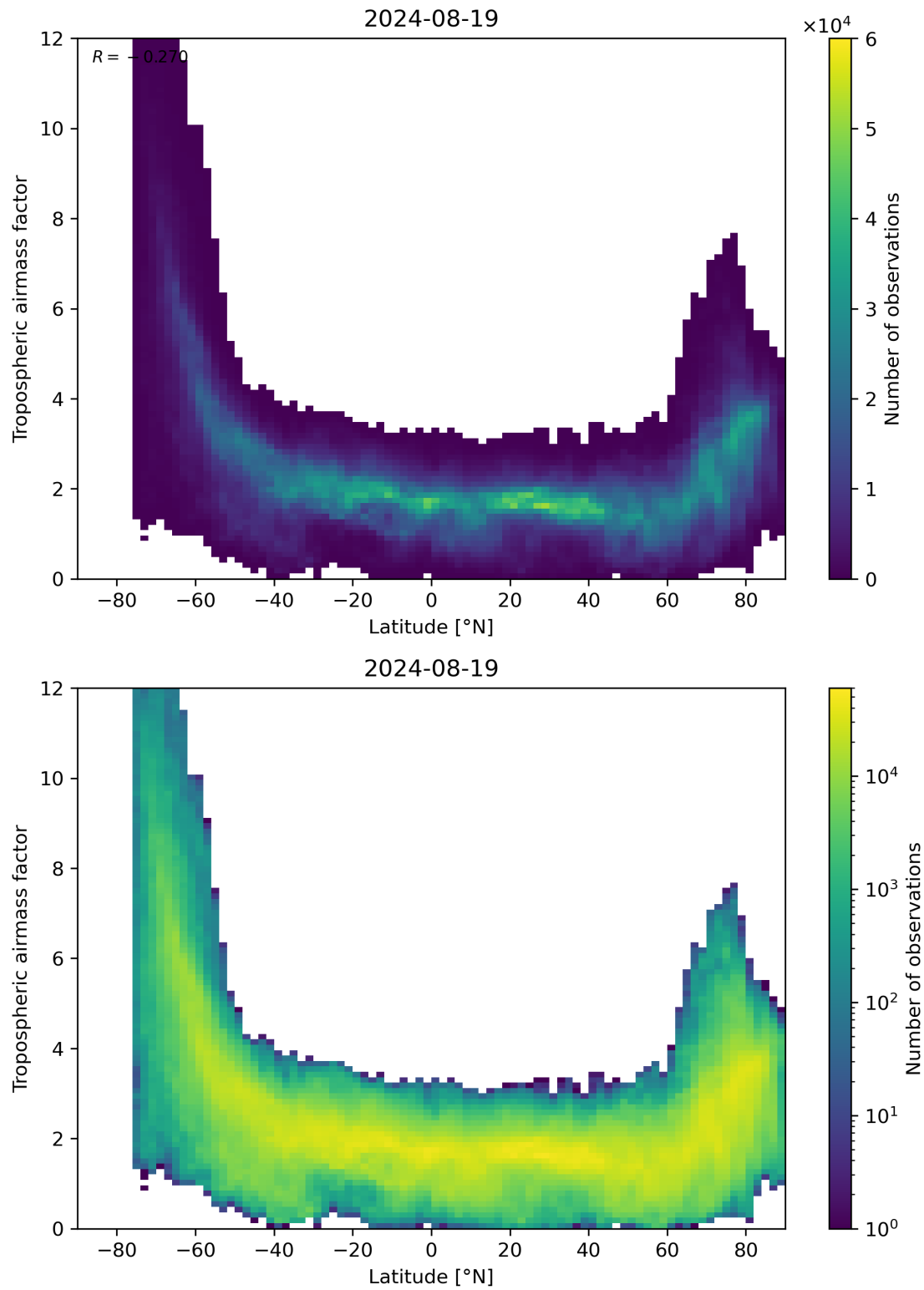
Figure 85: Scatter density plot of “Latitude” against “Tropospheric air mass factor” for 2024-08-18 to 2024-08-20.
