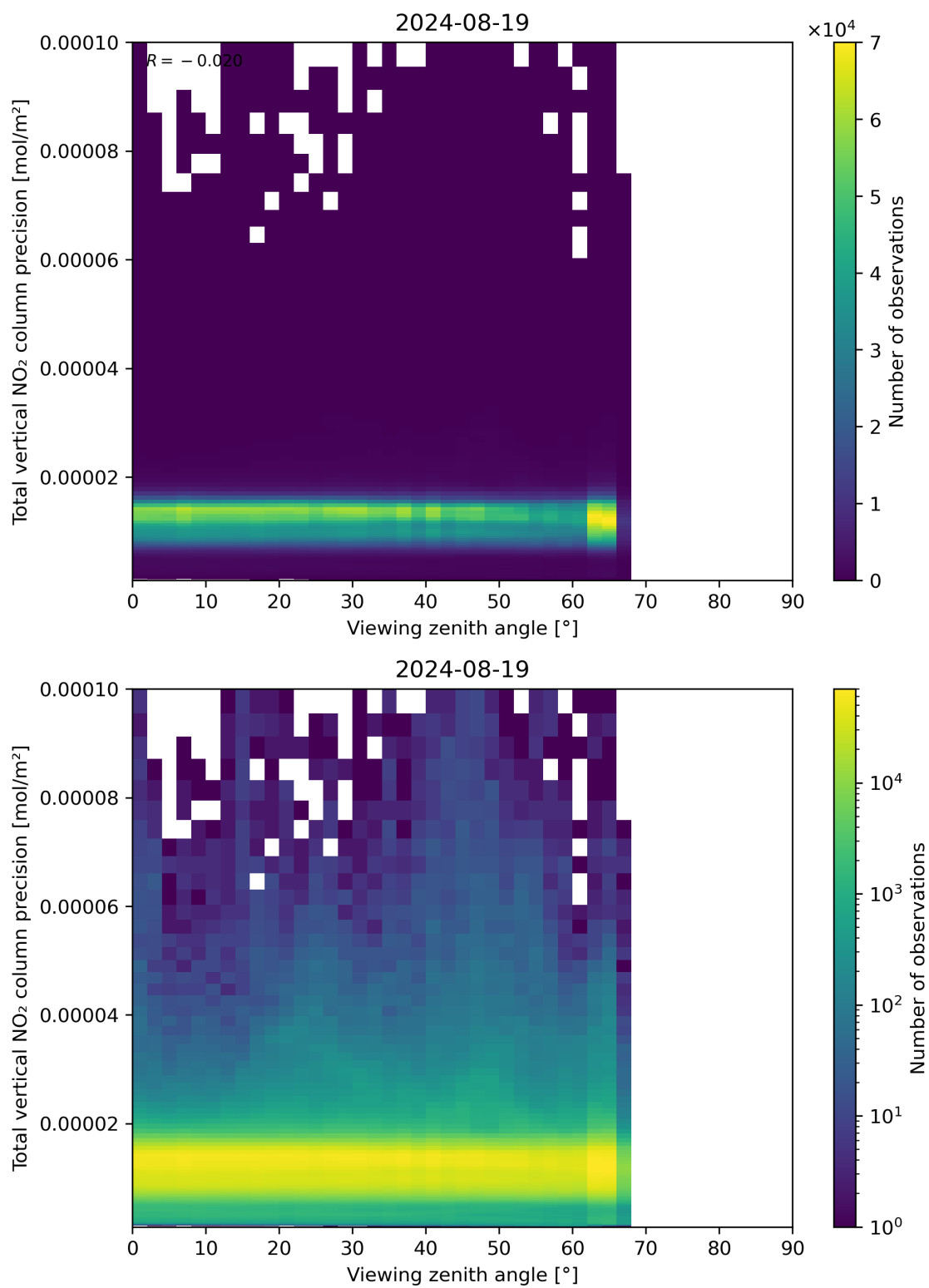
Figure 168: Scatter density plot of “Viewing zenith angle” against “Total vertical NO 2 column precision” for 2024-08-18 to 2024-08-20.
