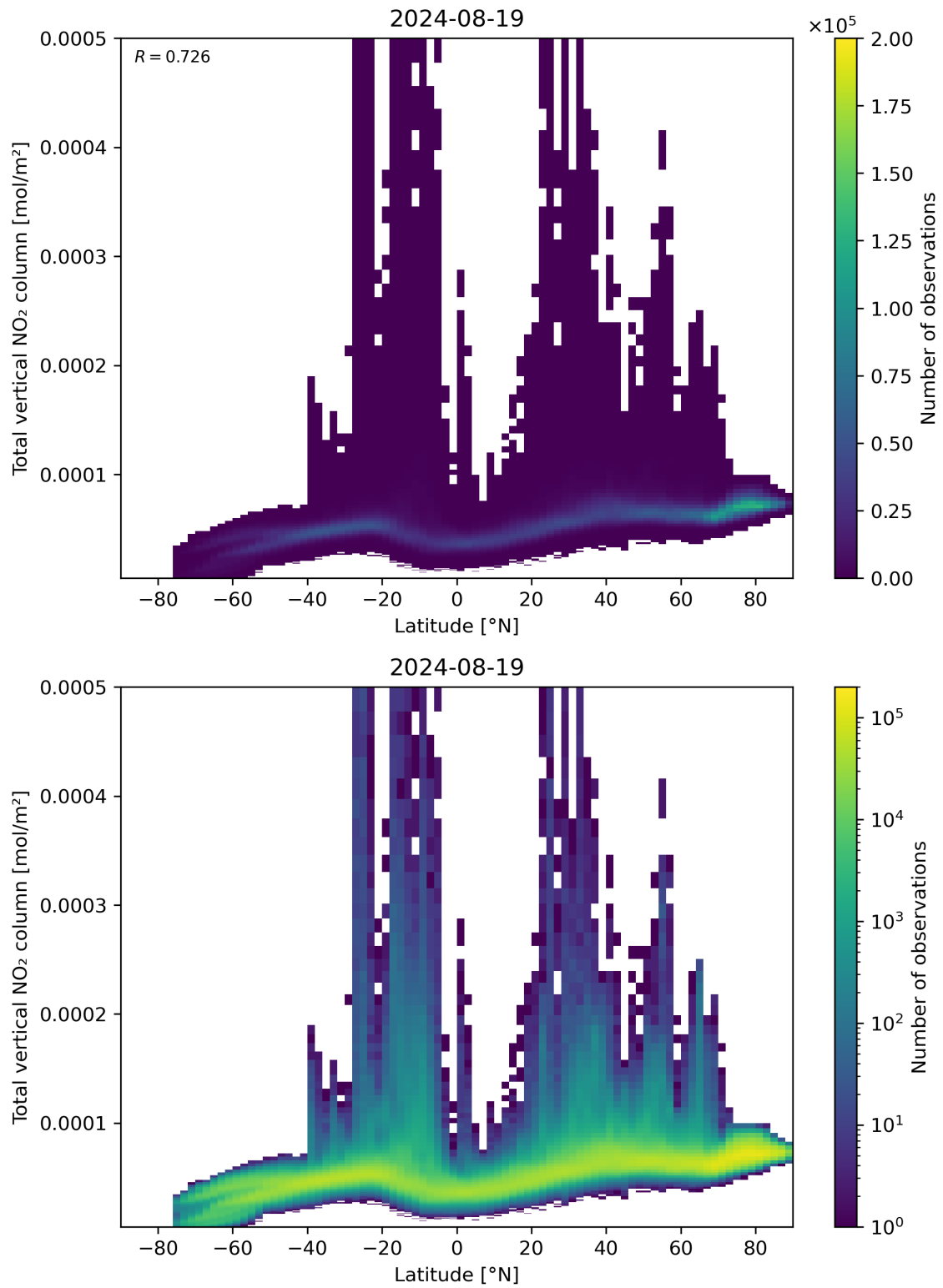
Figure 90: Scatter density plot of “Latitude” against “Total vertical NO 2 column” for 2024-08-18 to 2024-08-20.
