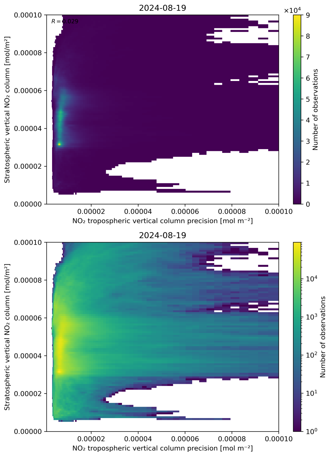
Figure 135: Scatter density plot of “NO 2 tropospheric vertical column precision” against “Stratospheric vertical NO 2 column” for 2024-08-18 to 2024-08-20.
