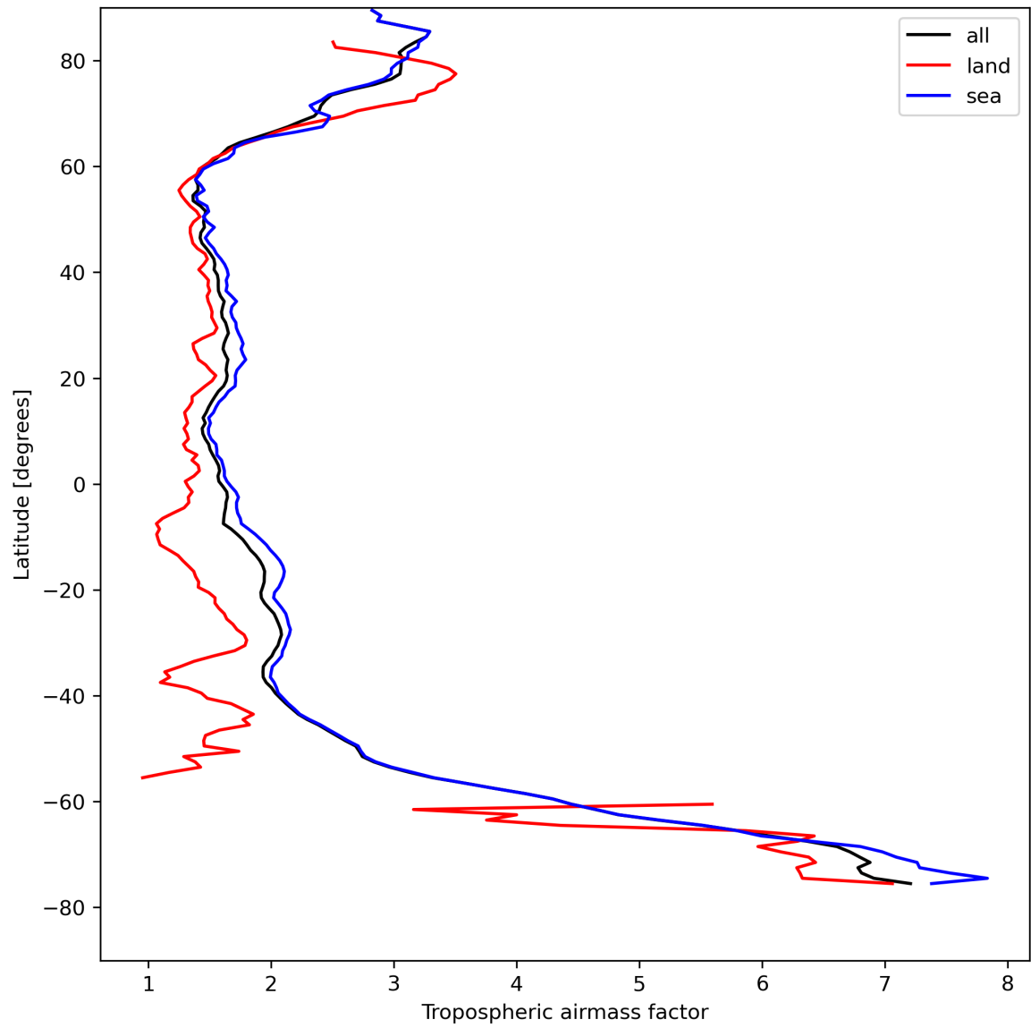
Figure 14: Zonal average of “Tropospheric airmass factor” for 2024-08-18 to 2024-08-20.
