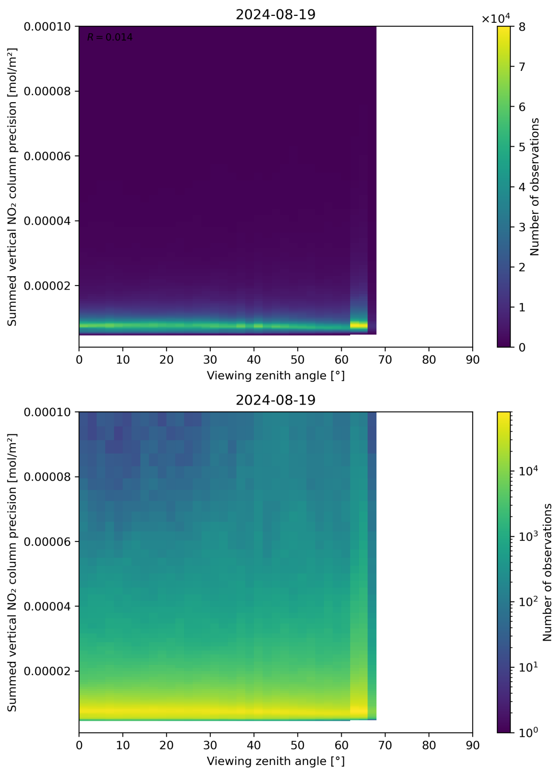
Figure 166: Scatter density plot of “Viewing zenith angle” against “Summed vertical NO 2 column precision” for 2024-08-18 to 2024-08-20.
