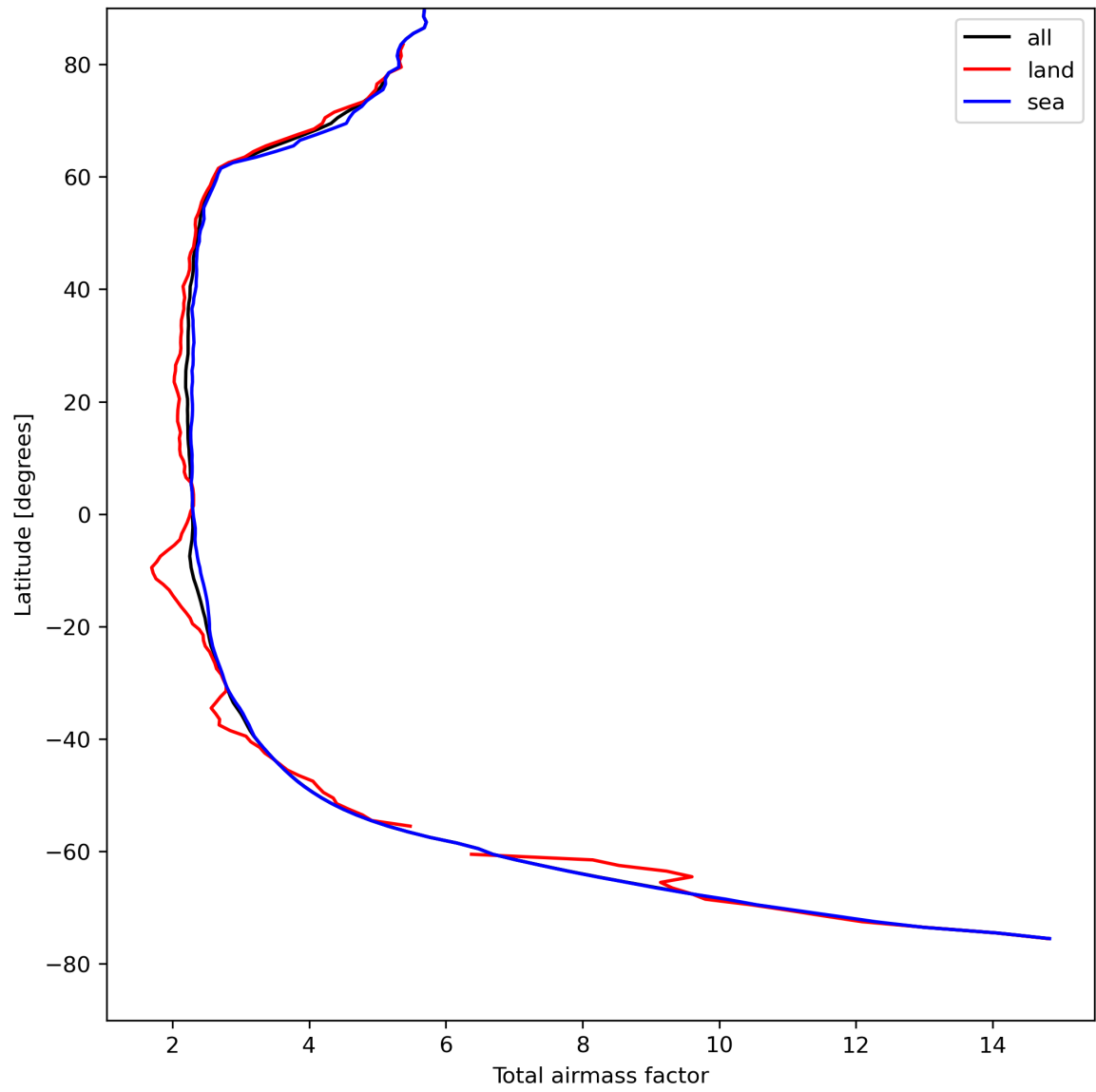
Figure 15: Zonal average of “Total airmass factor” for 2024-08-18 to 2024-08-20.
