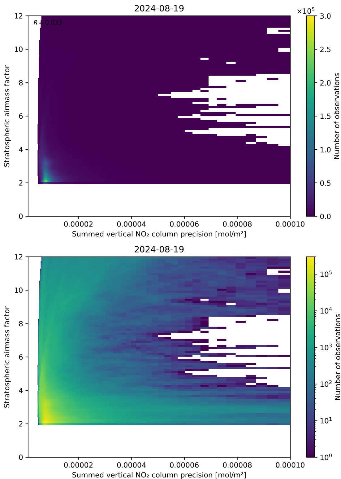
Figure 106: Scatter density plot of “Summed vertical NO 2 column precision” against “Stratospheric airmass factor” for 2024-08-18 to 2024-08-20.
