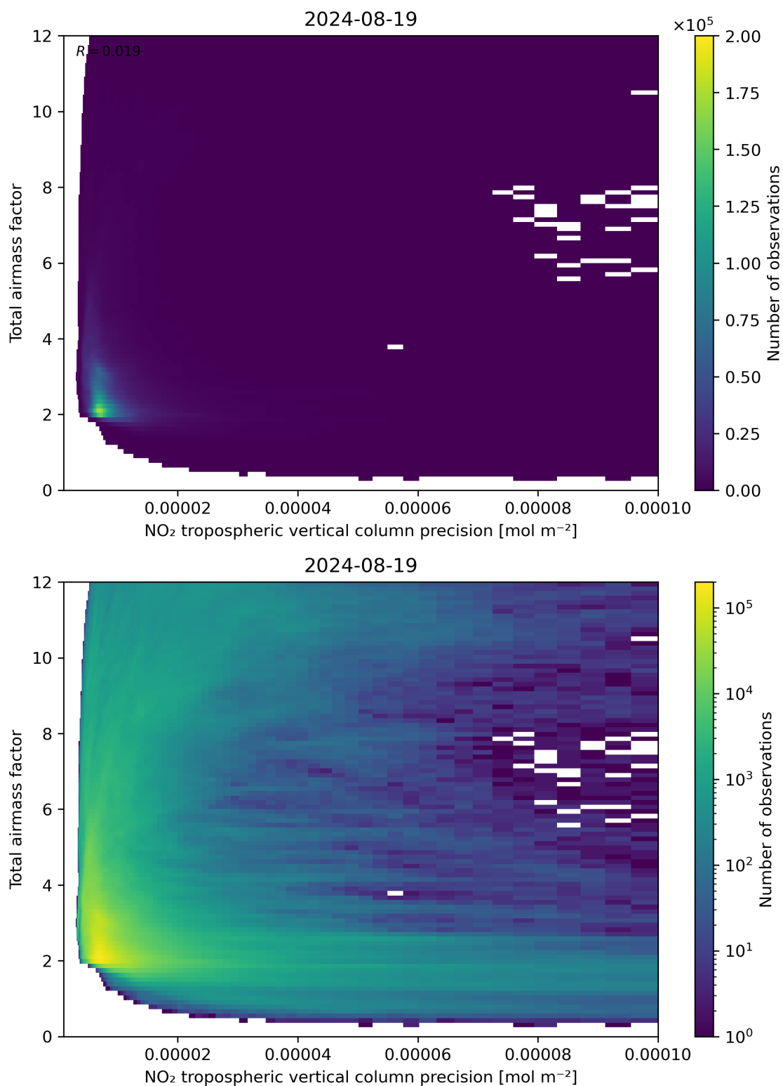
Figure 132: Scatter density plot of “NO 2 tropospheric vertical column precision” against “Total air mass factor” for 2024-08-18 to 2024-08-20.
