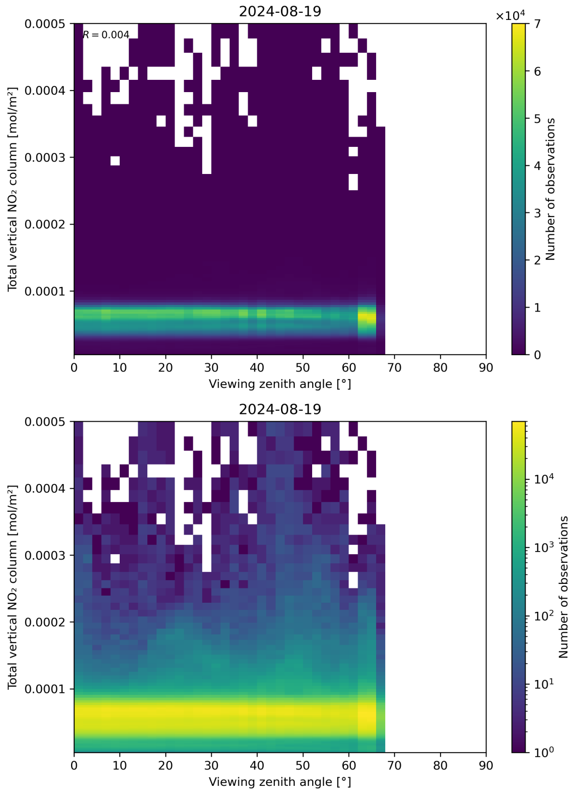
Figure 167: Scatter density plot of “Viewing zenith angle” against “Total vertical NO 2 column” for 2024-08-18 to 2024-08-20.
