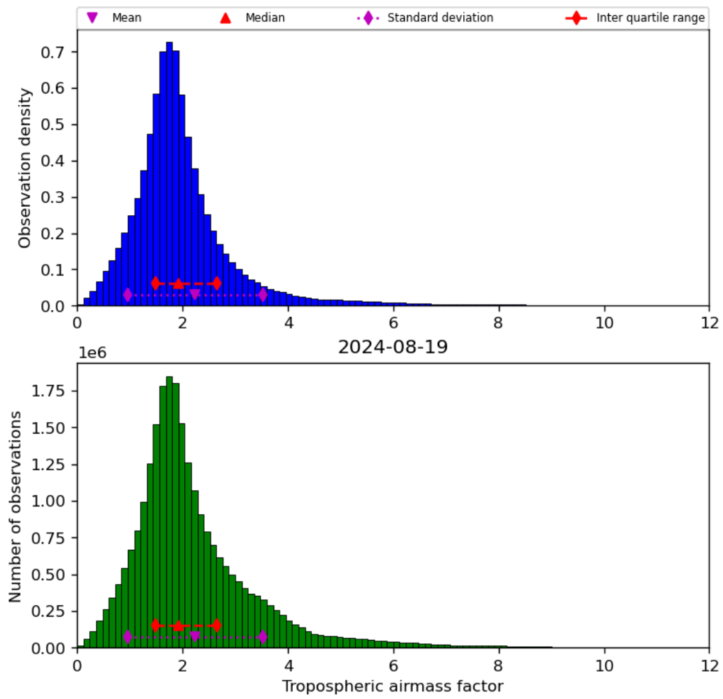
Figure 31: Histogram of “Tropospheric airmass factor” for 2024-08-18 to 2024-08-20
