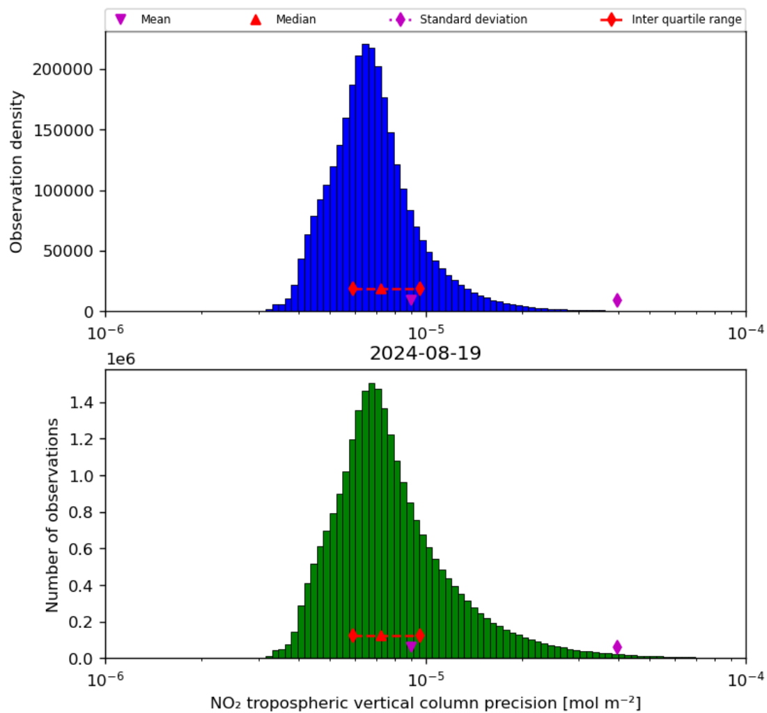
Figure 30: Histogram of “NO 2 tropospheric vertical column precision” for 2024-08-18 to 2024-08-20
