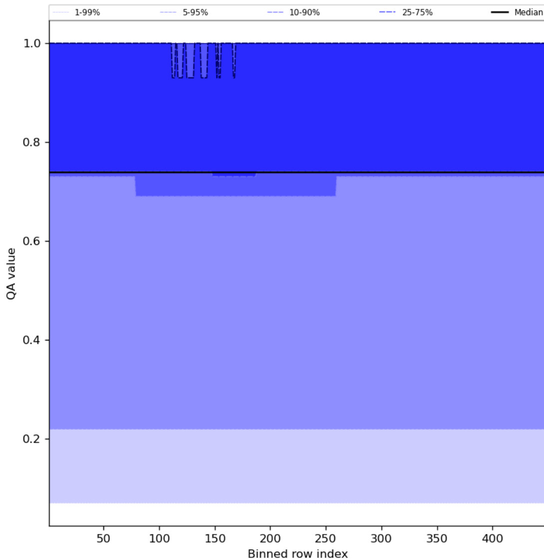
Figure 45: Along track statistics of “QA value” for 2024-08-18 to 2024-08-20
