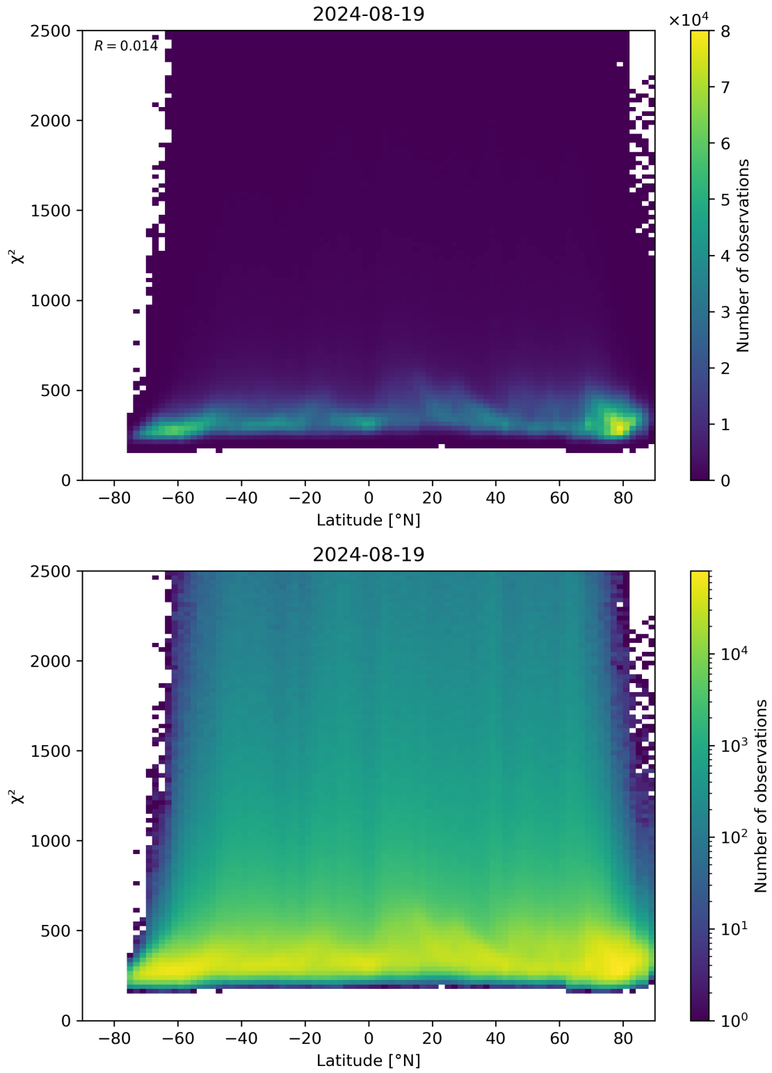
Figure 86: Scatter density plot of “Latitude” against “ \chi^2 ” for 2024-08-18 to 2024-08-20.
