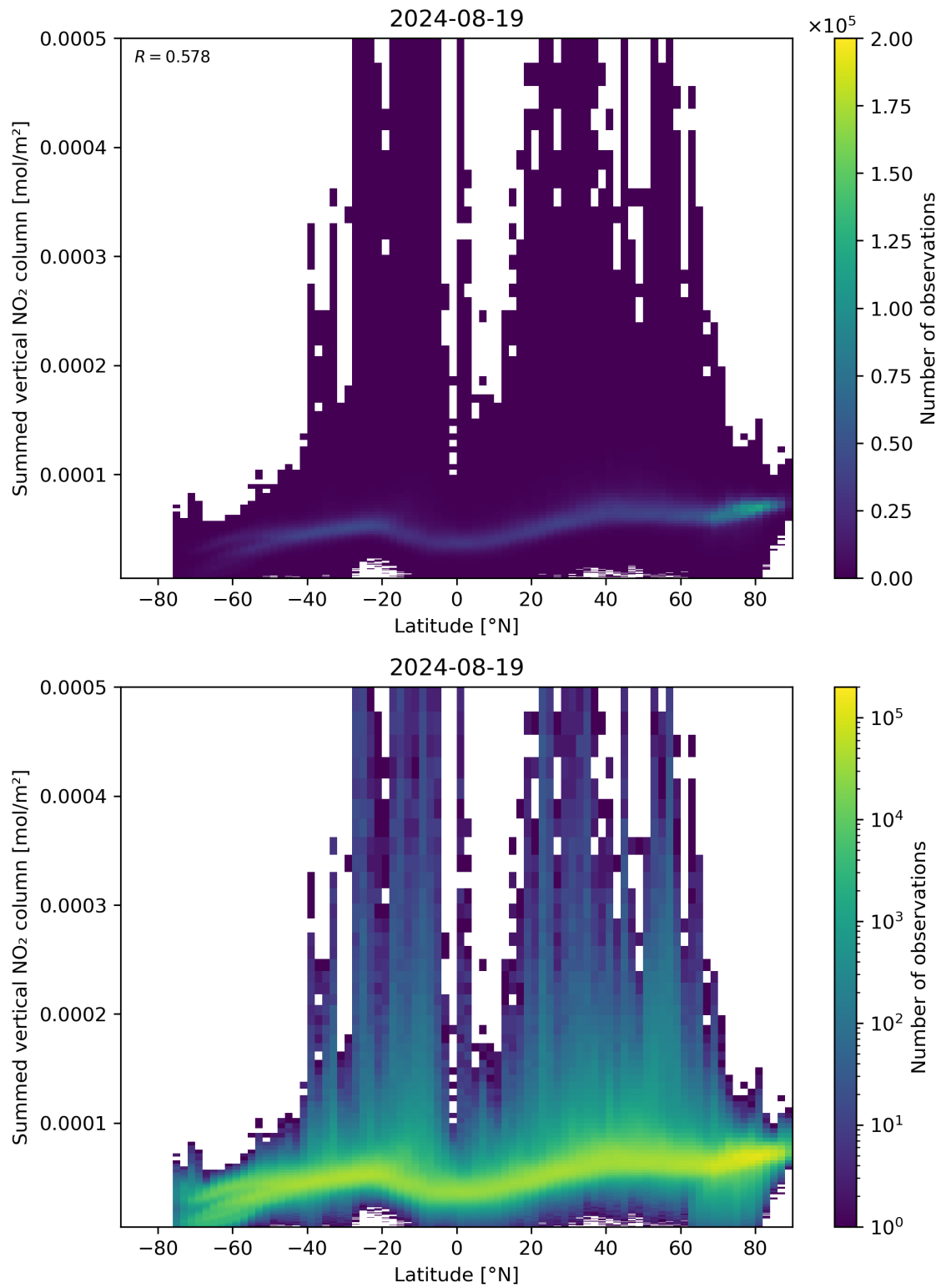
Figure 88: Scatter density plot of “Latitude” against “Summed vertical NO 2 column” for 2024-08-18 to 2024-08-20.
