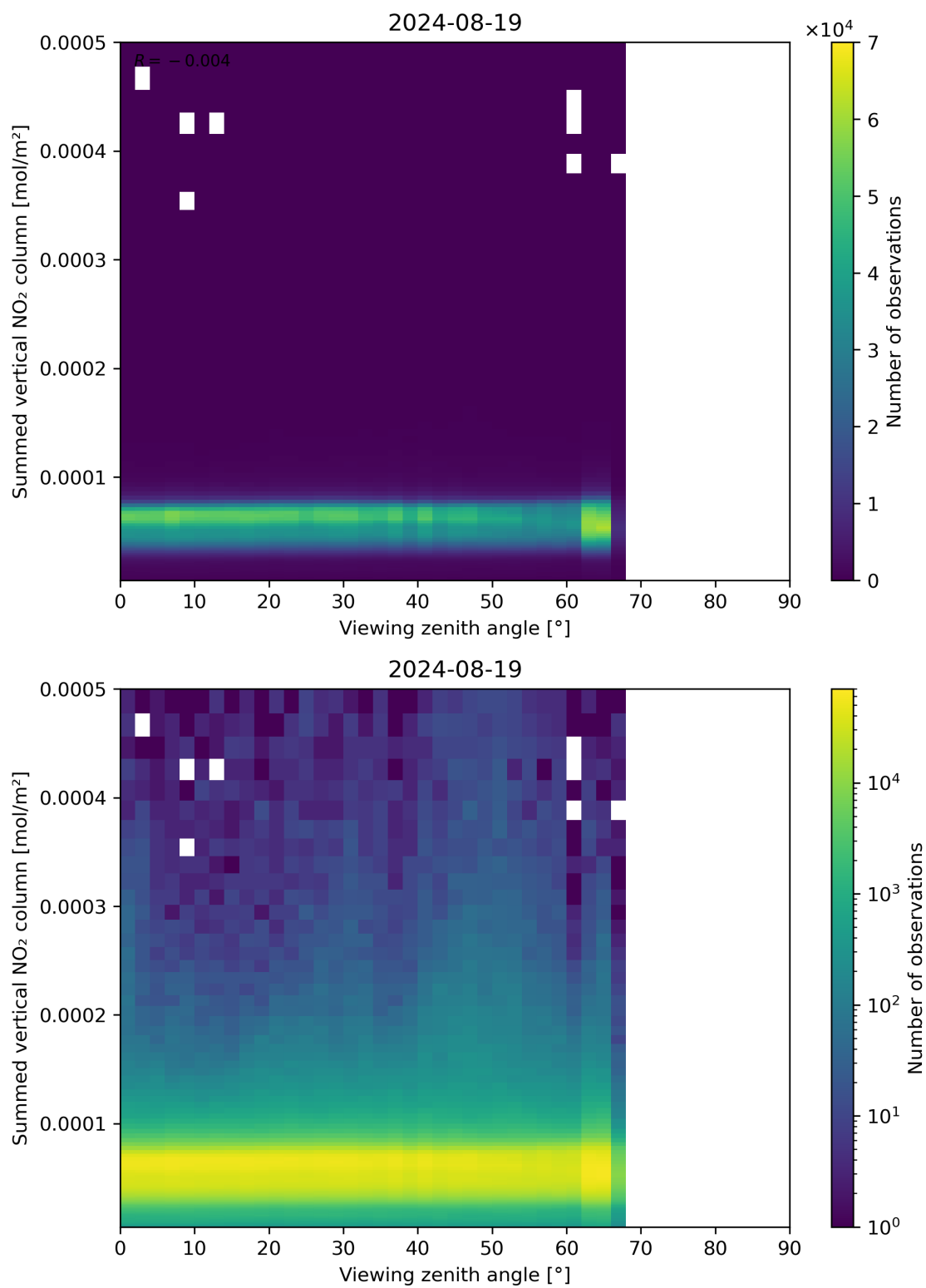
Figure 165: Scatter density plot of “Viewing zenith angle” against “Summed vertical NO 2 column” for 2024-08-18 to 2024-08-20.
