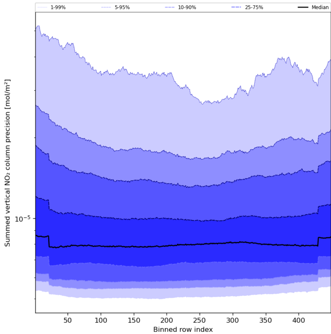
Figure 58: Along track statistics of “Summed vertical NO 2 column precision” for 2024-08-18 to 2024-08-20
