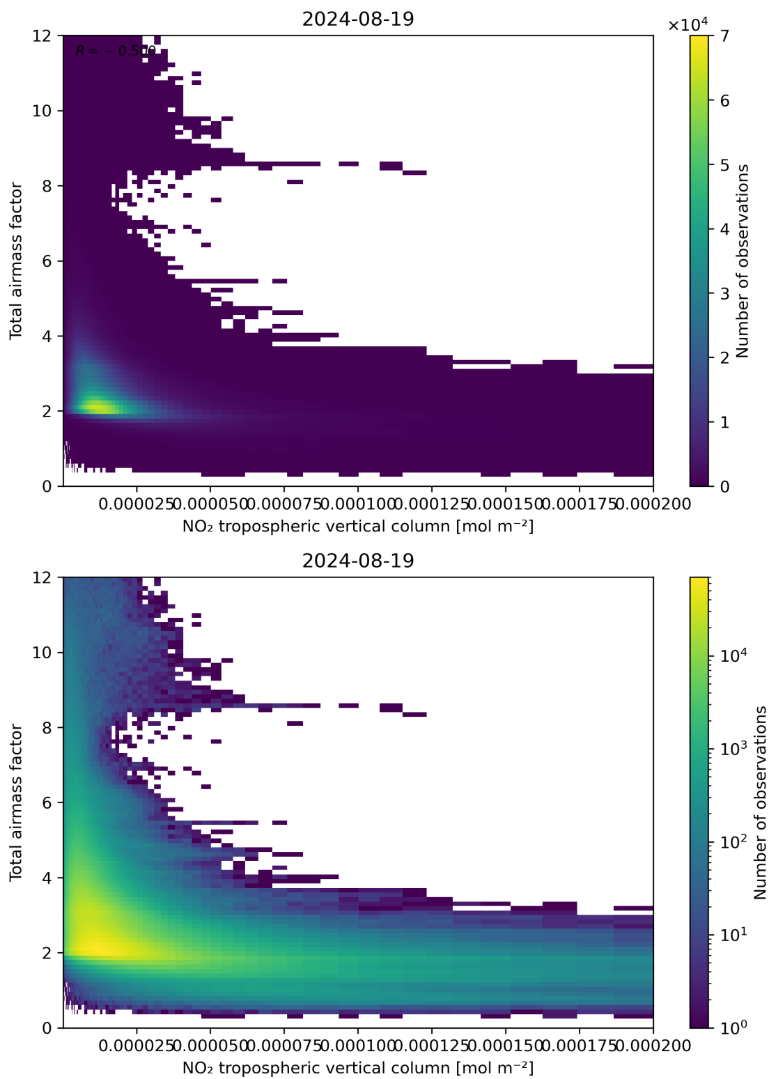
Figure 122: Scatter density plot of “NO 2 tropospheric vertical column” against “Total air mass factor” for 2024-08-18 to 2024-08-20.
