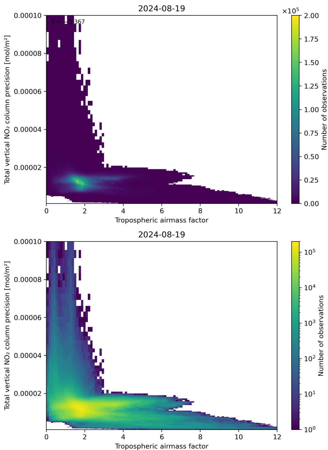
Figure 78: Scatter density plot of “Tropospheric air mass factor” against “Total vertical NO 2 column precision” for 2024-08-18 to 2024-08-20.
