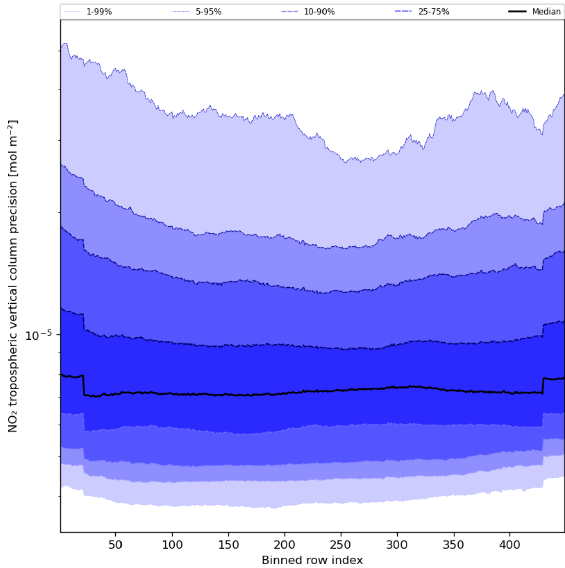
Figure 47: Along track statistics of “NO 2 tropospheric vertical column precision” for 2024-08-18 to 2024-08-20
