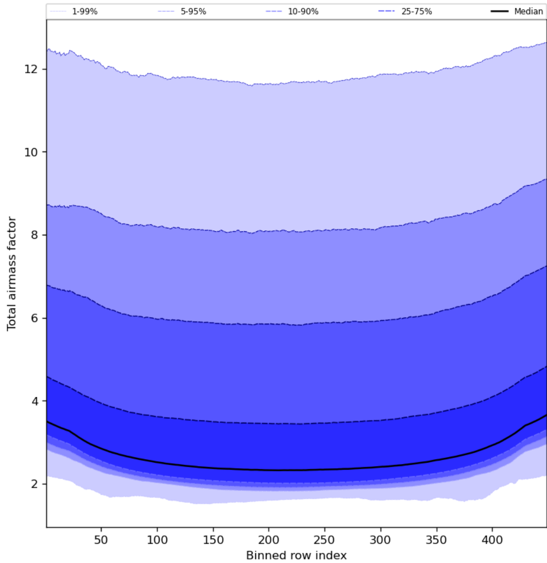
Figure 49: Along track statistics of “Total airmass factor” for 2024-08-18 to 2024-08-20
