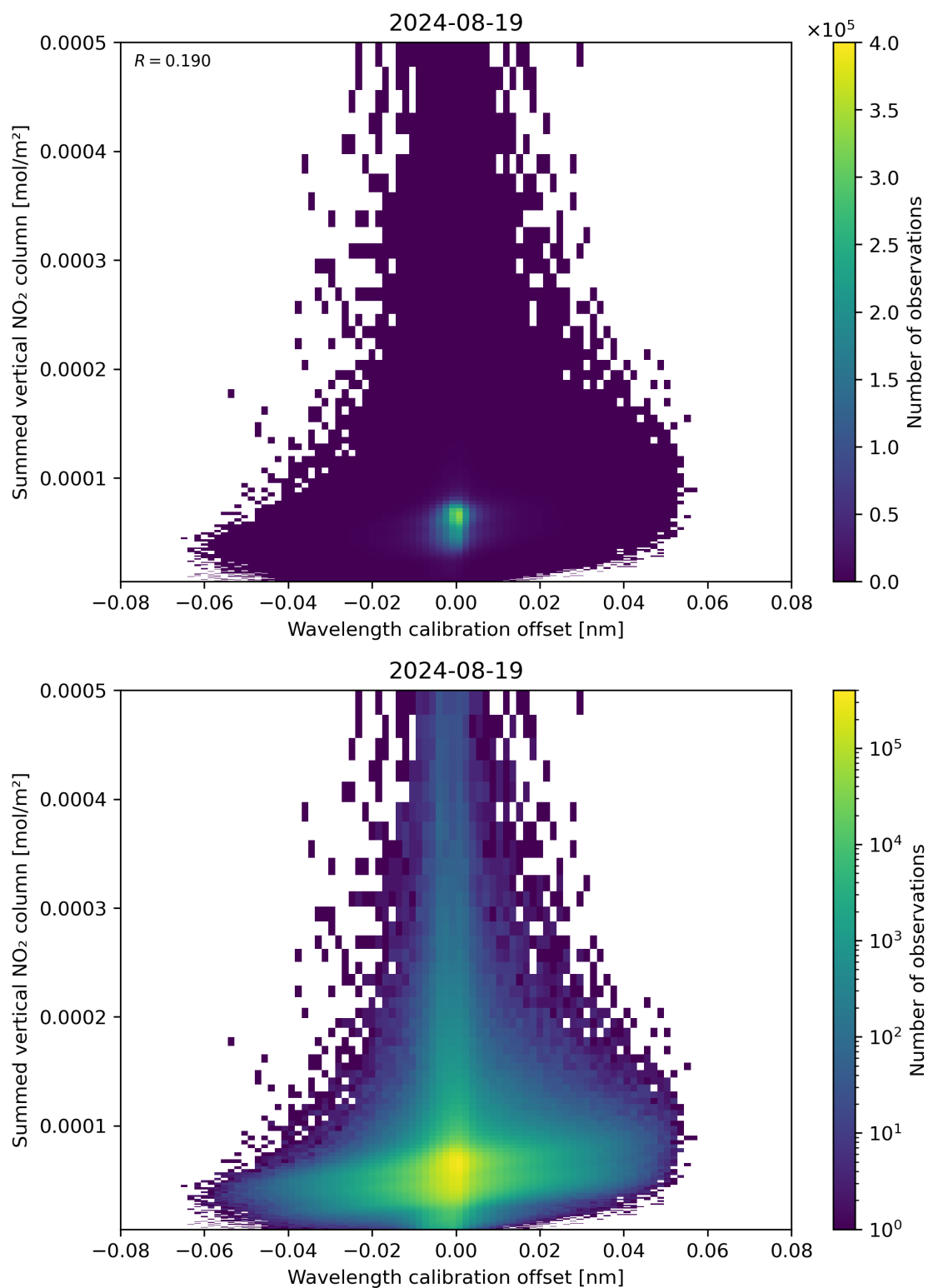
Figure 177: Scatter density plot of “Wavelength calibration offset” against “Summed vertical NO 2 column” for 2024-08-18 to 2024-08-20.
