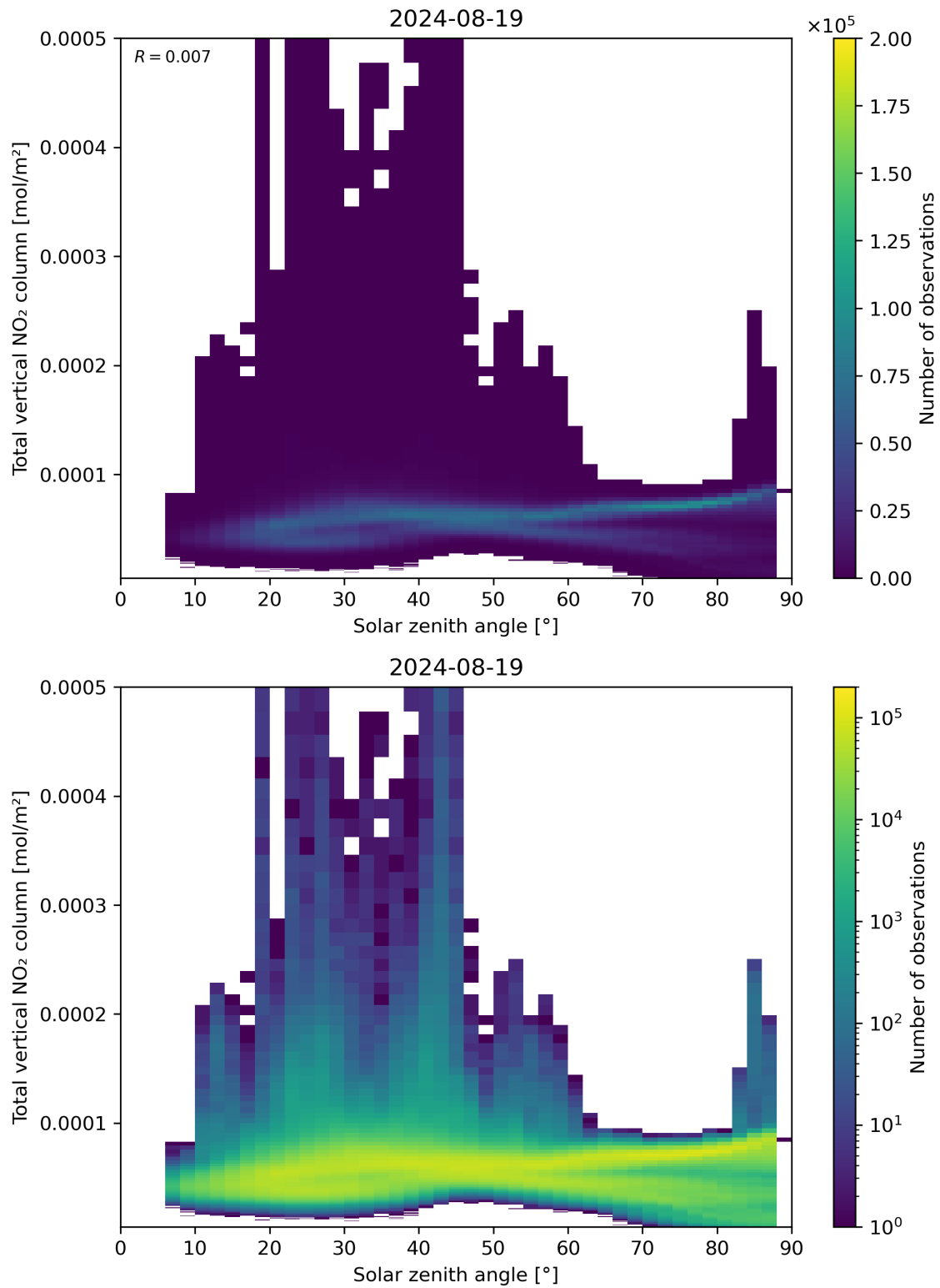
Figure 153: Scatter density plot of “Solar zenith angle” against “Total vertical NO 2 column” for 2024-08-18 to 2024-08-20.
