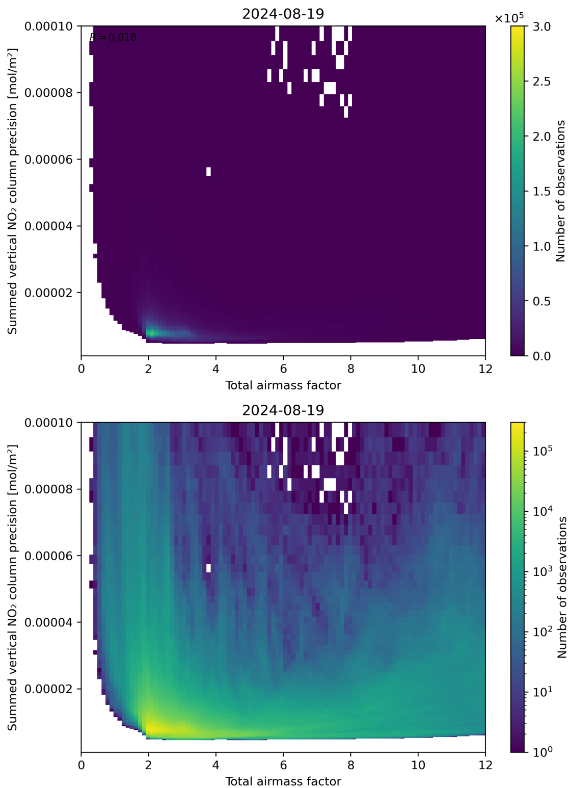
Figure 66: Scatter density plot of “Total airmass factor” against “Summed vertical NO 2 column precision” for 2024-08-18 to 2024-08-20.
