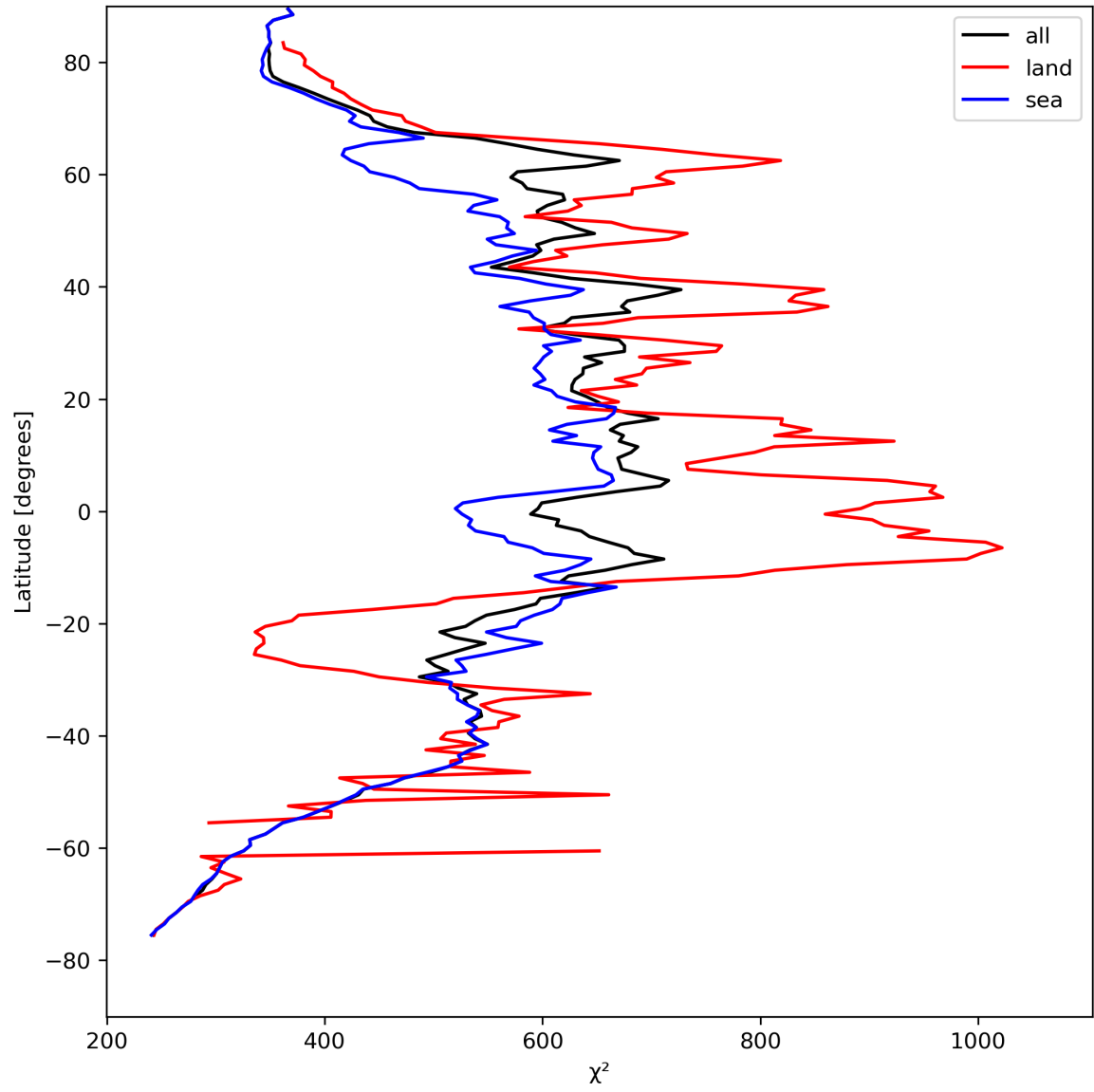
Figure 25: Zonal average of “ \chi^2 ” for 2024-08-18 to 2024-08-20.
