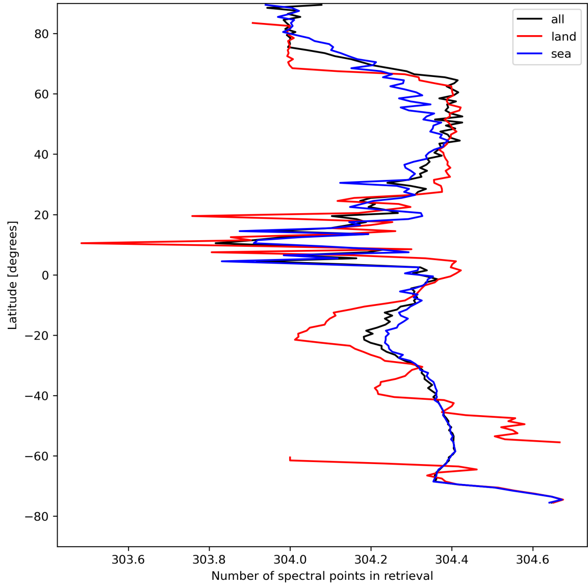
Figure 16: Zonal average of “Number of spectral points in retrieval” for 2024-08-18 to 2024-08-20.
