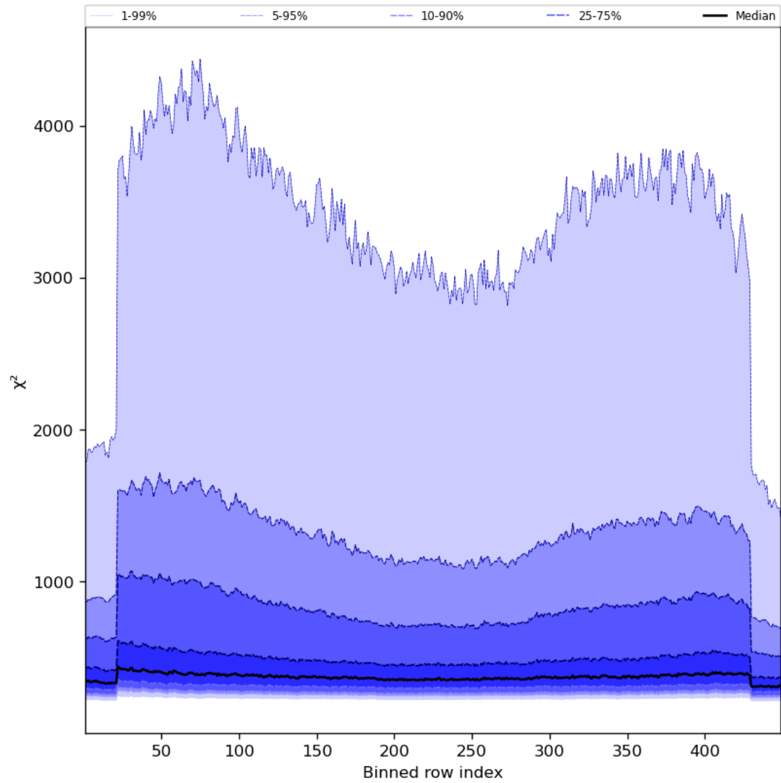
Figure 59: Along track statistics of “ \chi^2 ” for 2024-08-18 to 2024-08-20
