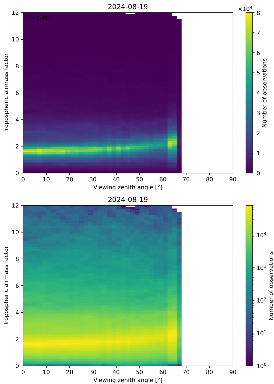
Figure 161: Scatter density plot of “Viewing zenith angle” against “Tropospheric airmass factor” for 2024-08-18 to 2024-08-20.
