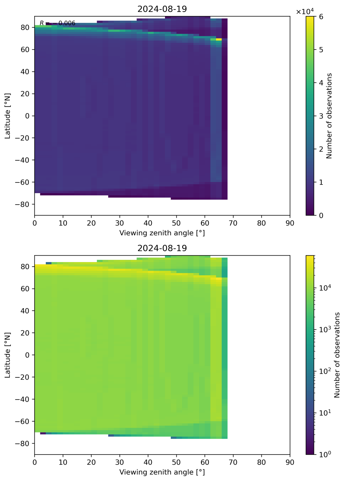
Figure 163: Scatter density plot of “Viewing zenith angle” against “Latitude” for 2024-08-18 to 2024-08-20.
