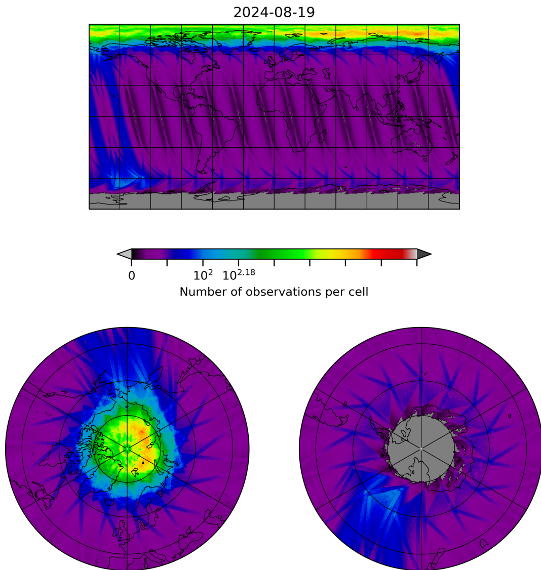
Figure 10: Map of the number of observations for 2024-08-18 to 2024-08-20
