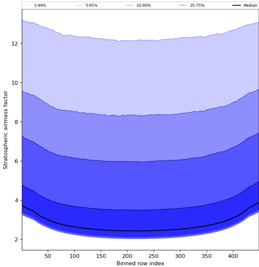
Figure 61: Along track statistics of “Stratospheric airmass factor” for 2024-08-18 to 2024-08-20
