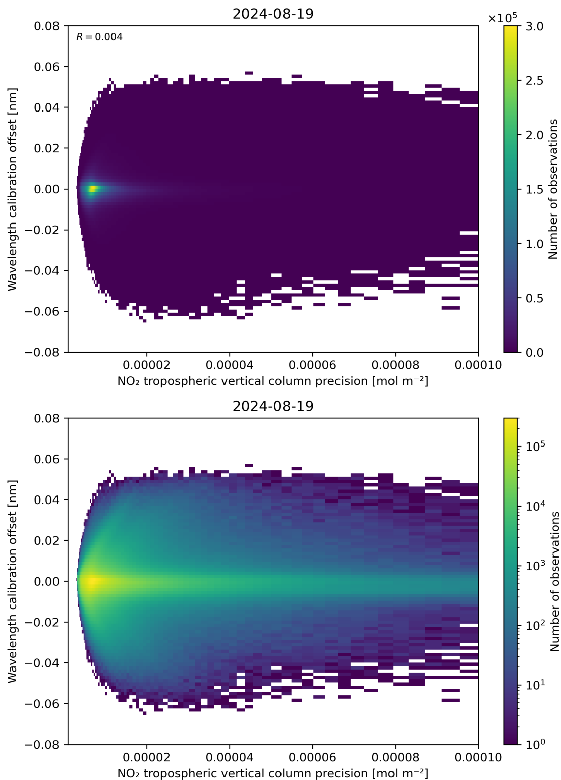
Figure 141: Scatter density plot of “NO 2 tropospheric vertical column precision” against “Wavelength calibration offset” for 2024-08-18 to 2024-08-20.
