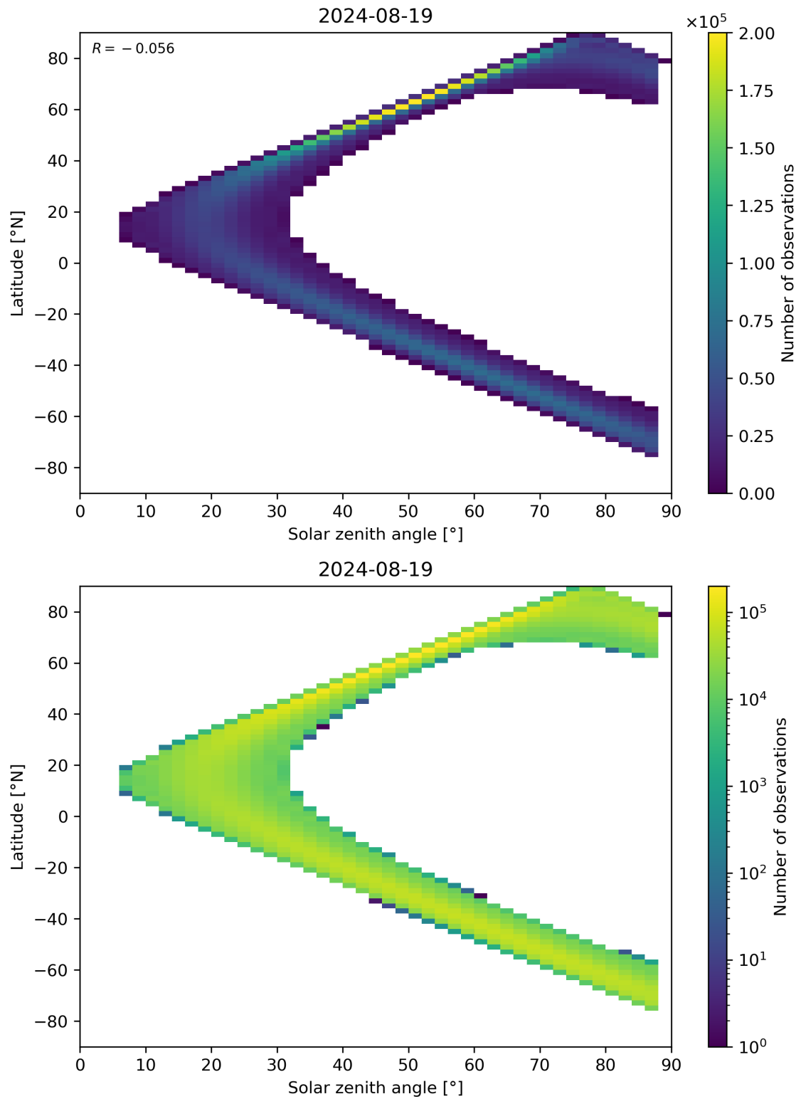
Figure 149: Scatter density plot of “Solar zenith angle” against “Latitude” for 2024-08-18 to 2024-08-20.
