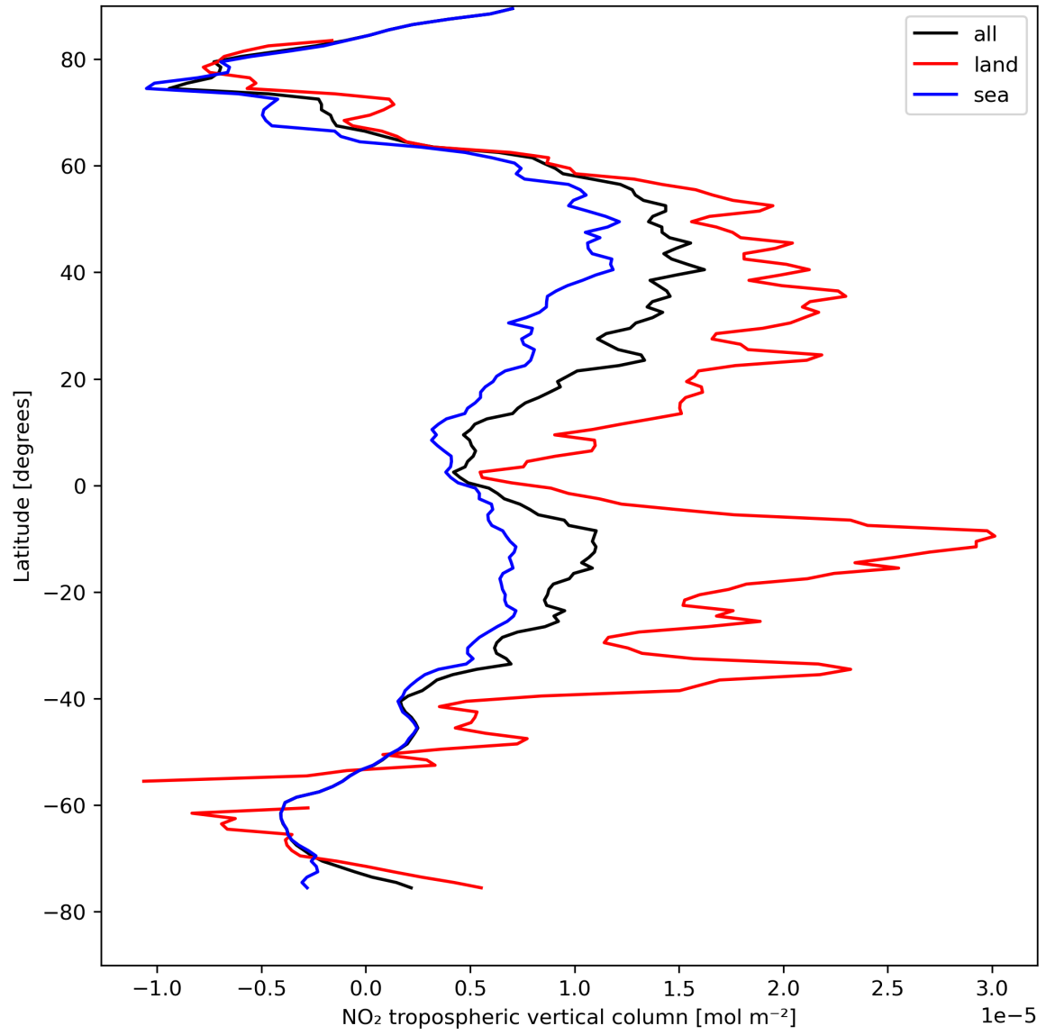
Figure 12: Zonal average of “NO 2 tropospheric vertical column” for 2024-08-18 to 2024-08-20.
