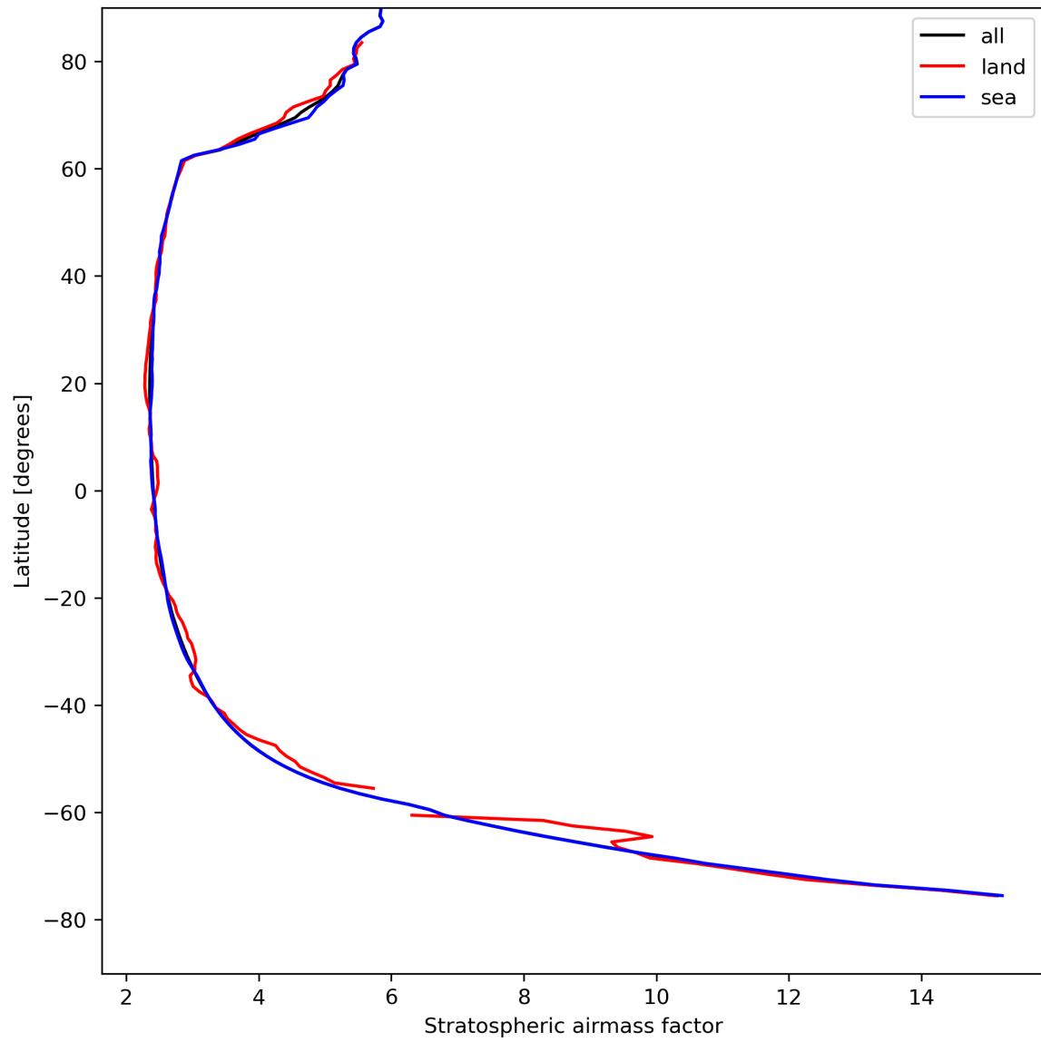
Figure 27: Zonal average of “Stratospheric airmass factor” for 2024-08-18 to 2024-08-20.
