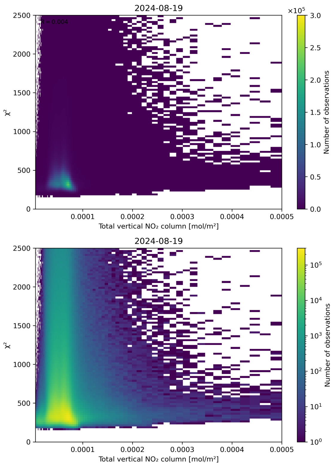
Figure 111: Scatter density plot of “Total vertical NO 2 column” against “ \chi^2 ” for 2024-08-18 to 2024-08-20.
