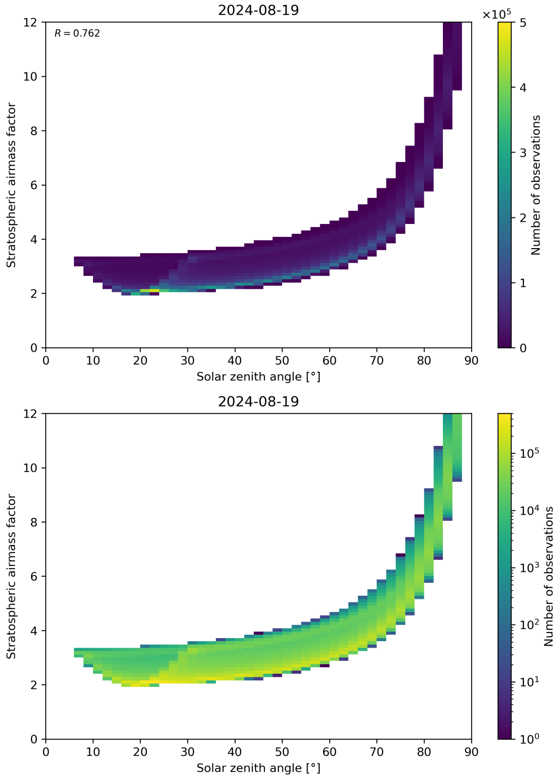
Figure 145: Scatter density plot of “Solar zenith angle” against “Stratospheric airmass factor” for 2024-08-18 to 2024-08-20.
