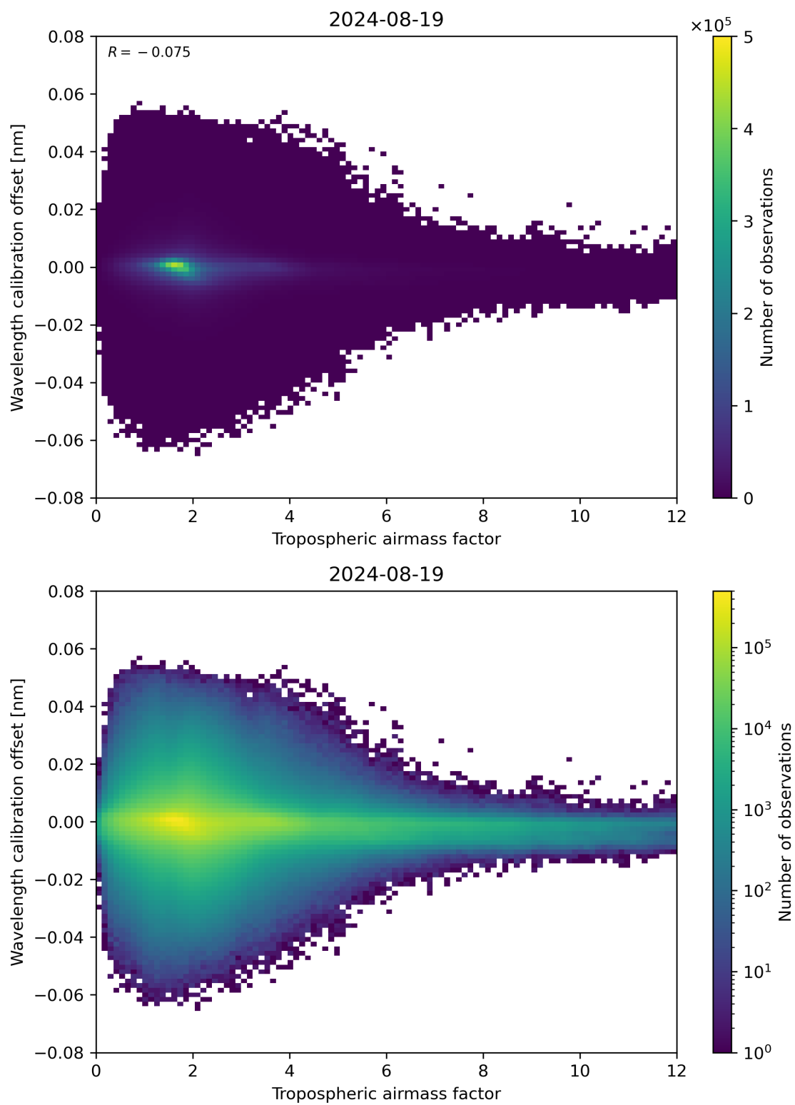
Figure 80: Scatter density plot of “Tropospheric airmass factor” against “Wavelength calibration offset” for 2024-08-18 to 2024-08-20.
