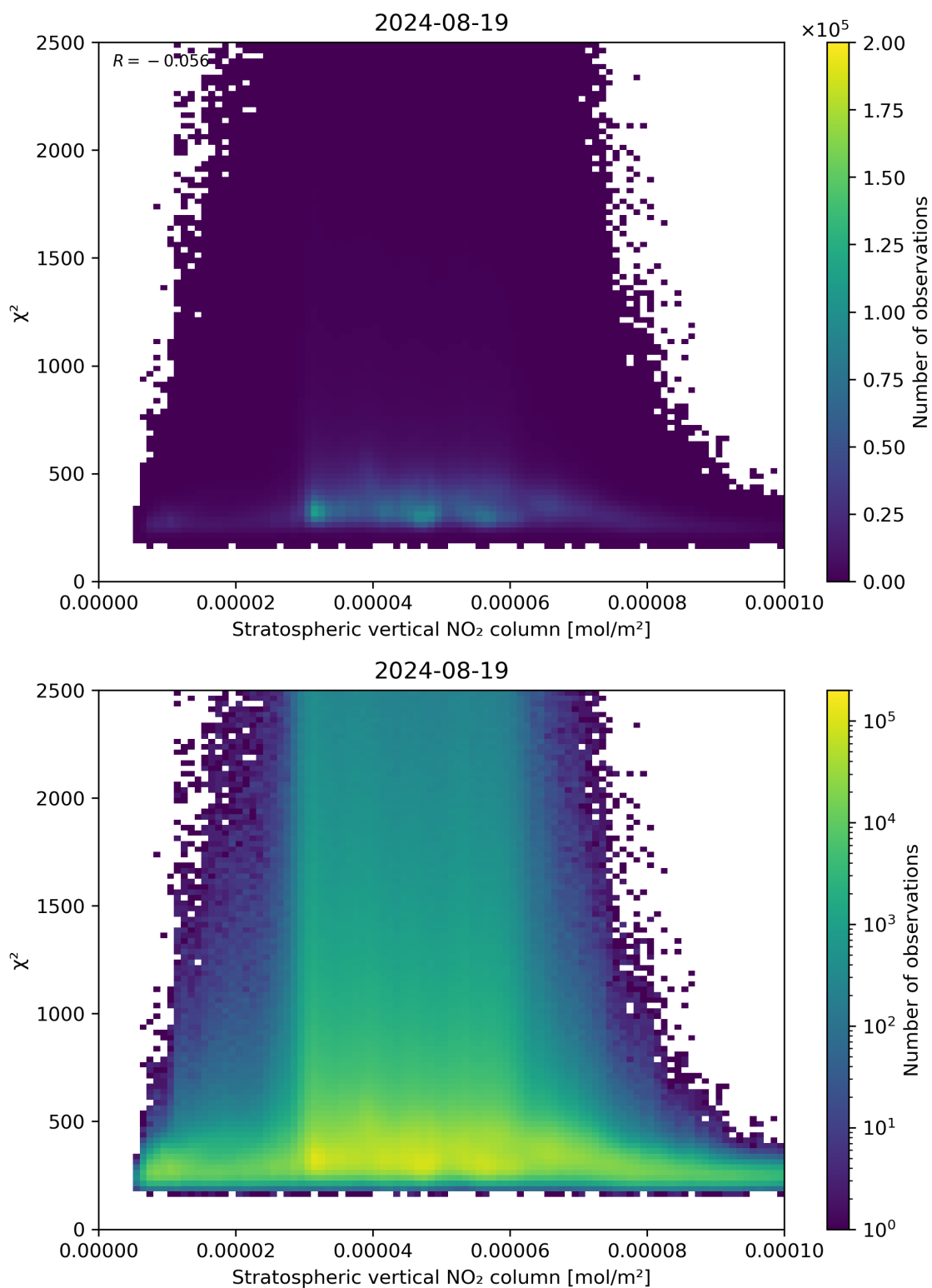
Figure 97: Scatter density plot of “Stratospheric vertical NO 2 column” against “ \chi^2 ” for 2024-08-18 to 2024-08-20.
