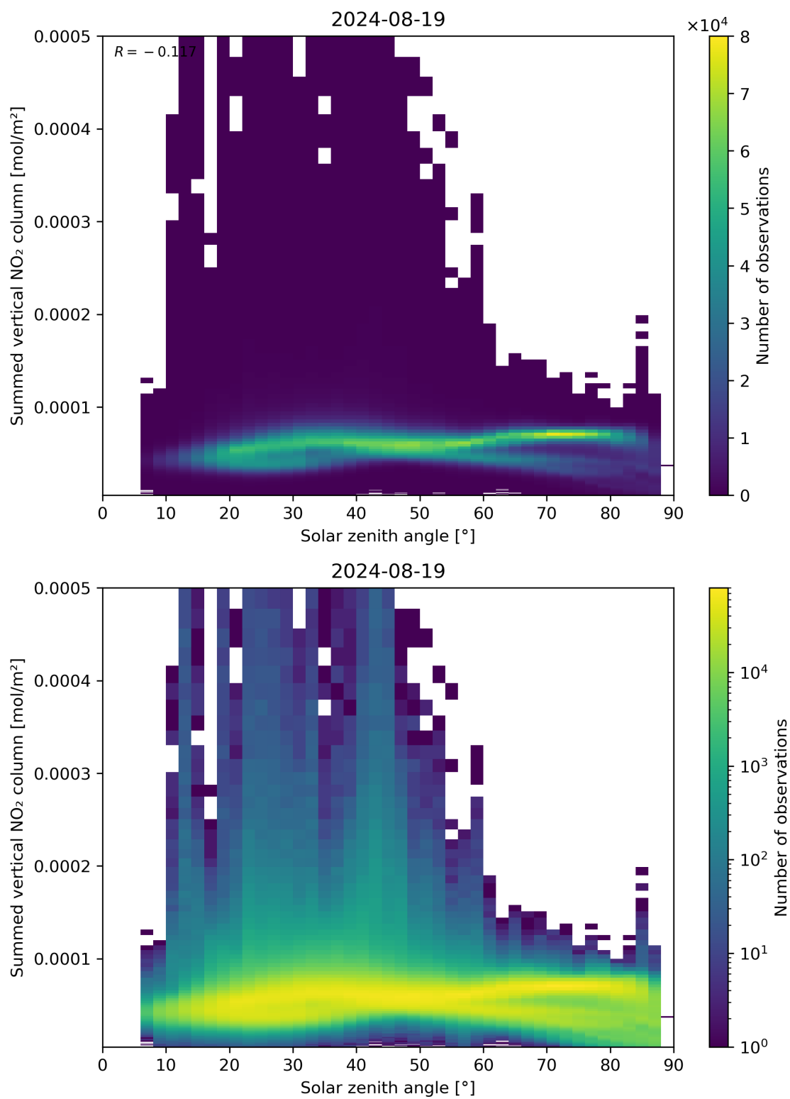
Figure 151: Scatter density plot of “Solar zenith angle” against “Summed vertical NO 2 column” for 2024-08-18 to 2024-08-20.
