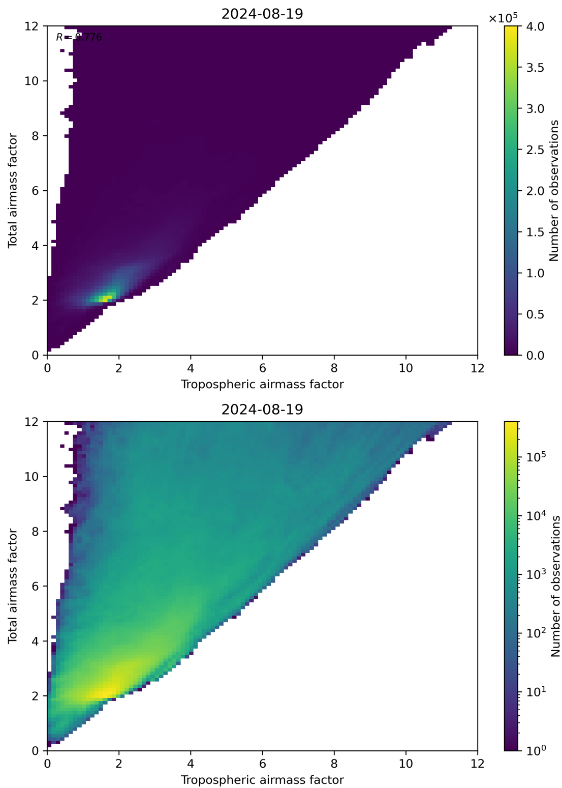
Figure 72: Scatter density plot of “Tropospheric airmass factor” against “Total airmass factor” for 2024-08-18 to 2024-08-20.
