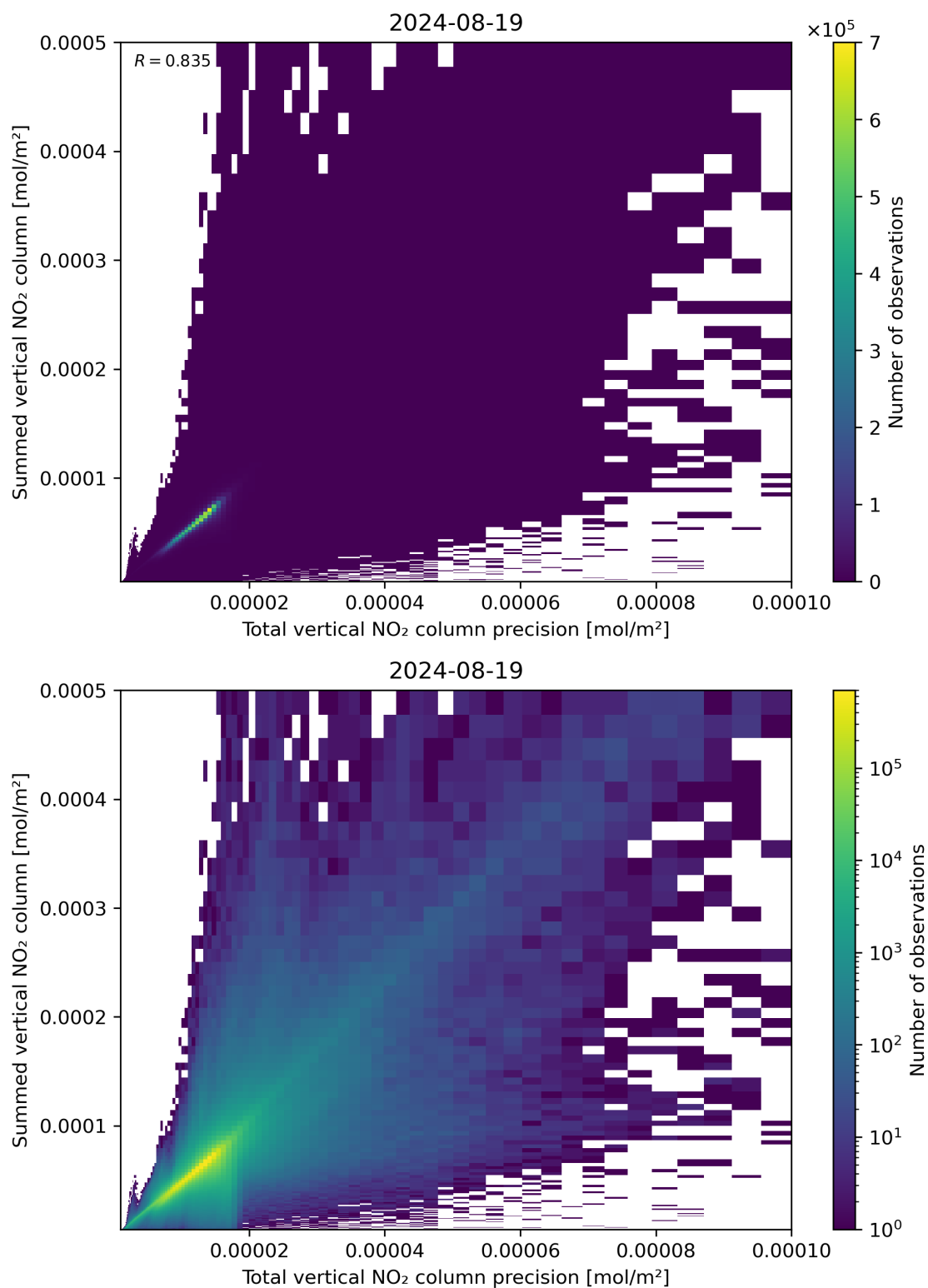
Figure 117: Scatter density plot of “Total vertical NO 2 column precision” against “Summed vertical NO 2 column” for 2024-08-18 to 2024-08-20.
