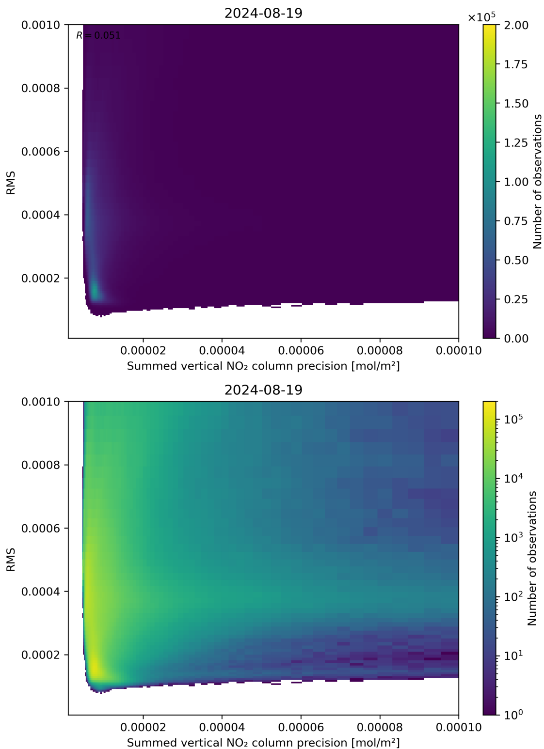
Figure 108: Scatter density plot of “Summed vertical NO 2 column precision” against “RMS” for 2024-08-18 to 2024-08-20.
