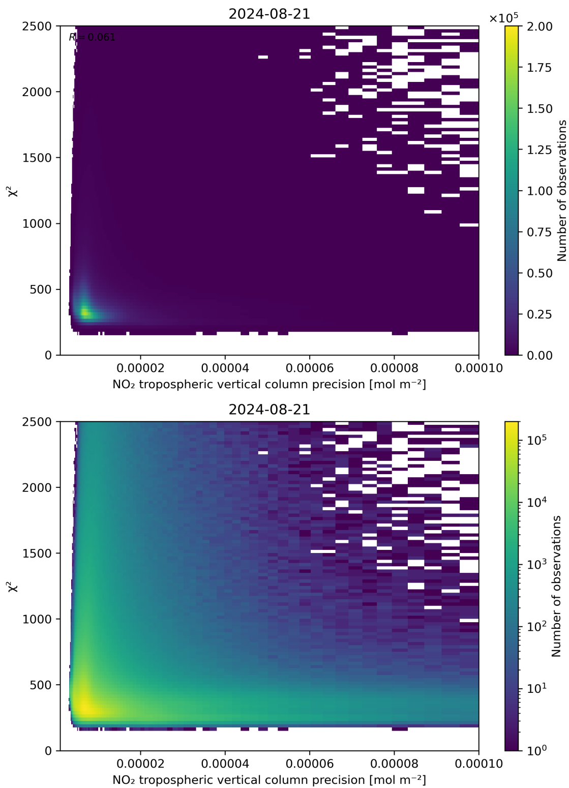
Figure 134: Scatter density plot of “NO 2 tropospheric vertical column precision” against “ \chi^2 ” for 2024-08-21 to 2024-08-22.
