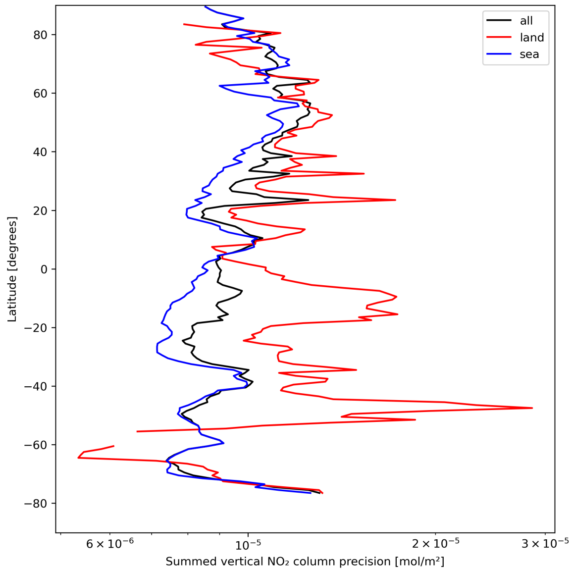
Figure 24: Zonal average of “Summed vertical NO 2 column precision” for 2024-08-21 to 2024-08-22.
