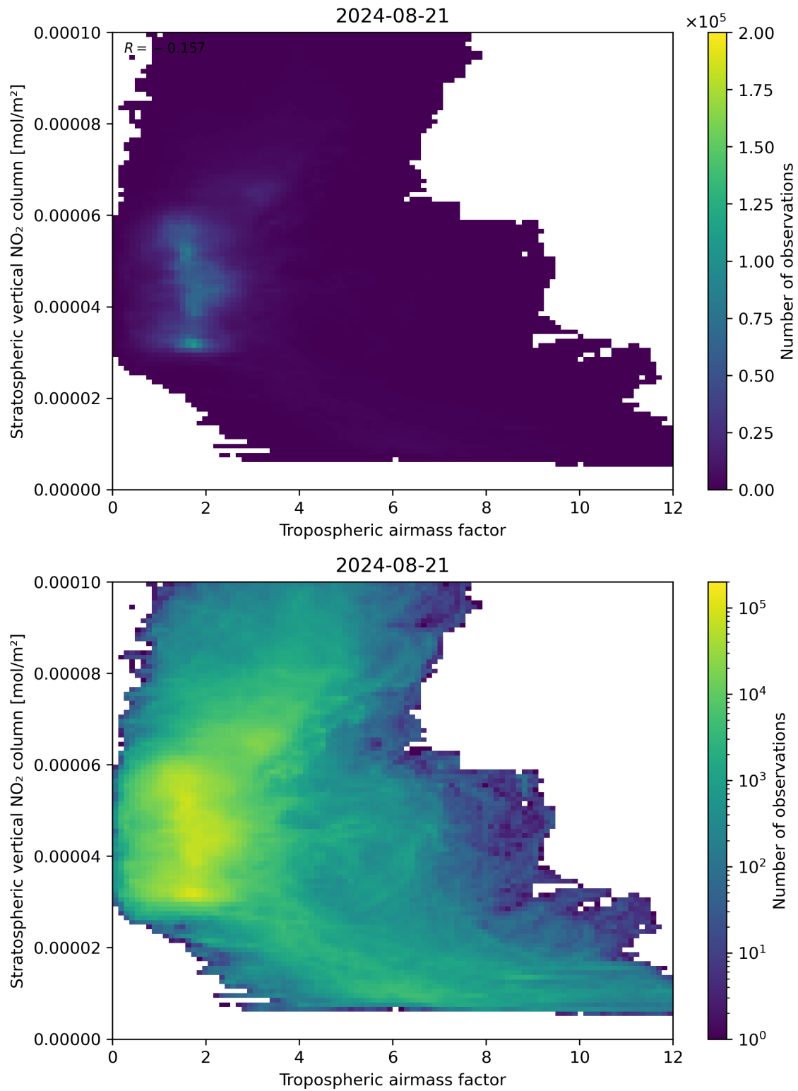
Figure 74: Scatter density plot of “Tropospheric air mass factor” against “Stratospheric vertical NO 2 column” for 2024-08-21 to 2024-08-22.
