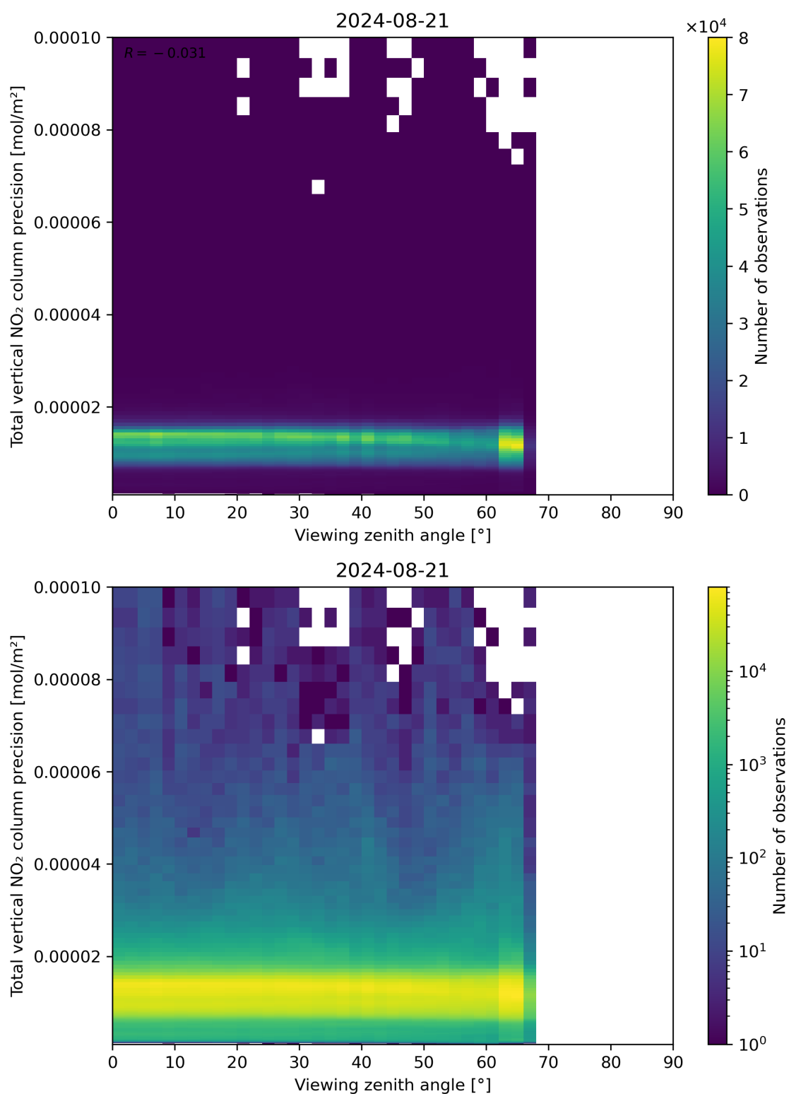
Figure 168: Scatter density plot of “Viewing zenith angle” against “Total vertical NO 2 column precision” for 2024-08-21 to 2024-08-22.
