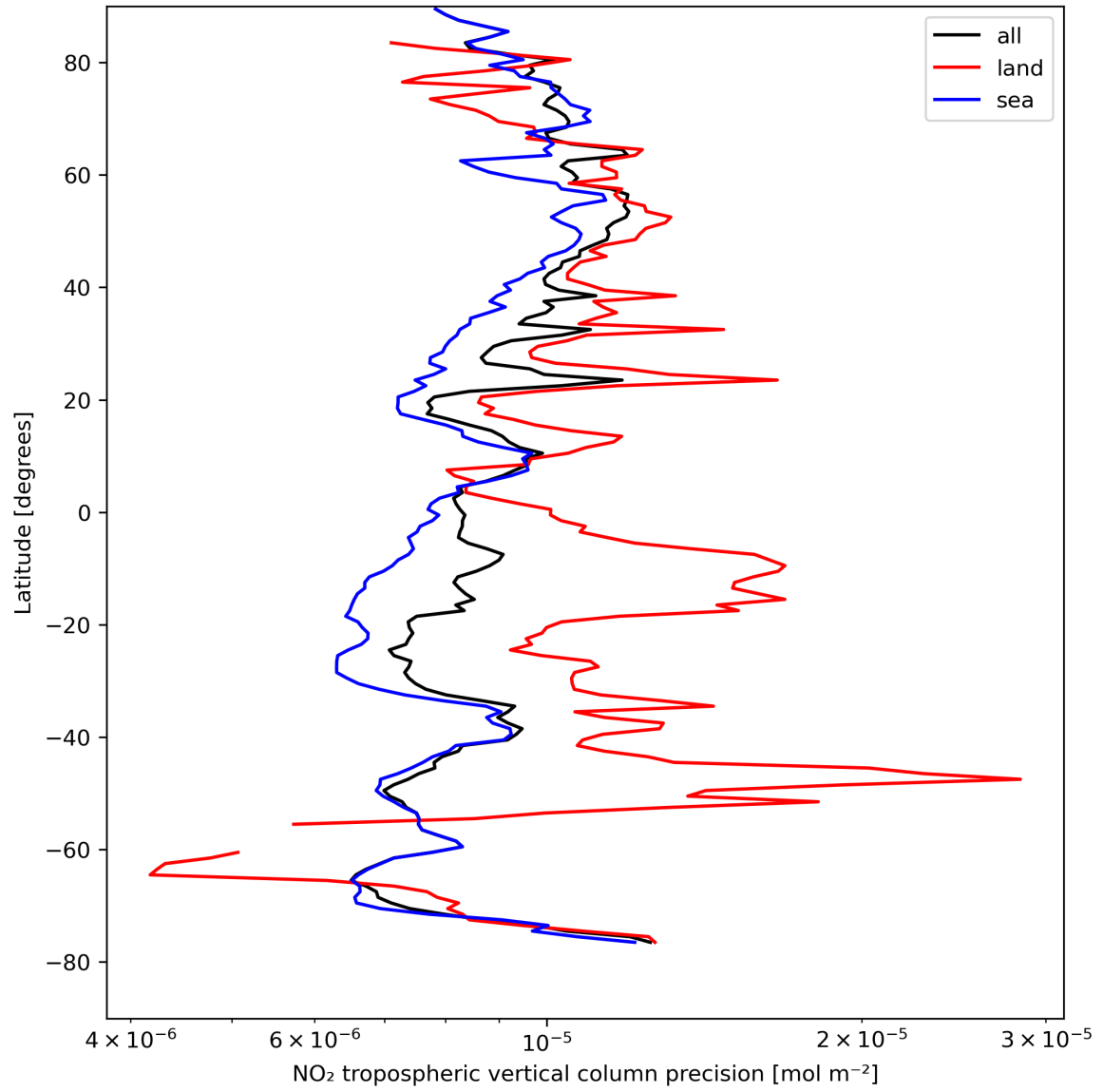
Figure 13: Zonal average of “NO 2 tropospheric vertical column precision” for 2024-08-21 to 2024-08-22.
