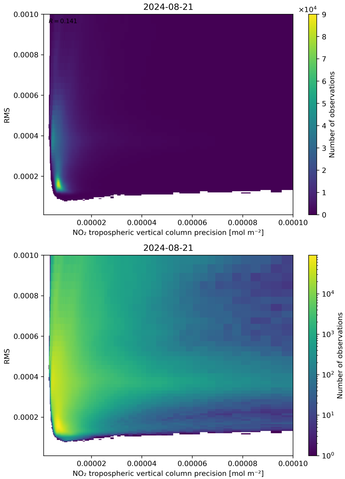
Figure 140: Scatter density plot of “NO 2 tropospheric vertical column precision” against “RMS” for 2024-08-21 to 2024-08-22.
