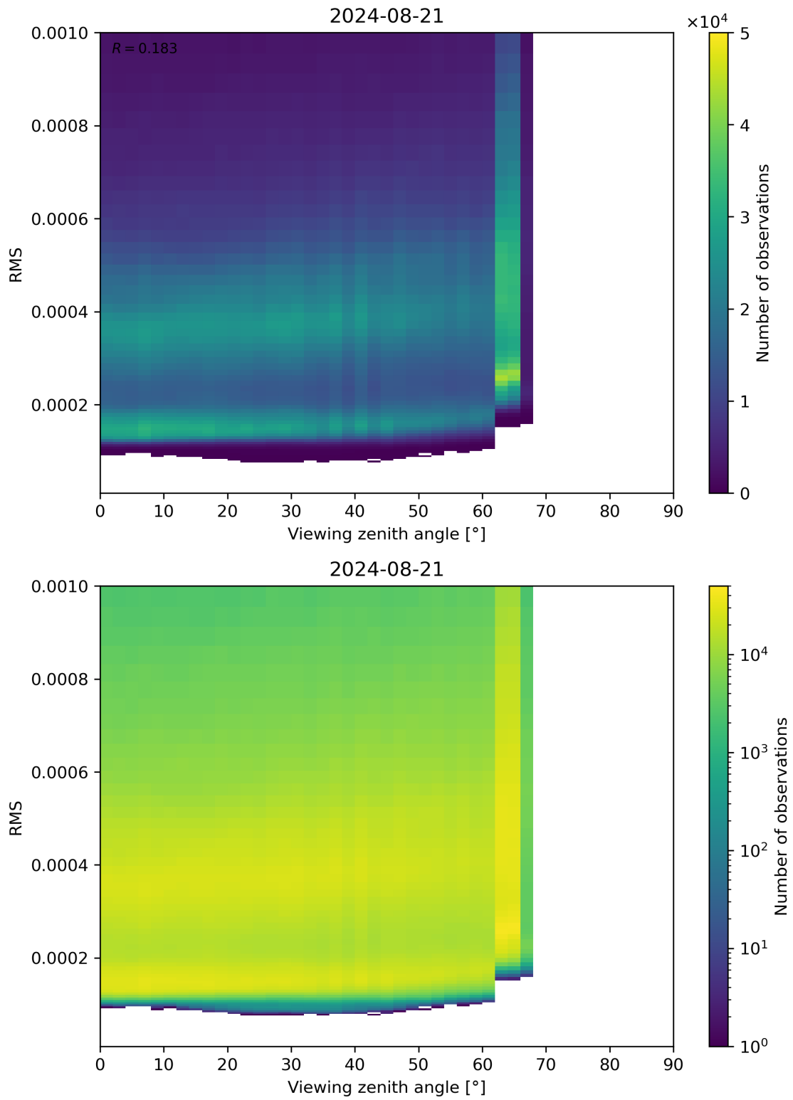
Figure 171: Scatter density plot of “Viewing zenith angle” against “RMS” for 2024-08-21 to 2024-08-22.
