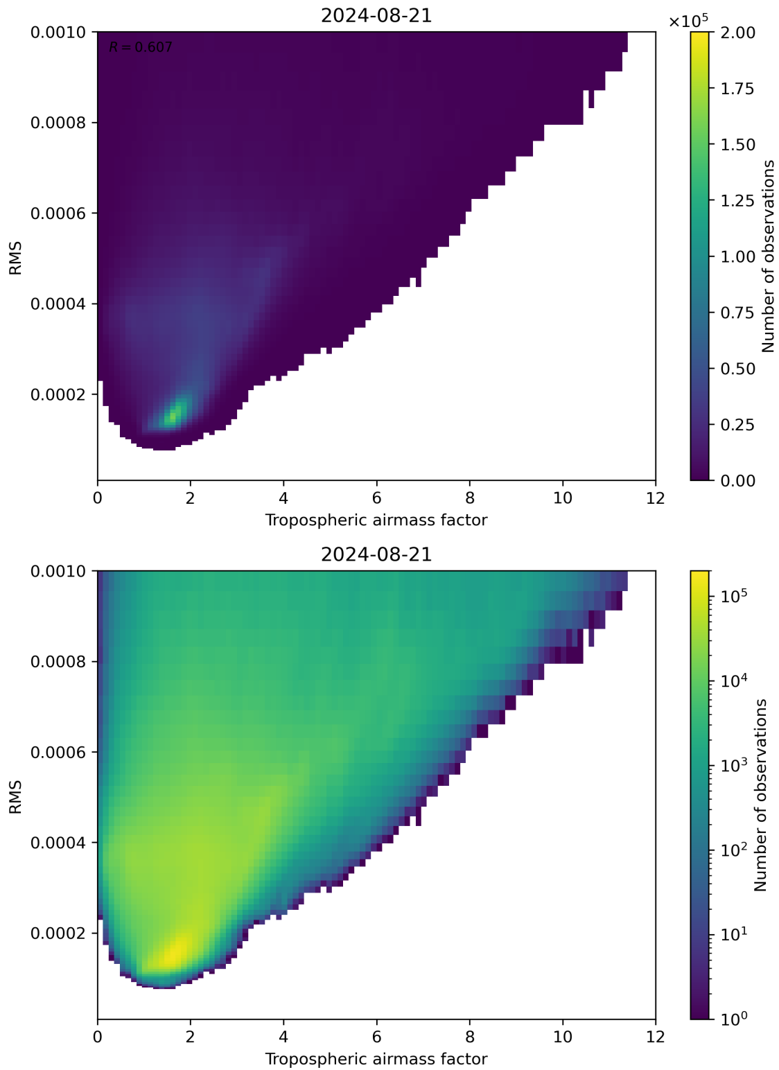
Figure 79: Scatter density plot of “Tropospheric airmass factor” against “RMS” for 2024-08-21 to 2024-08-22.
