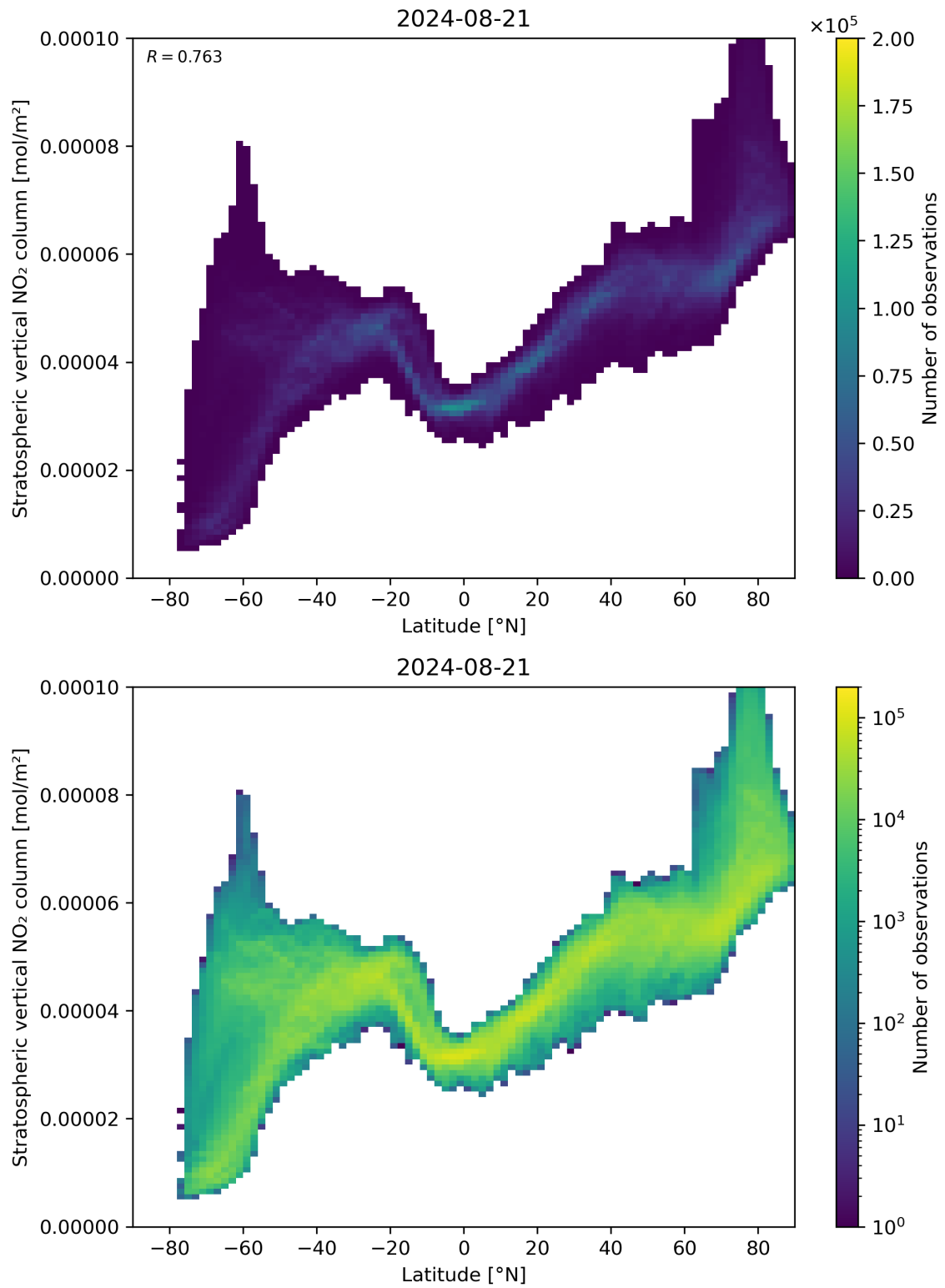
Figure 87: Scatter density plot of “Latitude” against “Stratospheric vertical NO 2 column” for 2024-08-21 to 2024-08-22.
