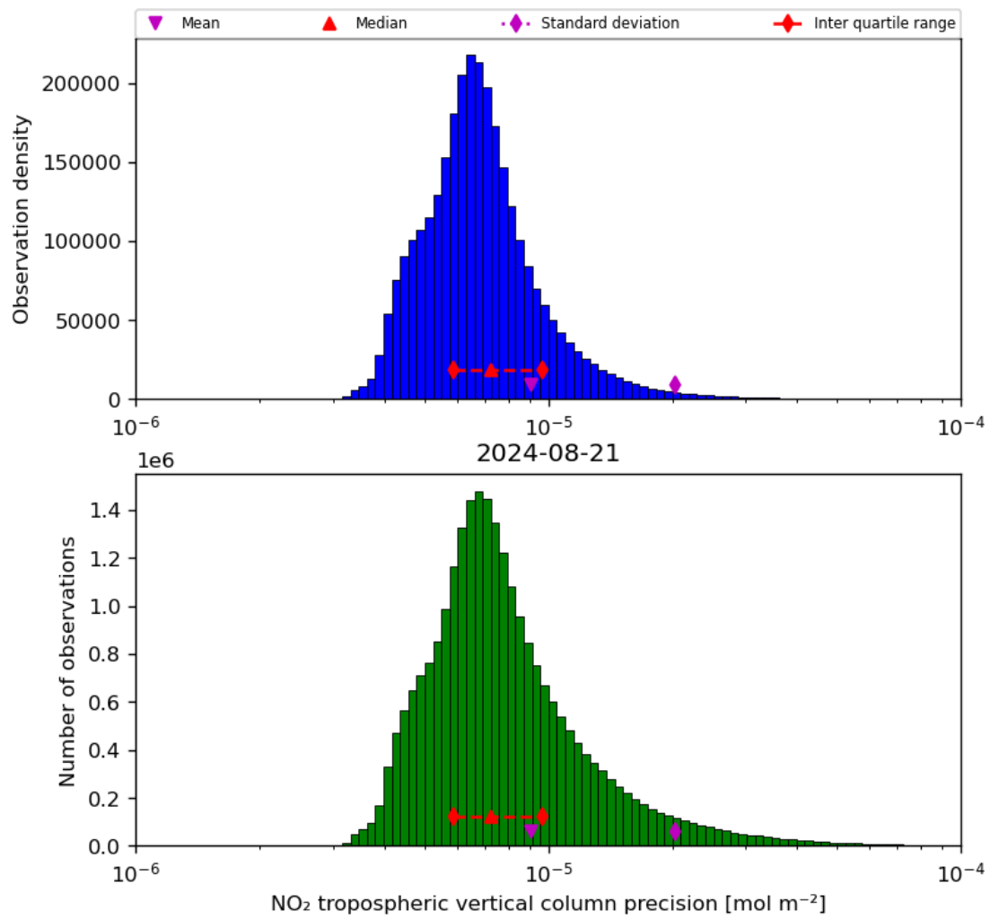
Figure 30: Histogram of “NO 2 tropospheric vertical column precision” for 2024-08-21 to 2024-08-22
