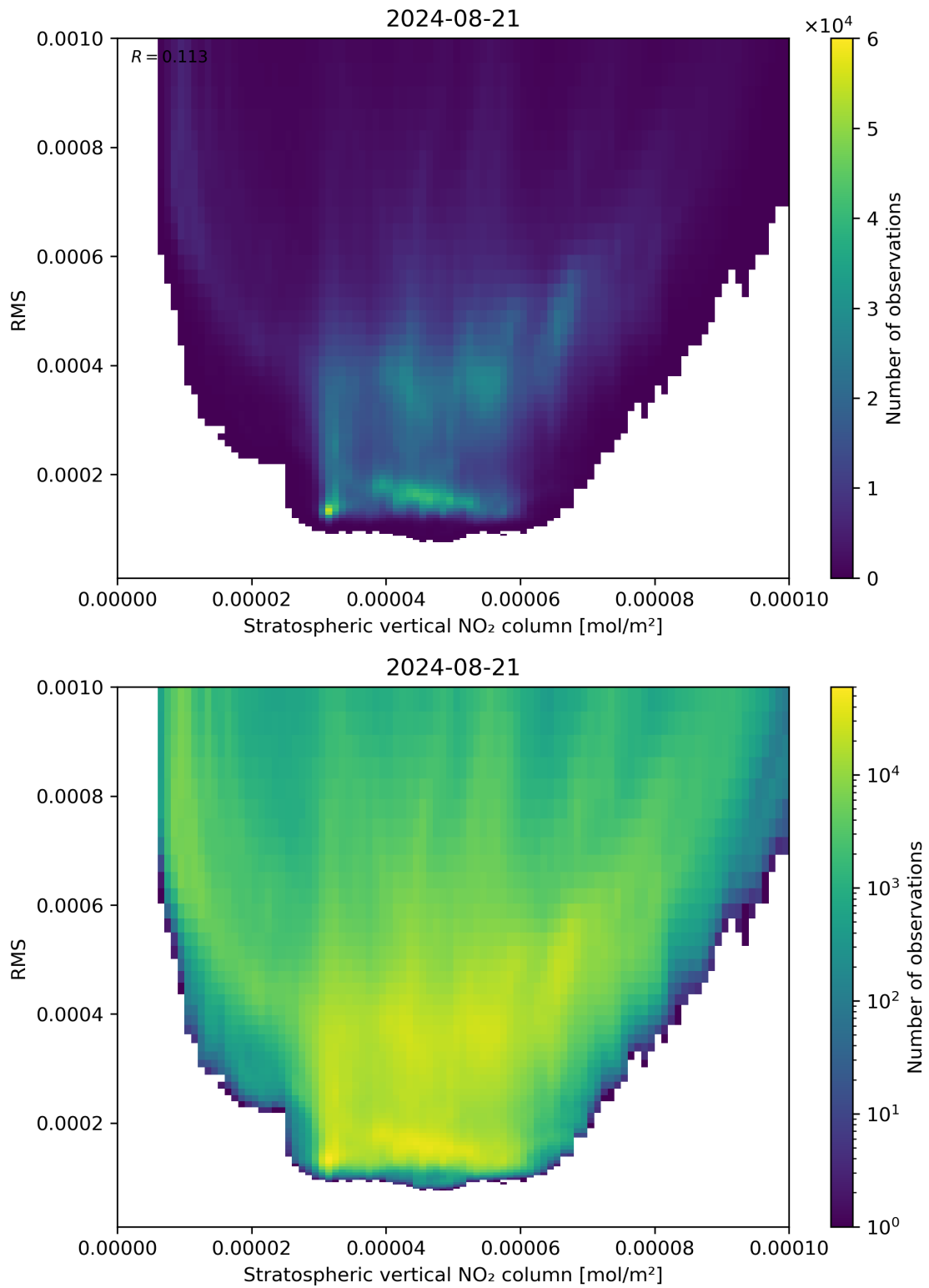
Figure 102: Scatter density plot of “Stratospheric vertical NO 2 column” against “RMS” for 2024-08-21 to 2024-08-22.
