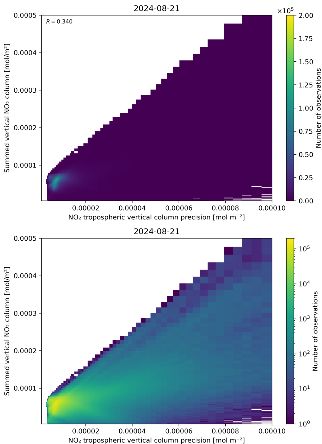
Figure 136: Scatter density plot of “NO 2 tropospheric vertical column precision” against “Summed vertical NO 2 column” for 2024-08-21 to 2024-08-22.
