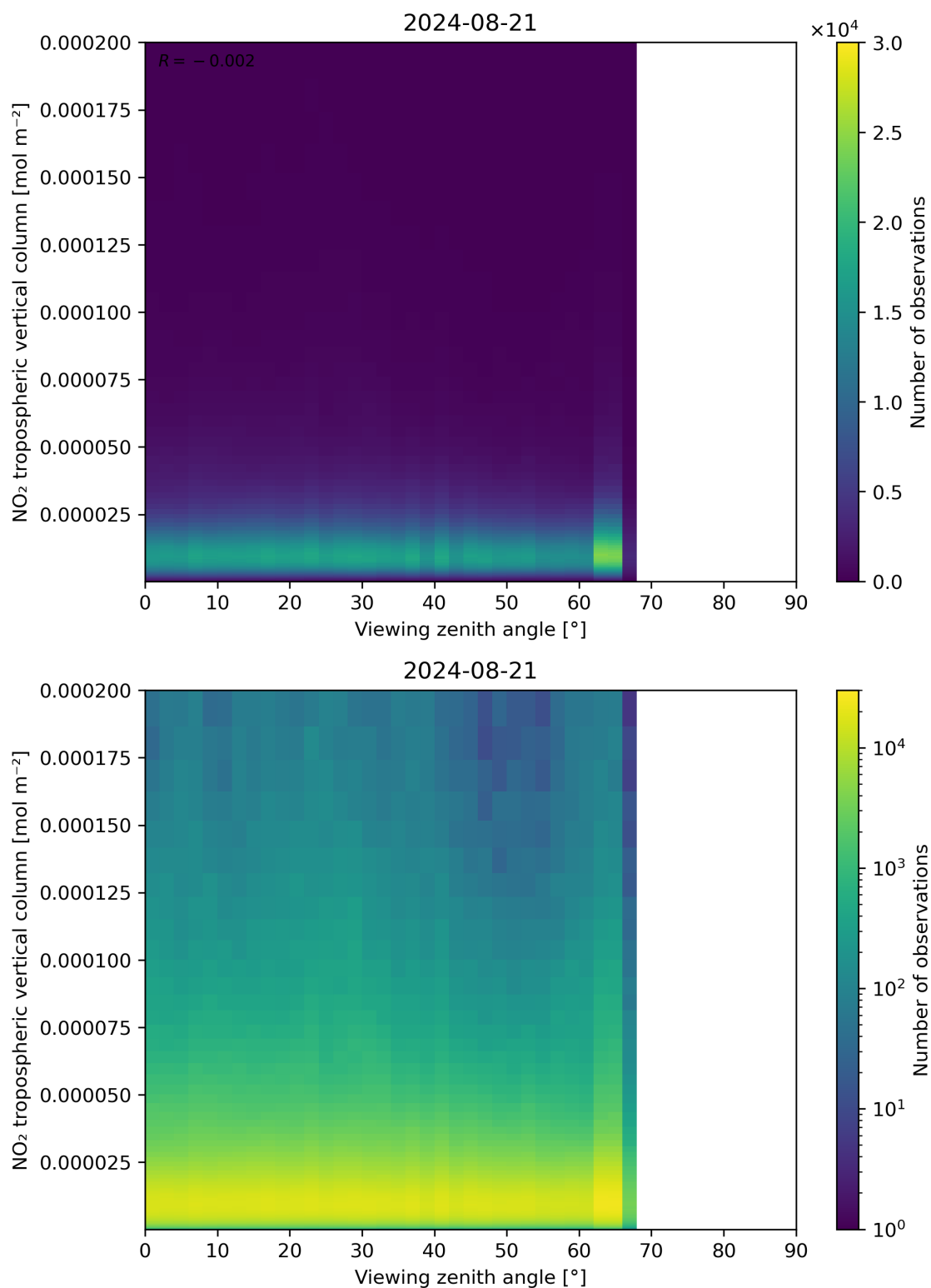
Figure 169: Scatter density plot of “Viewing zenith angle” against “NO 2 tropospheric vertical column” for 2024-08-21 to 2024-08-22.
