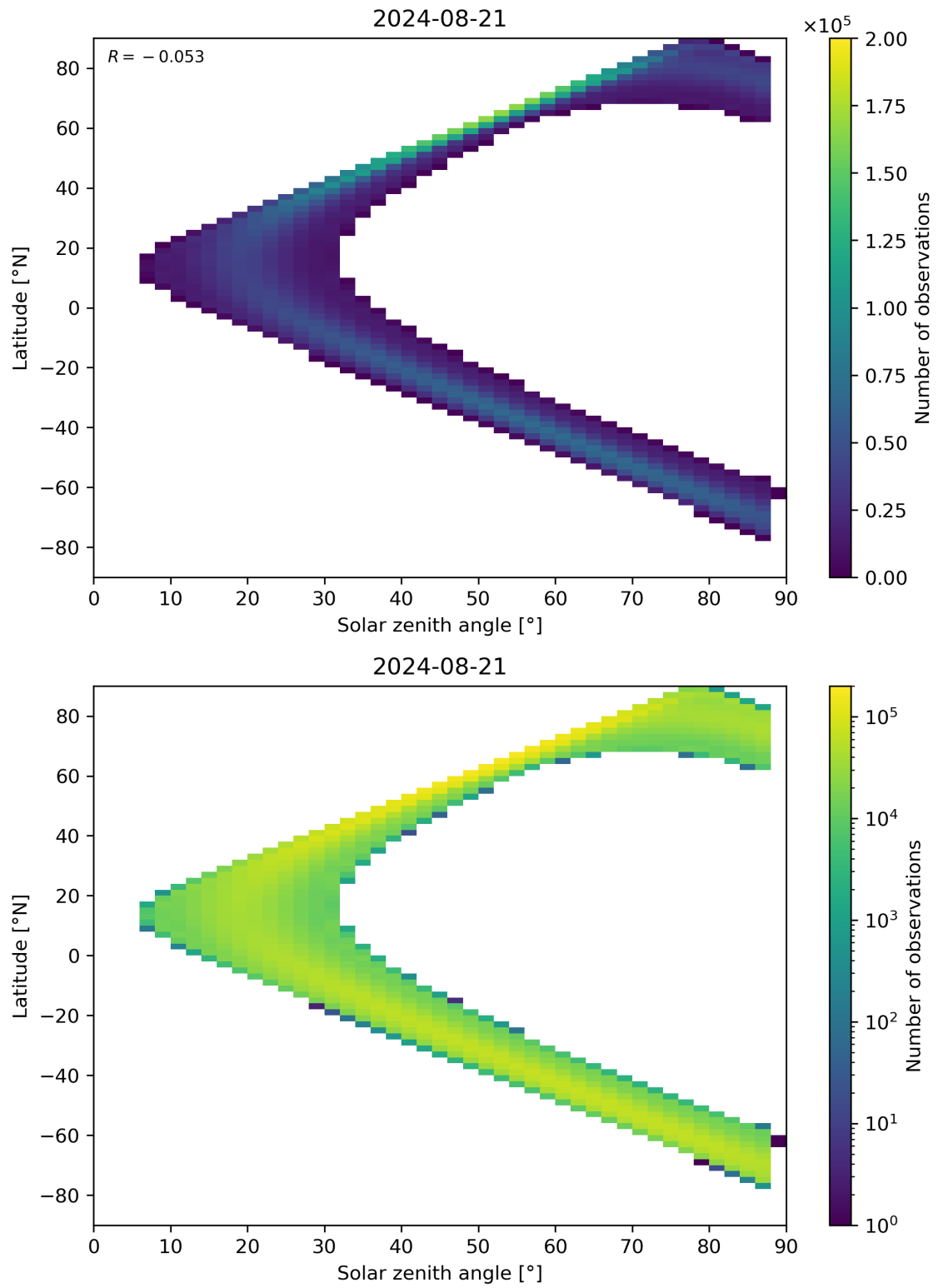
Figure 149: Scatter density plot of “Solar zenith angle” against “Latitude” for 2024-08-21 to 2024-08-22.
