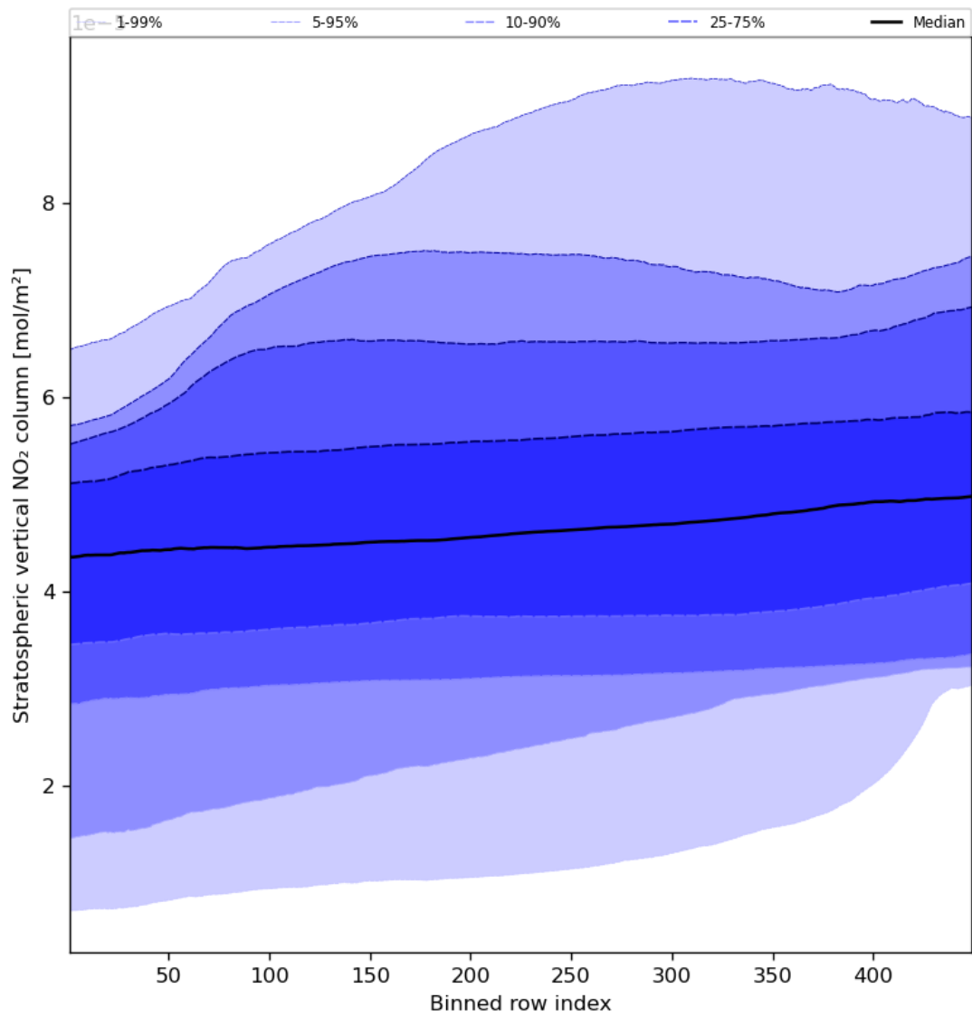
Figure 53: Along track statistics of “Stratospheric vertical NO 2 column” for 2024-08-21 to 2024-08-22
