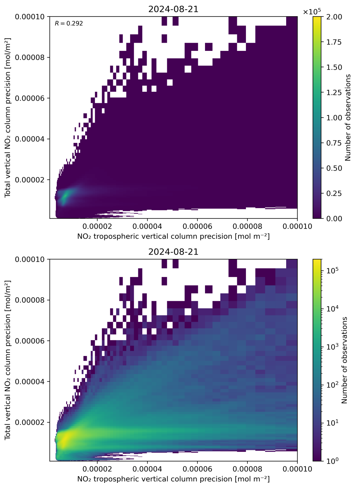
Figure 139: Scatter density plot of “NO 2 tropospheric vertical column precision” against “Total vertical NO 2 column precision” for 2024-08-21 to 2024-08-22.
