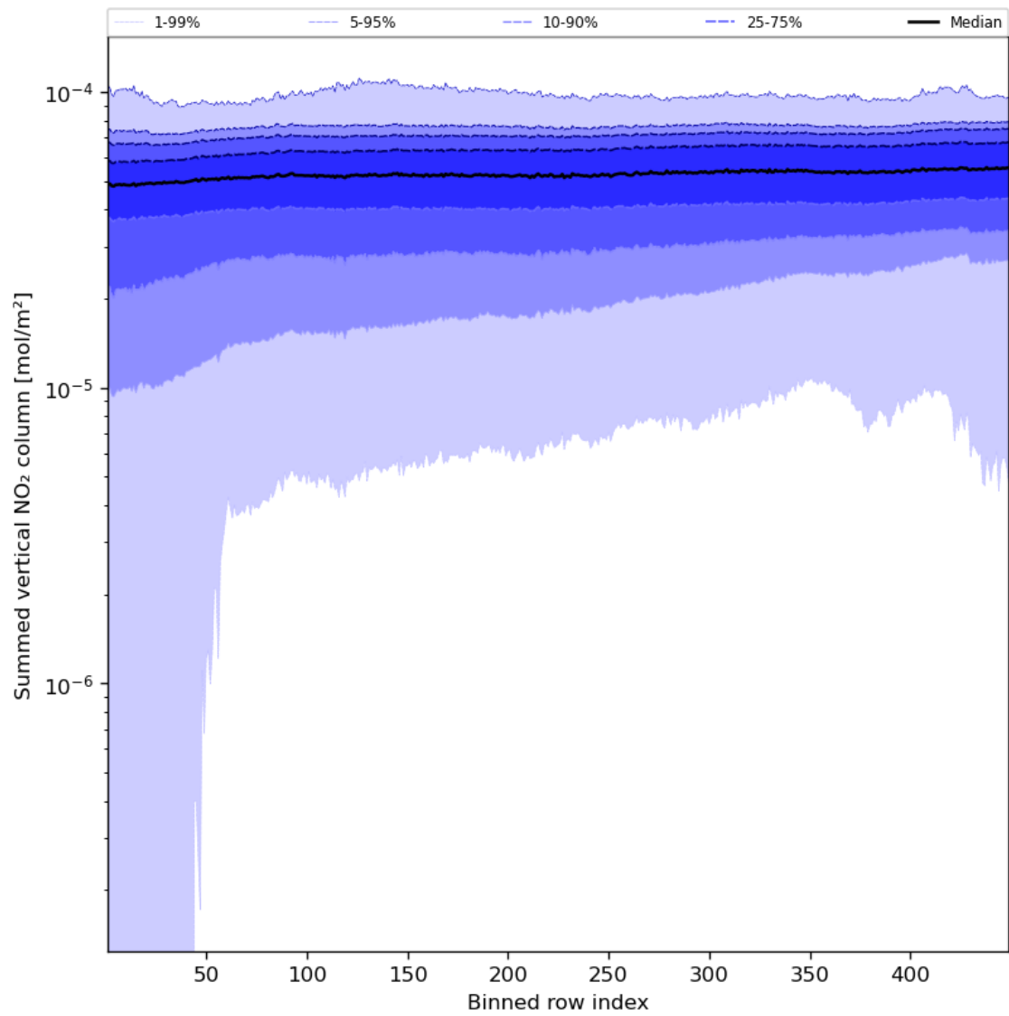
Figure 57: Along track statistics of “Summed vertical NO 2 column” for 2024-08-21 to 2024-08-22
