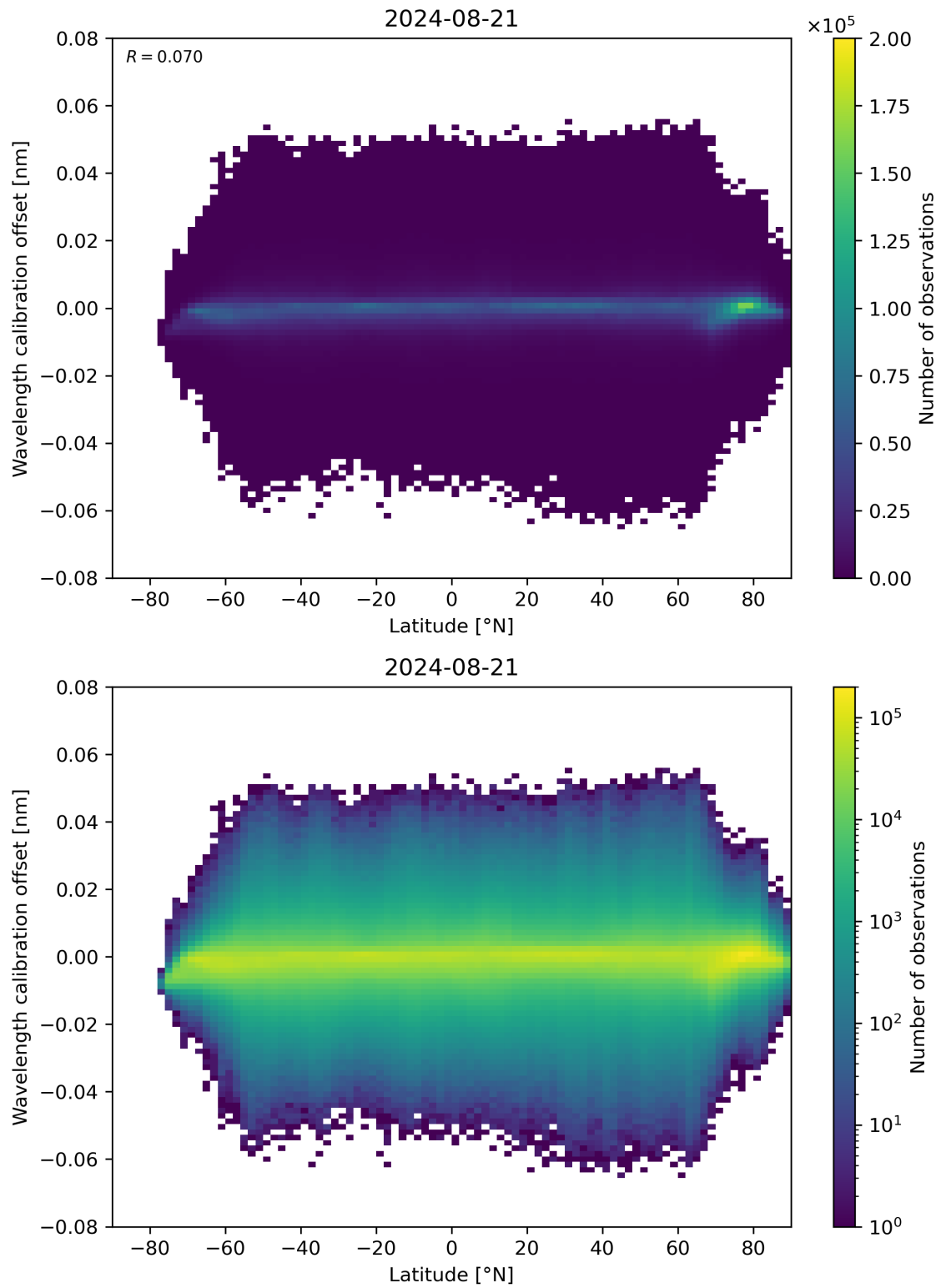
Figure 95: Scatter density plot of “Latitude” against “Wavelength calibration offset” for 2024-08-21 to 2024-08-22.
