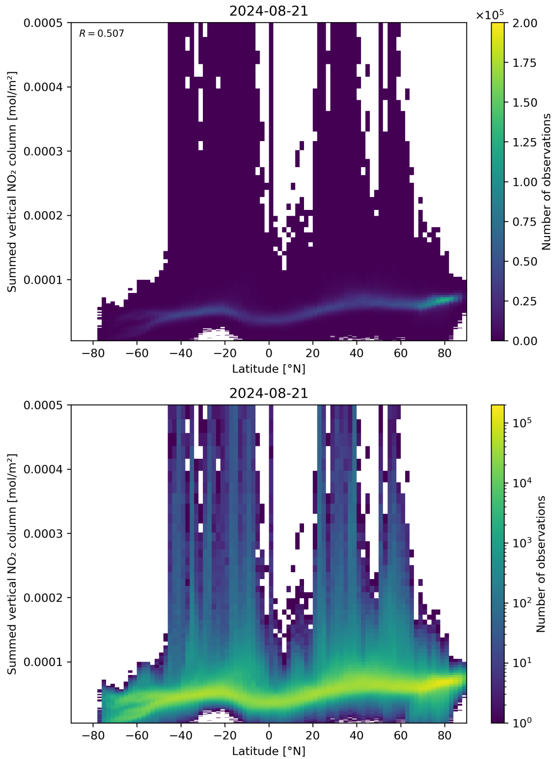
Figure 88: Scatter density plot of “Latitude” against “Summed vertical NO 2 column” for 2024-08-21 to 2024-08-22.
