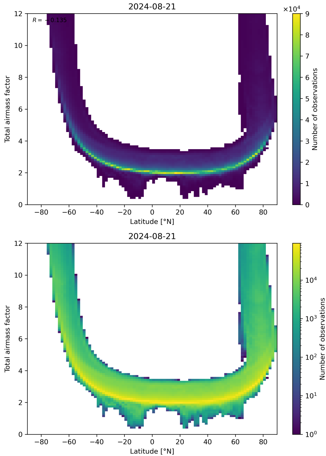
Figure 84: Scatter density plot of “Latitude” against “Total airmass factor” for 2024-08-21 to 2024-08-22.
