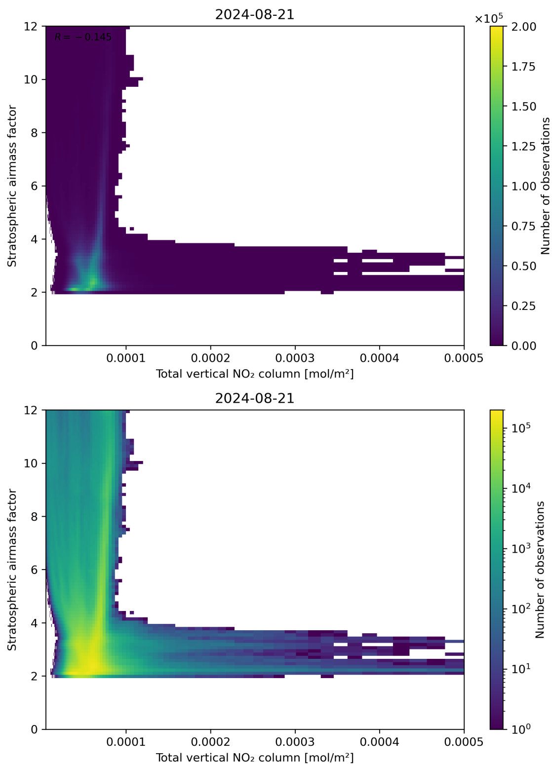
Figure 110: Scatter density plot of “Total vertical NO 2 column” against “Stratospheric airmass factor” for 2024-08-21 to 2024-08-22.
