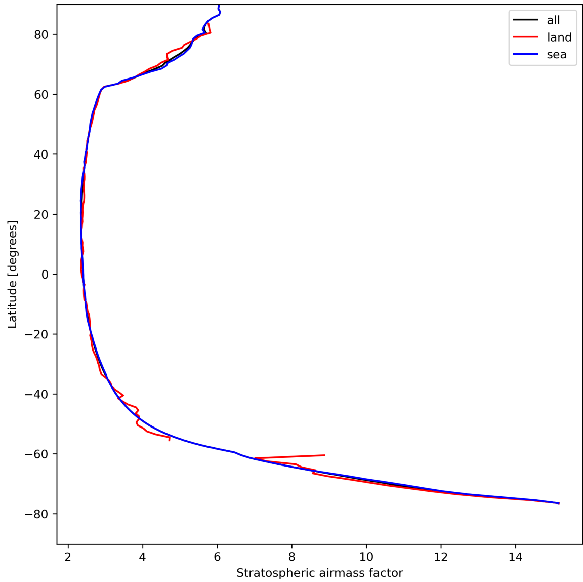
Figure 27: Zonal average of “Stratospheric airmass factor” for 2024-08-21 to 2024-08-22.
