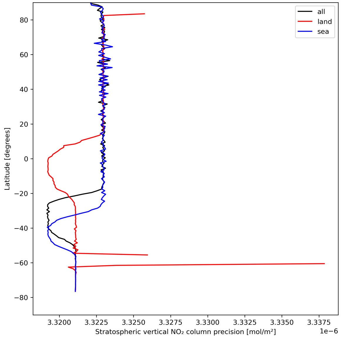
Figure 20: Zonal average of “Stratospheric vertical NO 2 column precision” for 2024-08-21 to 2024-08-22.
