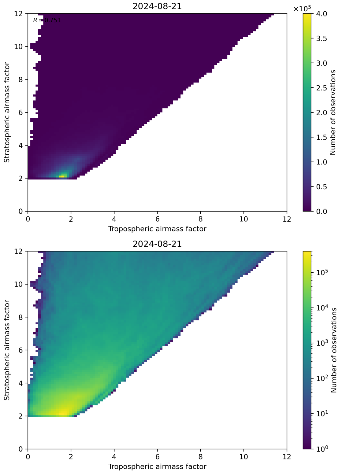
Figure 71: Scatter density plot of “Tropospheric airmass factor” against “Stratospheric airmass factor” for 2024-08-21 to 2024-08-22.
