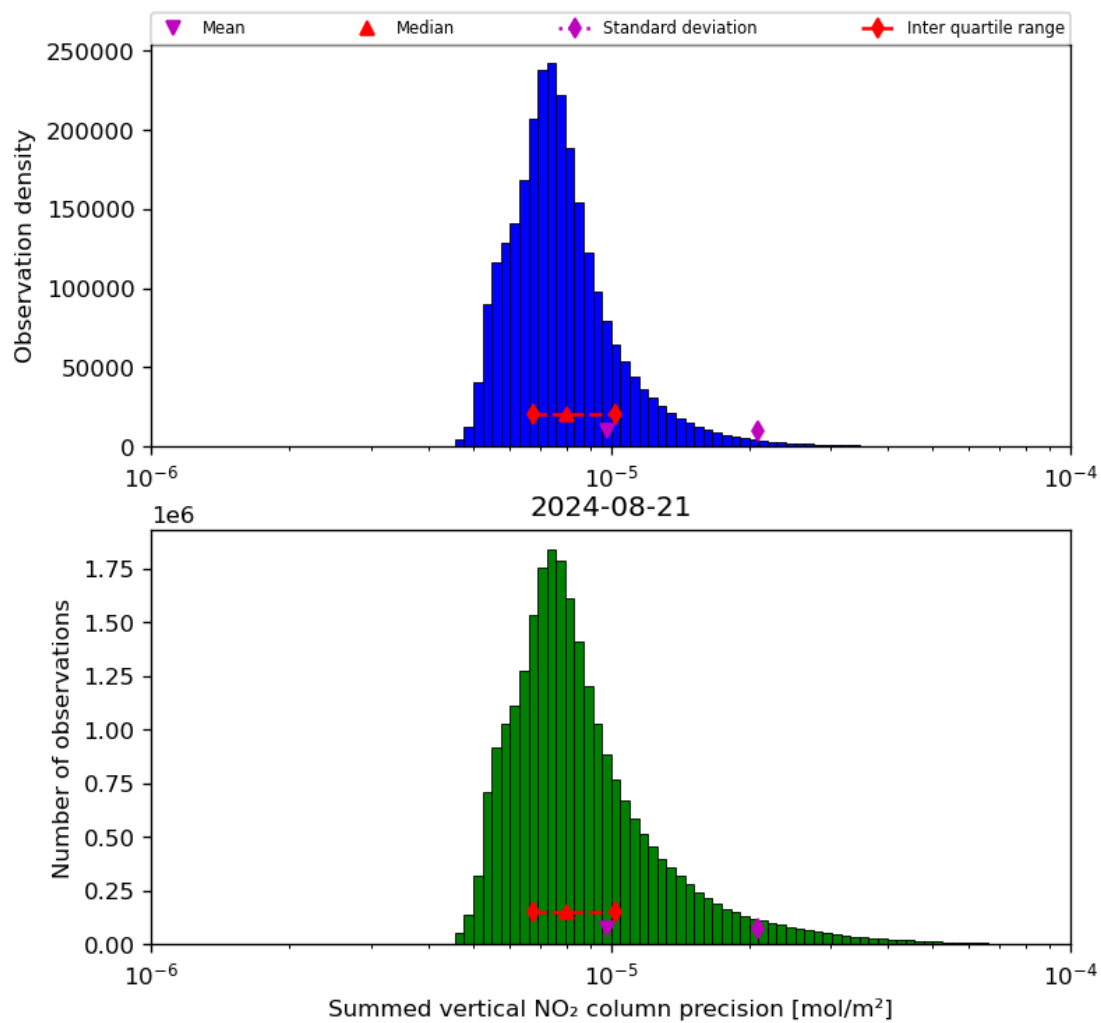
Figure 41: Histogram of “Summed vertical NO 2 column precision” for 2024-08-21 to 2024-08-22
