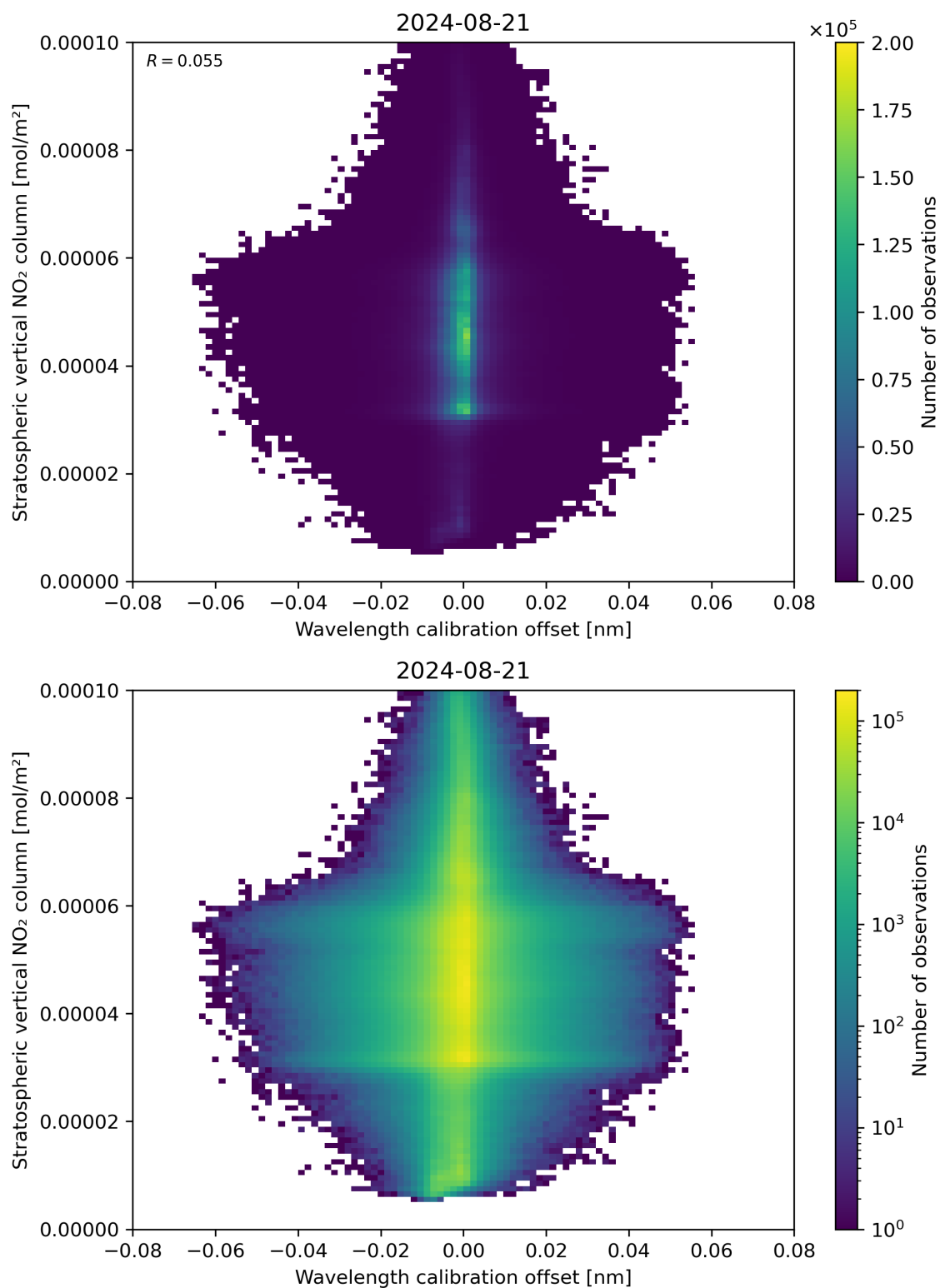
Figure 176: Scatter density plot of “Wavelength calibration offset” against “Stratospheric vertical NO 2 column” for 2024-08-21 to 2024-08-22.
