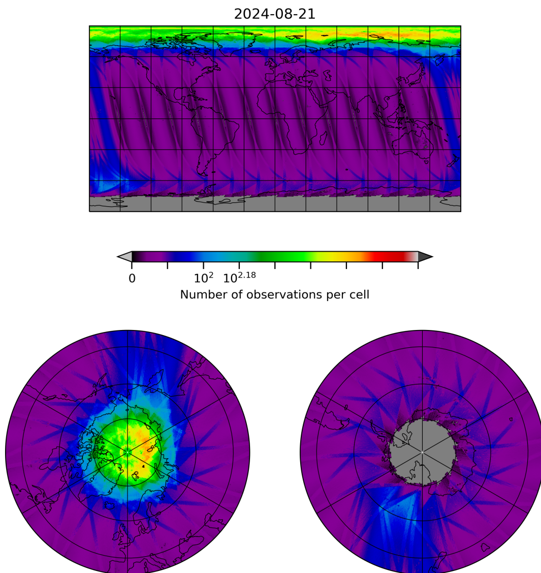
Figure 10: Map of the number of observations for 2024-08-21 to 2024-08-22
