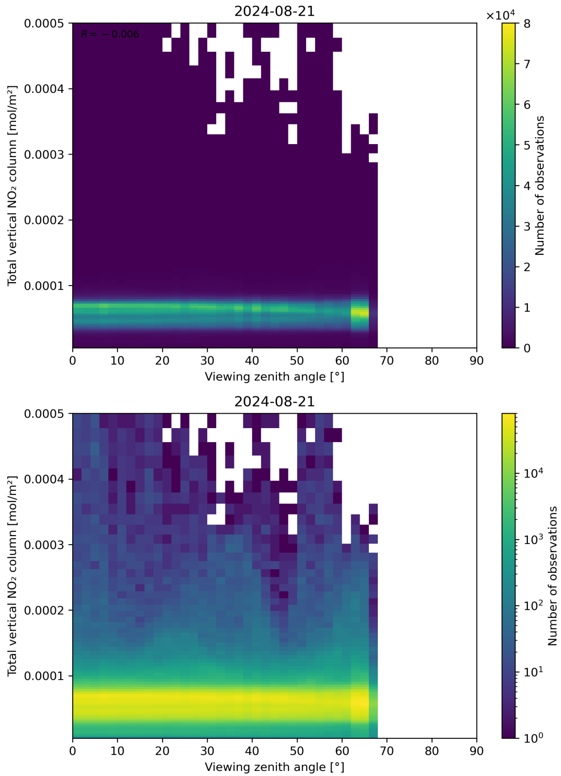
Figure 167: Scatter density plot of “Viewing zenith angle” against “Total vertical NO 2 column” for 2024-08-21 to 2024-08-22.
