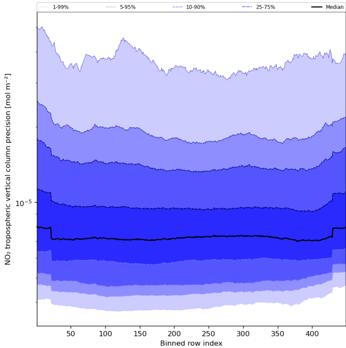
Figure 47: Along track statistics of “NO 2 tropospheric vertical column precision” for 2024-08-21 to 2024-08-22
