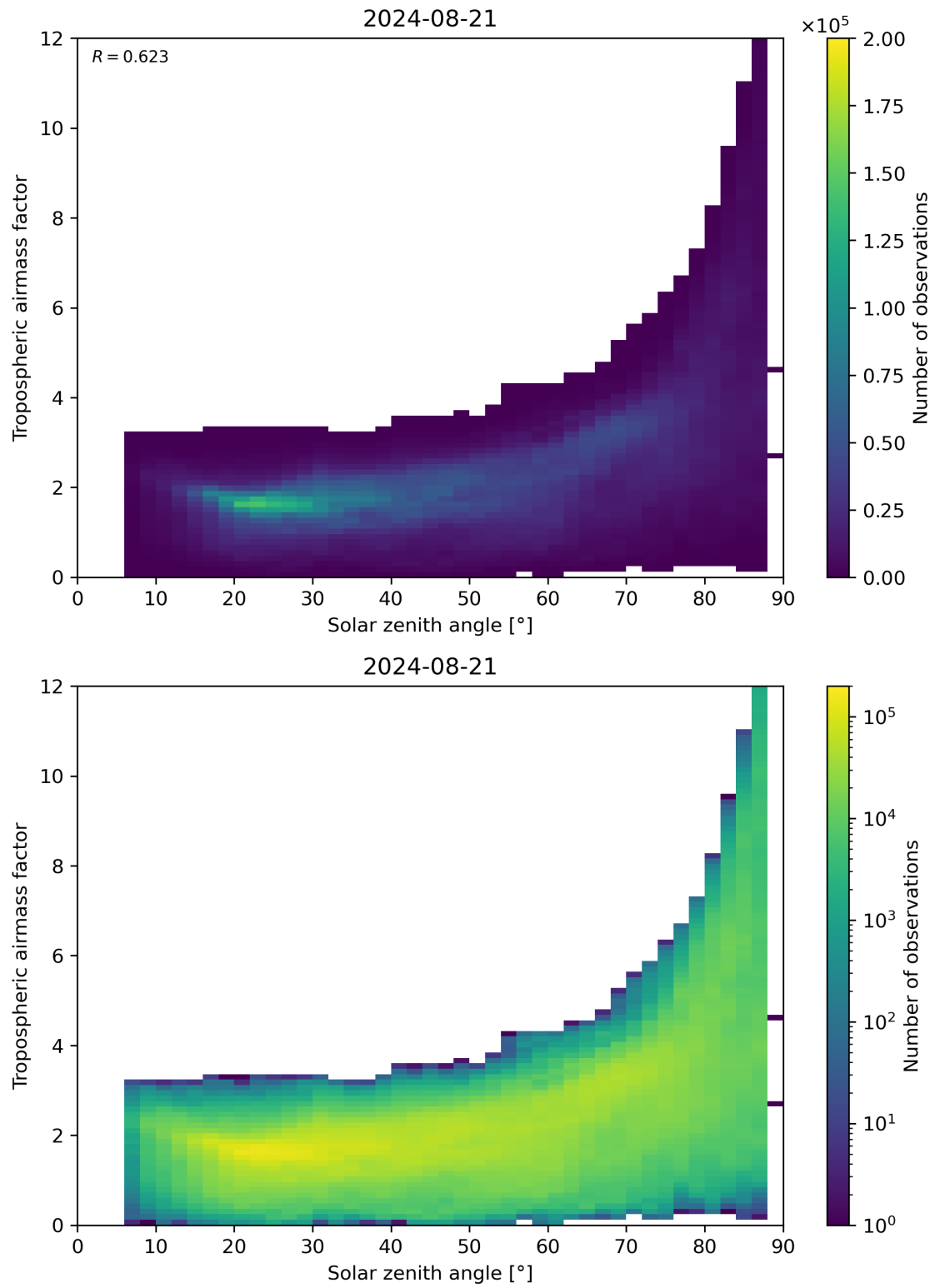
Figure 147: Scatter density plot of “Solar zenith angle” against “Tropospheric airmass factor” for 2024-08-21 to 2024-08-22.
