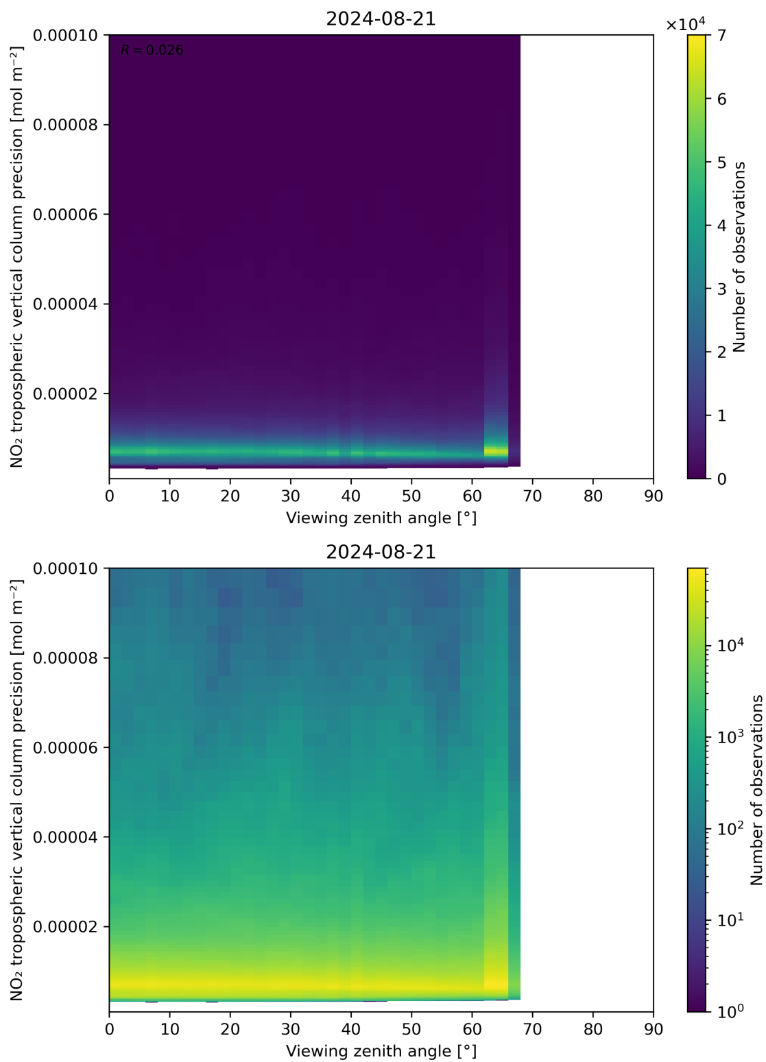
Figure 170: Scatter density plot of “Viewing zenith angle” against “NO 2 tropospheric vertical column precision” for 2024-08-21 to 2024-08-22.
