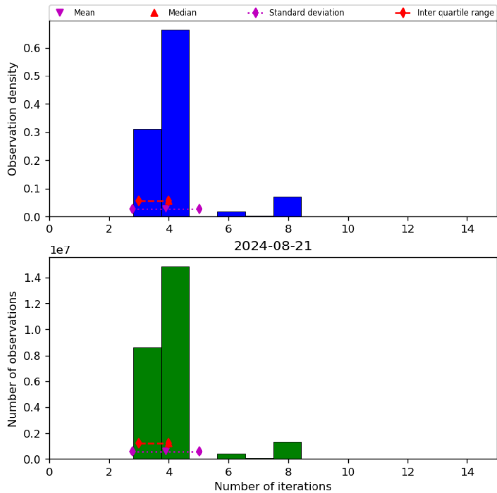
Figure 34: Histogram of “Number of iterations” for 2024-08-21 to 2024-08-22
