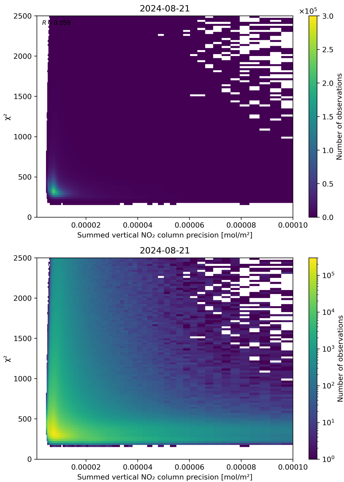
Figure 107: Scatter density plot of “Summed vertical NO 2 column precision” against “ \chi^2 ” for 2024-08-21 to 2024-08-22.
