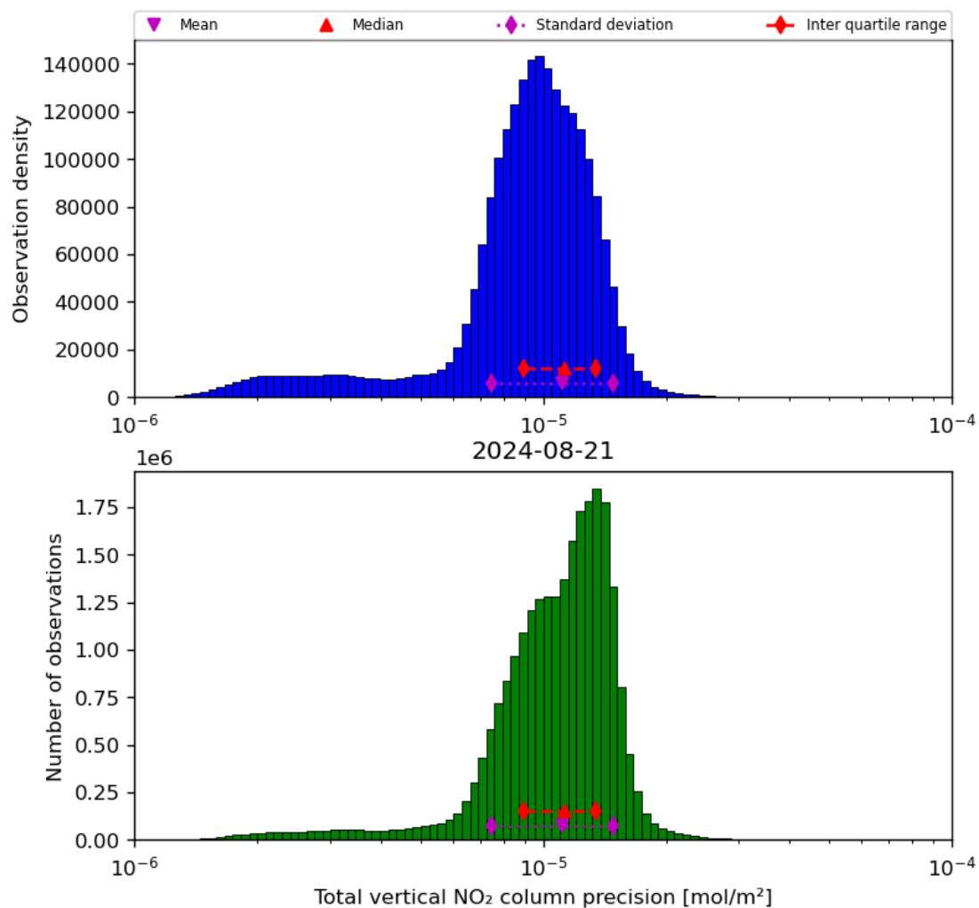
Figure 39: Histogram of “Total vertical NO 2 column precision” for 2024-08-21 to 2024-08-22
