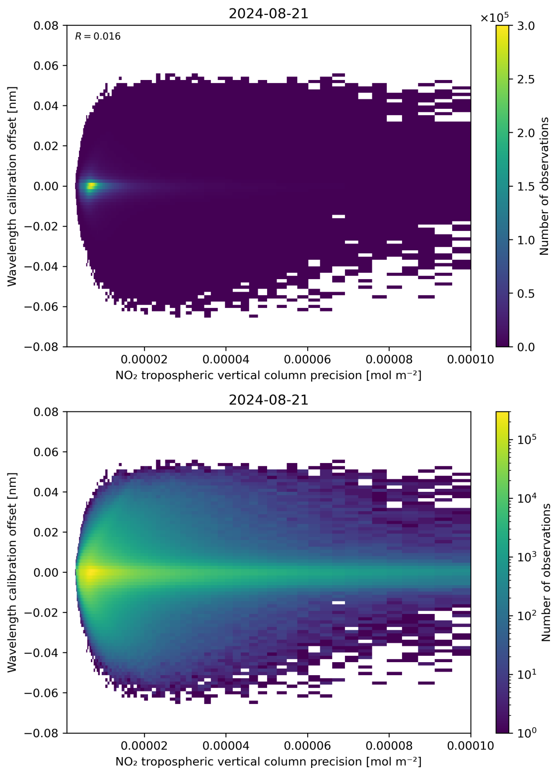
Figure 141: Scatter density plot of “NO 2 tropospheric vertical column precision” against “Wavelength calibration offset” for 2024-08-21 to 2024-08-22.
