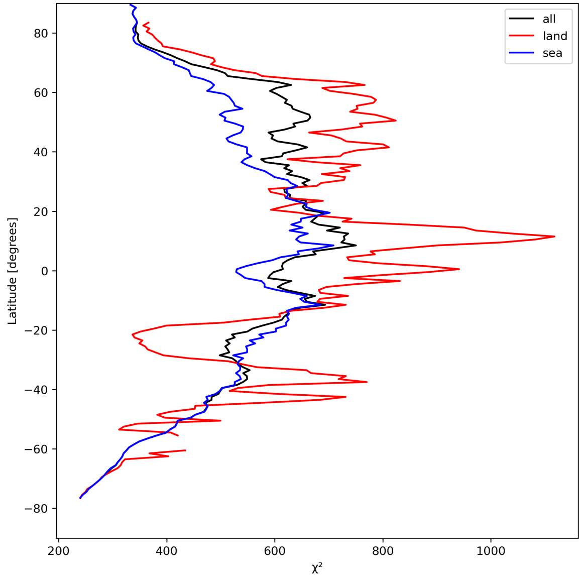
Figure 25: Zonal average of “ \chi^2 ” for 2024-08-21 to 2024-08-22.
