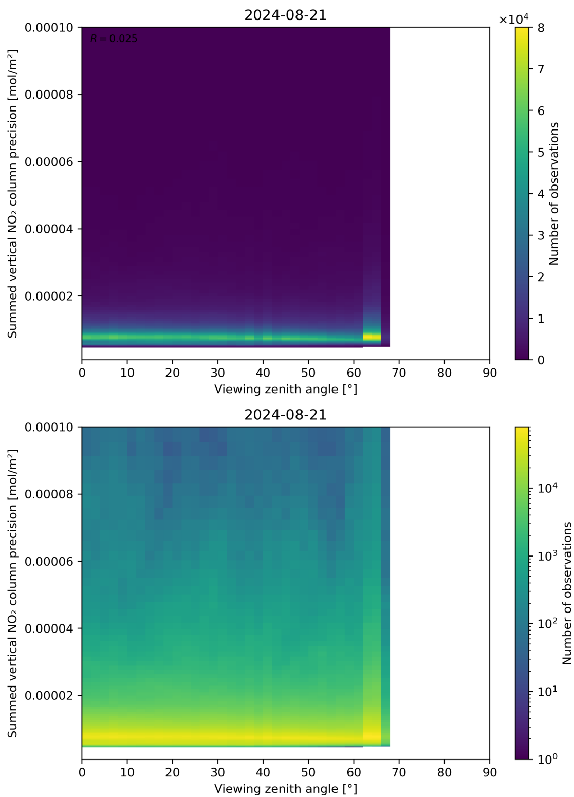
Figure 166: Scatter density plot of “Viewing zenith angle” against “Summed vertical NO 2 column precision” for 2024-08-21 to 2024-08-22.
