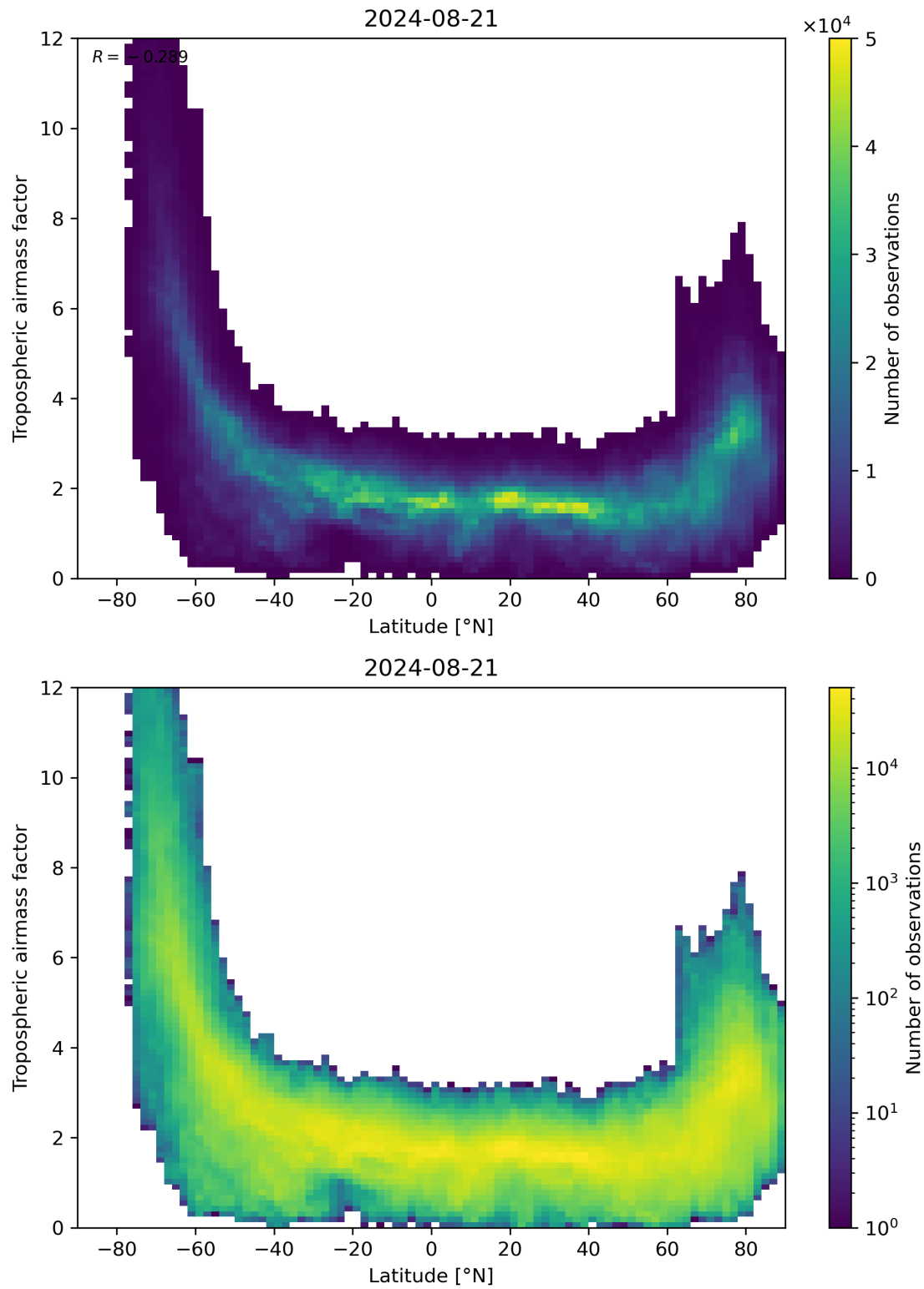
Figure 85: Scatter density plot of “Latitude” against “Tropospheric airmass factor” for 2024-08-21 to 2024-08-22.
