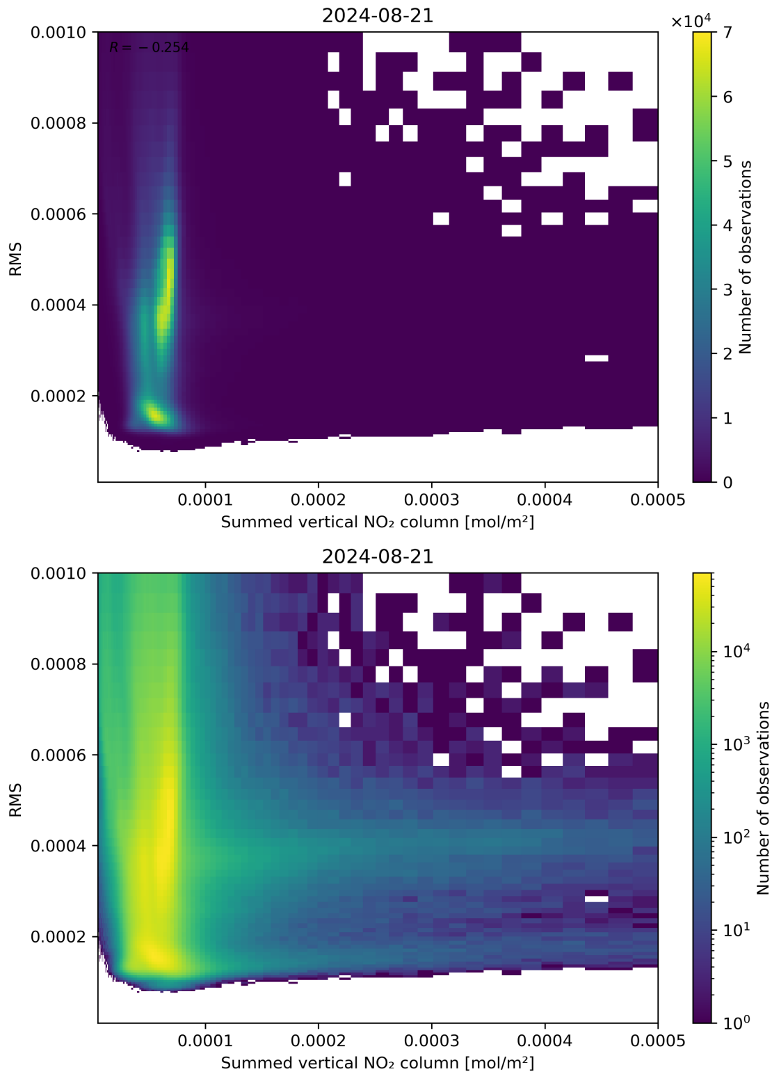
Figure 109: Scatter density plot of “Summed vertical NO 2 column” against “RMS” for 2024-08-21 to 2024-08-22.
