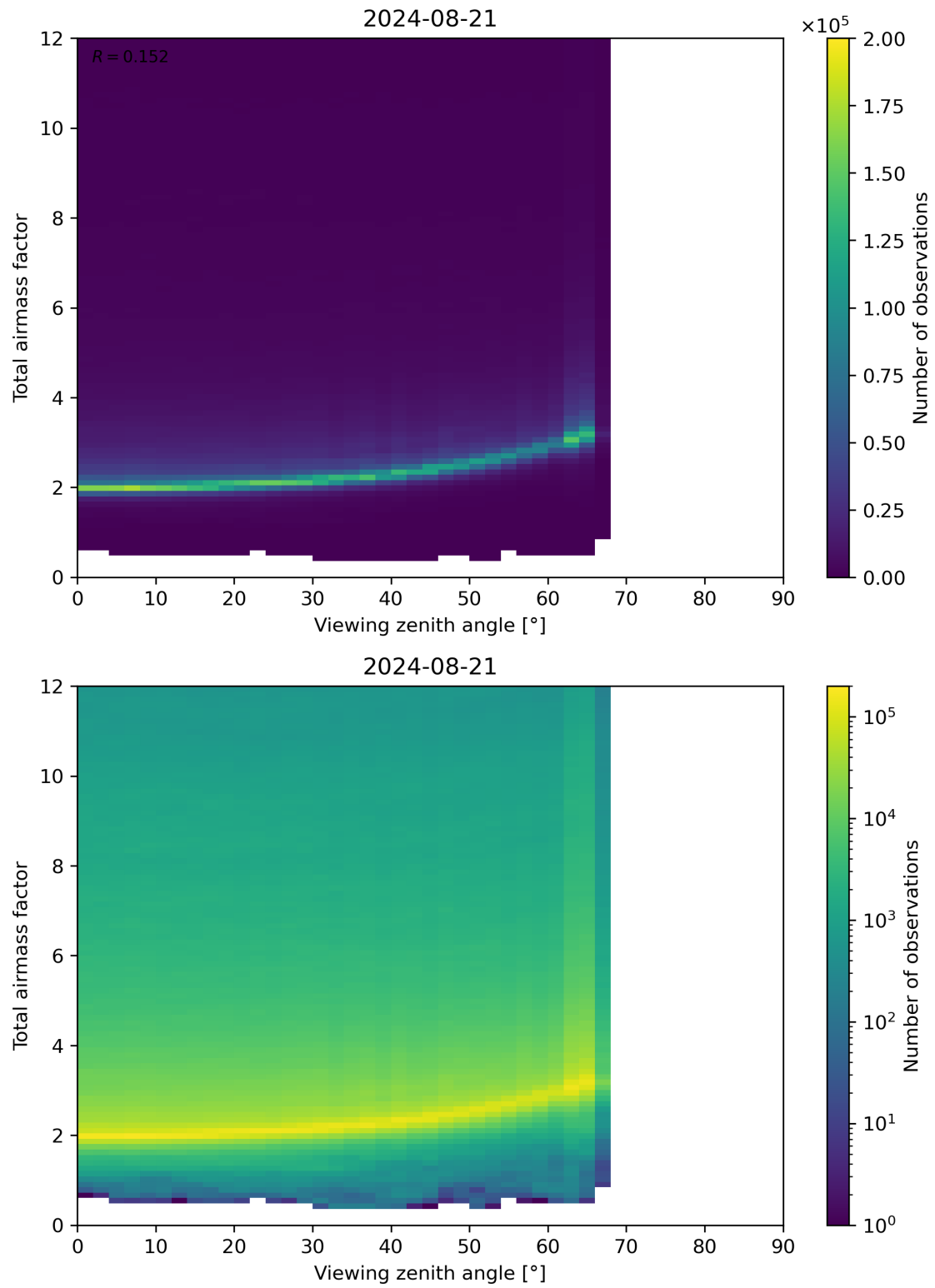
Figure 160: Scatter density plot of “Viewing zenith angle” against “Total airmass factor” for 2024-08-21 to 2024-08-22.
