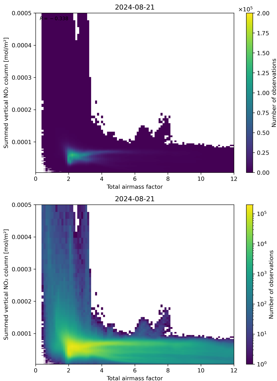
Figure 65: Scatter density plot of “Total airmass factor” against “Summed vertical NO 2 column” for 2024-08-21 to 2024-08-22.
