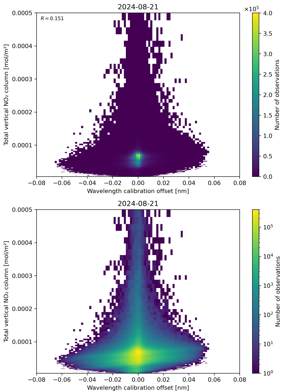
Figure 179: Scatter density plot of “Wavelength calibration offset” against “Total vertical NO 2 column” for 2024-08-21 to 2024-08-22.
