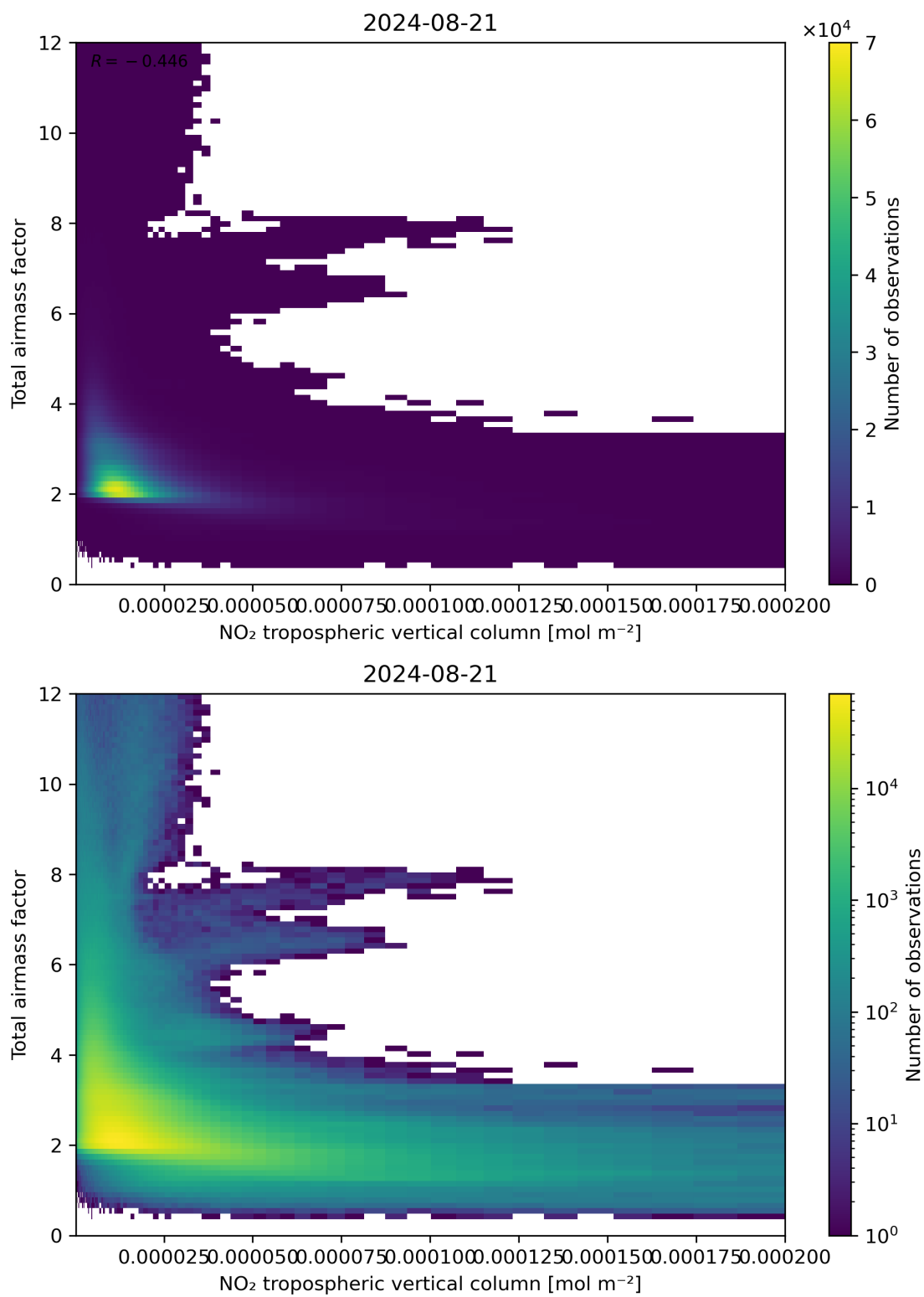
Figure 122: Scatter density plot of “NO 2 tropospheric vertical column” against “Total air mass factor” for 2024-08-21 to 2024-08-22.
