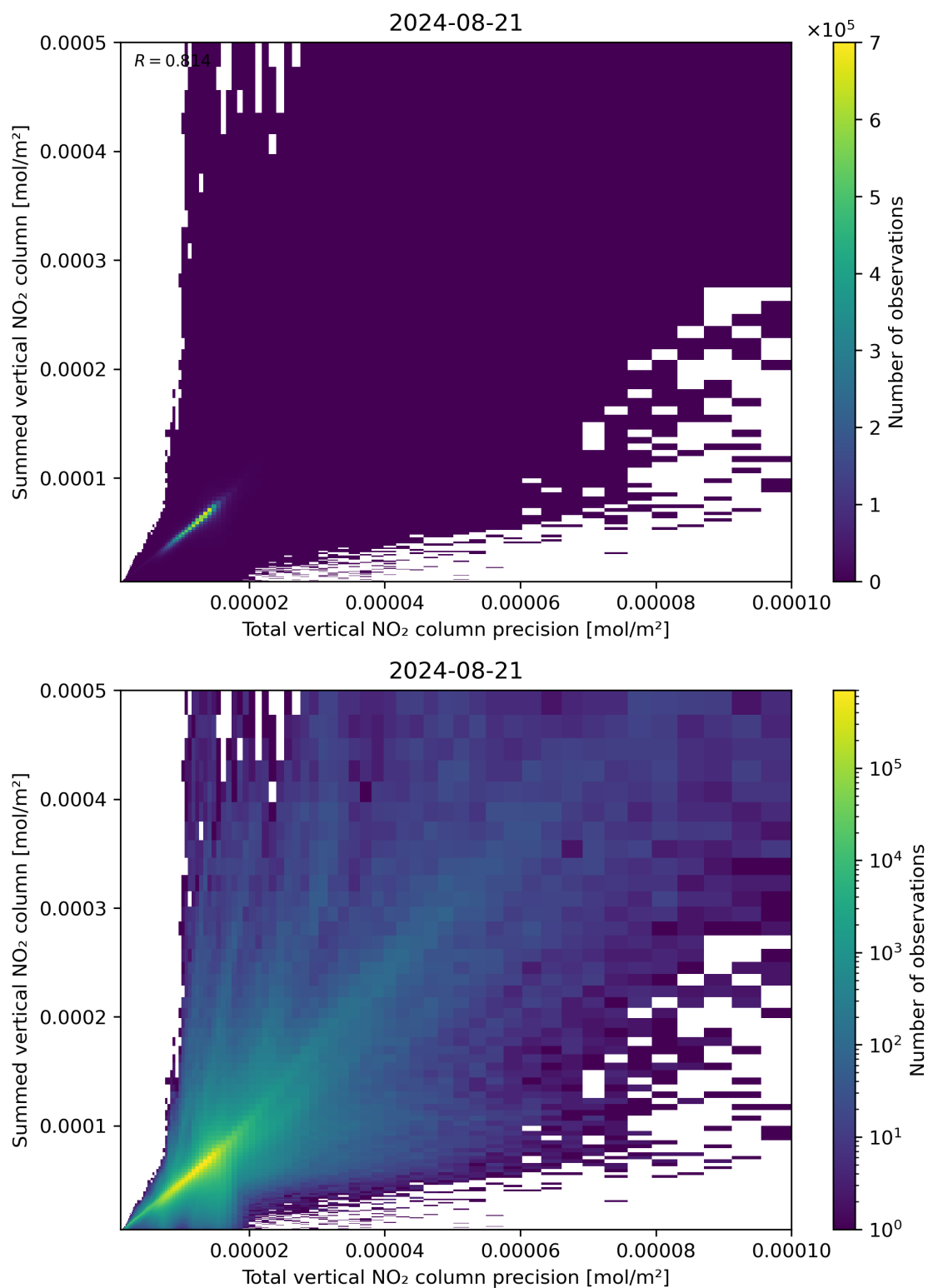
Figure 117: Scatter density plot of “Total vertical NO 2 column precision” against “Summed vertical NO 2 column” for 2024-08-21 to 2024-08-22.
