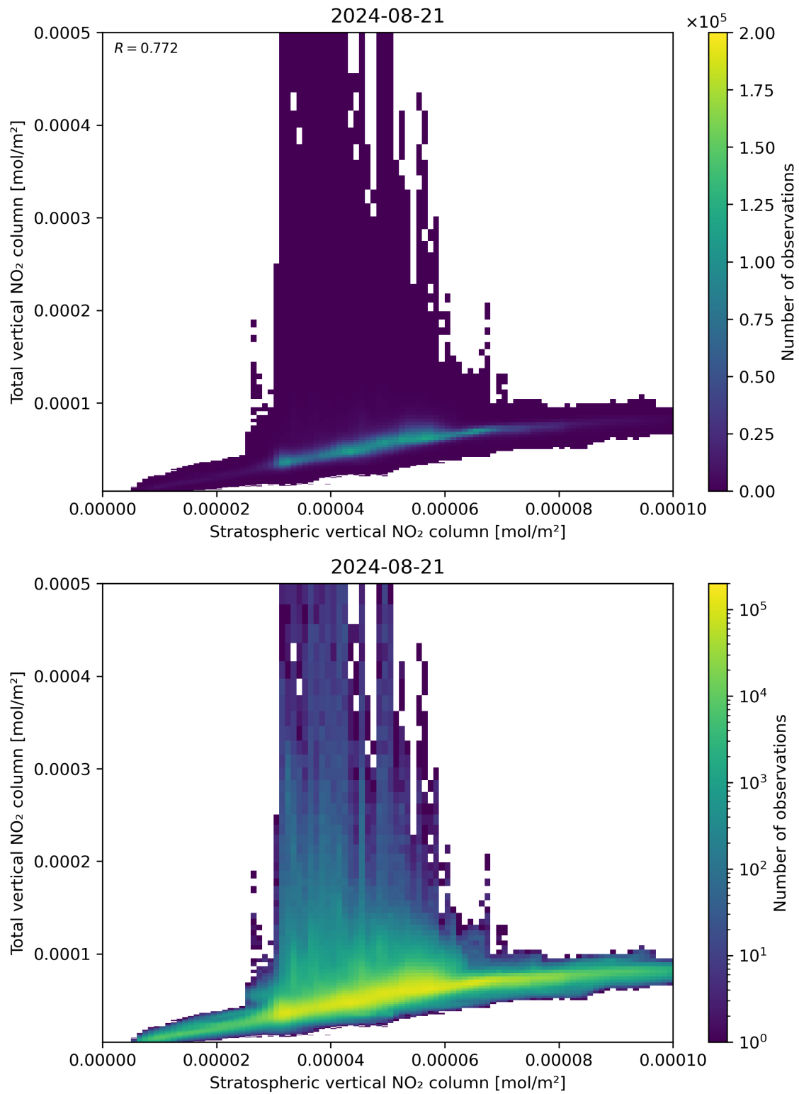
Figure 100: Scatter density plot of “Stratospheric vertical NO 2 column” against “Total vertical NO 2 column” for 2024-08-21 to 2024-08-22.
