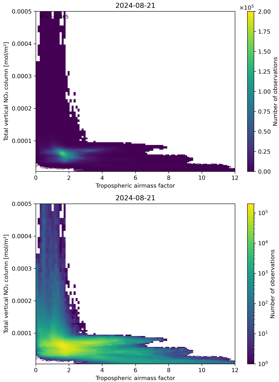
Figure 77: Scatter density plot of “Tropospheric airmass factor” against “Total vertical \text{NO}_2 column” for 2024-08-21 to 2024-08-22.
