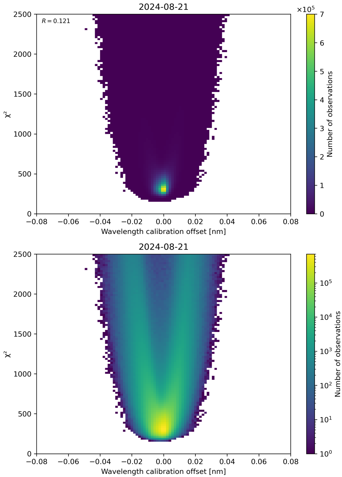
Figure 175: Scatter density plot of “Wavelength calibration offset” against “ \chi^2 ” for 2024-08-21 to 2024-08-22.
