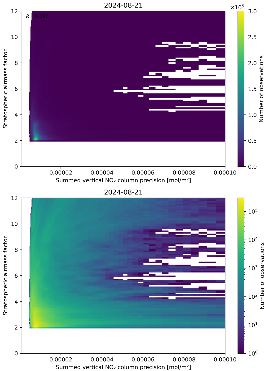
Figure 106: Scatter density plot of “Summed vertical NO 2 column precision” against “Stratospheric airmass factor” for 2024-08-21 to 2024-08-22.
