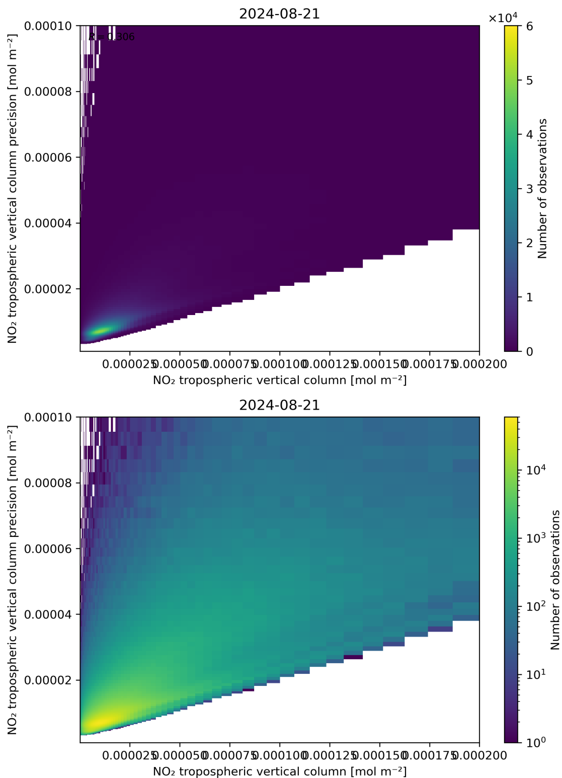
Figure 130: Scatter density plot of “NO 2 tropospheric vertical column” against “NO 2 tropospheric vertical column precision” for 2024-08-21 to 2024-08-22.
