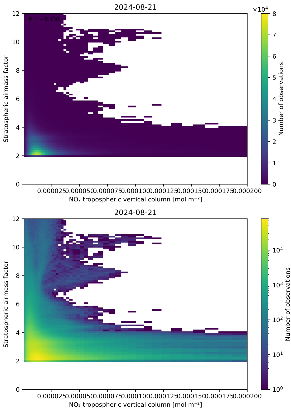
Figure 121: Scatter density plot of “NO 2 tropospheric vertical column” against “Stratospheric air mass factor” for 2024-08-21 to 2024-08-22.
