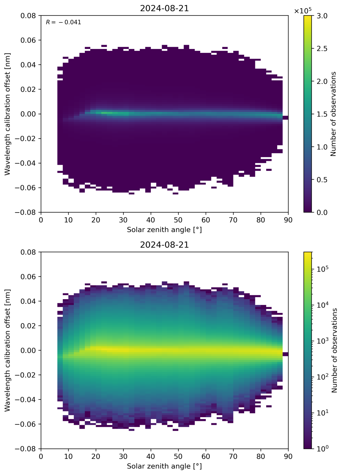
Figure 158: Scatter density plot of “Solar zenith angle” against “Wavelength calibration offset” for 2024-08-21 to 2024-08-22.
