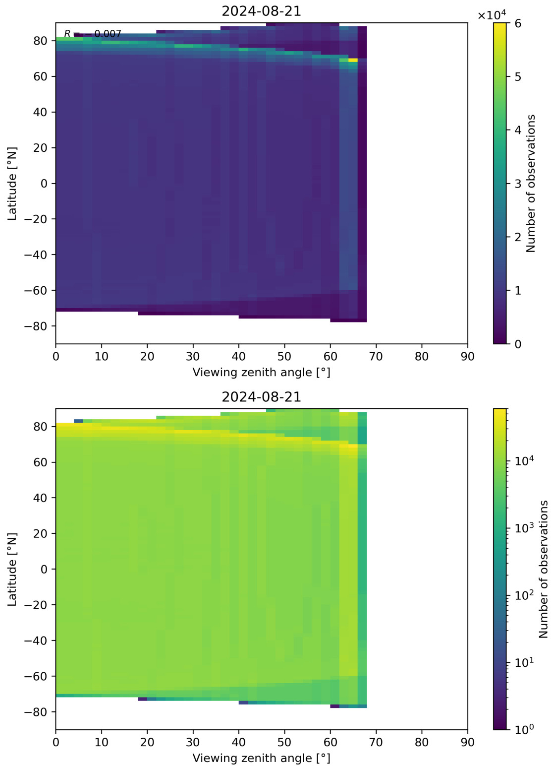
Figure 163: Scatter density plot of “Viewing zenith angle” against “Latitude” for 2024-08-21 to 2024-08-22.
