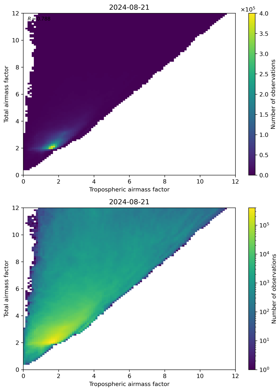
Figure 72: Scatter density plot of “Tropospheric airmass factor” against “Total airmass factor” for 2024-08-21 to 2024-08-22.
