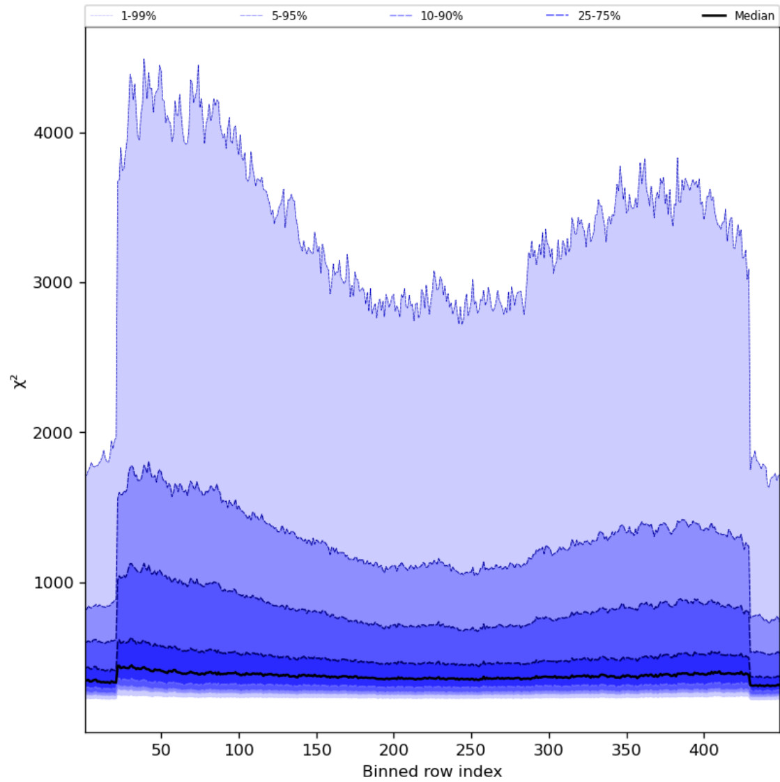
Figure 59: Along track statistics of “ \chi^2 ” for 2024-08-21 to 2024-08-22
