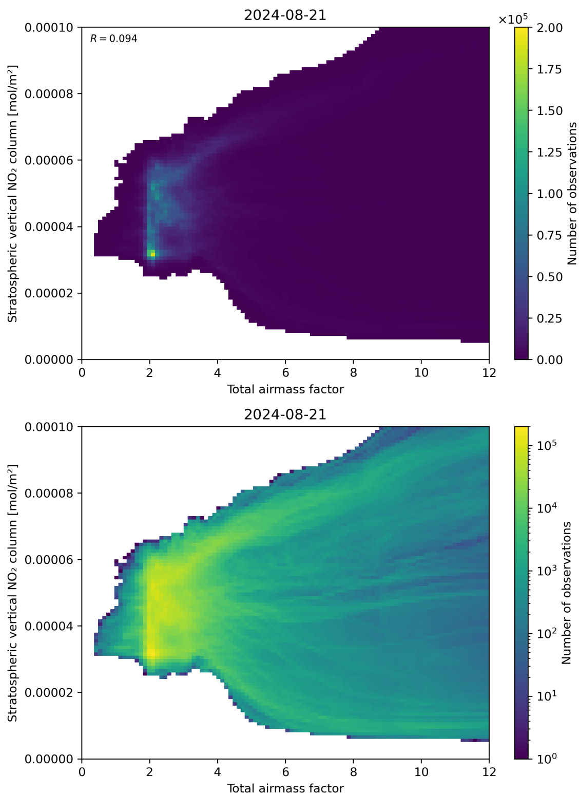
Figure 64: Scatter density plot of “Total airmass factor” against “Stratospheric vertical NO 2 column” for 2024-08-21 to 2024-08-22.
