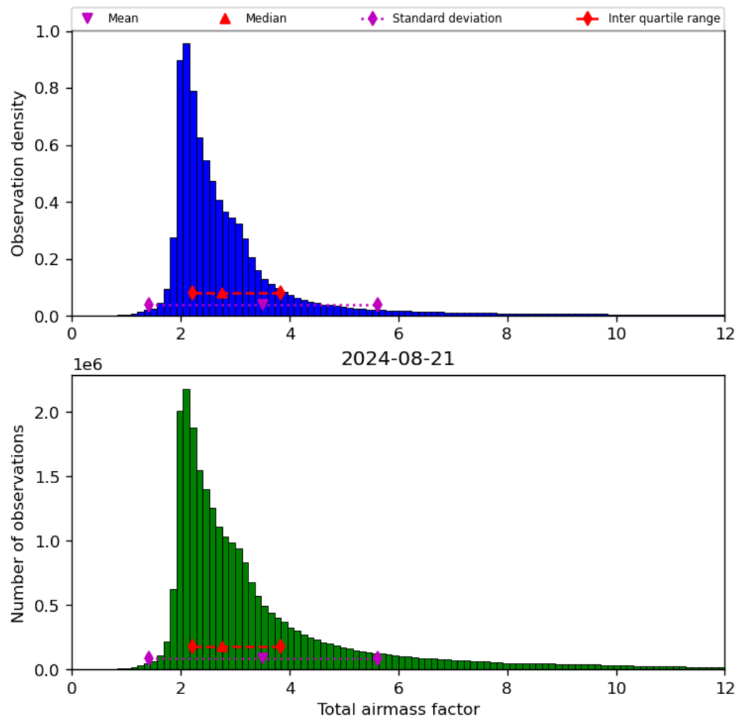
Figure 32: Histogram of “Total airmass factor” for 2024-08-21 to 2024-08-22
