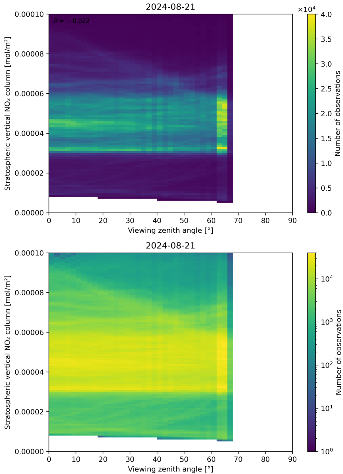
Figure 164: Scatter density plot of “Viewing zenith angle” against “Stratospheric vertical NO 2 column” for 2024-08-21 to 2024-08-22.
