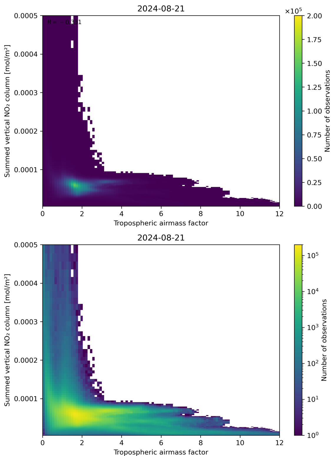
Figure 75: Scatter density plot of “Tropospheric airmass factor” against “Summed vertical NO 2 column” for 2024-08-21 to 2024-08-22.
