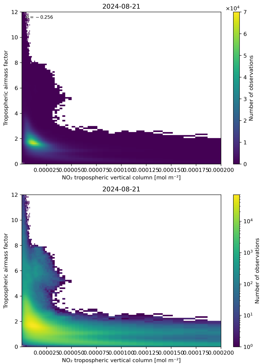
Figure 123: Scatter density plot of “NO 2 tropospheric vertical column” against “Tropospheric air mass factor” for 2024-08-21 to 2024-08-22.
