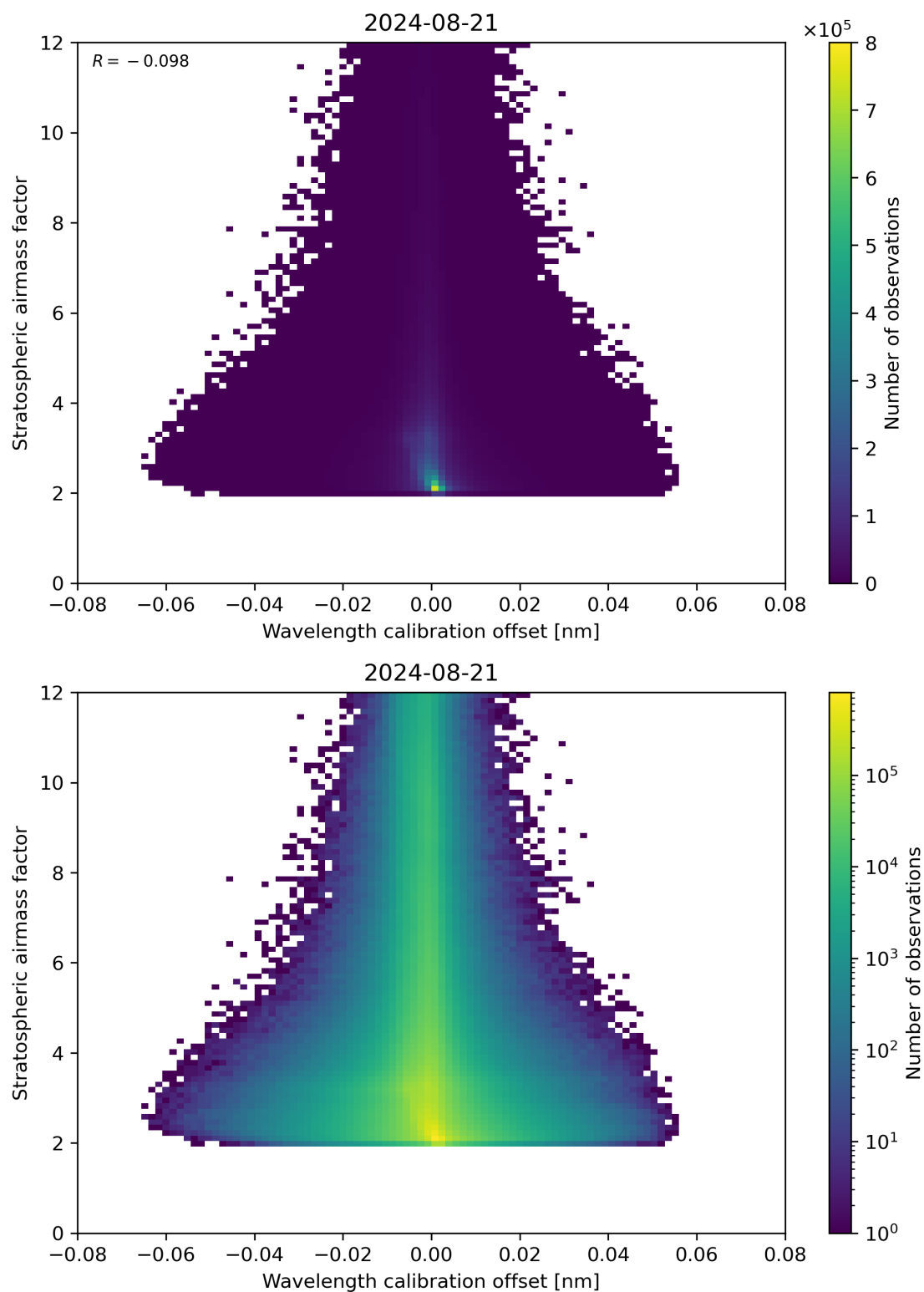
Figure 174: Scatter density plot of “Wavelength calibration offset” against “Stratospheric air mass factor” for 2024-08-21 to 2024-08-22.
