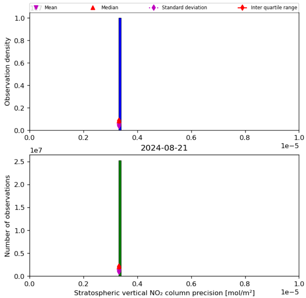
Figure 37: Histogram of “Stratospheric vertical NO 2 column precision” for 2024-08-21 to 2024-08-22
