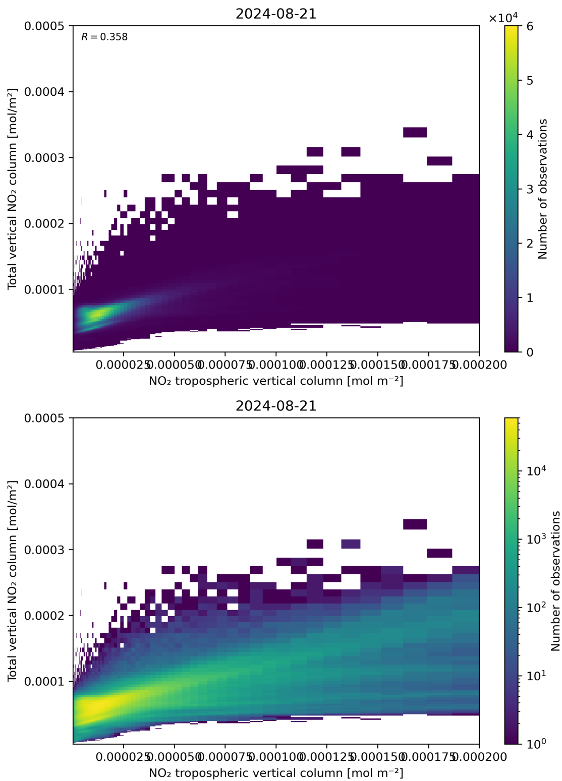
Figure 128: Scatter density plot of “NO 2 tropospheric vertical column” against “Total vertical NO 2 column” for 2024-08-21 to 2024-08-22.
