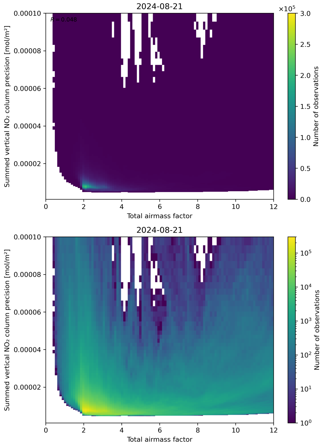
Figure 66: Scatter density plot of “Total airmass factor” against “Summed vertical NO 2 column precision” for 2024-08-21 to 2024-08-22.
