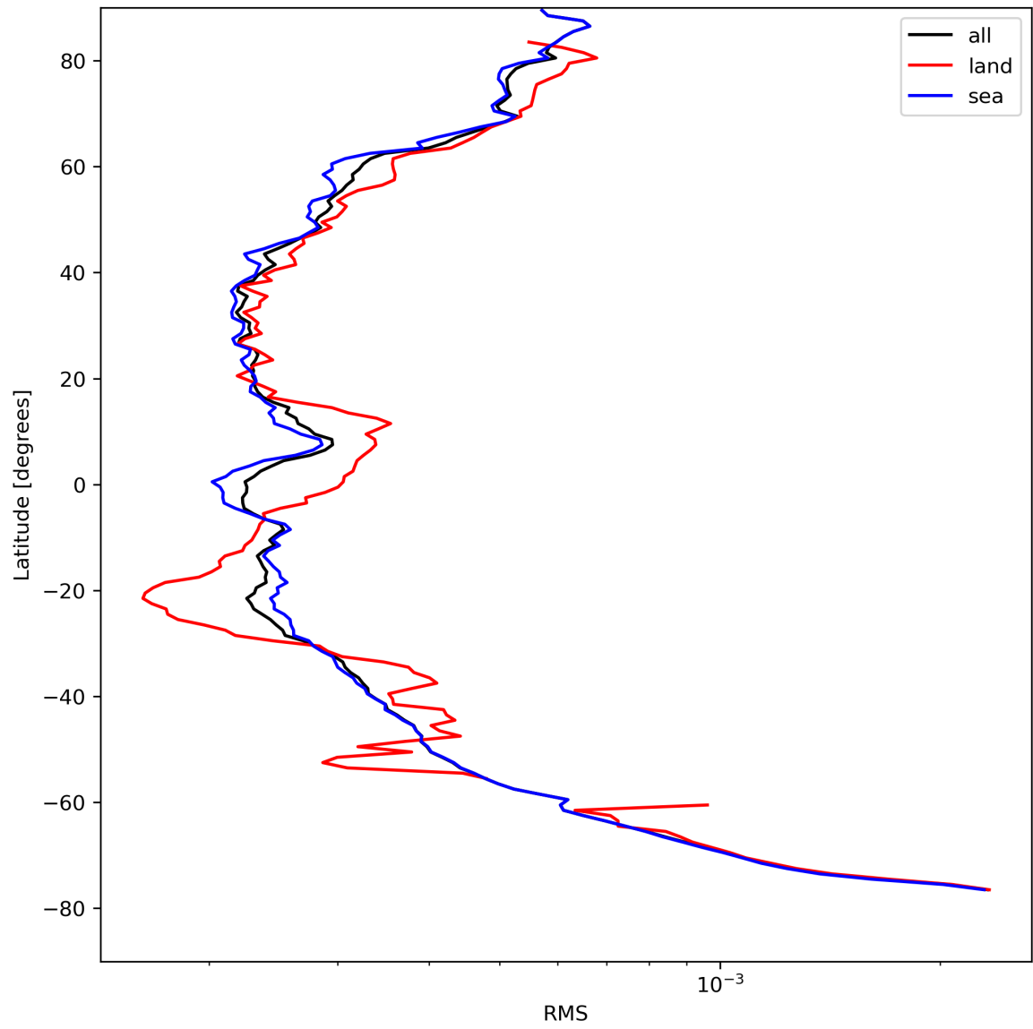
Figure 26: Zonal average of “RMS” for 2024-08-21 to 2024-08-22.
