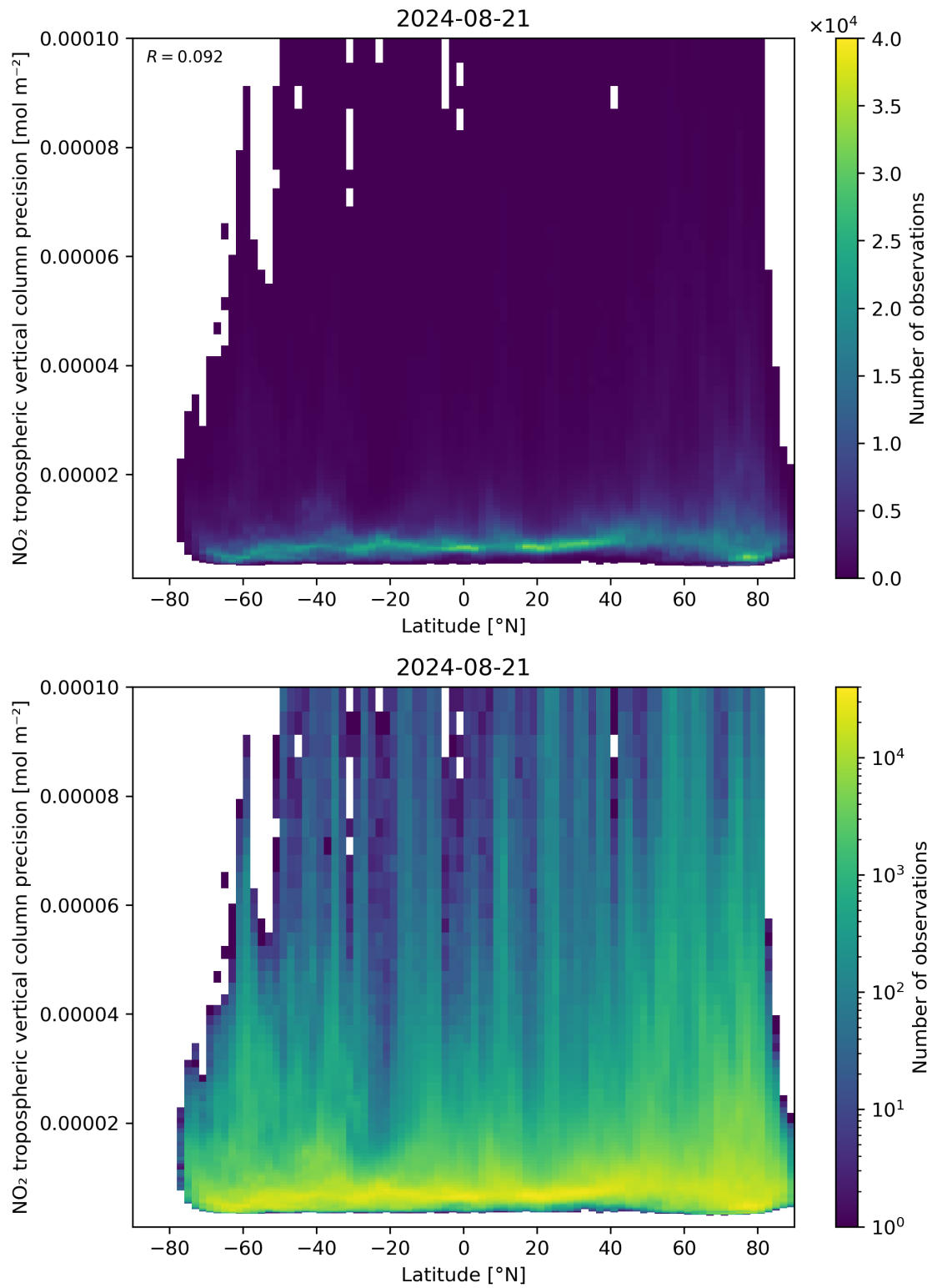
Figure 93: Scatter density plot of “Latitude” against “NO 2 tropospheric vertical column precision” for 2024-08-21 to 2024-08-22.
