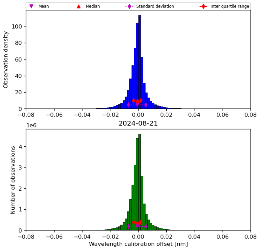
Figure 35: Histogram of “Wavelength calibration offset” for 2024-08-21 to 2024-08-22
