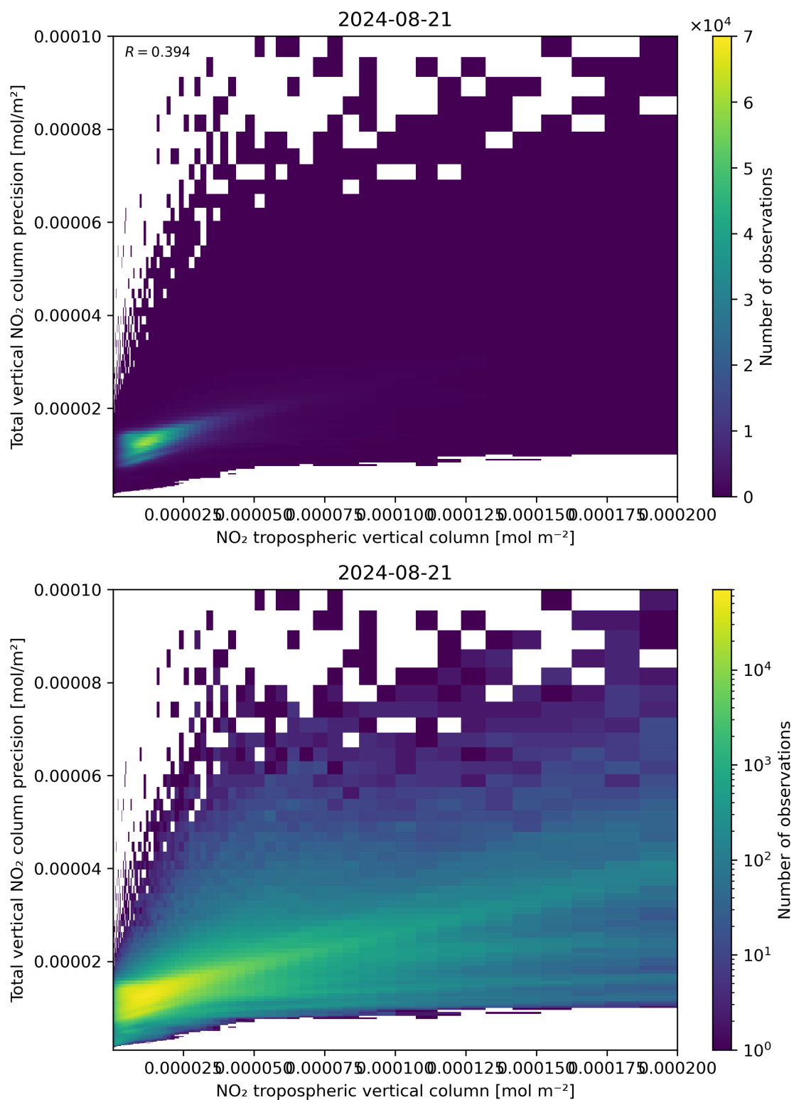
Figure 129: Scatter density plot of “NO 2 tropospheric vertical column” against “Total vertical NO 2 column precision” for 2024-08-21 to 2024-08-22.
