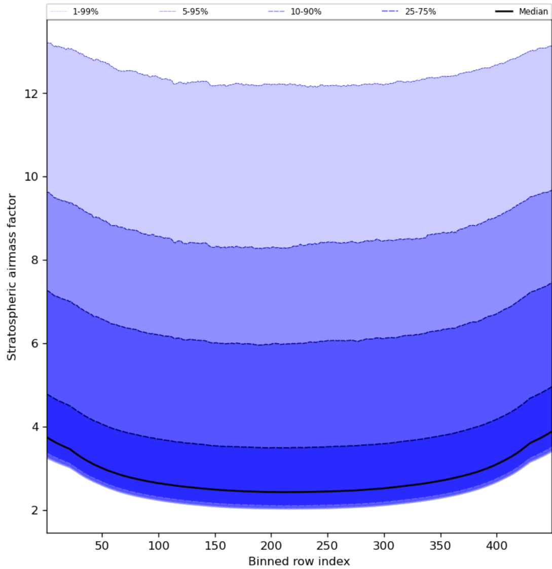
Figure 61: Along track statistics of “Stratospheric airmass factor” for 2024-08-21 to 2024-08-22
