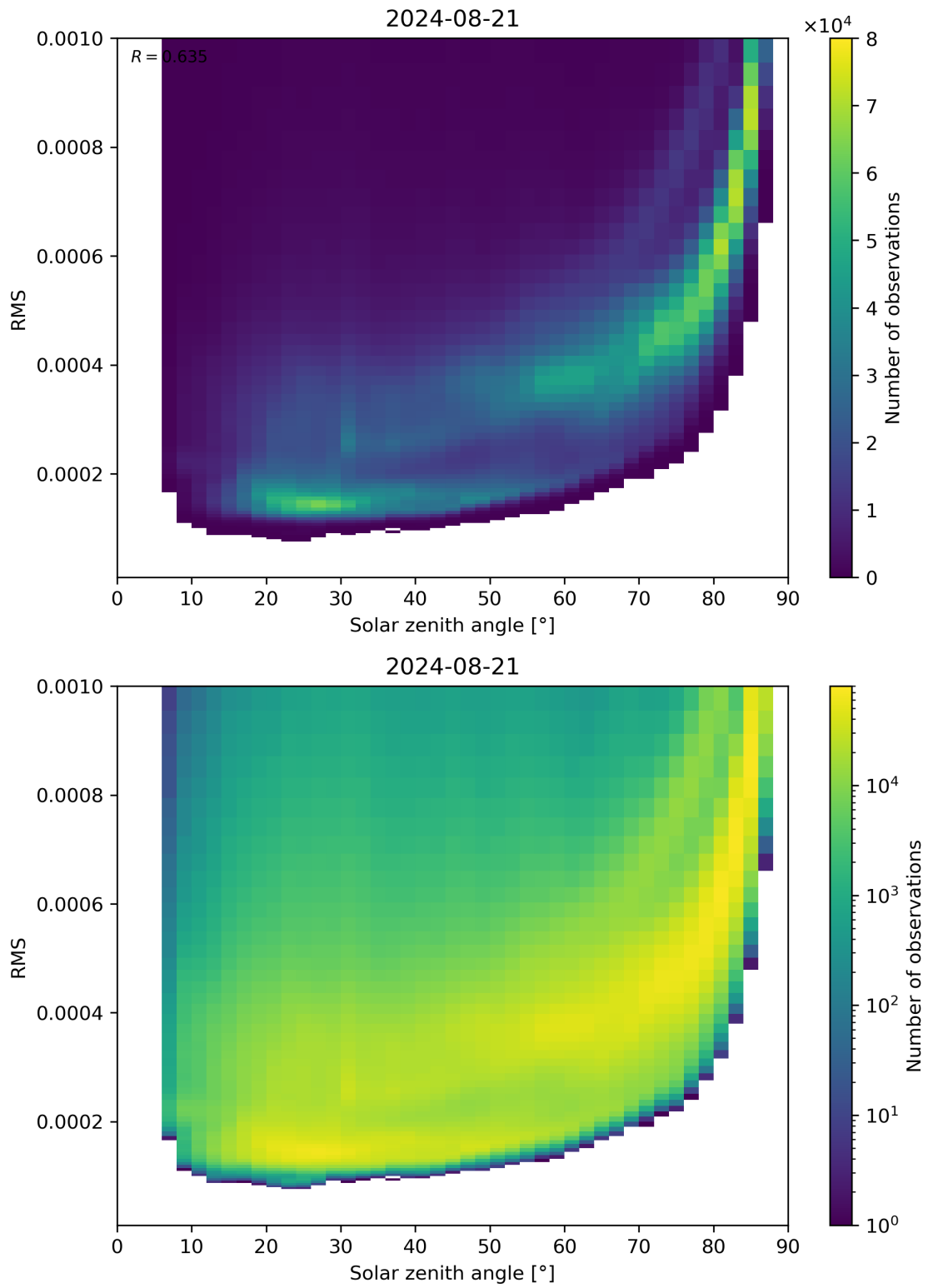
Figure 157: Scatter density plot of “Solar zenith angle” against “RMS” for 2024-08-21 to 2024-08-22.
