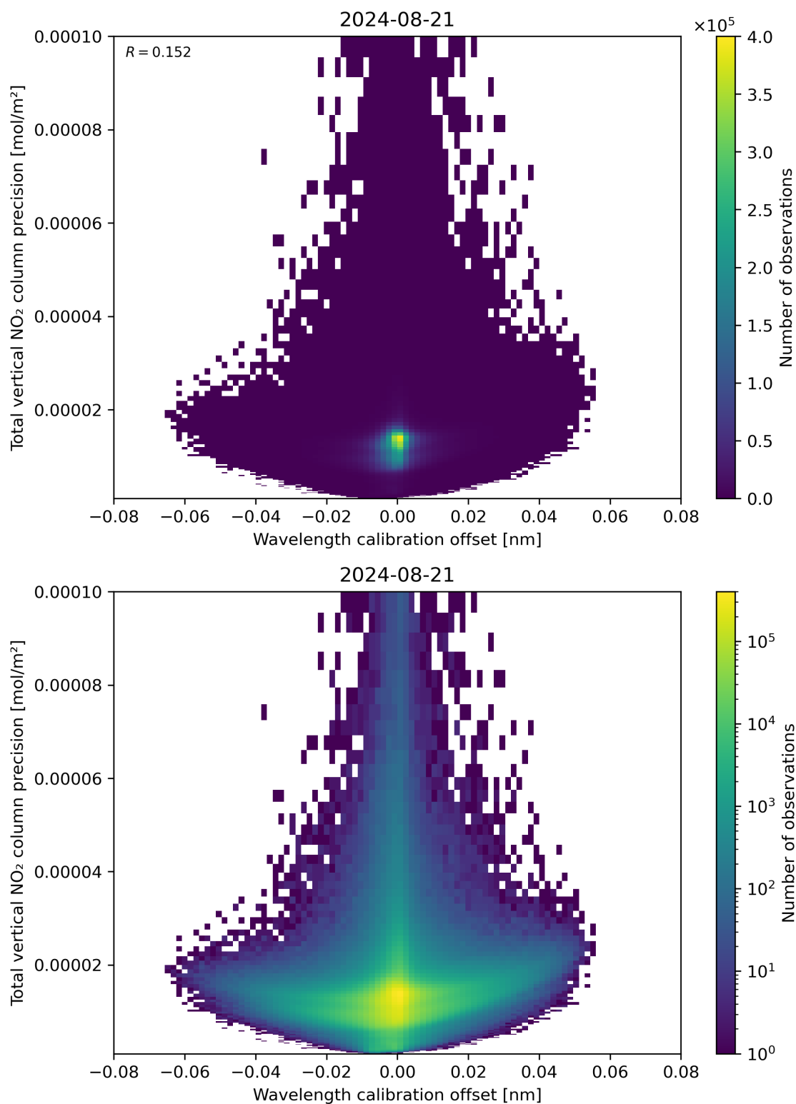
Figure 180: Scatter density plot of “Wavelength calibration offset” against “Total vertical NO 2 column precision” for 2024-08-21 to 2024-08-22.
