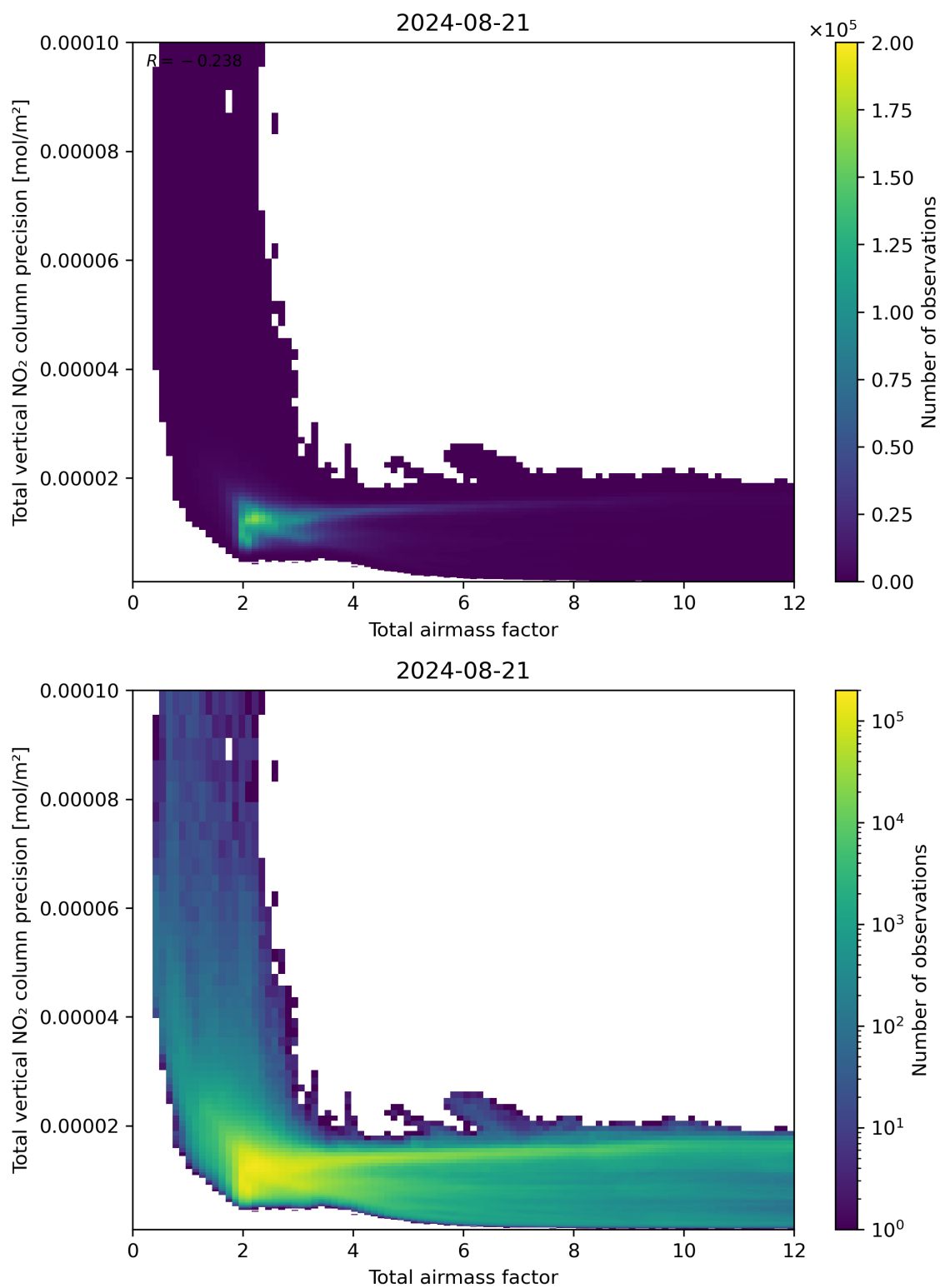
Figure 68: Scatter density plot of “Total airmass factor” against “Total vertical NO 2 column precision” for 2024-08-21 to 2024-08-22.
