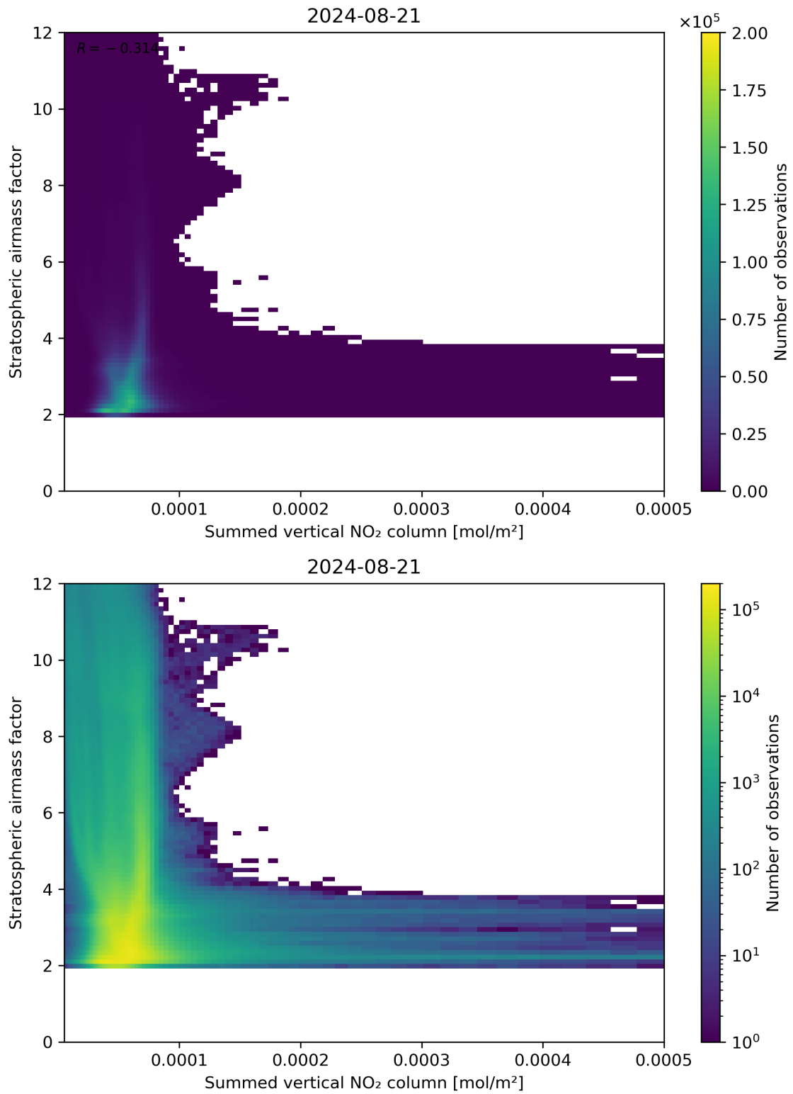
Figure 103: Scatter density plot of “Summed vertical NO 2 column” against “Stratospheric airmass factor” for 2024-08-21 to 2024-08-22.
