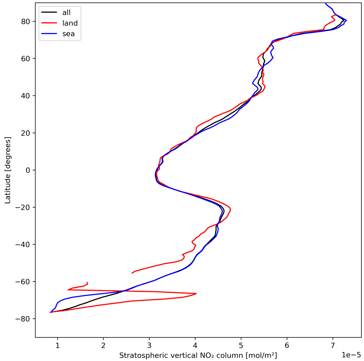
Figure 19: Zonal average of “Stratospheric vertical NO 2 column” for 2024-08-21 to 2024-08-22.
