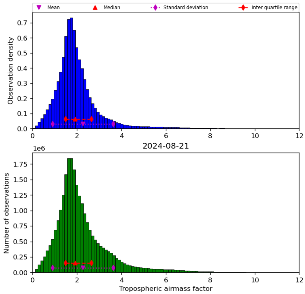
Figure 31: Histogram of “Tropospheric airmass factor” for 2024-08-21 to 2024-08-22
