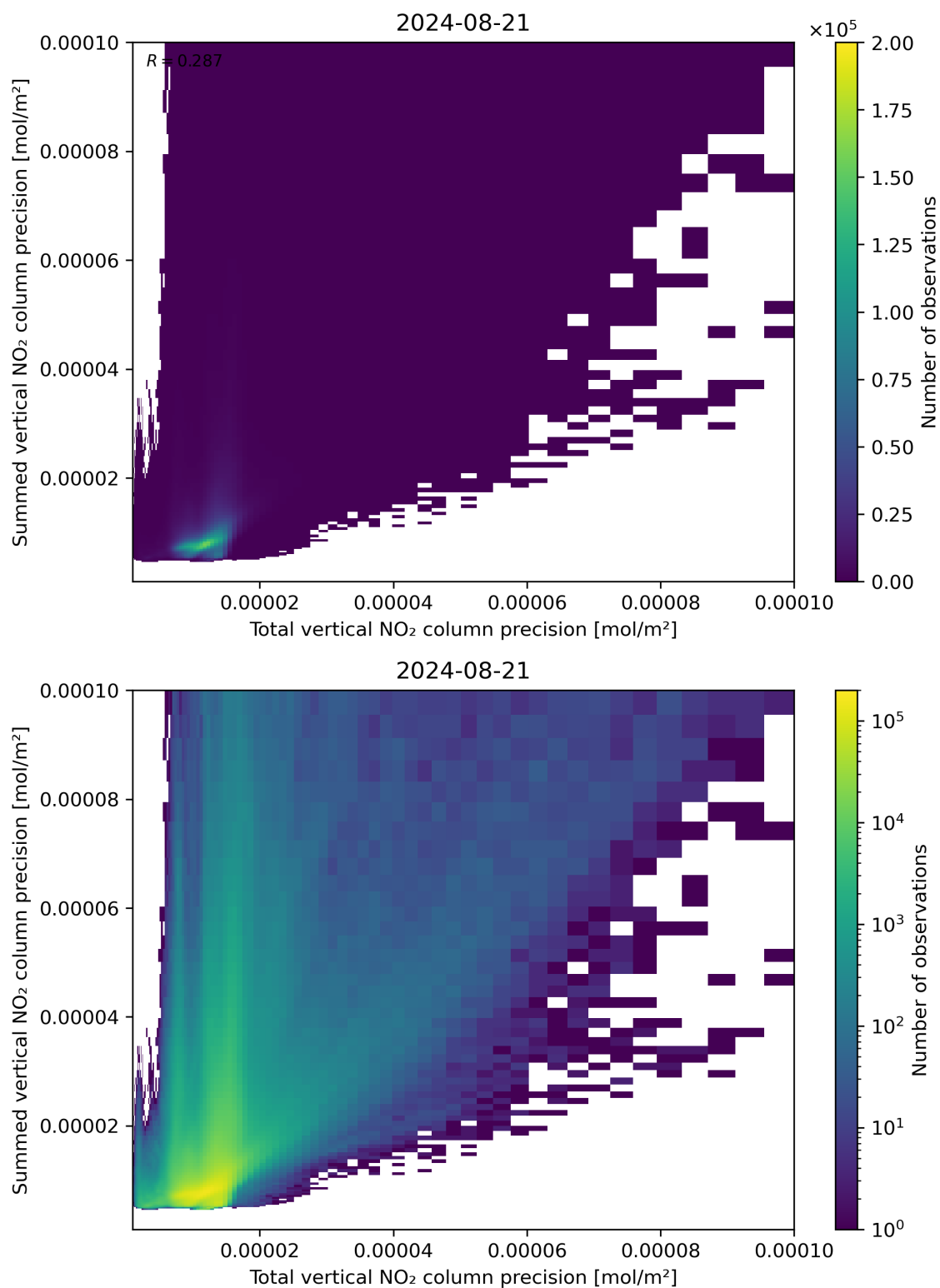
Figure 118: Scatter density plot of “Total vertical NO 2 column precision” against “Summed vertical NO 2 column precision” for 2024-08-21 to 2024-08-22.
