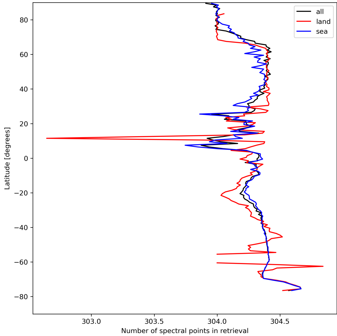
Figure 16: Zonal average of “Number of spectral points in retrieval” for 2024-08-21 to 2024-08-22.
