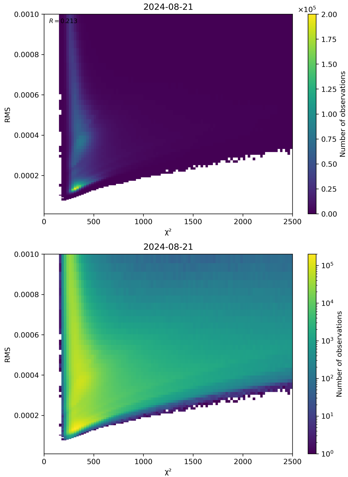
Figure 82: Scatter density plot of “ \chi^2 ” against “RMS” for 2024-08-21 to 2024-08-22.
