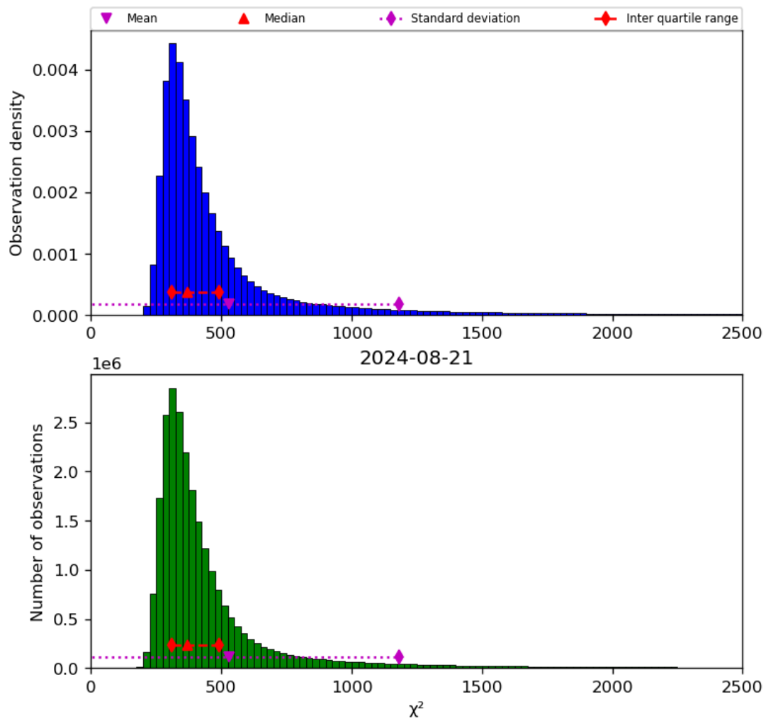
Figure 42: Histogram of " \chi^2 " for 2024-08-21 to 2024-08-22
