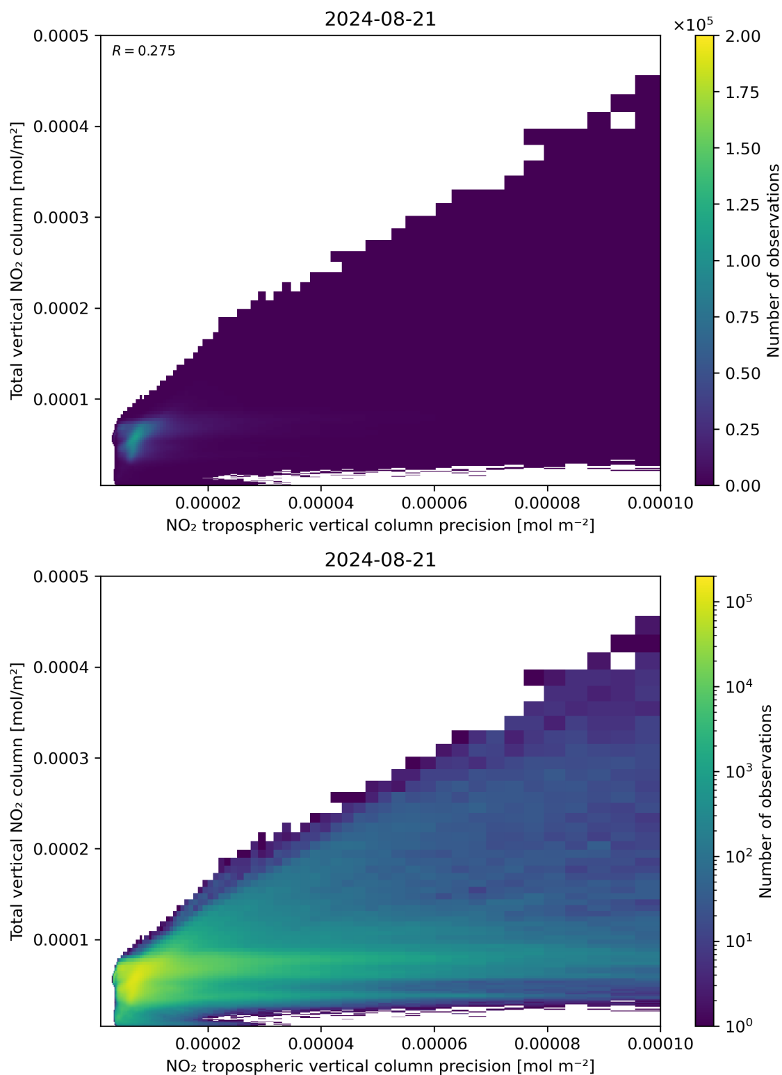
Figure 138: Scatter density plot of “NO 2 tropospheric vertical column precision” against “Total vertical NO 2 column” for 2024-08-21 to 2024-08-22.
