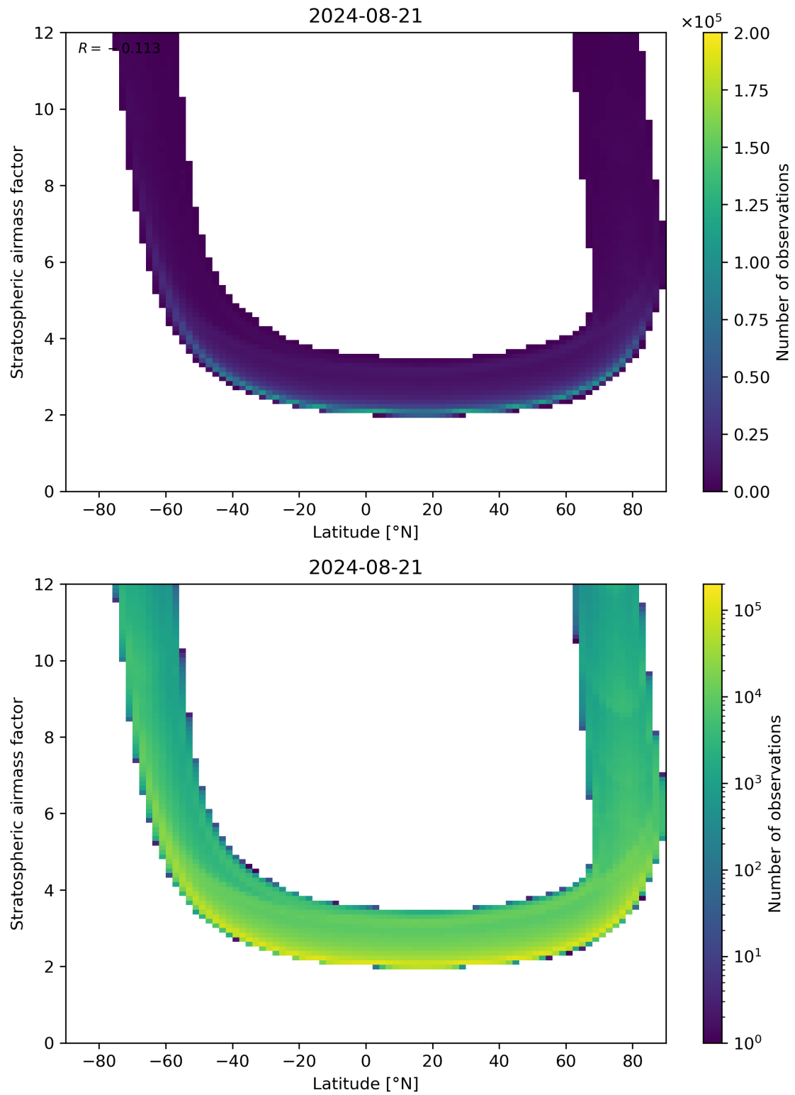
Figure 83: Scatter density plot of “Latitude” against “Stratospheric air mass factor” for 2024-08-21 to 2024-08-22.
