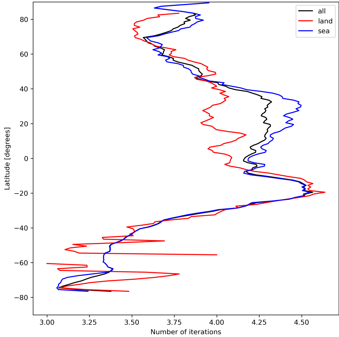
Figure 17: Zonal average of “Number of iterations” for 2024-08-21 to 2024-08-22.
