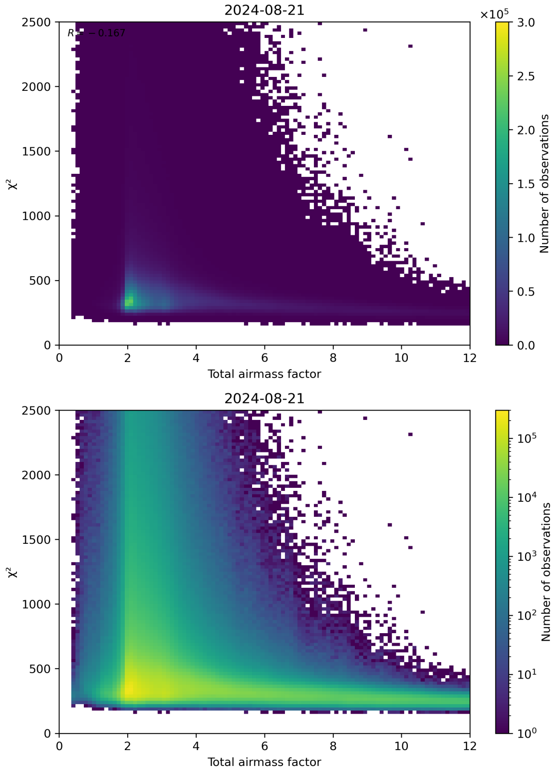
Figure 63: Scatter density plot of “Total airmass factor” against “ \chi^2 ” for 2024-08-21 to 2024-08-22.
