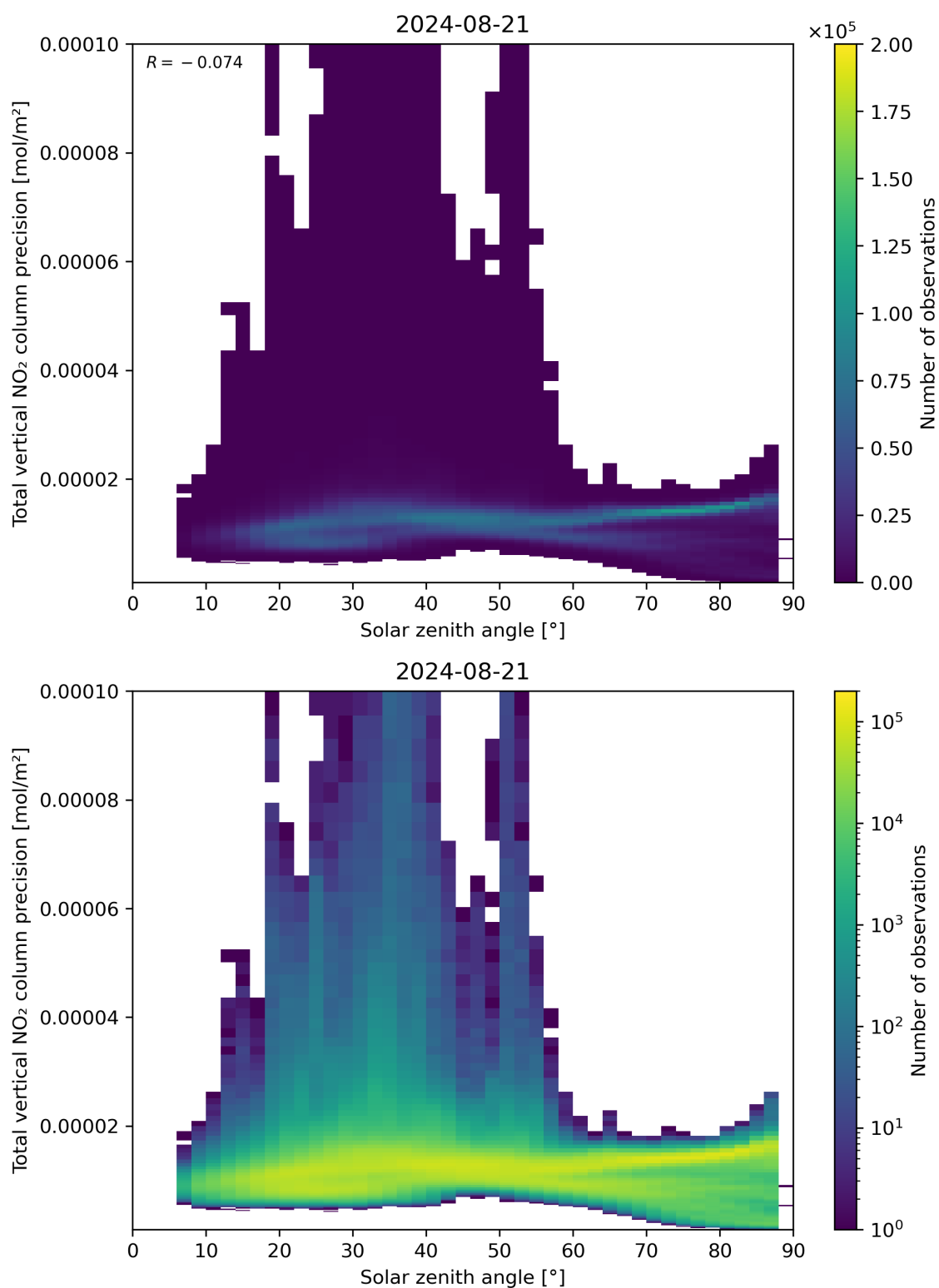
Figure 154: Scatter density plot of “Solar zenith angle” against “Total vertical NO 2 column precision” for 2024-08-21 to 2024-08-22.
