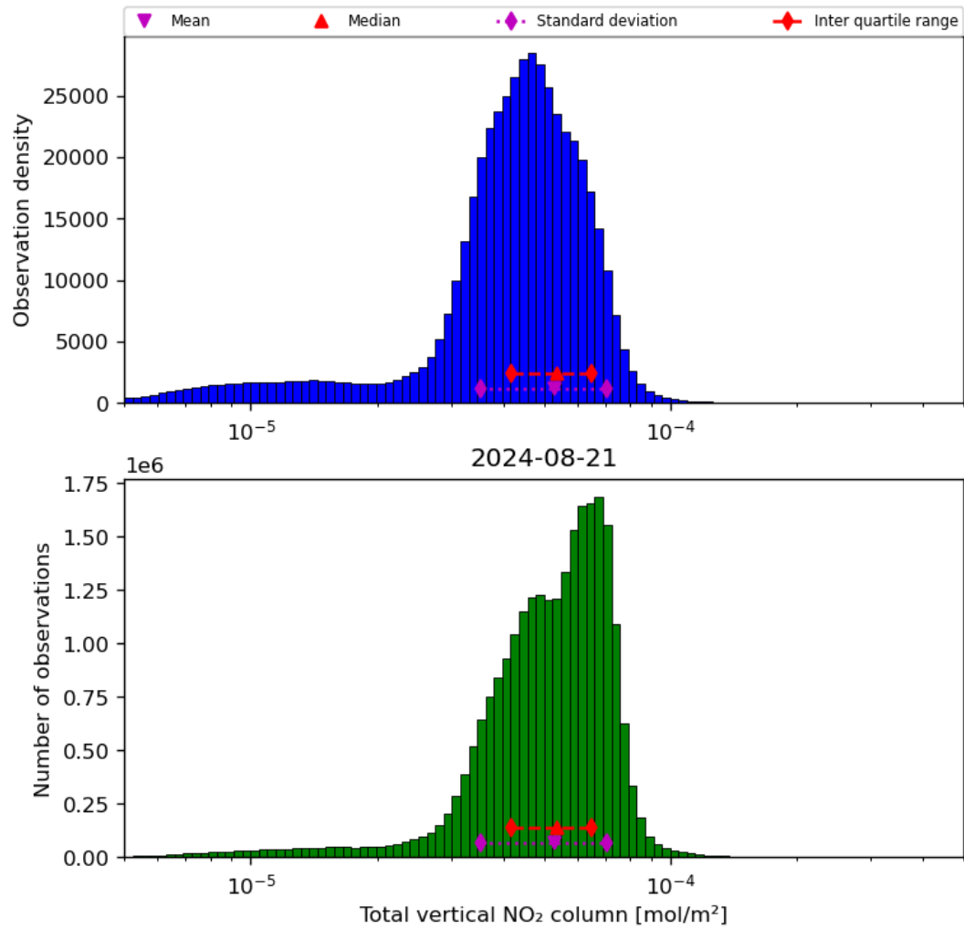
Figure 38: Histogram of “Total vertical NO 2 column” for 2024-08-21 to 2024-08-22
