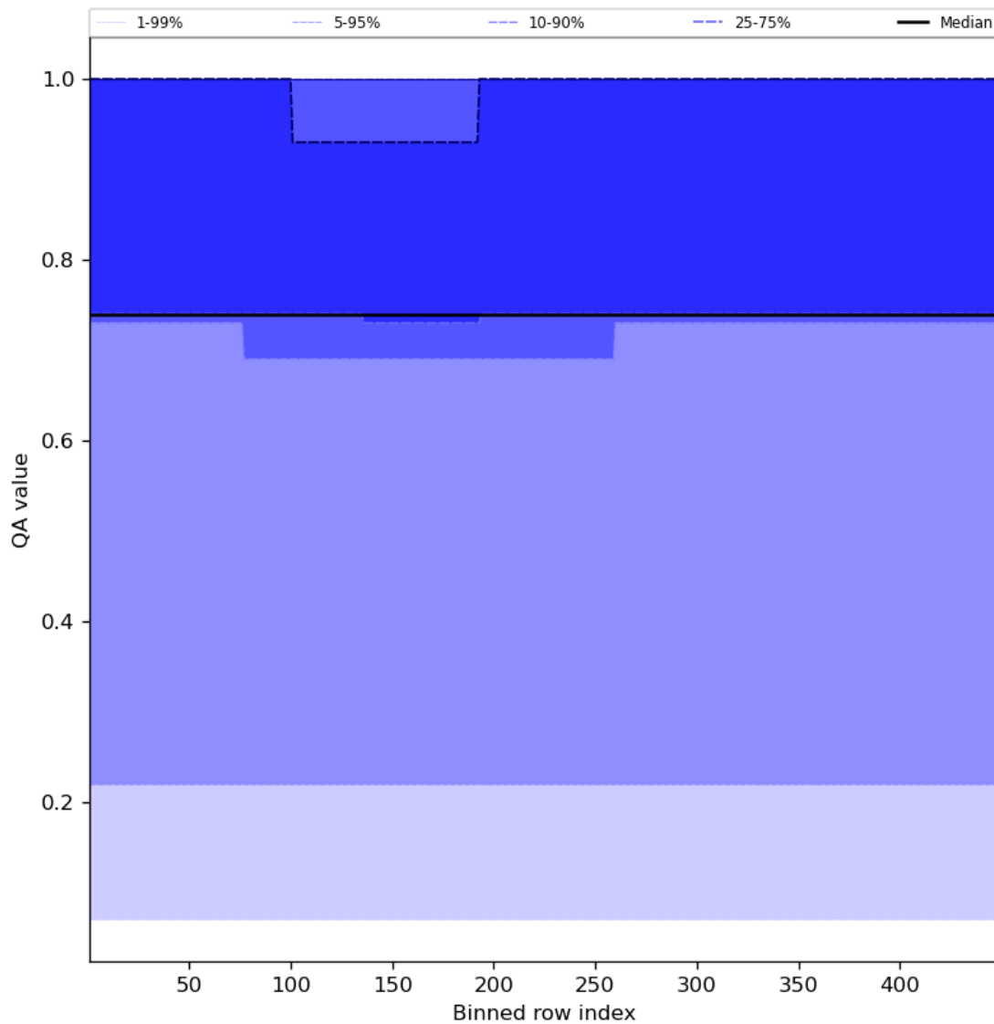
Figure 45: Along track statistics of “QA value” for 2024-08-21 to 2024-08-22
