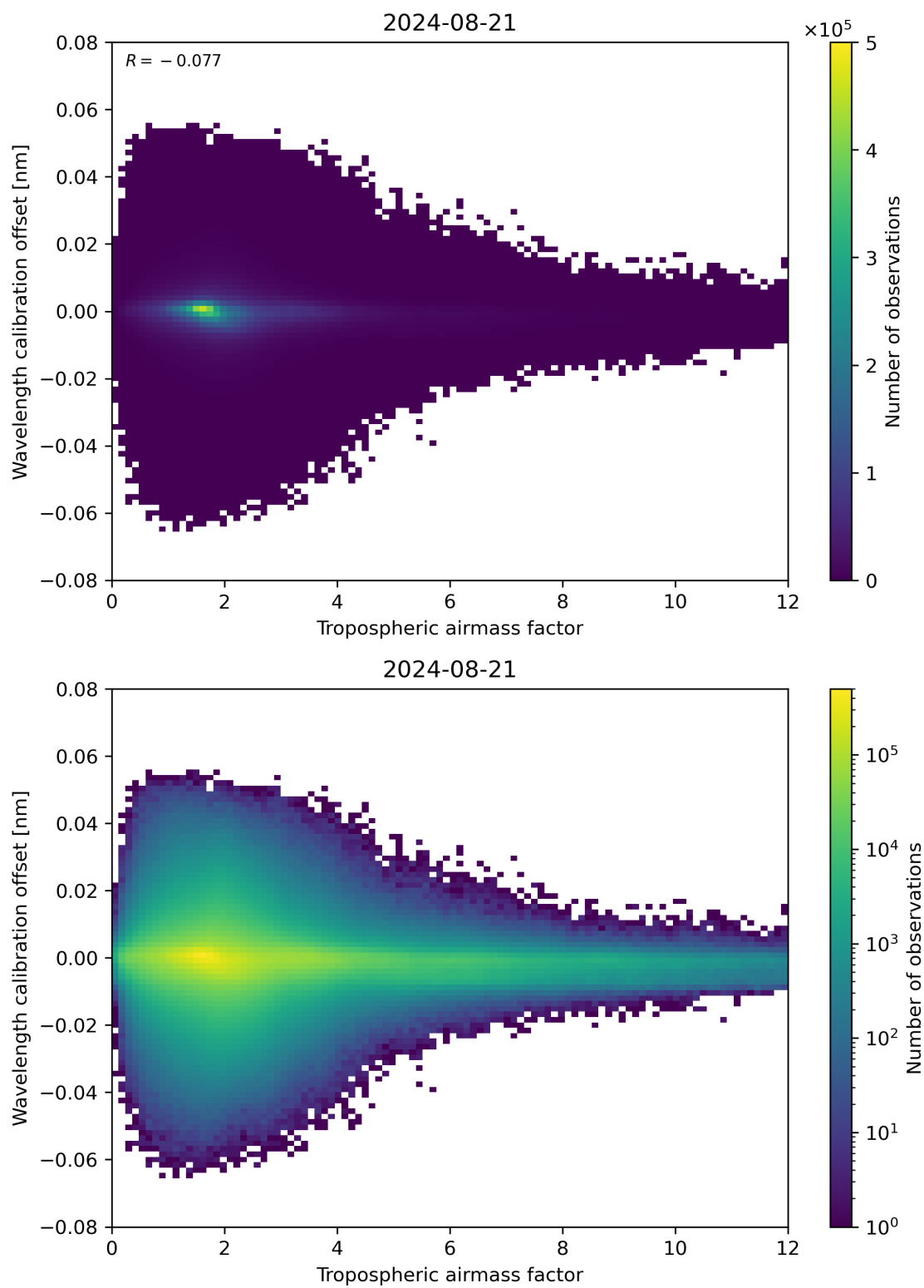
Figure 80: Scatter density plot of “Tropospheric air mass factor” against “Wavelength calibration offset” for 2024-08-21 to 2024-08-22.
