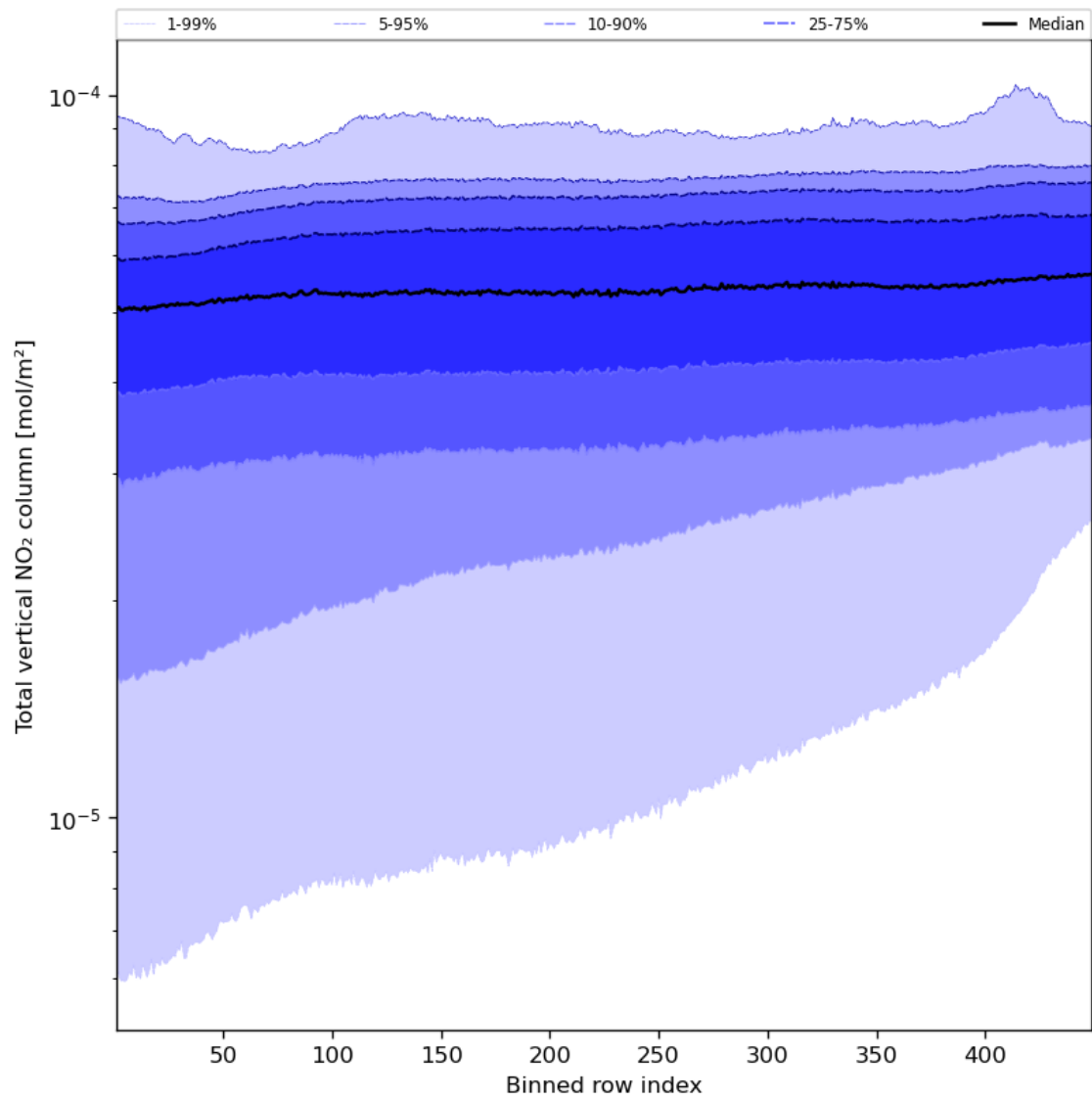
Figure 55: Along track statistics of “Total vertical NO 2 column” for 2024-08-21 to 2024-08-22
