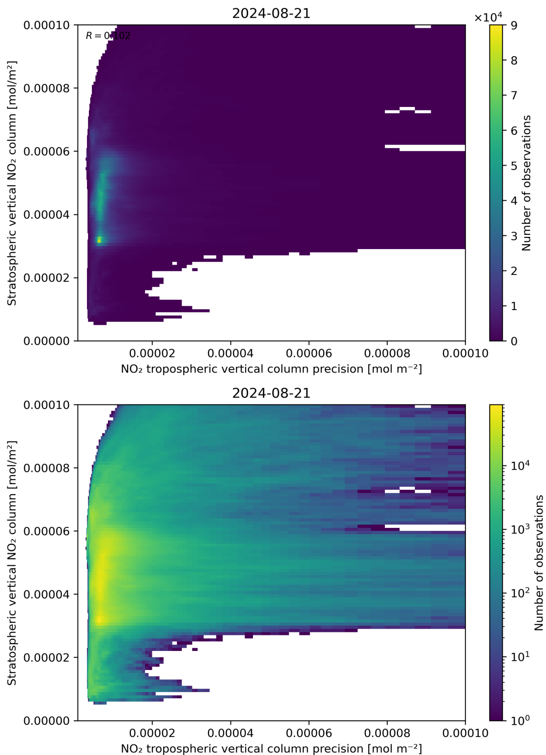
Figure 135: Scatter density plot of “NO 2 tropospheric vertical column precision” against “Stratospheric vertical NO 2 column” for 2024-08-21 to 2024-08-22.
