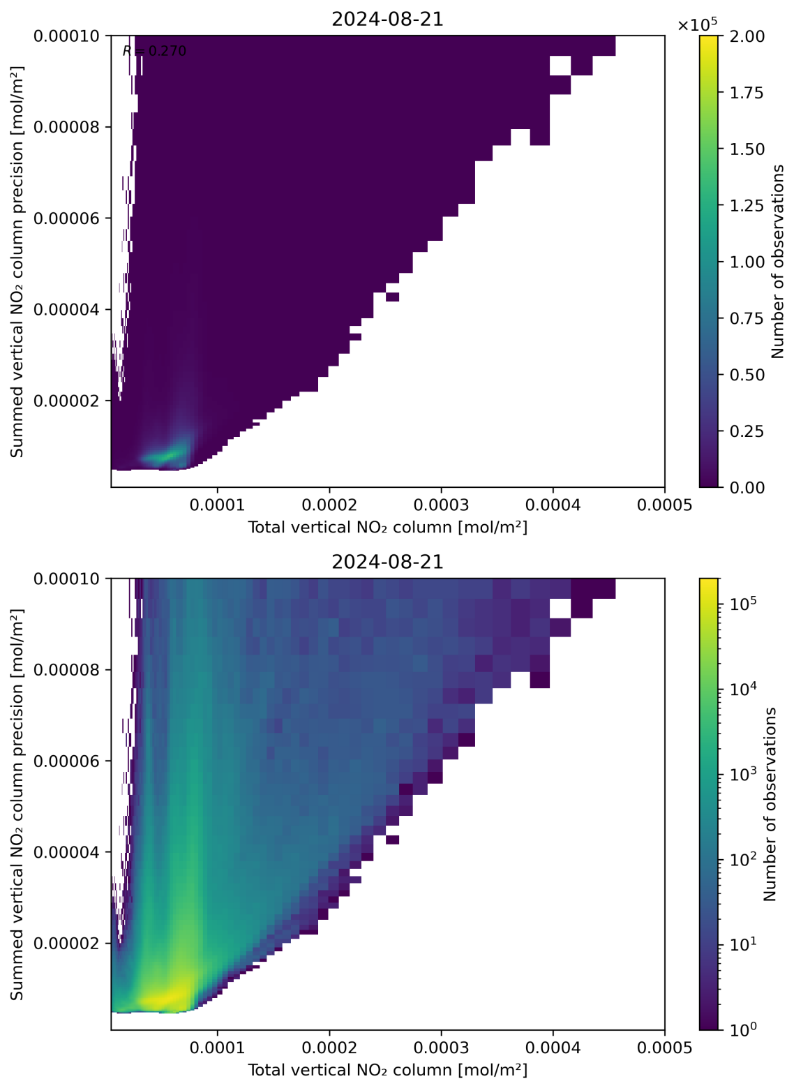
Figure 113: Scatter density plot of “Total vertical NO 2 column” against “Summed vertical NO 2 column precision” for 2024-08-21 to 2024-08-22.
