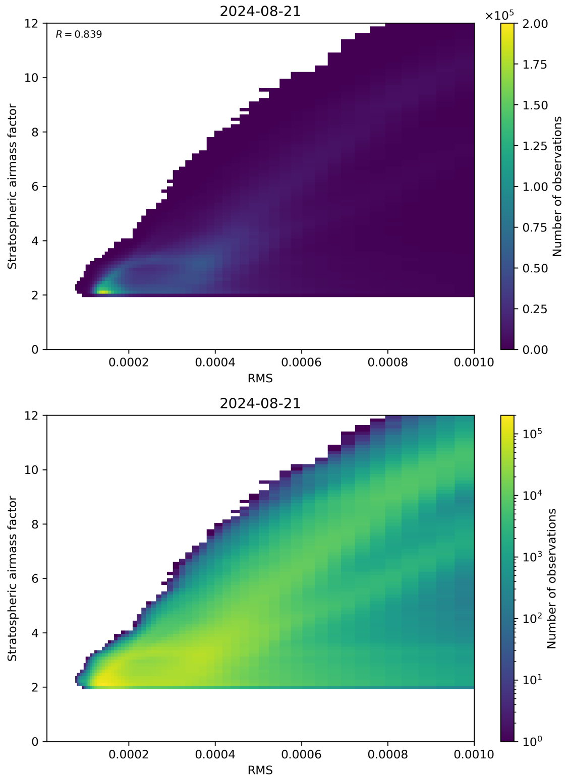
Figure 144: Scatter density plot of “RMS” against “Stratospheric airmass factor” for 2024-08-21 to 2024-08-22.
