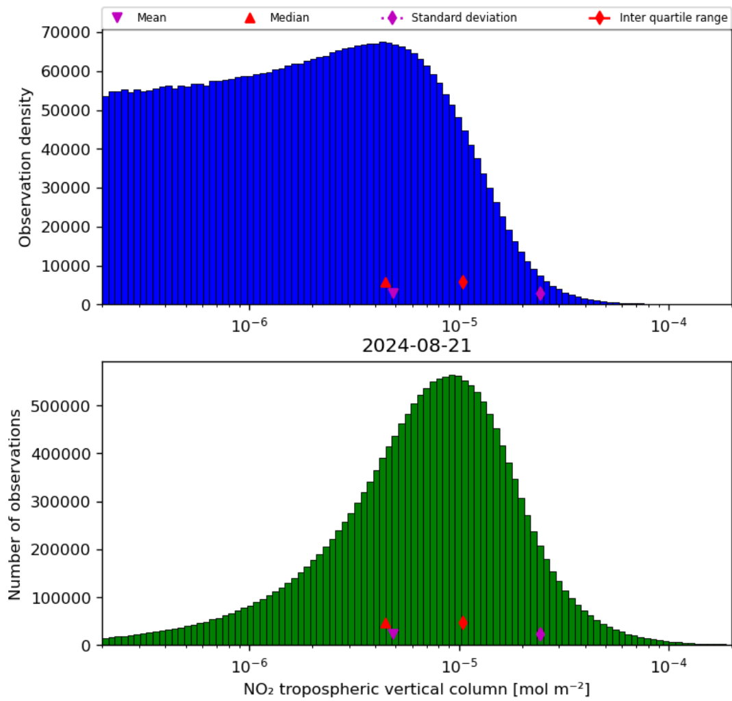
Figure 29: Histogram of “NO 2 tropospheric vertical column” for 2024-08-21 to 2024-08-22
