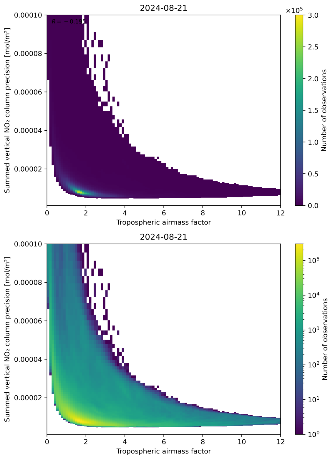
Figure 76: Scatter density plot of “Tropospheric air mass factor” against “Summed vertical NO 2 column precision” for 2024-08-21 to 2024-08-22.
