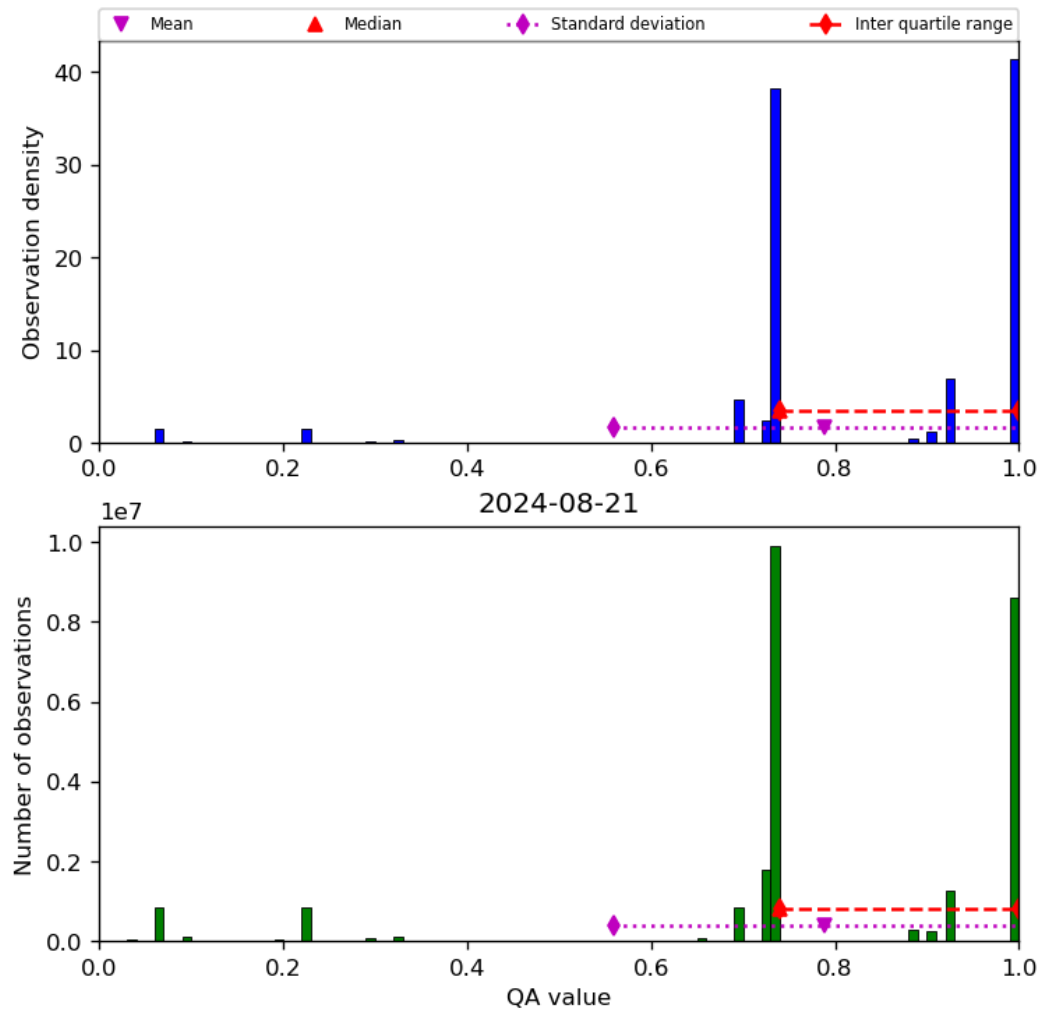
Figure 28: Histogram of “QA value” for 2024-08-21 to 2024-08-22
