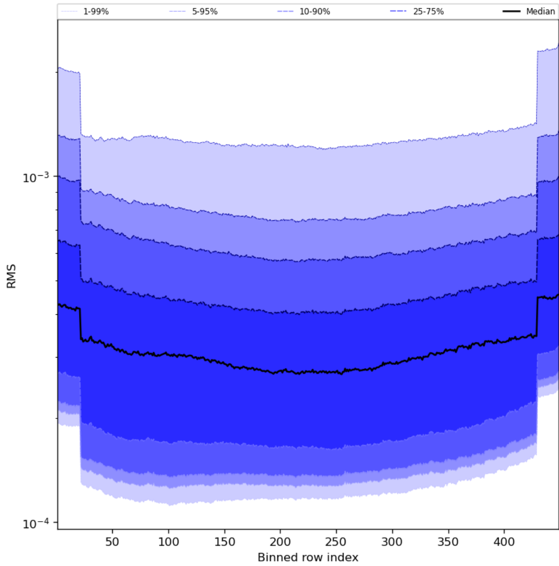
Figure 60: Along track statistics of “RMS” for 2024-08-21 to 2024-08-22
