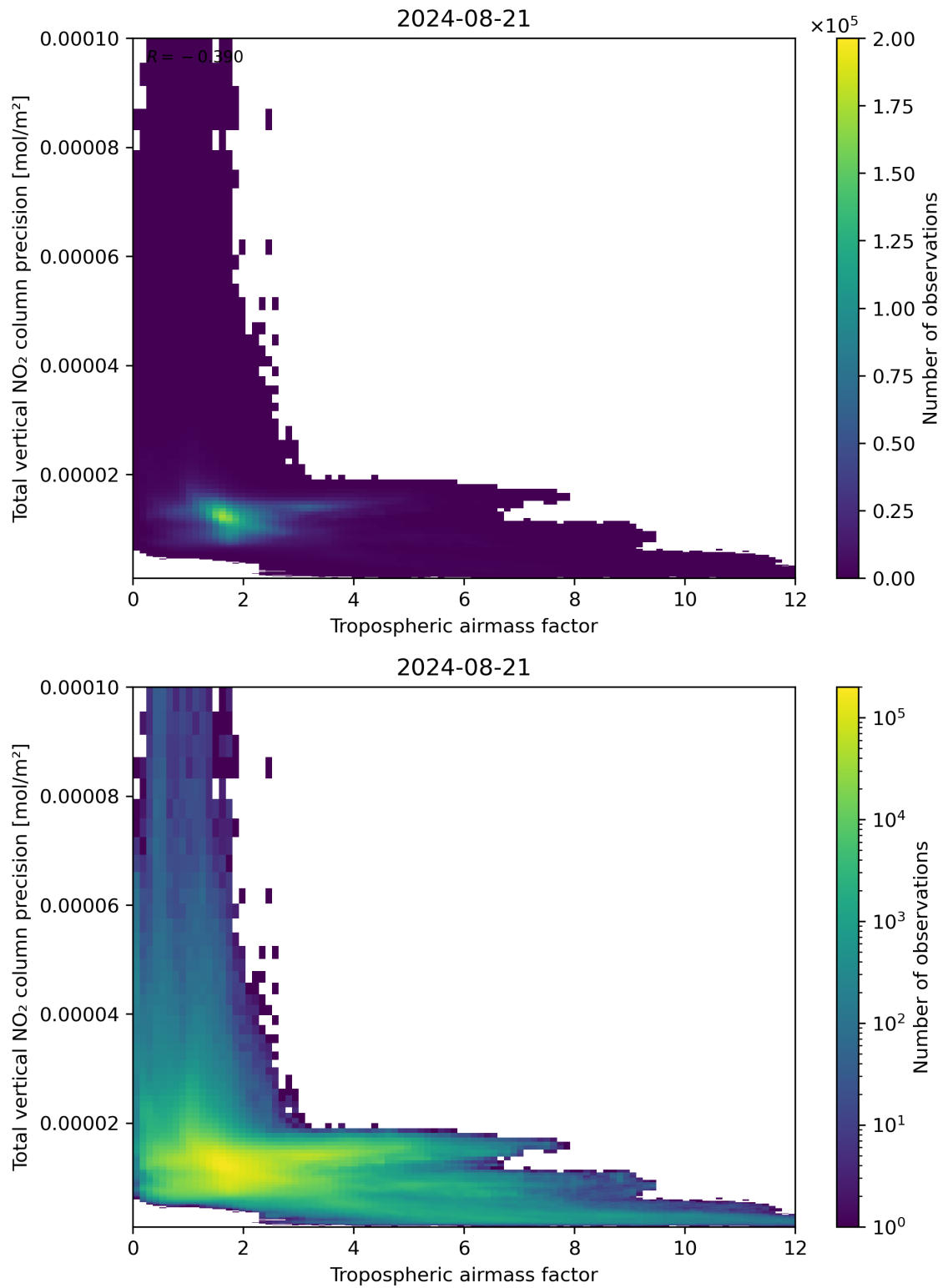
Figure 78: Scatter density plot of “Tropospheric air mass factor” against “Total vertical NO 2 column precision” for 2024-08-21 to 2024-08-22.
