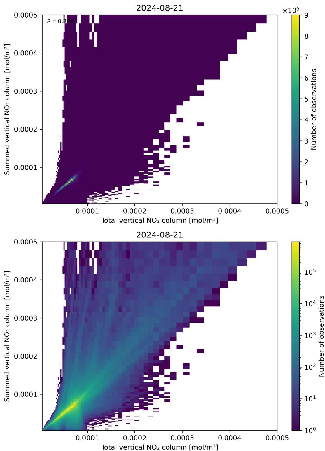
Figure 112: Scatter density plot of “Total vertical NO 2 column” against “Summed vertical NO 2 column” for 2024-08-21 to 2024-08-22.
