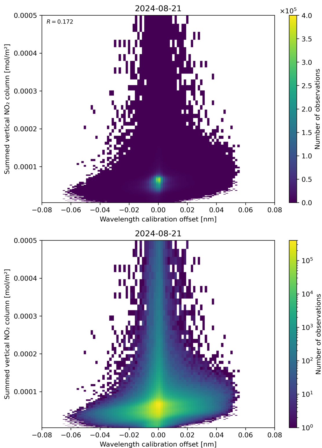
Figure 177: Scatter density plot of “Wavelength calibration offset” against “Summed vertical NO 2 column” for 2024-08-21 to 2024-08-22.
