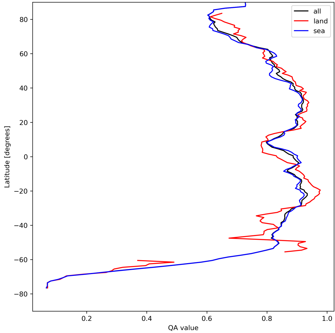
Figure 11: Zonal average of “QA value” for 2024-08-21 to 2024-08-22.
