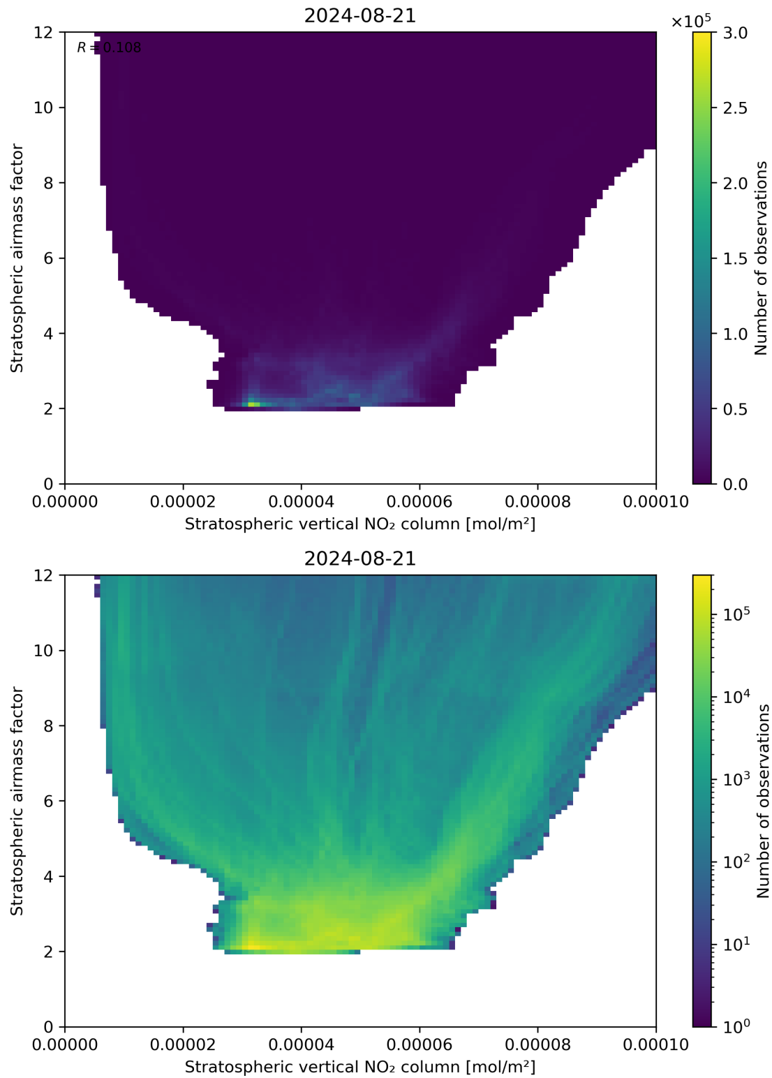
Figure 96: Scatter density plot of “Stratospheric vertical NO 2 column” against “Stratospheric airmass factor” for 2024-08-21 to 2024-08-22.
