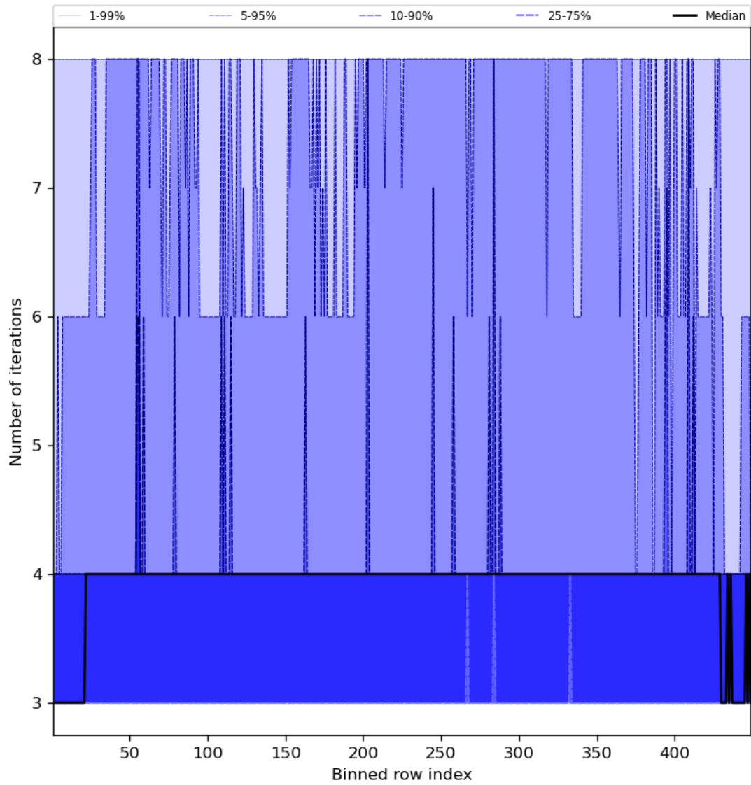
Figure 51: Along track statistics of “Number of iterations” for 2024-08-21 to 2024-08-22
