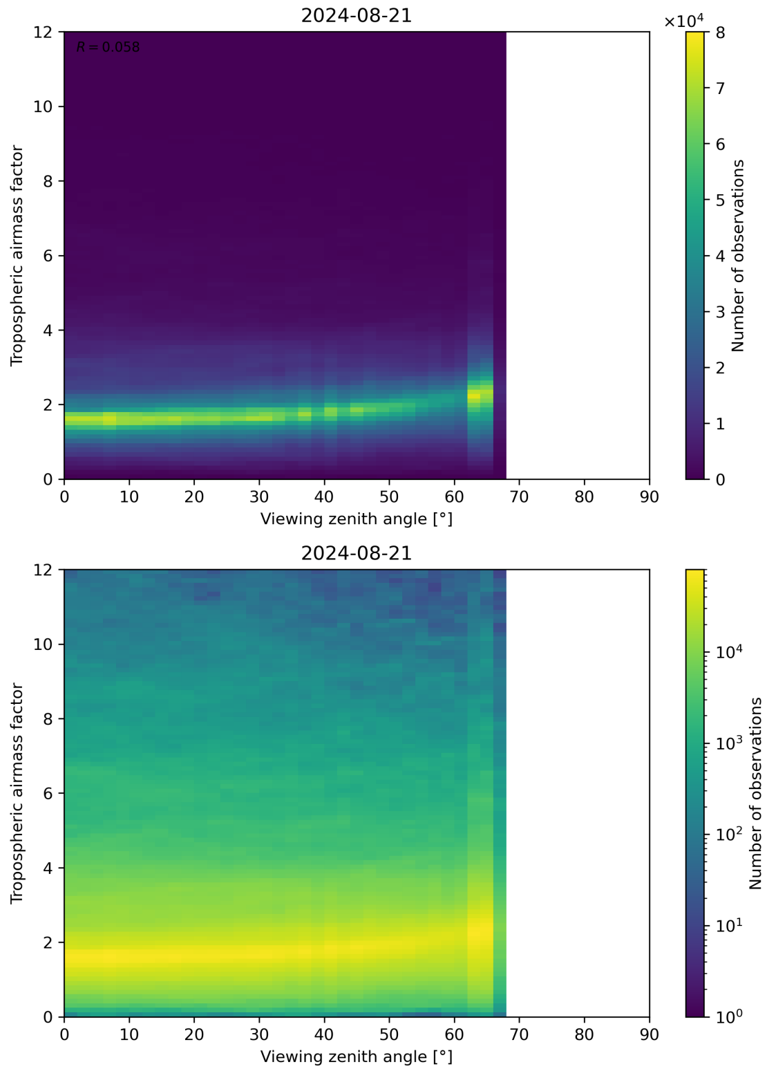
Figure 161: Scatter density plot of “Viewing zenith angle” against “Tropospheric airmass factor” for 2024-08-21 to 2024-08-22.
