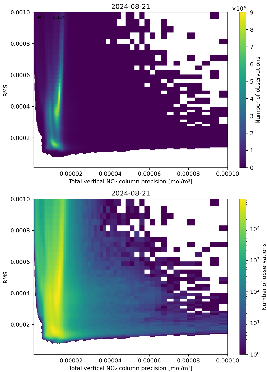
Figure 119: Scatter density plot of “Total vertical NO 2 column precision” against “RMS” for 2024-08-21 to 2024-08-22.
