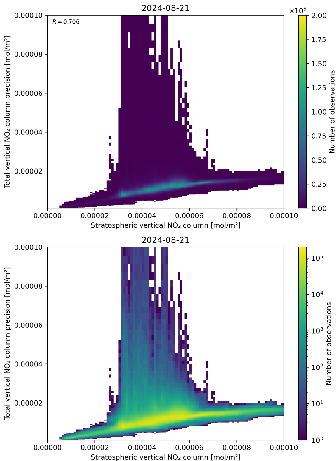
Figure 101: Scatter density plot of “Stratospheric vertical NO 2 column” against “Total vertical NO 2 column precision” for 2024-08-21 to 2024-08-22.
