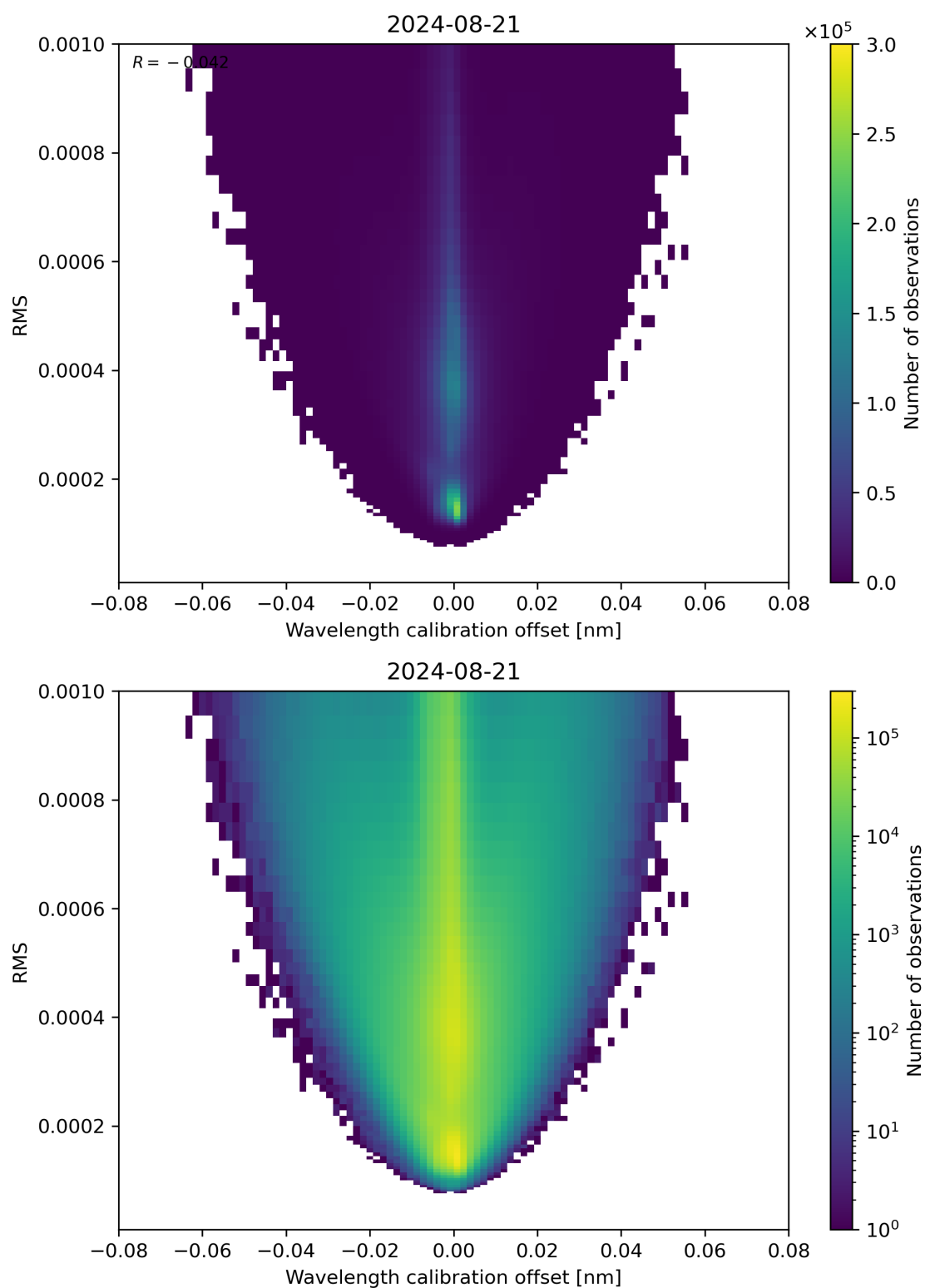
Figure 181: Scatter density plot of “Wavelength calibration offset” against “RMS” for 2024-08-21 to 2024-08-22.
