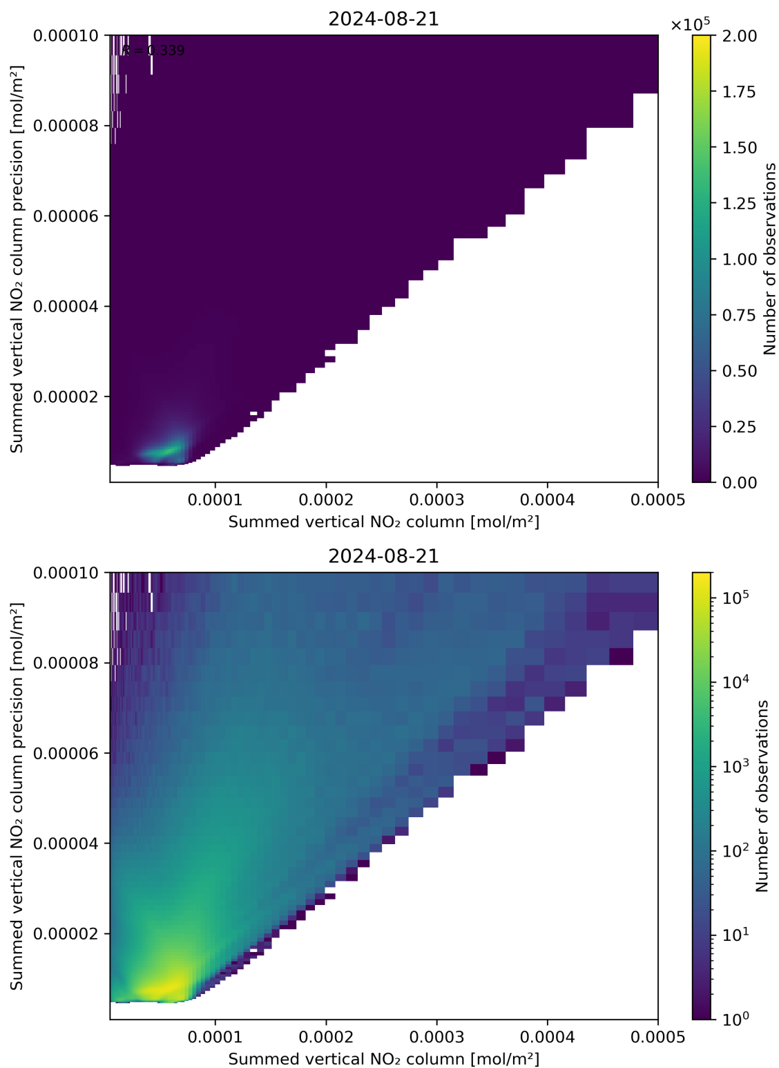
Figure 105: Scatter density plot of “Summed vertical NO 2 column” against “Summed vertical NO 2 column precision” for 2024-08-21 to 2024-08-22.
