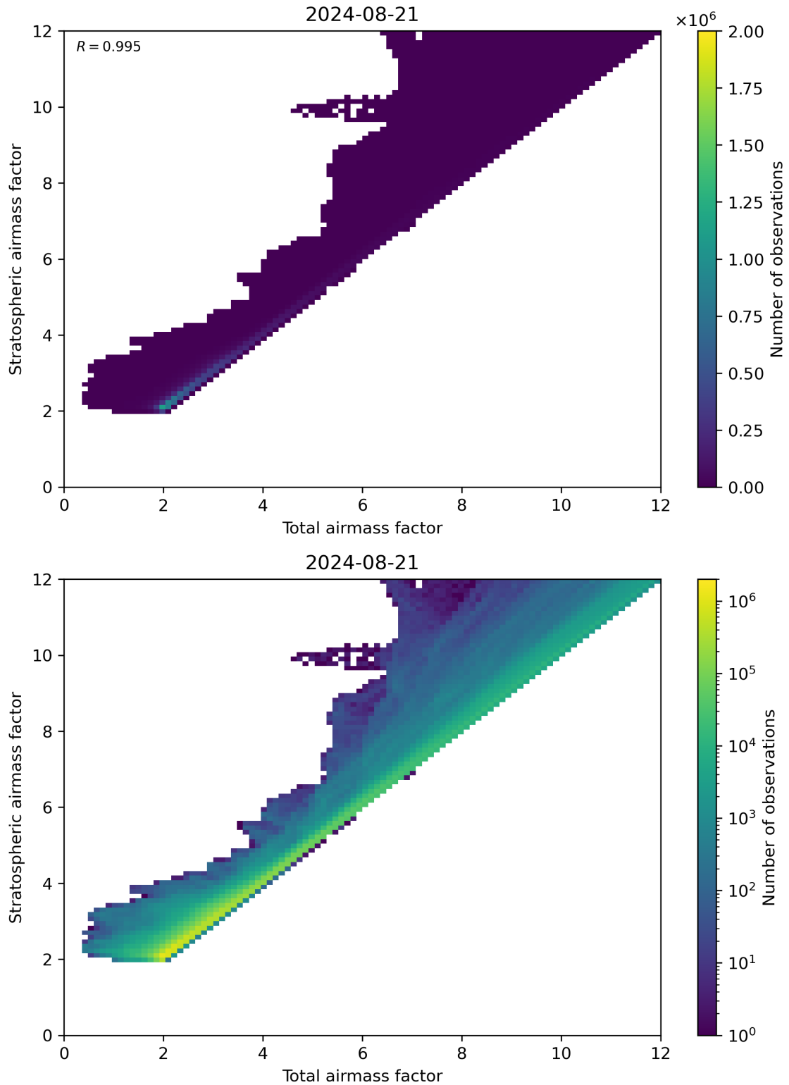
Figure 62: Scatter density plot of “Total airmass factor” against “Stratospheric airmass factor” for 2024-08-21 to 2024-08-22.
