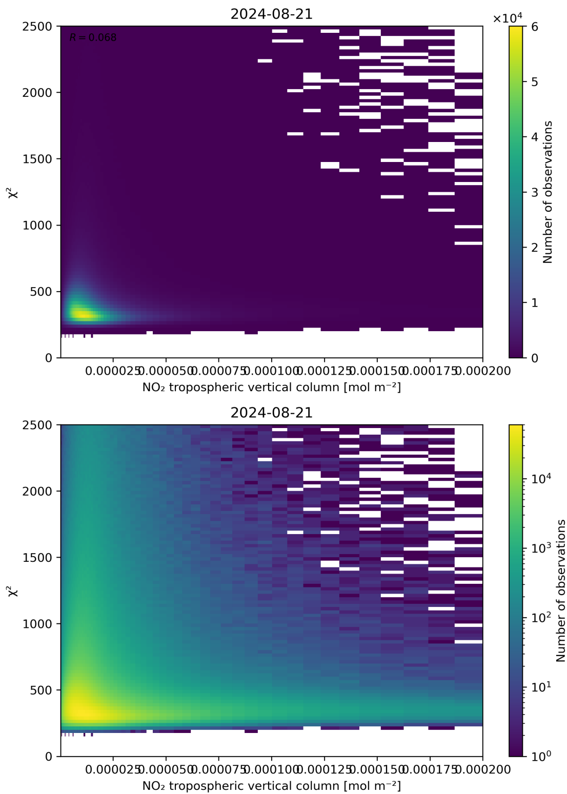
Figure 124: Scatter density plot of “NO 2 tropospheric vertical column” against “ \chi^2 ” for 2024-08-21 to 2024-08-22.
