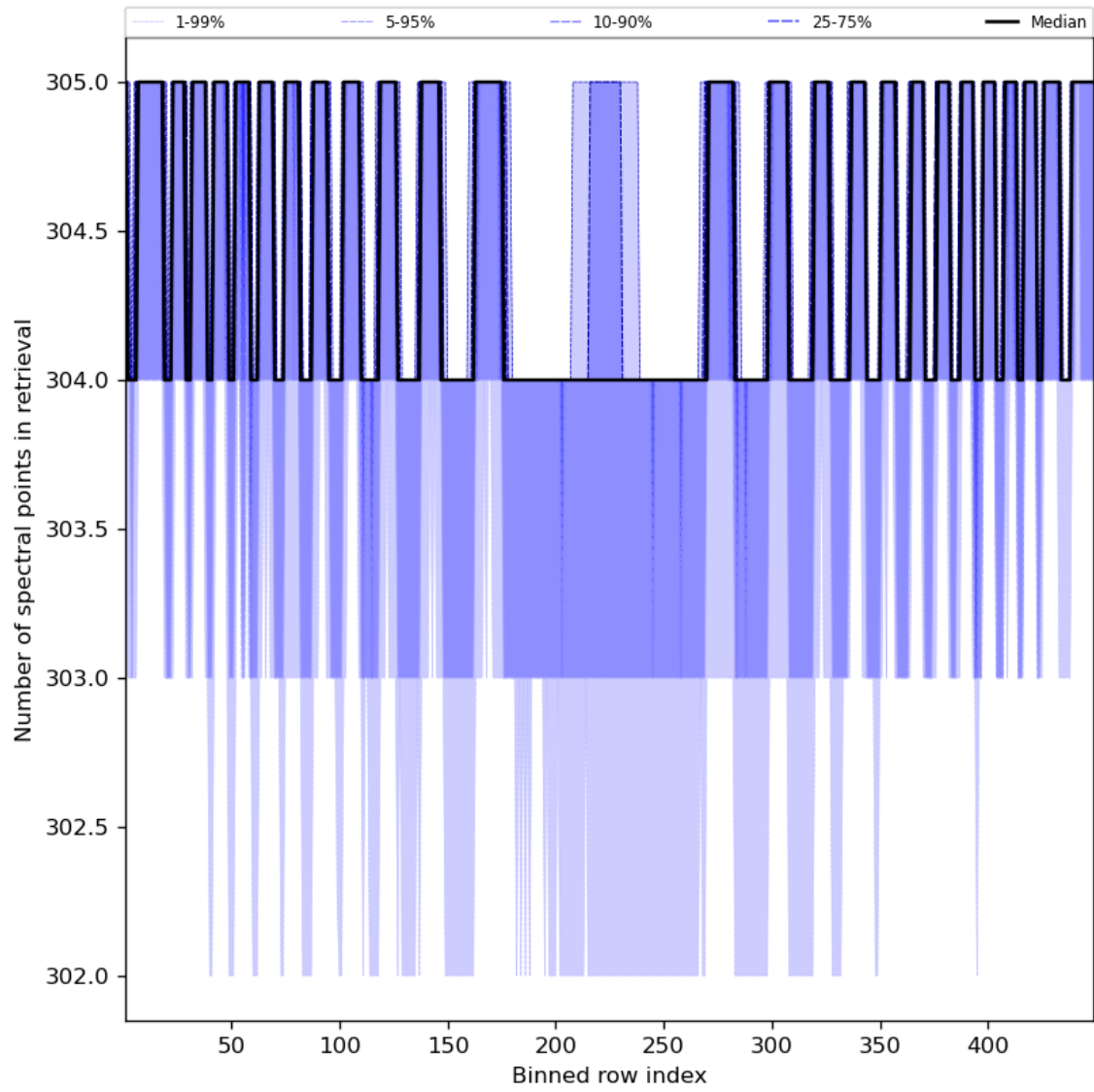
Figure 50: Along track statistics of “Number of spectral points in retrieval” for 2024-08-21 to 2024-08-22
