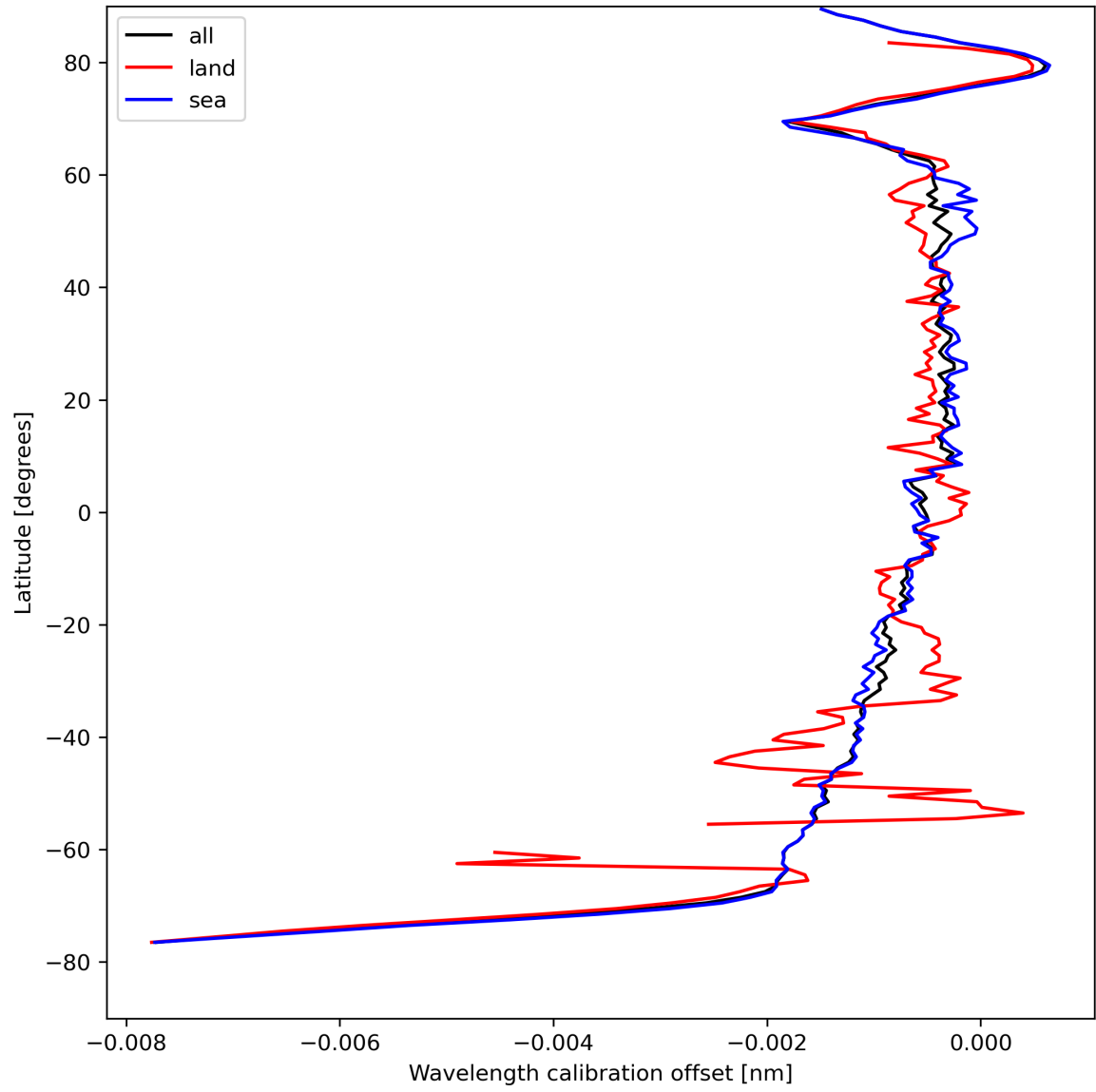
Figure 18: Zonal average of “Wavelength calibration offset” for 2024-08-21 to 2024-08-22.
