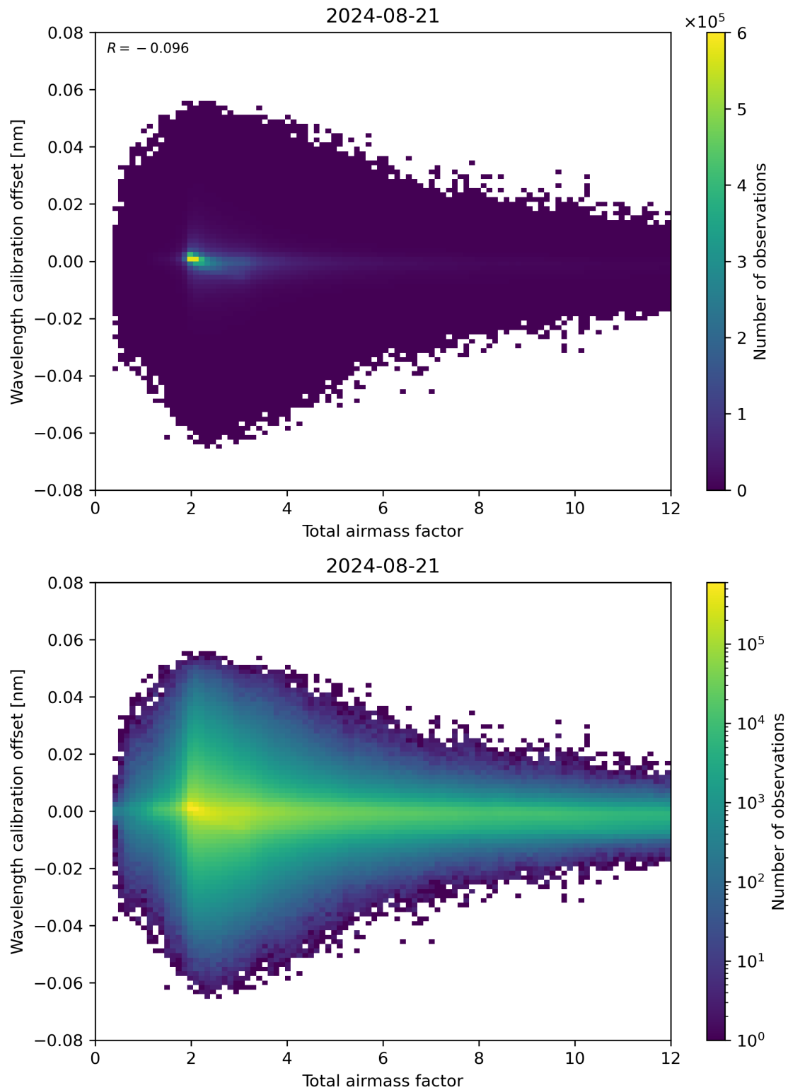
Figure 70: Scatter density plot of “Total airmass factor” against “Wavelength calibration offset” for 2024-08-21 to 2024-08-22.
