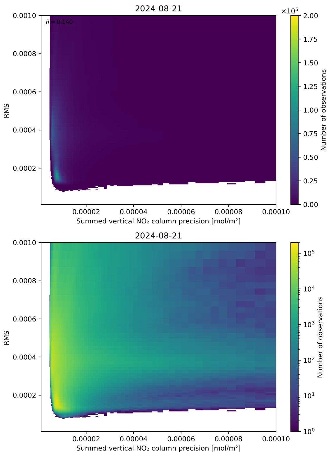
Figure 108: Scatter density plot of “Summed vertical NO 2 column precision” against “RMS” for 2024-08-21 to 2024-08-22.
