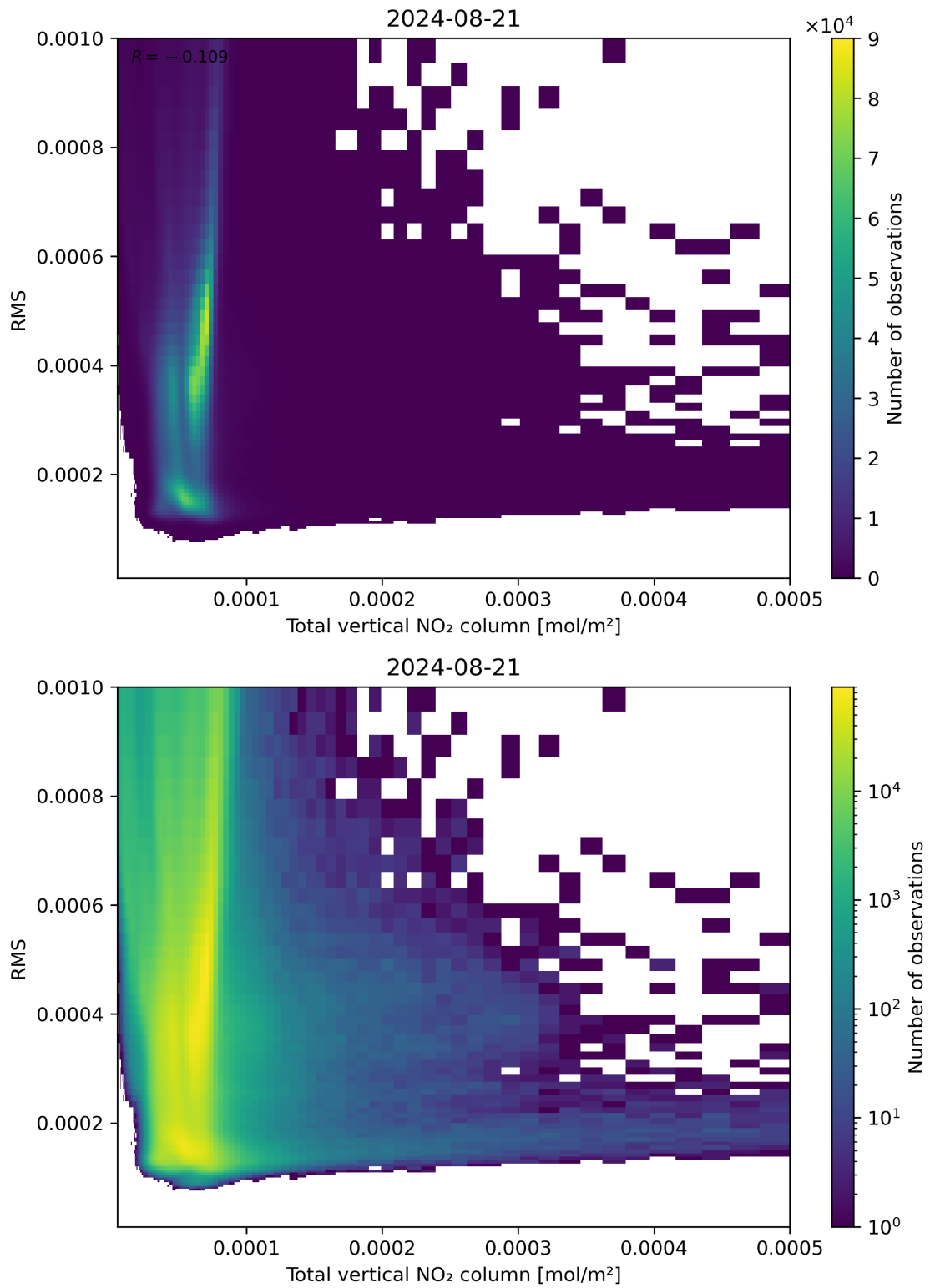
Figure 120: Scatter density plot of “Total vertical NO 2 column” against “RMS” for 2024-08-21 to 2024-08-22.
