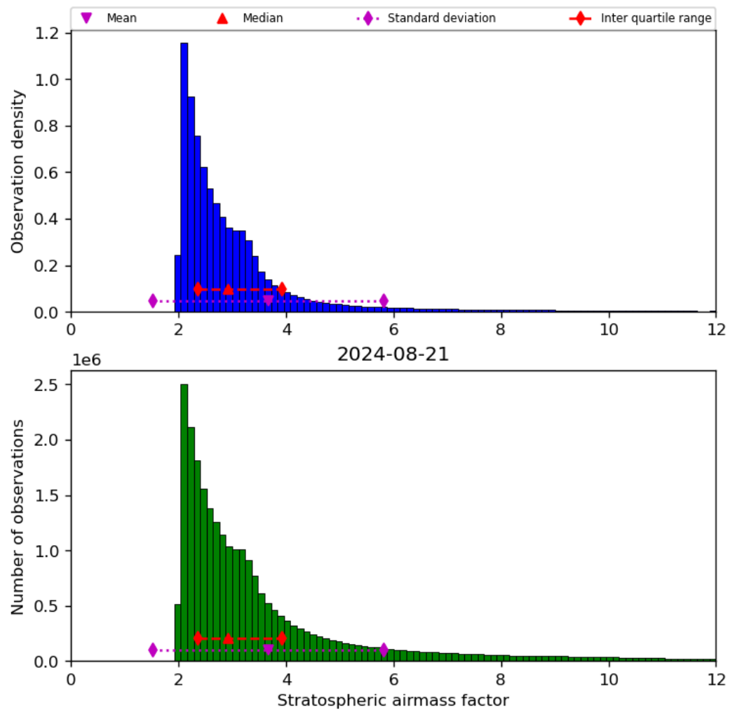
Figure 44: Histogram of “Stratospheric airmass factor” for 2024-08-21 to 2024-08-22
