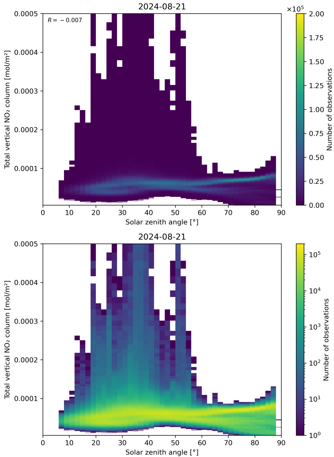
Figure 153: Scatter density plot of “Solar zenith angle” against “Total vertical NO 2 column” for 2024-08-21 to 2024-08-22.
