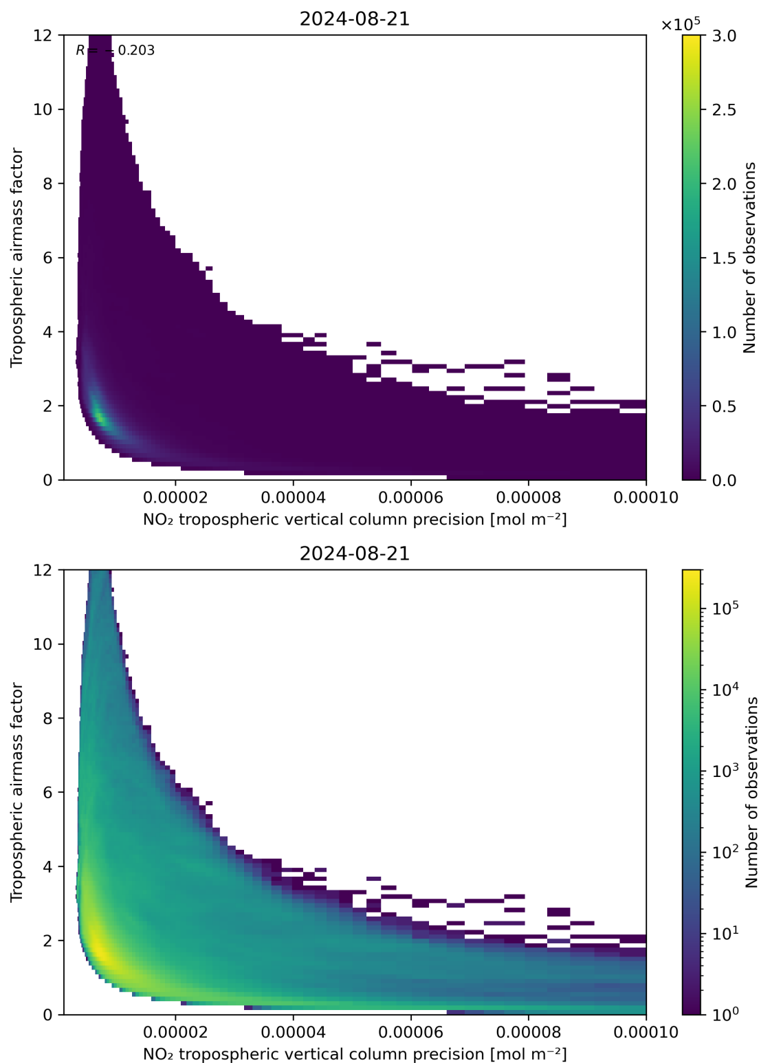
Figure 133: Scatter density plot of “NO 2 tropospheric vertical column precision” against “Tropospheric airmass factor” for 2024-08-21 to 2024-08-22.
