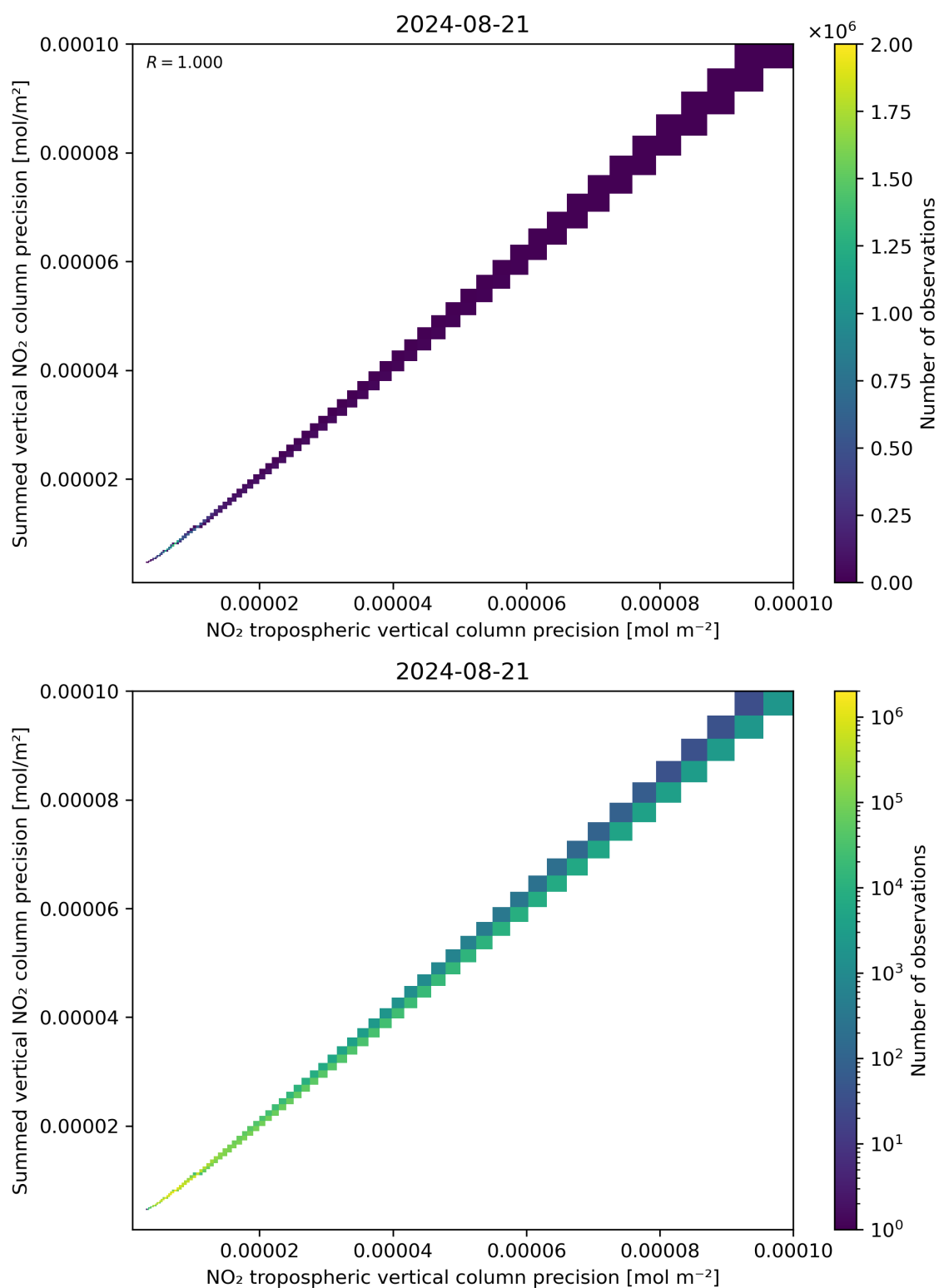
Figure 137: Scatter density plot of “NO 2 tropospheric vertical column precision” against “Summed vertical NO 2 column precision” for 2024-08-21 to 2024-08-22.
