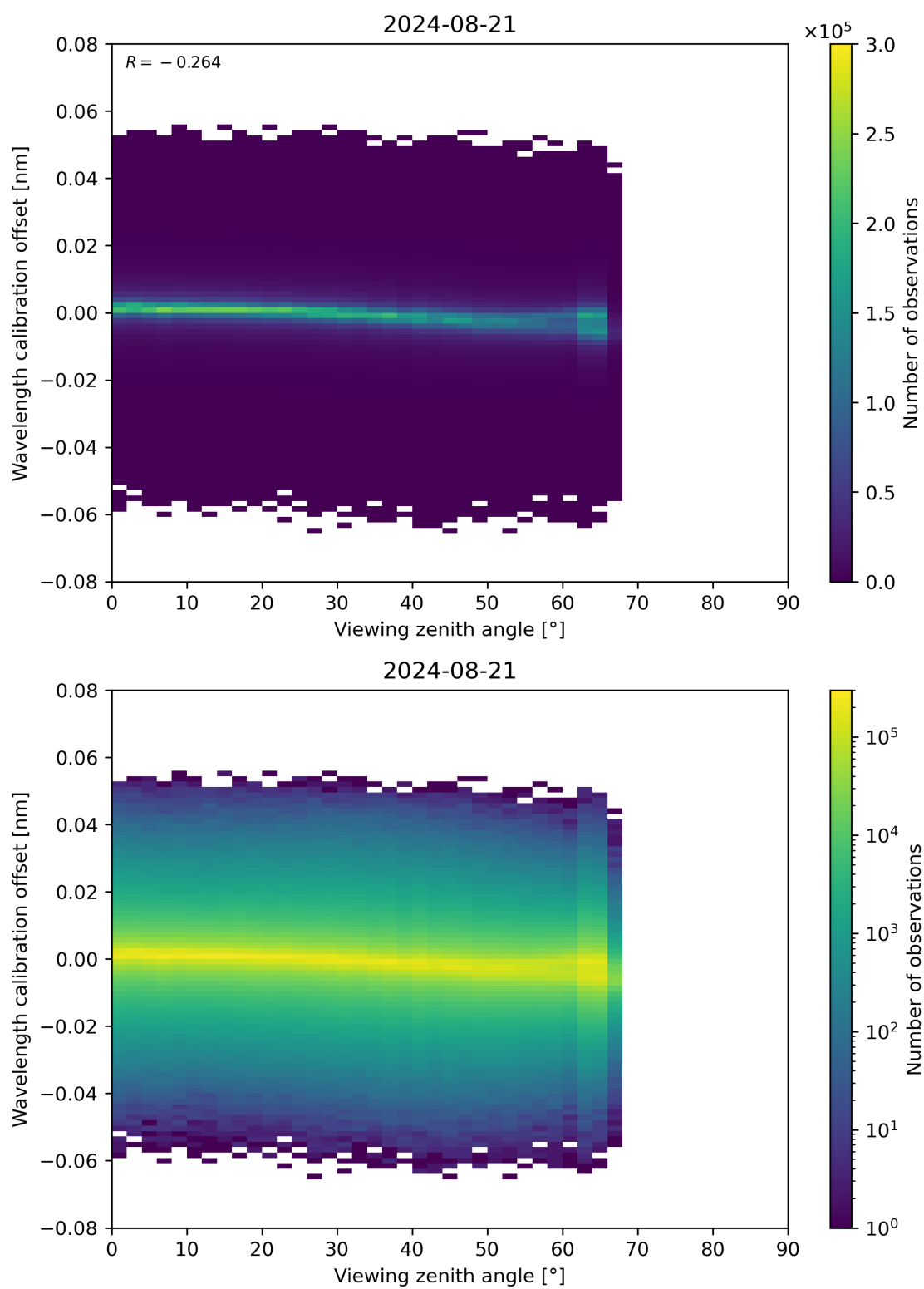
Figure 173: Scatter density plot of “Viewing zenith angle” against “Wavelength calibration offset” for 2024-08-21 to 2024-08-22.
