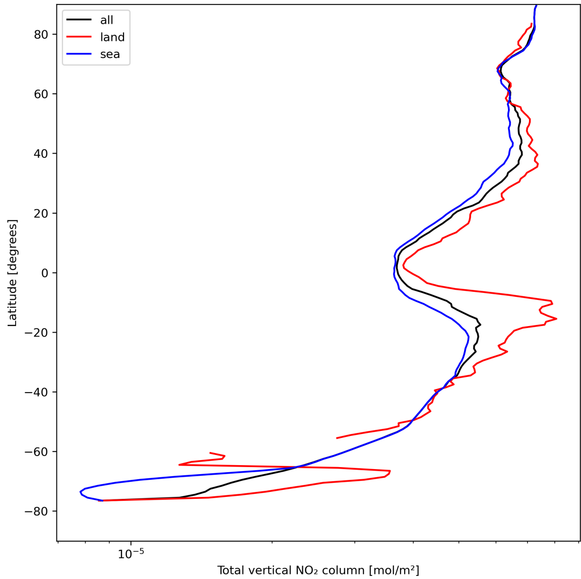
Figure 21: Zonal average of “Total vertical NO 2 column” for 2024-08-21 to 2024-08-22.
