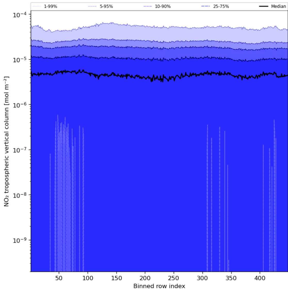
Figure 46: Along track statistics of “NO 2 tropospheric vertical column” for 2024-08-21 to 2024-08-22
