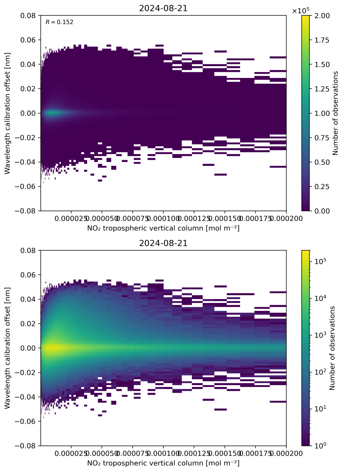
Figure 143: Scatter density plot of “NO 2 tropospheric vertical column” against “Wavelength calibration offset” for 2024-08-21 to 2024-08-22.
