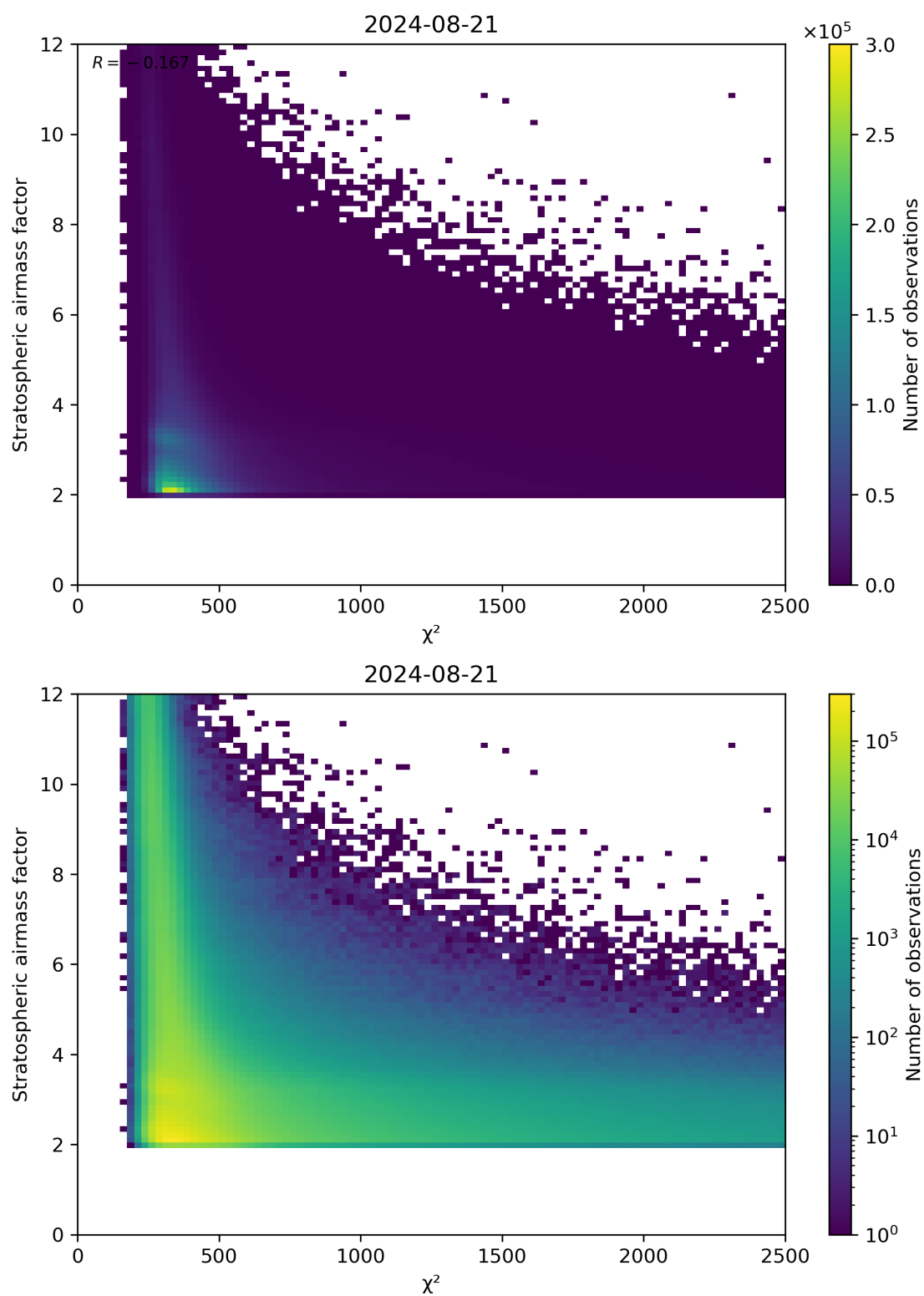
Figure 81: Scatter density plot of " \chi^2 " against "Stratospheric airmass factor" for 2024-08-21 to 2024-08-22.
