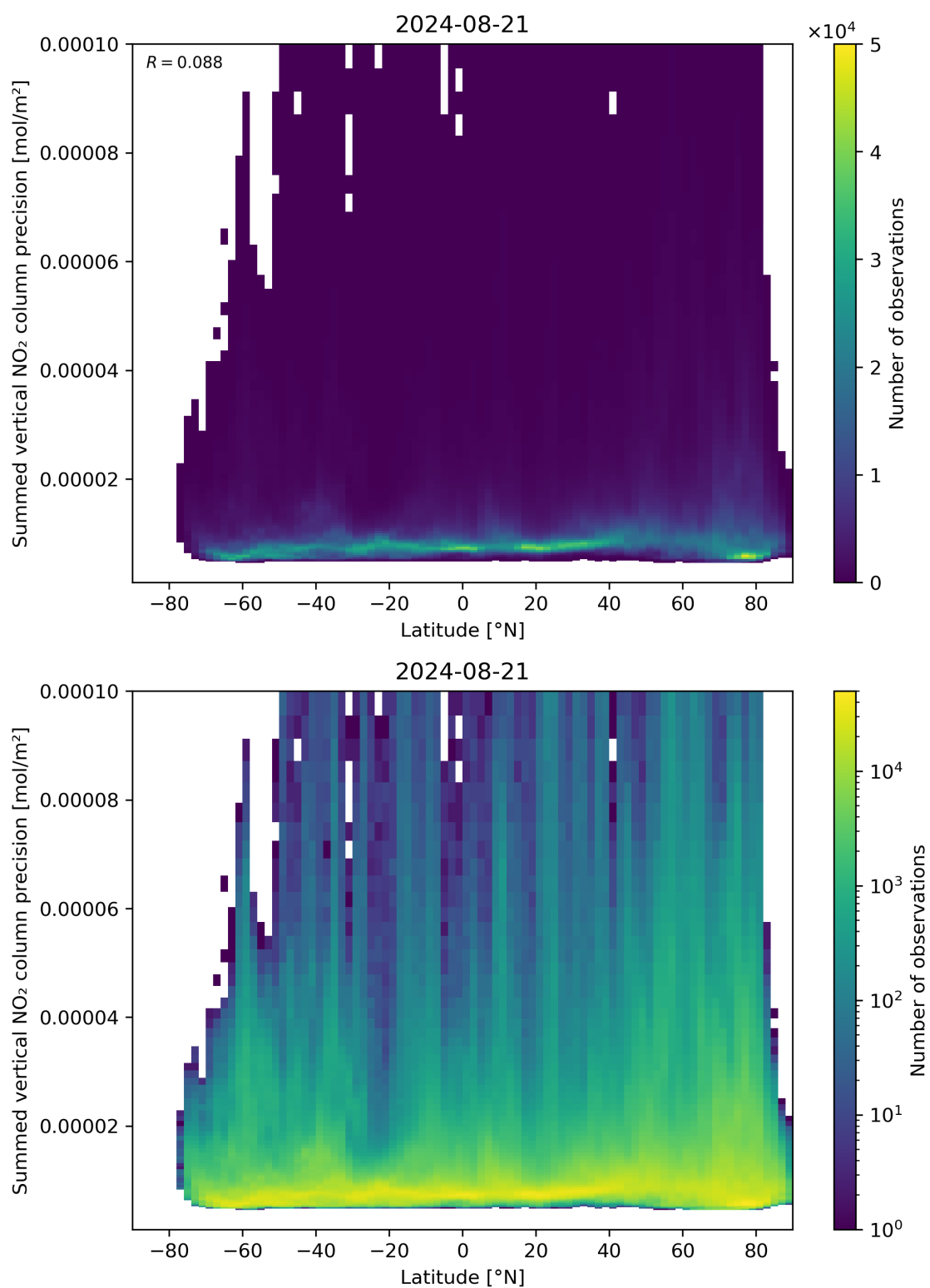
Figure 89: Scatter density plot of “Latitude” against “Summed vertical NO 2 column precision” for 2024-08-21 to 2024-08-22.
