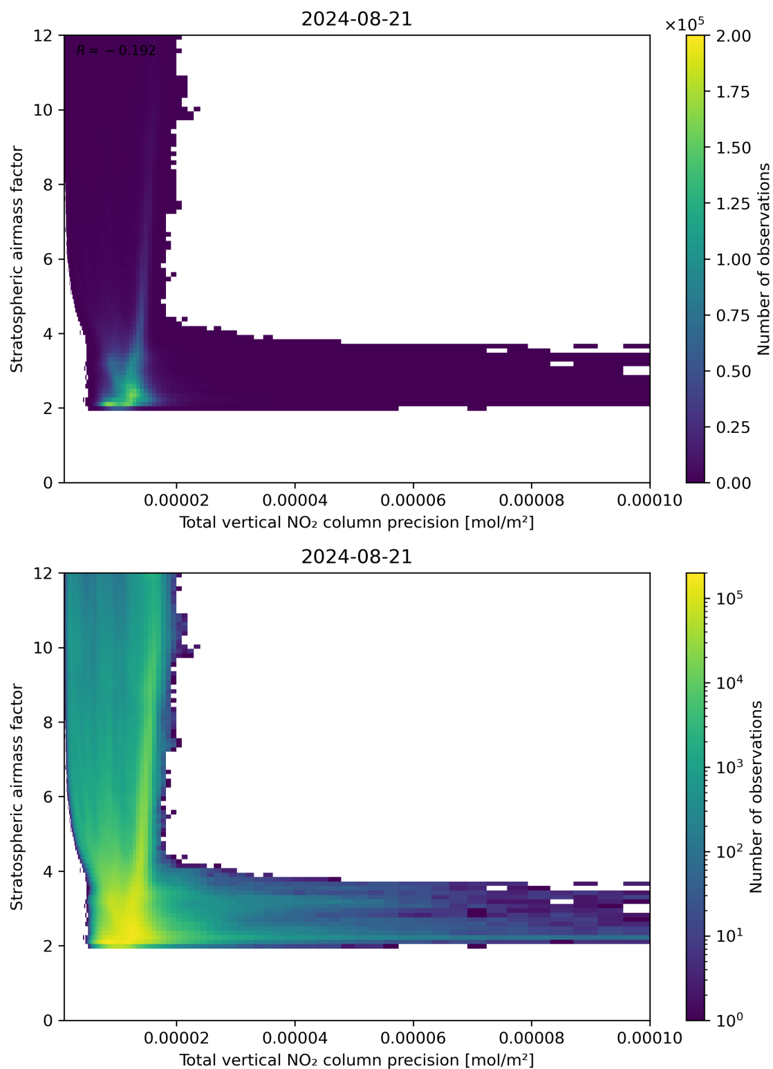
Figure 115: Scatter density plot of “Total vertical NO 2 column precision” against “Stratospheric airmass factor” for 2024-08-21 to 2024-08-22.
