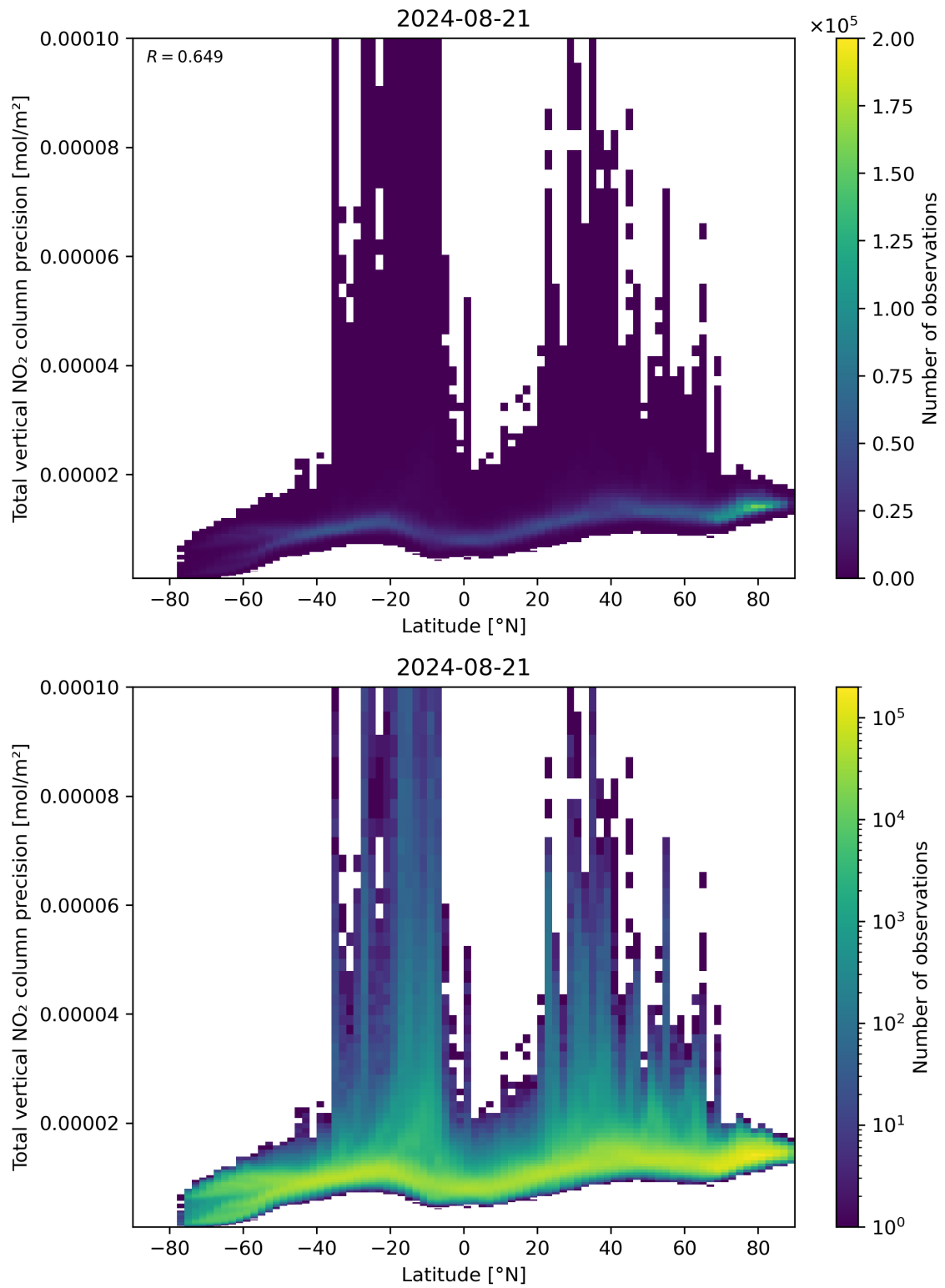
Figure 91: Scatter density plot of “Latitude” against “Total vertical NO 2 column precision” for 2024-08-21 to 2024-08-22.
