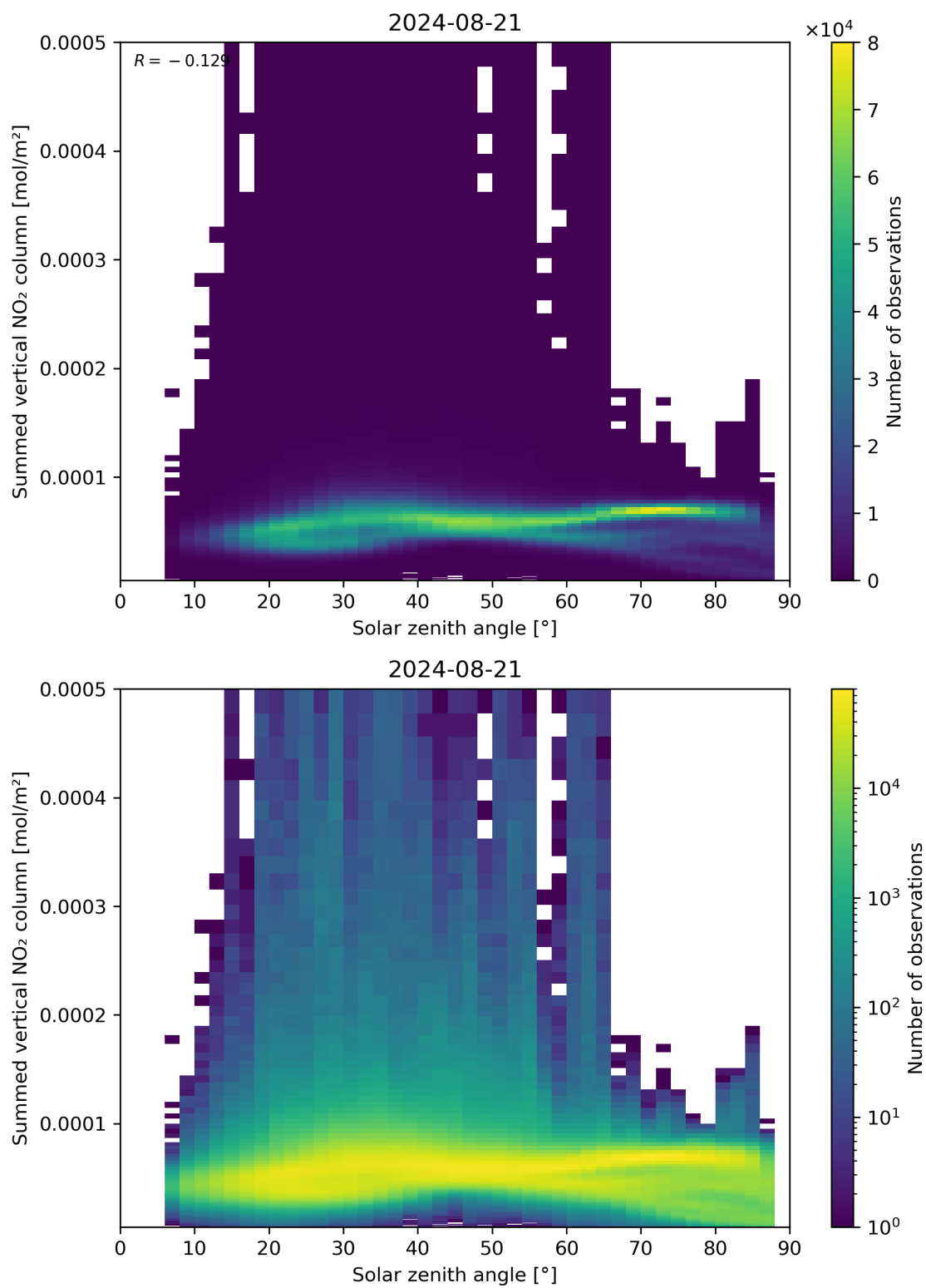
Figure 151: Scatter density plot of “Solar zenith angle” against “Summed vertical NO 2 column” for 2024-08-21 to 2024-08-22.
