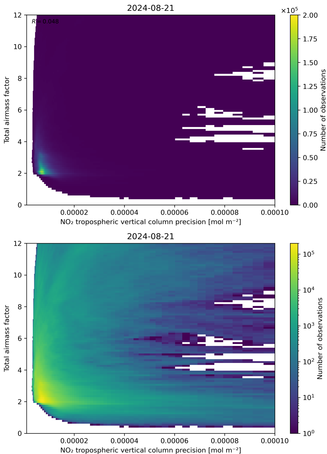
Figure 132: Scatter density plot of “NO 2 tropospheric vertical column precision” against “Total air mass factor” for 2024-08-21 to 2024-08-22.
