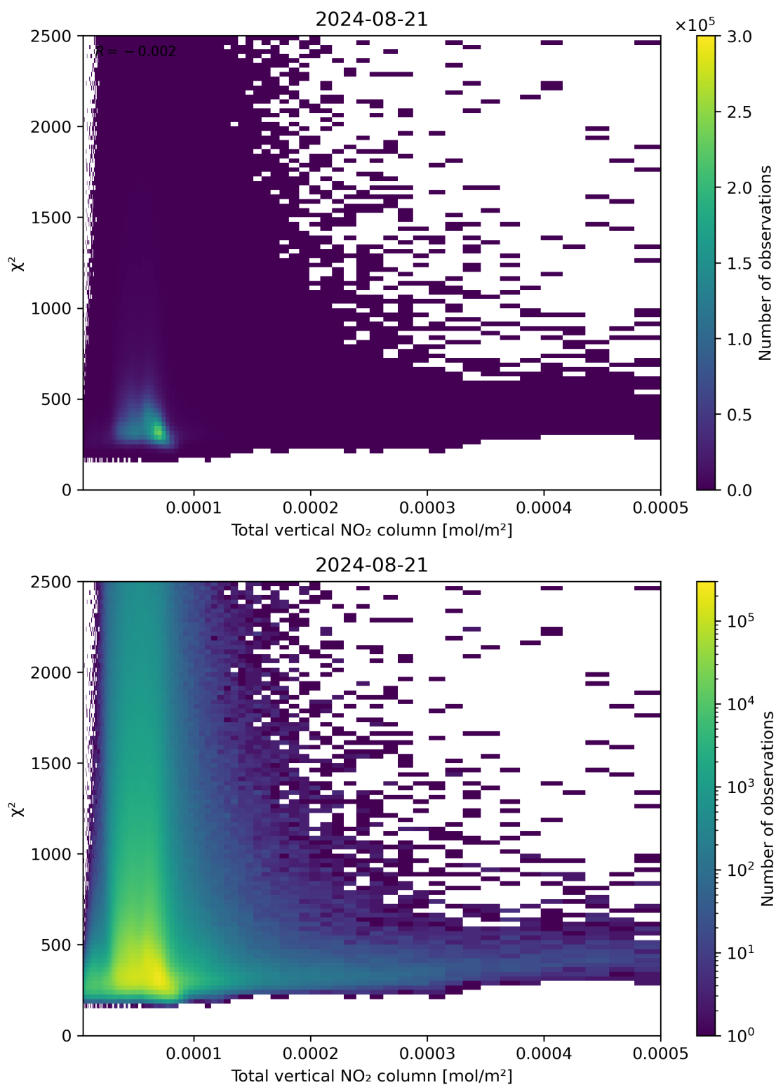
Figure 111: Scatter density plot of “Total vertical NO 2 column” against “ \chi^2 ” for 2024-08-21 to 2024-08-22.
