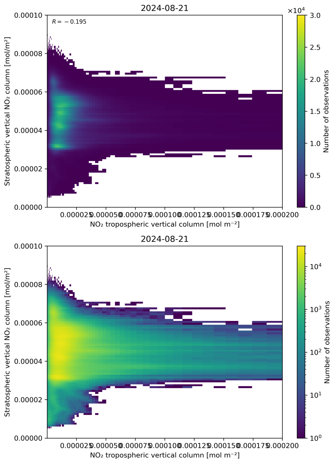
Figure 125: Scatter density plot of “NO 2 tropospheric vertical column” against “Stratospheric vertical NO 2 column” for 2024-08-21 to 2024-08-22.
