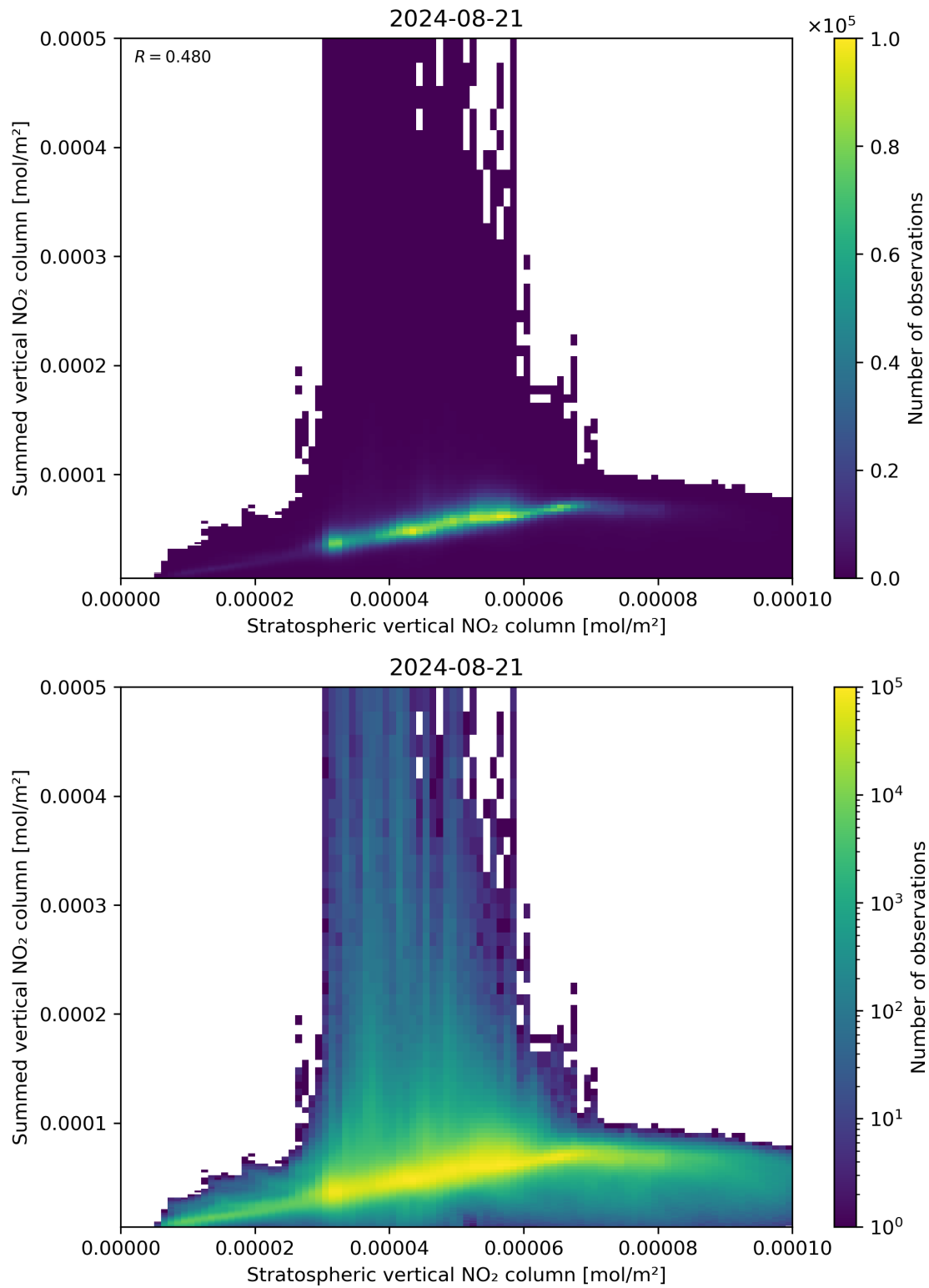
Figure 98: Scatter density plot of “Stratospheric vertical NO 2 column” against “Summed vertical NO 2 column” for 2024-08-21 to 2024-08-22.
