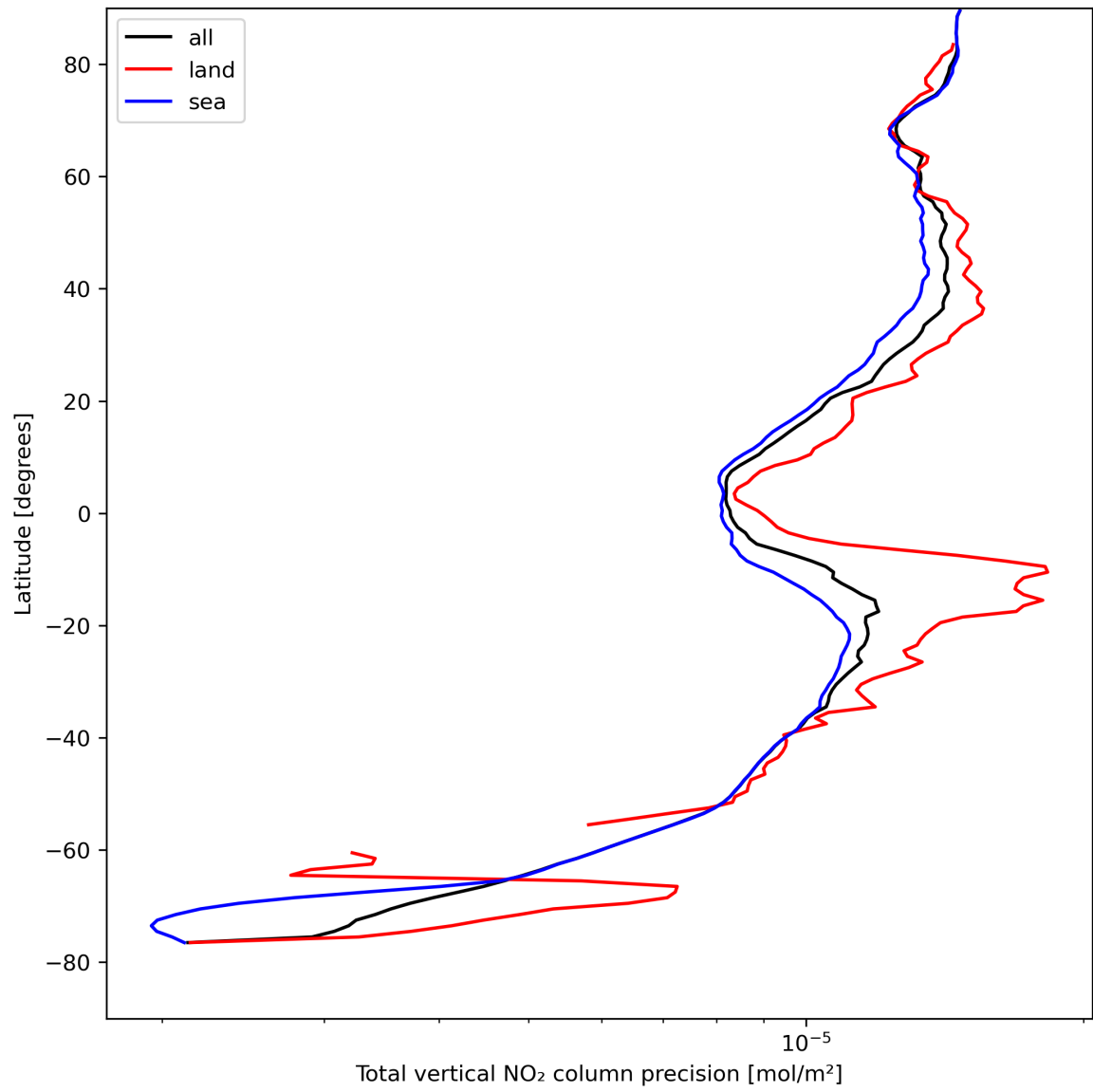
Figure 22: Zonal average of “Total vertical NO 2 column precision” for 2024-08-21 to 2024-08-22.
