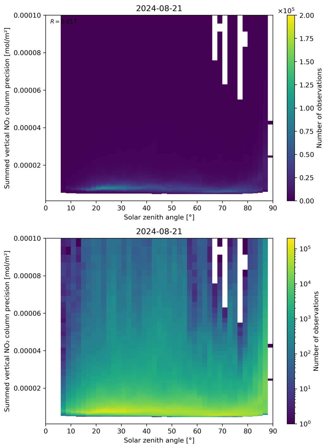
Figure 152: Scatter density plot of “Solar zenith angle” against “Summed vertical NO 2 column precision” for 2024-08-21 to 2024-08-22.
