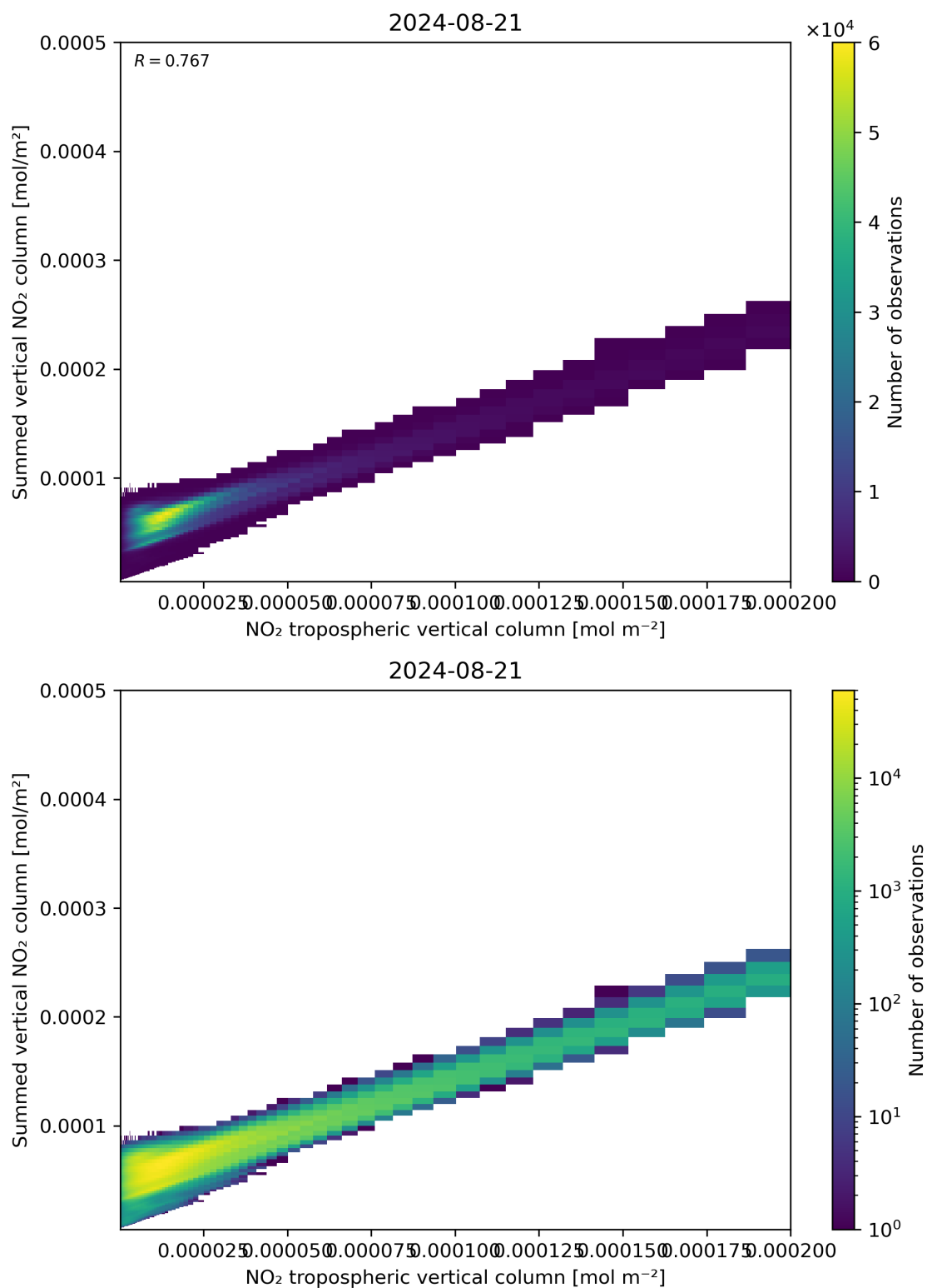
Figure 126: Scatter density plot of “NO 2 tropospheric vertical column” against “Summed vertical NO 2 column” for 2024-08-21 to 2024-08-22.
