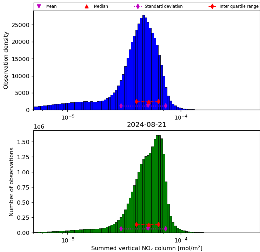
Figure 40: Histogram of “Summed vertical NO 2 column” for 2024-08-21 to 2024-08-22
