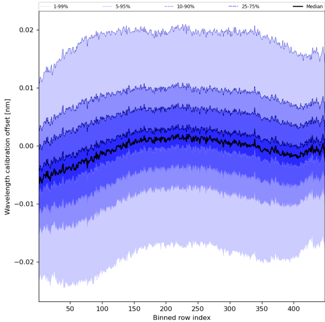
Figure 52: Along track statistics of “Wavelength calibration offset” for 2024-08-21 to 2024-08-22
