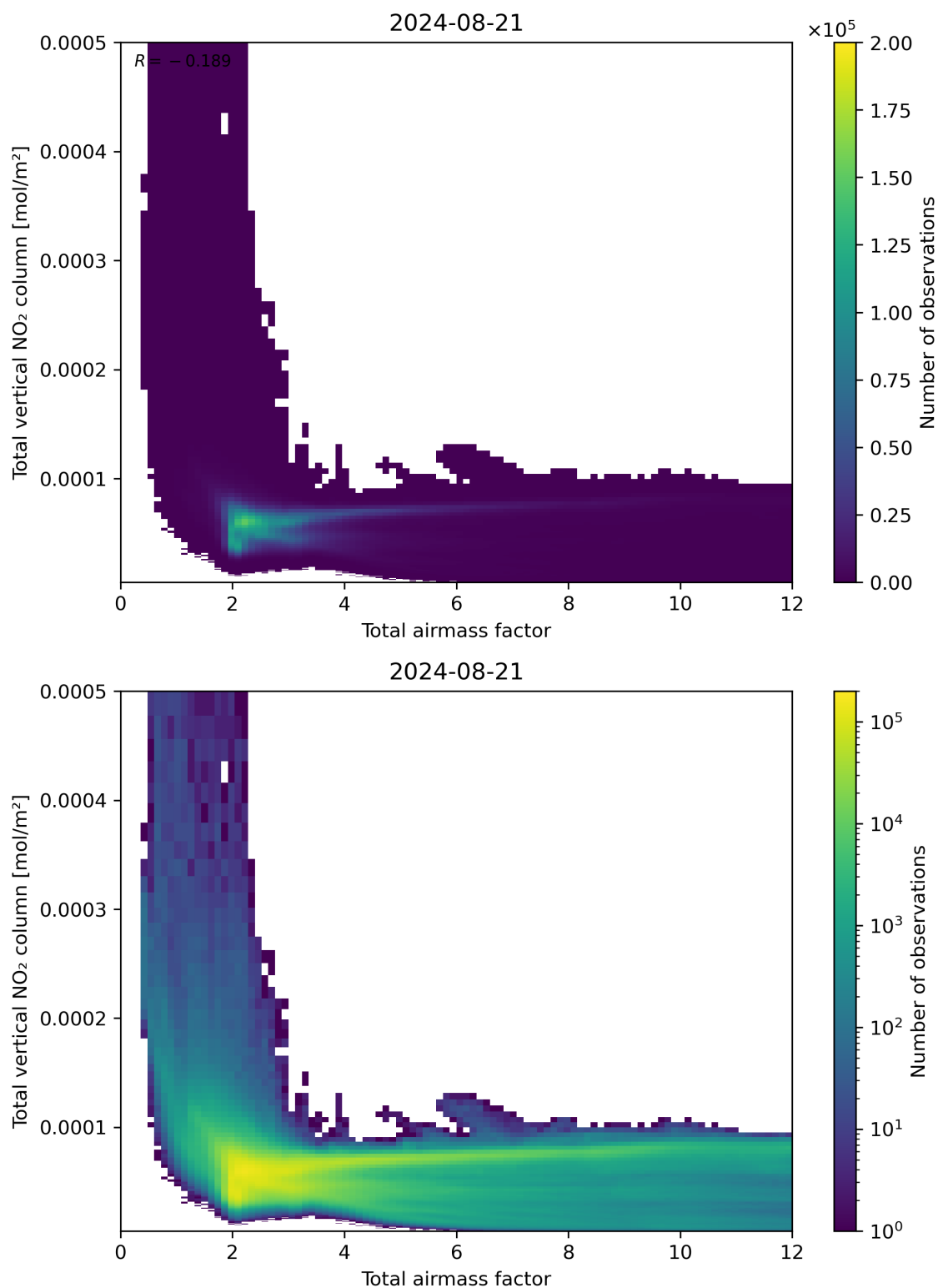
Figure 67: Scatter density plot of “Total airmass factor” against “Total vertical NO 2 column” for 2024-08-21 to 2024-08-22.
