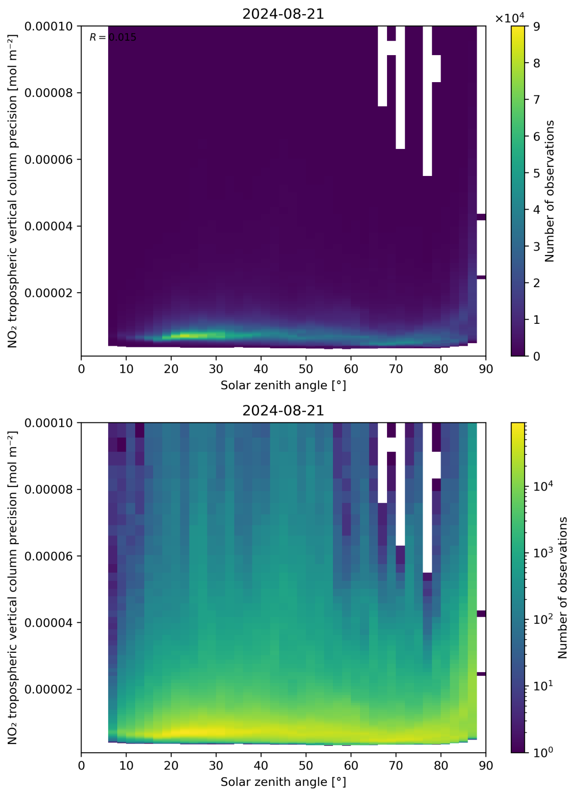
Figure 156: Scatter density plot of “Solar zenith angle” against “NO 2 tropospheric vertical column precision” for 2024-08-21 to 2024-08-22.
