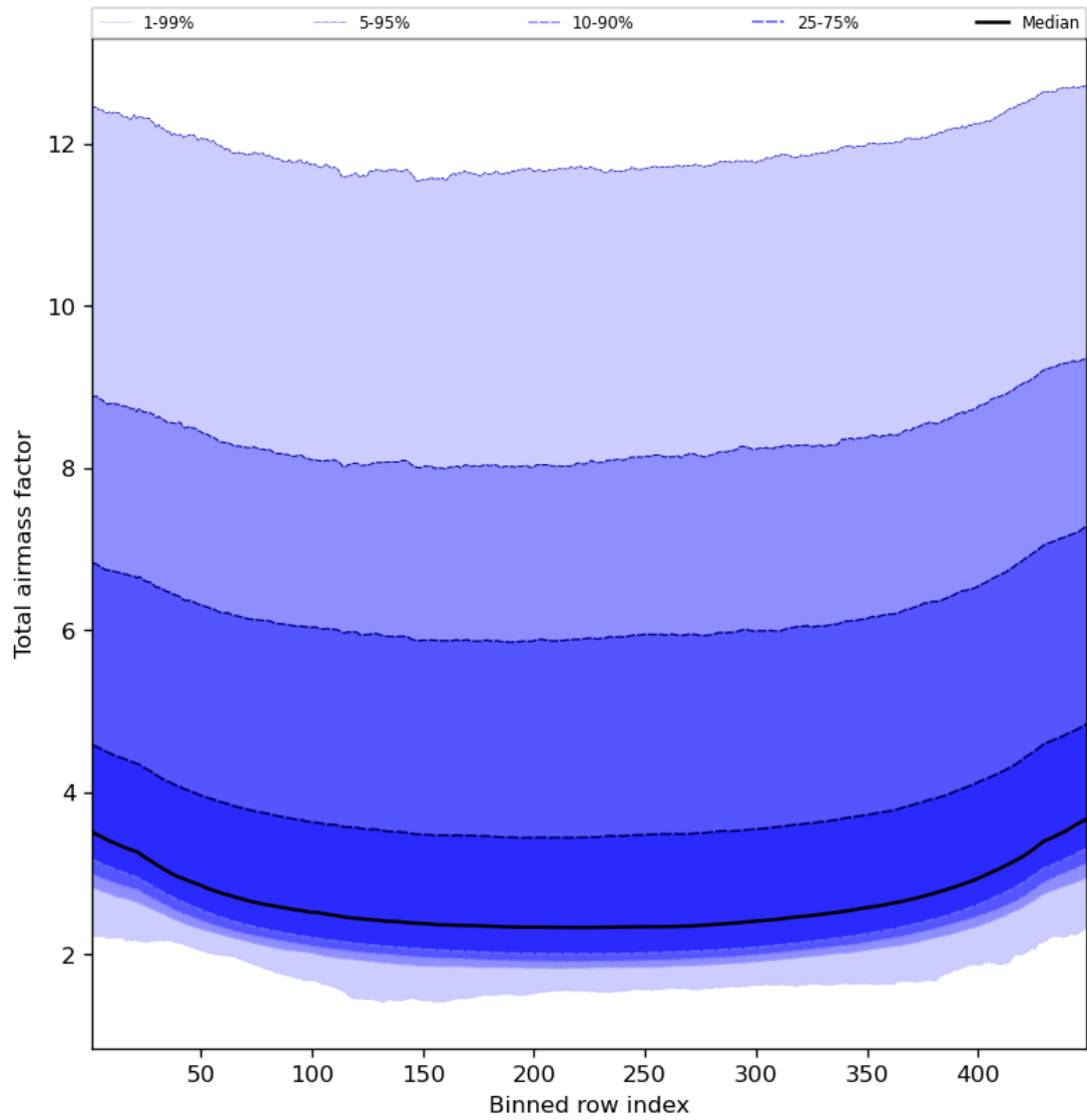
Figure 49: Along track statistics of “Total airmass factor” for 2024-08-21 to 2024-08-22
