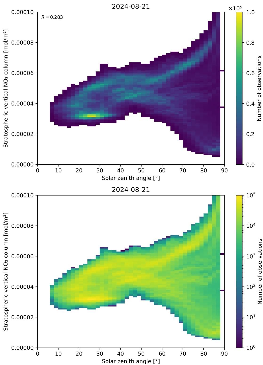
Figure 150: Scatter density plot of “Solar zenith angle” against “Stratospheric vertical NO 2 column” for 2024-08-21 to 2024-08-22.
