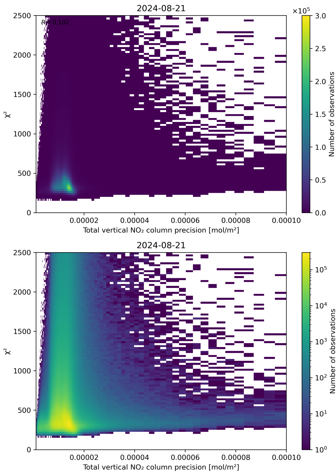
Figure 116: Scatter density plot of “Total vertical NO 2 column precision” against “ \chi^2 ” for 2024-08-21 to 2024-08-22.
