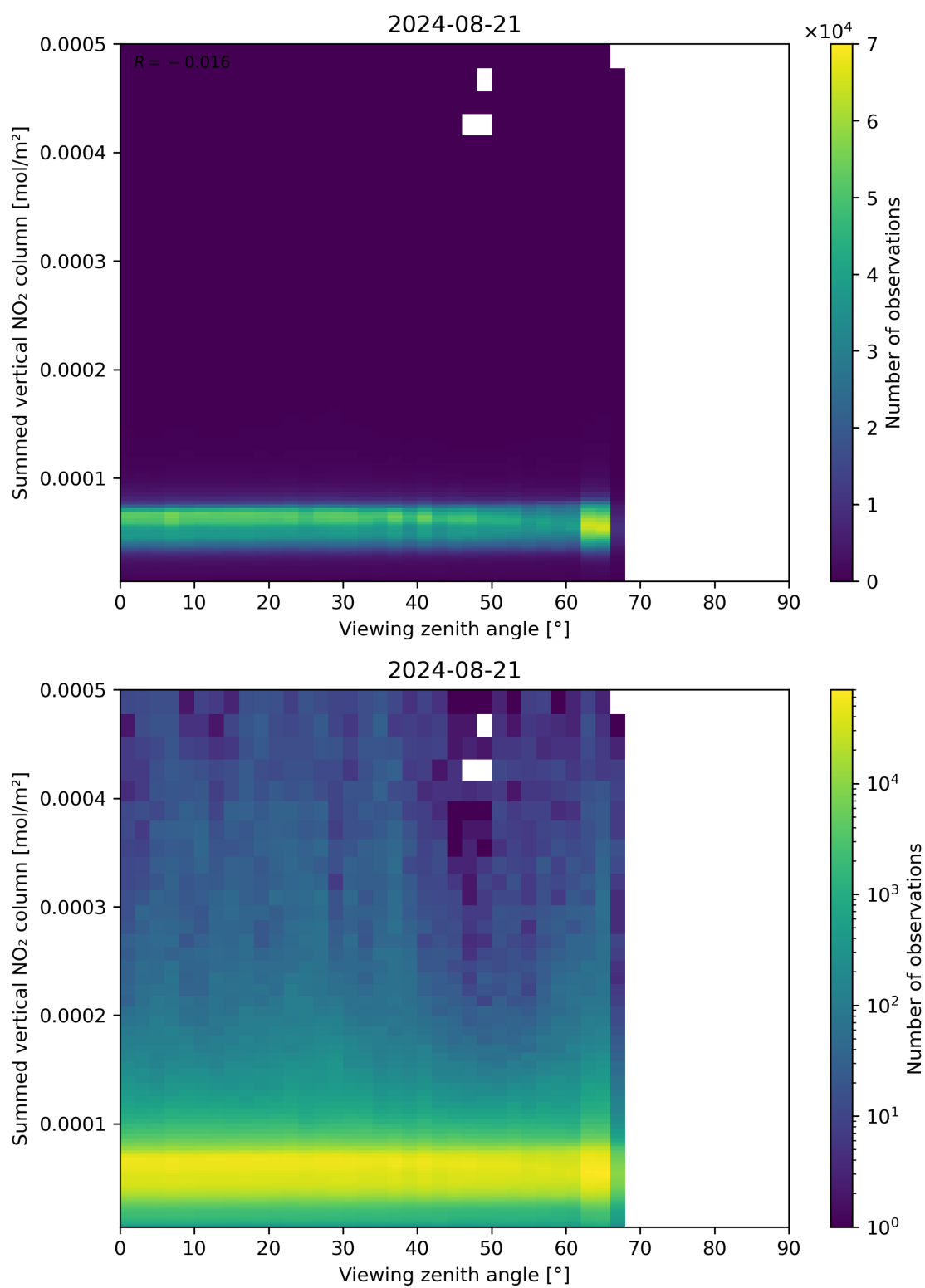
Figure 165: Scatter density plot of “Viewing zenith angle” against “Summed vertical NO 2 column” for 2024-08-21 to 2024-08-22.
