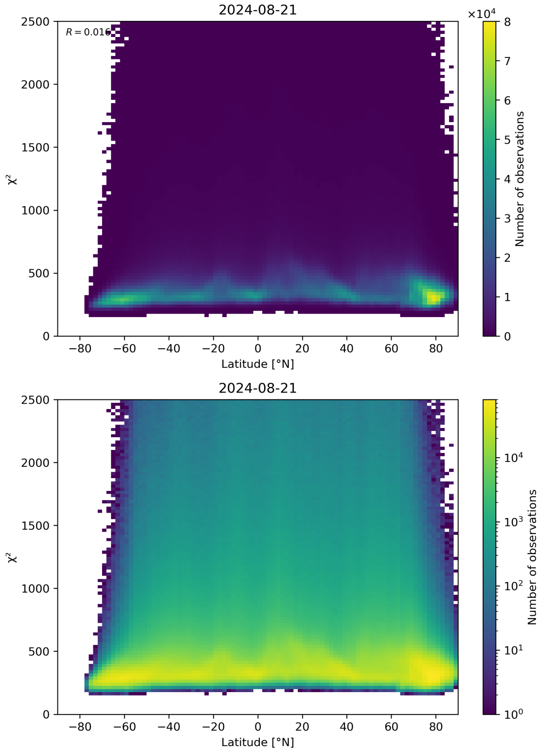
Figure 86: Scatter density plot of “Latitude” against “ \chi^2 ” for 2024-08-21 to 2024-08-22.
