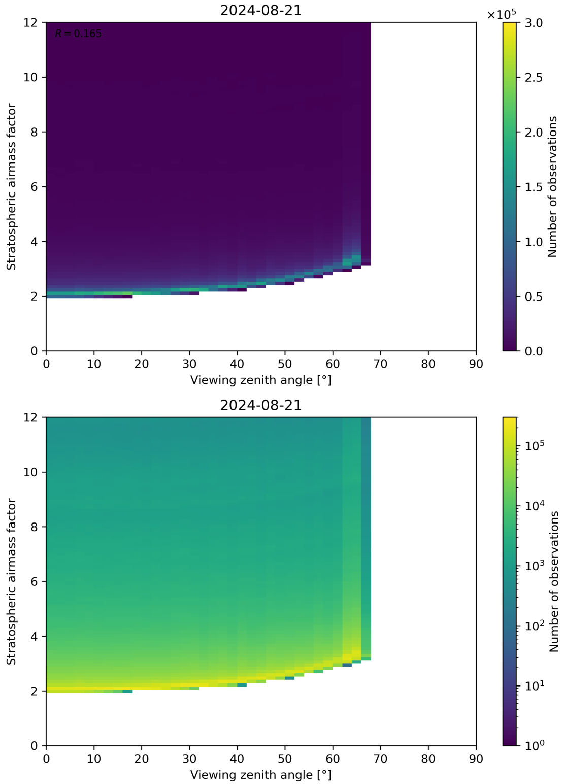
Figure 159: Scatter density plot of “Viewing zenith angle” against “Stratospheric airmass factor” for 2024-08-21 to 2024-08-22.
