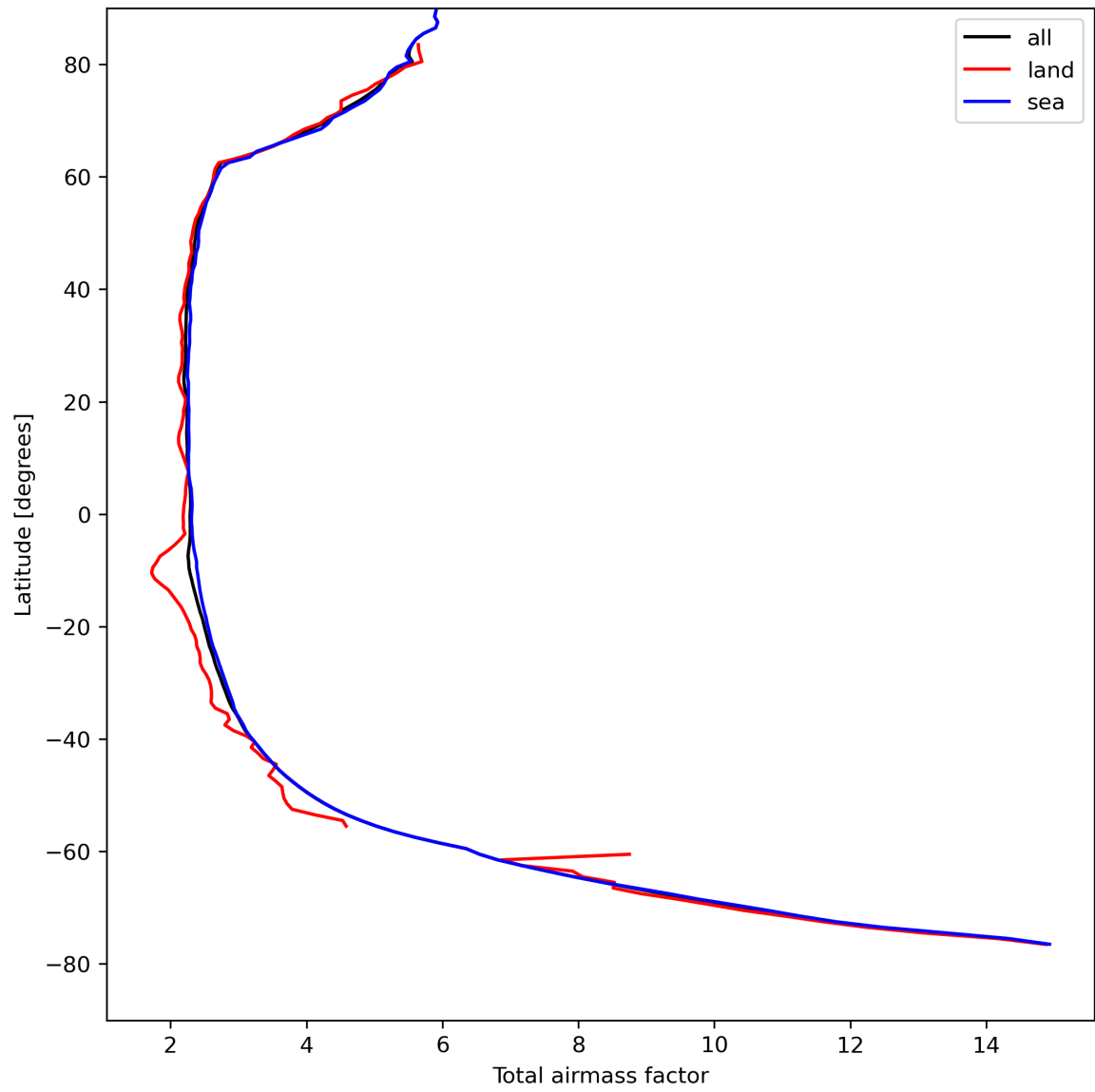
Figure 15: Zonal average of “Total airmass factor” for 2024-08-21 to 2024-08-22.
