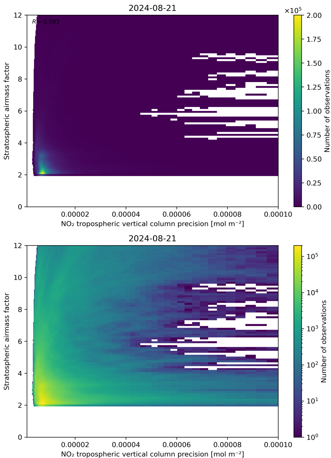
Figure 131: Scatter density plot of “NO 2 tropospheric vertical column precision” against “Stratospheric airmass factor” for 2024-08-21 to 2024-08-22.
