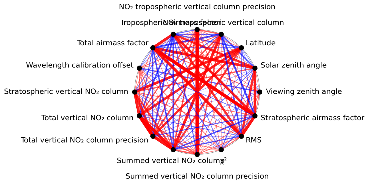
Figure 1: Map of correlation graph for 2024-08-21 to 2024-08-22.
