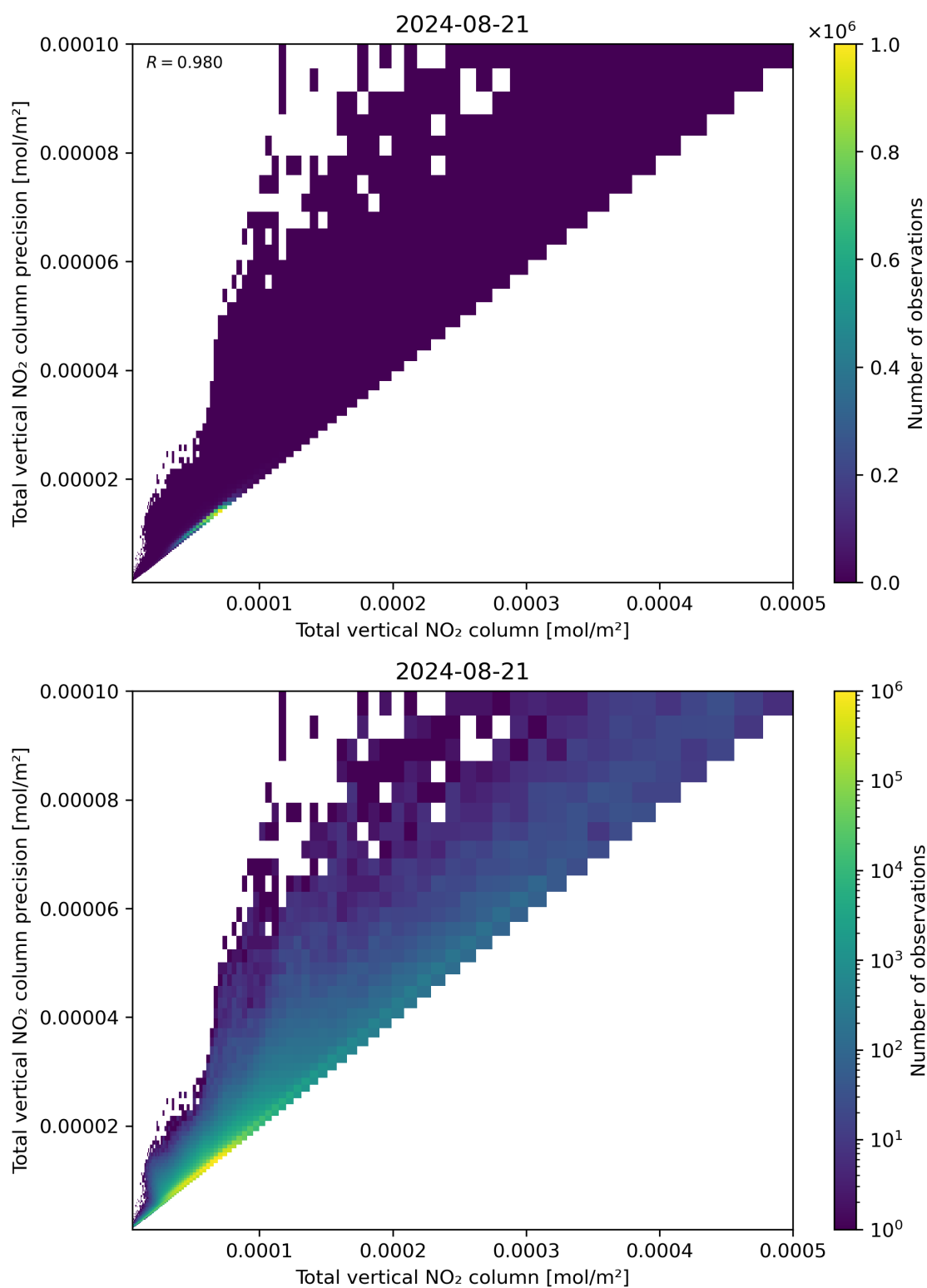
Figure 114: Scatter density plot of “Total vertical NO 2 column” against “Total vertical NO 2 column precision” for 2024-08-21 to 2024-08-22.
