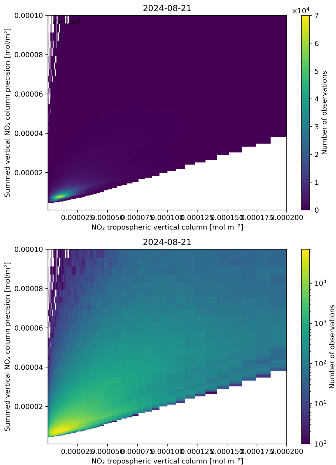
Figure 127: Scatter density plot of “NO 2 tropospheric vertical column” against “Summed vertical NO 2 column precision” for 2024-08-21 to 2024-08-22.
