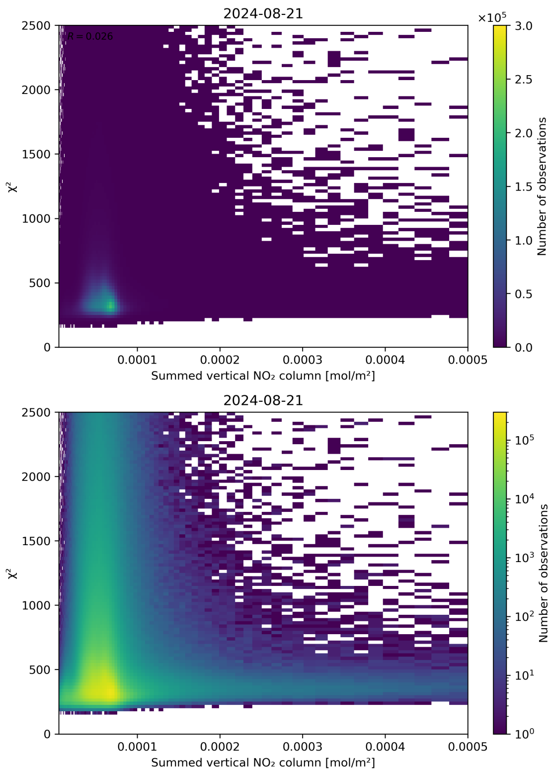
Figure 104: Scatter density plot of “Summed vertical NO 2 column” against “ \chi^2 ” for 2024-08-21 to 2024-08-22.
