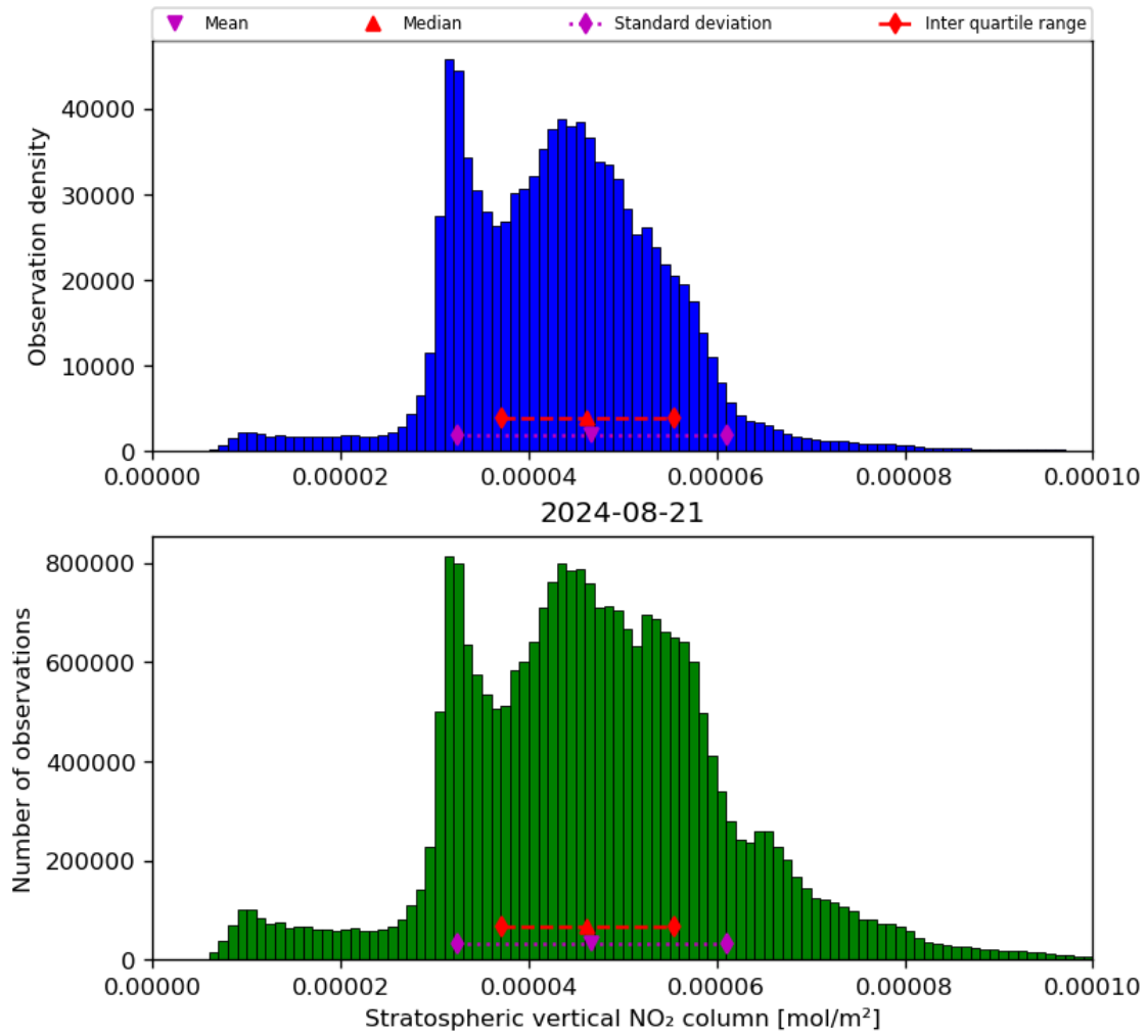
Figure 36: Histogram of “Stratospheric vertical NO 2 column” for 2024-08-21 to 2024-08-22
