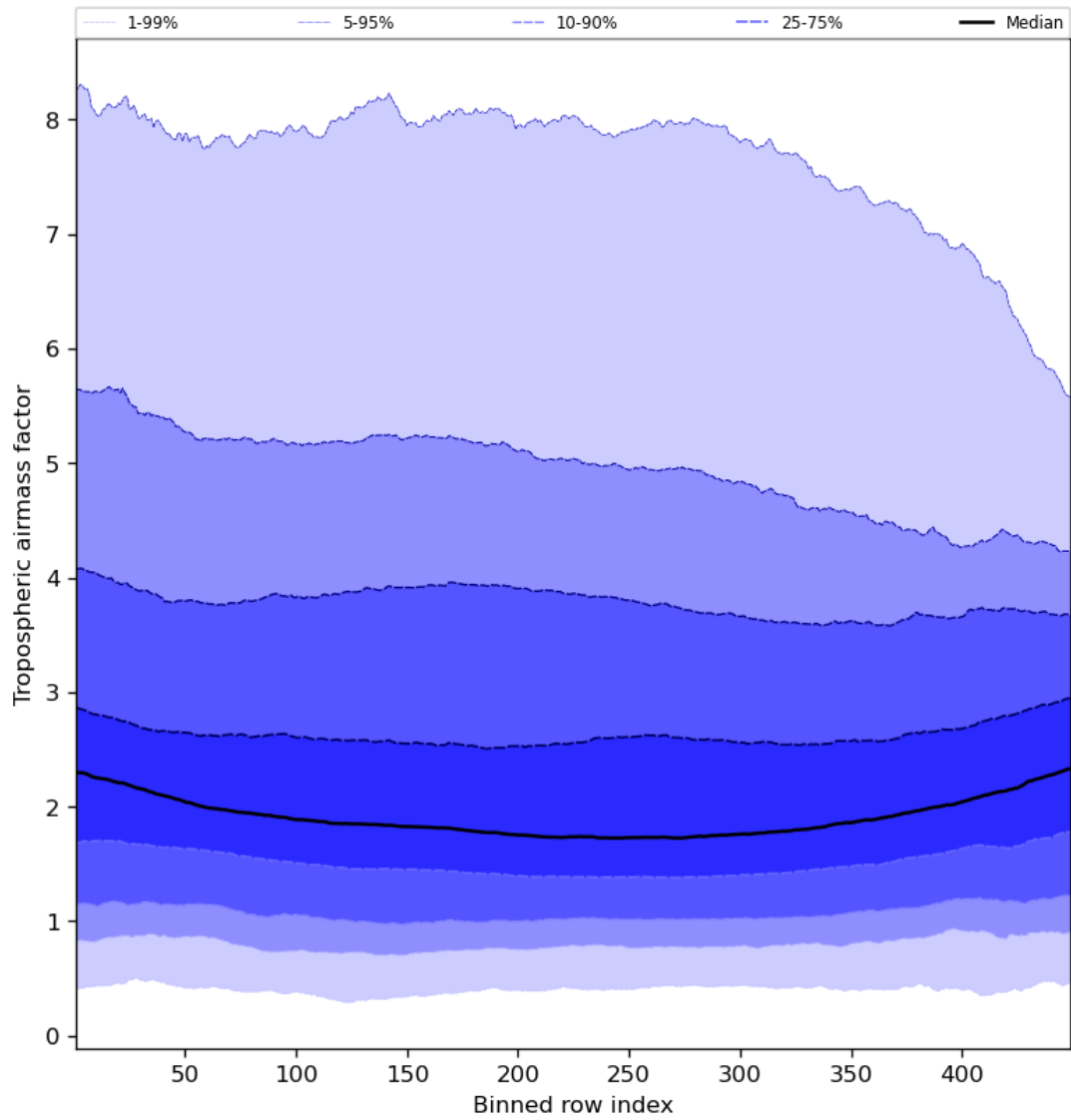
Figure 48: Along track statistics of “Tropospheric air mass factor” for 2024-08-21 to 2024-08-22
