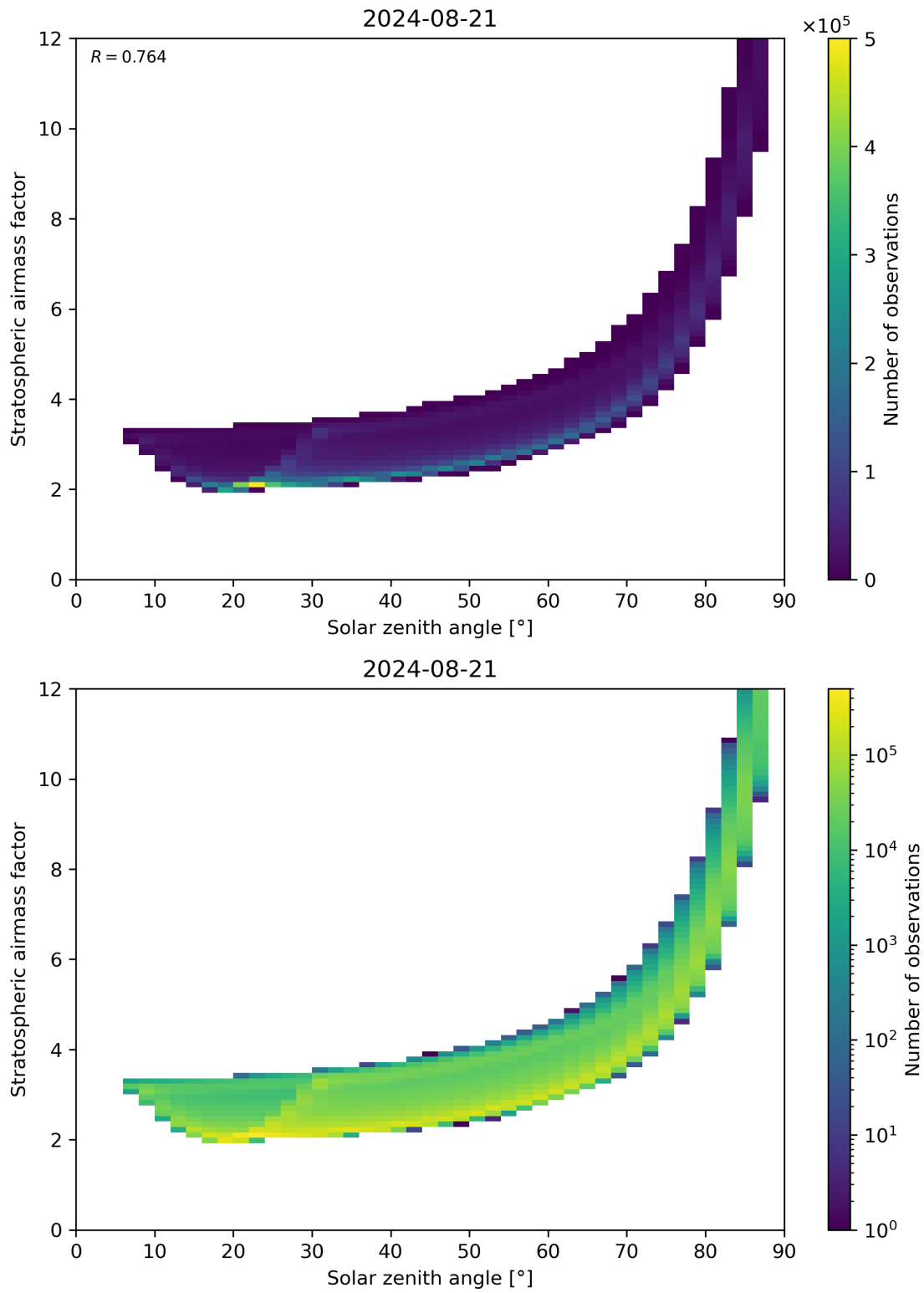
Figure 145: Scatter density plot of “Solar zenith angle” against “Stratospheric airmass factor” for 2024-08-21 to 2024-08-22.
