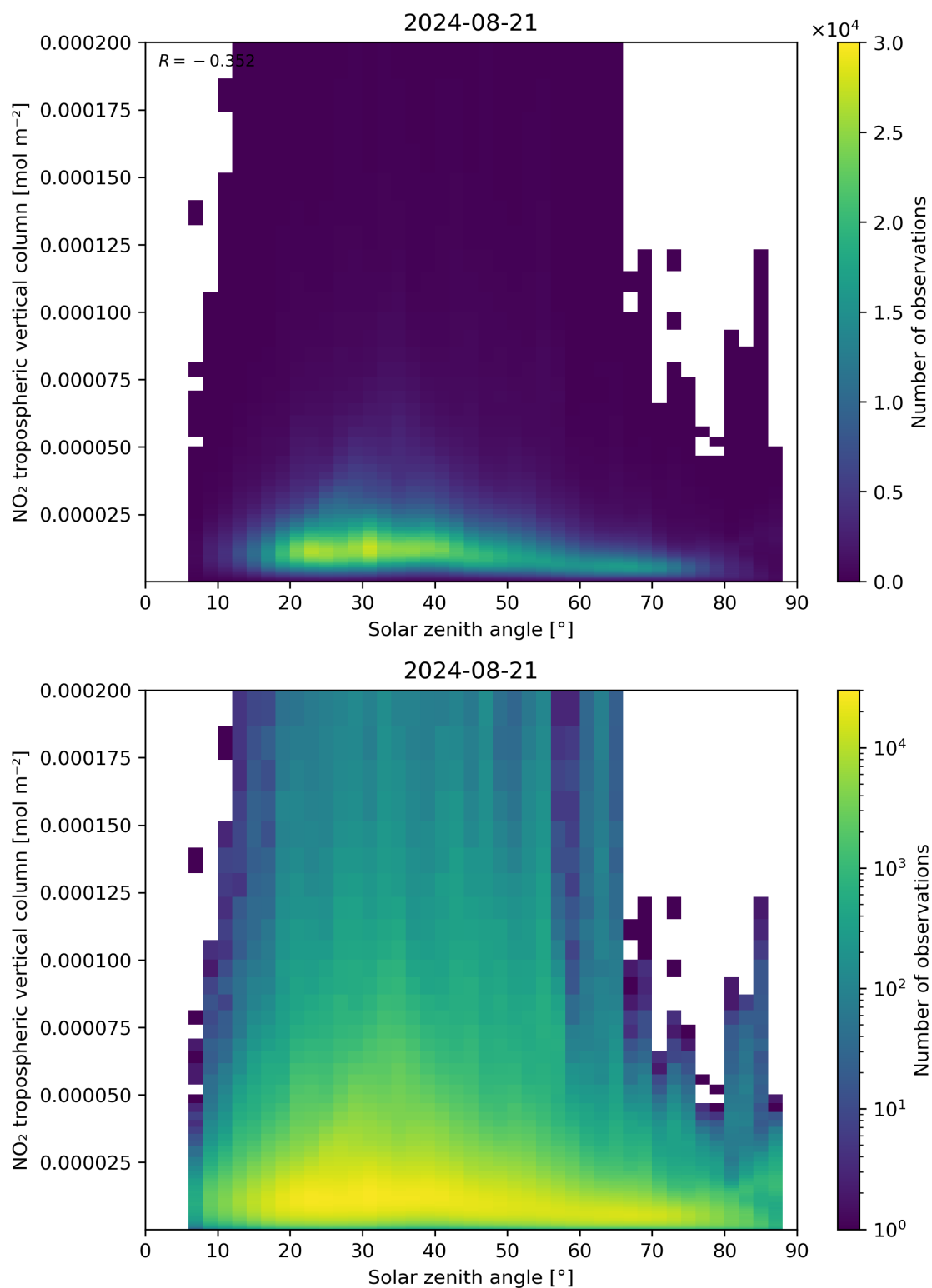
Figure 155: Scatter density plot of “Solar zenith angle” against “NO 2 tropospheric vertical column” for 2024-08-21 to 2024-08-22.
