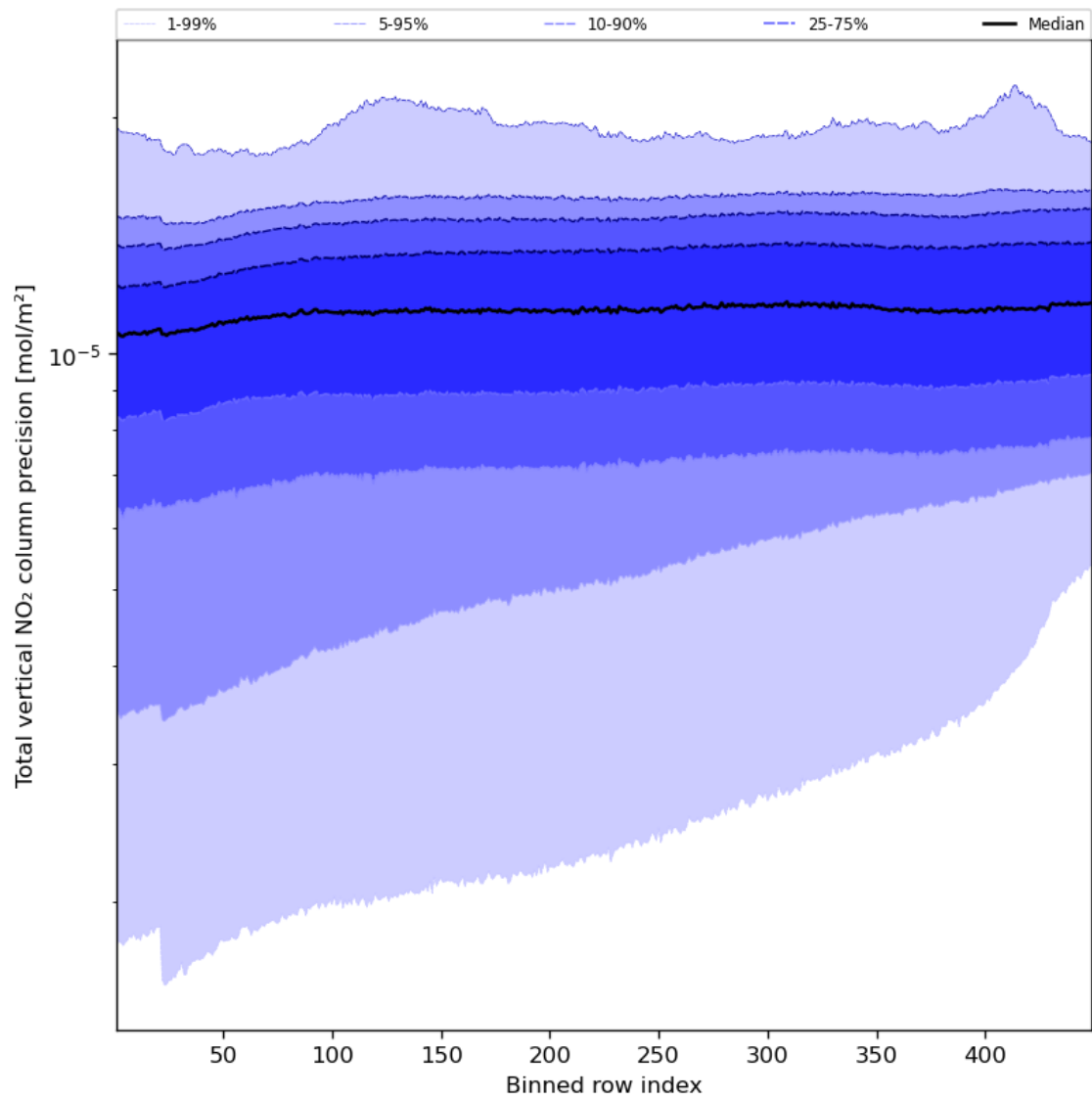
Figure 56: Along track statistics of “Total vertical NO 2 column precision” for 2024-08-21 to 2024-08-22
