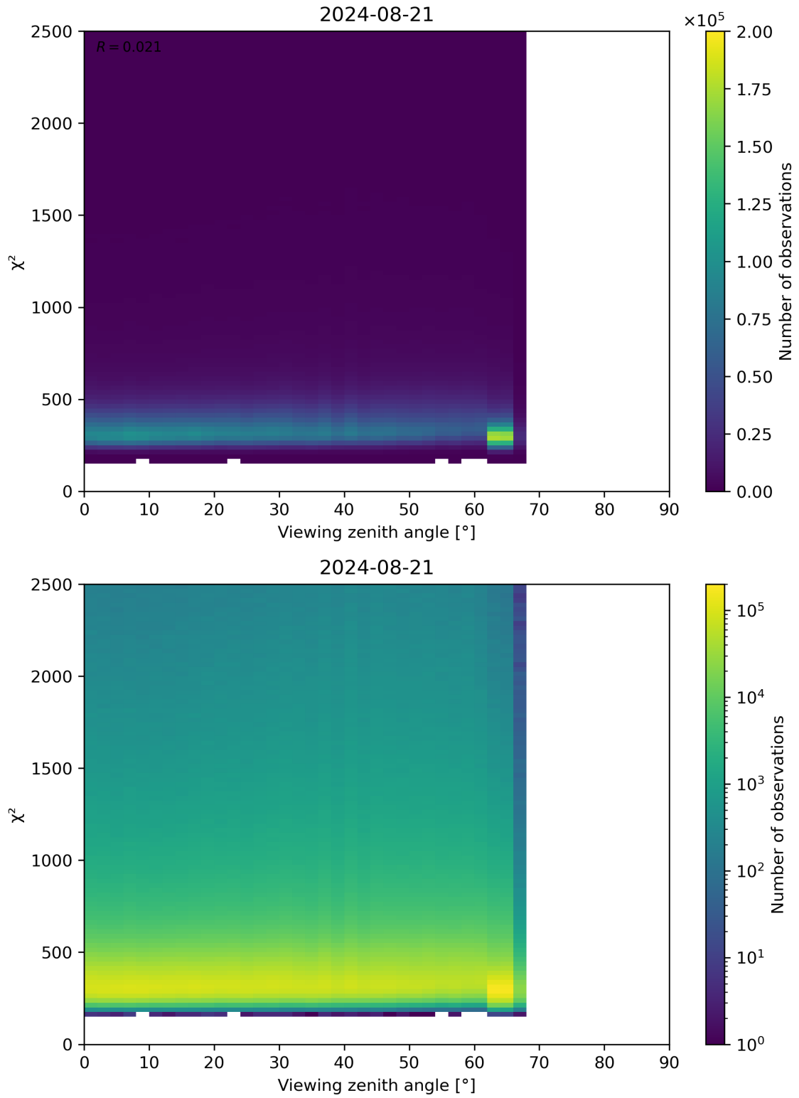
Figure 162: Scatter density plot of “Viewing zenith angle” against “ \chi^2 ” for 2024-08-21 to 2024-08-22.
