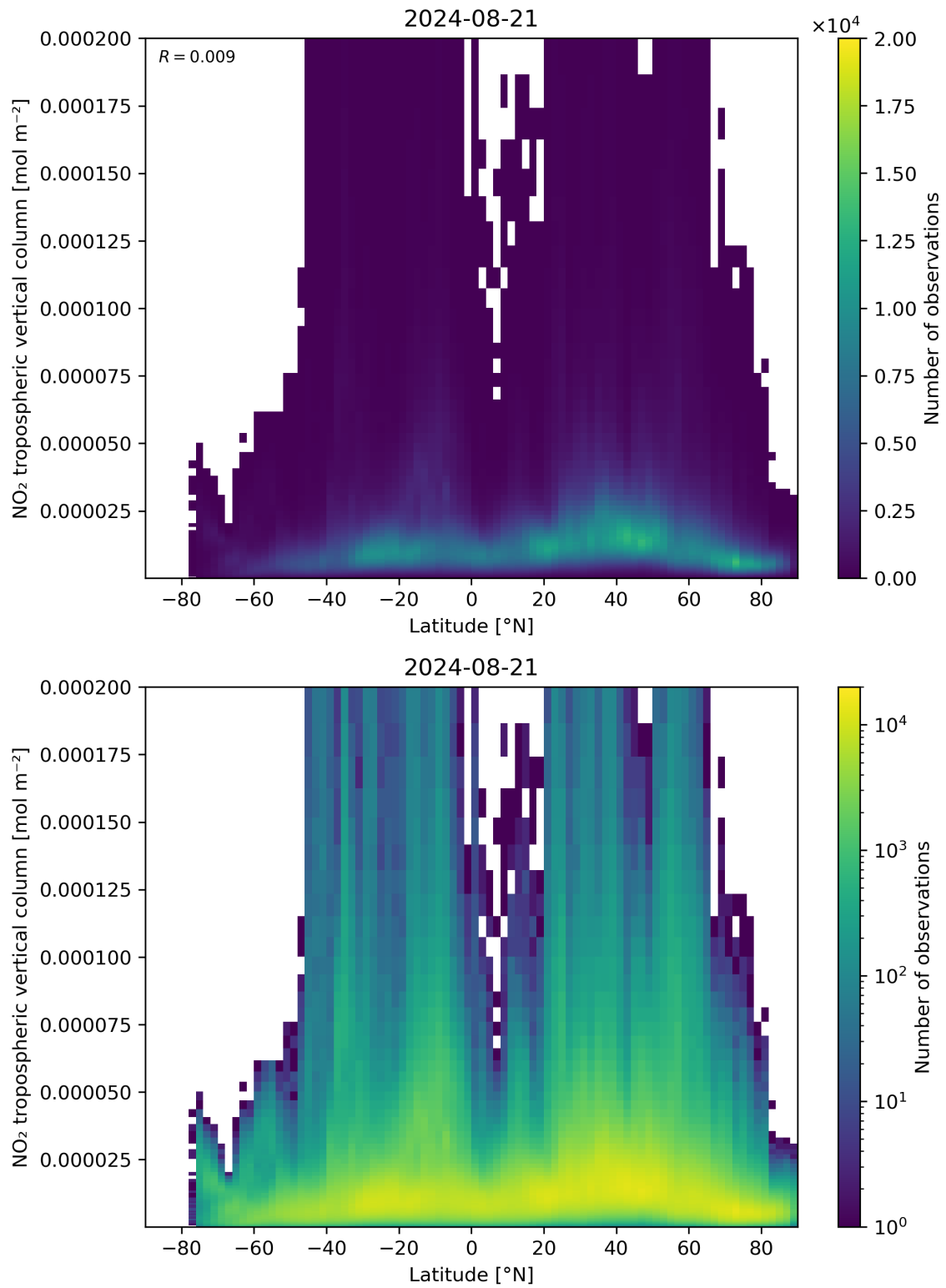
Figure 92: Scatter density plot of “Latitude” against “NO 2 tropospheric vertical column” for 2024-08-21 to 2024-08-22.
