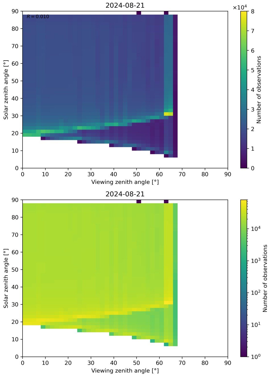
Figure 172: Scatter density plot of “Viewing zenith angle” against “Solar zenith angle” for 2024-08-21 to 2024-08-22.
