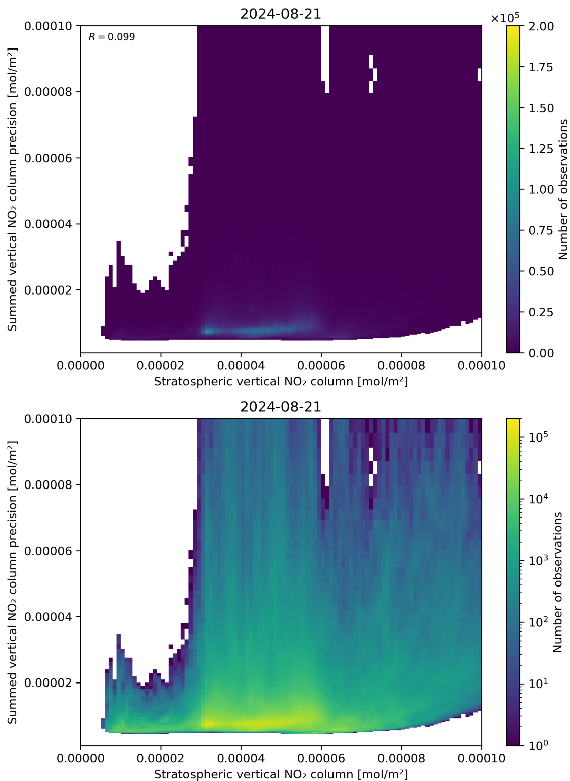
Figure 99: Scatter density plot of “Stratospheric vertical NO 2 column” against “Summed vertical NO 2 column precision” for 2024-08-21 to 2024-08-22.
