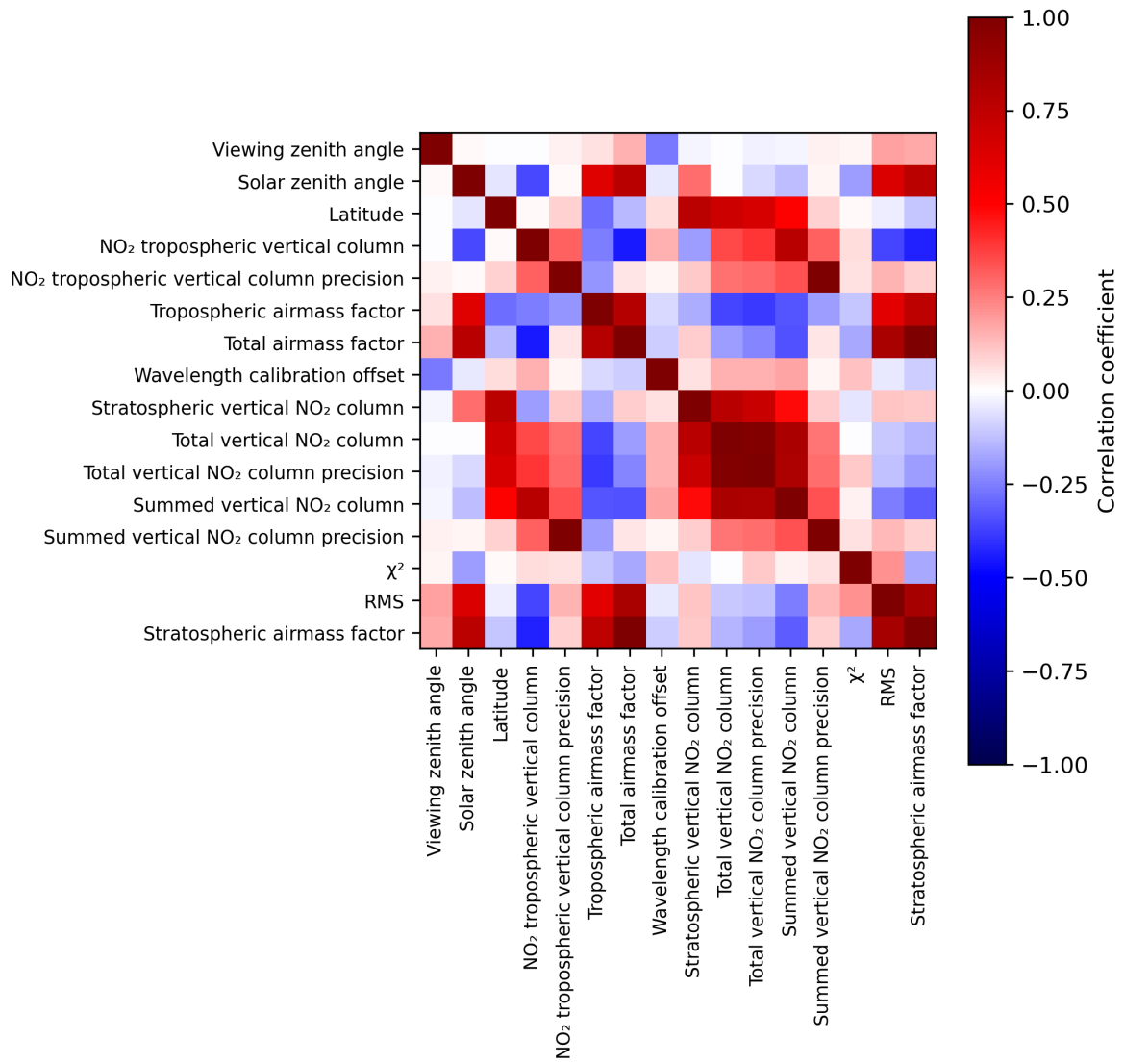
Figure 2: Map of correlation matrix for 2024-08-21 to 2024-08-22.
