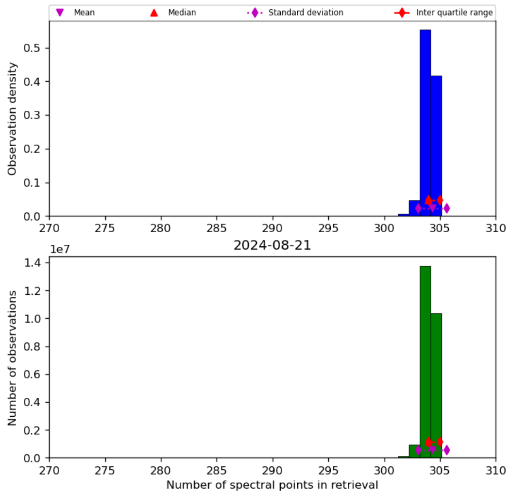
Figure 33: Histogram of “Number of spectral points in retrieval” for 2024-08-21 to 2024-08-22
