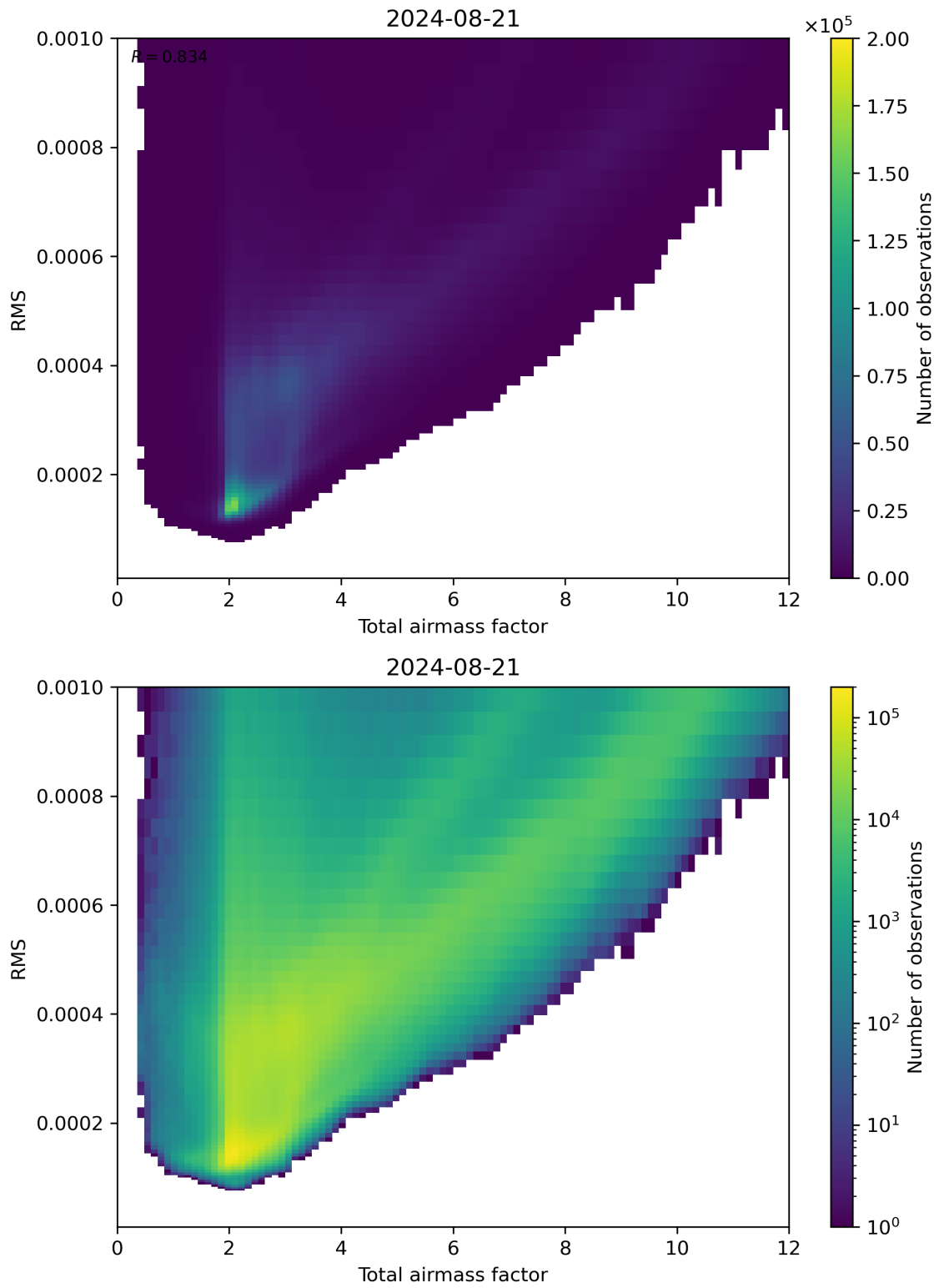
Figure 69: Scatter density plot of “Total airmass factor” against “RMS” for 2024-08-21 to 2024-08-22.
