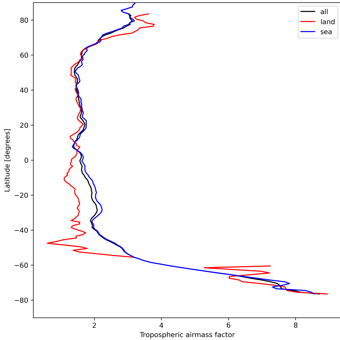
Figure 14: Zonal average of “Tropospheric airmass factor” for 2024-08-21 to 2024-08-22.
