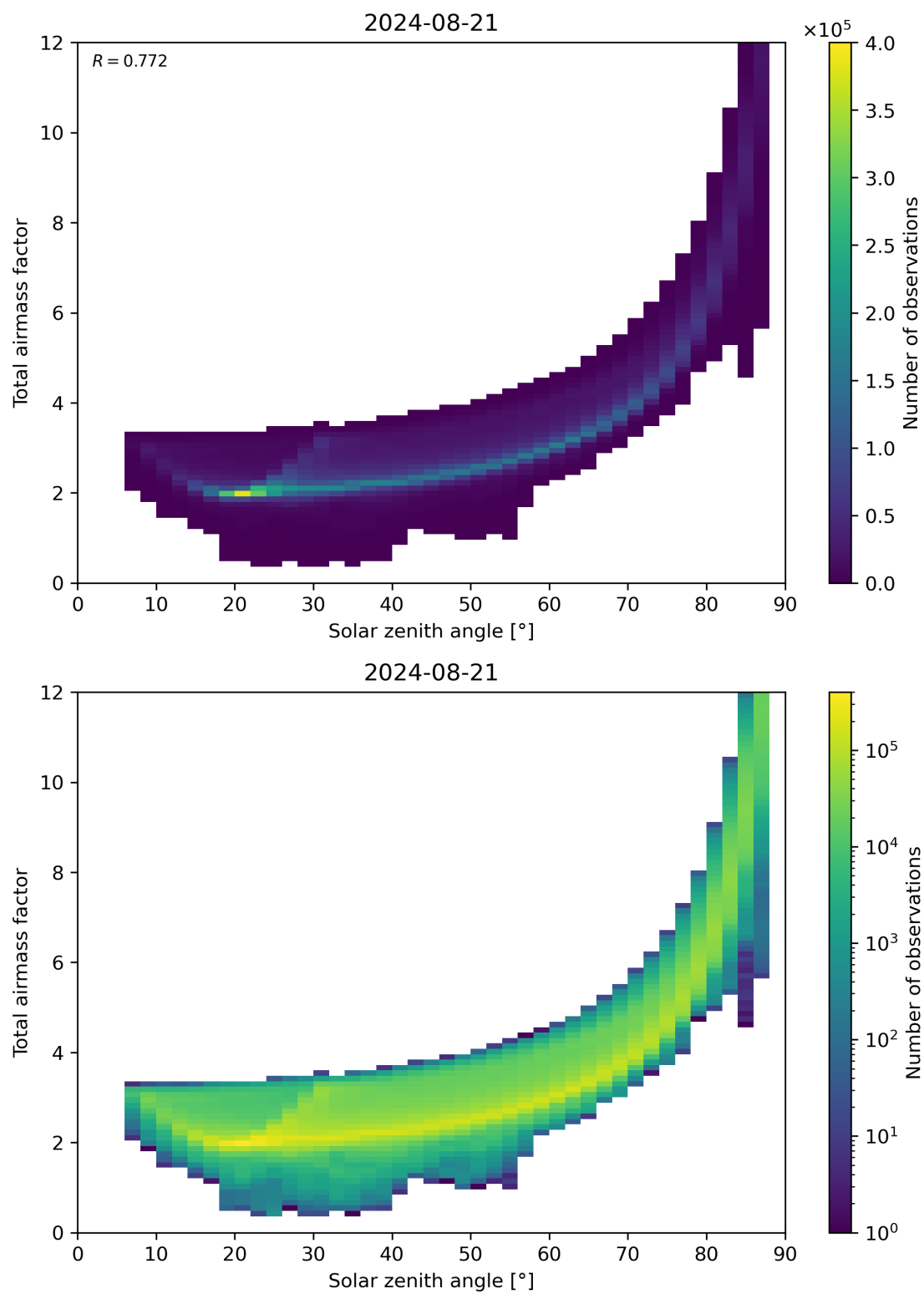
Figure 146: Scatter density plot of “Solar zenith angle” against “Total air mass factor” for 2024-08-21 to 2024-08-22.
