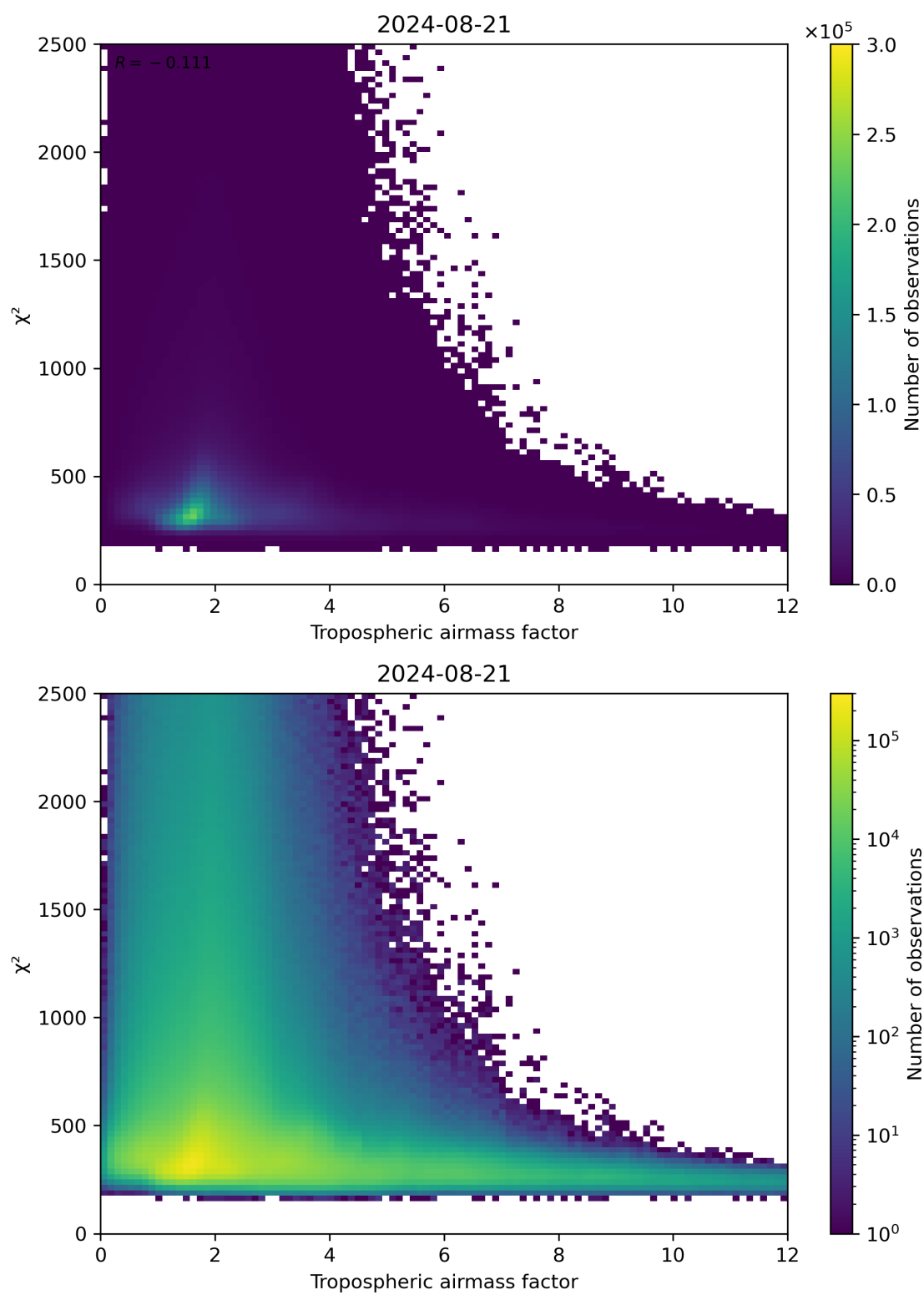
Figure 73: Scatter density plot of “Tropospheric airmass factor” against “ \chi^2 ” for 2024-08-21 to 2024-08-22.
