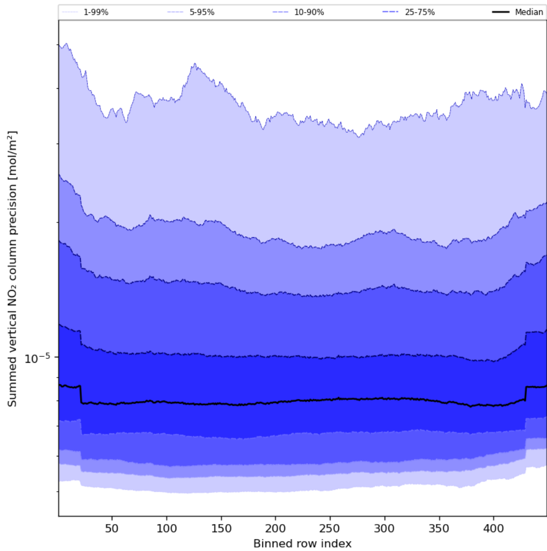
Figure 58: Along track statistics of “Summed vertical NO 2 column precision” for 2024-08-21 to 2024-08-22
