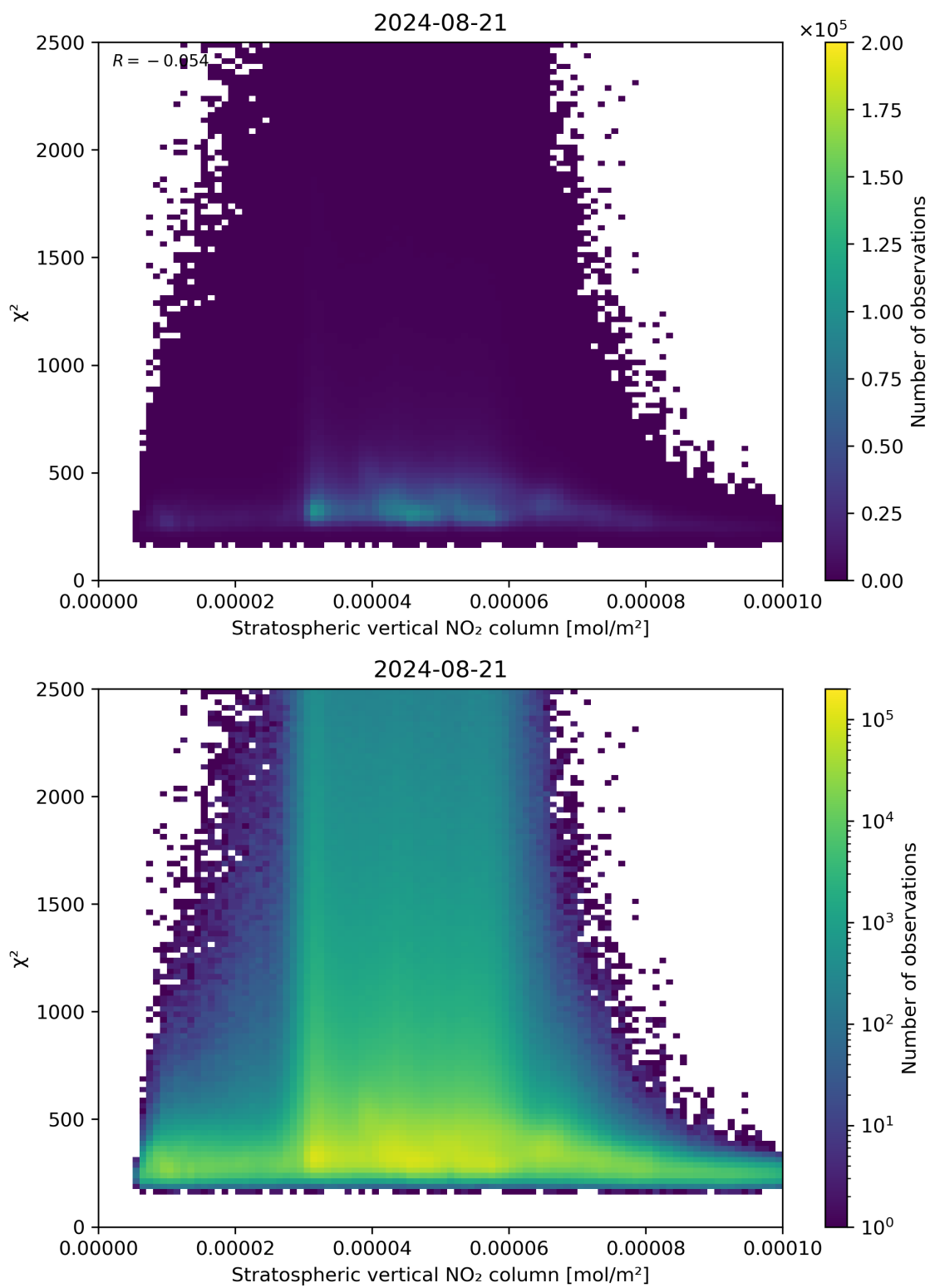
Figure 97: Scatter density plot of “Stratospheric vertical NO 2 column” against “ \chi^2 ” for 2024-08-21 to 2024-08-22.
