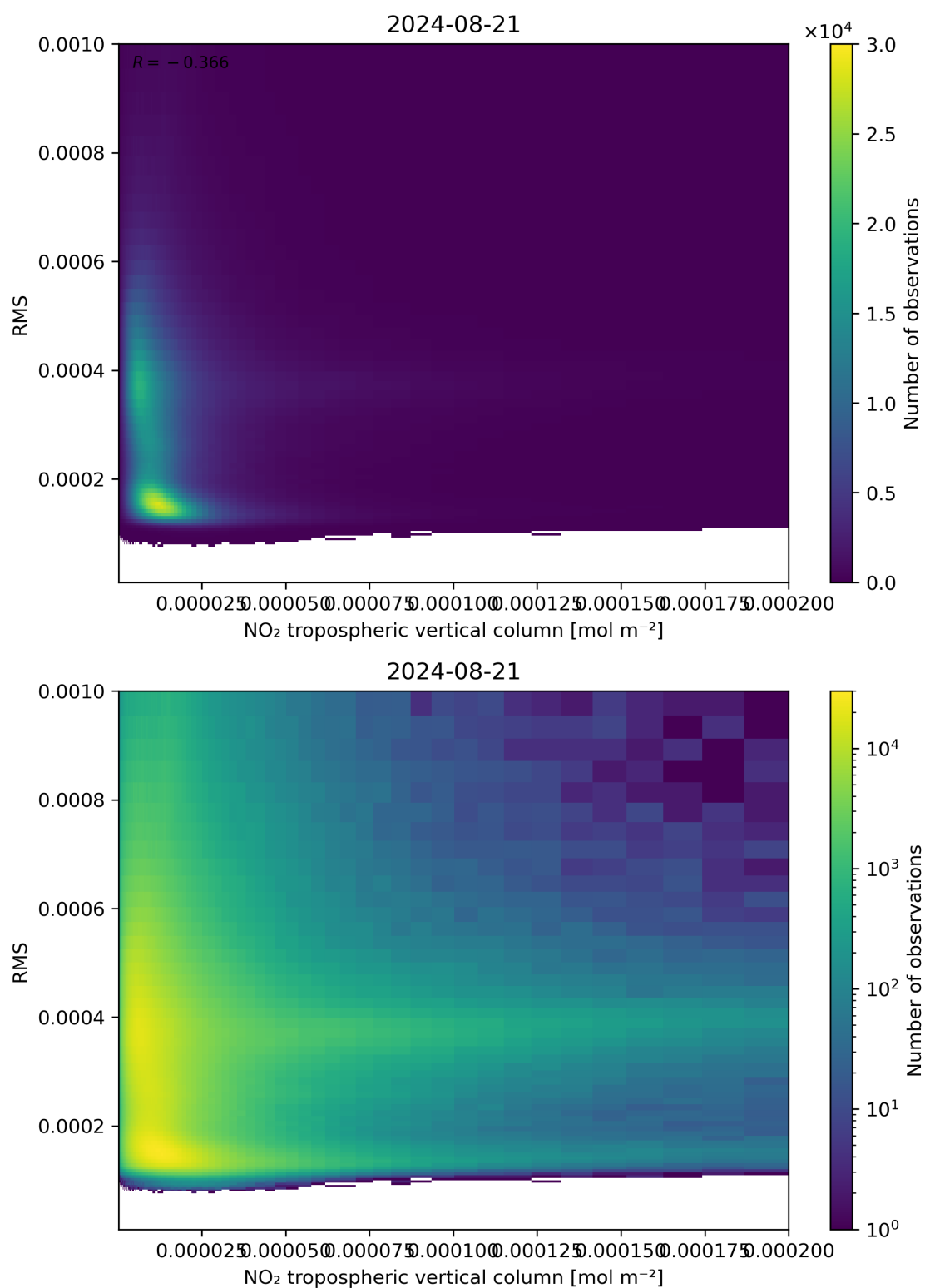
Figure 142: Scatter density plot of “NO 2 tropospheric vertical column” against “RMS” for 2024-08-21 to 2024-08-22.
