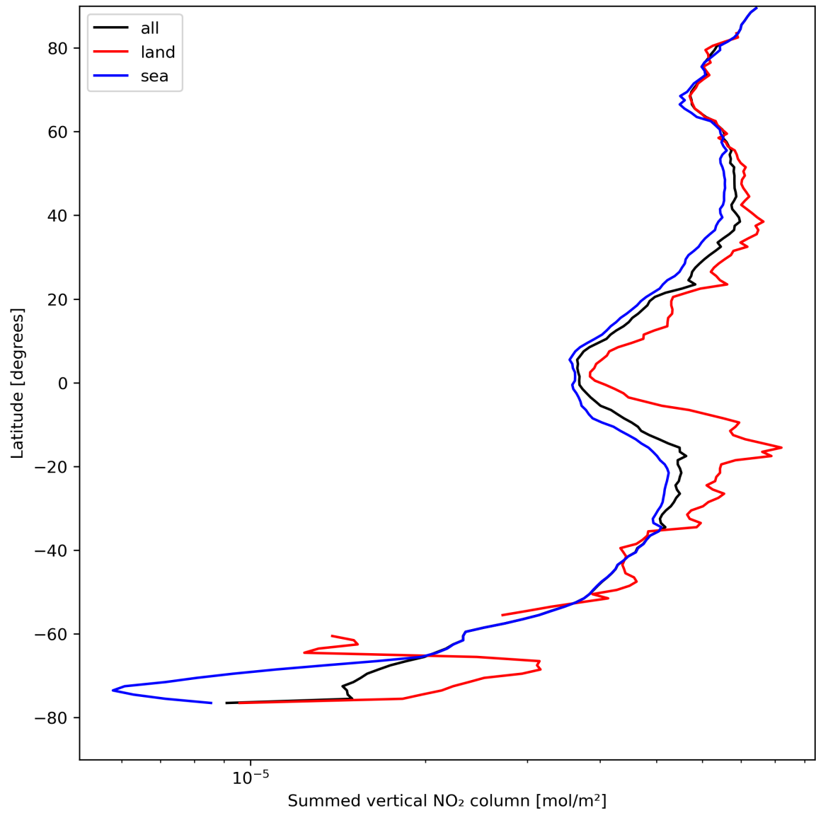
Figure 23: Zonal average of “Summed vertical NO 2 column” for 2024-08-21 to 2024-08-22.
