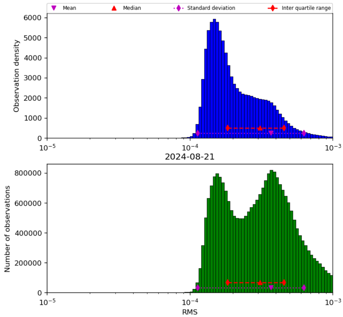
Figure 43: Histogram of “RMS” for 2024-08-21 to 2024-08-22
