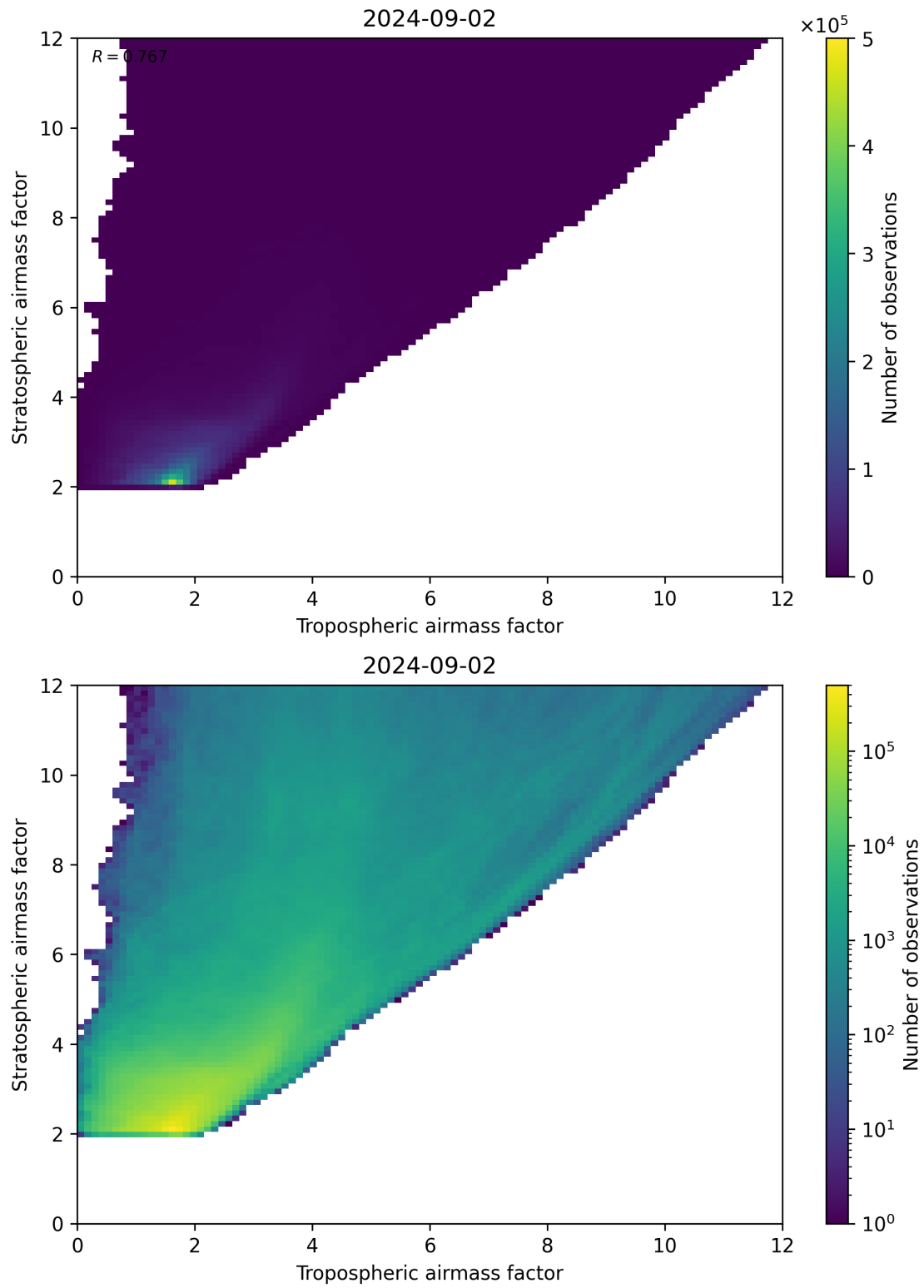
Figure 71: Scatter density plot of “Tropospheric airmass factor” against “Stratospheric airmass factor” for 2024-09-01 to 2024-09-03.
