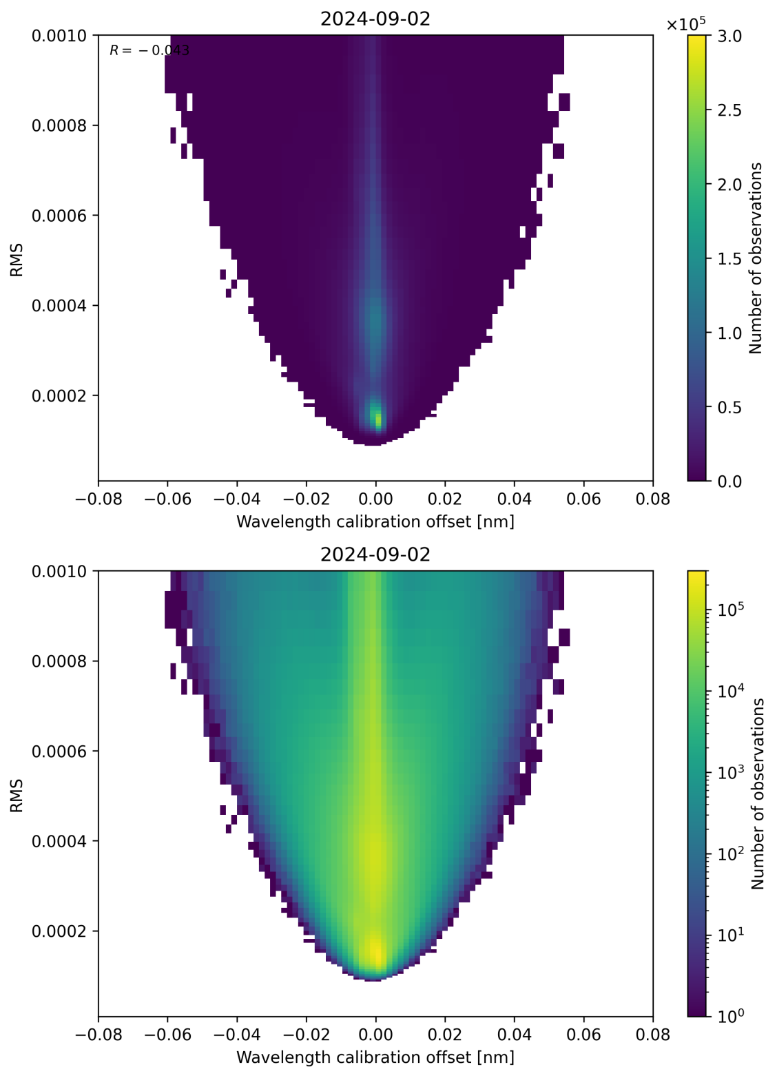
Figure 181: Scatter density plot of “Wavelength calibration offset” against “RMS” for 2024-09-01 to 2024-09-03.
