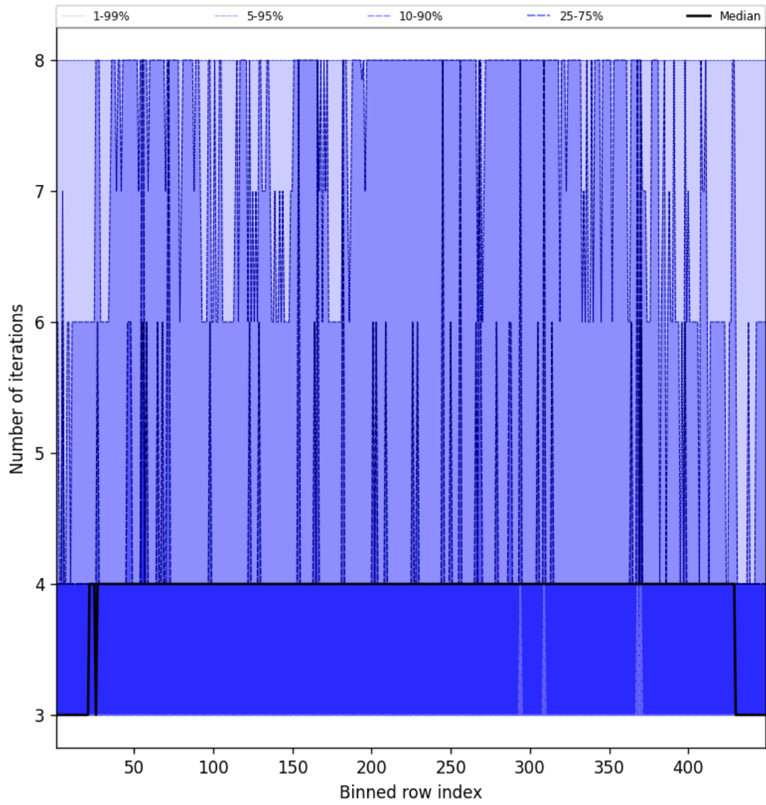
Figure 51: Along track statistics of “Number of iterations” for 2024-09-01 to 2024-09-03
