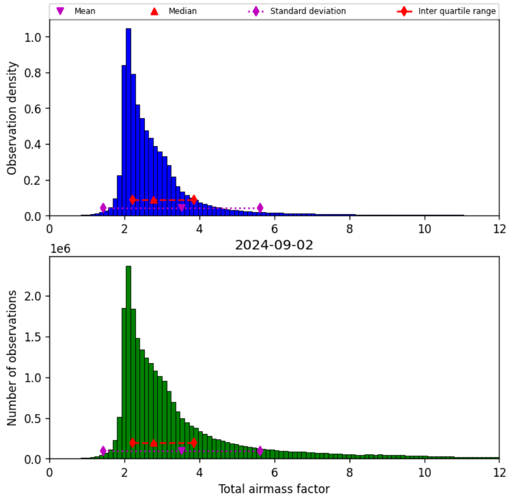
Figure 32: Histogram of “Total airmass factor” for 2024-09-01 to 2024-09-03
