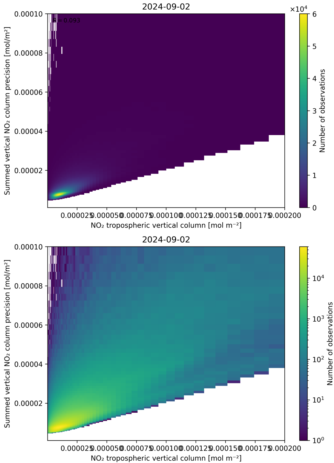
Figure 127: Scatter density plot of “NO 2 tropospheric vertical column” against “Summed vertical NO 2 column precision” for 2024-09-01 to 2024-09-03.
