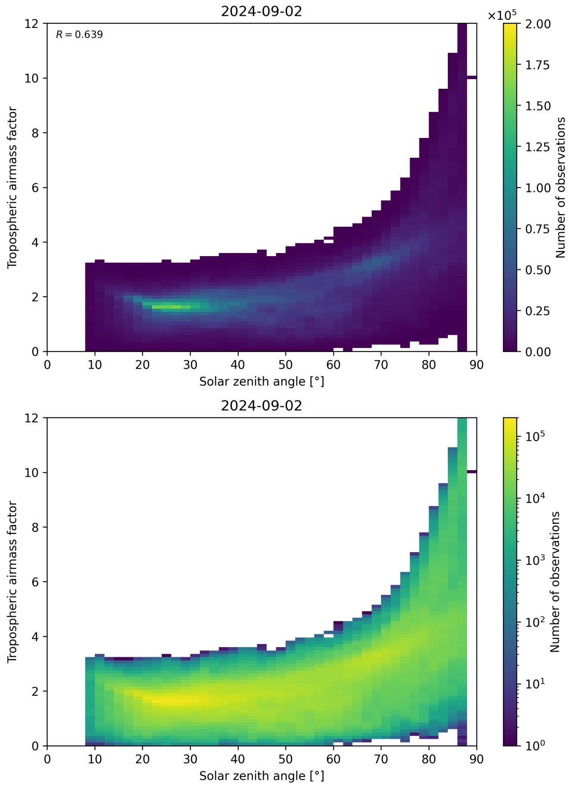
Figure 147: Scatter density plot of “Solar zenith angle” against “Tropospheric airmass factor” for 2024-09-01 to 2024-09-03.
