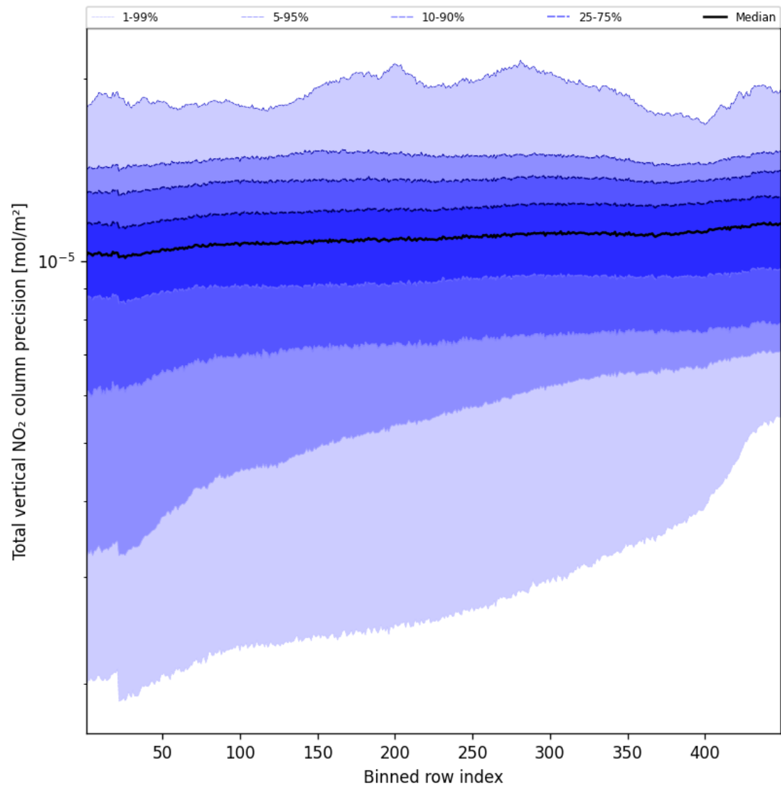
Figure 56: Along track statistics of “Total vertical NO 2 column precision” for 2024-09-01 to 2024-09-03
