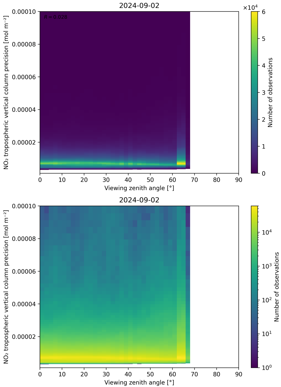
Figure 170: Scatter density plot of “Viewing zenith angle” against “NO 2 tropospheric vertical column precision” for 2024-09-01 to 2024-09-03.
