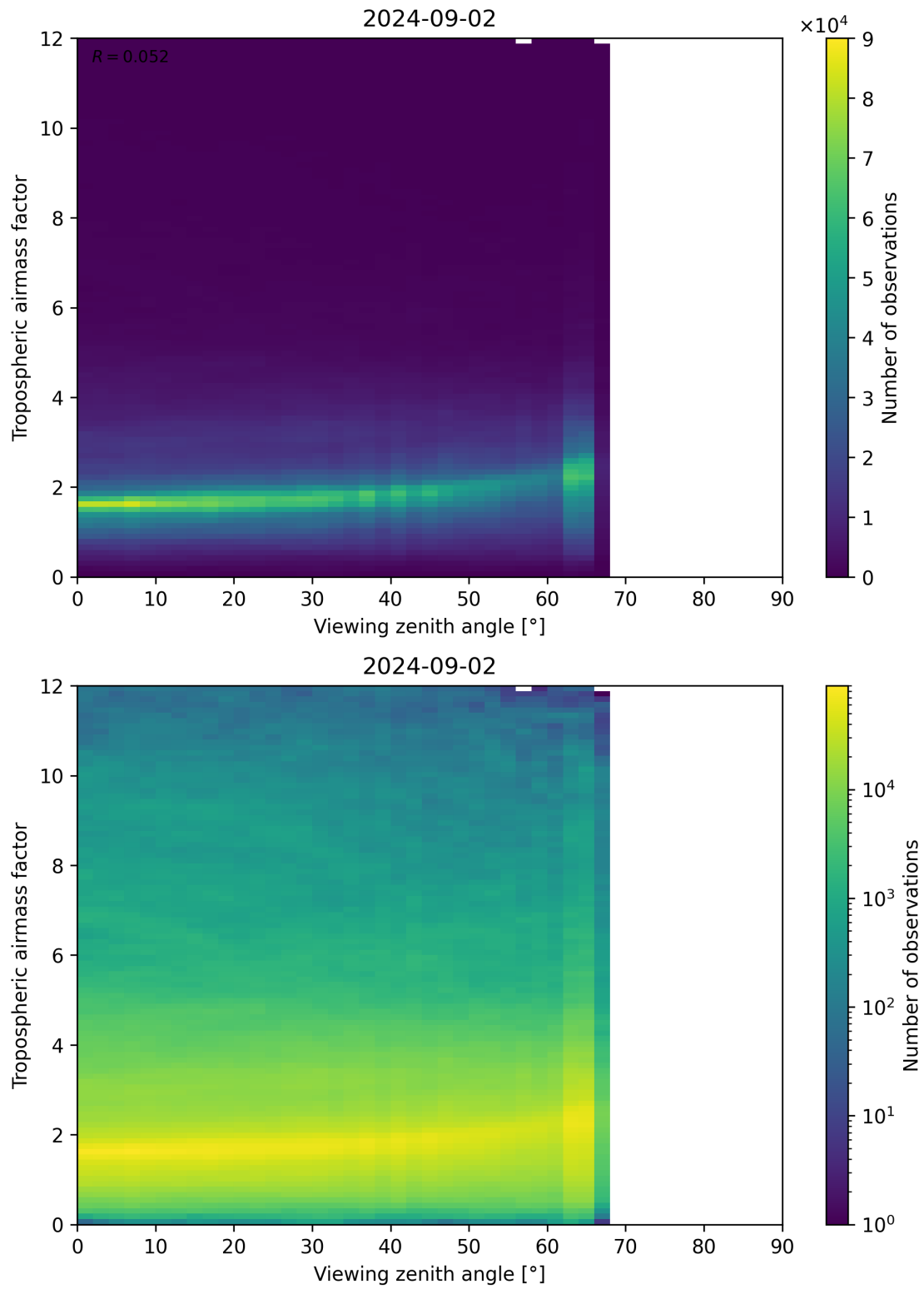
Figure 161: Scatter density plot of “Viewing zenith angle” against “Tropospheric airmass factor” for 2024-09-01 to 2024-09-03.
