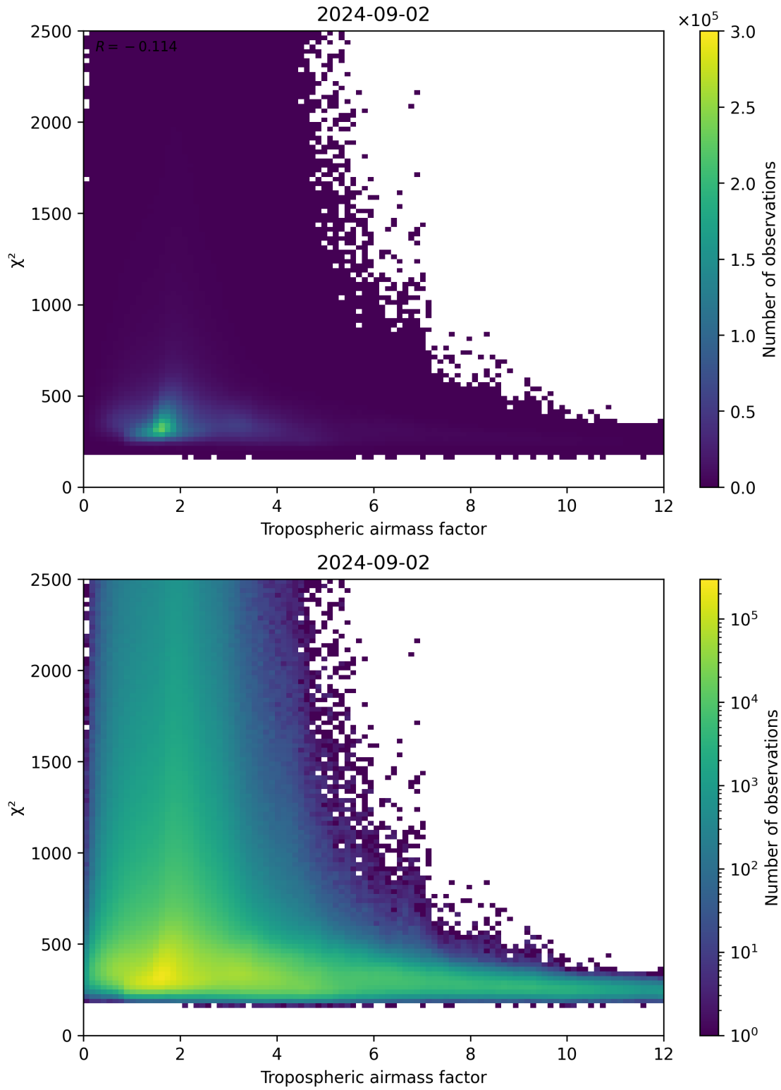
Figure 73: Scatter density plot of “Tropospheric airmass factor” against “ \chi^2 ” for 2024-09-01 to 2024-09-03.
