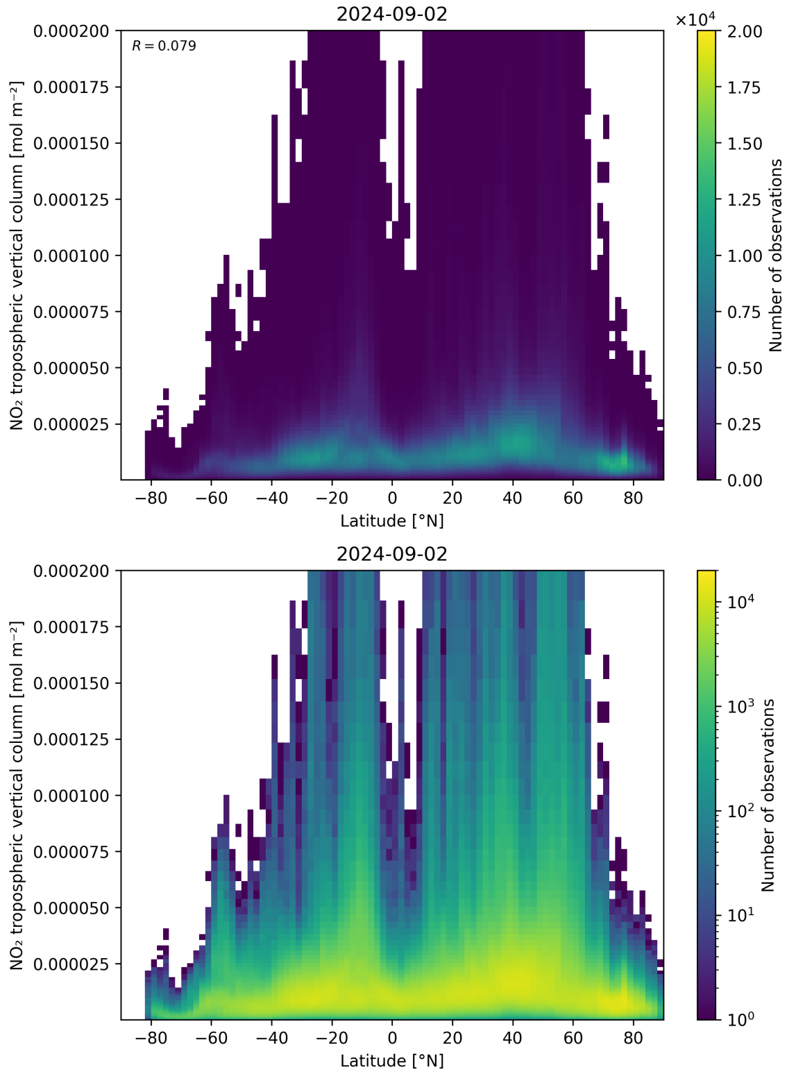
Figure 92: Scatter density plot of “Latitude” against “NO 2 tropospheric vertical column” for 2024-09-01 to 2024-09-03.
