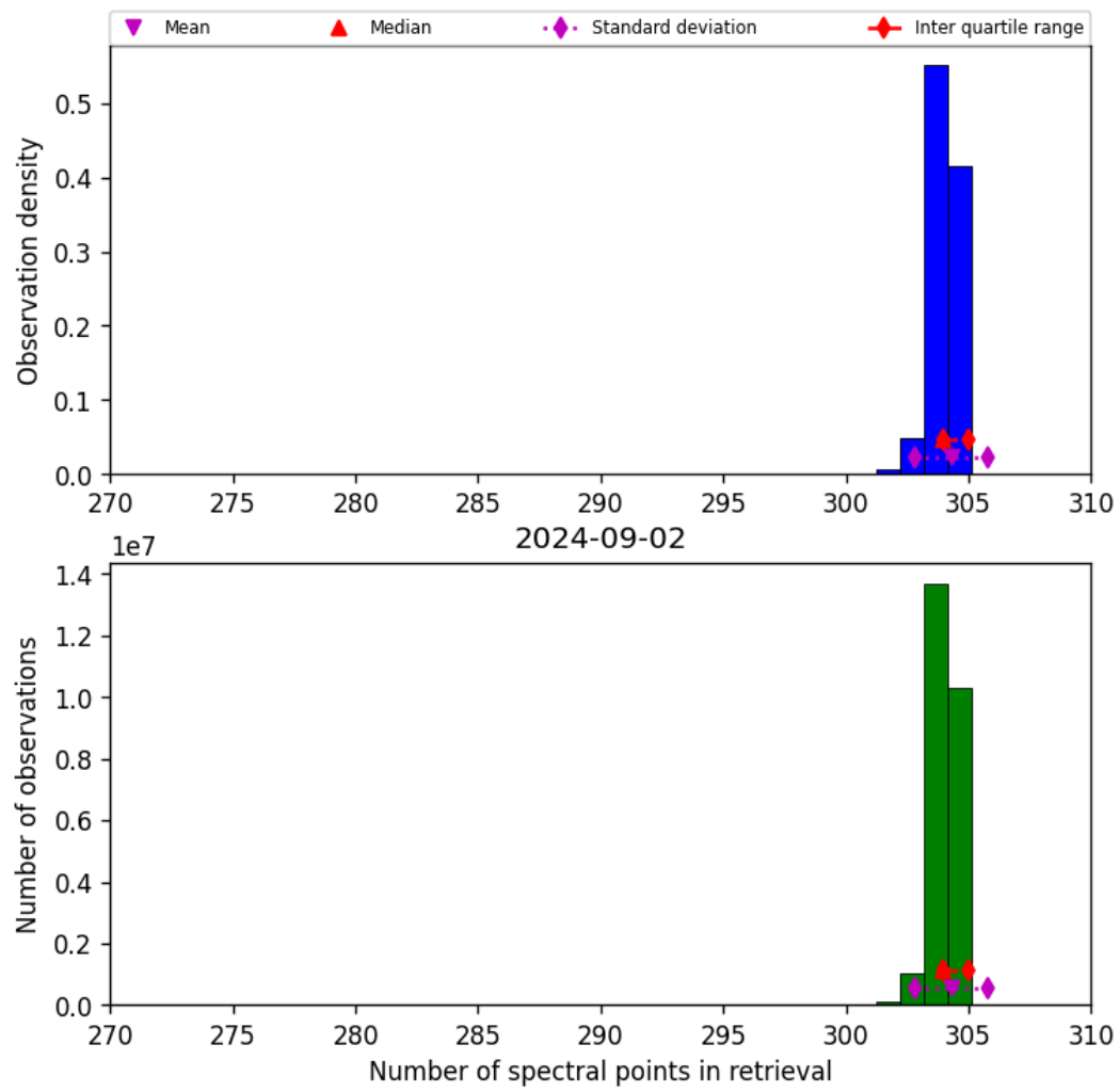
Figure 33: Histogram of “Number of spectral points in retrieval” for 2024-09-01 to 2024-09-03
