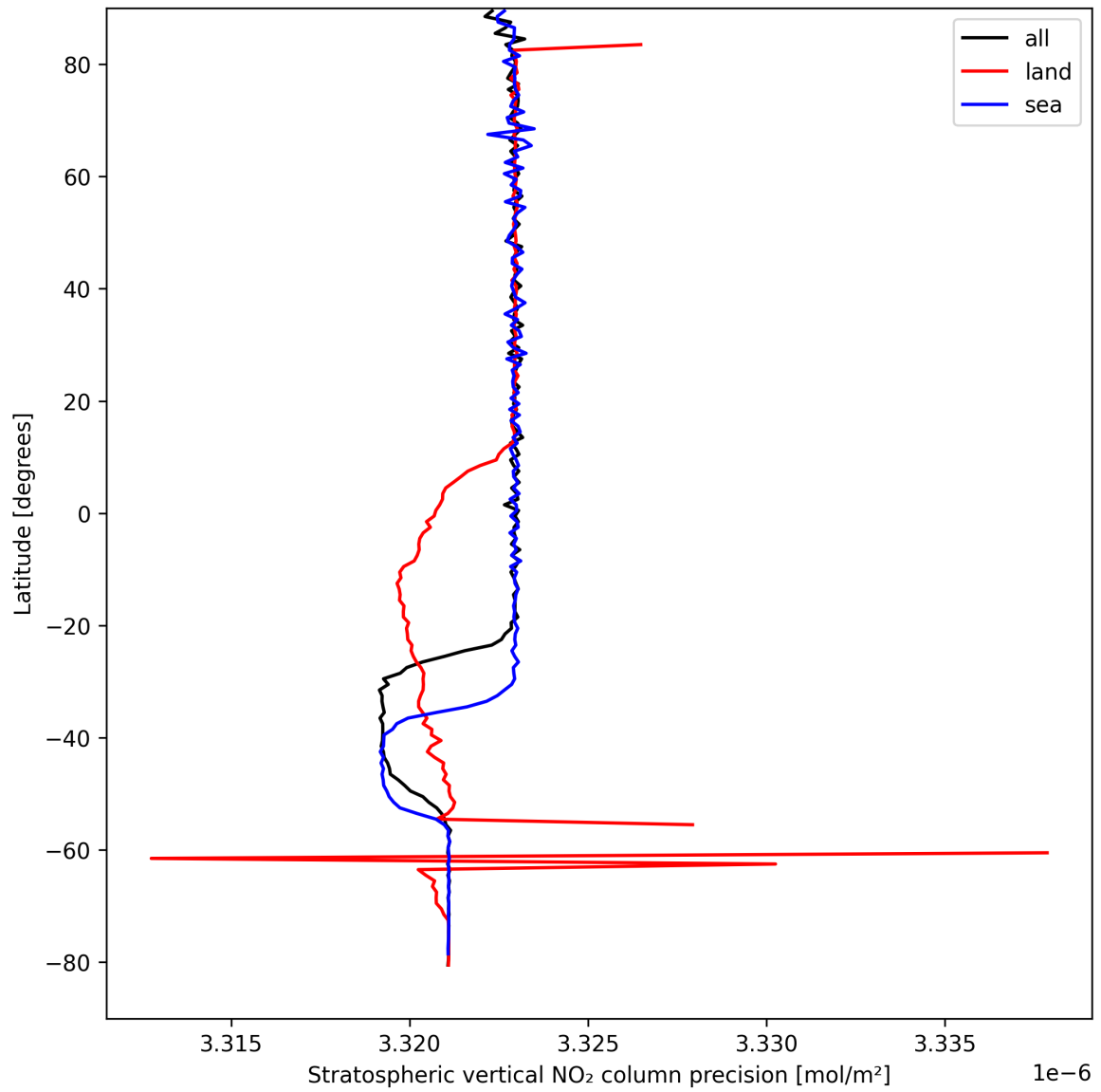
Figure 20: Zonal average of “Stratospheric vertical NO 2 column precision” for 2024-09-01 to 2024-09-03.
