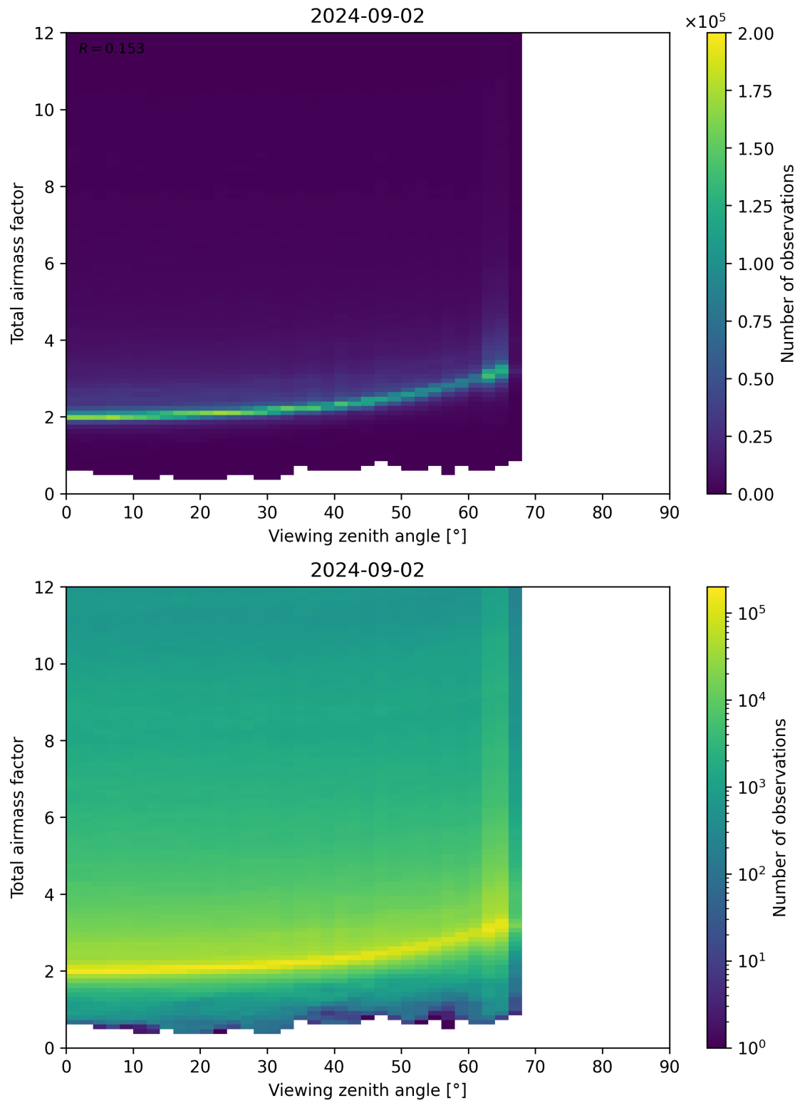
Figure 160: Scatter density plot of “Viewing zenith angle” against “Total airmass factor” for 2024-09-01 to 2024-09-03.
