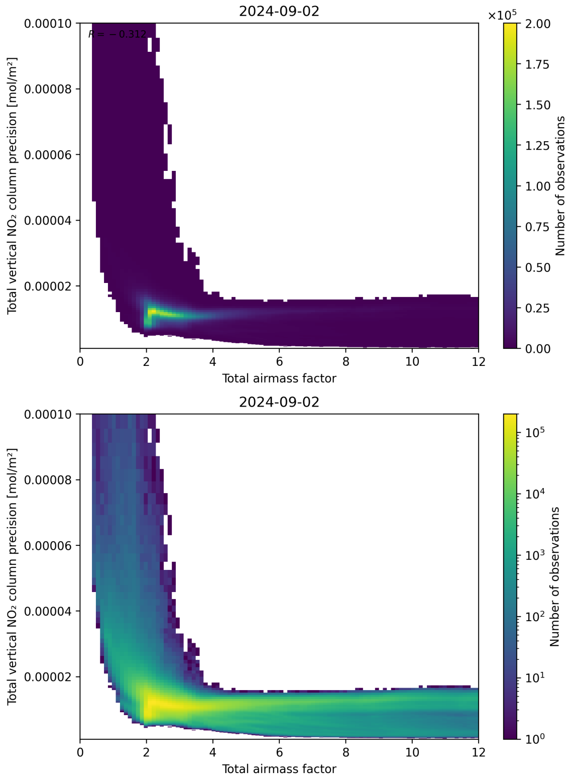
Figure 68: Scatter density plot of “Total airmass factor” against “Total vertical NO 2 column precision” for 2024-09-01 to 2024-09-03.
