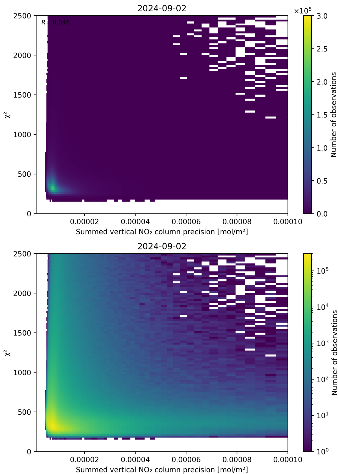
Figure 107: Scatter density plot of “Summed vertical NO 2 column precision” against “ \chi^2 ” for 2024-09-01 to 2024-09-03.
