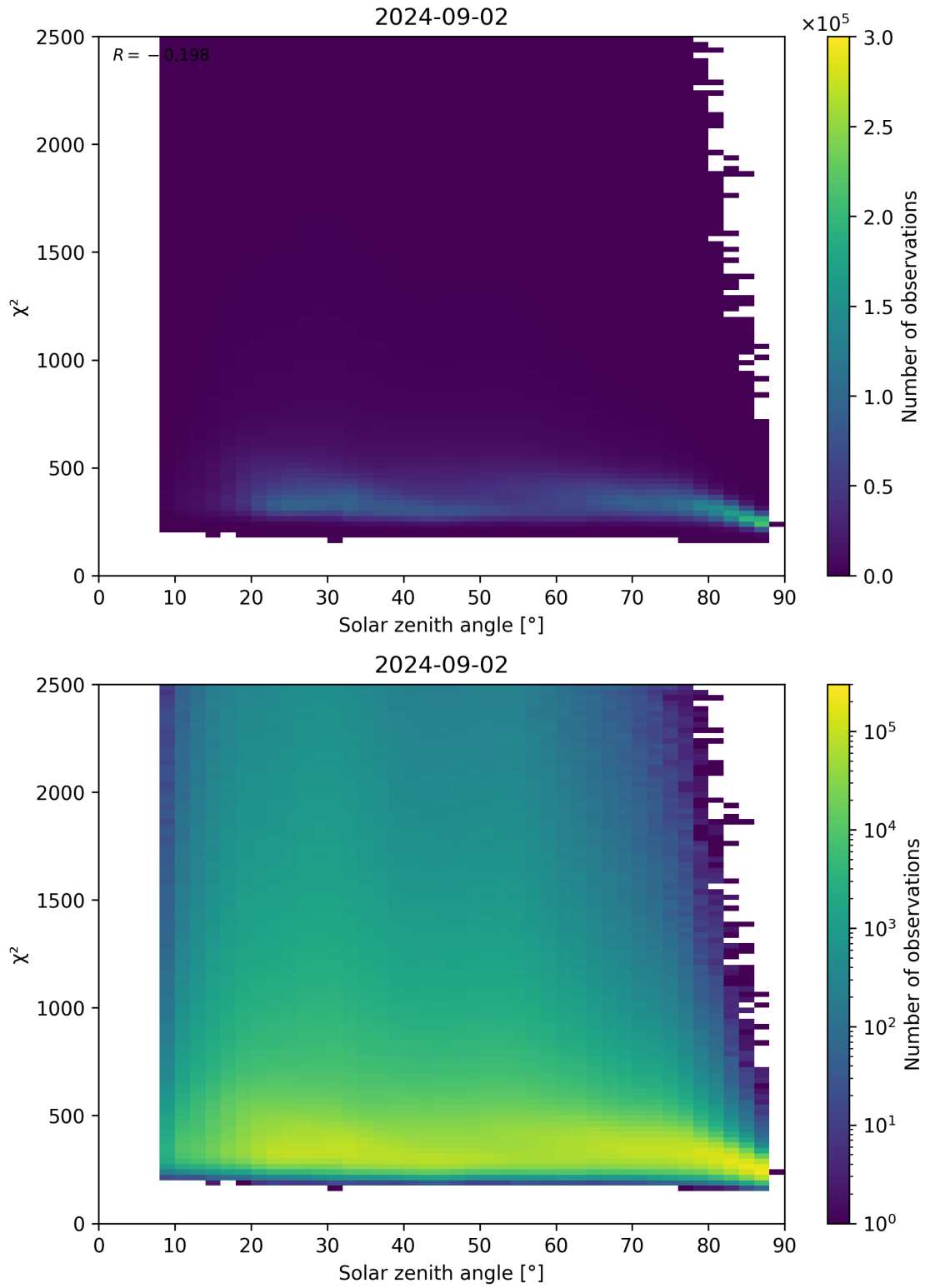
Figure 148: Scatter density plot of “Solar zenith angle” against “ \chi^2 ” for 2024-09-01 to 2024-09-03.
