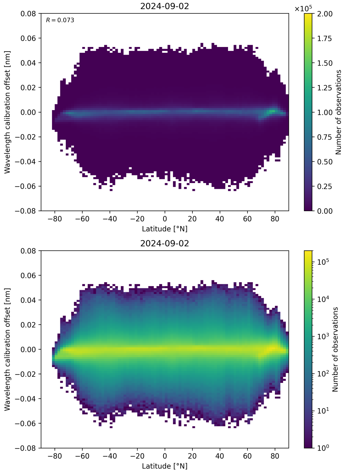
Figure 95: Scatter density plot of “Latitude” against “Wavelength calibration offset” for 2024-09-01 to 2024-09-03.
