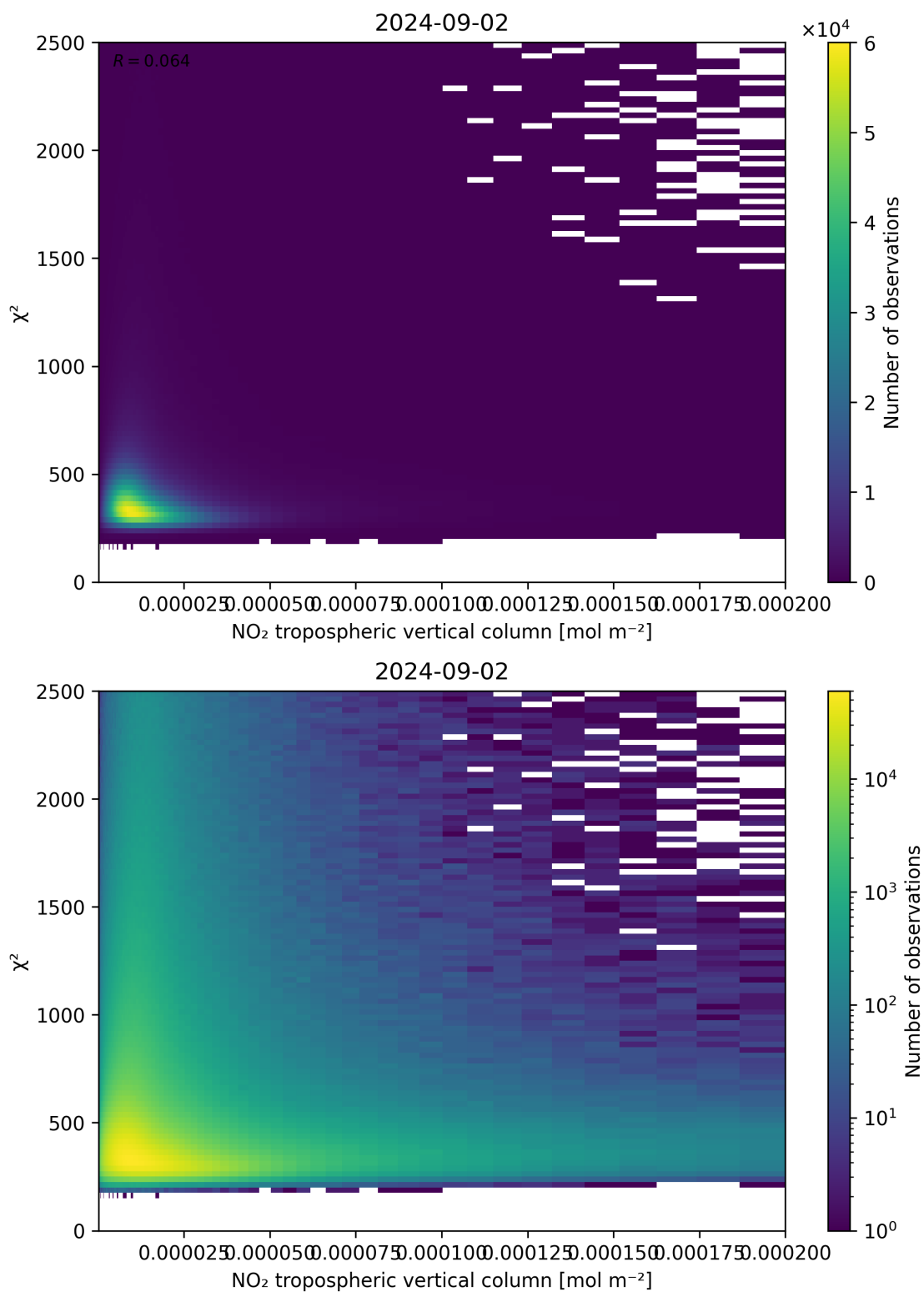
Figure 124: Scatter density plot of “NO 2 tropospheric vertical column” against “ \chi^2 ” for 2024-09-01 to 2024-09-03.
