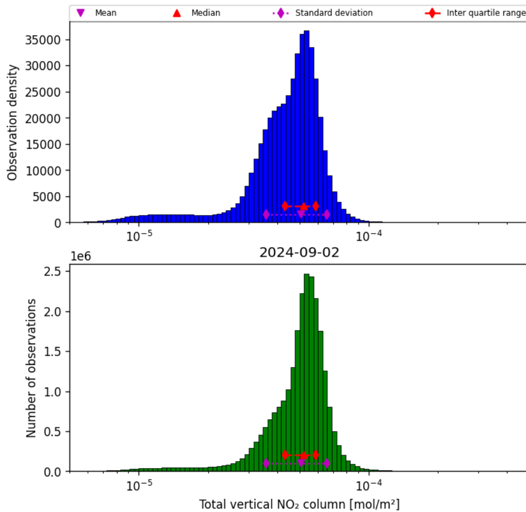
Figure 38: Histogram of "Total vertical NO 2 column" for 2024-09-01 to 2024-09-03
