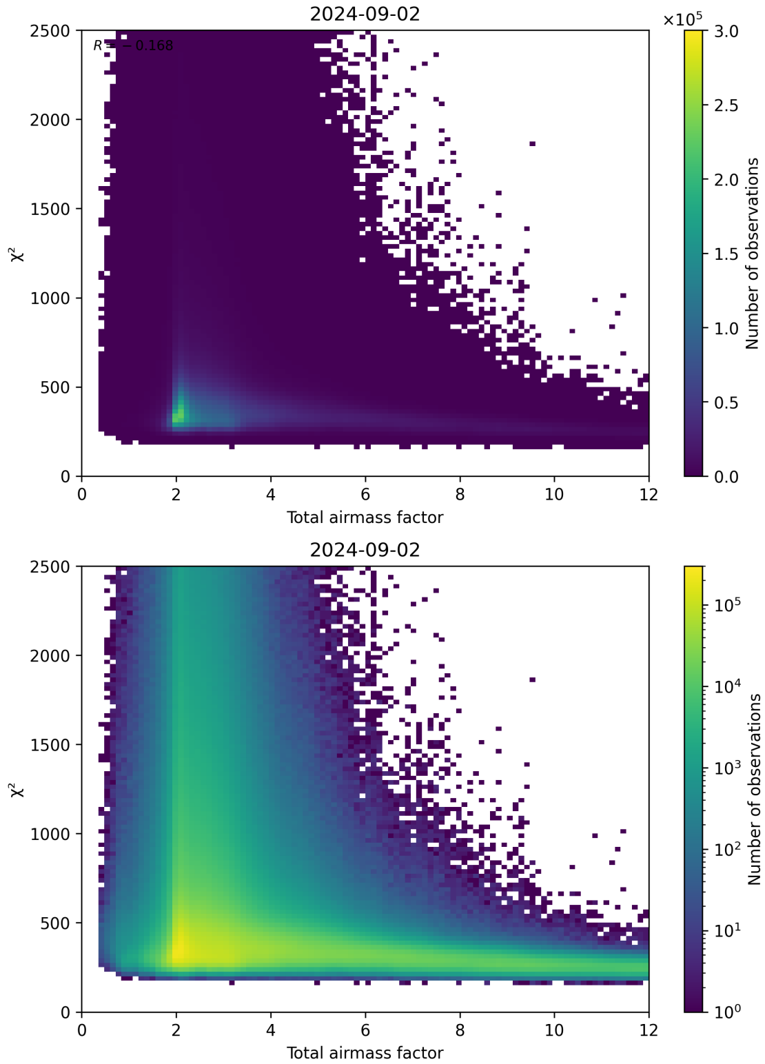
Figure 63: Scatter density plot of “Total airmass factor” against “ \chi^2 ” for 2024-09-01 to 2024-09-03.
