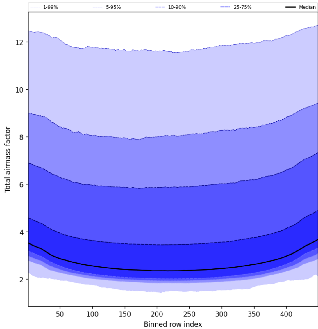
Figure 49: Along track statistics of “Total airmass factor” for 2024-09-01 to 2024-09-03
