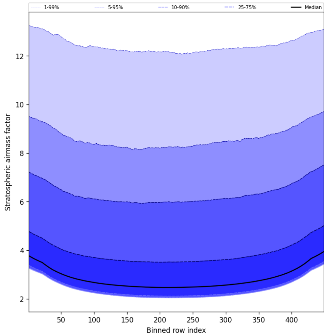
Figure 61: Along track statistics of “Stratospheric airmass factor” for 2024-09-01 to 2024-09-03
