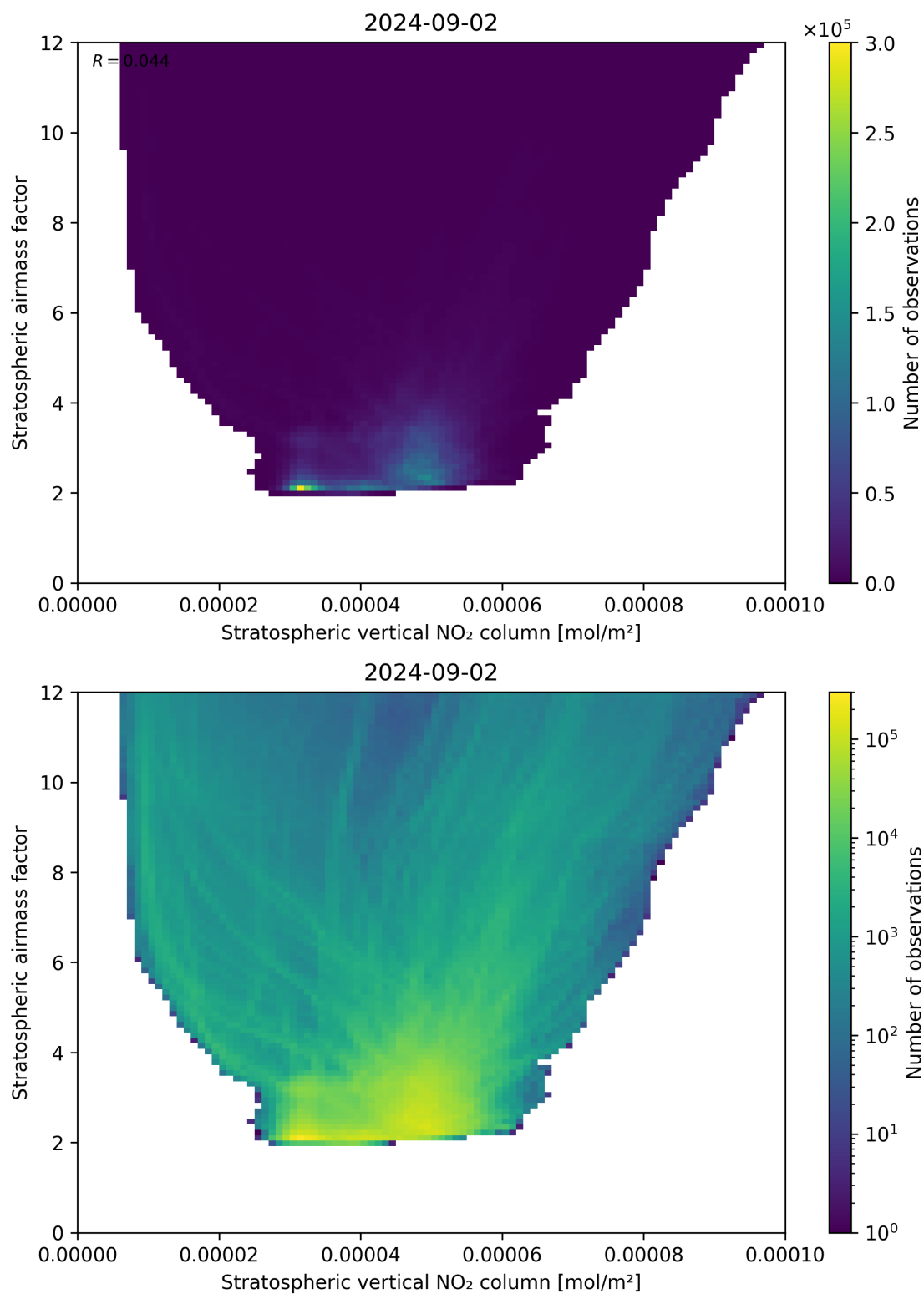
Figure 96: Scatter density plot of “Stratospheric vertical NO 2 column” against “Stratospheric airmass factor” for 2024-09-01 to 2024-09-03.
