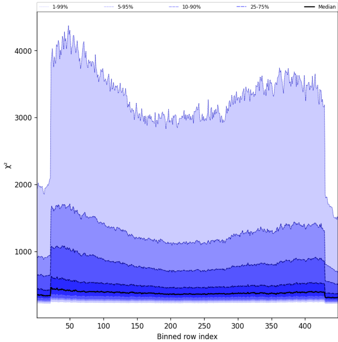
Figure 59: Along track statistics of “ \chi^2 ” for 2024-09-01 to 2024-09-03
