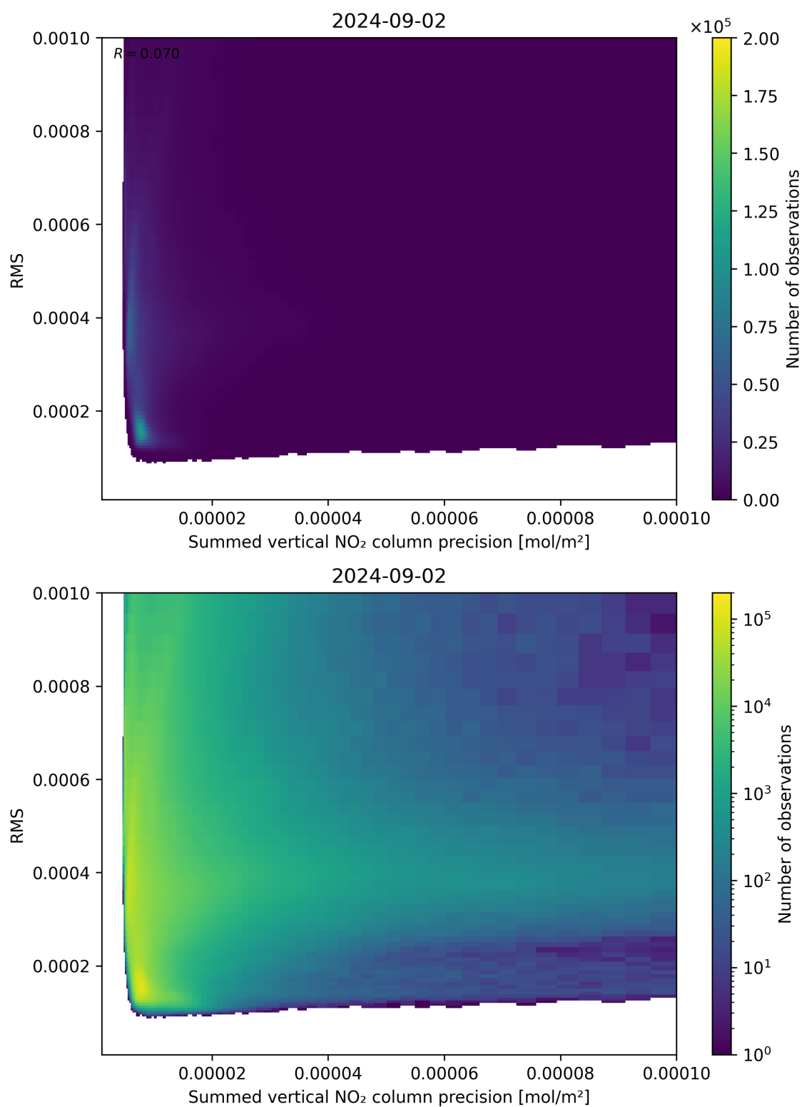
Figure 108: Scatter density plot of “Summed vertical NO 2 column precision” against “RMS” for 2024-09-01 to 2024-09-03.
