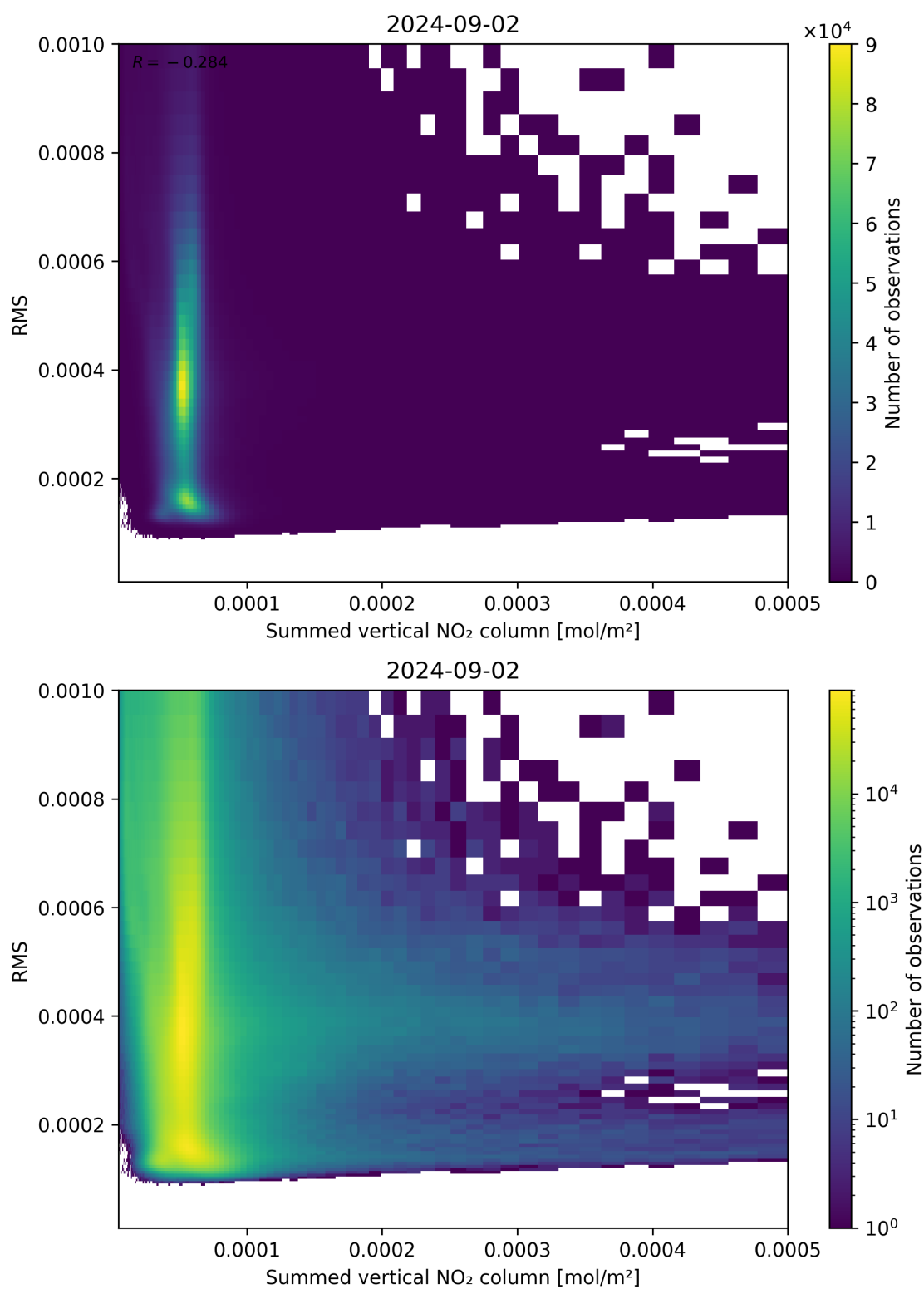
Figure 109: Scatter density plot of “Summed vertical NO 2 column” against “RMS” for 2024-09-01 to 2024-09-03.
