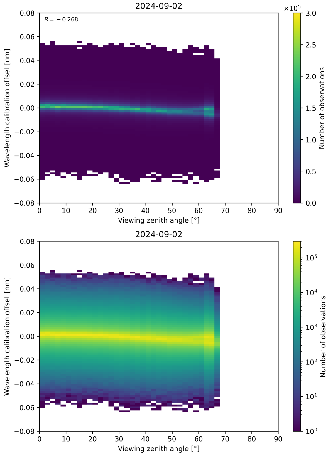
Figure 173: Scatter density plot of “Viewing zenith angle” against “Wavelength calibration offset” for 2024-09-01 to 2024-09-03.
