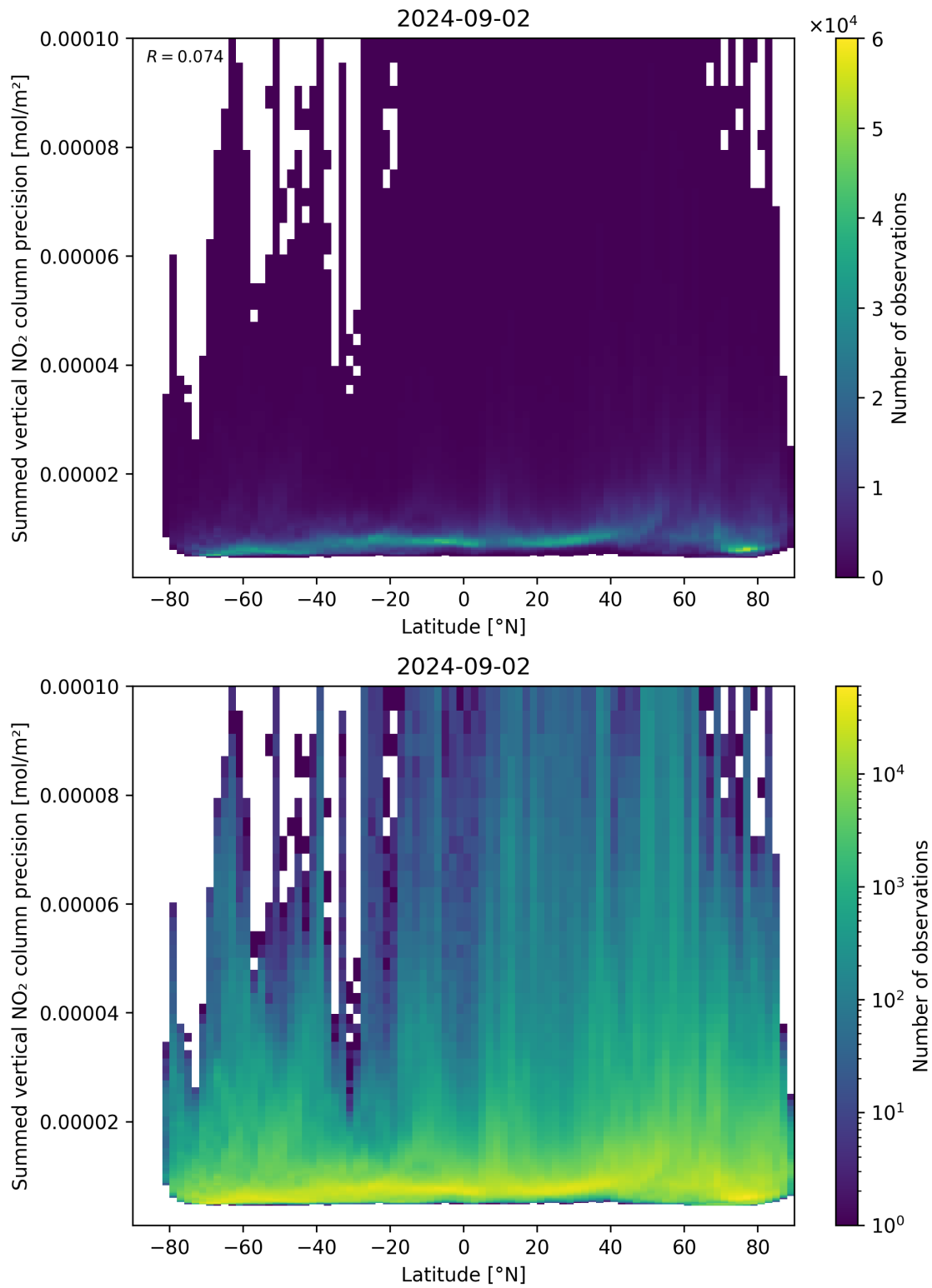
Figure 89: Scatter density plot of “Latitude” against “Summed vertical NO 2 column precision” for 2024-09-01 to 2024-09-03.
