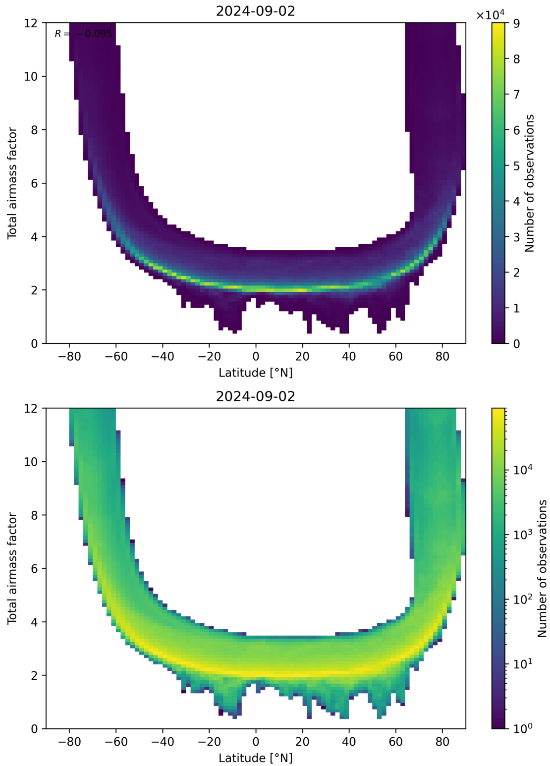
Figure 84: Scatter density plot of “Latitude” against “Total airmass factor” for 2024-09-01 to 2024-09-03.
