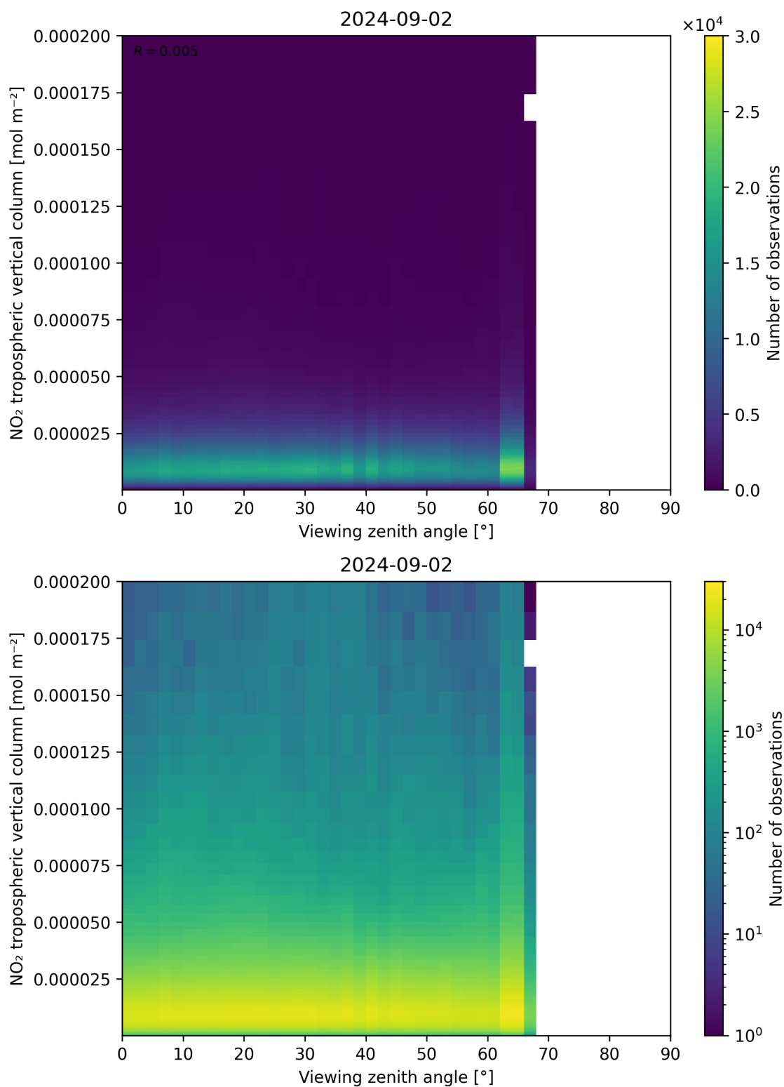
Figure 169: Scatter density plot of “Viewing zenith angle” against “NO 2 tropospheric vertical column” for 2024-09-01 to 2024-09-03.
