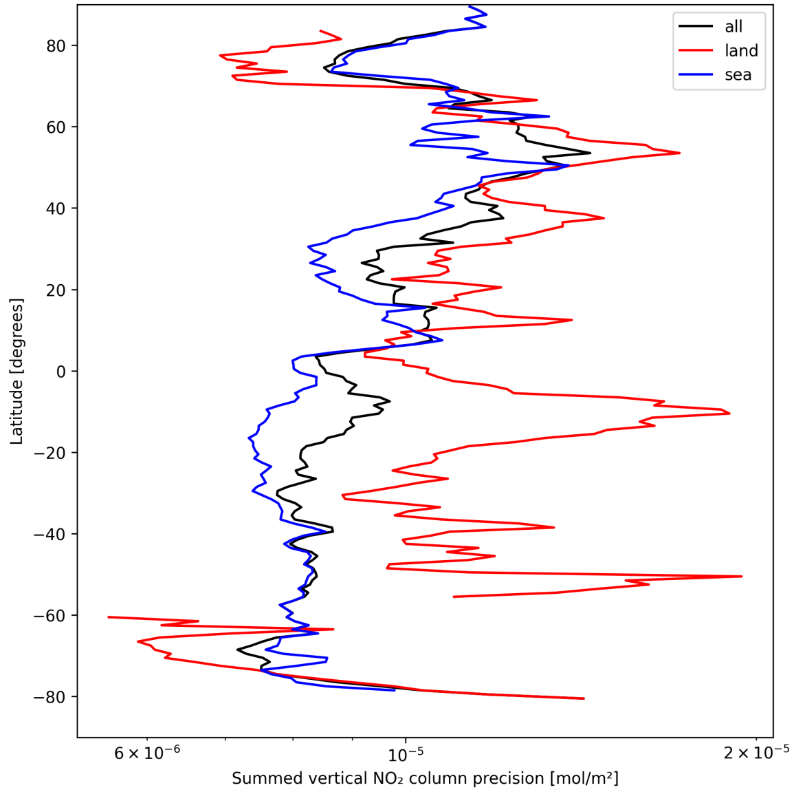
Figure 24: Zonal average of “Summed vertical NO 2 column precision” for 2024-09-01 to 2024-09-03.
