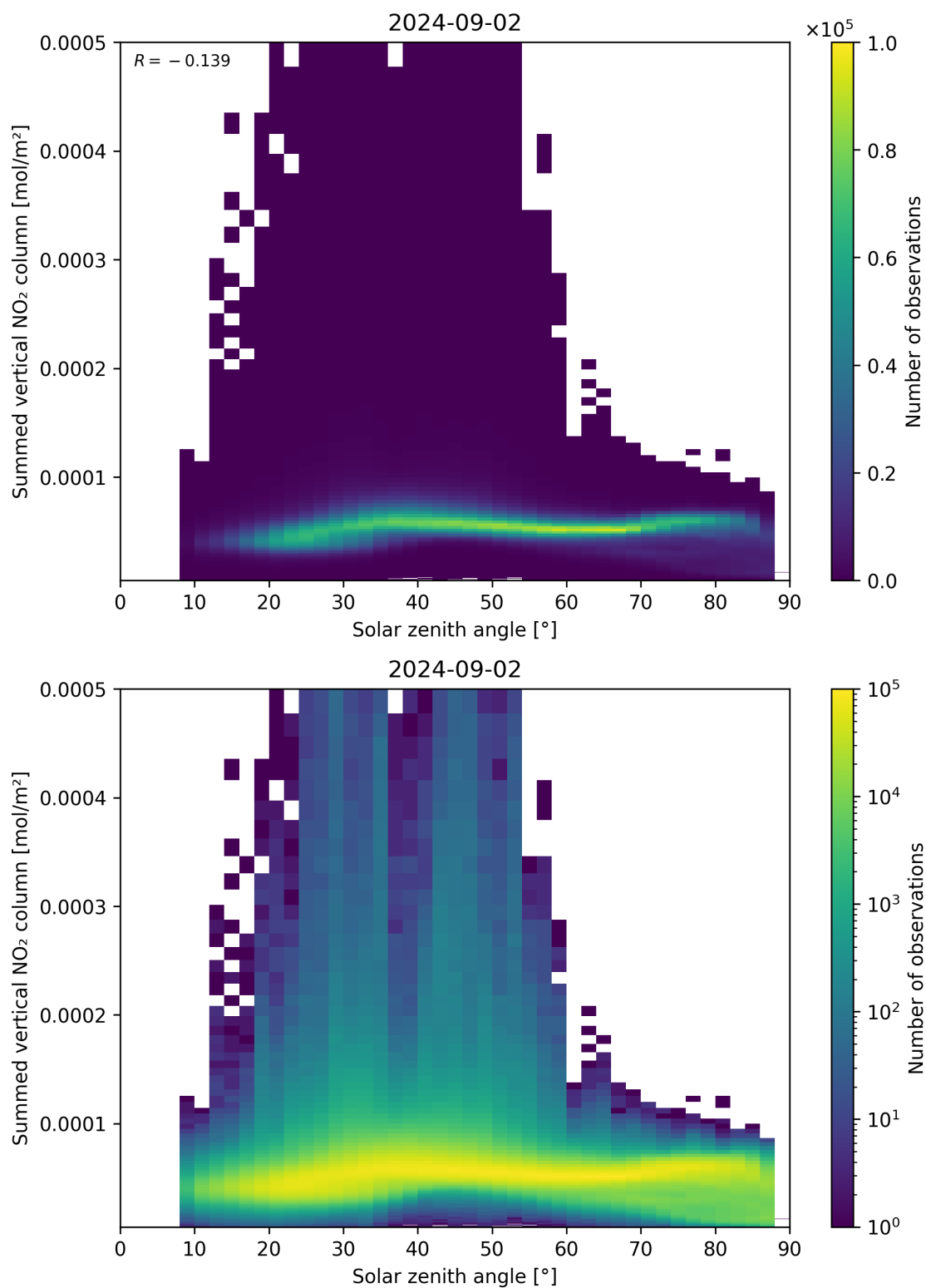
Figure 151: Scatter density plot of “Solar zenith angle” against “Summed vertical NO 2 column” for 2024-09-01 to 2024-09-03.
