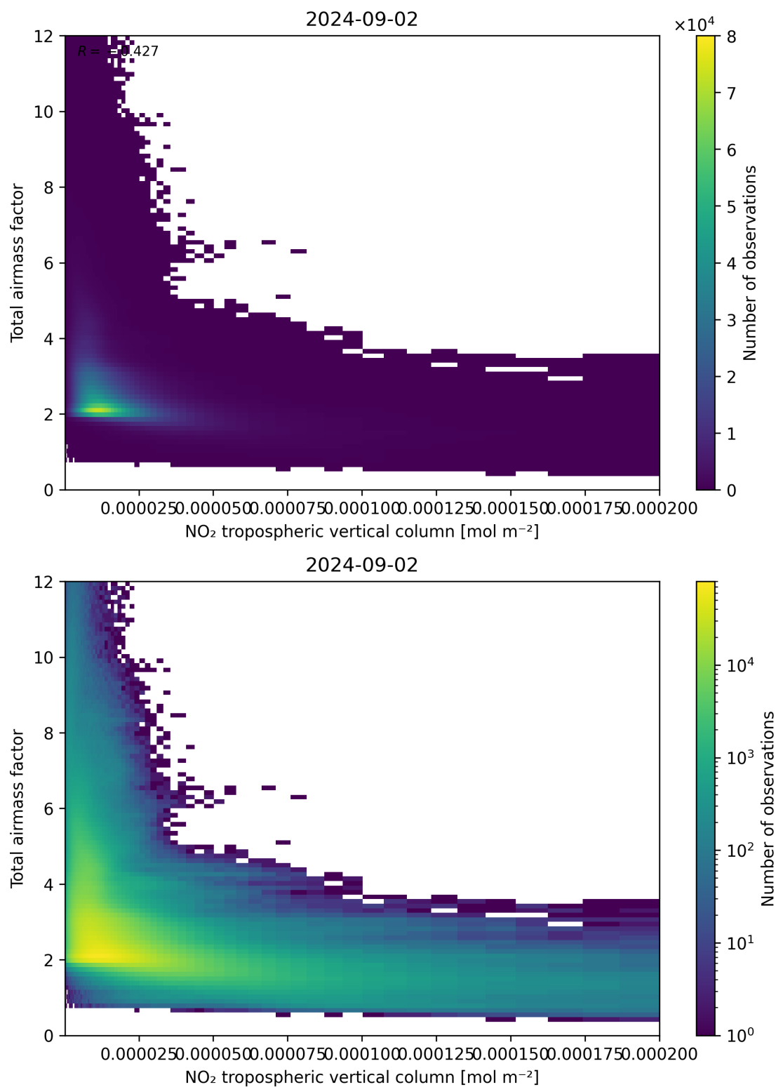
Figure 122: Scatter density plot of “NO 2 tropospheric vertical column” against “Total air mass factor” for 2024-09-01 to 2024-09-03.
