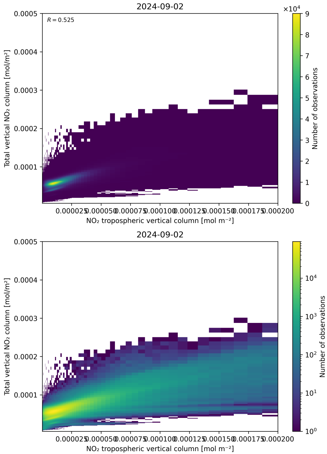
Figure 128: Scatter density plot of “NO 2 tropospheric vertical column” against “Total vertical NO 2 column” for 2024-09-01 to 2024-09-03.
