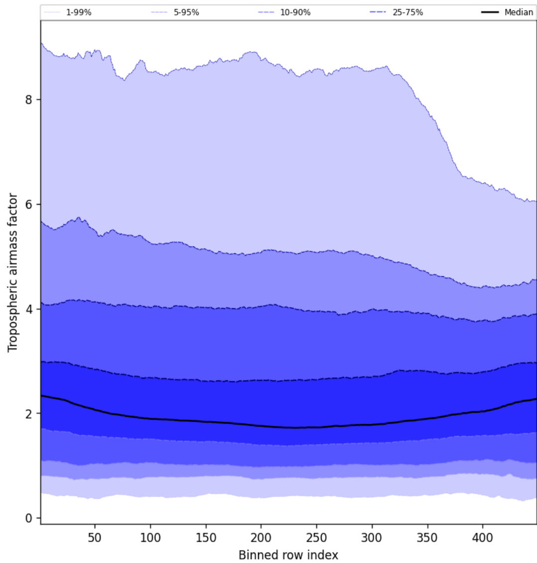
Figure 48: Along track statistics of “Tropospheric air mass factor” for 2024-09-01 to 2024-09-03
