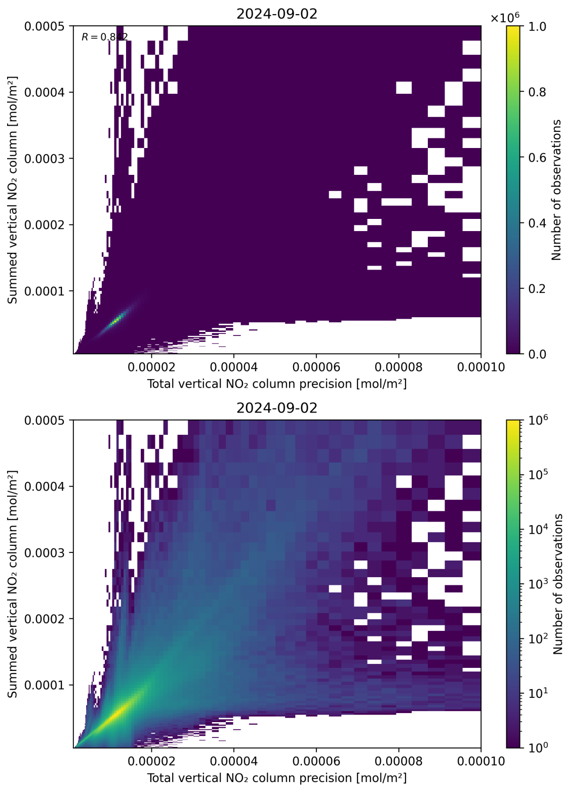
Figure 117: Scatter density plot of “Total vertical NO 2 column precision” against “Summed vertical NO 2 column” for 2024-09-01 to 2024-09-03.
