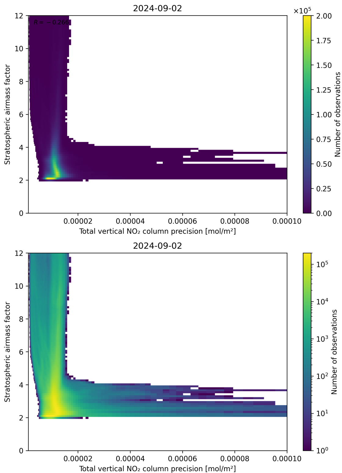
Figure 115: Scatter density plot of “Total vertical NO 2 column precision” against “Stratospheric air mass factor” for 2024-09-01 to 2024-09-03.
