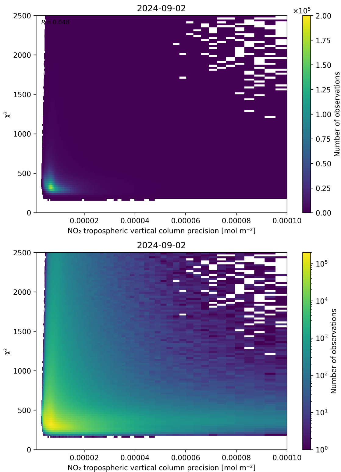
Figure 134: Scatter density plot of “NO 2 tropospheric vertical column precision” against “ \chi^2 ” for 2024-09-01 to 2024-09-03.
