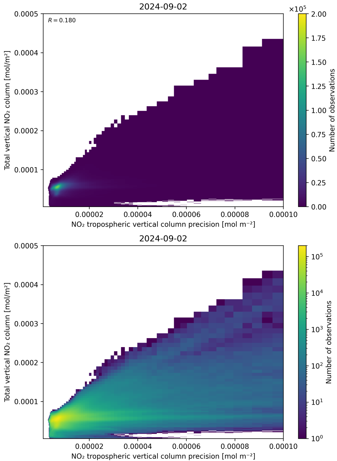
Figure 138: Scatter density plot of “NO 2 tropospheric vertical column precision” against “Total vertical NO 2 column” for 2024-09-01 to 2024-09-03.
