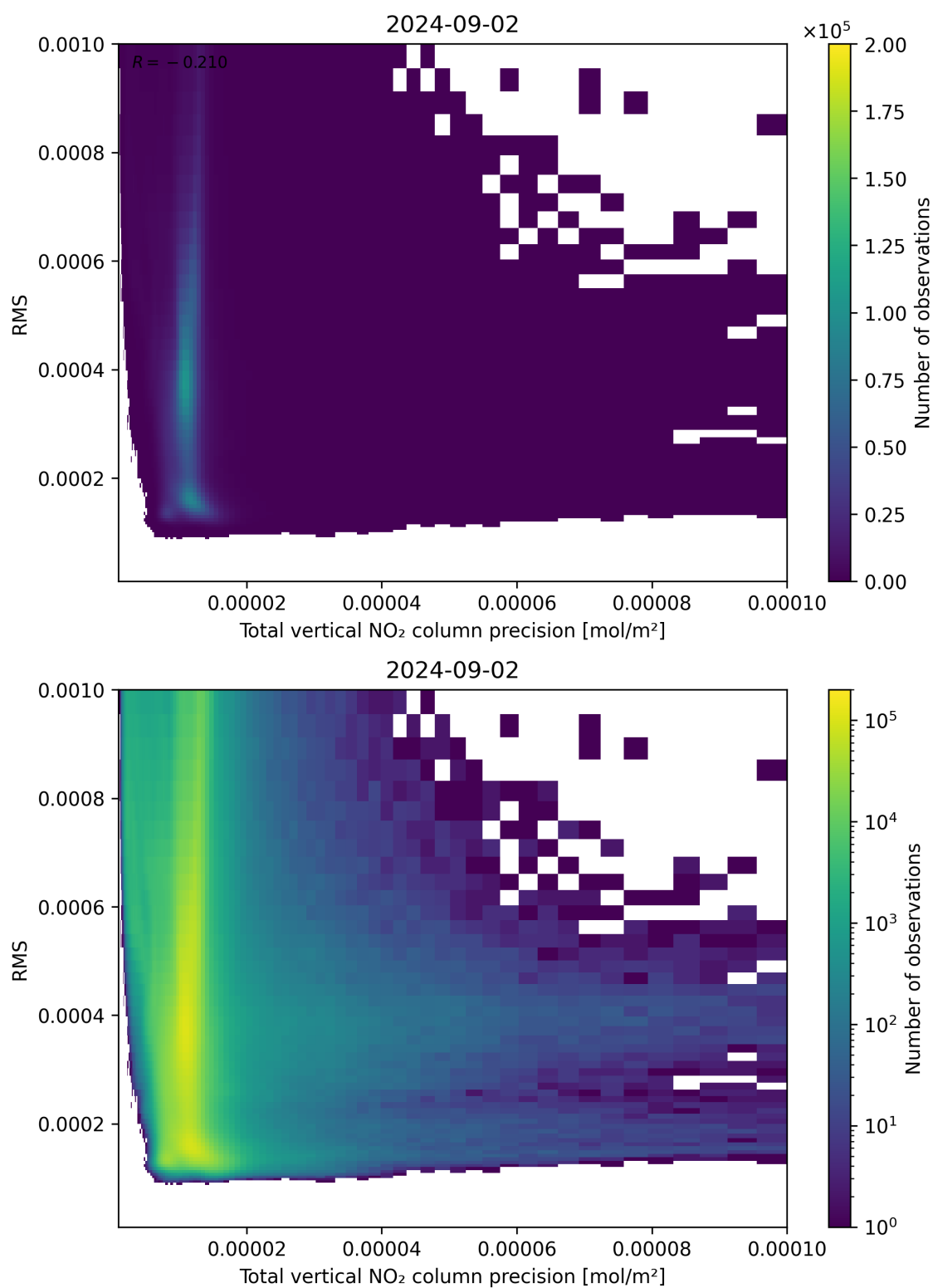
Figure 119: Scatter density plot of “Total vertical NO 2 column precision” against “RMS” for 2024-09-01 to 2024-09-03.
