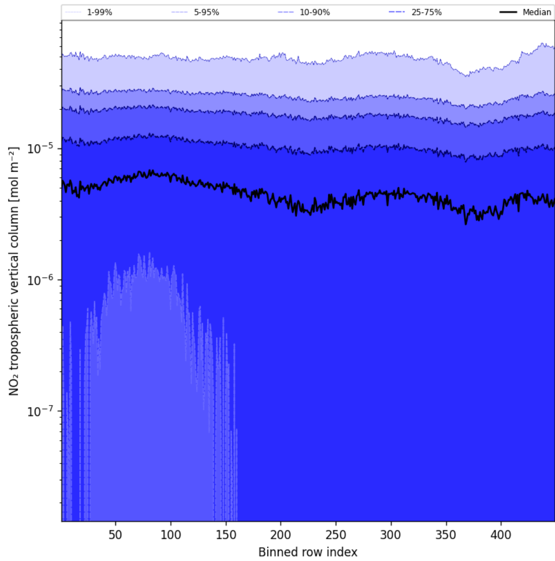
Figure 46: Along track statistics of “NO 2 tropospheric vertical column” for 2024-09-01 to 2024-09-03
