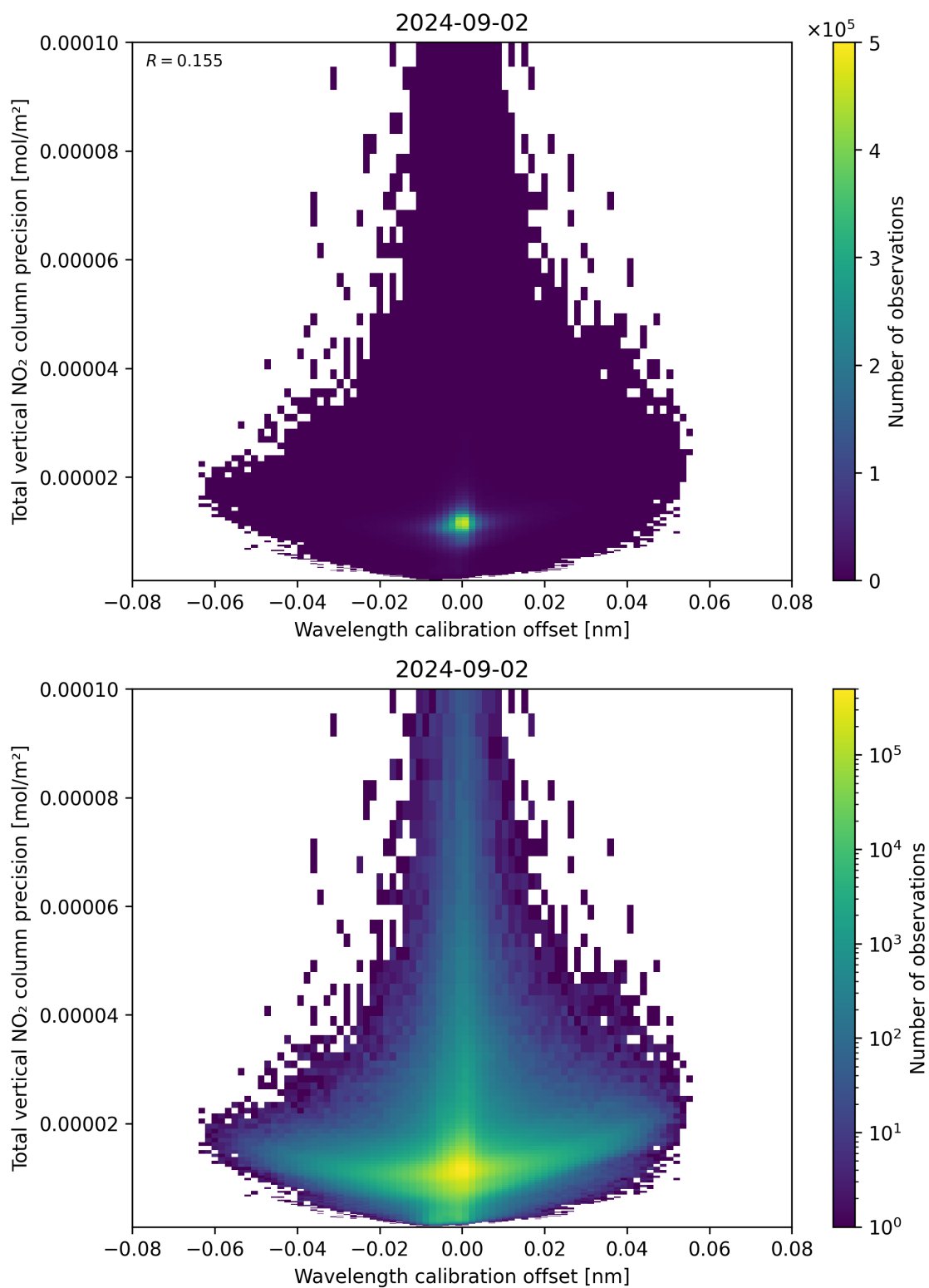
Figure 180: Scatter density plot of “Wavelength calibration offset” against “Total vertical NO 2 column precision” for 2024-09-01 to 2024-09-03.
