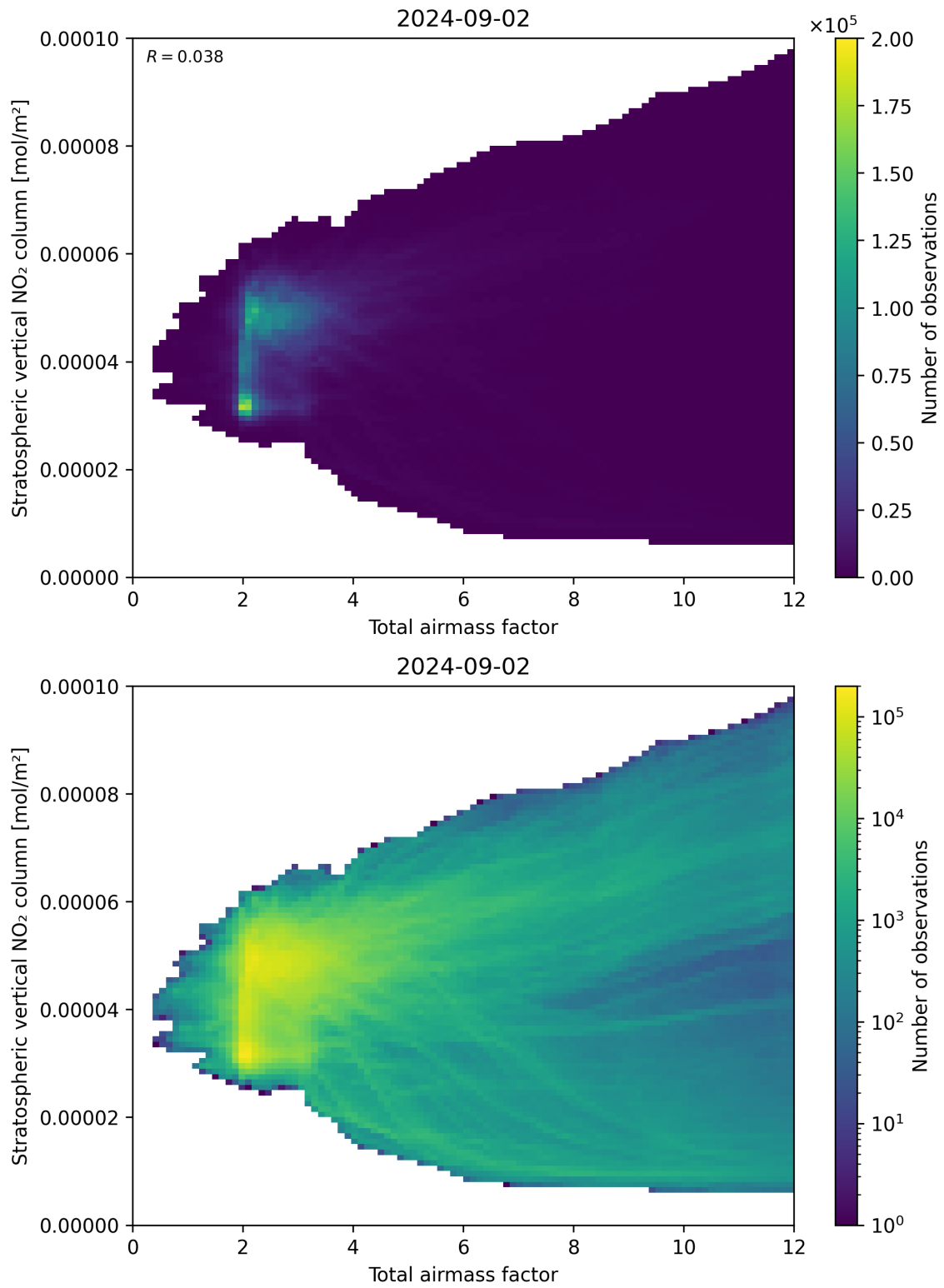
Figure 64: Scatter density plot of “Total airmass factor” against “Stratospheric vertical NO 2 column” for 2024-09-01 to 2024-09-03.
