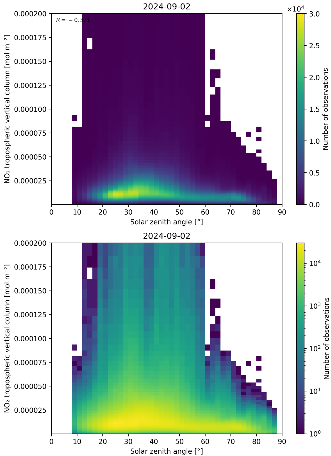
Figure 155: Scatter density plot of “Solar zenith angle” against “NO 2 tropospheric vertical column” for 2024-09-01 to 2024-09-03.
