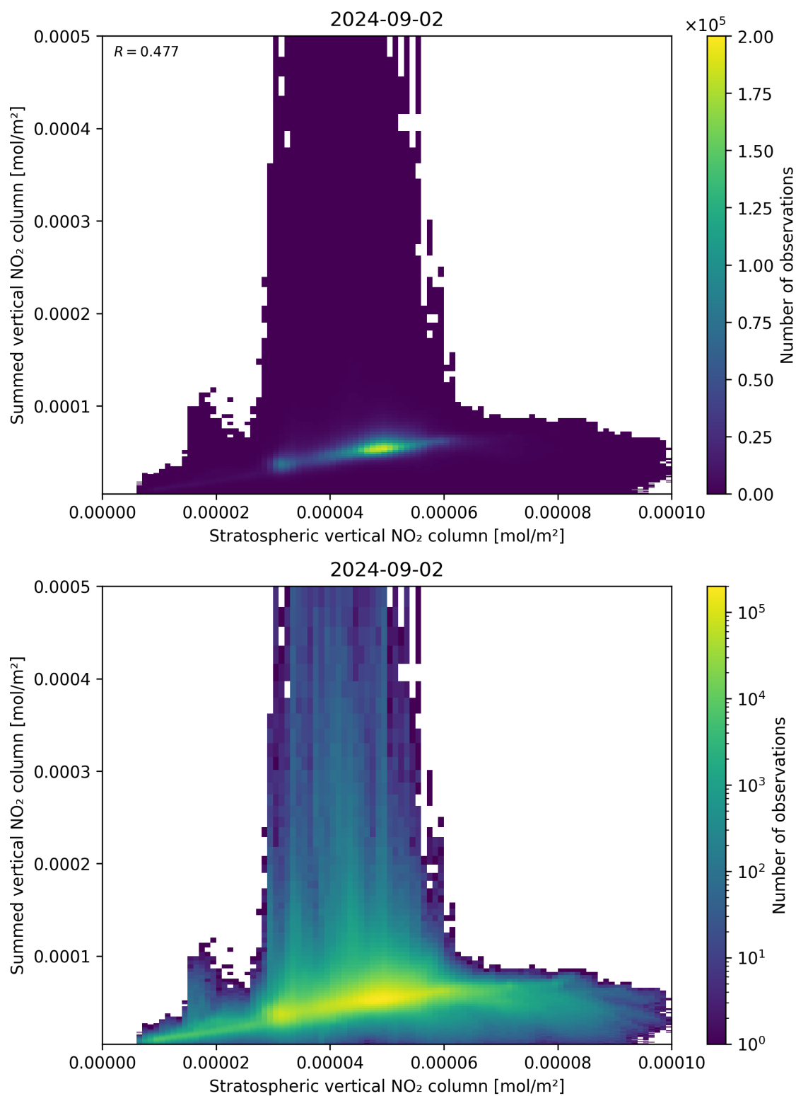
Figure 98: Scatter density plot of “Stratospheric vertical NO 2 column” against “Summed vertical NO 2 column” for 2024-09-01 to 2024-09-03.
