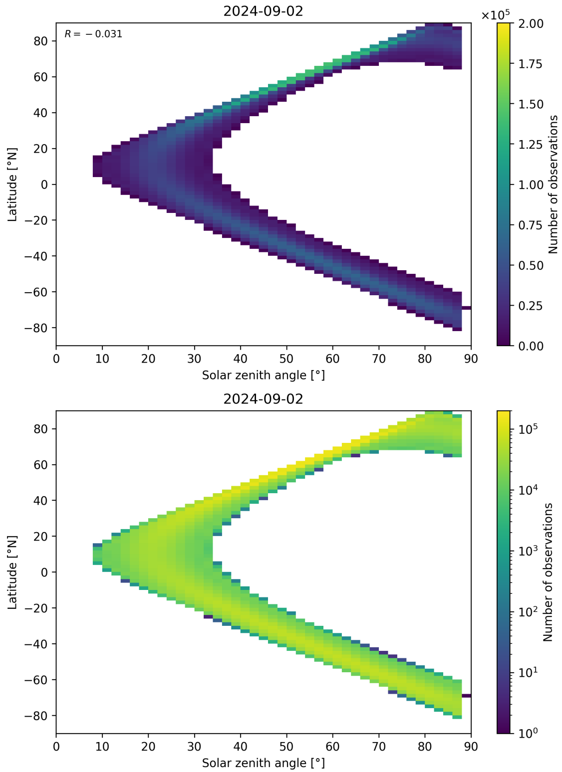
Figure 149: Scatter density plot of “Solar zenith angle” against “Latitude” for 2024-09-01 to 2024-09-03.
