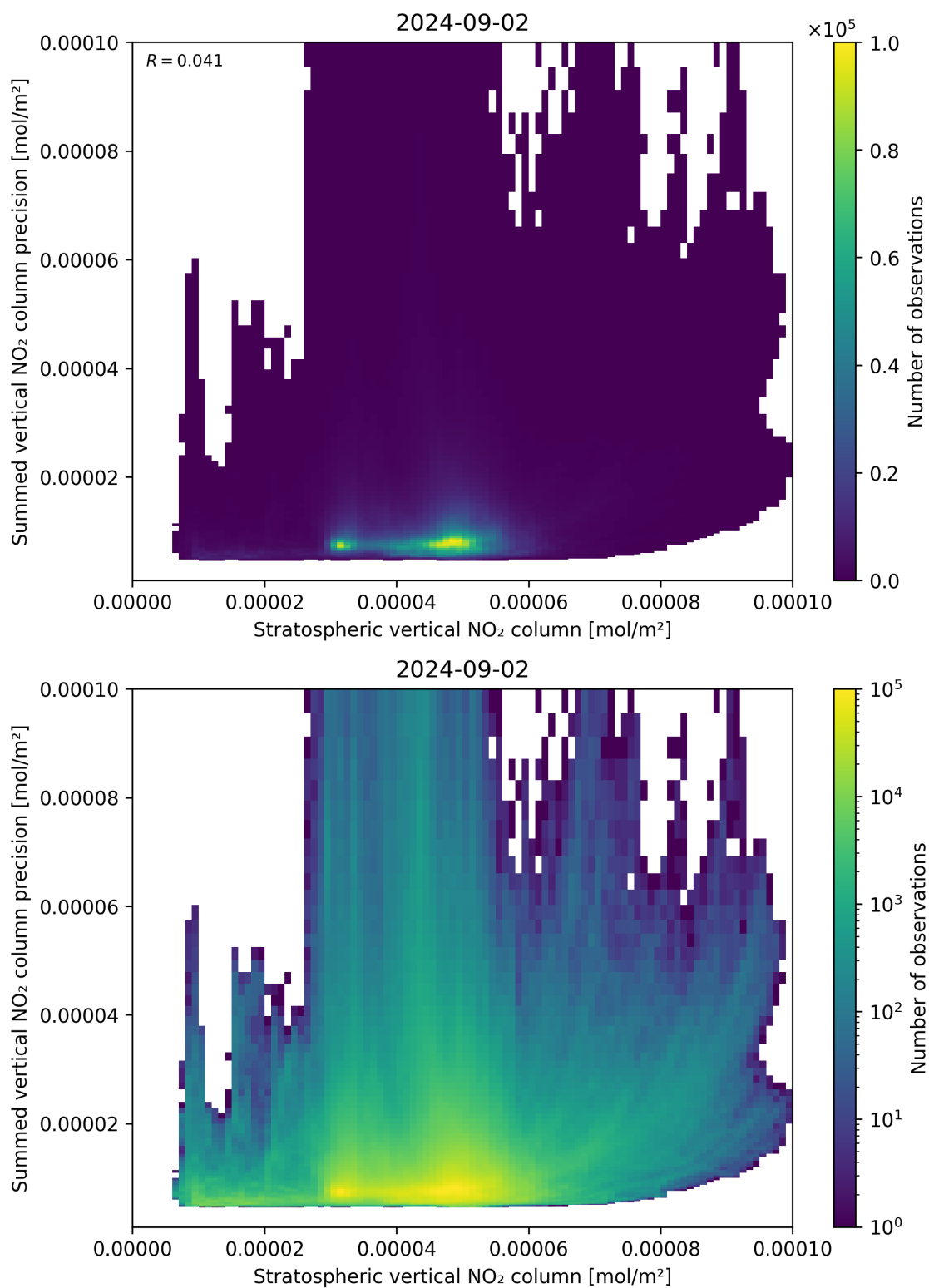
Figure 99: Scatter density plot of “Stratospheric vertical NO 2 column” against “Summed vertical NO 2 column precision” for 2024-09-01 to 2024-09-03.
