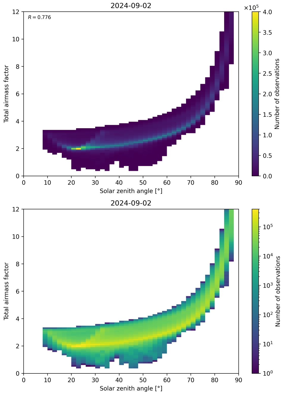
Figure 146: Scatter density plot of “Solar zenith angle” against “Total airmass factor” for 2024-09-01 to 2024-09-03.
