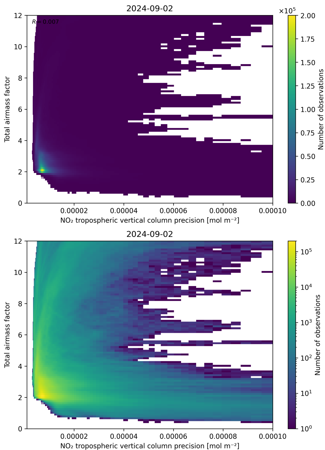
Figure 132: Scatter density plot of “NO 2 tropospheric vertical column precision” against “Total air mass factor” for 2024-09-01 to 2024-09-03.
