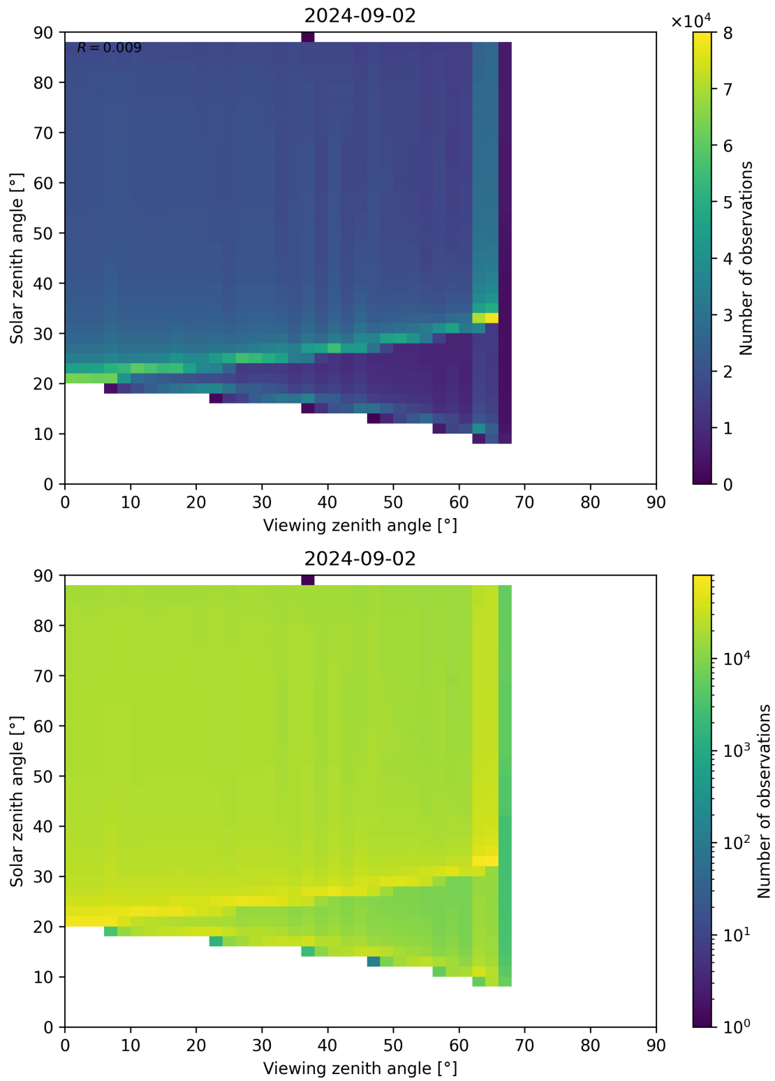
Figure 172: Scatter density plot of “Viewing zenith angle” against “Solar zenith angle” for 2024-09-01 to 2024-09-03.
