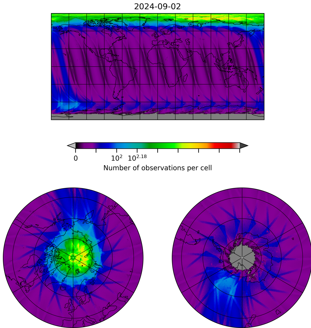
Figure 10: Map of the number of observations for 2024-09-01 to 2024-09-03
