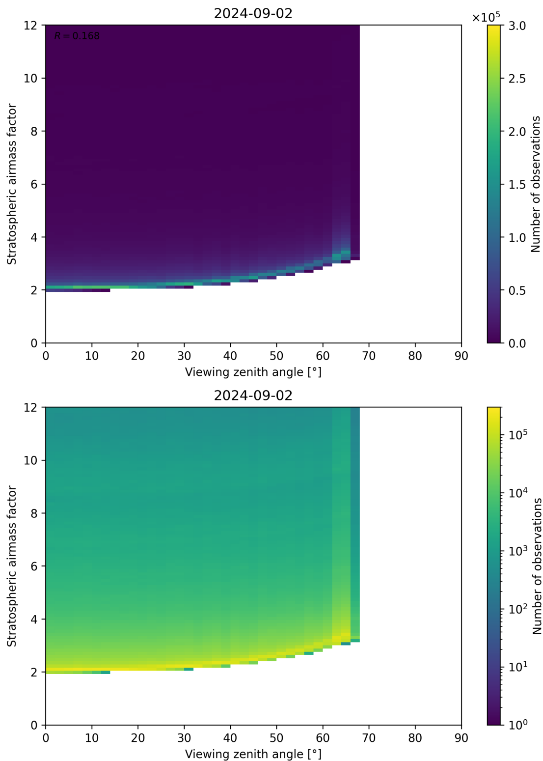
Figure 159: Scatter density plot of “Viewing zenith angle” against “Stratospheric airmass factor” for 2024-09-01 to 2024-09-03.
