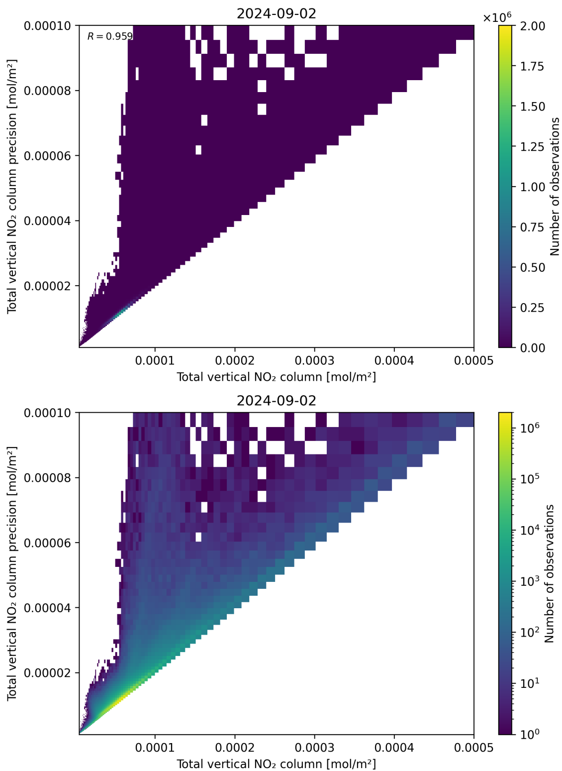
Figure 114: Scatter density plot of “Total vertical NO 2 column” against “Total vertical NO 2 column precision” for 2024-09-01 to 2024-09-03.
