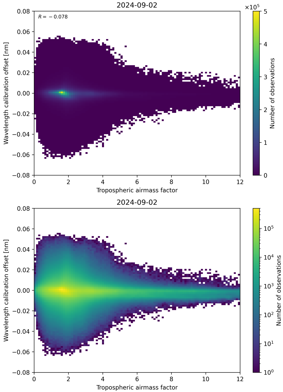
Figure 80: Scatter density plot of “Tropospheric airmass factor” against “Wavelength calibration offset” for 2024-09-01 to 2024-09-03.
