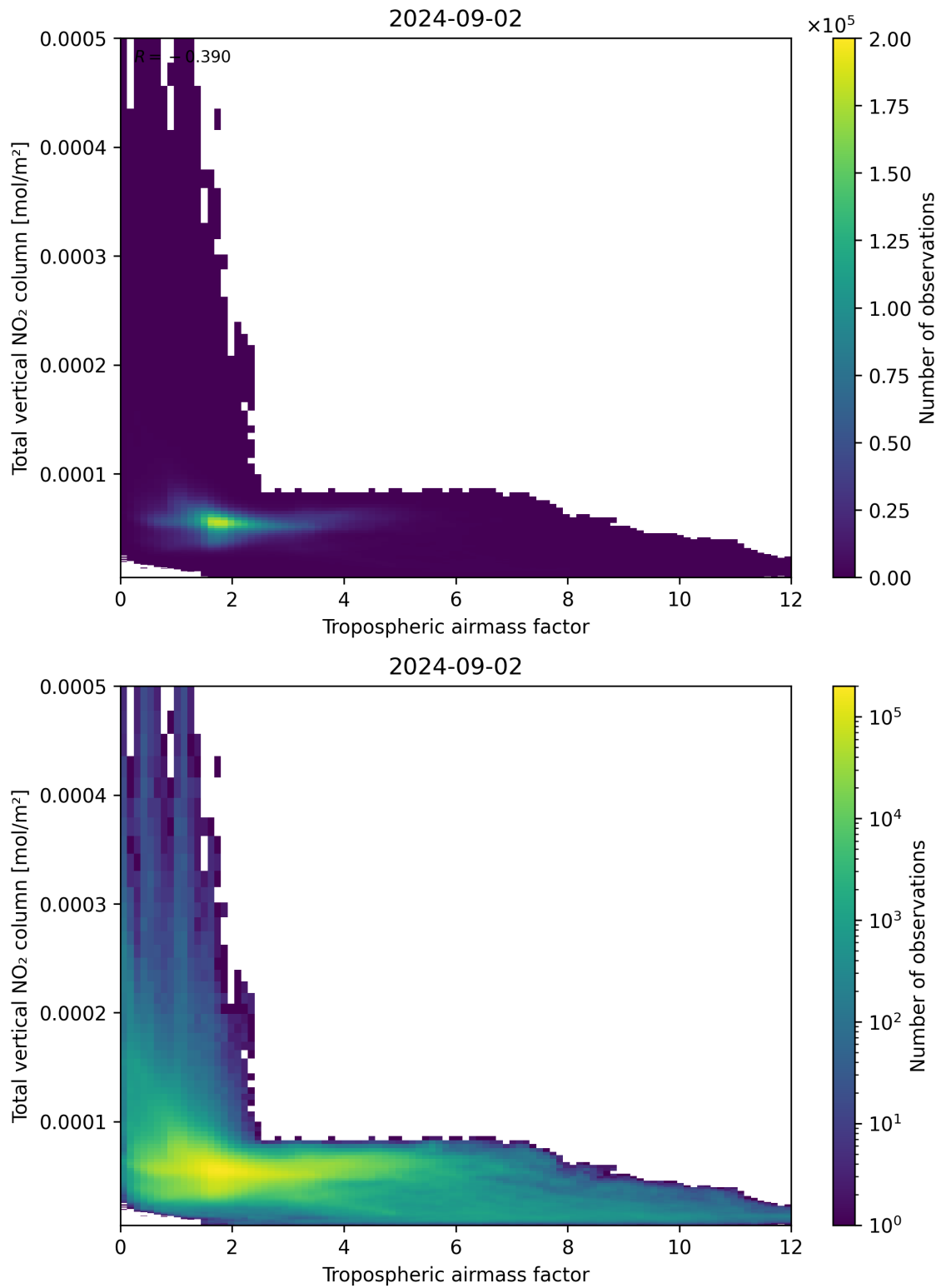
Figure 77: Scatter density plot of “Tropospheric airmass factor” against “Total vertical NO 2 column” for 2024-09-01 to 2024-09-03.
