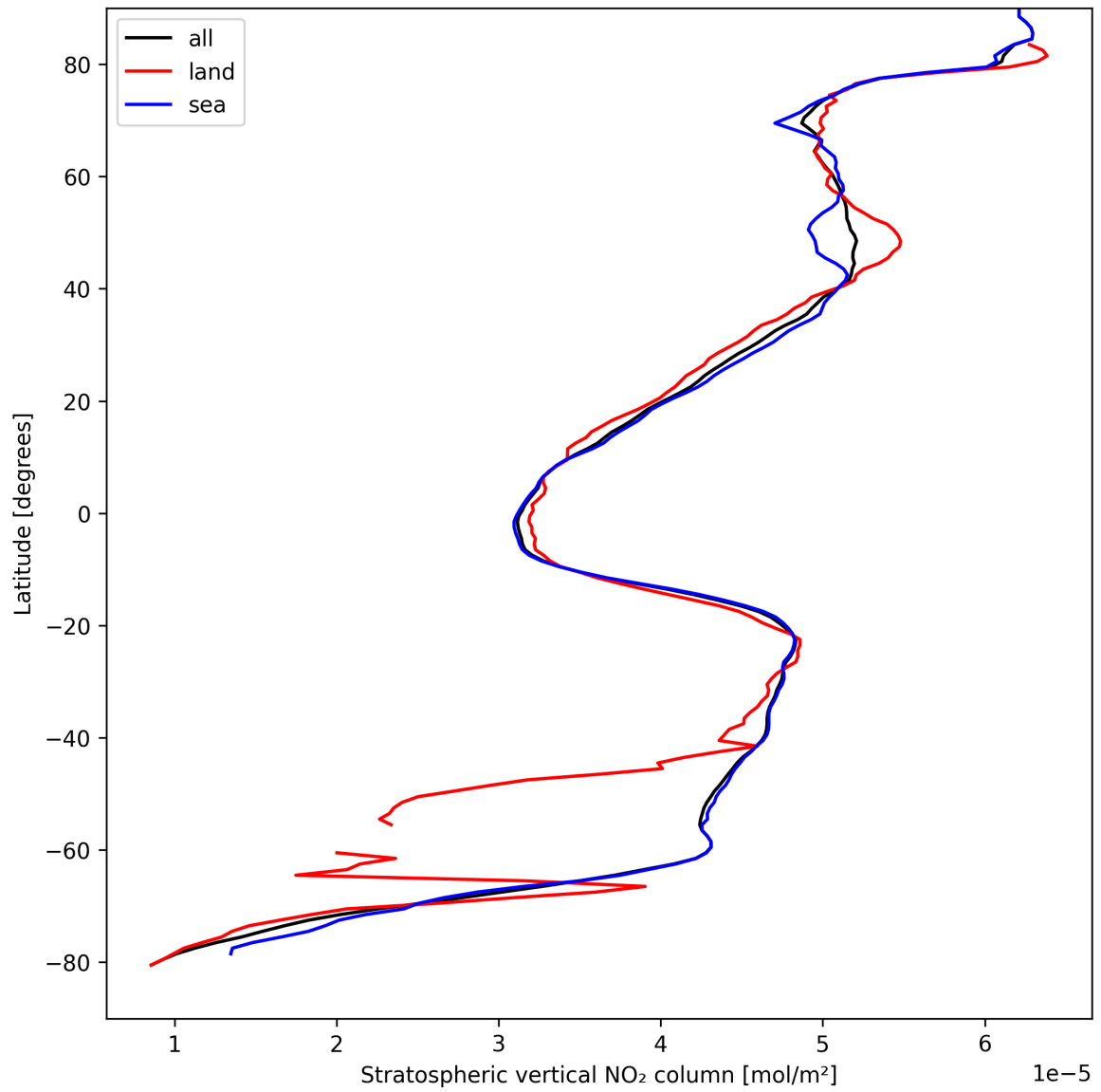
Figure 19: Zonal average of “Stratospheric vertical NO 2 column” for 2024-09-01 to 2024-09-03.
