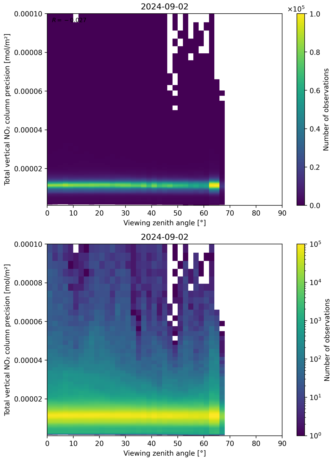
Figure 168: Scatter density plot of “Viewing zenith angle” against “Total vertical NO 2 column precision” for 2024-09-01 to 2024-09-03.
