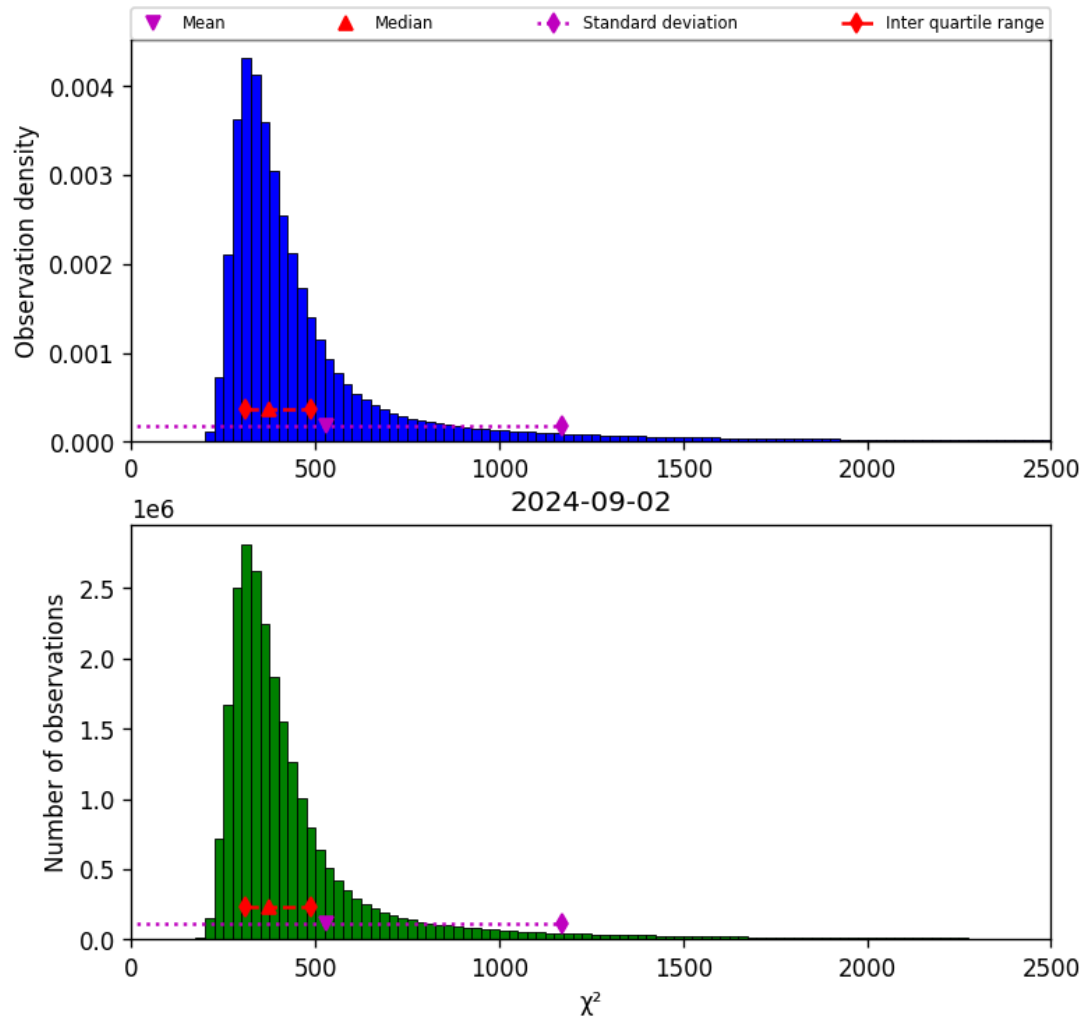
Figure 42: Histogram of “ \chi^2 ” for 2024-09-01 to 2024-09-03
