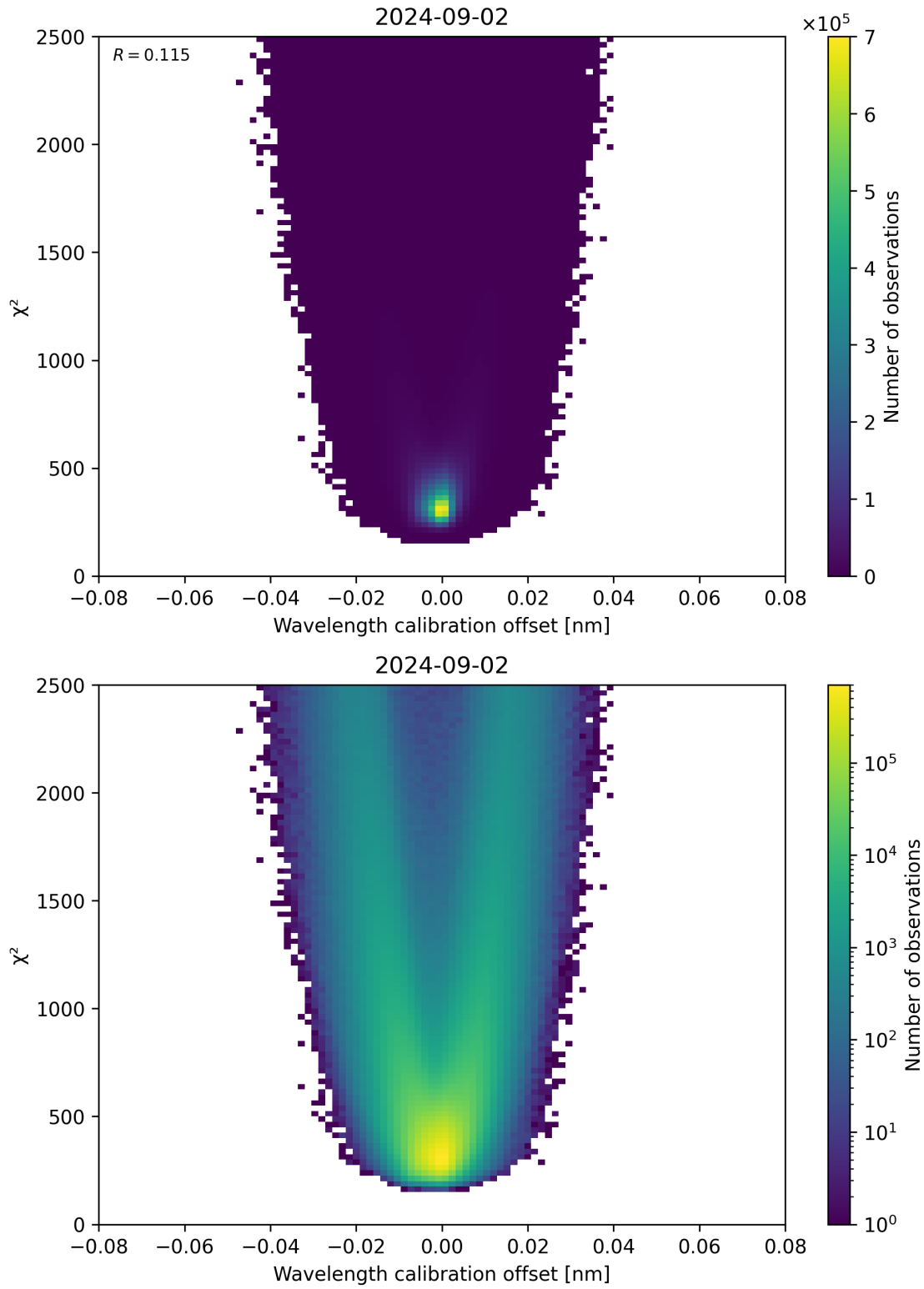
Figure 175: Scatter density plot of “Wavelength calibration offset” against “ \chi^2 ” for 2024-09-01 to 2024-09-03.
