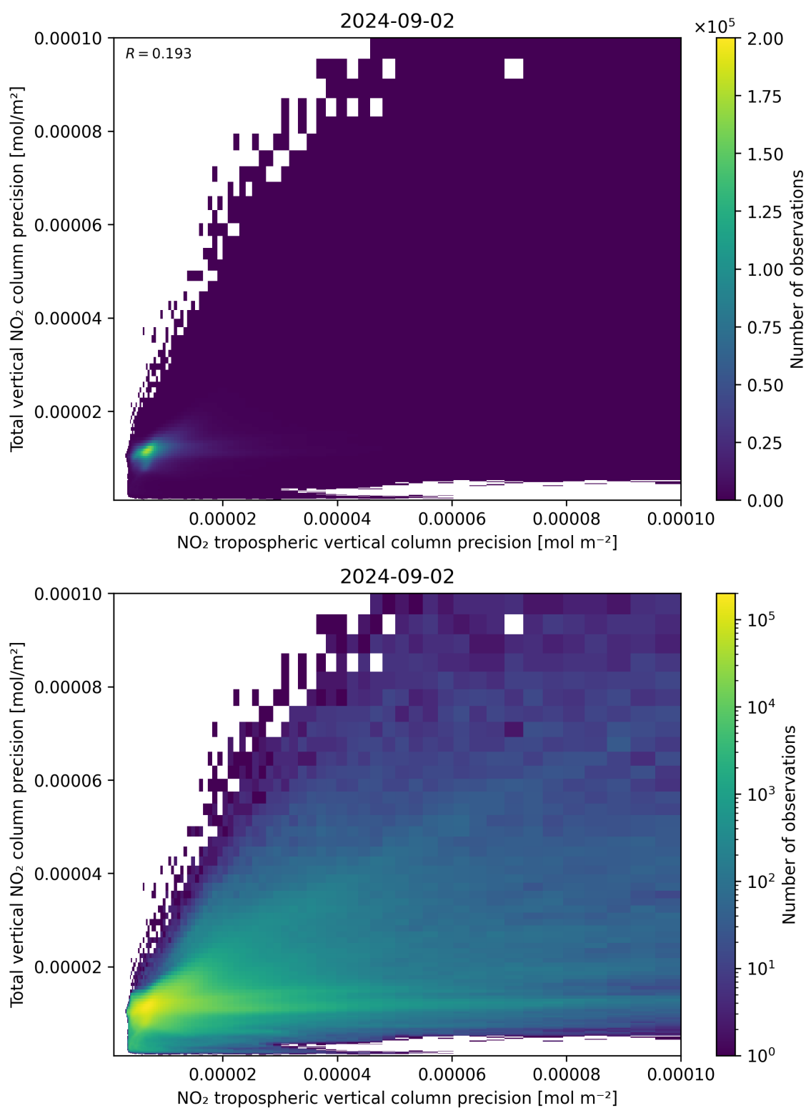
Figure 139: Scatter density plot of “NO 2 tropospheric vertical column precision” against “Total vertical NO 2 column precision” for 2024-09-01 to 2024-09-03.
