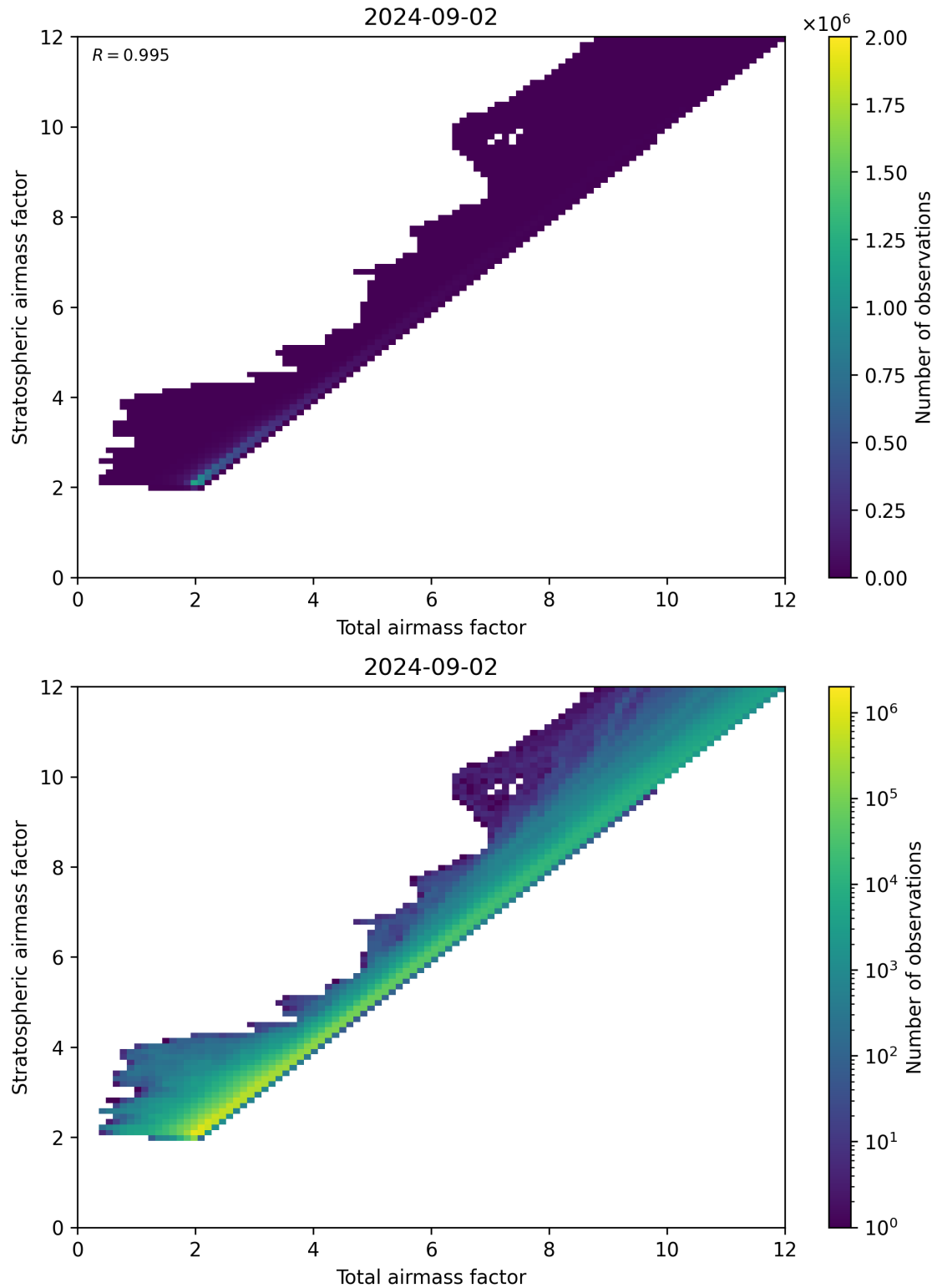
Figure 62: Scatter density plot of “Total airmass factor” against “Stratospheric airmass factor” for 2024-09-01 to 2024-09-03.
