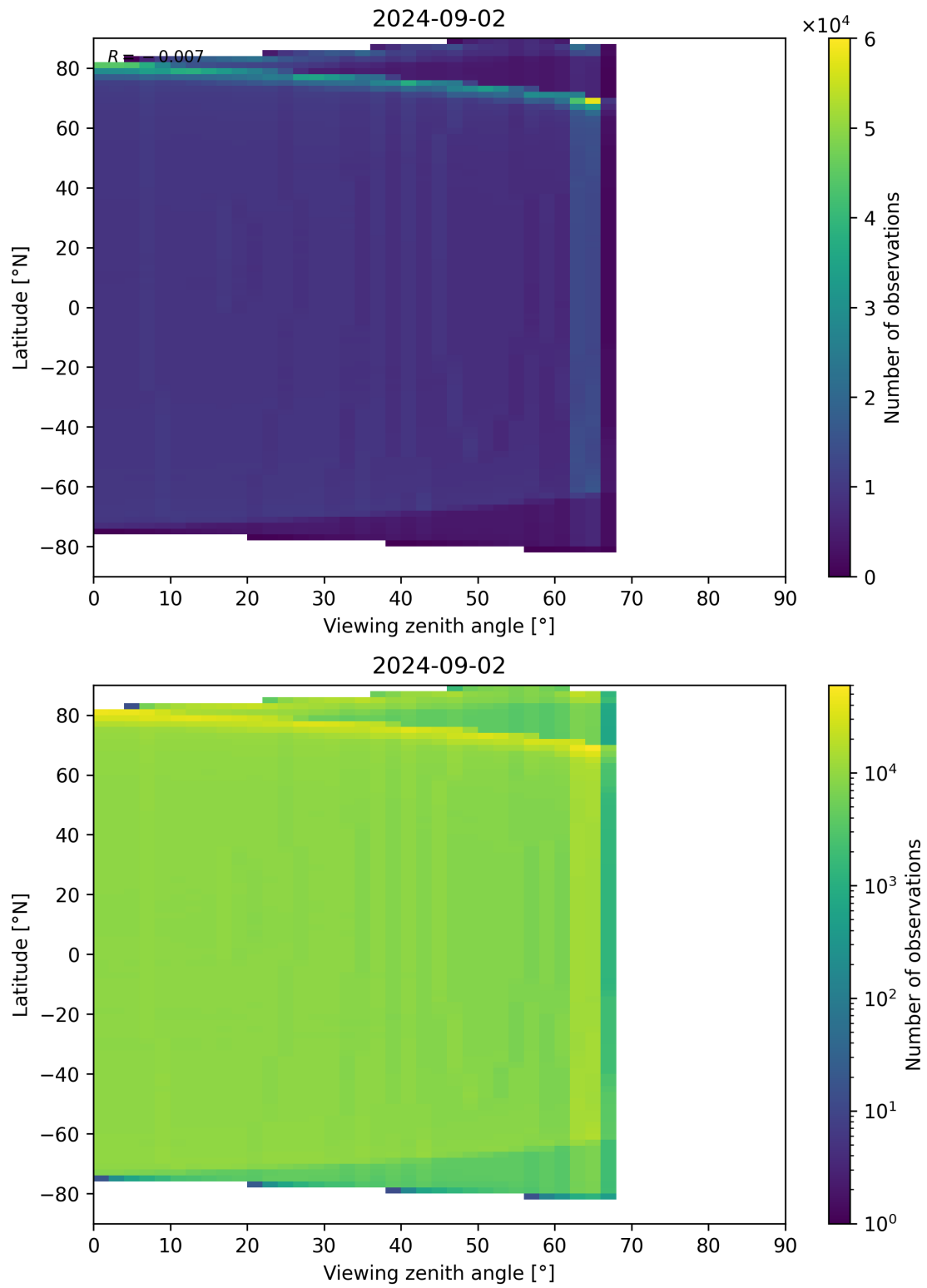
Figure 163: Scatter density plot of “Viewing zenith angle” against “Latitude” for 2024-09-01 to 2024-09-03.
