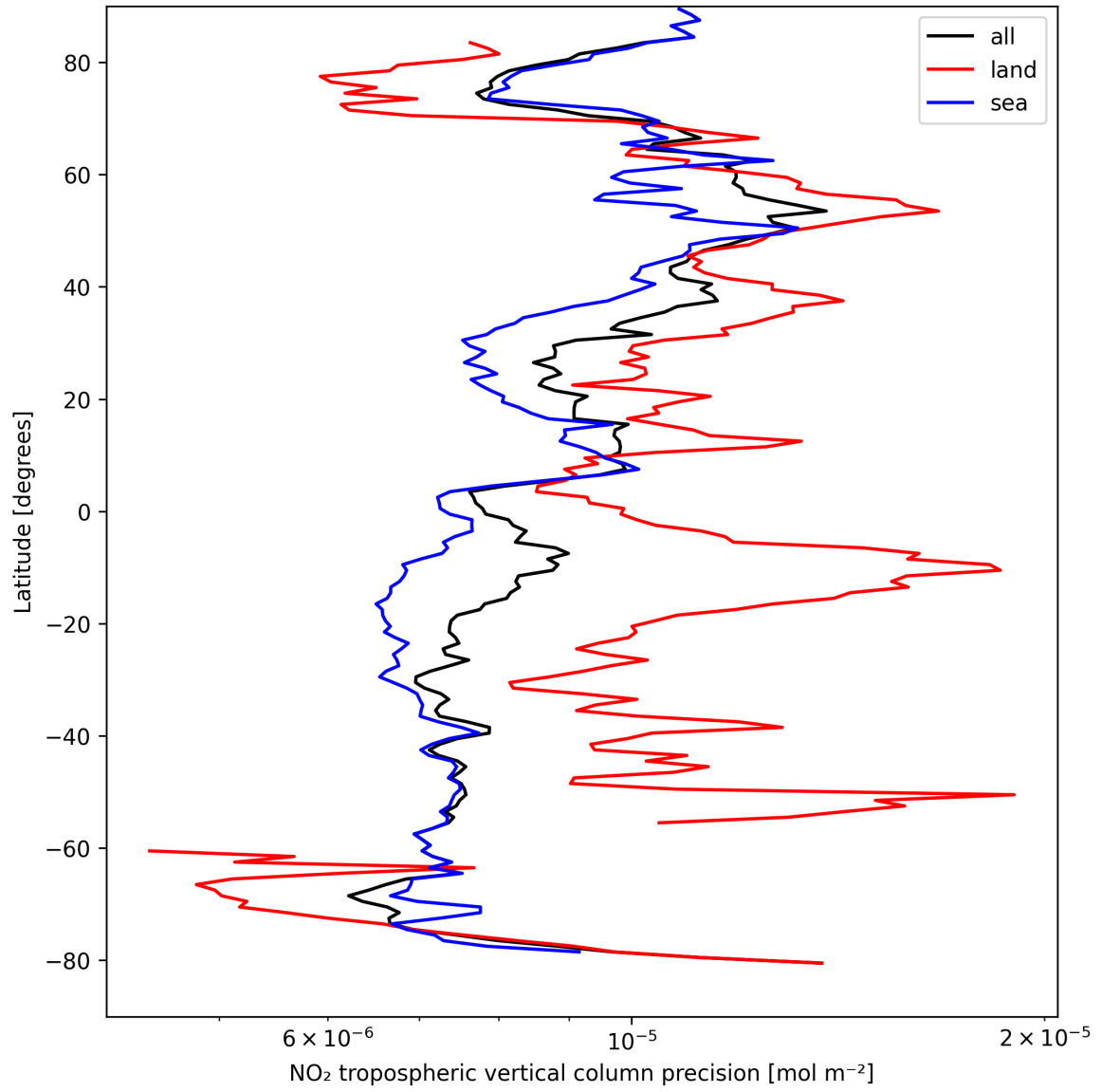
Figure 13: Zonal average of “NO 2 tropospheric vertical column precision” for 2024-09-01 to 2024-09-03.
