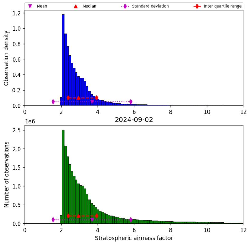
Figure 44: Histogram of “Stratospheric airmass factor” for 2024-09-01 to 2024-09-03
