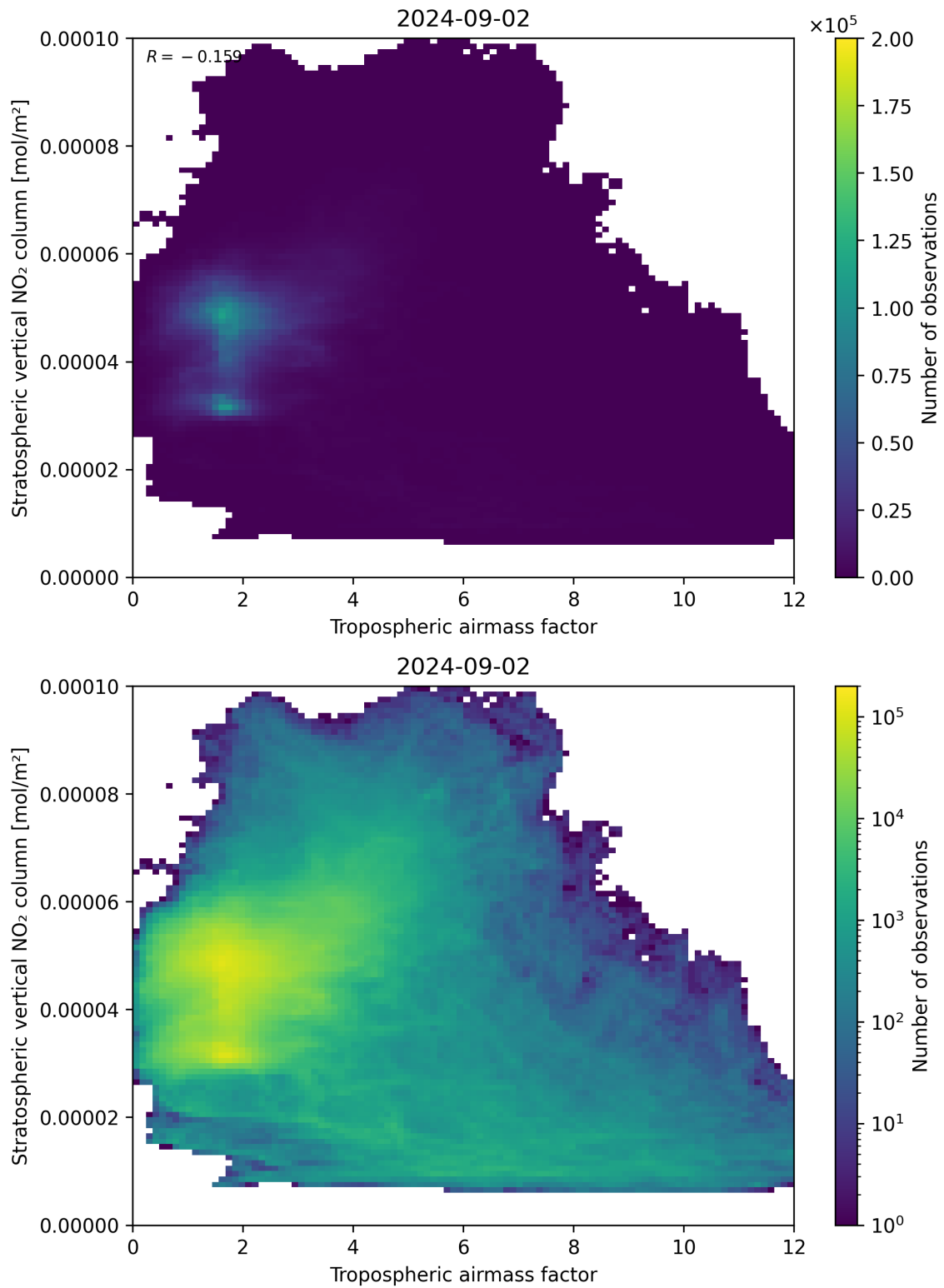
Figure 74: Scatter density plot of “Tropospheric air mass factor” against “Stratospheric vertical NO 2 column” for 2024-09-01 to 2024-09-03.
