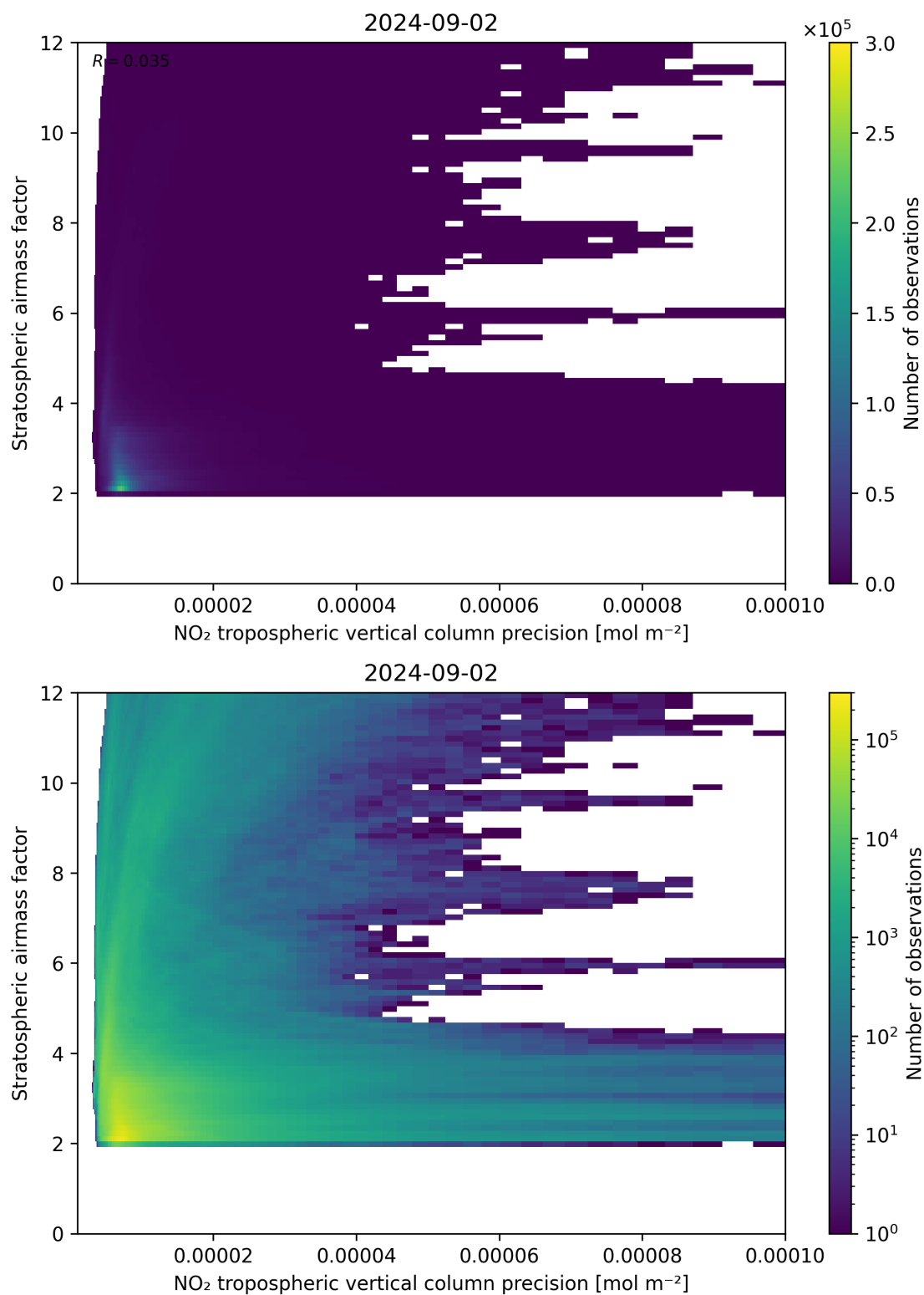
Figure 131: Scatter density plot of “NO 2 tropospheric vertical column precision” against “Stratospheric airmass factor” for 2024-09-01 to 2024-09-03.
