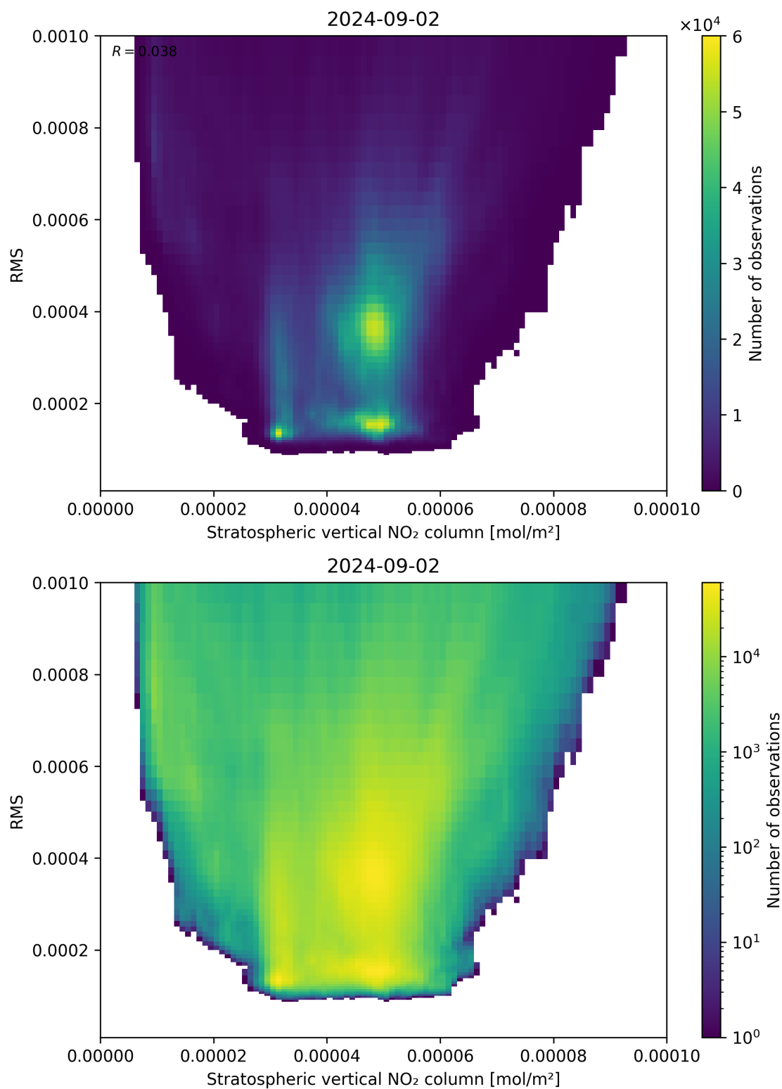
Figure 102: Scatter density plot of “Stratospheric vertical NO 2 column” against “RMS” for 2024-09-01 to 2024-09-03.
