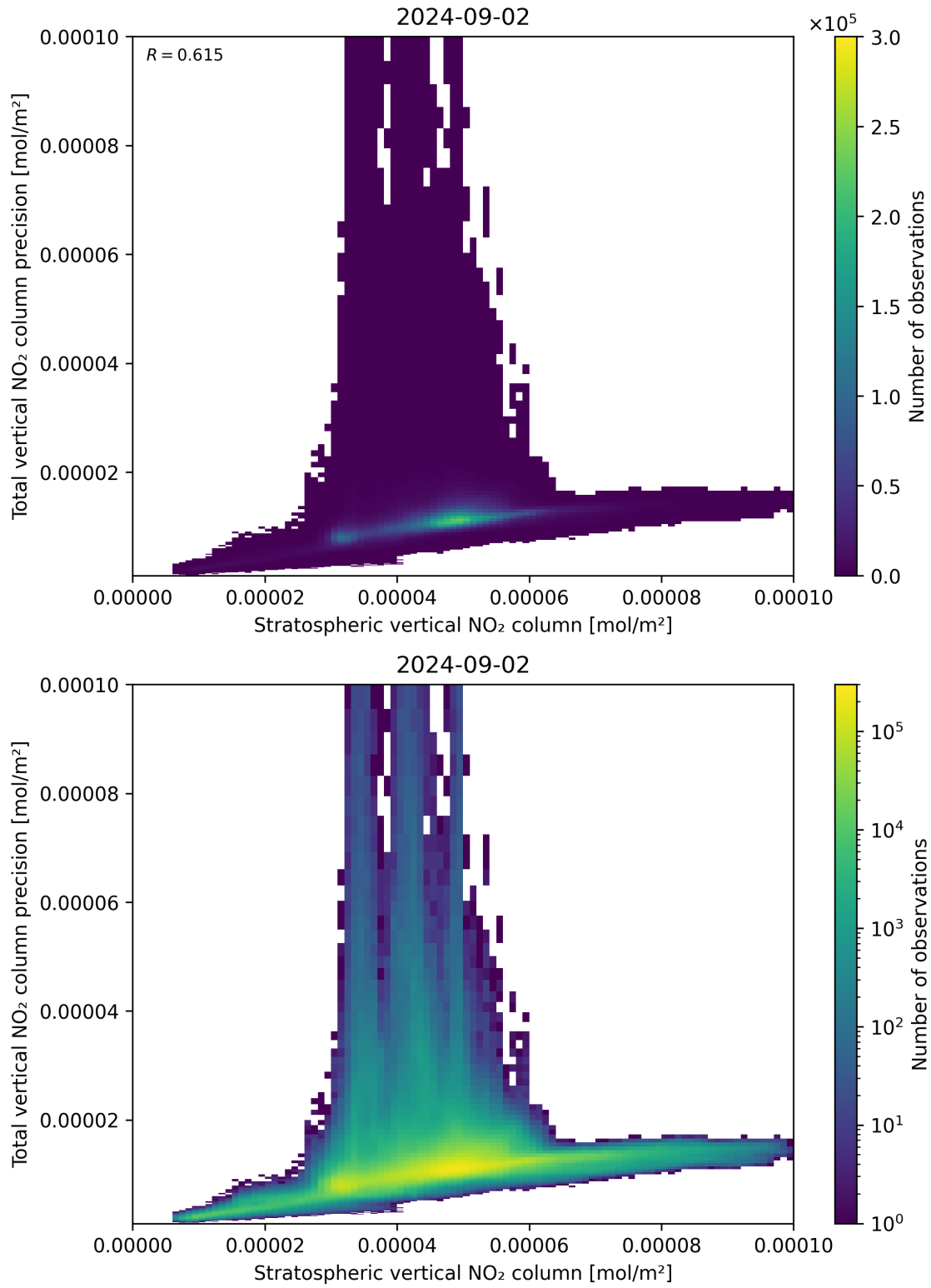
Figure 101: Scatter density plot of “Stratospheric vertical NO 2 column” against “Total vertical NO 2 column precision” for 2024-09-01 to 2024-09-03.
