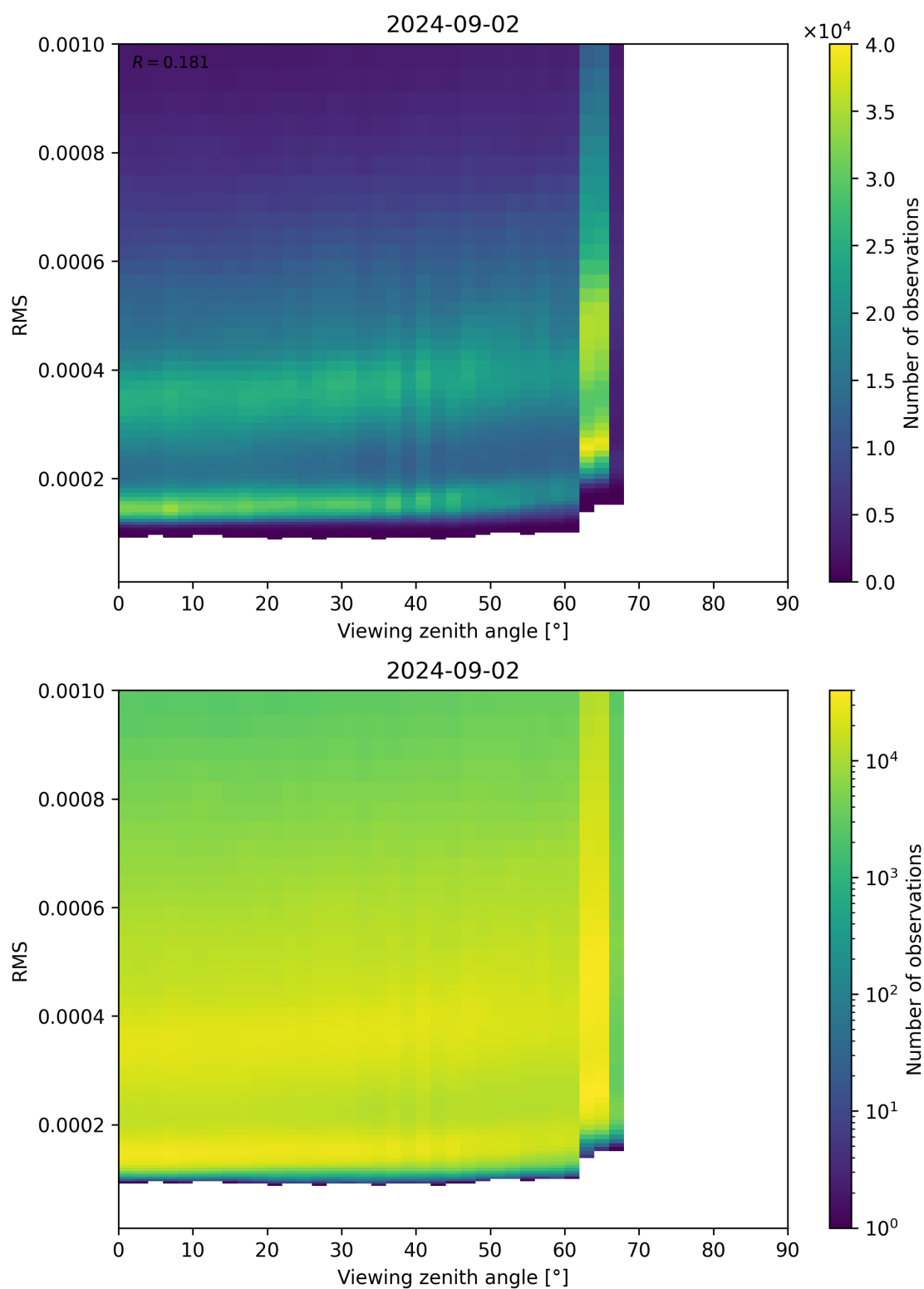
Figure 171: Scatter density plot of “Viewing zenith angle” against “RMS” for 2024-09-01 to 2024-09-03.
