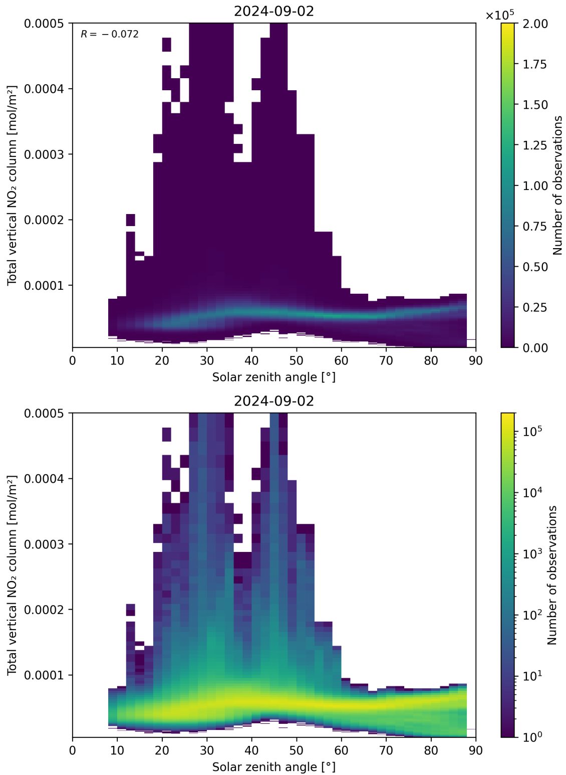
Figure 153: Scatter density plot of “Solar zenith angle” against “Total vertical NO 2 column” for 2024-09-01 to 2024-09-03.
