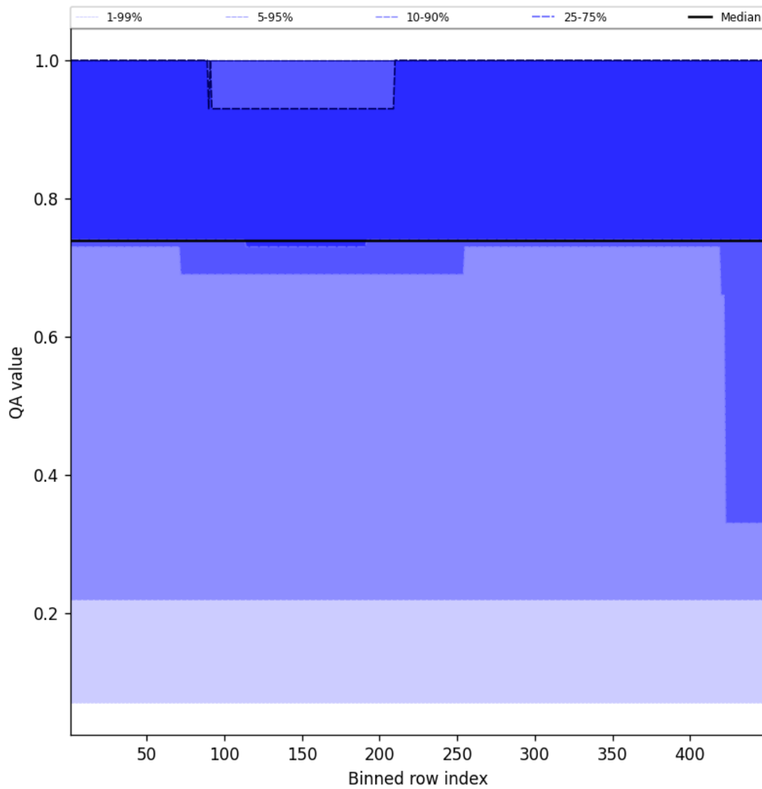
Figure 45: Along track statistics of “QA value” for 2024-09-01 to 2024-09-03
