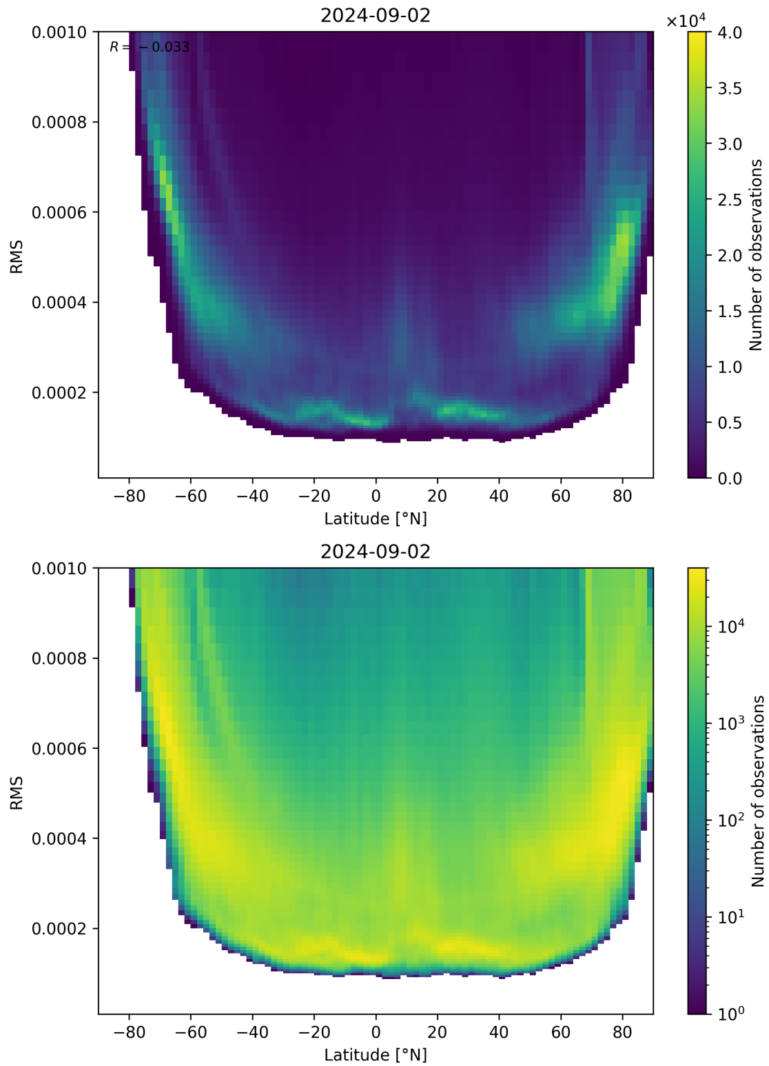
Figure 94: Scatter density plot of “Latitude” against “RMS” for 2024-09-01 to 2024-09-03.
