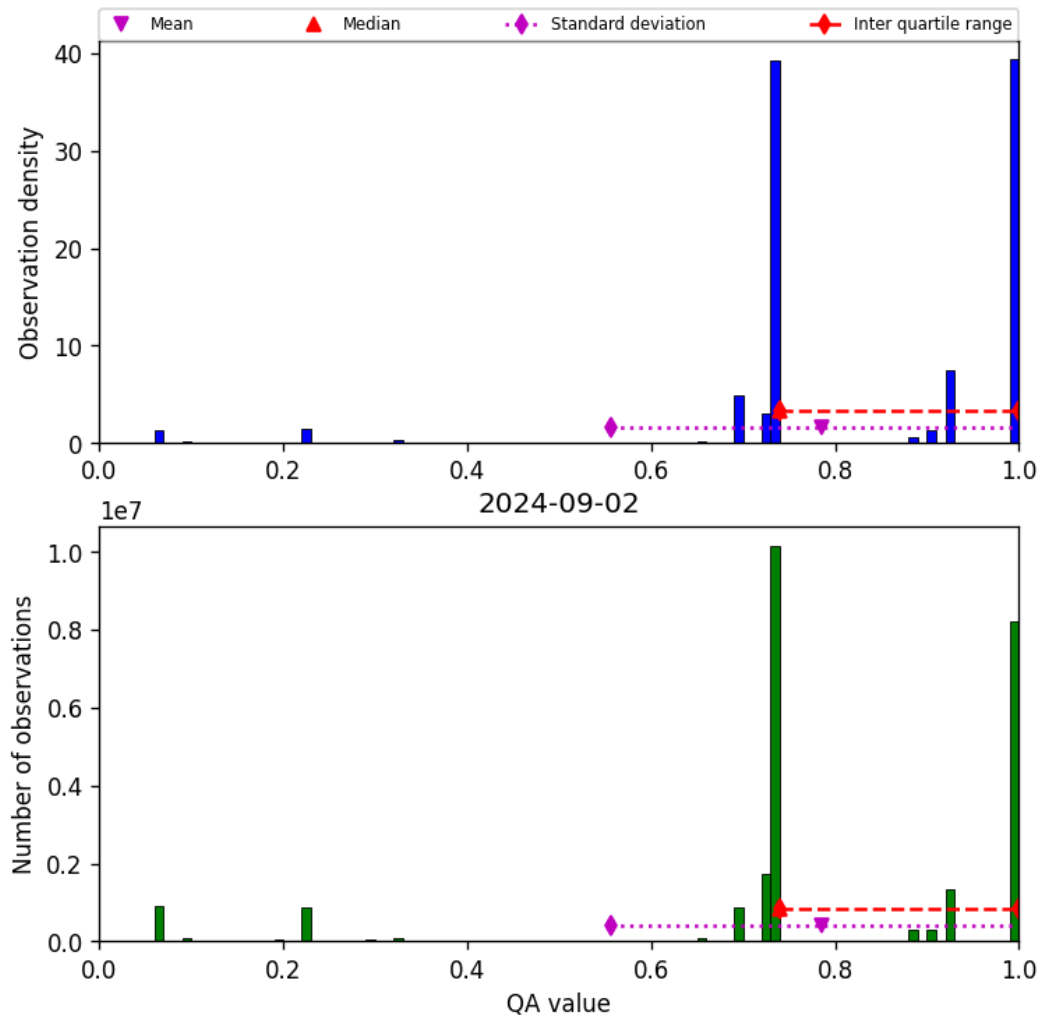
Figure 28: Histogram of “QA value” for 2024-09-01 to 2024-09-03
