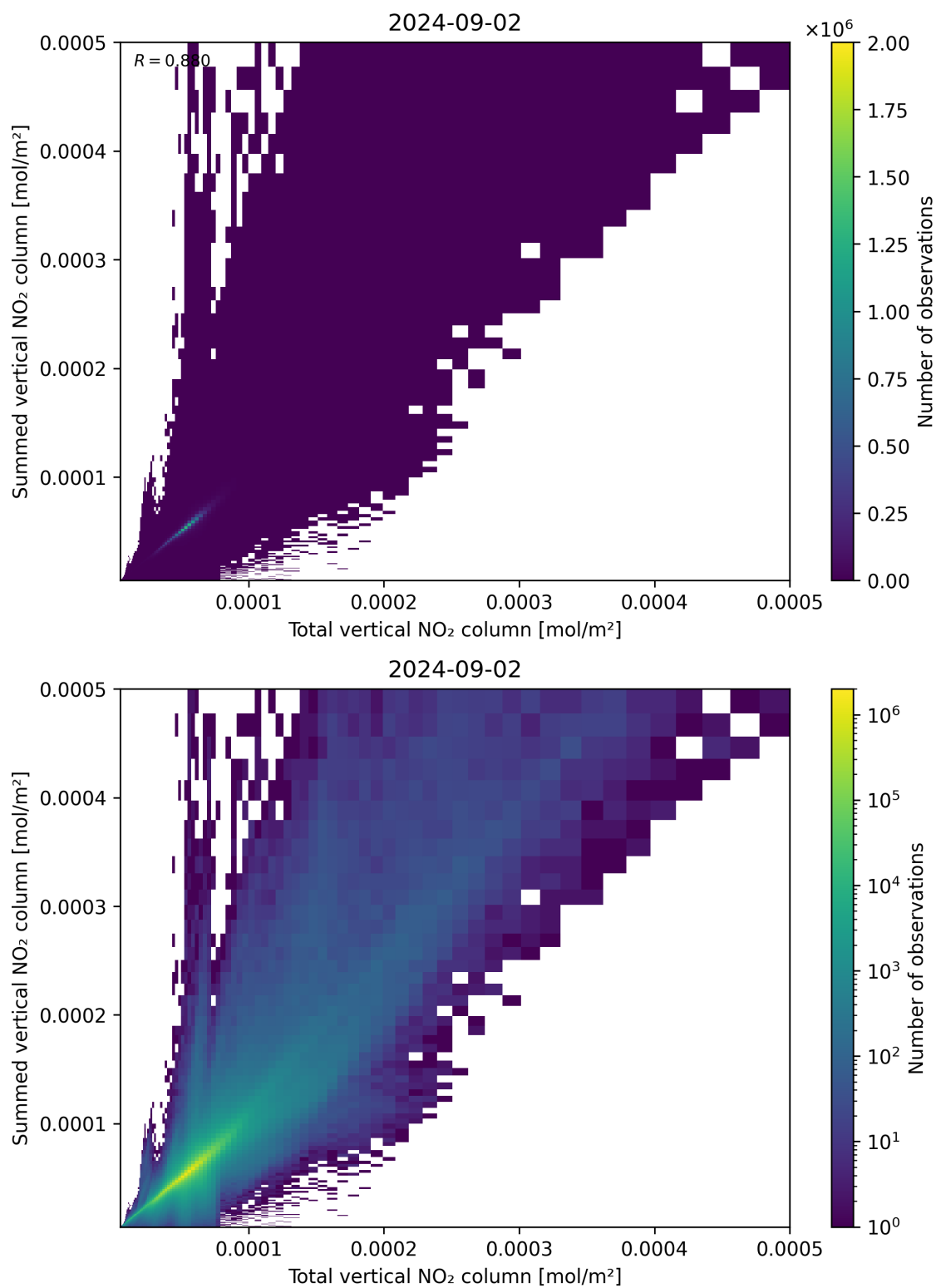
Figure 112: Scatter density plot of “Total vertical NO 2 column” against “Summed vertical NO 2 column” for 2024-09-01 to 2024-09-03.
