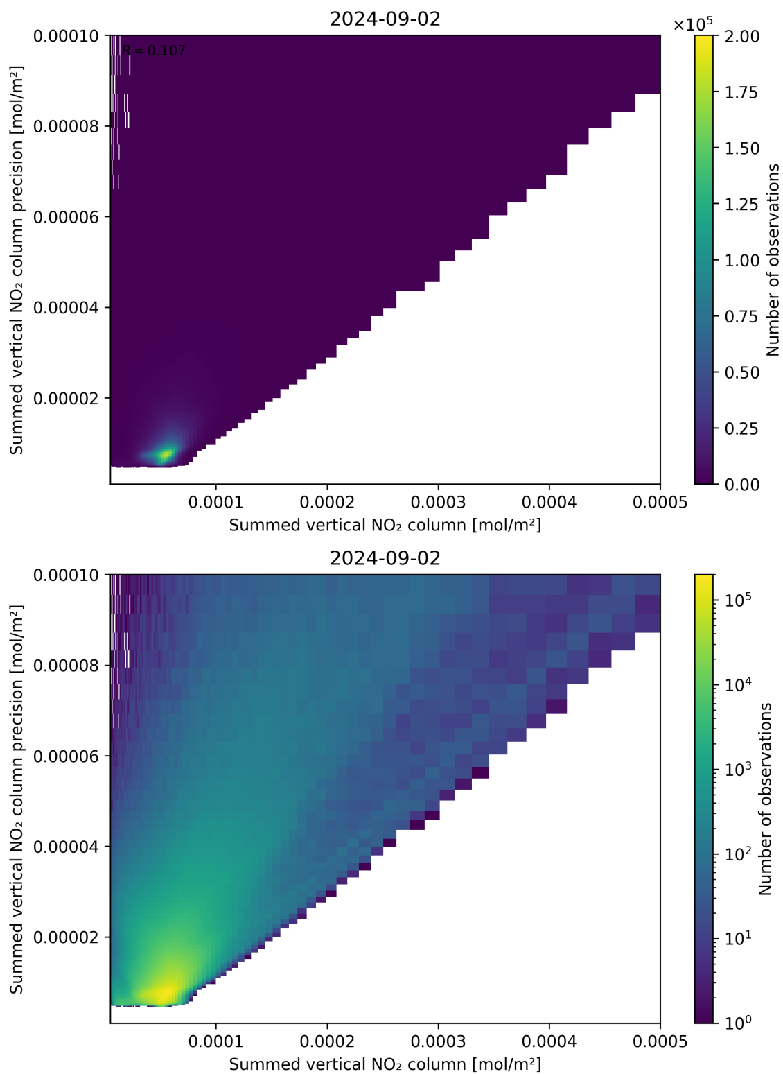
Figure 105: Scatter density plot of “Summed vertical NO 2 column” against “Summed vertical NO 2 column precision” for 2024-09-01 to 2024-09-03.
