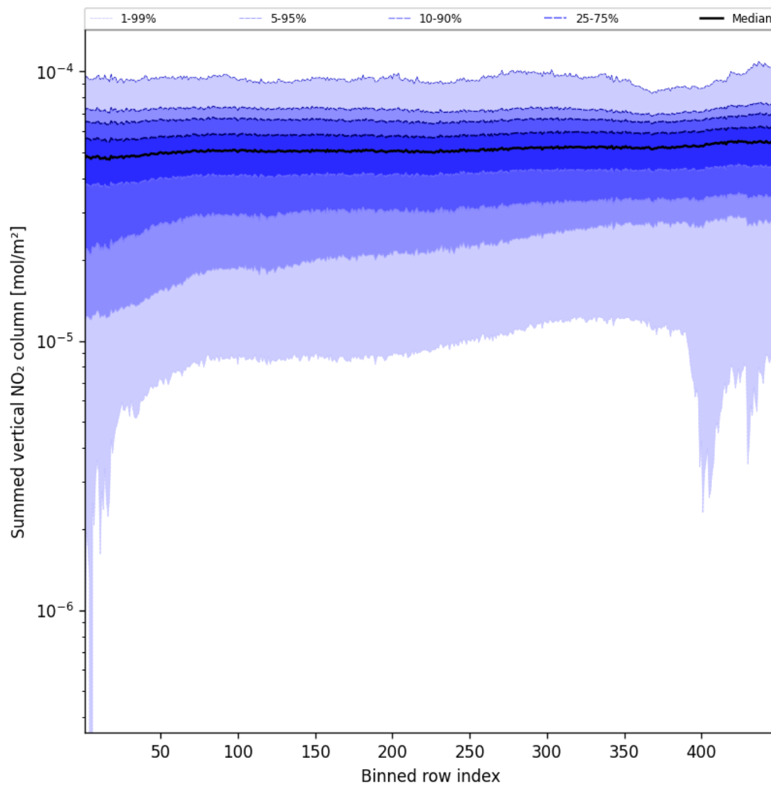
Figure 57: Along track statistics of “Summed vertical NO 2 column” for 2024-09-01 to 2024-09-03
