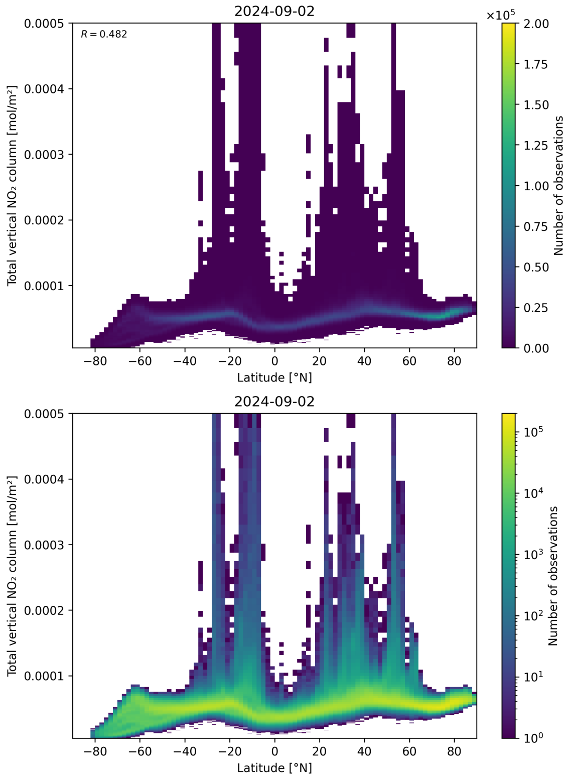
Figure 90: Scatter density plot of “Latitude” against “Total vertical NO 2 column” for 2024-09-01 to 2024-09-03.
