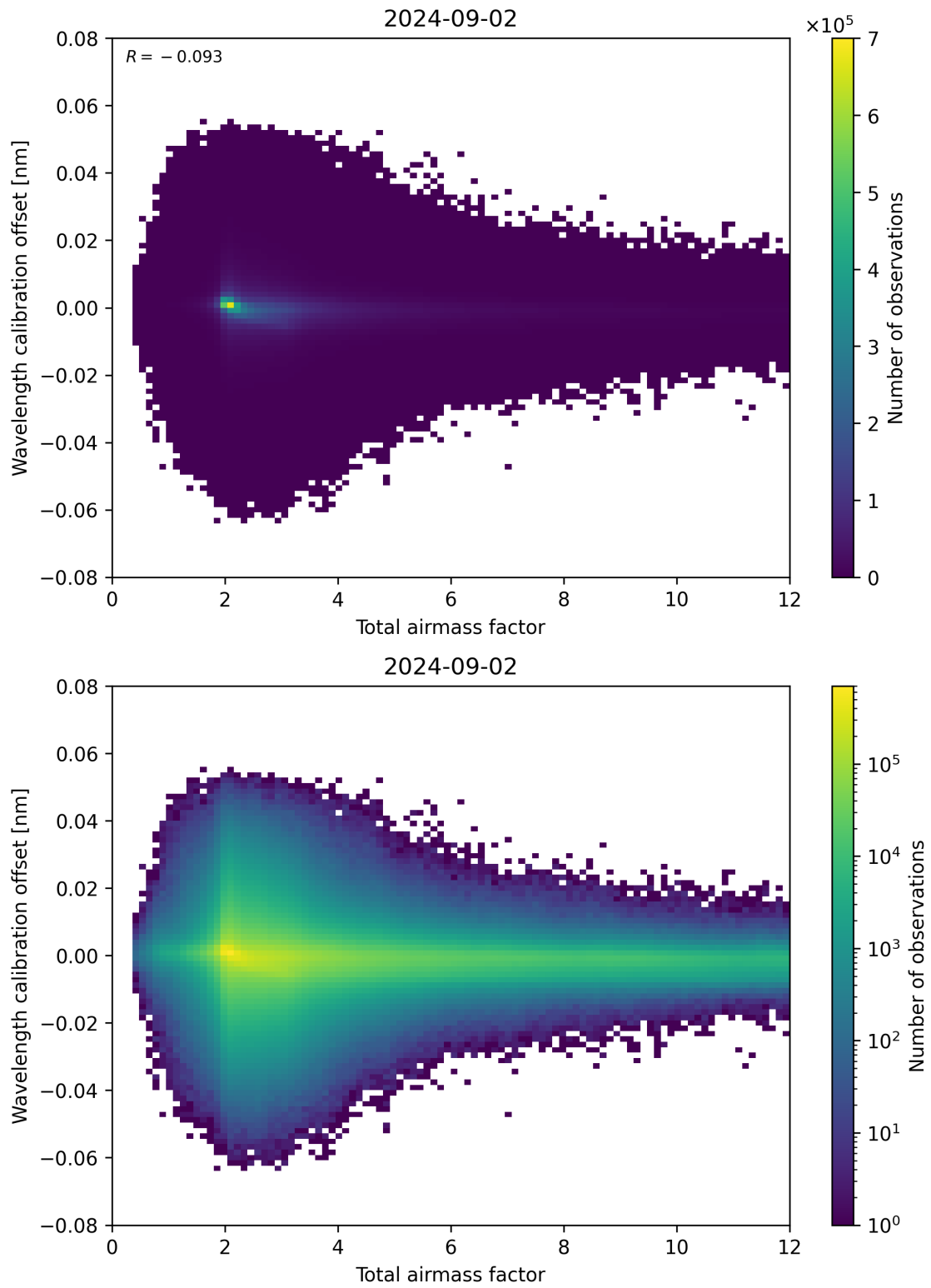
Figure 70: Scatter density plot of “Total airmass factor” against “Wavelength calibration offset” for 2024-09-01 to 2024-09-03.
