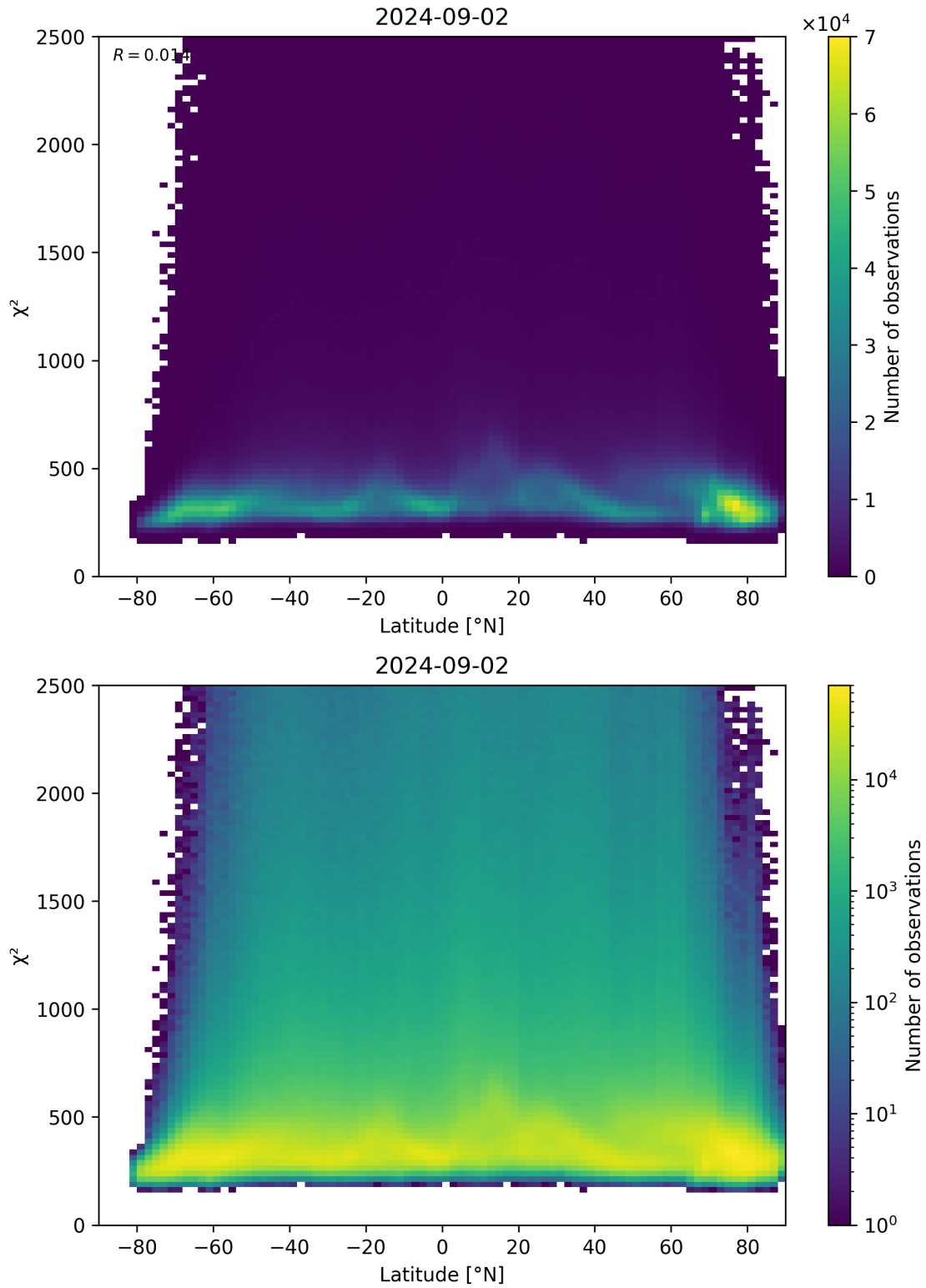
Figure 86: Scatter density plot of “Latitude” against “ \chi^2 ” for 2024-09-01 to 2024-09-03.
