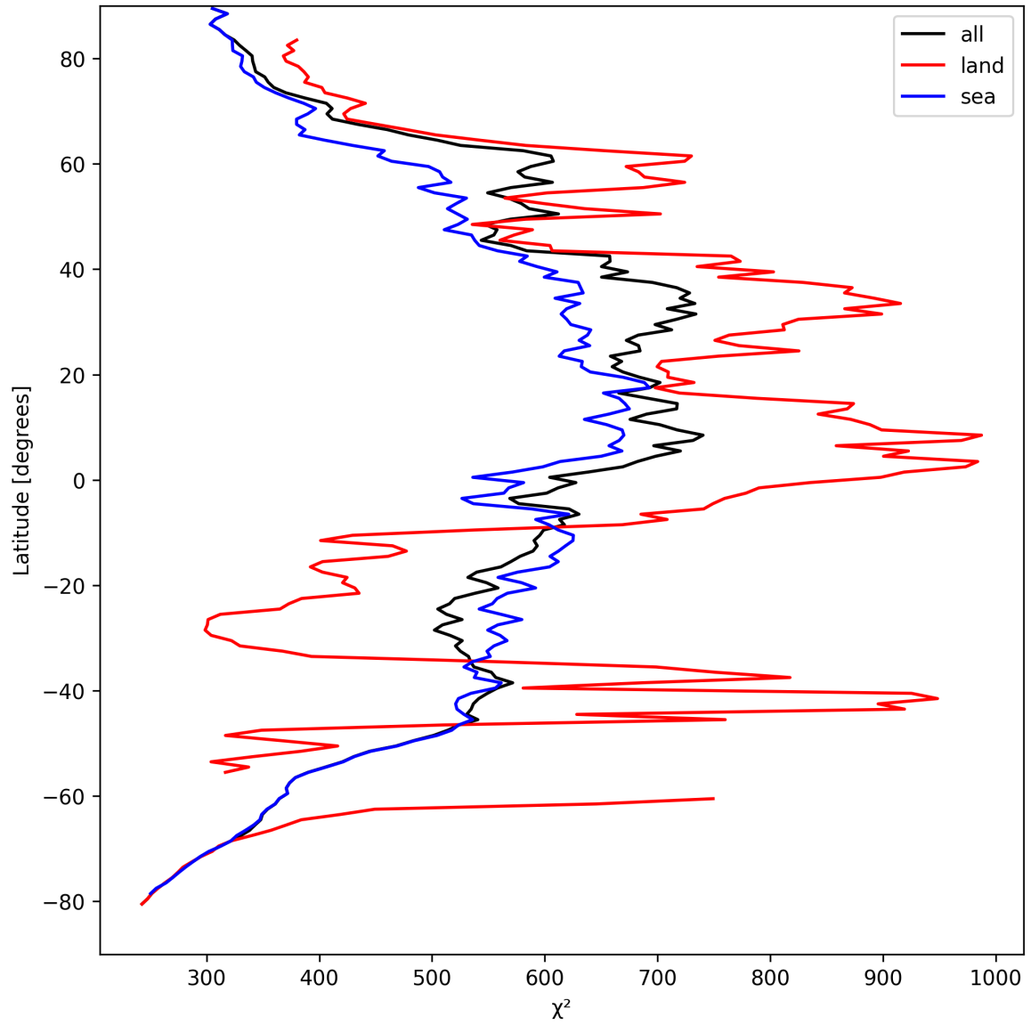
Figure 25: Zonal average of “ \chi^2 ” for 2024-09-01 to 2024-09-03.
