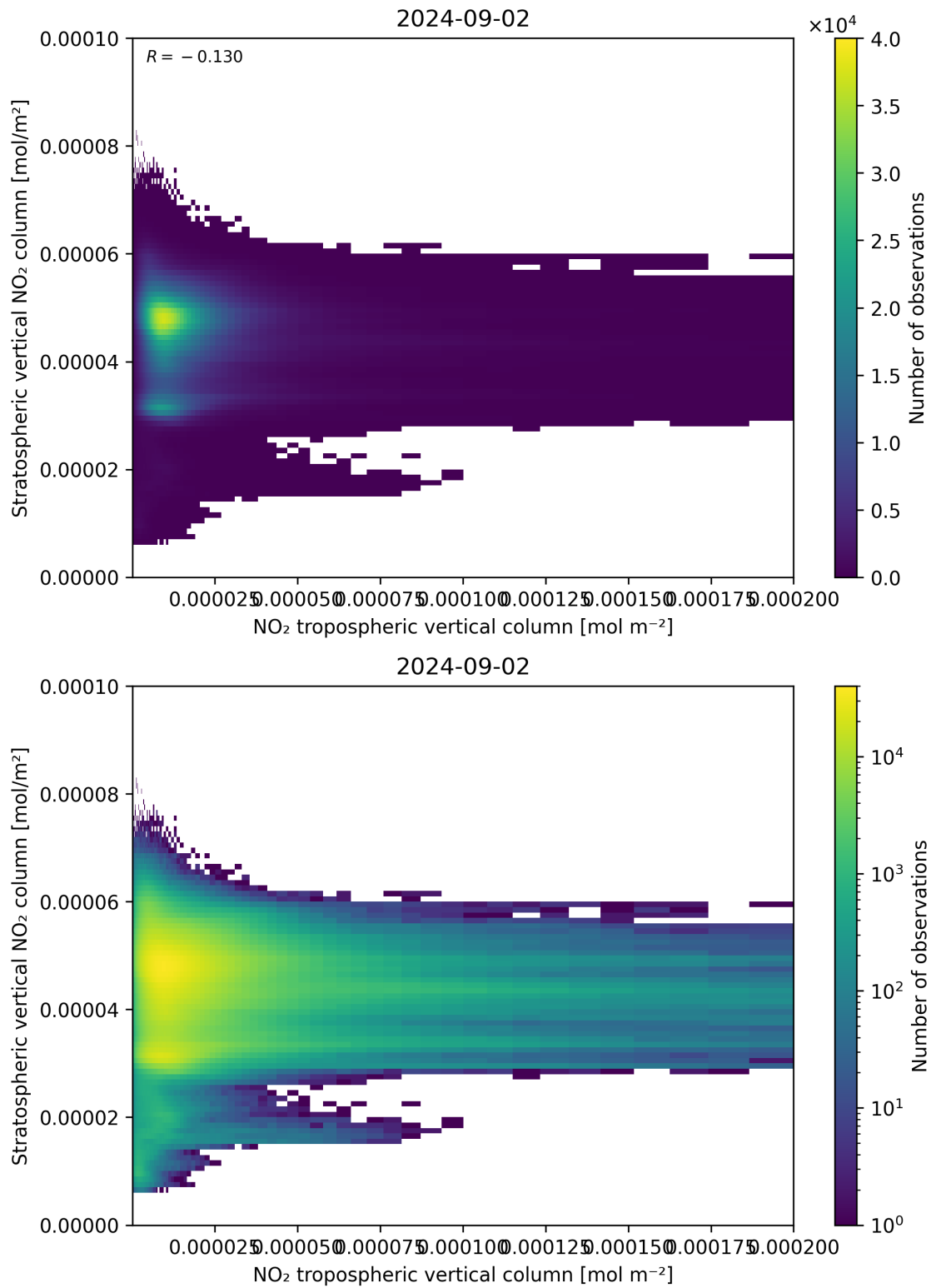
Figure 125: Scatter density plot of “NO 2 tropospheric vertical column” against “Stratospheric vertical NO 2 column” for 2024-09-01 to 2024-09-03.
