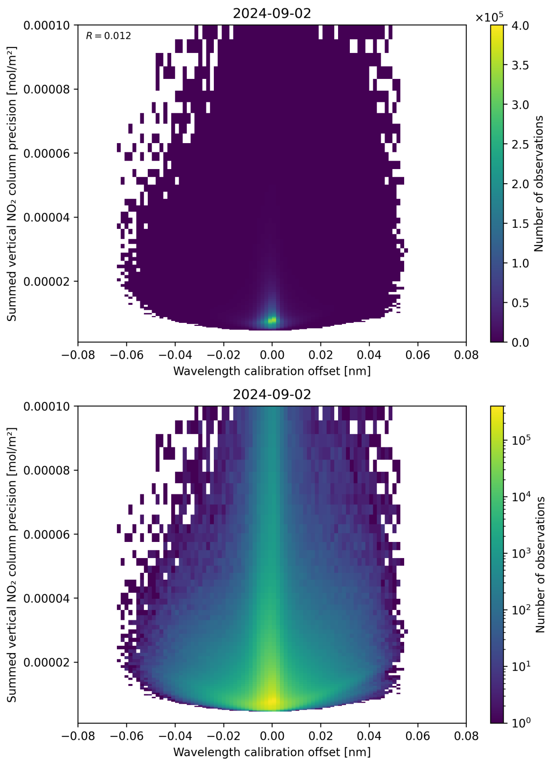
Figure 178: Scatter density plot of “Wavelength calibration offset” against “Summed vertical NO 2 column precision” for 2024-09-01 to 2024-09-03.
