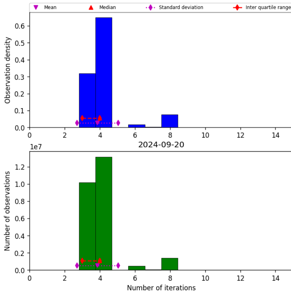
Figure 34: Histogram of “Number of iterations” for 2024-09-19 to 2024-09-21
