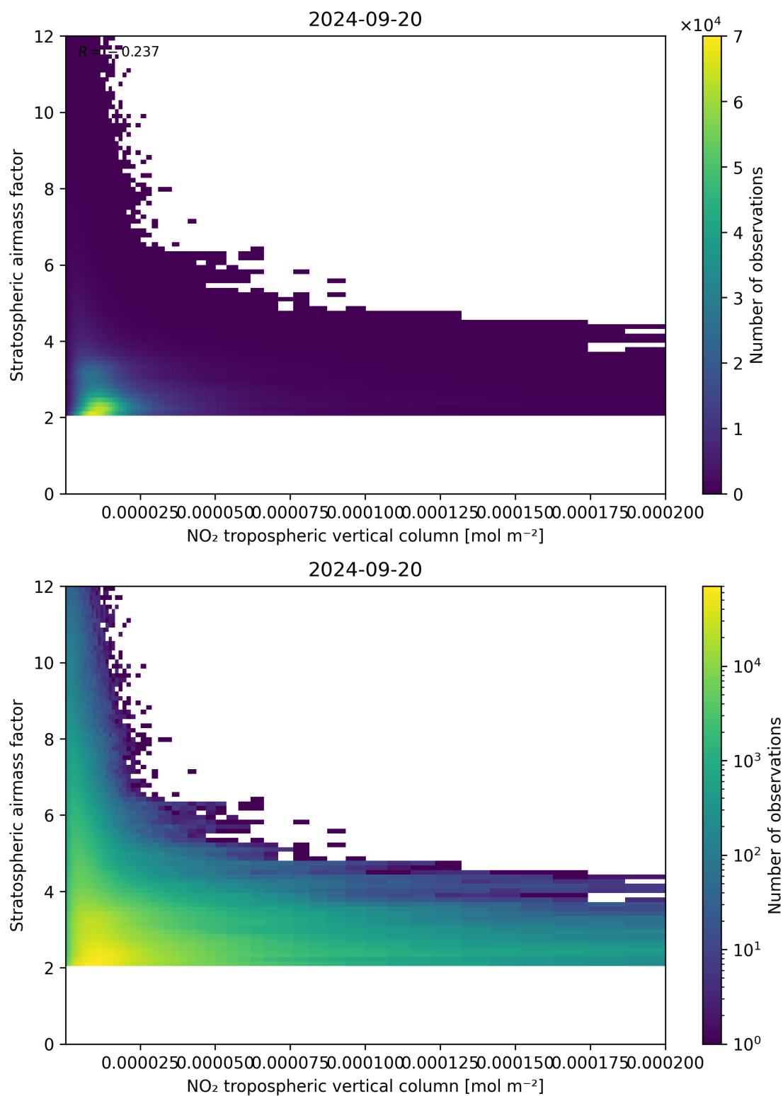
Figure 121: Scatter density plot of “NO 2 tropospheric vertical column” against “Stratospheric air mass factor” for 2024-09-19 to 2024-09-21.
