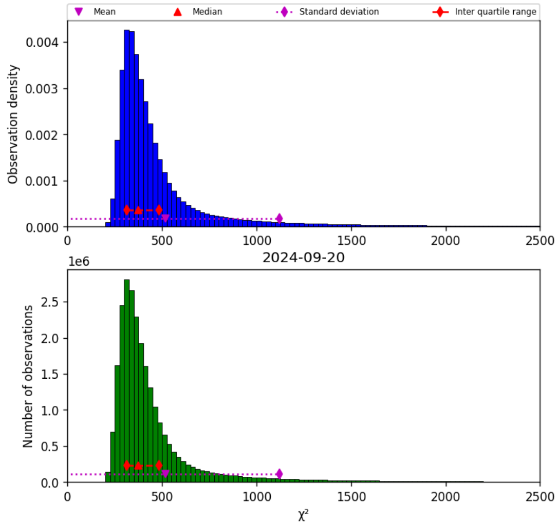
Figure 42: Histogram of “ \chi^2 ” for 2024-09-19 to 2024-09-21
