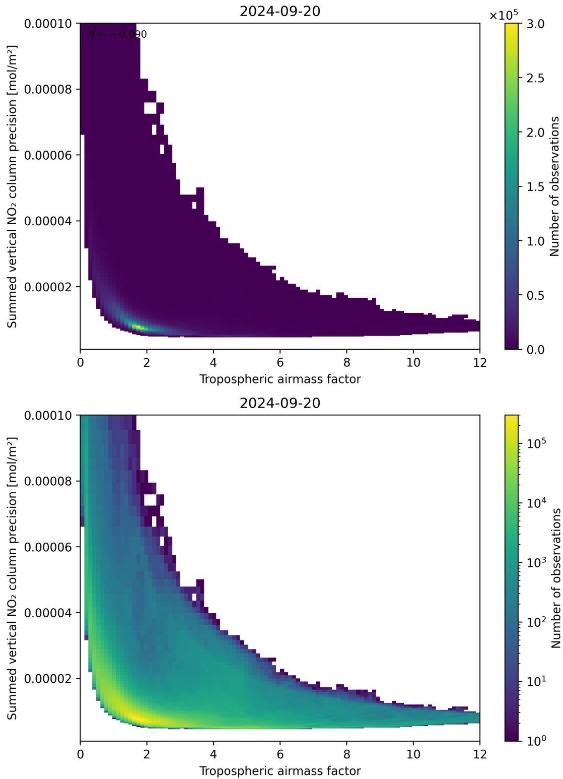
Figure 76: Scatter density plot of “Tropospheric air mass factor” against “Summed vertical NO 2 column precision” for 2024-09-19 to 2024-09-21.
