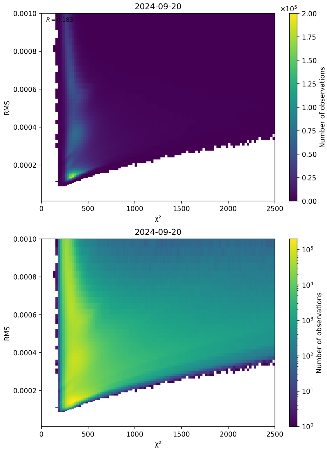
Figure 82: Scatter density plot of “ \chi^2 ” against “RMS” for 2024-09-19 to 2024-09-21.
