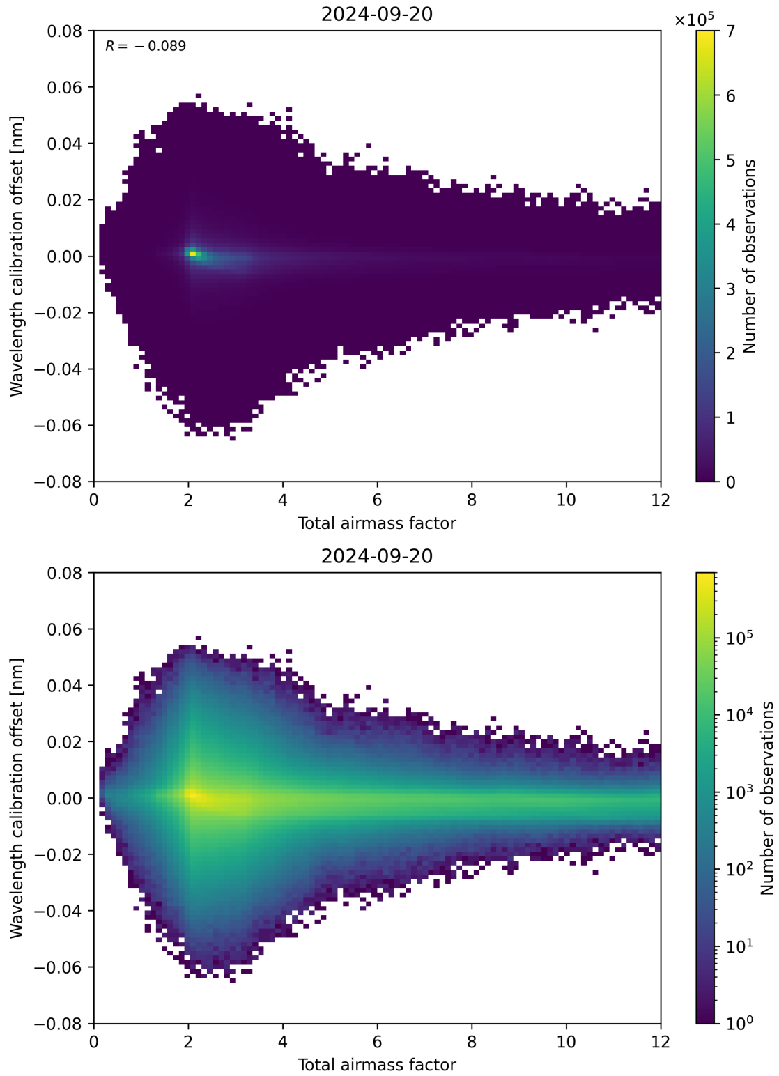
Figure 70: Scatter density plot of “Total airmass factor” against “Wavelength calibration offset” for 2024-09-19 to 2024-09-21.
