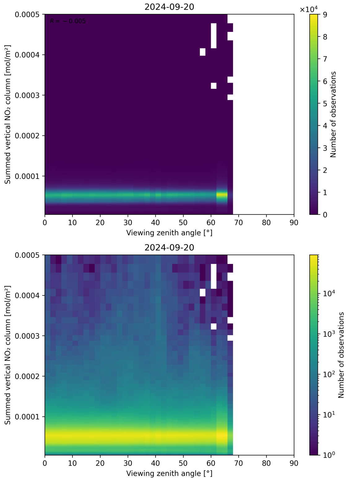
Figure 165: Scatter density plot of “Viewing zenith angle” against “Summed vertical NO 2 column” for 2024-09-19 to 2024-09-21.
