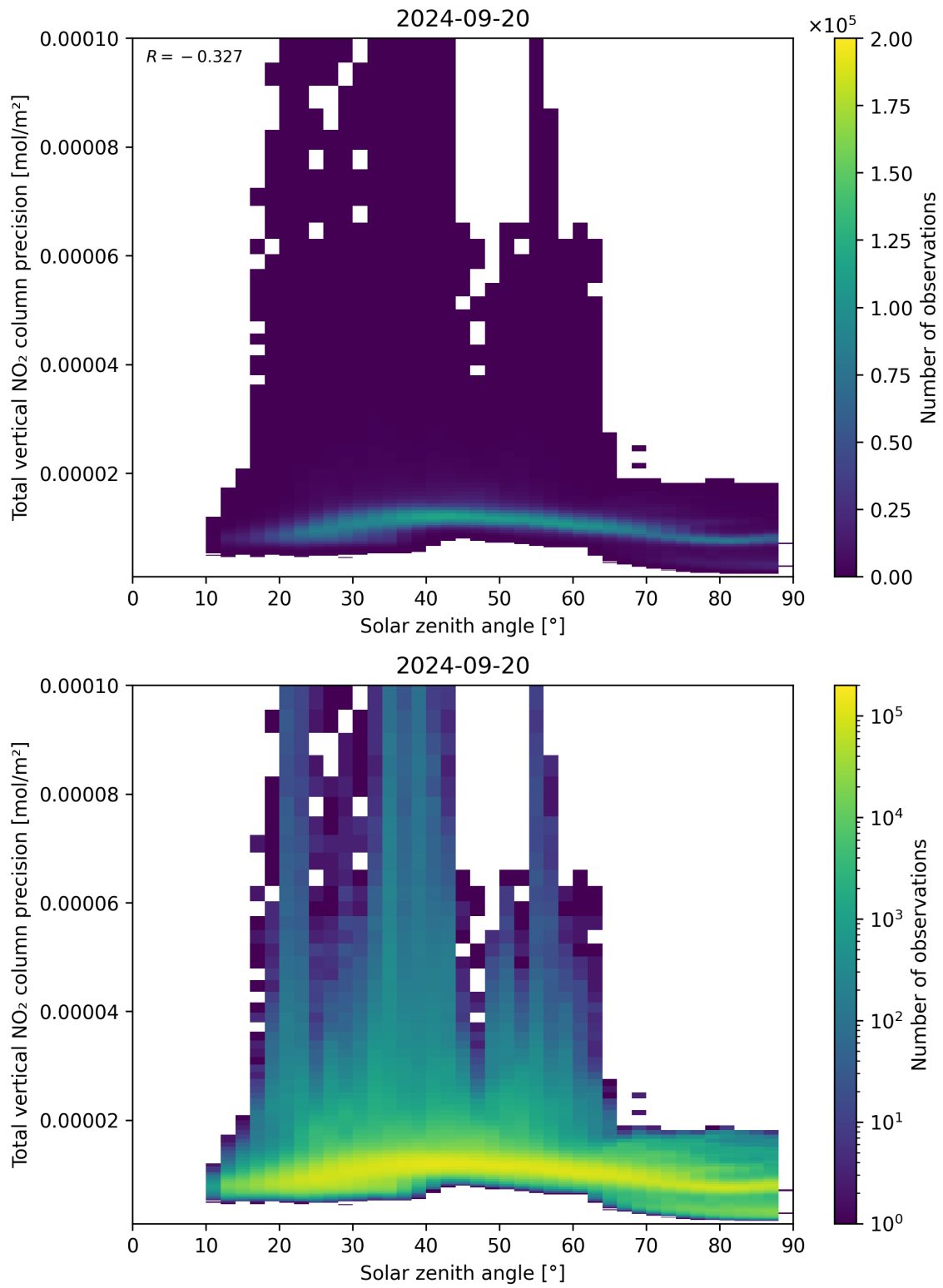
Figure 154: Scatter density plot of “Solar zenith angle” against “Total vertical NO 2 column precision” for 2024-09-19 to 2024-09-21.
