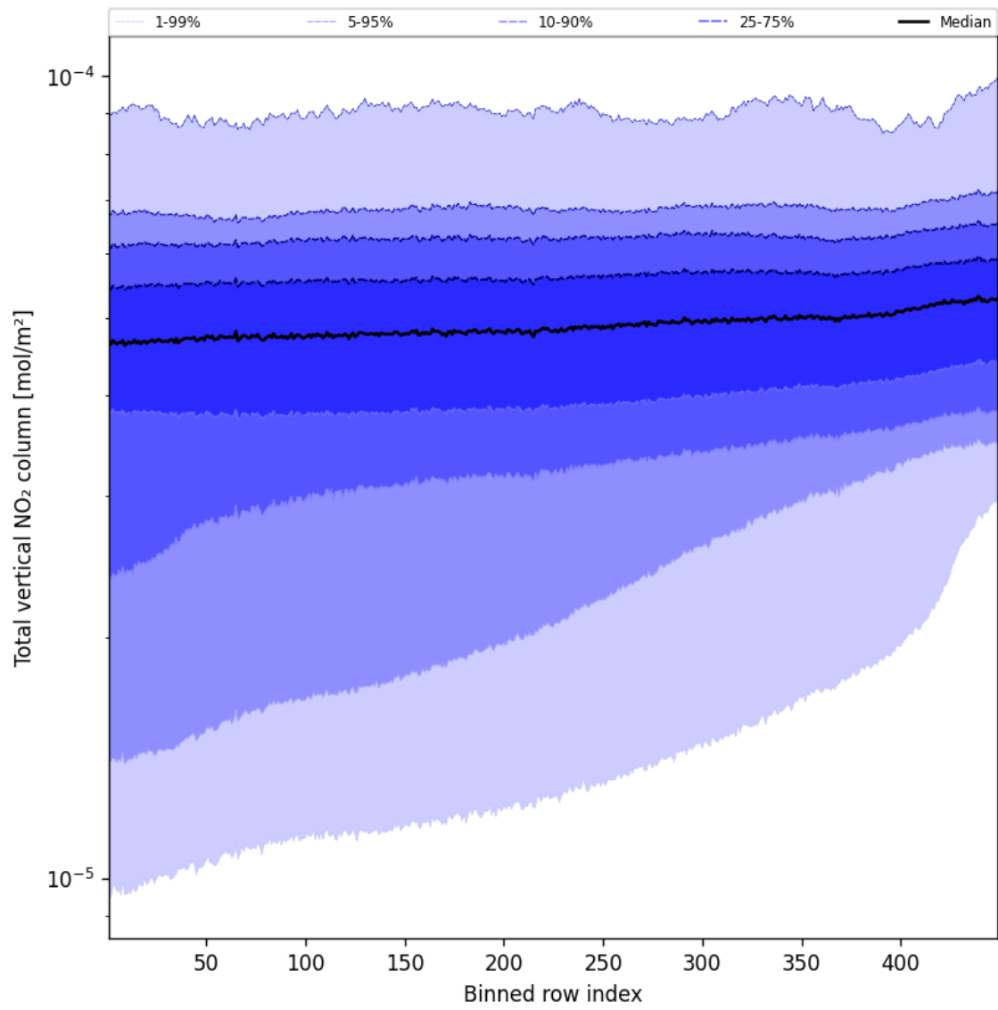
Figure 55: Along track statistics of “Total vertical NO 2 column” for 2024-09-19 to 2024-09-21
