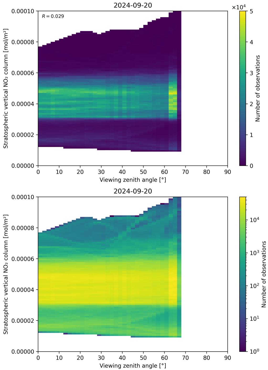
Figure 164: Scatter density plot of “Viewing zenith angle” against “Stratospheric vertical NO 2 column” for 2024-09-19 to 2024-09-21.
