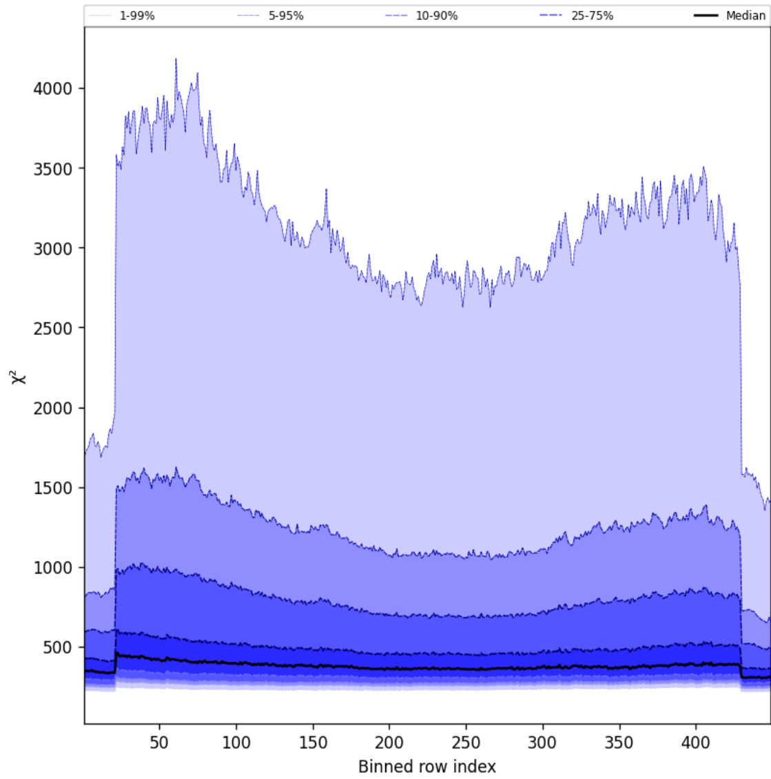
Figure 59: Along track statistics of “ \chi^2 ” for 2024-09-19 to 2024-09-21
