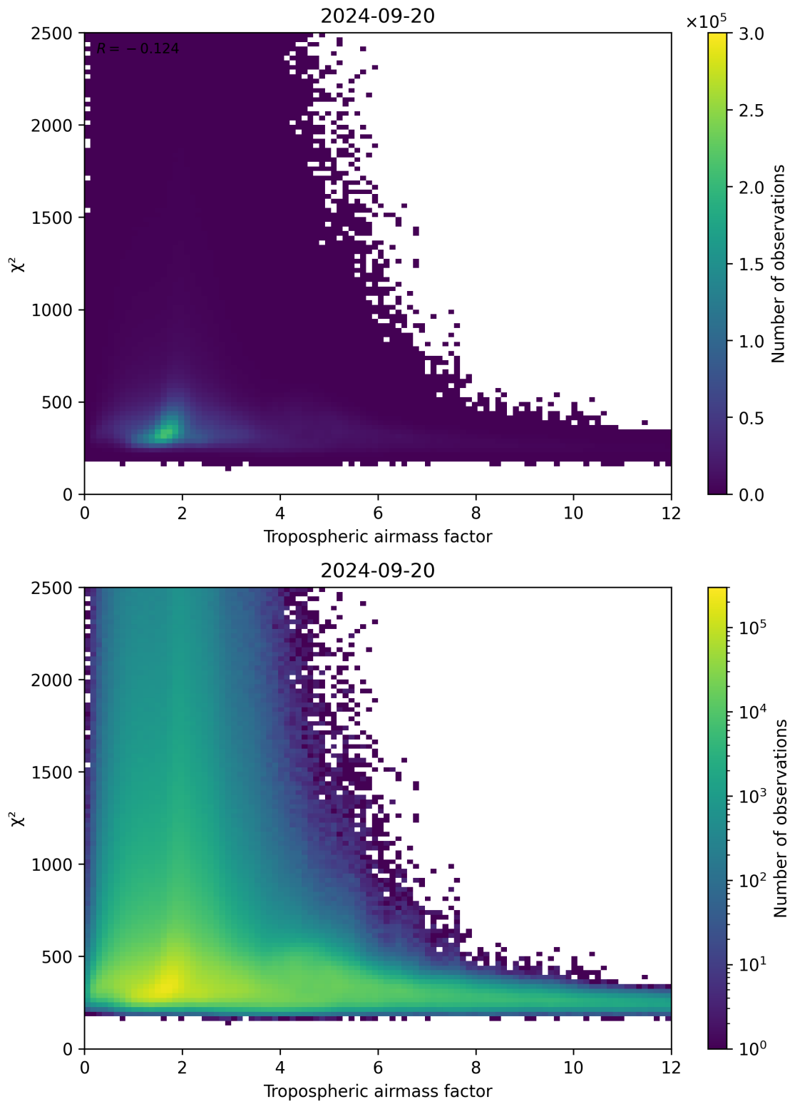
Figure 73: Scatter density plot of “Tropospheric airmass factor” against “ \chi^2 ” for 2024-09-19 to 2024-09-21.
