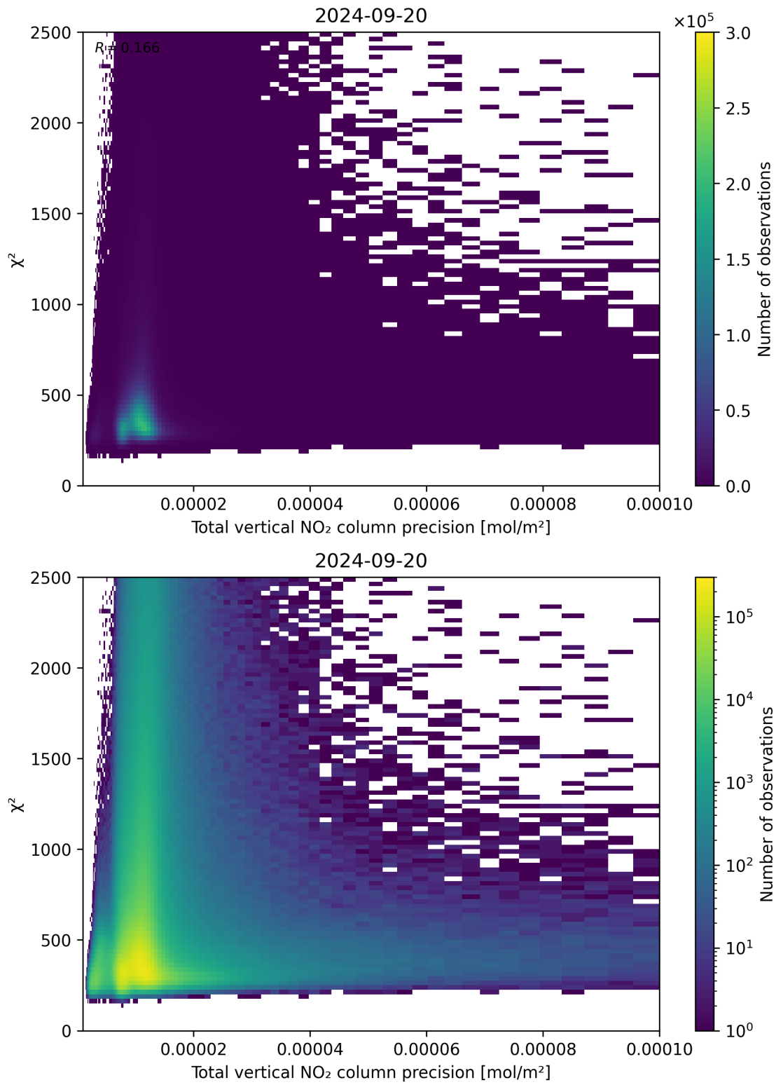
Figure 116: Scatter density plot of “Total vertical NO 2 column precision” against “ \chi^2 ” for 2024-09-19 to 2024-09-21.
