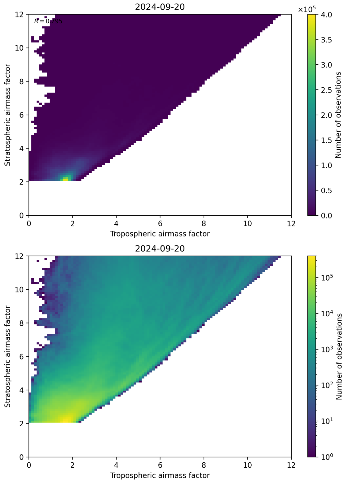
Figure 71: Scatter density plot of “Tropospheric airmass factor” against “Stratospheric airmass factor” for 2024-09-19 to 2024-09-21.
