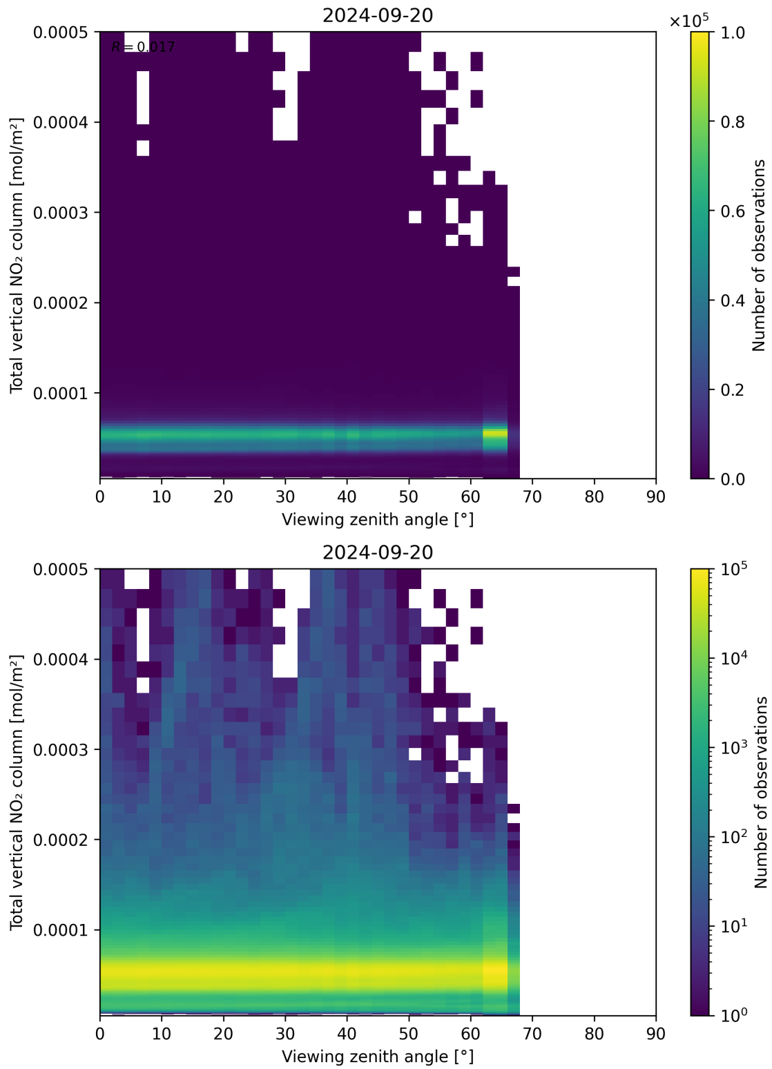
Figure 167: Scatter density plot of “Viewing zenith angle” against “Total vertical NO 2 column” for 2024-09-19 to 2024-09-21.
