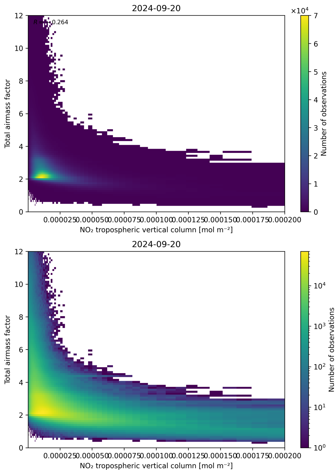
Figure 122: Scatter density plot of “NO 2 tropospheric vertical column” against “Total air mass factor” for 2024-09-19 to 2024-09-21.
