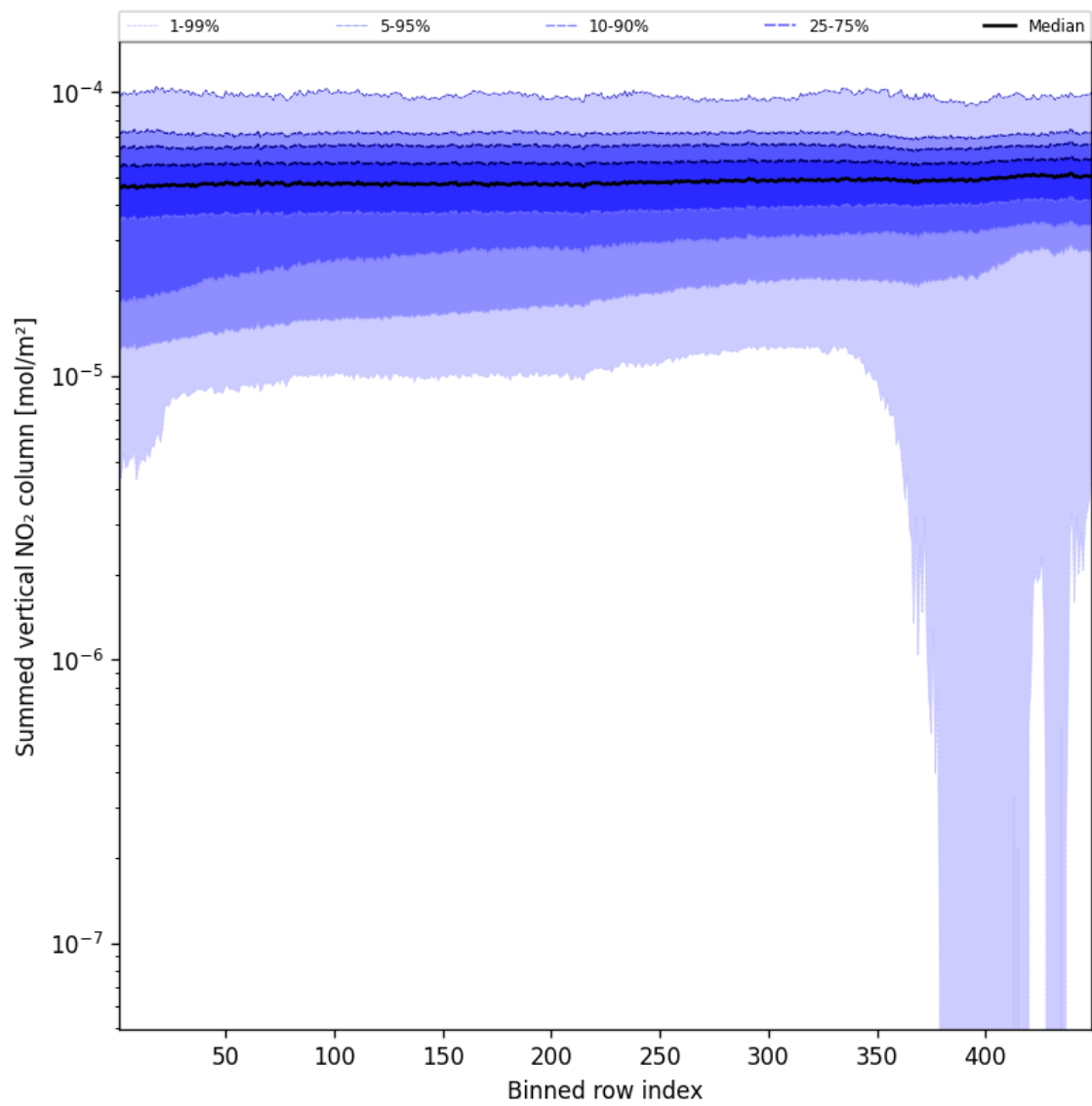
Figure 57: Along track statistics of “Summed vertical NO 2 column” for 2024-09-19 to 2024-09-21
