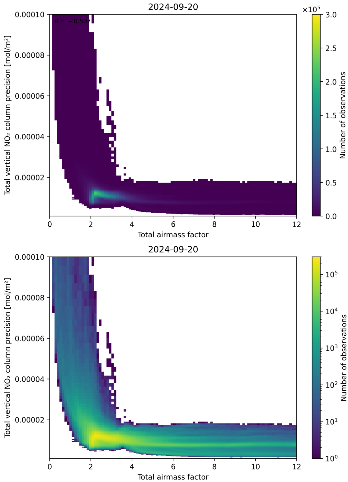
Figure 68: Scatter density plot of “Total airmass factor” against “Total vertical NO 2 column precision” for 2024-09-19 to 2024-09-21.
