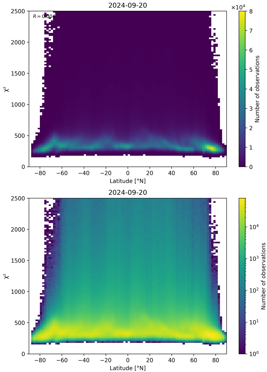
Figure 86: Scatter density plot of “Latitude” against “ \chi^2 ” for 2024-09-19 to 2024-09-21.
