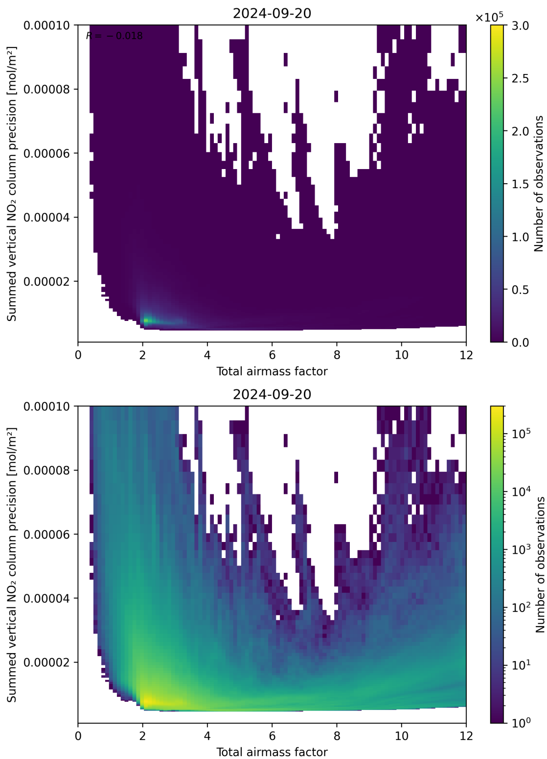
Figure 66: Scatter density plot of “Total airmass factor” against “Summed vertical NO 2 column precision” for 2024-09-19 to 2024-09-21.
