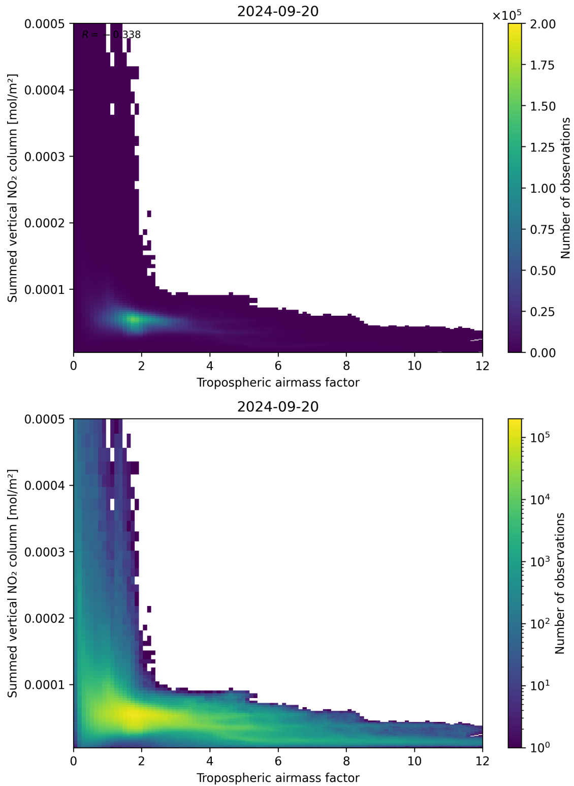
Figure 75: Scatter density plot of “Tropospheric air mass factor” against “Summed vertical NO 2 column” for 2024-09-19 to 2024-09-21.
