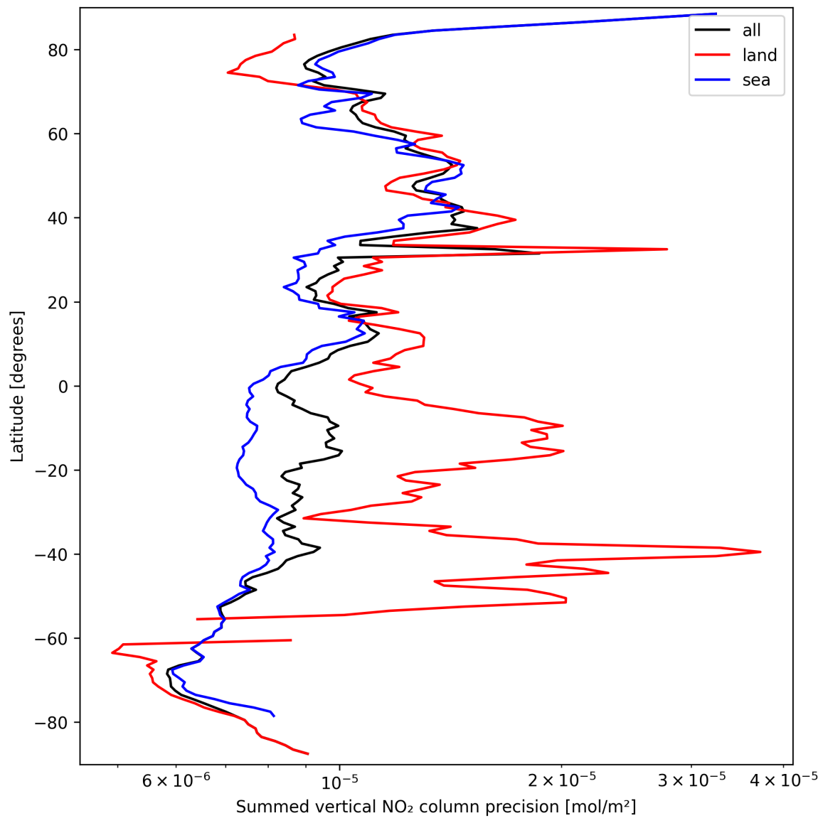
Figure 24: Zonal average of “Summed vertical NO 2 column precision” for 2024-09-19 to 2024-09-21.
