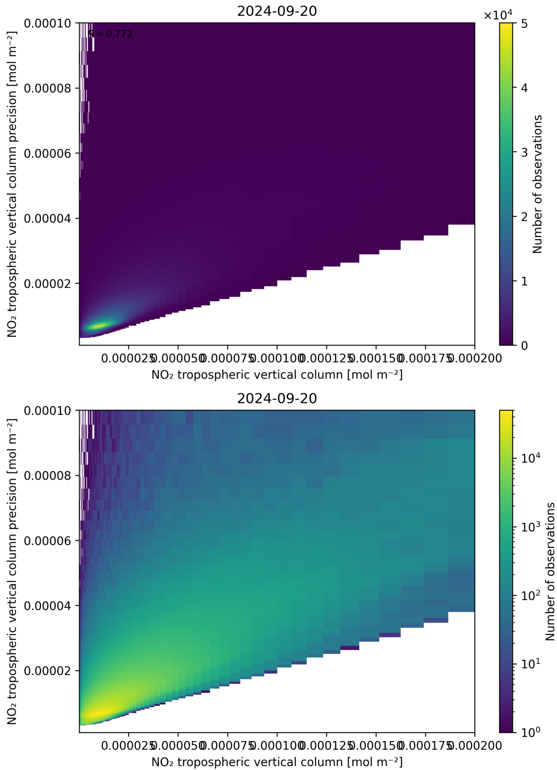
Figure 130: Scatter density plot of “NO 2 tropospheric vertical column” against “NO 2 tropospheric vertical column precision” for 2024-09-19 to 2024-09-21.
