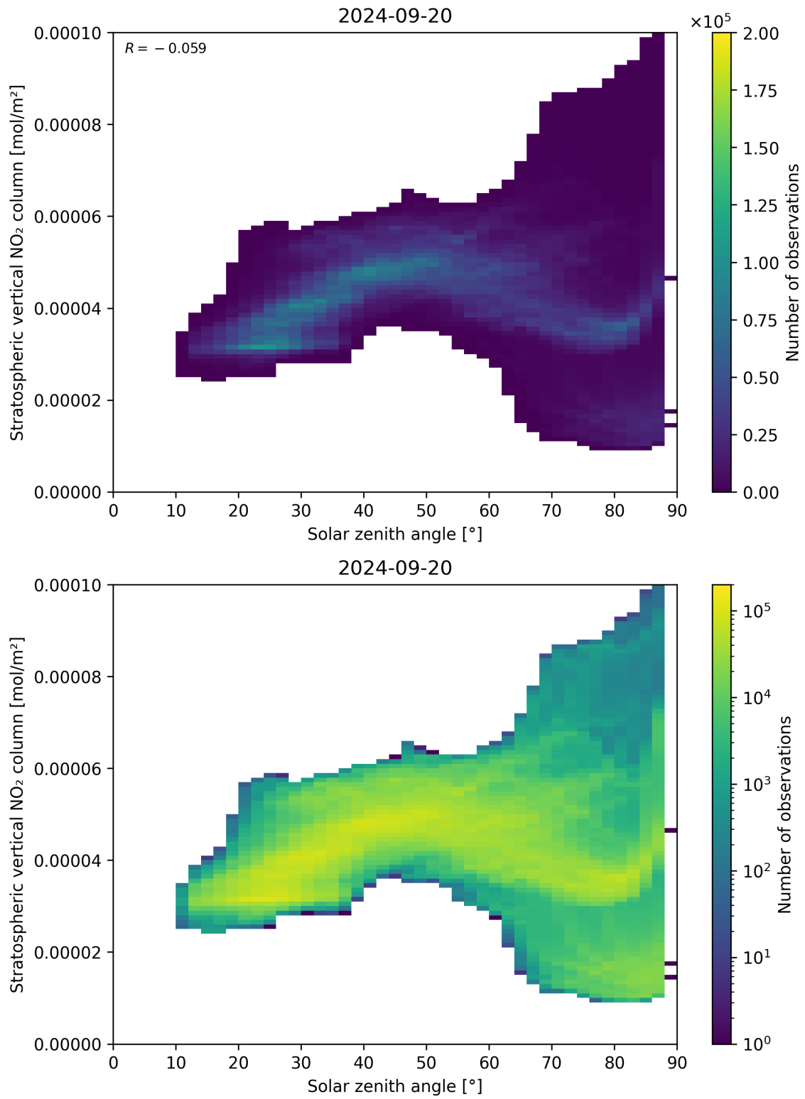
Figure 150: Scatter density plot of “Solar zenith angle” against “Stratospheric vertical NO 2 column” for 2024-09-19 to 2024-09-21.
