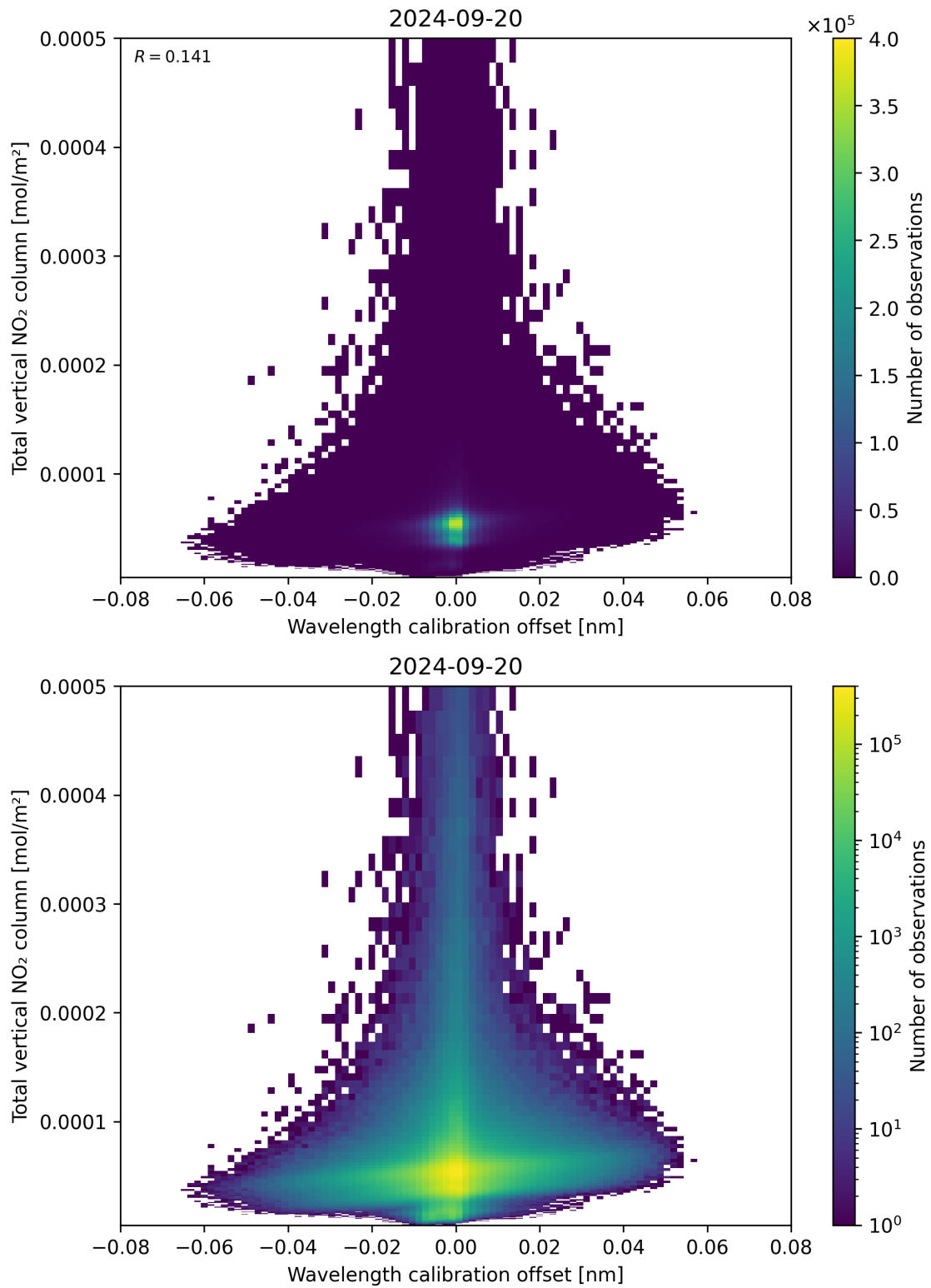
Figure 179: Scatter density plot of “Wavelength calibration offset” against “Total vertical NO 2 column” for 2024-09-19 to 2024-09-21.
