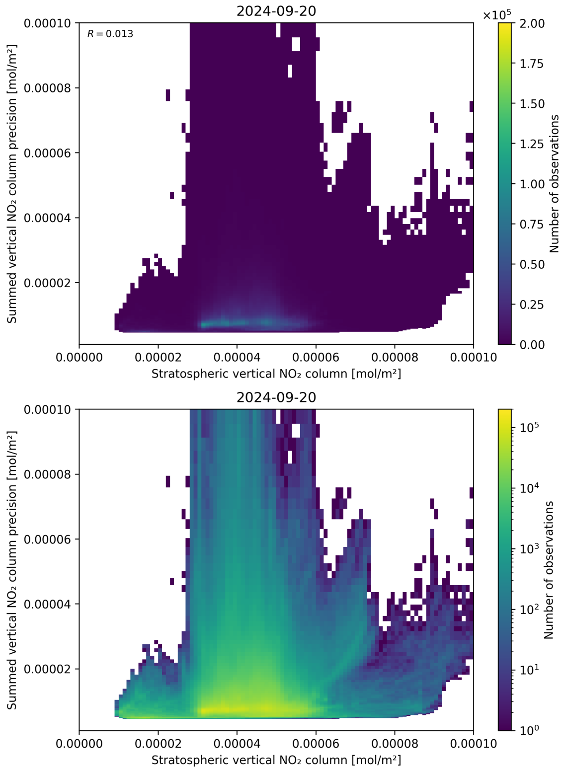
Figure 99: Scatter density plot of “Stratospheric vertical NO 2 column” against “Summed vertical NO 2 column precision” for 2024-09-19 to 2024-09-21.
