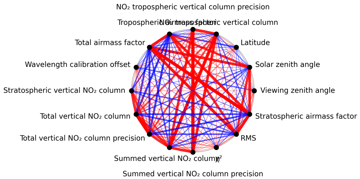
Figure 1: Map of correlation graph for 2024-09-19 to 2024-09-21.
