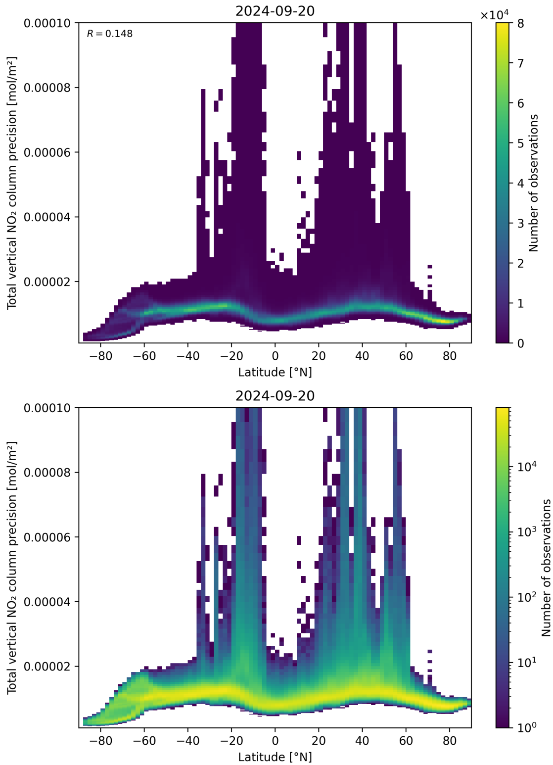
Figure 91: Scatter density plot of “Latitude” against “Total vertical NO 2 column precision” for 2024-09-19 to 2024-09-21.
