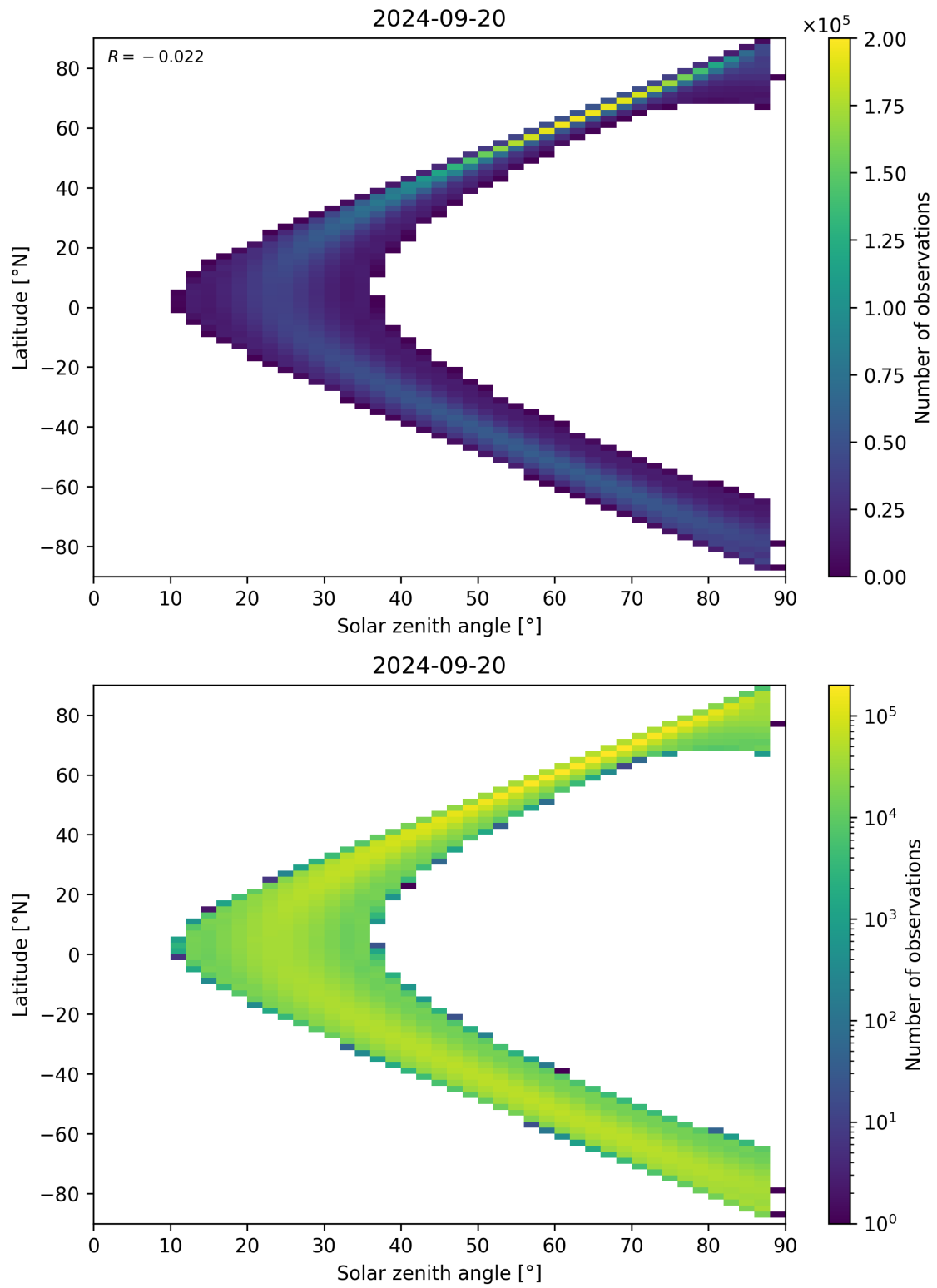
Figure 149: Scatter density plot of “Solar zenith angle” against “Latitude” for 2024-09-19 to 2024-09-21.
