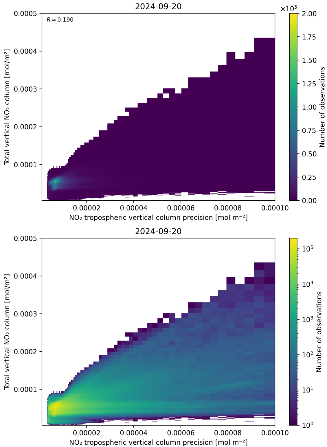
Figure 138: Scatter density plot of “NO 2 tropospheric vertical column precision” against “Total vertical NO 2 column” for 2024-09-19 to 2024-09-21.
