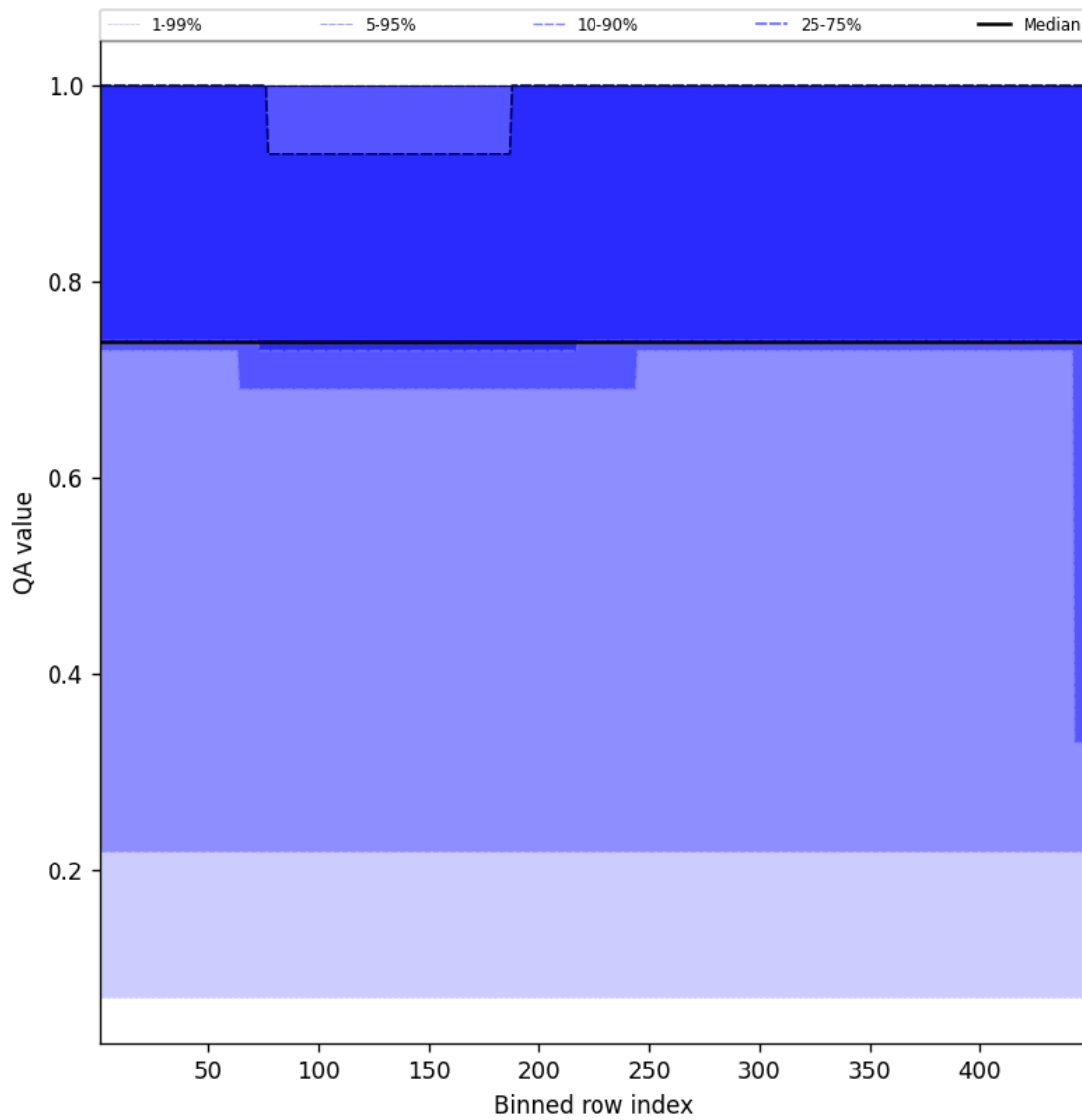
Figure 45: Along track statistics of “QA value” for 2024-09-19 to 2024-09-21
