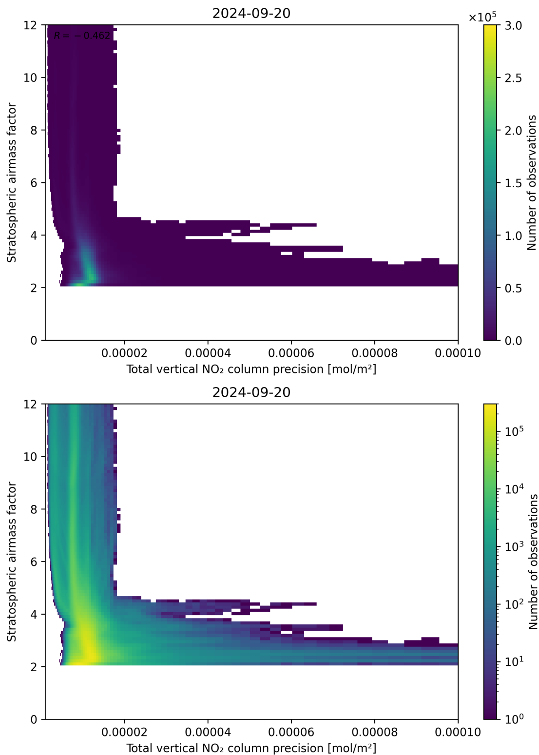
Figure 115: Scatter density plot of “Total vertical NO 2 column precision” against “Stratospheric air mass factor” for 2024-09-19 to 2024-09-21.
