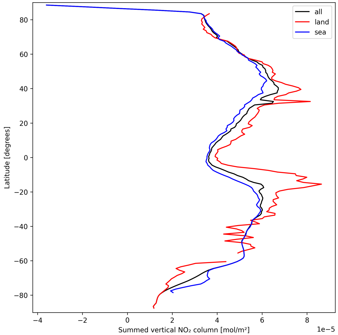
Figure 23: Zonal average of “Summed vertical NO 2 column” for 2024-09-19 to 2024-09-21.
