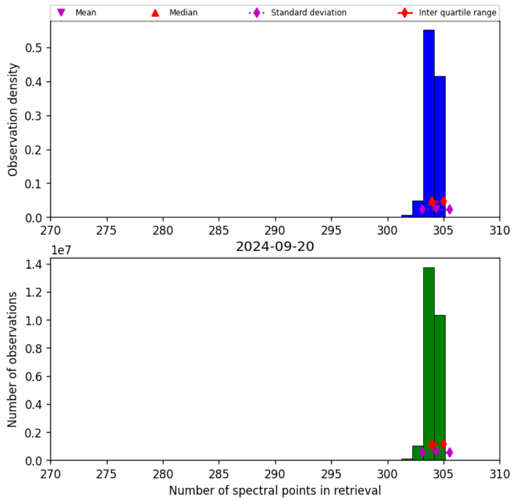
Figure 33: Histogram of “Number of spectral points in retrieval” for 2024-09-19 to 2024-09-21
