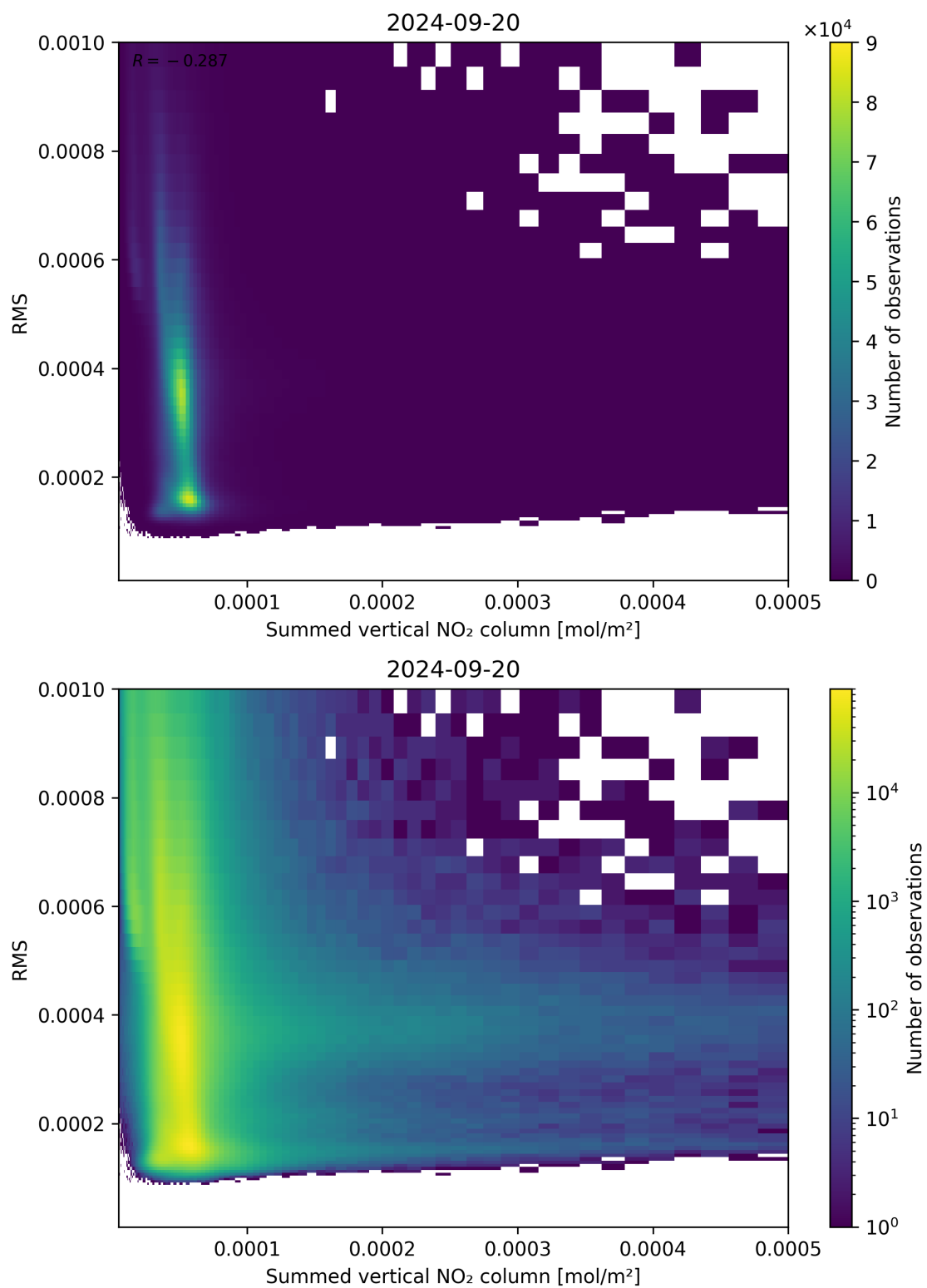
Figure 109: Scatter density plot of “Summed vertical NO 2 column” against “RMS” for 2024-09-19 to 2024-09-21.
