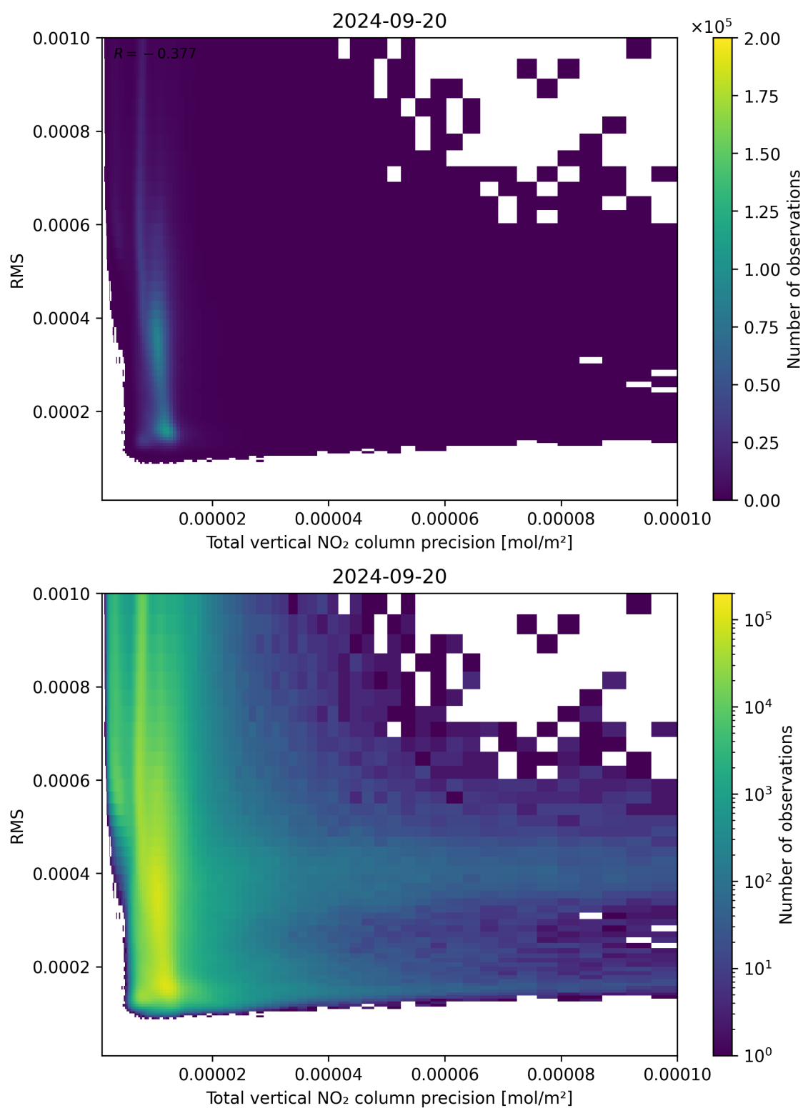
Figure 119: Scatter density plot of “Total vertical NO 2 column precision” against “RMS” for 2024-09-19 to 2024-09-21.
