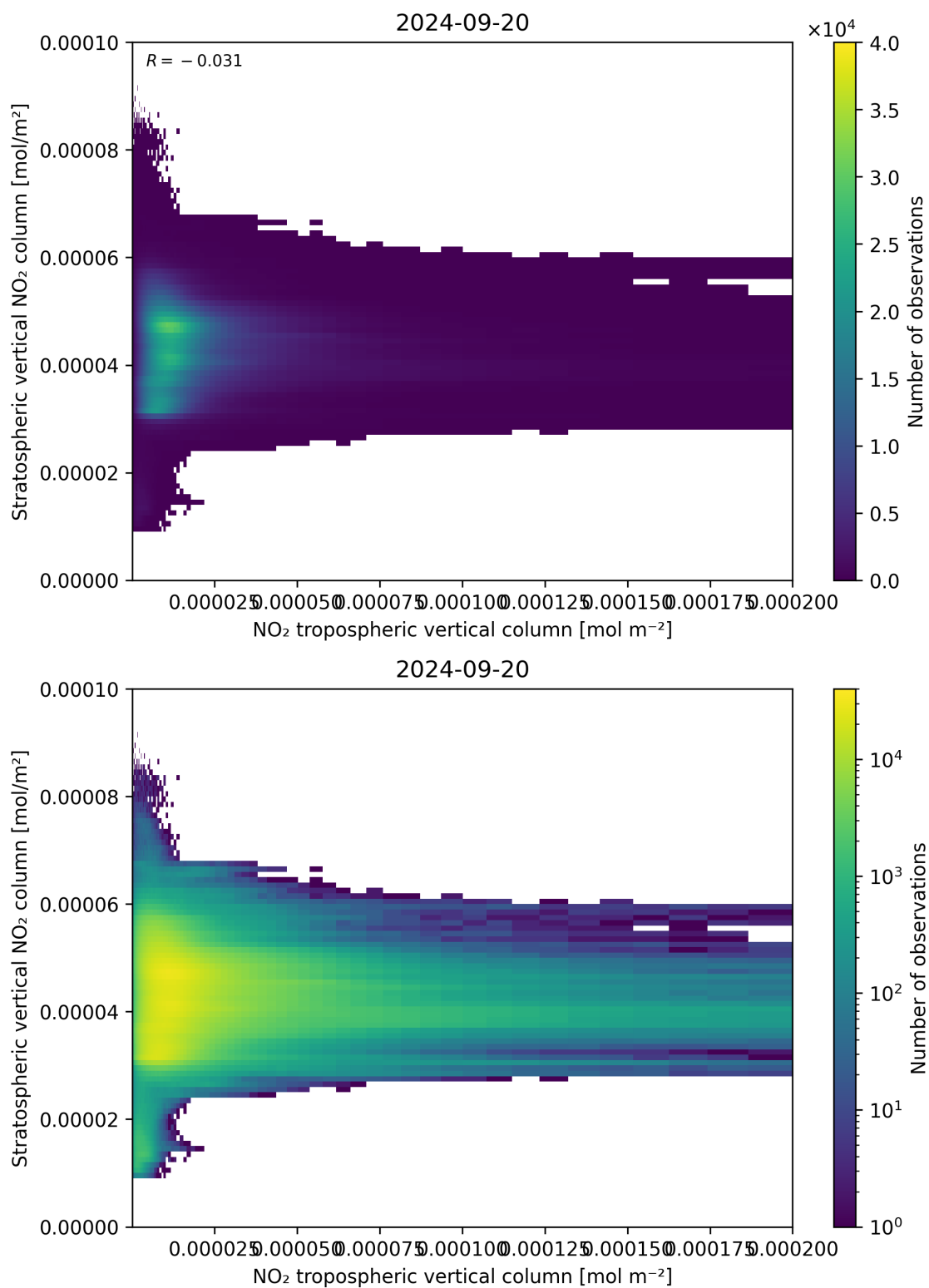
Figure 125: Scatter density plot of “NO 2 tropospheric vertical column” against “Stratospheric vertical NO 2 column” for 2024-09-19 to 2024-09-21.
