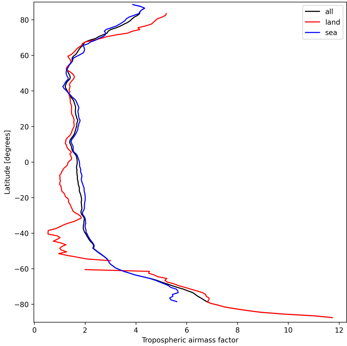
Figure 14: Zonal average of “Tropospheric air mass factor” for 2024-09-19 to 2024-09-21.
