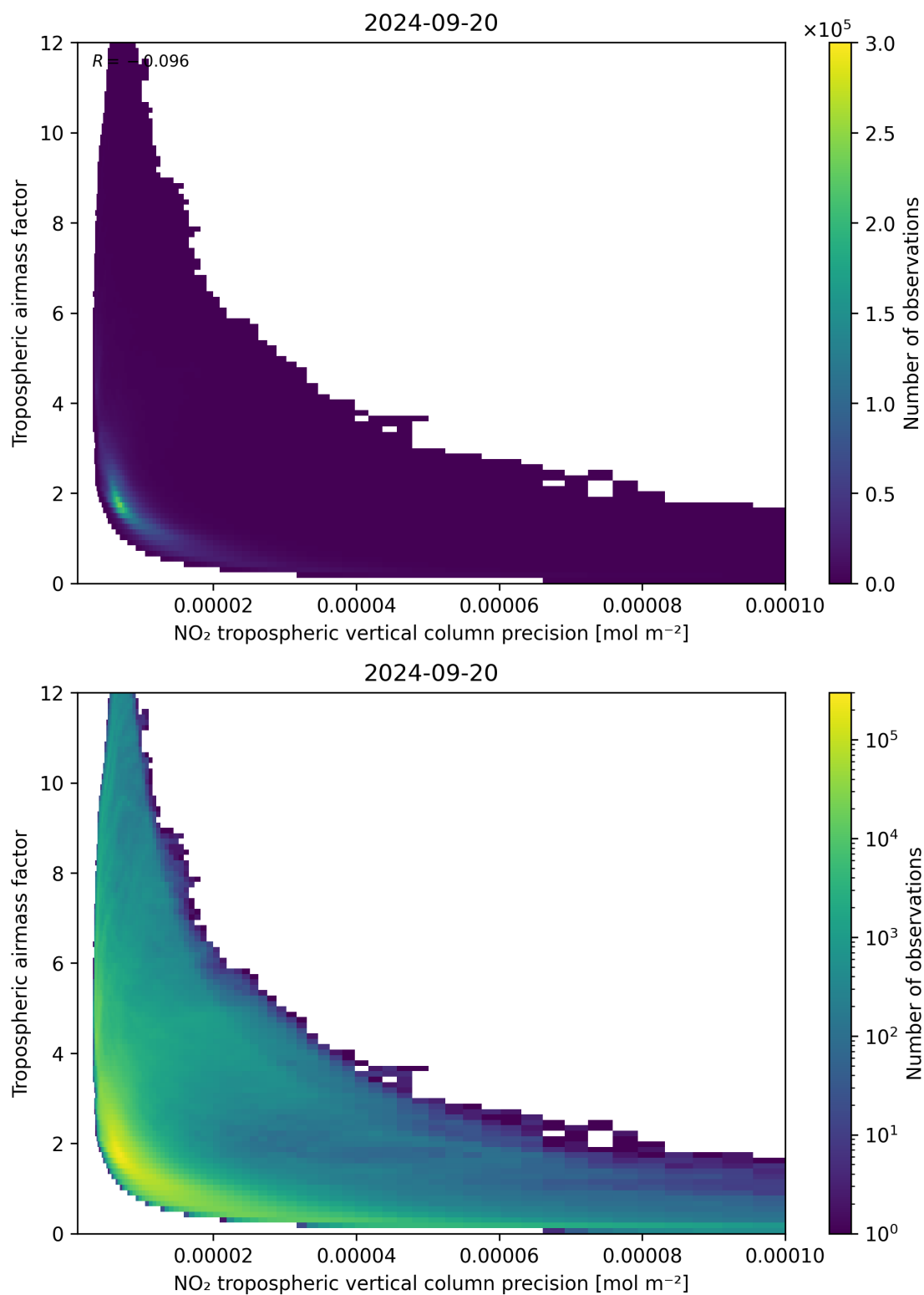
Figure 133: Scatter density plot of “NO 2 tropospheric vertical column precision” against “Tropospheric airmass factor” for 2024-09-19 to 2024-09-21.
