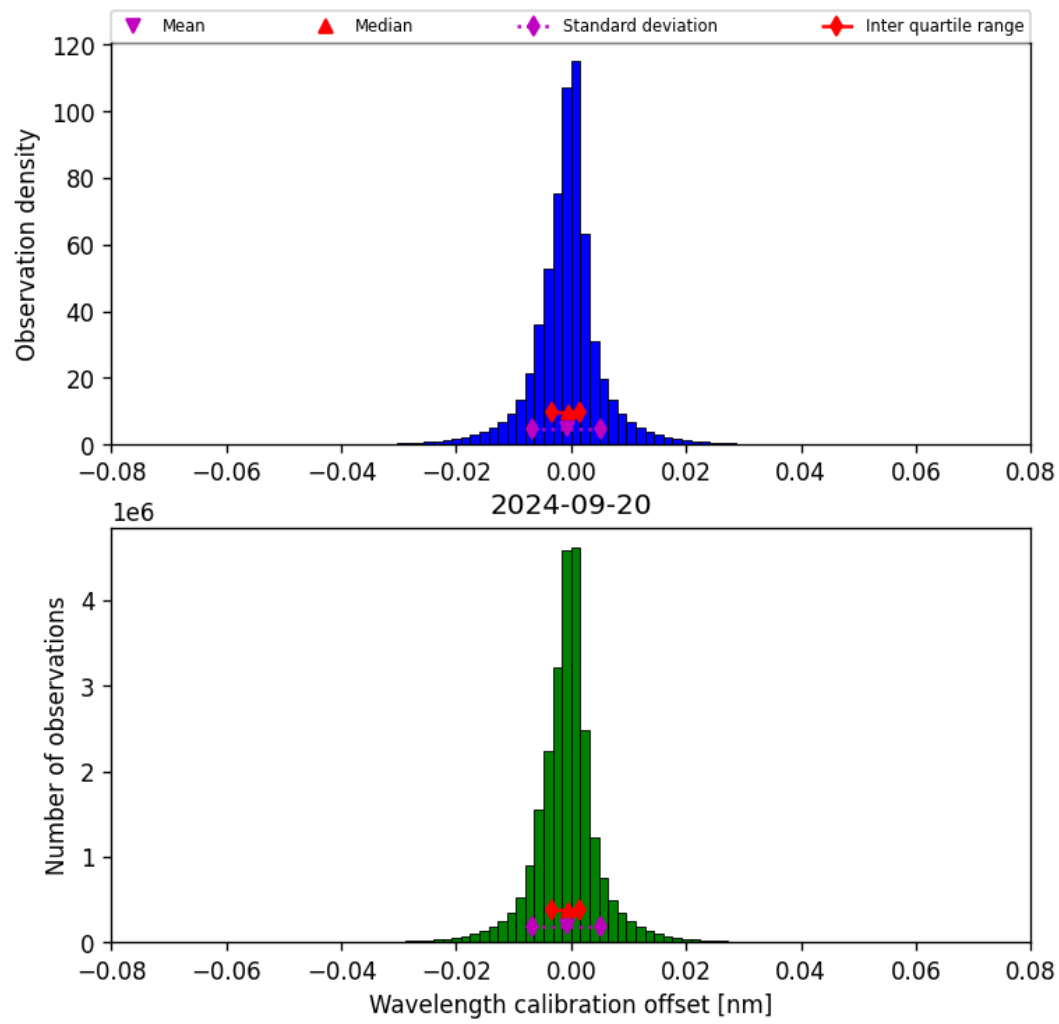
Figure 35: Histogram of “Wavelength calibration offset” for 2024-09-19 to 2024-09-21
