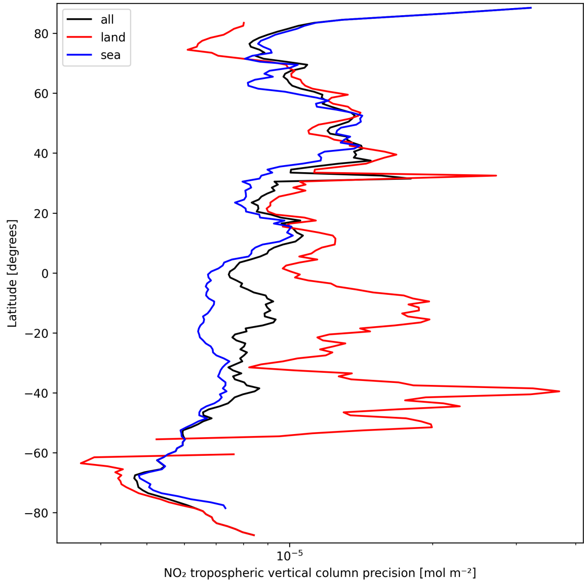
Figure 13: Zonal average of “NO 2 tropospheric vertical column precision” for 2024-09-19 to 2024-09-21.
