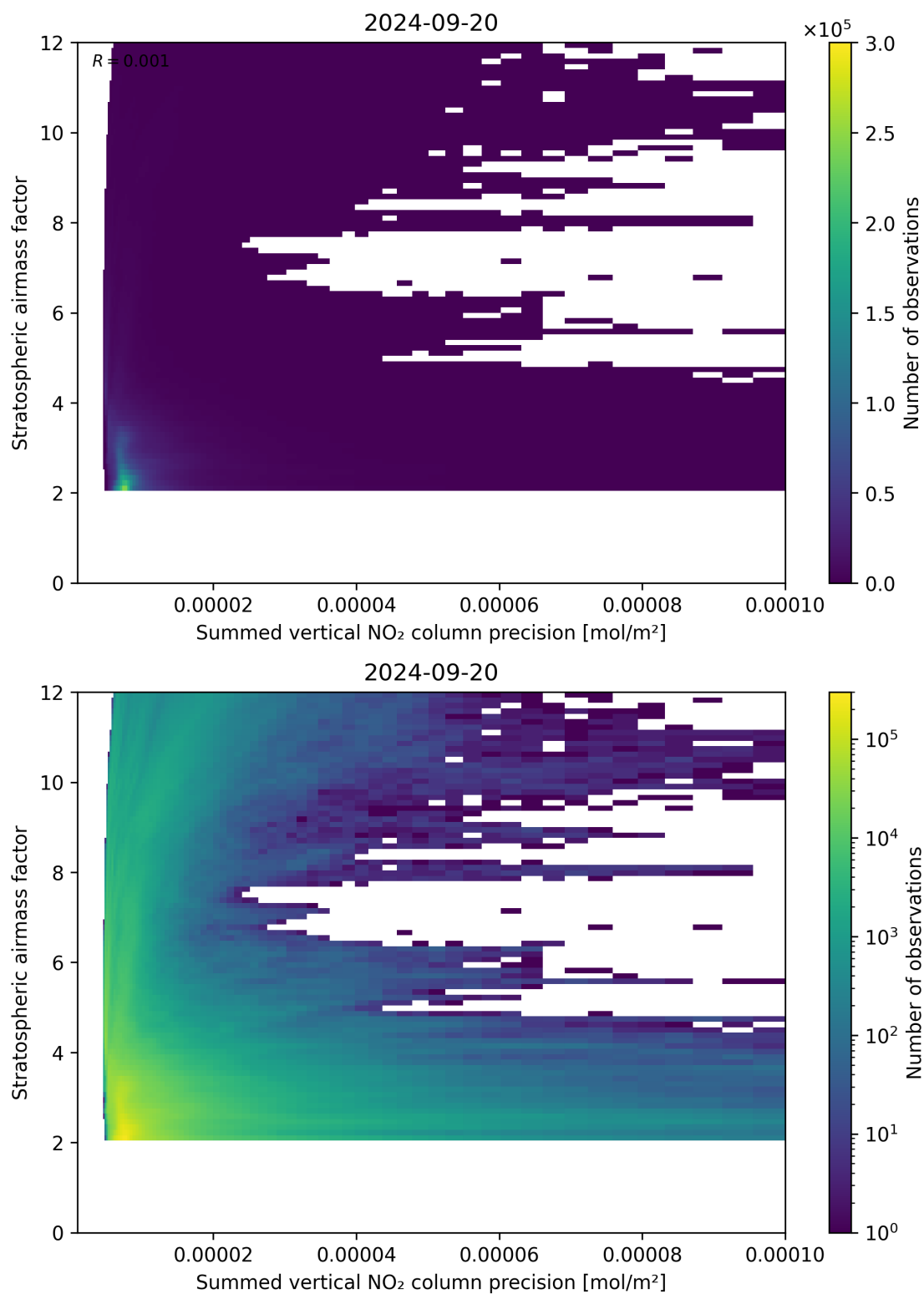
Figure 106: Scatter density plot of “Summed vertical NO 2 column precision” against “Stratospheric airmass factor” for 2024-09-19 to 2024-09-21.
