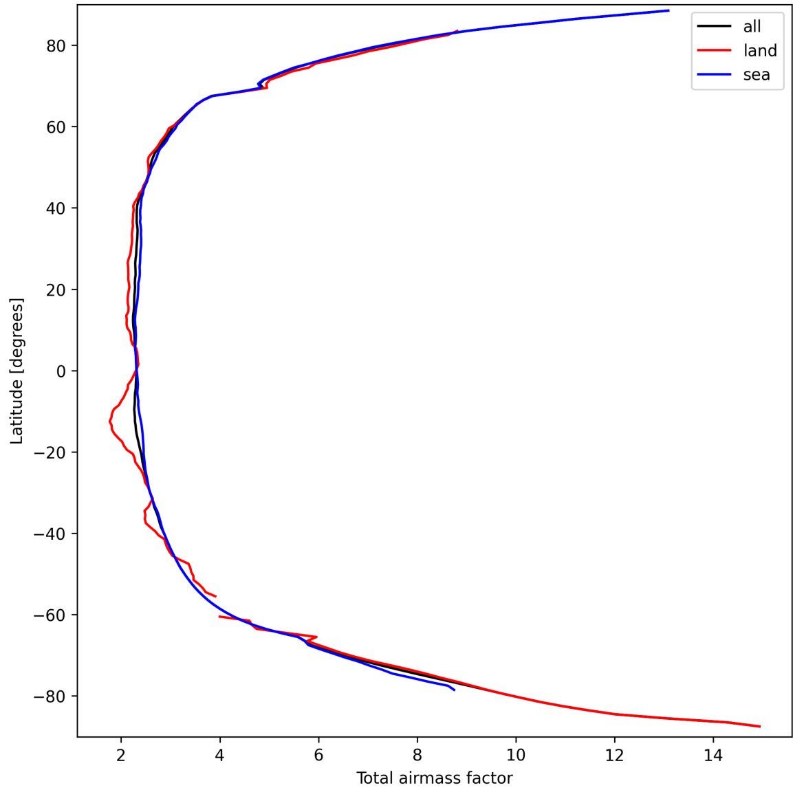
Figure 15: Zonal average of “Total airmass factor” for 2024-09-19 to 2024-09-21.
