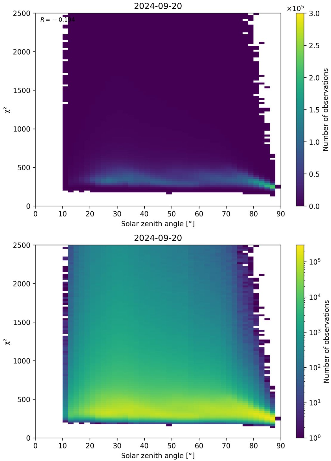
Figure 148: Scatter density plot of “Solar zenith angle” against “ \chi^2 ” for 2024-09-19 to 2024-09-21.
