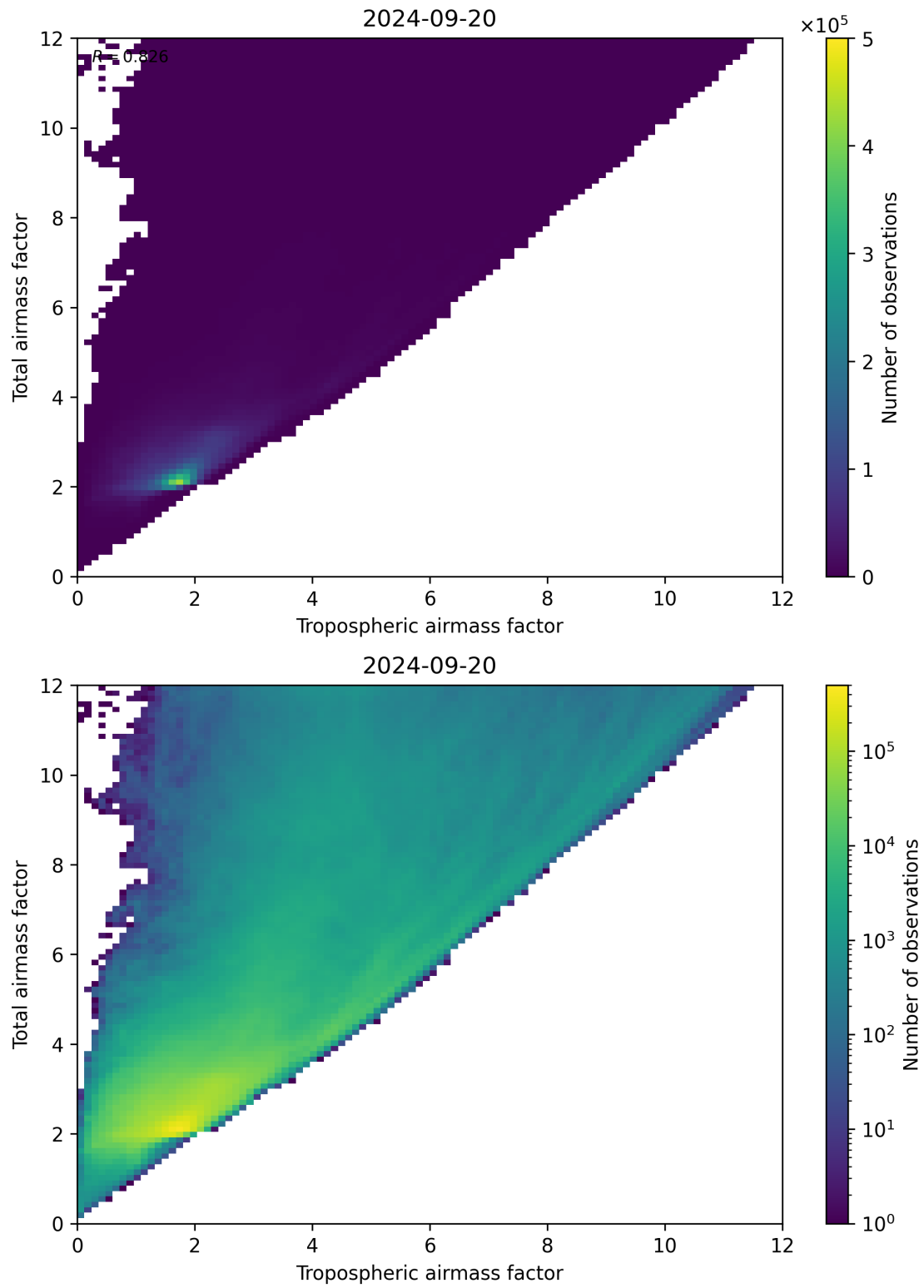
Figure 72: Scatter density plot of “Tropospheric airmass factor” against “Total airmass factor” for 2024-09-19 to 2024-09-21.
