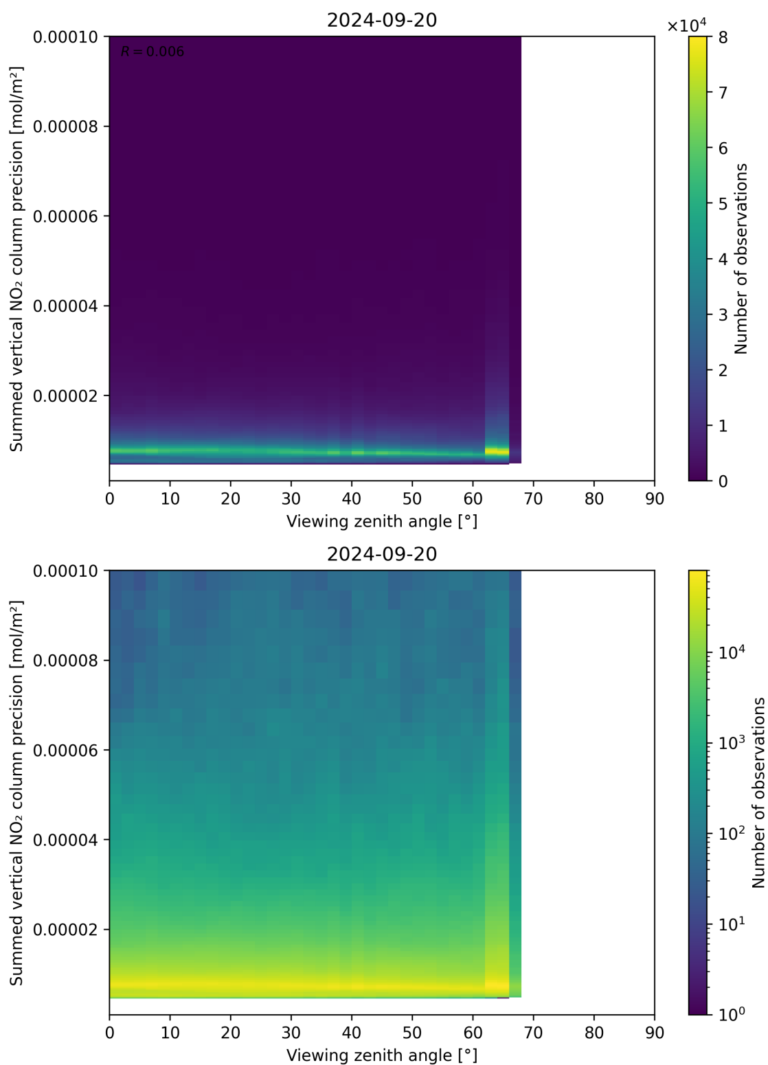
Figure 166: Scatter density plot of “Viewing zenith angle” against “Summed vertical NO 2 column precision” for 2024-09-19 to 2024-09-21.
