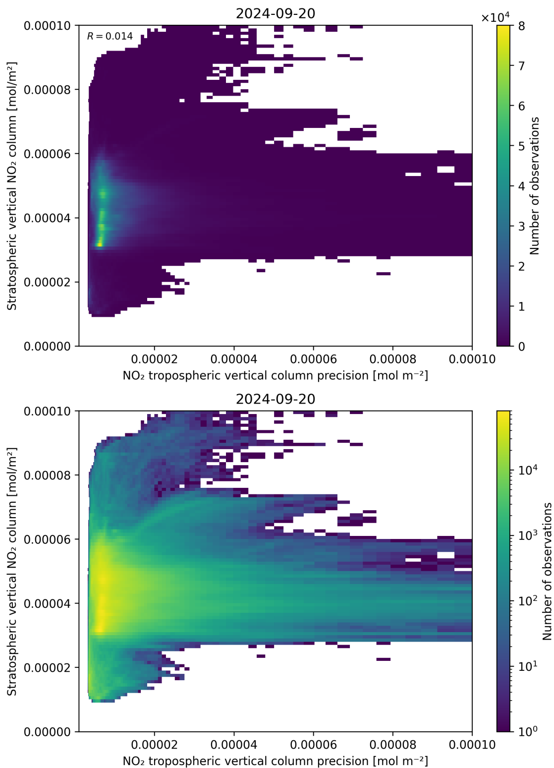
Figure 135: Scatter density plot of “NO 2 tropospheric vertical column precision” against “Stratospheric vertical NO 2 column” for 2024-09-19 to 2024-09-21.
