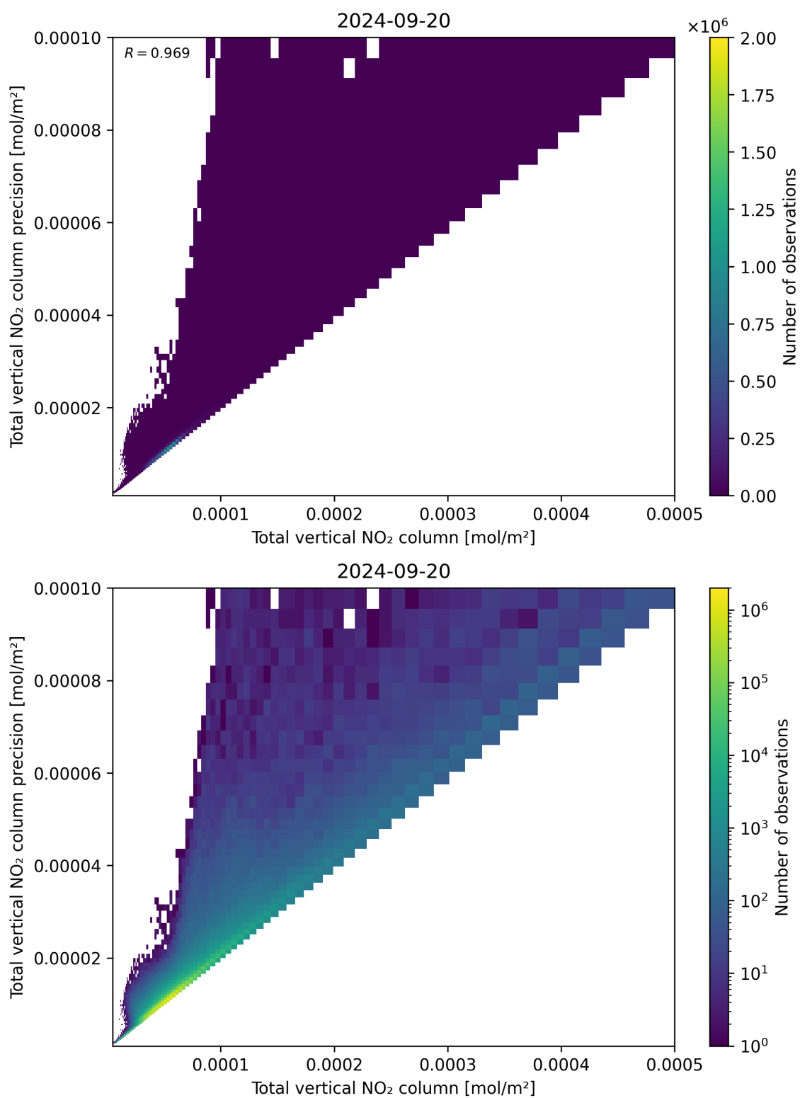
Figure 114: Scatter density plot of “Total vertical NO 2 column” against “Total vertical NO 2 column precision” for 2024-09-19 to 2024-09-21.
