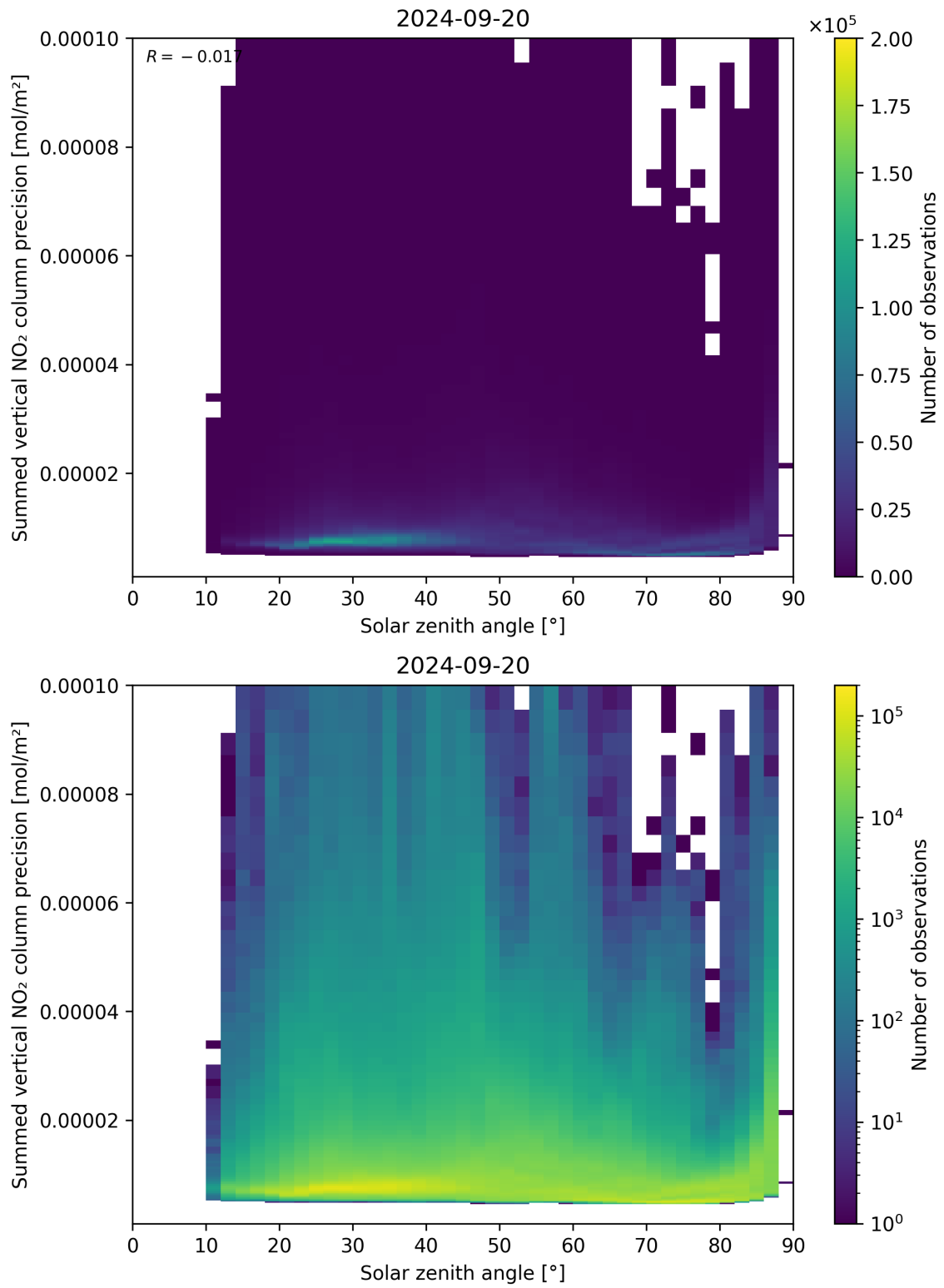
Figure 152: Scatter density plot of “Solar zenith angle” against “Summed vertical NO 2 column precision” for 2024-09-19 to 2024-09-21.
