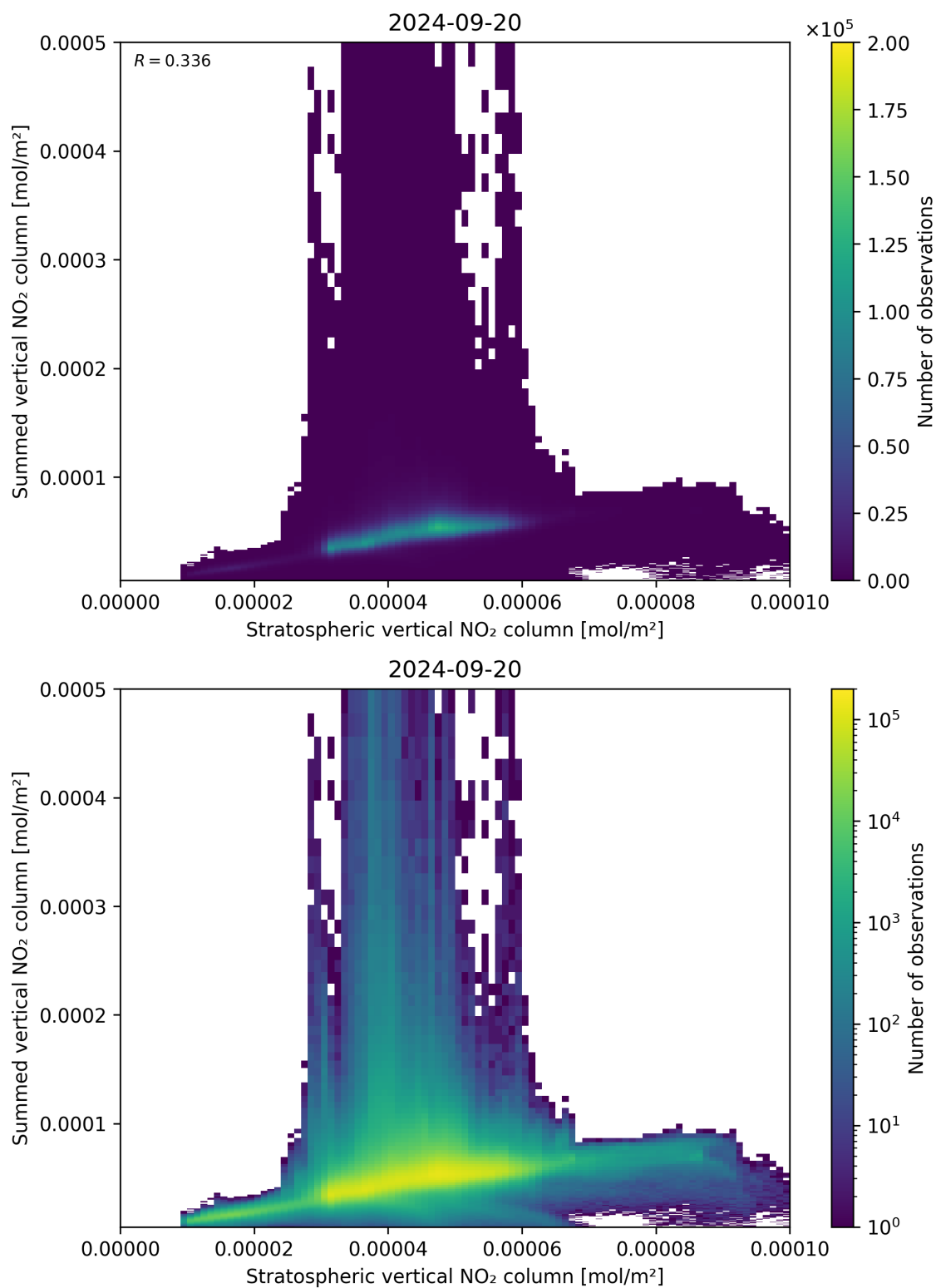
Figure 98: Scatter density plot of “Stratospheric vertical NO 2 column” against “Summed vertical NO 2 column” for 2024-09-19 to 2024-09-21.
