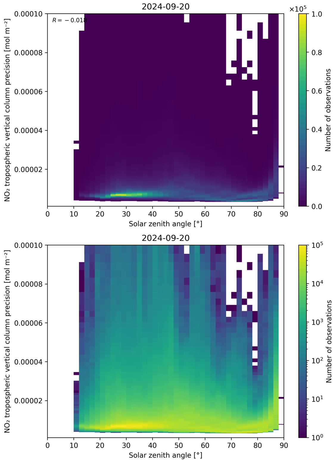
Figure 156: Scatter density plot of “Solar zenith angle” against “NO 2 tropospheric vertical column precision” for 2024-09-19 to 2024-09-21.
