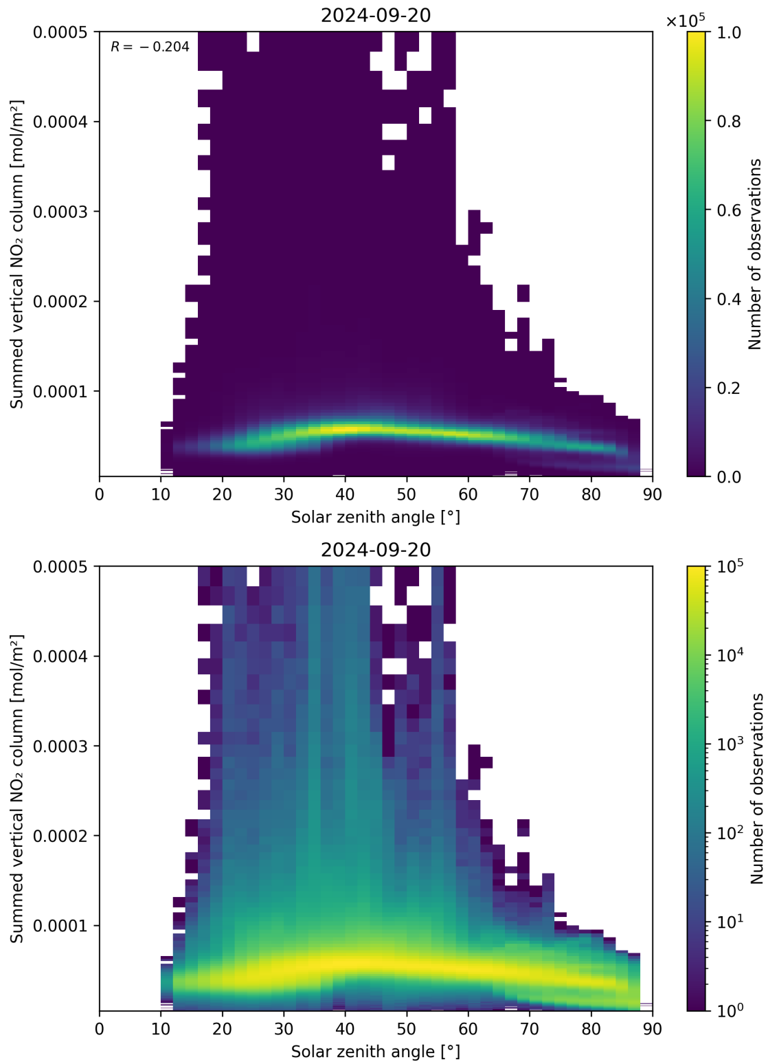
Figure 151: Scatter density plot of “Solar zenith angle” against “Summed vertical NO 2 column” for 2024-09-19 to 2024-09-21.
