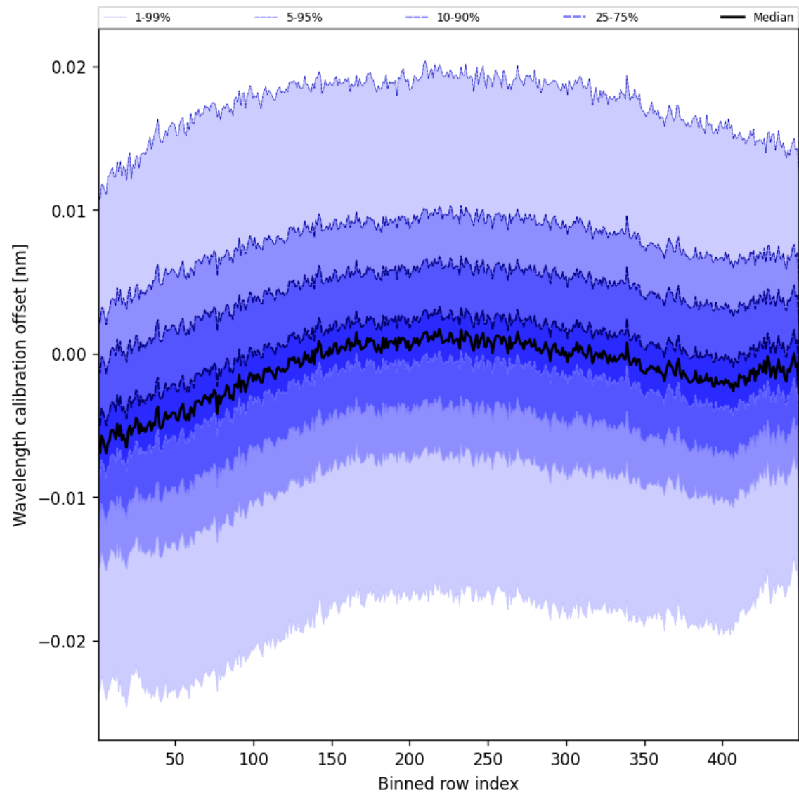
Figure 52: Along track statistics of “Wavelength calibration offset” for 2024-10-11 to 2024-10-13
