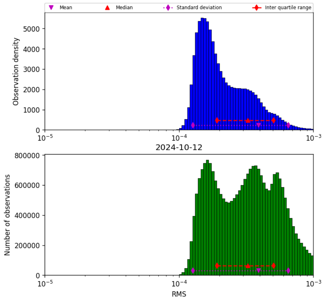
Figure 43: Histogram of “RMS” for 2024-10-11 to 2024-10-13
