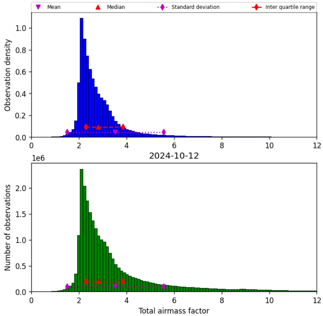
Figure 32: Histogram of “Total airmass factor” for 2024-10-11 to 2024-10-13
