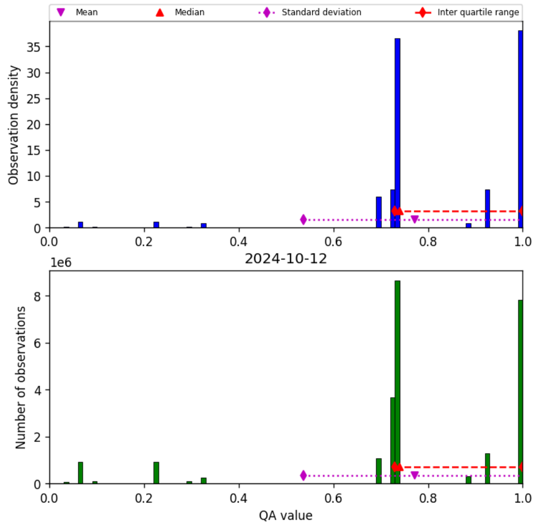
Figure 28: Histogram of “QA value” for 2024-10-11 to 2024-10-13
