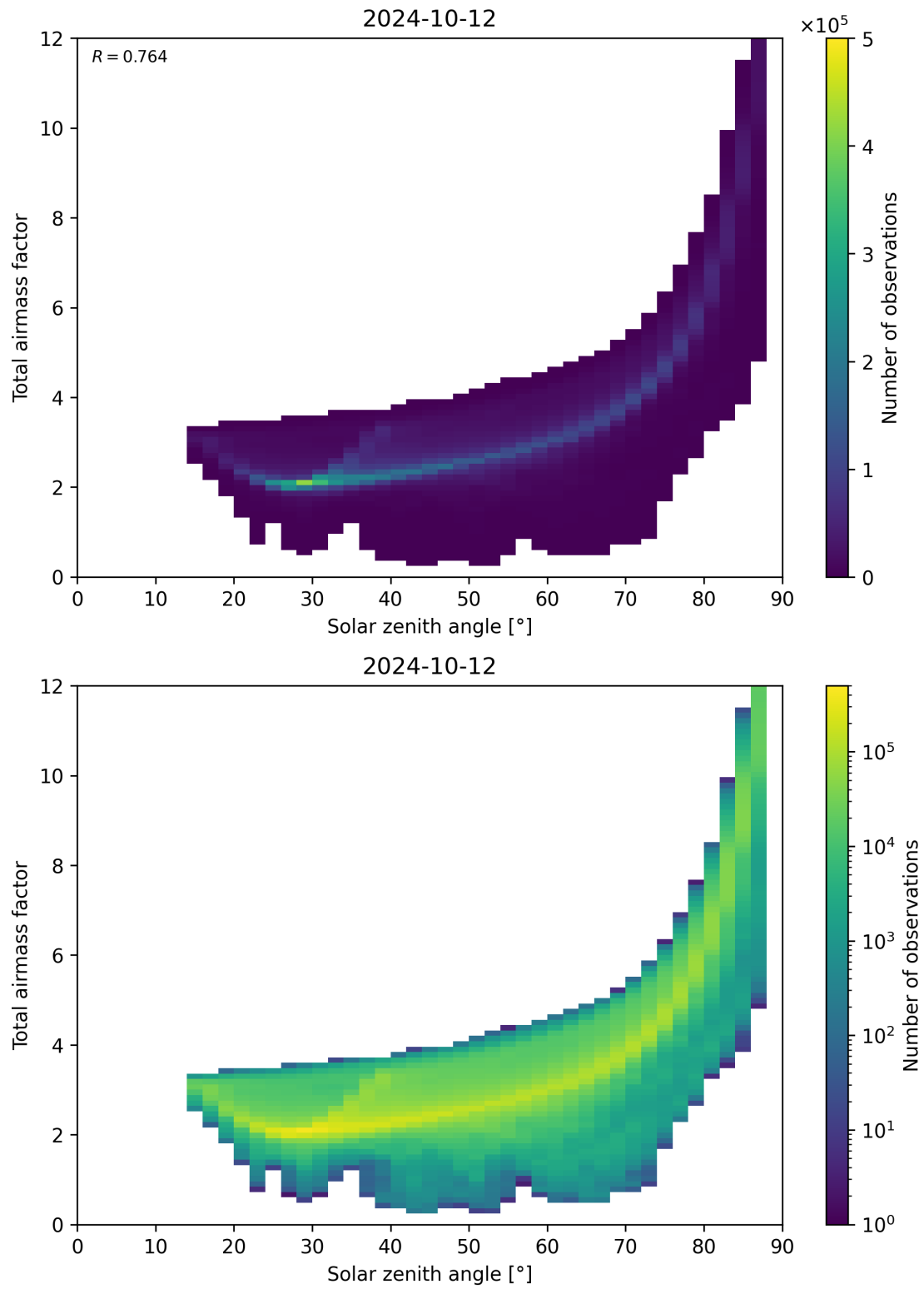
Figure 146: Scatter density plot of “Solar zenith angle” against “Total airmass factor” for 2024-10-11 to 2024-10-13.
