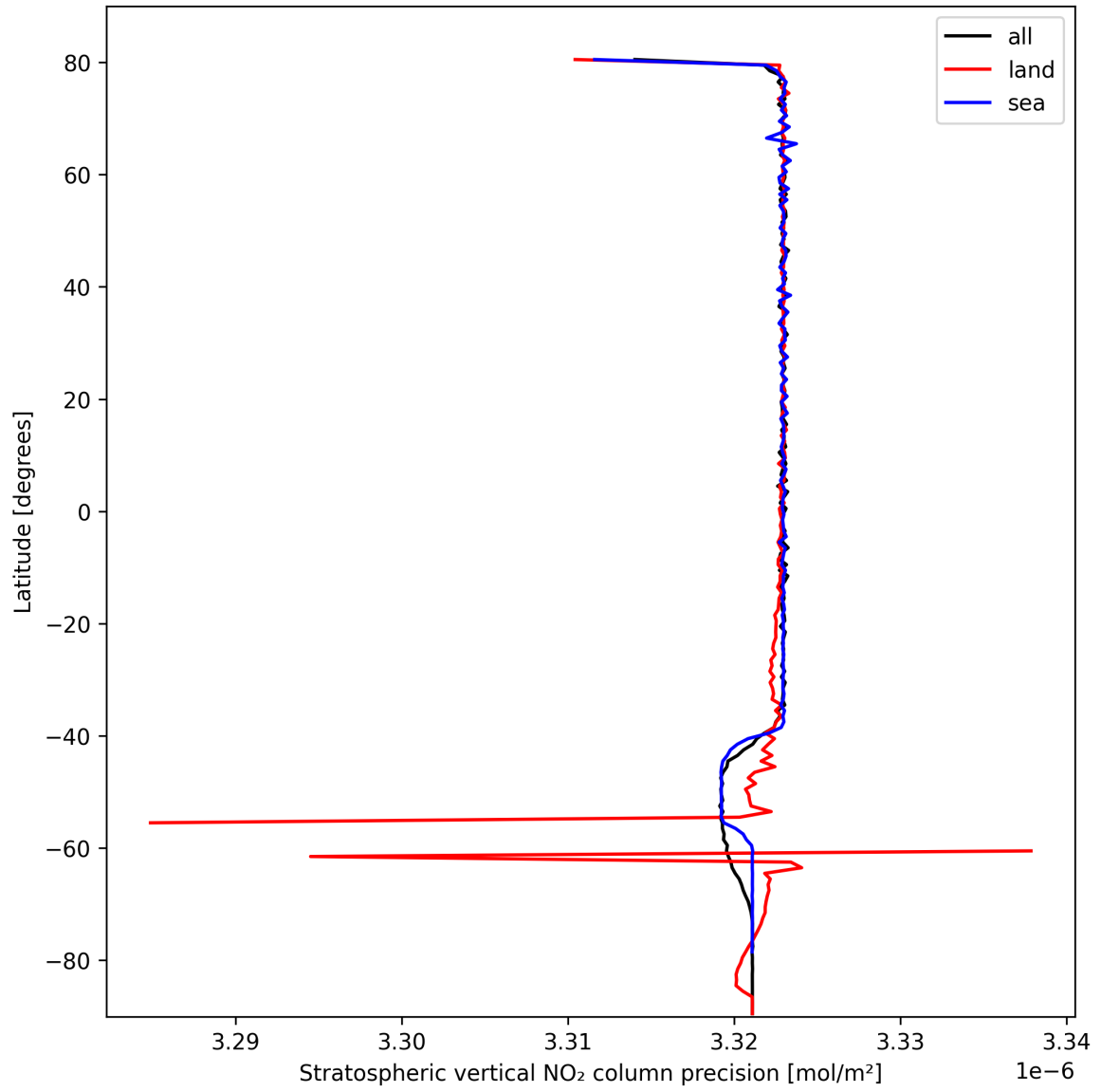
Figure 20: Zonal average of "Stratospheric vertical NO 2 column precision" for 2024-10-11 to 2024-10-13.
