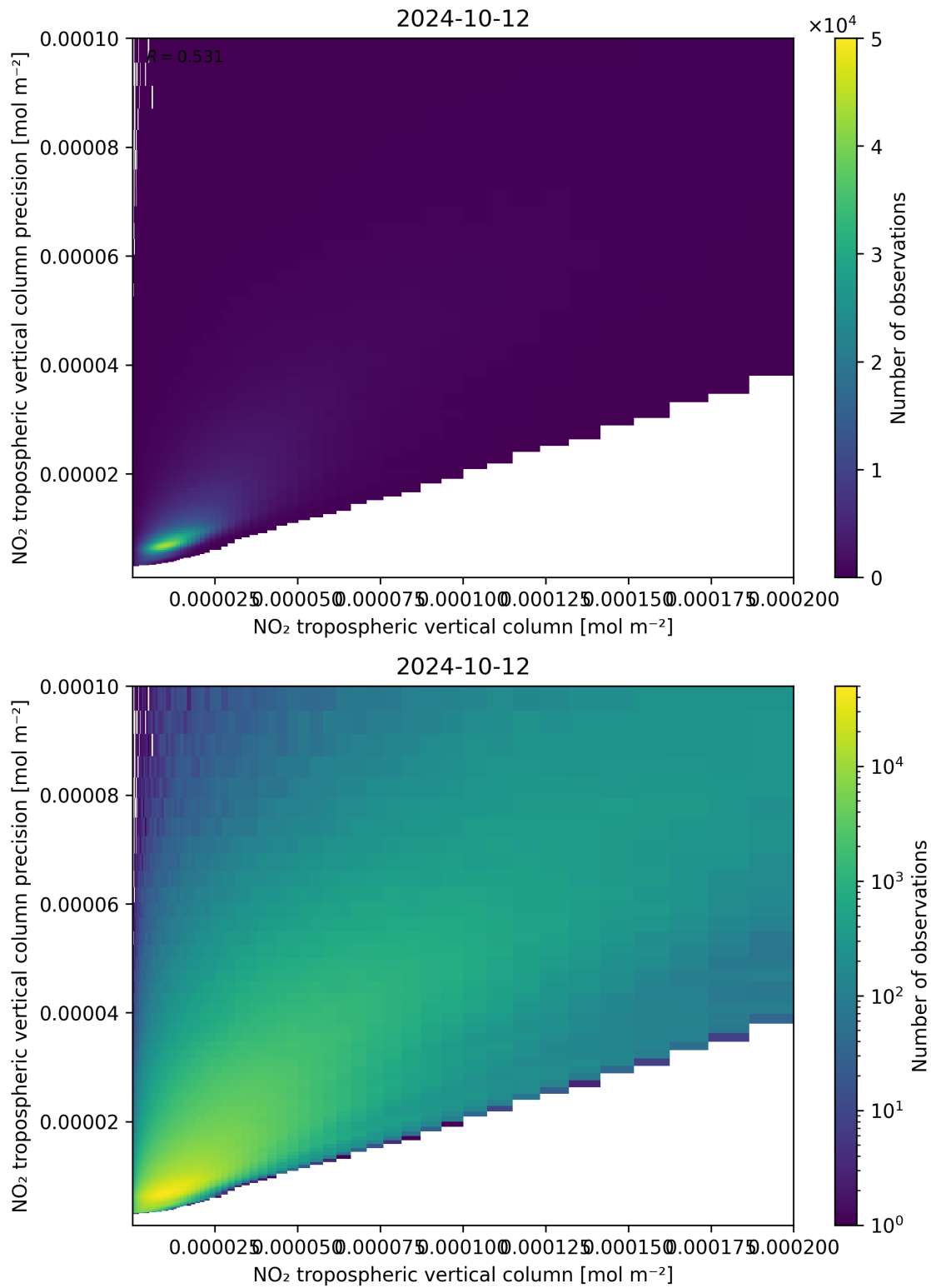
Figure 130: Scatter density plot of “NO 2 tropospheric vertical column” against “NO 2 tropospheric vertical column precision” for 2024-10-11 to 2024-10-13.
