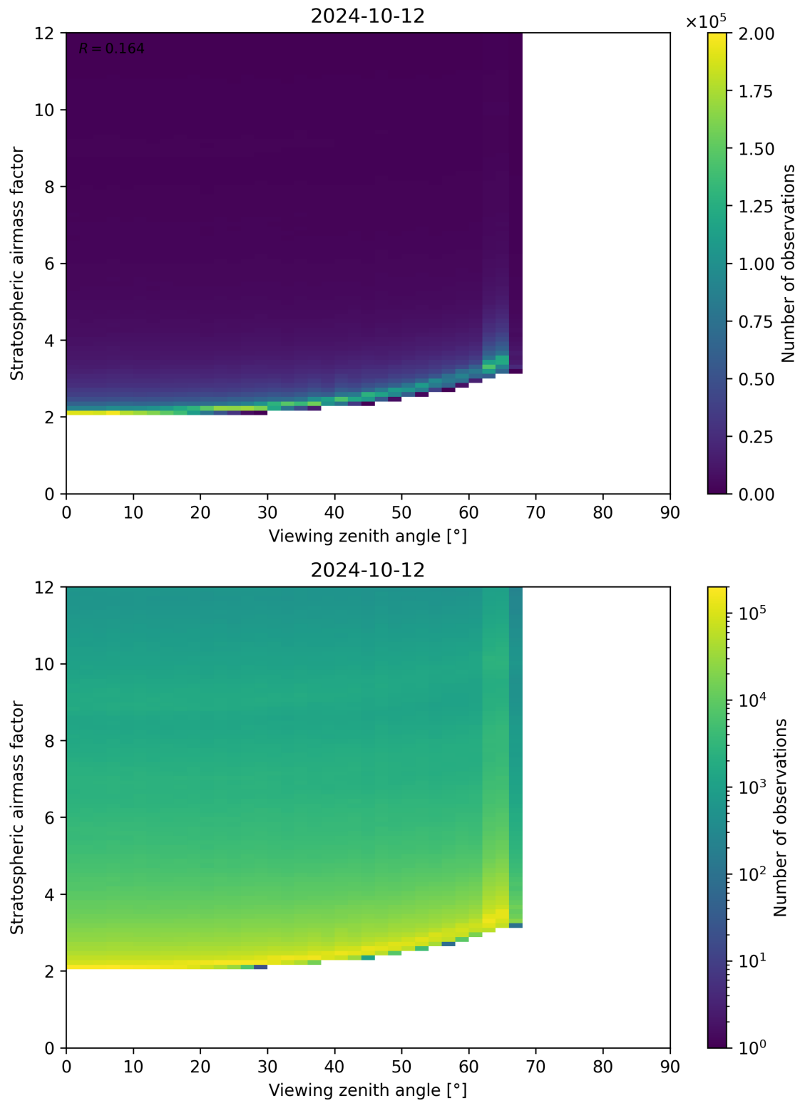
Figure 159: Scatter density plot of “Viewing zenith angle” against “Stratospheric airmass factor” for 2024-10-11 to 2024-10-13.
