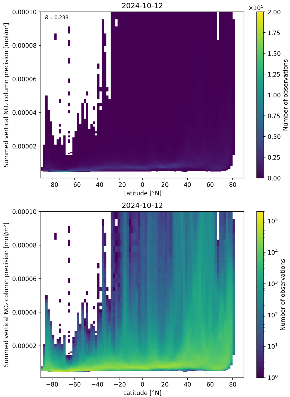
Figure 89: Scatter density plot of “Latitude” against “Summed vertical NO 2 column precision” for 2024-10-11 to 2024-10-13.
