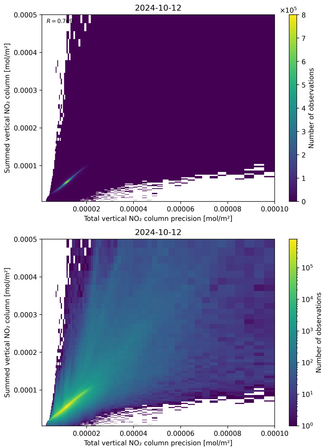
Figure 117: Scatter density plot of “Total vertical NO 2 column precision” against “Summed vertical NO 2 column” for 2024-10-11 to 2024-10-13.
