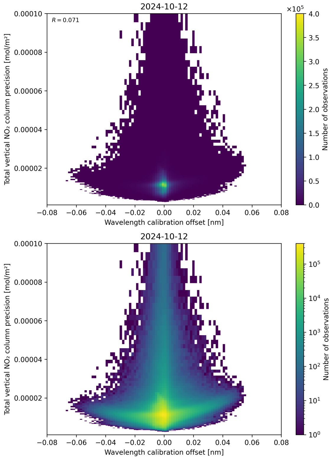
Figure 180: Scatter density plot of “Wavelength calibration offset” against “Total vertical NO 2 column precision” for 2024-10-11 to 2024-10-13.
