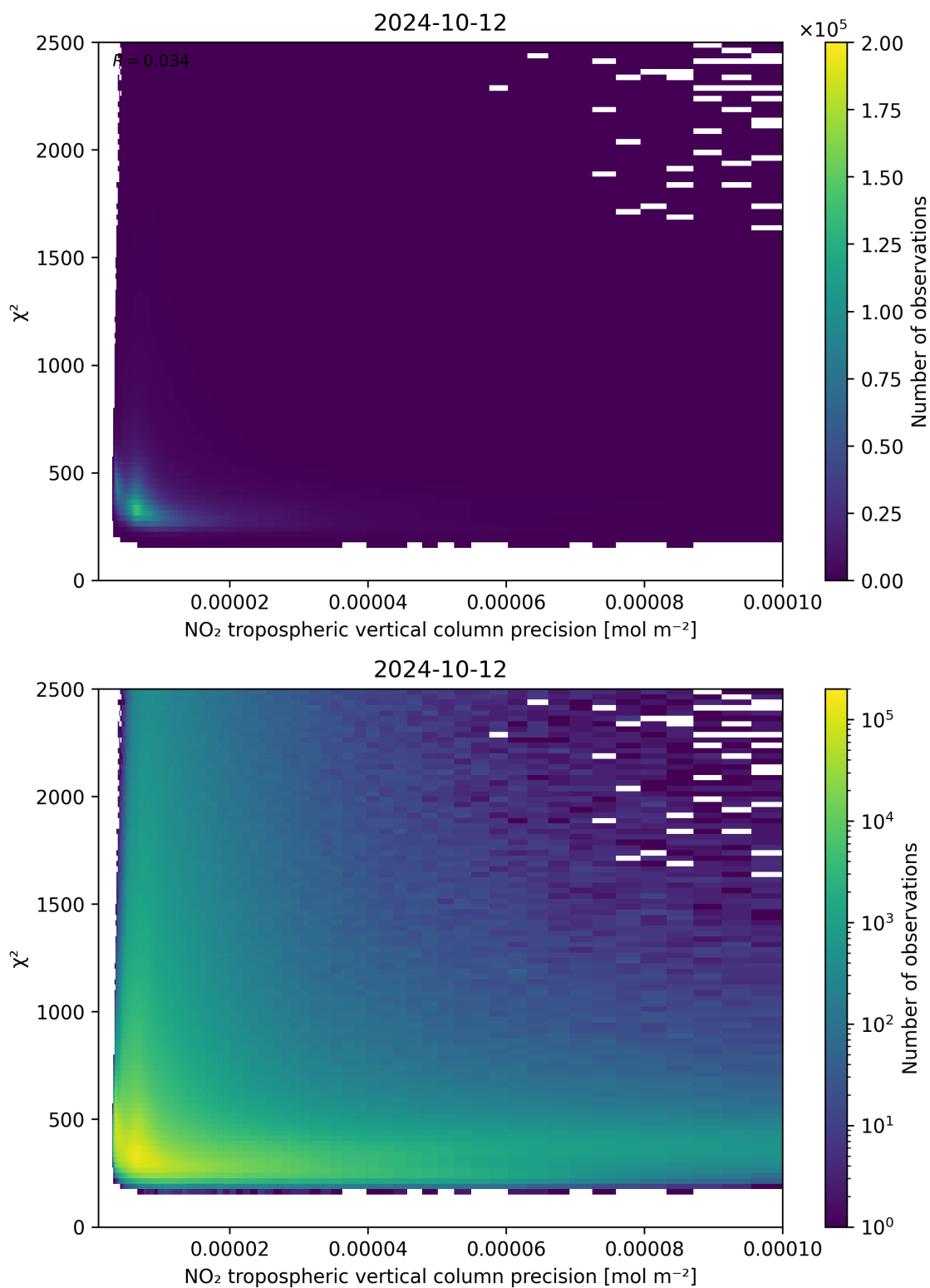
Figure 134: Scatter density plot of “NO 2 tropospheric vertical column precision” against “ \chi^2 ” for 2024-10-11 to 2024-10-13.
