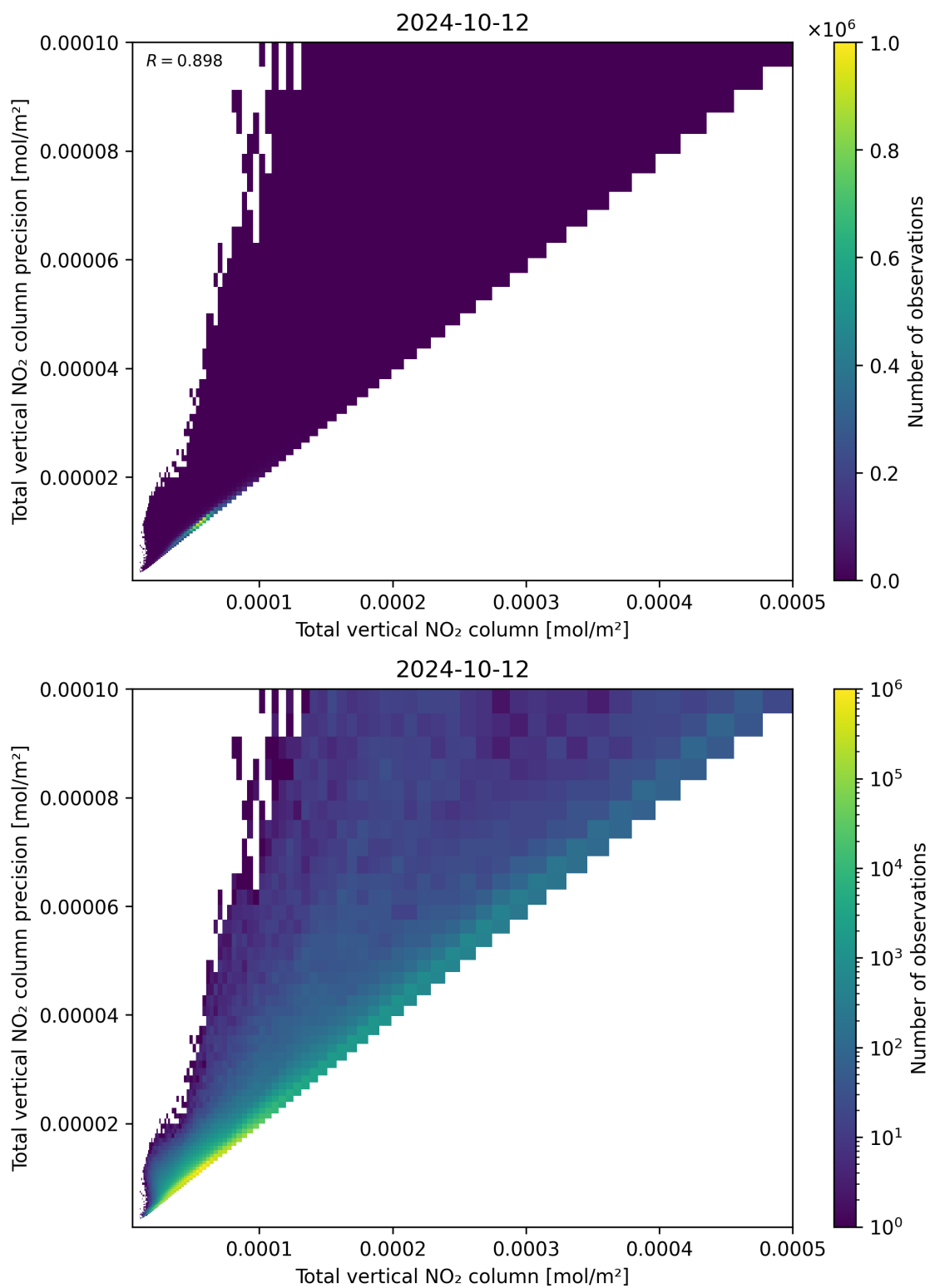
Figure 114: Scatter density plot of “Total vertical NO 2 column” against “Total vertical NO 2 column precision” for 2024-10-11 to 2024-10-13.
