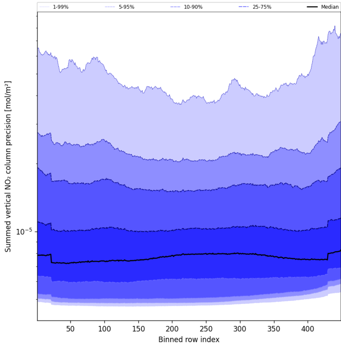
Figure 58: Along track statistics of “Summed vertical NO 2 column precision” for 2024-10-11 to 2024-10-13
