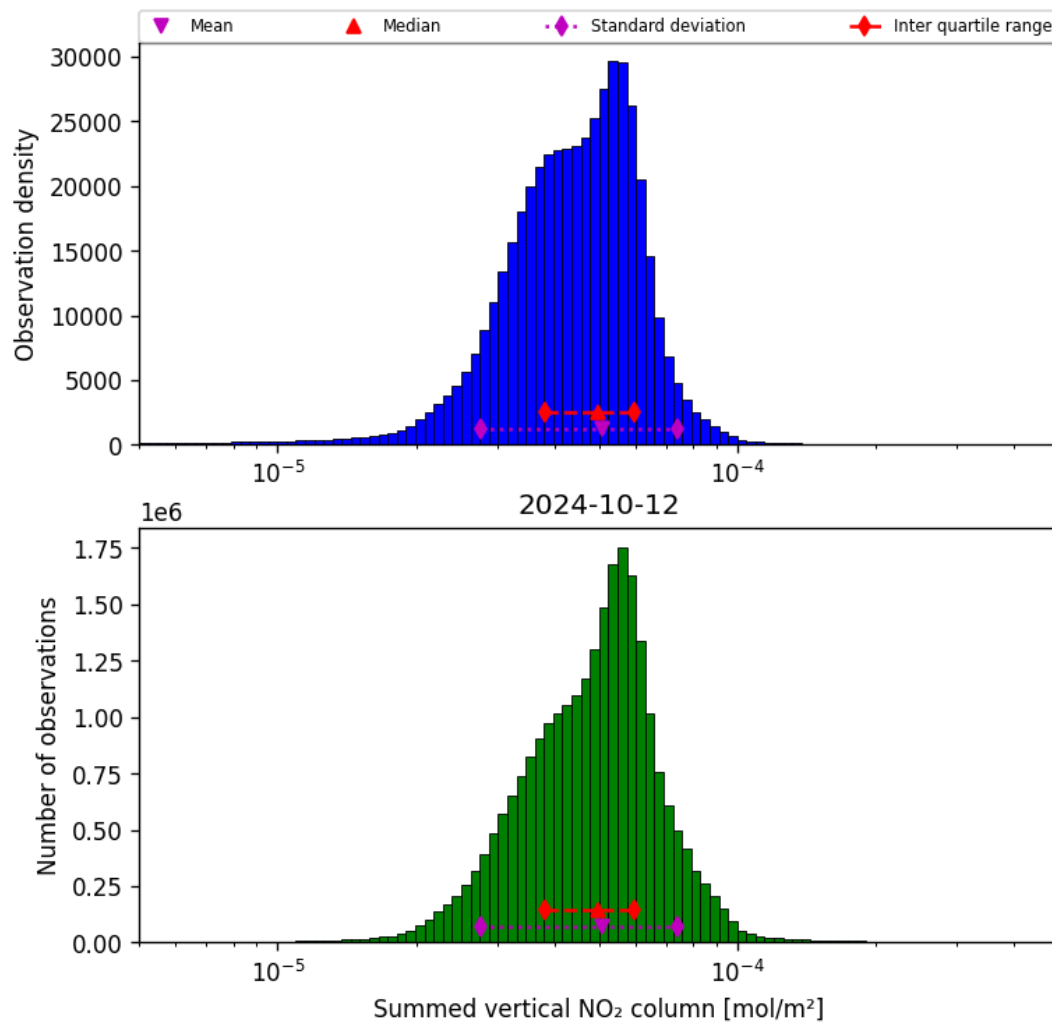
Figure 40: Histogram of “Summed vertical NO 2 column” for 2024-10-11 to 2024-10-13
