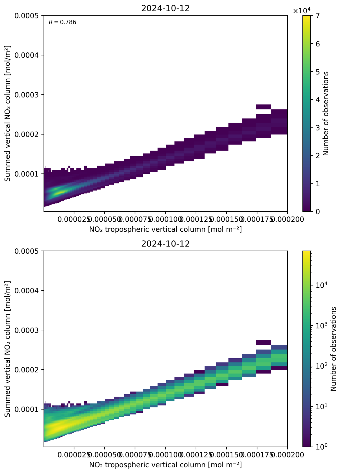
Figure 126: Scatter density plot of “NO 2 tropospheric vertical column” against “Summed vertical NO 2 column” for 2024-10-11 to 2024-10-13.
