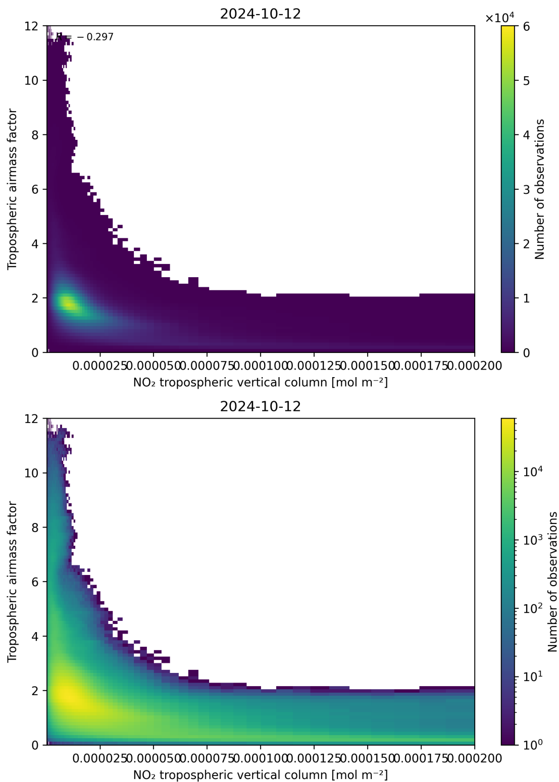
Figure 123: Scatter density plot of “NO 2 tropospheric vertical column” against “Tropospheric air mass factor” for 2024-10-11 to 2024-10-13.
