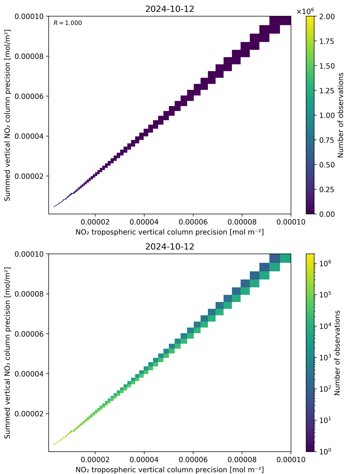
Figure 137: Scatter density plot of “NO 2 tropospheric vertical column precision” against “Summed vertical NO 2 column precision” for 2024-10-11 to 2024-10-13.
