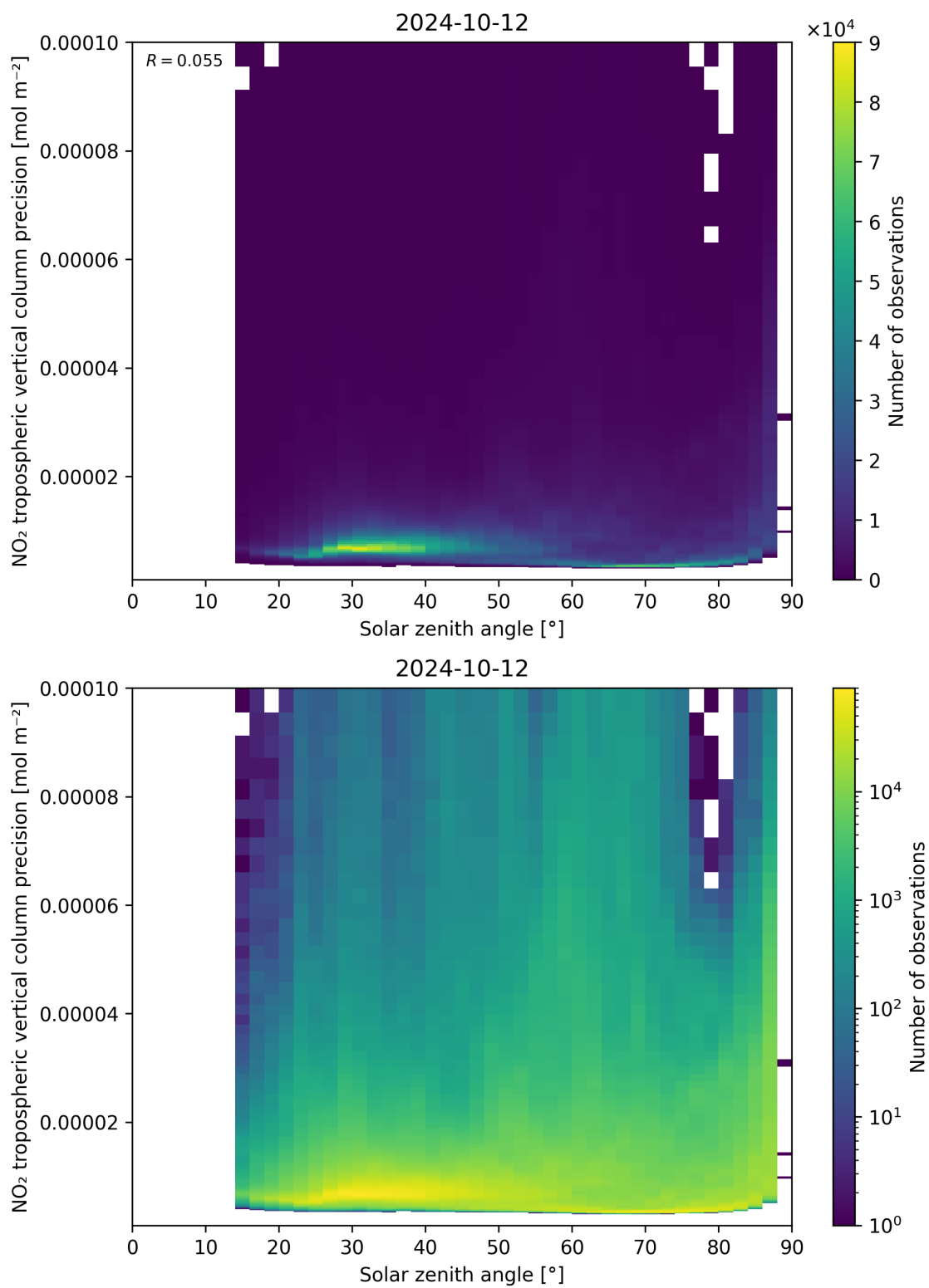
Figure 156: Scatter density plot of “Solar zenith angle” against “NO 2 tropospheric vertical column precision” for 2024-10-11 to 2024-10-13.
