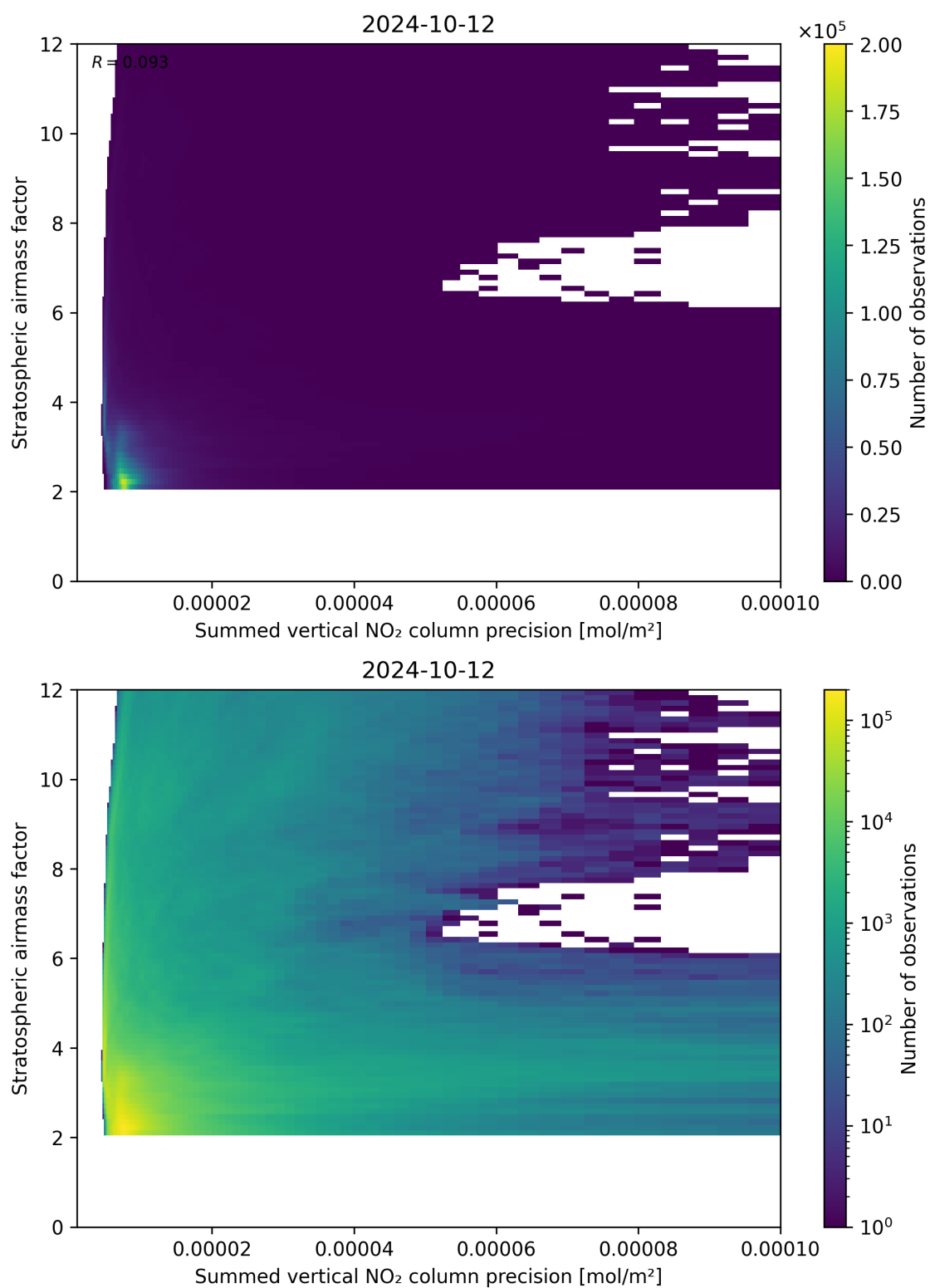
Figure 106: Scatter density plot of “Summed vertical NO 2 column precision” against “Stratospheric airmass factor” for 2024-10-11 to 2024-10-13.
