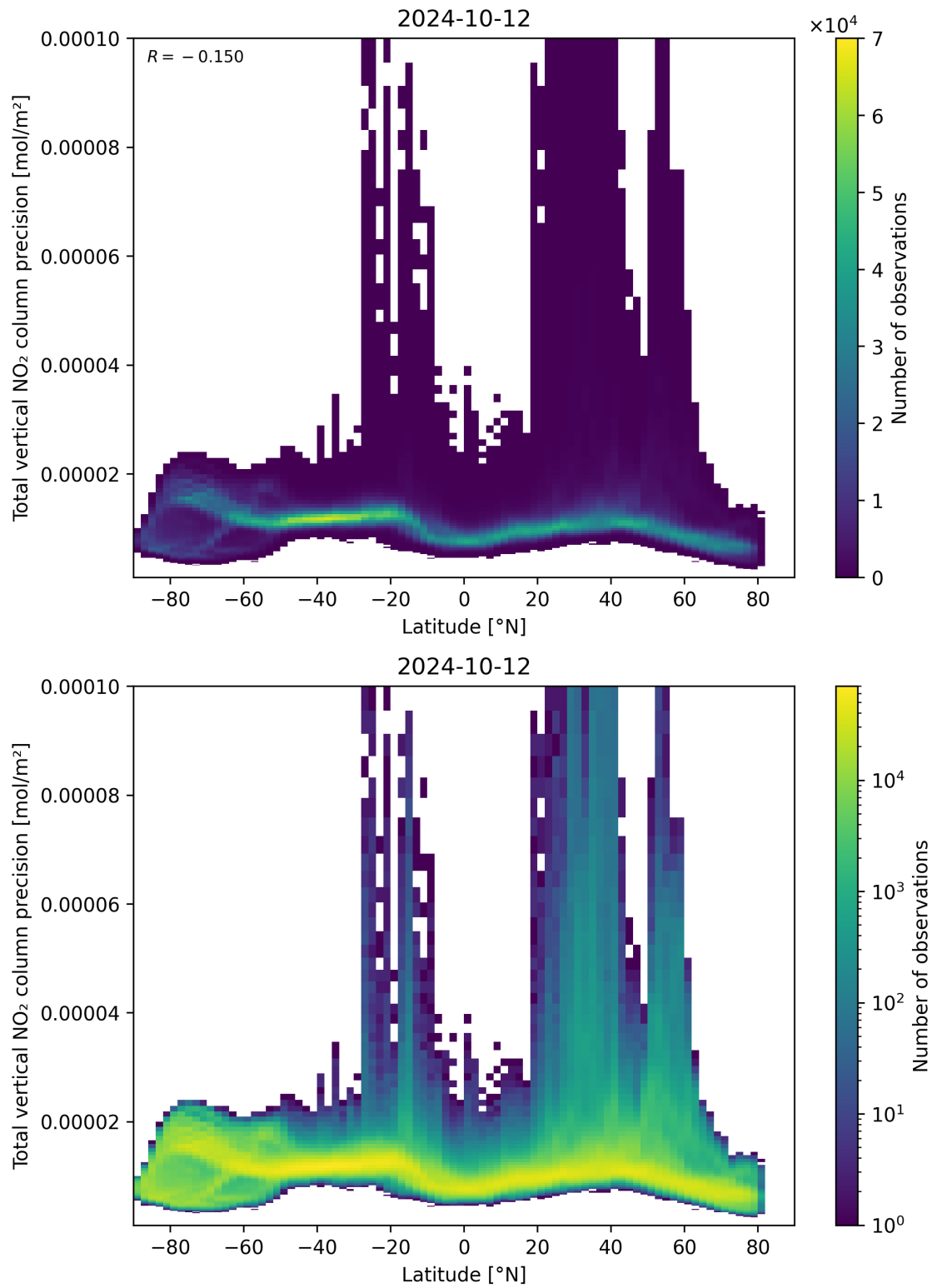
Figure 91: Scatter density plot of “Latitude” against “Total vertical NO 2 column precision” for 2024-10-11 to 2024-10-13.
