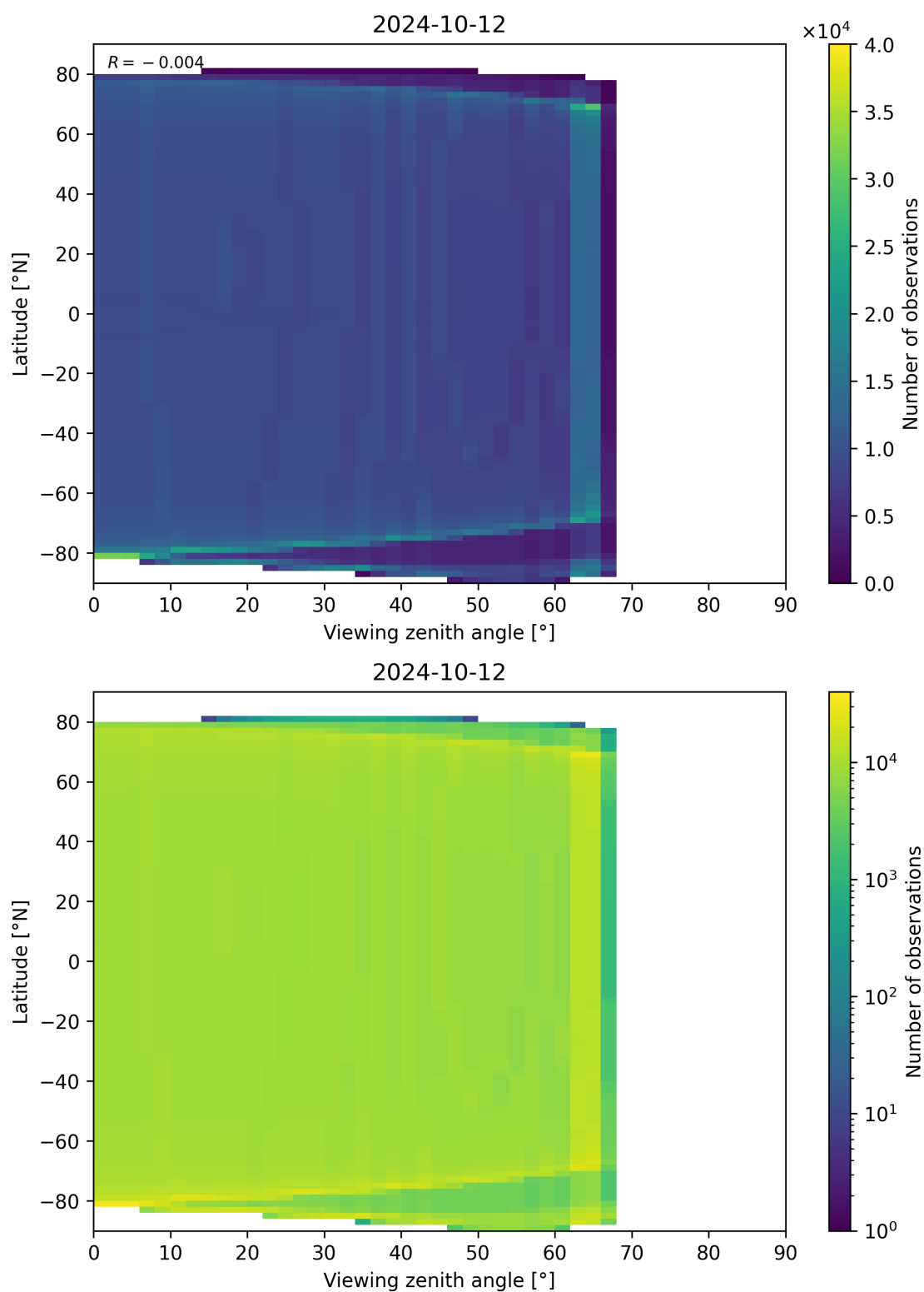
Figure 163: Scatter density plot of “Viewing zenith angle” against “Latitude” for 2024-10-11 to 2024-10-13.
