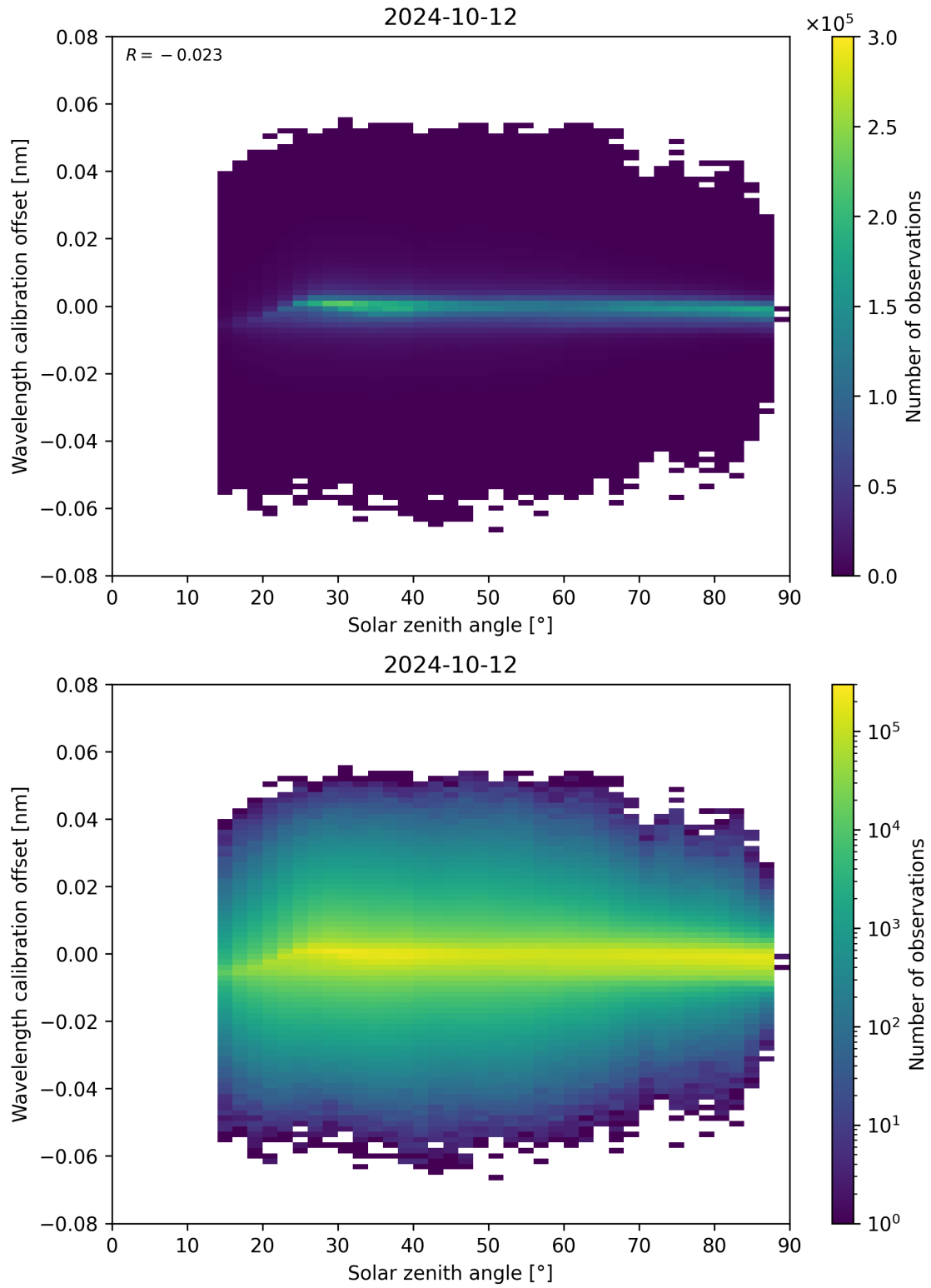
Figure 158: Scatter density plot of “Solar zenith angle” against “Wavelength calibration offset” for 2024-10-11 to 2024-10-13.
