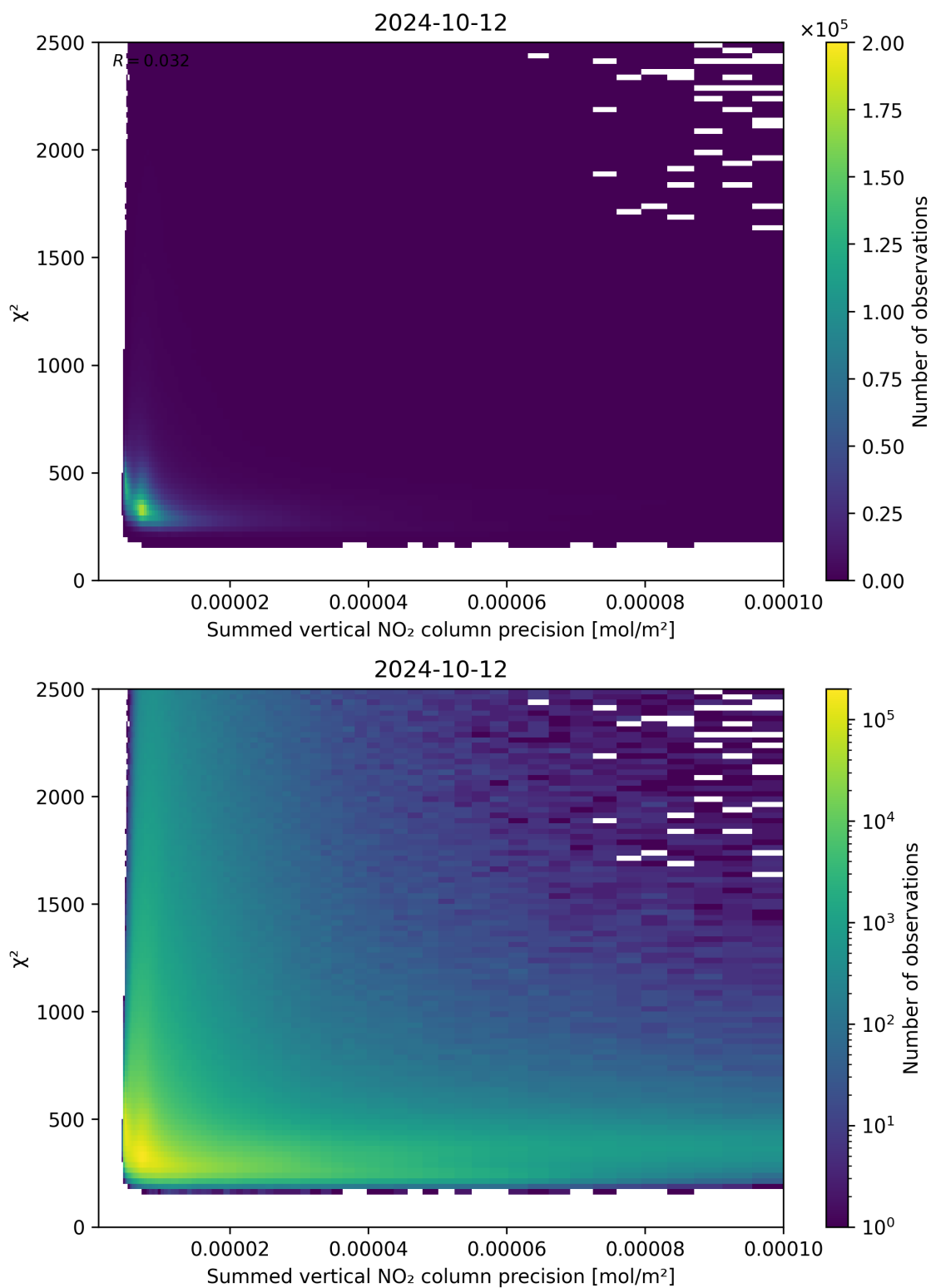
Figure 107: Scatter density plot of “Summed vertical NO 2 column precision” against “ \chi^2 ” for 2024-10-11 to 2024-10-13.
