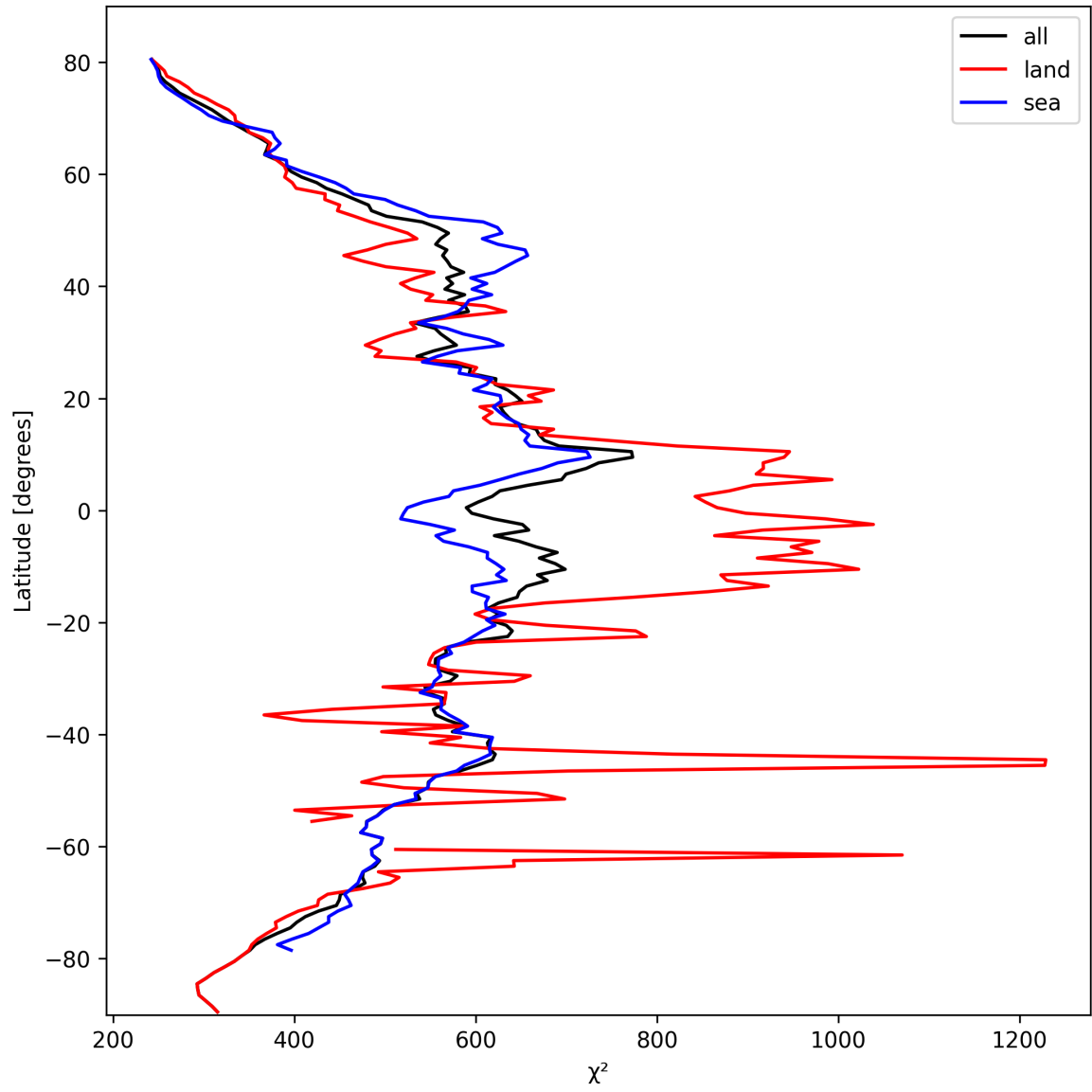
Figure 25: Zonal average of “ \chi^2 ” for 2024-10-11 to 2024-10-13.
