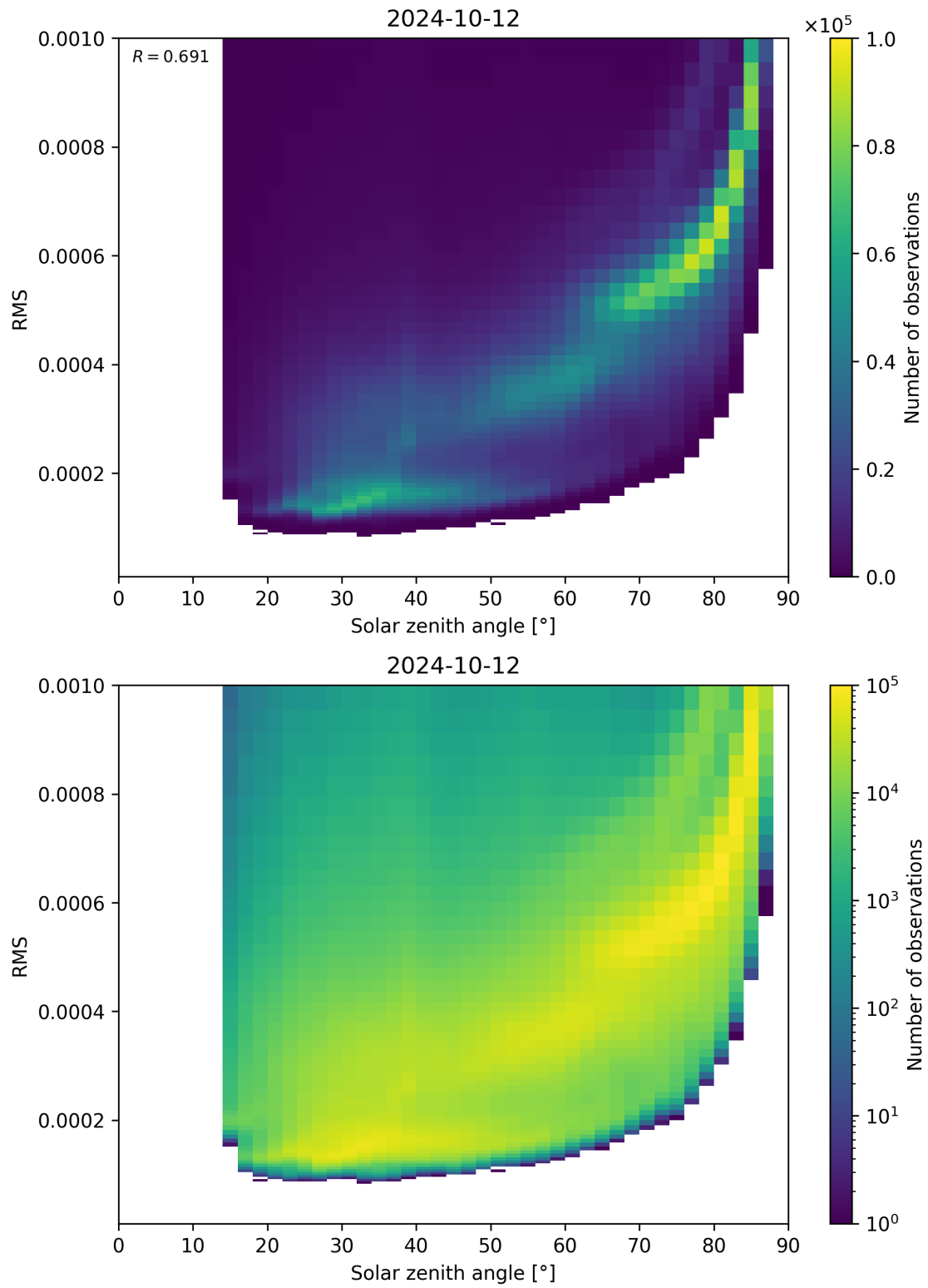
Figure 157: Scatter density plot of “Solar zenith angle” against “RMS” for 2024-10-11 to 2024-10-13.
