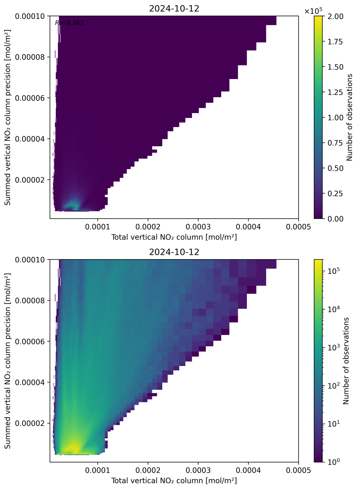
Figure 113: Scatter density plot of “Total vertical NO 2 column” against “Summed vertical NO 2 column precision” for 2024-10-11 to 2024-10-13.
