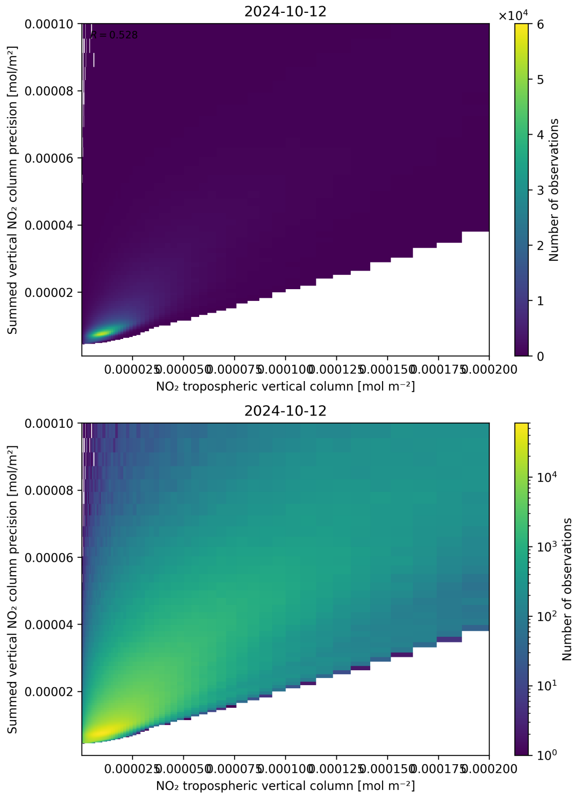
Figure 127: Scatter density plot of “NO 2 tropospheric vertical column” against “Summed vertical NO 2 column precision” for 2024-10-11 to 2024-10-13.
