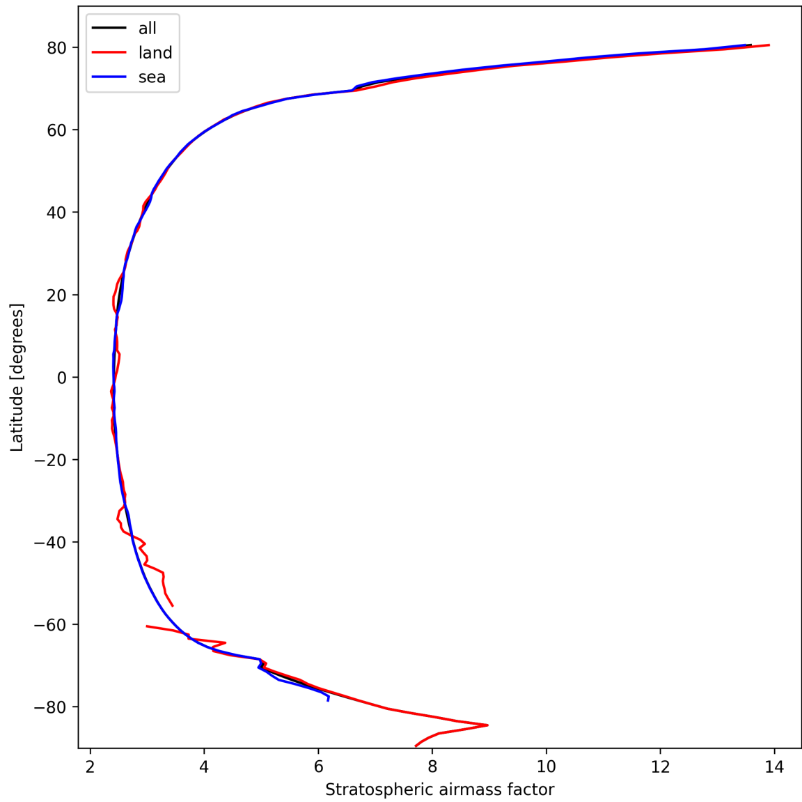
Figure 27: Zonal average of “Stratospheric air mass factor” for 2024-10-11 to 2024-10-13.
