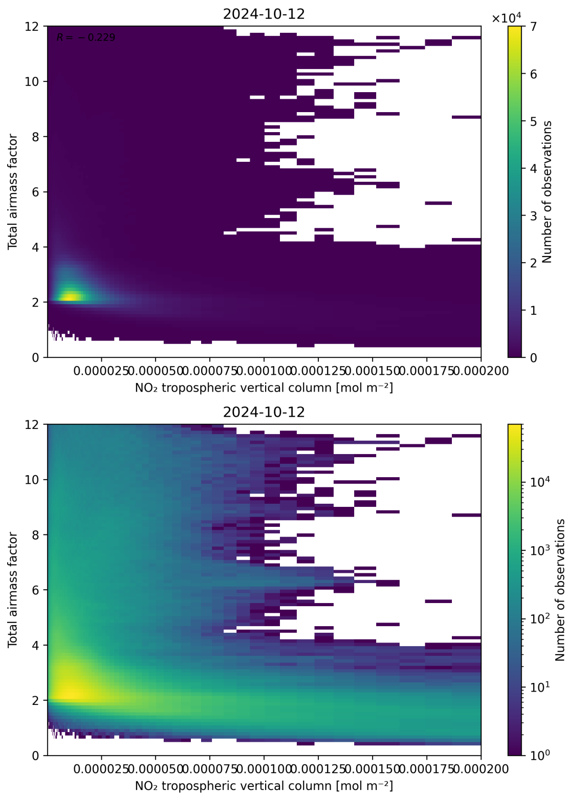
Figure 122: Scatter density plot of “NO 2 tropospheric vertical column” against “Total air mass factor” for 2024-10-11 to 2024-10-13.
