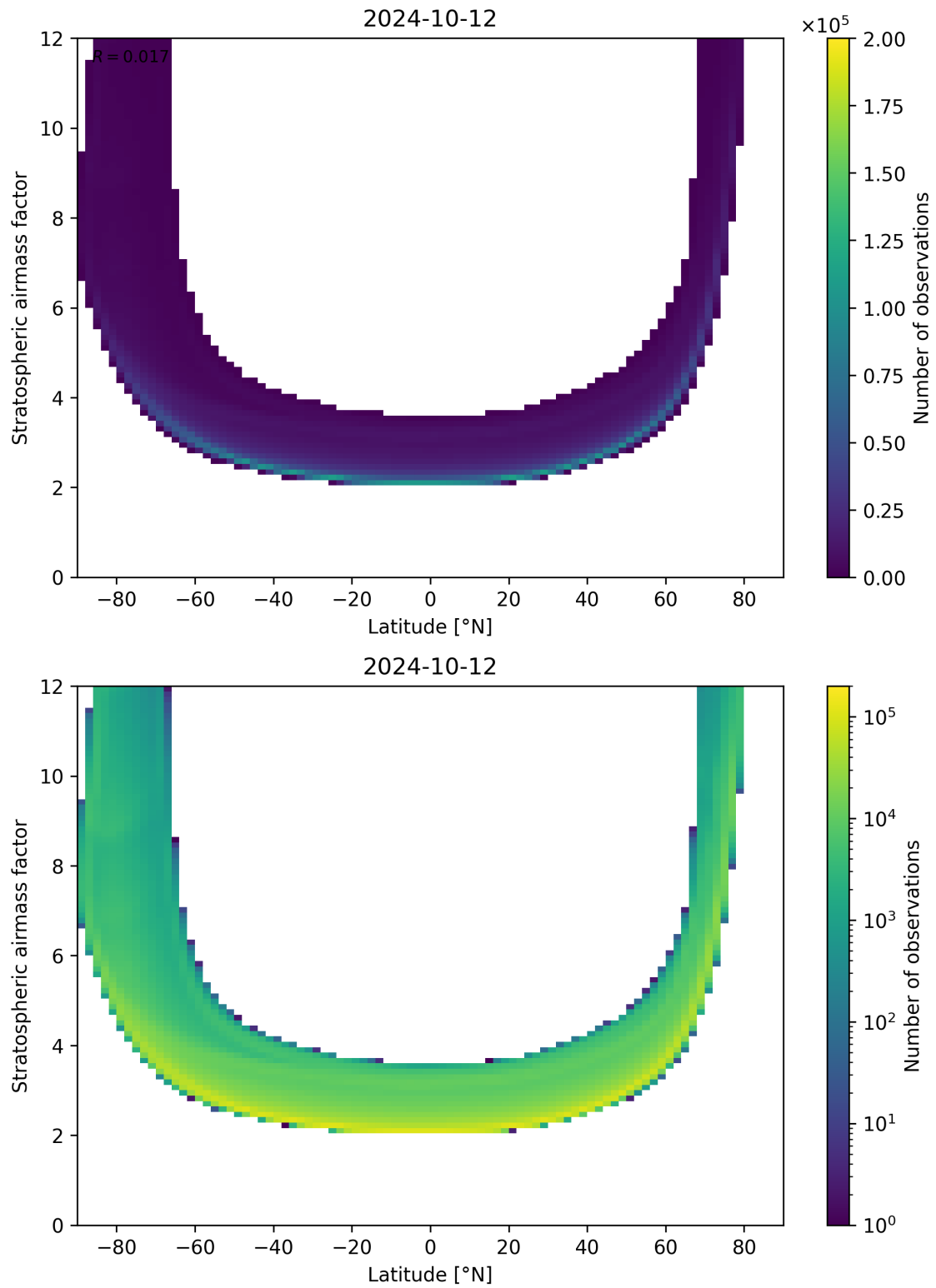
Figure 83: Scatter density plot of “Latitude” against “Stratospheric airmass factor” for 2024-10-11 to 2024-10-13.
