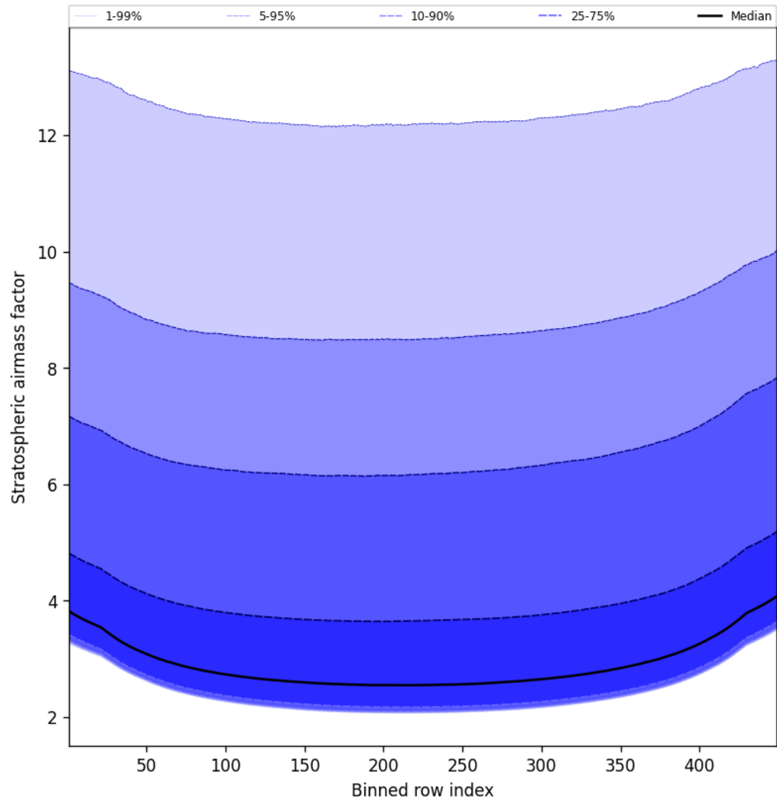
Figure 61: Along track statistics of “Stratospheric airmass factor” for 2024-10-11 to 2024-10-13
