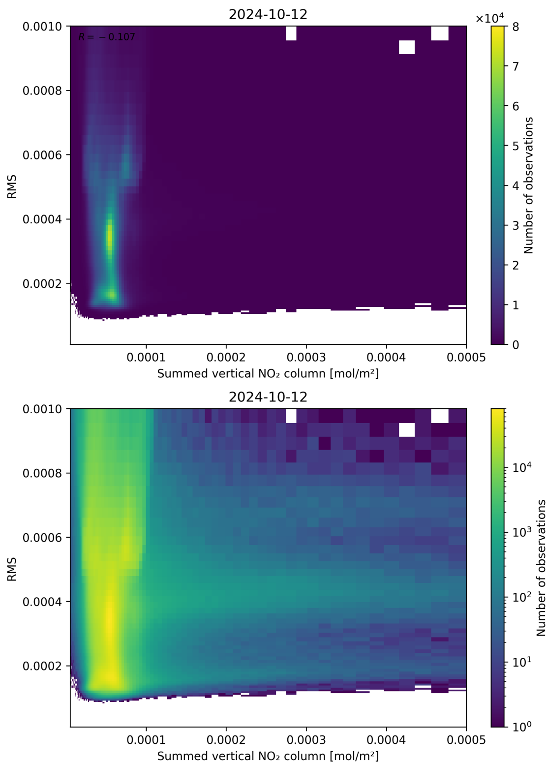
Figure 109: Scatter density plot of “Summed vertical NO 2 column” against “RMS” for 2024-10-11 to 2024-10-13.
