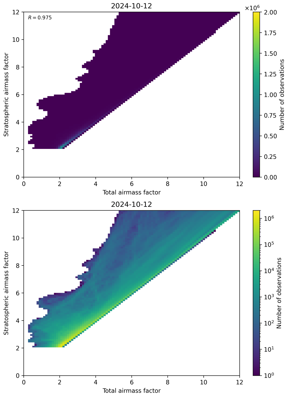
Figure 62: Scatter density plot of “Total airmass factor” against “Stratospheric airmass factor” for 2024-10-11 to 2024-10-13.
