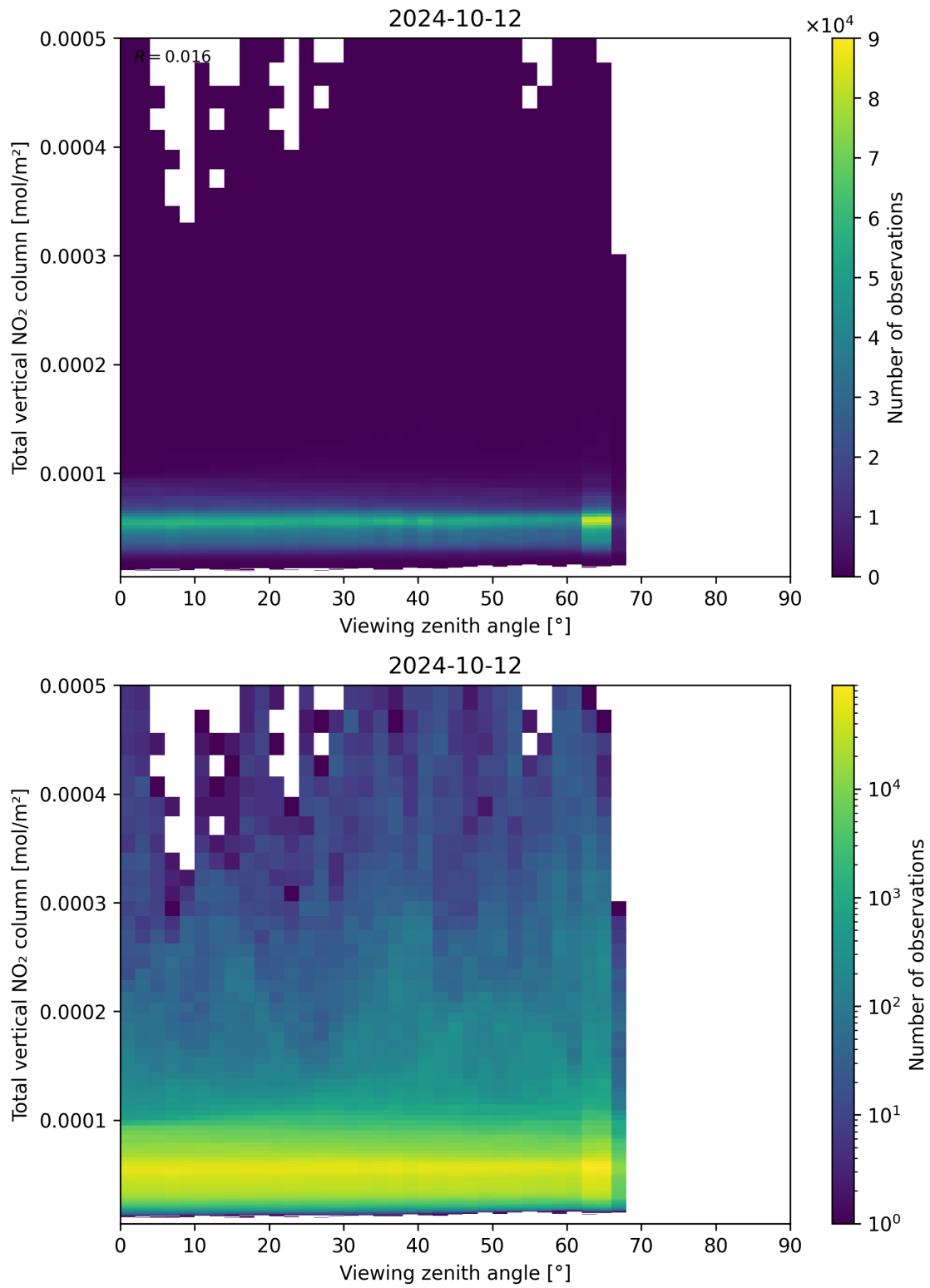
Figure 167: Scatter density plot of “Viewing zenith angle” against “Total vertical NO 2 column” for 2024-10-11 to 2024-10-13.
