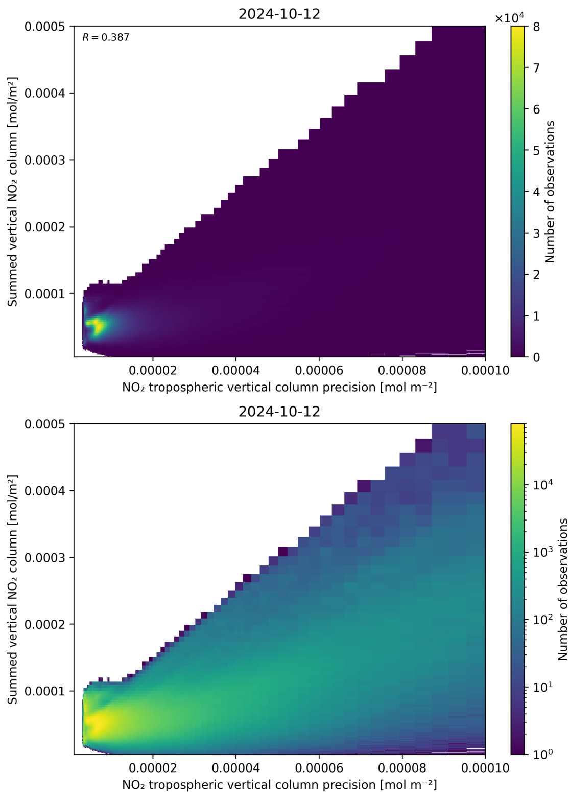
Figure 136: Scatter density plot of “NO 2 tropospheric vertical column precision” against “Summed vertical NO 2 column” for 2024-10-11 to 2024-10-13.
