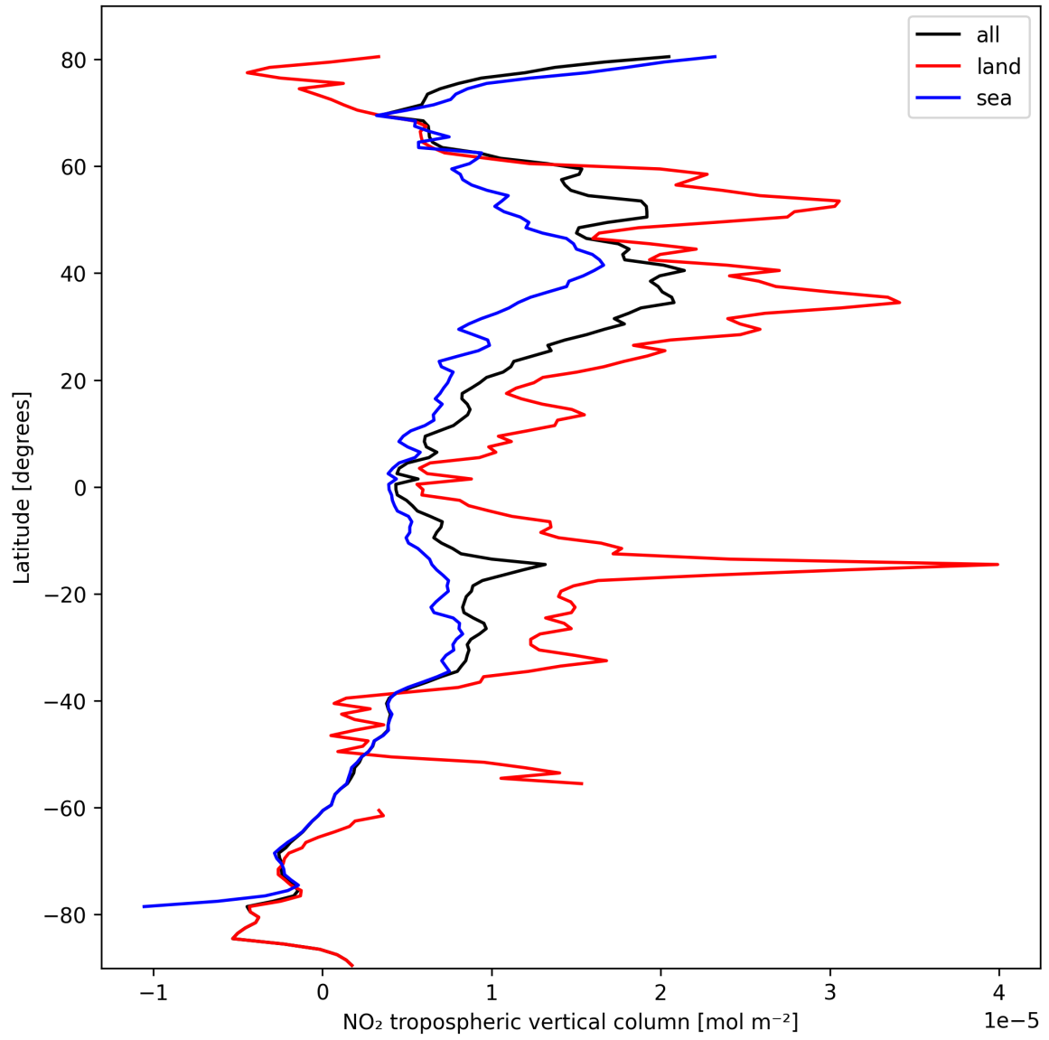
Figure 12: Zonal average of “NO 2 tropospheric vertical column” for 2024-10-11 to 2024-10-13.
