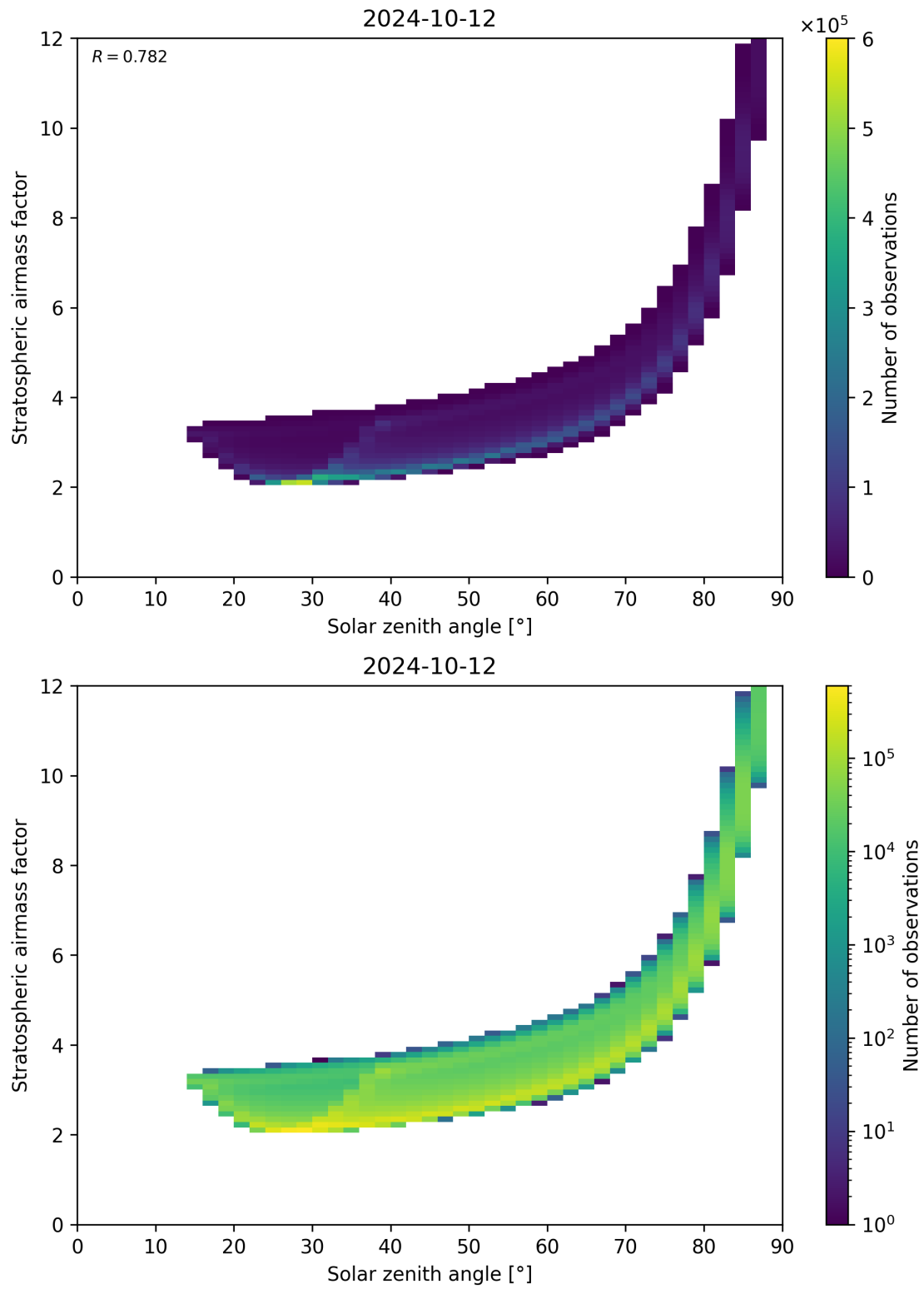
Figure 145: Scatter density plot of “Solar zenith angle” against “Stratospheric airmass factor” for 2024-10-11 to 2024-10-13.
