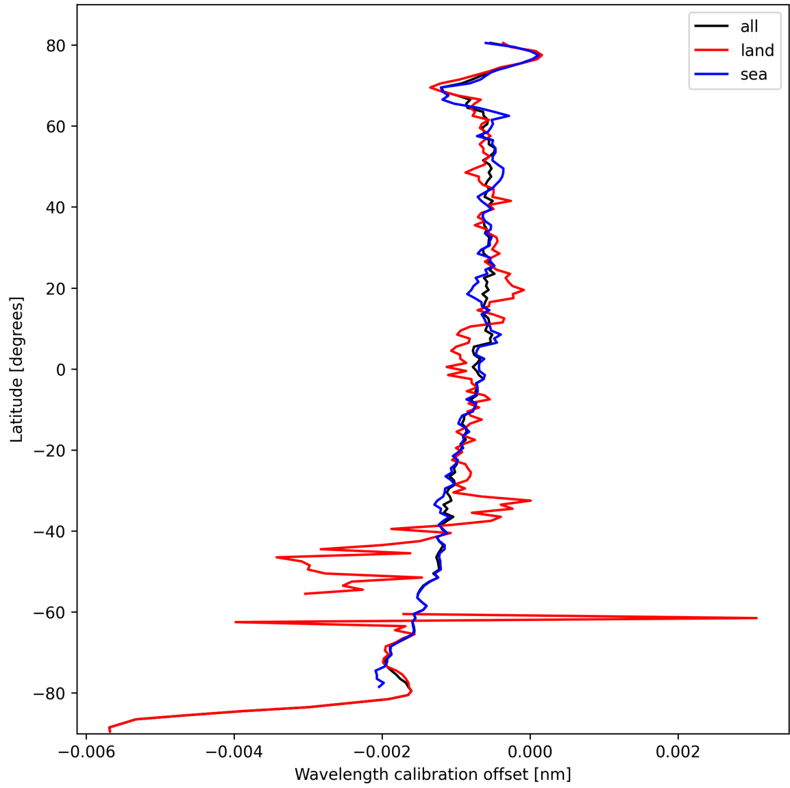
Figure 18: Zonal average of “Wavelength calibration offset” for 2024-10-11 to 2024-10-13.
