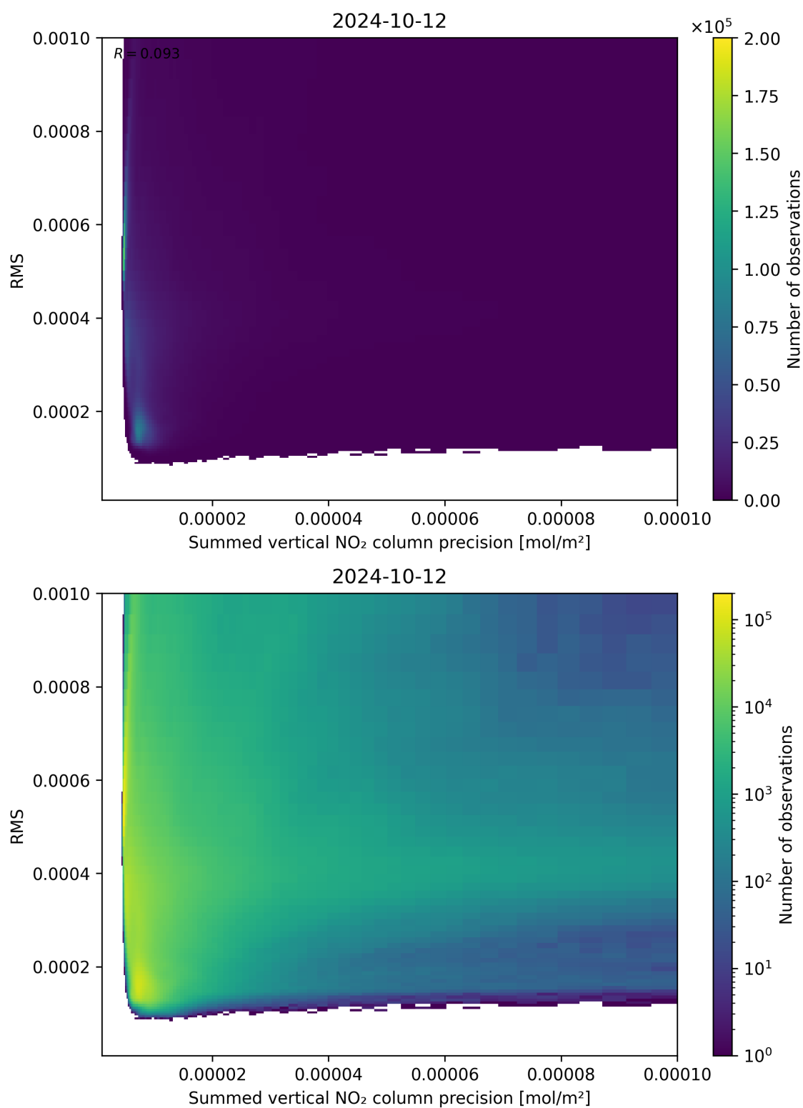
Figure 108: Scatter density plot of “Summed vertical NO 2 column precision” against “RMS” for 2024-10-11 to 2024-10-13.
