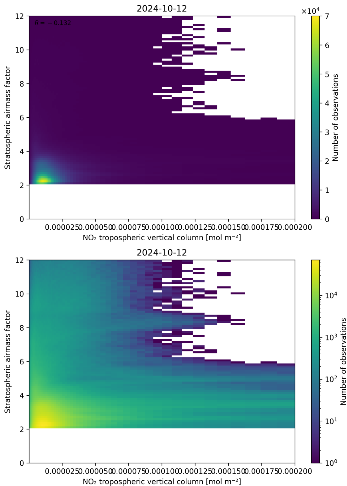
Figure 121: Scatter density plot of “NO 2 tropospheric vertical column” against “Stratospheric airmass factor” for 2024-10-11 to 2024-10-13.
