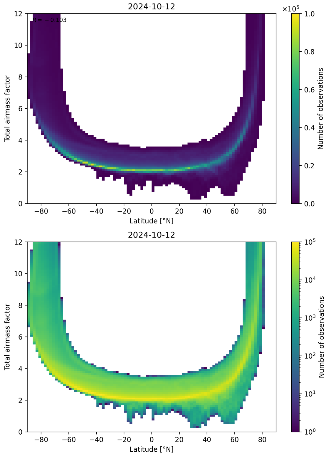
Figure 84: Scatter density plot of “Latitude” against “Total airmass factor” for 2024-10-11 to 2024-10-13.
