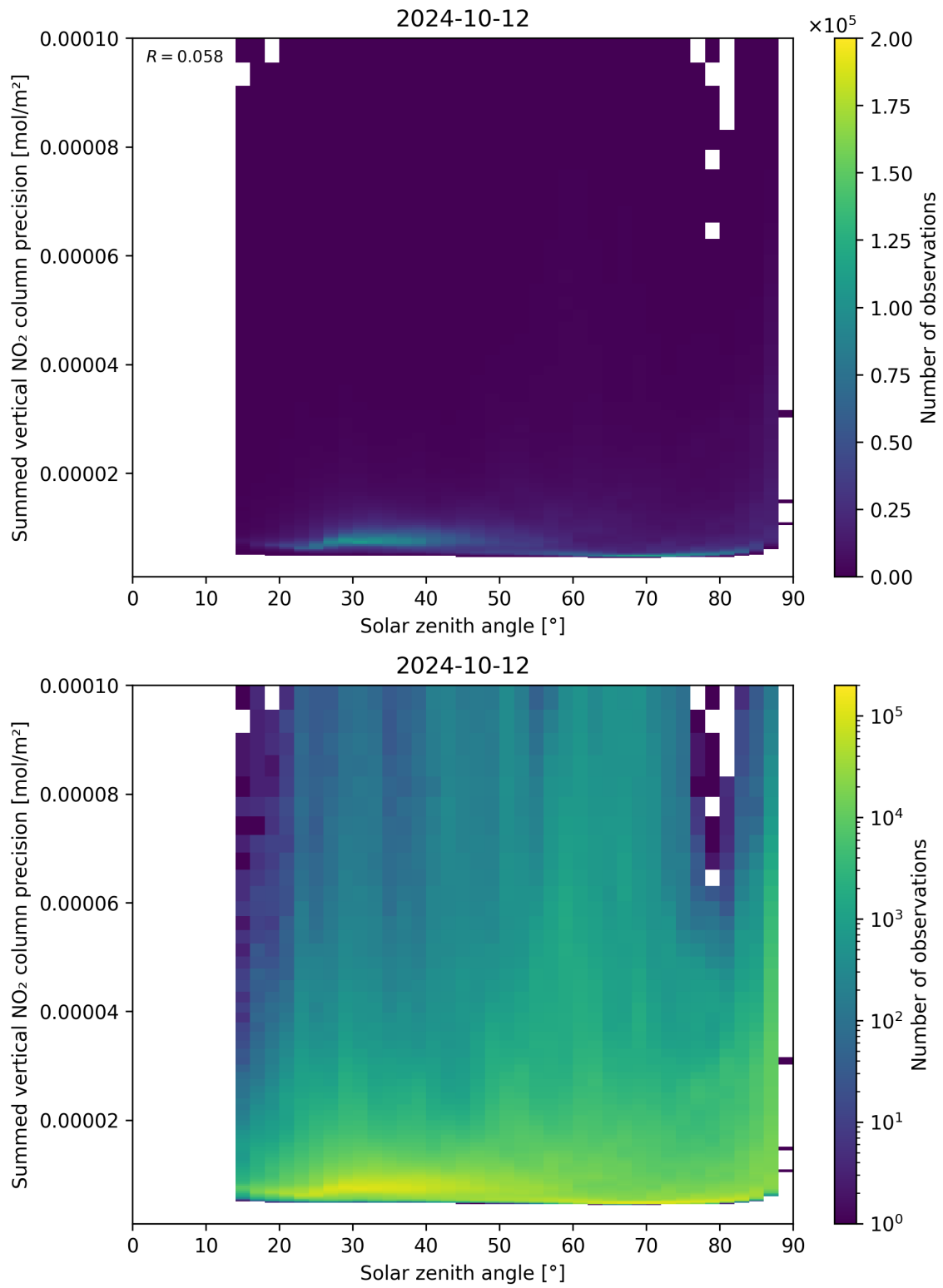
Figure 152: Scatter density plot of “Solar zenith angle” against “Summed vertical NO 2 column precision” for 2024-10-11 to 2024-10-13.
