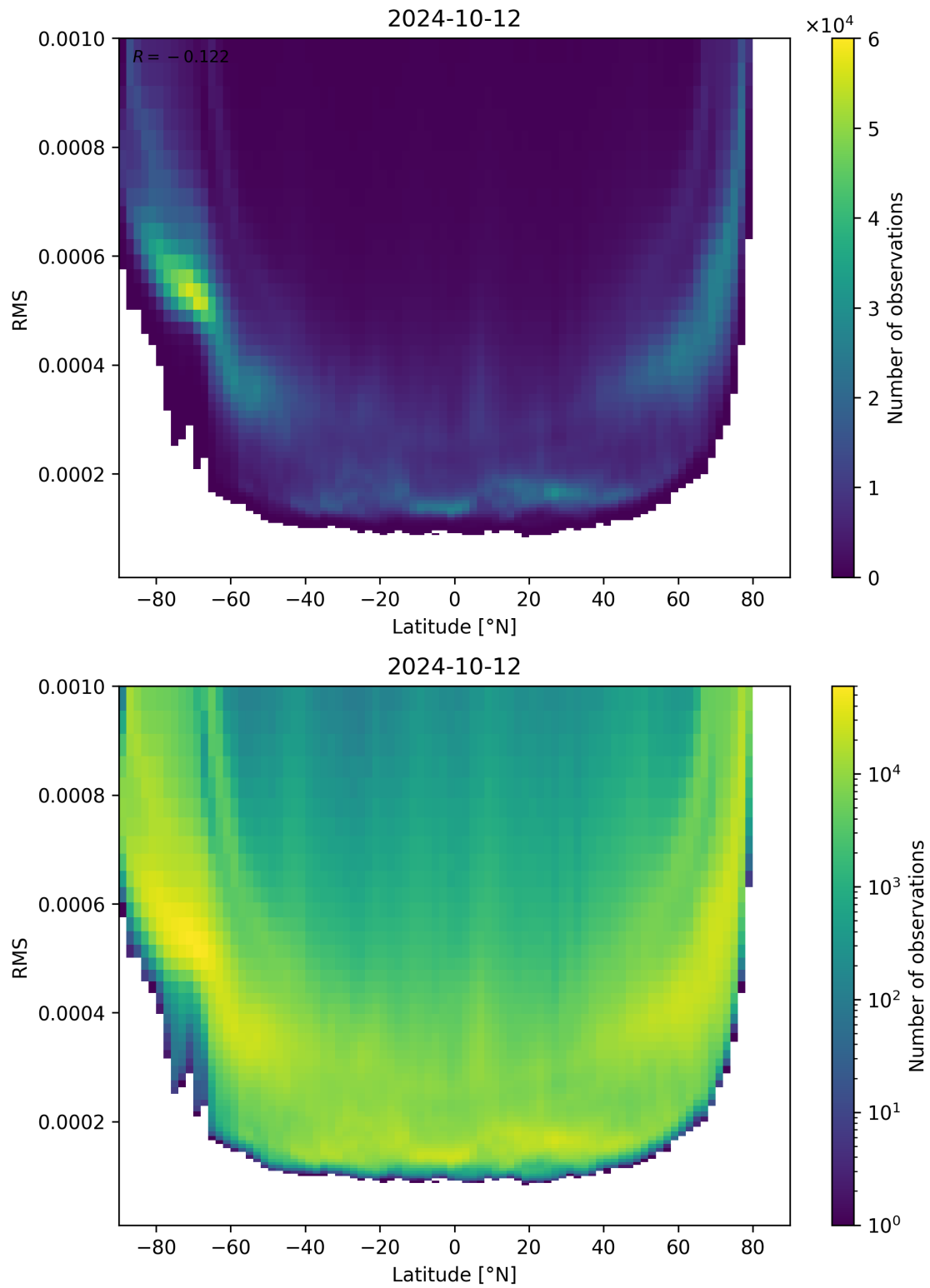
Figure 94: Scatter density plot of “Latitude” against “RMS” for 2024-10-11 to 2024-10-13.
