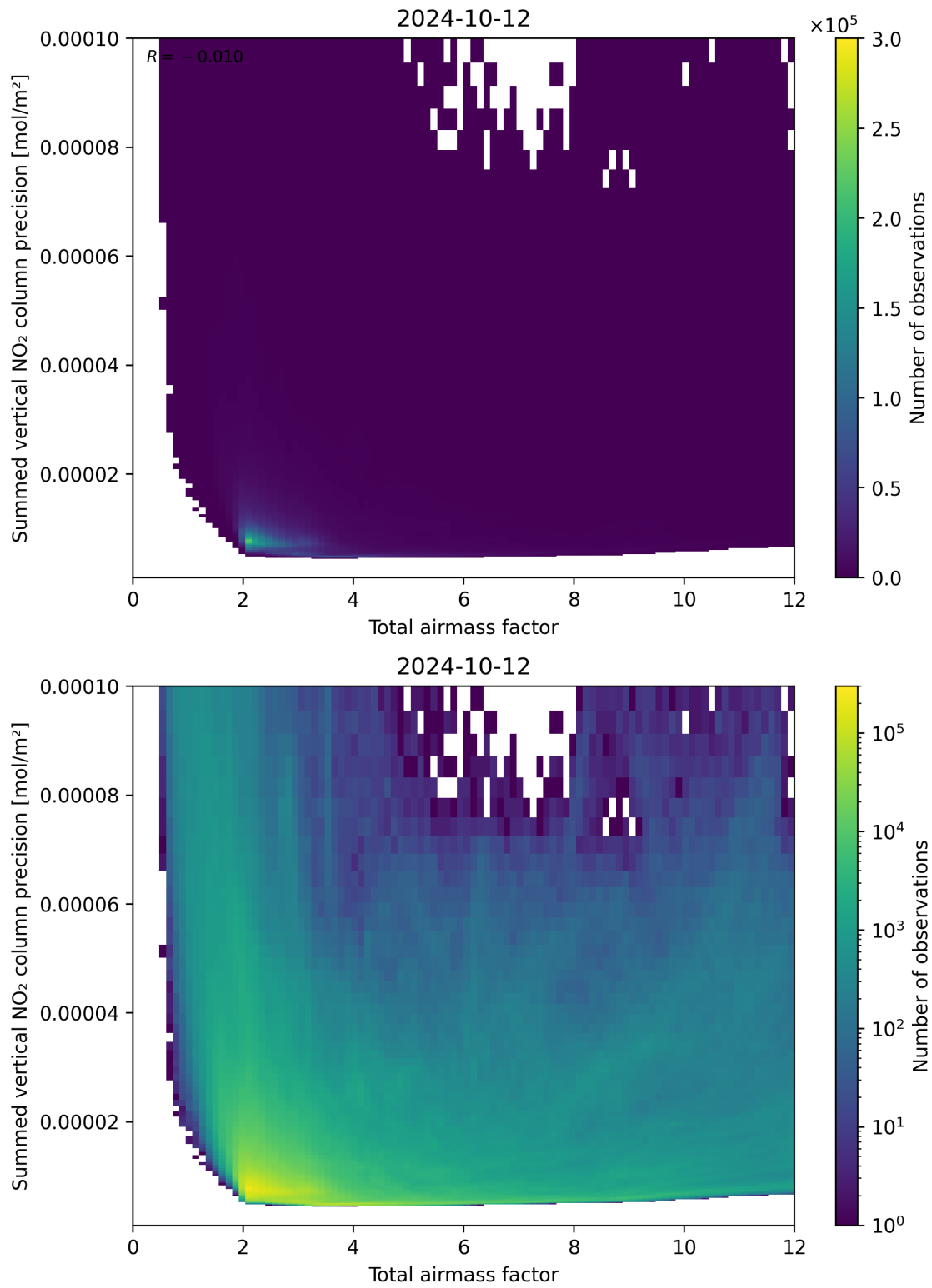
Figure 66: Scatter density plot of “Total airmass factor” against “Summed vertical NO 2 column precision” for 2024-10-11 to 2024-10-13.
