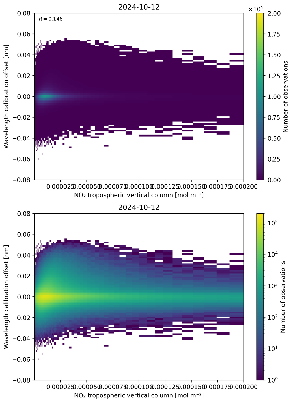
Figure 143: Scatter density plot of “NO 2 tropospheric vertical column” against “Wavelength calibration offset” for 2024-10-11 to 2024-10-13.
