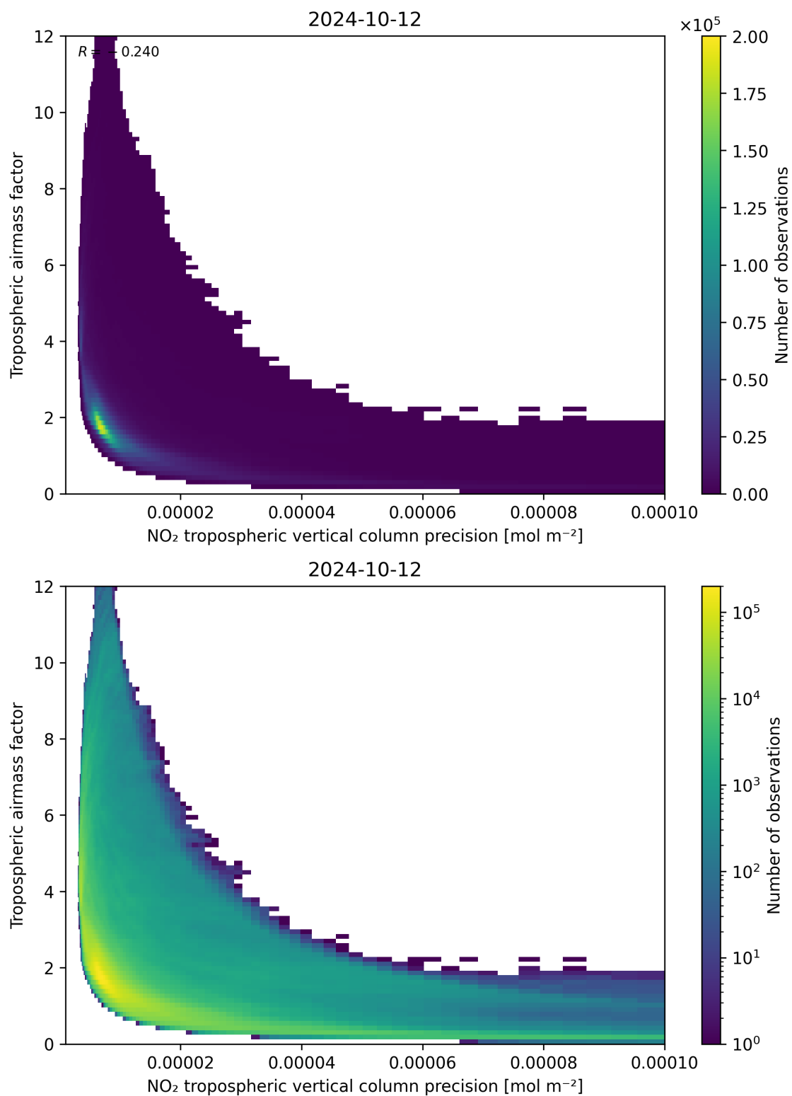
Figure 133: Scatter density plot of “NO 2 tropospheric vertical column precision” against “Tropospheric airmass factor” for 2024-10-11 to 2024-10-13.
