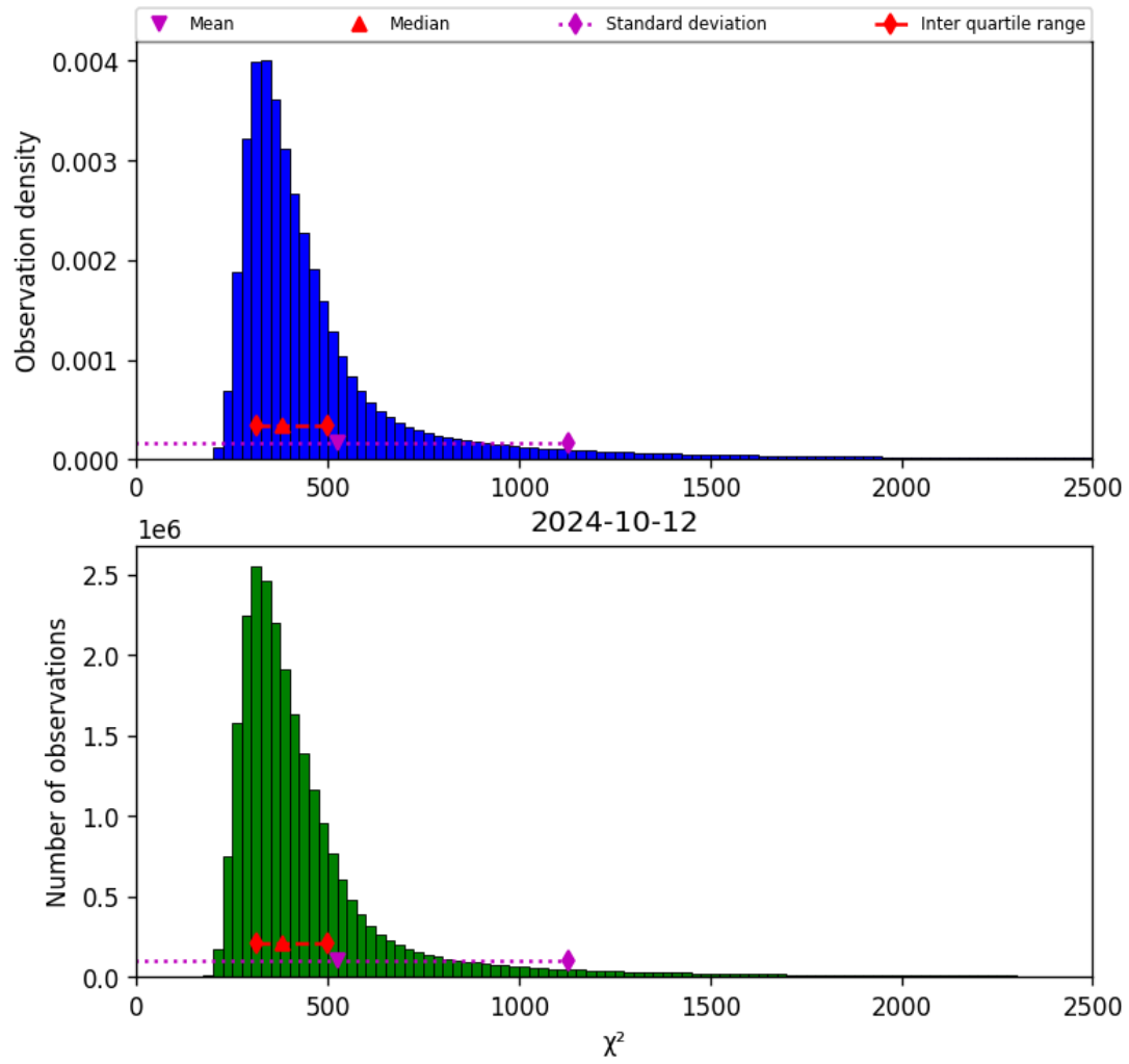
Figure 42: Histogram of “ \chi^2 ” for 2024-10-11 to 2024-10-13
