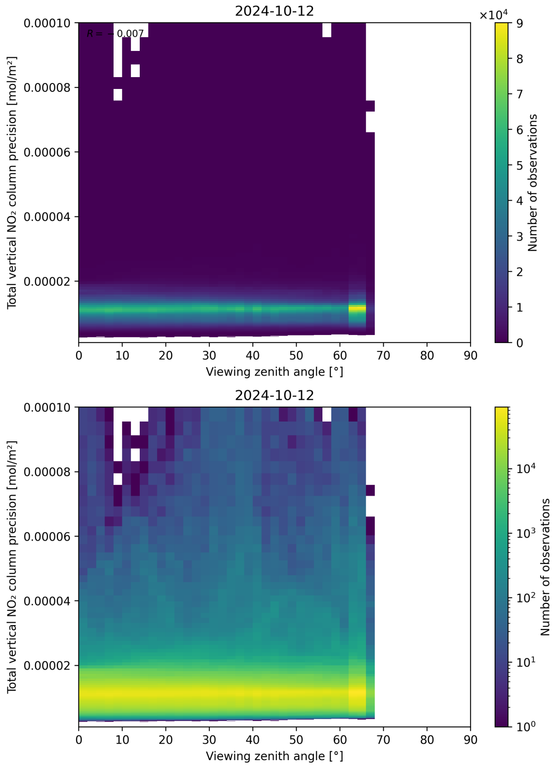
Figure 168: Scatter density plot of “Viewing zenith angle” against “Total vertical NO 2 column precision” for 2024-10-11 to 2024-10-13.
