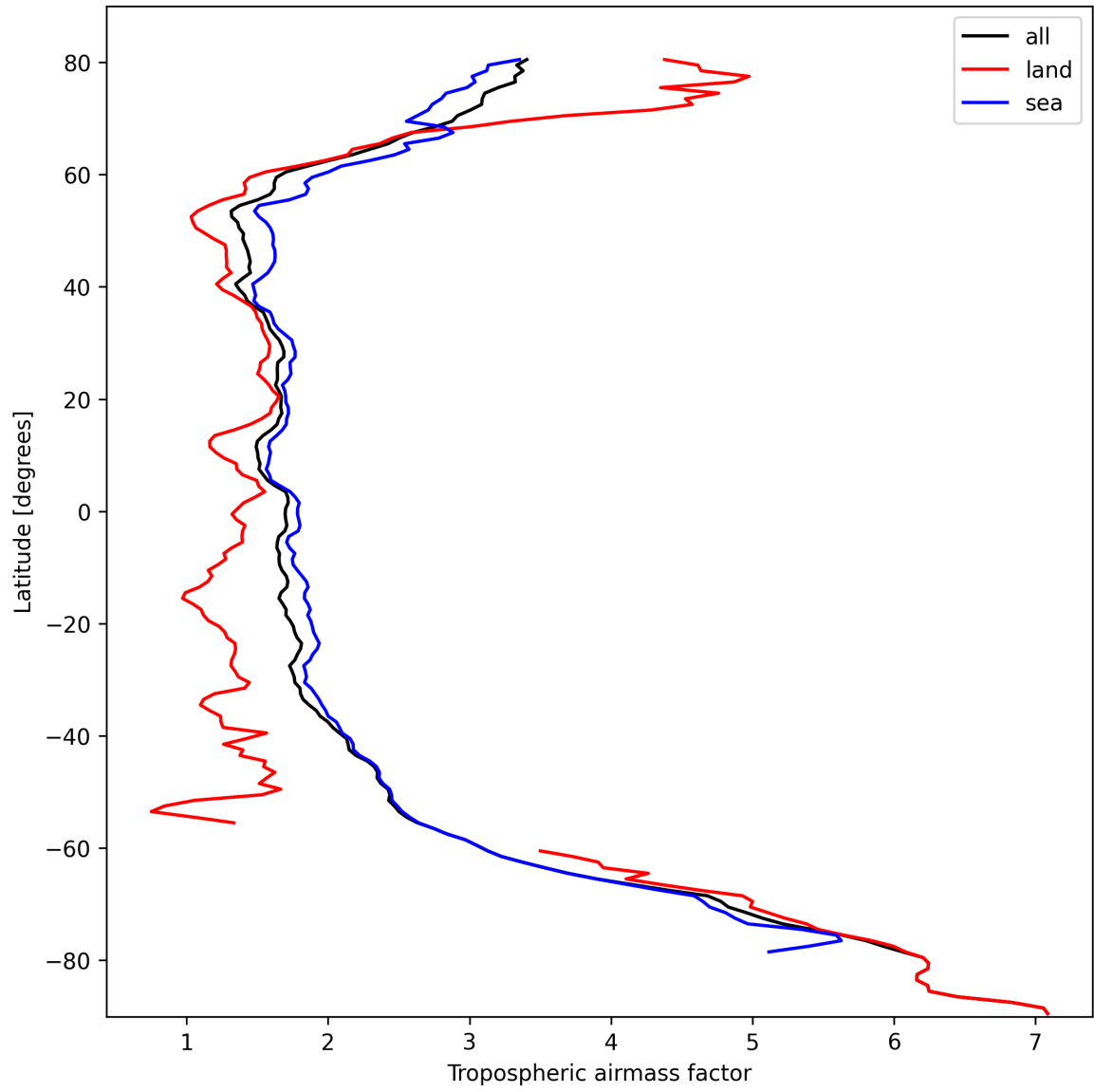
Figure 14: Zonal average of “Tropospheric air mass factor” for 2024-10-11 to 2024-10-13.
