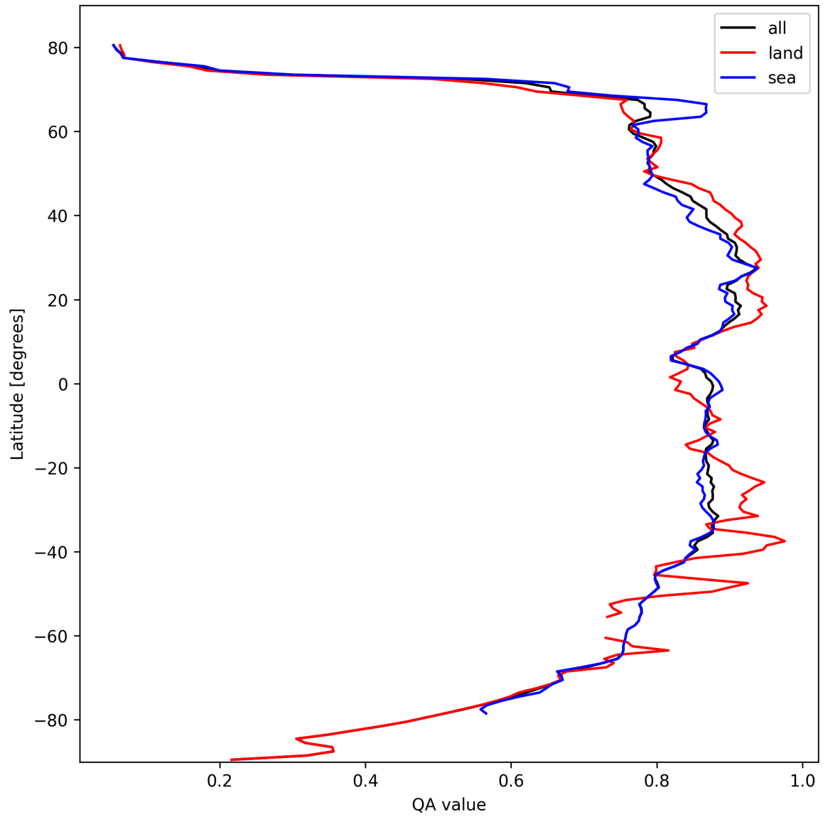
Figure 11: Zonal average of “QA value” for 2024-10-11 to 2024-10-13.
