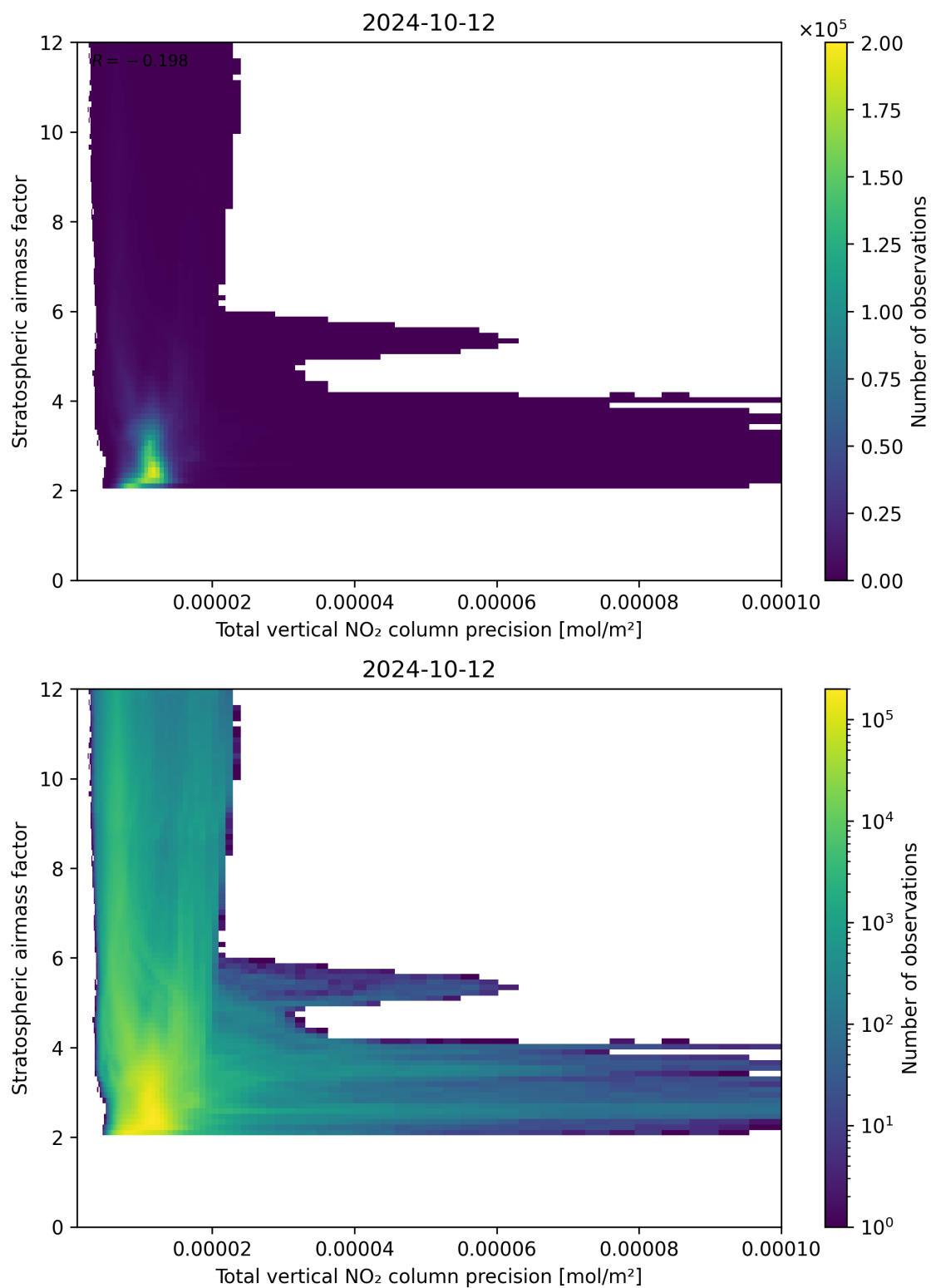
Figure 115: Scatter density plot of “Total vertical NO 2 column precision” against “Stratospheric airmass factor” for 2024-10-11 to 2024-10-13.
