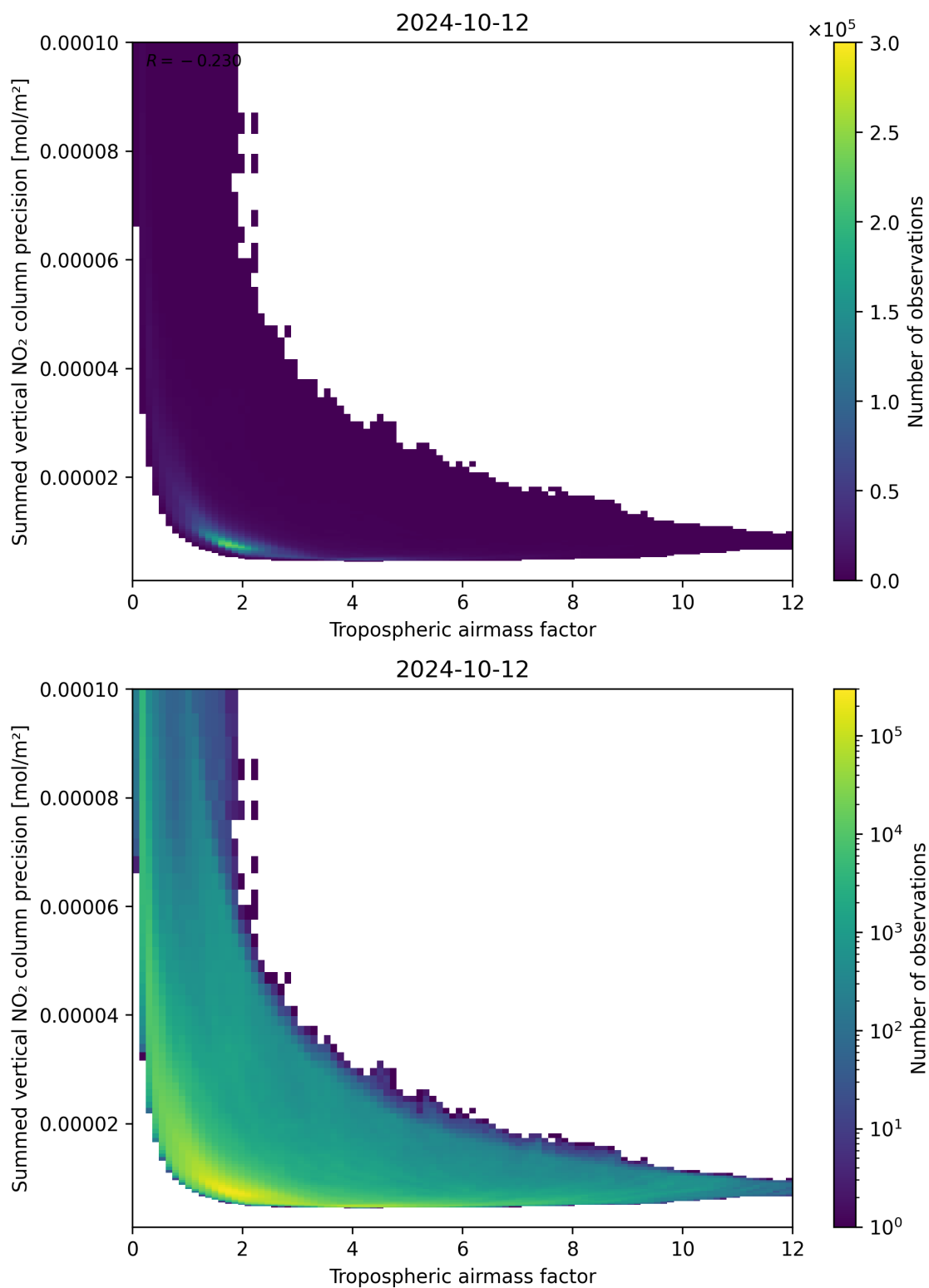
Figure 76: Scatter density plot of “Tropospheric airmass factor” against “Summed vertical NO 2 column precision” for 2024-10-11 to 2024-10-13.
