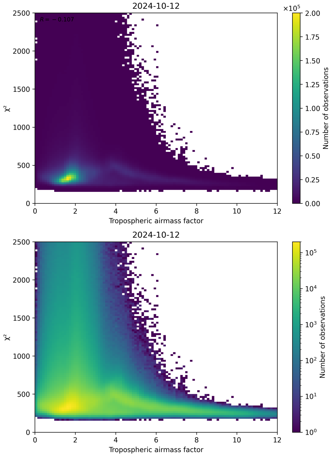
Figure 73: Scatter density plot of “Tropospheric airmass factor” against “ \chi^2 ” for 2024-10-11 to 2024-10-13.
