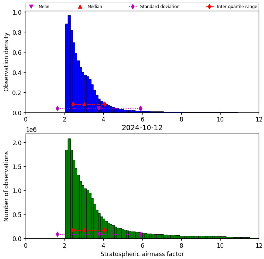
Figure 44: Histogram of “Stratospheric airmass factor” for 2024-10-11 to 2024-10-13
