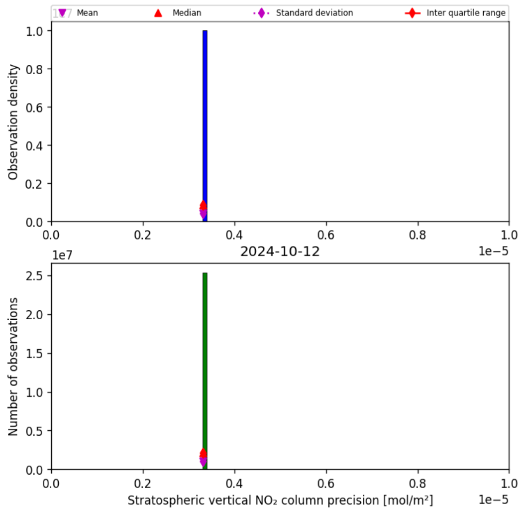
Figure 37: Histogram of “Stratospheric vertical NO 2 column precision” for 2024-10-11 to 2024-10-13
