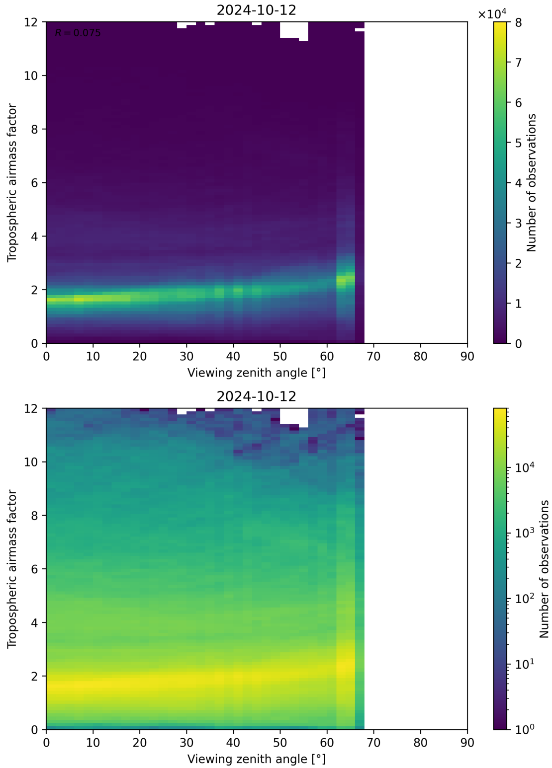
Figure 161: Scatter density plot of “Viewing zenith angle” against “Tropospheric airmass factor” for 2024-10-11 to 2024-10-13.
