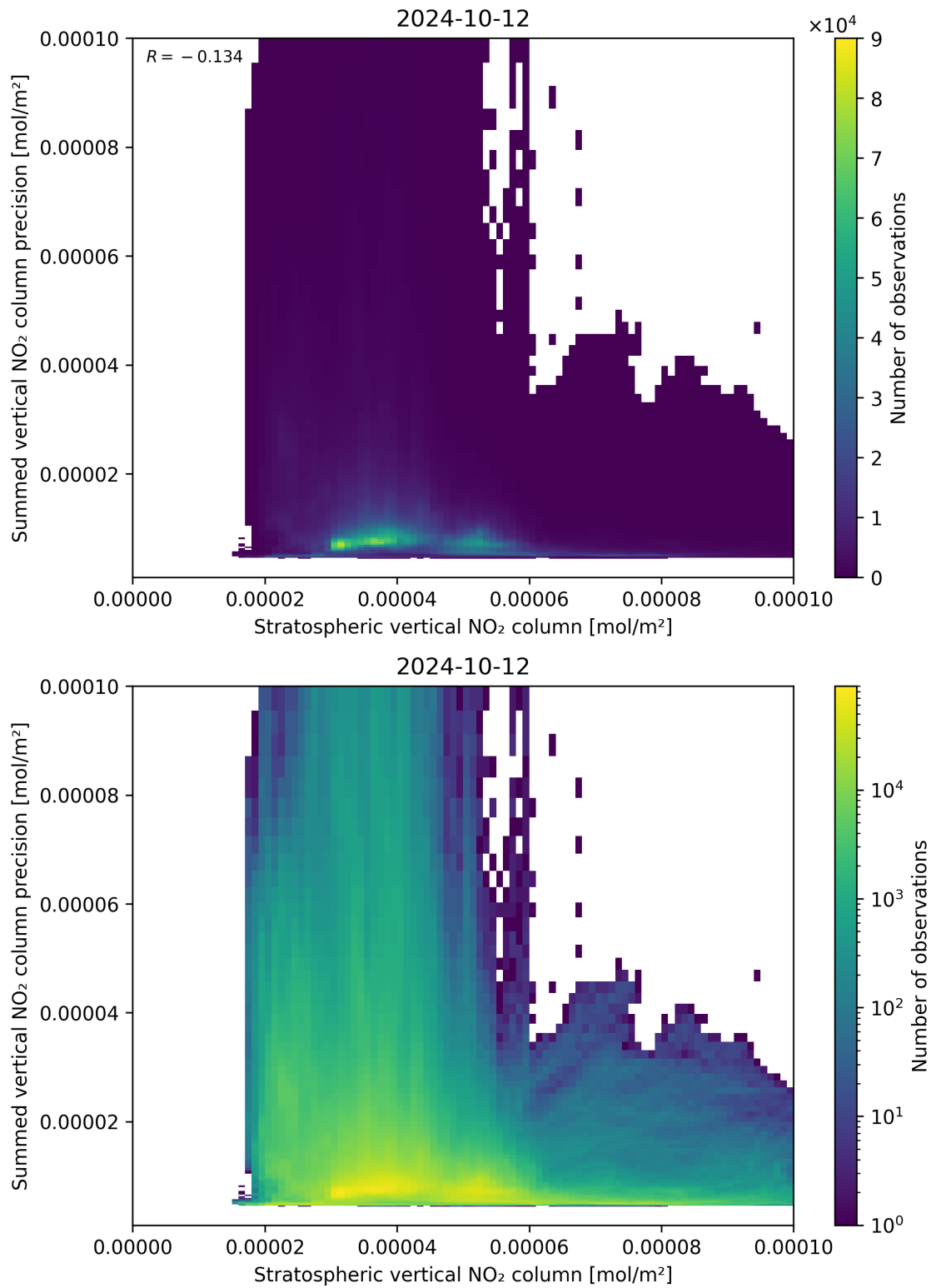
Figure 99: Scatter density plot of “Stratospheric vertical NO 2 column” against “Summed vertical NO 2 column precision” for 2024-10-11 to 2024-10-13.
