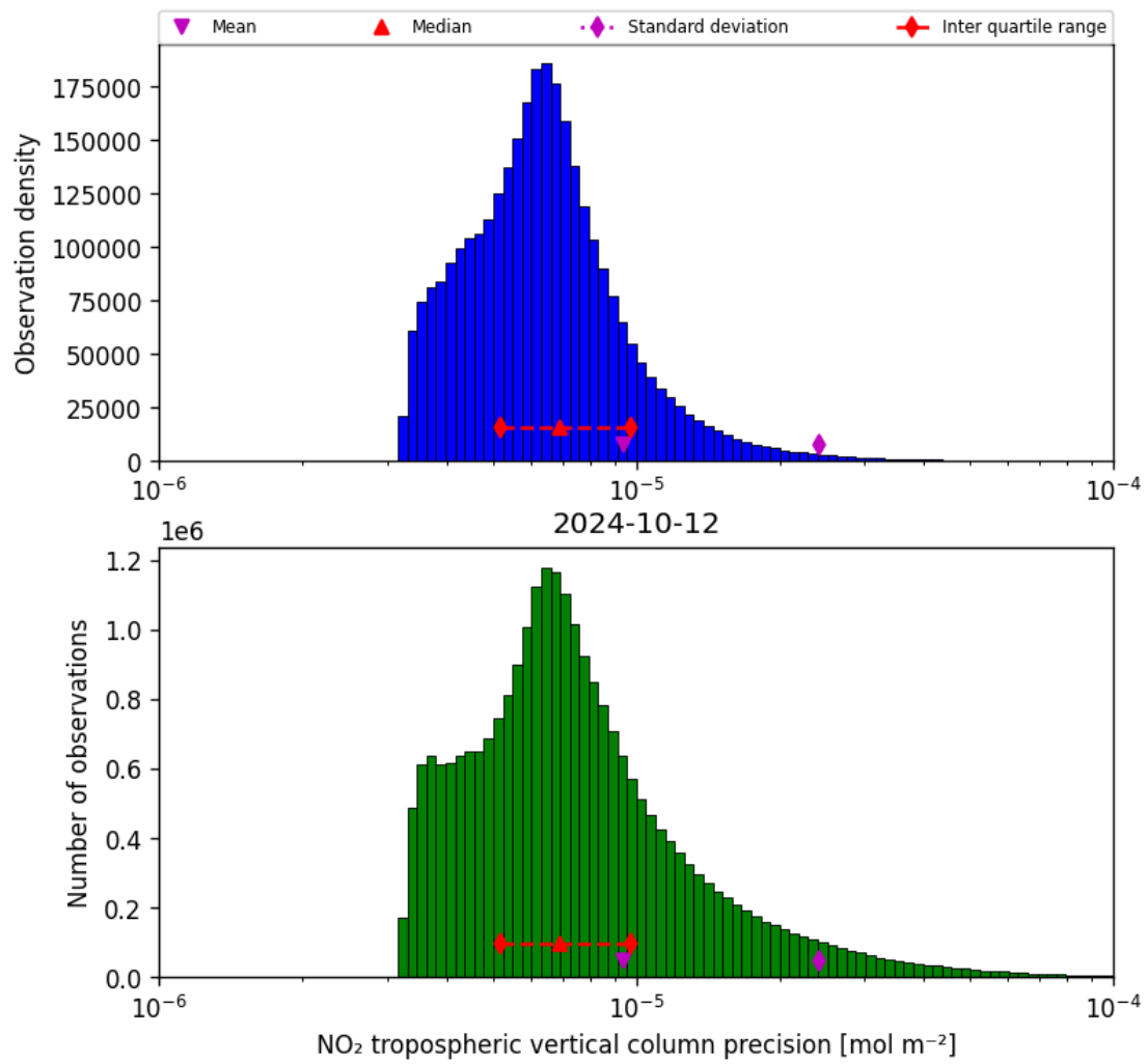
Figure 30: Histogram of “NO 2 tropospheric vertical column precision” for 2024-10-11 to 2024-10-13
