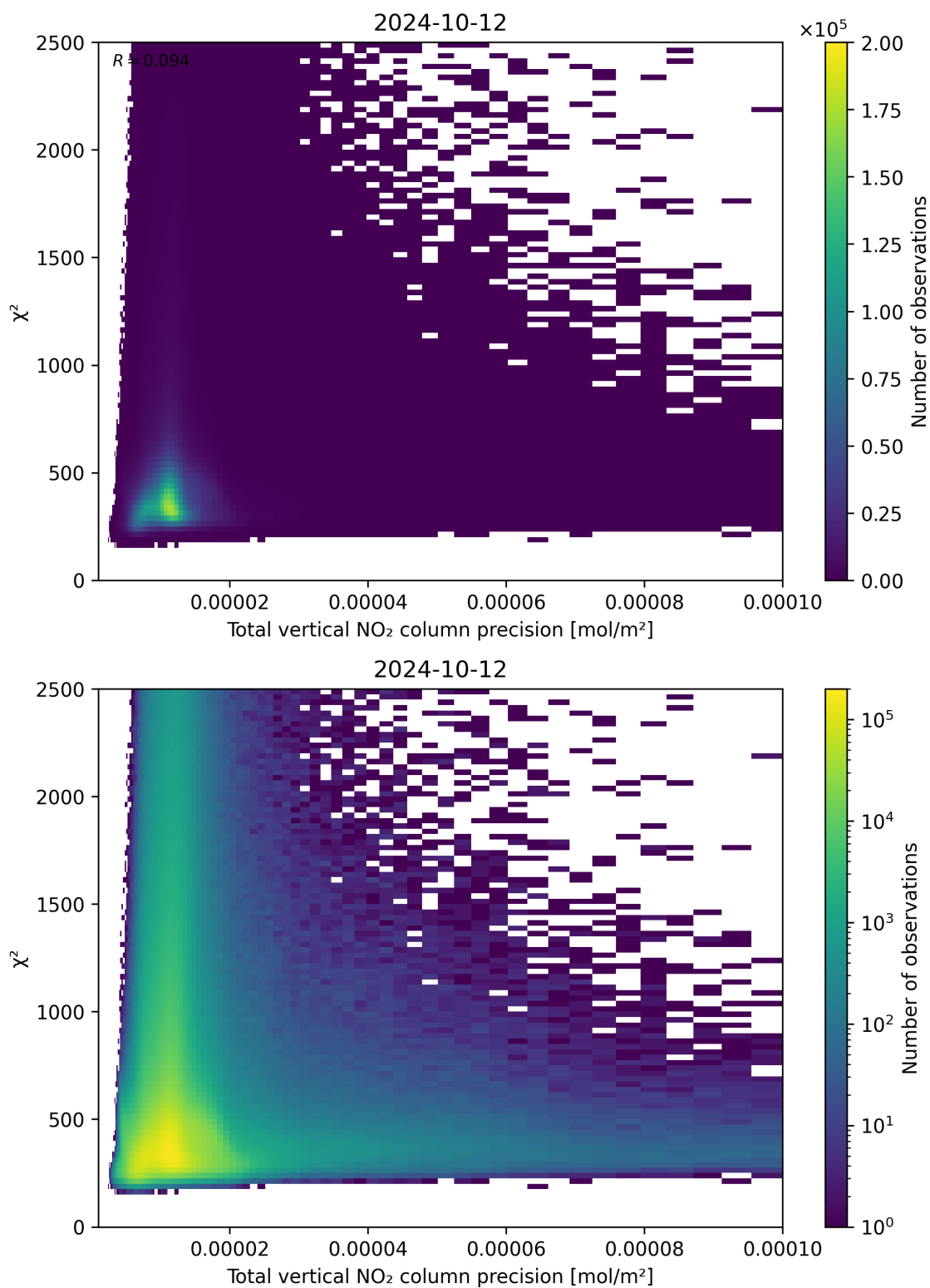
Figure 116: Scatter density plot of “Total vertical NO 2 column precision” against “ \chi^2 ” for 2024-10-11 to 2024-10-13.
