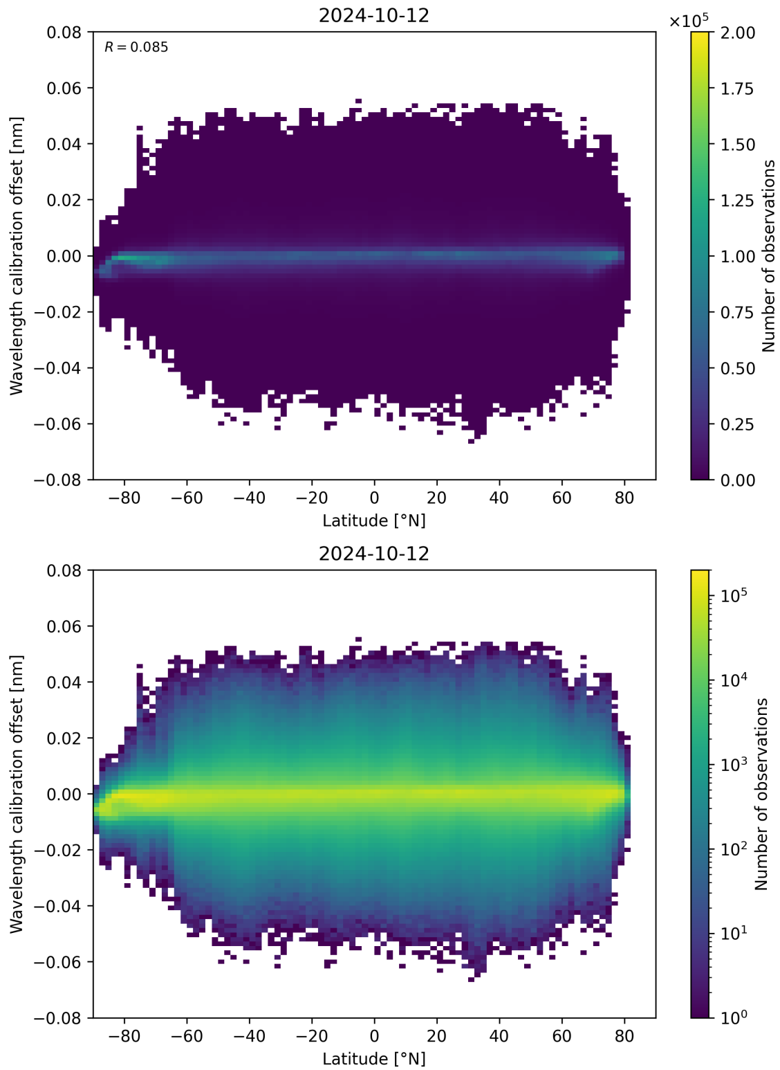
Figure 95: Scatter density plot of “Latitude” against “Wavelength calibration offset” for 2024-10-11 to 2024-10-13.
