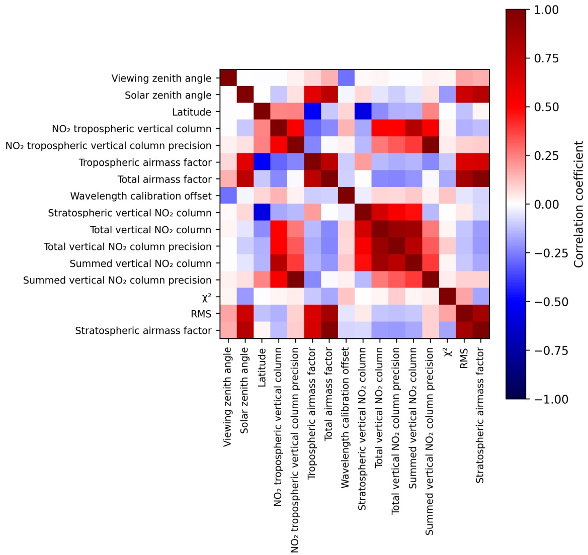
Figure 2: Map of correlation matrix for 2024-10-11 to 2024-10-13.
