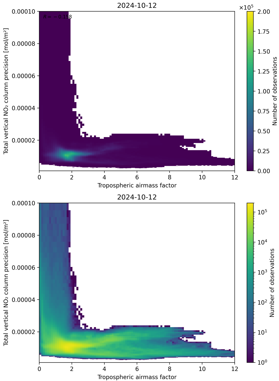
Figure 78: Scatter density plot of “Tropospheric air mass factor” against “Total vertical NO 2 column precision” for 2024-10-11 to 2024-10-13.
