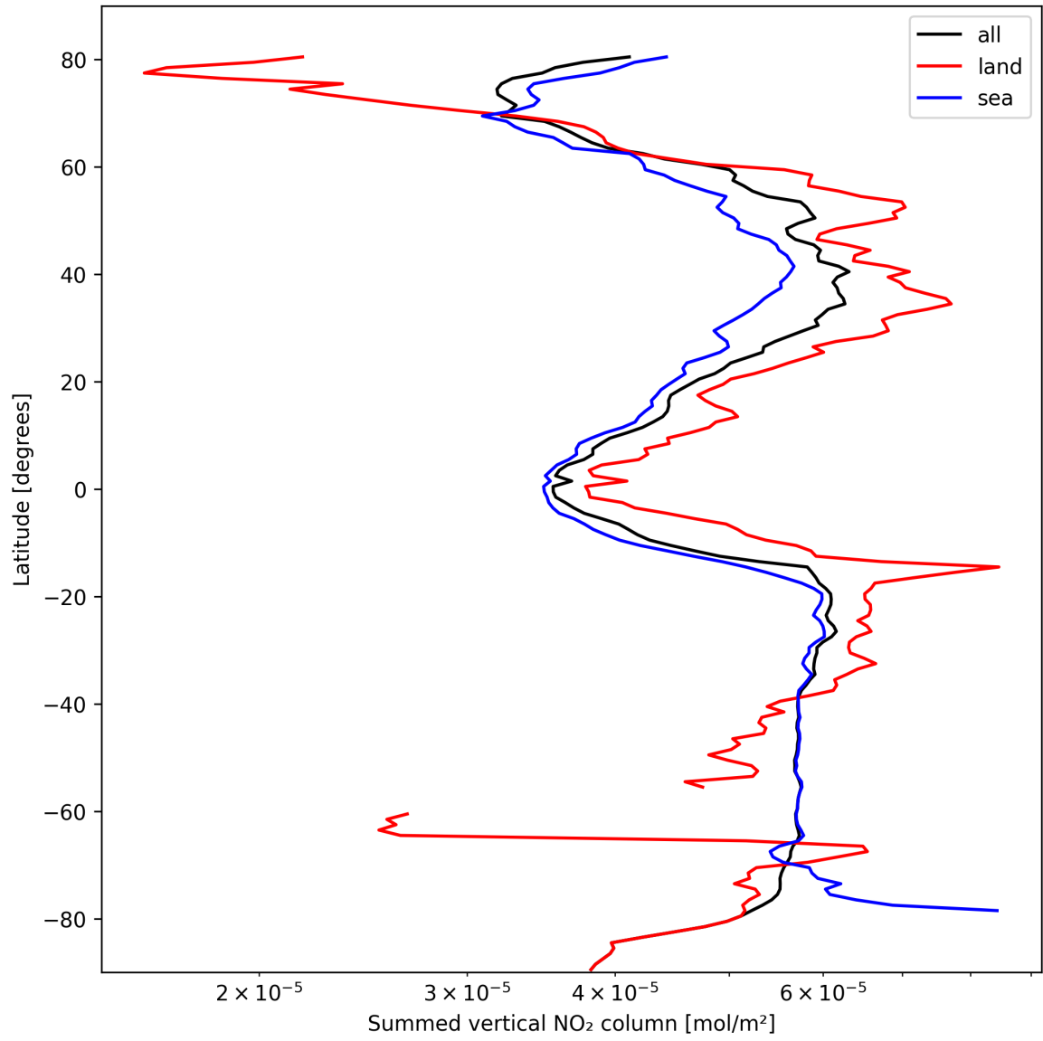
Figure 23: Zonal average of “Summed vertical NO 2 column” for 2024-10-11 to 2024-10-13.
