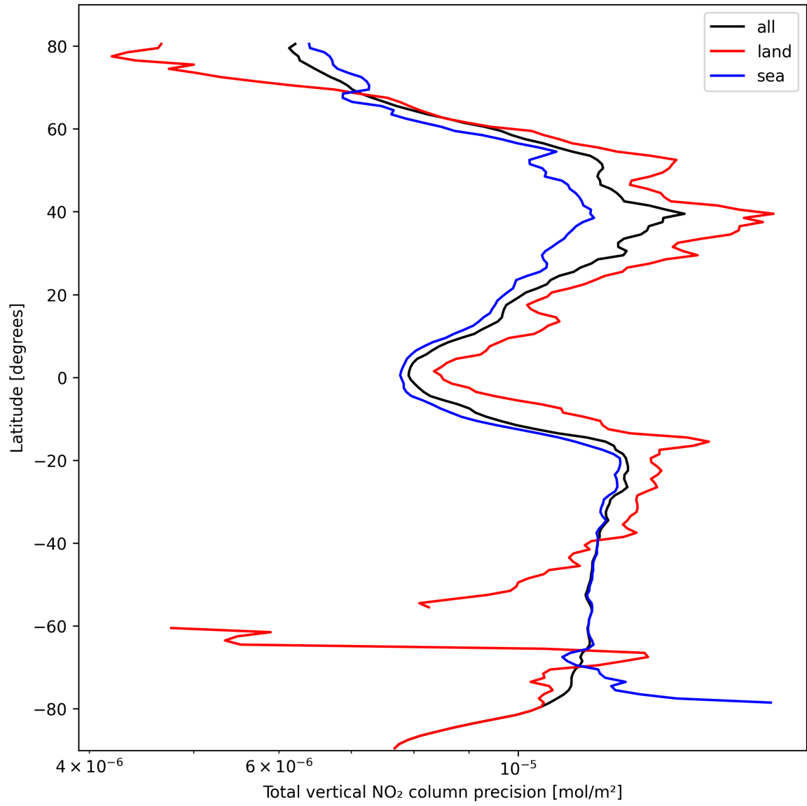
Figure 22: Zonal average of “Total vertical NO 2 column precision” for 2024-10-11 to 2024-10-13.
