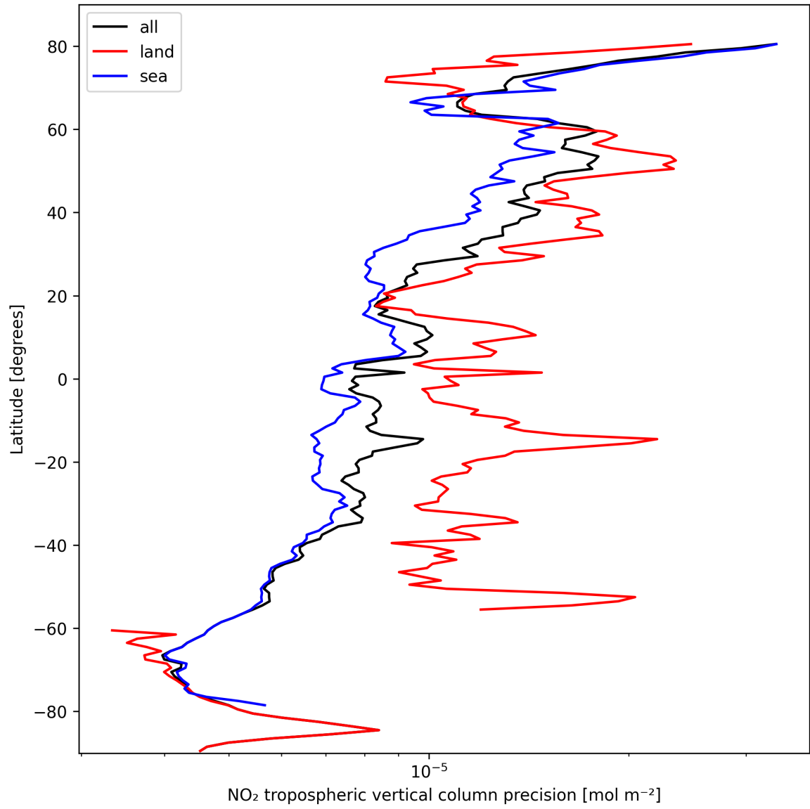
Figure 13: Zonal average of “NO 2 tropospheric vertical column precision” for 2024-10-11 to 2024-10-13.
