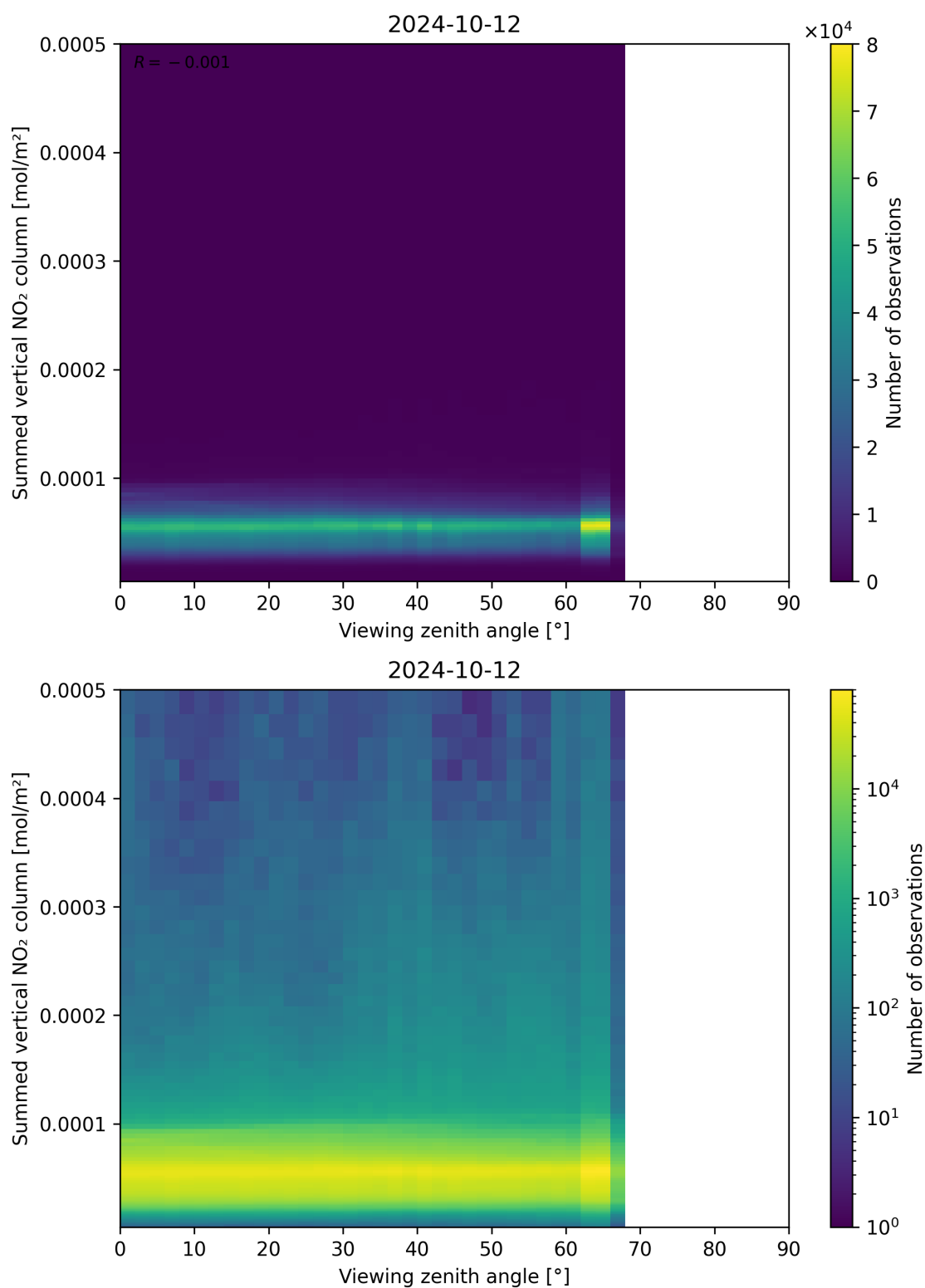
Figure 165: Scatter density plot of “Viewing zenith angle” against “Summed vertical NO 2 column” for 2024-10-11 to 2024-10-13.
