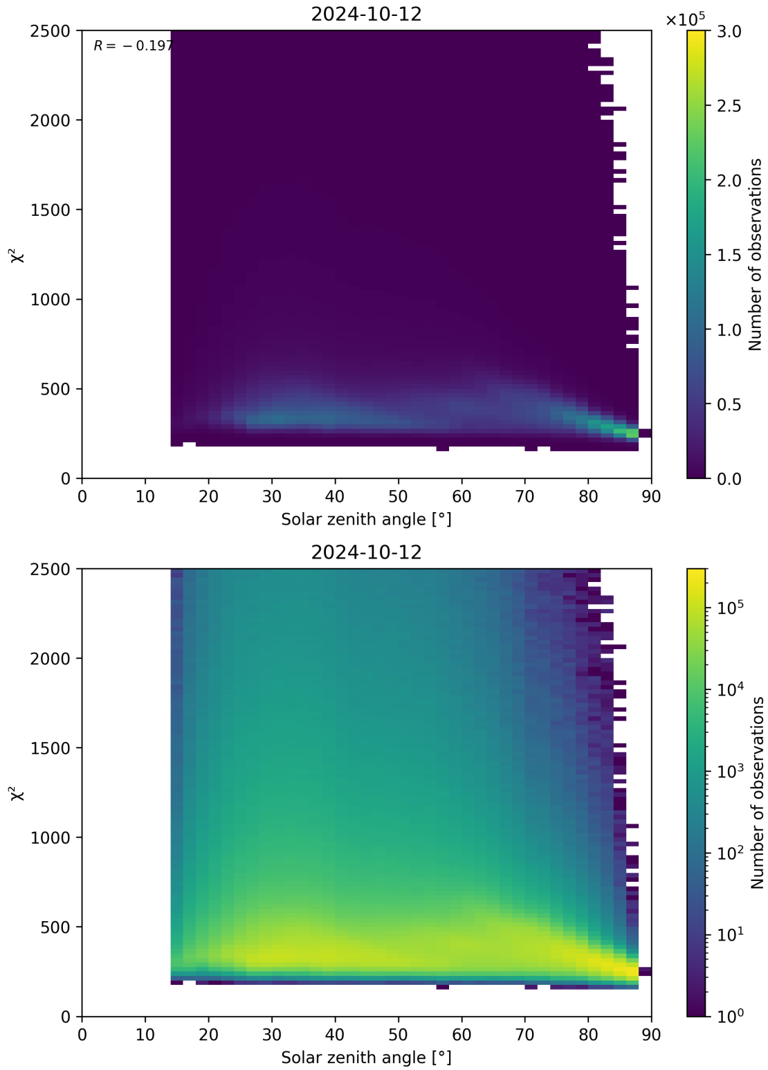
Figure 148: Scatter density plot of “Solar zenith angle” against “ \chi^2 ” for 2024-10-11 to 2024-10-13.
