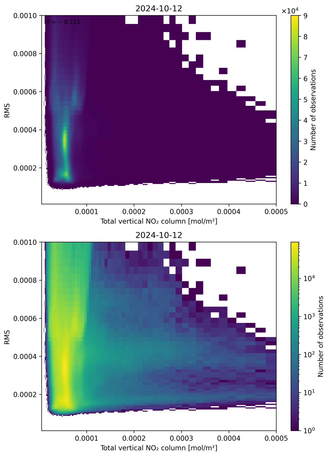
Figure 120: Scatter density plot of “Total vertical NO 2 column” against “RMS” for 2024-10-11 to 2024-10-13.
