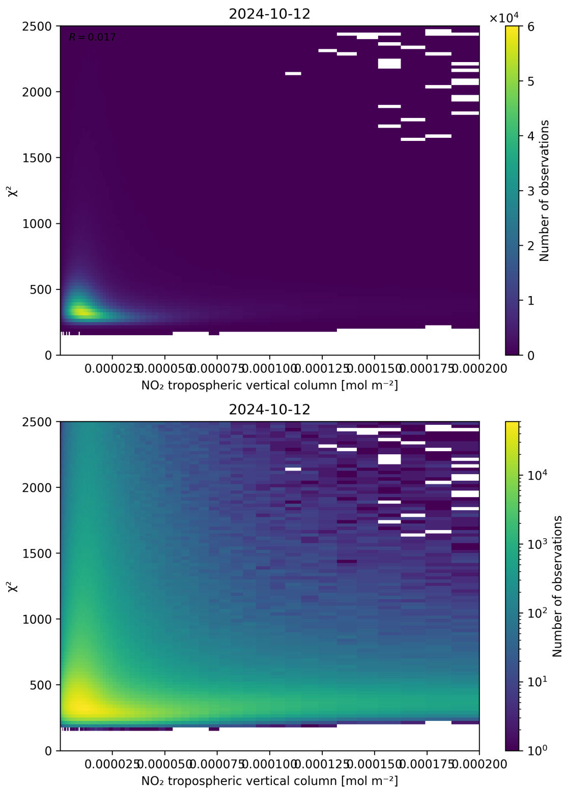
Figure 124: Scatter density plot of “NO 2 tropospheric vertical column” against “ \chi^2 ” for 2024-10-11 to 2024-10-13.
