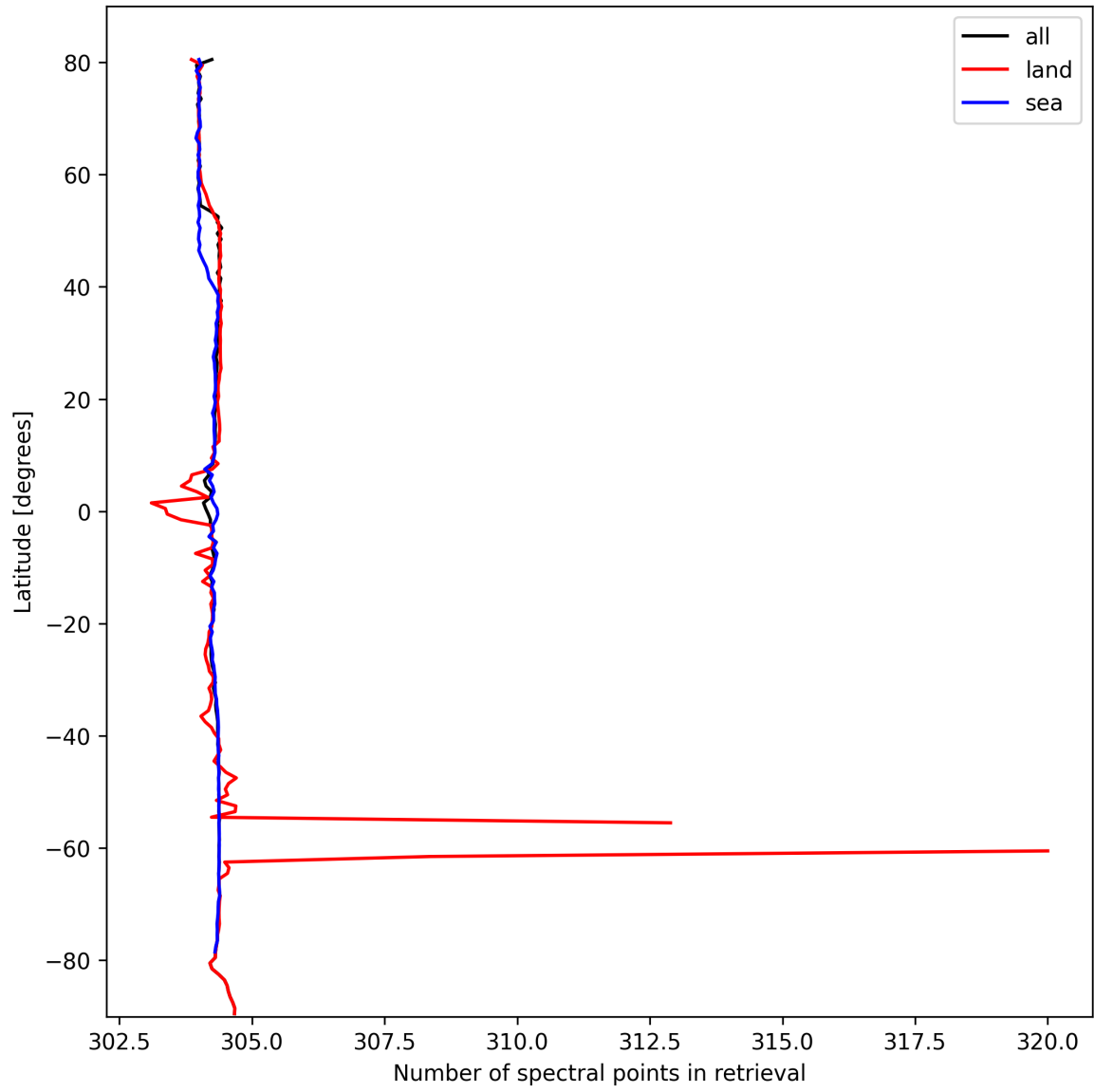
Figure 16: Zonal average of “Number of spectral points in retrieval” for 2024-10-11 to 2024-10-13.
