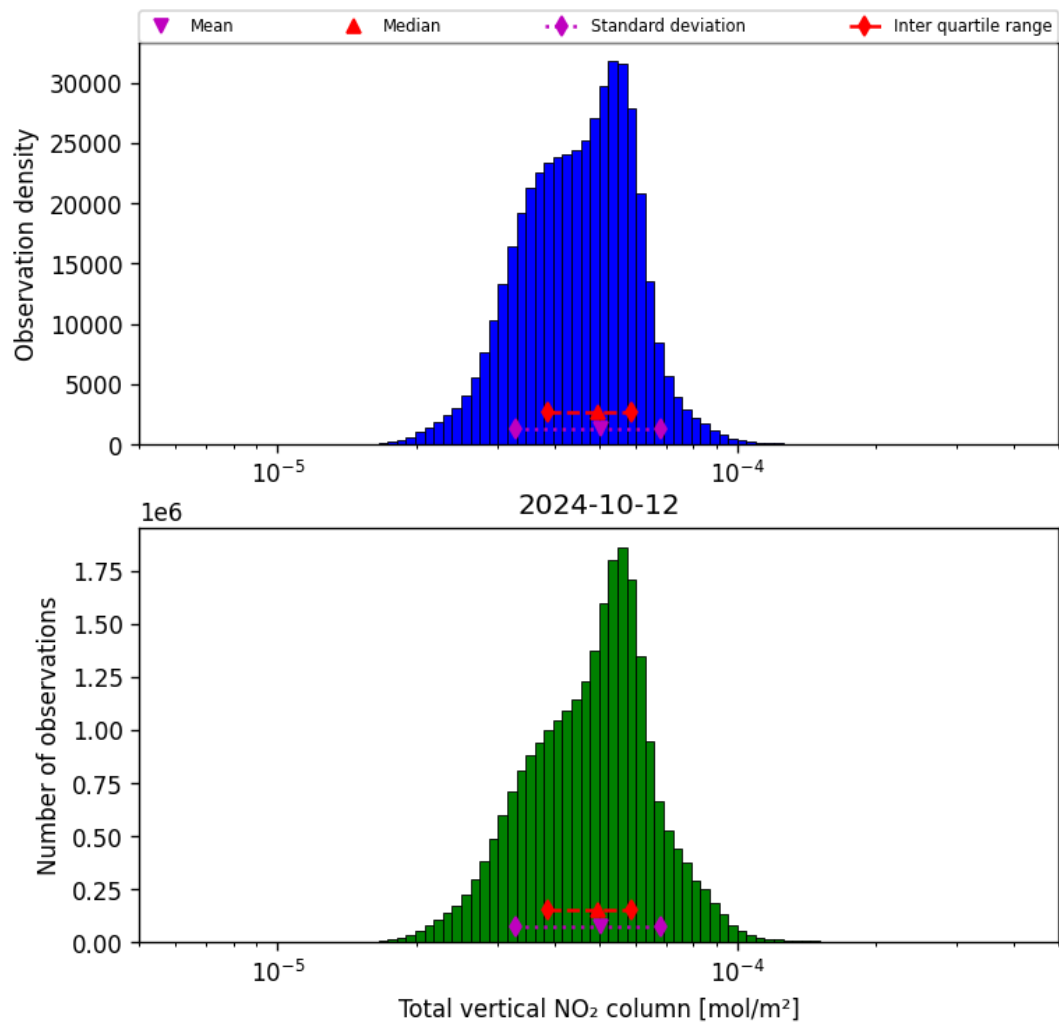
Figure 38: Histogram of “Total vertical NO 2 column” for 2024-10-11 to 2024-10-13
