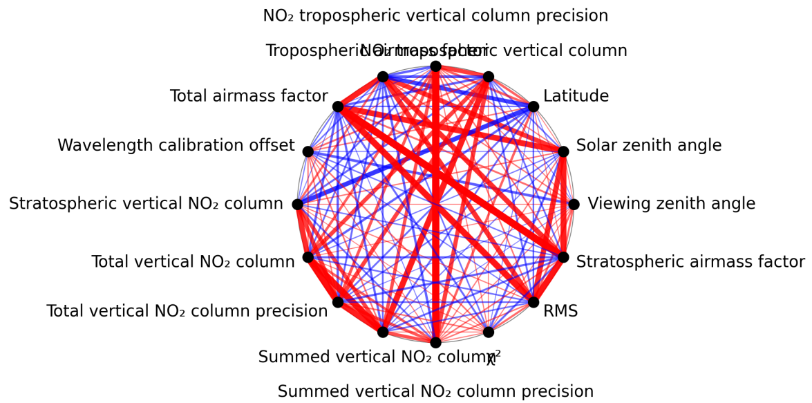
Figure 1: Map of correlation graph for 2024-10-11 to 2024-10-13.
