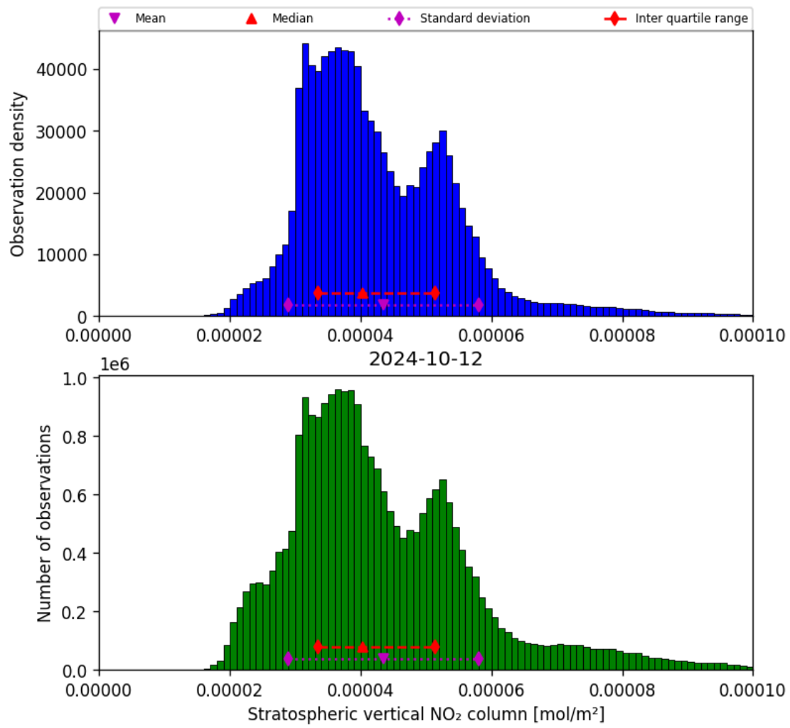
Figure 36: Histogram of “Stratospheric vertical NO 2 column” for 2024-10-11 to 2024-10-13
