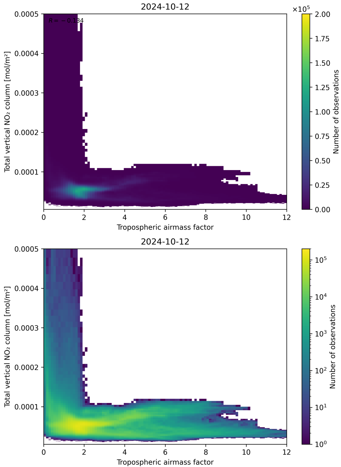
Figure 77: Scatter density plot of “Tropospheric airmass factor” against “Total vertical NO 2 column” for 2024-10-11 to 2024-10-13.
