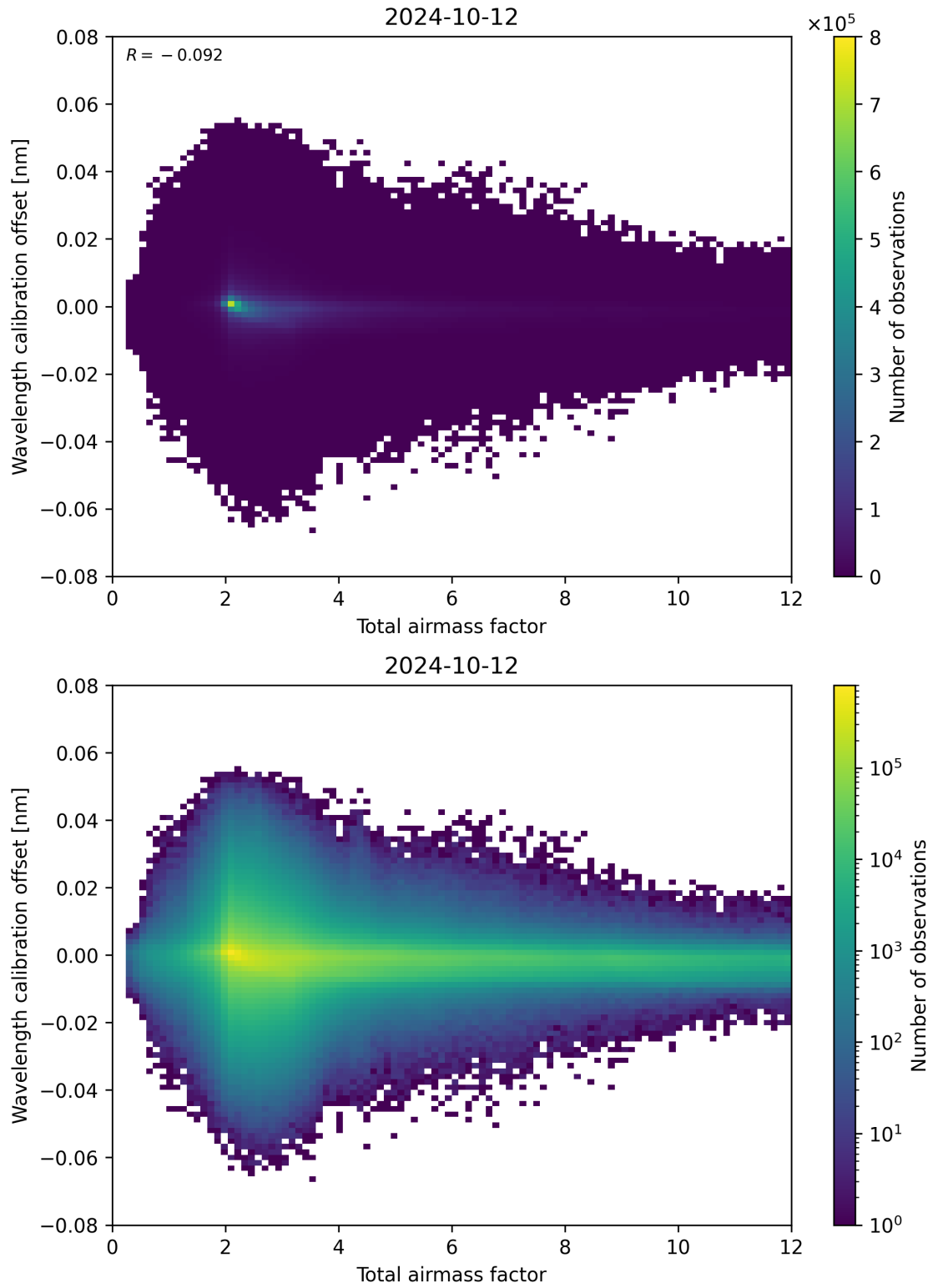
Figure 70: Scatter density plot of “Total airmass factor” against “Wavelength calibration offset” for 2024-10-11 to 2024-10-13.
