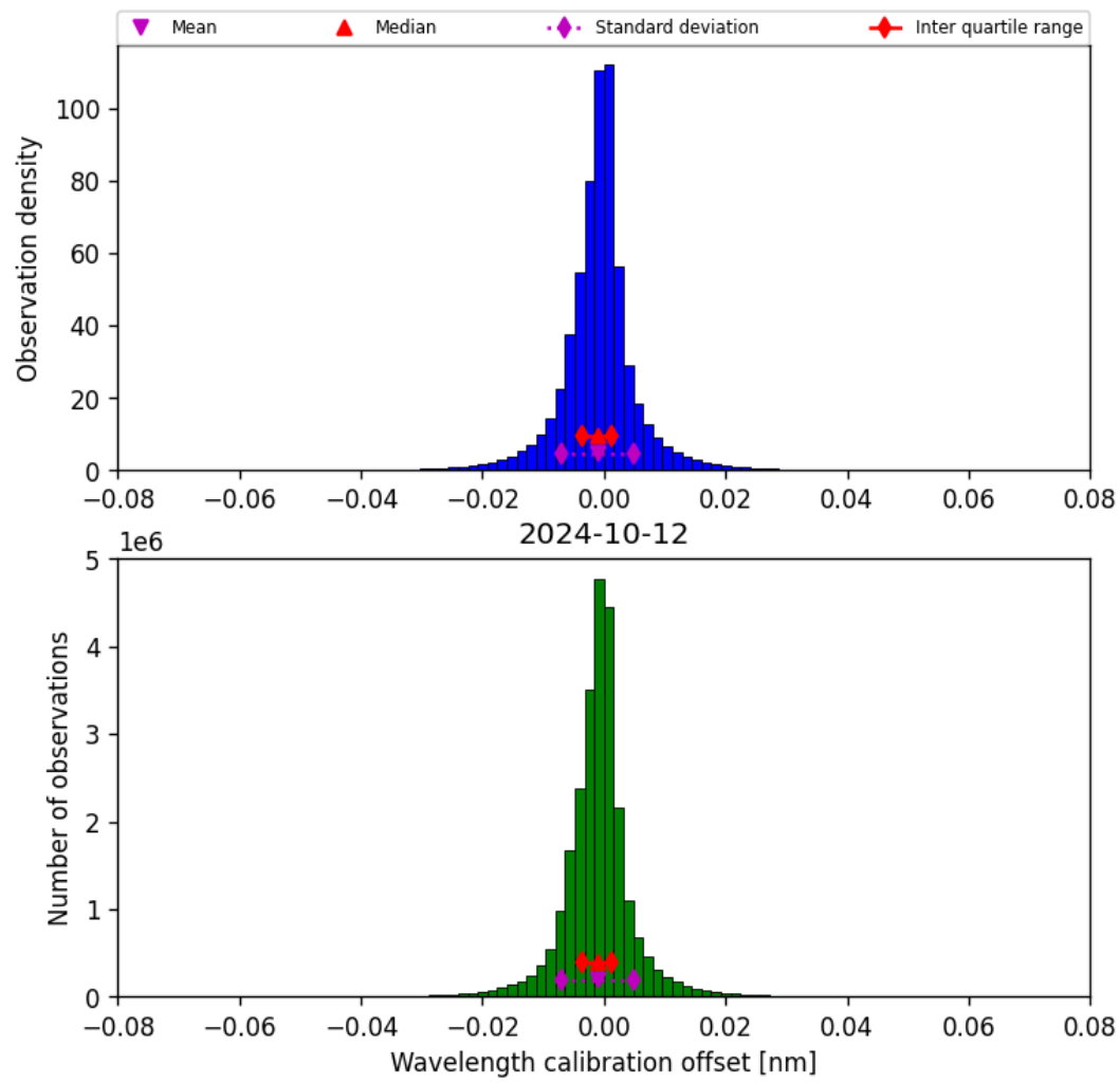
Figure 35: Histogram of “Wavelength calibration offset” for 2024-10-11 to 2024-10-13
