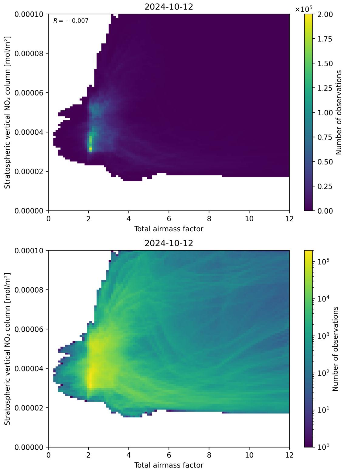
Figure 64: Scatter density plot of “Total airmass factor” against “Stratospheric vertical NO 2 column” for 2024-10-11 to 2024-10-13.
