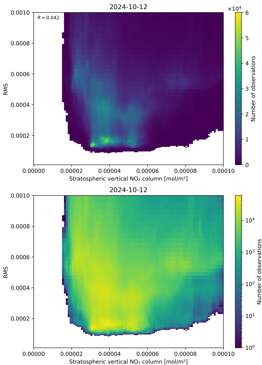
Figure 102: Scatter density plot of “Stratospheric vertical NO 2 column” against “RMS” for 2024-10-11 to 2024-10-13.
