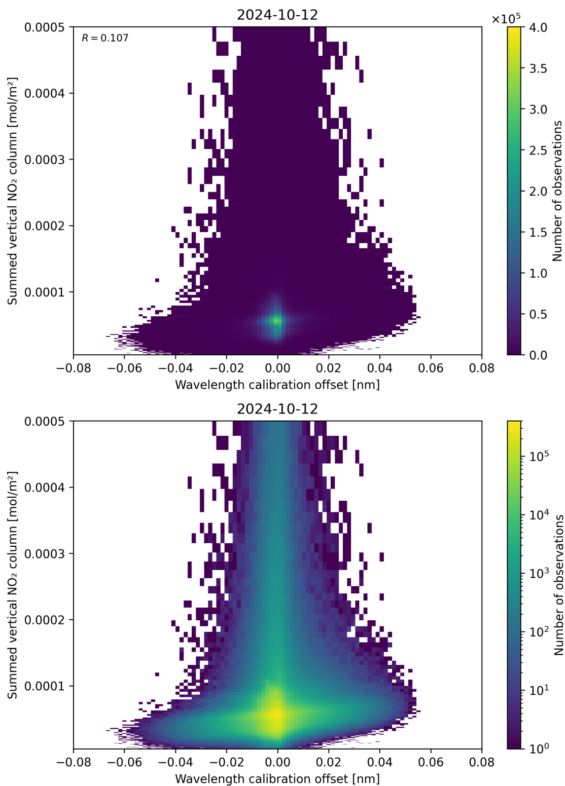
Figure 177: Scatter density plot of “Wavelength calibration offset” against “Summed vertical NO 2 column” for 2024-10-11 to 2024-10-13.
