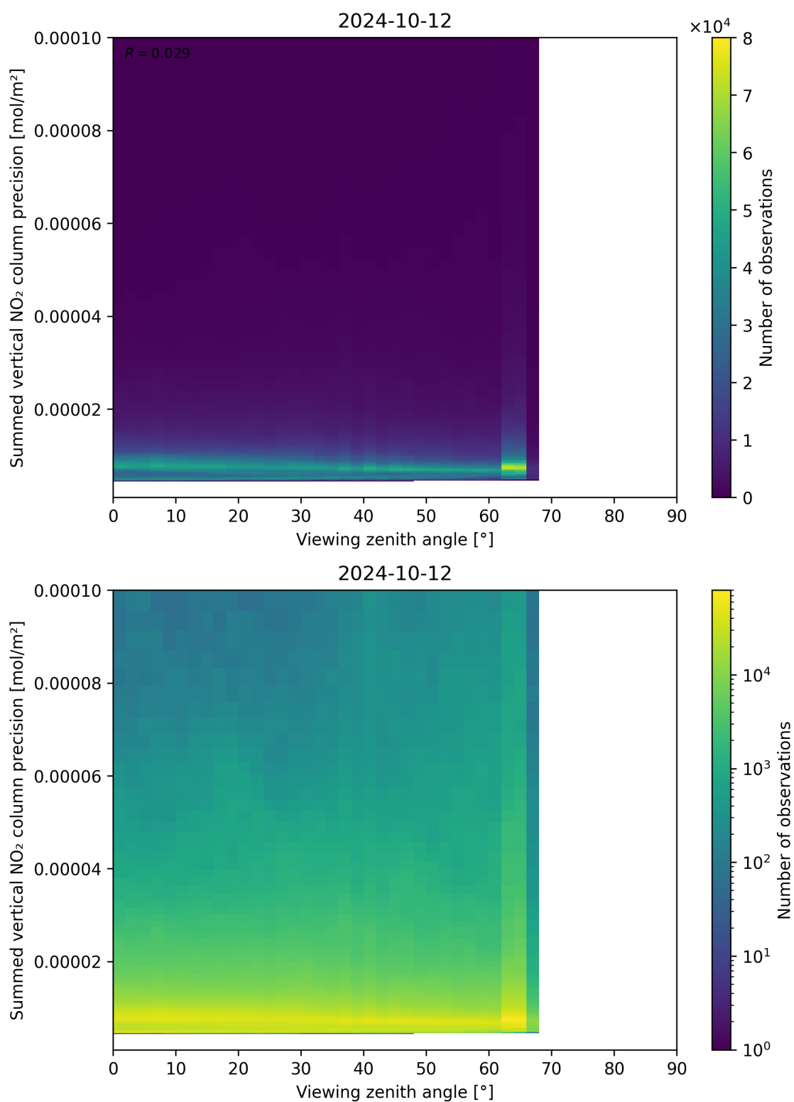
Figure 166: Scatter density plot of “Viewing zenith angle” against “Summed vertical NO 2 column precision” for 2024-10-11 to 2024-10-13.
