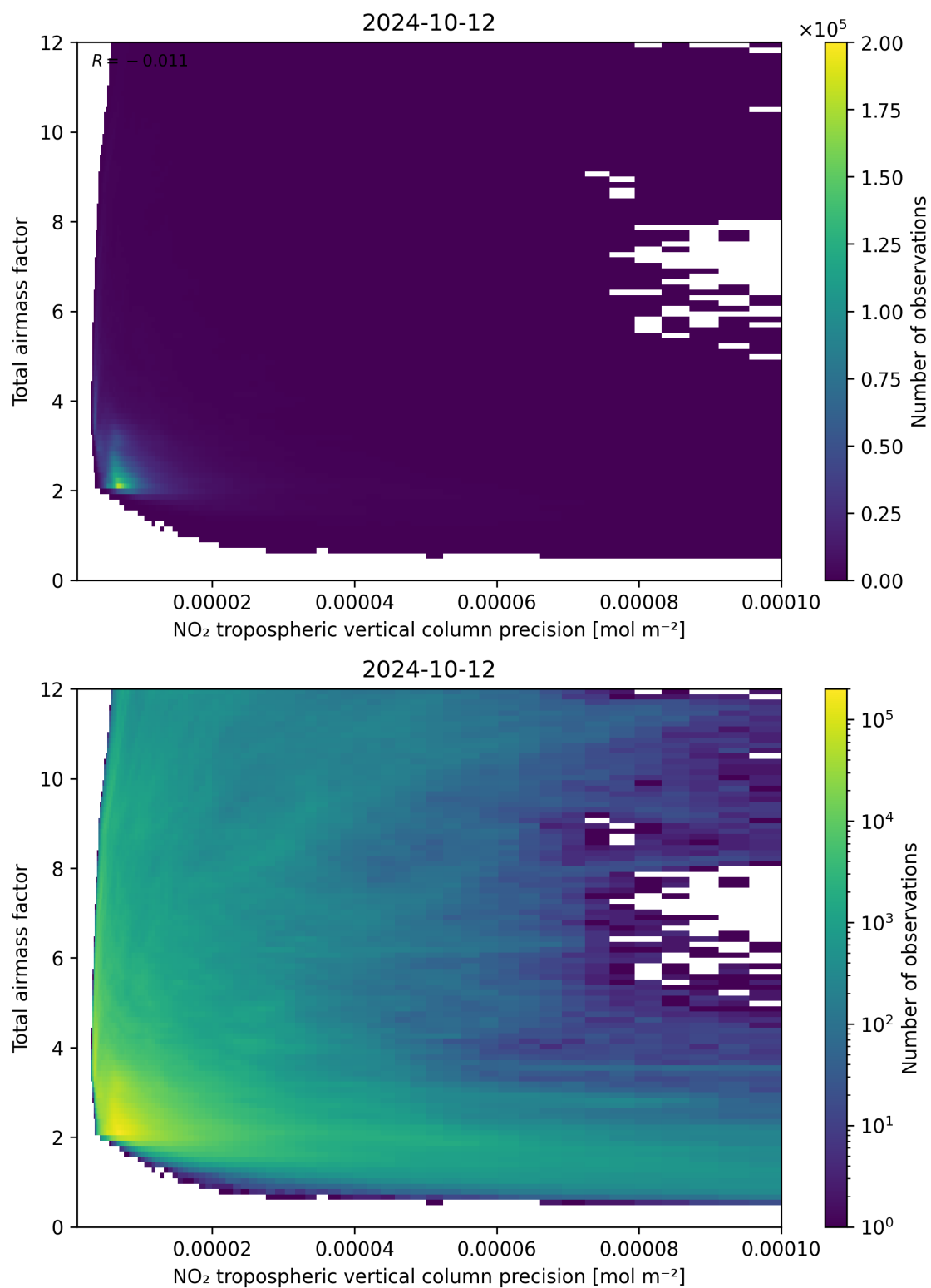
Figure 132: Scatter density plot of “NO 2 tropospheric vertical column precision” against “Total air mass factor” for 2024-10-11 to 2024-10-13.
