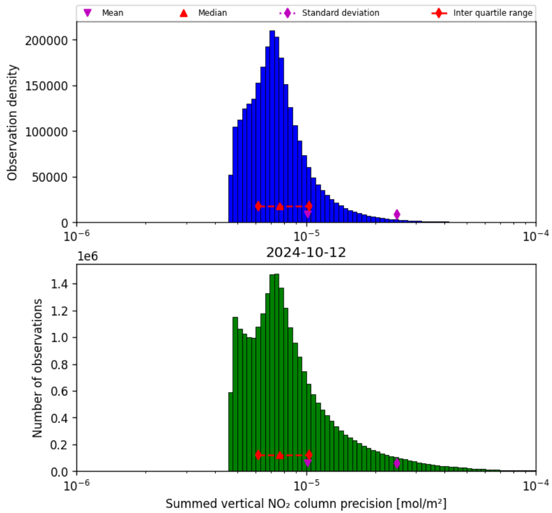
Figure 41: Histogram of "Summed vertical NO 2 column precision" for 2024-10-11 to 2024-10-13
