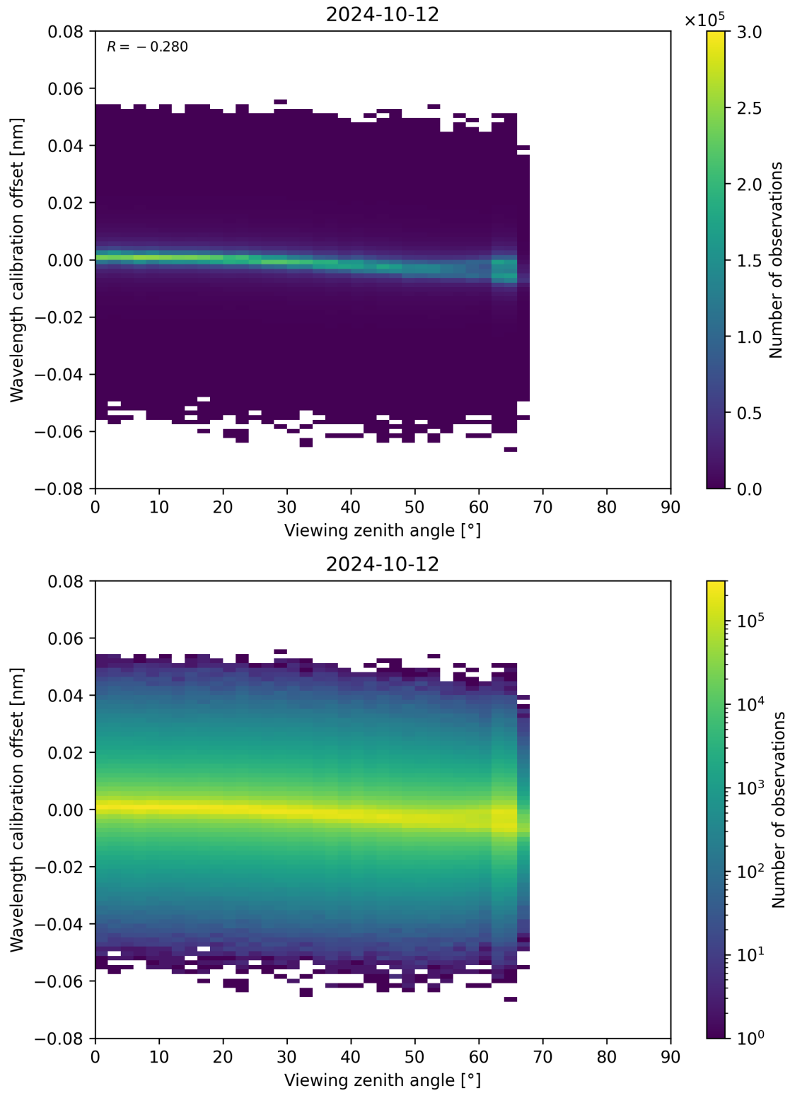
Figure 173: Scatter density plot of “Viewing zenith angle” against “Wavelength calibration offset” for 2024-10-11 to 2024-10-13.
