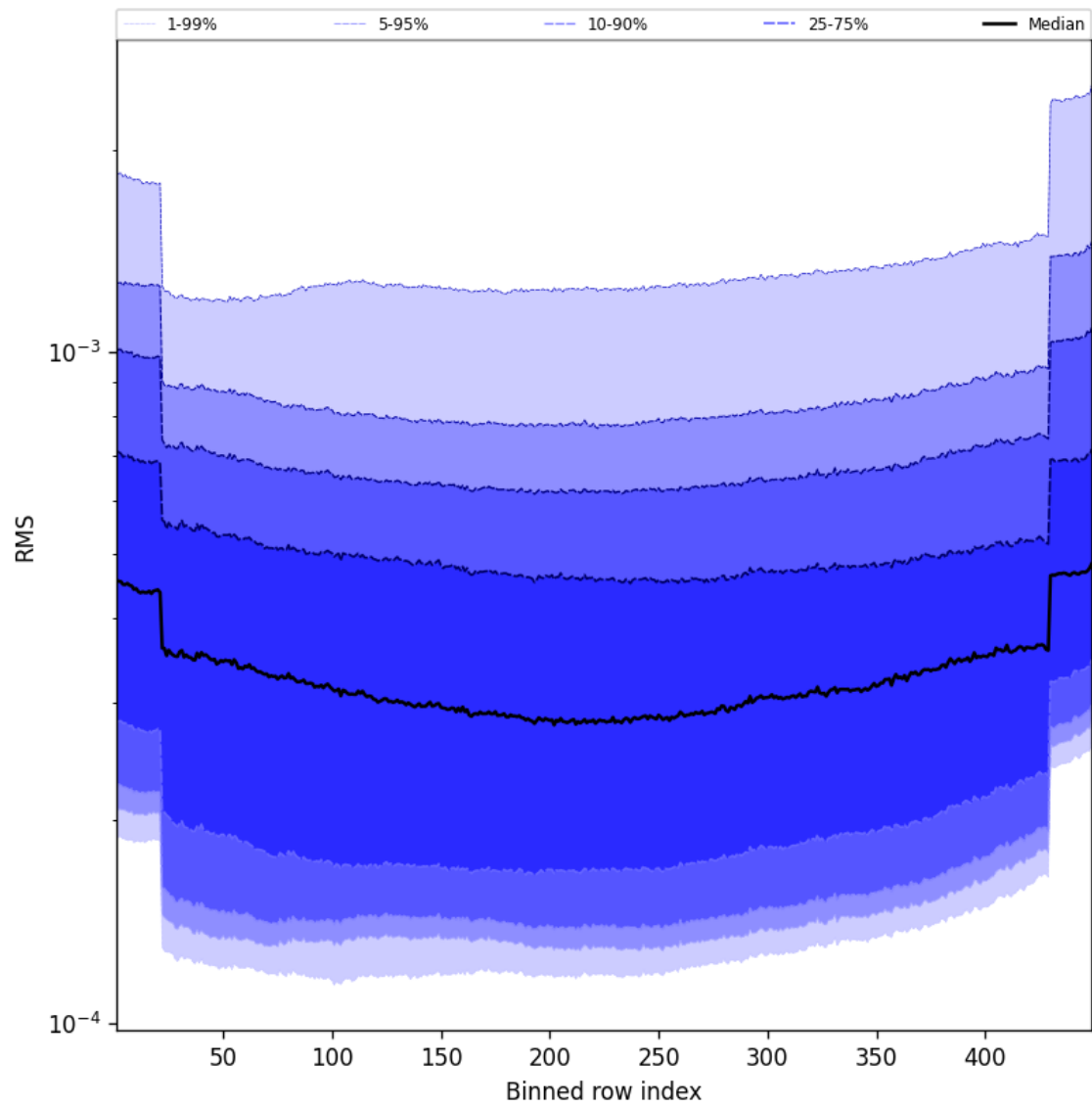
Figure 60: Along track statistics of “RMS” for 2024-10-11 to 2024-10-13
