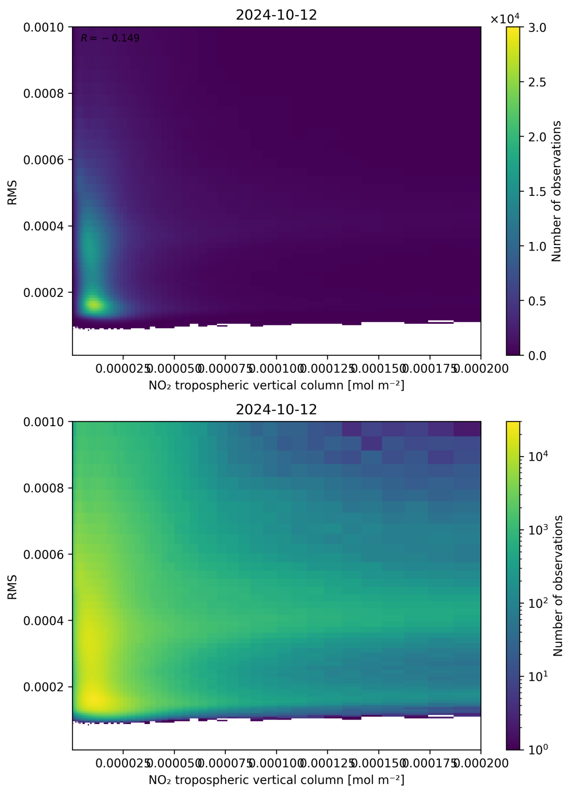
Figure 142: Scatter density plot of “NO 2 tropospheric vertical column” against “RMS” for 2024-10-11 to 2024-10-13.
