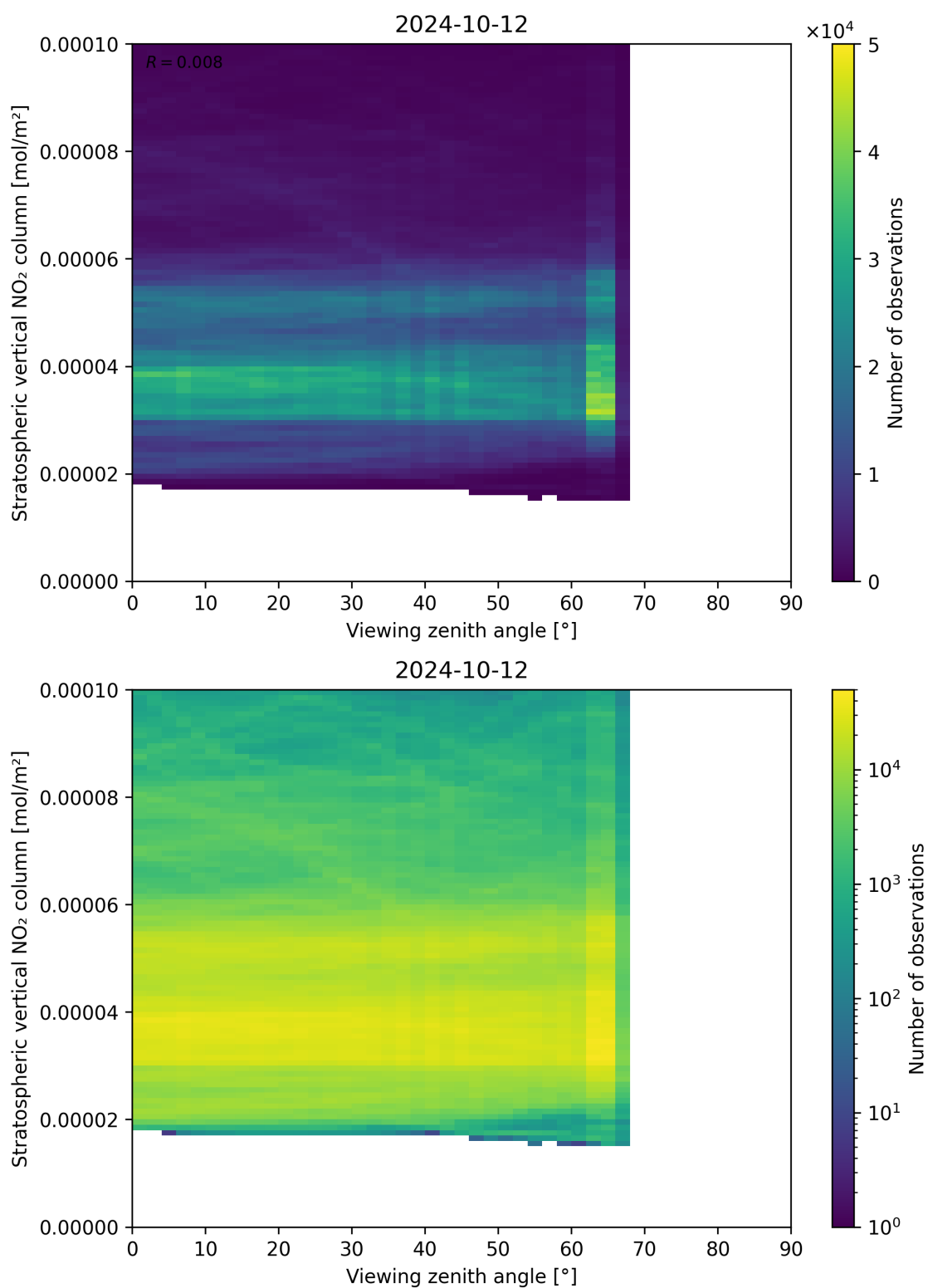
Figure 164: Scatter density plot of “Viewing zenith angle” against “Stratospheric vertical NO 2 column” for 2024-10-11 to 2024-10-13.
