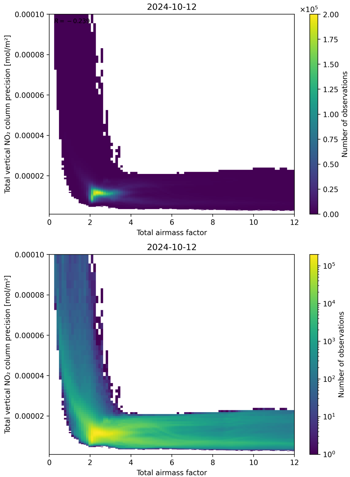
Figure 68: Scatter density plot of “Total airmass factor” against “Total vertical NO 2 column precision” for 2024-10-11 to 2024-10-13.
