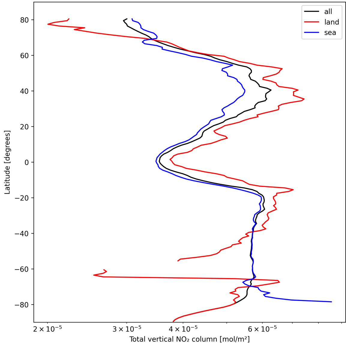
Figure 21: Zonal average of “Total vertical NO 2 column” for 2024-10-11 to 2024-10-13.
