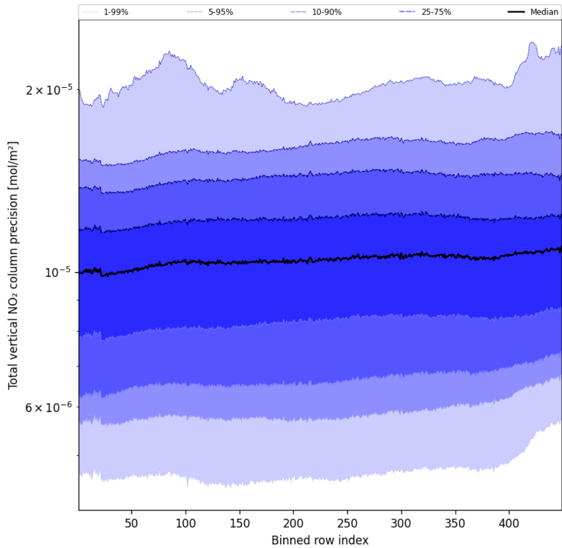
Figure 56: Along track statistics of “Total vertical NO 2 column precision” for 2024-10-11 to 2024-10-13
