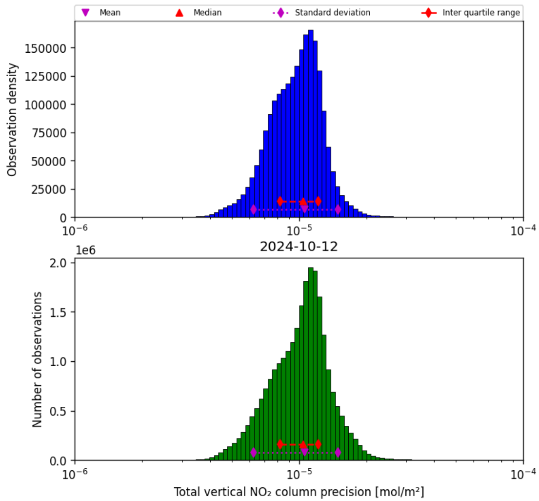
Figure 39: Histogram of “Total vertical NO 2 column precision” for 2024-10-11 to 2024-10-13
