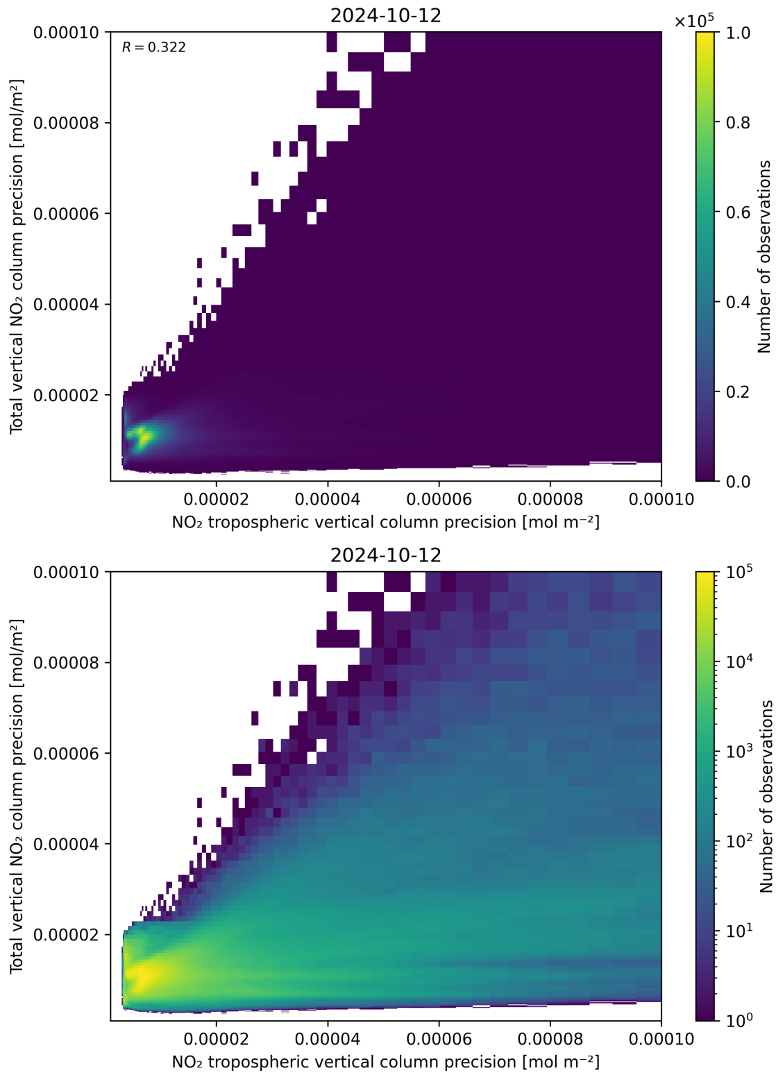
Figure 139: Scatter density plot of “NO 2 tropospheric vertical column precision” against “Total vertical NO 2 column precision” for 2024-10-11 to 2024-10-13.
