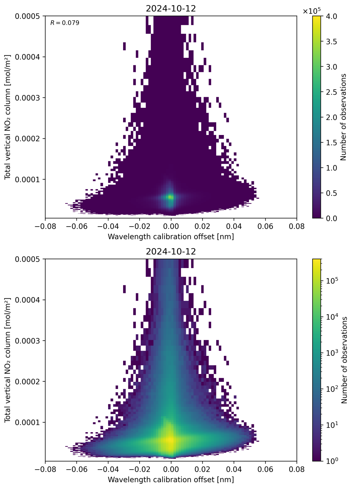
Figure 179: Scatter density plot of “Wavelength calibration offset” against “Total vertical NO 2 column” for 2024-10-11 to 2024-10-13.
