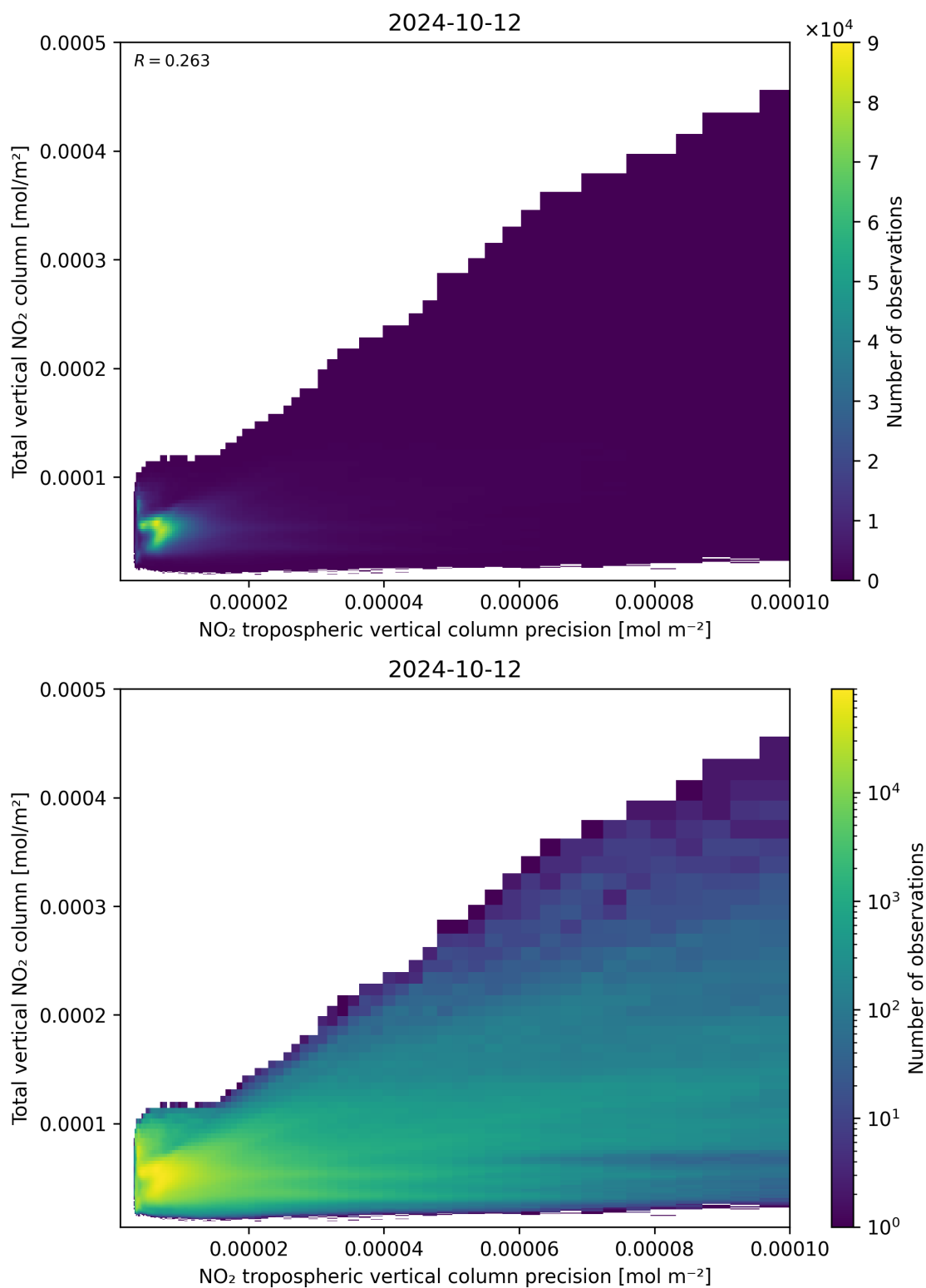
Figure 138: Scatter density plot of “NO 2 tropospheric vertical column precision” against “Total vertical NO 2 column” for 2024-10-11 to 2024-10-13.
