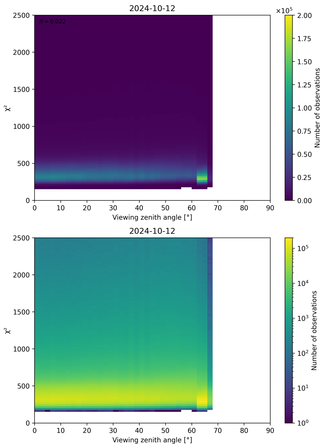
Figure 162: Scatter density plot of “Viewing zenith angle” against “ \chi^2 ” for 2024-10-11 to 2024-10-13.
