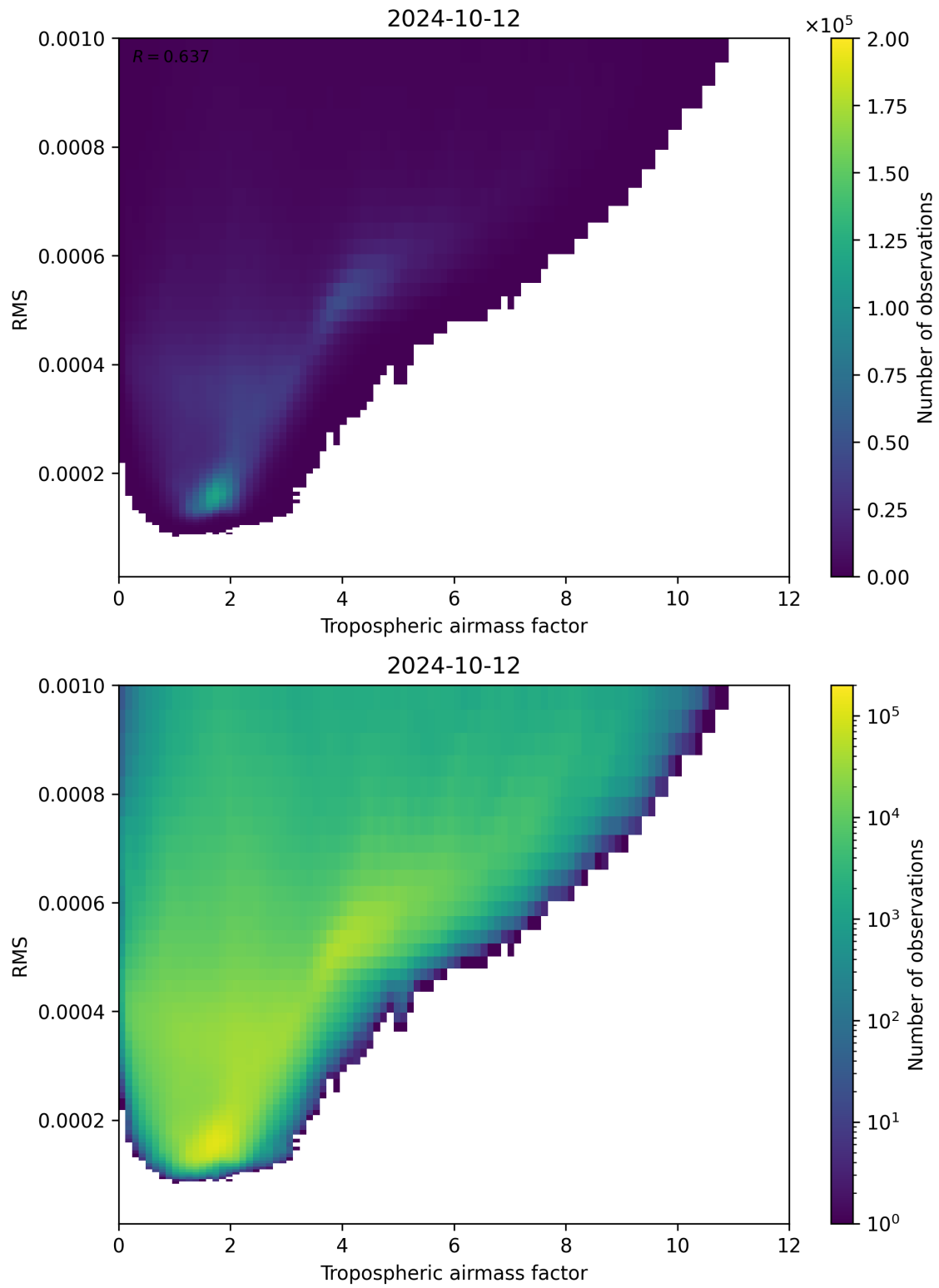
Figure 79: Scatter density plot of “Tropospheric airmass factor” against “RMS” for 2024-10-11 to 2024-10-13.
