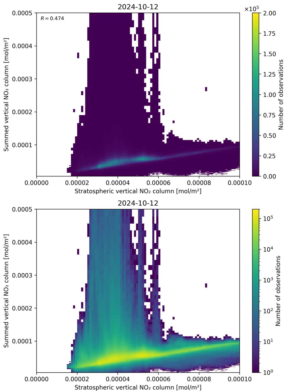
Figure 98: Scatter density plot of “Stratospheric vertical NO 2 column” against “Summed vertical NO 2 column” for 2024-10-11 to 2024-10-13.
