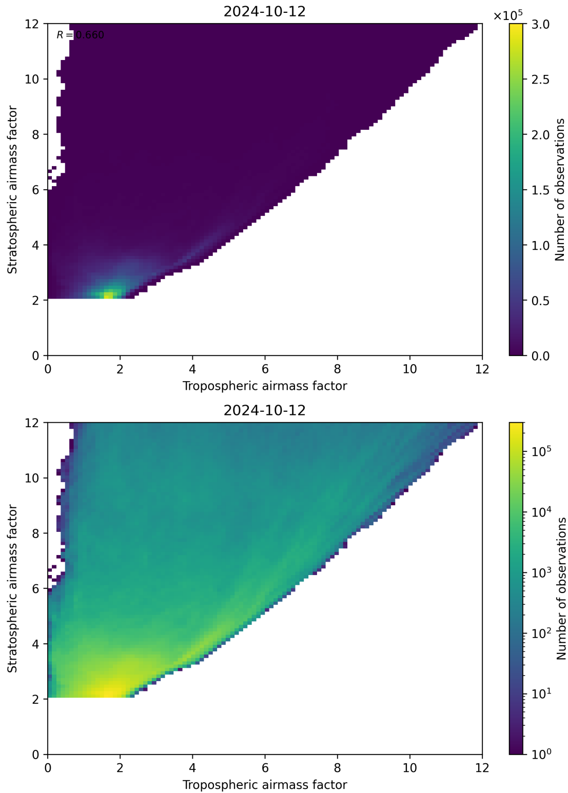
Figure 71: Scatter density plot of “Tropospheric airmass factor” against “Stratospheric airmass factor” for 2024-10-11 to 2024-10-13.
