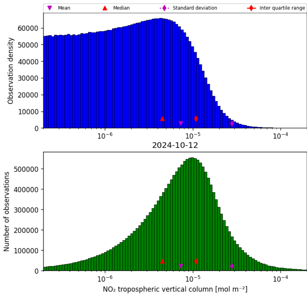
Figure 29: Histogram of “NO 2 tropospheric vertical column” for 2024-10-11 to 2024-10-13
