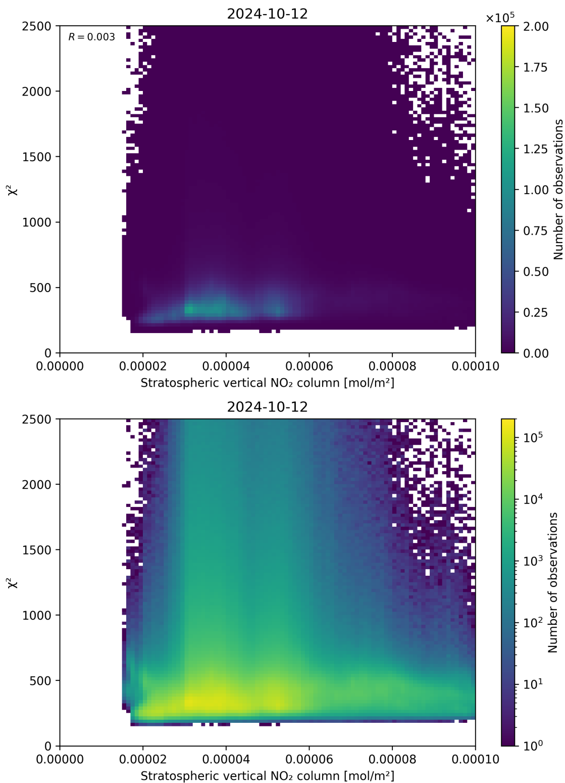
Figure 97: Scatter density plot of “Stratospheric vertical NO 2 column” against “ \chi^2 ” for 2024-10-11 to 2024-10-13.
