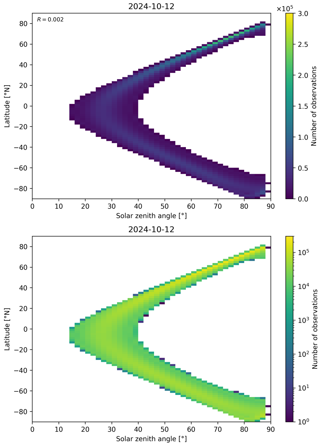
Figure 149: Scatter density plot of “Solar zenith angle” against “Latitude” for 2024-10-11 to 2024-10-13.
