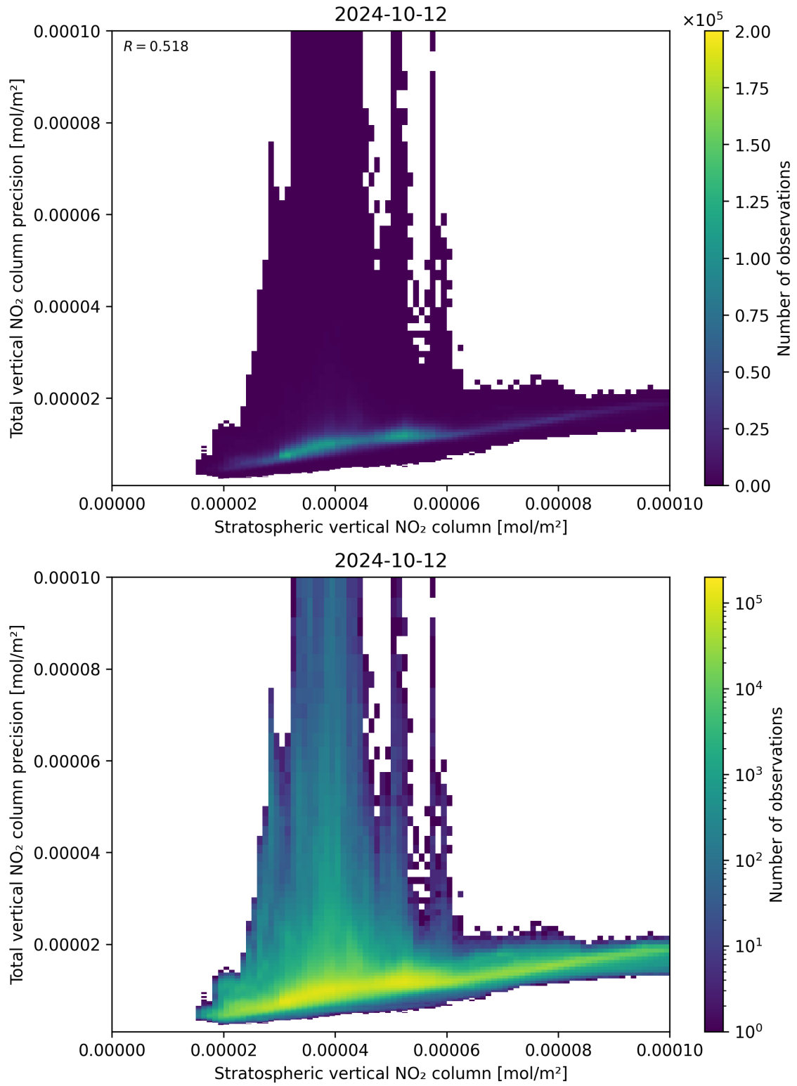
Figure 101: Scatter density plot of “Stratospheric vertical NO 2 column” against “Total vertical NO 2 column precision” for 2024-10-11 to 2024-10-13.
