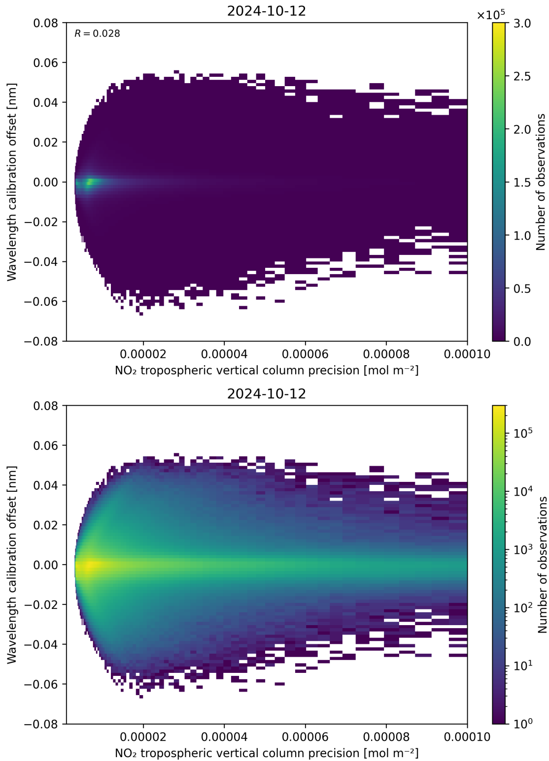
Figure 141: Scatter density plot of “NO 2 tropospheric vertical column precision” against “Wavelength calibration offset” for 2024-10-11 to 2024-10-13.
