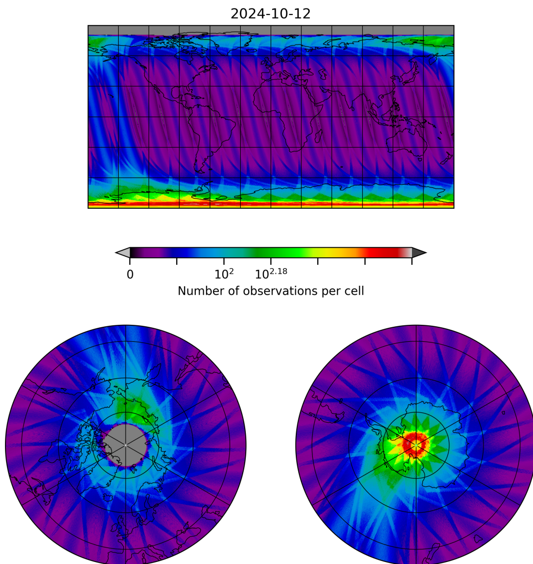
Figure 10: Map of the number of observations for 2024-10-11 to 2024-10-13
