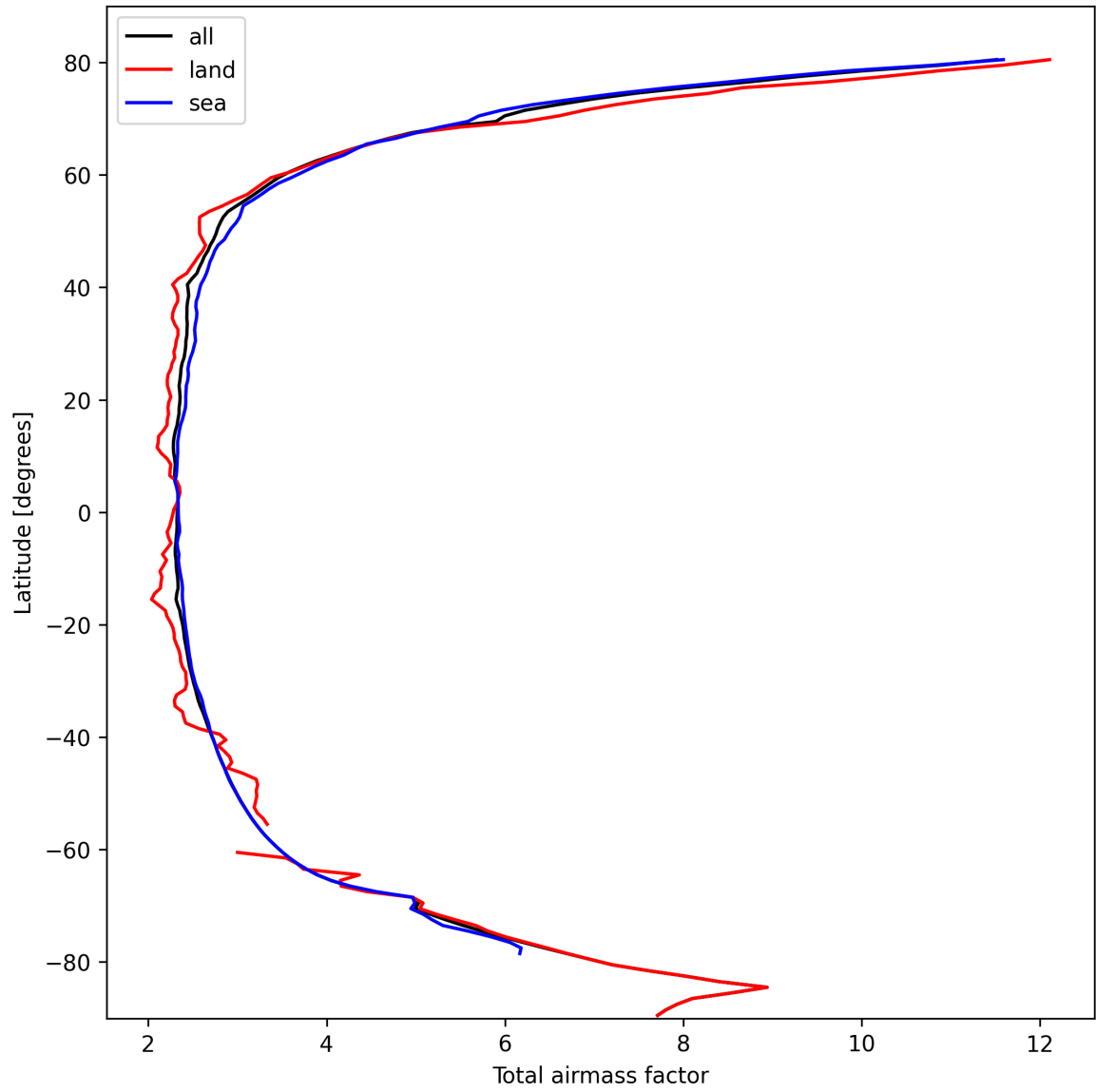
Figure 15: Zonal average of “Total airmass factor” for 2024-10-11 to 2024-10-13.
