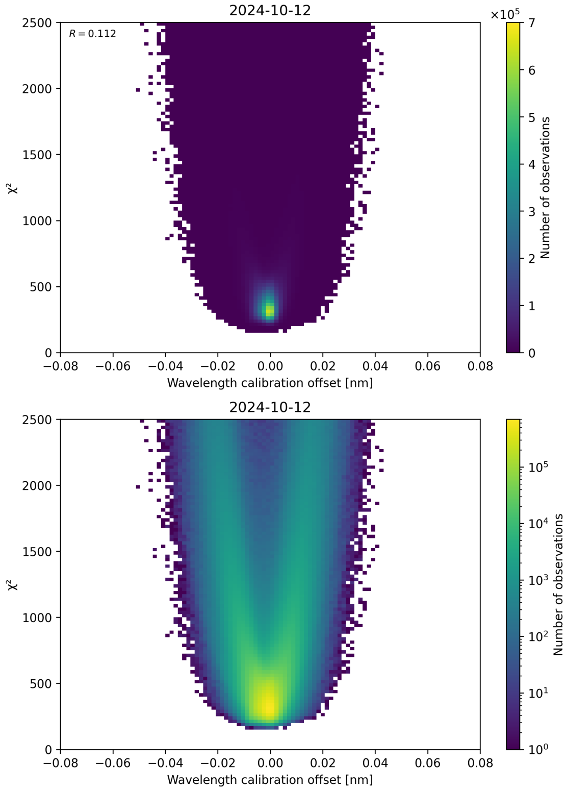
Figure 175: Scatter density plot of “Wavelength calibration offset” against “ \chi^2 ” for 2024-10-11 to 2024-10-13.
