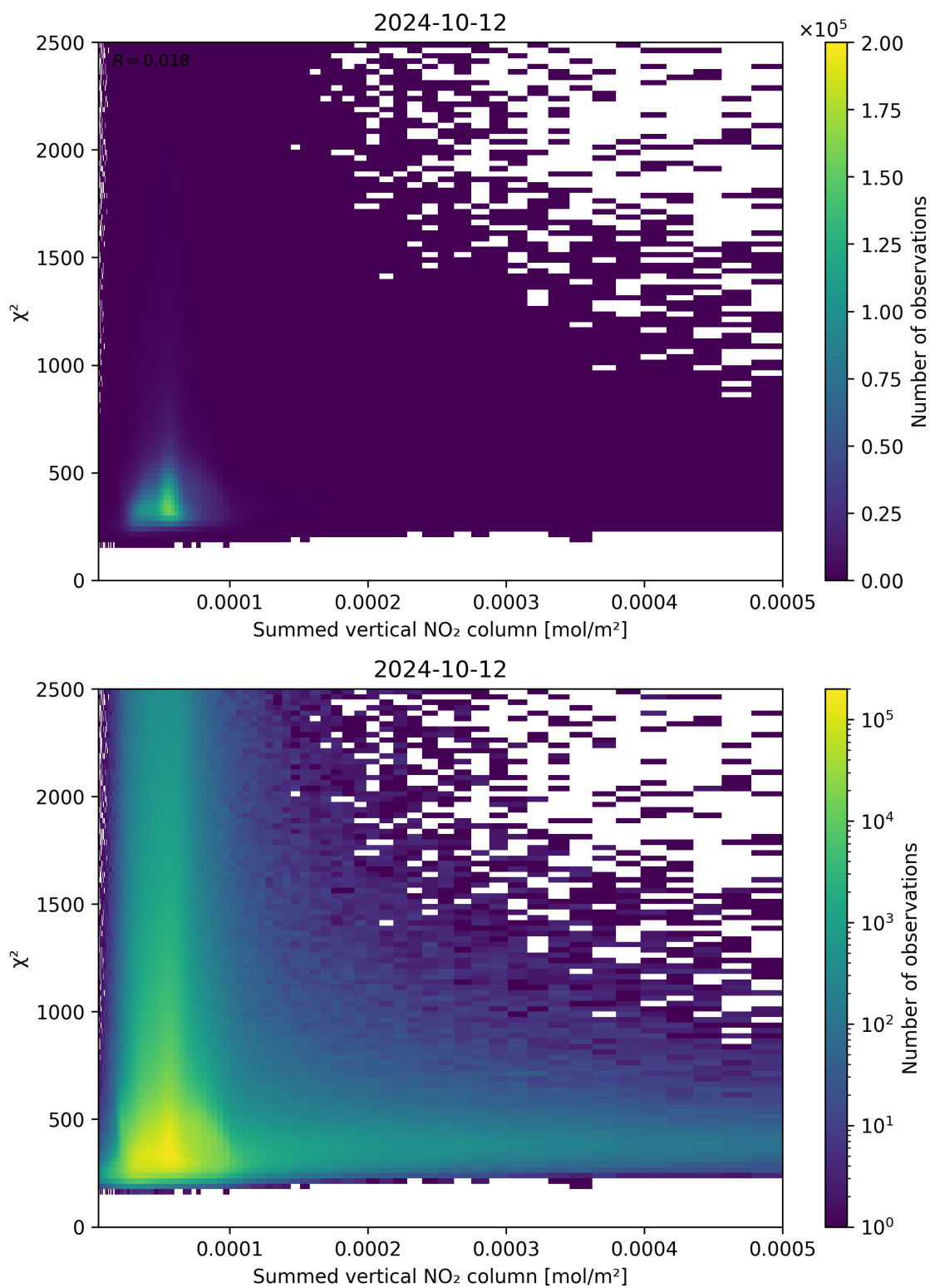
Figure 104: Scatter density plot of “Summed vertical NO 2 column” against “ \chi^2 ” for 2024-10-11 to 2024-10-13.
