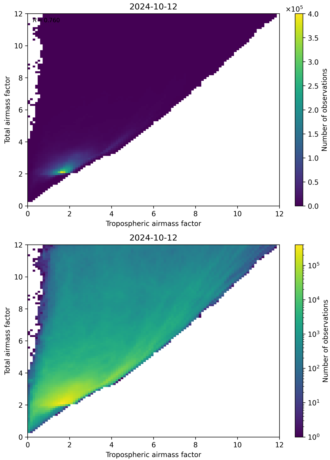
Figure 72: Scatter density plot of “Tropospheric airmass factor” against “Total airmass factor” for 2024-10-11 to 2024-10-13.
