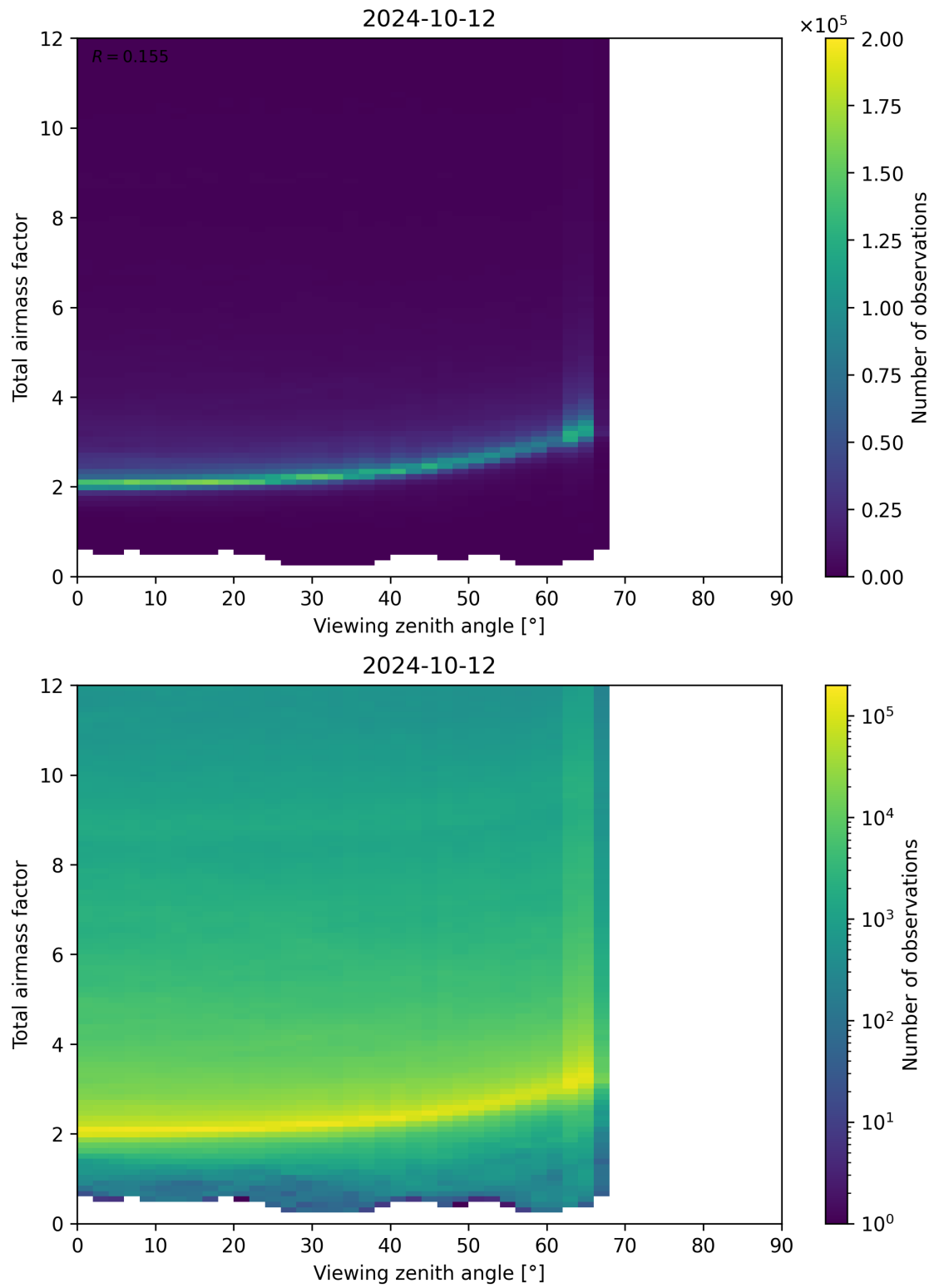
Figure 160: Scatter density plot of “Viewing zenith angle” against “Total airmass factor” for 2024-10-11 to 2024-10-13.
