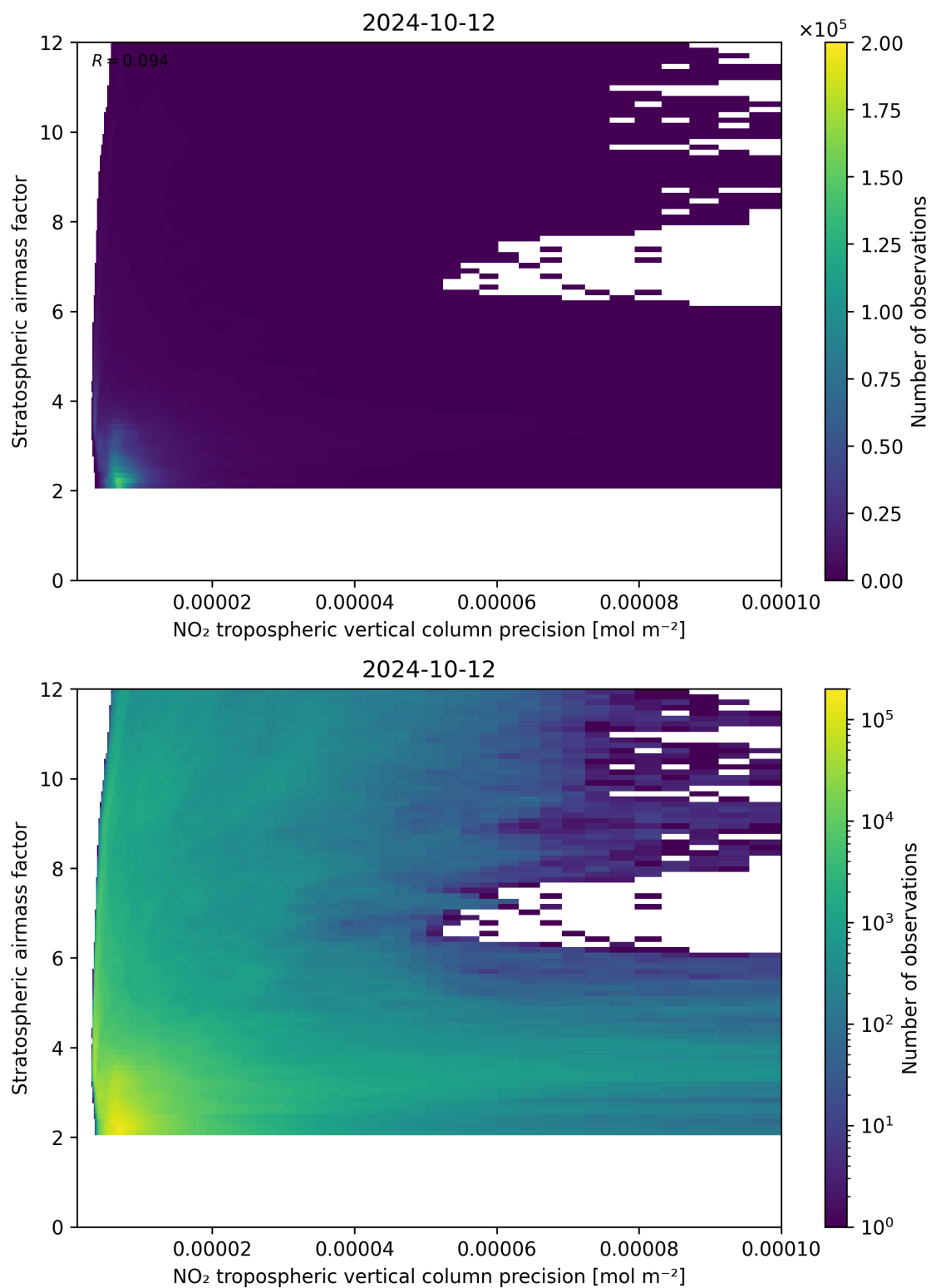
Figure 131: Scatter density plot of “NO 2 tropospheric vertical column precision” against “Stratospheric airmass factor” for 2024-10-11 to 2024-10-13.
