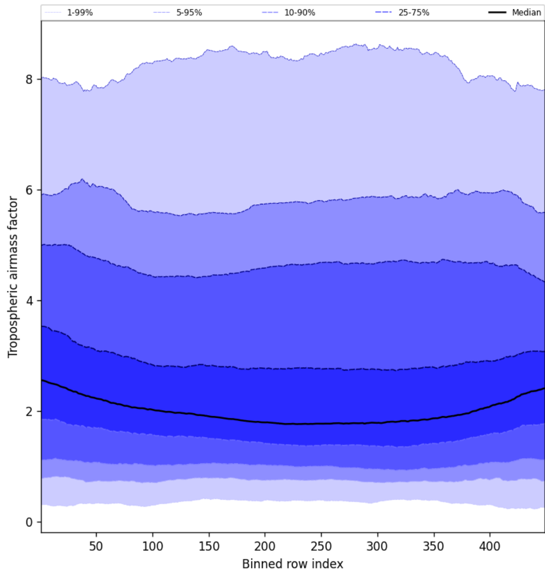
Figure 48: Along track statistics of “Tropospheric air mass factor” for 2024-10-11 to 2024-10-13
