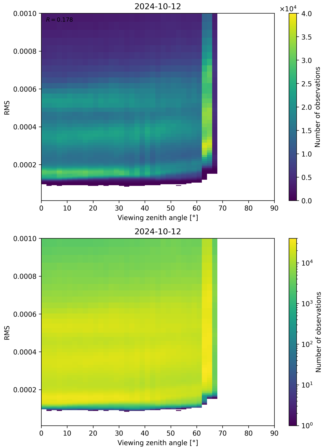
Figure 171: Scatter density plot of “Viewing zenith angle” against “RMS” for 2024-10-11 to 2024-10-13.
