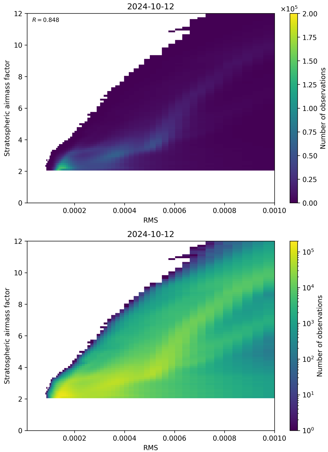
Figure 144: Scatter density plot of “RMS” against “Stratospheric airmass factor” for 2024-10-11 to 2024-10-13.
