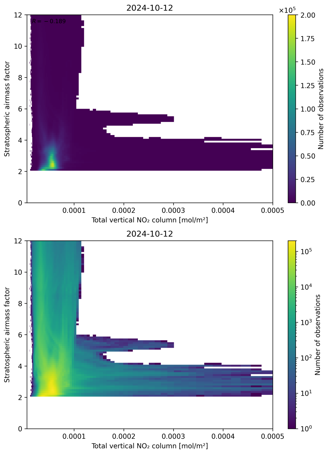
Figure 110: Scatter density plot of “Total vertical NO 2 column” against “Stratospheric airmass factor” for 2024-10-11 to 2024-10-13.
