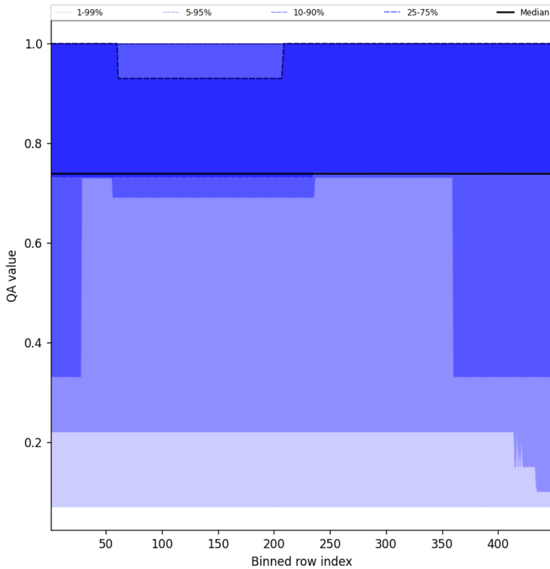
Figure 45: Along track statistics of “QA value” for 2024-10-11 to 2024-10-13
