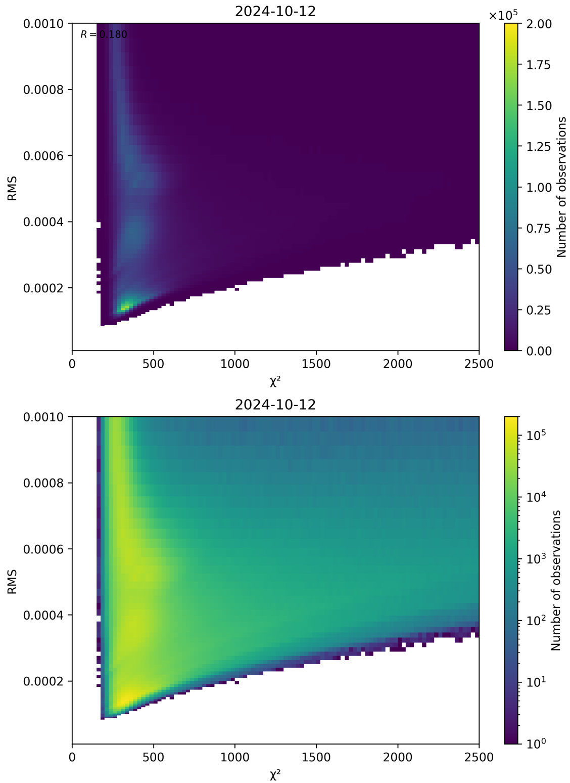
Figure 82: Scatter density plot of “ \chi^2 ” against “RMS” for 2024-10-11 to 2024-10-13.
