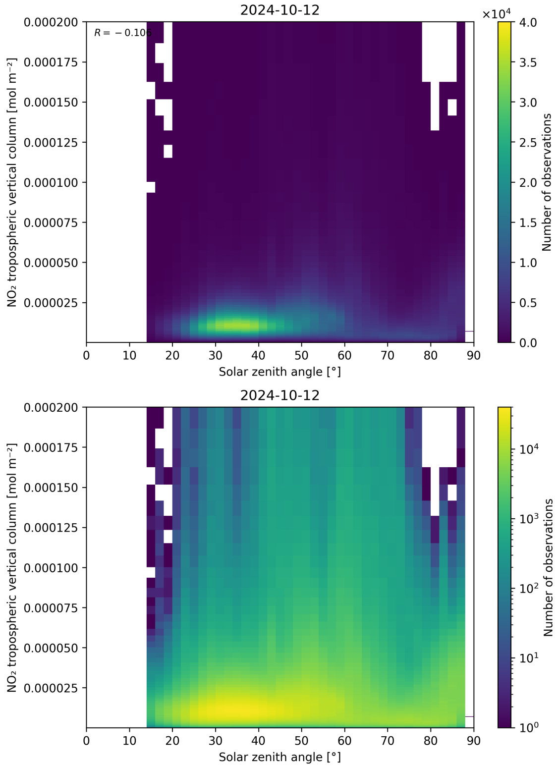
Figure 155: Scatter density plot of “Solar zenith angle” against “NO 2 tropospheric vertical column” for 2024-10-11 to 2024-10-13.
