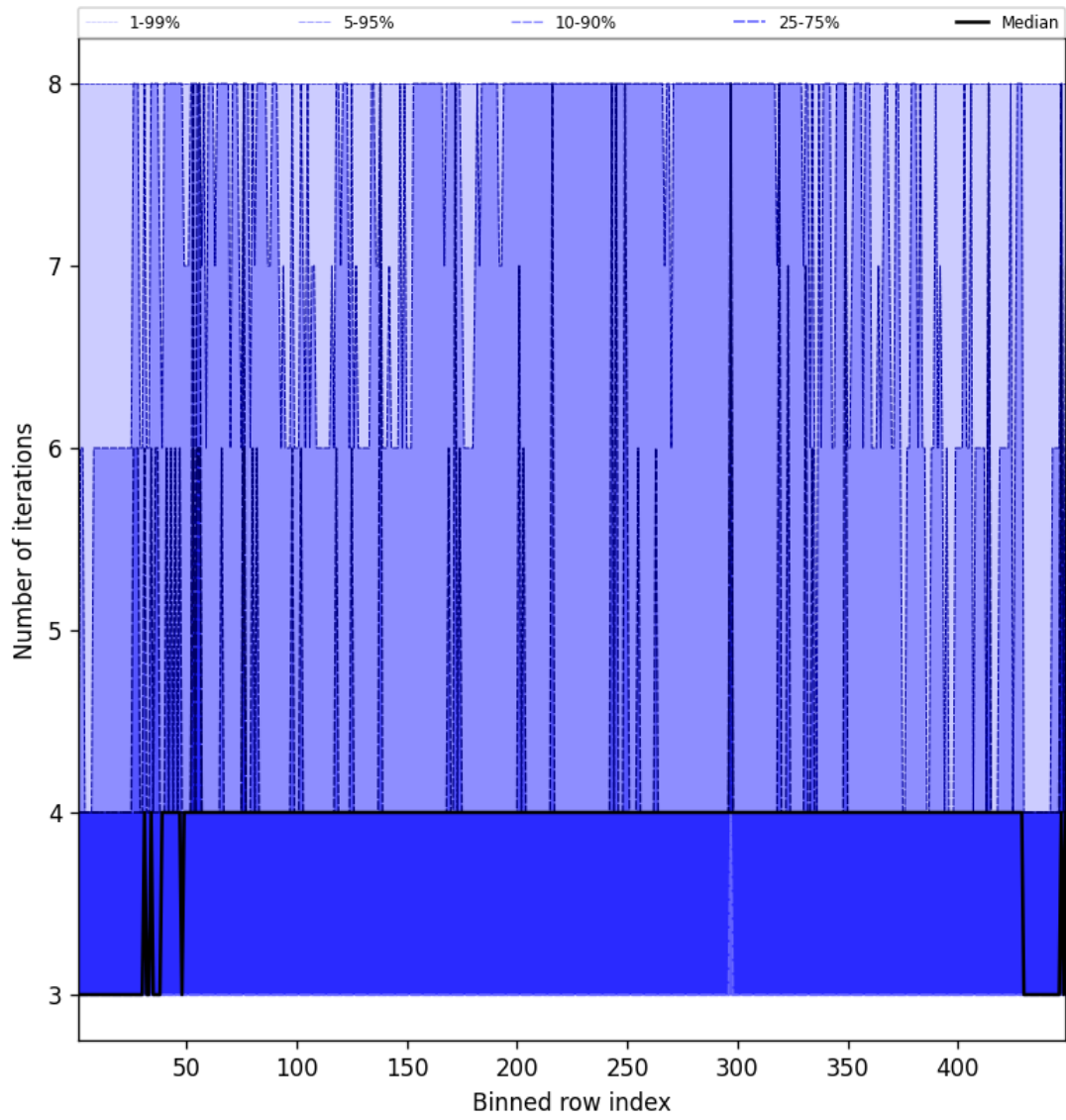
Figure 51: Along track statistics of “Number of iterations” for 2024-10-11 to 2024-10-13
