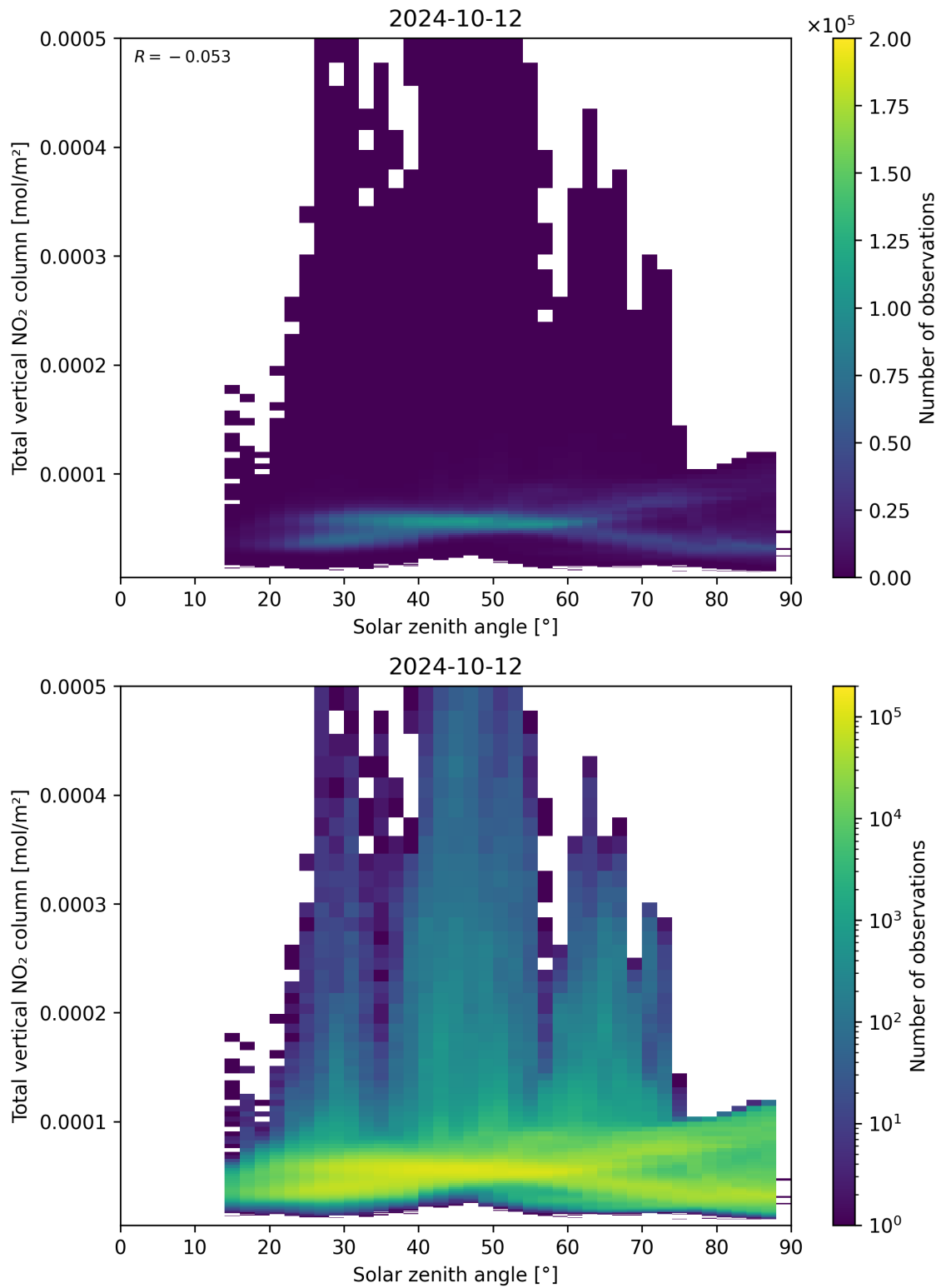
Figure 153: Scatter density plot of “Solar zenith angle” against “Total vertical NO 2 column” for 2024-10-11 to 2024-10-13.
