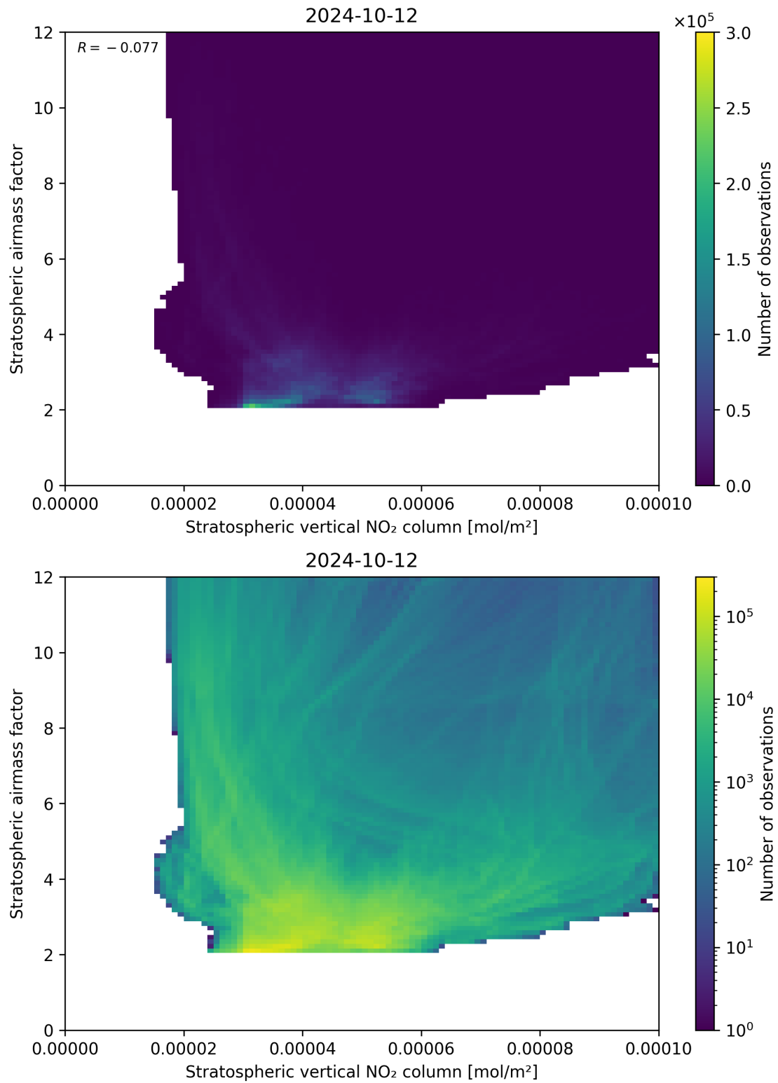
Figure 96: Scatter density plot of “Stratospheric vertical NO 2 column” against “Stratospheric airmass factor” for 2024-10-11 to 2024-10-13.
