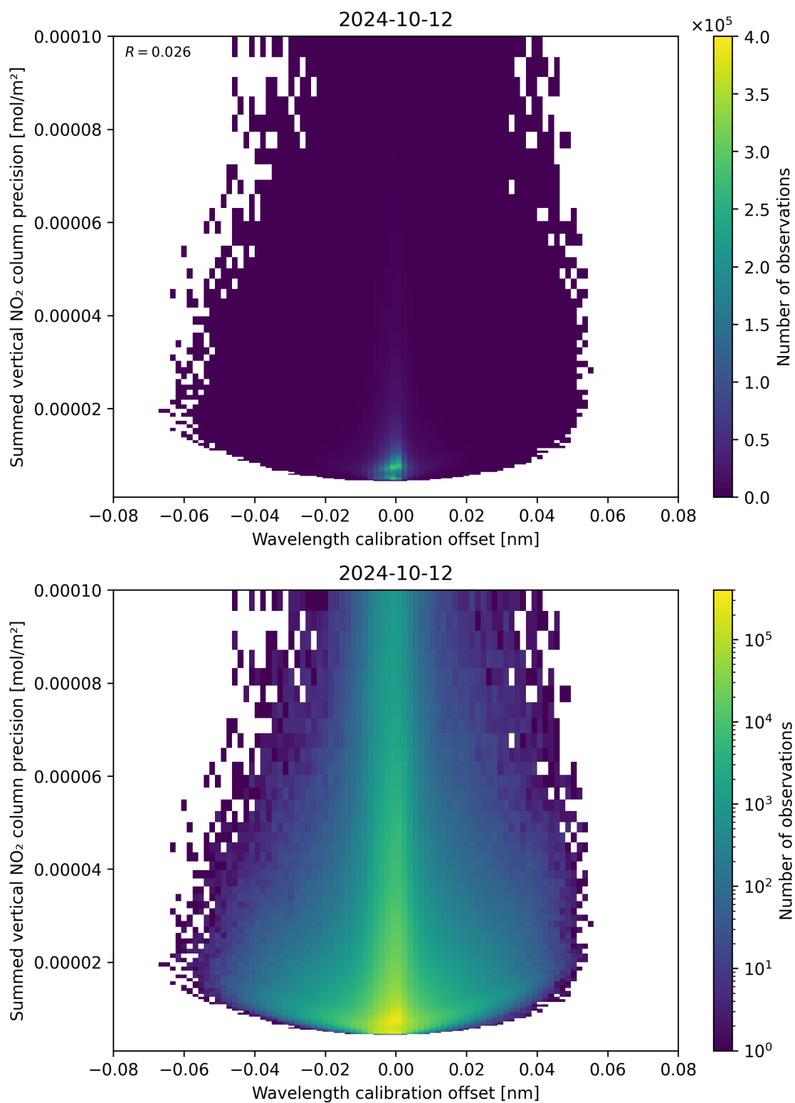
Figure 178: Scatter density plot of “Wavelength calibration offset” against “Summed vertical NO 2 column precision” for 2024-10-11 to 2024-10-13.
