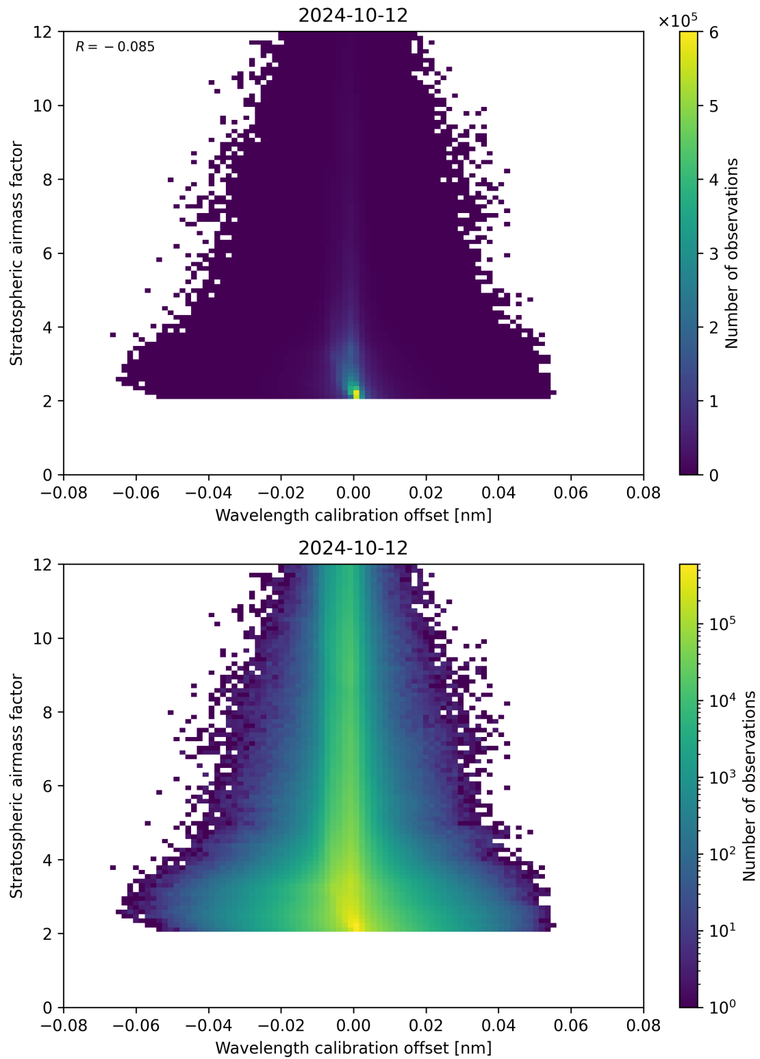
Figure 174: Scatter density plot of “Wavelength calibration offset” against “Stratospheric air mass factor” for 2024-10-11 to 2024-10-13.
