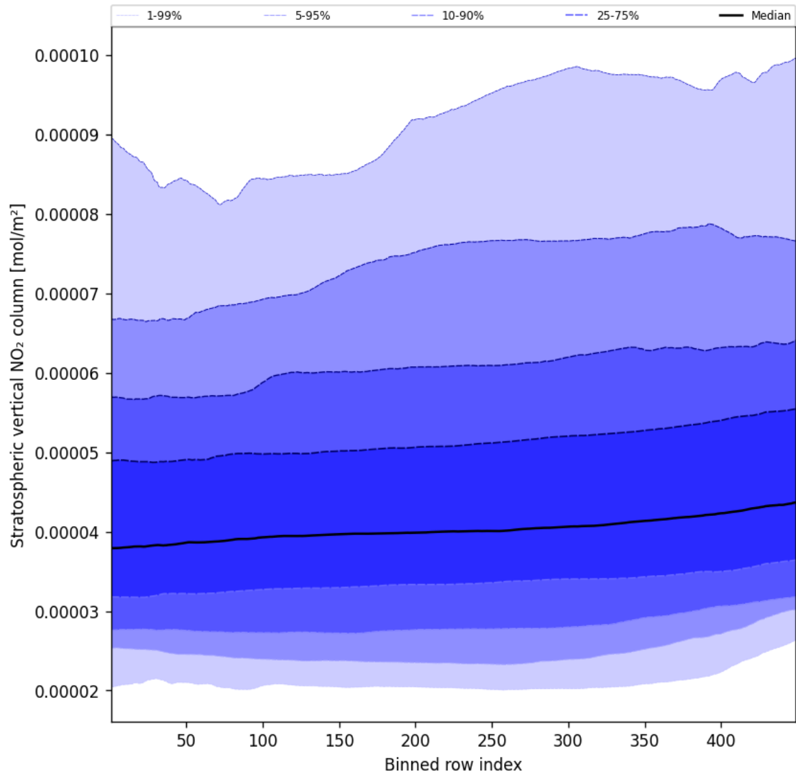
Figure 53: Along track statistics of “Stratospheric vertical NO 2 column” for 2024-10-11 to 2024-10-13
