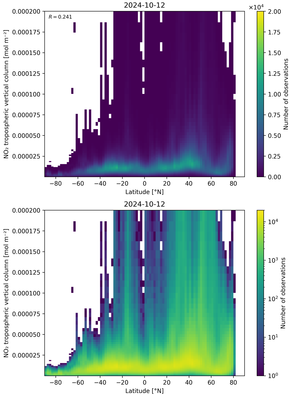
Figure 92: Scatter density plot of “Latitude” against “NO 2 tropospheric vertical column” for 2024-10-11 to 2024-10-13.
