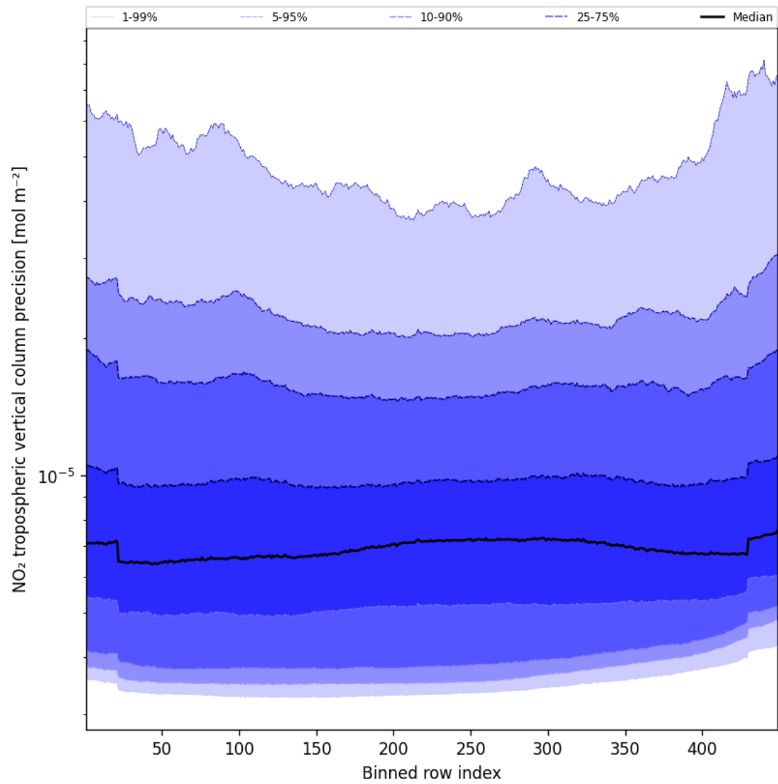
Figure 47: Along track statistics of “NO 2 tropospheric vertical column precision” for 2024-10-11 to 2024-10-13
