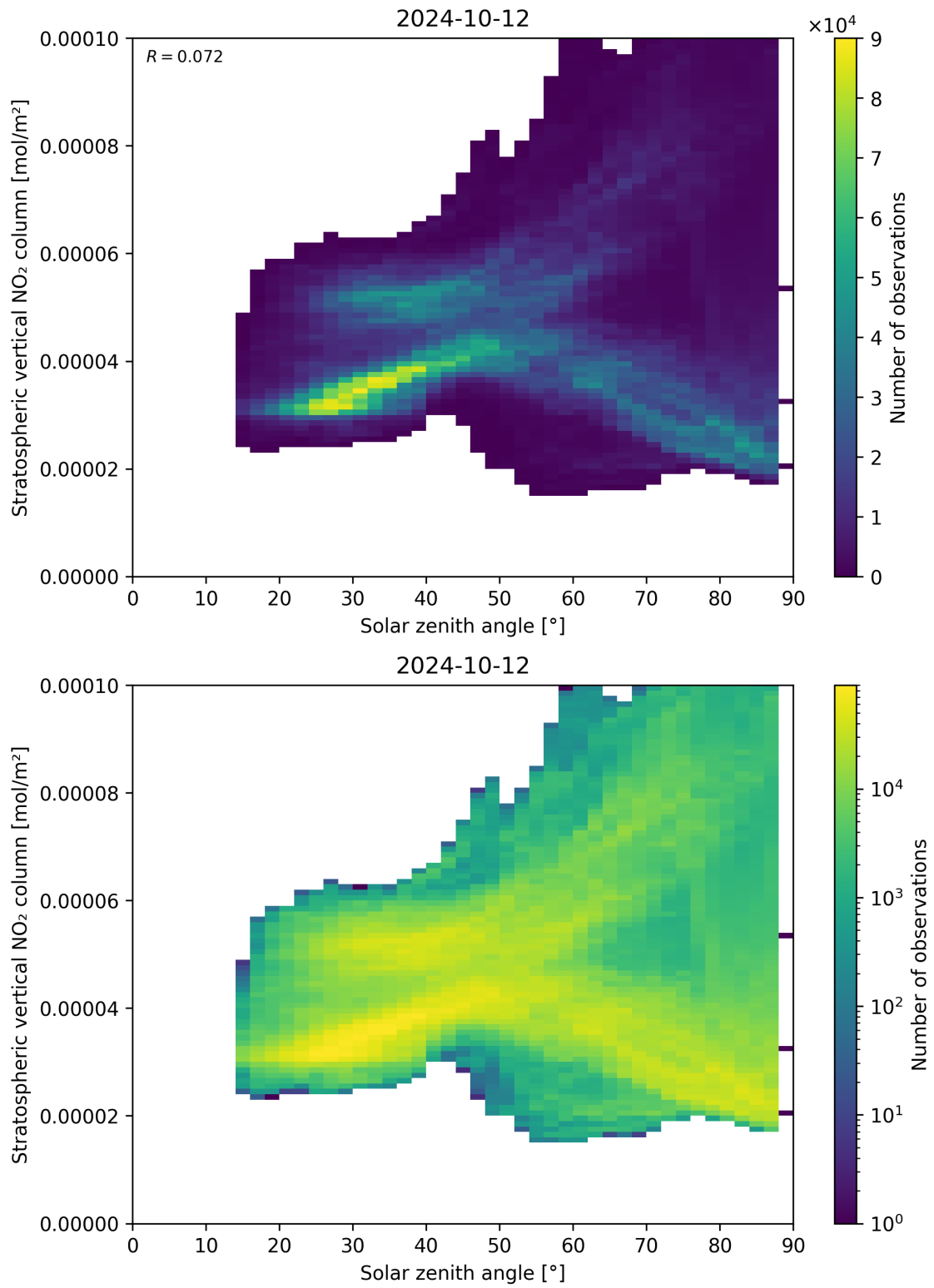
Figure 150: Scatter density plot of “Solar zenith angle” against “Stratospheric vertical NO 2 column” for 2024-10-11 to 2024-10-13.
