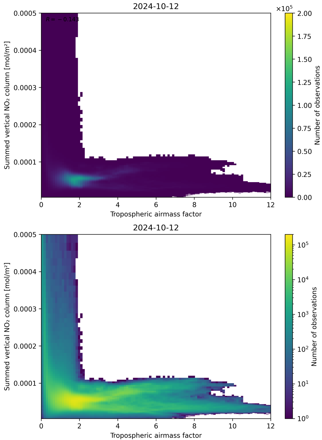
Figure 75: Scatter density plot of “Tropospheric air mass factor” against “Summed vertical NO 2 column” for 2024-10-11 to 2024-10-13.
