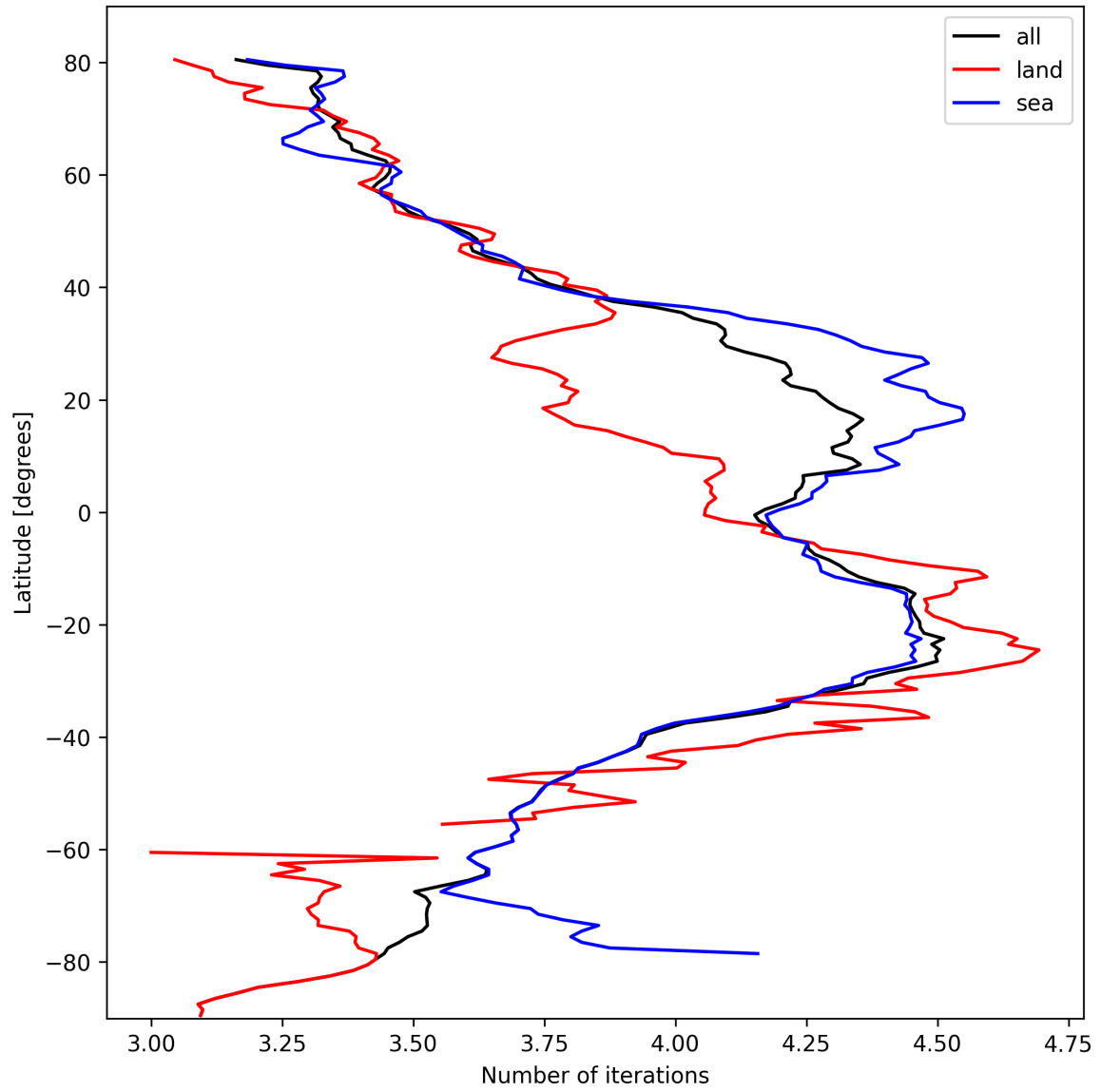
Figure 17: Zonal average of “Number of iterations” for 2024-10-11 to 2024-10-13.
