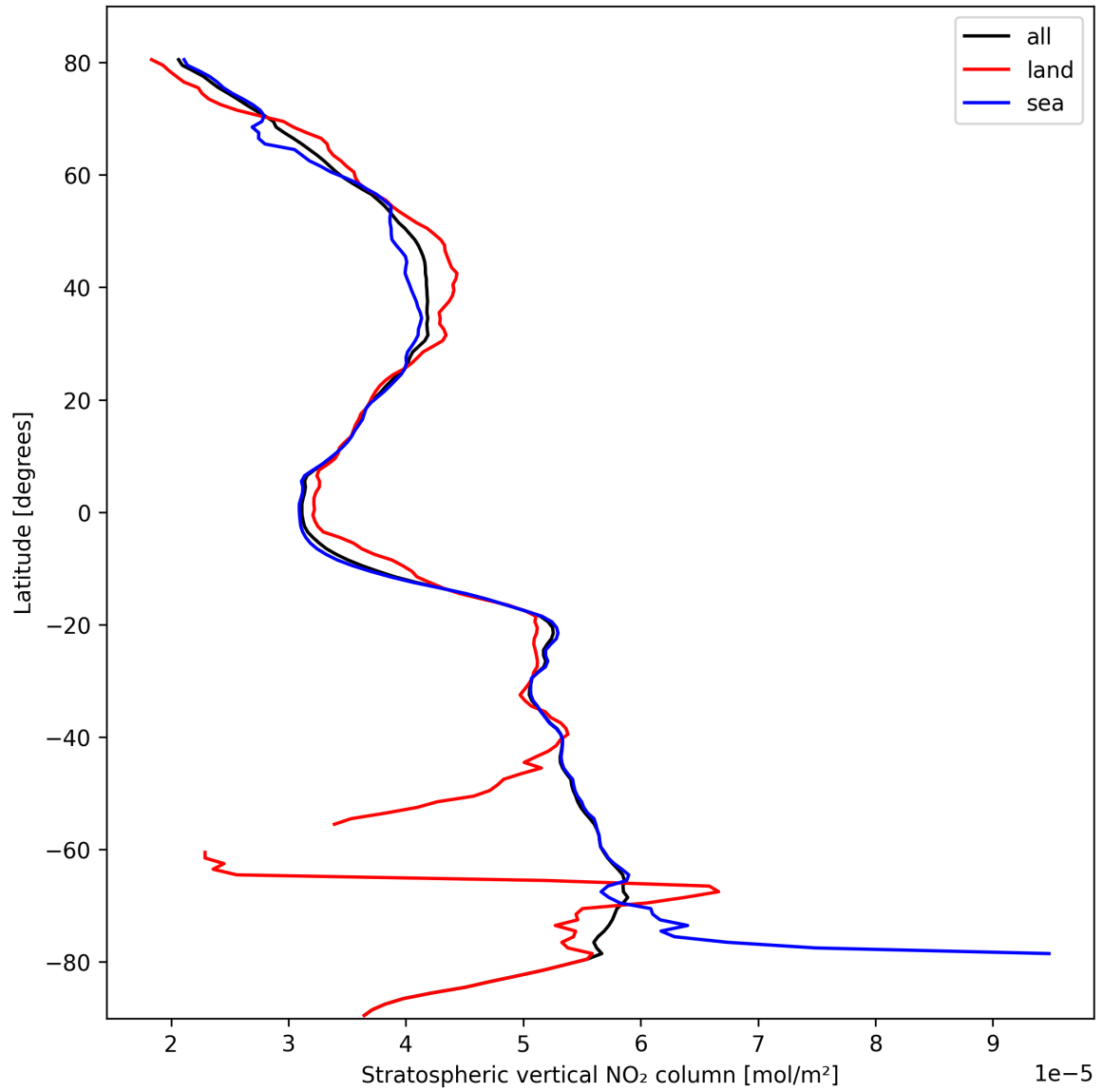
Figure 19: Zonal average of “Stratospheric vertical NO 2 column” for 2024-10-11 to 2024-10-13.
