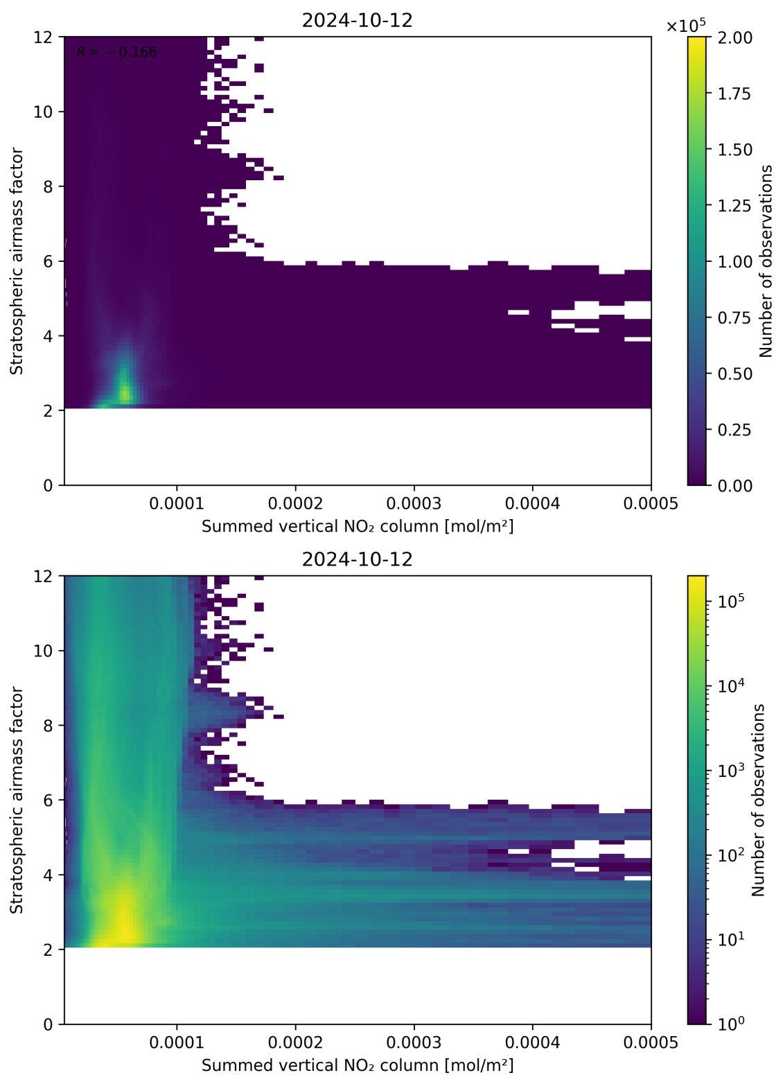
Figure 103: Scatter density plot of “Summed vertical NO 2 column” against “Stratospheric airmass factor” for 2024-10-11 to 2024-10-13.
