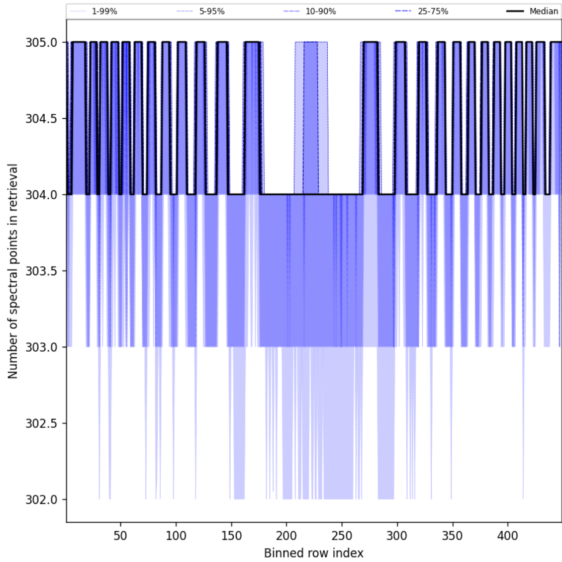
Figure 50: Along track statistics of “Number of spectral points in retrieval” for 2024-10-11 to 2024-10-13
