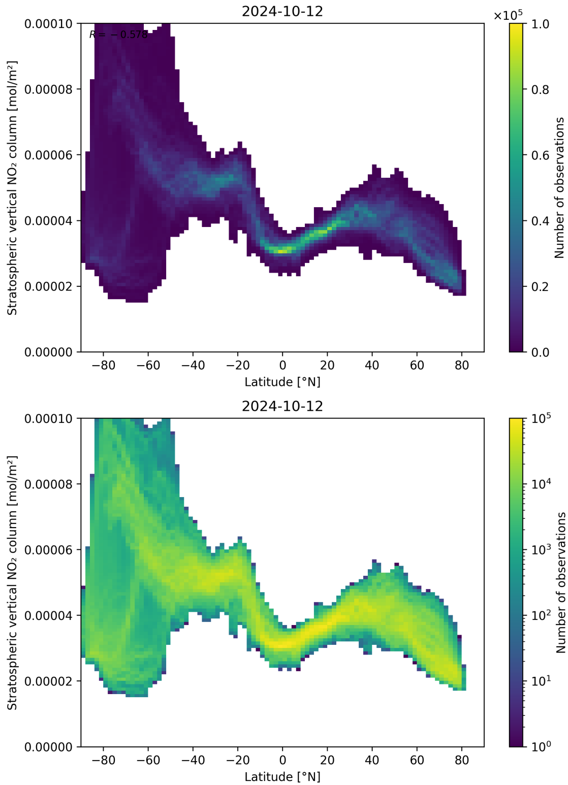
Figure 87: Scatter density plot of “Latitude” against “Stratospheric vertical NO 2 column” for 2024-10-11 to 2024-10-13.
