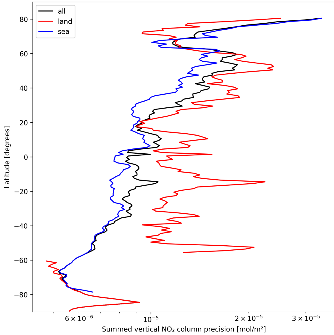
Figure 24: Zonal average of “Summed vertical NO 2 column precision” for 2024-10-11 to 2024-10-13.
