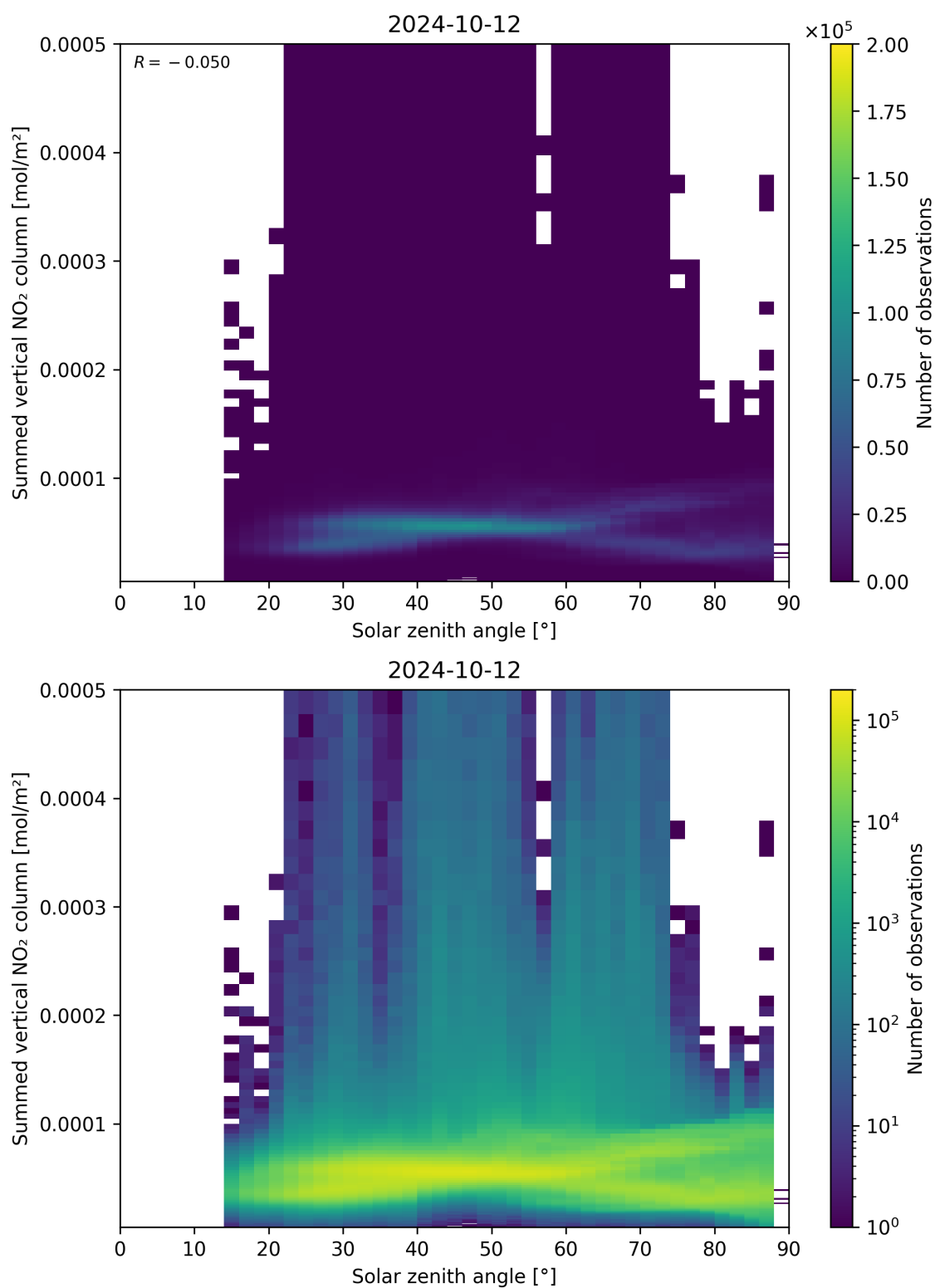
Figure 151: Scatter density plot of “Solar zenith angle” against “Summed vertical NO 2 column” for 2024-10-11 to 2024-10-13.
