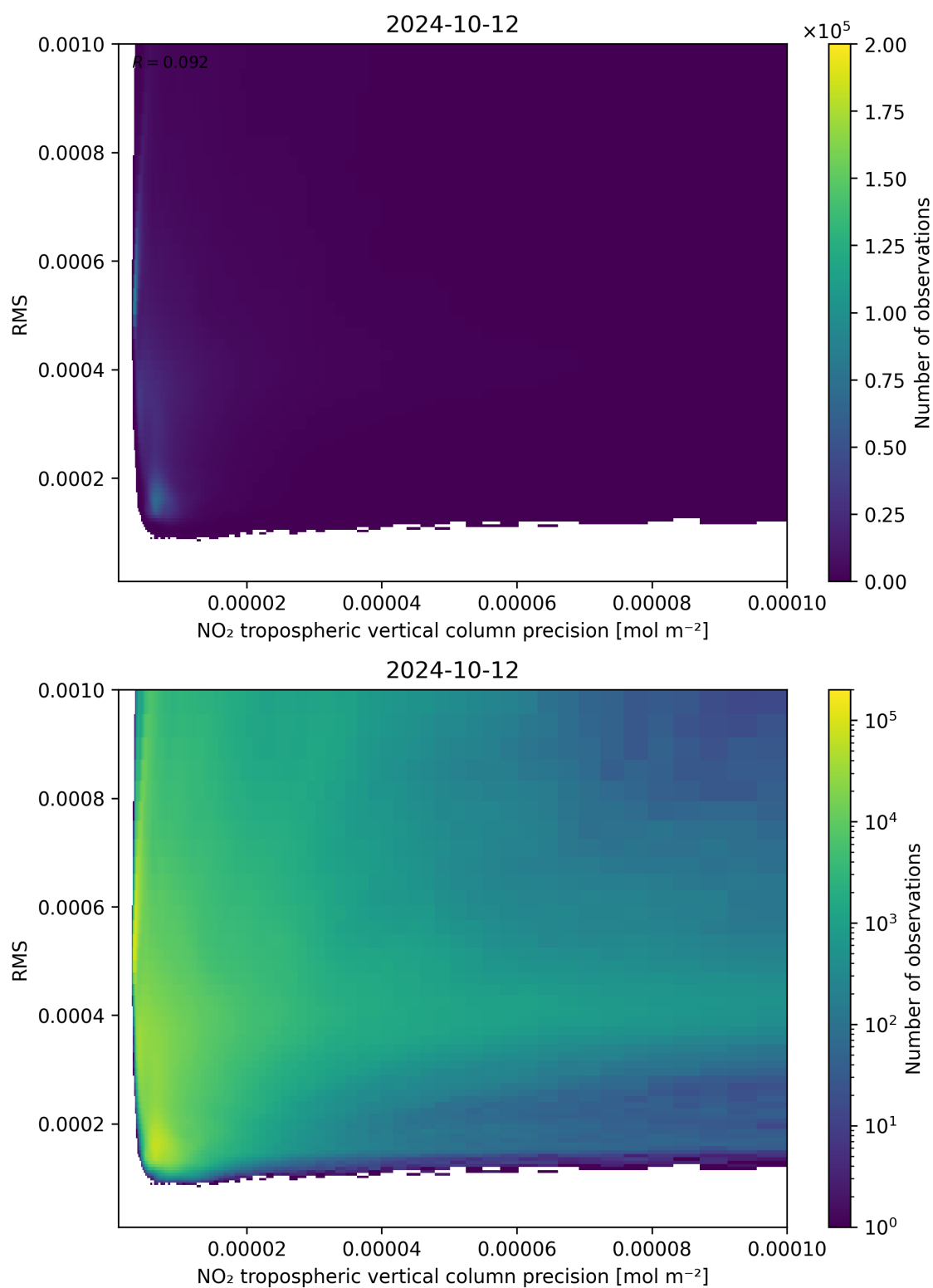
Figure 140: Scatter density plot of “NO 2 tropospheric vertical column precision” against “RMS” for 2024-10-11 to 2024-10-13.
