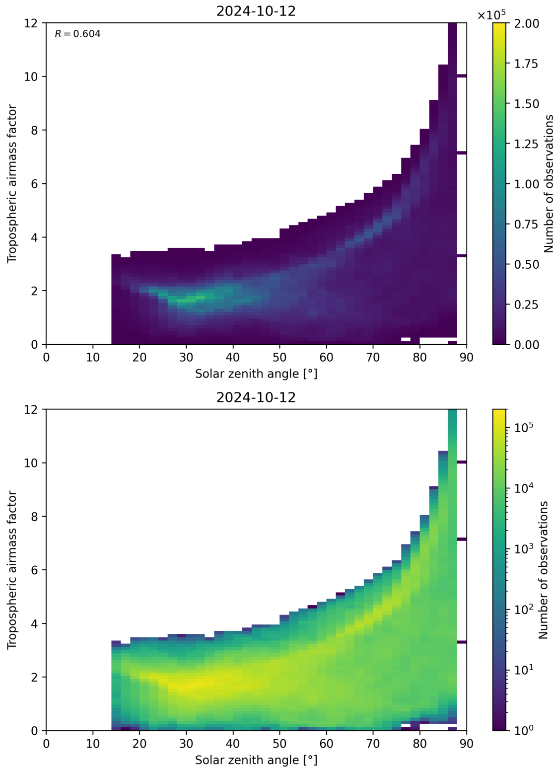
Figure 147: Scatter density plot of “Solar zenith angle” against “Tropospheric airmass factor” for 2024-10-11 to 2024-10-13.
