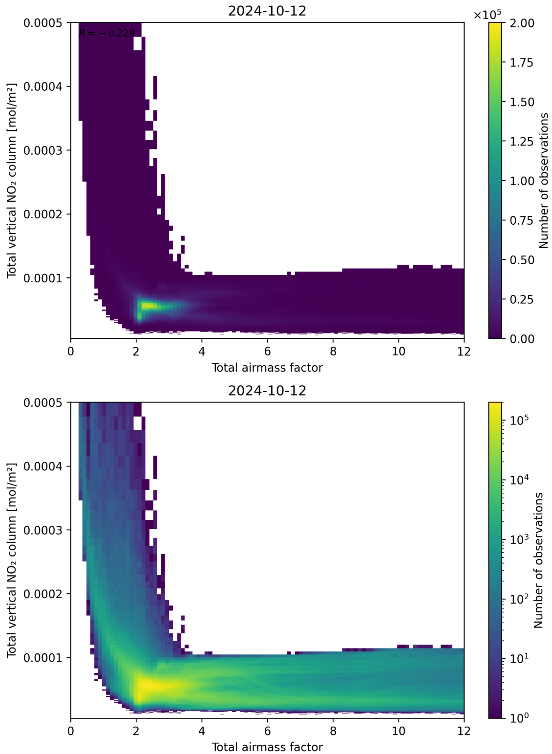
Figure 67: Scatter density plot of “Total airmass factor” against “Total vertical NO 2 column” for 2024-10-11 to 2024-10-13.
