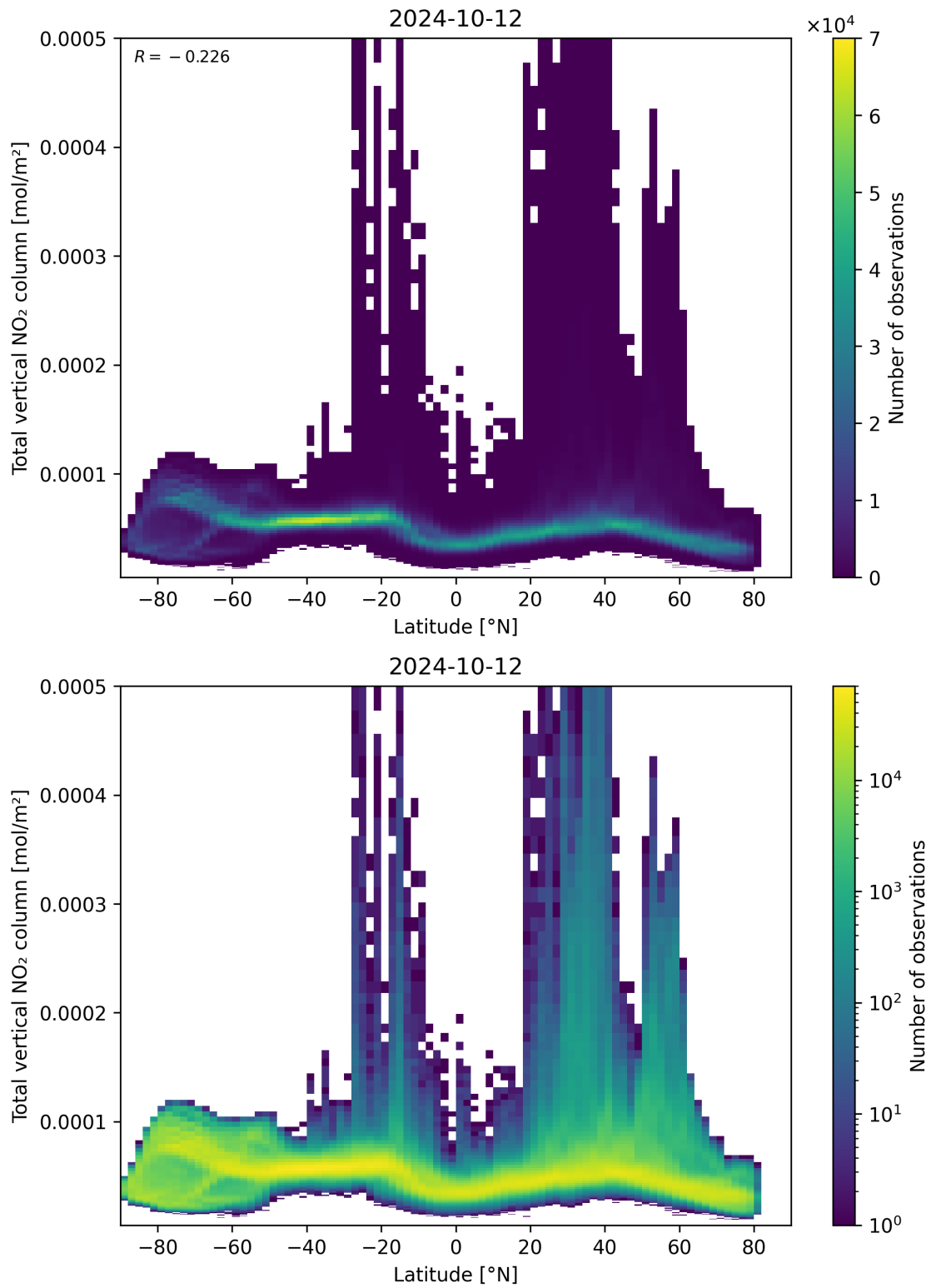
Figure 90: Scatter density plot of “Latitude” against “Total vertical NO 2 column” for 2024-10-11 to 2024-10-13.
