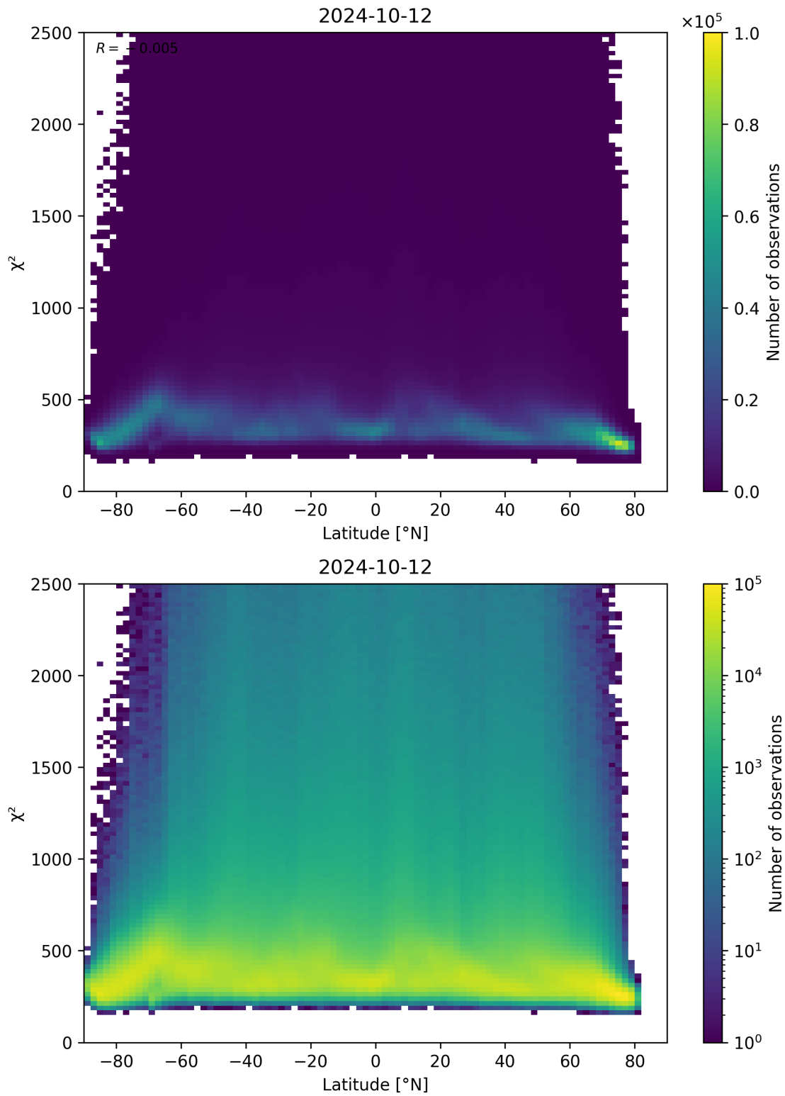
Figure 86: Scatter density plot of “Latitude” against “ \chi^2 ” for 2024-10-11 to 2024-10-13.
