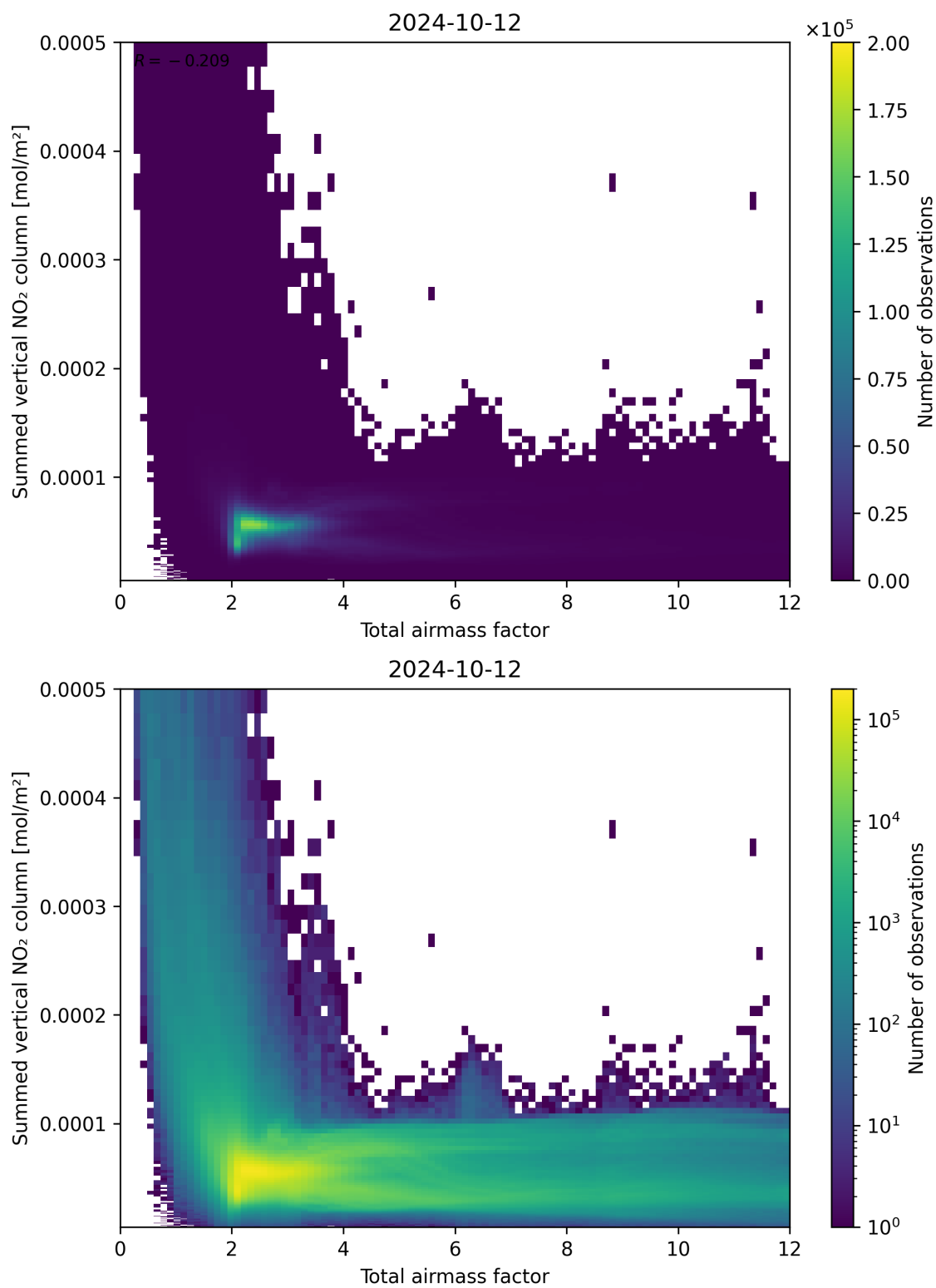
Figure 65: Scatter density plot of “Total airmass factor” against “Summed vertical NO 2 column” for 2024-10-11 to 2024-10-13.
