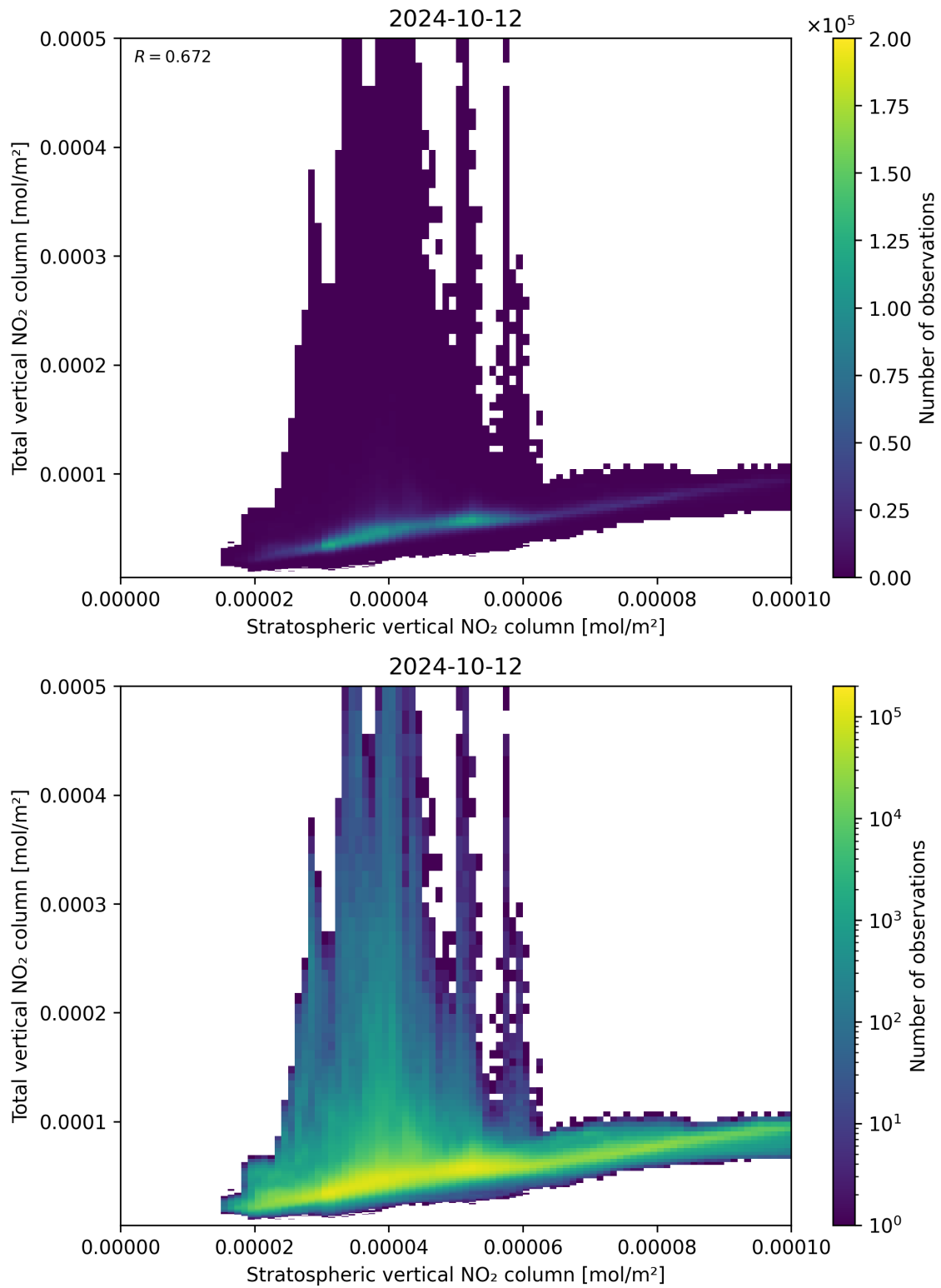
Figure 100: Scatter density plot of “Stratospheric vertical NO 2 column” against “Total vertical NO 2 column” for 2024-10-11 to 2024-10-13.
