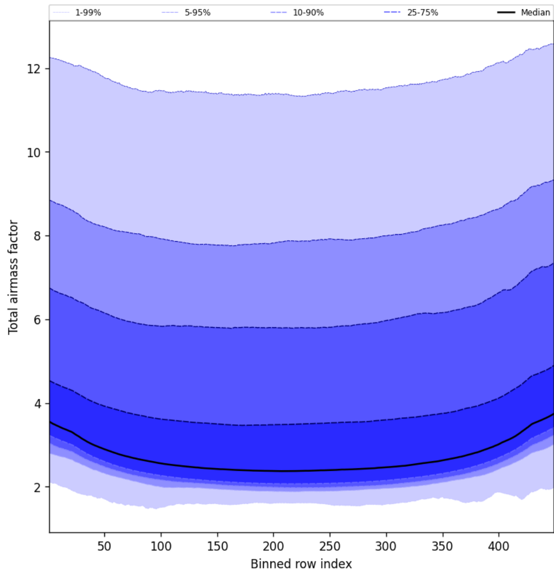
Figure 49: Along track statistics of “Total airmass factor” for 2024-10-11 to 2024-10-13
