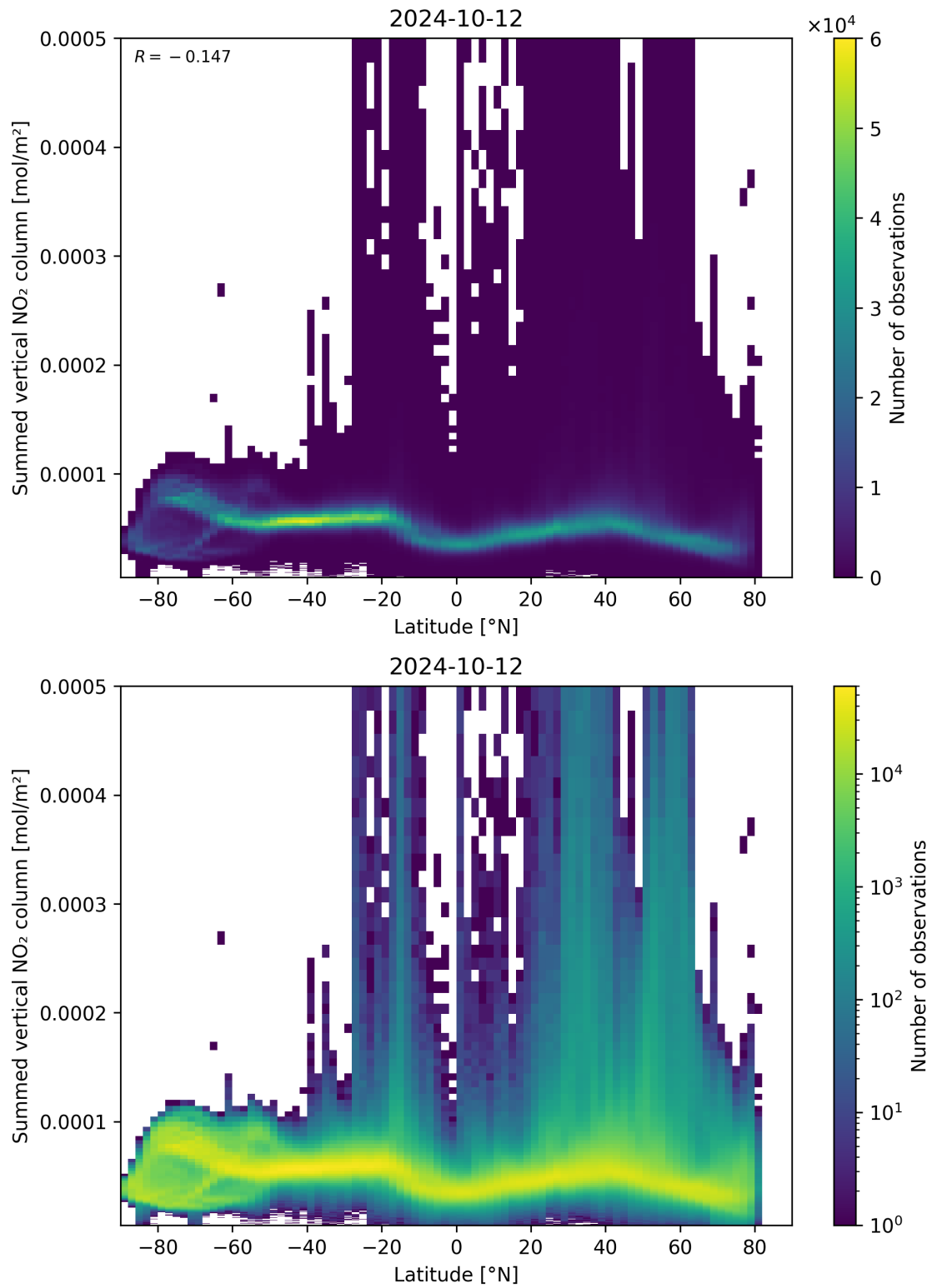
Figure 88: Scatter density plot of “Latitude” against “Summed vertical NO 2 column” for 2024-10-11 to 2024-10-13.
