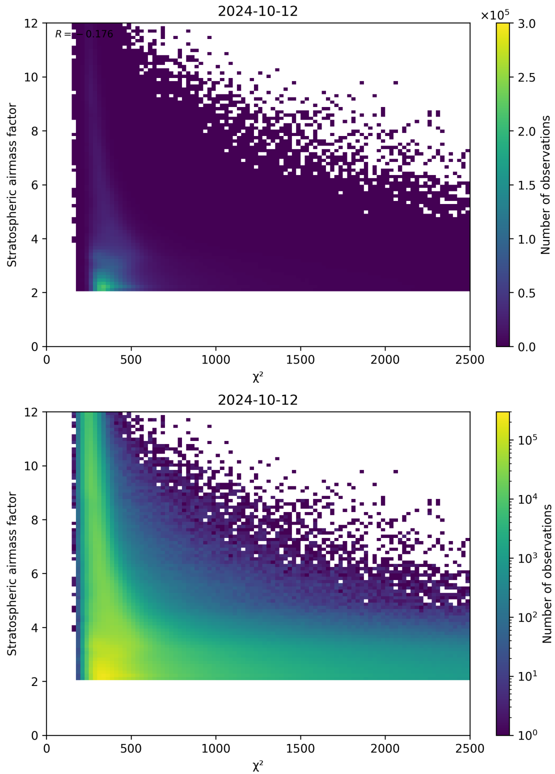
Figure 81: Scatter density plot of “ \chi^2 ” against “Stratospheric airmass factor” for 2024-10-11 to 2024-10-13.
