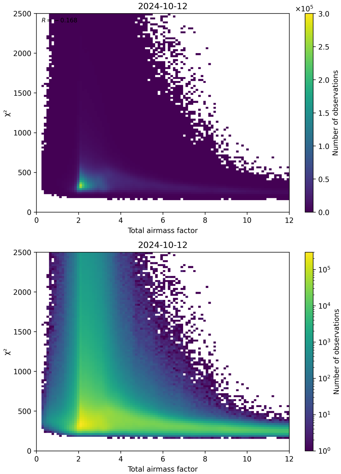
Figure 63: Scatter density plot of “Total airmass factor” against “ \chi^2 ” for 2024-10-11 to 2024-10-13.
