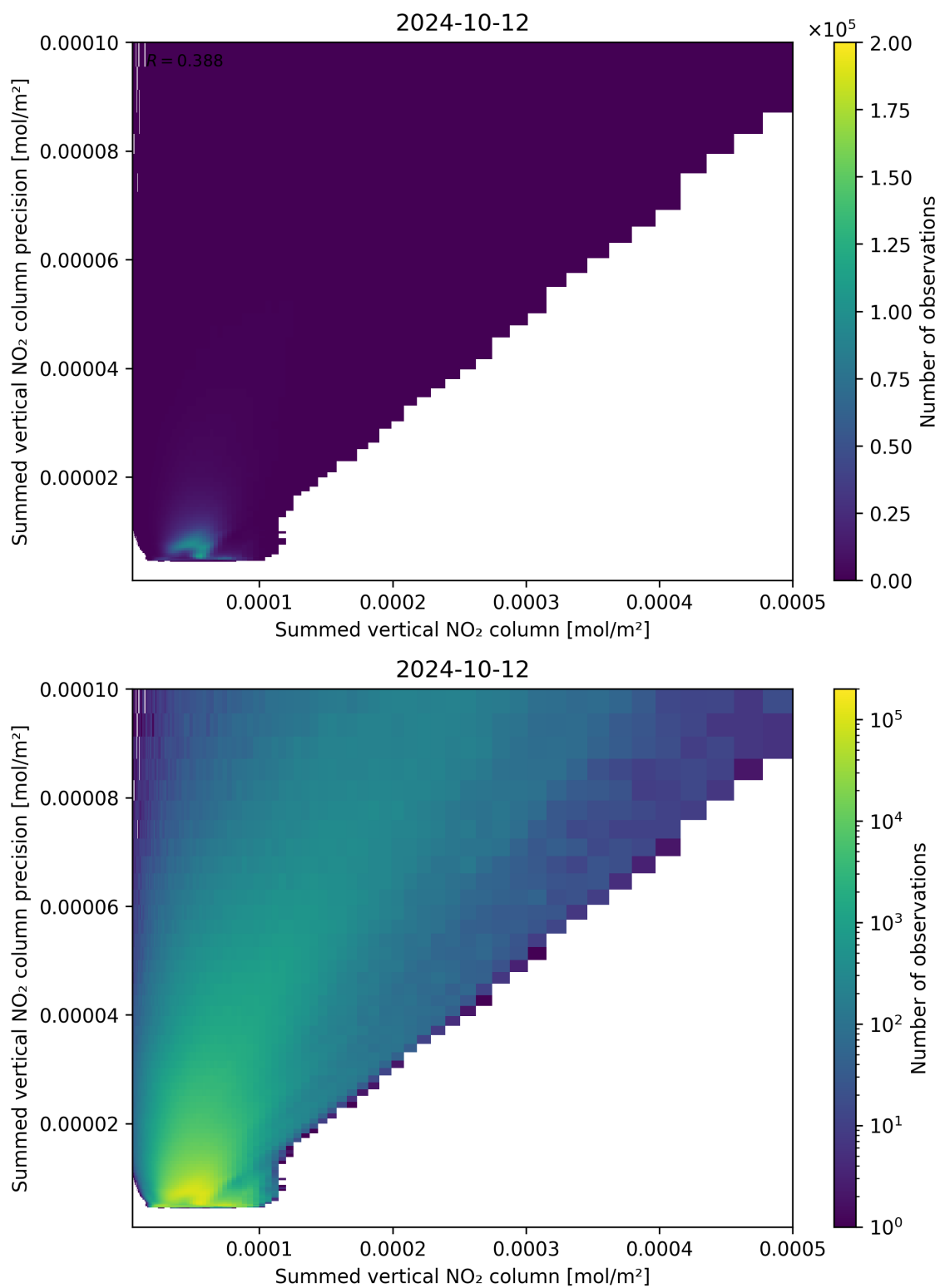
Figure 105: Scatter density plot of “Summed vertical NO 2 column” against “Summed vertical NO 2 column precision” for 2024-10-11 to 2024-10-13.
