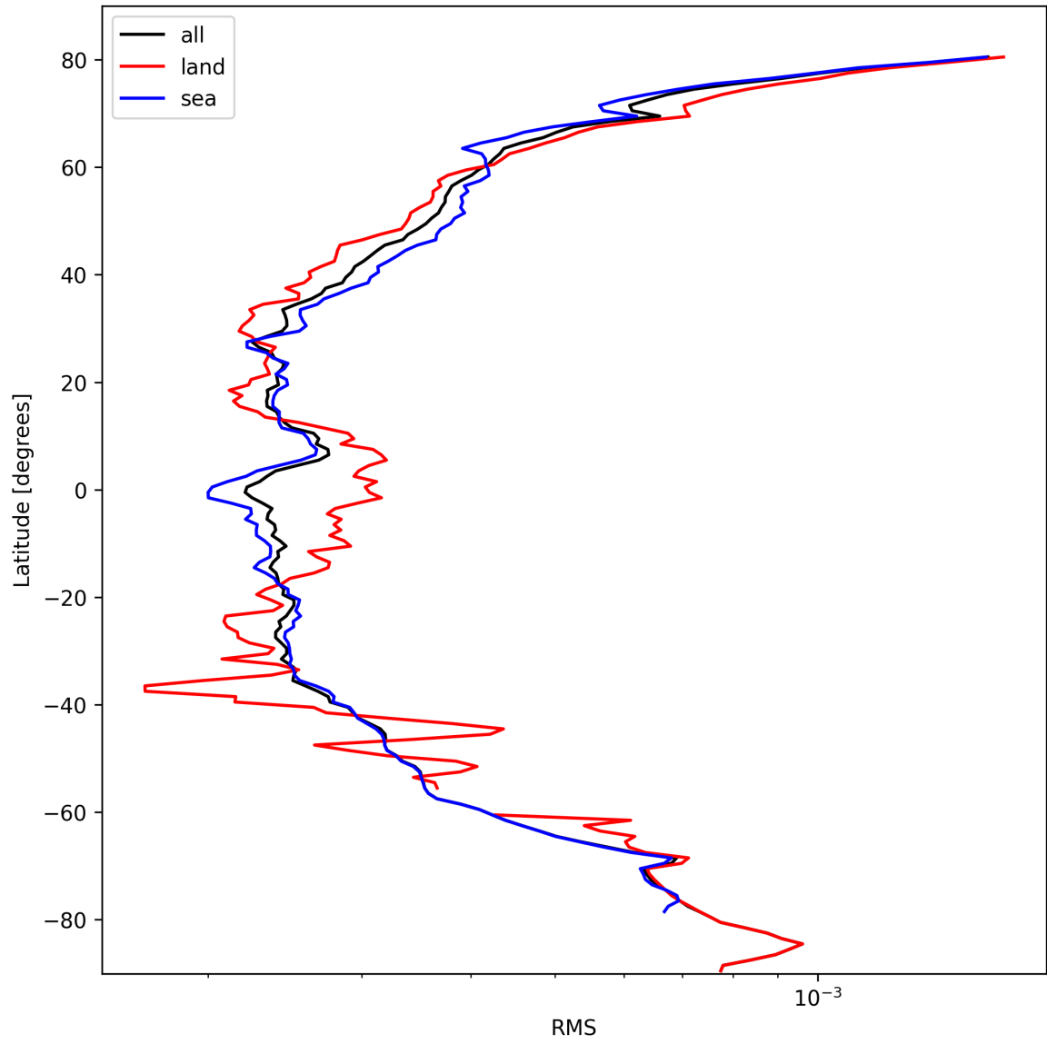
Figure 26: Zonal average of “RMS” for 2024-10-11 to 2024-10-13.
