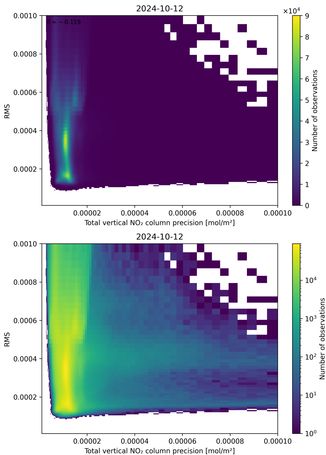
Figure 119: Scatter density plot of “Total vertical NO 2 column precision” against “RMS” for 2024-10-11 to 2024-10-13.
