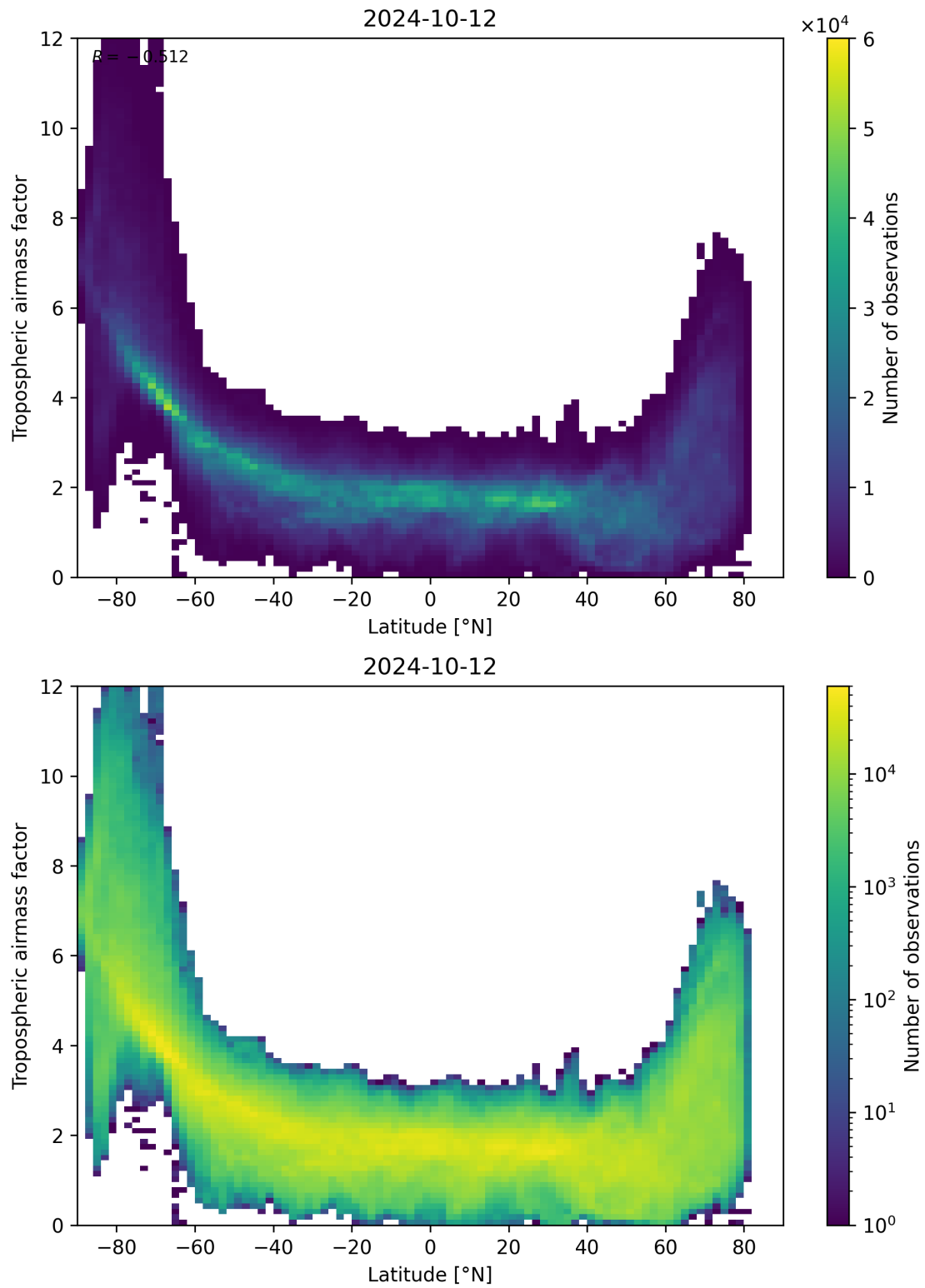
Figure 85: Scatter density plot of “Latitude” against “Tropospheric airmass factor” for 2024-10-11 to 2024-10-13.
