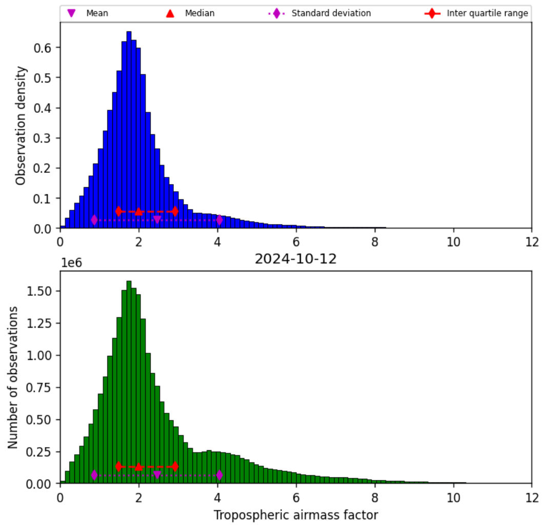
Figure 31: Histogram of “Tropospheric airmass factor” for 2024-10-11 to 2024-10-13
