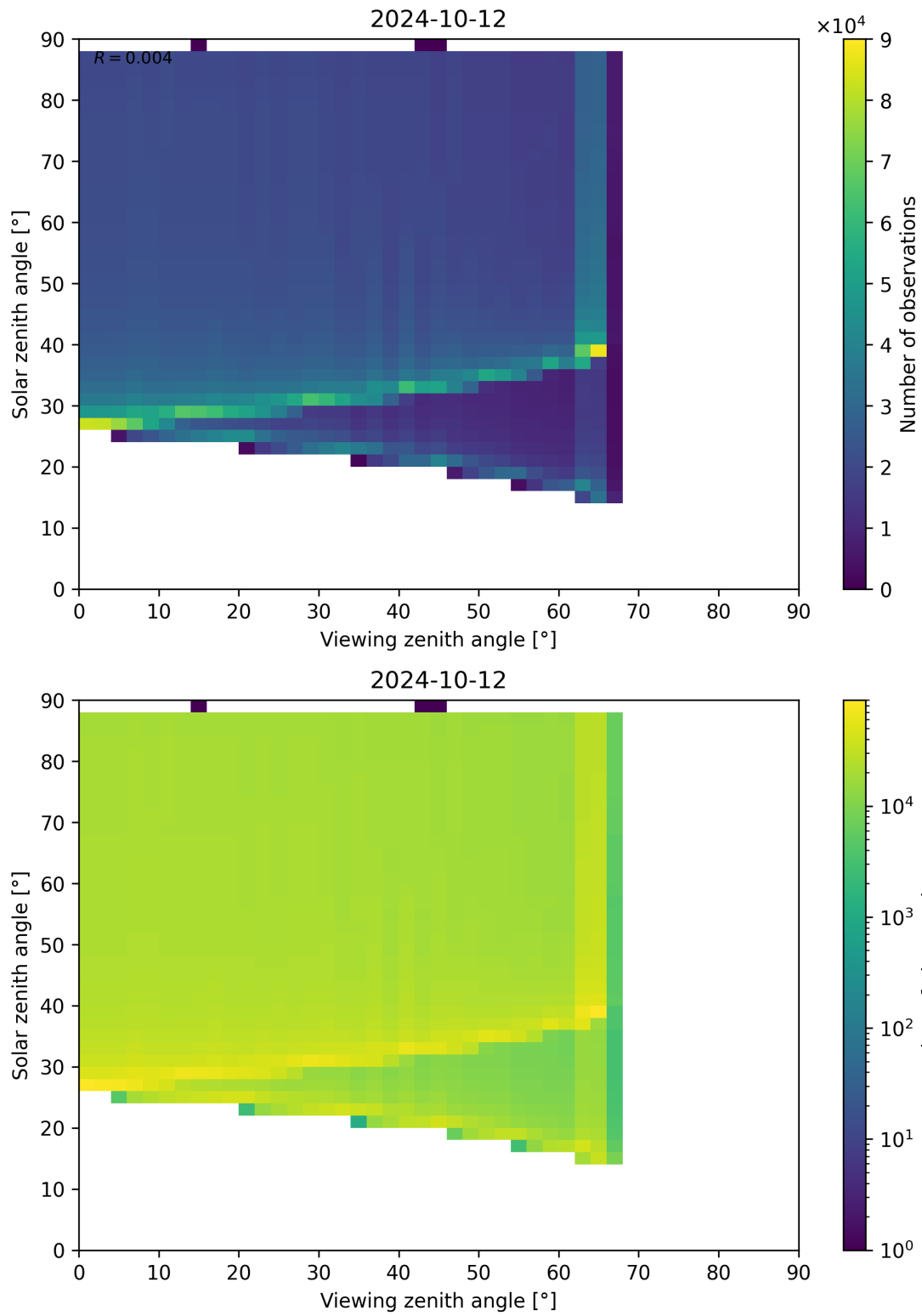
Figure 172: Scatter density plot of “Viewing zenith angle” against “Solar zenith angle” for 2024-10-11 to 2024-10-13.
