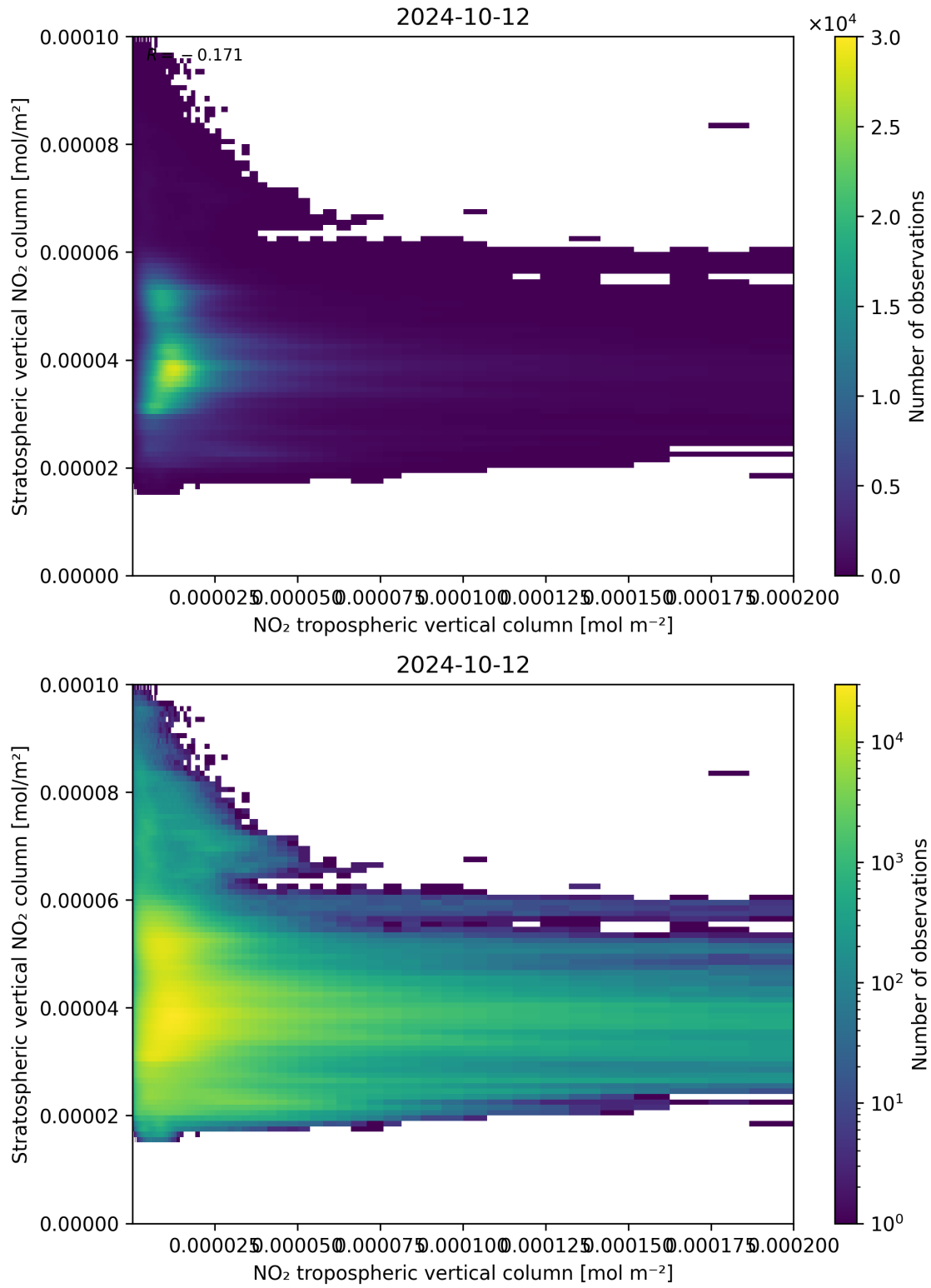
Figure 125: Scatter density plot of “NO 2 tropospheric vertical column” against “Stratospheric vertical NO 2 column” for 2024-10-11 to 2024-10-13.
