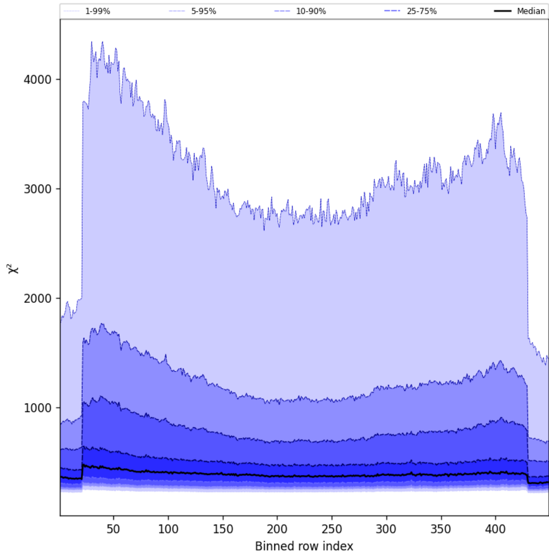
Figure 59: Along track statistics of “ \chi^2 ” for 2024-10-11 to 2024-10-13
