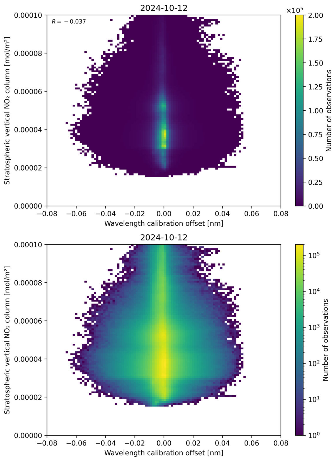
Figure 176: Scatter density plot of “Wavelength calibration offset” against “Stratospheric vertical NO 2 column” for 2024-10-11 to 2024-10-13.
