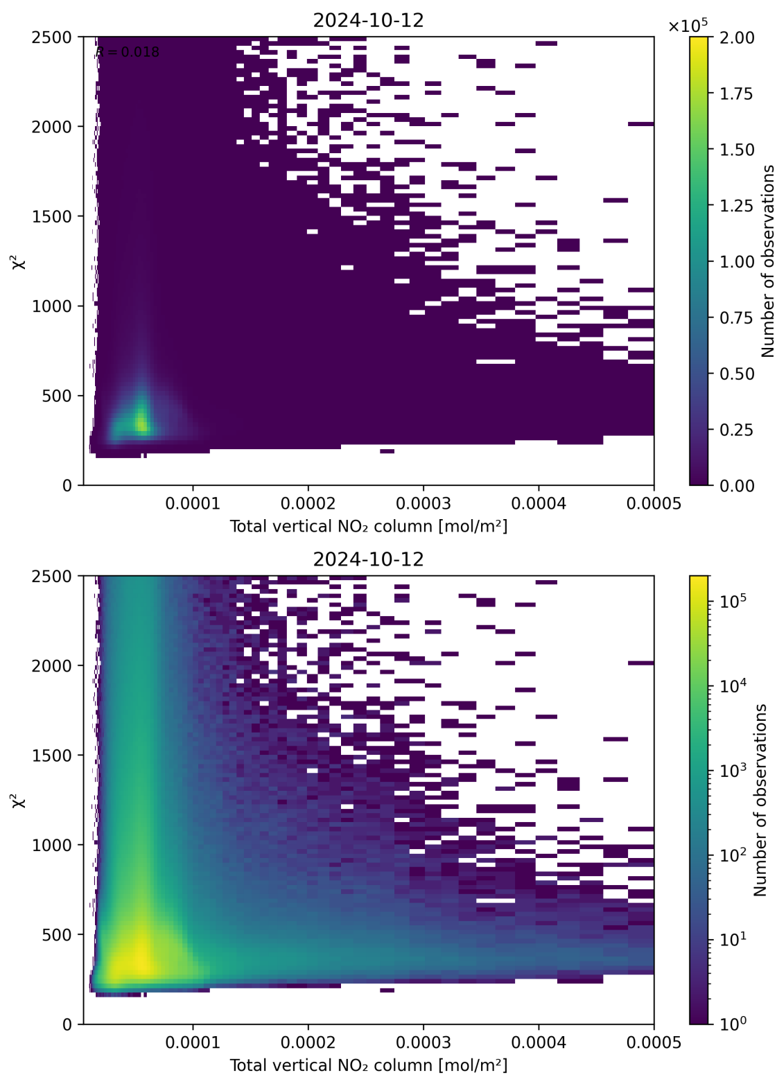
Figure 111: Scatter density plot of “Total vertical NO 2 column” against “ \chi^2 ” for 2024-10-11 to 2024-10-13.
