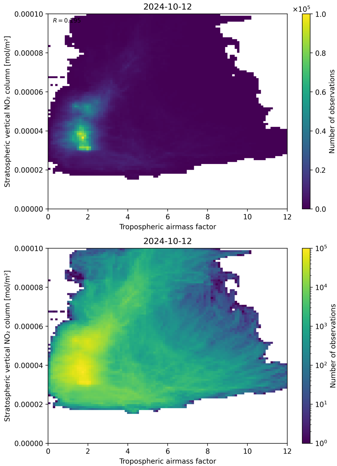
Figure 74: Scatter density plot of “Tropospheric air mass factor” against “Stratospheric vertical NO 2 column” for 2024-10-11 to 2024-10-13.
