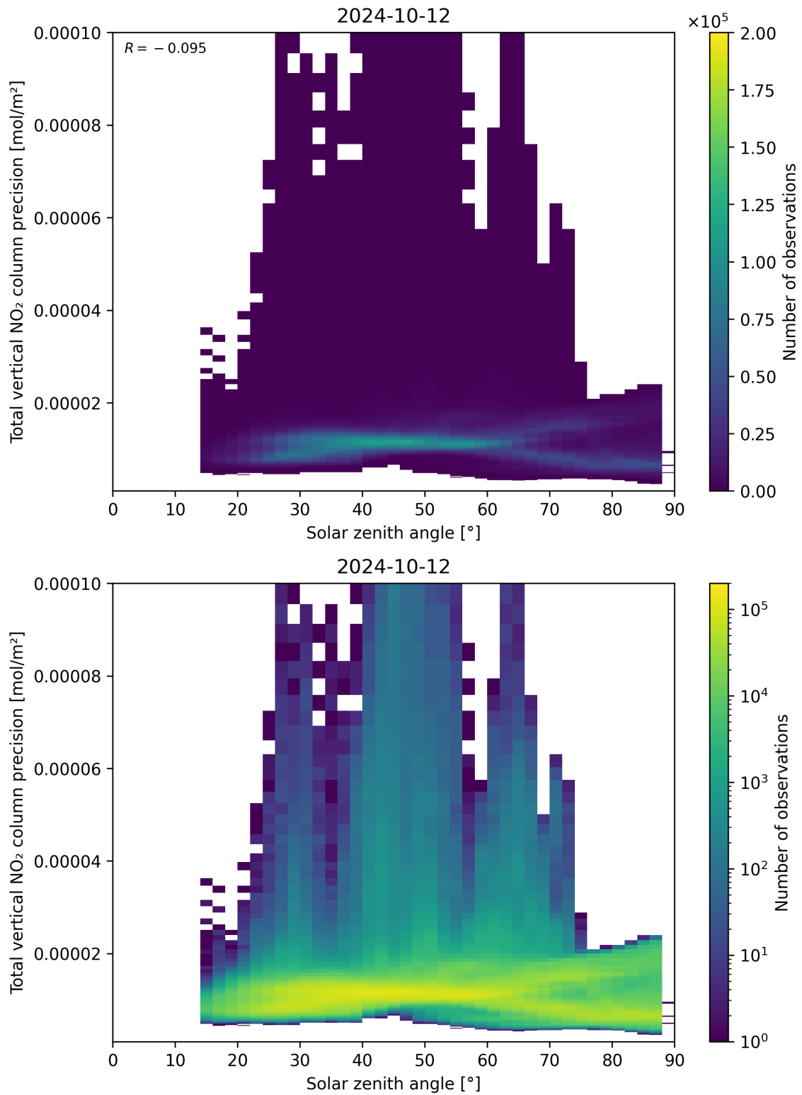
Figure 154: Scatter density plot of “Solar zenith angle” against “Total vertical NO 2 column precision” for 2024-10-11 to 2024-10-13.
