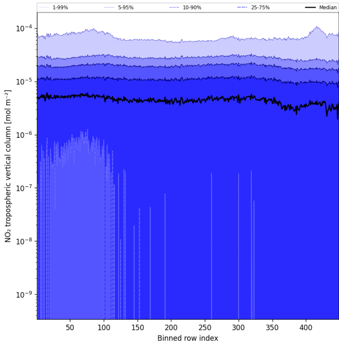
Figure 46: Along track statistics of “NO 2 tropospheric vertical column” for 2024-10-11 to 2024-10-13
