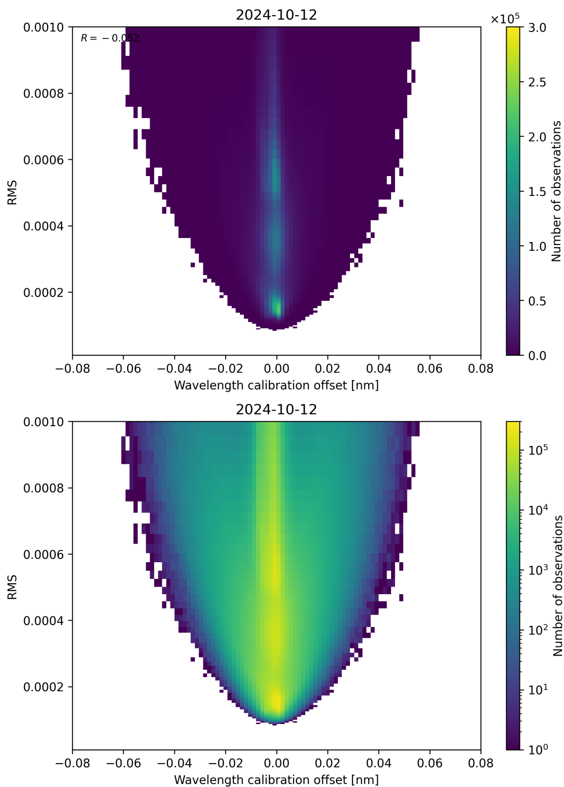
Figure 181: Scatter density plot of “Wavelength calibration offset” against “RMS” for 2024-10-11 to 2024-10-13.
