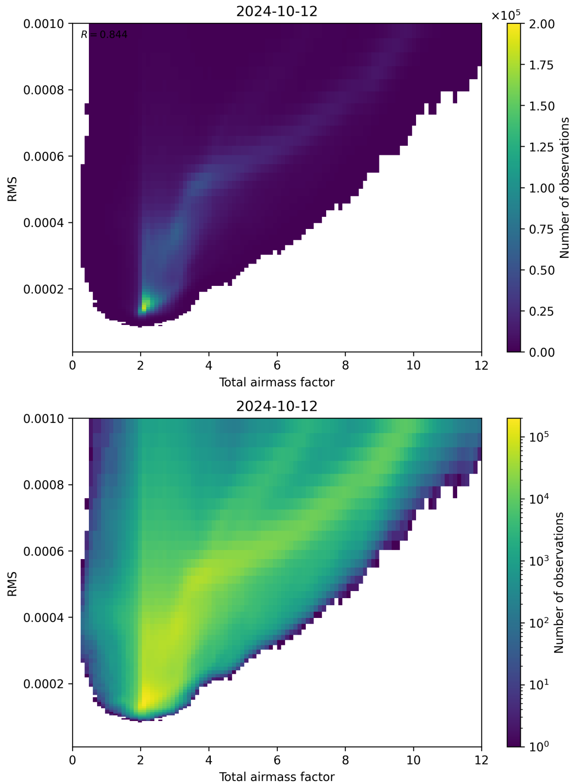
Figure 69: Scatter density plot of “Total airmass factor” against “RMS” for 2024-10-11 to 2024-10-13.
