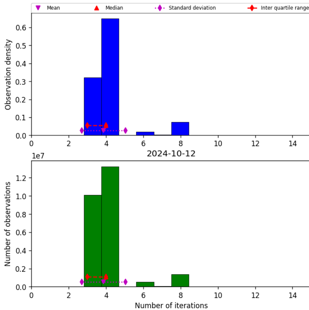
Figure 34: Histogram of “Number of iterations” for 2024-10-11 to 2024-10-13
