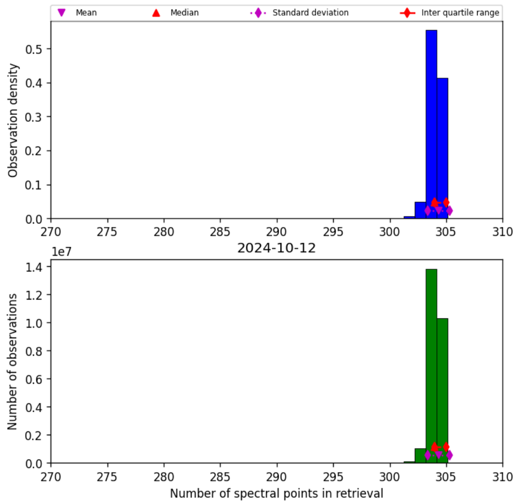
Figure 33: Histogram of “Number of spectral points in retrieval” for 2024-10-11 to 2024-10-13
