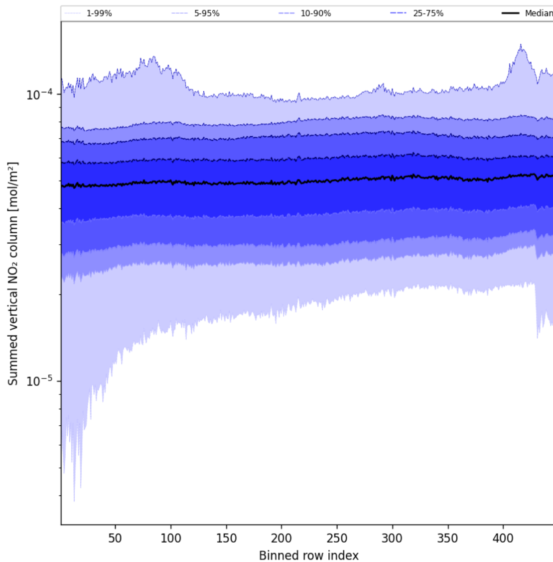
Figure 57: Along track statistics of “Summed vertical NO 2 column” for 2024-10-11 to 2024-10-13
