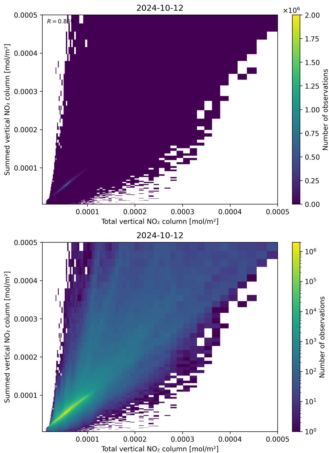
Figure 112: Scatter density plot of “Total vertical NO 2 column” against “Summed vertical NO 2 column” for 2024-10-11 to 2024-10-13.
