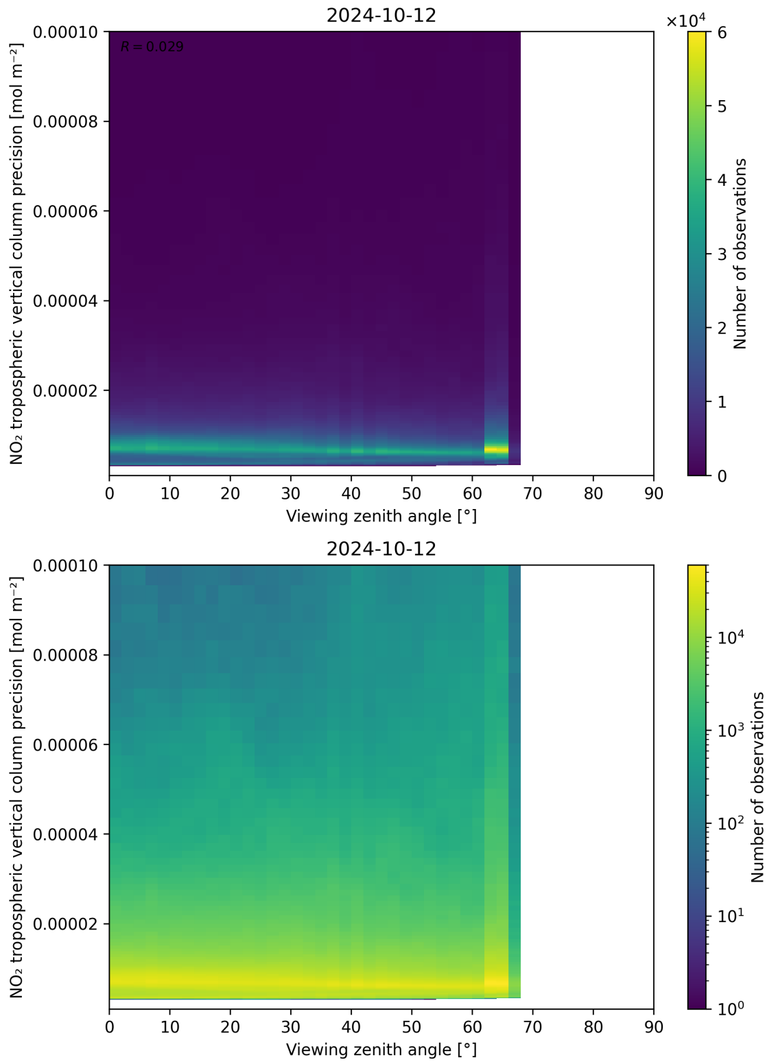
Figure 170: Scatter density plot of “Viewing zenith angle” against “NO 2 tropospheric vertical column precision” for 2024-10-11 to 2024-10-13.
