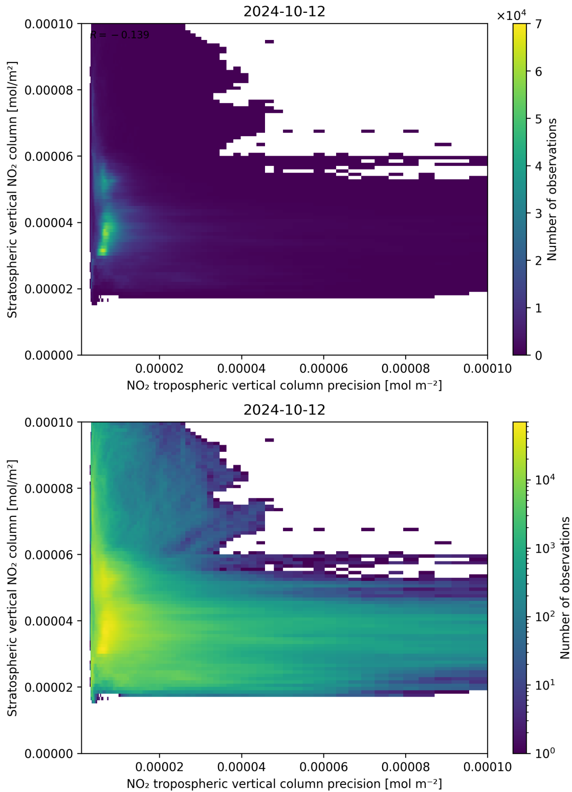
Figure 135: Scatter density plot of “NO 2 tropospheric vertical column precision” against “Stratospheric vertical NO 2 column” for 2024-10-11 to 2024-10-13.
