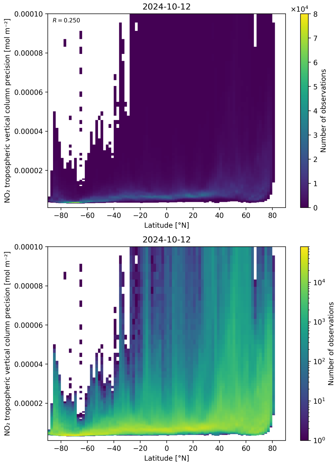
Figure 93: Scatter density plot of “Latitude” against “NO 2 tropospheric vertical column precision” for 2024-10-11 to 2024-10-13.
