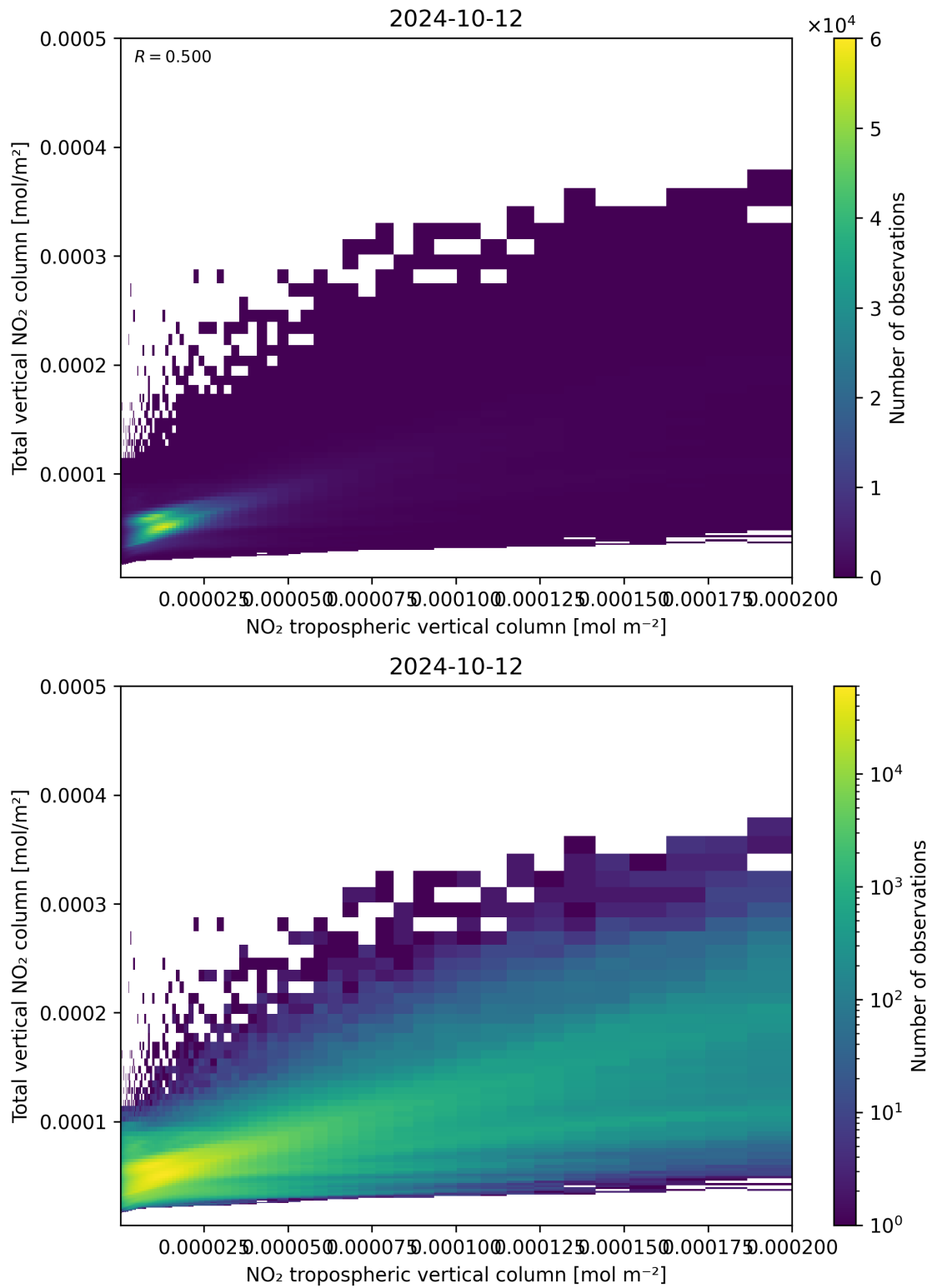
Figure 128: Scatter density plot of “NO 2 tropospheric vertical column” against “Total vertical NO 2 column” for 2024-10-11 to 2024-10-13.
