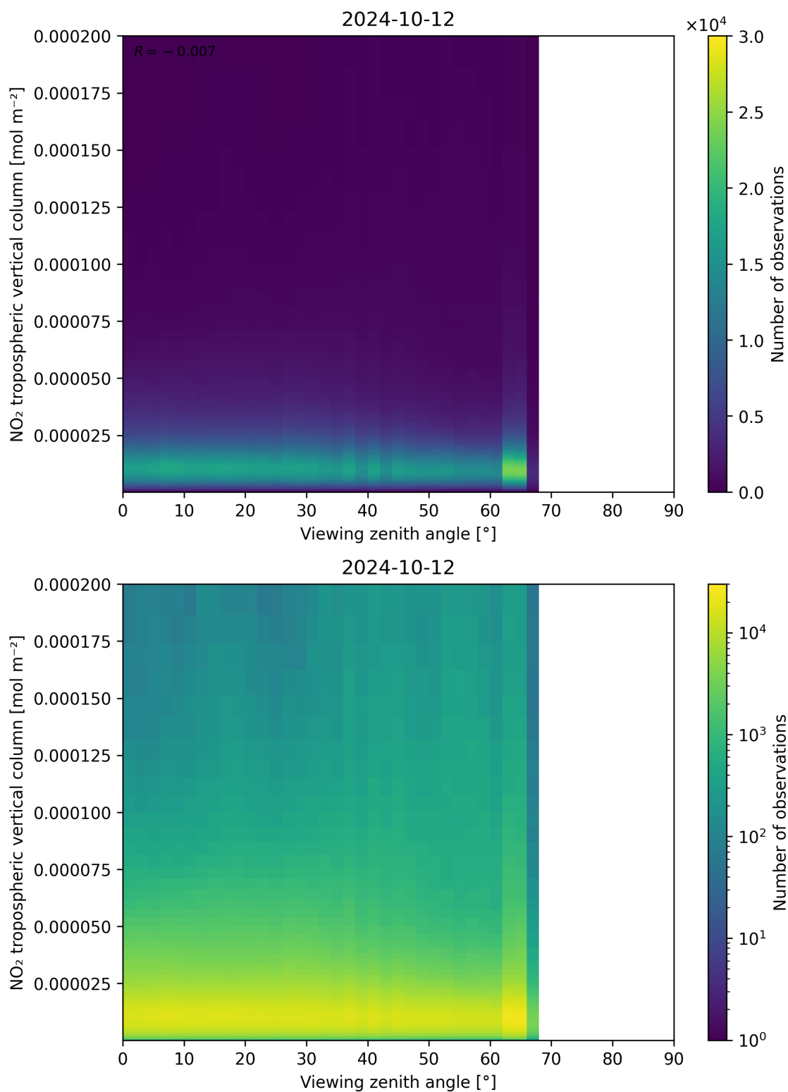
Figure 169: Scatter density plot of “Viewing zenith angle” against “NO 2 tropospheric vertical column” for 2024-10-11 to 2024-10-13.
