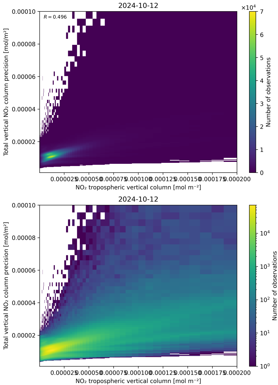
Figure 129: Scatter density plot of “NO 2 tropospheric vertical column” against “Total vertical NO 2 column precision” for 2024-10-11 to 2024-10-13.
