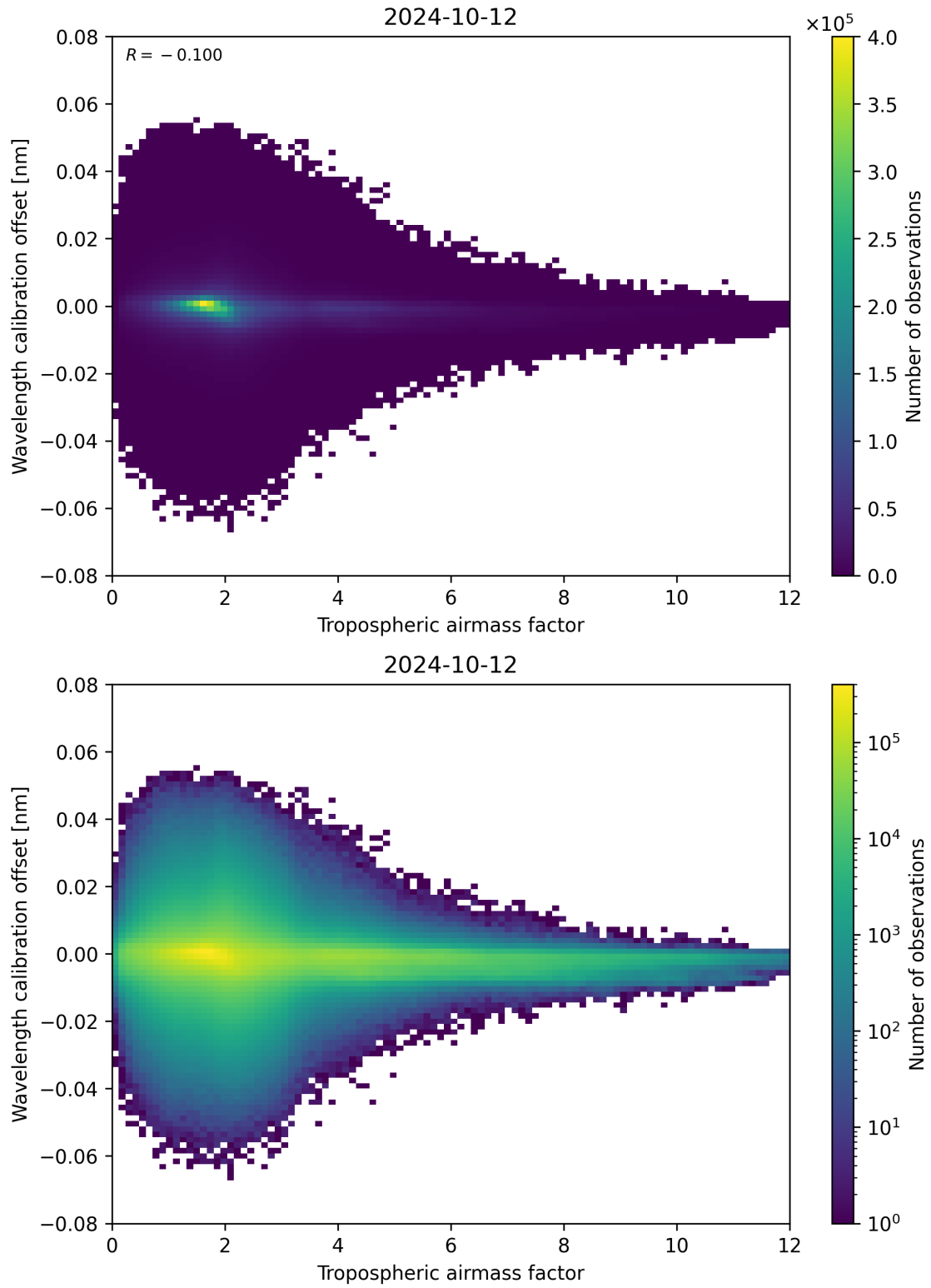
Figure 80: Scatter density plot of “Tropospheric airmass factor” against “Wavelength calibration offset” for 2024-10-11 to 2024-10-13.
