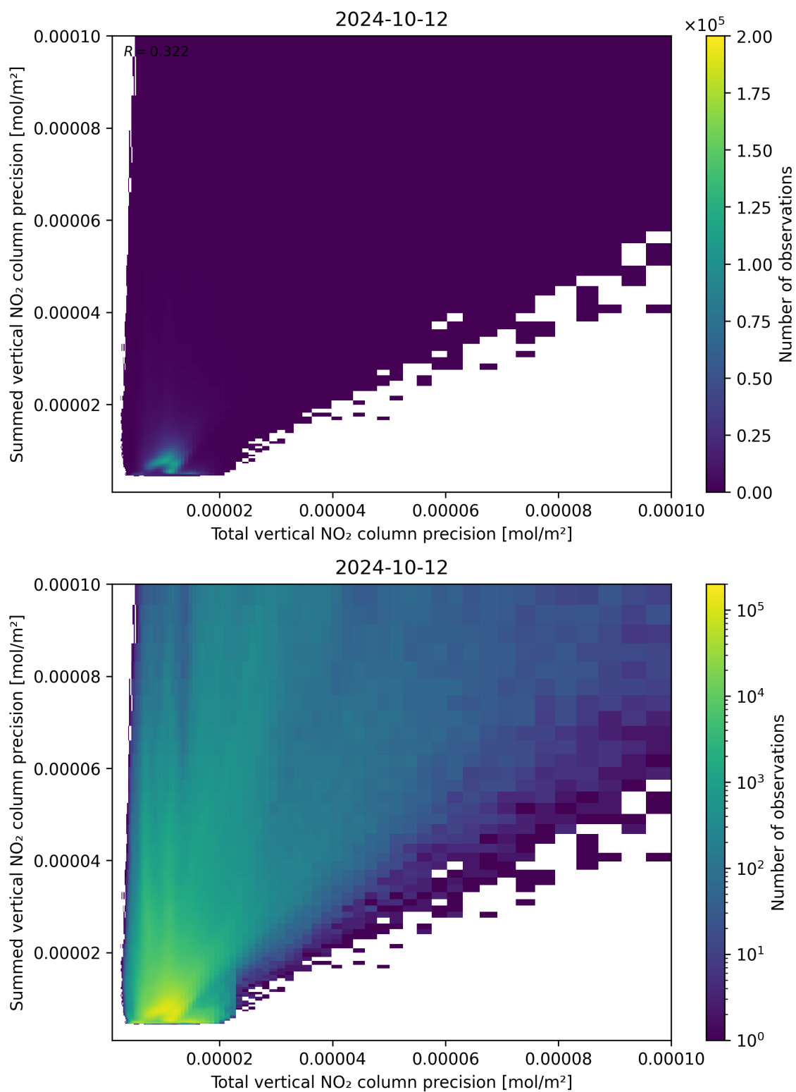
Figure 118: Scatter density plot of “Total vertical NO 2 column precision” against “Summed vertical NO 2 column precision” for 2024-10-11 to 2024-10-13.
