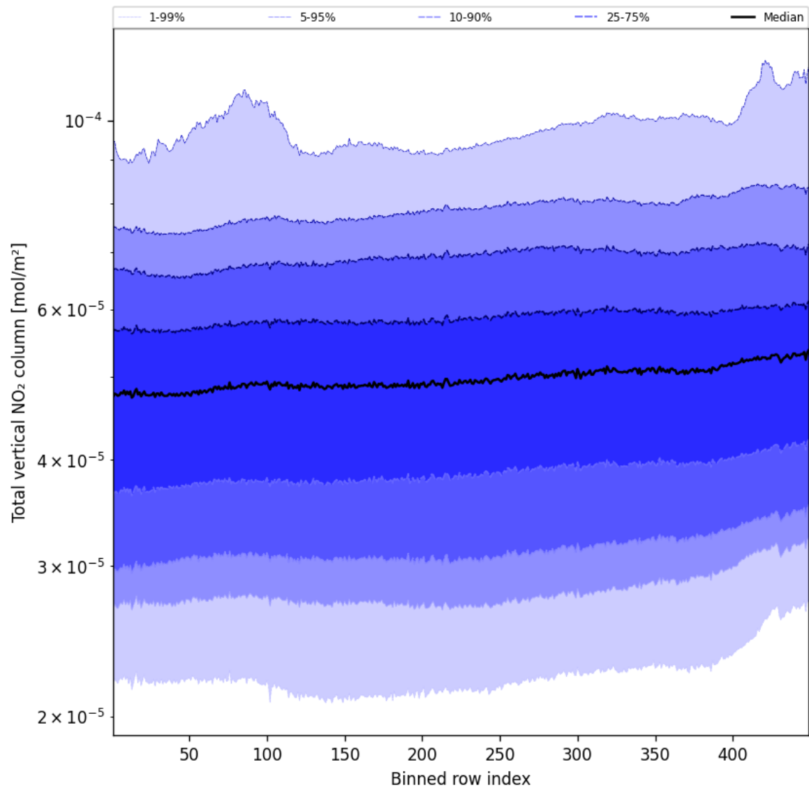
Figure 55: Along track statistics of “Total vertical NO 2 column” for 2024-10-11 to 2024-10-13
