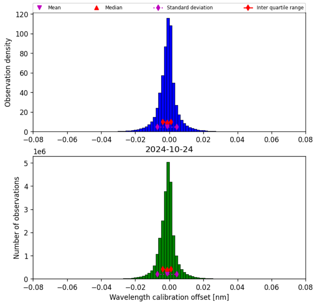
Figure 35: Histogram of “Wavelength calibration offset” for 2024-10-24 to 2024-10-25
