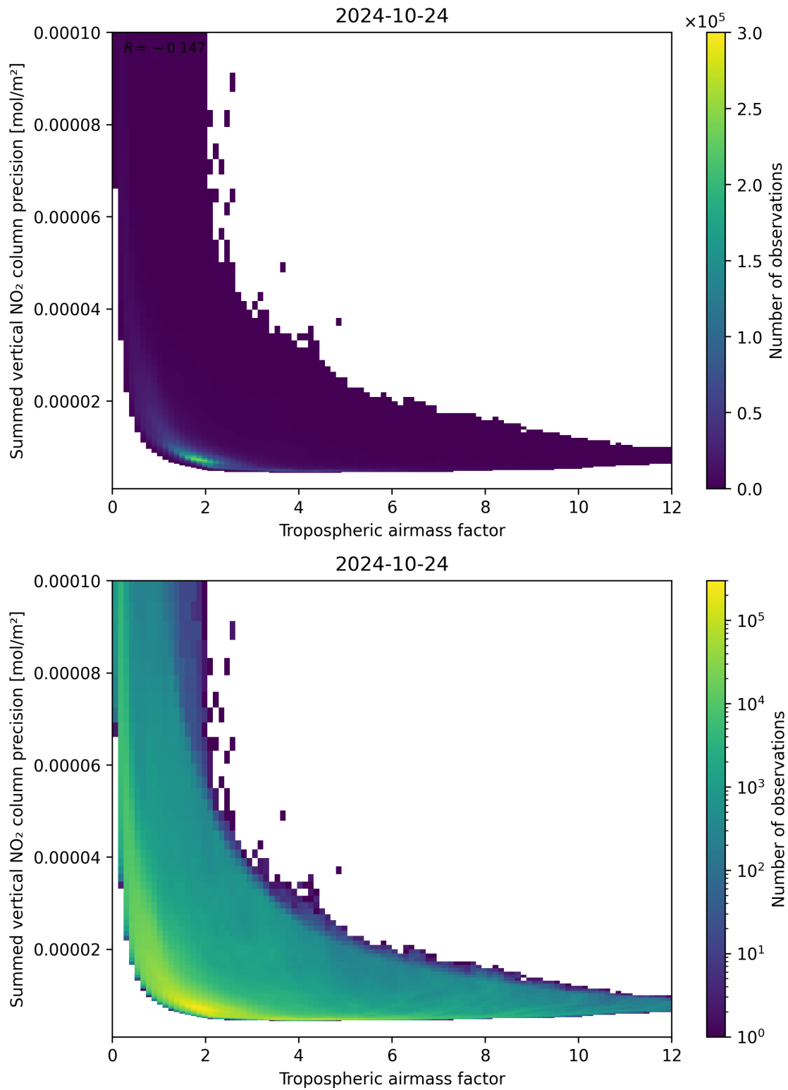
Figure 76: Scatter density plot of “Tropospheric airmass factor” against “Summed vertical NO 2 column precision” for 2024-10-24 to 2024-10-25.
