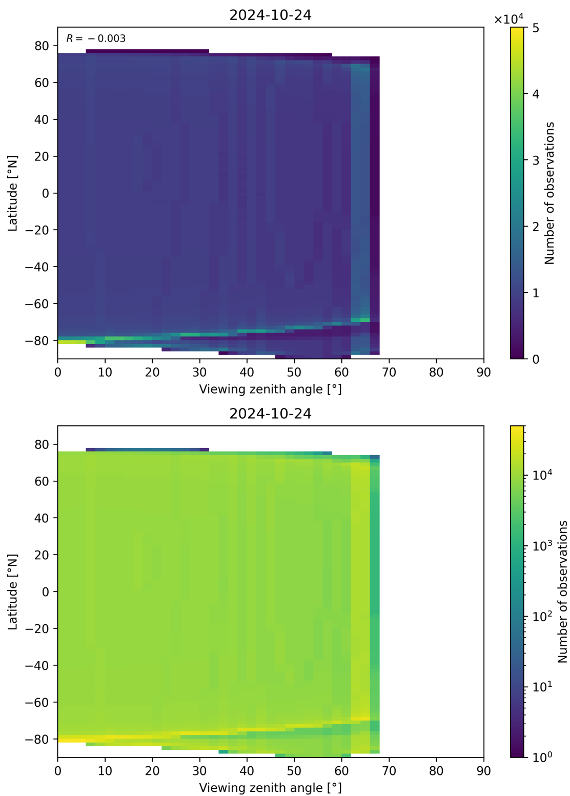
Figure 163: Scatter density plot of “Viewing zenith angle” against “Latitude” for 2024-10-24 to 2024-10-25.
