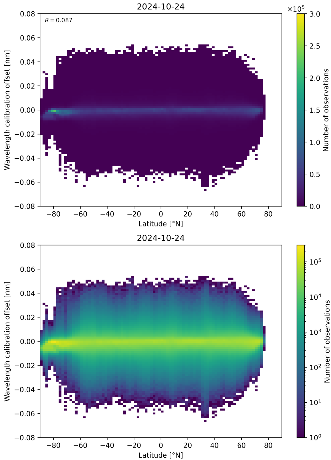
Figure 95: Scatter density plot of “Latitude” against “Wavelength calibration offset” for 2024-10-24 to 2024-10-25.
