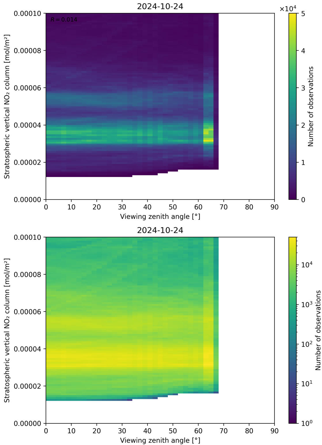
Figure 164: Scatter density plot of “Viewing zenith angle” against “Stratospheric vertical NO 2 column” for 2024-10-24 to 2024-10-25.
