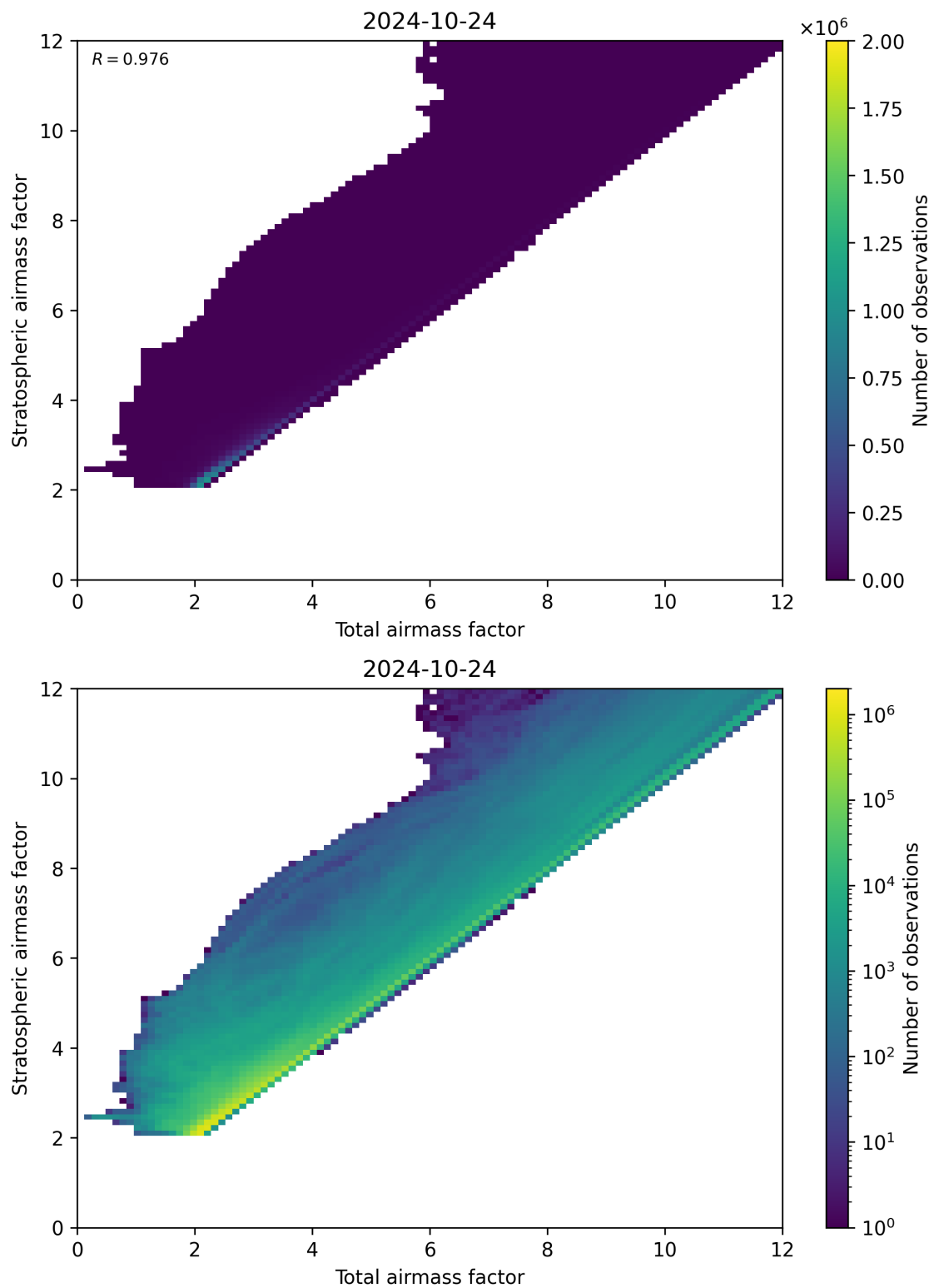
Figure 62: Scatter density plot of “Total airmass factor” against “Stratospheric airmass factor” for 2024-10-24 to 2024-10-25.
