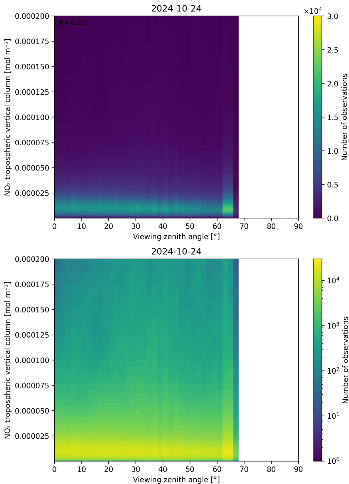
Figure 169: Scatter density plot of “Viewing zenith angle” against “NO 2 tropospheric vertical column” for 2024-10-24 to 2024-10-25.
