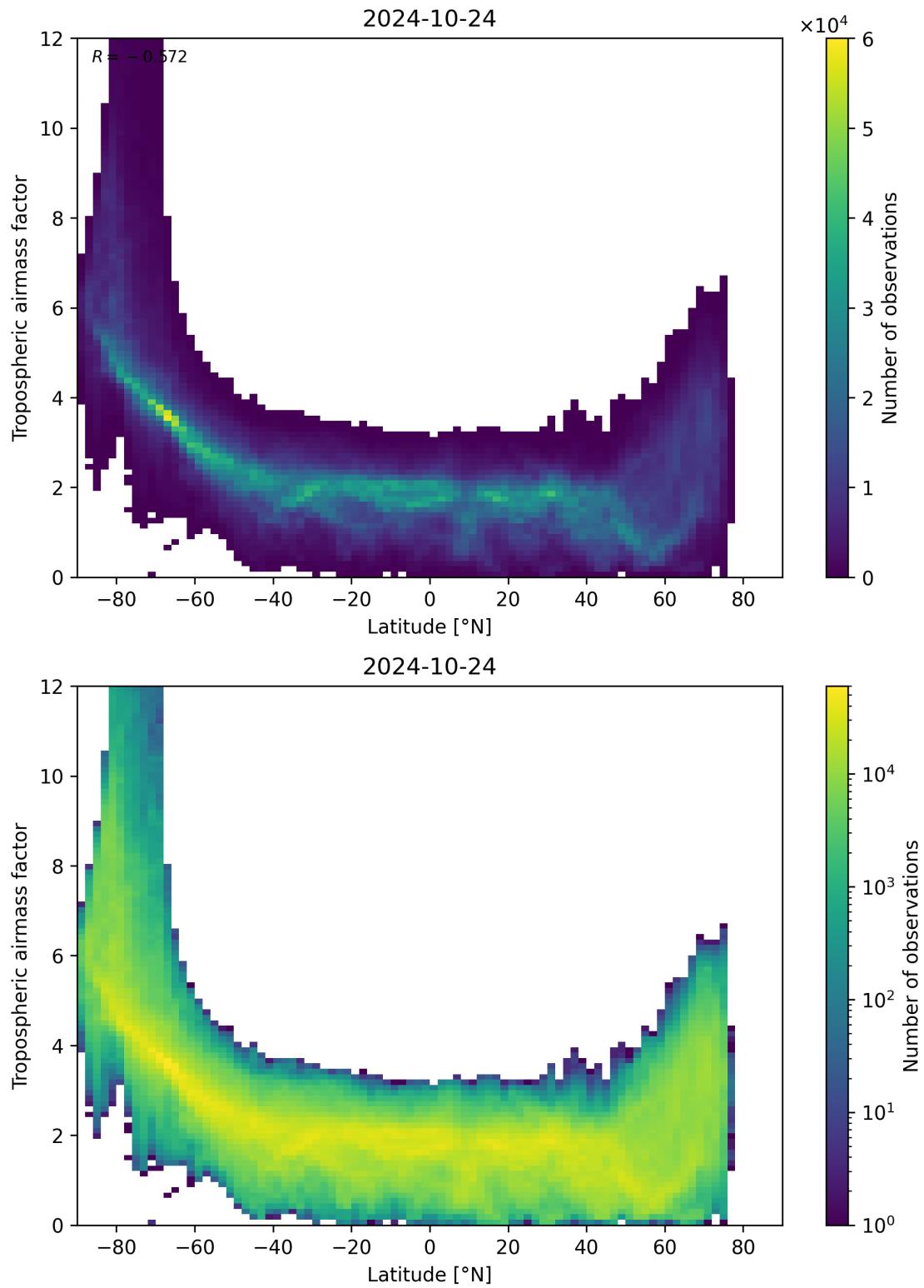
Figure 85: Scatter density plot of “Latitude” against “Tropospheric air mass factor” for 2024-10-24 to 2024-10-25.
