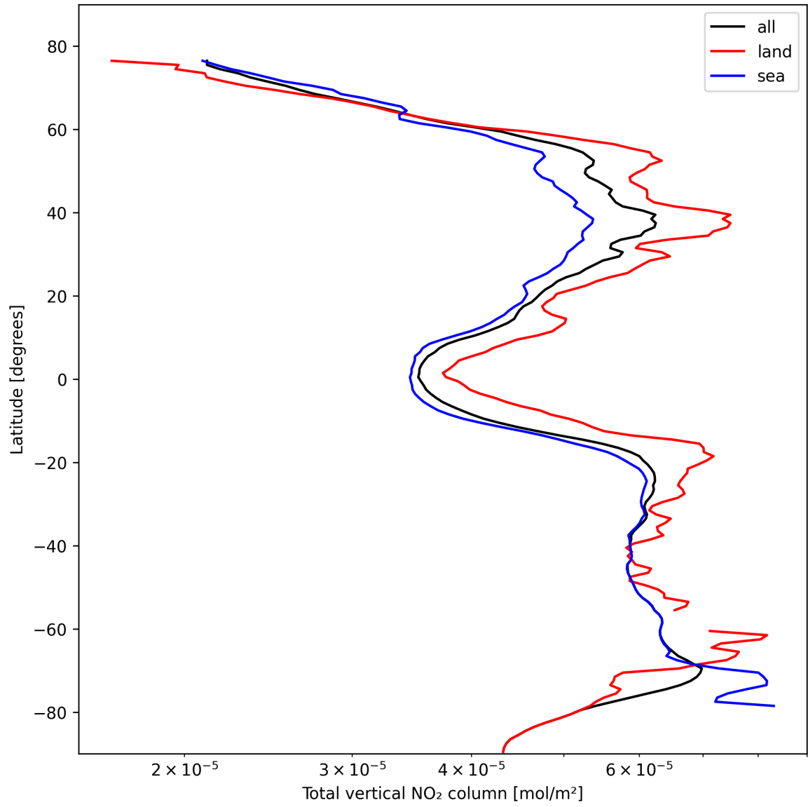
Figure 21: Zonal average of “Total vertical NO 2 column” for 2024-10-24 to 2024-10-25.
