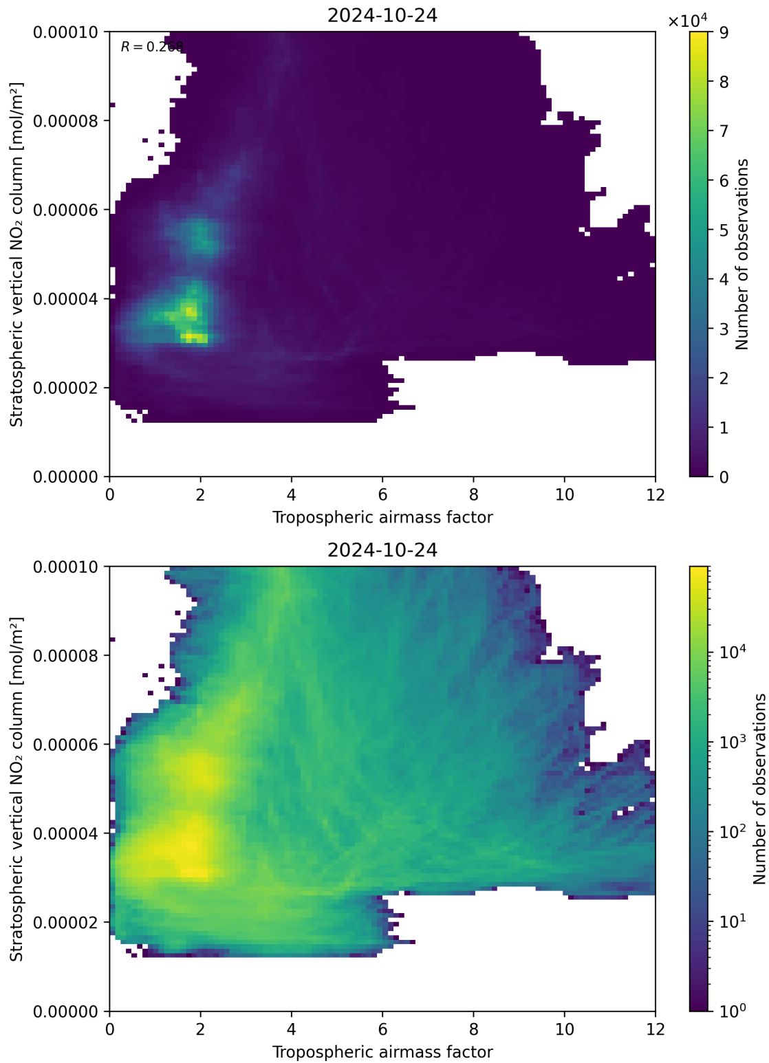
Figure 74: Scatter density plot of “Tropospheric air mass factor” against “Stratospheric vertical NO 2 column” for 2024-10-24 to 2024-10-25.
