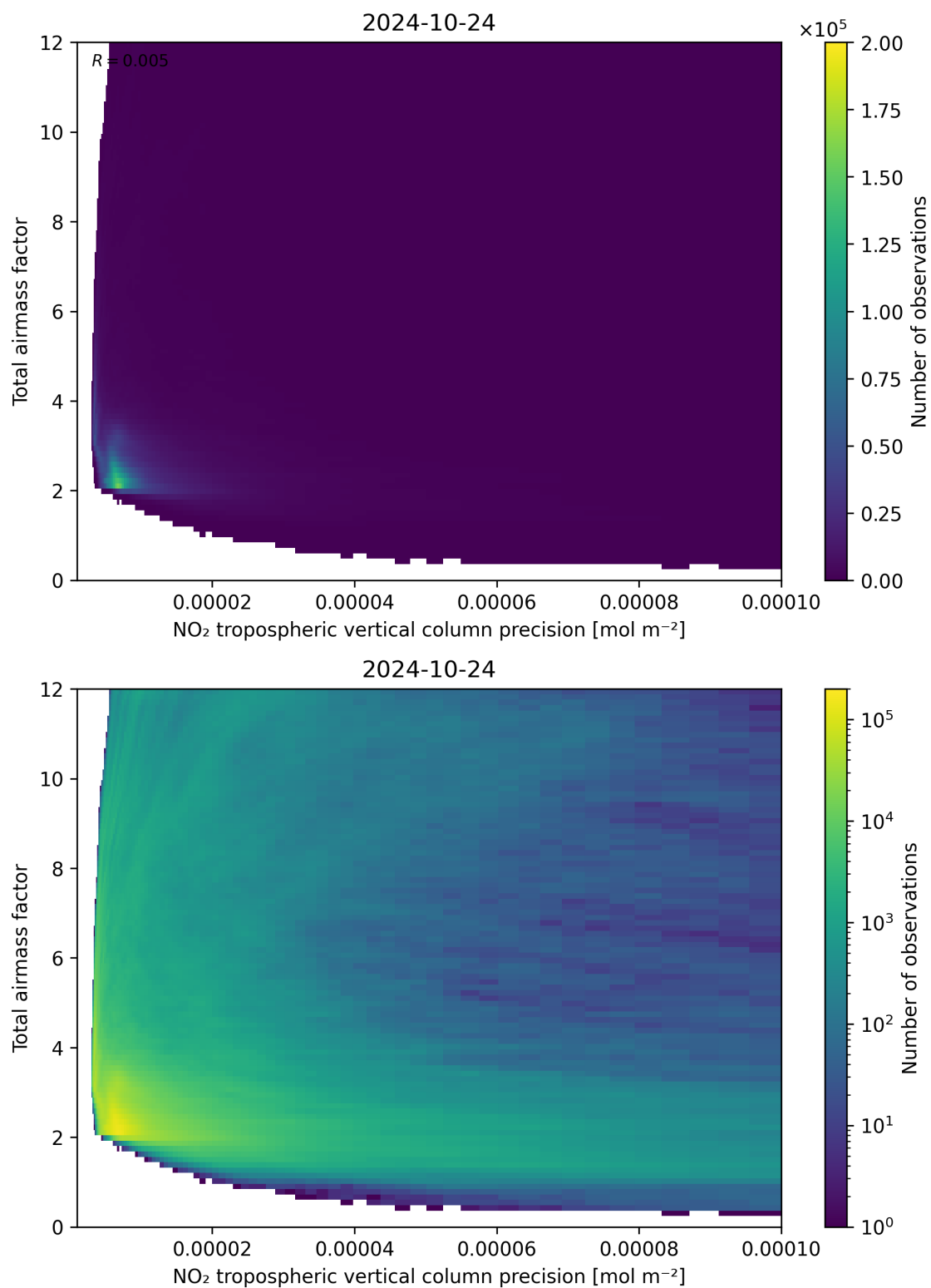
Figure 132: Scatter density plot of “NO 2 tropospheric vertical column precision” against “Total air mass factor” for 2024-10-24 to 2024-10-25.
