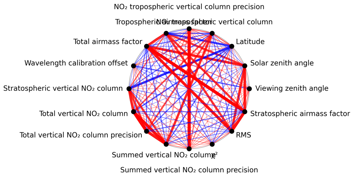
Figure 1: Map of correlation graph for 2024-10-24 to 2024-10-25.
