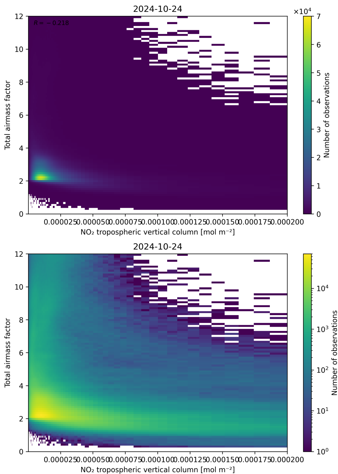
Figure 122: Scatter density plot of “NO 2 tropospheric vertical column” against “Total airmass factor” for 2024-10-24 to 2024-10-25.
