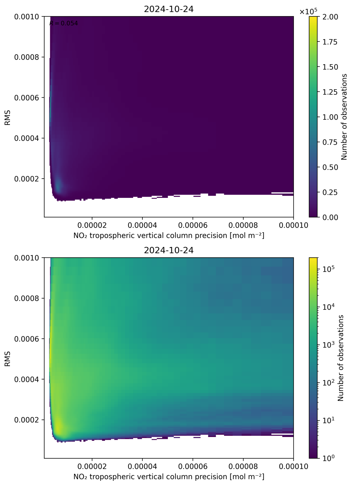
Figure 140: Scatter density plot of “NO 2 tropospheric vertical column precision” against “RMS” for 2024-10-24 to 2024-10-25.
