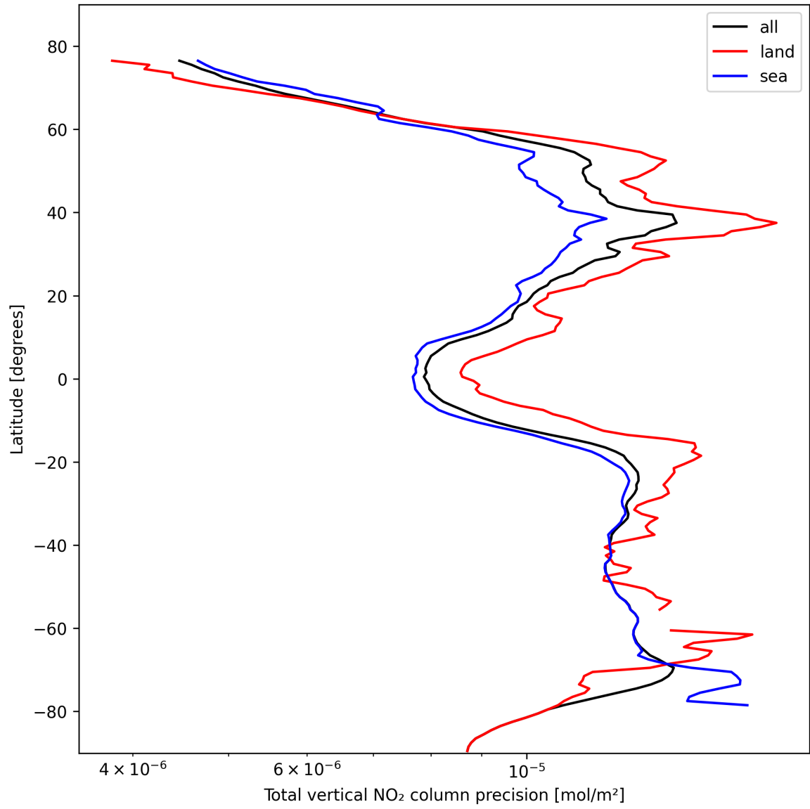
Figure 22: Zonal average of “Total vertical NO 2 column precision” for 2024-10-24 to 2024-10-25.
