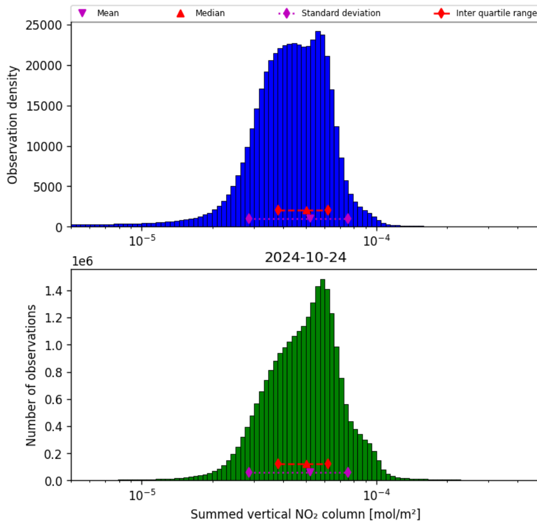
Figure 40: Histogram of “Summed vertical NO 2 column” for 2024-10-24 to 2024-10-25
