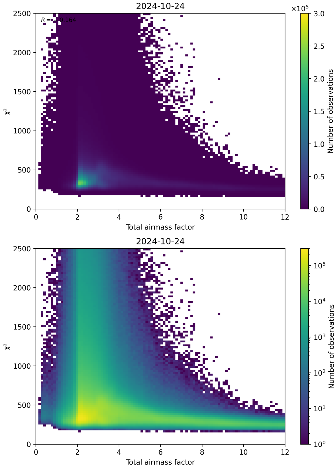
Figure 63: Scatter density plot of “Total airmass factor” against “ \chi^2 ” for 2024-10-24 to 2024-10-25.
