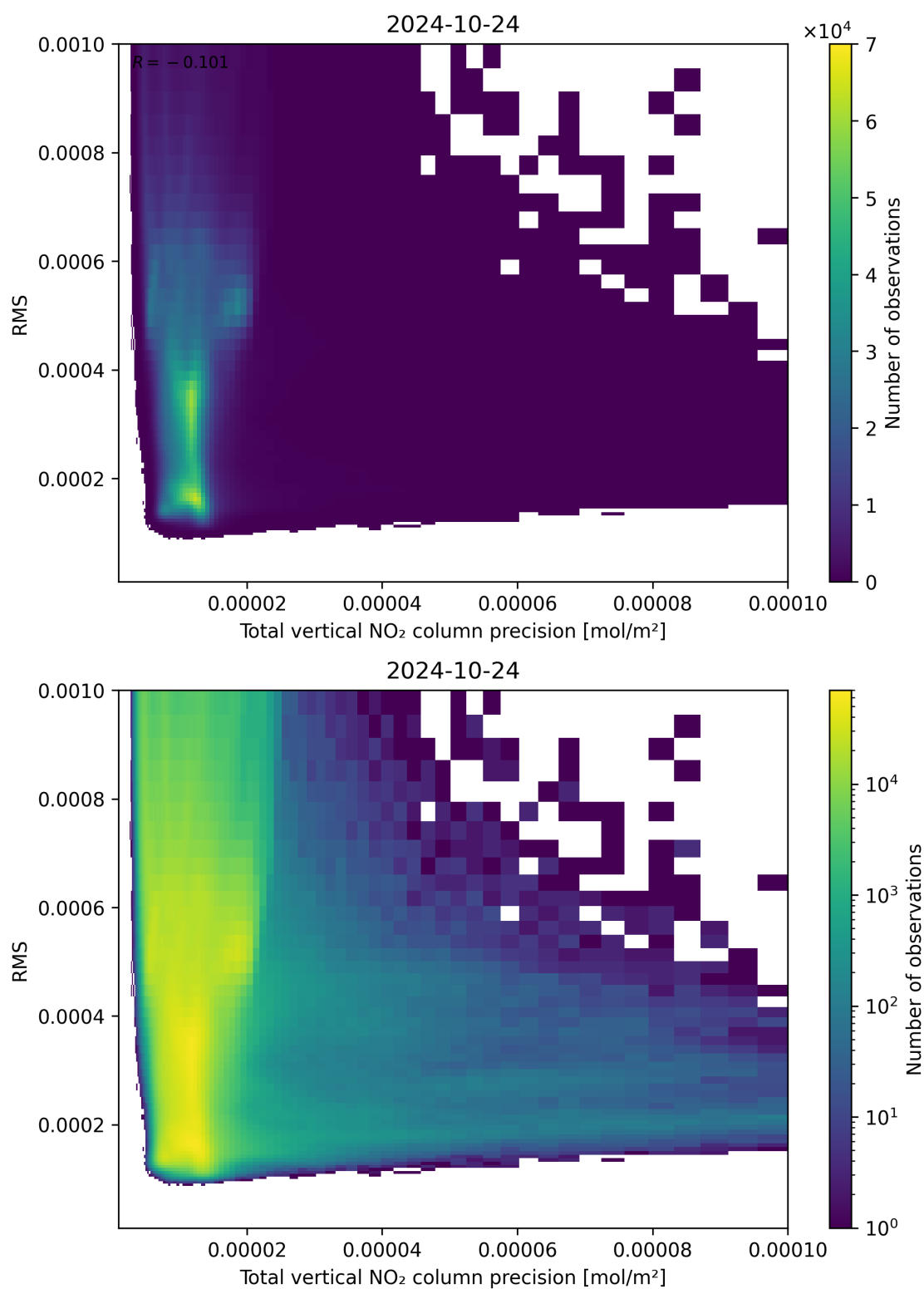
Figure 119: Scatter density plot of “Total vertical NO 2 column precision” against “RMS” for 2024-10-24 to 2024-10-25.
