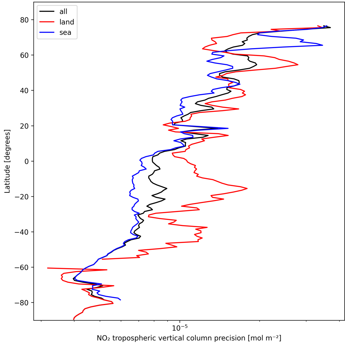
Figure 13: Zonal average of “NO 2 tropospheric vertical column precision” for 2024-10-24 to 2024-10-25.
