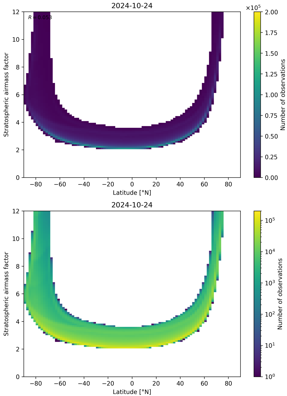
Figure 83: Scatter density plot of “Latitude” against “Stratospheric airmass factor” for 2024-10-24 to 2024-10-25.
