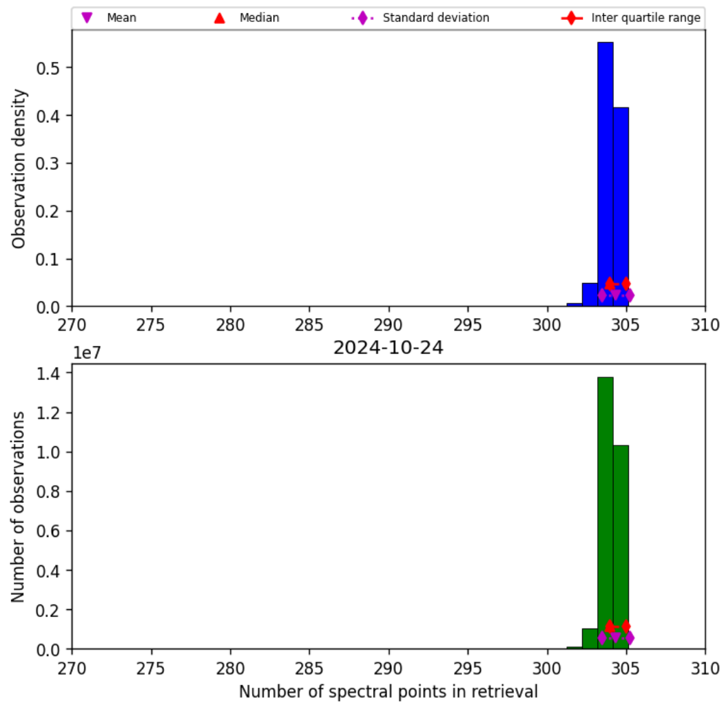
Figure 33: Histogram of “Number of spectral points in retrieval” for 2024-10-24 to 2024-10-25
