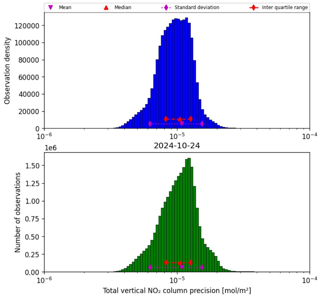
Figure 39: Histogram of “Total vertical NO 2 column precision” for 2024-10-24 to 2024-10-25
