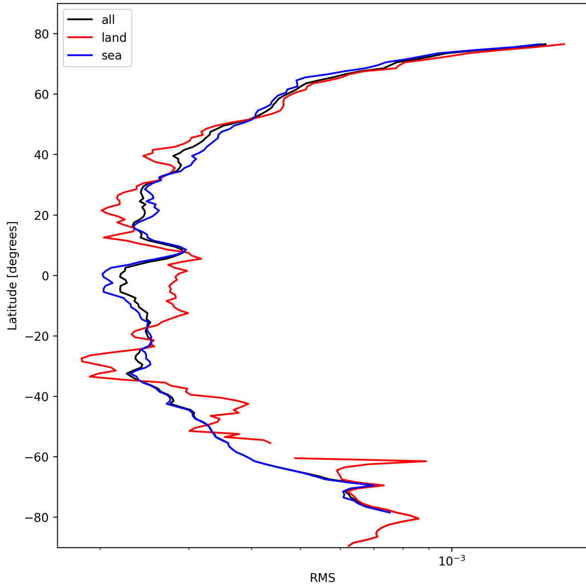
Figure 26: Zonal average of “RMS” for 2024-10-24 to 2024-10-25.
