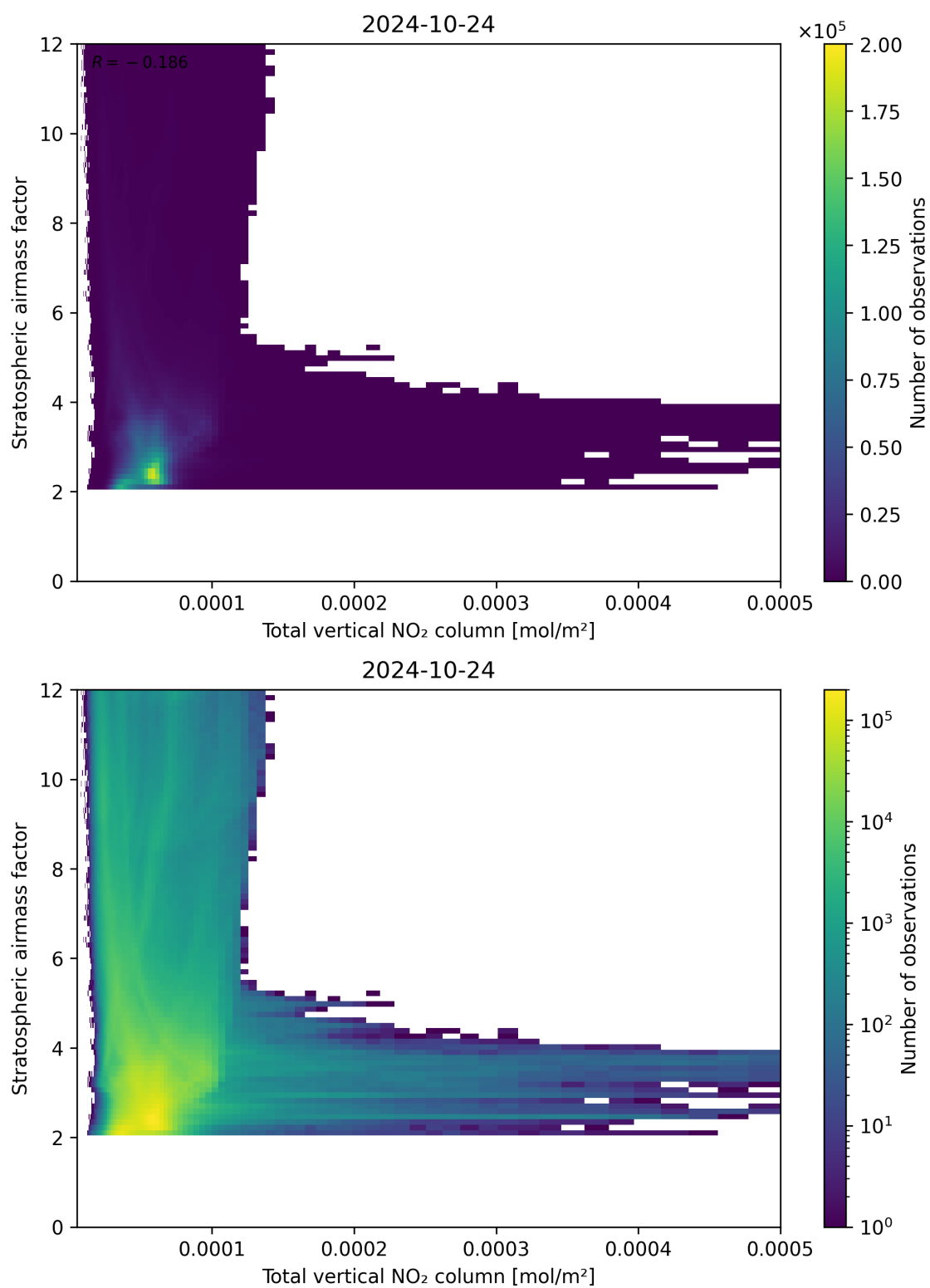
Figure 110: Scatter density plot of “Total vertical NO 2 column” against “Stratospheric airmass factor” for 2024-10-24 to 2024-10-25.
