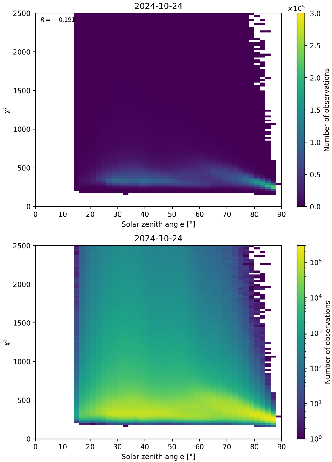
Figure 148: Scatter density plot of “Solar zenith angle” against “ \chi^2 ” for 2024-10-24 to 2024-10-25.
