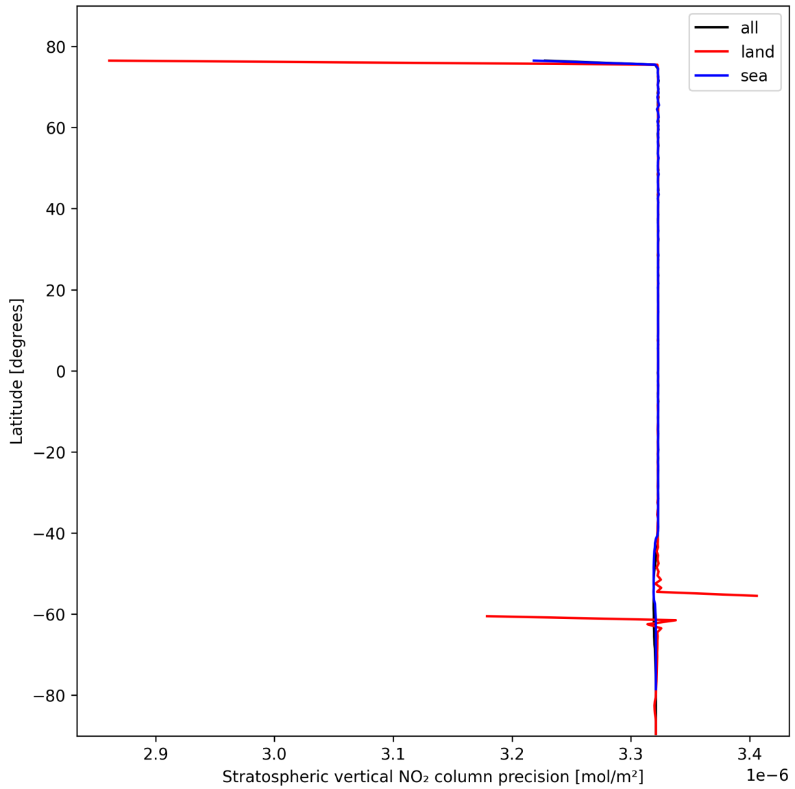
Figure 20: Zonal average of “Stratospheric vertical NO 2 column precision” for 2024-10-24 to 2024-10-25.
