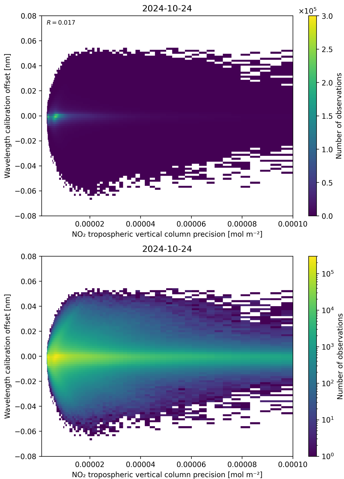
Figure 141: Scatter density plot of “NO 2 tropospheric vertical column precision” against “Wavelength calibration offset” for 2024-10-24 to 2024-10-25.
