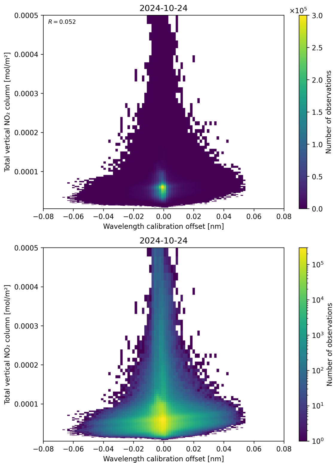
Figure 179: Scatter density plot of “Wavelength calibration offset” against “Total vertical NO 2 column” for 2024-10-24 to 2024-10-25.
