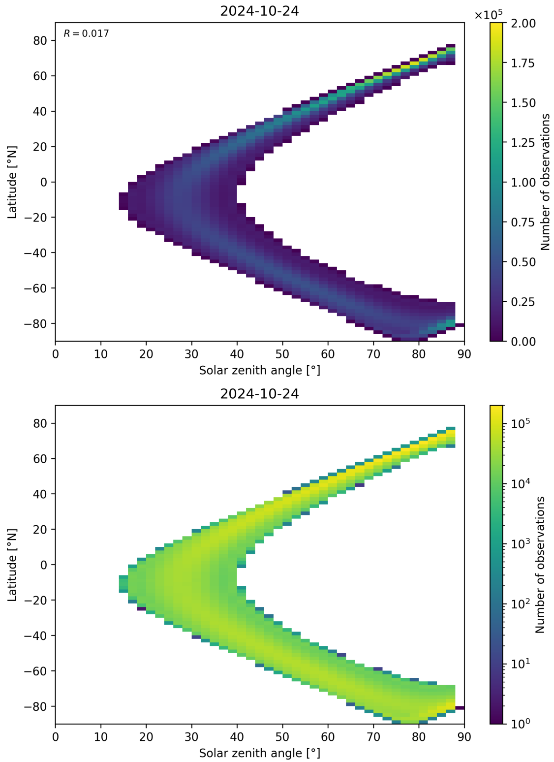
Figure 149: Scatter density plot of “Solar zenith angle” against “Latitude” for 2024-10-24 to 2024-10-25.
