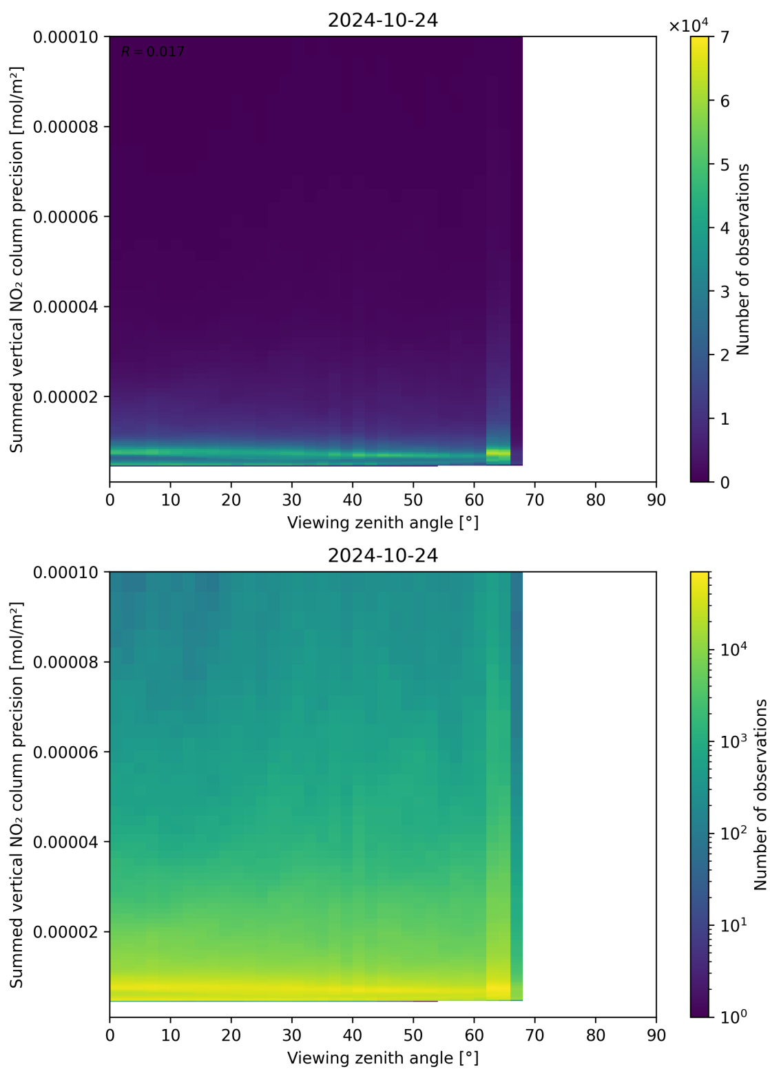
Figure 166: Scatter density plot of “Viewing zenith angle” against “Summed vertical NO 2 column precision” for 2024-10-24 to 2024-10-25.
