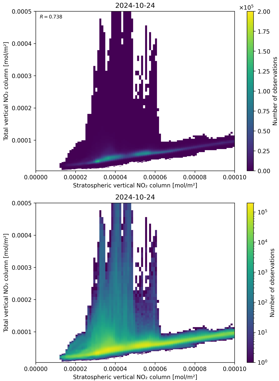
Figure 100: Scatter density plot of “Stratospheric vertical NO 2 column” against “Total vertical NO 2 column” for 2024-10-24 to 2024-10-25.
