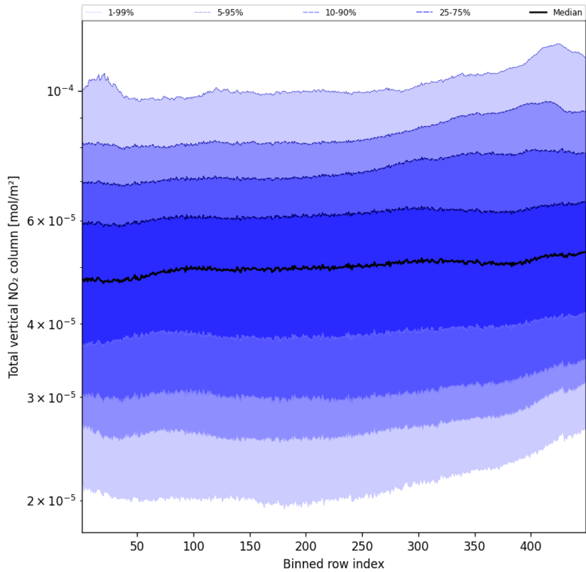
Figure 55: Along track statistics of “Total vertical NO 2 column” for 2024-10-24 to 2024-10-25
