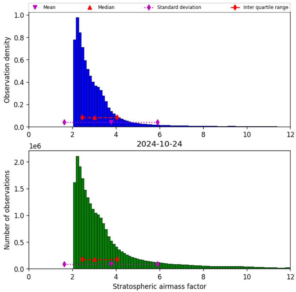
Figure 44: Histogram of “Stratospheric airmass factor” for 2024-10-24 to 2024-10-25
