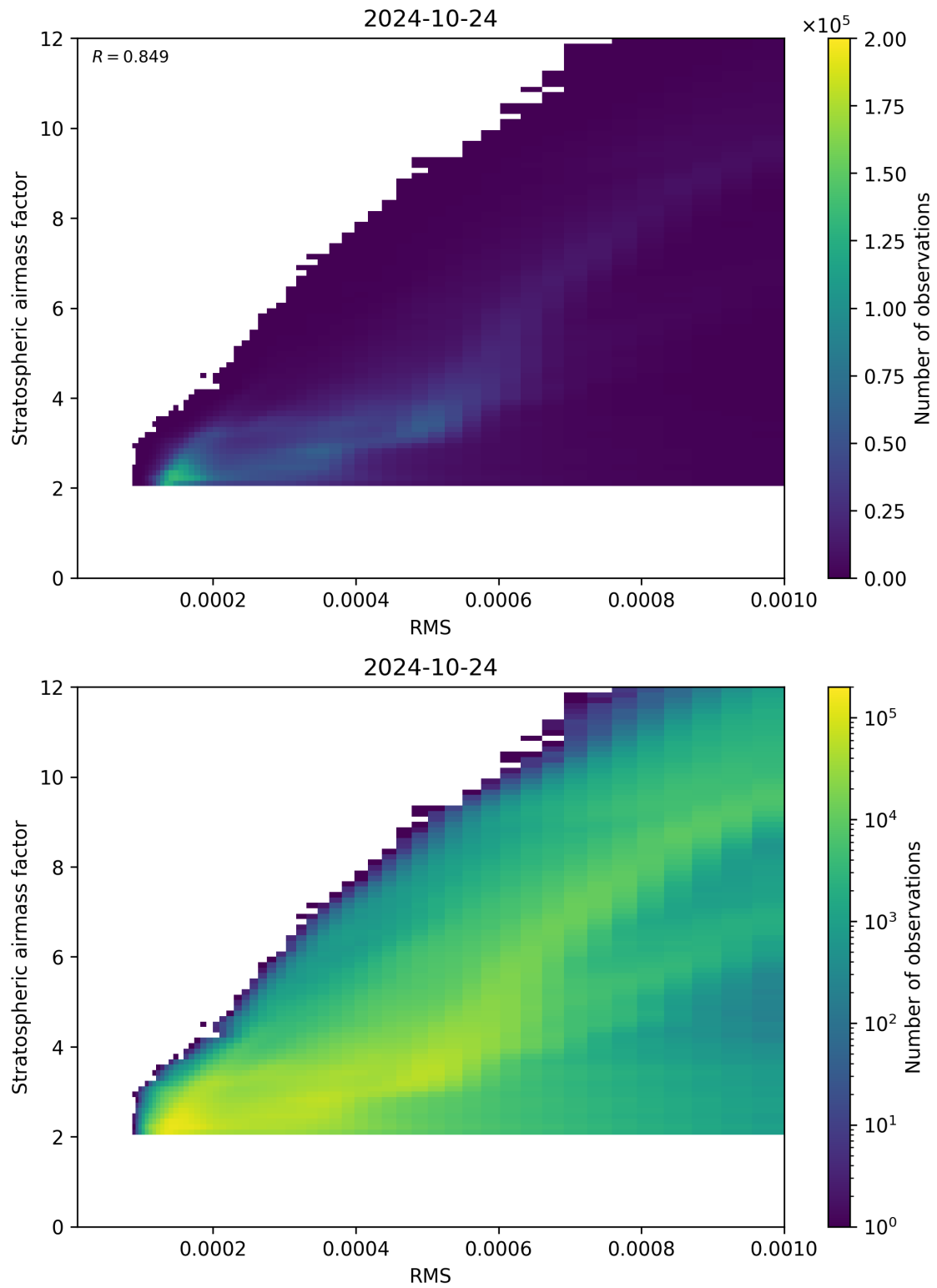
Figure 144: Scatter density plot of “RMS” against “Stratospheric airmass factor” for 2024-10-24 to 2024-10-25.
