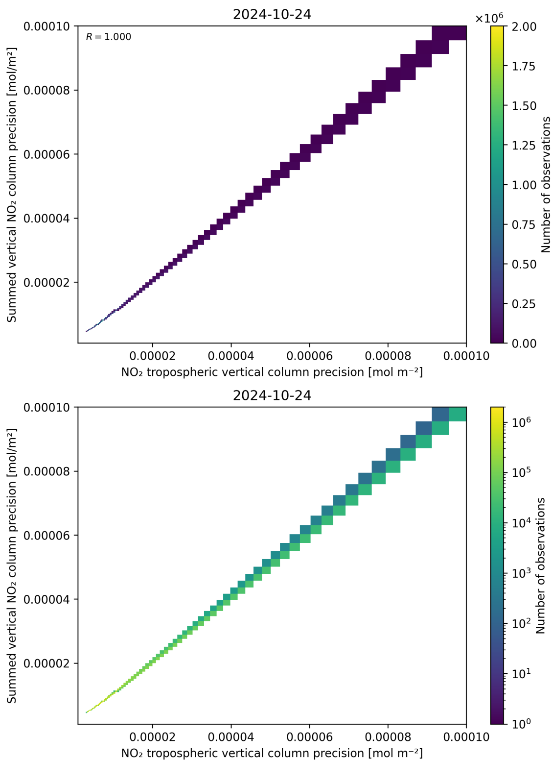
Figure 137: Scatter density plot of “NO 2 tropospheric vertical column precision” against “Summed vertical NO 2 column precision” for 2024-10-24 to 2024-10-25.
