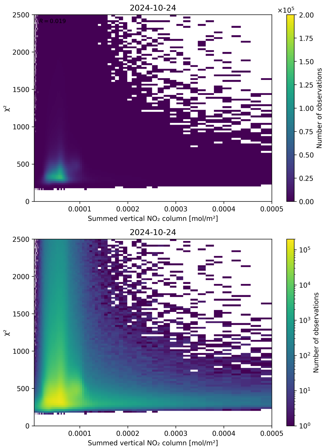
Figure 104: Scatter density plot of “Summed vertical NO 2 column” against “ \chi^2 ” for 2024-10-24 to 2024-10-25.
