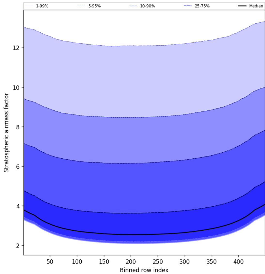
Figure 61: Along track statistics of “Stratospheric airmass factor” for 2024-10-24 to 2024-10-25
