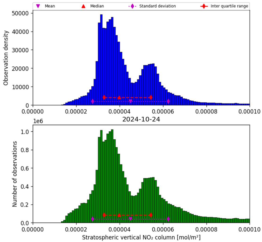
Figure 36: Histogram of “Stratospheric vertical NO 2 column” for 2024-10-24 to 2024-10-25
