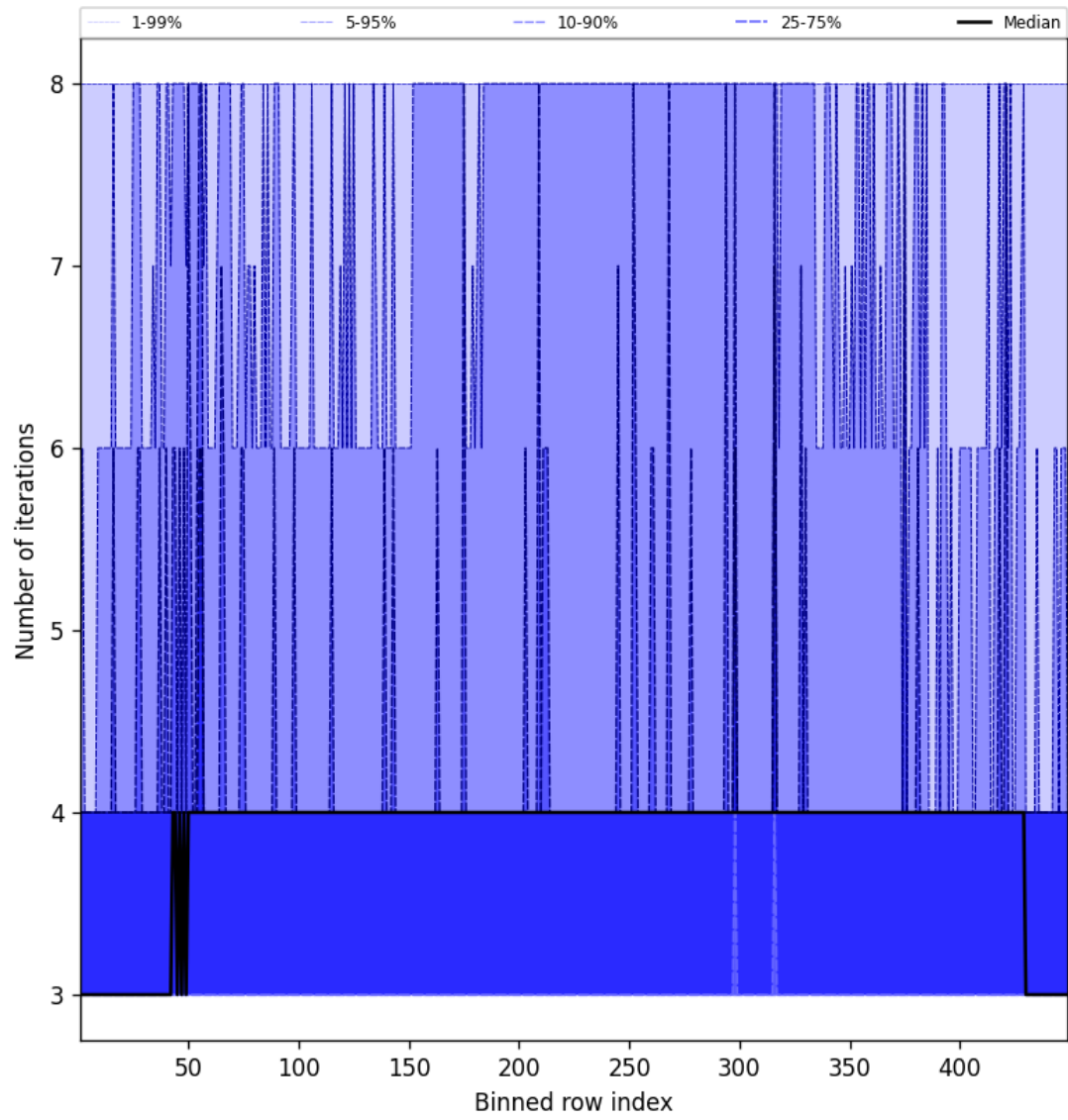
Figure 51: Along track statistics of “Number of iterations” for 2024-10-24 to 2024-10-25
