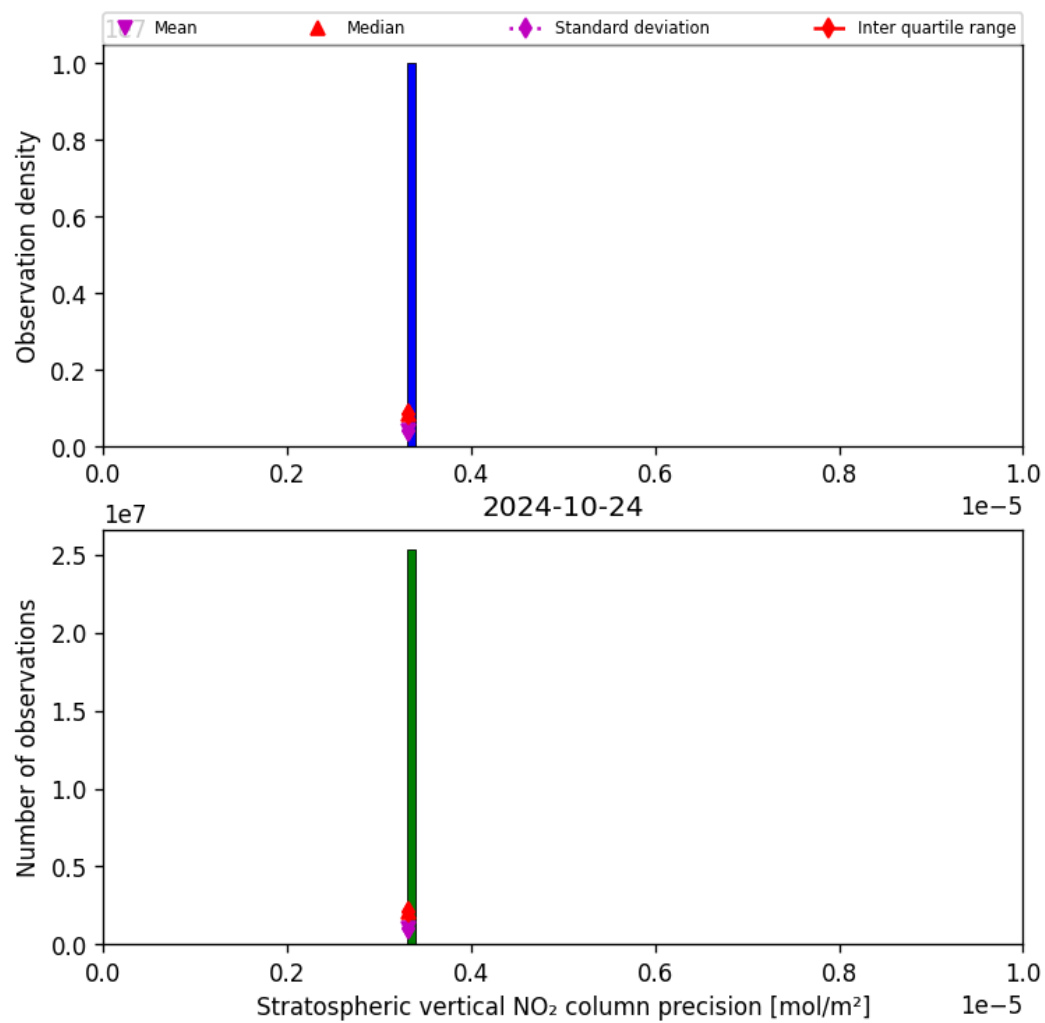
Figure 37: Histogram of “Stratospheric vertical NO 2 column precision” for 2024-10-24 to 2024-10-25
