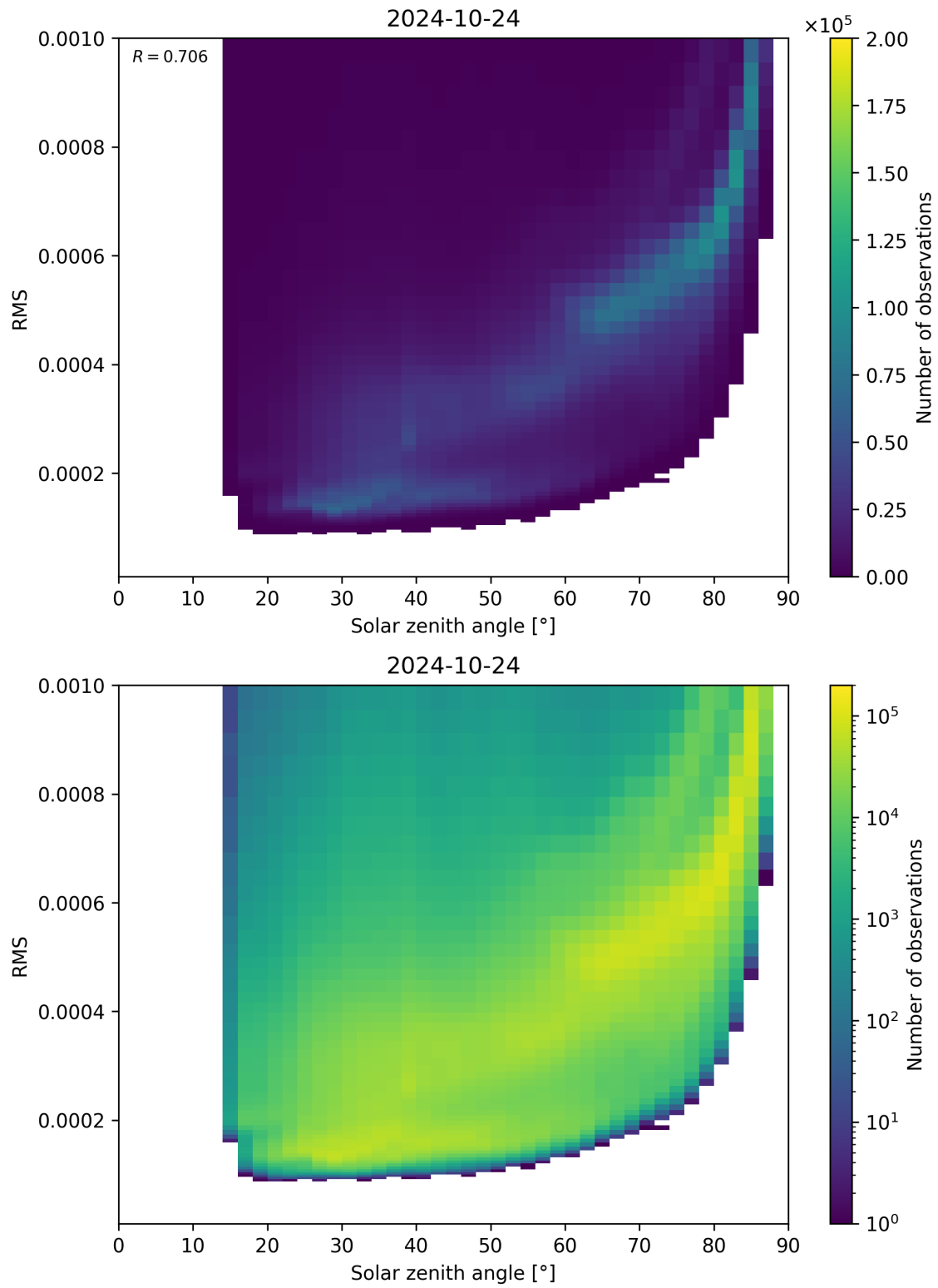
Figure 157: Scatter density plot of “Solar zenith angle” against “RMS” for 2024-10-24 to 2024-10-25.
