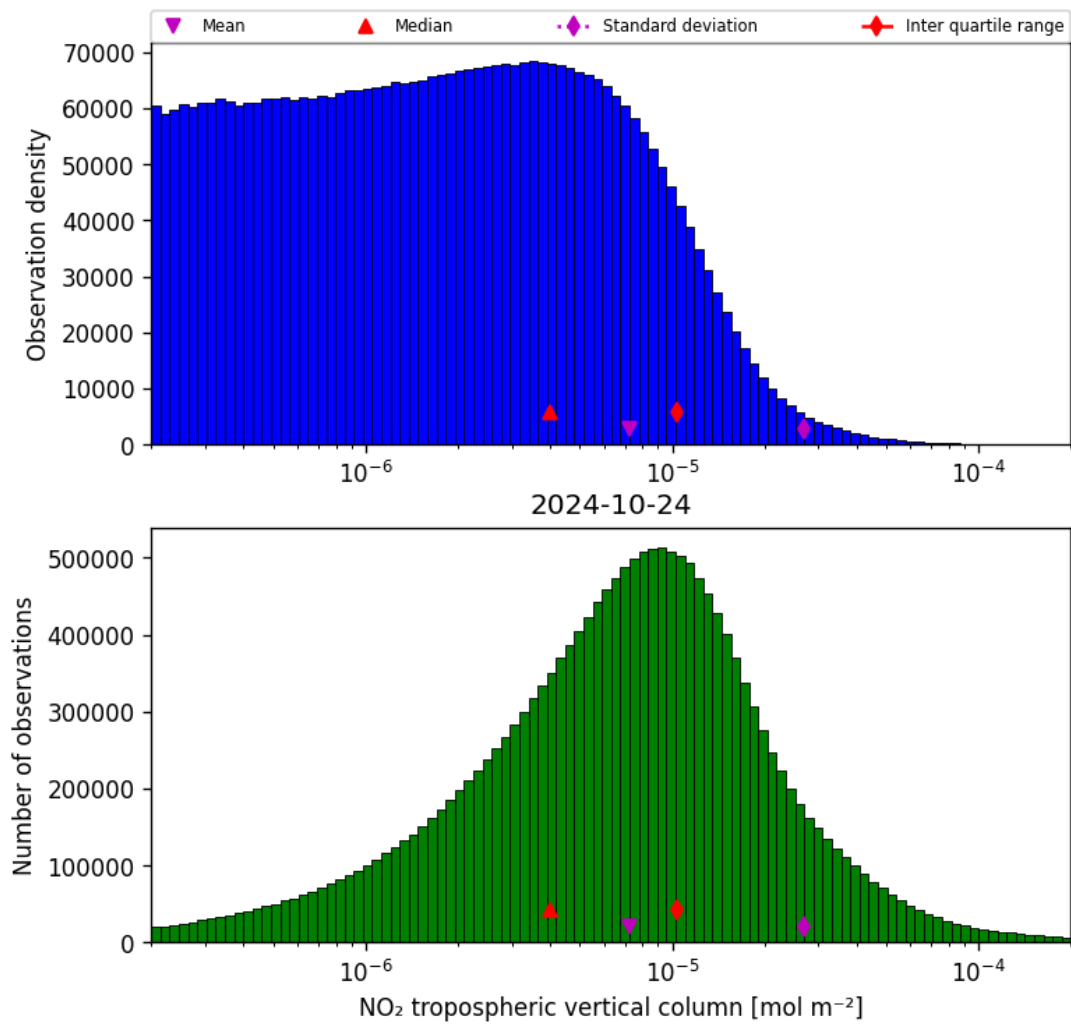
Figure 29: Histogram of “NO 2 tropospheric vertical column” for 2024-10-24 to 2024-10-25
