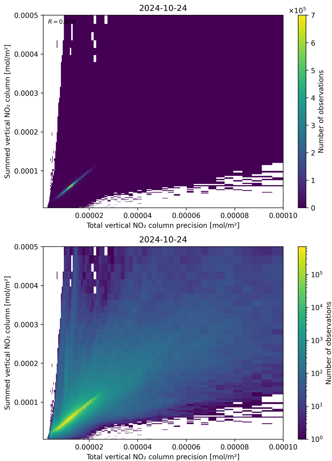
Figure 117: Scatter density plot of “Total vertical NO 2 column precision” against “Summed vertical NO 2 column” for 2024-10-24 to 2024-10-25.
