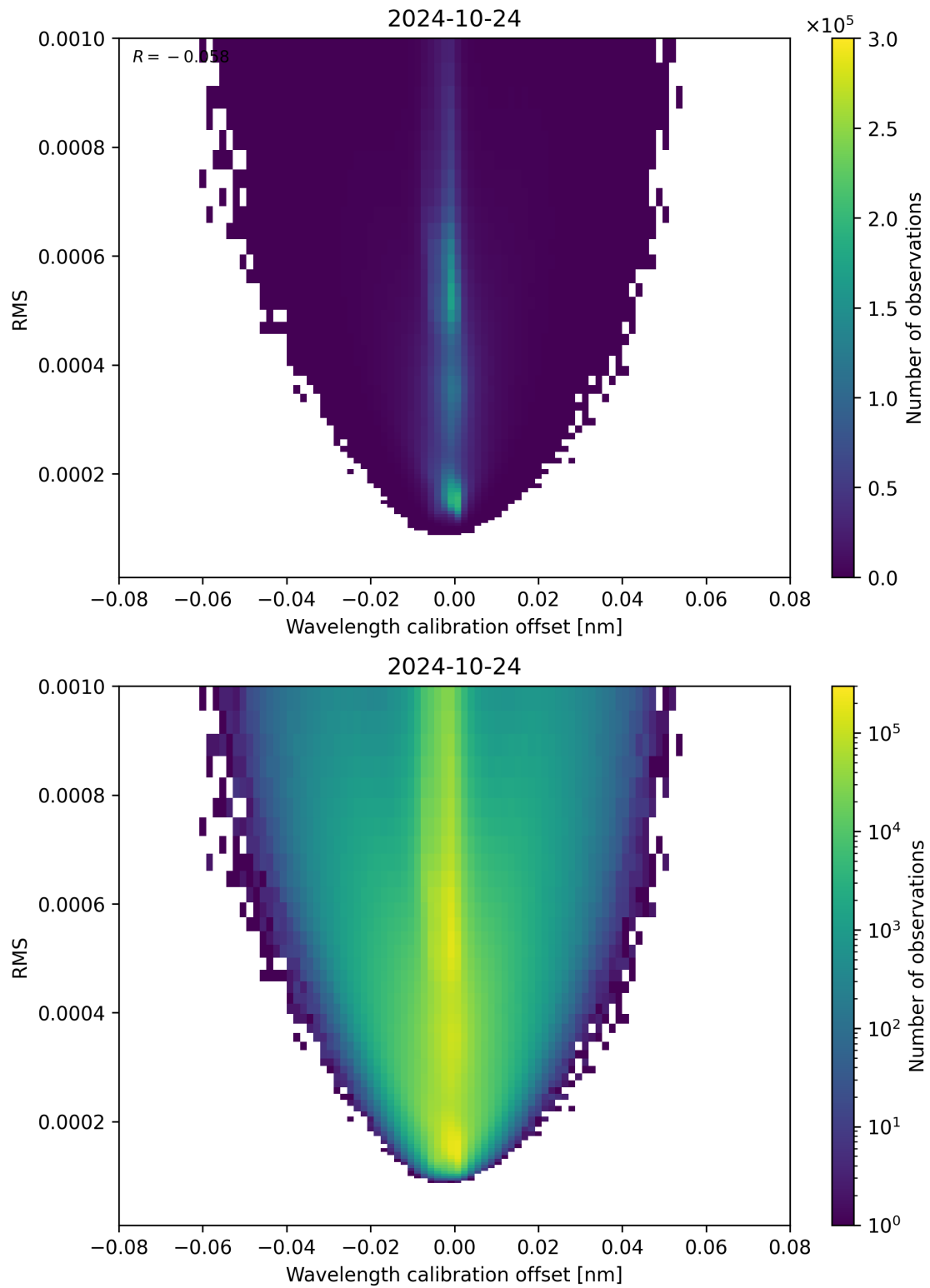
Figure 181: Scatter density plot of “Wavelength calibration offset” against “RMS” for 2024-10-24 to 2024-10-25.
