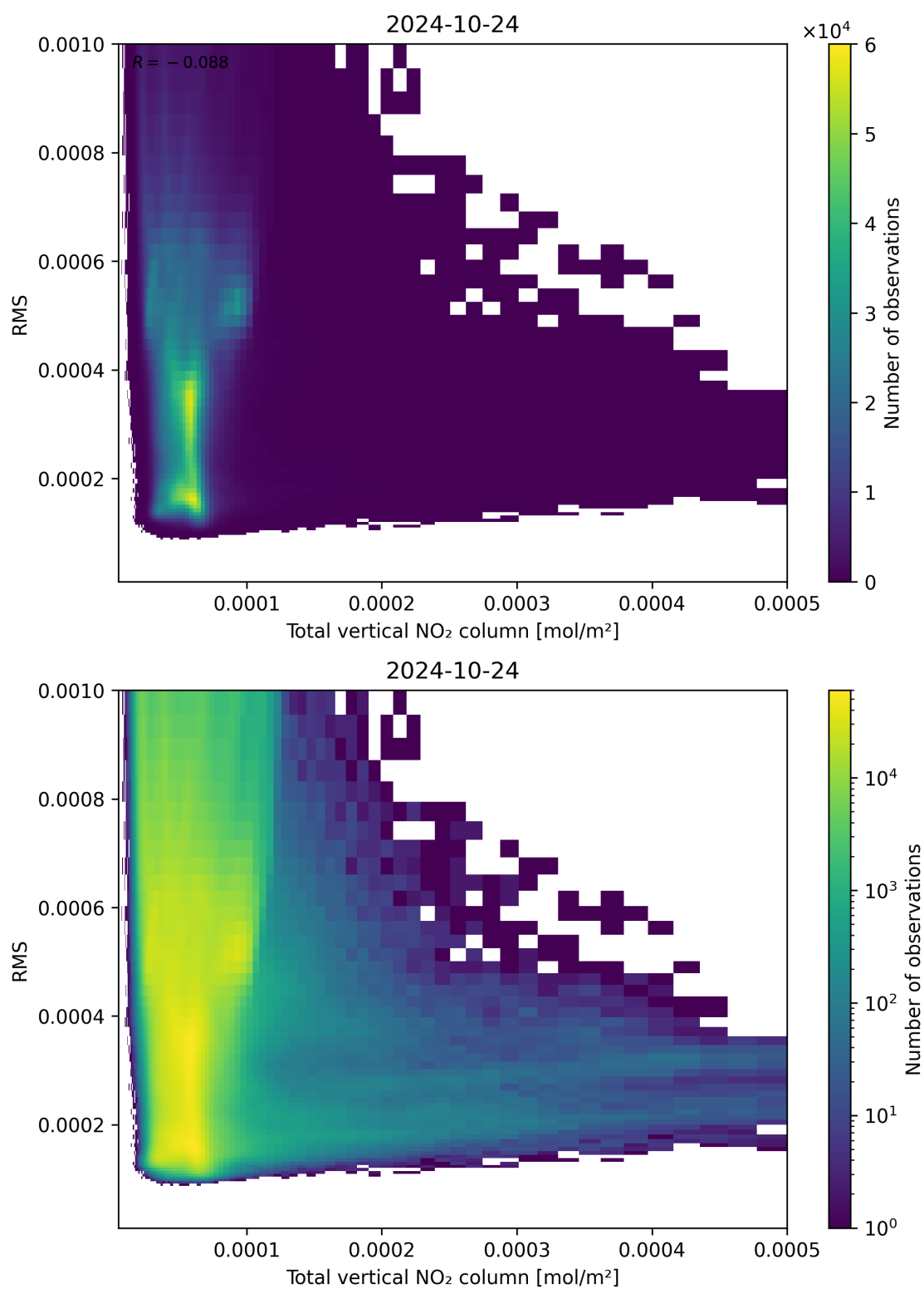
Figure 120: Scatter density plot of “Total vertical NO 2 column” against “RMS” for 2024-10-24 to 2024-10-25.
