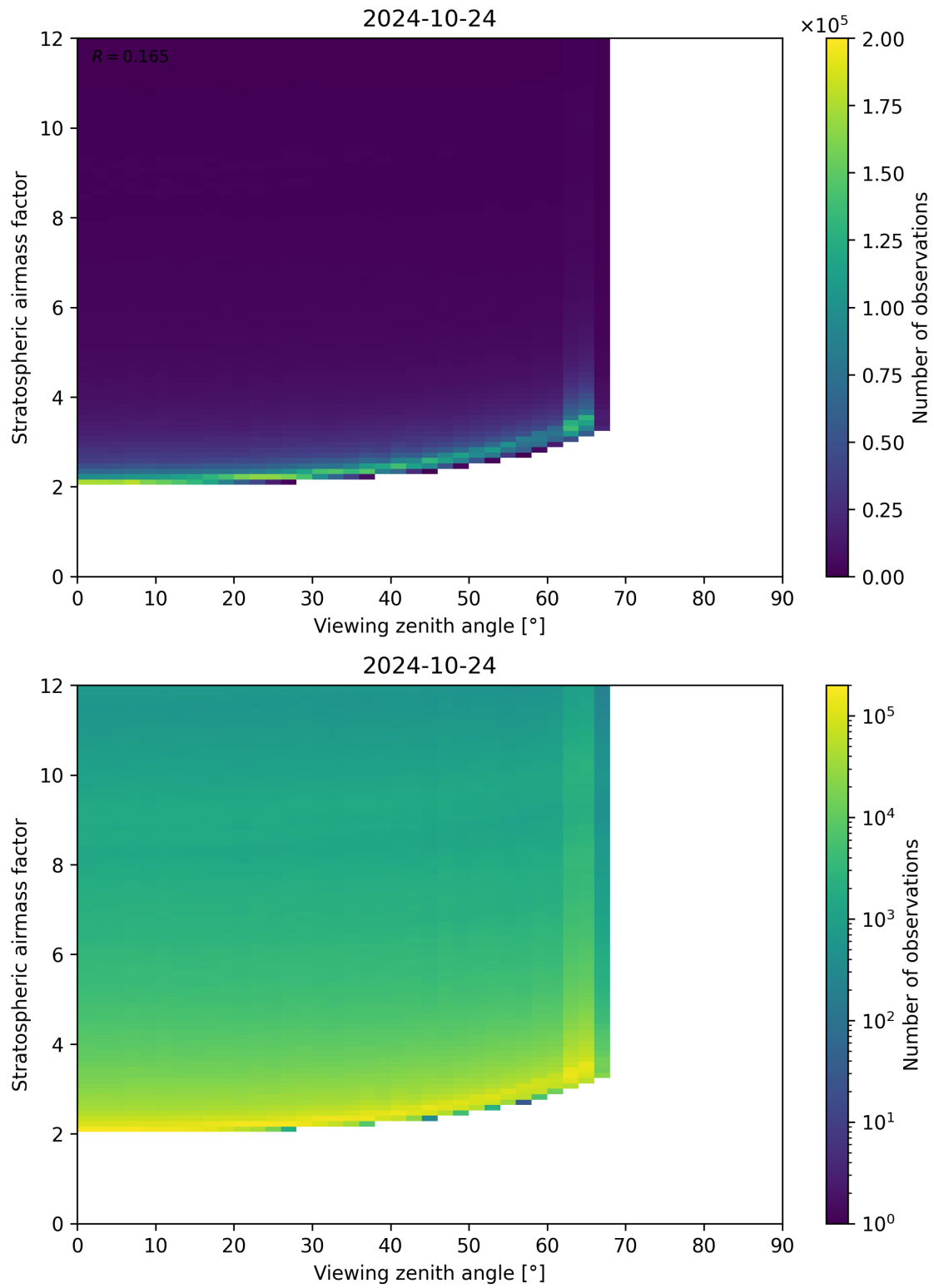
Figure 159: Scatter density plot of “Viewing zenith angle” against “Stratospheric airmass factor” for 2024-10-24 to 2024-10-25.
