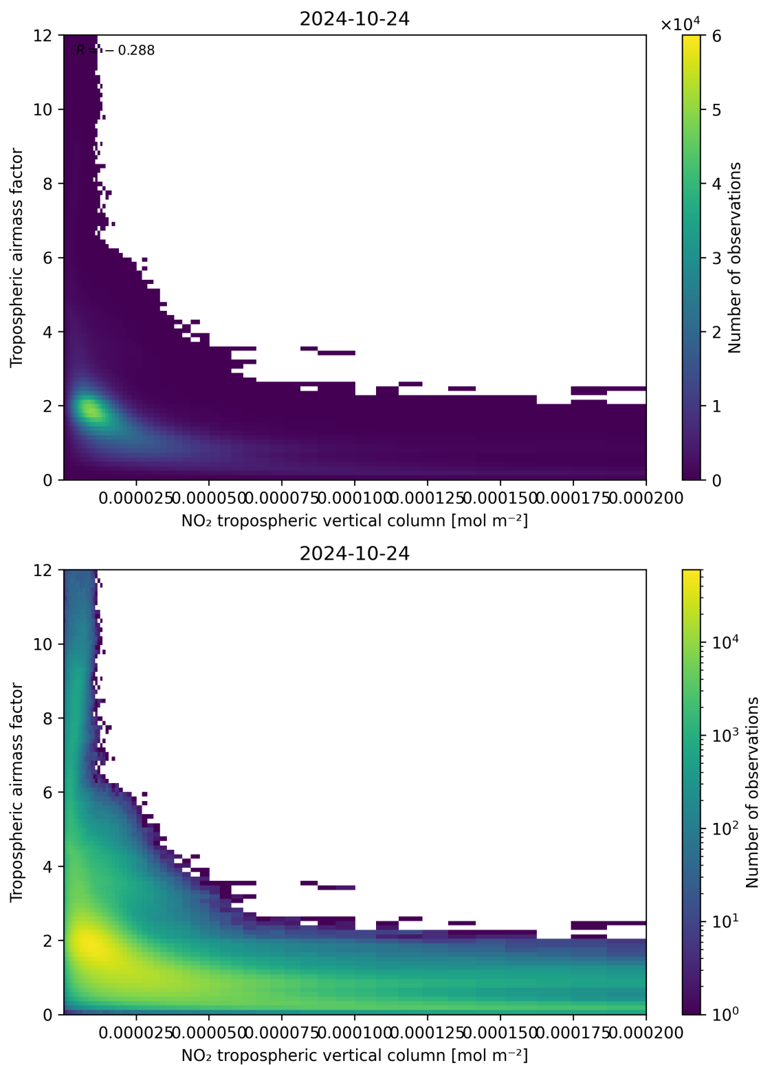
Figure 123: Scatter density plot of “NO 2 tropospheric vertical column” against “Tropospheric air mass factor” for 2024-10-24 to 2024-10-25.
