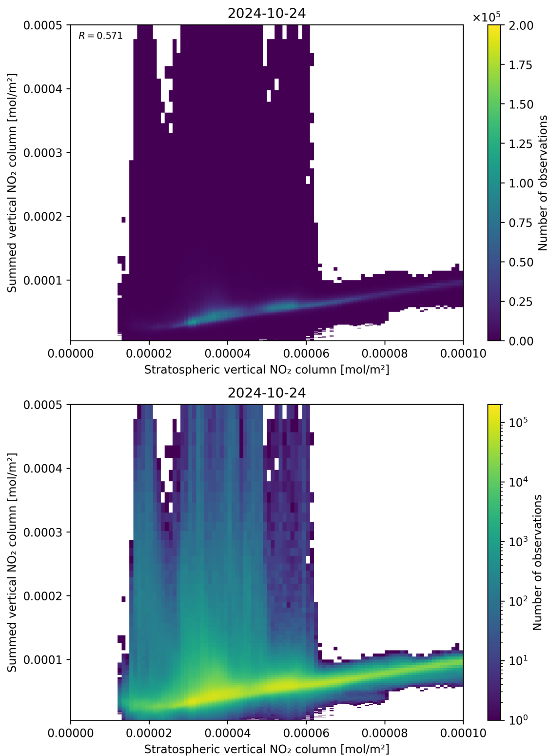
Figure 98: Scatter density plot of “Stratospheric vertical NO 2 column” against “Summed vertical NO 2 column” for 2024-10-24 to 2024-10-25.
