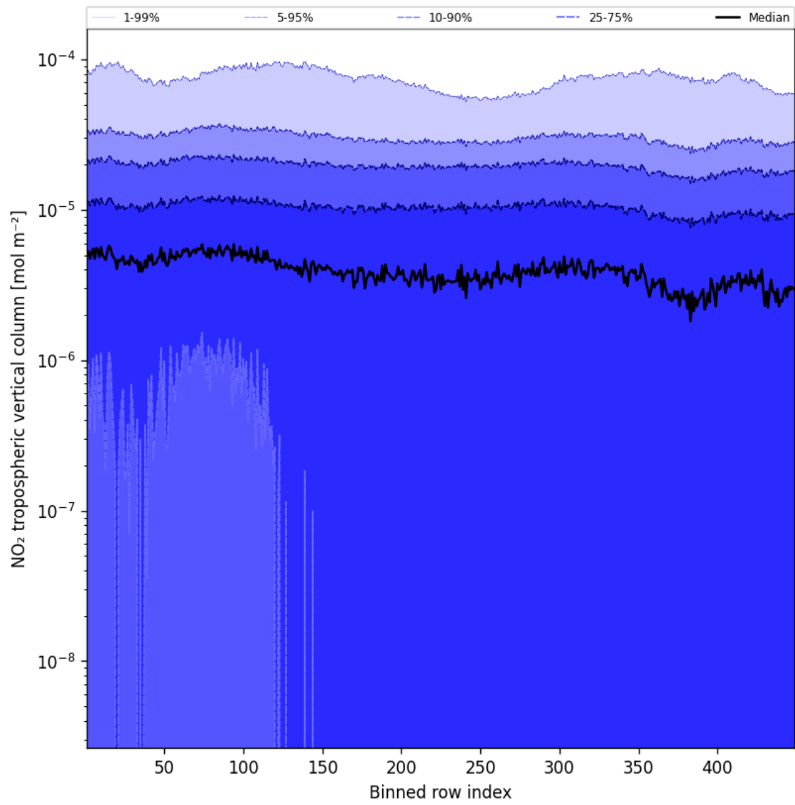
Figure 46: Along track statistics of “NO 2 tropospheric vertical column” for 2024-10-24 to 2024-10-25
