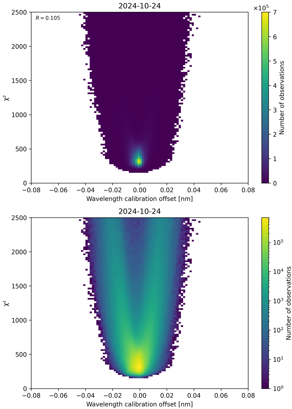
Figure 175: Scatter density plot of “Wavelength calibration offset” against “ \chi^2 ” for 2024-10-24 to 2024-10-25.
