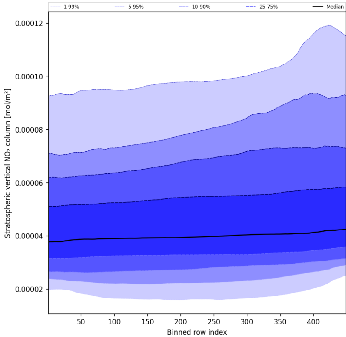
Figure 53: Along track statistics of “Stratospheric vertical NO 2 column” for 2024-10-24 to 2024-10-25
