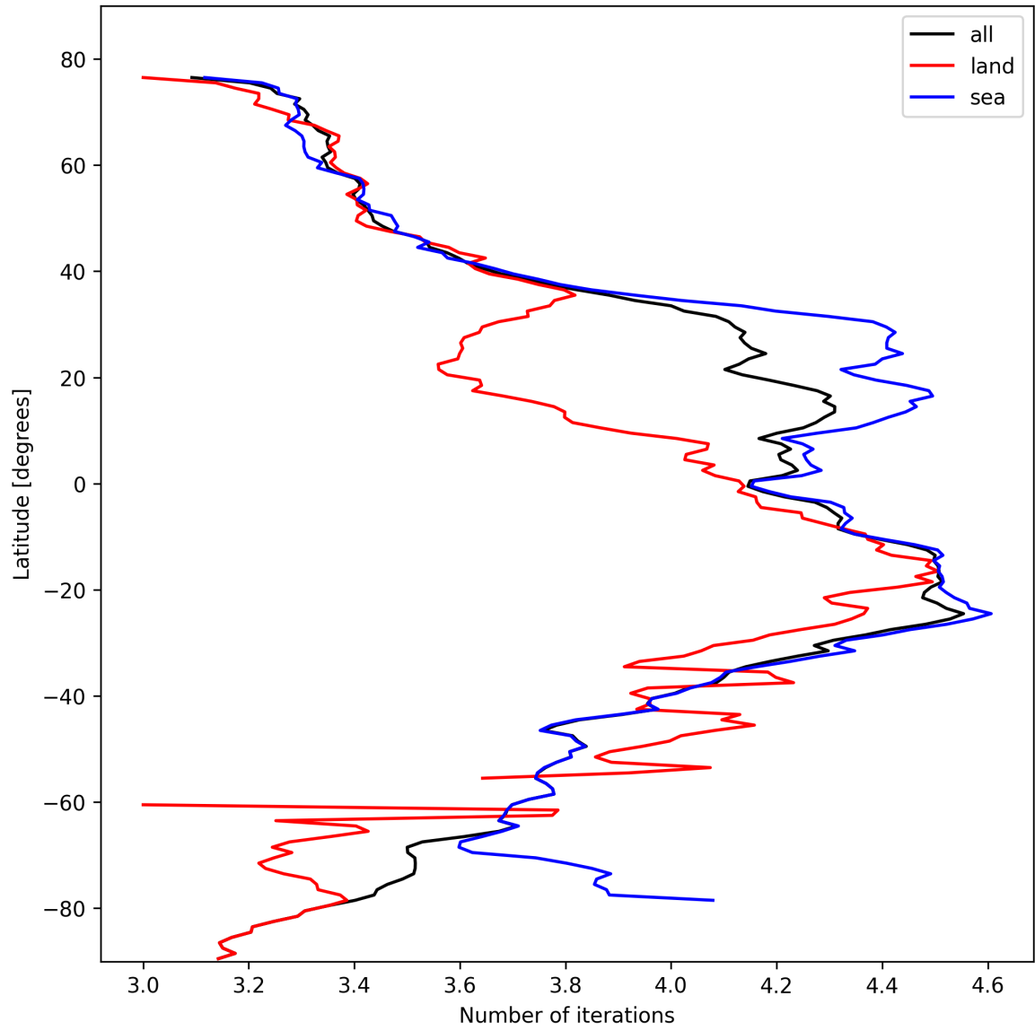
Figure 17: Zonal average of “Number of iterations” for 2024-10-24 to 2024-10-25.
