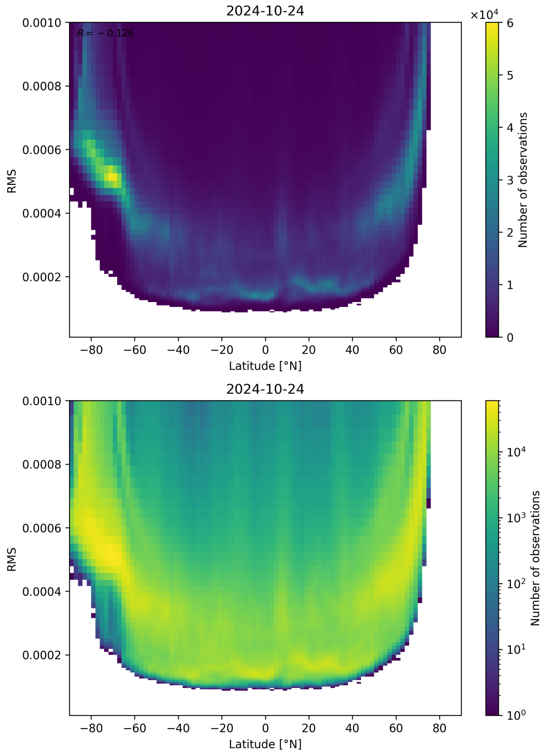
Figure 94: Scatter density plot of “Latitude” against “RMS” for 2024-10-24 to 2024-10-25.
