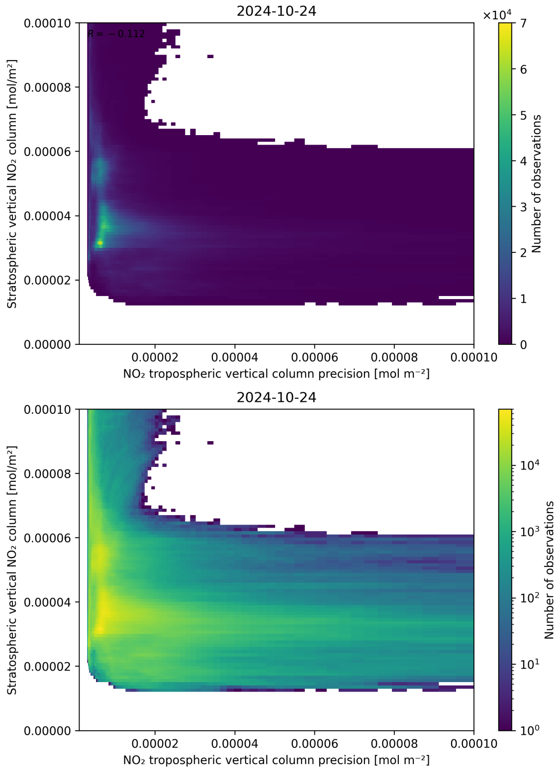
Figure 135: Scatter density plot of “NO 2 tropospheric vertical column precision” against “Stratospheric vertical NO 2 column” for 2024-10-24 to 2024-10-25.
