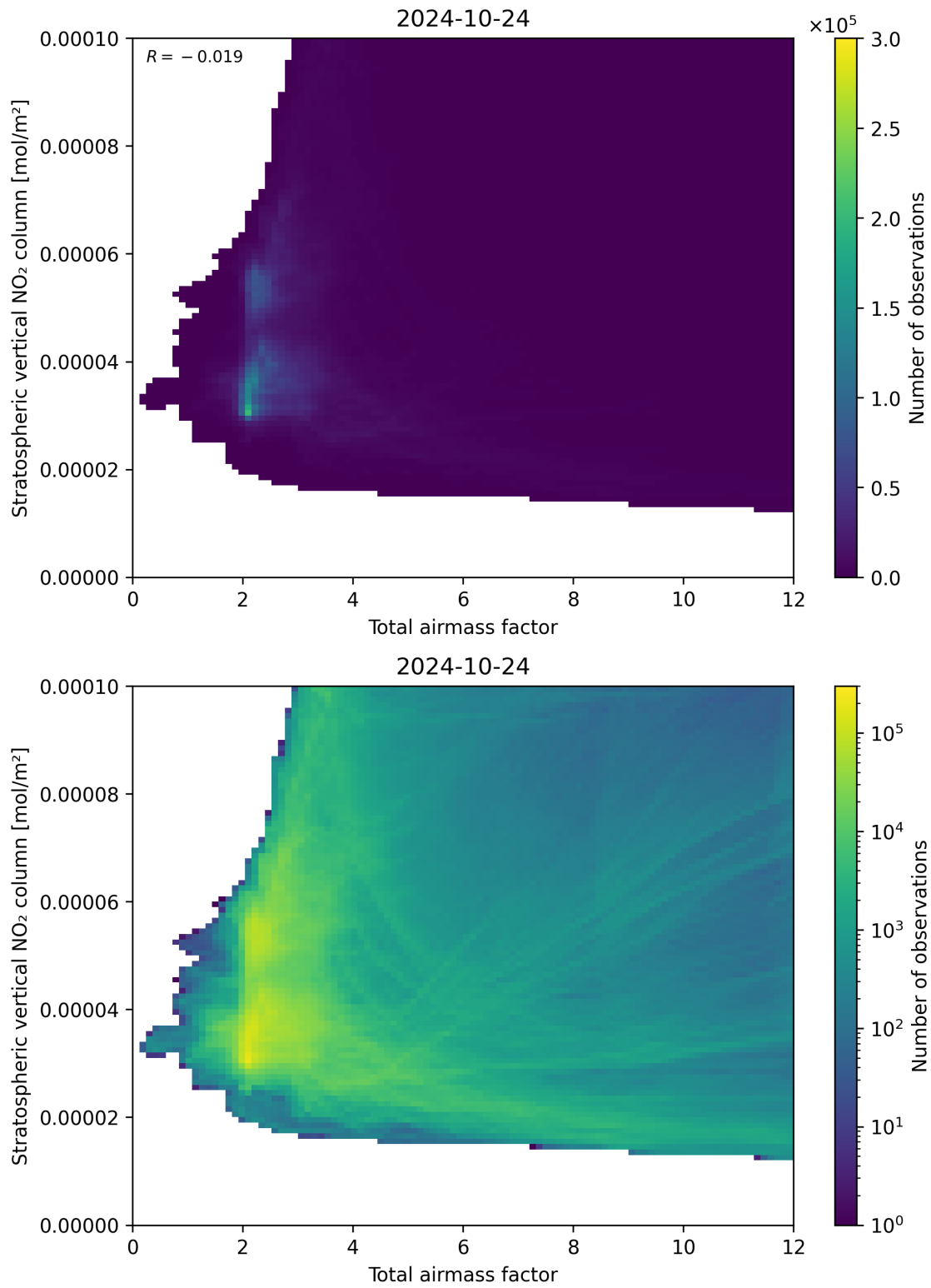
Figure 64: Scatter density plot of “Total airmass factor” against “Stratospheric vertical NO 2 column” for 2024-10-24 to 2024-10-25.
