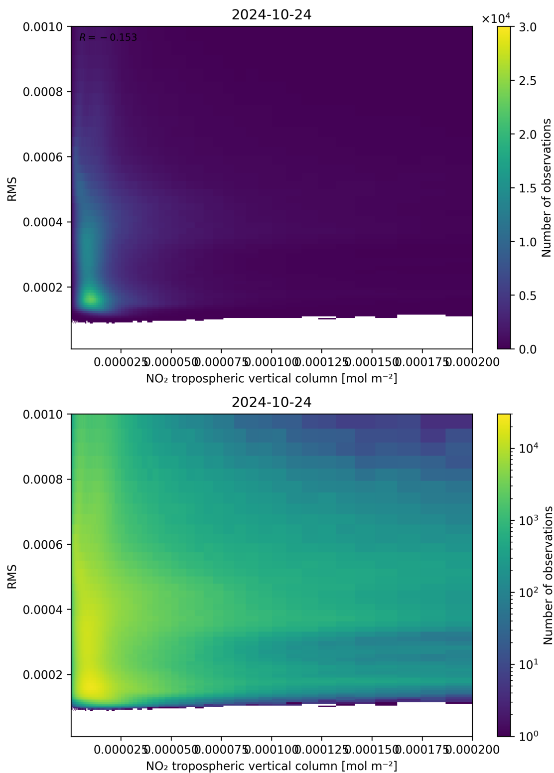
Figure 142: Scatter density plot of “NO 2 tropospheric vertical column” against “RMS” for 2024-10-24 to 2024-10-25.
