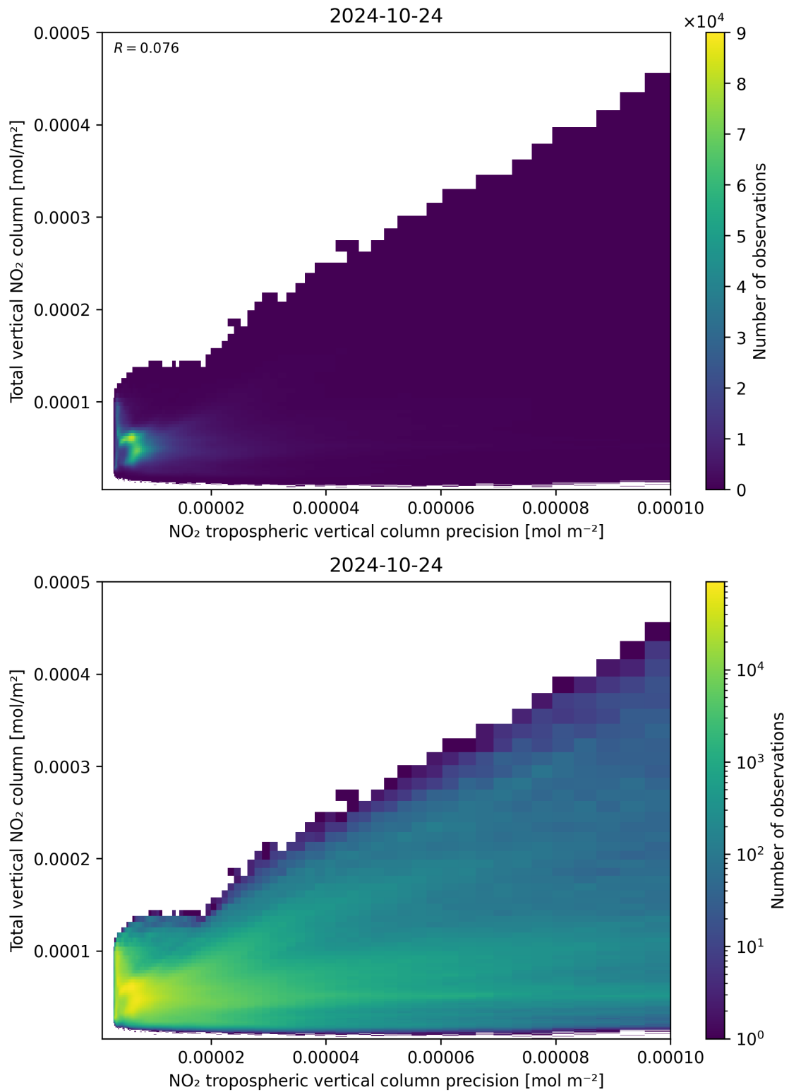
Figure 138: Scatter density plot of “NO 2 tropospheric vertical column precision” against “Total vertical NO 2 column” for 2024-10-24 to 2024-10-25.
