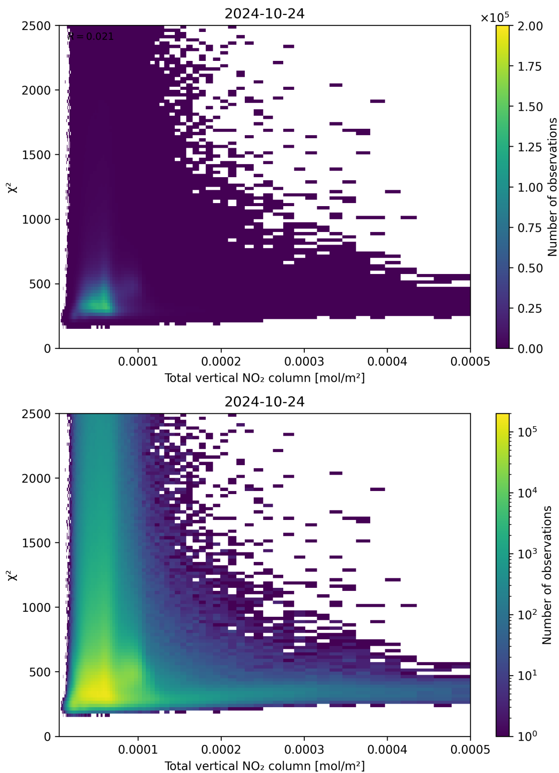
Figure 111: Scatter density plot of “Total vertical NO 2 column” against “ \chi^2 ” for 2024-10-24 to 2024-10-25.
