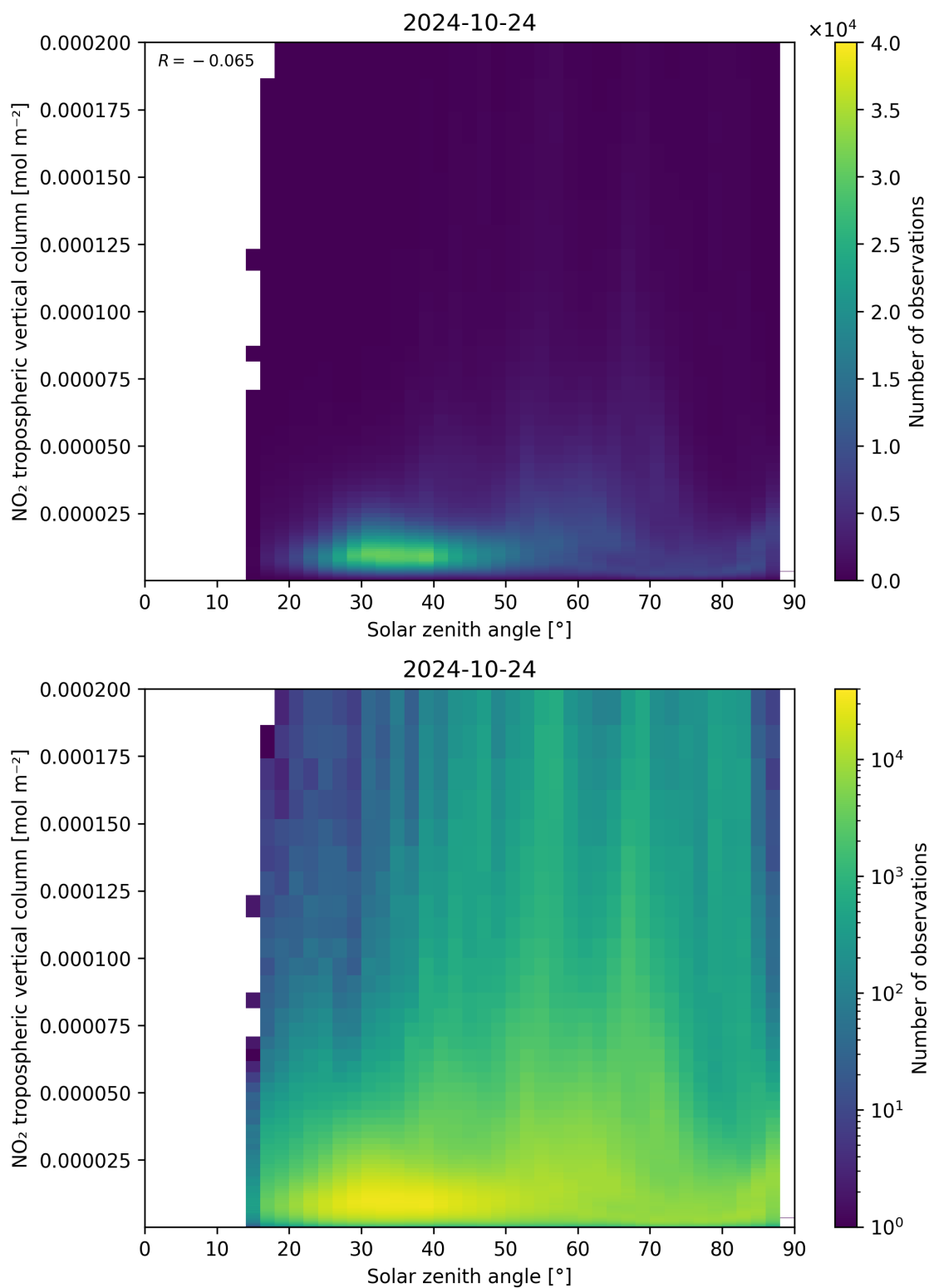
Figure 155: Scatter density plot of “Solar zenith angle” against “NO 2 tropospheric vertical column” for 2024-10-24 to 2024-10-25.
