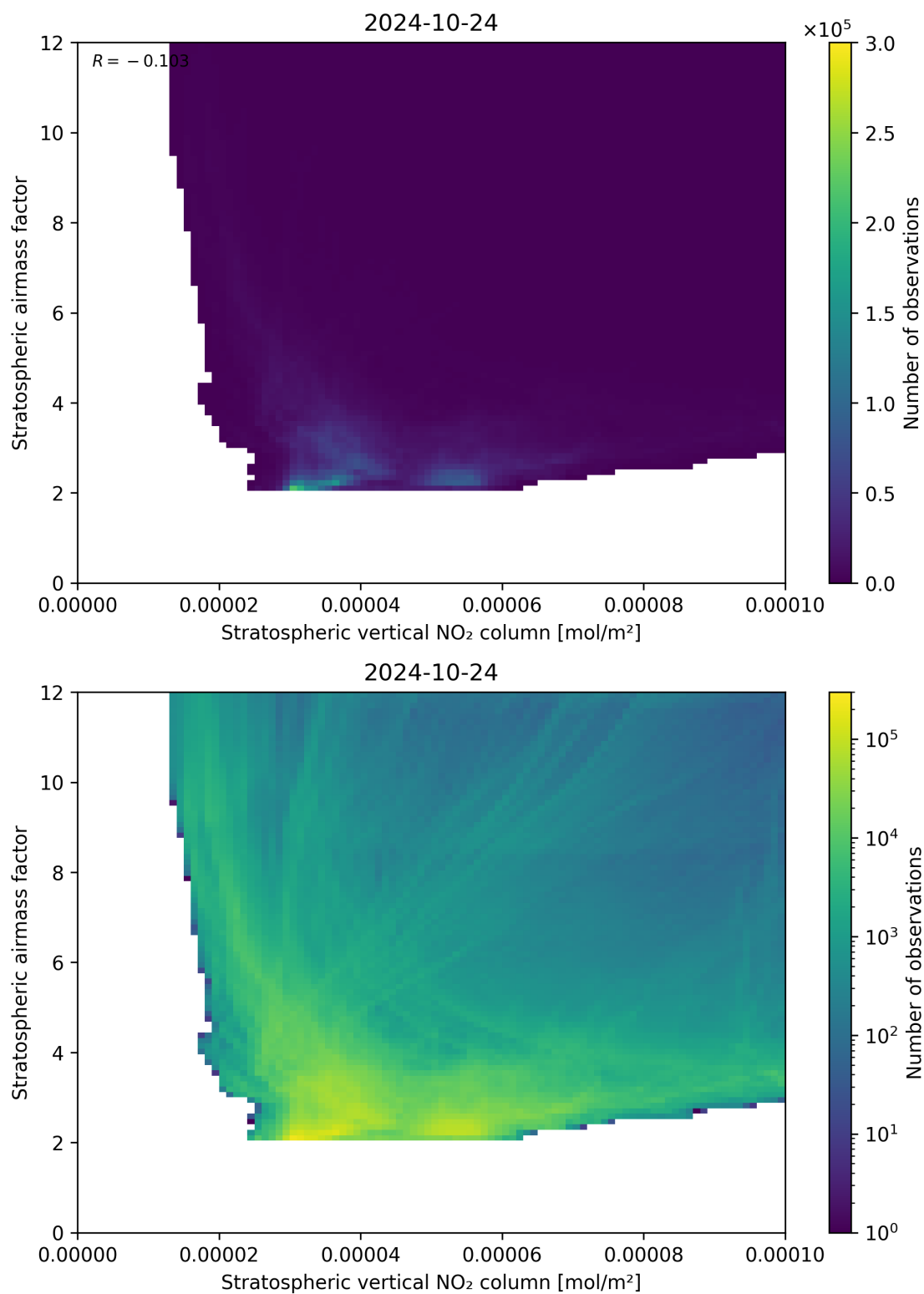
Figure 96: Scatter density plot of “Stratospheric vertical NO 2 column” against “Stratospheric airmass factor” for 2024-10-24 to 2024-10-25.
