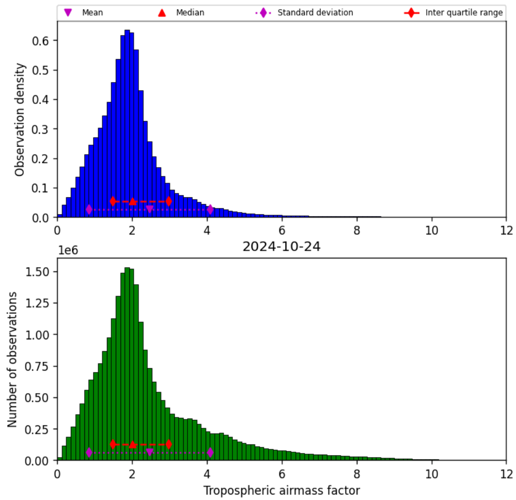
Figure 31: Histogram of “Tropospheric airmass factor” for 2024-10-24 to 2024-10-25
