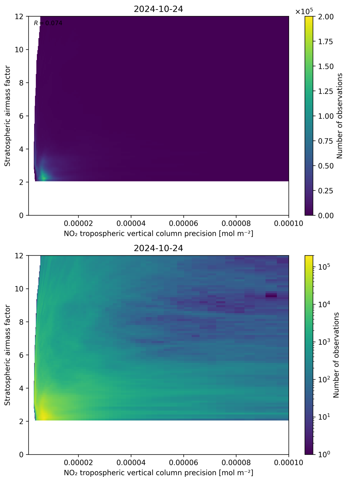
Figure 131: Scatter density plot of “NO 2 tropospheric vertical column precision” against “Stratospheric airmass factor” for 2024-10-24 to 2024-10-25.
