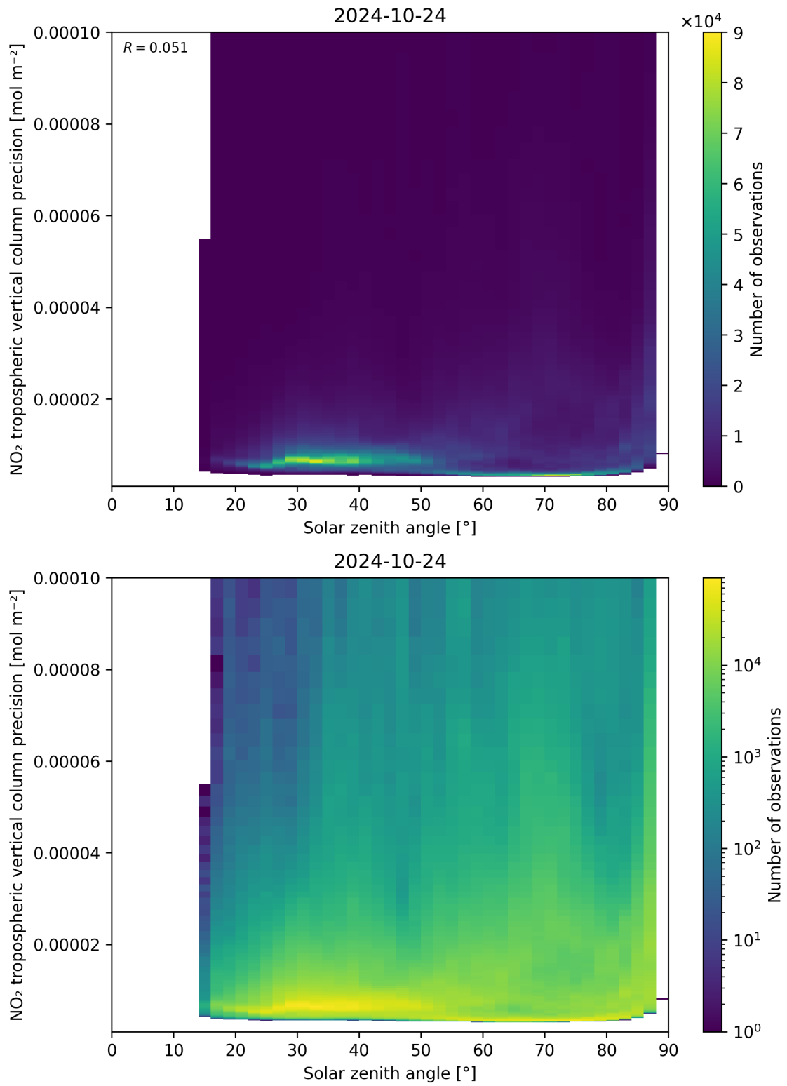
Figure 156: Scatter density plot of “Solar zenith angle” against “NO 2 tropospheric vertical column precision” for 2024-10-24 to 2024-10-25.
