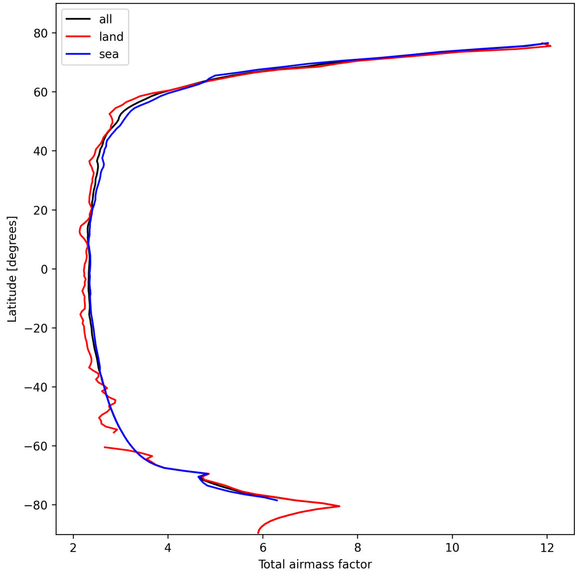
Figure 15: Zonal average of “Total airmass factor” for 2024-10-24 to 2024-10-25.
