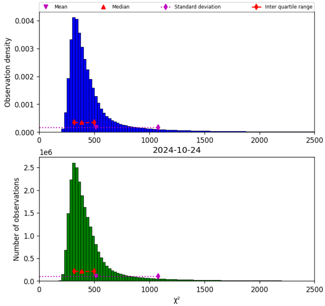
Figure 42: Histogram of “ \chi^2 ” for 2024-10-24 to 2024-10-25
