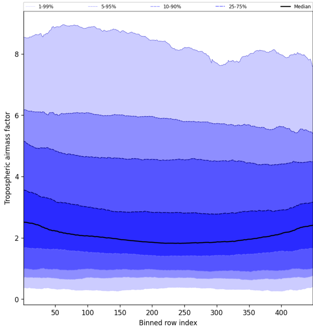
Figure 48: Along track statistics of “Tropospheric air mass factor” for 2024-10-24 to 2024-10-25
