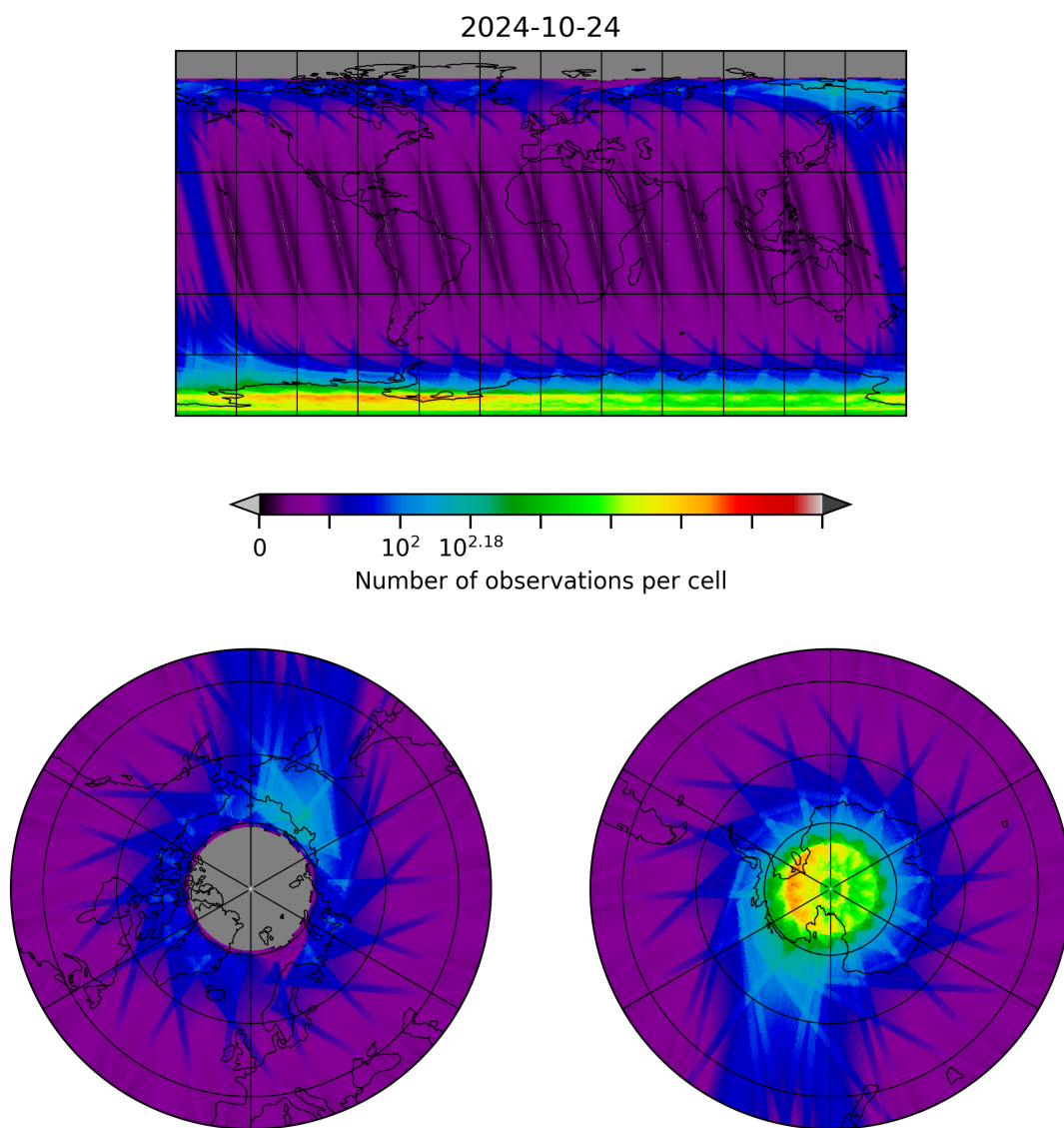
Figure 10: Map of the number of observations for 2024-10-24 to 2024-10-25
