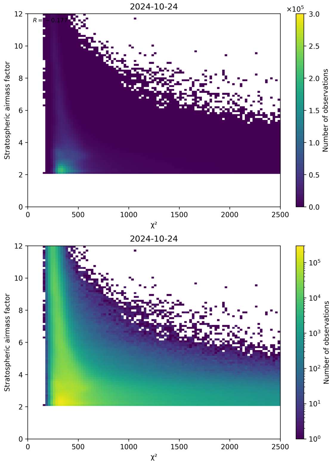
Figure 81: Scatter density plot of “ \chi^2 ” against “Stratospheric airmass factor” for 2024-10-24 to 2024-10-25.
