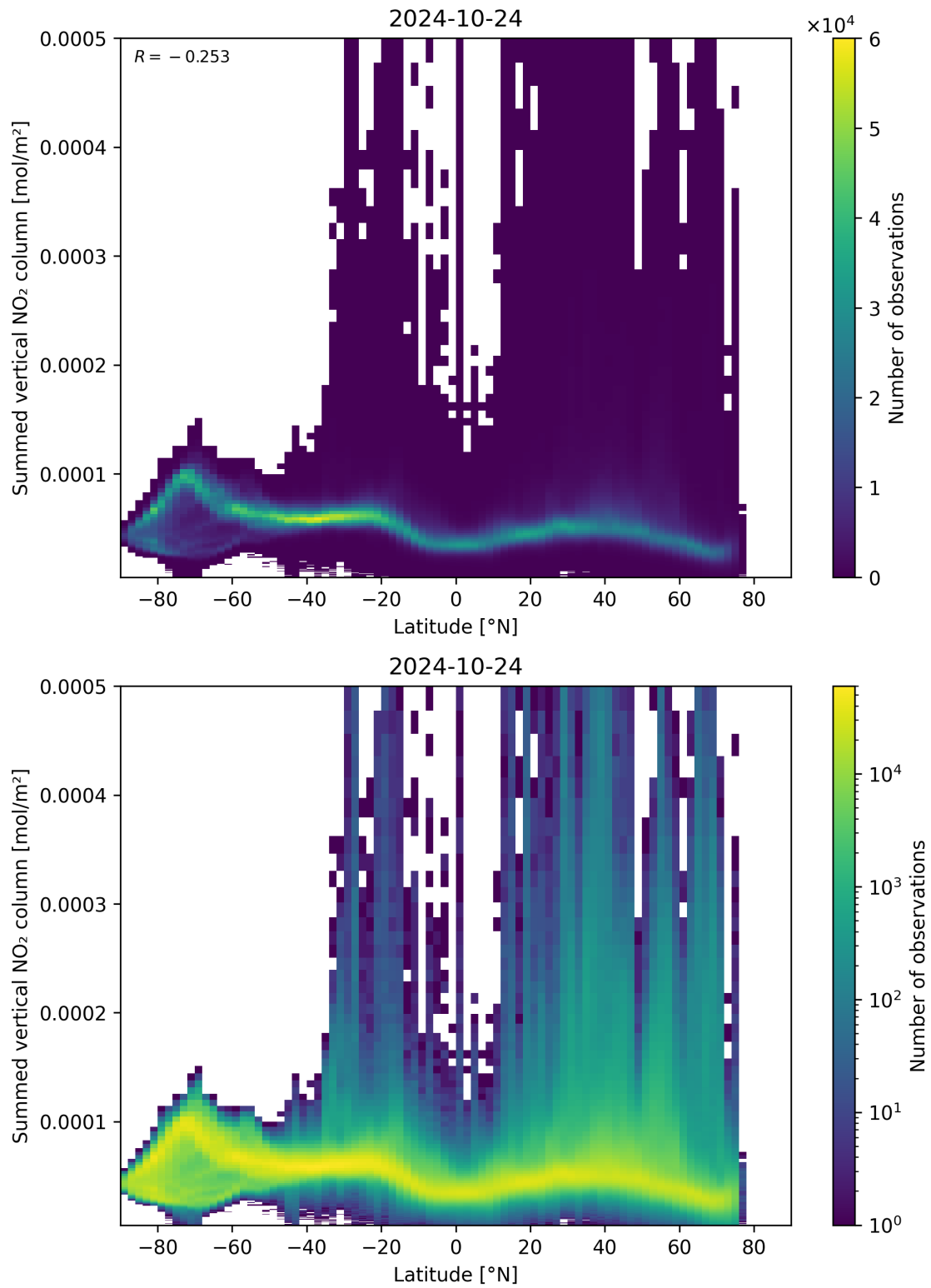
Figure 88: Scatter density plot of “Latitude” against “Summed vertical NO 2 column” for 2024-10-24 to 2024-10-25.
