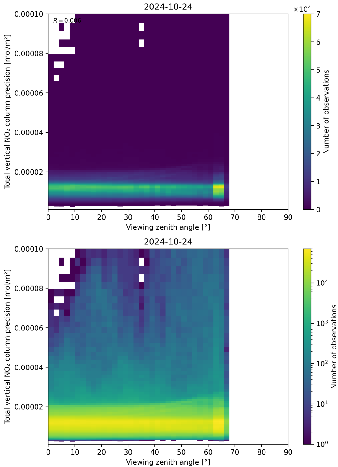
Figure 168: Scatter density plot of “Viewing zenith angle” against “Total vertical NO 2 column precision” for 2024-10-24 to 2024-10-25.
