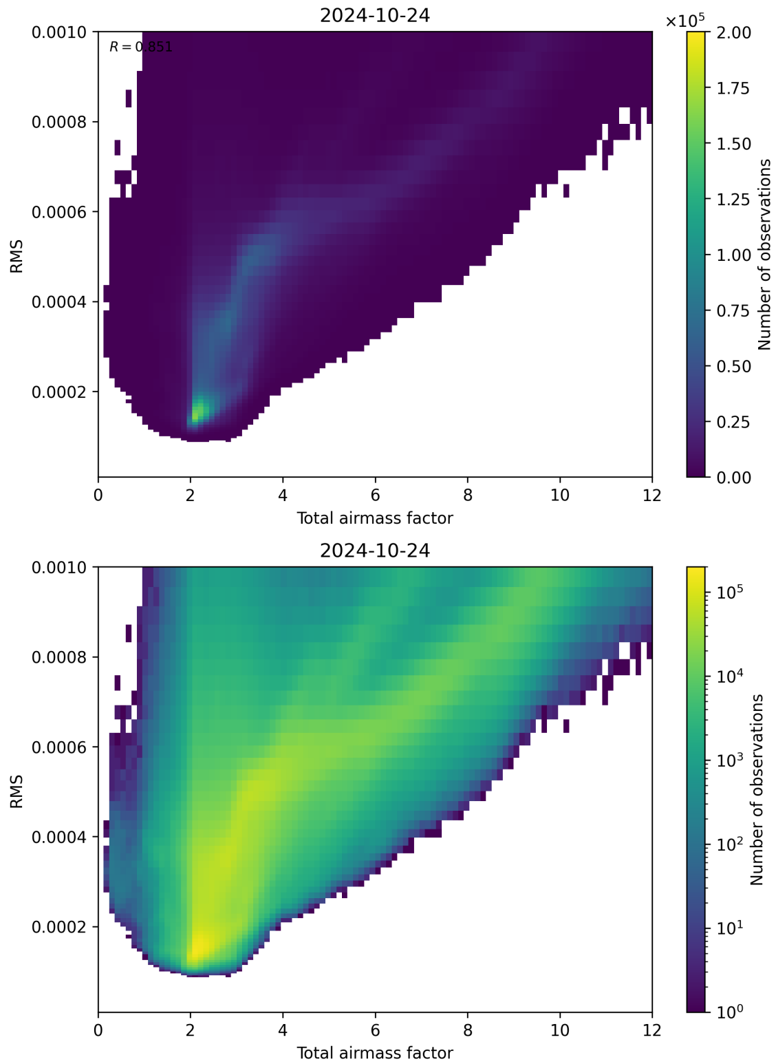
Figure 69: Scatter density plot of “Total airmass factor” against “RMS” for 2024-10-24 to 2024-10-25.
