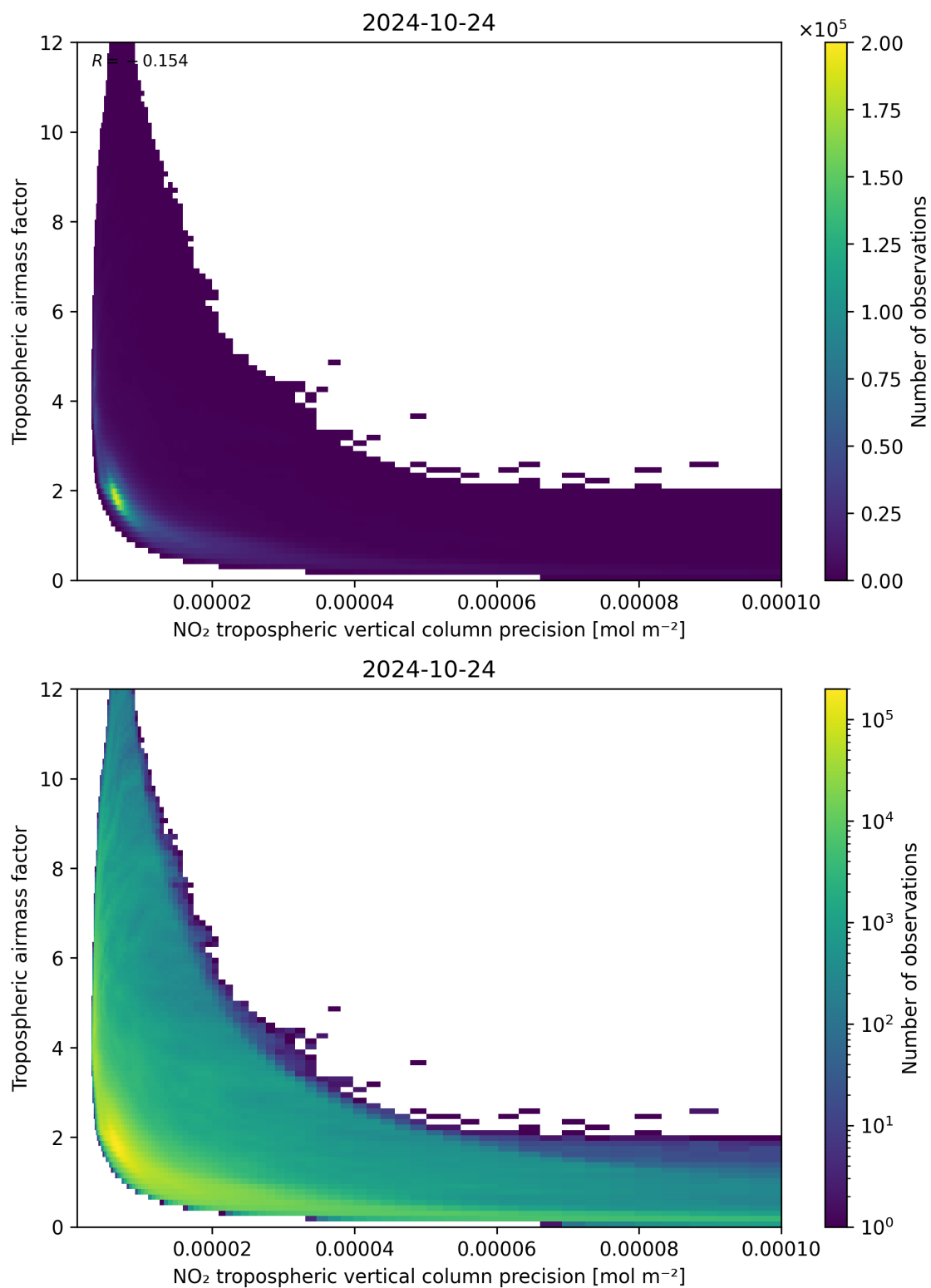
Figure 133: Scatter density plot of “NO 2 tropospheric vertical column precision” against “Tropospheric air mass factor” for 2024-10-24 to 2024-10-25.
