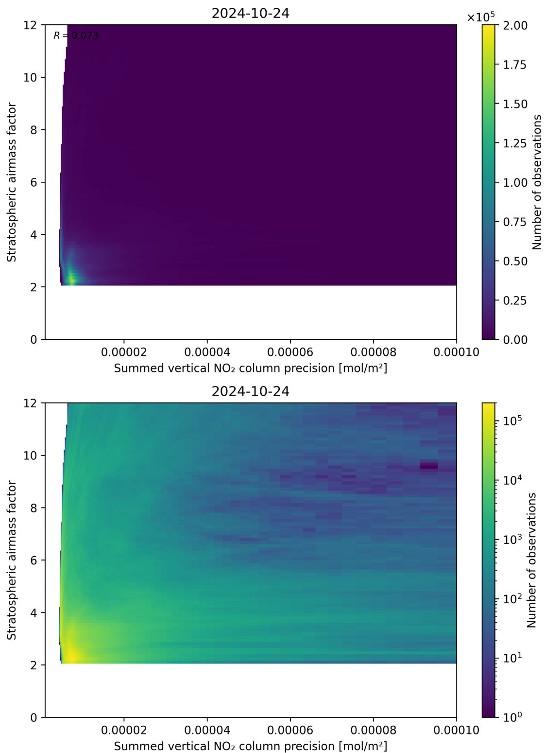
Figure 106: Scatter density plot of “Summed vertical NO 2 column precision” against “Stratospheric airmass factor” for 2024-10-24 to 2024-10-25.
