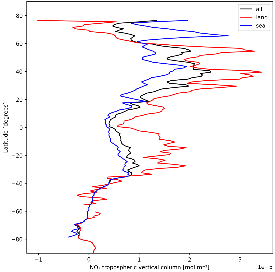
Figure 12: Zonal average of “NO 2 tropospheric vertical column” for 2024-10-24 to 2024-10-25.
