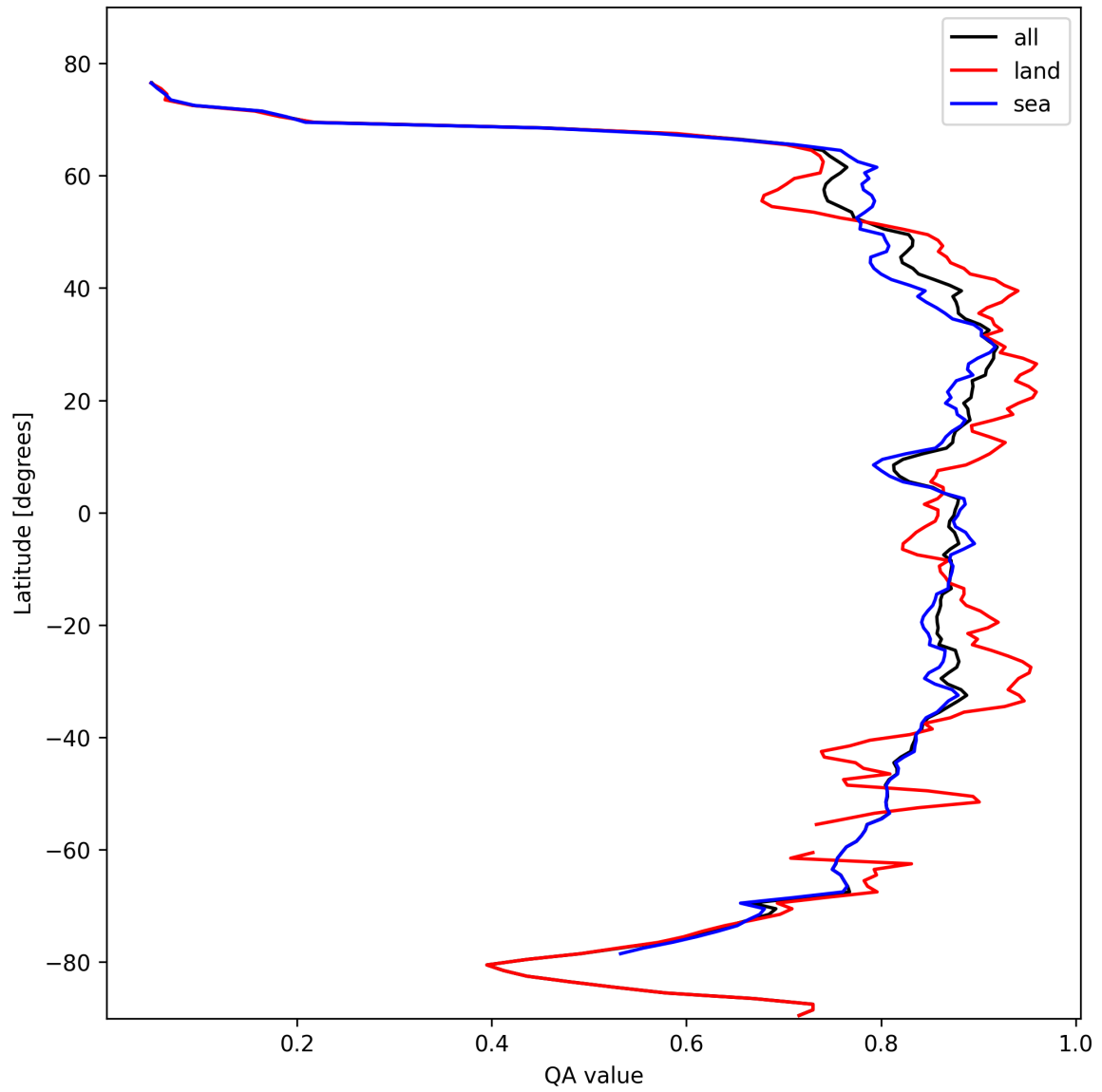
Figure 11: Zonal average of “QA value” for 2024-10-24 to 2024-10-25.
