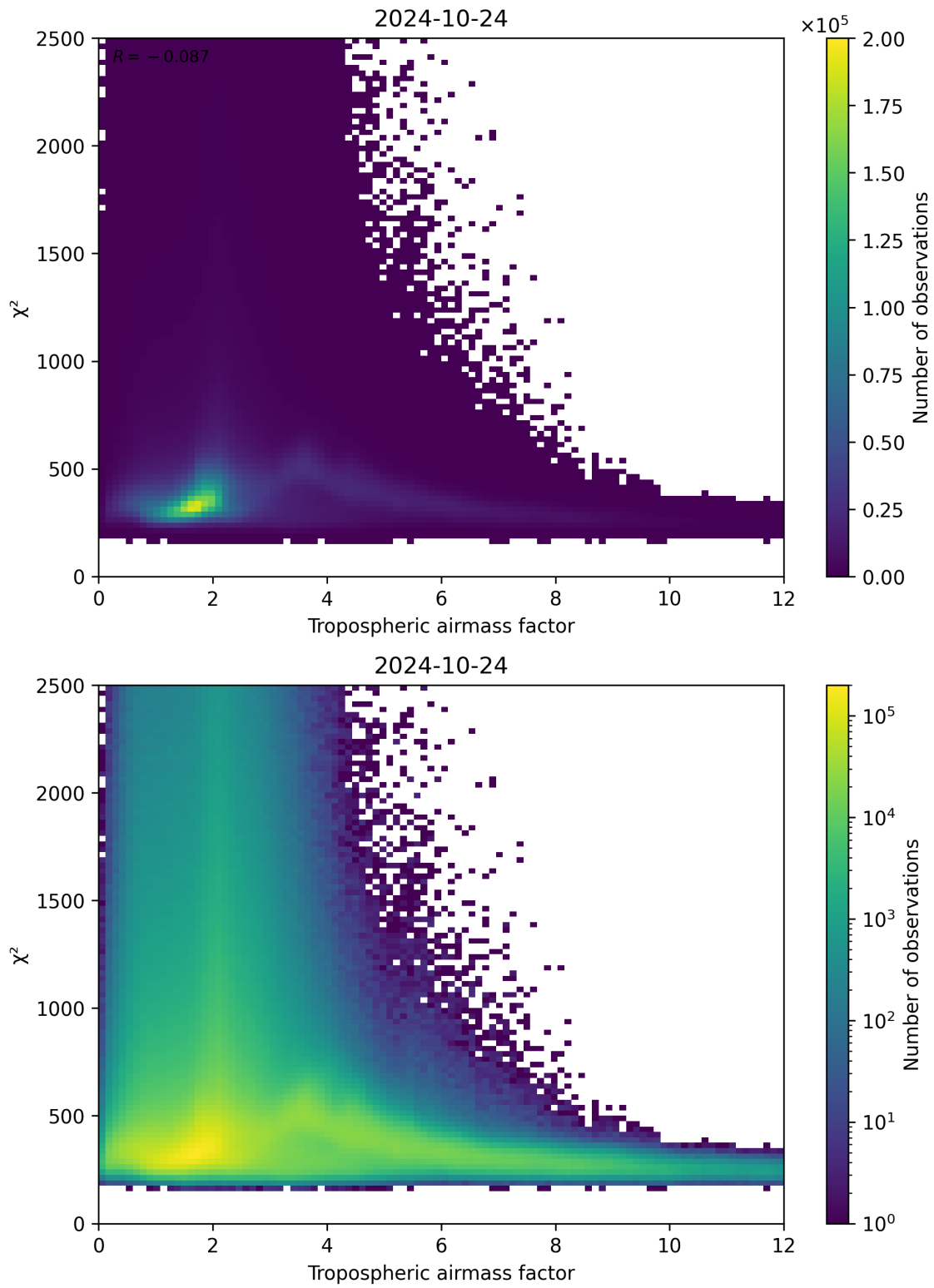
Figure 73: Scatter density plot of “Tropospheric airmass factor” against “ \chi^2 ” for 2024-10-24 to 2024-10-25.
