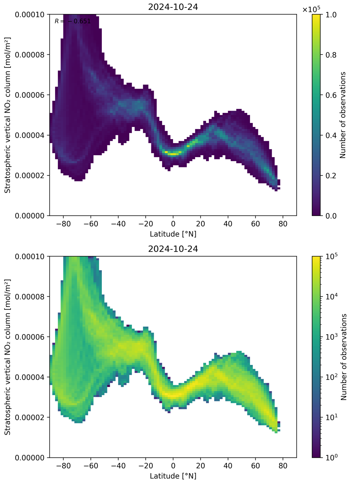
Figure 87: Scatter density plot of “Latitude” against “Stratospheric vertical NO 2 column” for 2024-10-24 to 2024-10-25.
