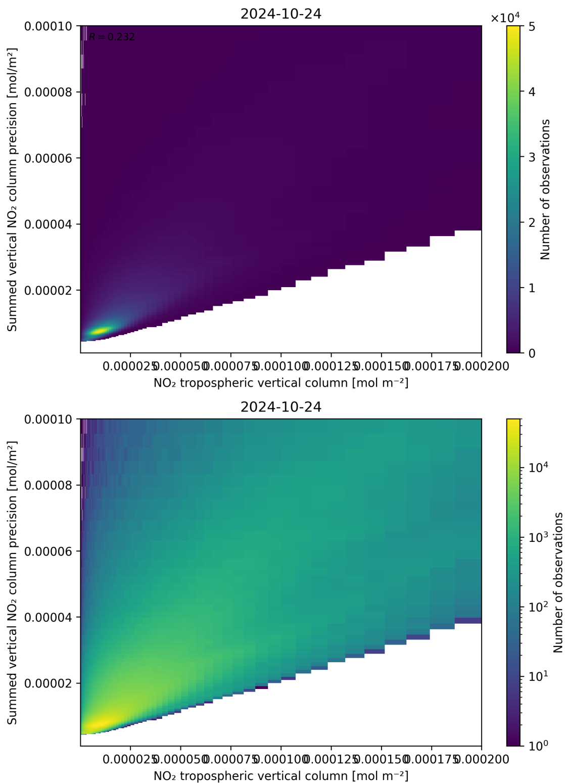
Figure 127: Scatter density plot of “NO 2 tropospheric vertical column” against “Summed vertical NO 2 column precision” for 2024-10-24 to 2024-10-25.
