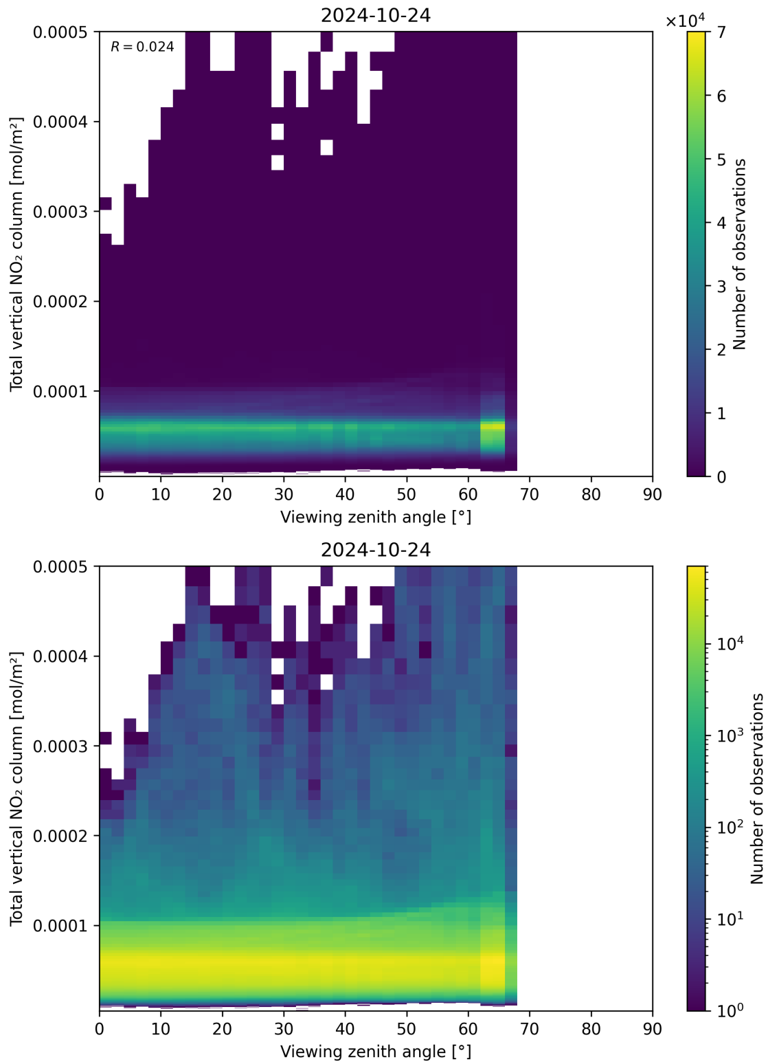
Figure 167: Scatter density plot of “Viewing zenith angle” against “Total vertical NO 2 column” for 2024-10-24 to 2024-10-25.
