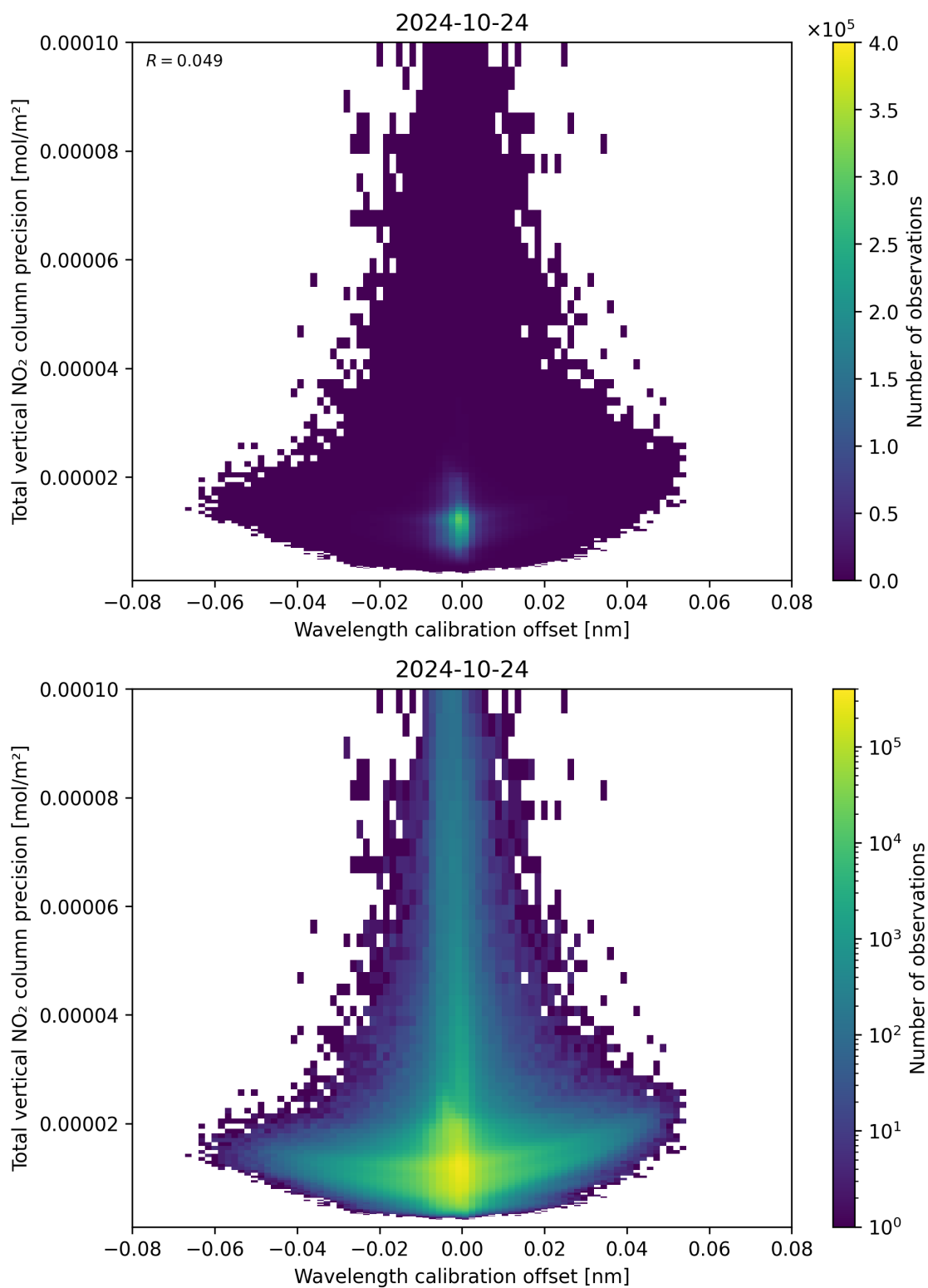
Figure 180: Scatter density plot of “Wavelength calibration offset” against “Total vertical NO 2 column precision” for 2024-10-24 to 2024-10-25.
