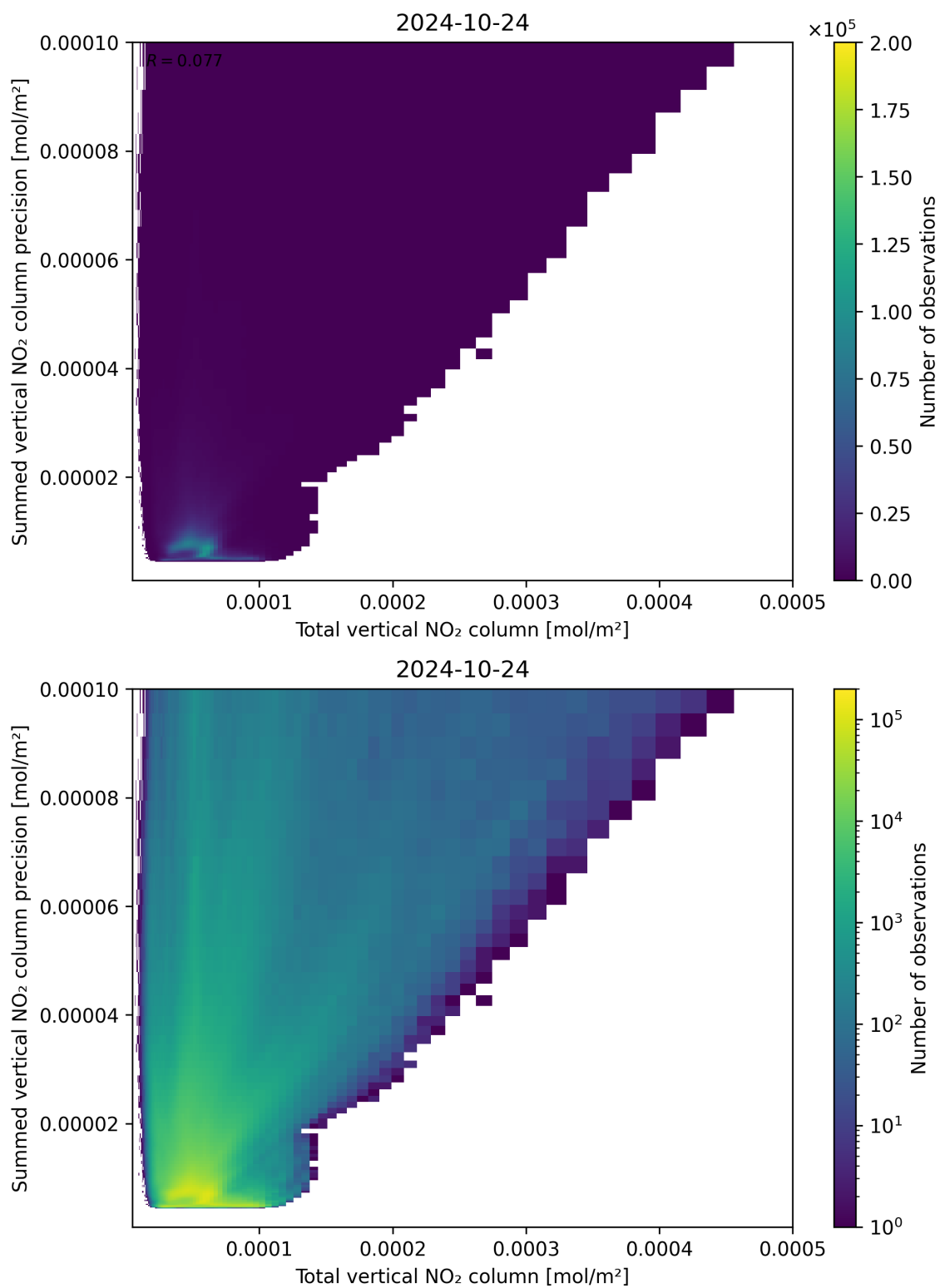
Figure 113: Scatter density plot of “Total vertical NO 2 column” against “Summed vertical NO 2 column precision” for 2024-10-24 to 2024-10-25.
