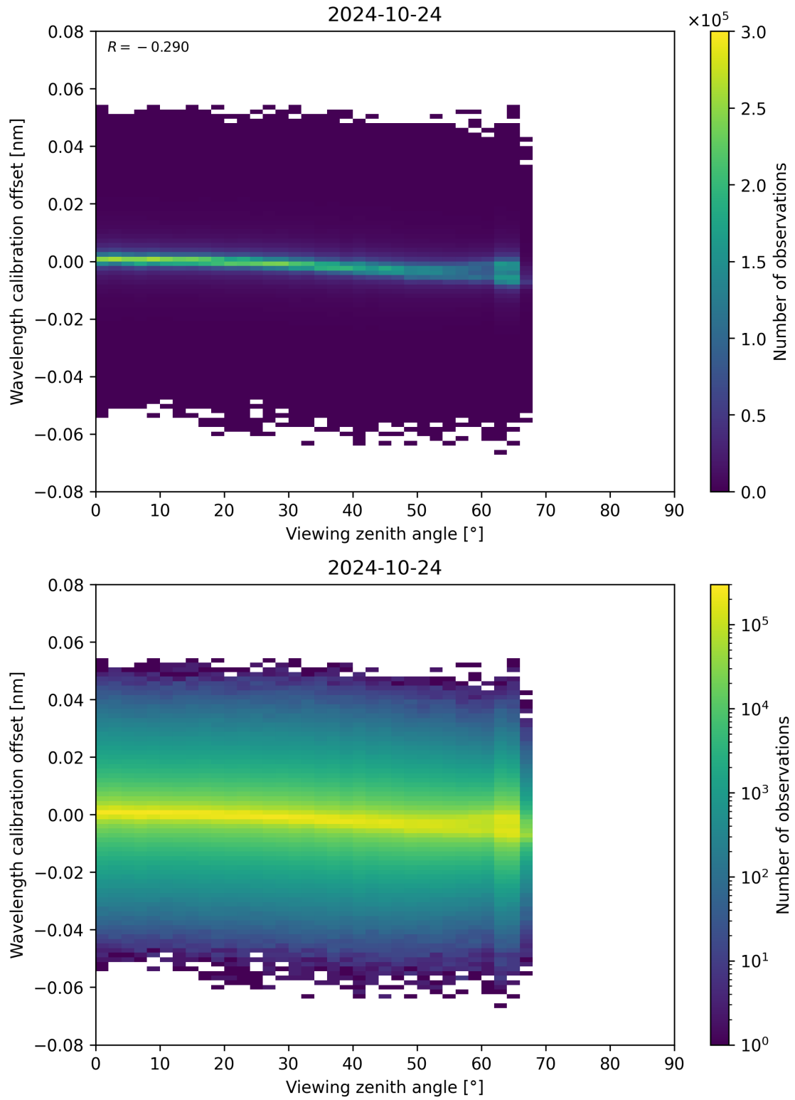
Figure 173: Scatter density plot of “Viewing zenith angle” against “Wavelength calibration offset” for 2024-10-24 to 2024-10-25.
