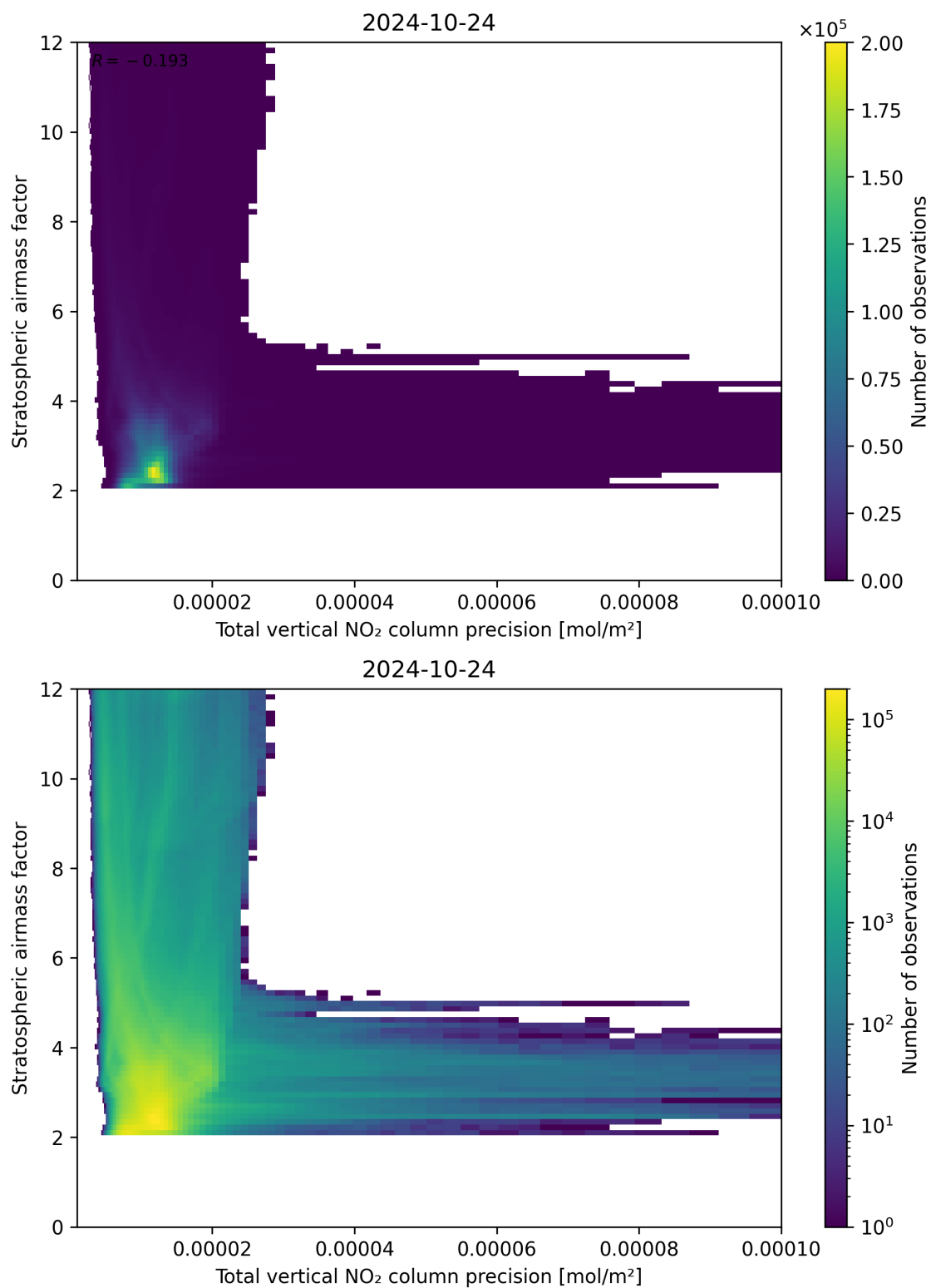
Figure 115: Scatter density plot of “Total vertical NO 2 column precision” against “Stratospheric airmass factor” for 2024-10-24 to 2024-10-25.
