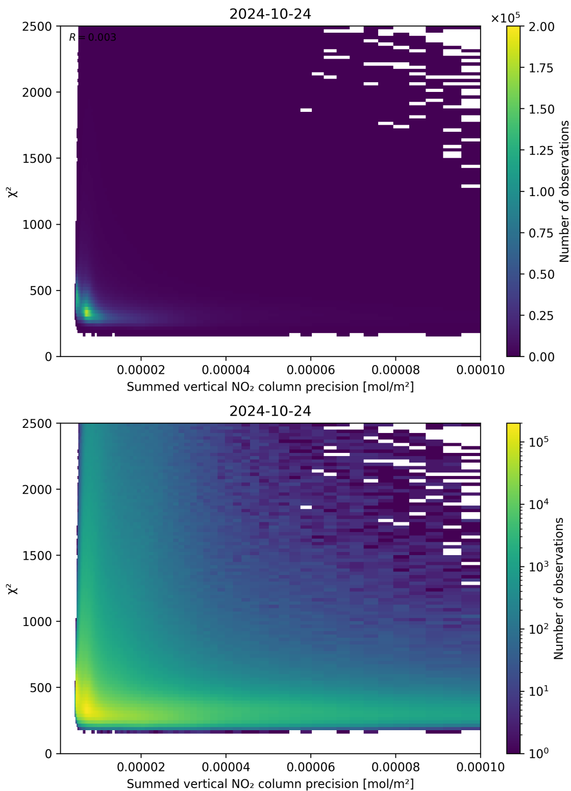
Figure 107: Scatter density plot of “Summed vertical NO 2 column precision” against “ \chi^2 ” for 2024-10-24 to 2024-10-25.
