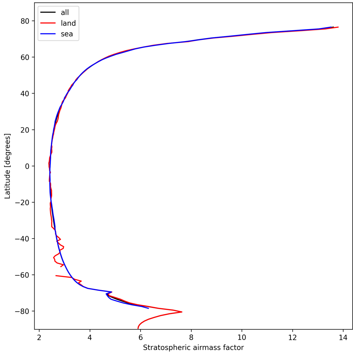
Figure 27: Zonal average of “Stratospheric airmass factor” for 2024-10-24 to 2024-10-25.
