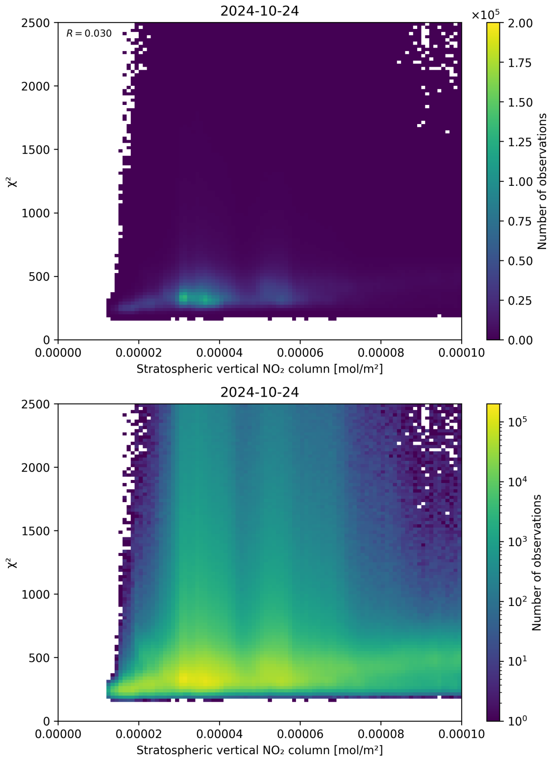
Figure 97: Scatter density plot of “Stratospheric vertical NO 2 column” against “ \chi^2 ” for 2024-10-24 to 2024-10-25.
