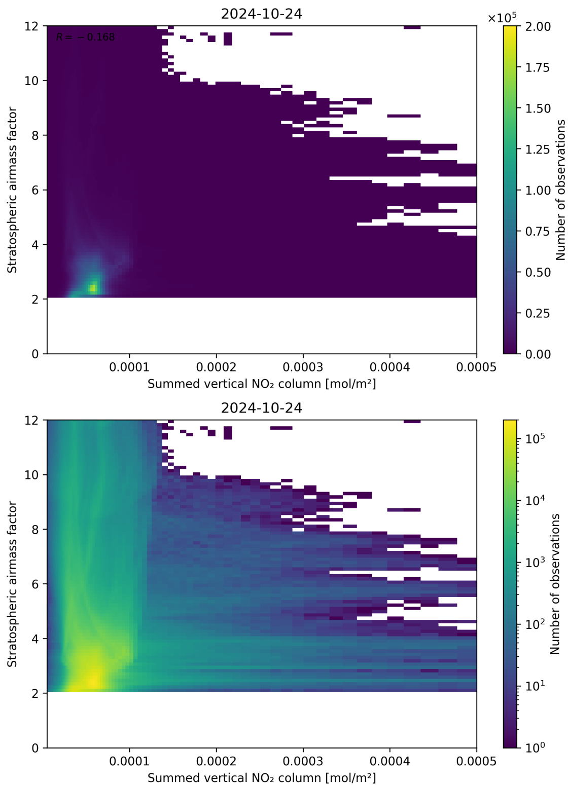
Figure 103: Scatter density plot of “Summed vertical NO 2 column” against “Stratospheric air mass factor” for 2024-10-24 to 2024-10-25.
