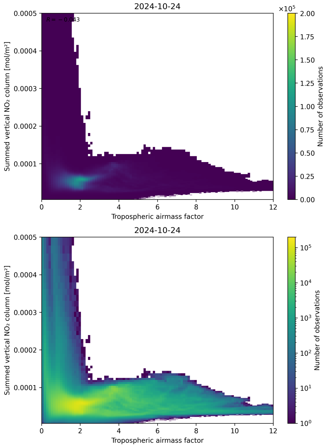
Figure 75: Scatter density plot of “Tropospheric airmass factor” against “Summed vertical NO 2 column” for 2024-10-24 to 2024-10-25.
