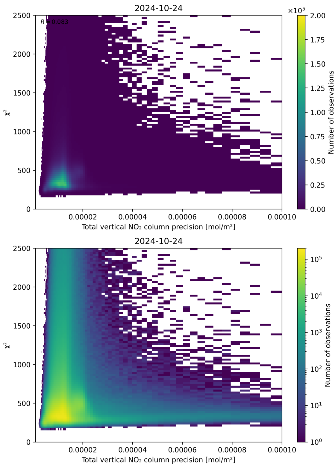
Figure 116: Scatter density plot of “Total vertical NO 2 column precision” against “ \chi^2 ” for 2024-10-24 to 2024-10-25.
