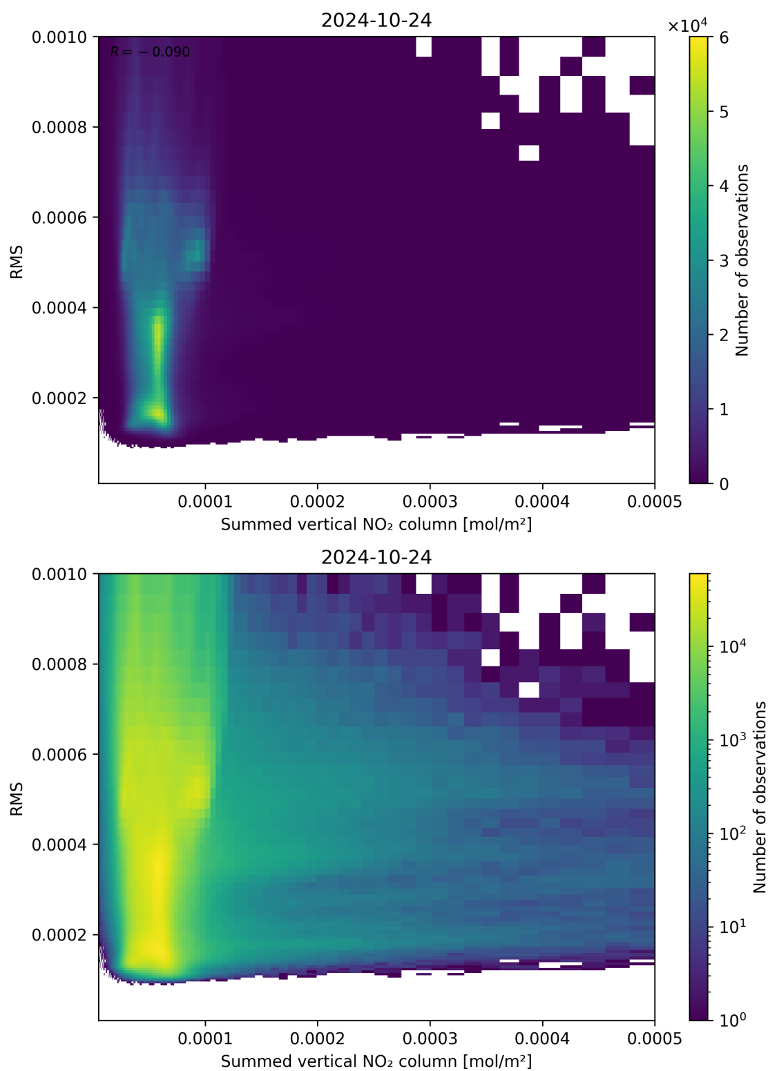
Figure 109: Scatter density plot of “Summed vertical NO 2 column” against “RMS” for 2024-10-24 to 2024-10-25.
