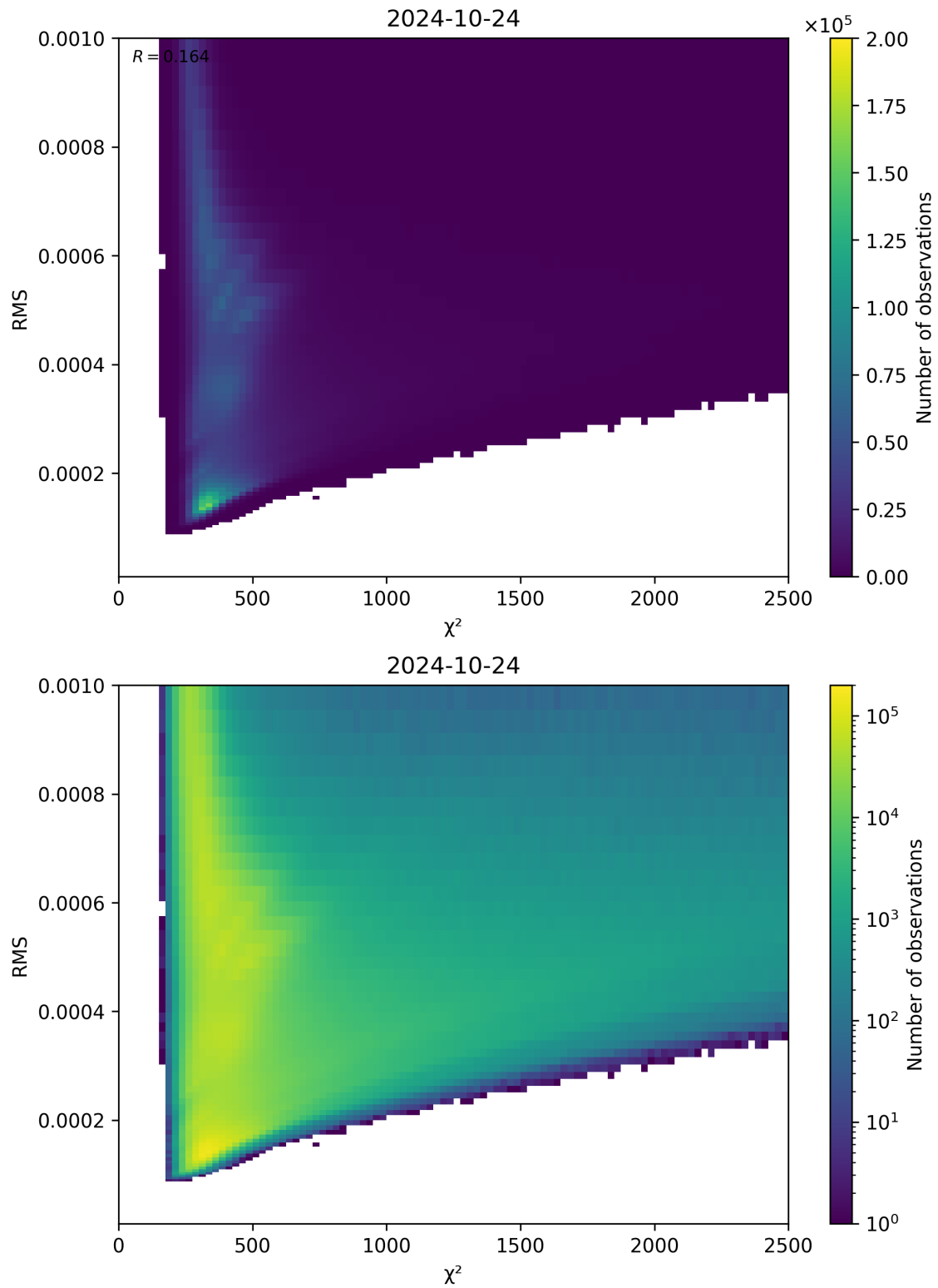
Figure 82: Scatter density plot of “ \chi^2 ” against “RMS” for 2024-10-24 to 2024-10-25.
