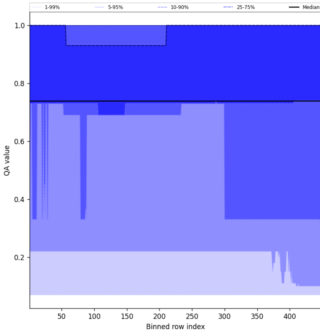
Figure 45: Along track statistics of “QA value” for 2024-10-24 to 2024-10-25
