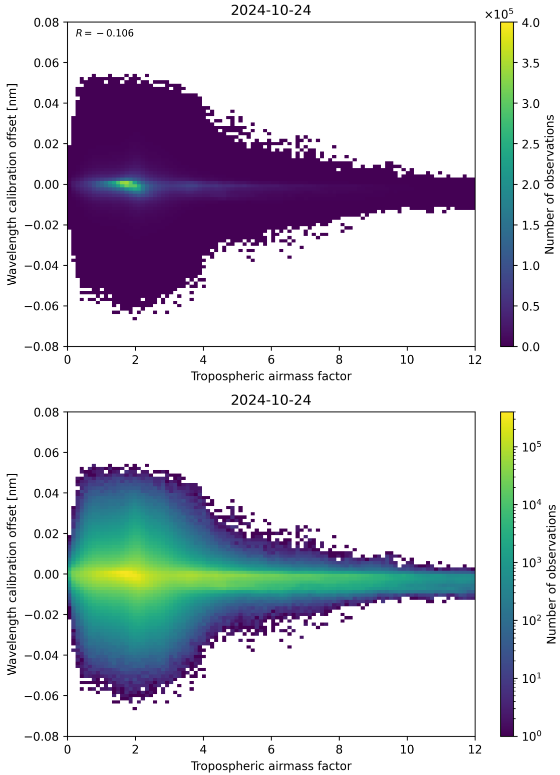
Figure 80: Scatter density plot of “Tropospheric airmass factor” against “Wavelength calibration offset” for 2024-10-24 to 2024-10-25.
