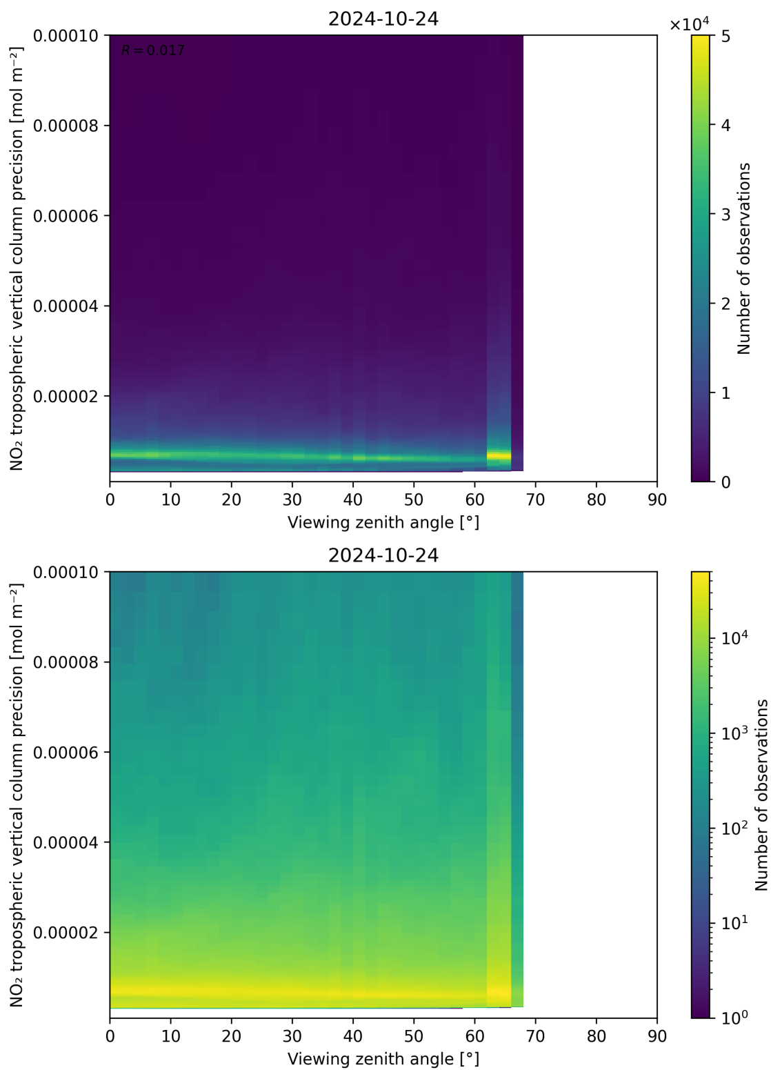
Figure 170: Scatter density plot of “Viewing zenith angle” against “NO 2 tropospheric vertical column precision” for 2024-10-24 to 2024-10-25.
