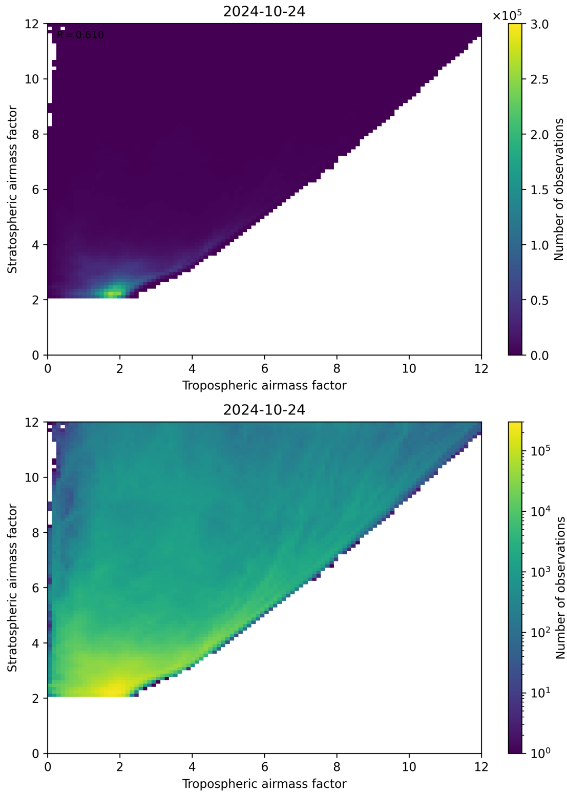
Figure 71: Scatter density plot of “Tropospheric airmass factor” against “Stratospheric airmass factor” for 2024-10-24 to 2024-10-25.
