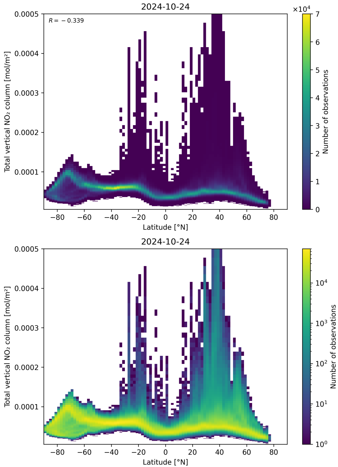
Figure 90: Scatter density plot of “Latitude” against “Total vertical NO 2 column” for 2024-10-24 to 2024-10-25.
