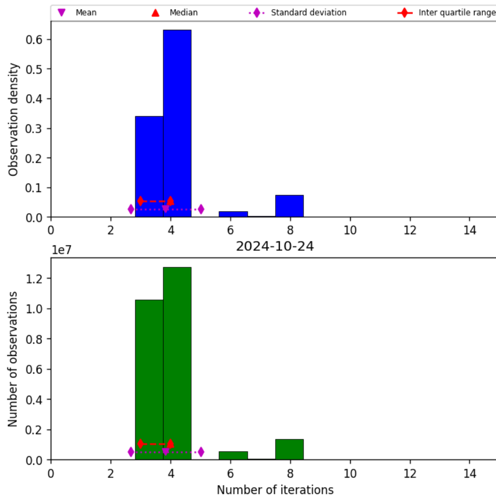
Figure 34: Histogram of “Number of iterations” for 2024-10-24 to 2024-10-25
