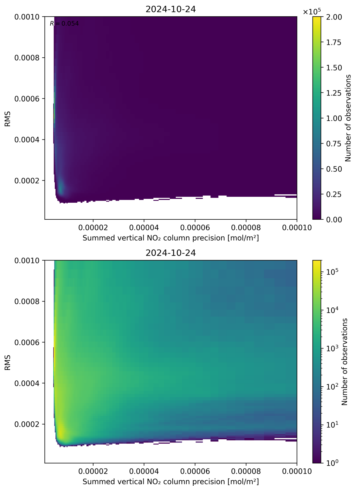
Figure 108: Scatter density plot of “Summed vertical NO 2 column precision” against “RMS” for 2024-10-24 to 2024-10-25.
