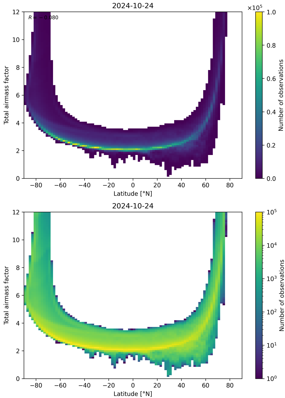
Figure 84: Scatter density plot of “Latitude” against “Total airmass factor” for 2024-10-24 to 2024-10-25.
