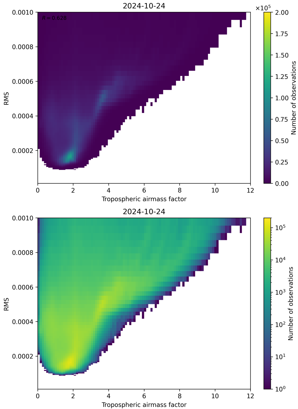
Figure 79: Scatter density plot of “Tropospheric airmass factor” against “RMS” for 2024-10-24 to 2024-10-25.
