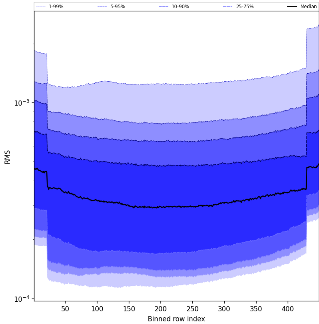
Figure 60: Along track statistics of “RMS” for 2024-10-24 to 2024-10-25
