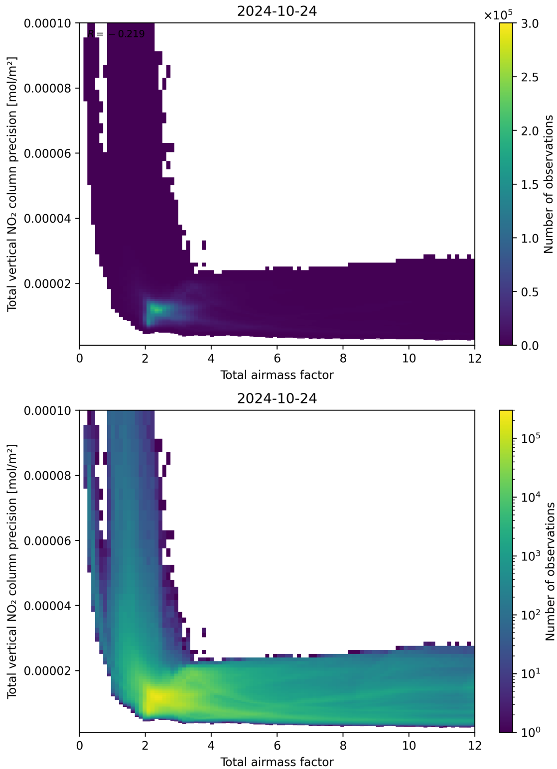
Figure 68: Scatter density plot of “Total airmass factor” against “Total vertical NO 2 column precision” for 2024-10-24 to 2024-10-25.
