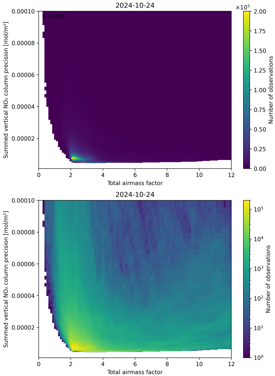
Figure 66: Scatter density plot of “Total airmass factor” against “Summed vertical NO 2 column precision” for 2024-10-24 to 2024-10-25.
