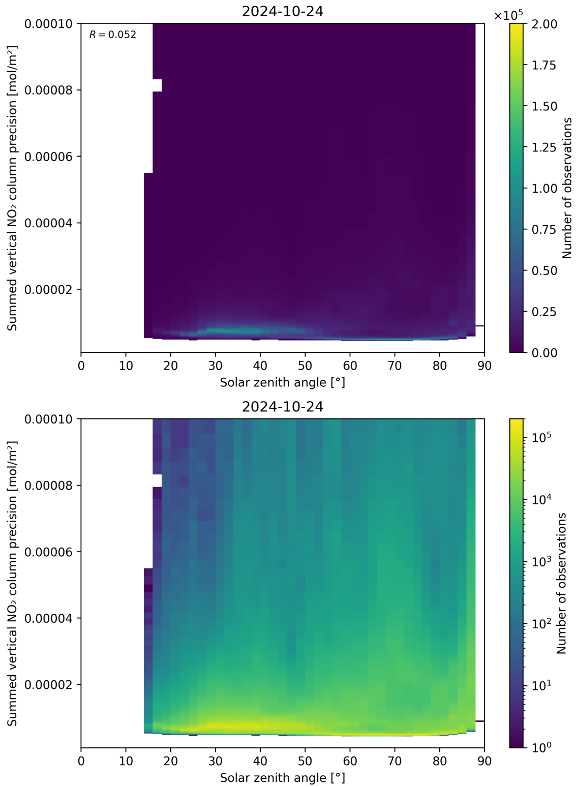
Figure 152: Scatter density plot of “Solar zenith angle” against “Summed vertical NO 2 column precision” for 2024-10-24 to 2024-10-25.
