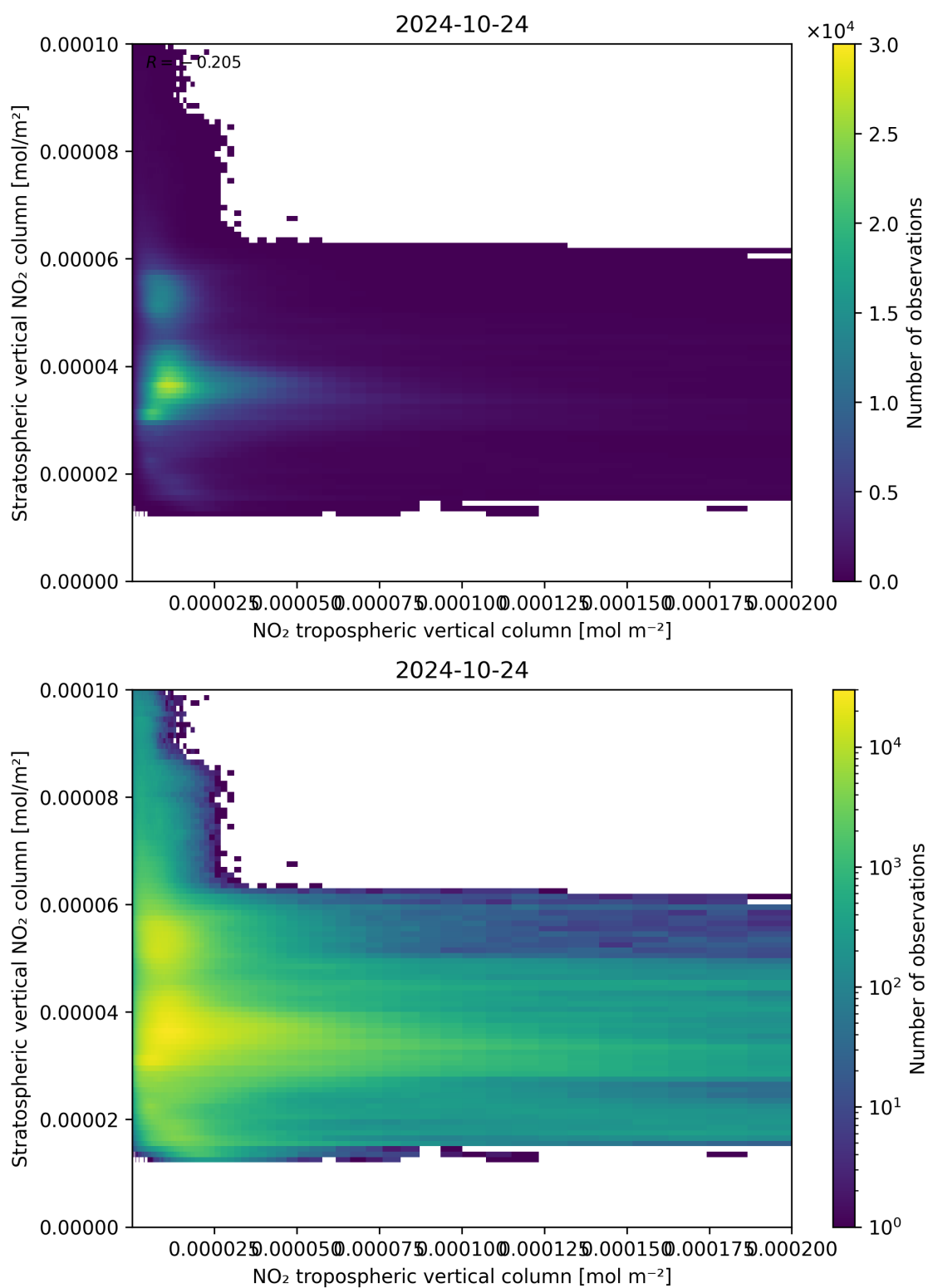
Figure 125: Scatter density plot of “NO 2 tropospheric vertical column” against “Stratospheric vertical NO 2 column” for 2024-10-24 to 2024-10-25.
