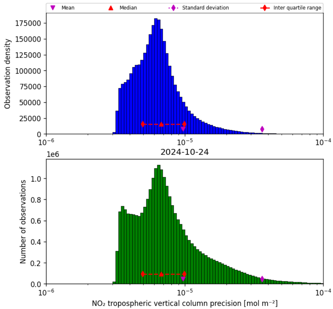
Figure 30: Histogram of “NO 2 tropospheric vertical column precision” for 2024-10-24 to 2024-10-25
