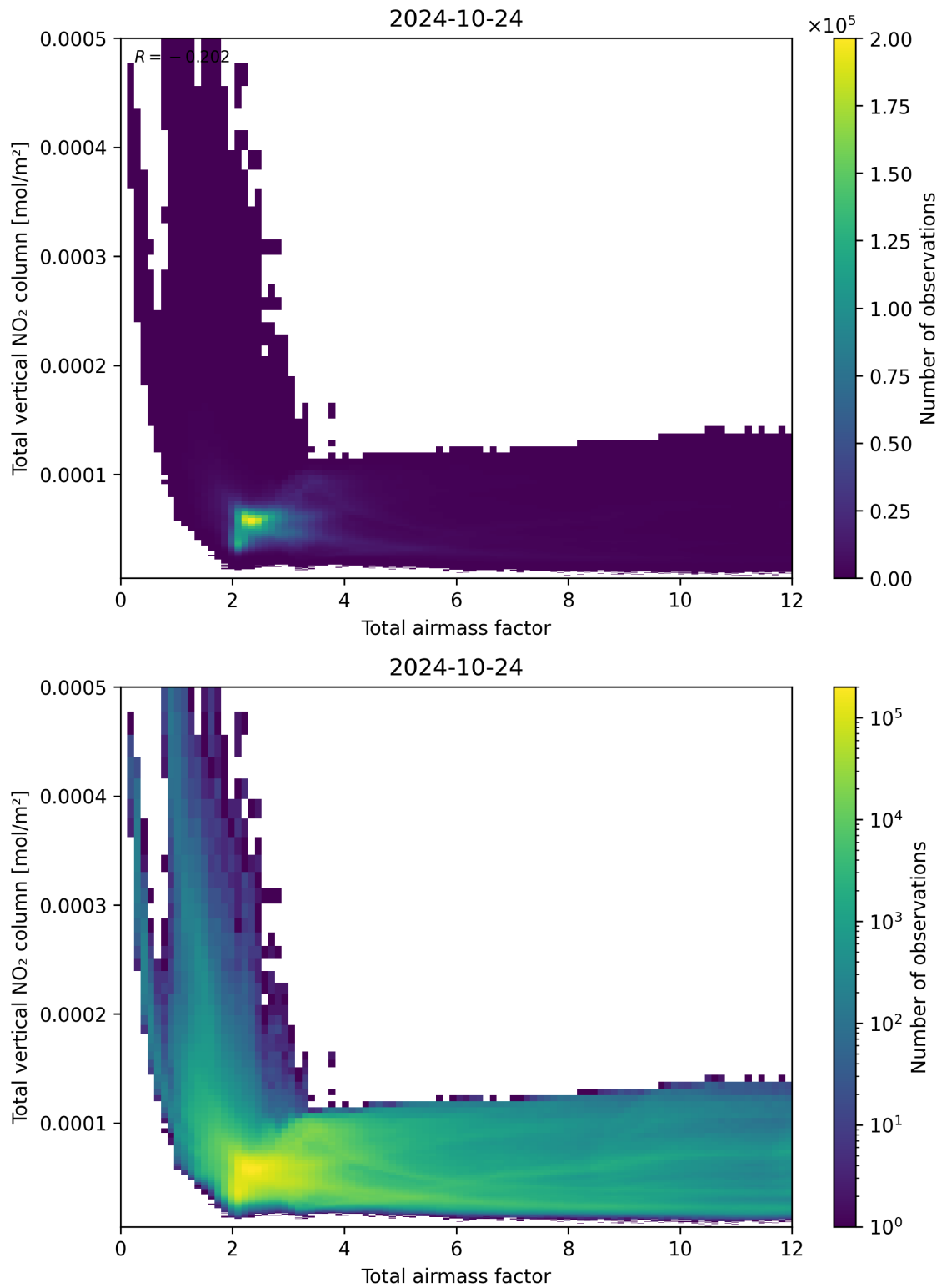
Figure 67: Scatter density plot of “Total air mass factor” against “Total vertical NO 2 column” for 2024-10-24 to 2024-10-25.
