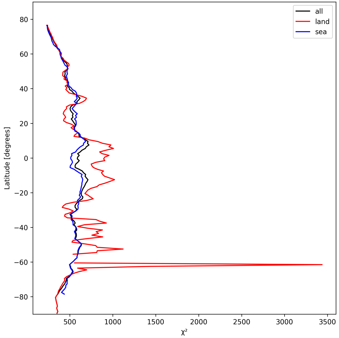
Figure 25: Zonal average of “ \chi^2 ” for 2024-10-24 to 2024-10-25.
