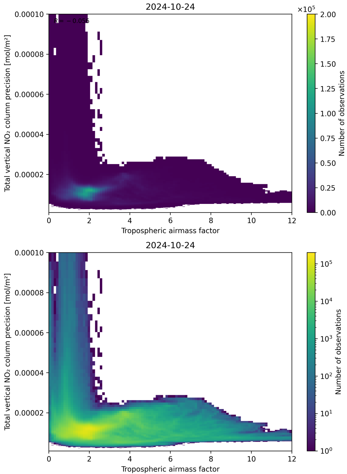
Figure 78: Scatter density plot of “Tropospheric air mass factor” against “Total vertical NO 2 column precision” for 2024-10-24 to 2024-10-25.
