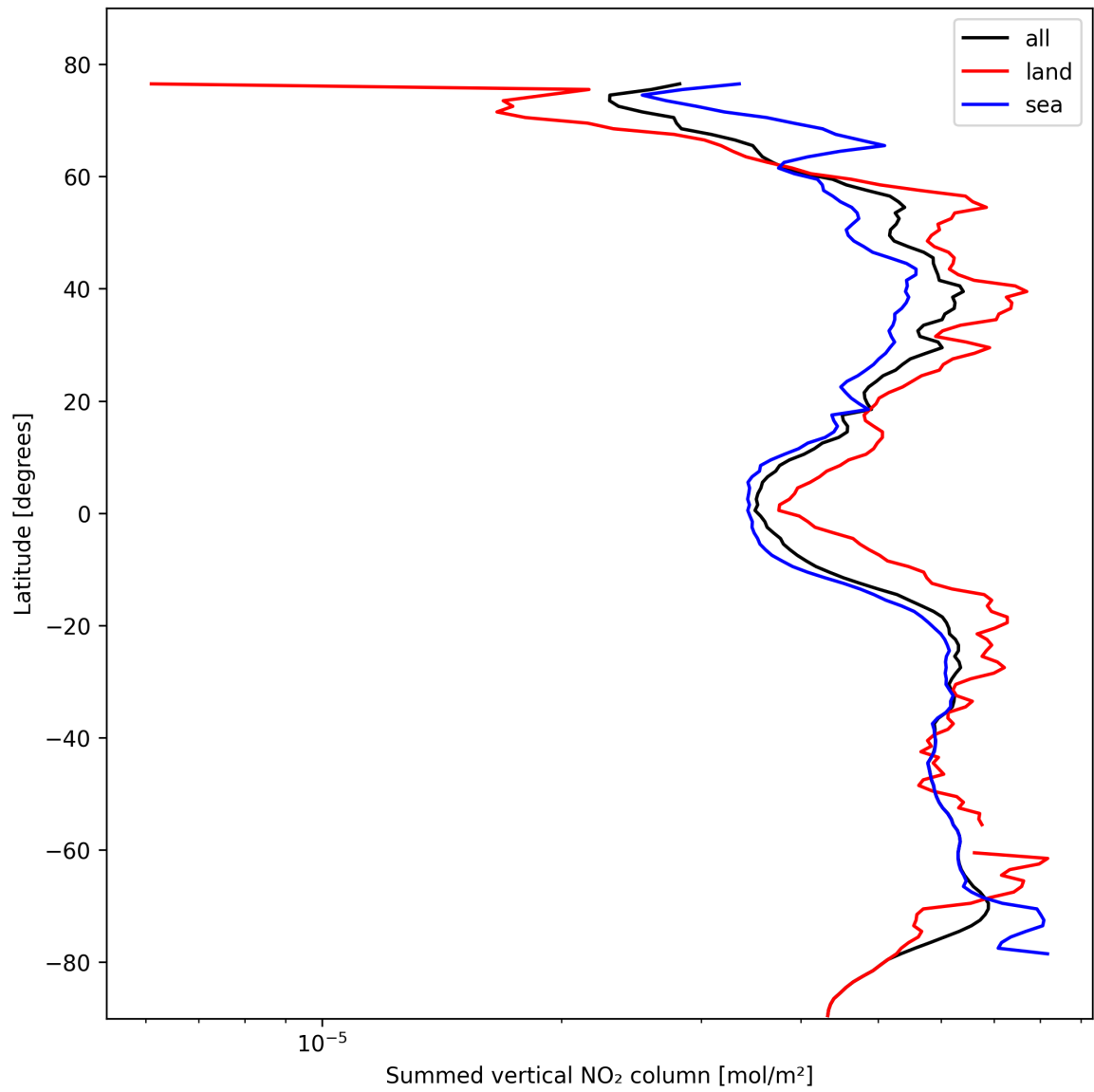
Figure 23: Zonal average of “Summed vertical NO 2 column” for 2024-10-24 to 2024-10-25.
