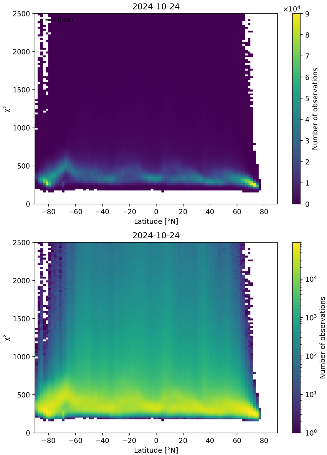
Figure 86: Scatter density plot of “Latitude” against “ \chi^2 ” for 2024-10-24 to 2024-10-25.
