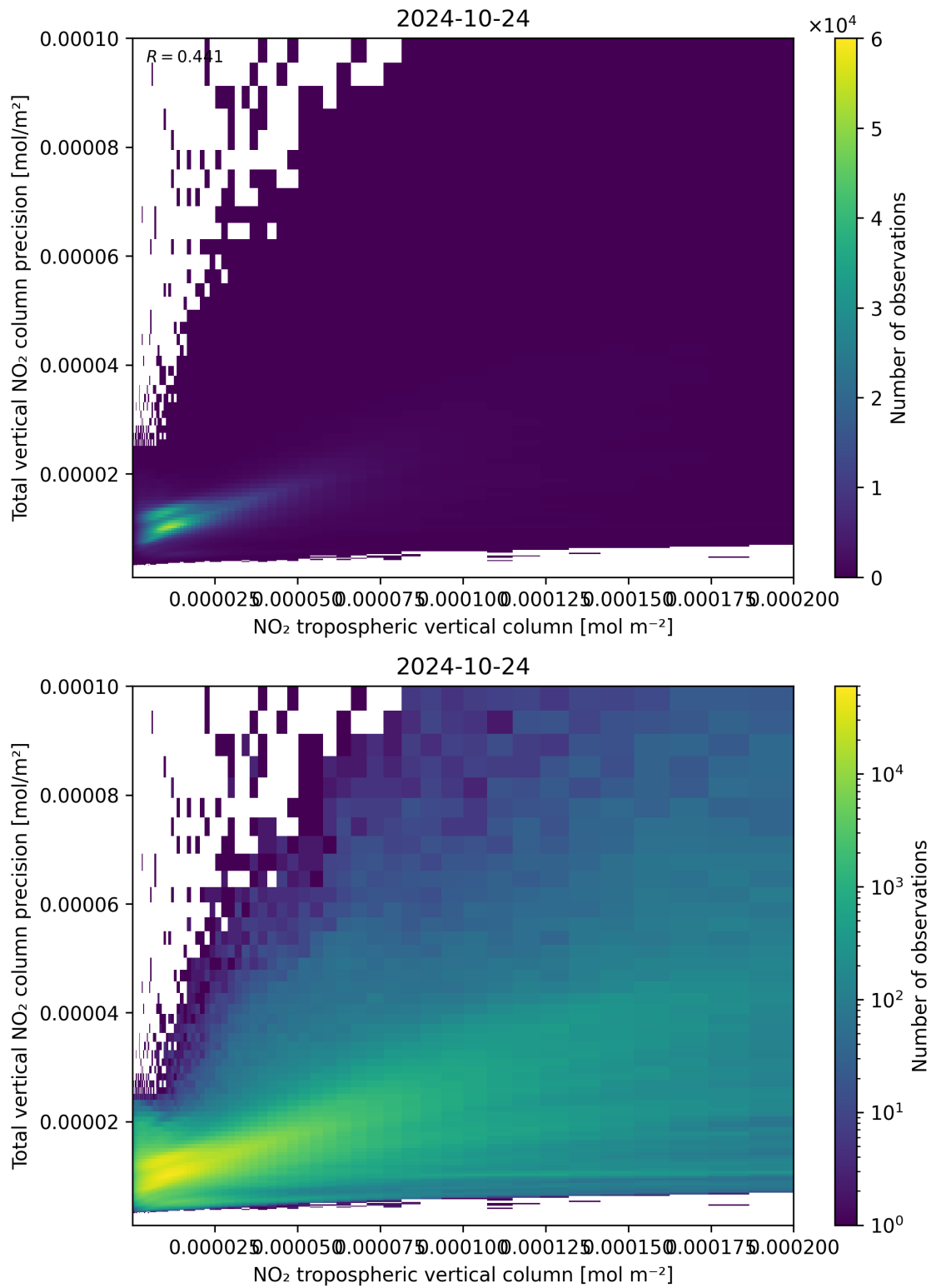
Figure 129: Scatter density plot of “NO 2 tropospheric vertical column” against “Total vertical NO 2 column precision” for 2024-10-24 to 2024-10-25.
