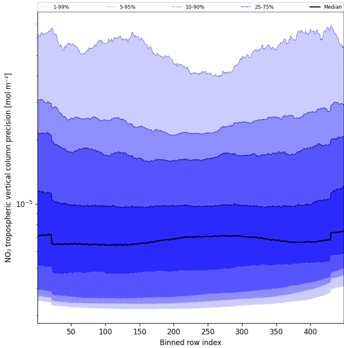
Figure 47: Along track statistics of “NO 2 tropospheric vertical column precision” for 2024-10-24 to 2024-10-25
