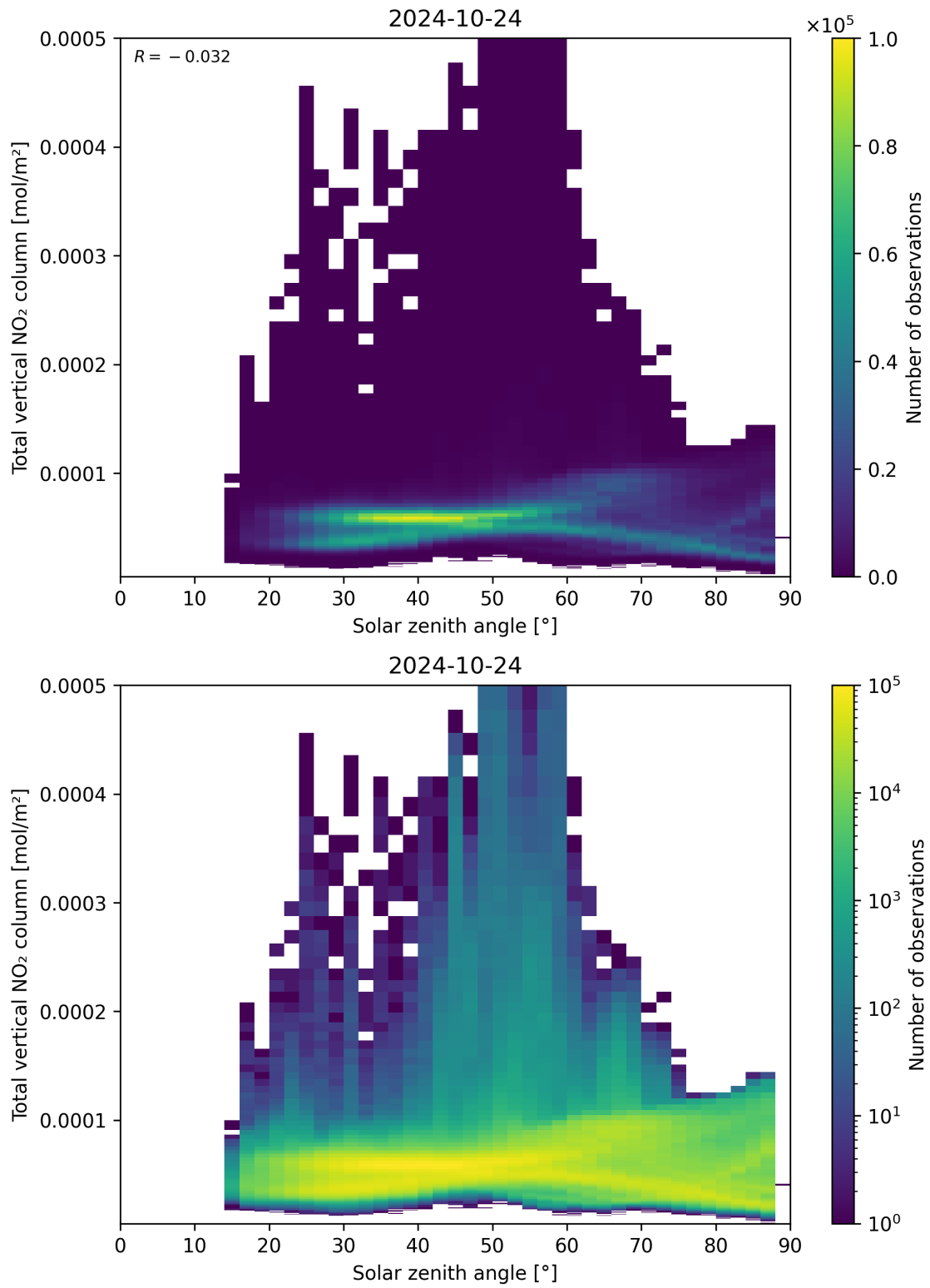
Figure 153: Scatter density plot of “Solar zenith angle” against “Total vertical NO 2 column” for 2024-10-24 to 2024-10-25.
