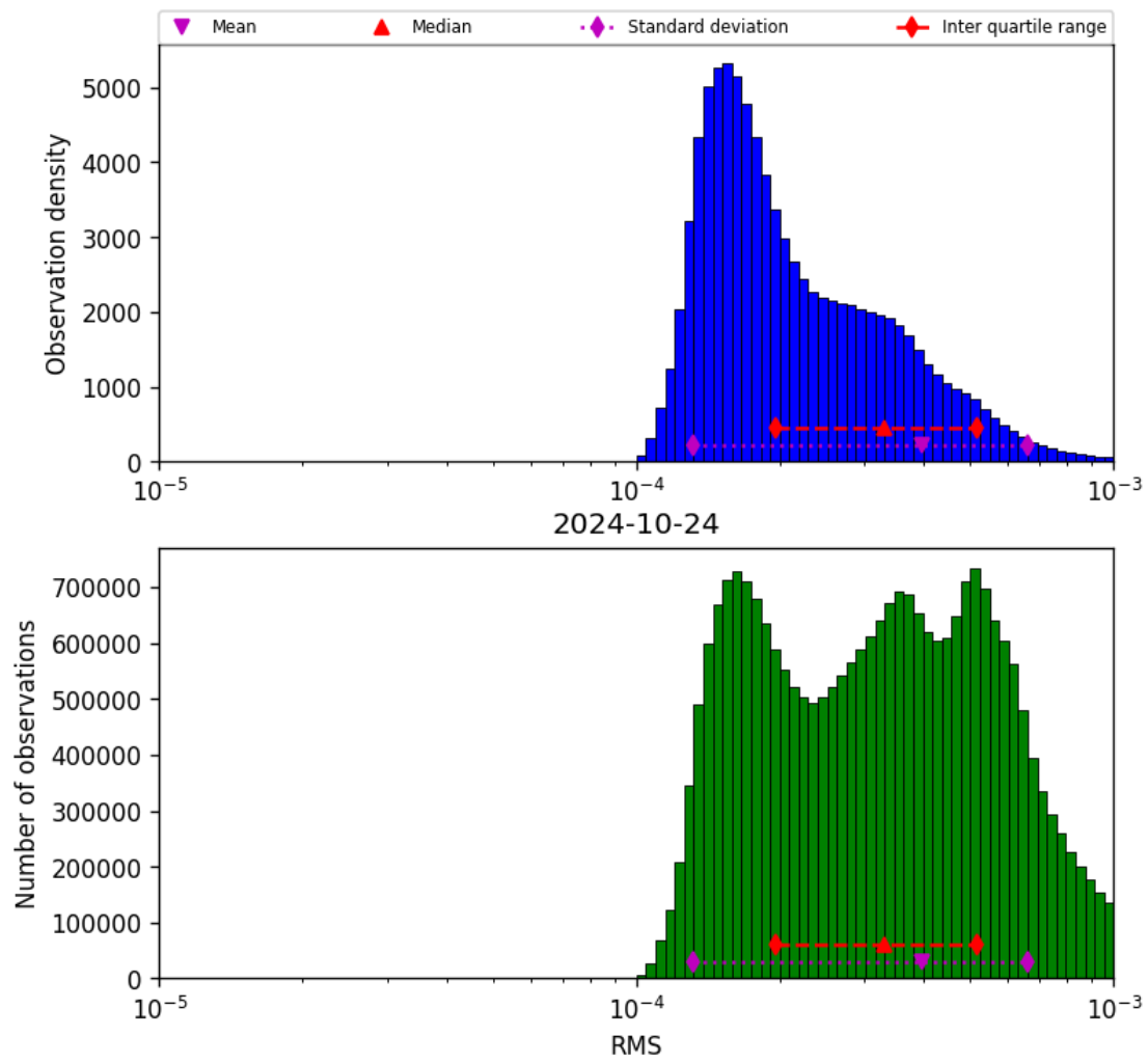
Figure 43: Histogram of “RMS” for 2024-10-24 to 2024-10-25
