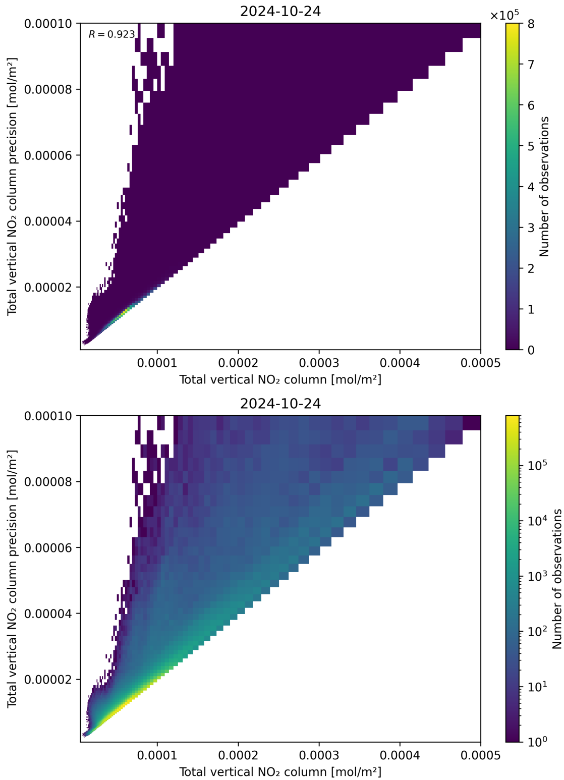
Figure 114: Scatter density plot of “Total vertical NO 2 column” against “Total vertical NO 2 column precision” for 2024-10-24 to 2024-10-25.
