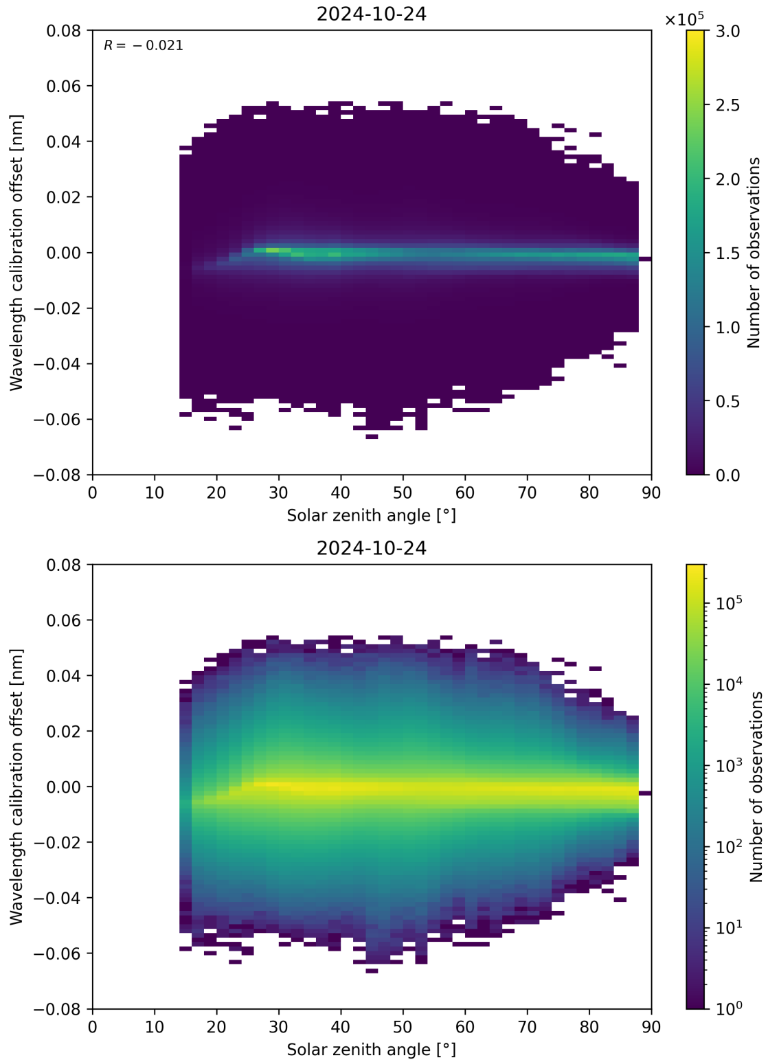
Figure 158: Scatter density plot of “Solar zenith angle” against “Wavelength calibration offset” for 2024-10-24 to 2024-10-25.
