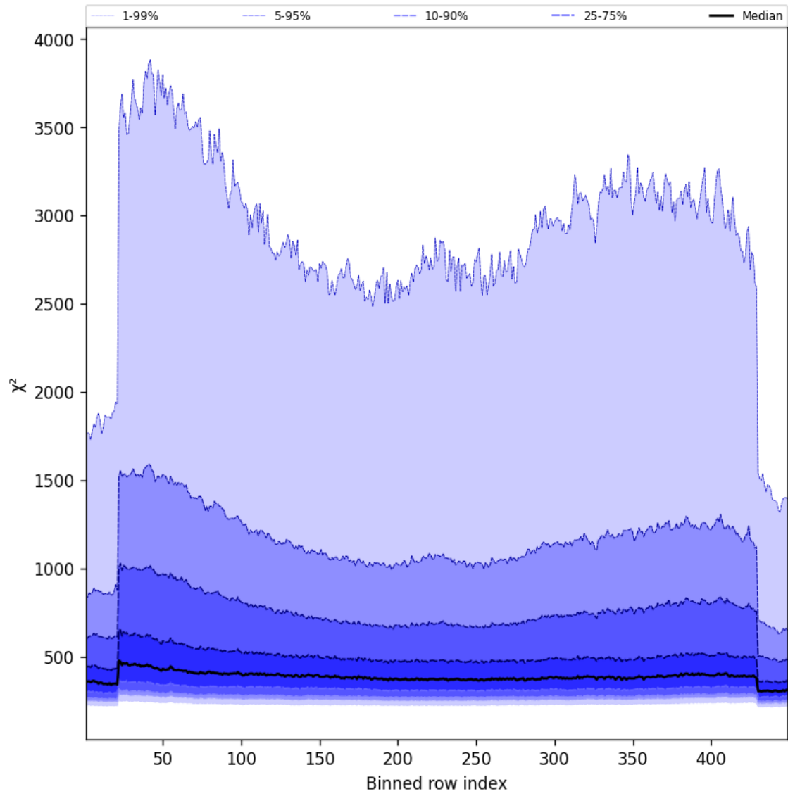
Figure 59: Along track statistics of “ \chi^2 ” for 2024-10-24 to 2024-10-25
