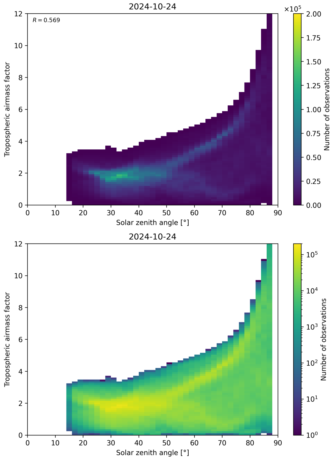
Figure 147: Scatter density plot of “Solar zenith angle” against “Tropospheric airmass factor” for 2024-10-24 to 2024-10-25.
