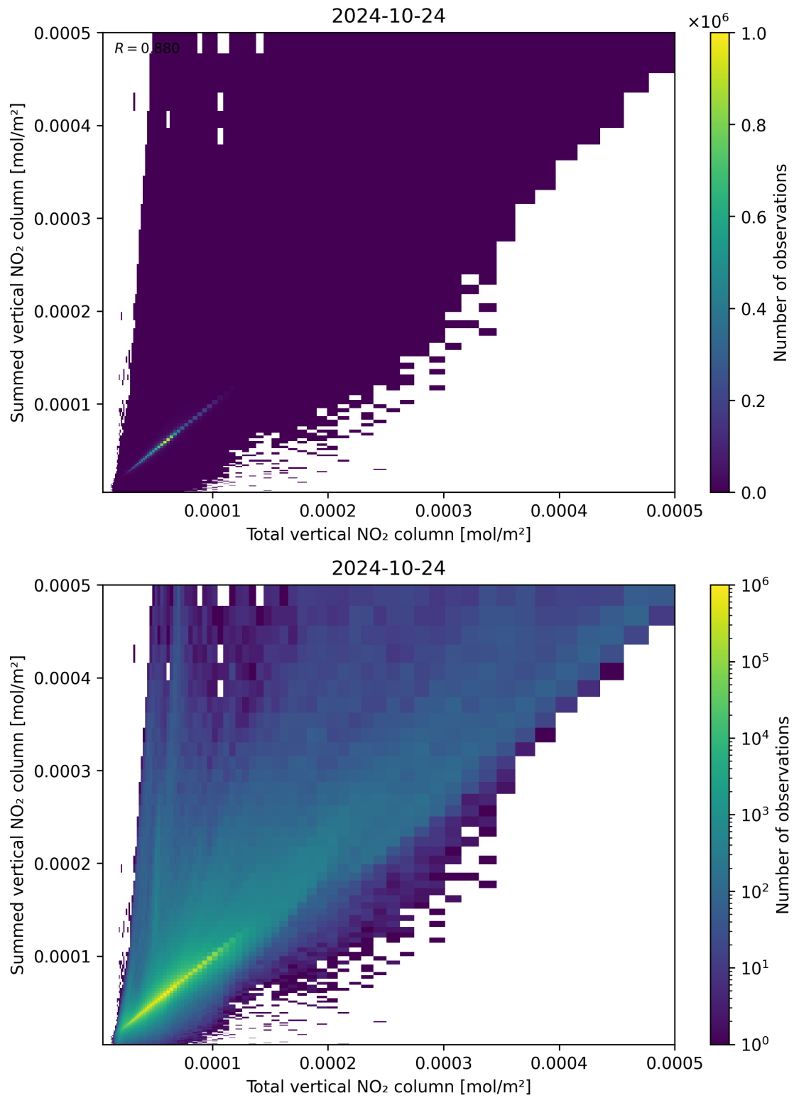
Figure 112: Scatter density plot of “Total vertical NO 2 column” against “Summed vertical NO 2 column” for 2024-10-24 to 2024-10-25.
