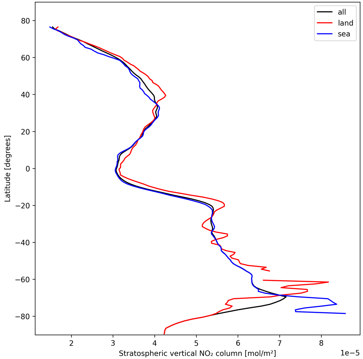
Figure 19: Zonal average of “Stratospheric vertical NO 2 column” for 2024-10-24 to 2024-10-25.
