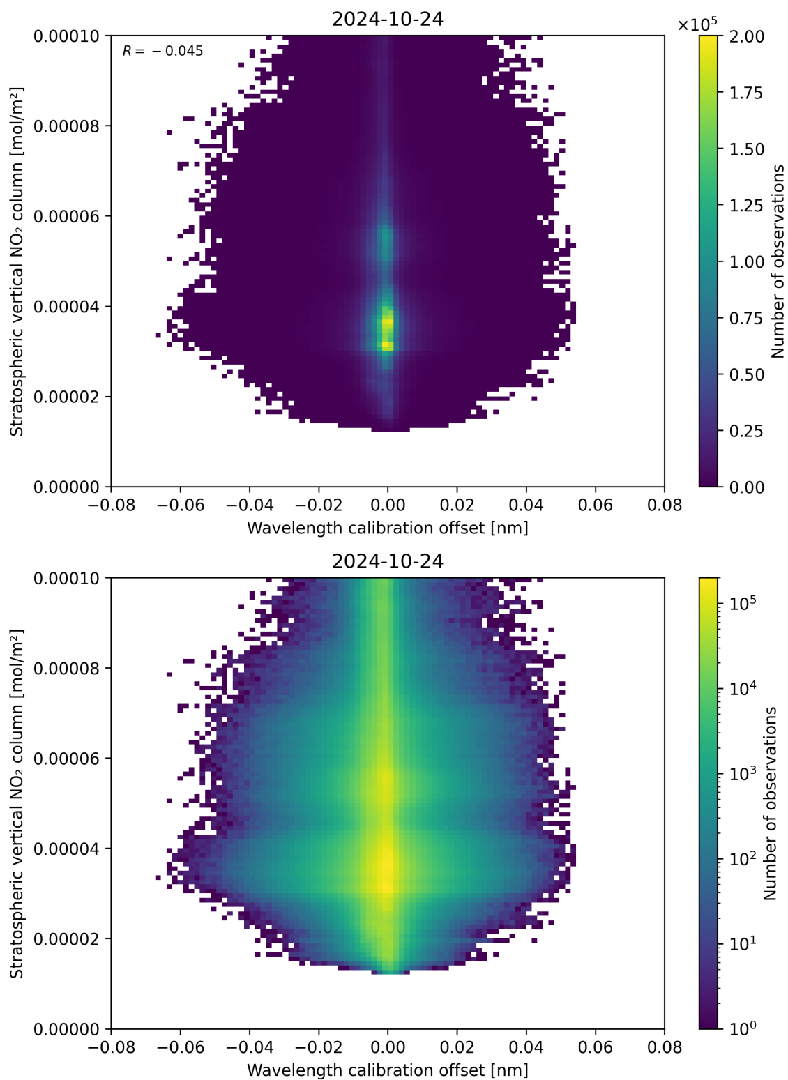
Figure 176: Scatter density plot of “Wavelength calibration offset” against “Stratospheric vertical NO 2 column” for 2024-10-24 to 2024-10-25.
