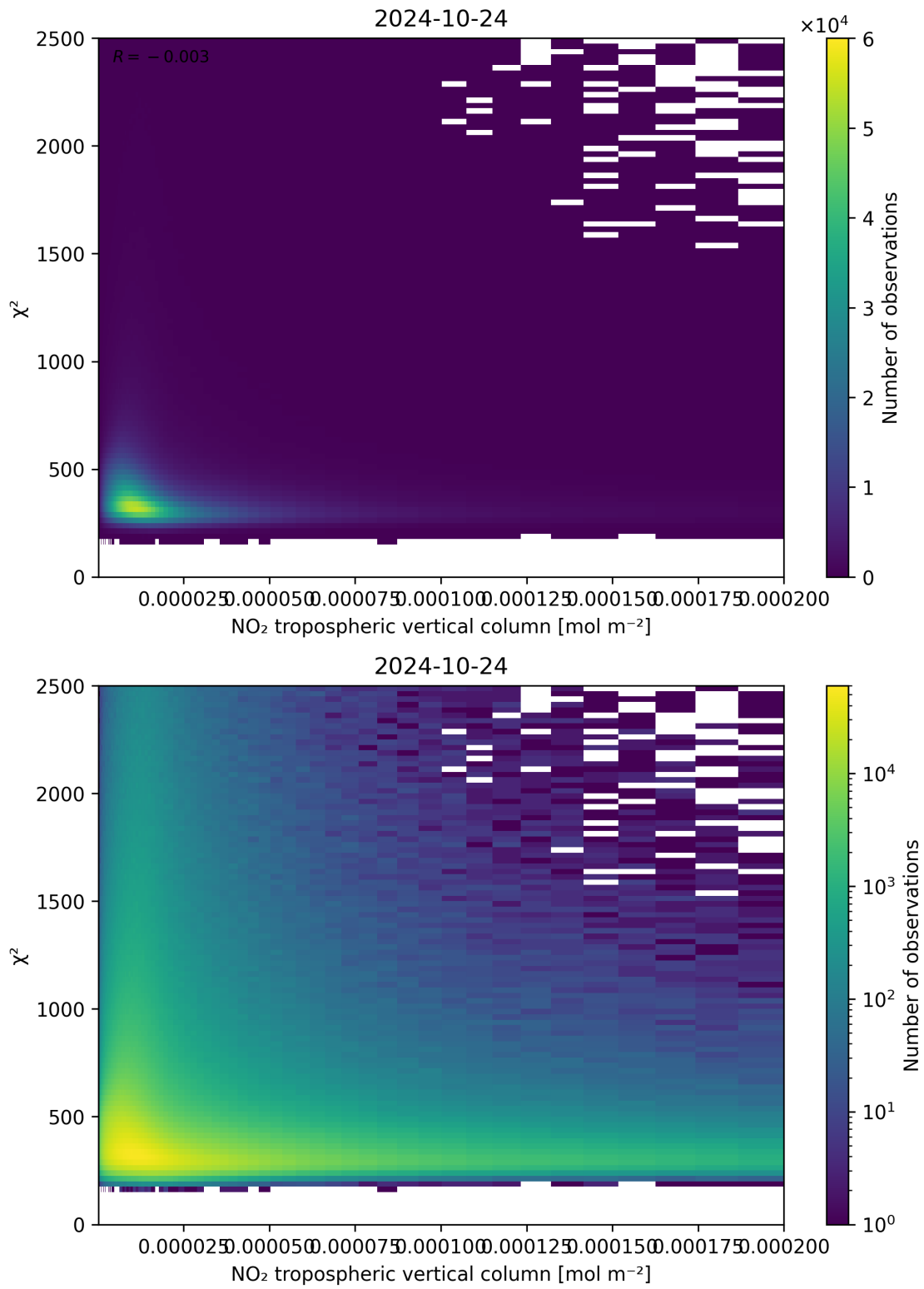
Figure 124: Scatter density plot of “NO 2 tropospheric vertical column” against “ \chi^2 ” for 2024-10-24 to 2024-10-25.
