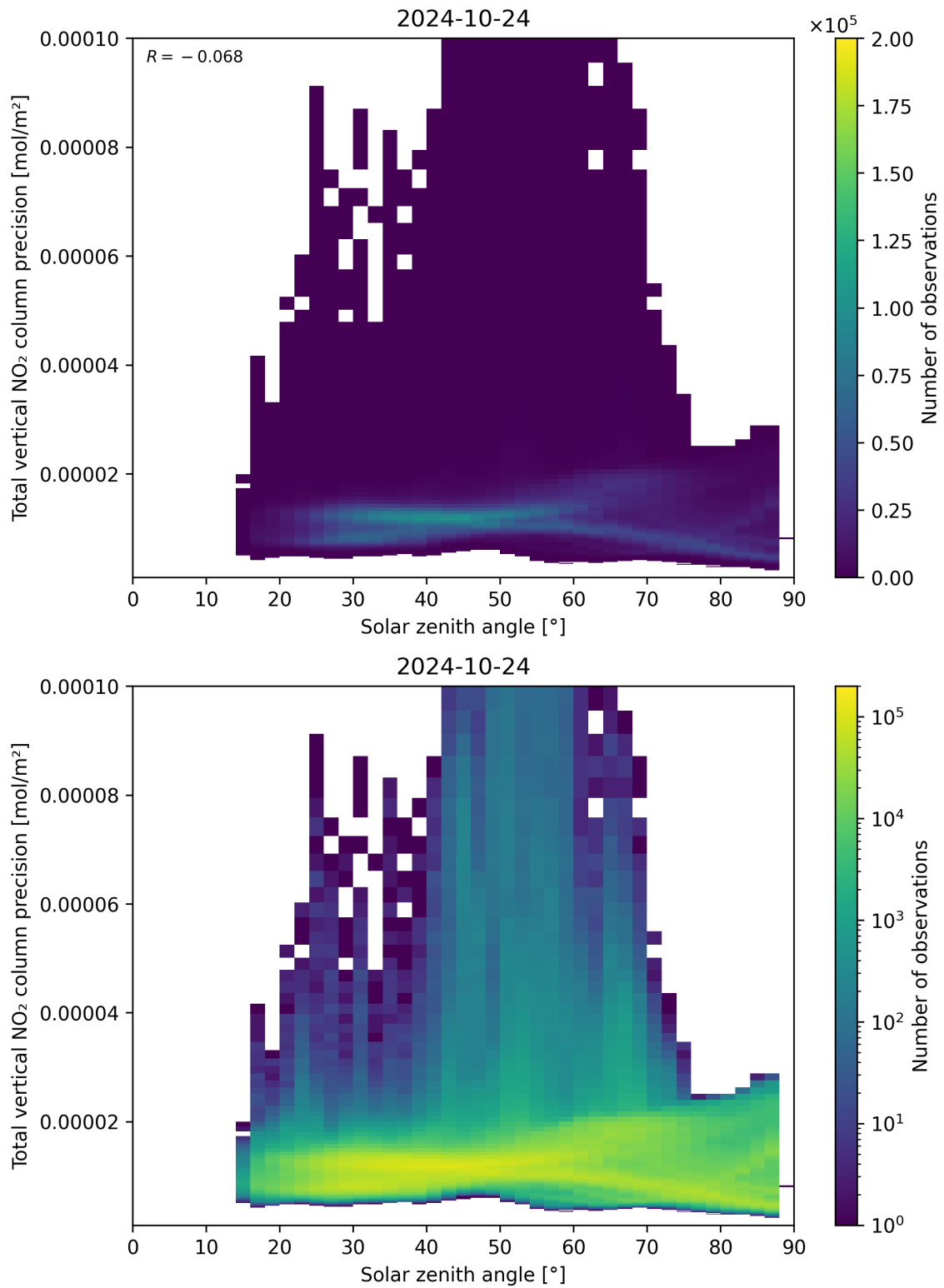
Figure 154: Scatter density plot of “Solar zenith angle” against “Total vertical NO 2 column precision” for 2024-10-24 to 2024-10-25.
