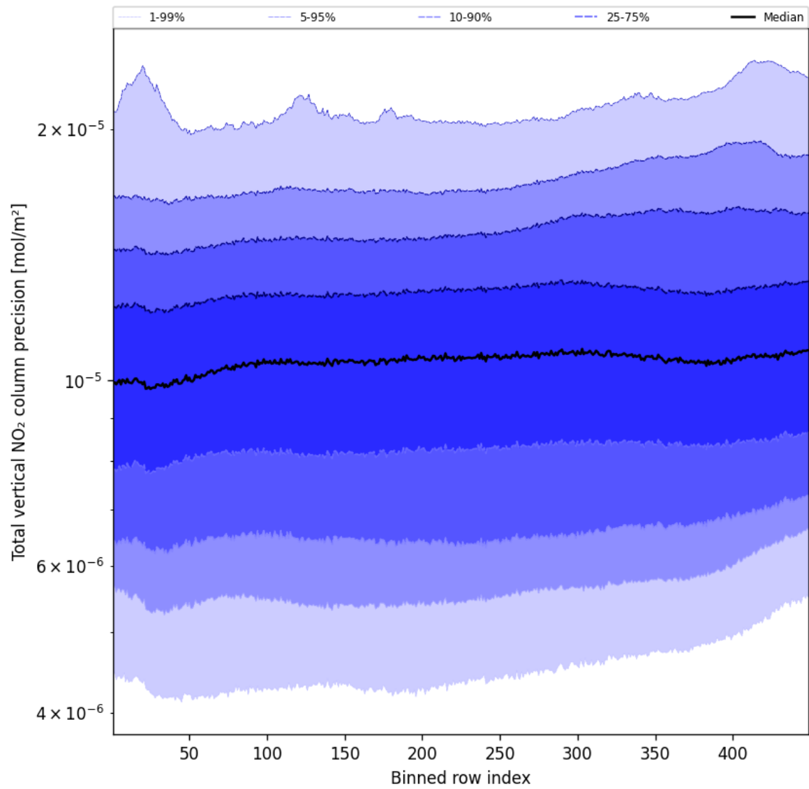
Figure 56: Along track statistics of “Total vertical NO 2 column precision” for 2024-10-24 to 2024-10-25
