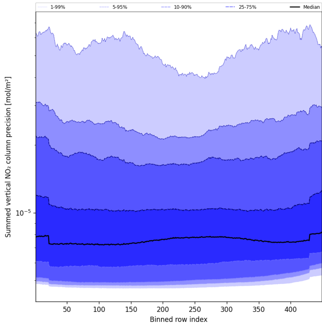
Figure 58: Along track statistics of “Summed vertical NO 2 column precision” for 2024-10-24 to 2024-10-25
