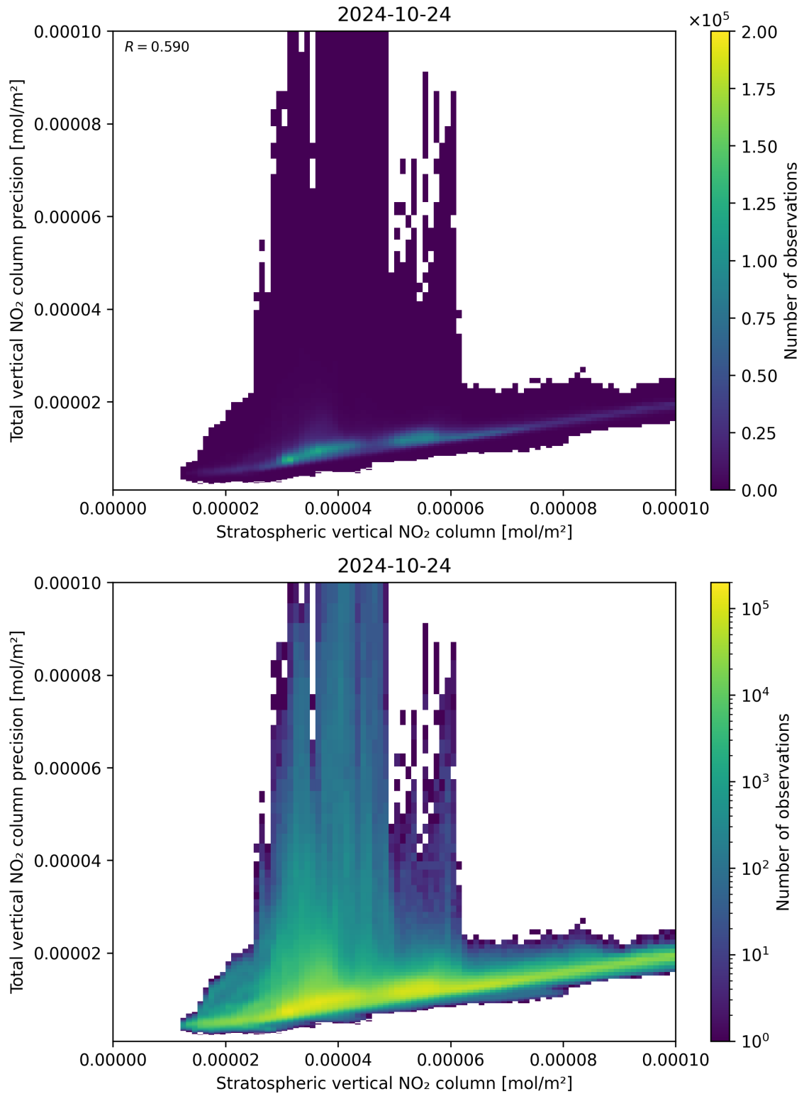
Figure 101: Scatter density plot of “Stratospheric vertical NO 2 column” against “Total vertical NO 2 column precision” for 2024-10-24 to 2024-10-25.
