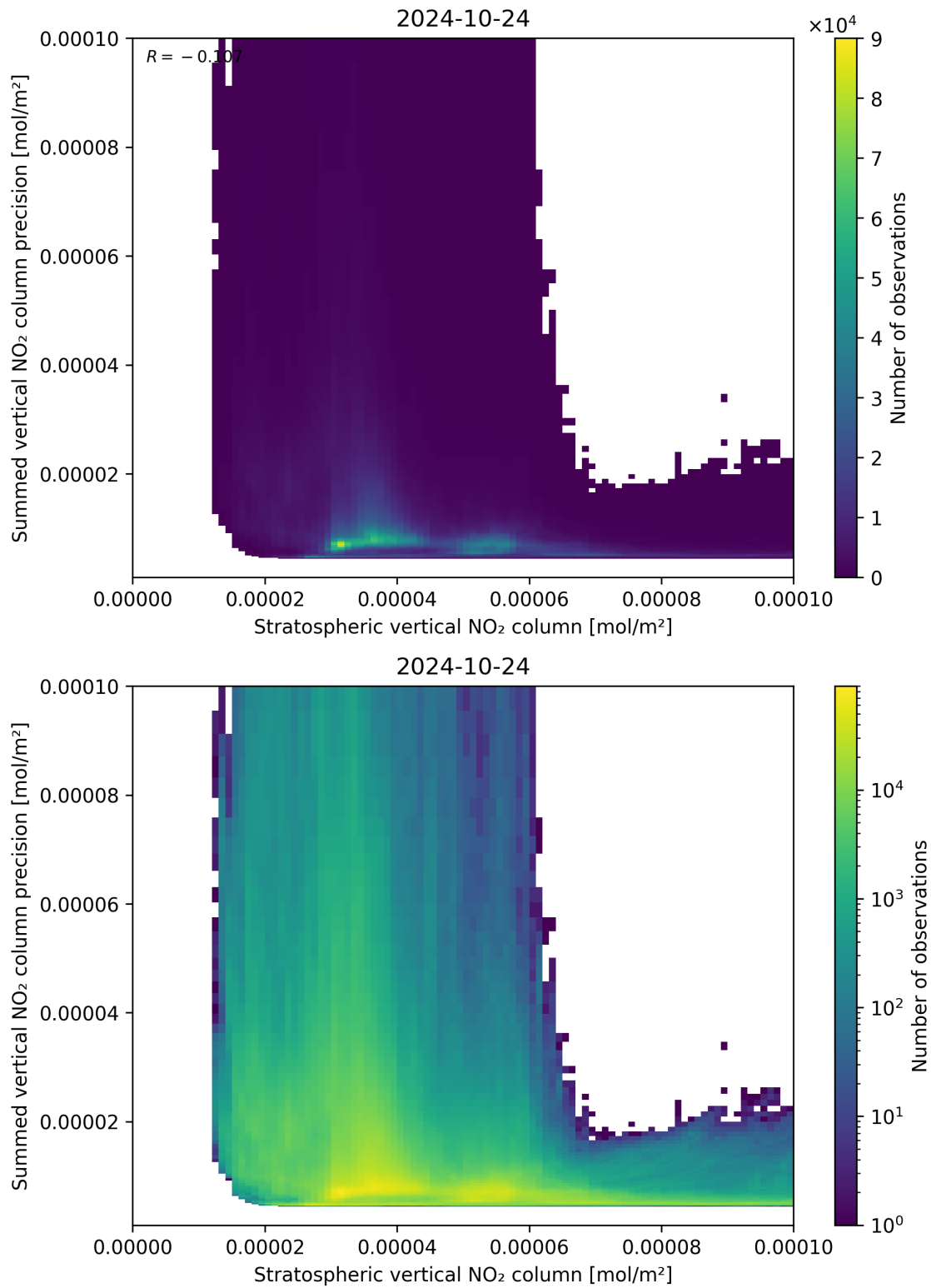
Figure 99: Scatter density plot of “Stratospheric vertical NO 2 column” against “Summed vertical NO 2 column precision” for 2024-10-24 to 2024-10-25.
