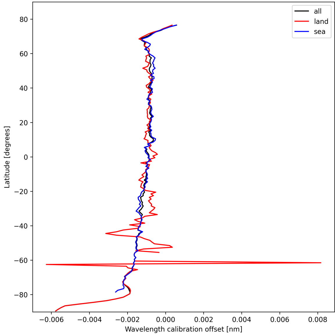
Figure 18: Zonal average of “Wavelength calibration offset” for 2024-10-24 to 2024-10-25.
