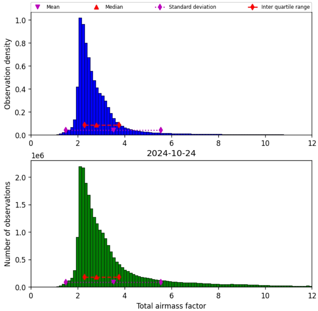
Figure 32: Histogram of “Total airmass factor” for 2024-10-24 to 2024-10-25
