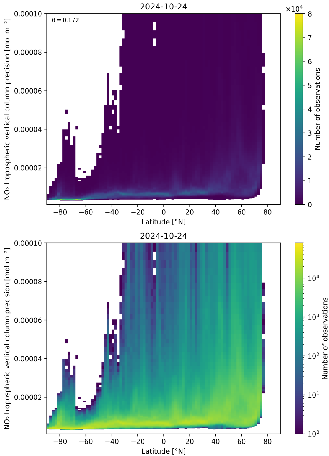
Figure 93: Scatter density plot of “Latitude” against “NO 2 tropospheric vertical column precision” for 2024-10-24 to 2024-10-25.
