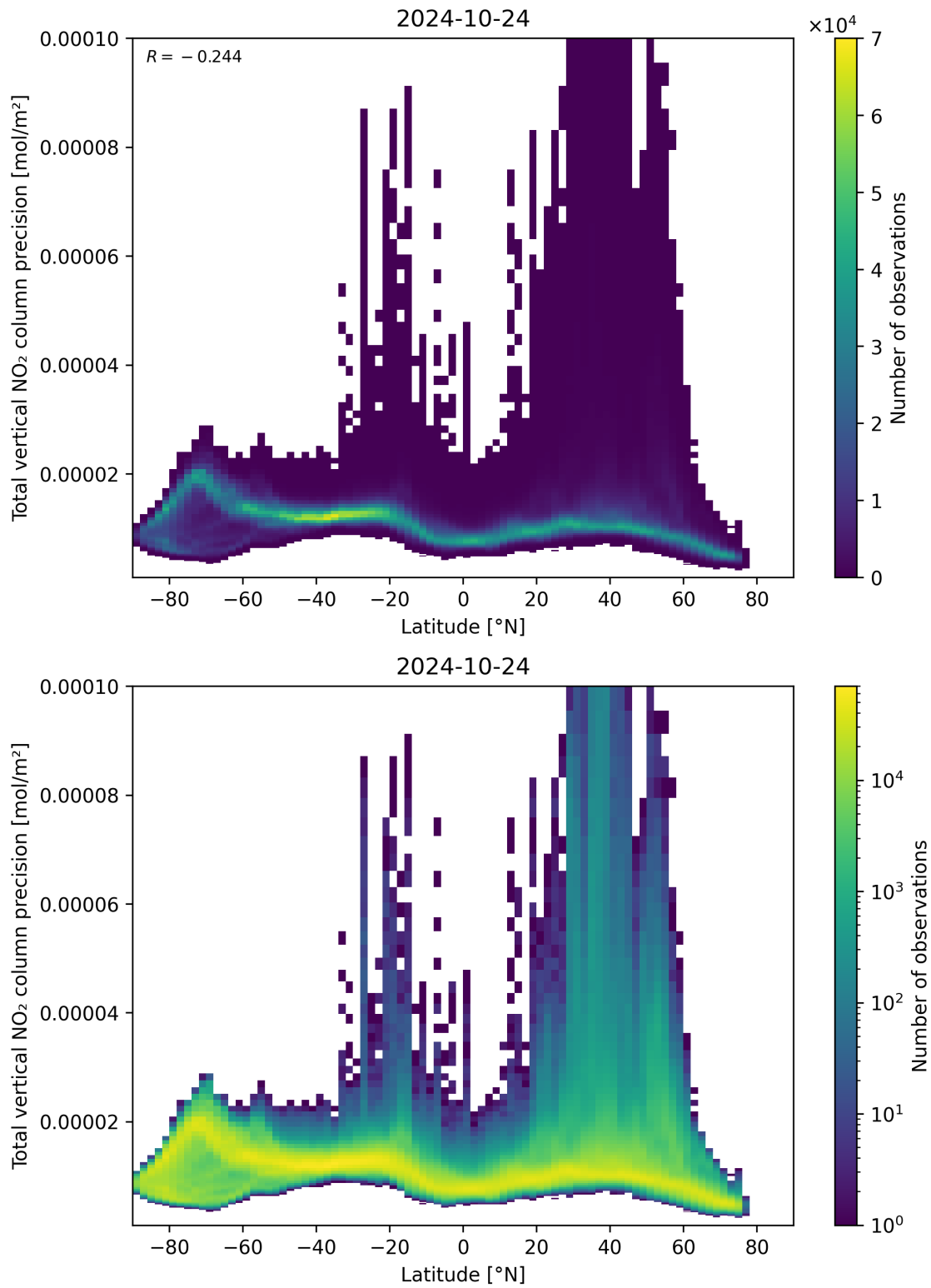
Figure 91: Scatter density plot of “Latitude” against “Total vertical NO 2 column precision” for 2024-10-24 to 2024-10-25.
