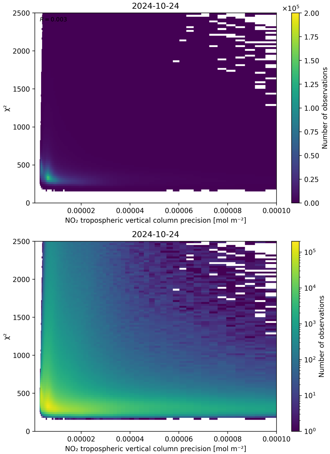
Figure 134: Scatter density plot of “NO 2 tropospheric vertical column precision” against “ \chi^2 ” for 2024-10-24 to 2024-10-25.
