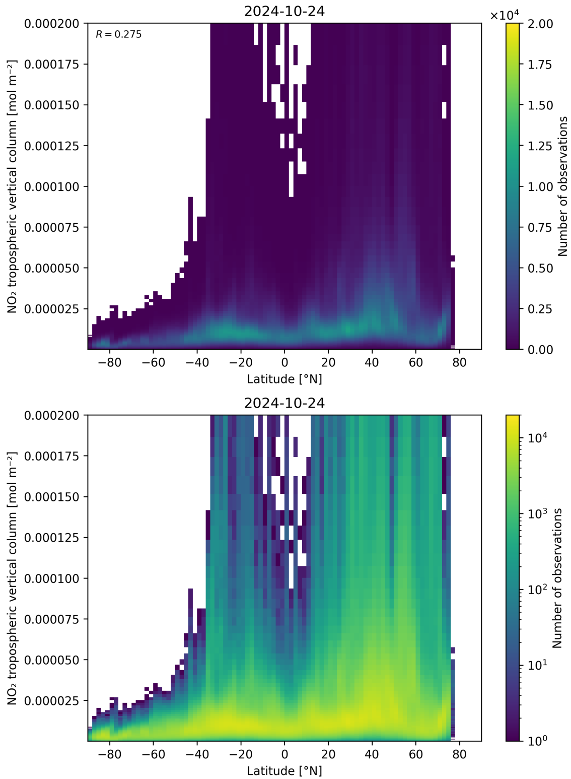
Figure 92: Scatter density plot of “Latitude” against “NO 2 tropospheric vertical column” for 2024-10-24 to 2024-10-25.
