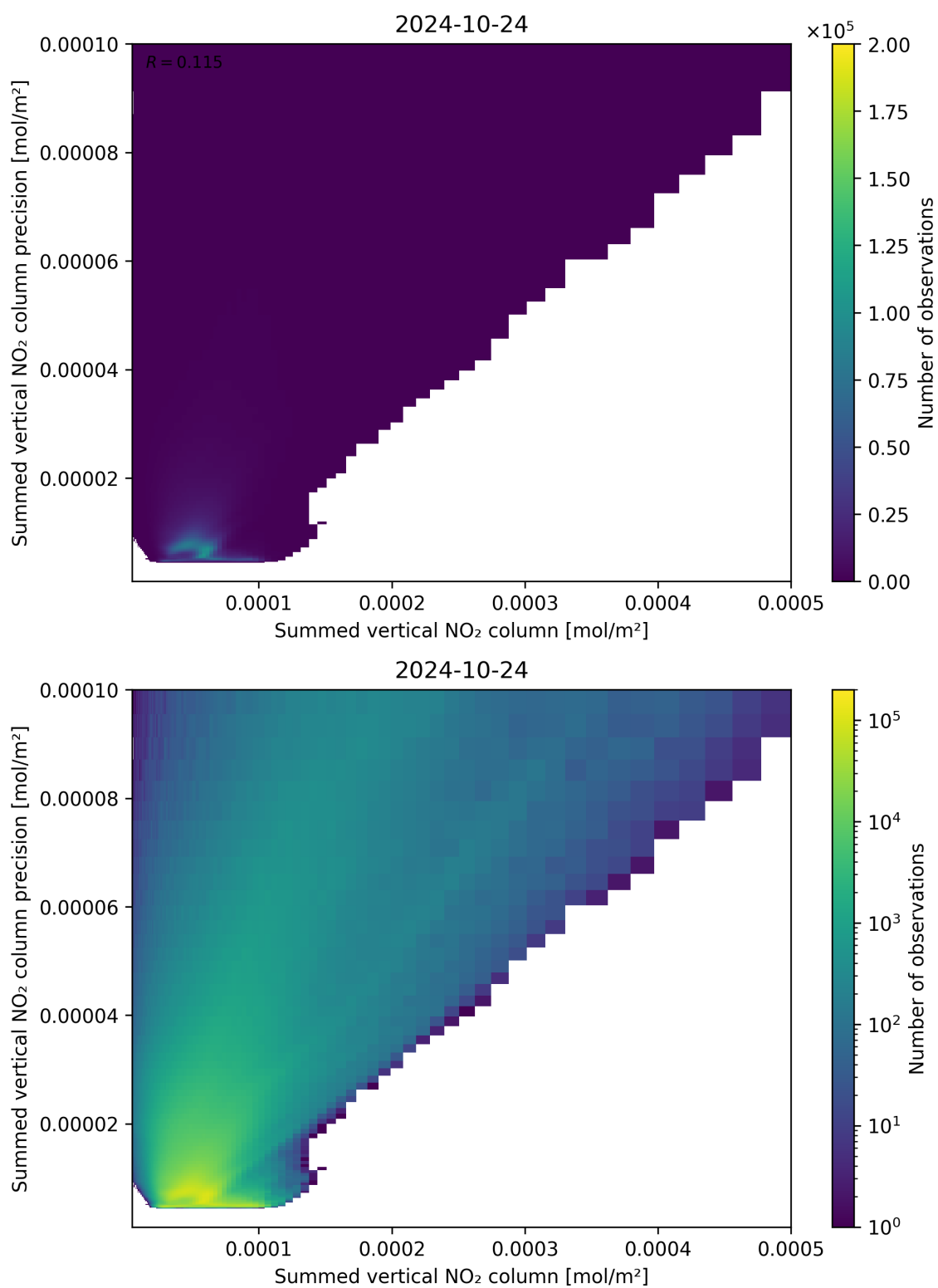
Figure 105: Scatter density plot of “Summed vertical NO 2 column” against “Summed vertical NO 2 column precision” for 2024-10-24 to 2024-10-25.
