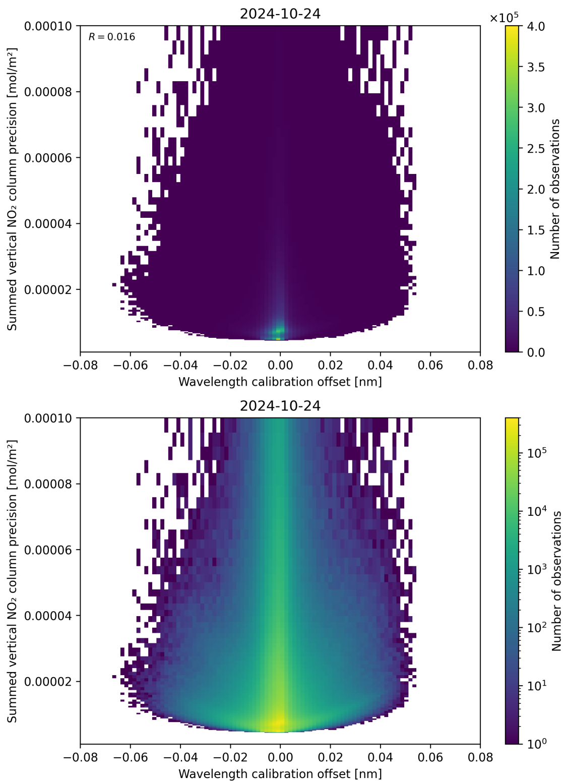
Figure 178: Scatter density plot of “Wavelength calibration offset” against “Summed vertical NO 2 column precision” for 2024-10-24 to 2024-10-25.
