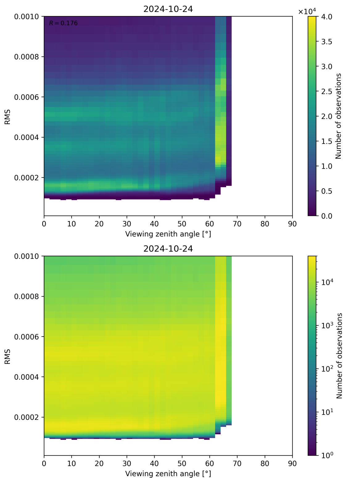
Figure 171: Scatter density plot of “Viewing zenith angle” against “RMS” for 2024-10-24 to 2024-10-25.
