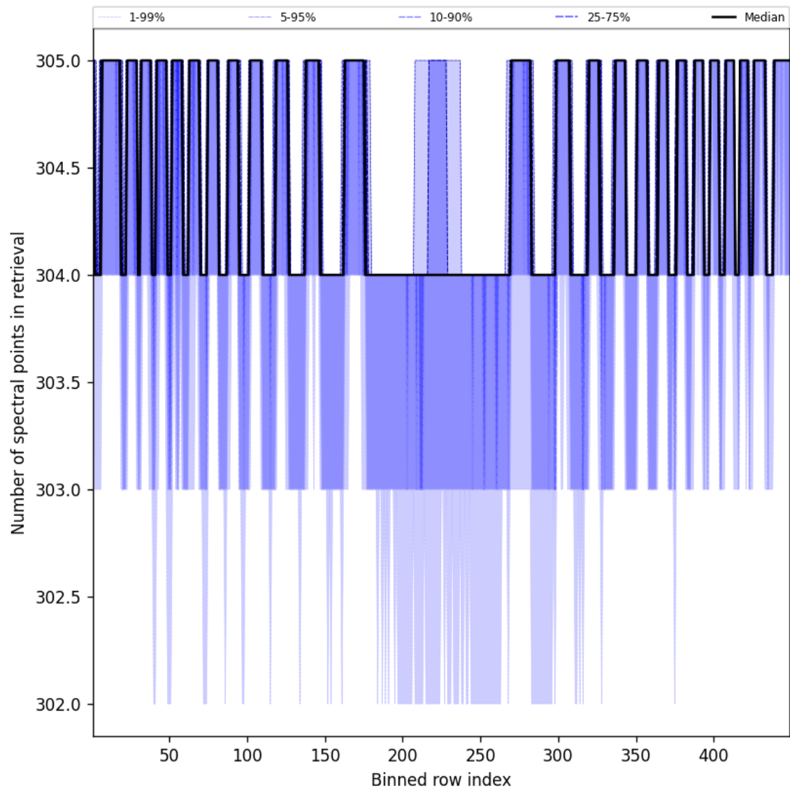
Figure 50: Along track statistics of “Number of spectral points in retrieval” for 2024-10-24 to 2024-10-25
