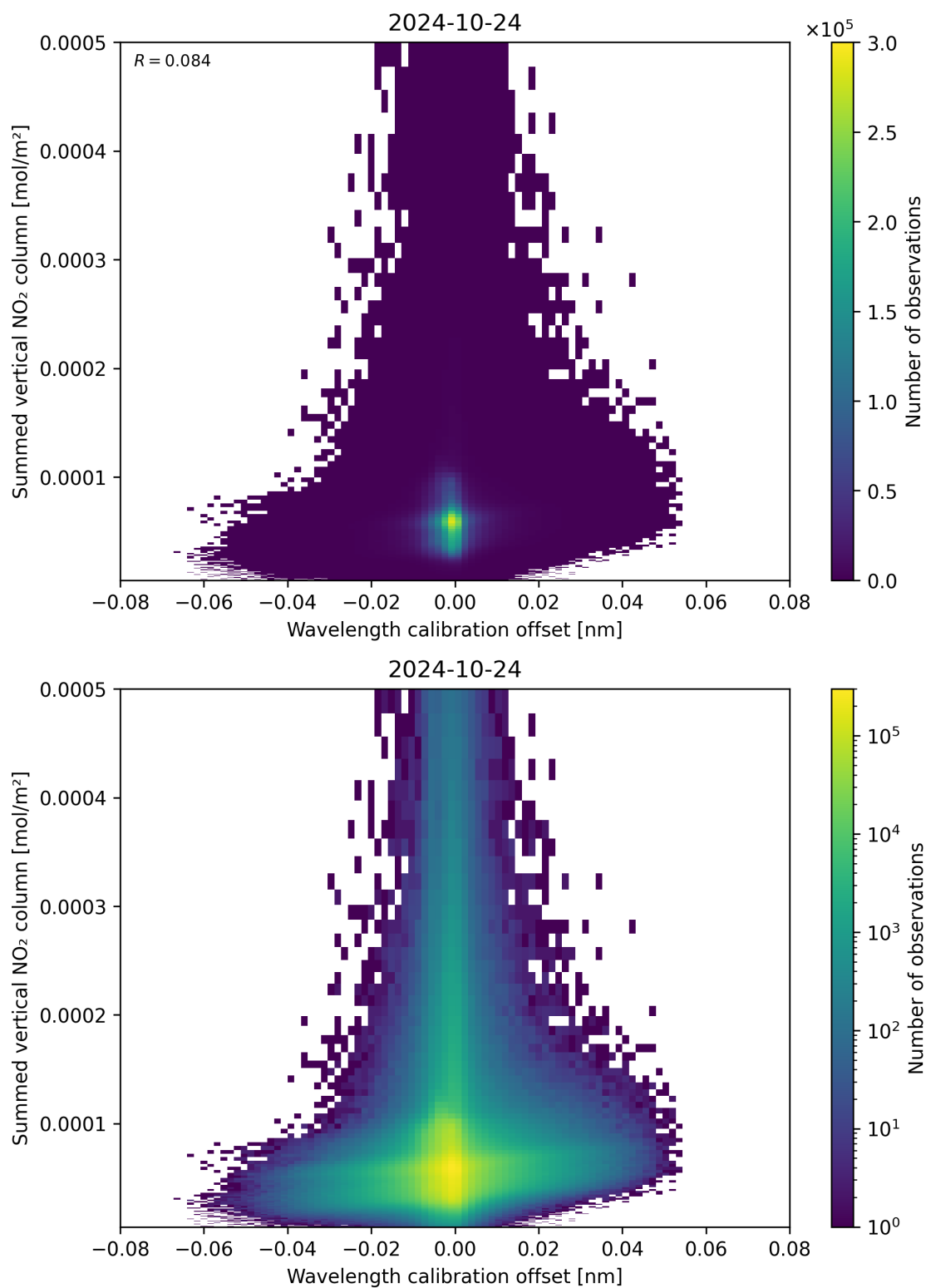
Figure 177: Scatter density plot of “Wavelength calibration offset” against “Summed vertical NO 2 column” for 2024-10-24 to 2024-10-25.
