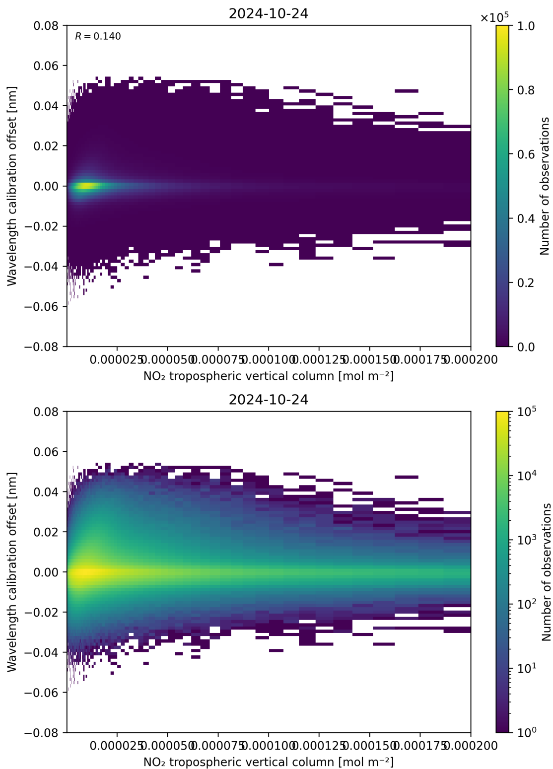
Figure 143: Scatter density plot of “NO 2 tropospheric vertical column” against “Wavelength calibration offset” for 2024-10-24 to 2024-10-25.
