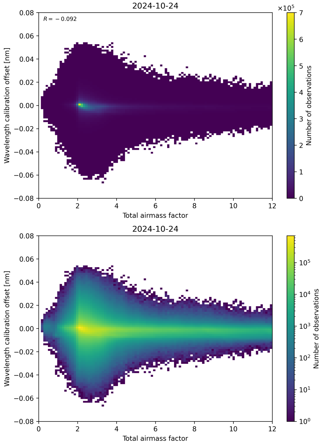
Figure 70: Scatter density plot of “Total airmass factor” against “Wavelength calibration offset” for 2024-10-24 to 2024-10-25.
