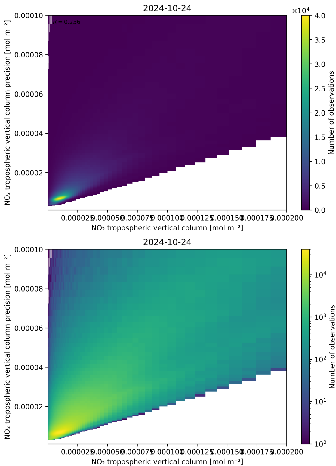
Figure 130: Scatter density plot of “NO 2 tropospheric vertical column” against “NO 2 tropospheric vertical column precision” for 2024-10-24 to 2024-10-25.
