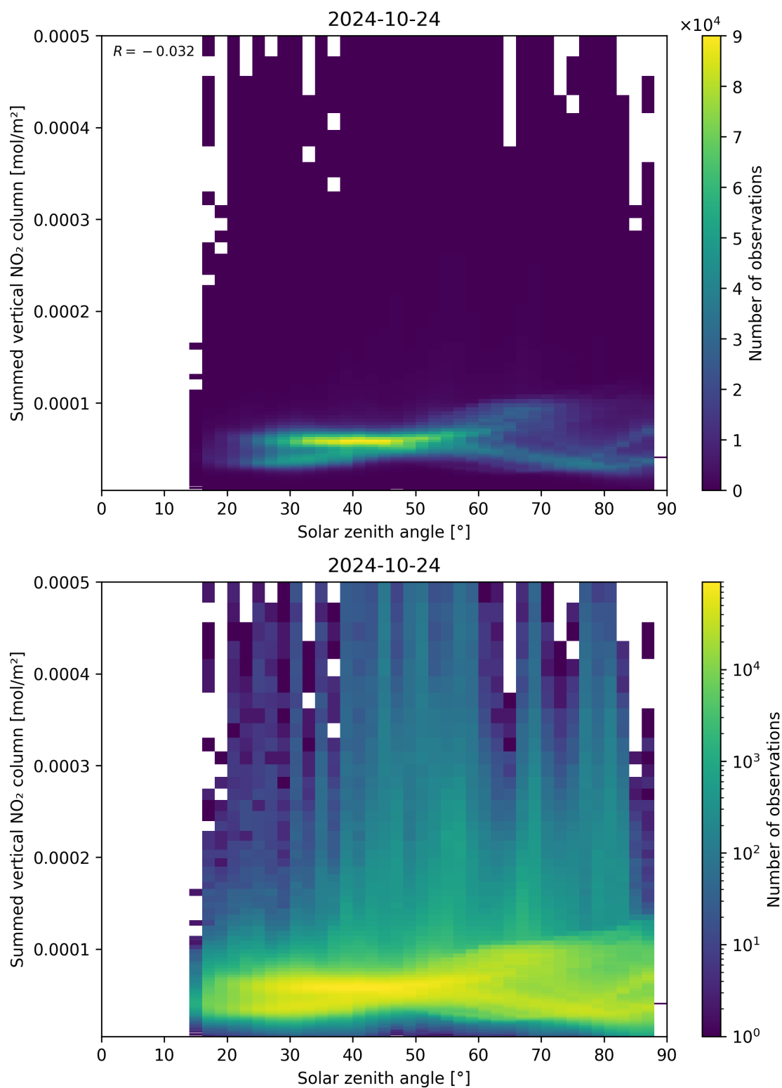
Figure 151: Scatter density plot of “Solar zenith angle” against “Summed vertical NO 2 column” for 2024-10-24 to 2024-10-25.
