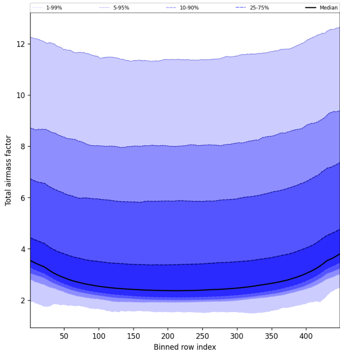
Figure 49: Along track statistics of “Total airmass factor” for 2024-10-24 to 2024-10-25
