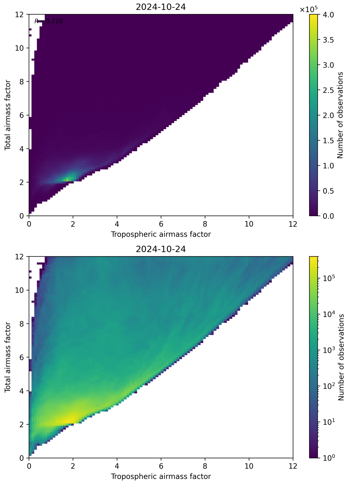
Figure 72: Scatter density plot of “Tropospheric airmass factor” against “Total airmass factor” for 2024-10-24 to 2024-10-25.
