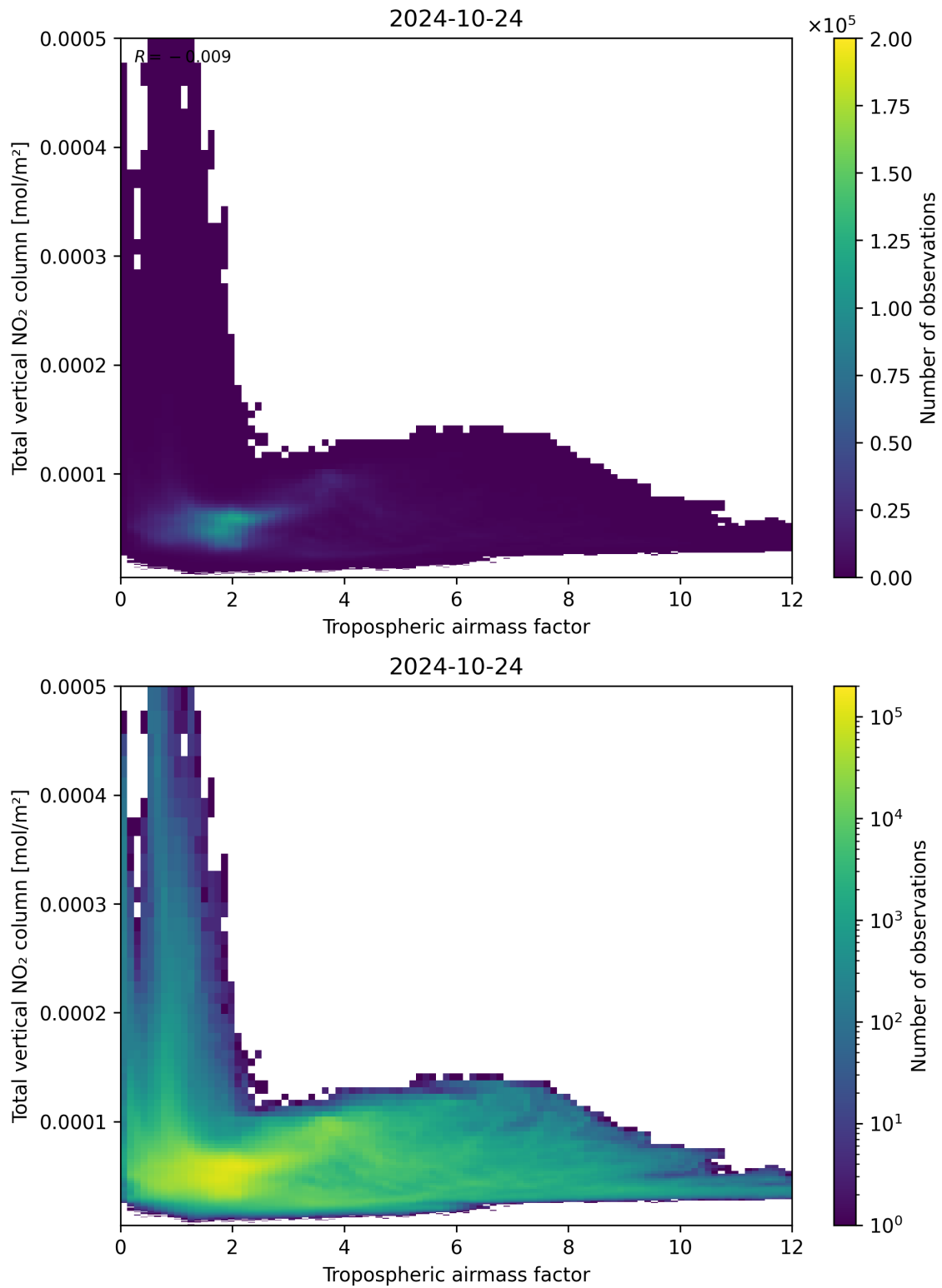
Figure 77: Scatter density plot of “Tropospheric airmass factor” against “Total vertical NO 2 column” for 2024-10-24 to 2024-10-25.
