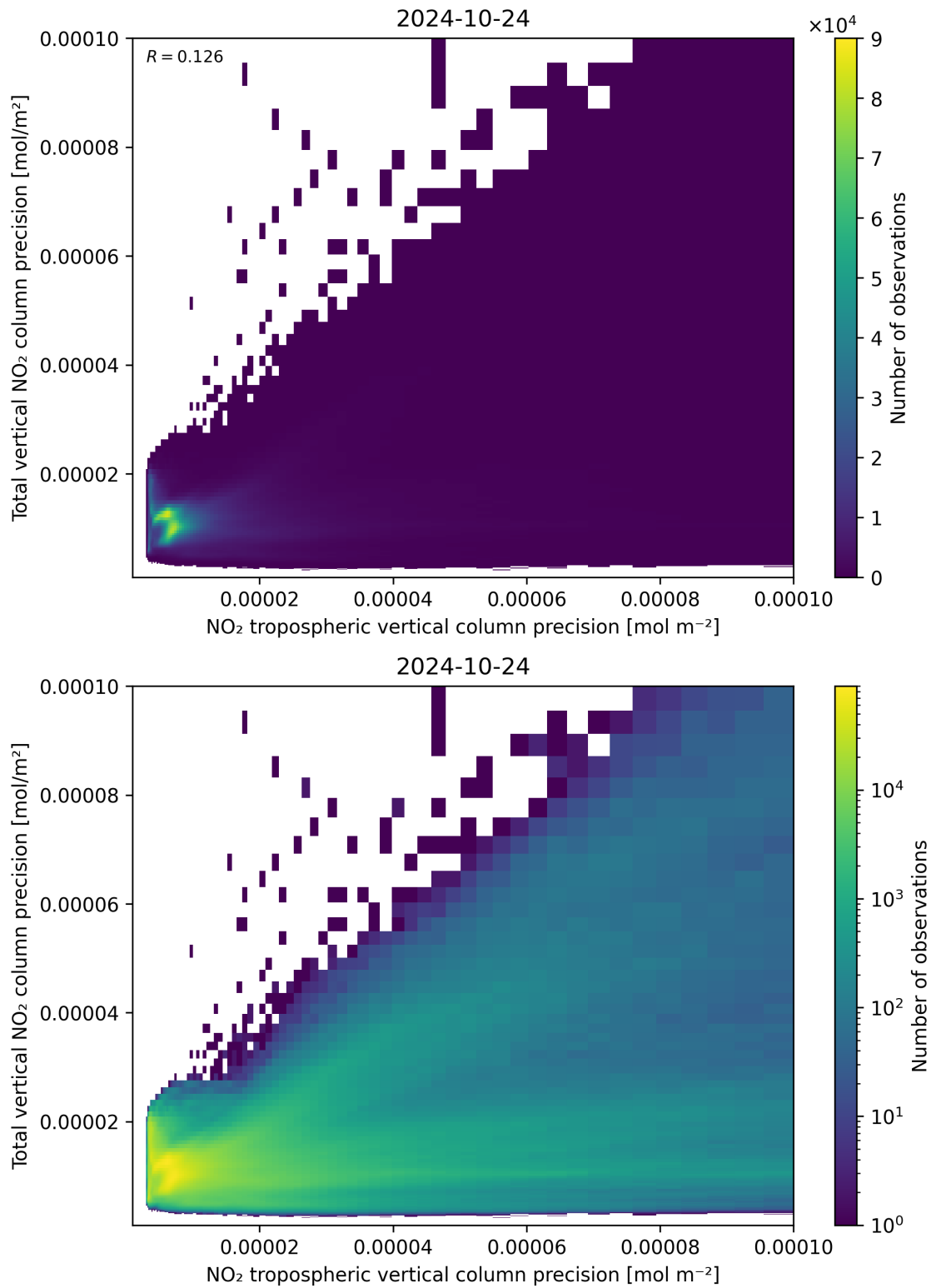
Figure 139: Scatter density plot of “NO 2 tropospheric vertical column precision” against “Total vertical NO 2 column precision” for 2024-10-24 to 2024-10-25.
