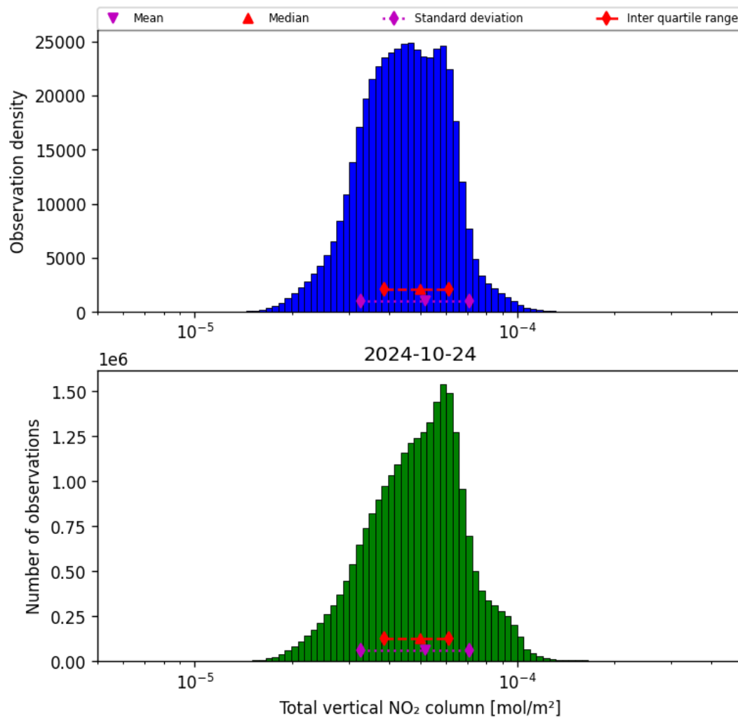
Figure 38: Histogram of “Total vertical NO 2 column” for 2024-10-24 to 2024-10-25
