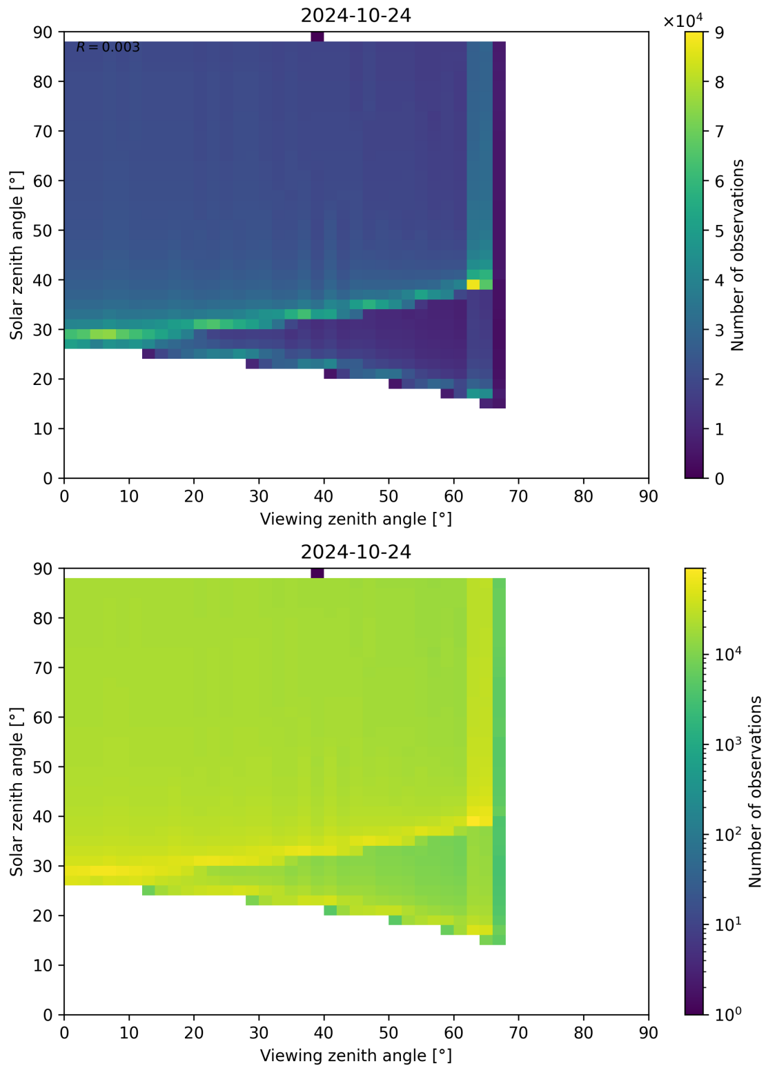
Figure 172: Scatter density plot of “Viewing zenith angle” against “Solar zenith angle” for 2024-10-24 to 2024-10-25.
