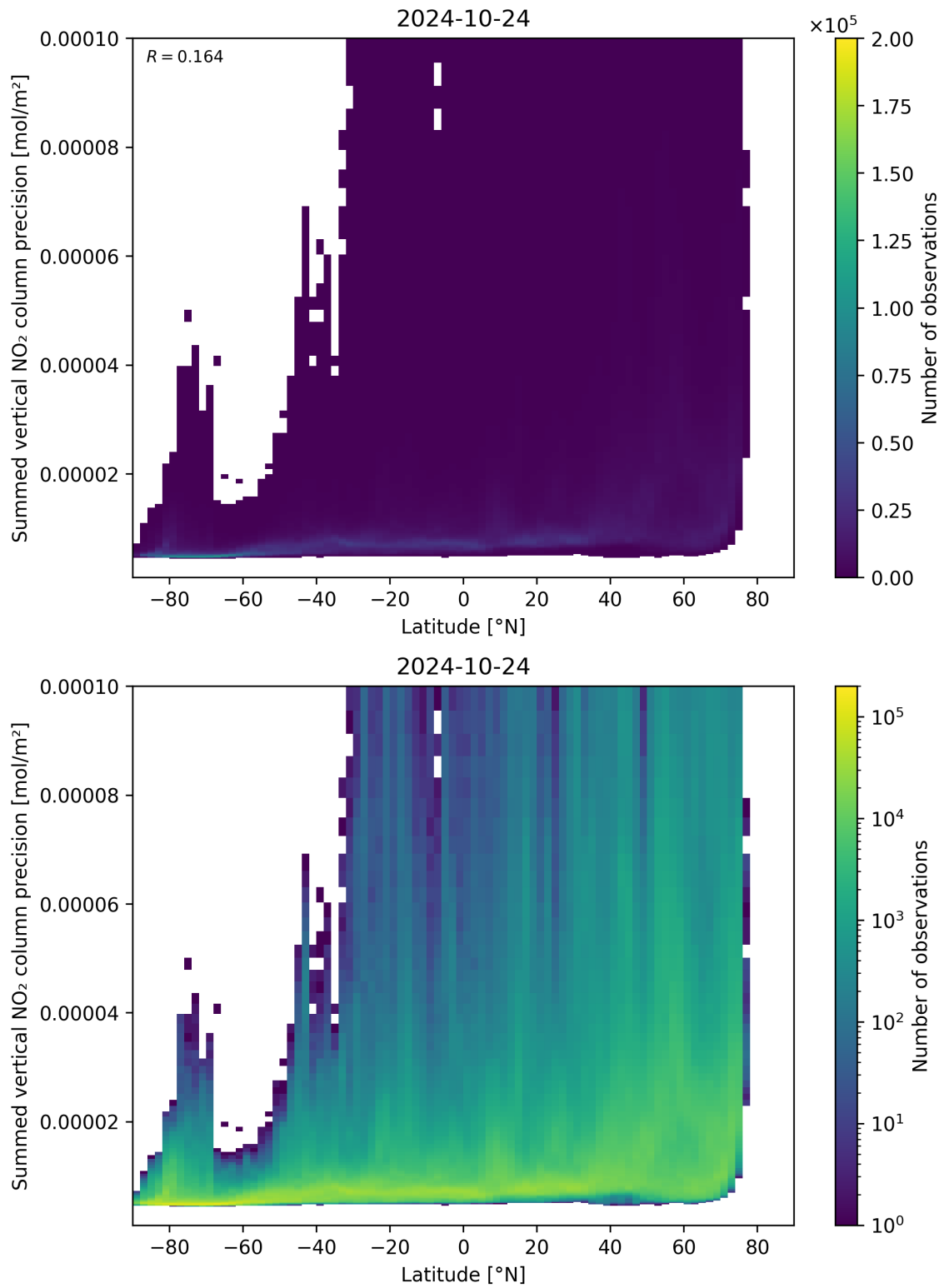
Figure 89: Scatter density plot of “Latitude” against “Summed vertical NO 2 column precision” for 2024-10-24 to 2024-10-25.
