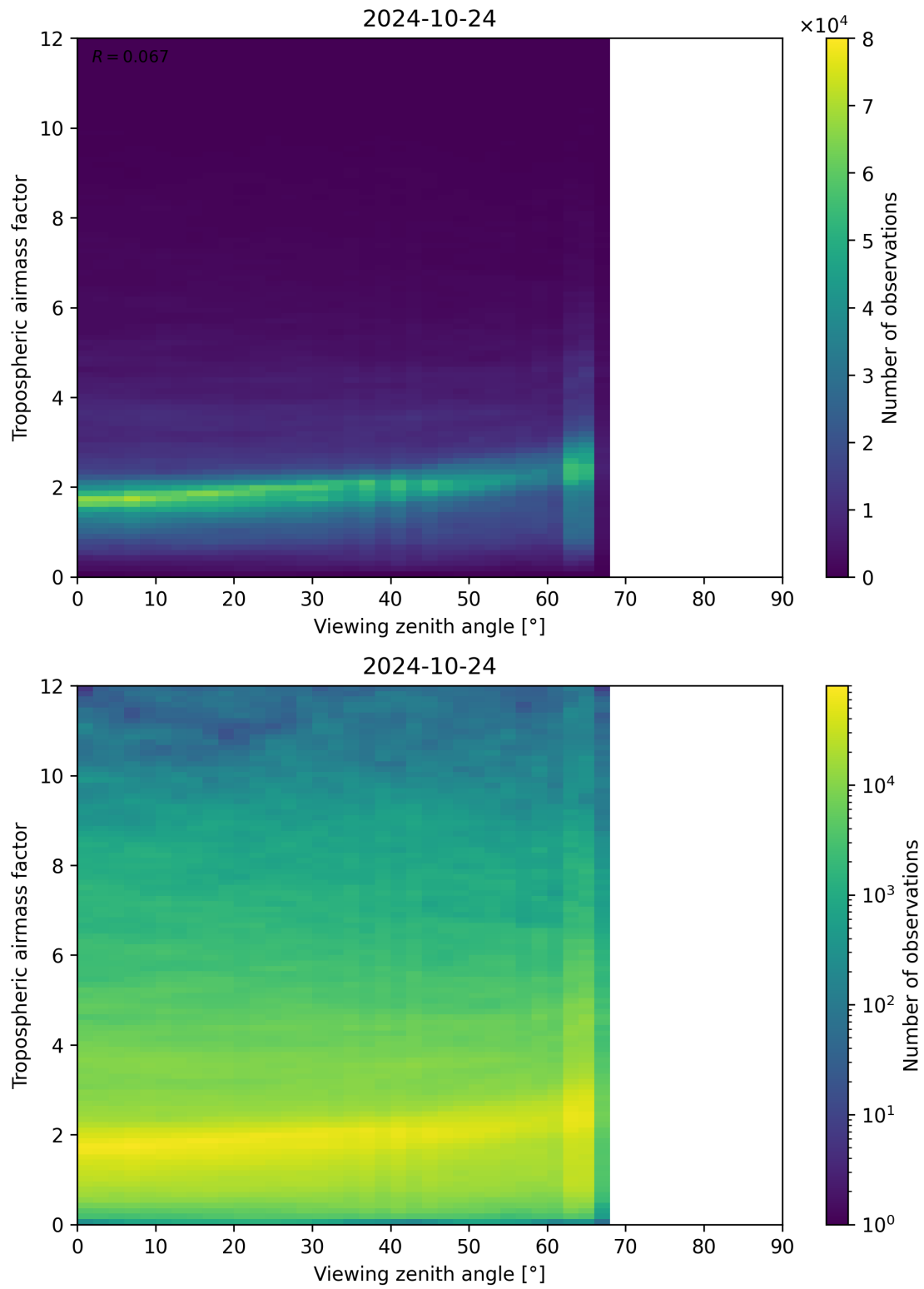
Figure 161: Scatter density plot of “Viewing zenith angle” against “Tropospheric airmass factor” for 2024-10-24 to 2024-10-25.
