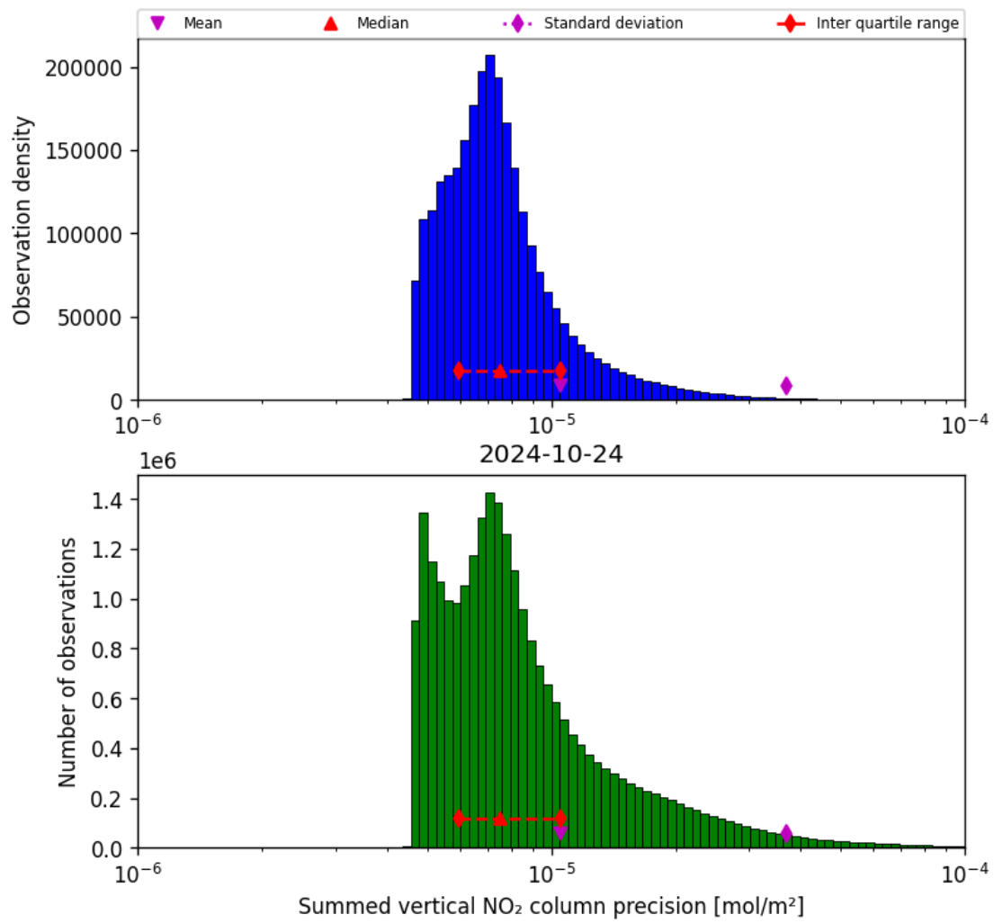
Figure 41: Histogram of "Summed vertical NO 2 column precision" for 2024-10-24 to 2024-10-25
