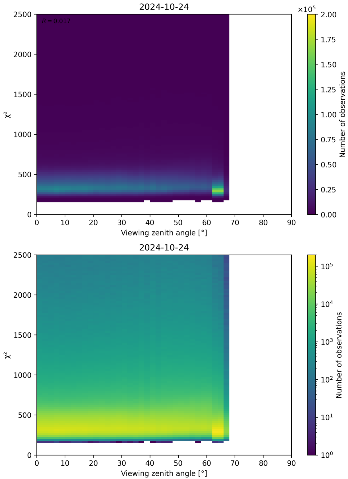
Figure 162: Scatter density plot of “Viewing zenith angle” against “ \chi^2 ” for 2024-10-24 to 2024-10-25.
