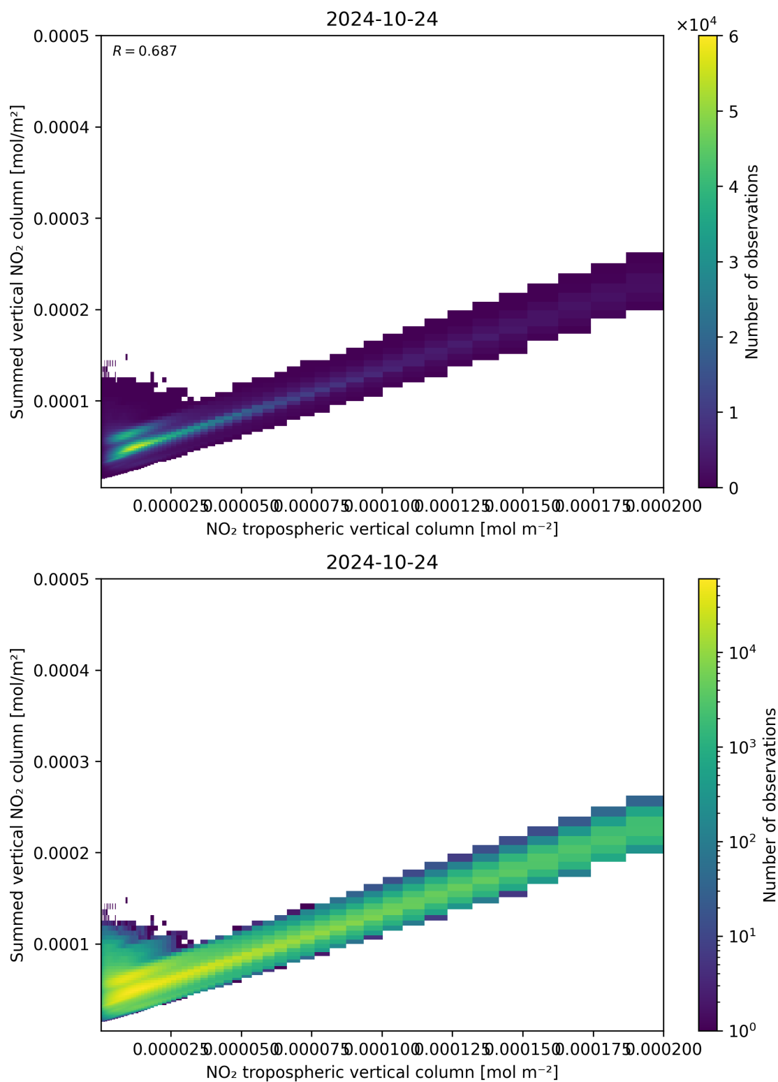
Figure 126: Scatter density plot of “NO 2 tropospheric vertical column” against “Summed vertical NO 2 column” for 2024-10-24 to 2024-10-25.
