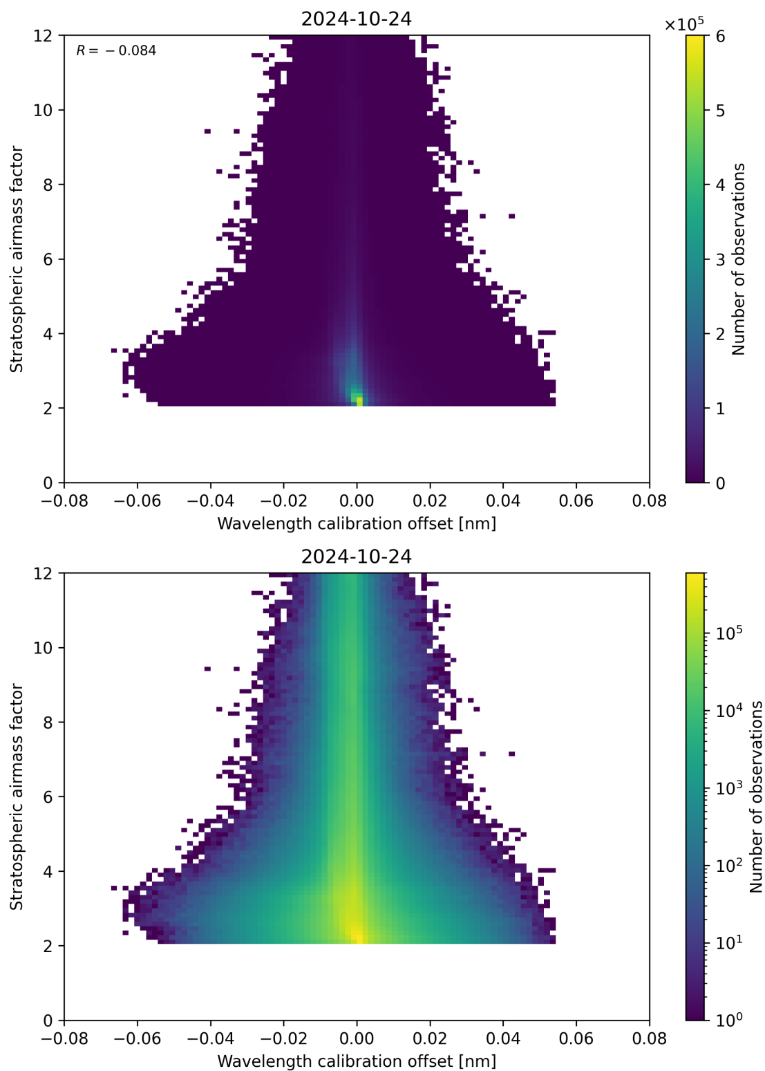
Figure 174: Scatter density plot of “Wavelength calibration offset” against “Stratospheric air mass factor” for 2024-10-24 to 2024-10-25.
