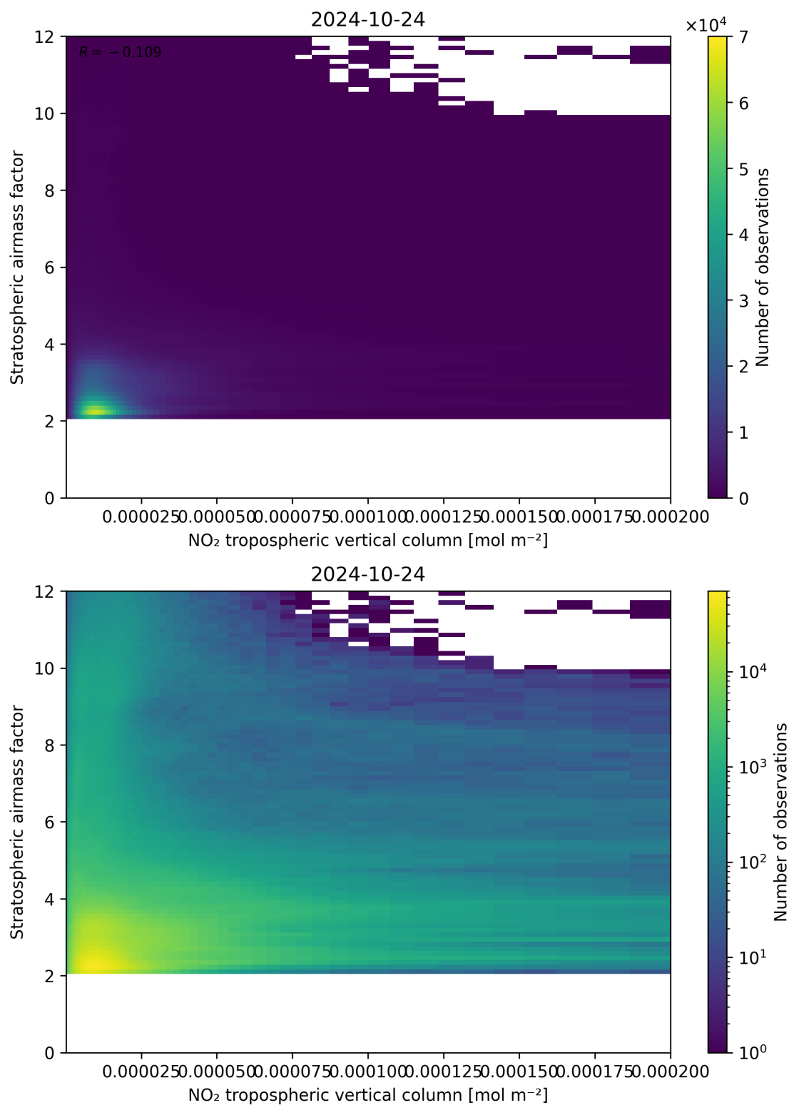
Figure 121: Scatter density plot of “NO 2 tropospheric vertical column” against “Stratospheric airmass factor” for 2024-10-24 to 2024-10-25.
