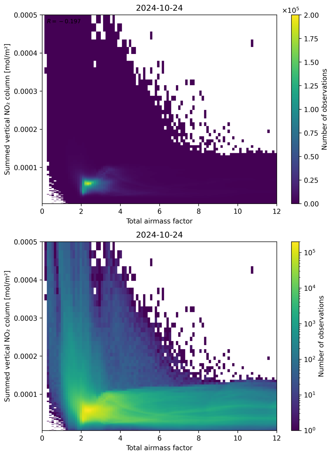
Figure 65: Scatter density plot of “Total airmass factor” against “Summed vertical NO 2 column” for 2024-10-24 to 2024-10-25.
