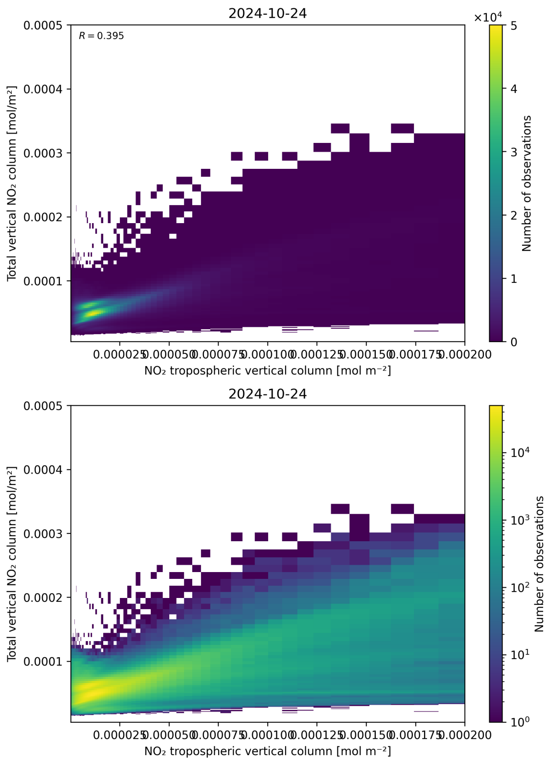
Figure 128: Scatter density plot of “NO 2 tropospheric vertical column” against “Total vertical NO 2 column” for 2024-10-24 to 2024-10-25.
