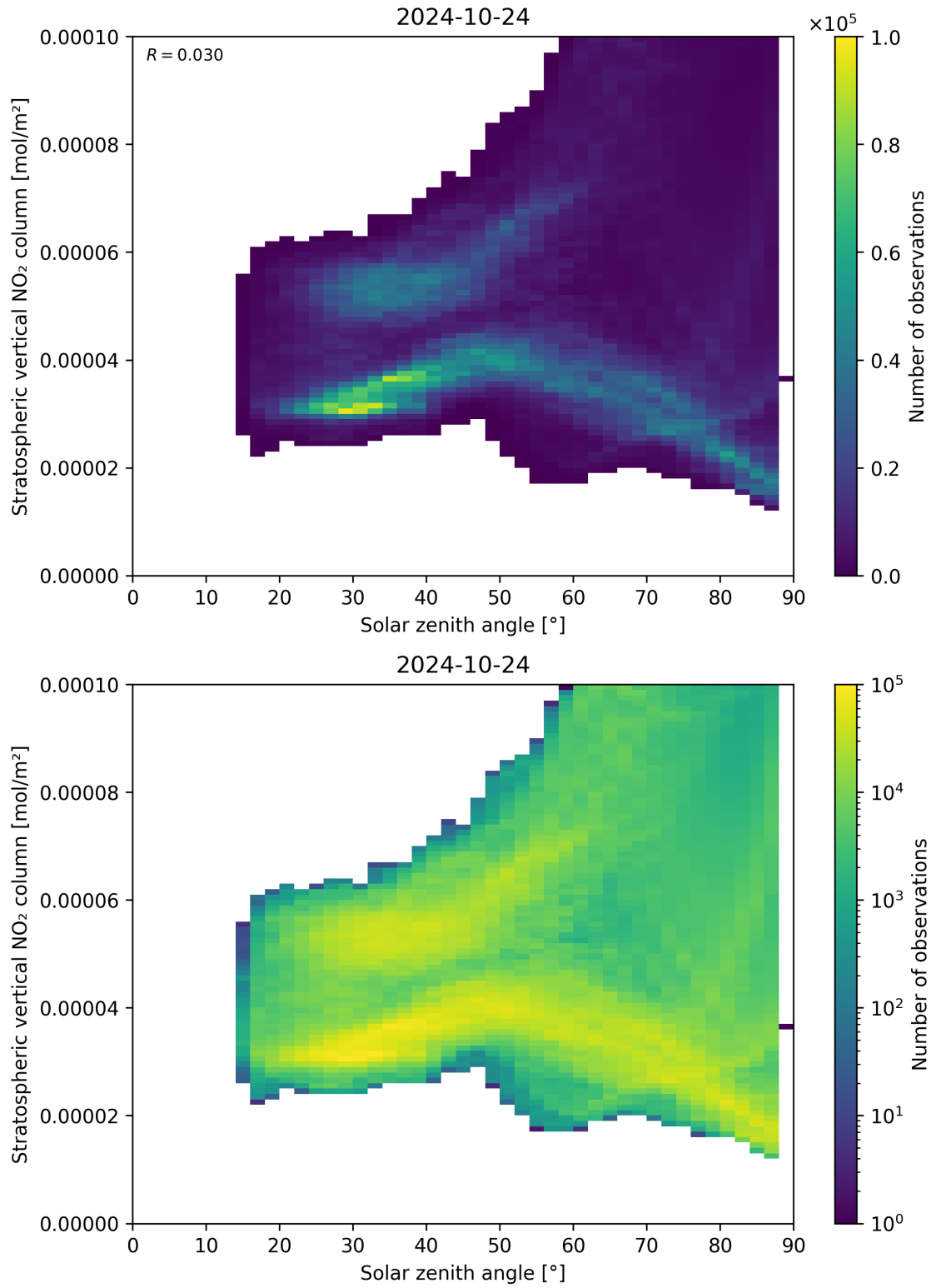
Figure 150: Scatter density plot of “Solar zenith angle” against “Stratospheric vertical NO 2 column” for 2024-10-24 to 2024-10-25.
