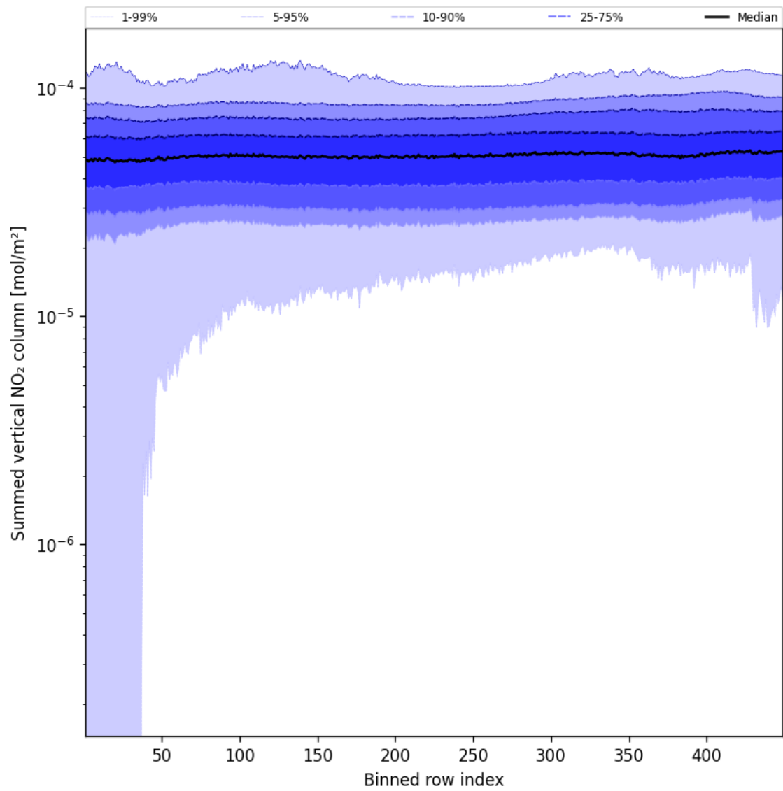
Figure 57: Along track statistics of “Summed vertical NO 2 column” for 2024-10-24 to 2024-10-25
