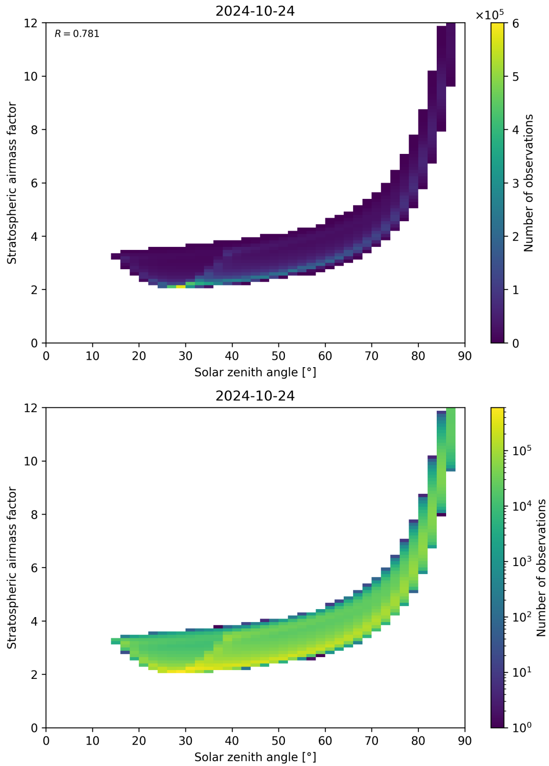
Figure 145: Scatter density plot of “Solar zenith angle” against “Stratospheric airmass factor” for 2024-10-24 to 2024-10-25.
