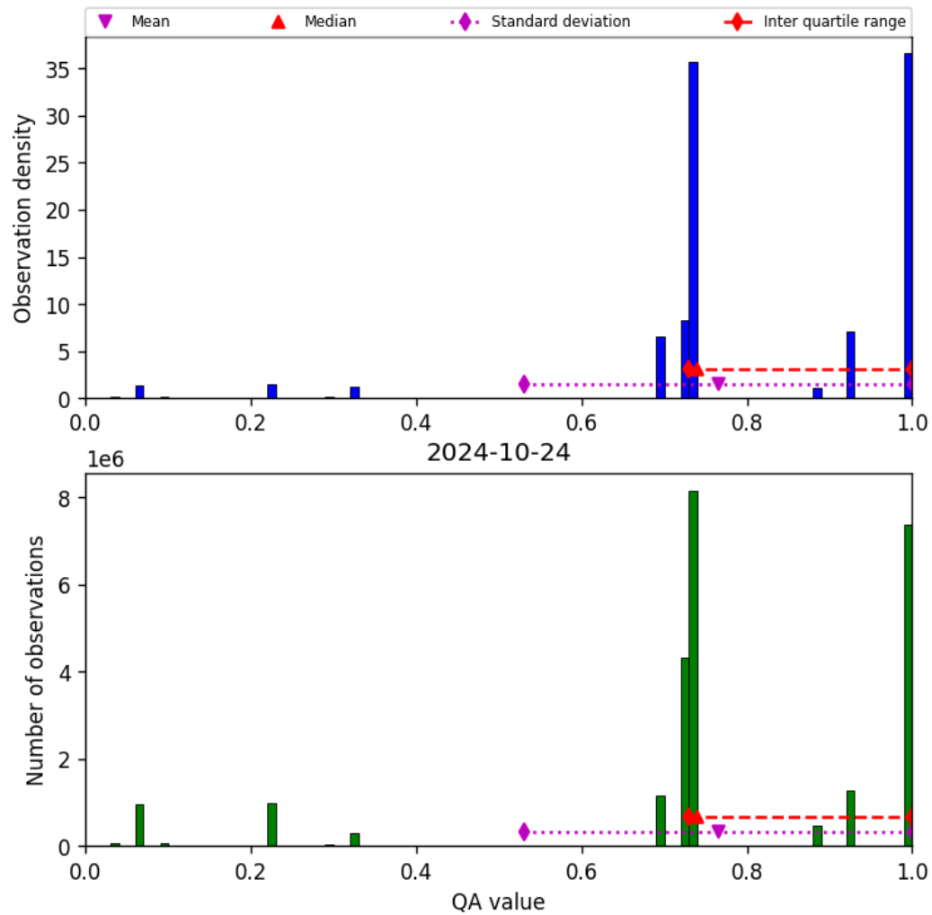
Figure 28: Histogram of “QA value” for 2024-10-24 to 2024-10-25
