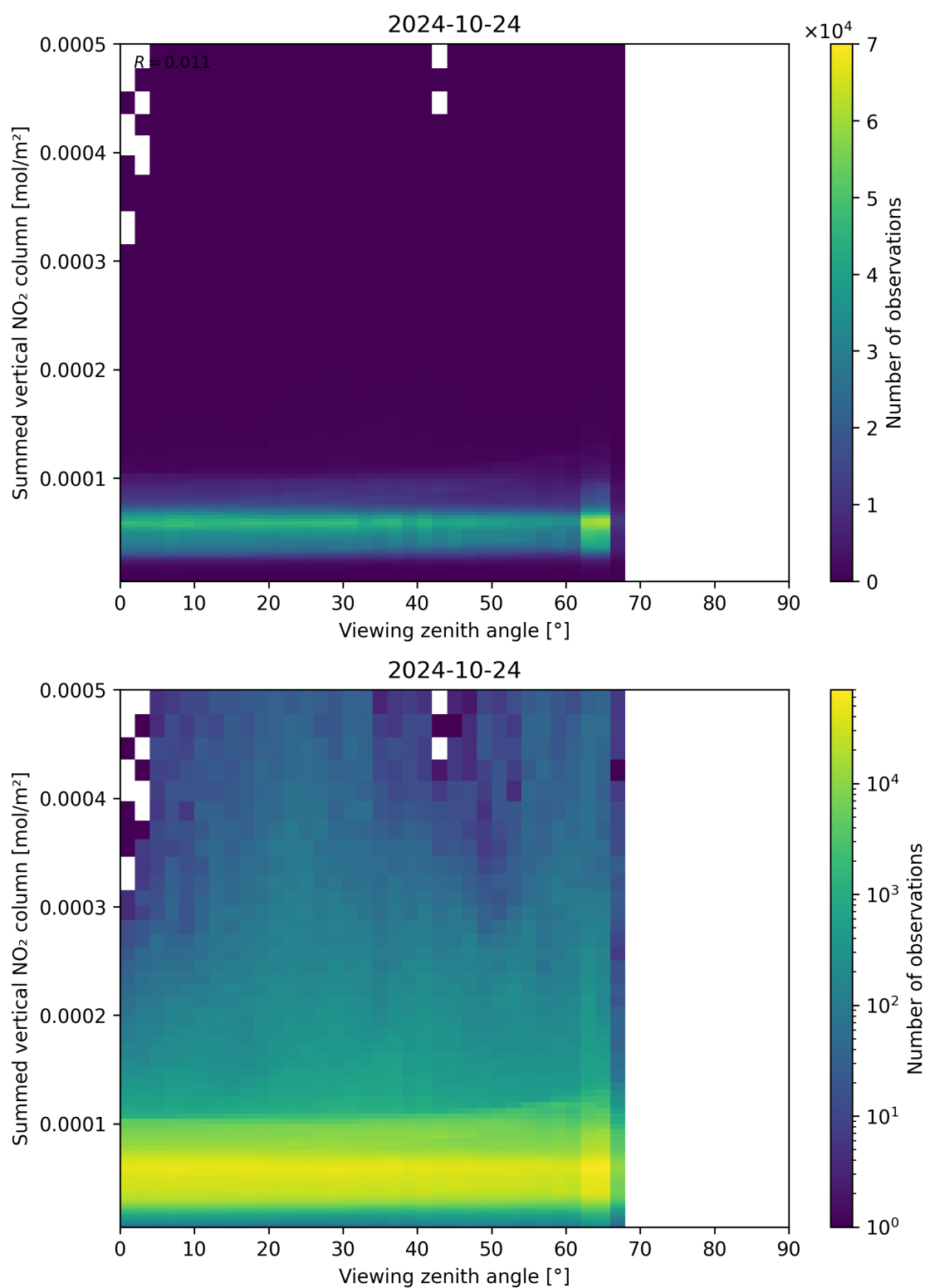
Figure 165: Scatter density plot of “Viewing zenith angle” against “Summed vertical NO 2 column” for 2024-10-24 to 2024-10-25.
