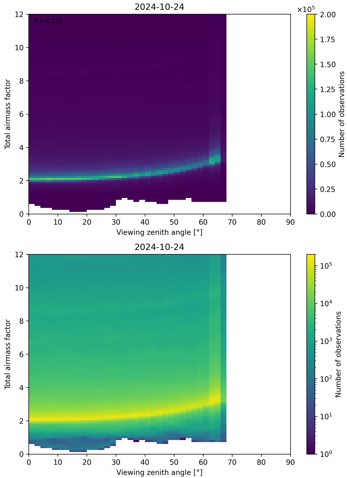
Figure 160: Scatter density plot of “Viewing zenith angle” against “Total airmass factor” for 2024-10-24 to 2024-10-25.
