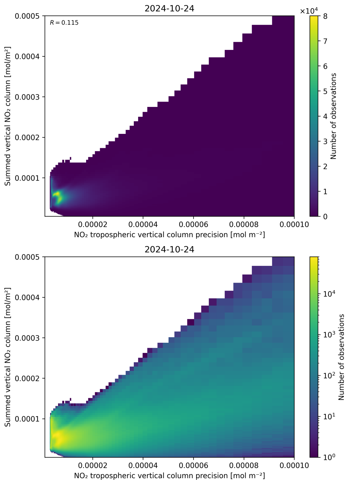
Figure 136: Scatter density plot of “NO 2 tropospheric vertical column precision” against “Summed vertical NO 2 column” for 2024-10-24 to 2024-10-25.
