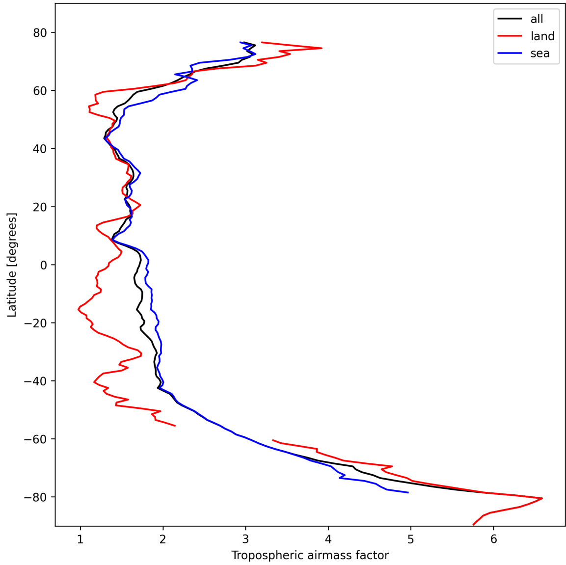
Figure 14: Zonal average of “Tropospheric air mass factor” for 2024-10-24 to 2024-10-25.
