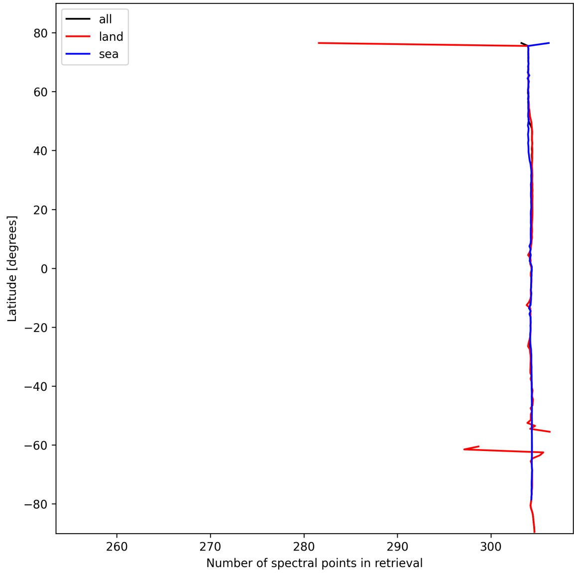
Figure 16: Zonal average of “Number of spectral points in retrieval” for 2024-10-24 to 2024-10-25.
