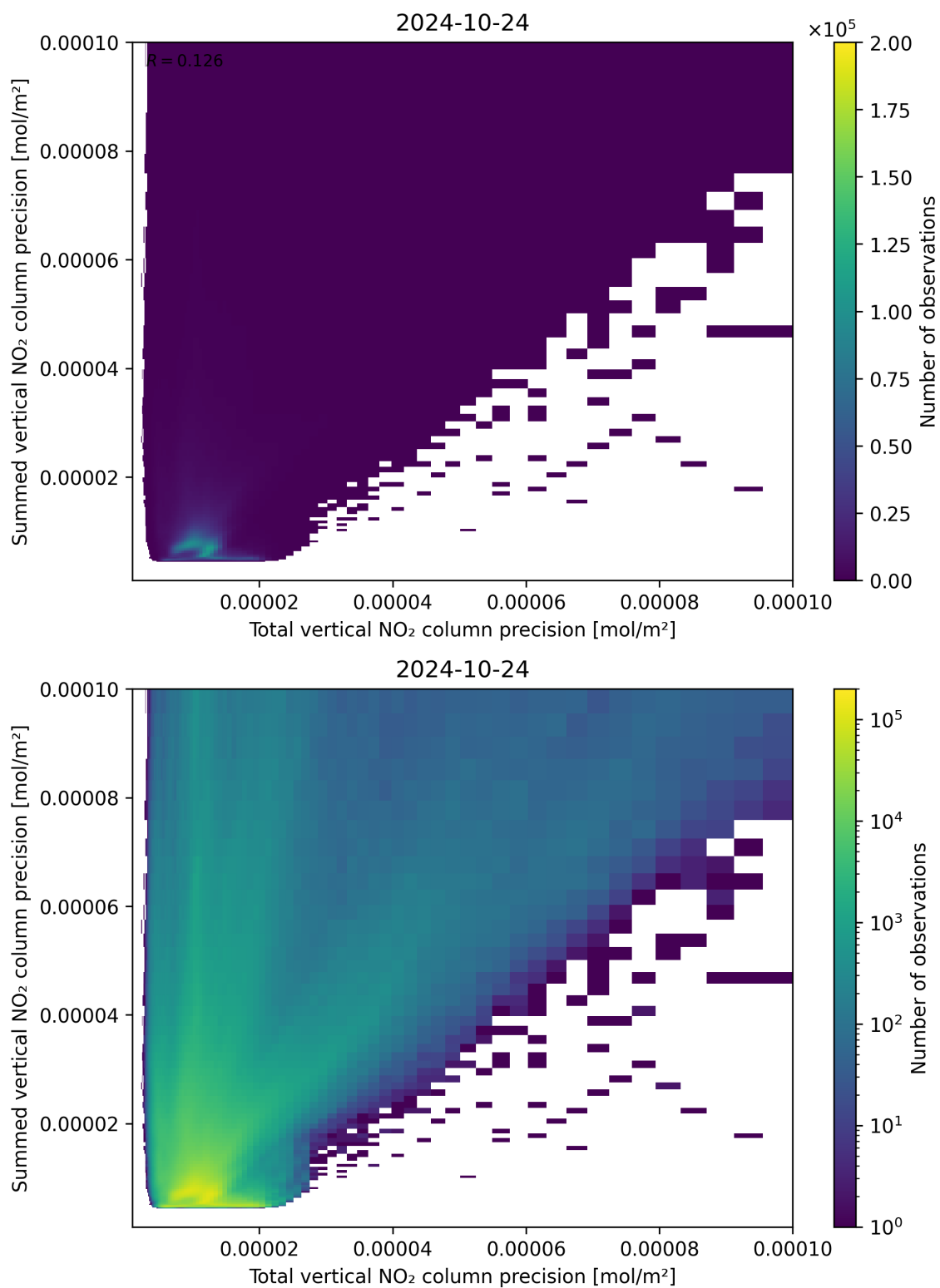
Figure 118: Scatter density plot of “Total vertical NO 2 column precision” against “Summed vertical NO 2 column precision” for 2024-10-24 to 2024-10-25.
