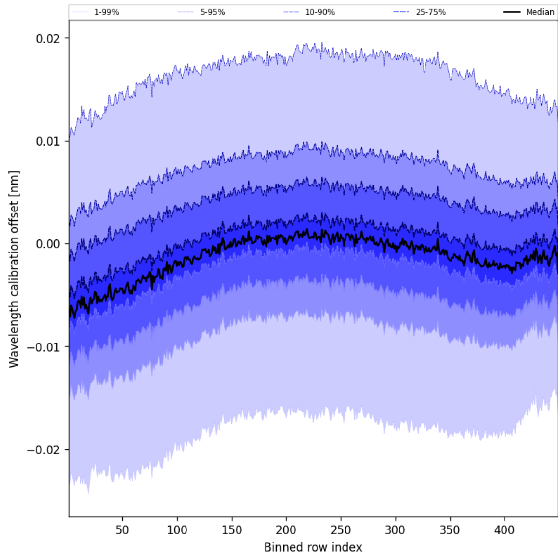
Figure 52: Along track statistics of “Wavelength calibration offset” for 2024-10-24 to 2024-10-25
