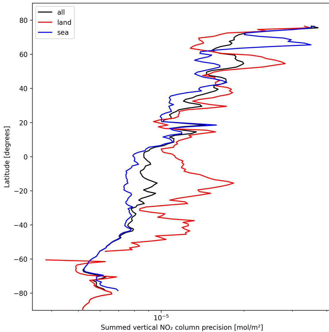
Figure 24: Zonal average of “Summed vertical NO 2 column precision” for 2024-10-24 to 2024-10-25.
