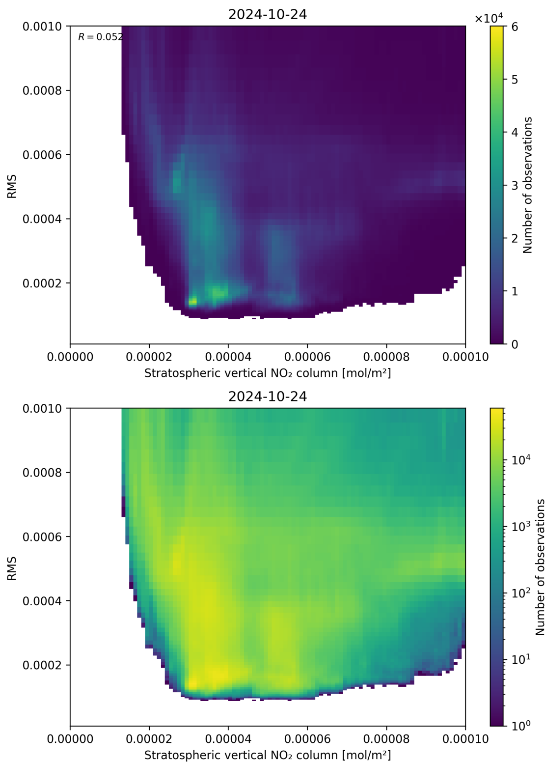
Figure 102: Scatter density plot of “Stratospheric vertical NO 2 column” against “RMS” for 2024-10-24 to 2024-10-25.
