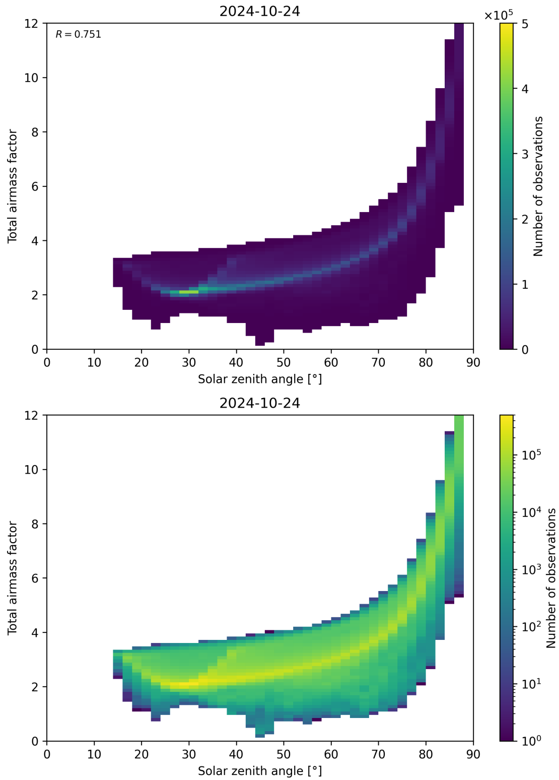
Figure 146: Scatter density plot of “Solar zenith angle” against “Total airmass factor” for 2024-10-24 to 2024-10-25.
