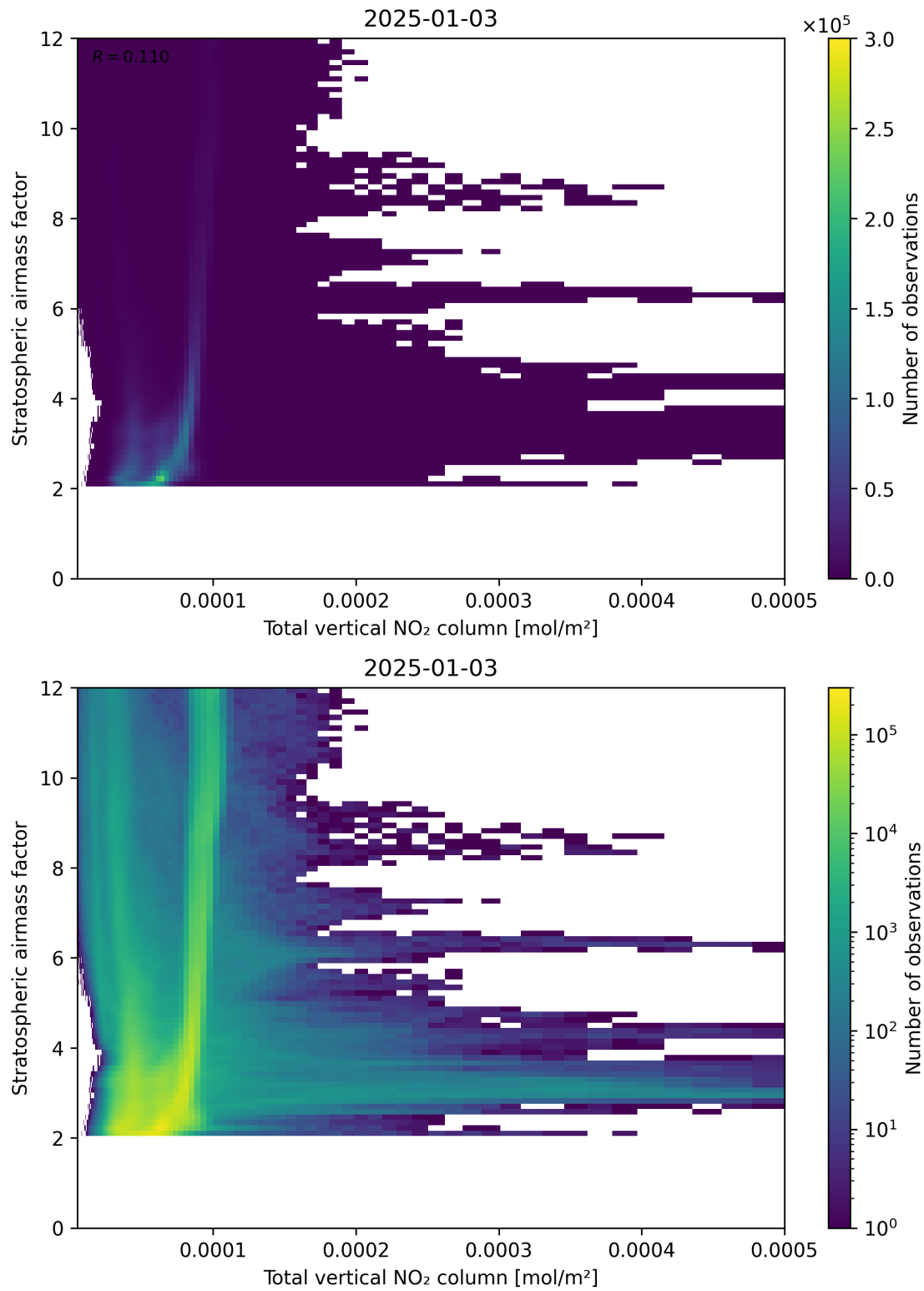
Figure 110: Scatter density plot of “Total vertical NO 2 column” against “Stratospheric airmass factor” for 2025-01-02 to 2025-01-04.
