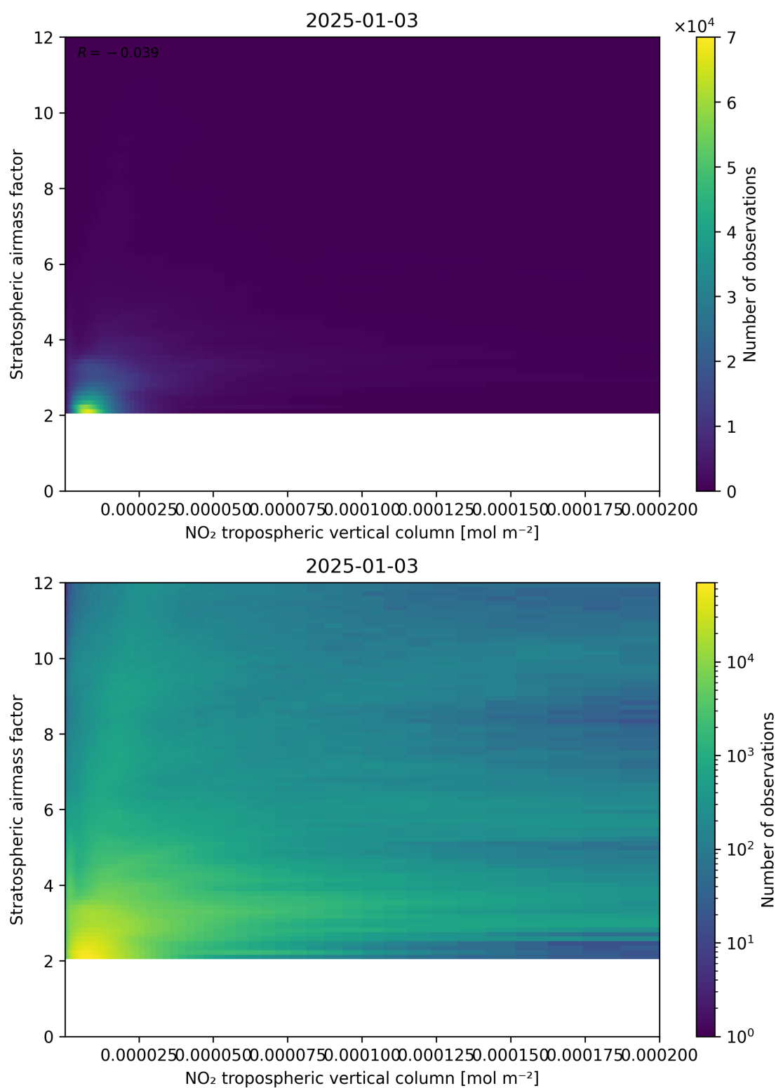
Figure 121: Scatter density plot of “NO 2 tropospheric vertical column” against “Stratospheric airmass factor” for 2025-01-02 to 2025-01-04.
