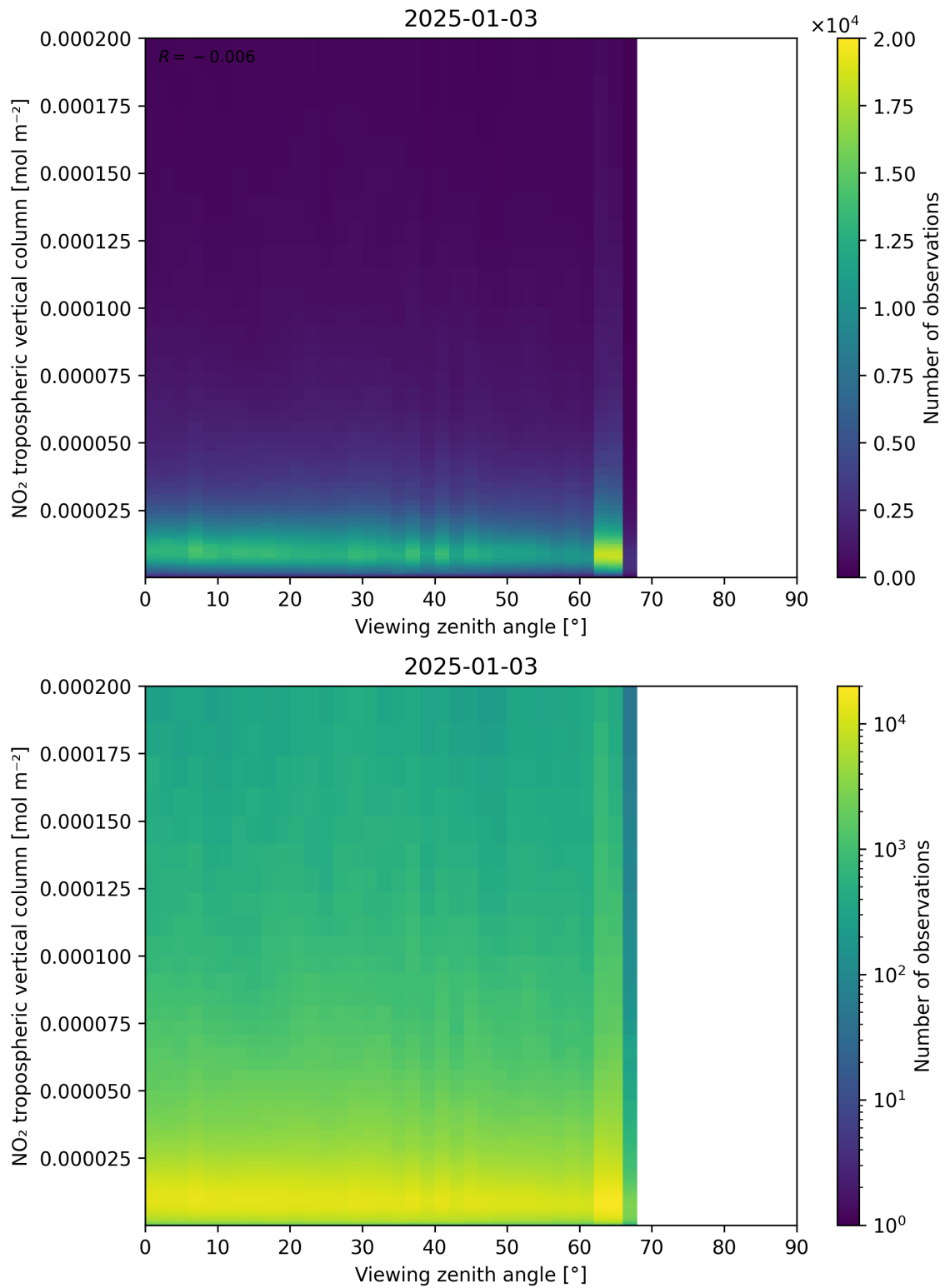
Figure 169: Scatter density plot of “Viewing zenith angle” against “NO 2 tropospheric vertical column” for 2025-01-02 to 2025-01-04.
