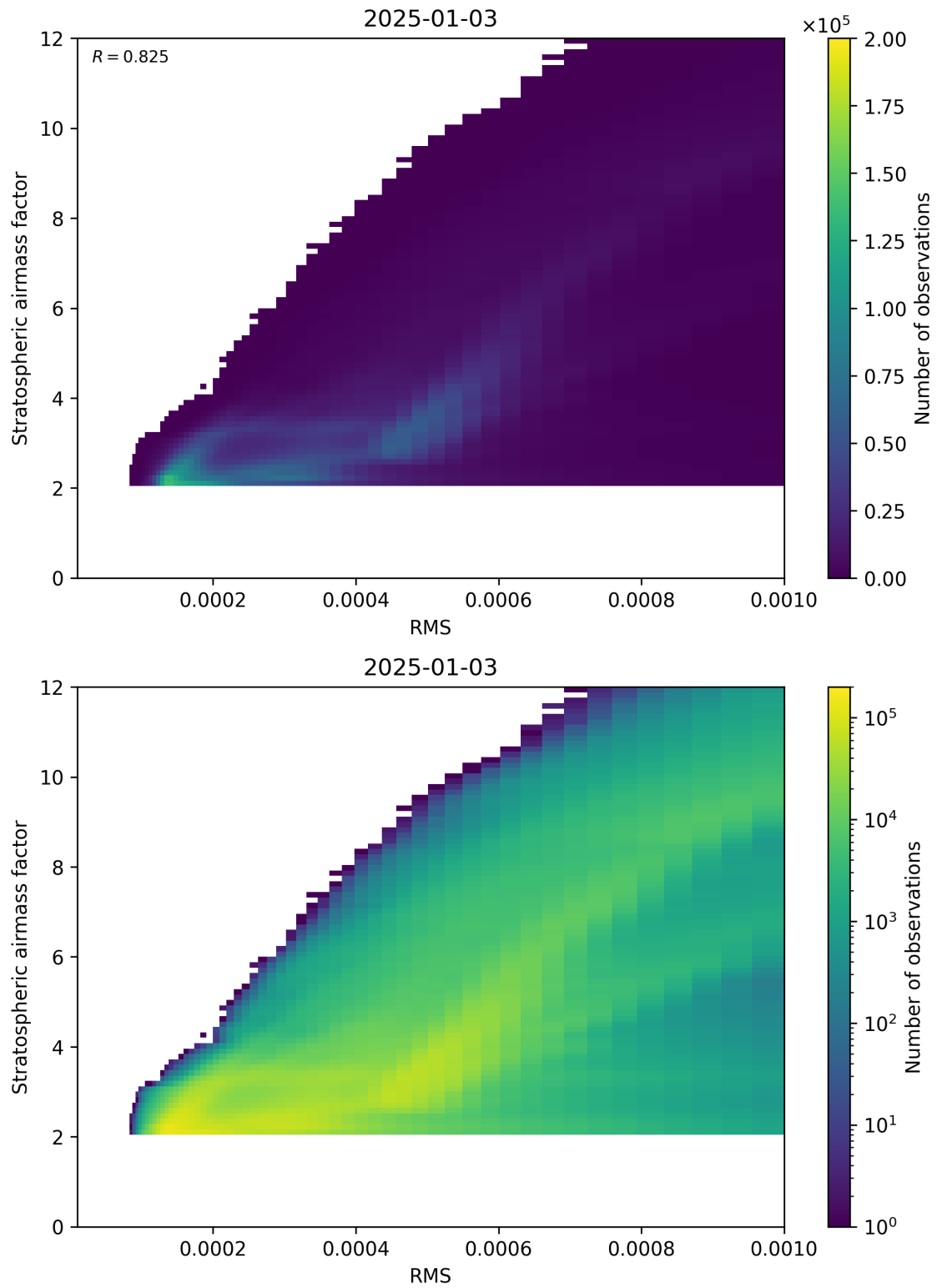
Figure 144: Scatter density plot of “RMS” against “Stratospheric airmass factor” for 2025-01-02 to 2025-01-04.
