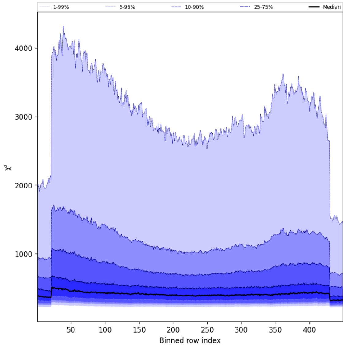
Figure 59: Along track statistics of “ \chi^2 ” for 2025-01-02 to 2025-01-04
