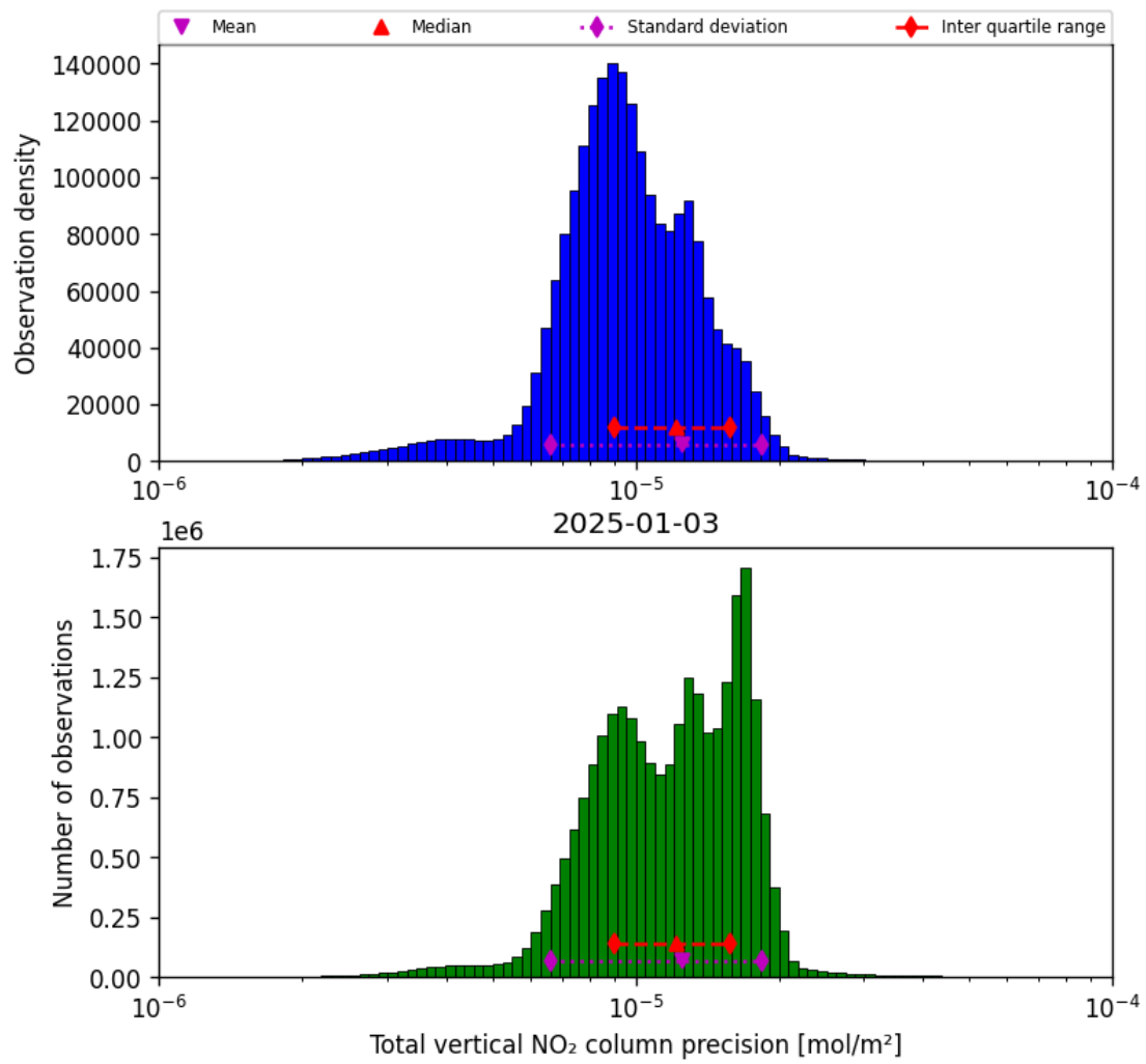
Figure 39: Histogram of “Total vertical NO 2 column precision” for 2025-01-02 to 2025-01-04
