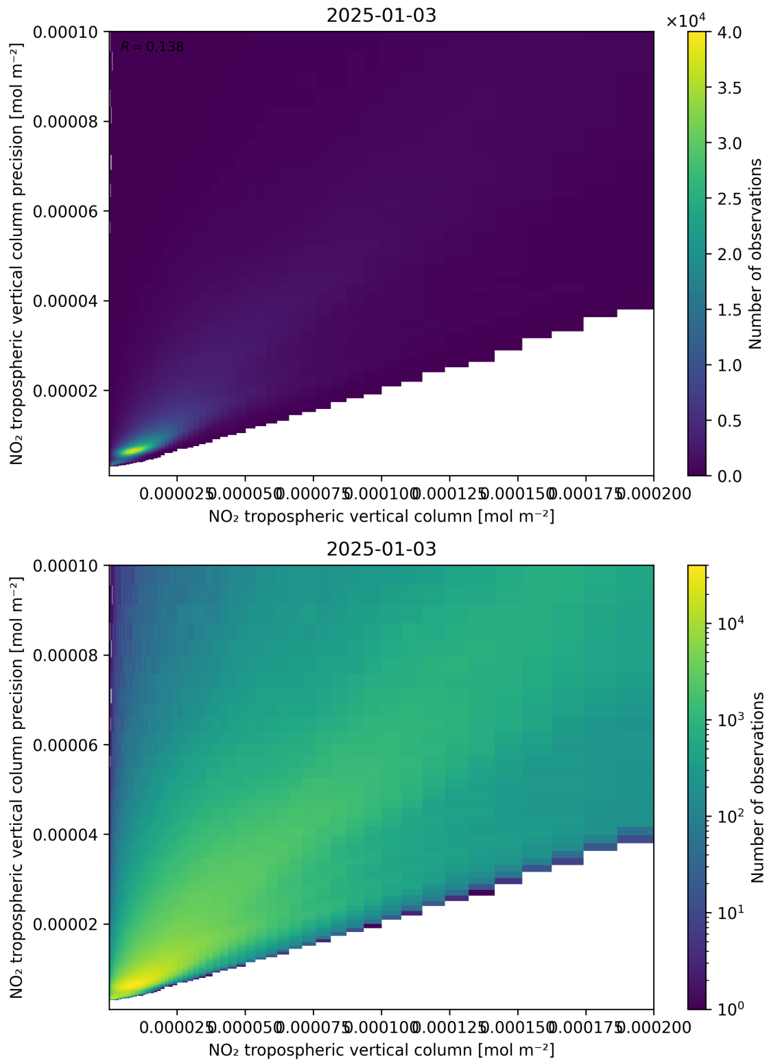
Figure 130: Scatter density plot of “NO 2 tropospheric vertical column” against “NO 2 tropospheric vertical column precision” for 2025-01-02 to 2025-01-04.
