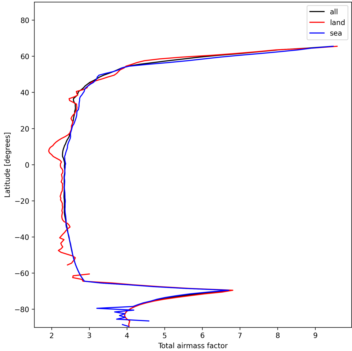
Figure 15: Zonal average of “Total airmass factor” for 2025-01-02 to 2025-01-04.
