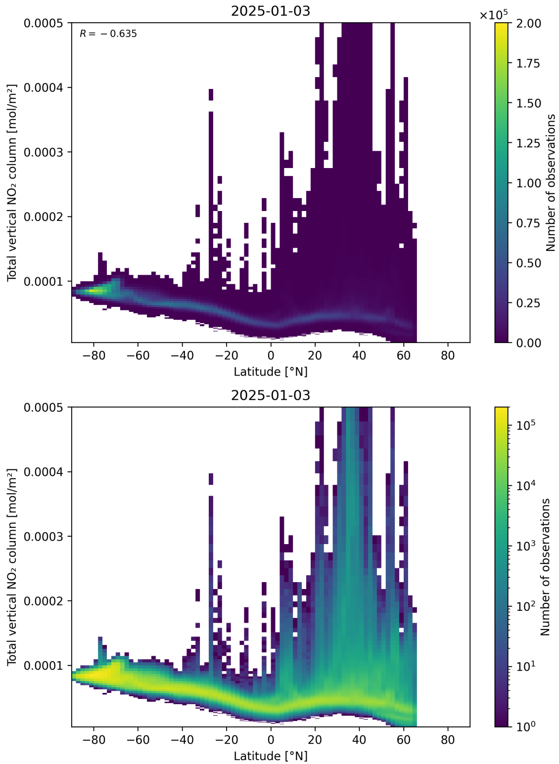
Figure 90: Scatter density plot of “Latitude” against “Total vertical NO 2 column” for 2025-01-02 to 2025-01-04.
