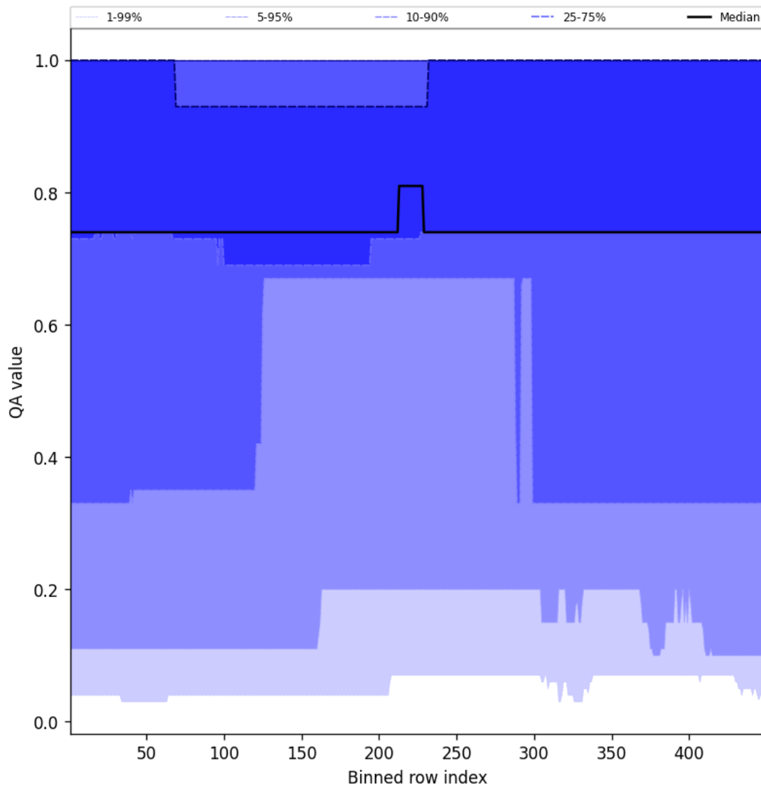
Figure 45: Along track statistics of “QA value” for 2025-01-02 to 2025-01-04
