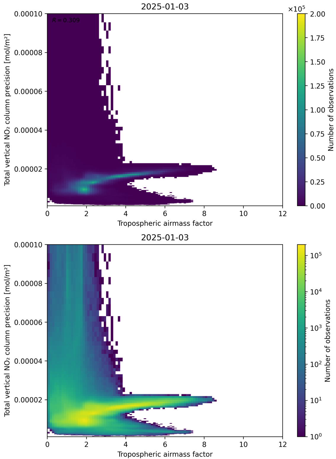
Figure 78: Scatter density plot of “Tropospheric air mass factor” against “Total vertical NO 2 column precision” for 2025-01-02 to 2025-01-04.
