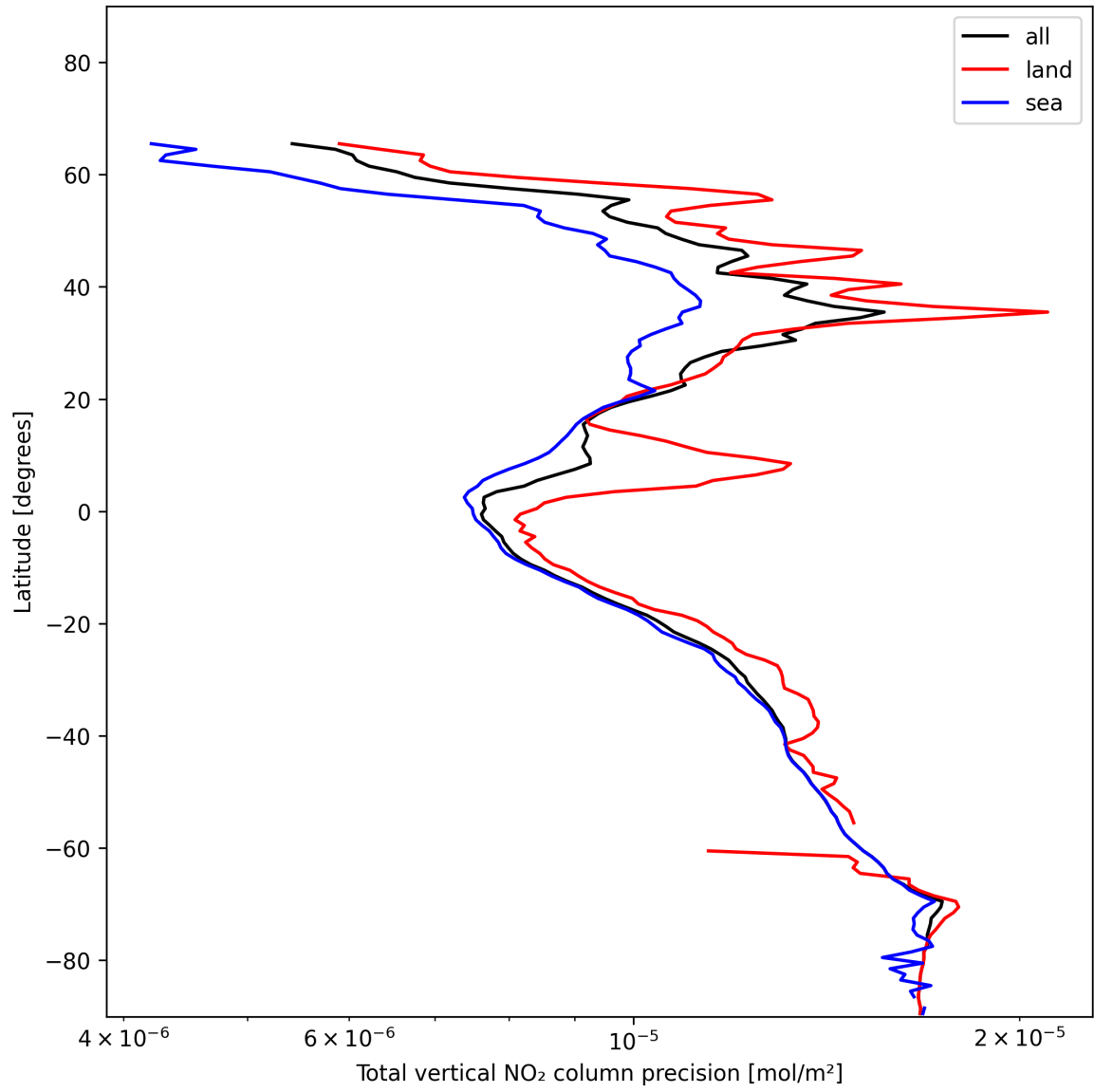
Figure 22: Zonal average of “Total vertical NO 2 column precision” for 2025-01-02 to 2025-01-04.
