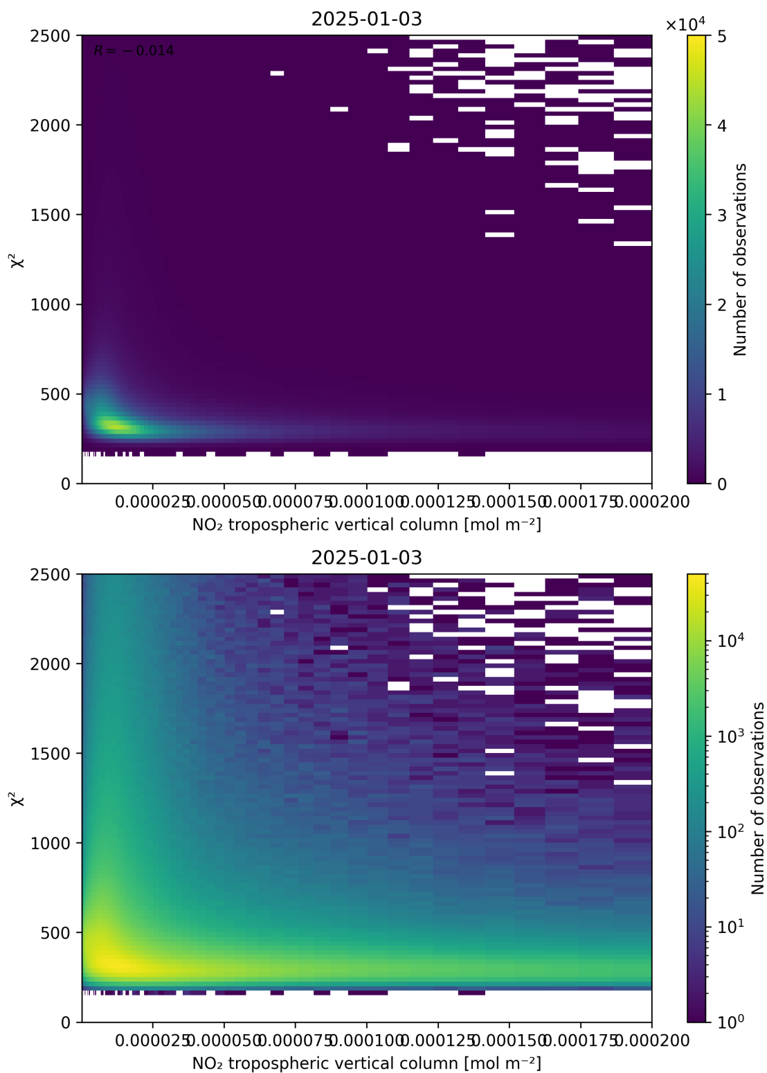
Figure 124: Scatter density plot of “NO 2 tropospheric vertical column” against “ \chi^2 ” for 2025-01-02 to 2025-01-04.
