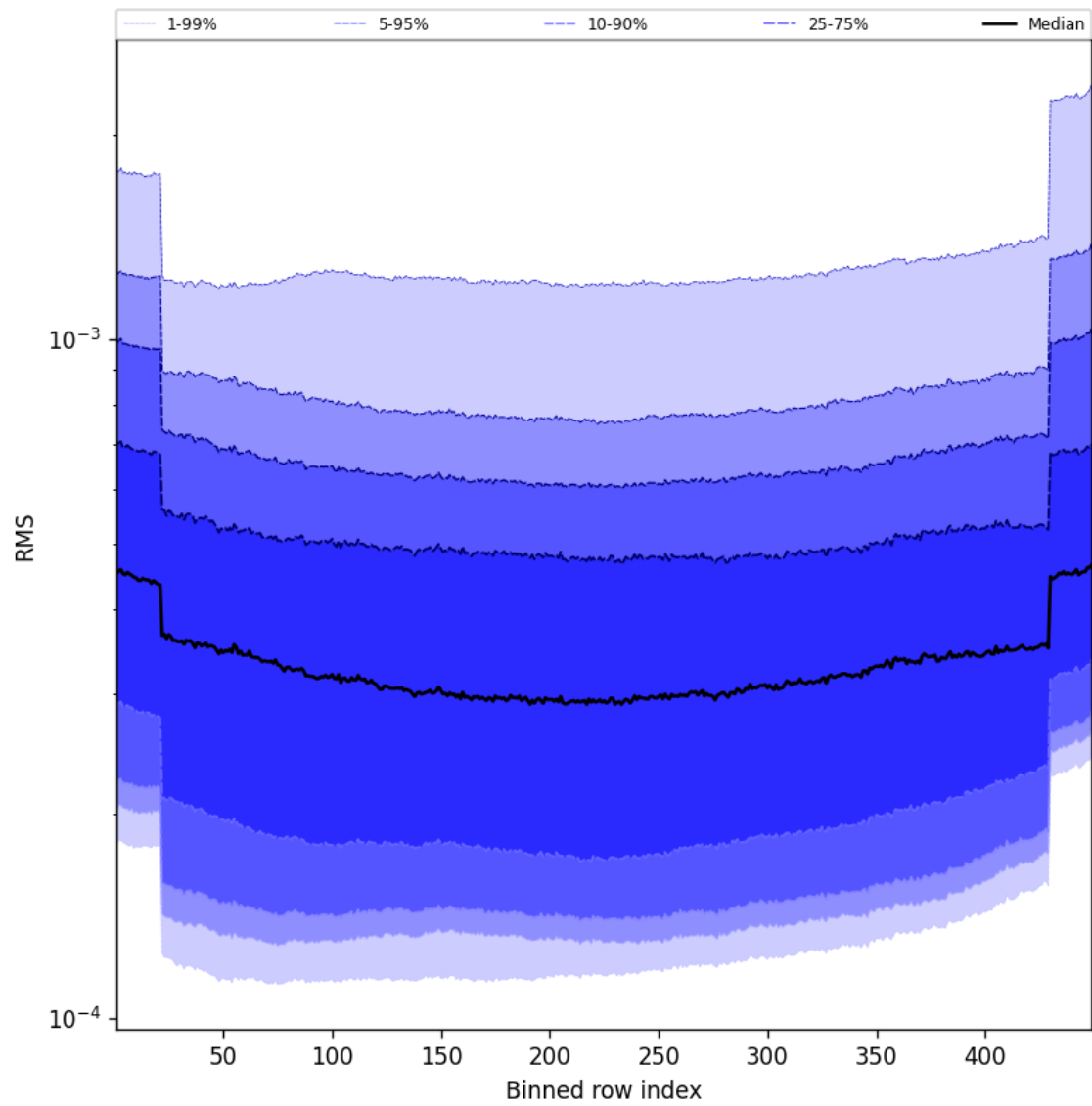
Figure 60: Along track statistics of “RMS” for 2025-01-02 to 2025-01-04
