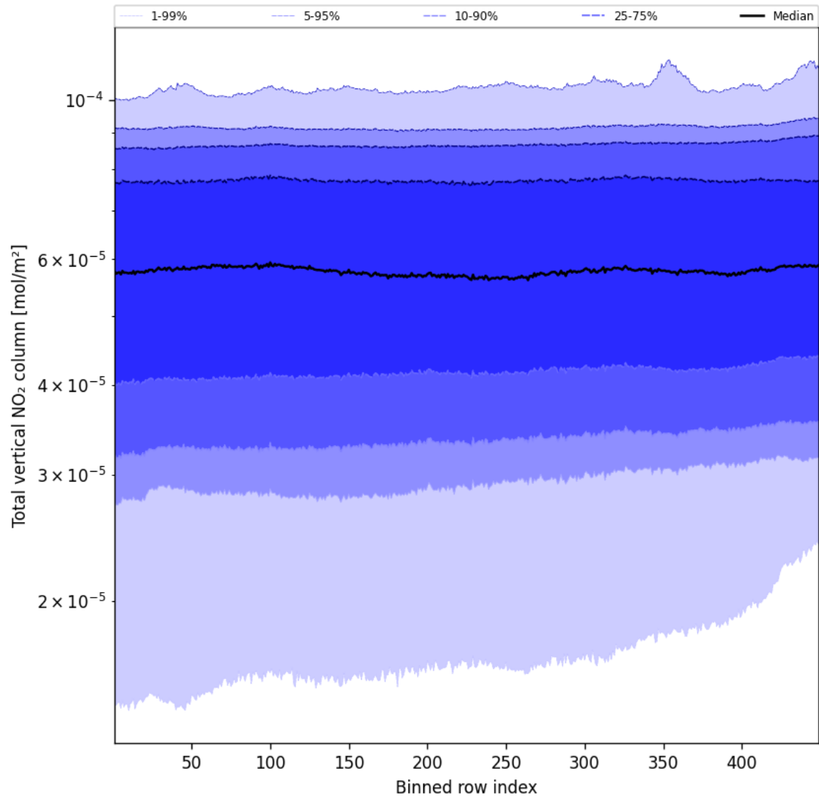
Figure 55: Along track statistics of “Total vertical NO 2 column” for 2025-01-02 to 2025-01-04
