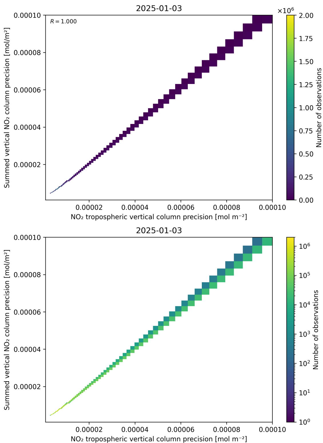
Figure 137: Scatter density plot of “NO 2 tropospheric vertical column precision” against “Summed vertical NO 2 column precision” for 2025-01-02 to 2025-01-04.
