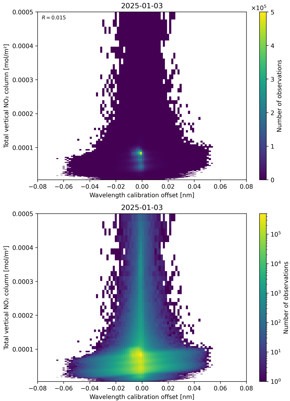
Figure 179: Scatter density plot of “Wavelength calibration offset” against “Total vertical NO 2 column” for 2025-01-02 to 2025-01-04.
