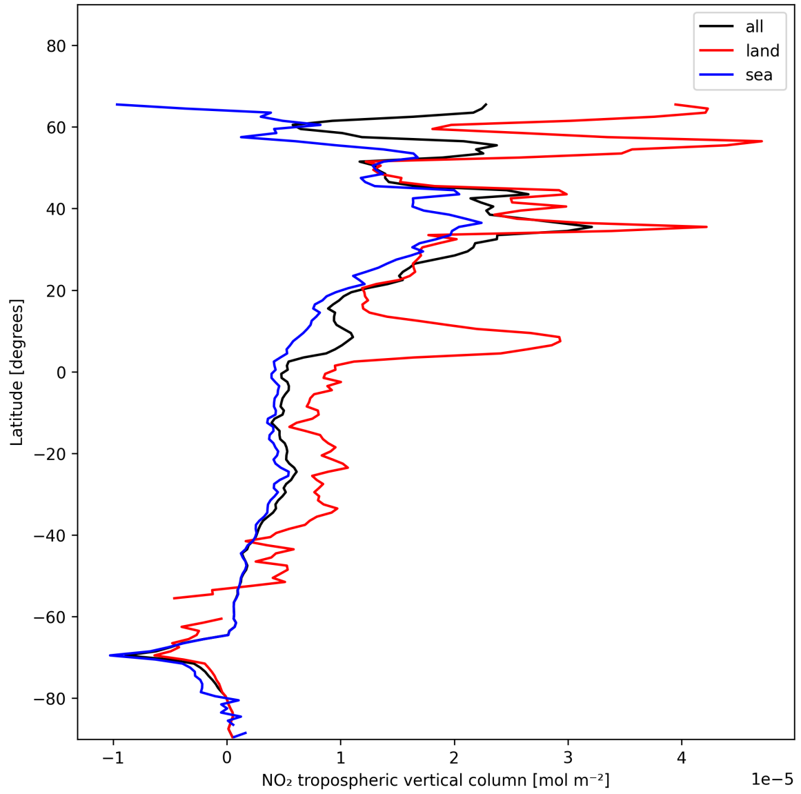
Figure 12: Zonal average of “NO 2 tropospheric vertical column” for 2025-01-02 to 2025-01-04.
