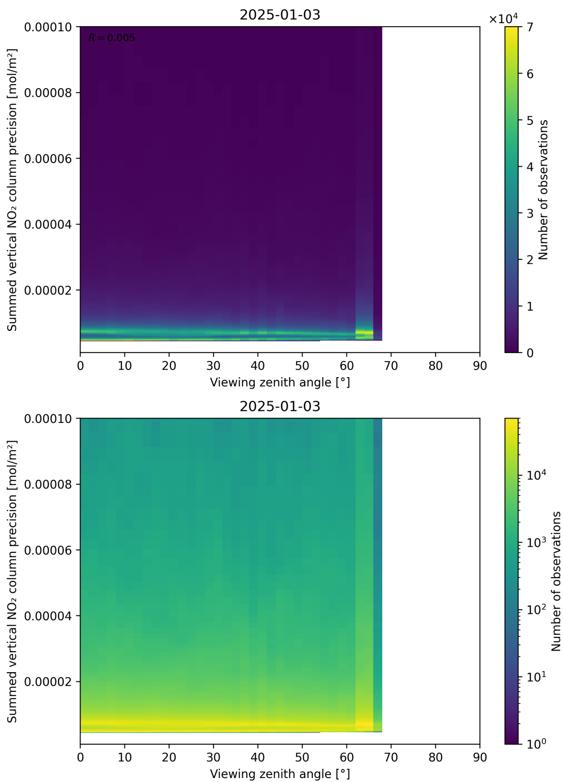
Figure 166: Scatter density plot of “Viewing zenith angle” against “Summed vertical NO 2 column precision” for 2025-01-02 to 2025-01-04.
