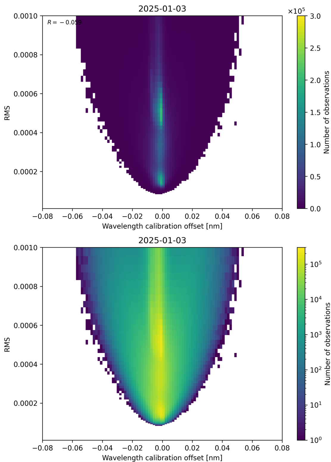
Figure 181: Scatter density plot of “Wavelength calibration offset” against “RMS” for 2025-01-02 to 2025-01-04.
