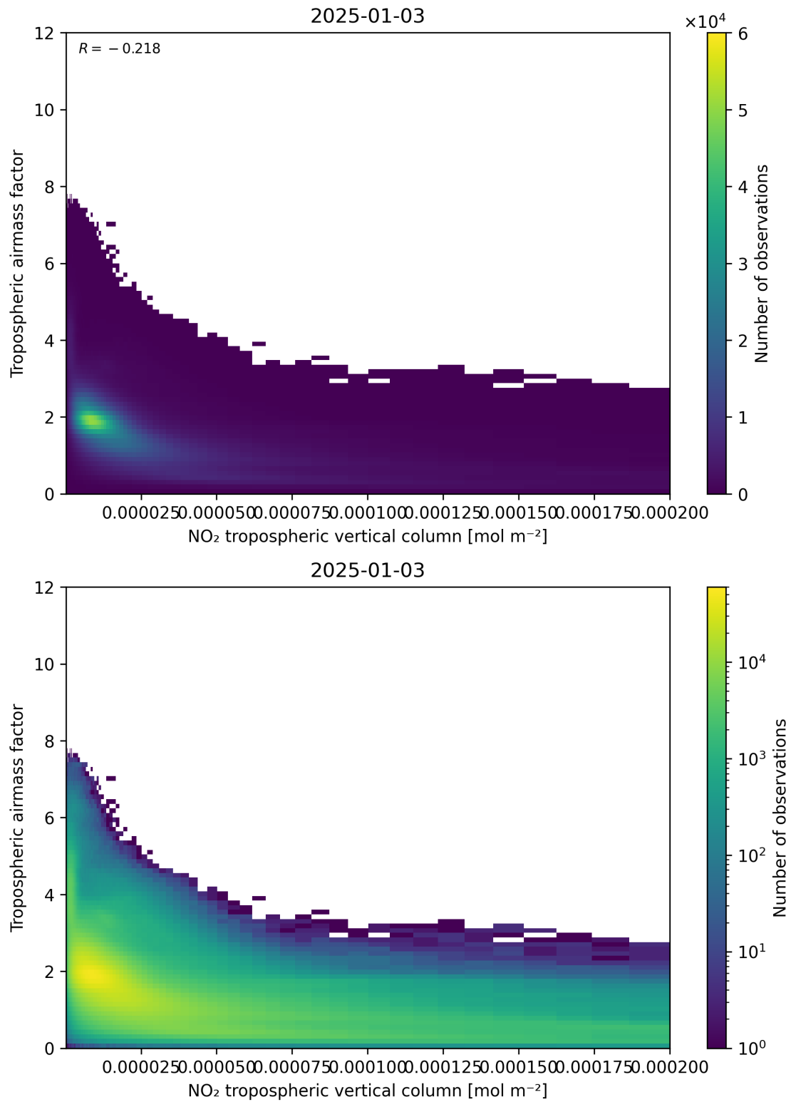
Figure 123: Scatter density plot of “NO 2 tropospheric vertical column” against “Tropospheric air mass factor” for 2025-01-02 to 2025-01-04.
