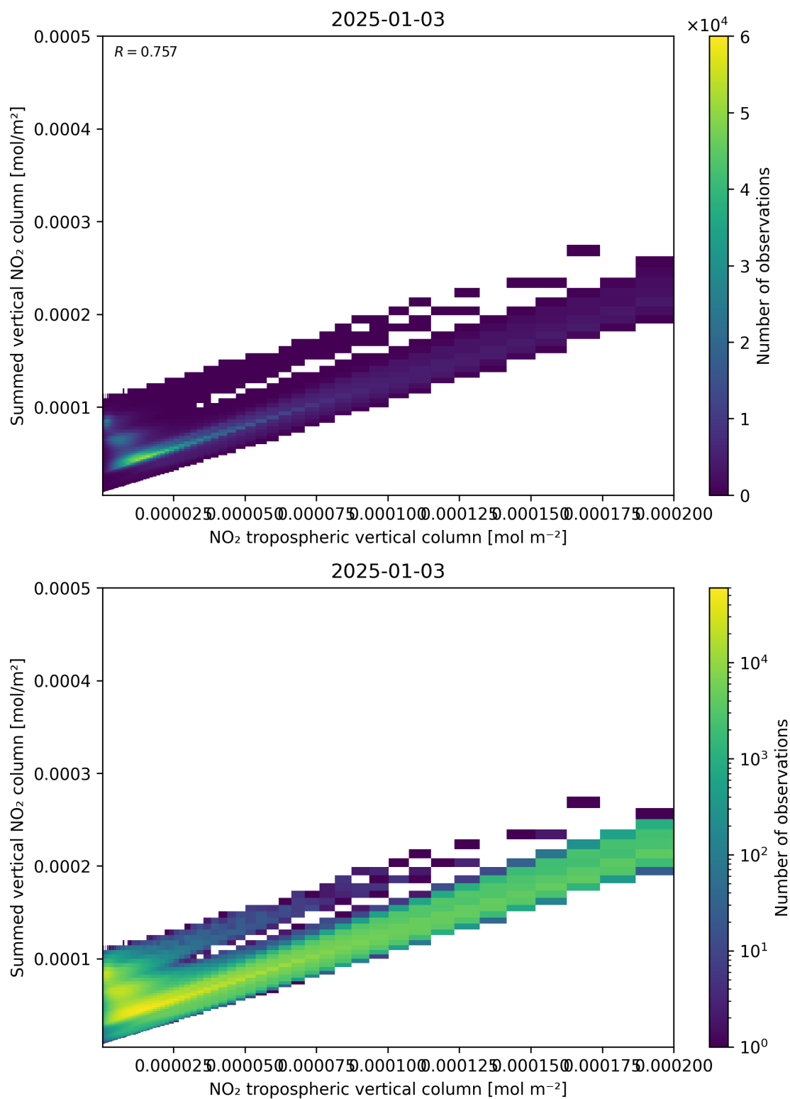
Figure 126: Scatter density plot of “NO 2 tropospheric vertical column” against “Summed vertical NO 2 column” for 2025-01-02 to 2025-01-04.
