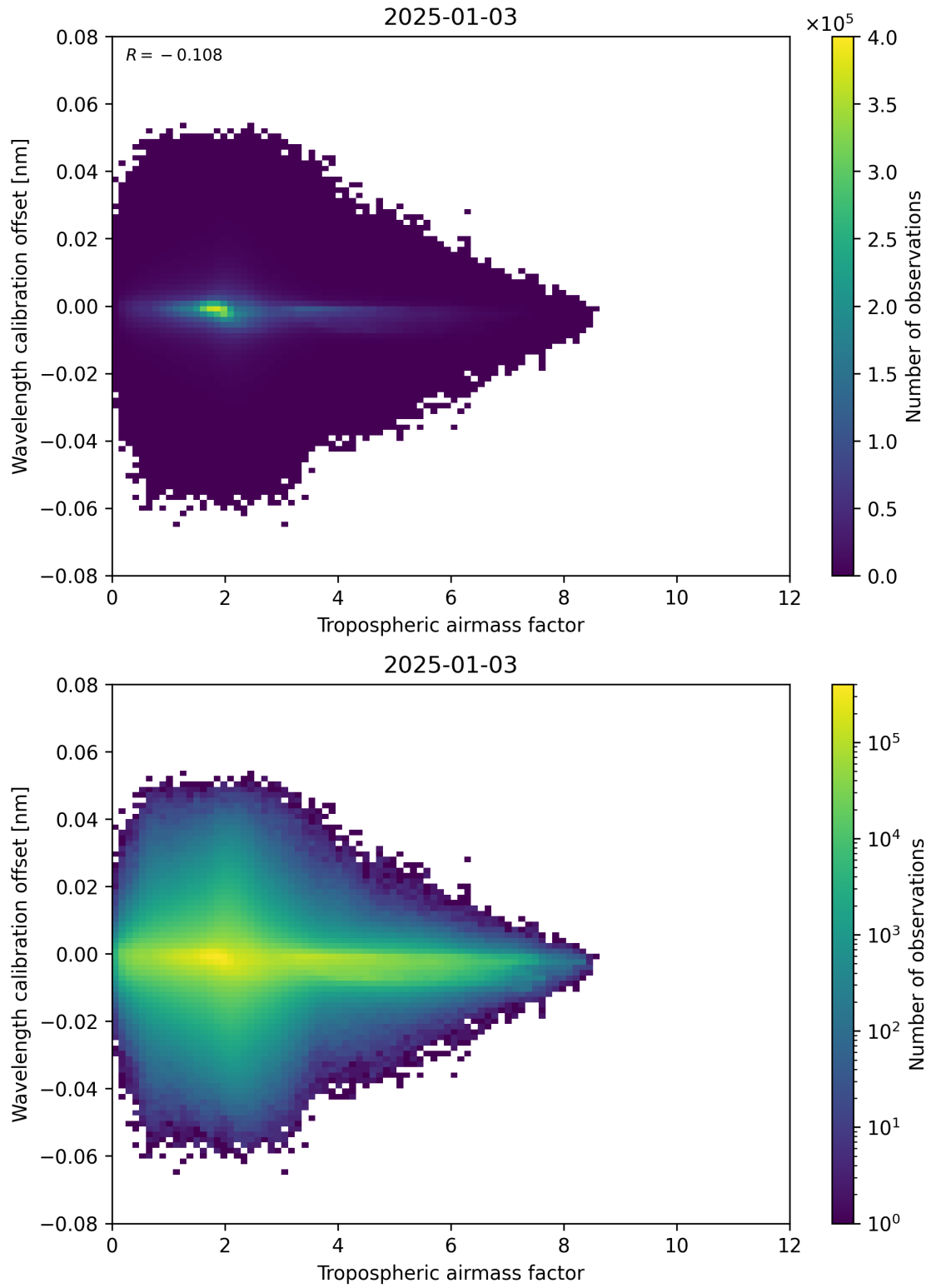
Figure 80: Scatter density plot of “Tropospheric airmass factor” against “Wavelength calibration offset” for 2025-01-02 to 2025-01-04.
