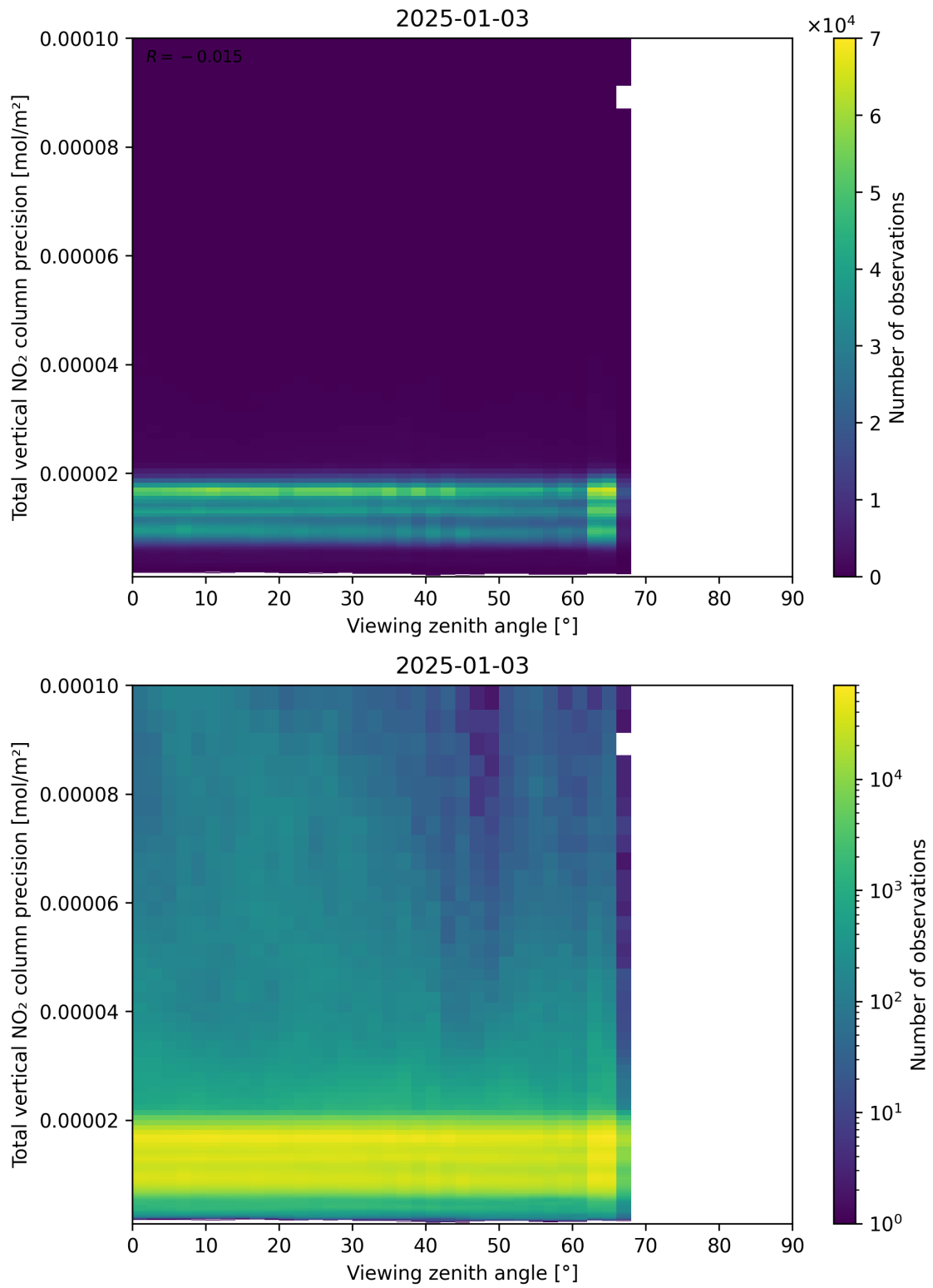
Figure 168: Scatter density plot of “Viewing zenith angle” against “Total vertical NO 2 column precision” for 2025-01-02 to 2025-01-04.
