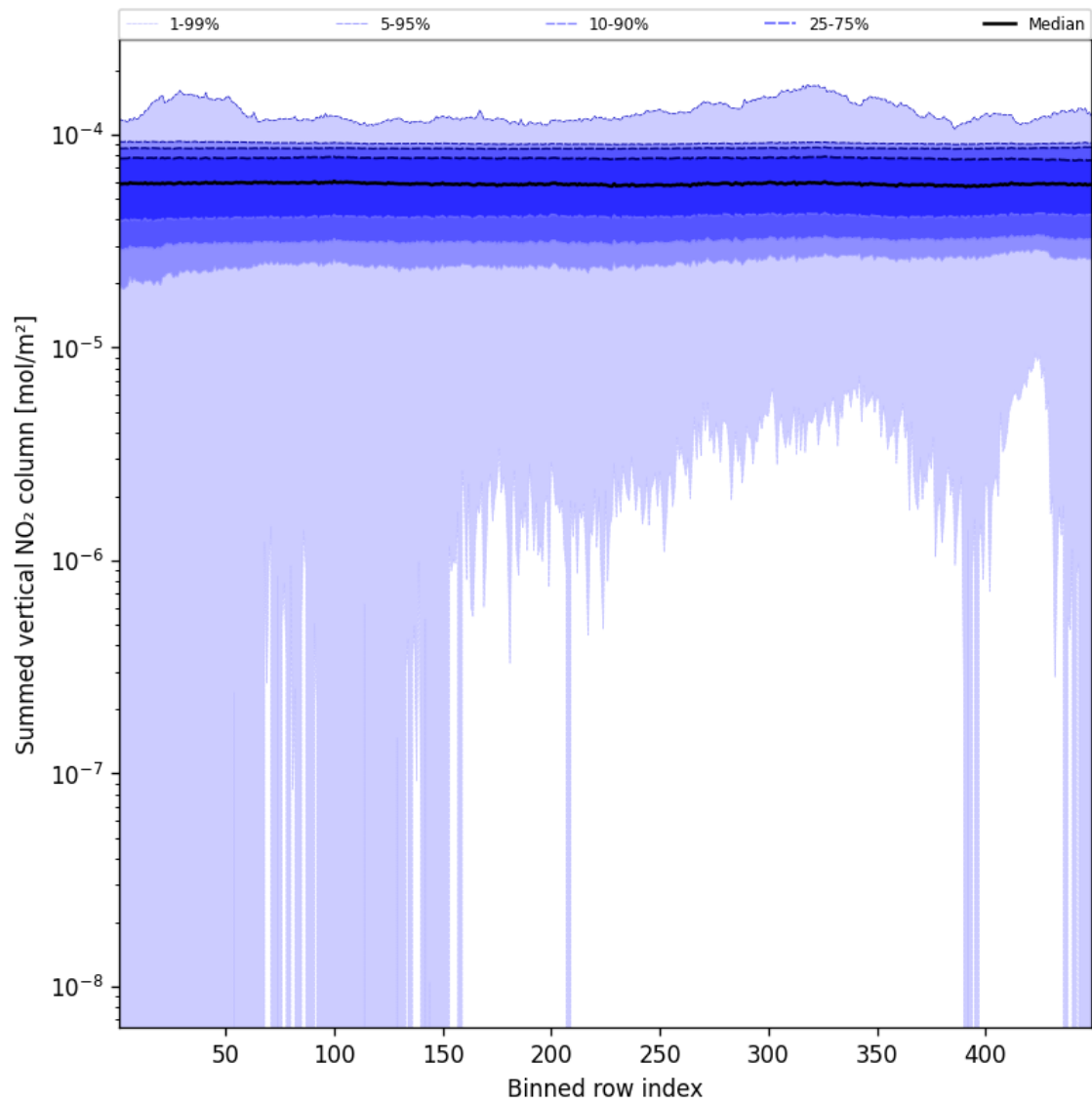
Figure 57: Along track statistics of “Summed vertical NO 2 column” for 2025-01-02 to 2025-01-04
