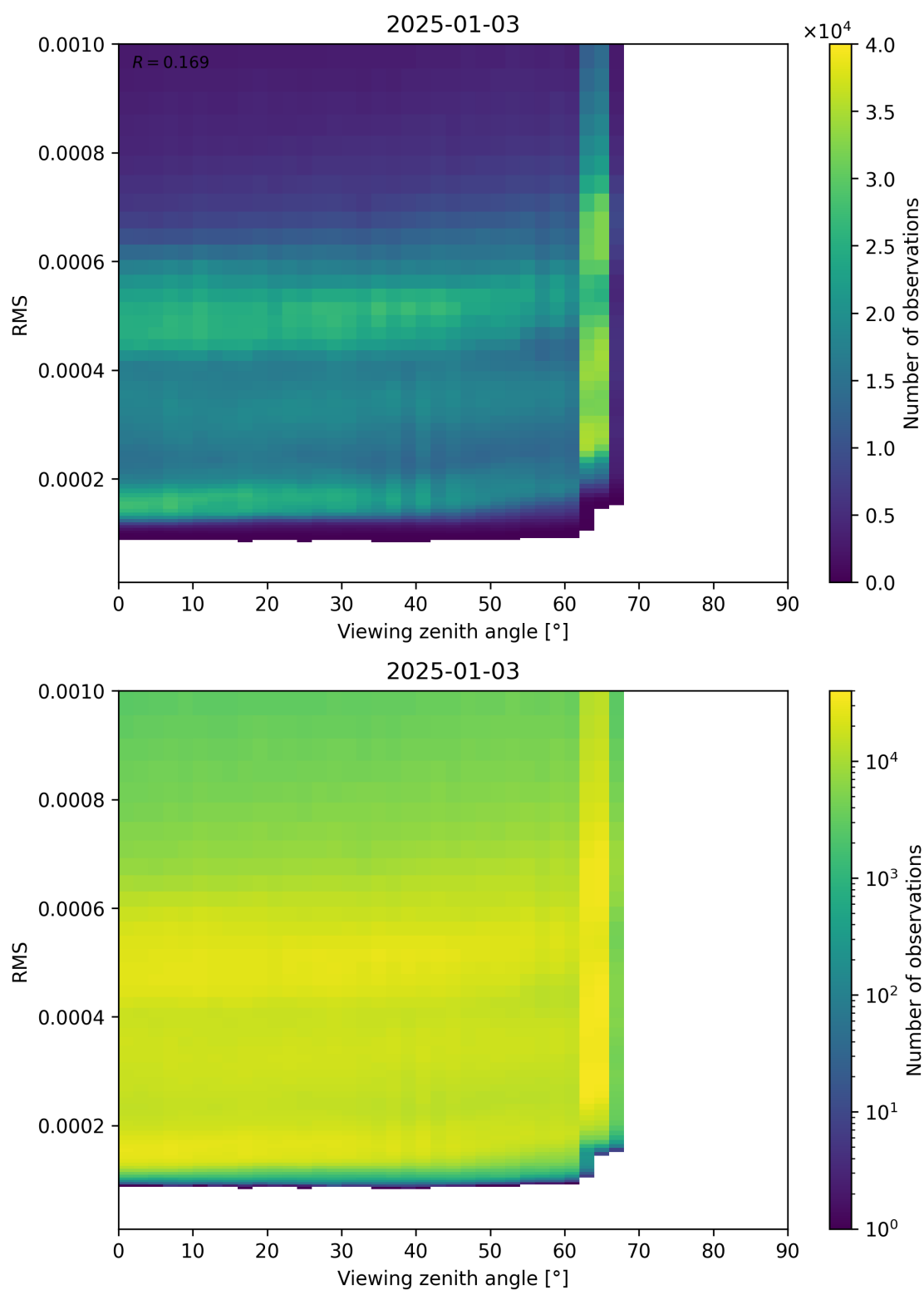
Figure 171: Scatter density plot of “Viewing zenith angle” against “RMS” for 2025-01-02 to 2025-01-04.
