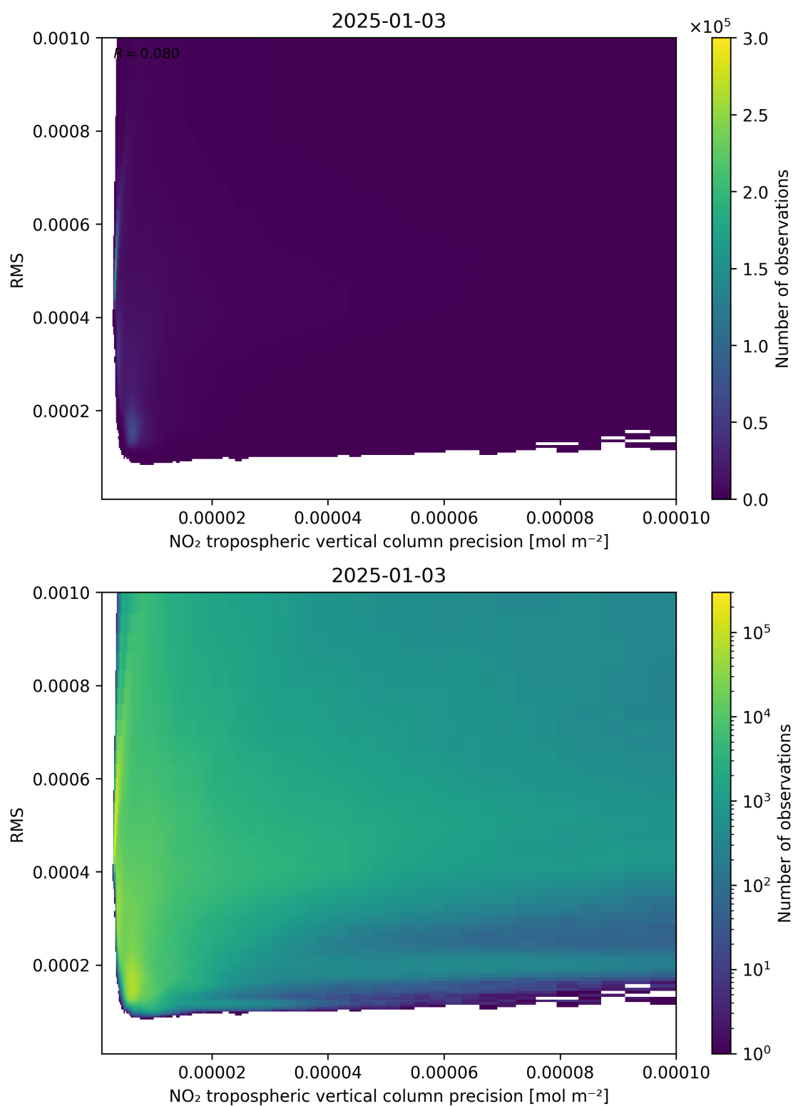
Figure 140: Scatter density plot of “NO 2 tropospheric vertical column precision” against “RMS” for 2025-01-02 to 2025-01-04.
