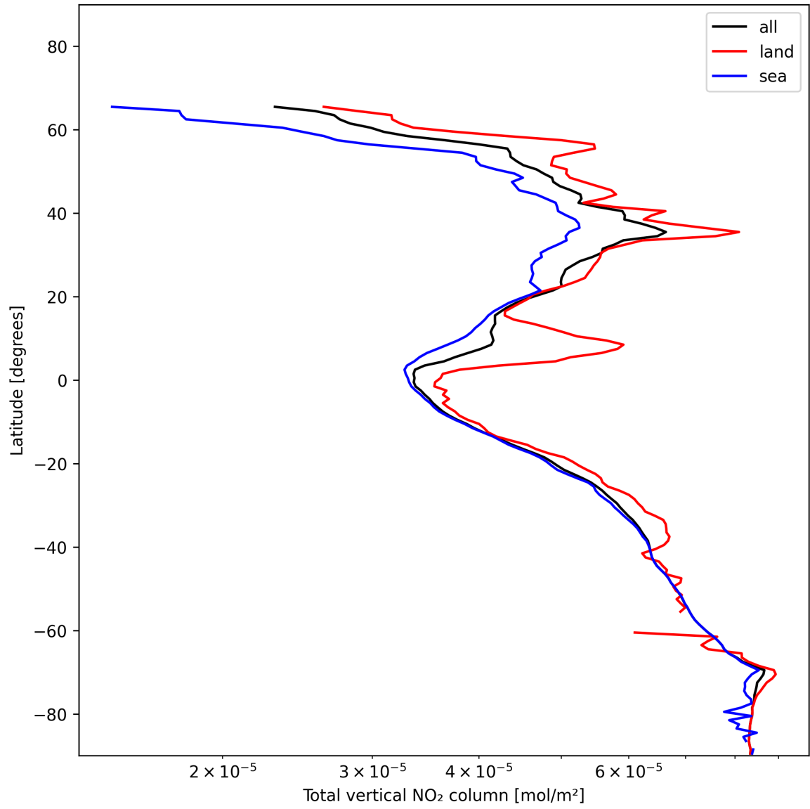
Figure 21: Zonal average of “Total vertical NO 2 column” for 2025-01-02 to 2025-01-04.
