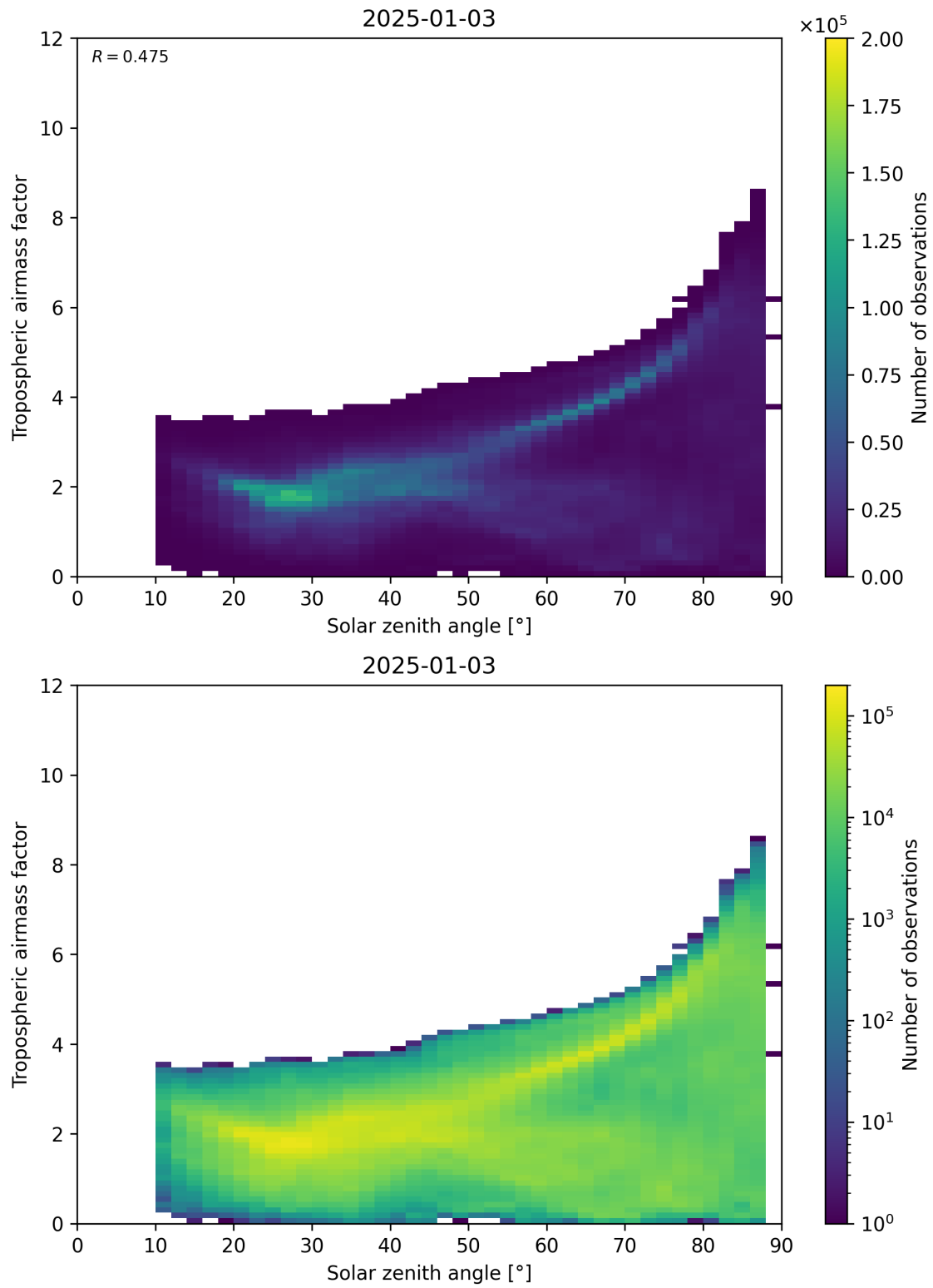
Figure 147: Scatter density plot of “Solar zenith angle” against “Tropospheric airmass factor” for 2025-01-02 to 2025-01-04.
