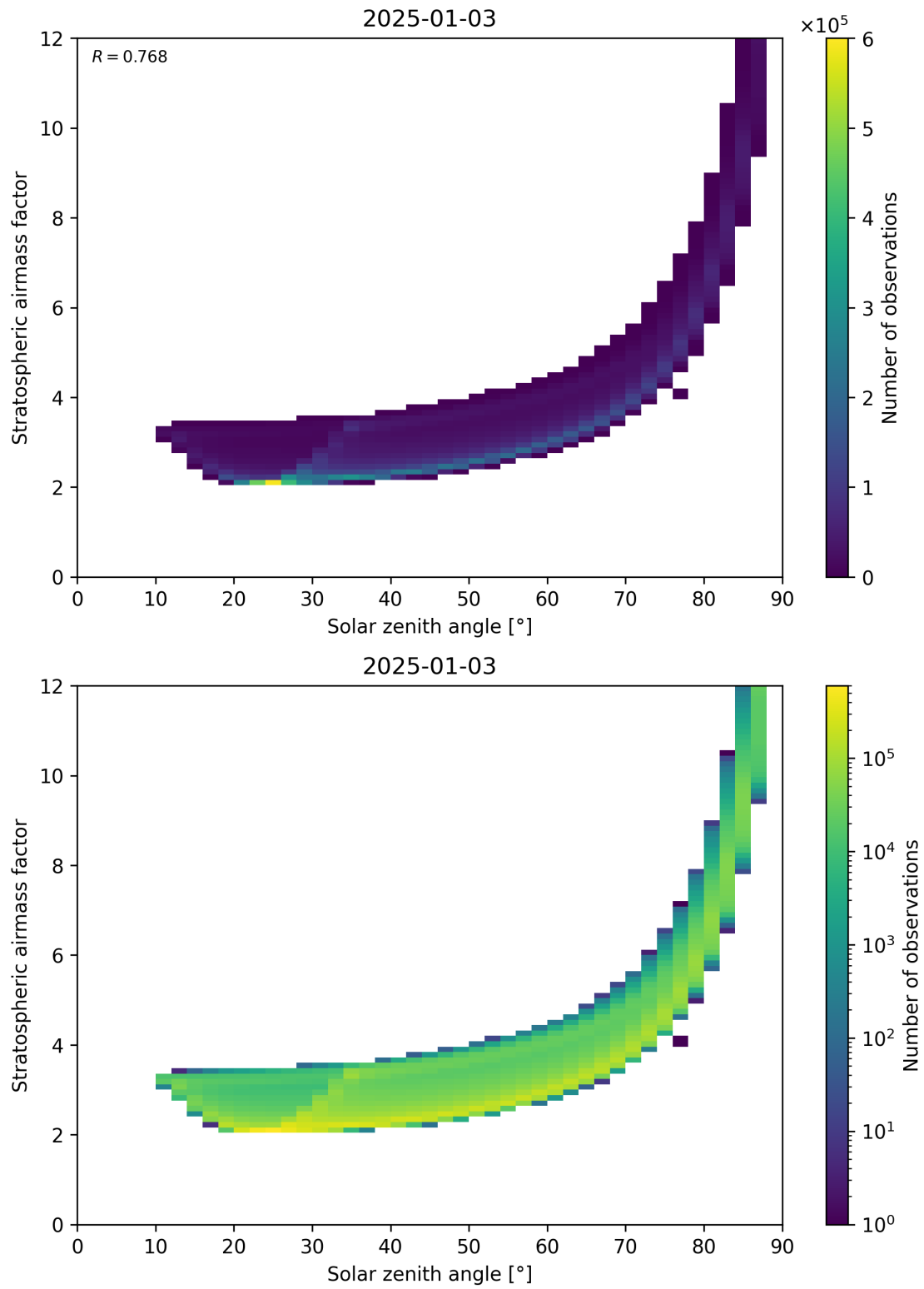
Figure 145: Scatter density plot of “Solar zenith angle” against “Stratospheric airmass factor” for 2025-01-02 to 2025-01-04.
