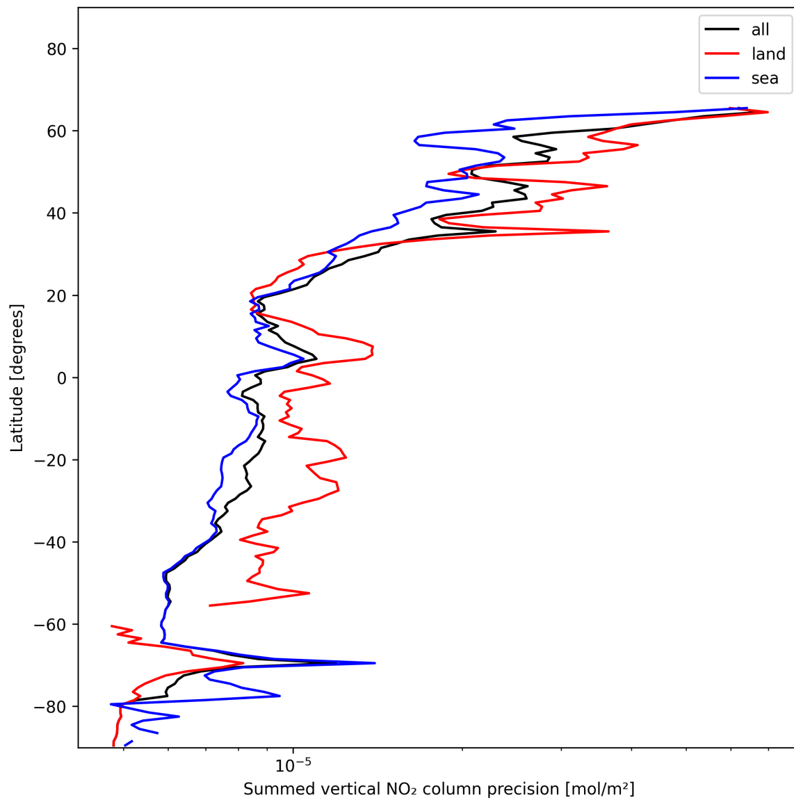
Figure 24: Zonal average of “Summed vertical NO 2 column precision” for 2025-01-02 to 2025-01-04.
