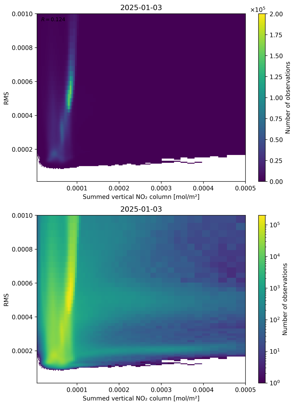
Figure 109: Scatter density plot of “Summed vertical NO 2 column” against “RMS” for 2025-01-02 to 2025-01-04.
