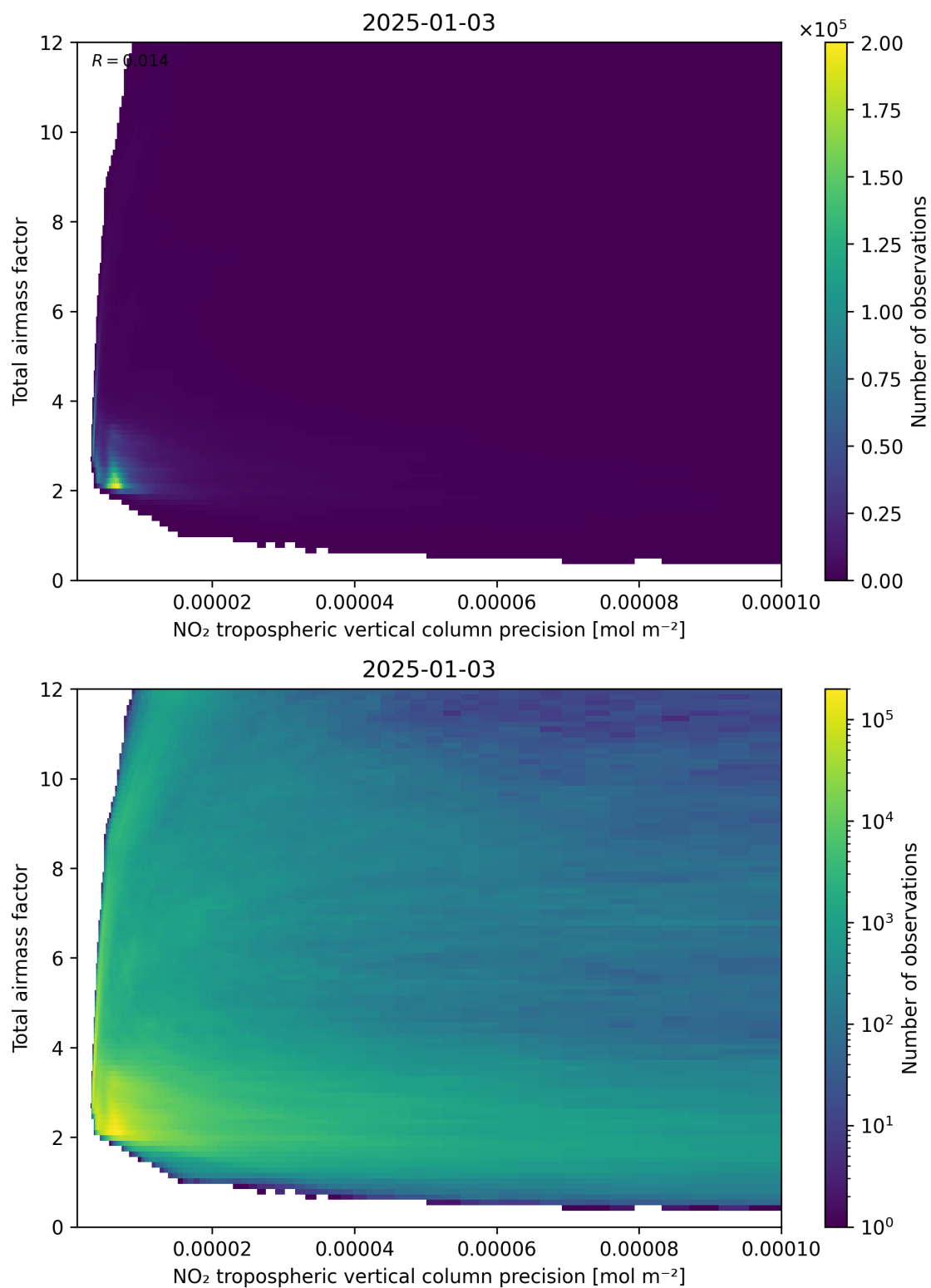
Figure 132: Scatter density plot of “NO 2 tropospheric vertical column precision” against “Total air mass factor” for 2025-01-02 to 2025-01-04.
