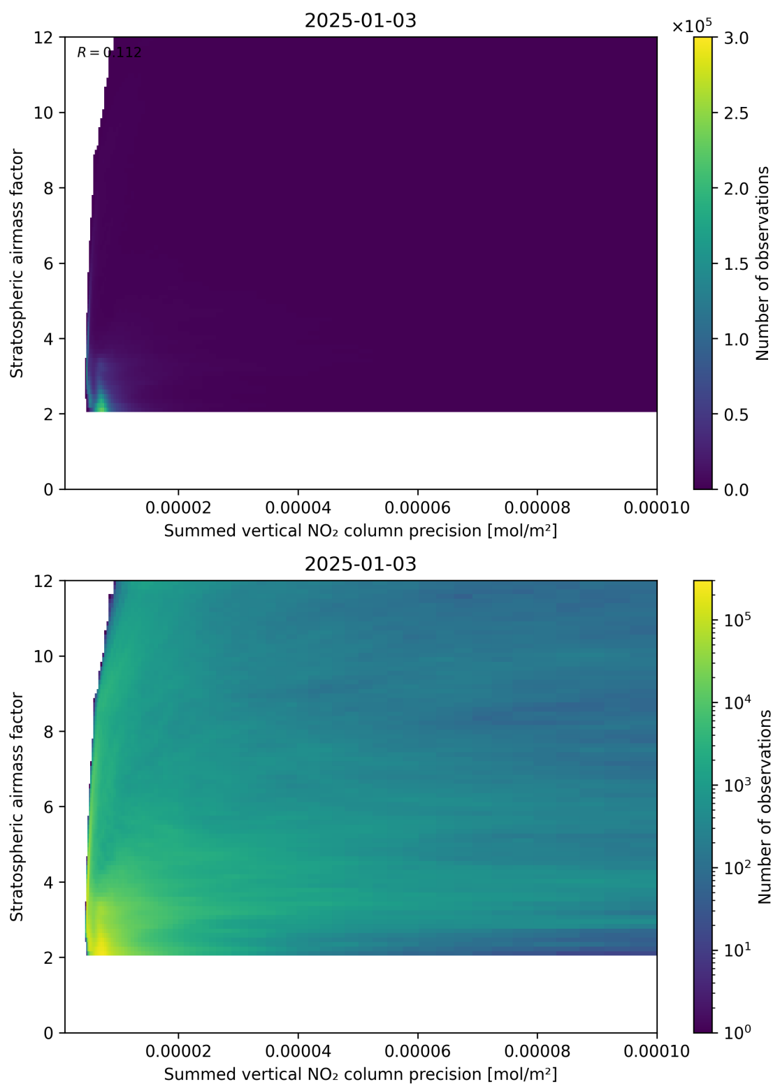
Figure 106: Scatter density plot of “Summed vertical NO 2 column precision” against “Stratospheric airmass factor” for 2025-01-02 to 2025-01-04.
