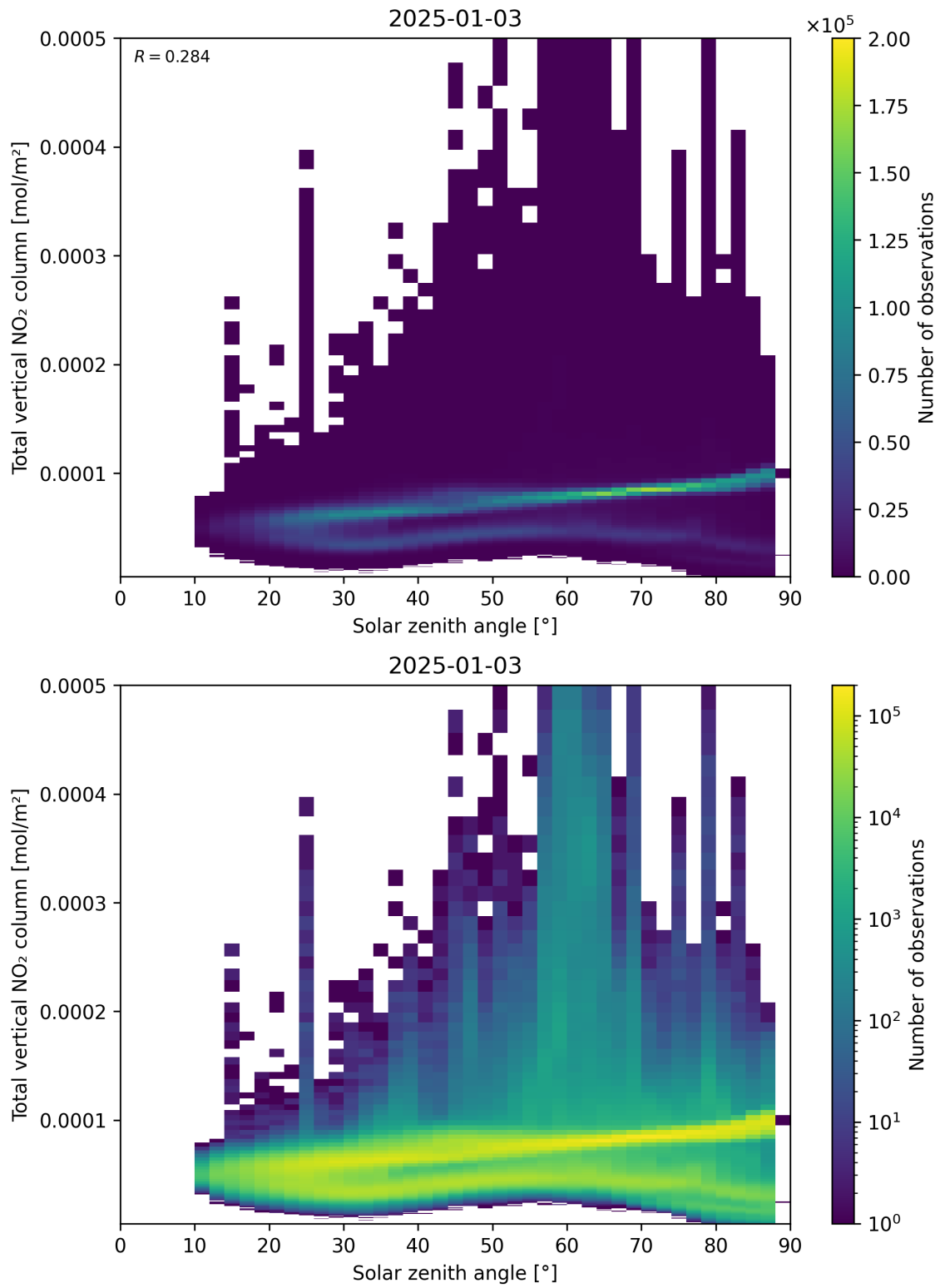
Figure 153: Scatter density plot of “Solar zenith angle” against “Total vertical NO 2 column” for 2025-01-02 to 2025-01-04.
