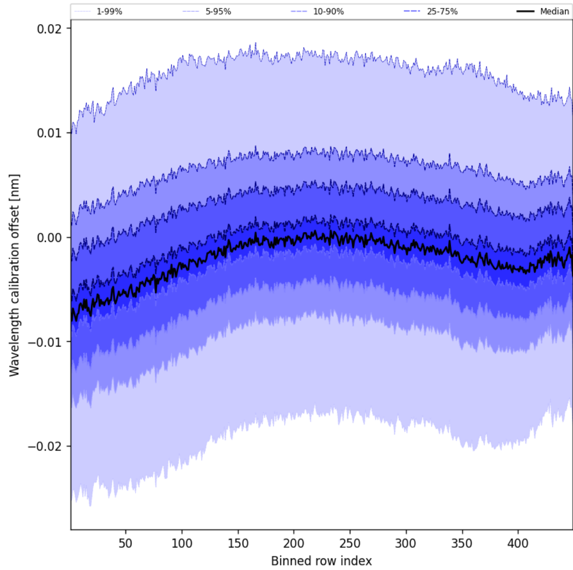
Figure 52: Along track statistics of “Wavelength calibration offset” for 2025-01-02 to 2025-01-04
