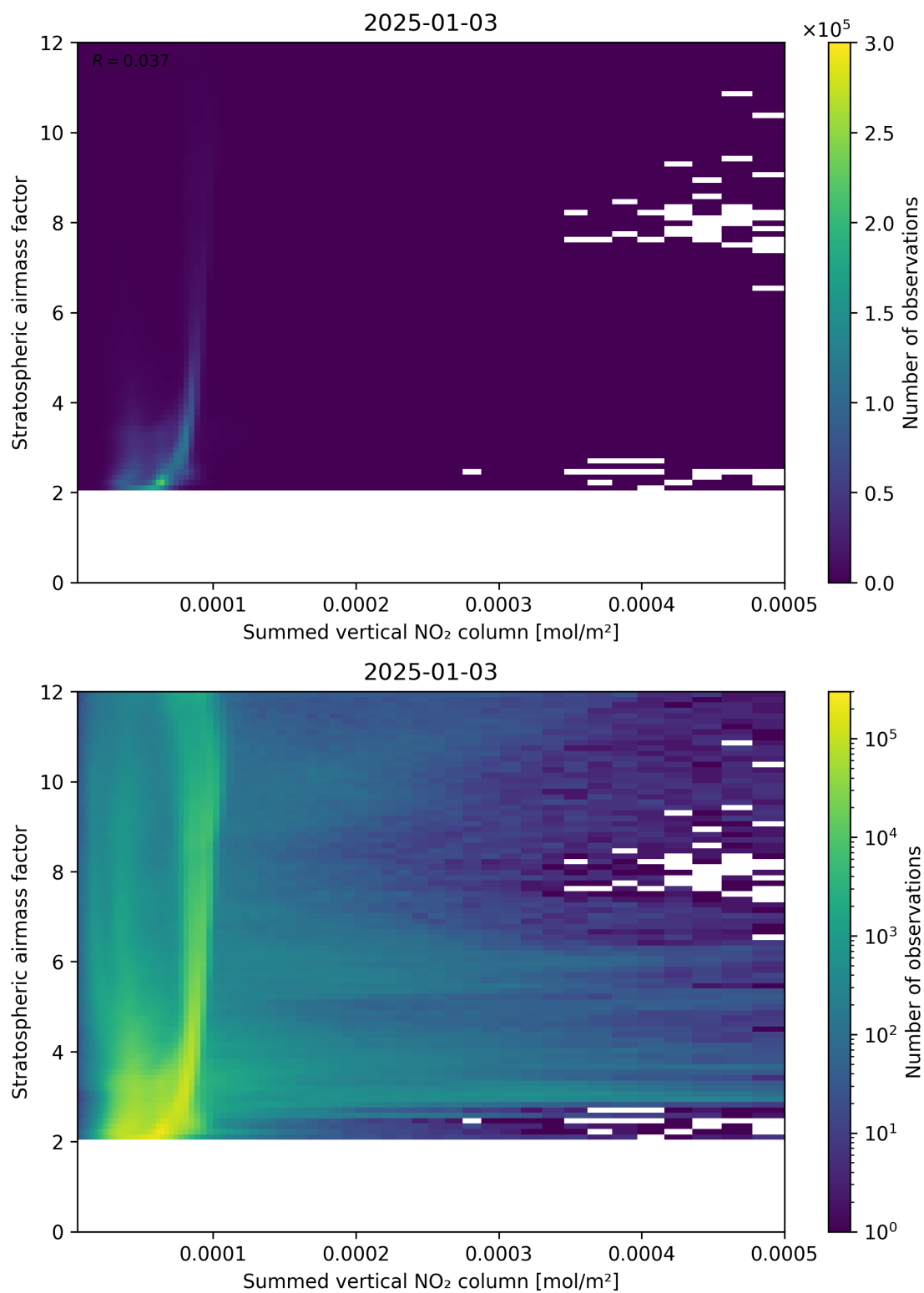
Figure 103: Scatter density plot of “Summed vertical NO 2 column” against “Stratospheric airmass factor” for 2025-01-02 to 2025-01-04.
