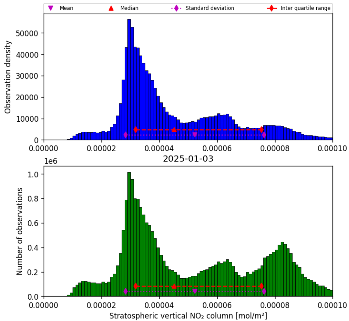
Figure 36: Histogram of “Stratospheric vertical NO 2 column” for 2025-01-02 to 2025-01-04
