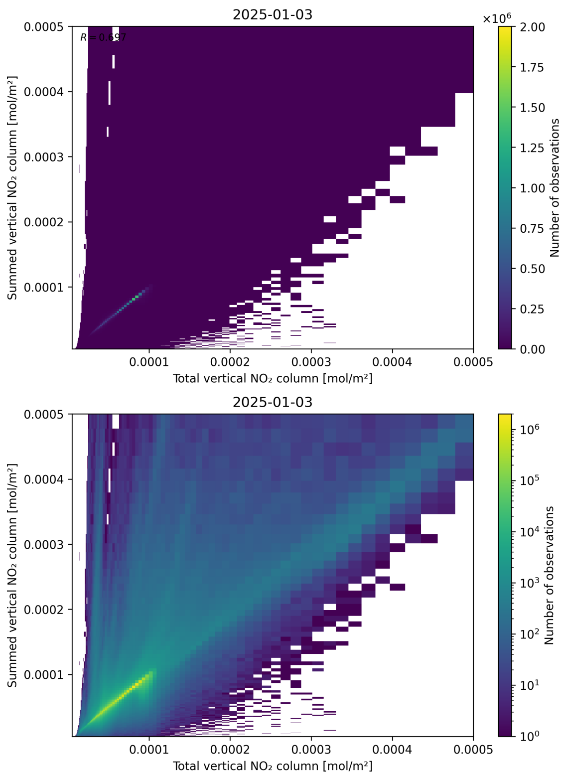
Figure 112: Scatter density plot of “Total vertical NO 2 column” against “Summed vertical NO 2 column” for 2025-01-02 to 2025-01-04.
