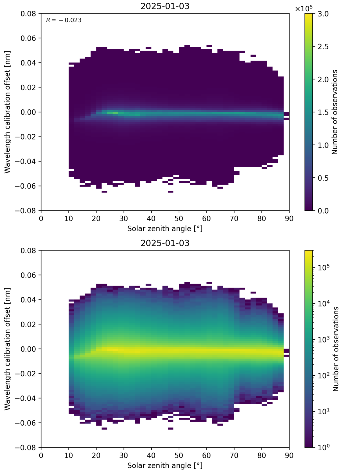
Figure 158: Scatter density plot of “Solar zenith angle” against “Wavelength calibration offset” for 2025-01-02 to 2025-01-04.
