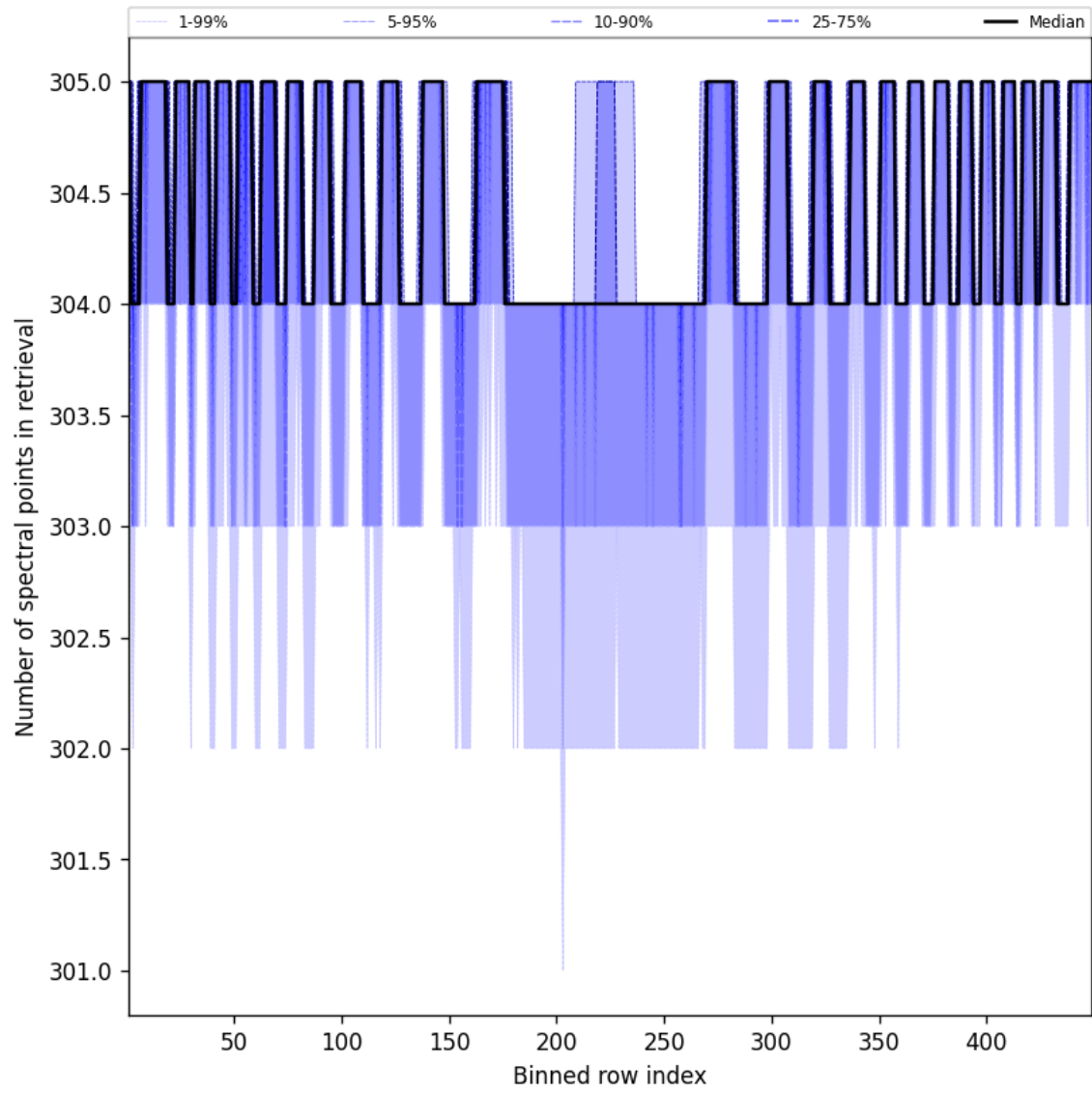
Figure 50: Along track statistics of “Number of spectral points in retrieval” for 2025-01-02 to 2025-01-04
