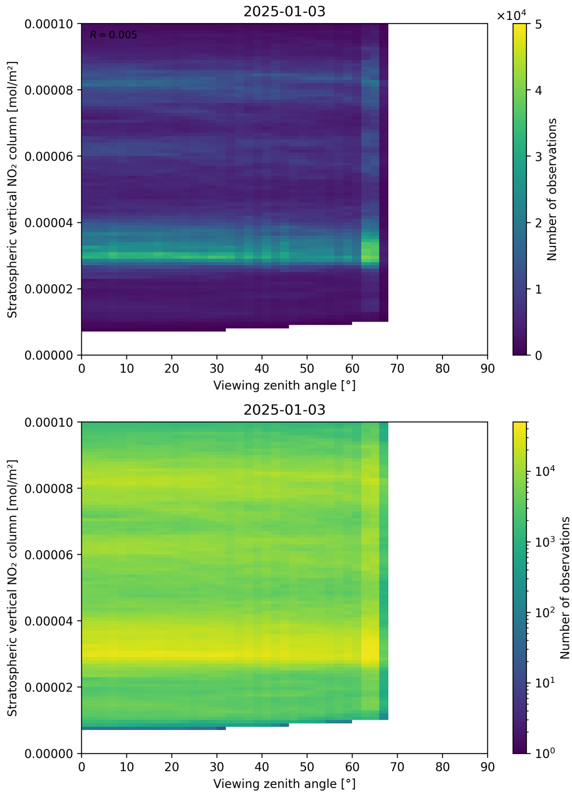
Figure 164: Scatter density plot of “Viewing zenith angle” against “Stratospheric vertical NO 2 column” for 2025-01-02 to 2025-01-04.
