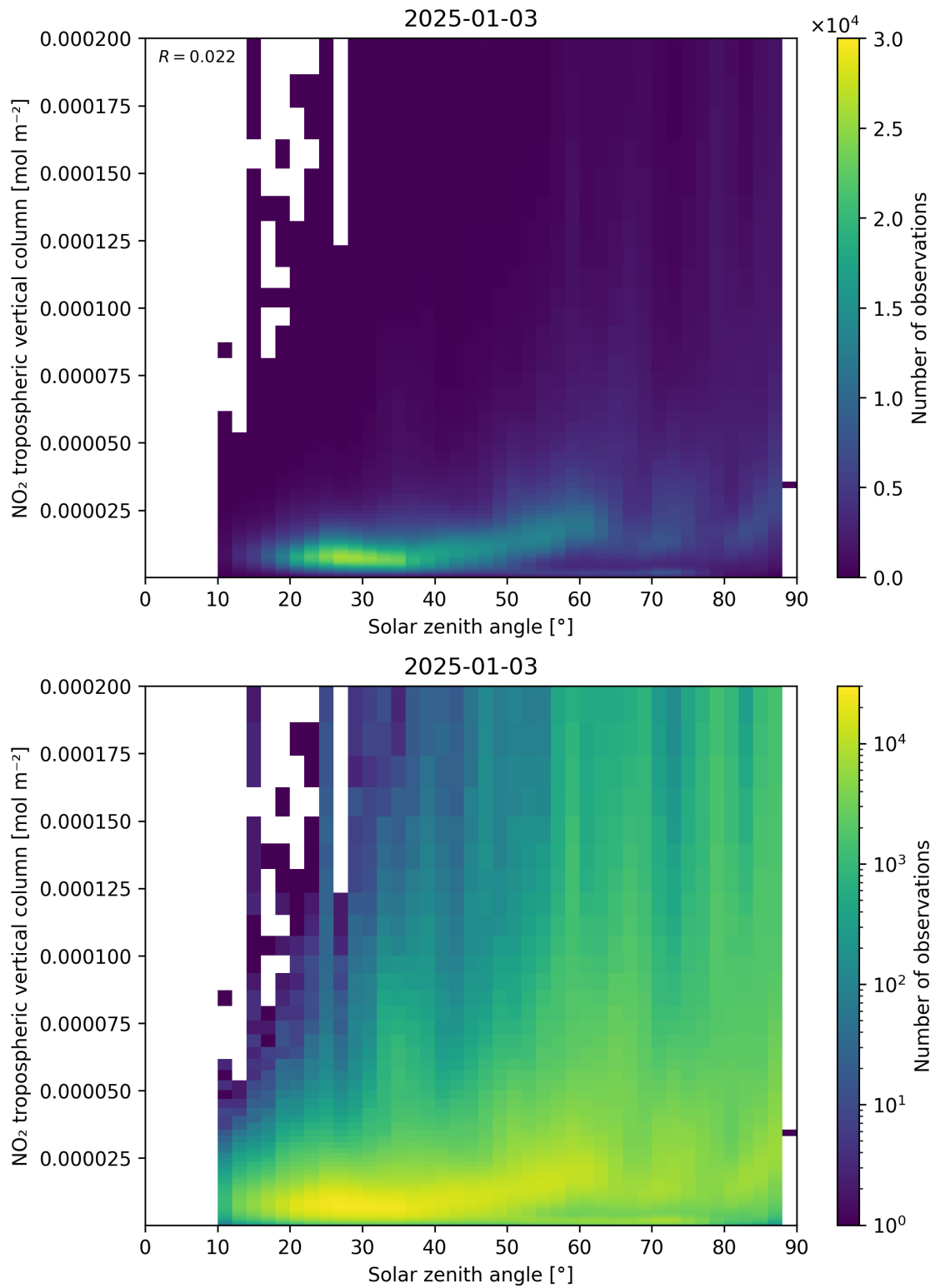
Figure 155: Scatter density plot of “Solar zenith angle” against “NO 2 tropospheric vertical column” for 2025-01-02 to 2025-01-04.
