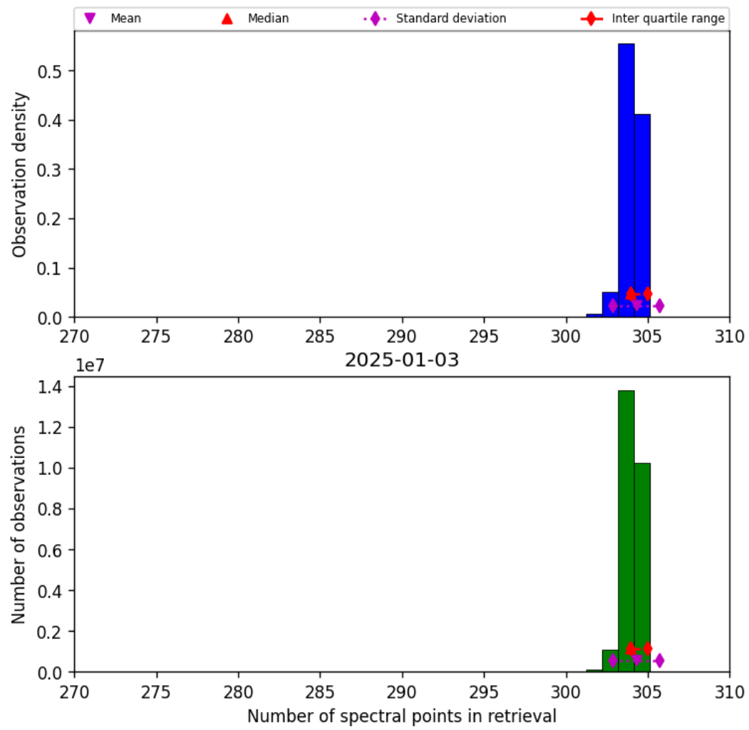
Figure 33: Histogram of “Number of spectral points in retrieval” for 2025-01-02 to 2025-01-04
