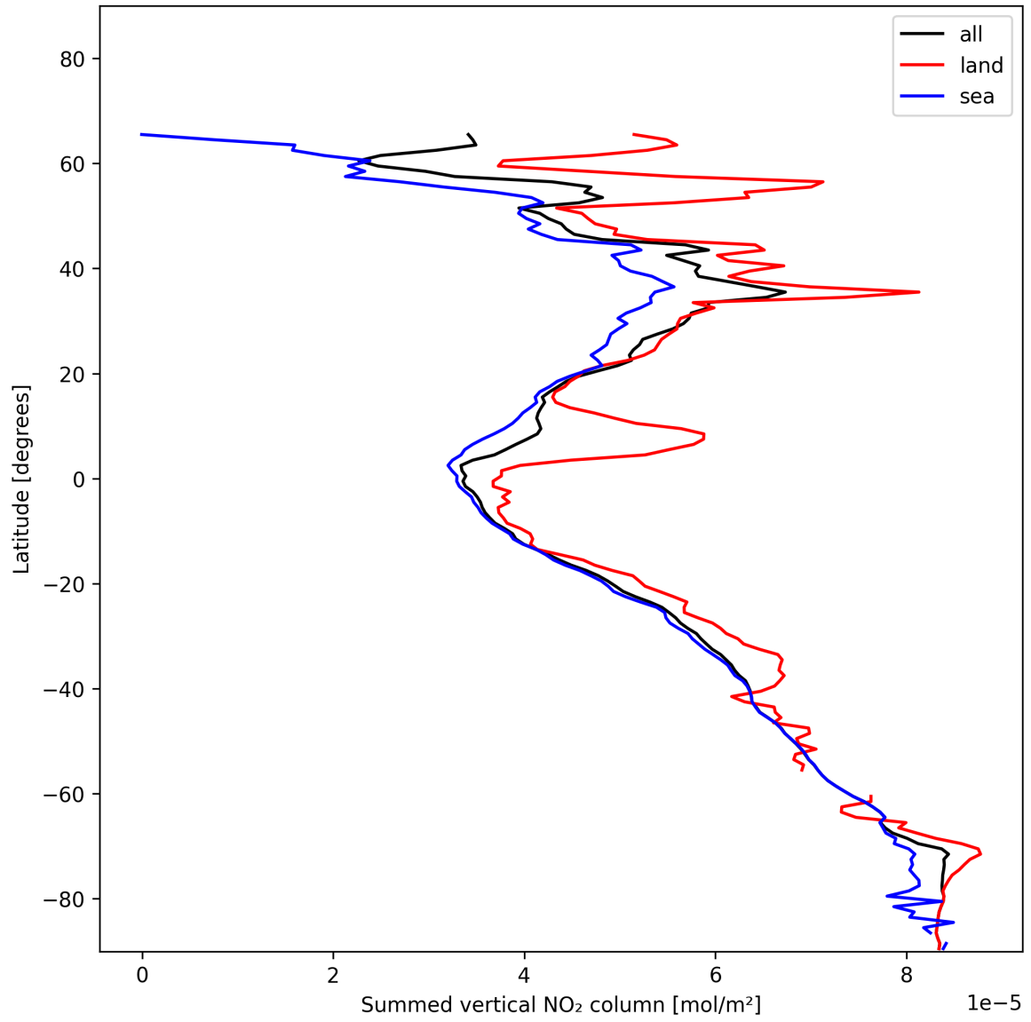
Figure 23: Zonal average of “Summed vertical NO 2 column” for 2025-01-02 to 2025-01-04.
