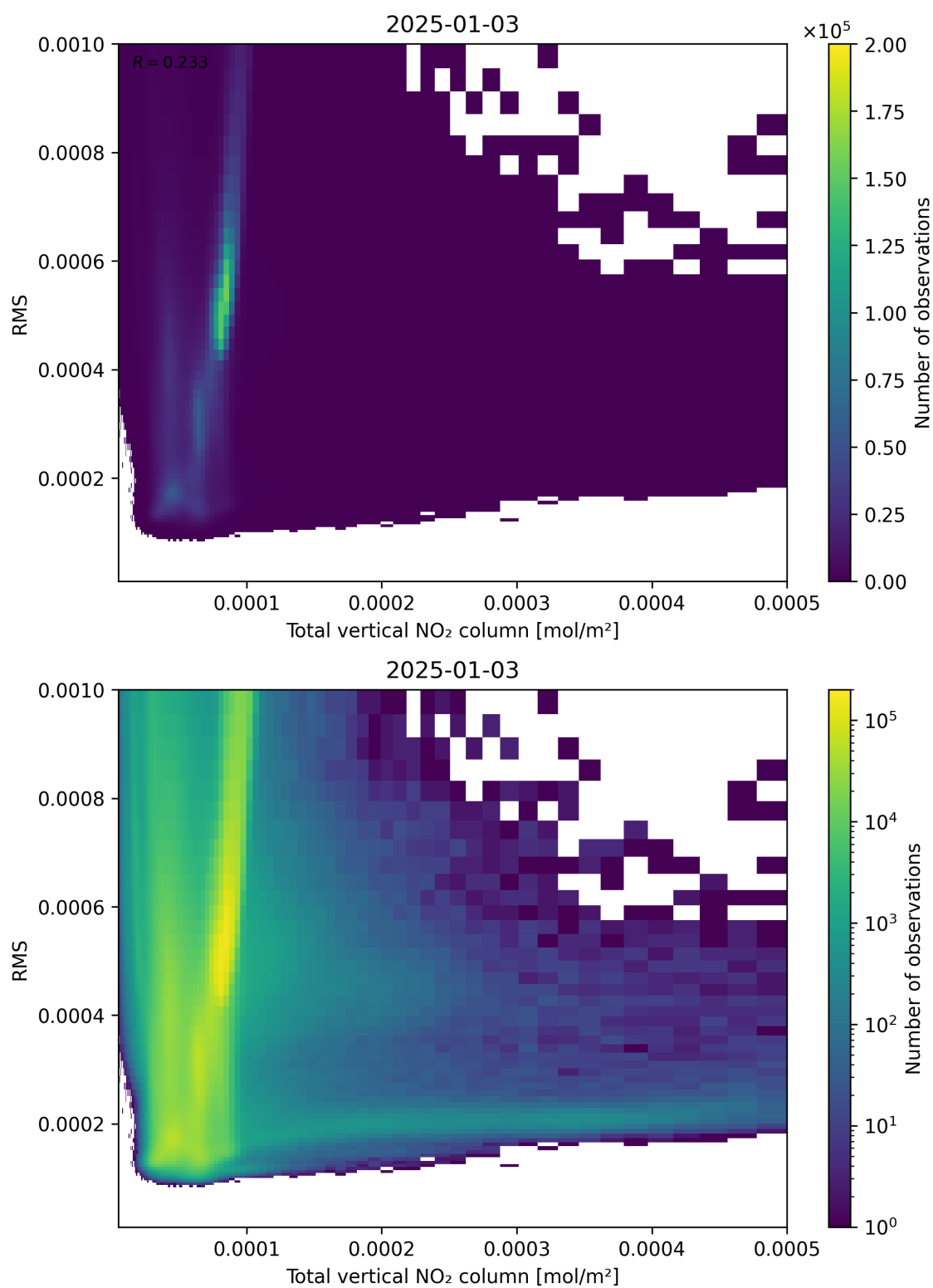
Figure 120: Scatter density plot of “Total vertical NO 2 column” against “RMS” for 2025-01-02 to 2025-01-04.
