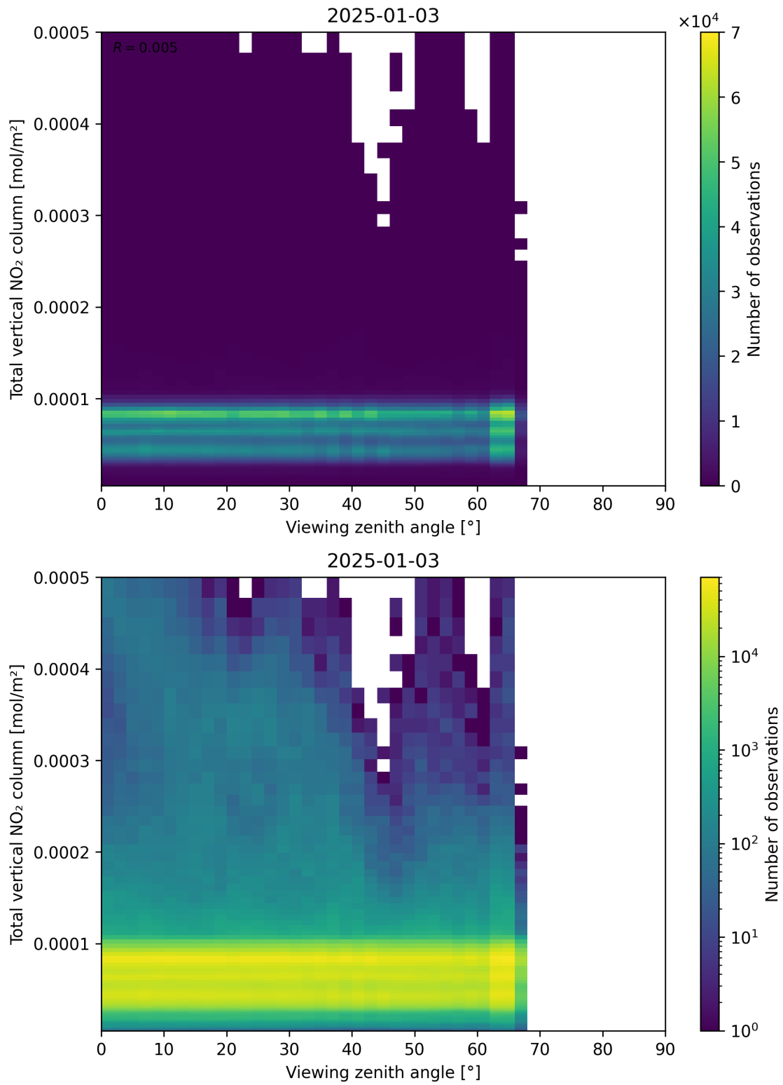
Figure 167: Scatter density plot of “Viewing zenith angle” against “Total vertical NO 2 column” for 2025-01-02 to 2025-01-04.
