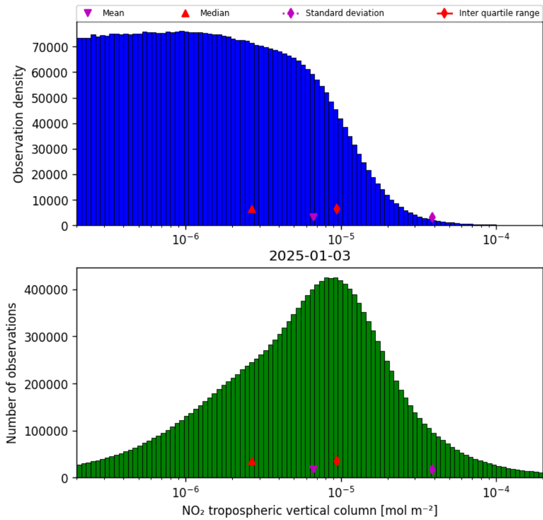
Figure 29: Histogram of “NO 2 tropospheric vertical column” for 2025-01-02 to 2025-01-04
