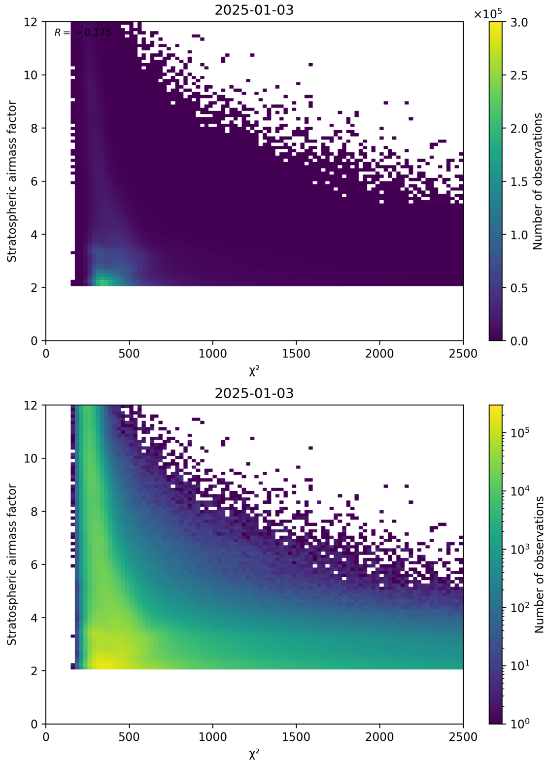
Figure 81: Scatter density plot of “ \chi^2 ” against “Stratospheric airmass factor” for 2025-01-02 to 2025-01-04.
