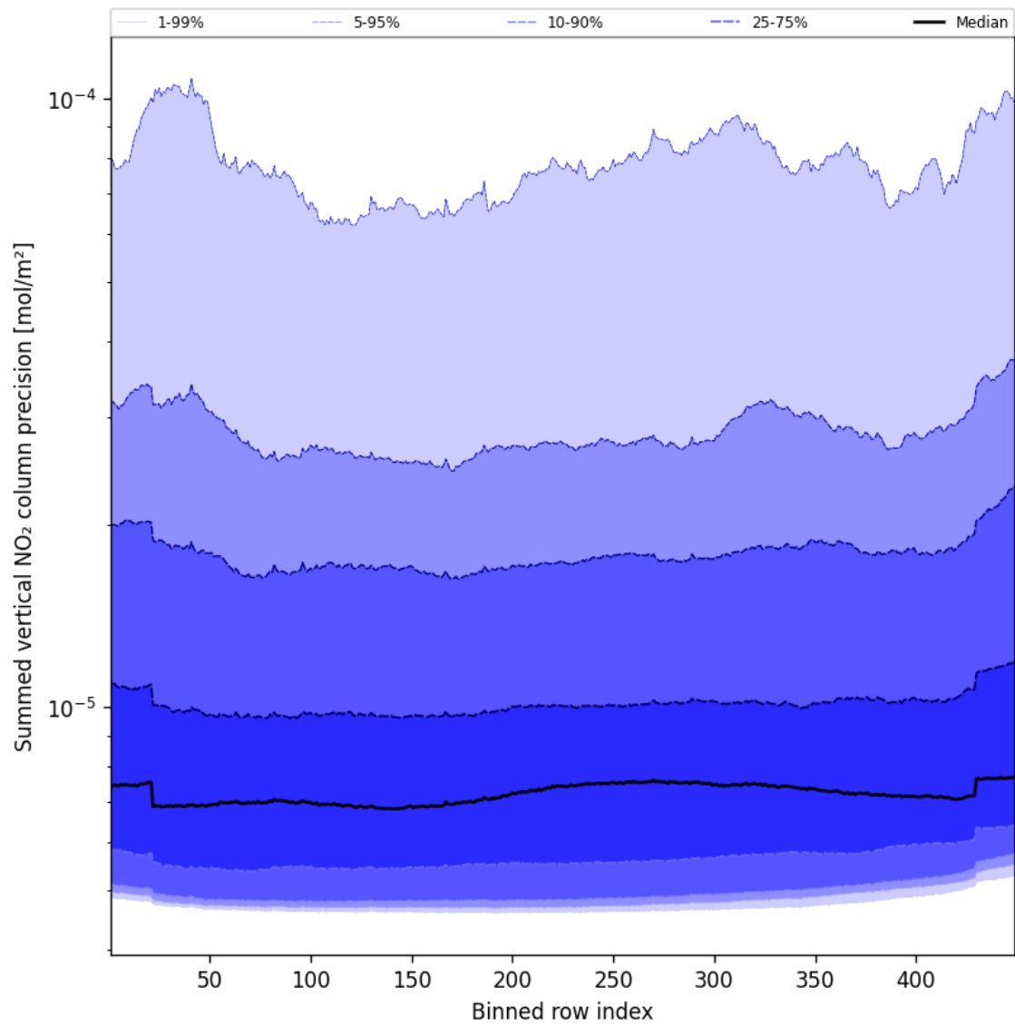
Figure 58: Along track statistics of “Summed vertical NO 2 column precision” for 2025-01-02 to 2025-01-04
