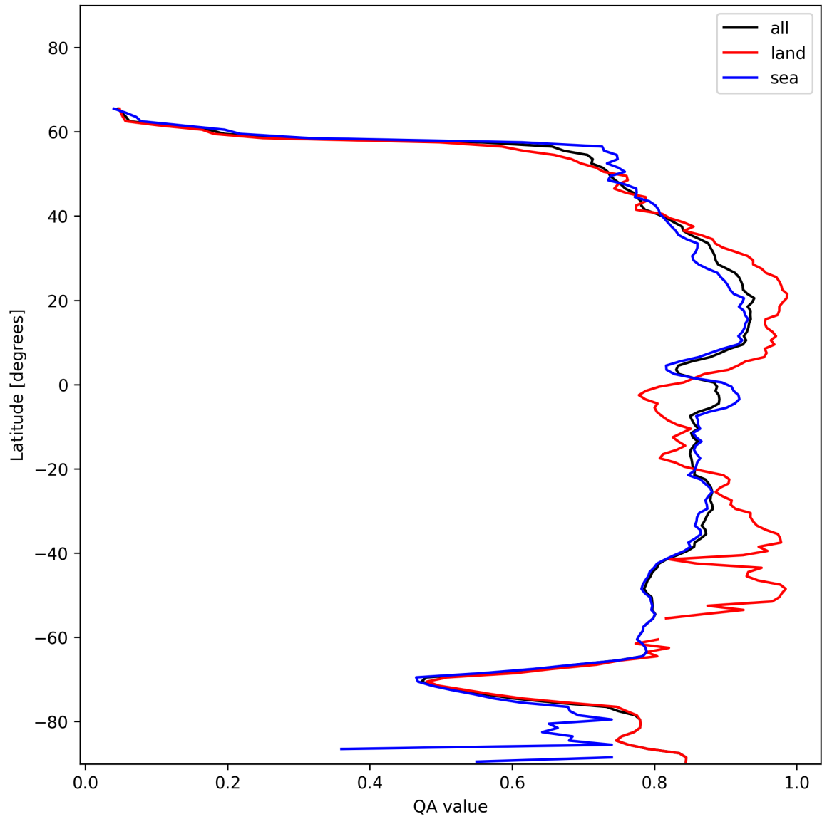
Figure 11: Zonal average of “QA value” for 2025-01-02 to 2025-01-04.
