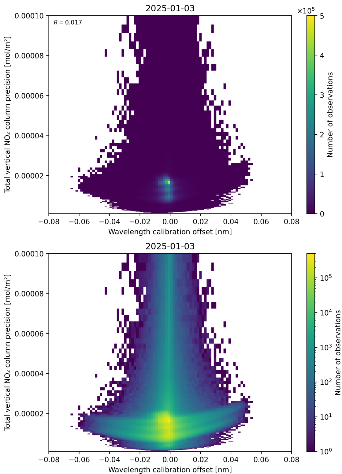
Figure 180: Scatter density plot of “Wavelength calibration offset” against “Total vertical NO 2 column precision” for 2025-01-02 to 2025-01-04.
