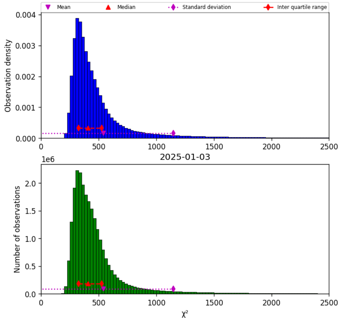
Figure 42: Histogram of " \chi^2 " for 2025-01-02 to 2025-01-04
