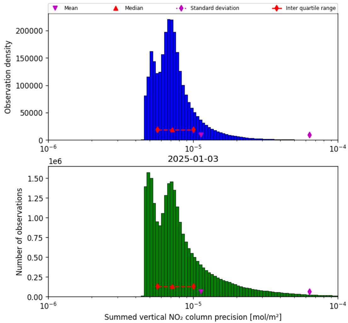
Figure 41: Histogram of “Summed vertical NO 2 column precision” for 2025-01-02 to 2025-01-04
