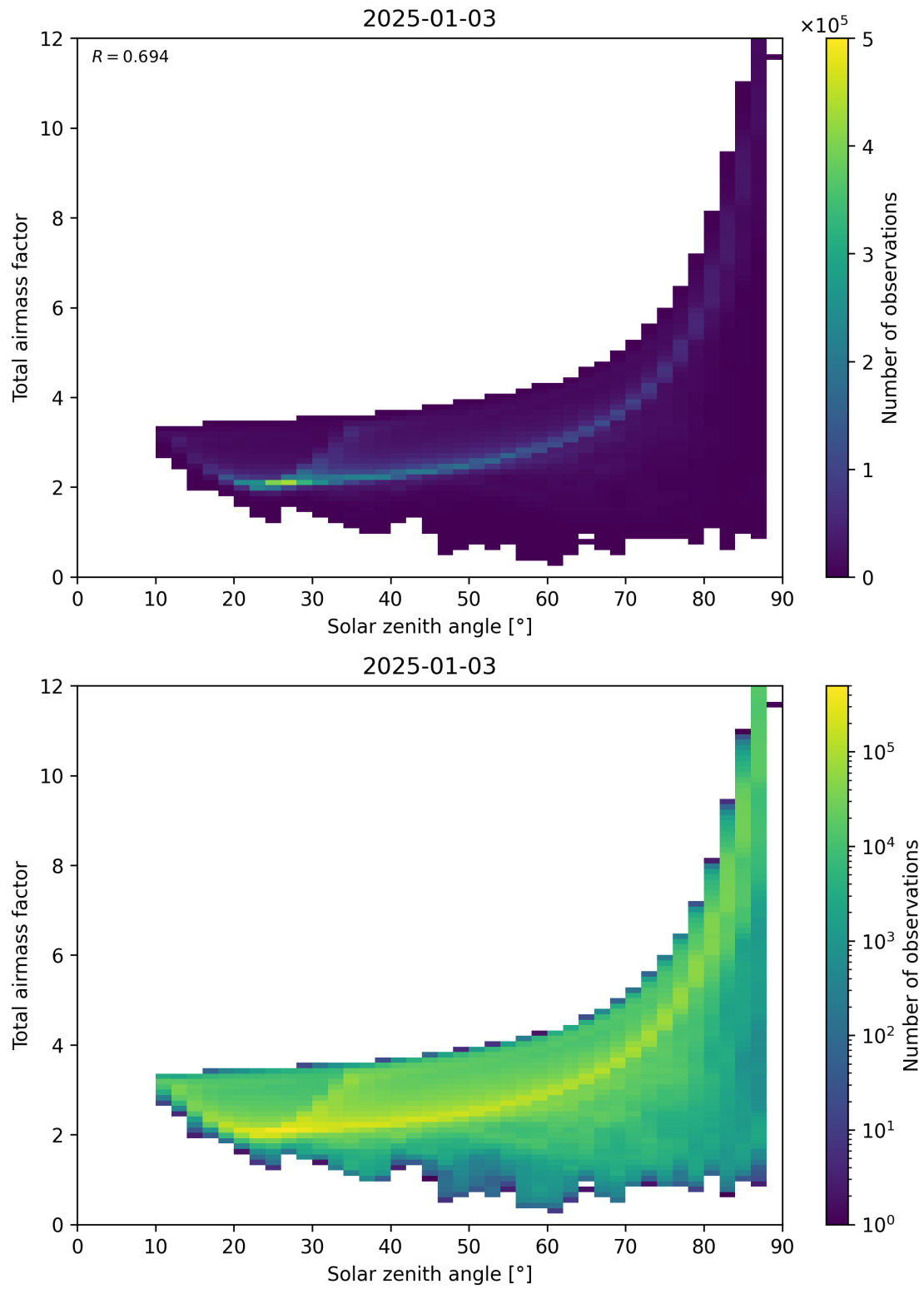
Figure 146: Scatter density plot of “Solar zenith angle” against “Total air mass factor” for 2025-01-02 to 2025-01-04.
