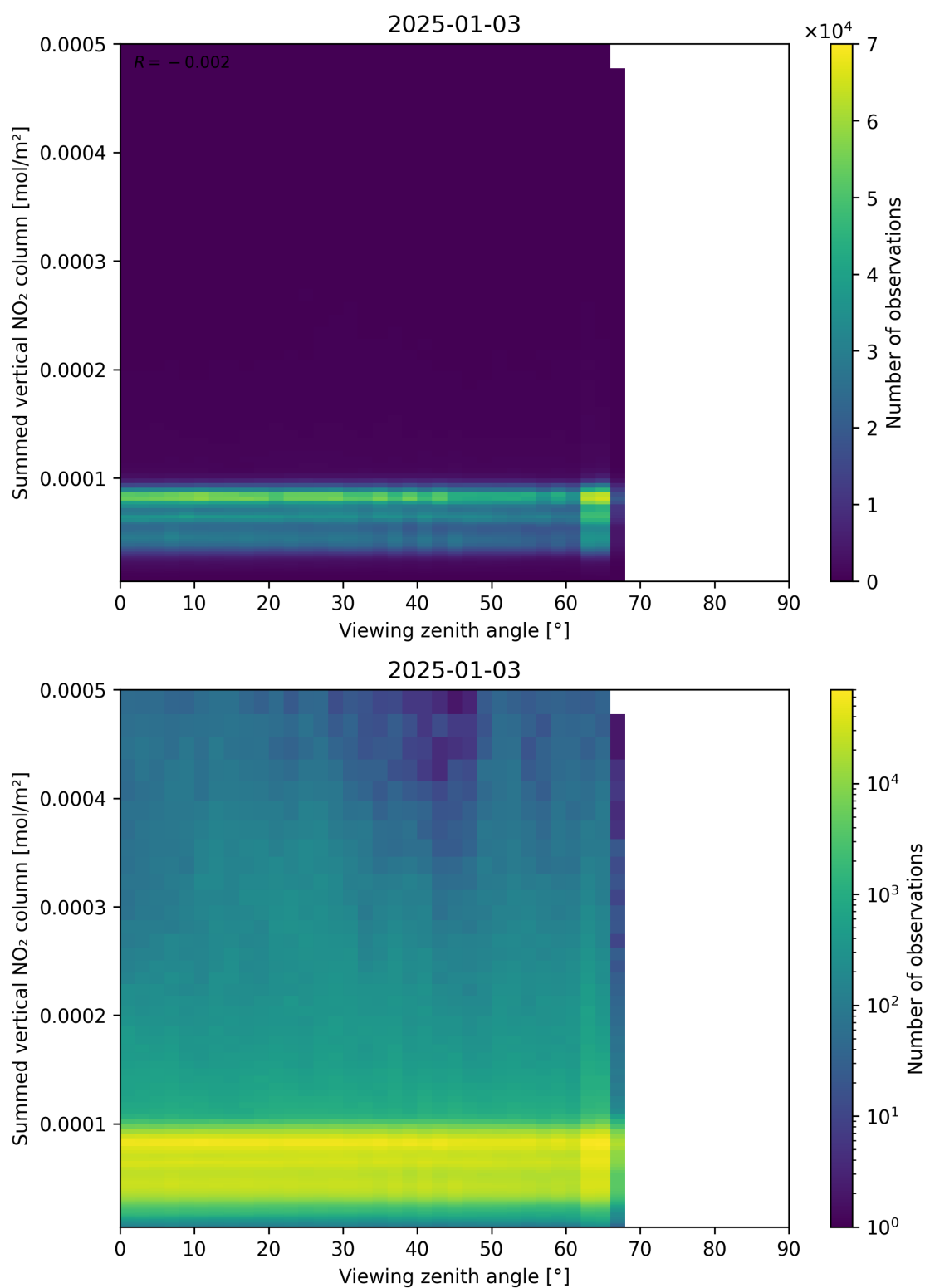
Figure 165: Scatter density plot of “Viewing zenith angle” against “Summed vertical NO 2 column” for 2025-01-02 to 2025-01-04.
