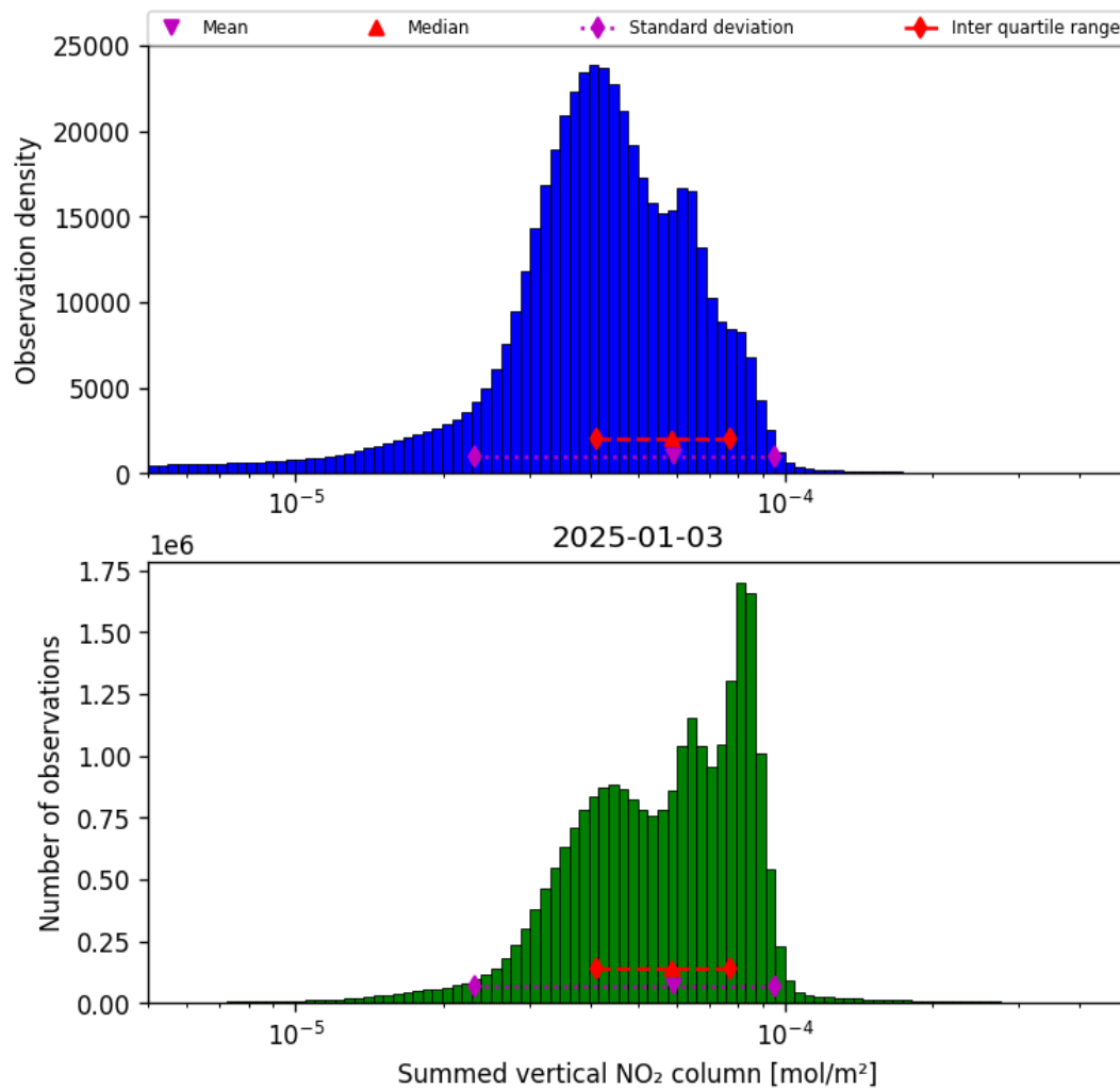
Figure 40: Histogram of “Summed vertical NO 2 column” for 2025-01-02 to 2025-01-04
