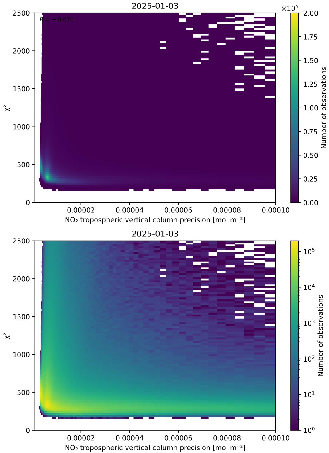
Figure 134: Scatter density plot of “NO 2 tropospheric vertical column precision” against “ \chi^2 ” for 2025-01-02 to 2025-01-04.
