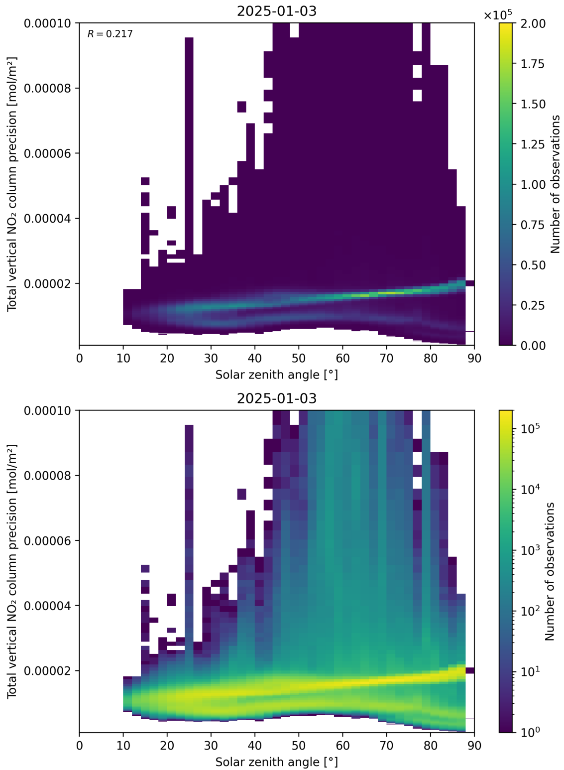
Figure 154: Scatter density plot of “Solar zenith angle” against “Total vertical NO 2 column precision” for 2025-01-02 to 2025-01-04.
