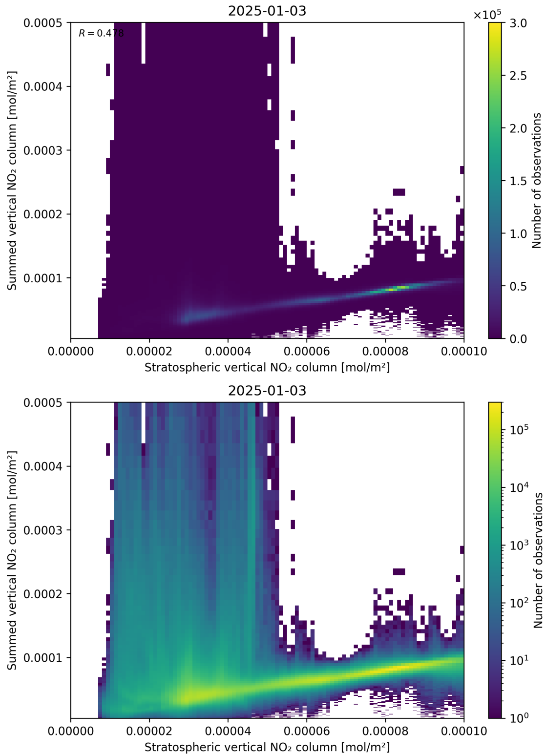
Figure 98: Scatter density plot of “Stratospheric vertical NO 2 column” against “Summed vertical NO 2 column” for 2025-01-02 to 2025-01-04.
