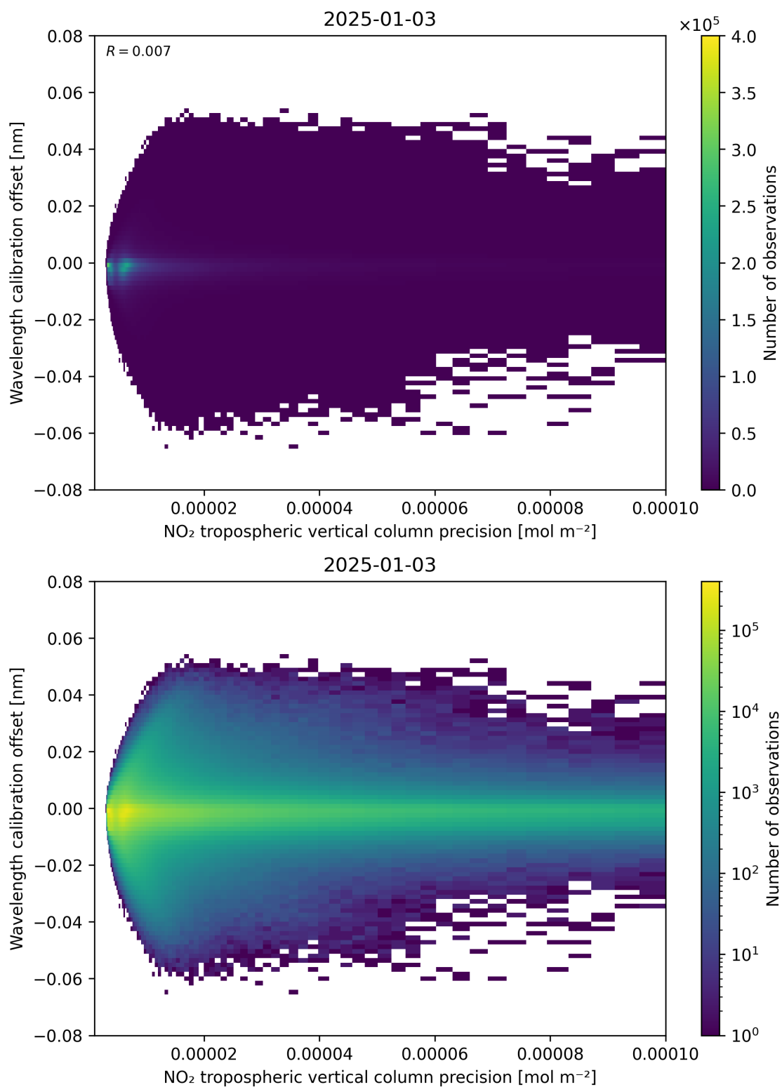
Figure 141: Scatter density plot of “NO 2 tropospheric vertical column precision” against “Wavelength calibration offset” for 2025-01-02 to 2025-01-04.
