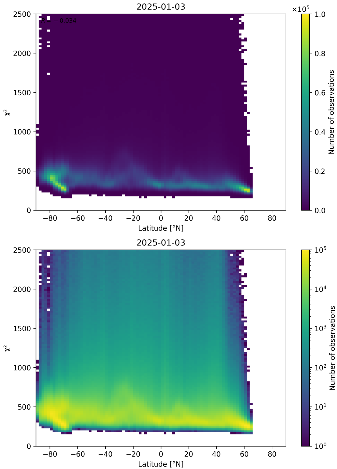
Figure 86: Scatter density plot of “Latitude” against “ \chi^2 ” for 2025-01-02 to 2025-01-04.
