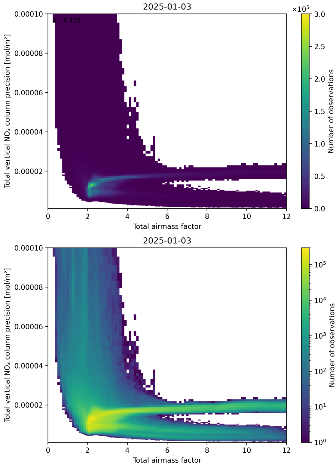
Figure 68: Scatter density plot of “Total airmass factor” against “Total vertical NO 2 column precision” for 2025-01-02 to 2025-01-04.
