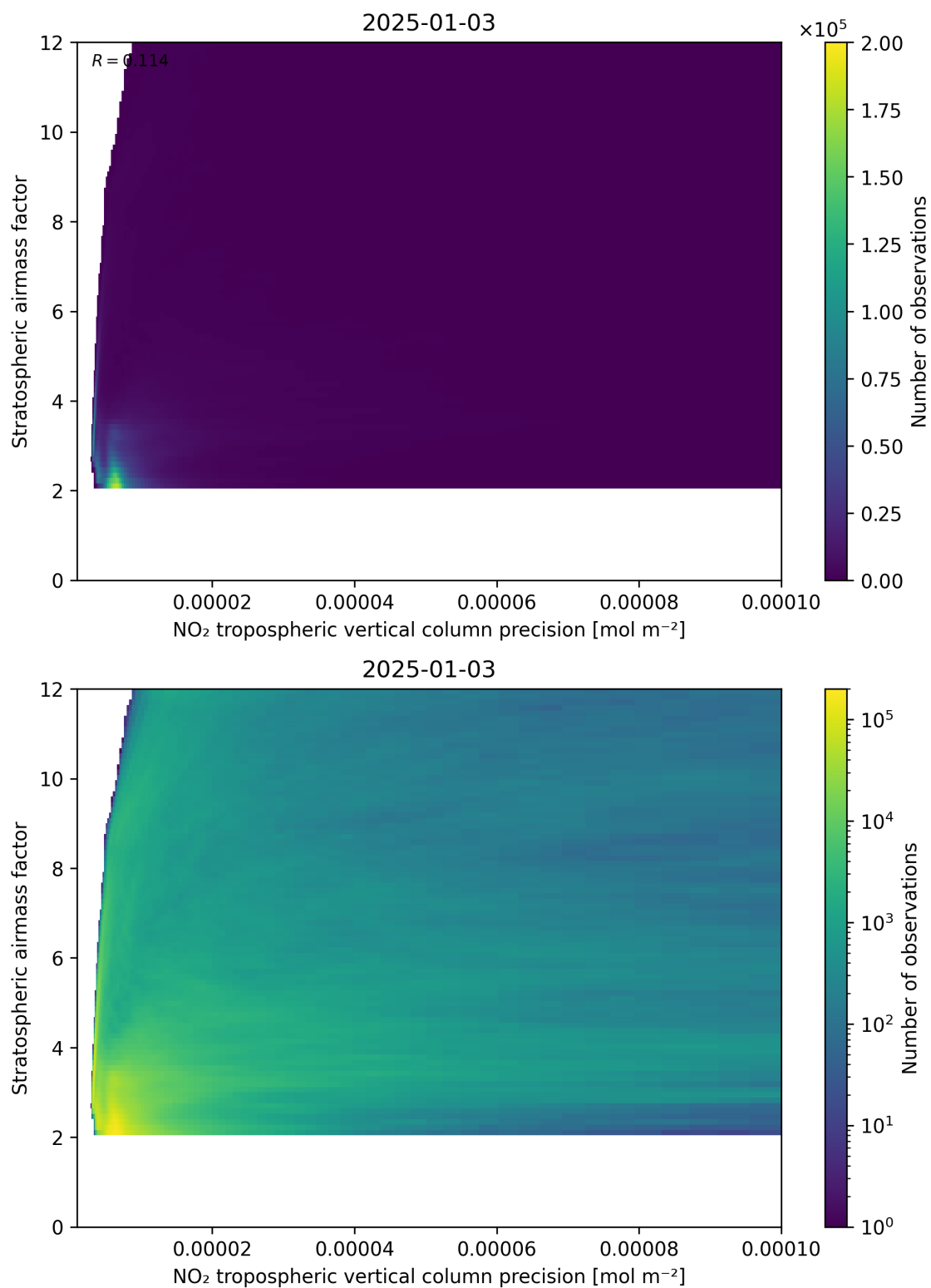
Figure 131: Scatter density plot of “NO 2 tropospheric vertical column precision” against “Stratospheric airmass factor” for 2025-01-02 to 2025-01-04.
