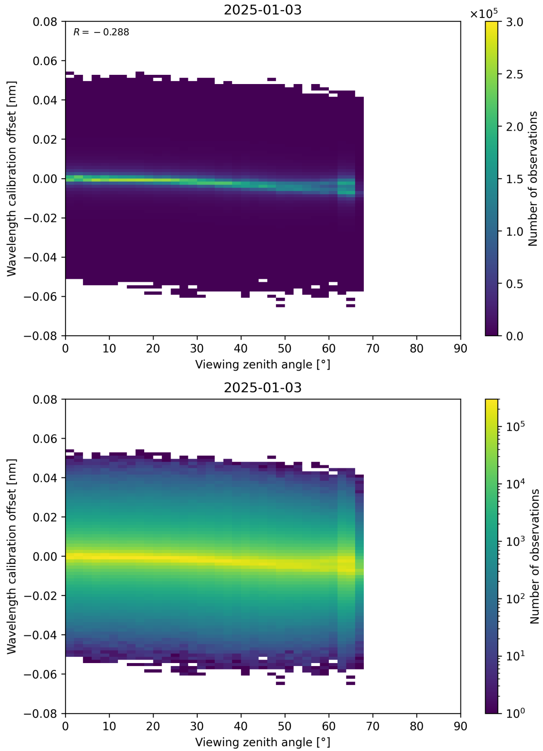
Figure 173: Scatter density plot of “Viewing zenith angle” against “Wavelength calibration offset” for 2025-01-02 to 2025-01-04.
