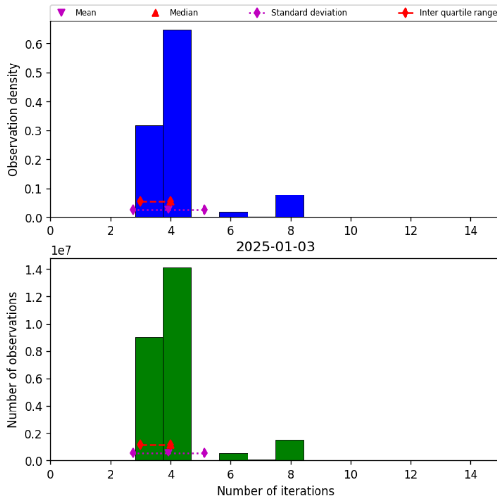
Figure 34: Histogram of “Number of iterations” for 2025-01-02 to 2025-01-04
