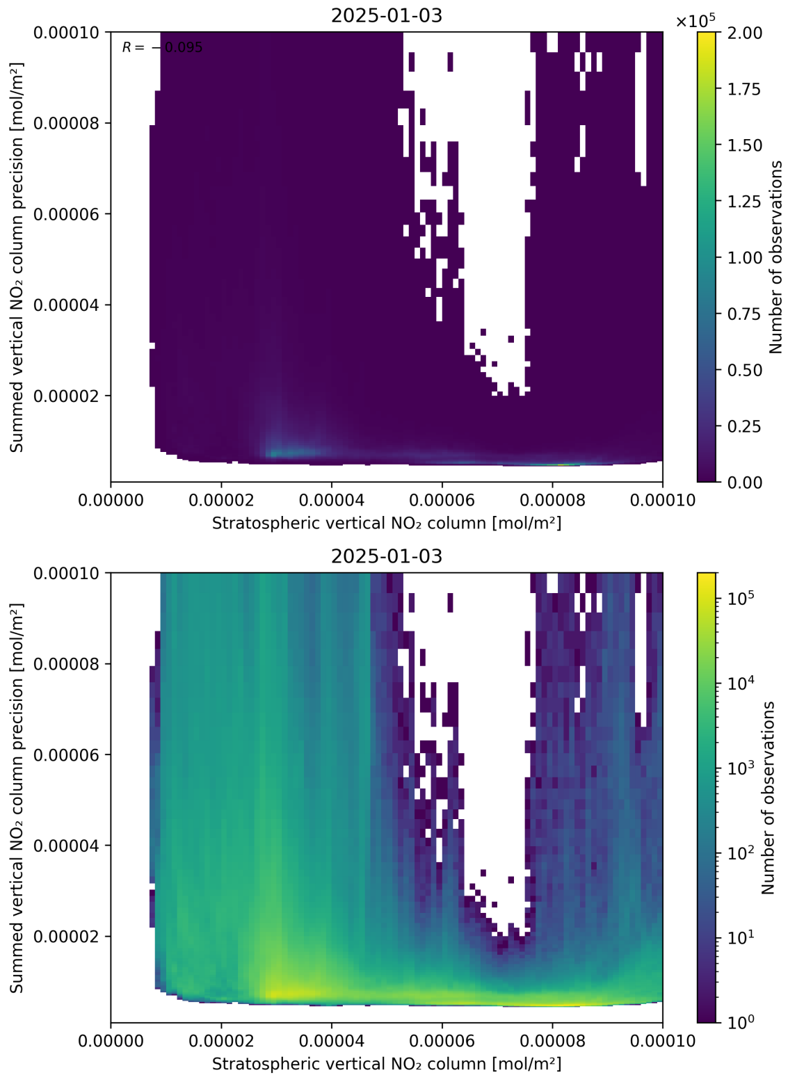
Figure 99: Scatter density plot of “Stratospheric vertical NO 2 column” against “Summed vertical NO 2 column precision” for 2025-01-02 to 2025-01-04.
