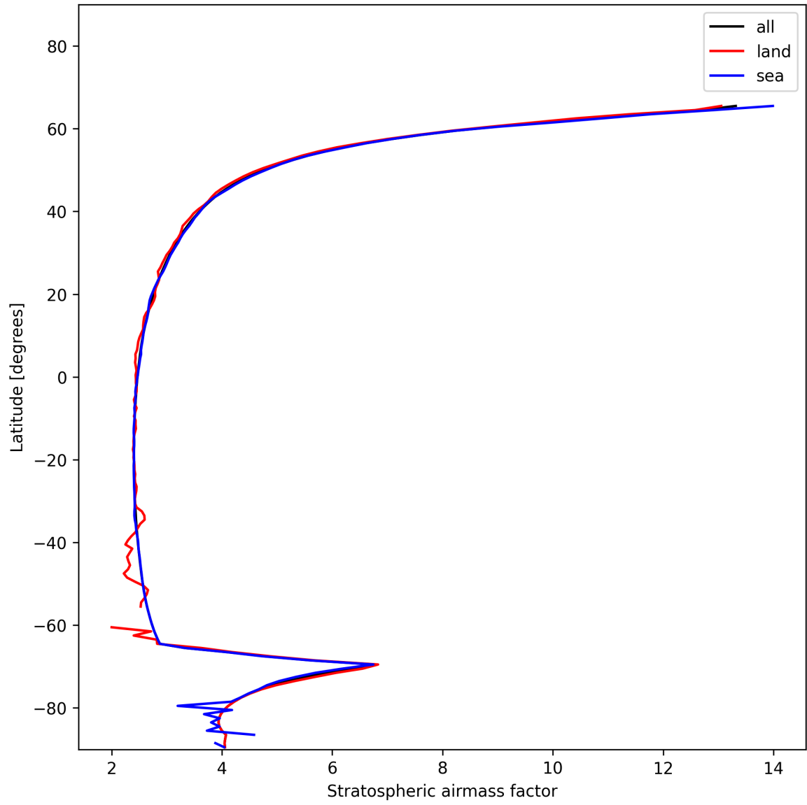
Figure 27: Zonal average of “Stratospheric airmass factor” for 2025-01-02 to 2025-01-04.
