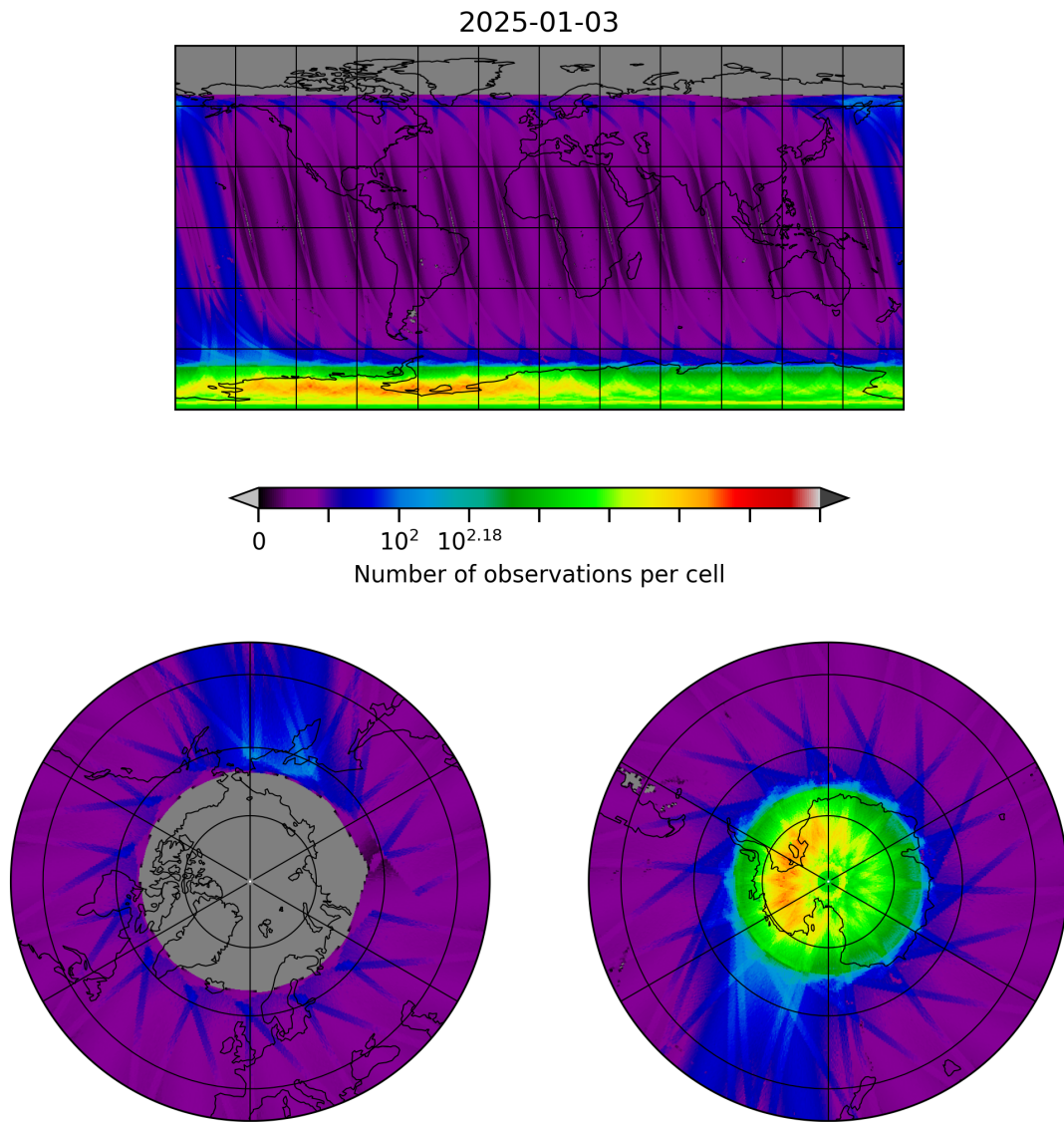
Figure 10: Map of the number of observations for 2025-01-02 to 2025-01-04
