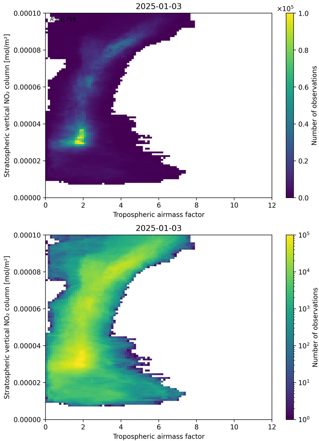
Figure 74: Scatter density plot of “Tropospheric airmass factor” against “Stratospheric vertical NO 2 column” for 2025-01-02 to 2025-01-04.
