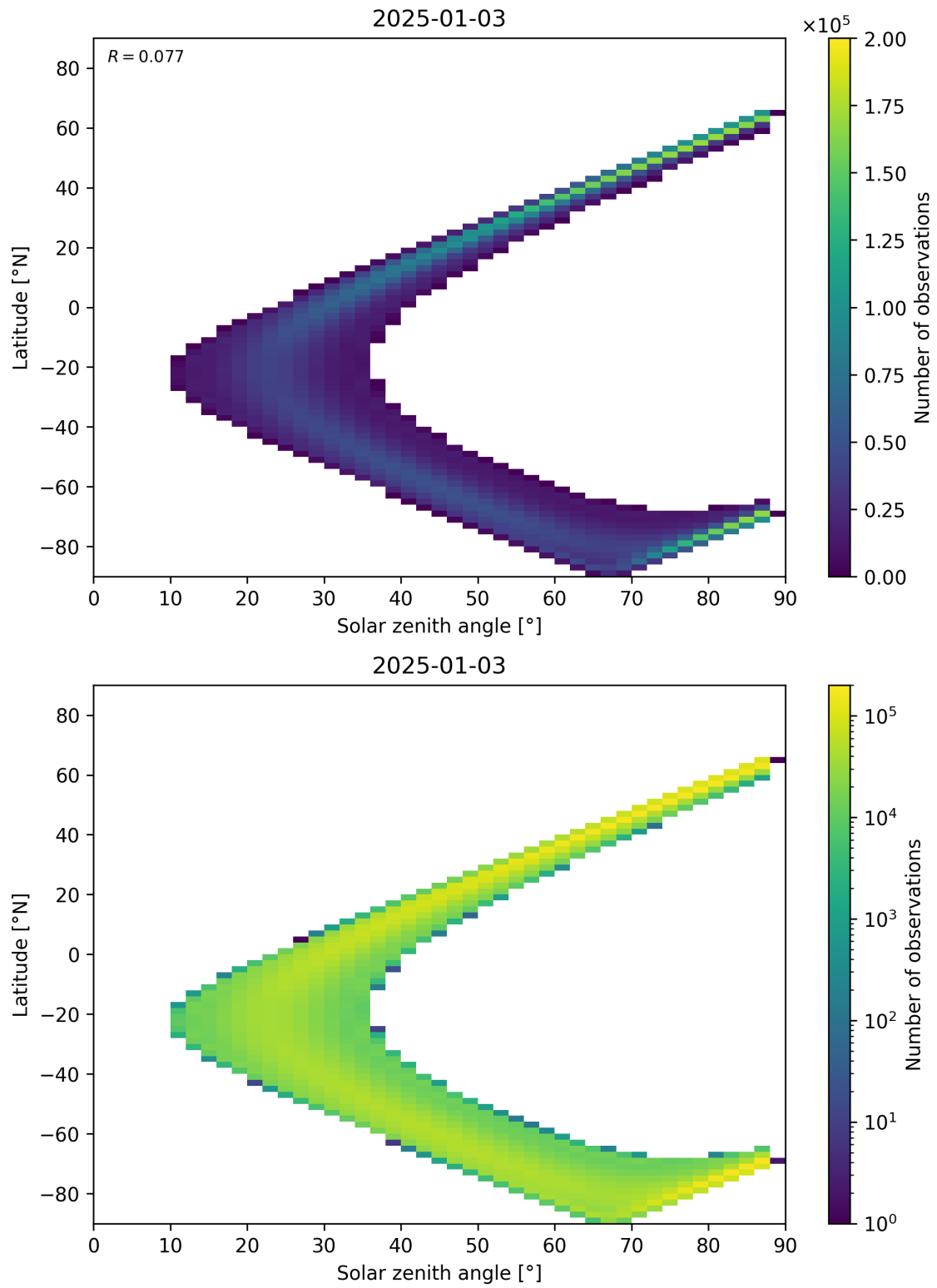
Figure 149: Scatter density plot of “Solar zenith angle” against “Latitude” for 2025-01-02 to 2025-01-04.
