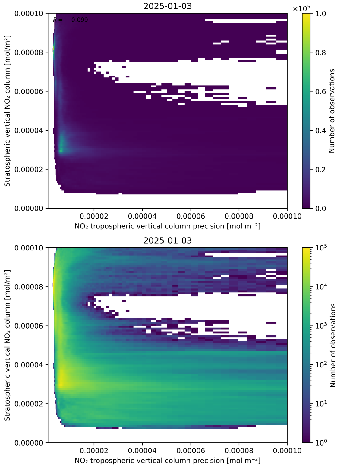
Figure 135: Scatter density plot of “NO 2 tropospheric vertical column precision” against “Stratospheric vertical NO 2 column” for 2025-01-02 to 2025-01-04.
