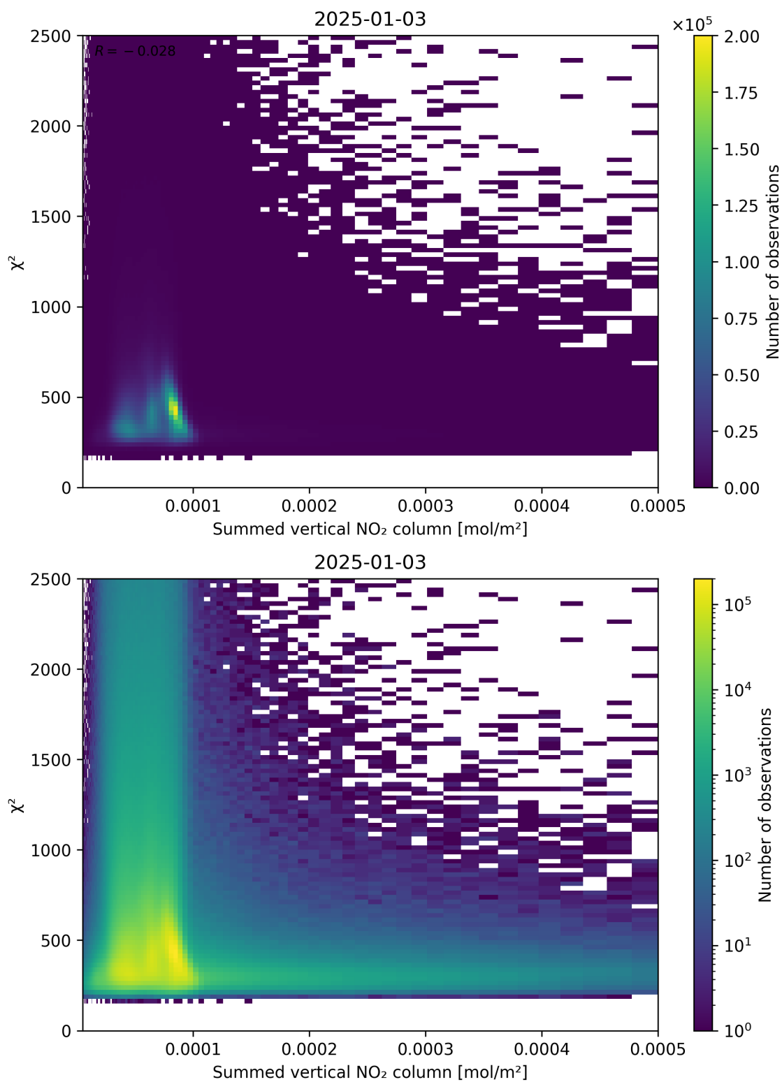
Figure 104: Scatter density plot of “Summed vertical NO 2 column” against “ \chi^2 ” for 2025-01-02 to 2025-01-04.
