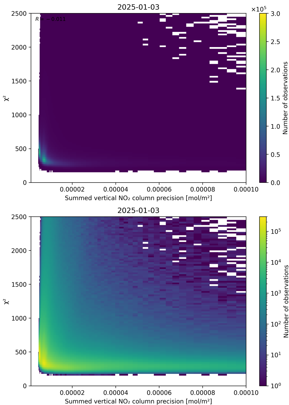
Figure 107: Scatter density plot of “Summed vertical NO 2 column precision” against “ \chi^2 ” for 2025-01-02 to 2025-01-04.
