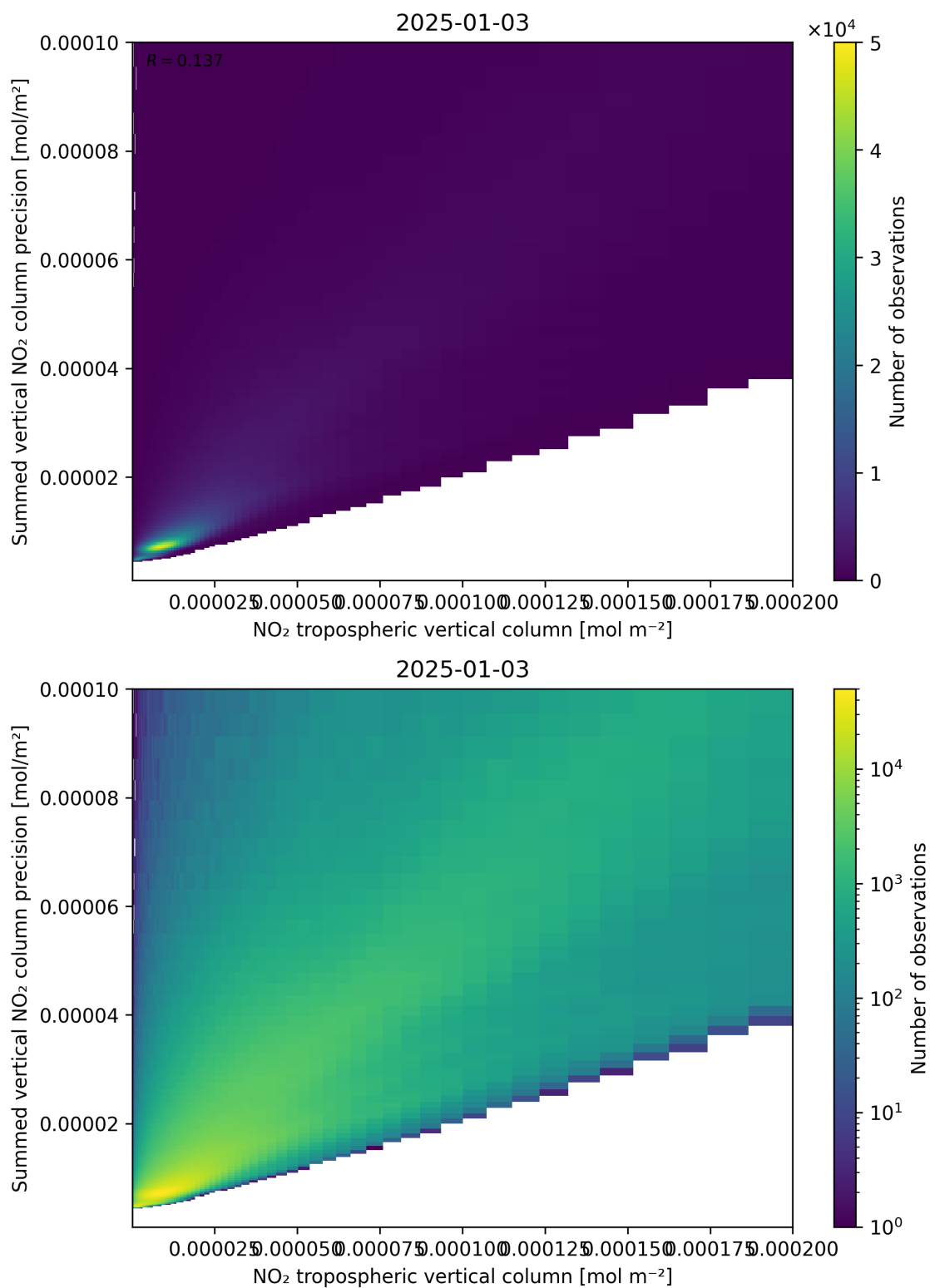
Figure 127: Scatter density plot of “NO 2 tropospheric vertical column” against “Summed vertical NO 2 column precision” for 2025-01-02 to 2025-01-04.
