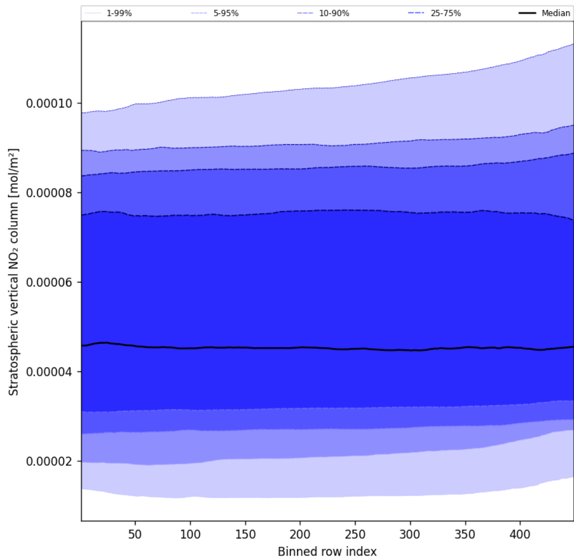
Figure 53: Along track statistics of “Stratospheric vertical NO 2 column” for 2025-01-02 to 2025-01-04
