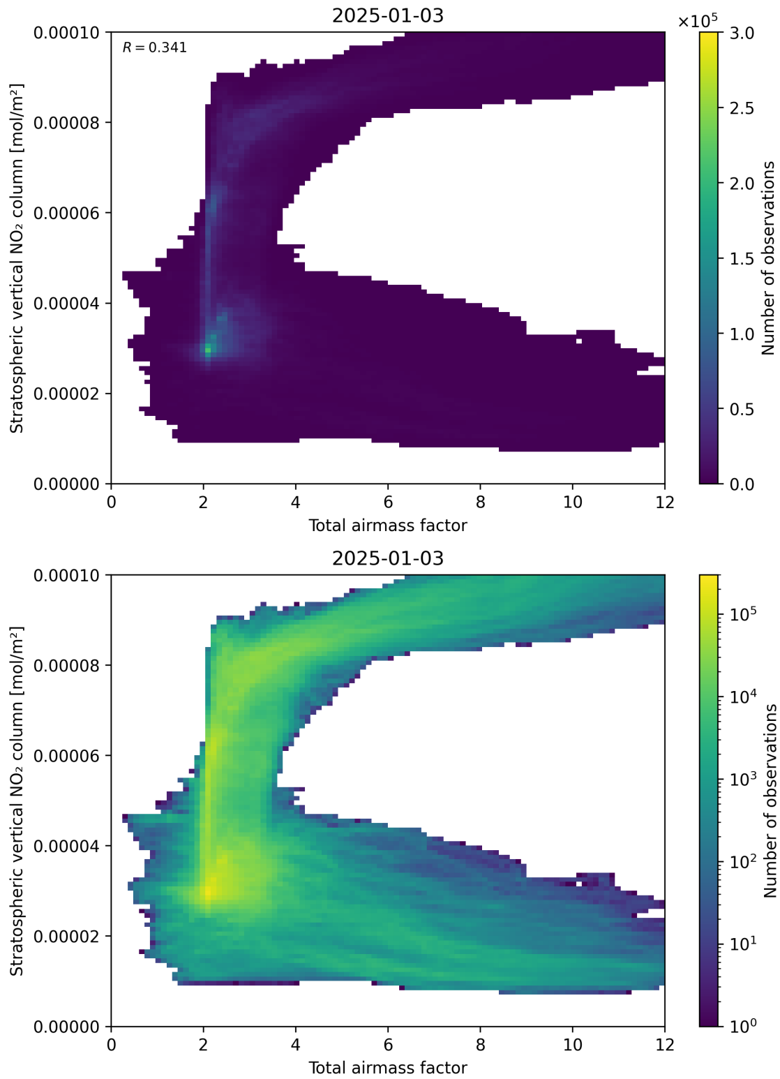
Figure 64: Scatter density plot of “Total airmass factor” against “Stratospheric vertical NO 2 column” for 2025-01-02 to 2025-01-04.
