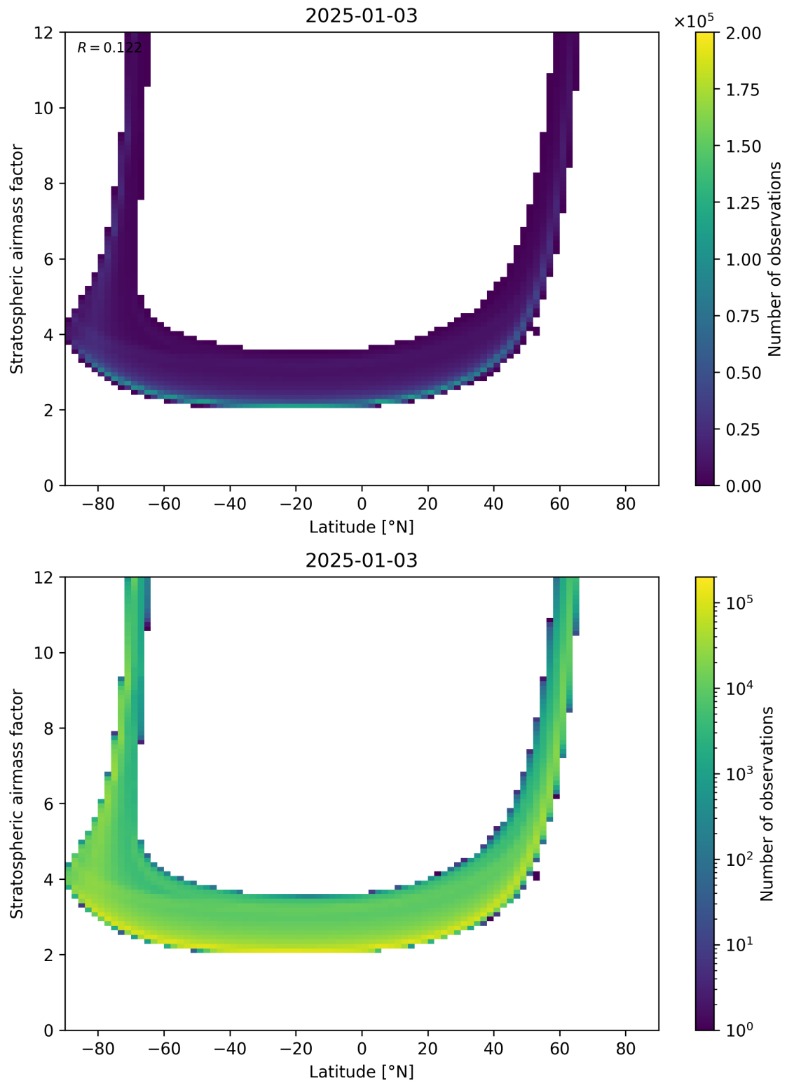
Figure 83: Scatter density plot of “Latitude” against “Stratospheric air mass factor” for 2025-01-02 to 2025-01-04.
