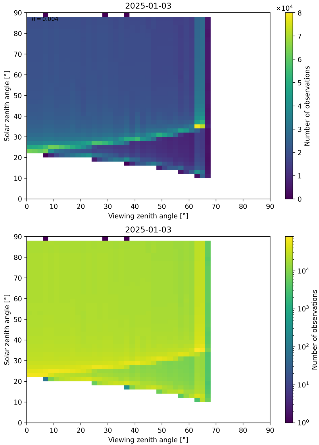
Figure 172: Scatter density plot of “Viewing zenith angle” against “Solar zenith angle” for 2025-01-02 to 2025-01-04.
