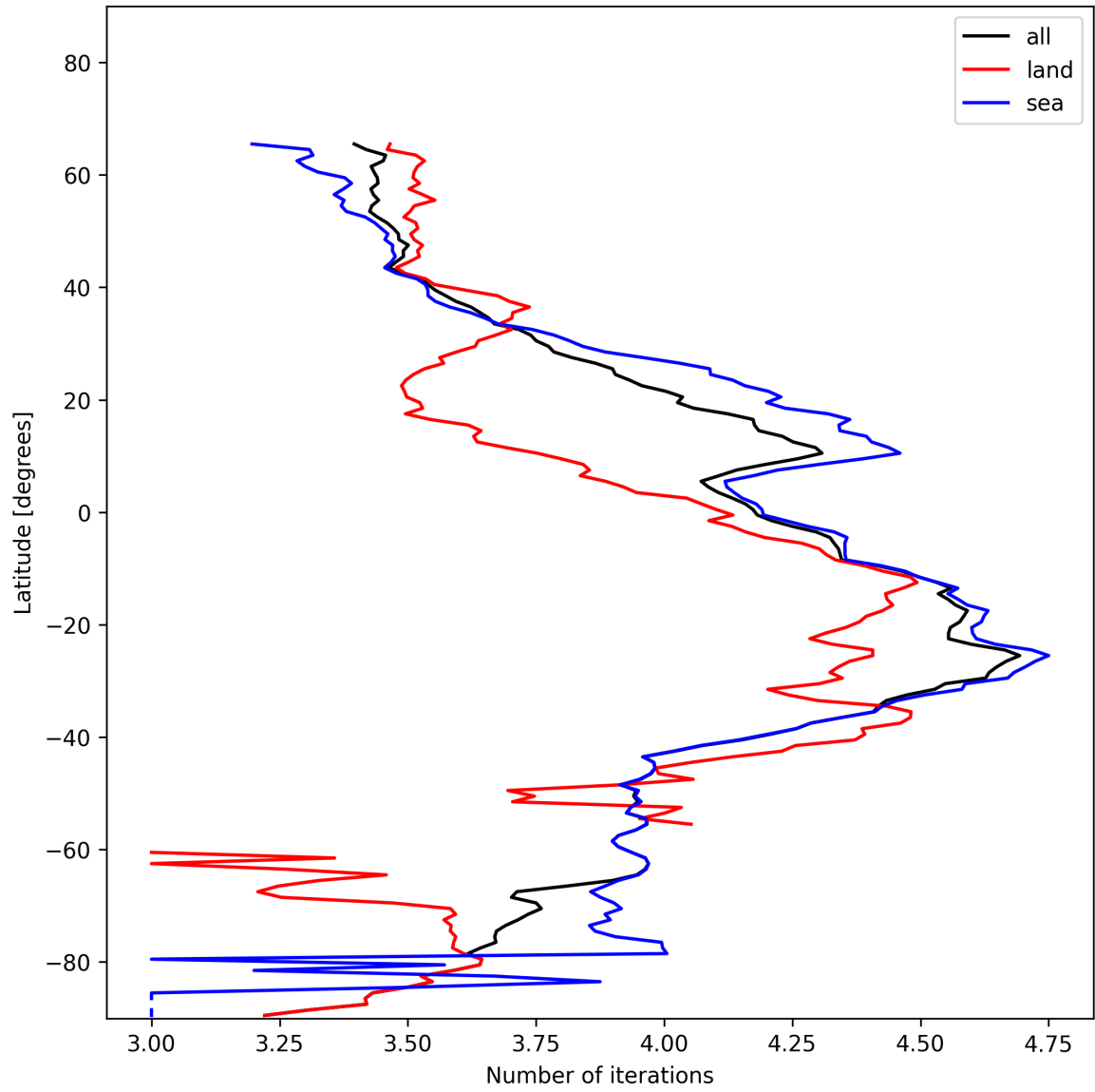
Figure 17: Zonal average of “Number of iterations” for 2025-01-02 to 2025-01-04.
