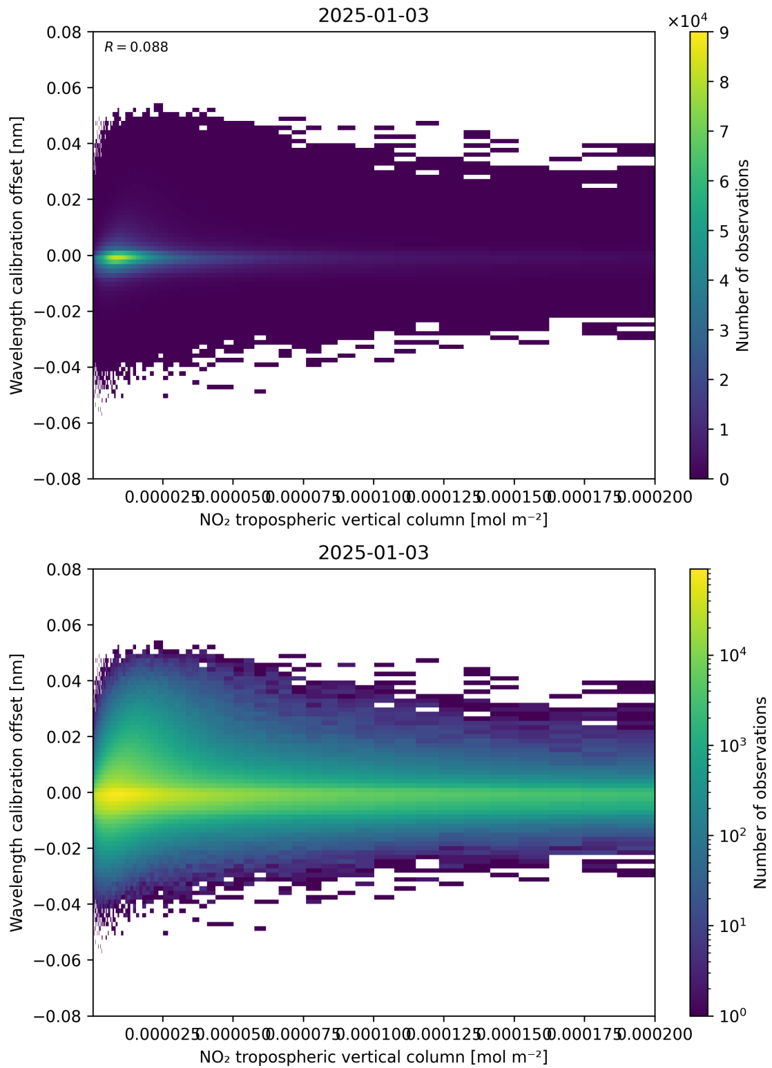
Figure 143: Scatter density plot of “NO 2 tropospheric vertical column” against “Wavelength calibration offset” for 2025-01-02 to 2025-01-04.
