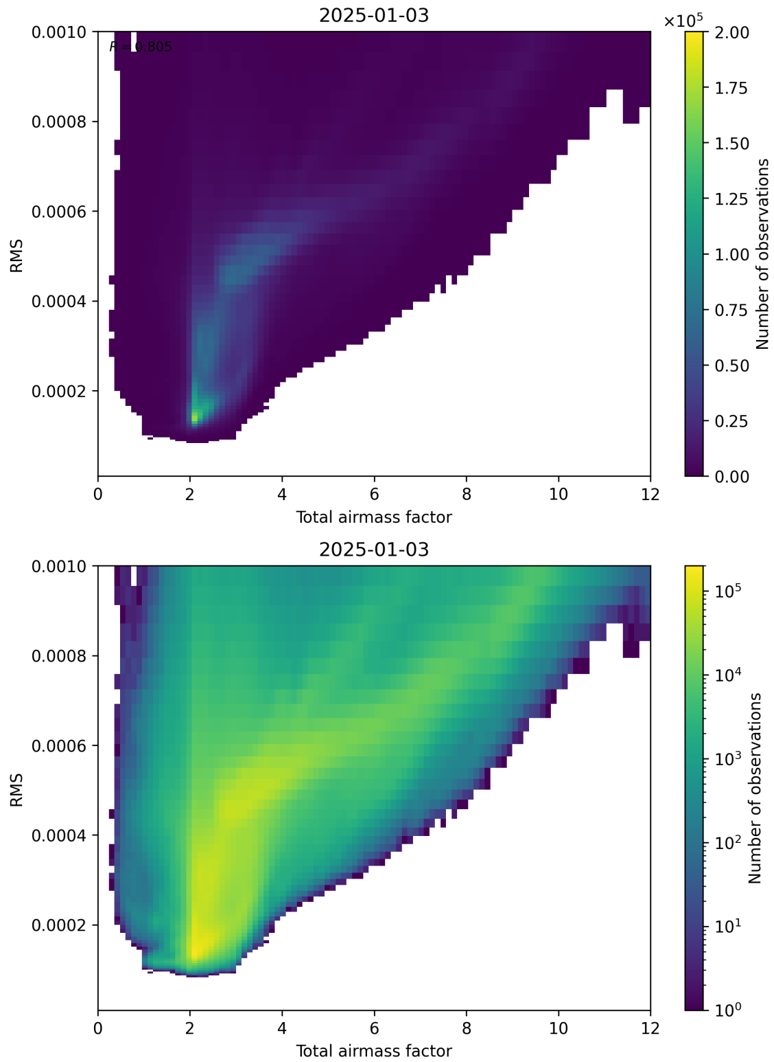
Figure 69: Scatter density plot of “Total airmass factor” against “RMS” for 2025-01-02 to 2025-01-04.
