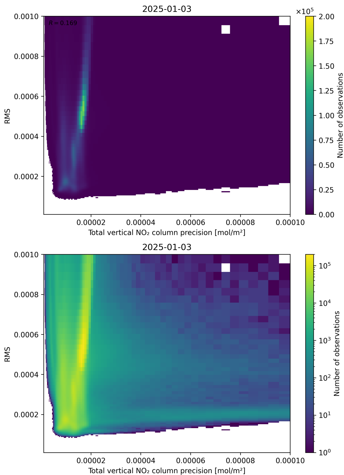
Figure 119: Scatter density plot of “Total vertical NO 2 column precision” against “RMS” for 2025-01-02 to 2025-01-04.
