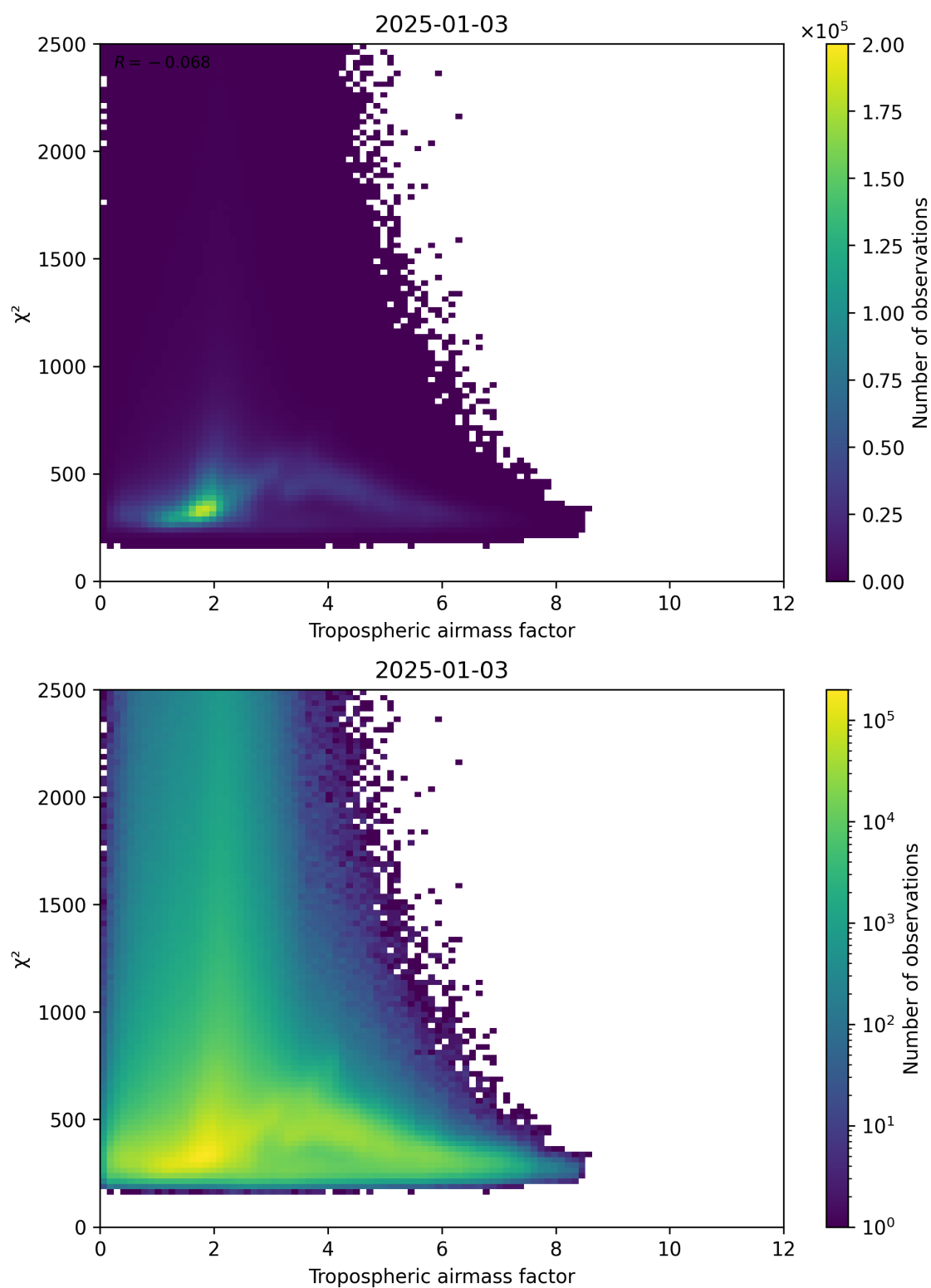
Figure 73: Scatter density plot of “Tropospheric airmass factor” against “ \chi^2 ” for 2025-01-02 to 2025-01-04.
