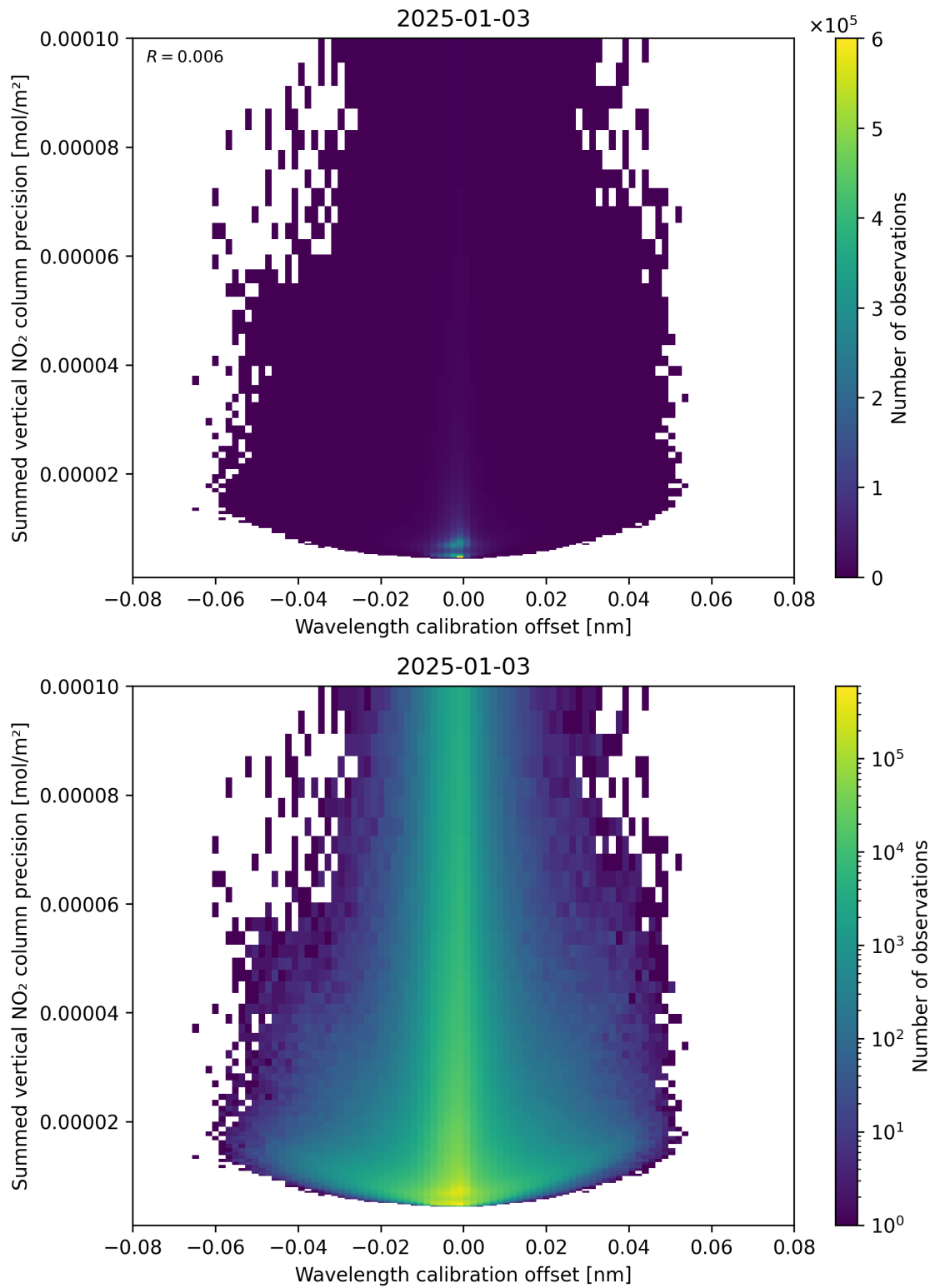
Figure 178: Scatter density plot of “Wavelength calibration offset” against “Summed vertical NO 2 column precision” for 2025-01-02 to 2025-01-04.
