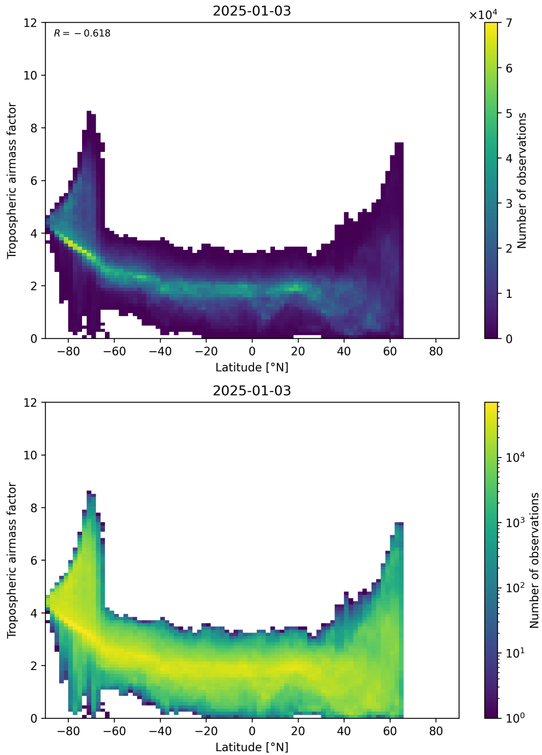
Figure 85: Scatter density plot of “Latitude” against “Tropospheric airmass factor” for 2025-01-02 to 2025-01-04.
