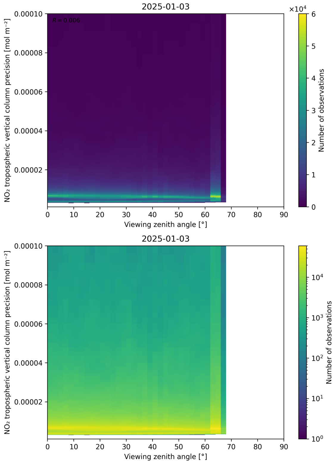
Figure 170: Scatter density plot of “Viewing zenith angle” against “NO 2 tropospheric vertical column precision” for 2025-01-02 to 2025-01-04.
