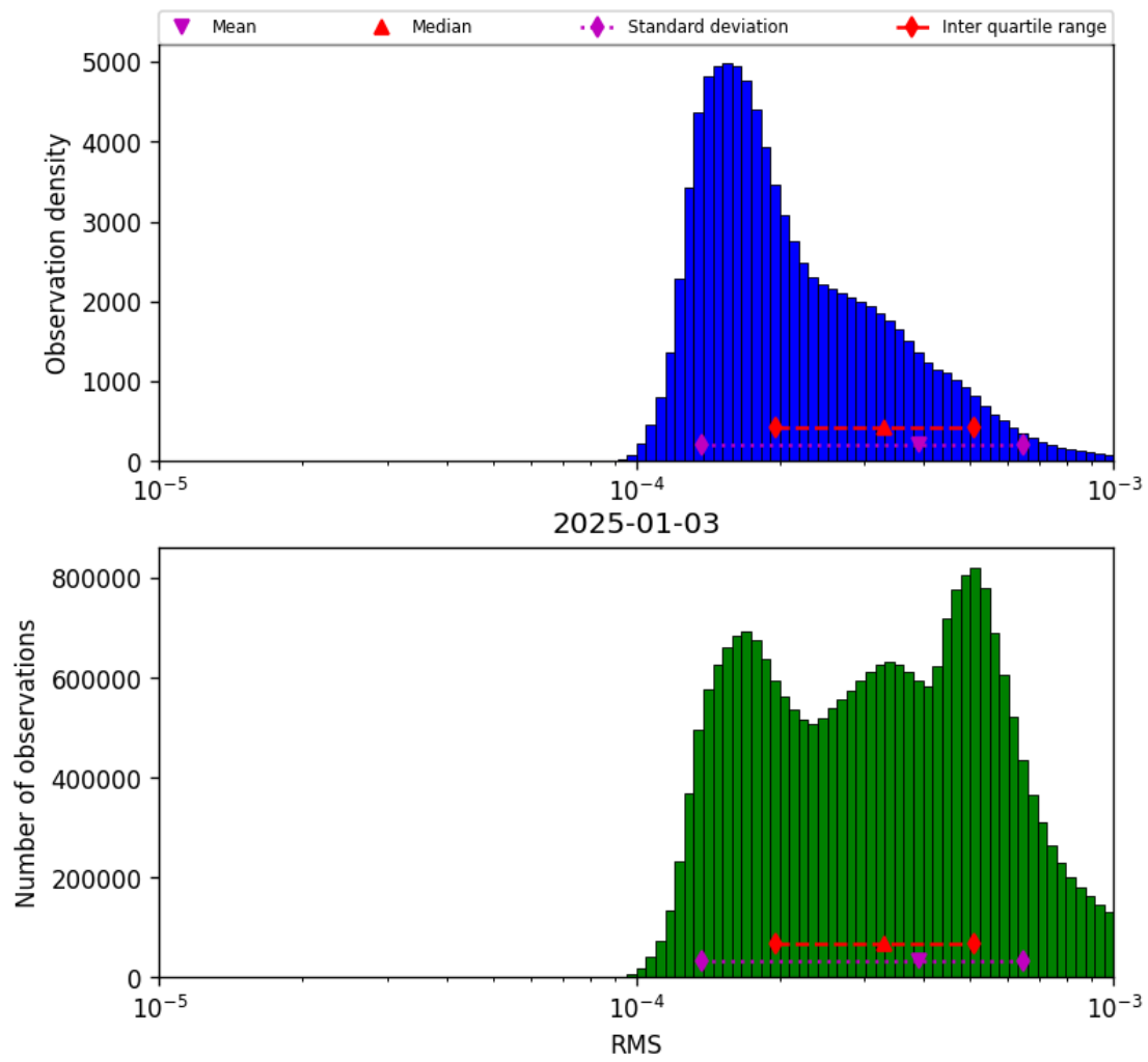
Figure 43: Histogram of “RMS” for 2025-01-02 to 2025-01-04
