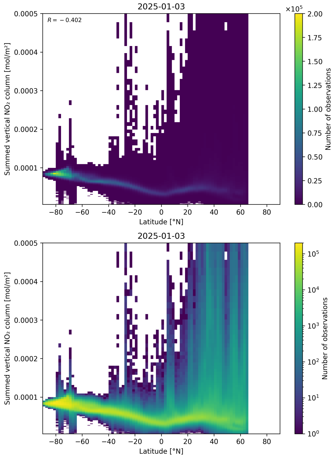
Figure 88: Scatter density plot of “Latitude” against “Summed vertical NO 2 column” for 2025-01-02 to 2025-01-04.
