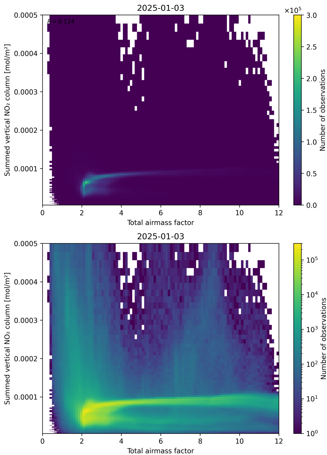
Figure 65: Scatter density plot of “Total airmass factor” against “Summed vertical NO 2 column” for 2025-01-02 to 2025-01-04.
