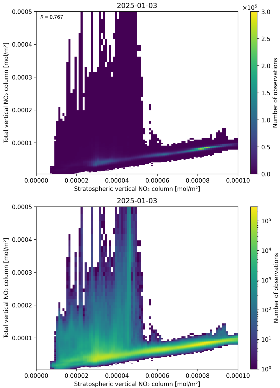
Figure 100: Scatter density plot of “Stratospheric vertical NO 2 column” against “Total vertical NO 2 column” for 2025-01-02 to 2025-01-04.
