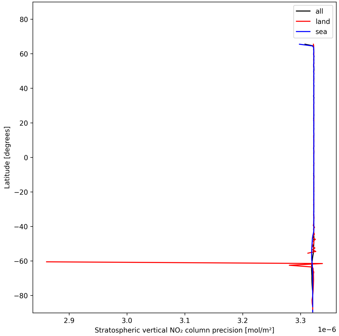
Figure 20: Zonal average of “Stratospheric vertical NO 2 column precision” for 2025-01-02 to 2025-01-04.
