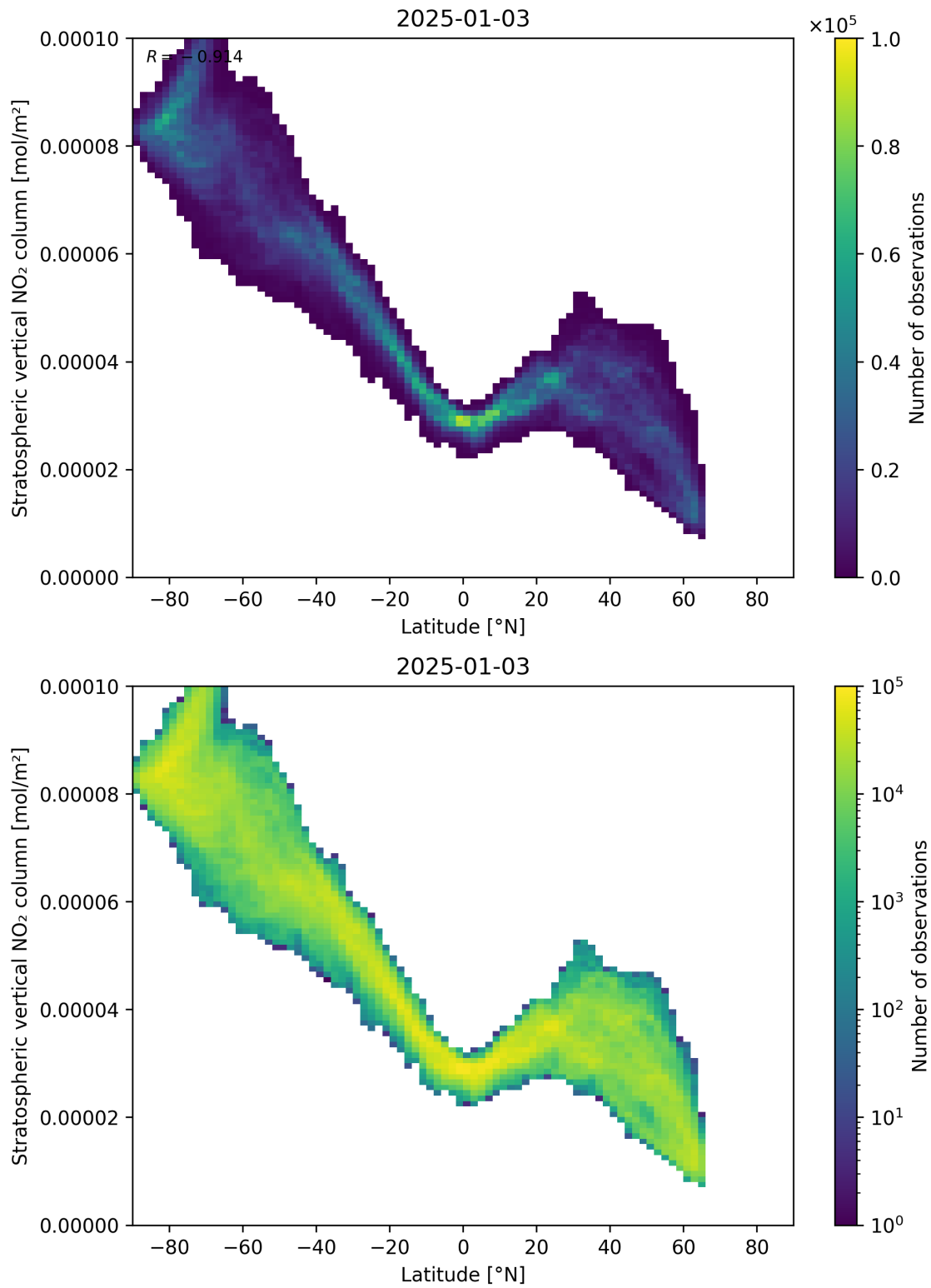
Figure 87: Scatter density plot of “Latitude” against “Stratospheric vertical NO 2 column” for 2025-01-02 to 2025-01-04.
