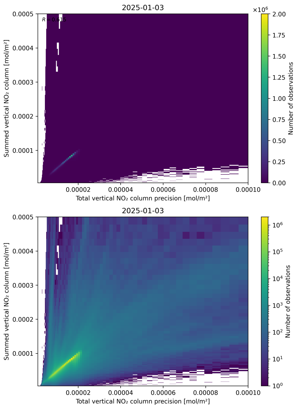
Figure 117: Scatter density plot of “Total vertical NO 2 column precision” against “Summed vertical NO 2 column” for 2025-01-02 to 2025-01-04.
