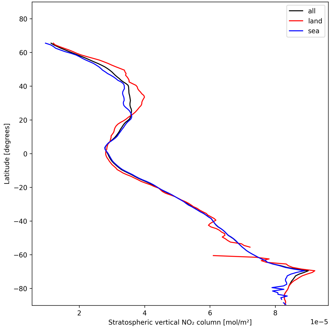
Figure 19: Zonal average of “Stratospheric vertical NO 2 column” for 2025-01-02 to 2025-01-04.
