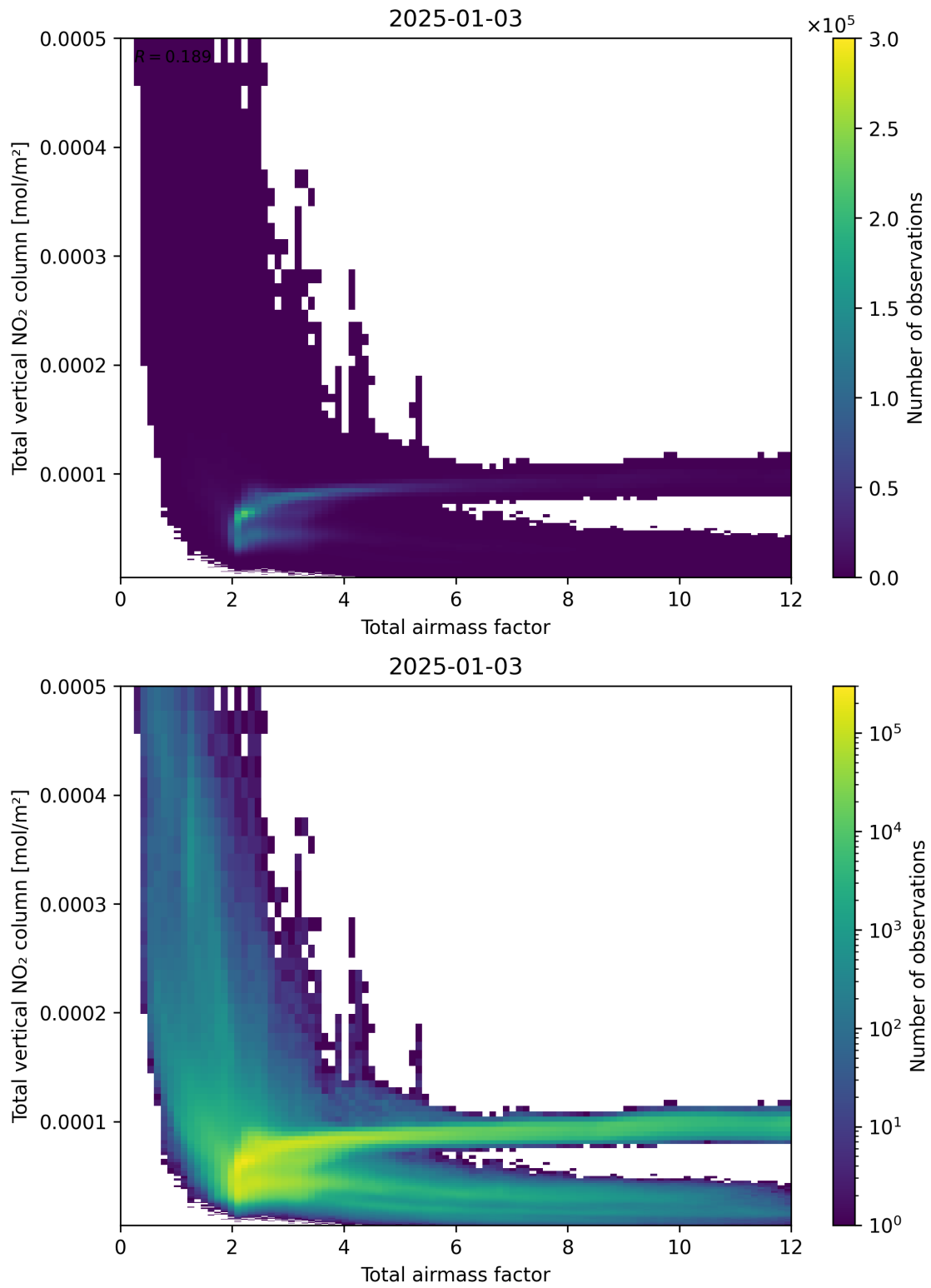
Figure 67: Scatter density plot of “Total airmass factor” against “Total vertical NO 2 column” for 2025-01-02 to 2025-01-04.
