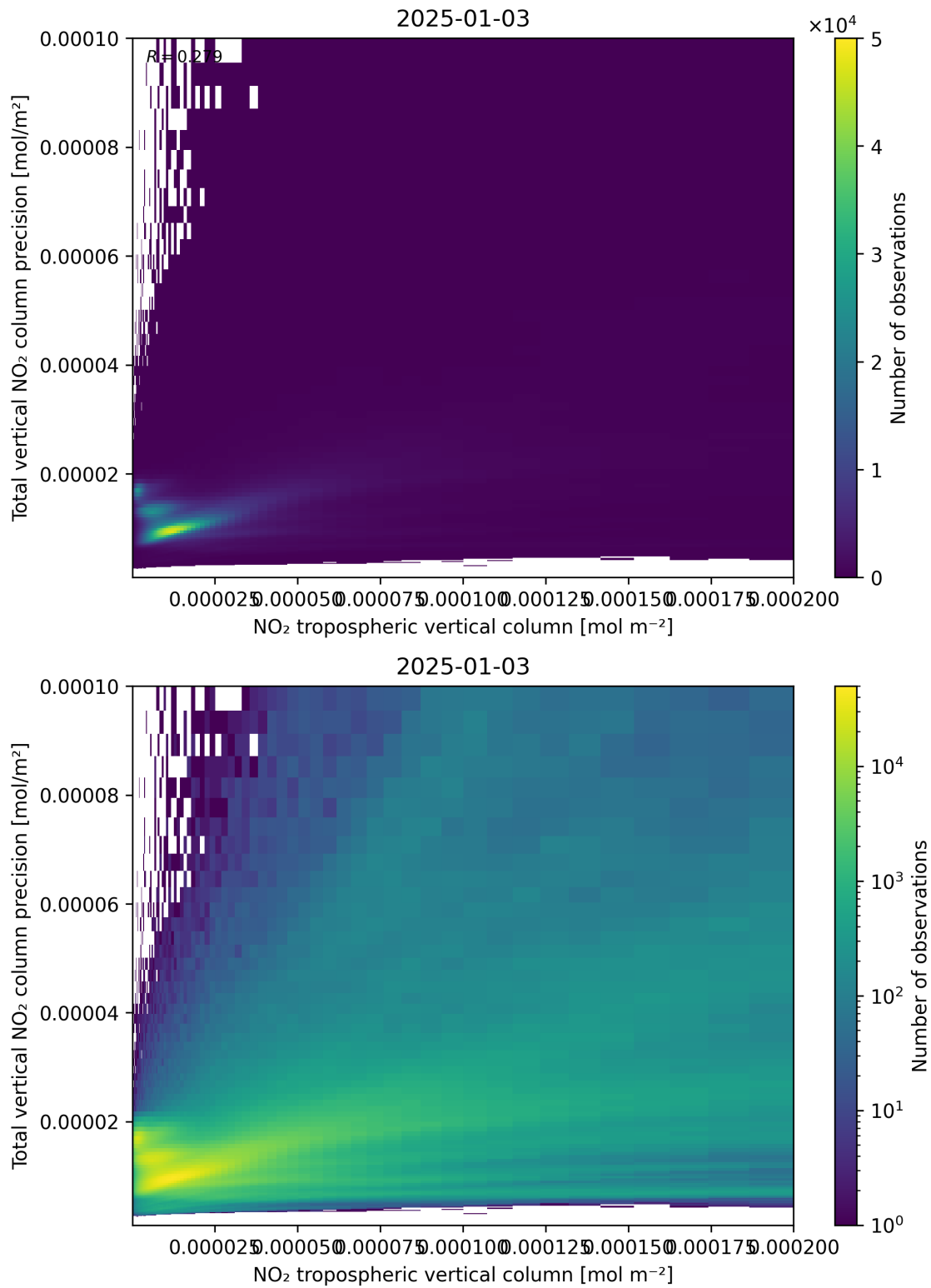
Figure 129: Scatter density plot of “NO 2 tropospheric vertical column” against “Total vertical NO 2 column precision” for 2025-01-02 to 2025-01-04.
