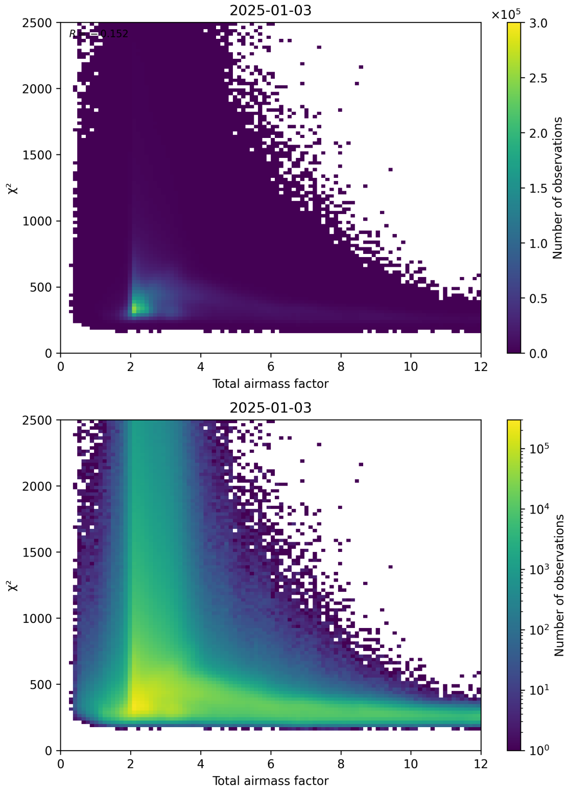
Figure 63: Scatter density plot of “Total airmass factor” against “ \chi^2 ” for 2025-01-02 to 2025-01-04.
