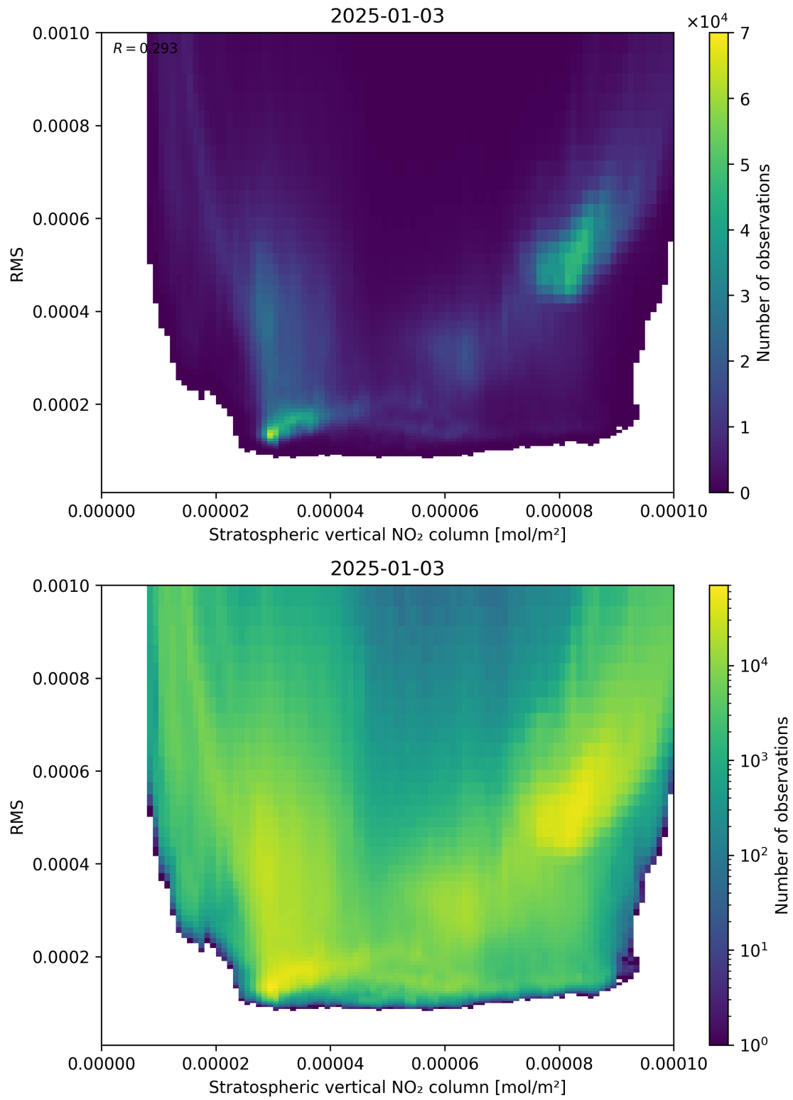
Figure 102: Scatter density plot of “Stratospheric vertical NO 2 column” against “RMS” for 2025-01-02 to 2025-01-04.
