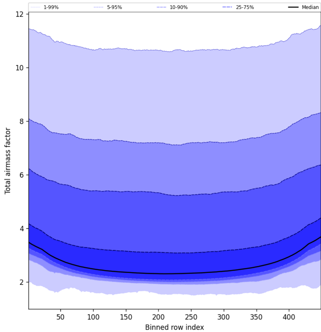
Figure 49: Along track statistics of “Total airmass factor” for 2025-01-02 to 2025-01-04
