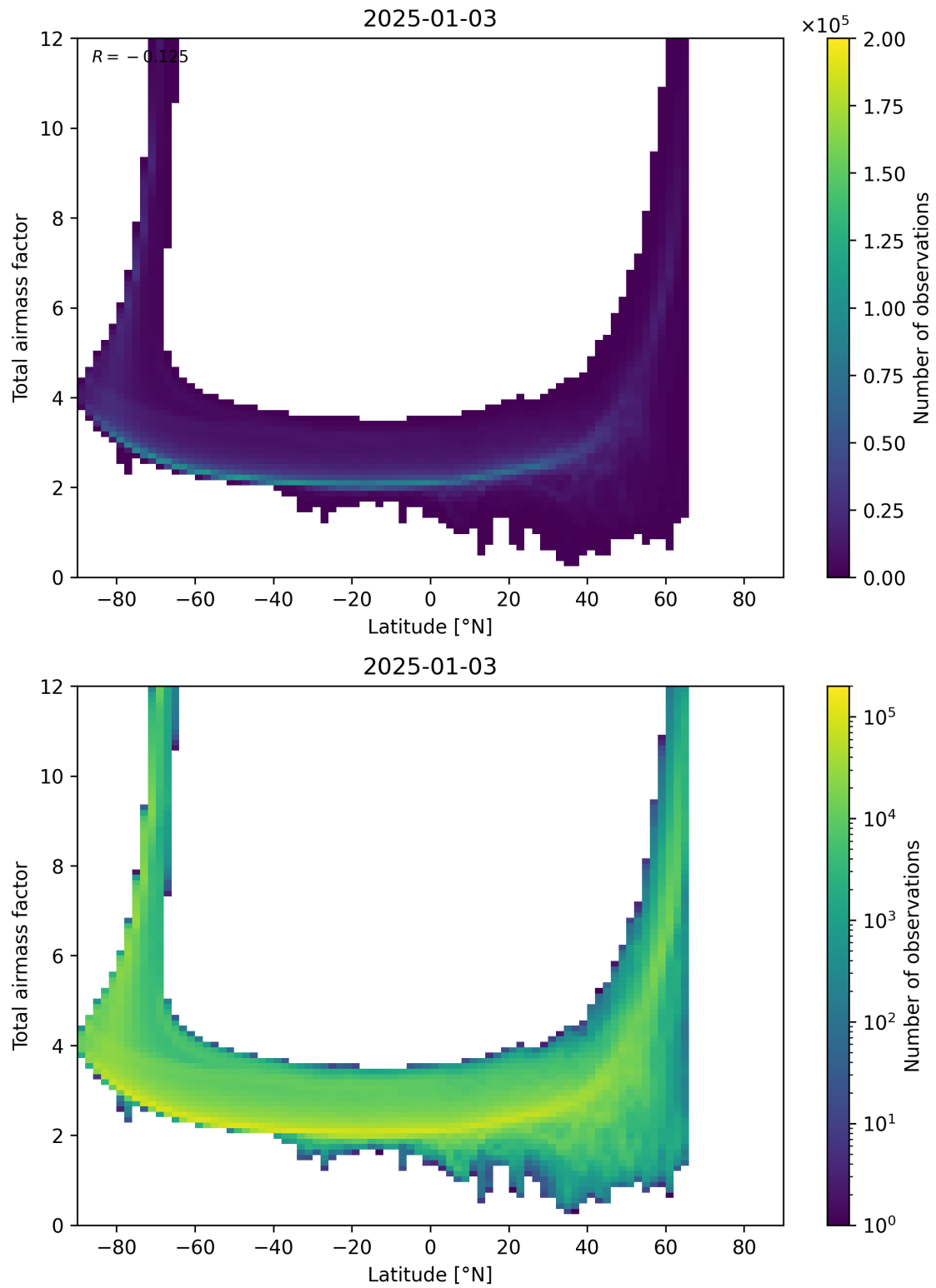
Figure 84: Scatter density plot of “Latitude” against “Total airmass factor” for 2025-01-02 to 2025-01-04.
