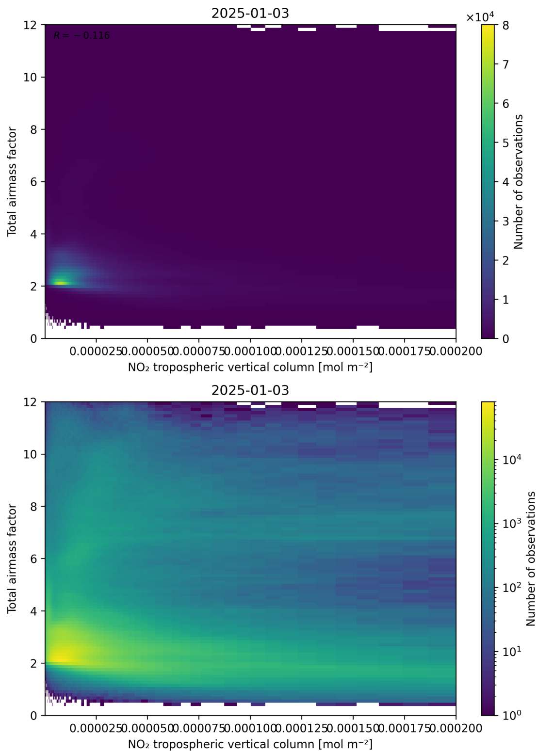
Figure 122: Scatter density plot of “NO 2 tropospheric vertical column” against “Total air mass factor” for 2025-01-02 to 2025-01-04.
