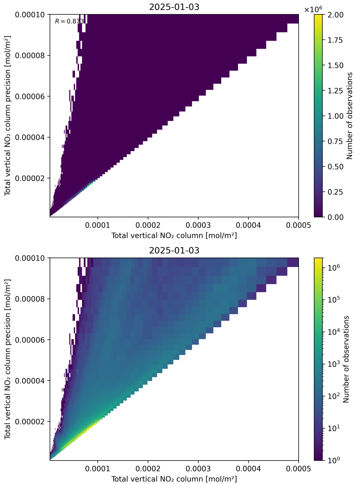
Figure 114: Scatter density plot of “Total vertical NO 2 column” against “Total vertical NO 2 column precision” for 2025-01-02 to 2025-01-04.
