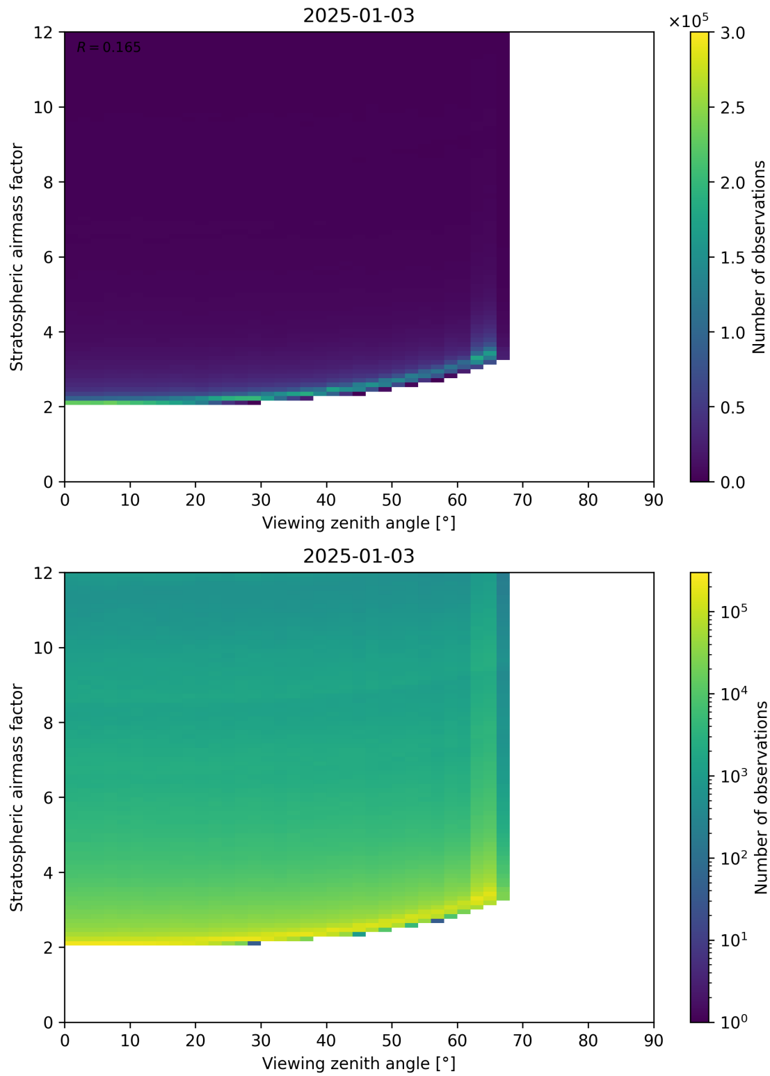
Figure 159: Scatter density plot of “Viewing zenith angle” against “Stratospheric airmass factor” for 2025-01-02 to 2025-01-04.
