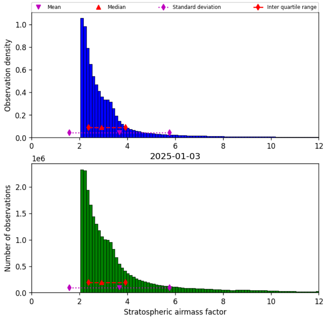
Figure 44: Histogram of “Stratospheric airmass factor” for 2025-01-02 to 2025-01-04
