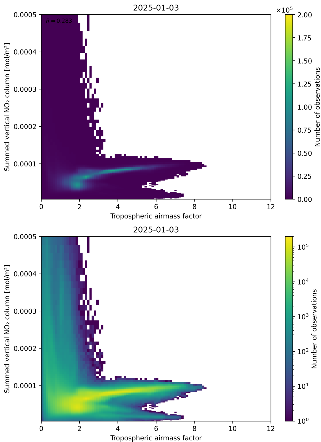
Figure 75: Scatter density plot of “Tropospheric airmass factor” against “Summed vertical NO 2 column” for 2025-01-02 to 2025-01-04.
