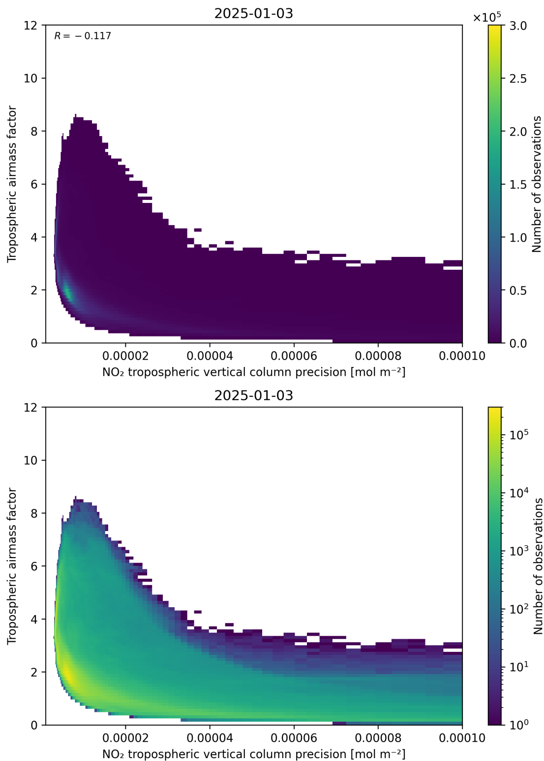
Figure 133: Scatter density plot of “NO 2 tropospheric vertical column precision” against “Tropospheric airmass factor” for 2025-01-02 to 2025-01-04.
