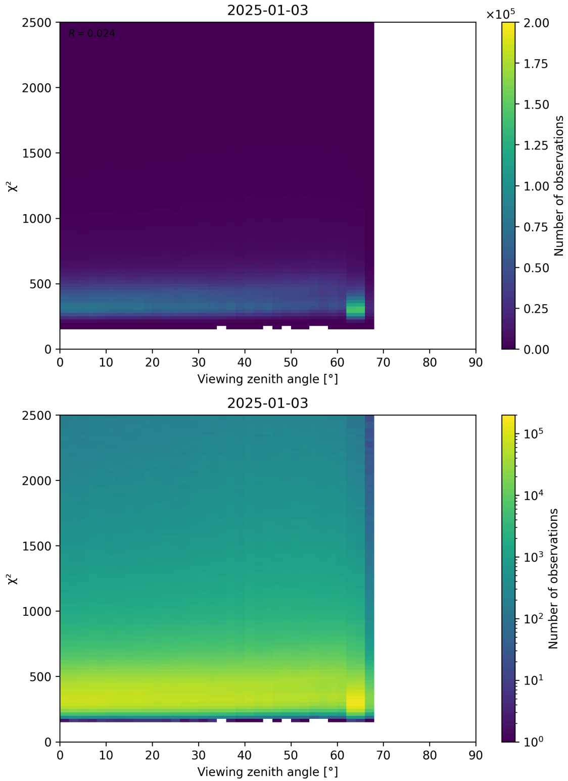
Figure 162: Scatter density plot of “Viewing zenith angle” against “ \chi^2 ” for 2025-01-02 to 2025-01-04.
