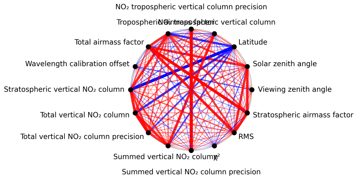
Figure 1: Map of correlation graph for 2025-01-02 to 2025-01-04.
