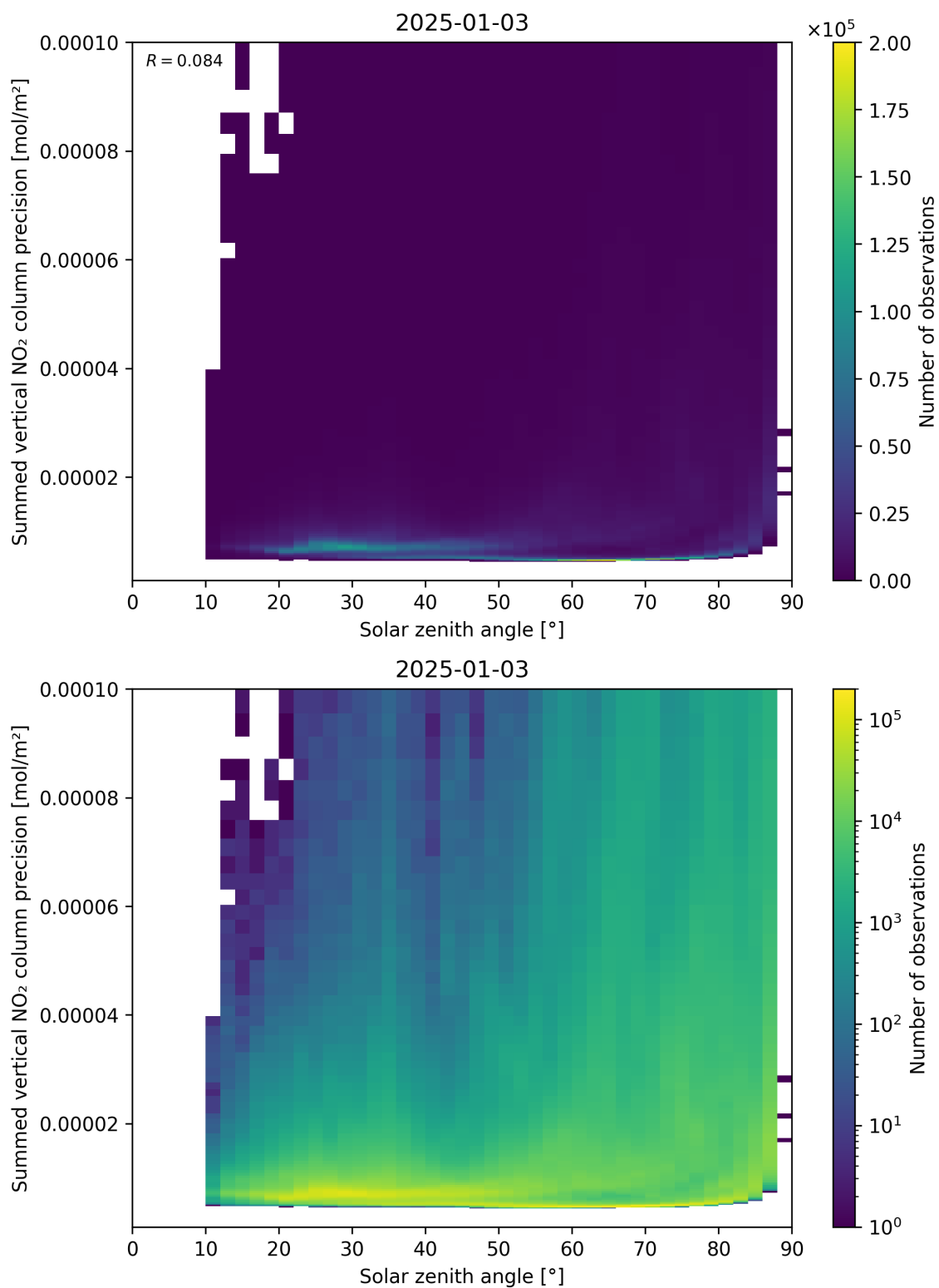
Figure 152: Scatter density plot of “Solar zenith angle” against “Summed vertical NO 2 column precision” for 2025-01-02 to 2025-01-04.
