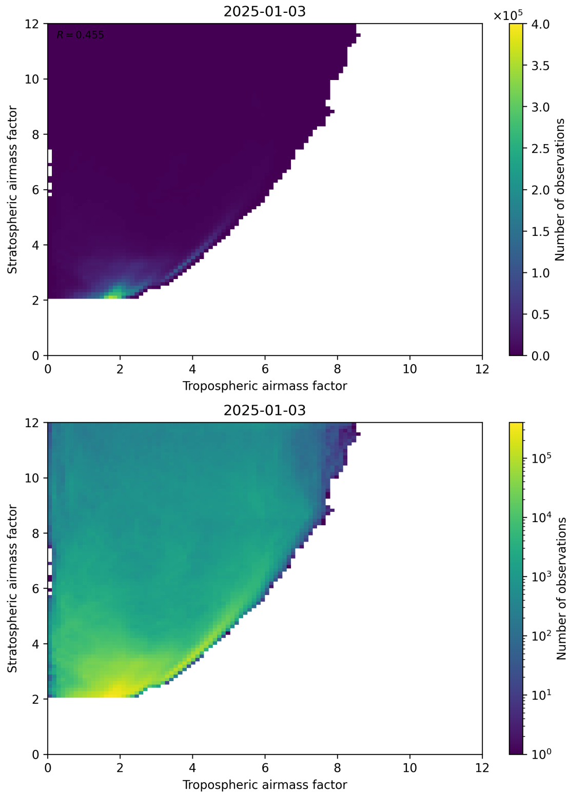
Figure 71: Scatter density plot of “Tropospheric airmass factor” against “Stratospheric airmass factor” for 2025-01-02 to 2025-01-04.
