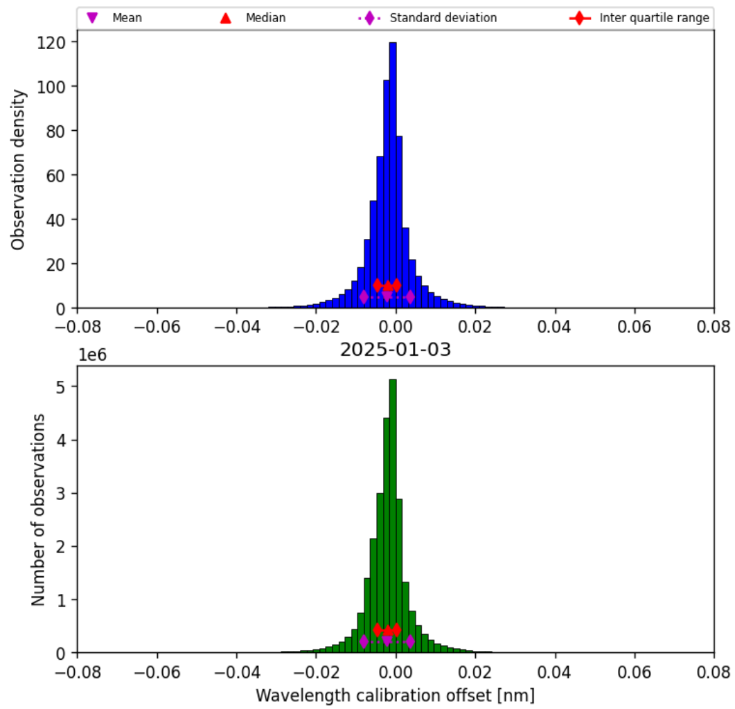
Figure 35: Histogram of “Wavelength calibration offset” for 2025-01-02 to 2025-01-04
