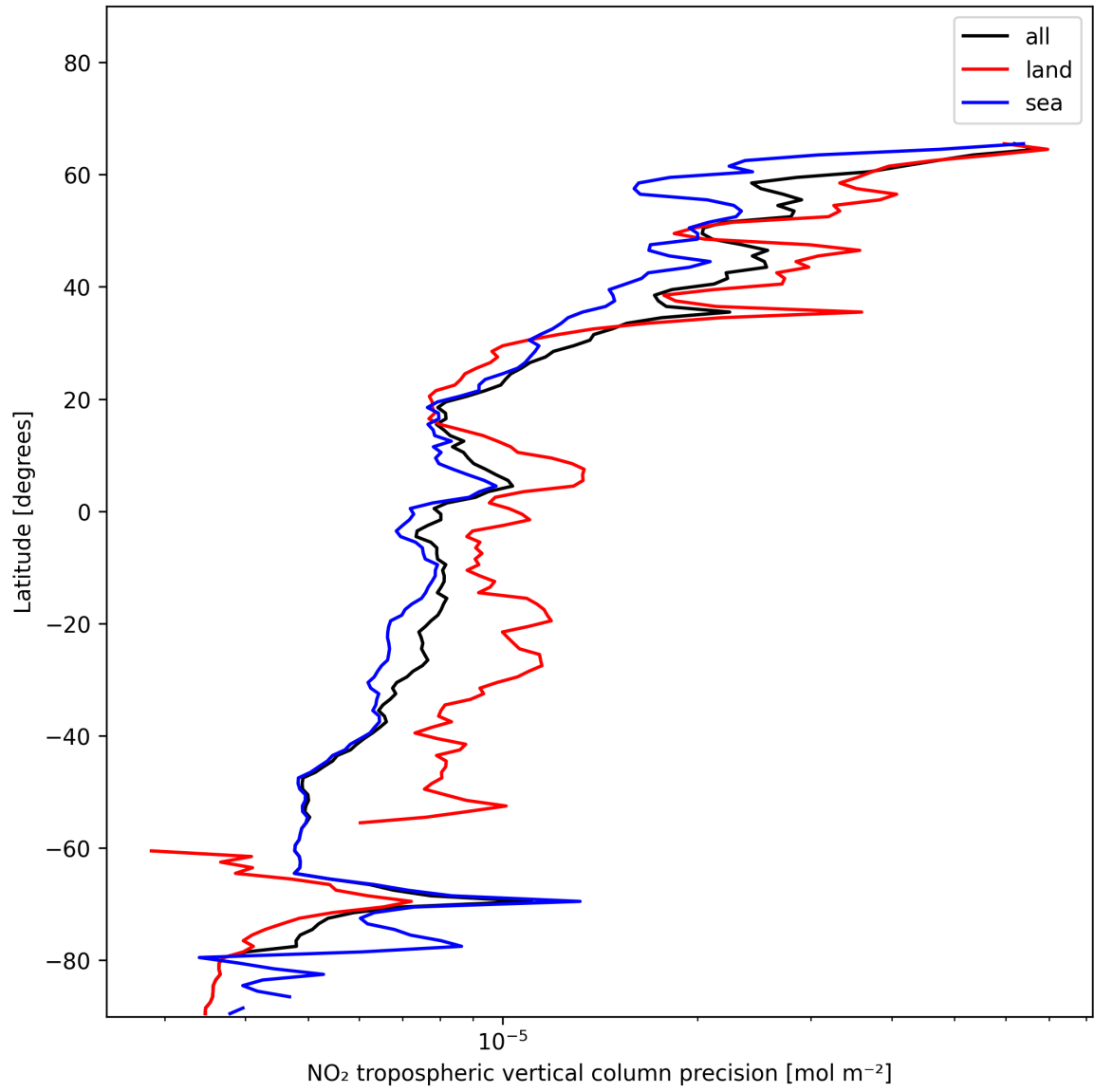
Figure 13: Zonal average of “NO 2 tropospheric vertical column precision” for 2025-01-02 to 2025-01-04.
