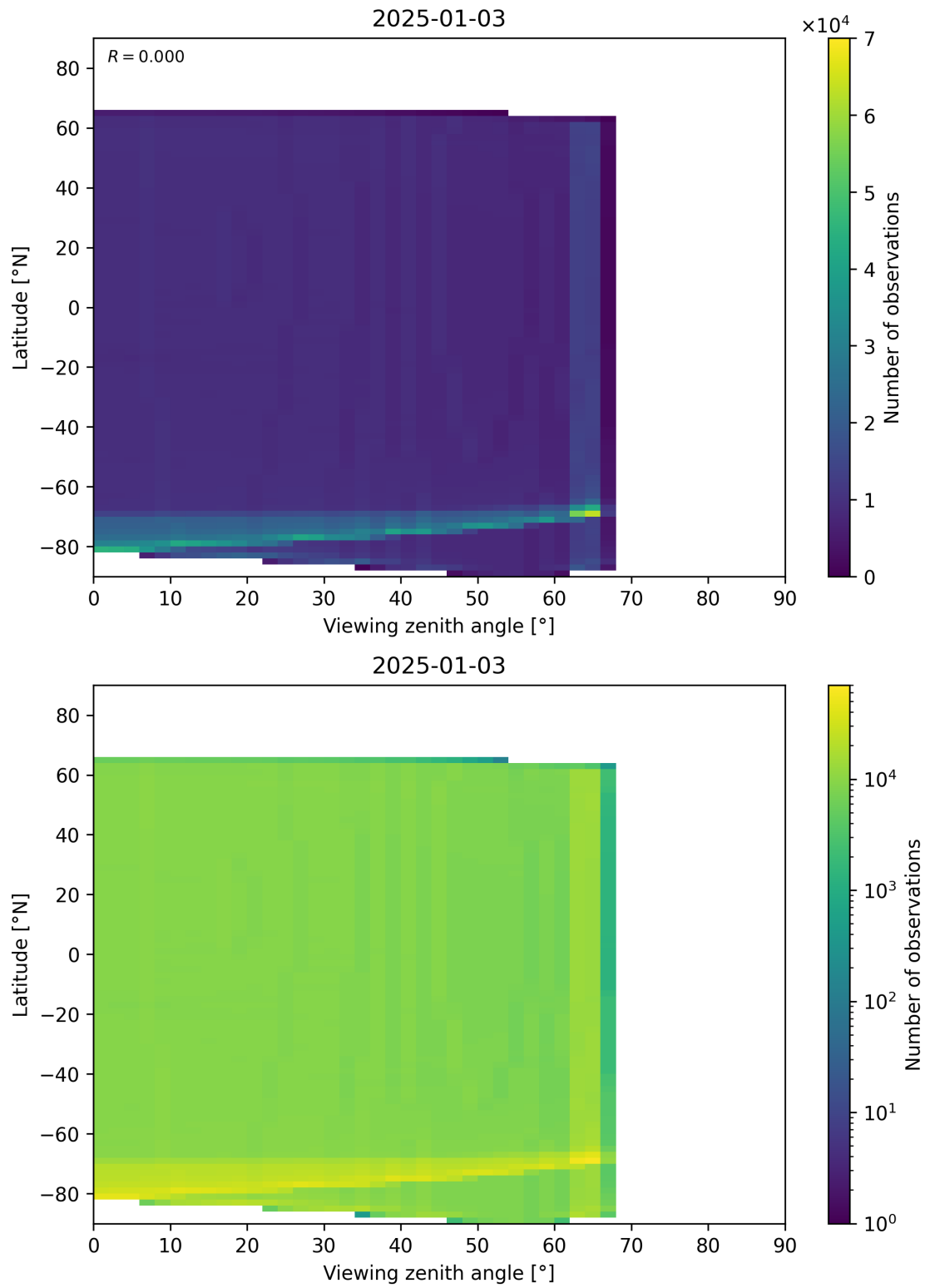
Figure 163: Scatter density plot of “Viewing zenith angle” against “Latitude” for 2025-01-02 to 2025-01-04.
