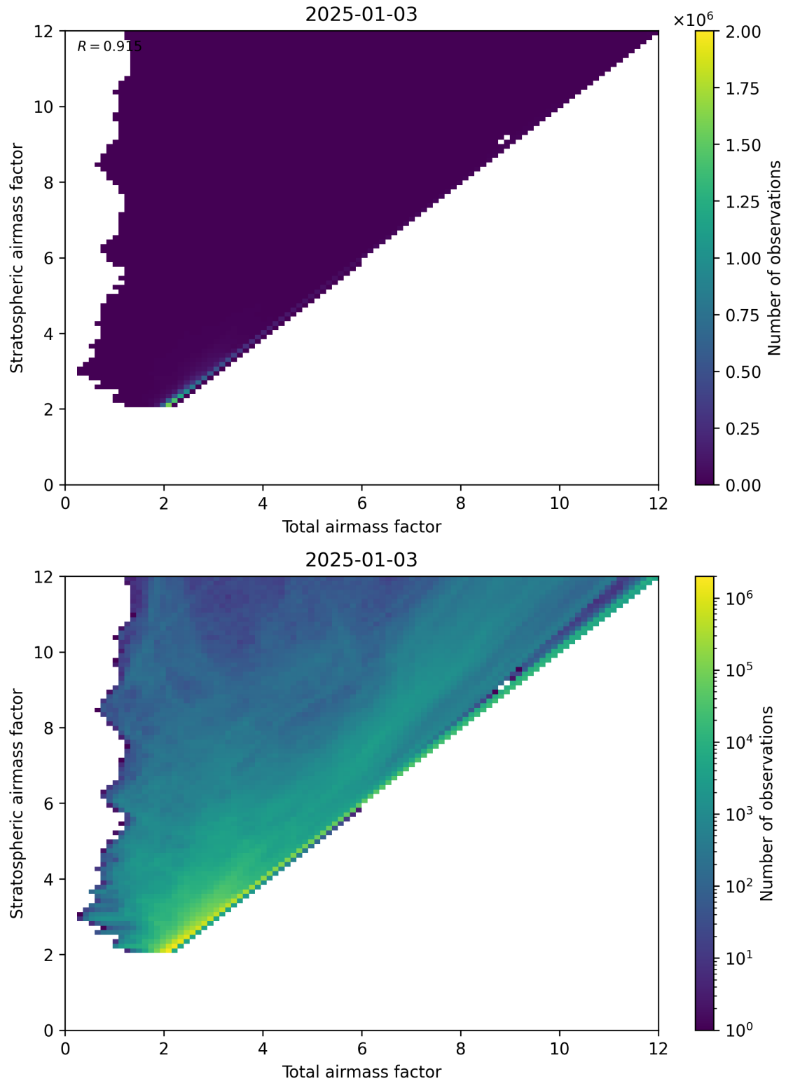
Figure 62: Scatter density plot of “Total airmass factor” against “Stratospheric airmass factor” for 2025-01-02 to 2025-01-04.
