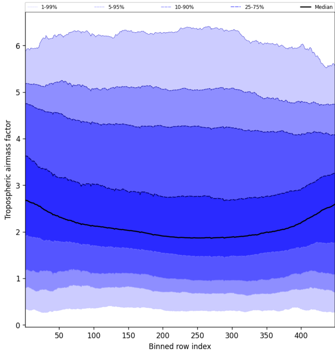
Figure 48: Along track statistics of “Tropospheric air mass factor” for 2025-01-02 to 2025-01-04
