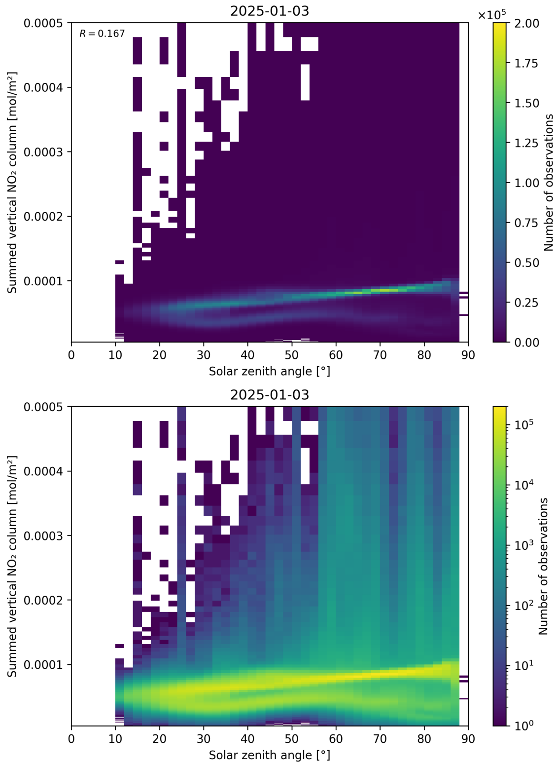
Figure 151: Scatter density plot of “Solar zenith angle” against “Summed vertical NO 2 column” for 2025-01-02 to 2025-01-04.
