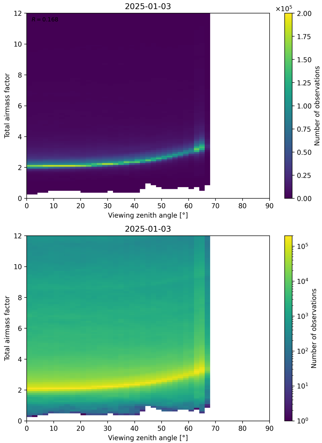
Figure 160: Scatter density plot of “Viewing zenith angle” against “Total airmass factor” for 2025-01-02 to 2025-01-04.
