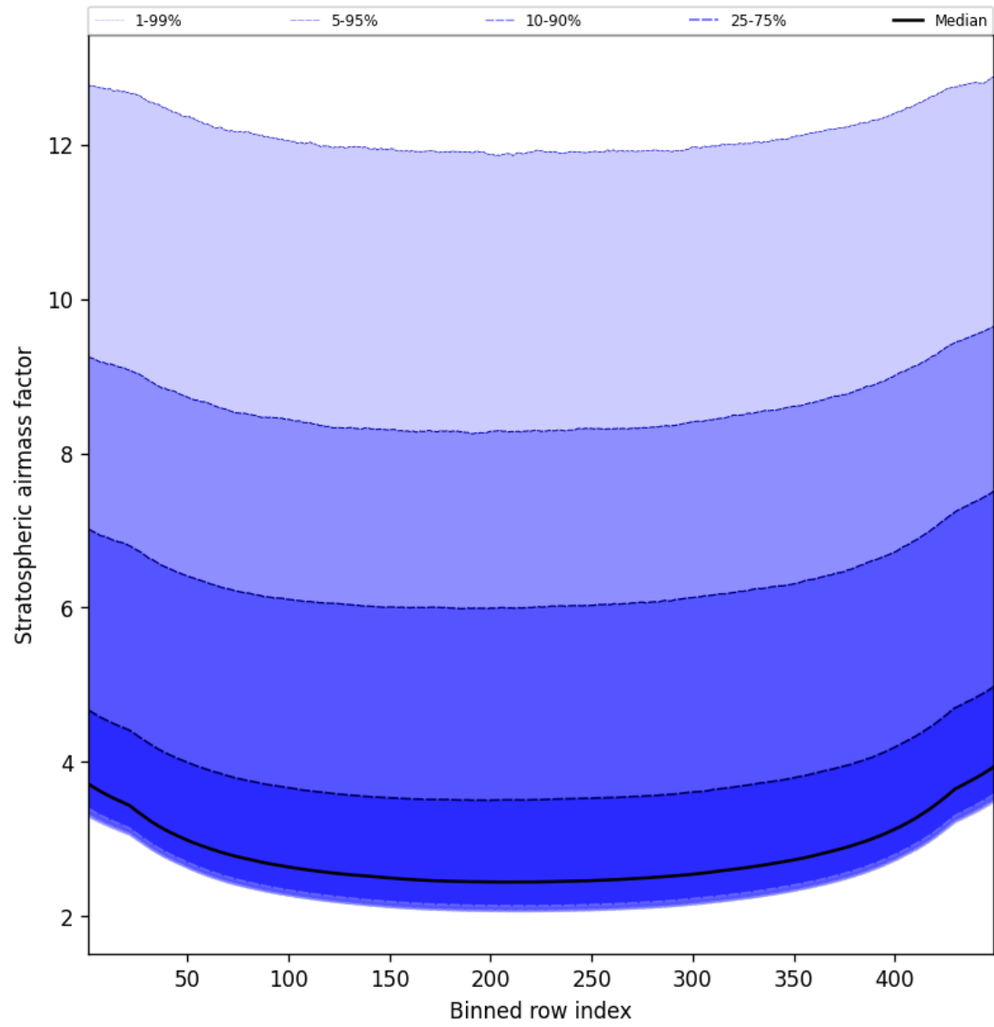
Figure 61: Along track statistics of “Stratospheric air mass factor” for 2025-01-02 to 2025-01-04
