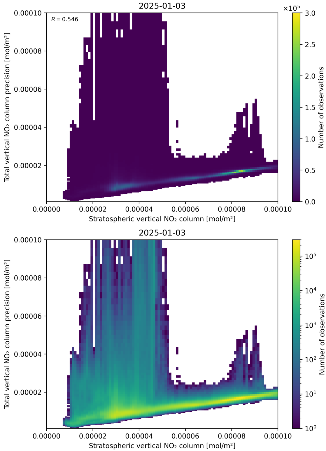
Figure 101: Scatter density plot of “Stratospheric vertical NO 2 column” against “Total vertical NO 2 column precision” for 2025-01-02 to 2025-01-04.
