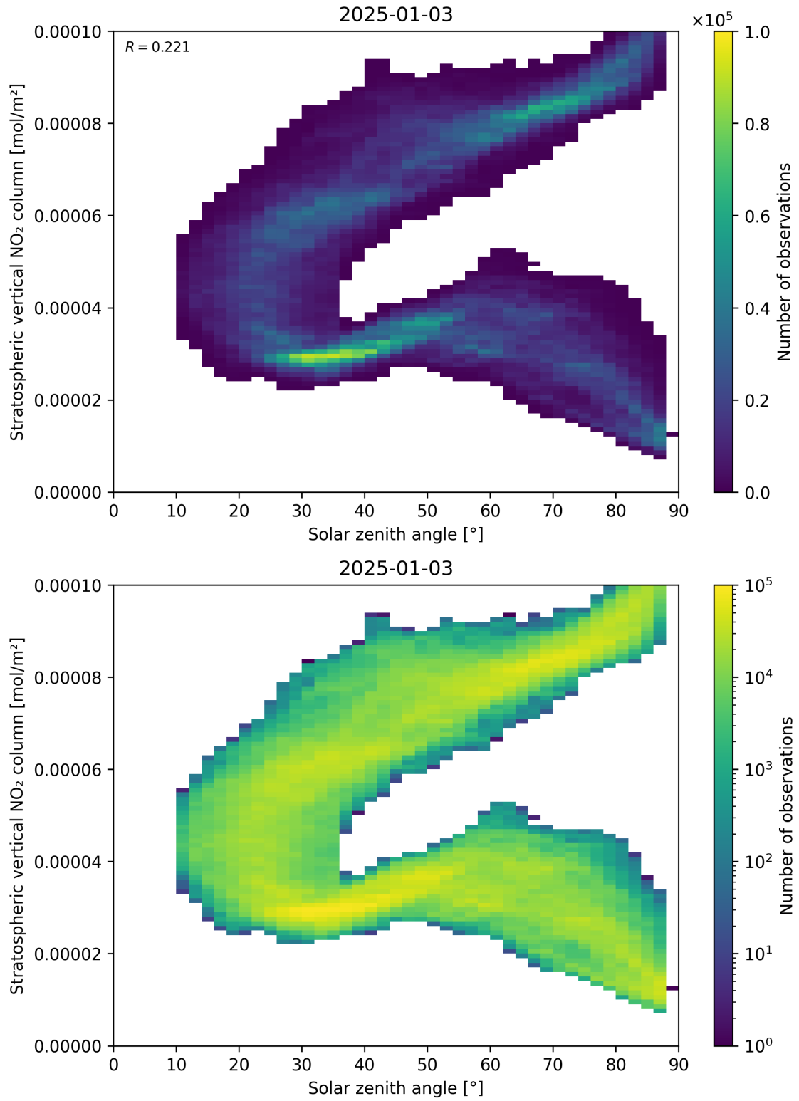
Figure 150: Scatter density plot of “Solar zenith angle” against “Stratospheric vertical NO 2 column” for 2025-01-02 to 2025-01-04.
