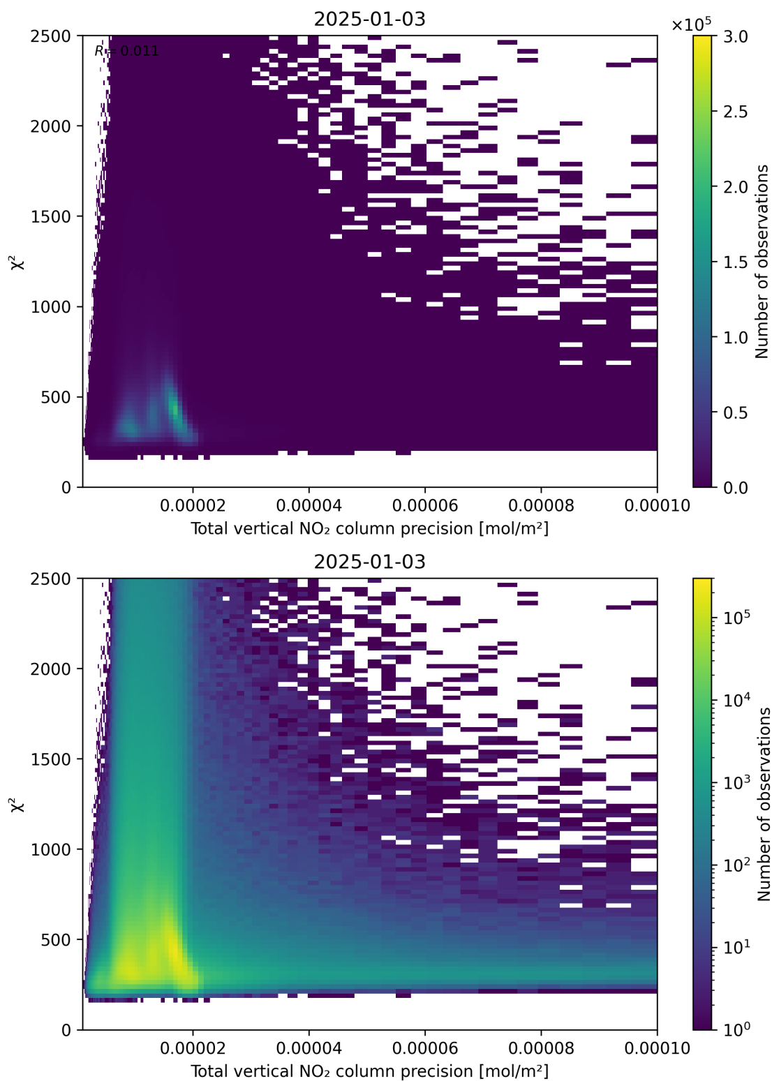
Figure 116: Scatter density plot of “Total vertical NO 2 column precision” against “ \chi^2 ” for 2025-01-02 to 2025-01-04.
