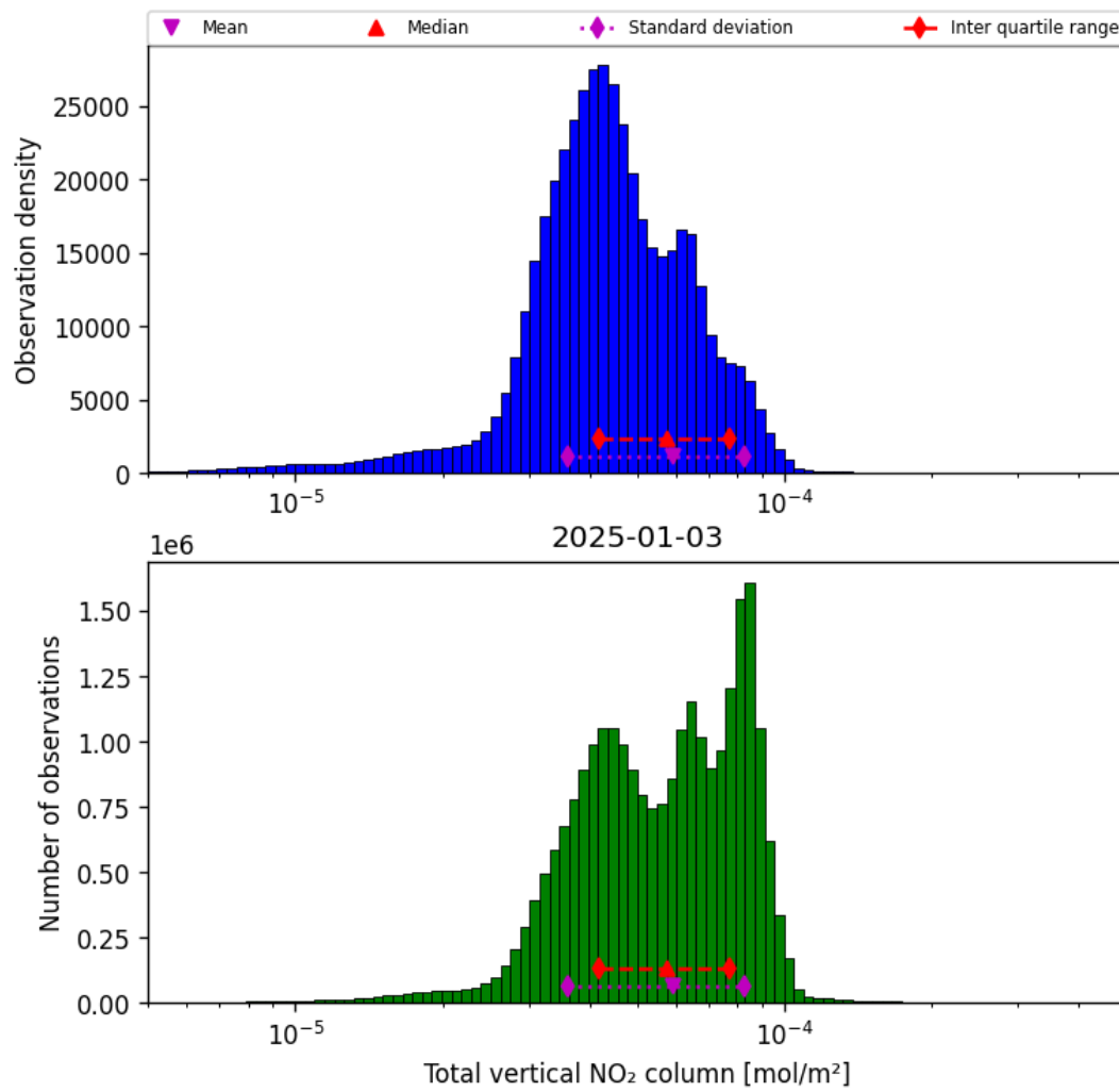
Figure 38: Histogram of “Total vertical NO 2 column” for 2025-01-02 to 2025-01-04
