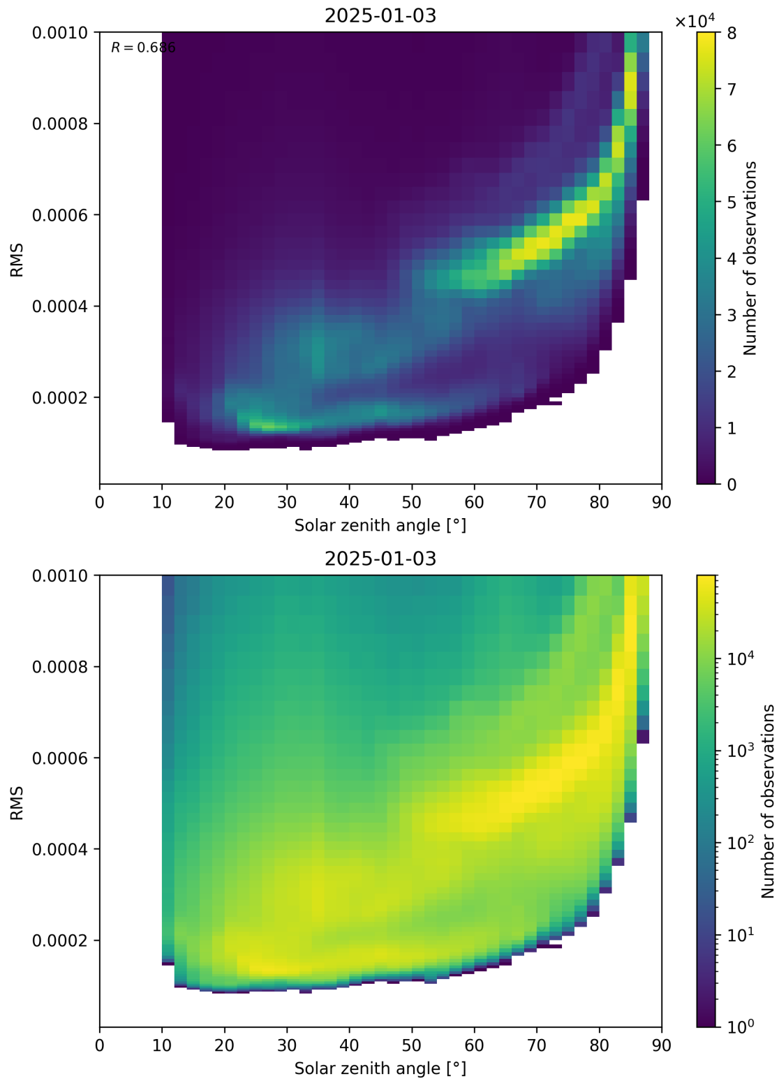
Figure 157: Scatter density plot of “Solar zenith angle” against “RMS” for 2025-01-02 to 2025-01-04.
