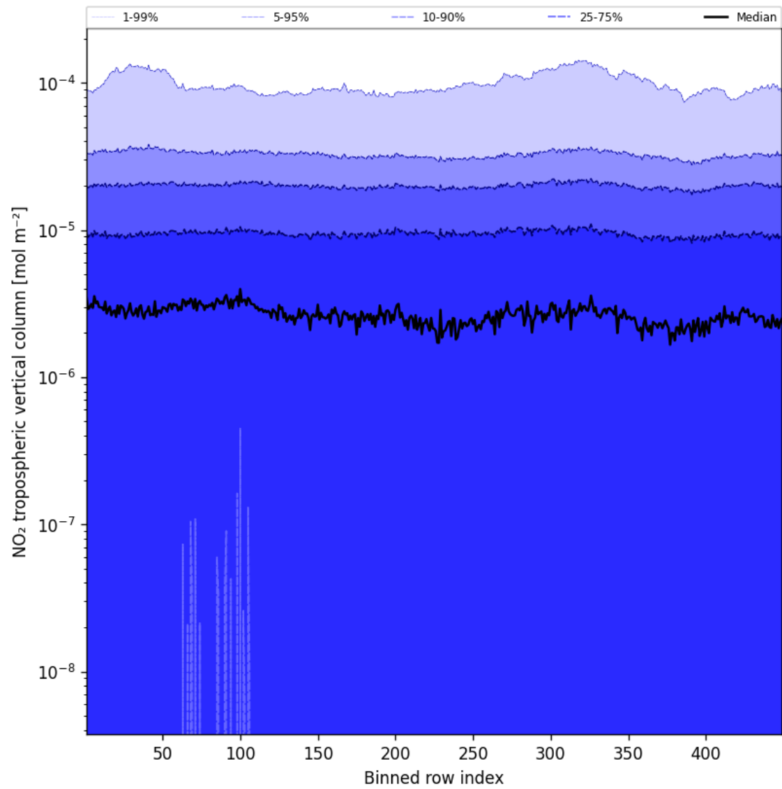
Figure 46: Along track statistics of “NO 2 tropospheric vertical column” for 2025-01-02 to 2025-01-04
