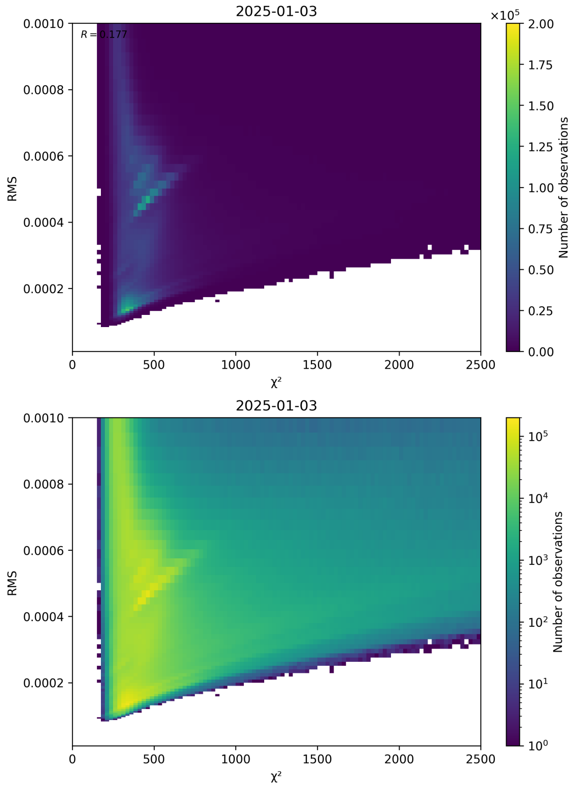
Figure 82: Scatter density plot of “ \chi^2 ” against “RMS” for 2025-01-02 to 2025-01-04.
