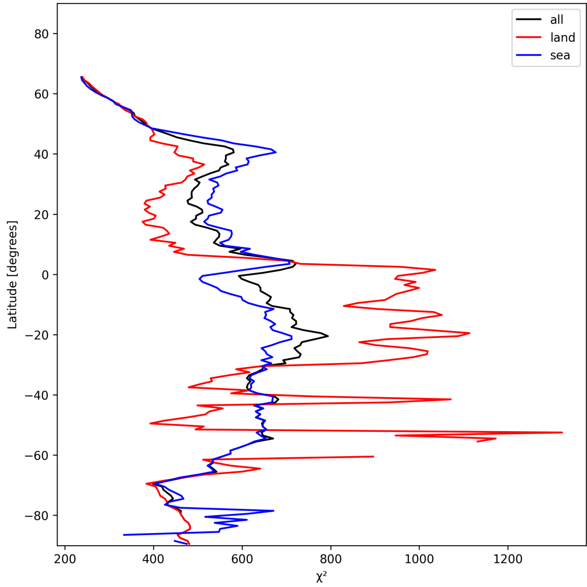
Figure 25: Zonal average of “ \chi^2 ” for 2025-01-02 to 2025-01-04.
