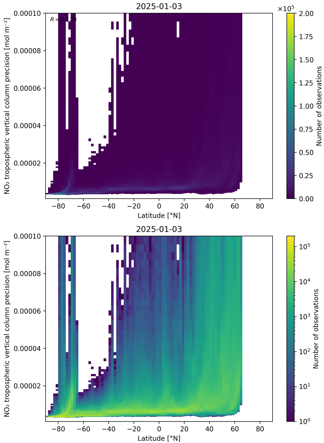
Figure 93: Scatter density plot of “Latitude” against “NO 2 tropospheric vertical column precision” for 2025-01-02 to 2025-01-04.
