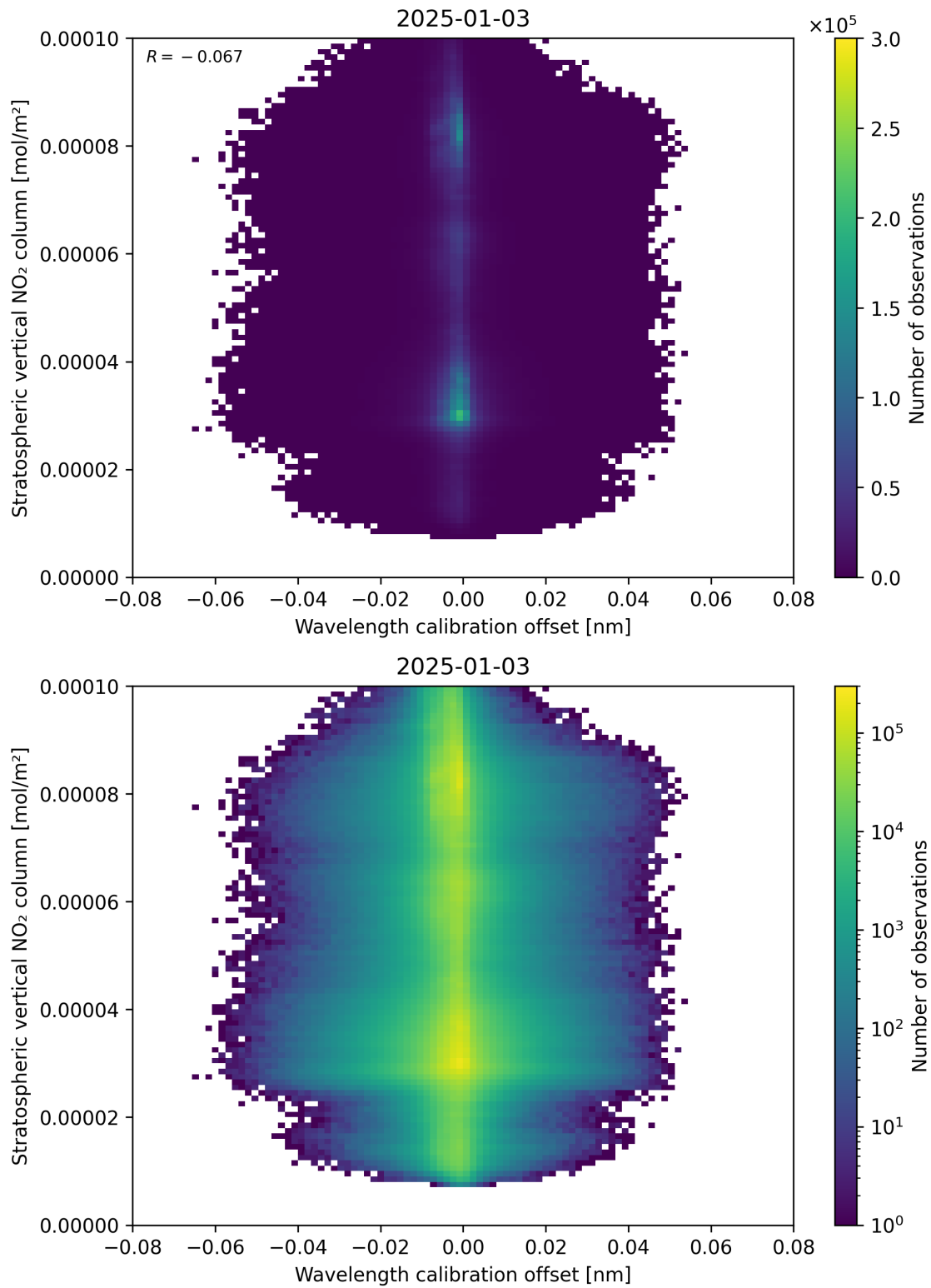
Figure 176: Scatter density plot of “Wavelength calibration offset” against “Stratospheric vertical NO 2 column” for 2025-01-02 to 2025-01-04.
