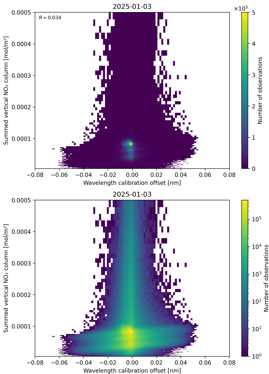
Figure 177: Scatter density plot of “Wavelength calibration offset” against “Summed vertical NO 2 column” for 2025-01-02 to 2025-01-04.
