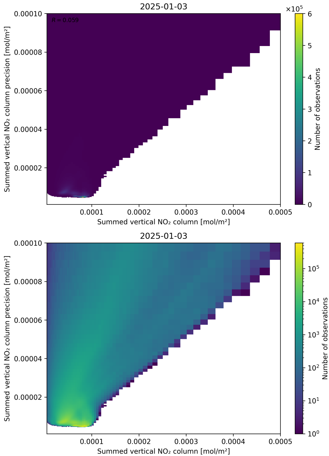
Figure 105: Scatter density plot of “Summed vertical NO 2 column” against “Summed vertical NO 2 column precision” for 2025-01-02 to 2025-01-04.
