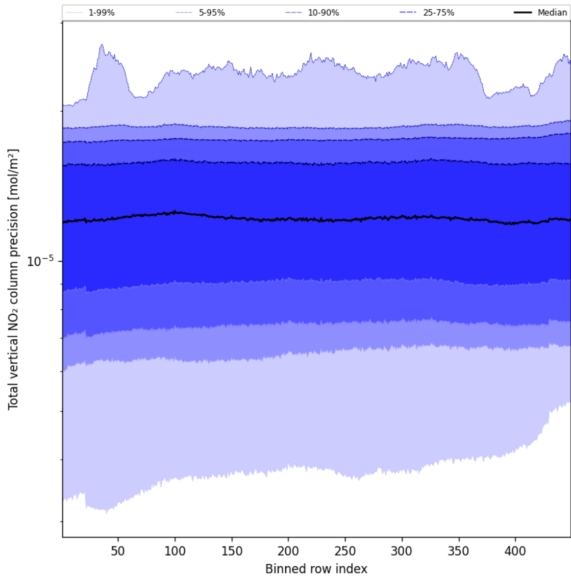
Figure 56: Along track statistics of “Total vertical NO 2 column precision” for 2025-01-02 to 2025-01-04
