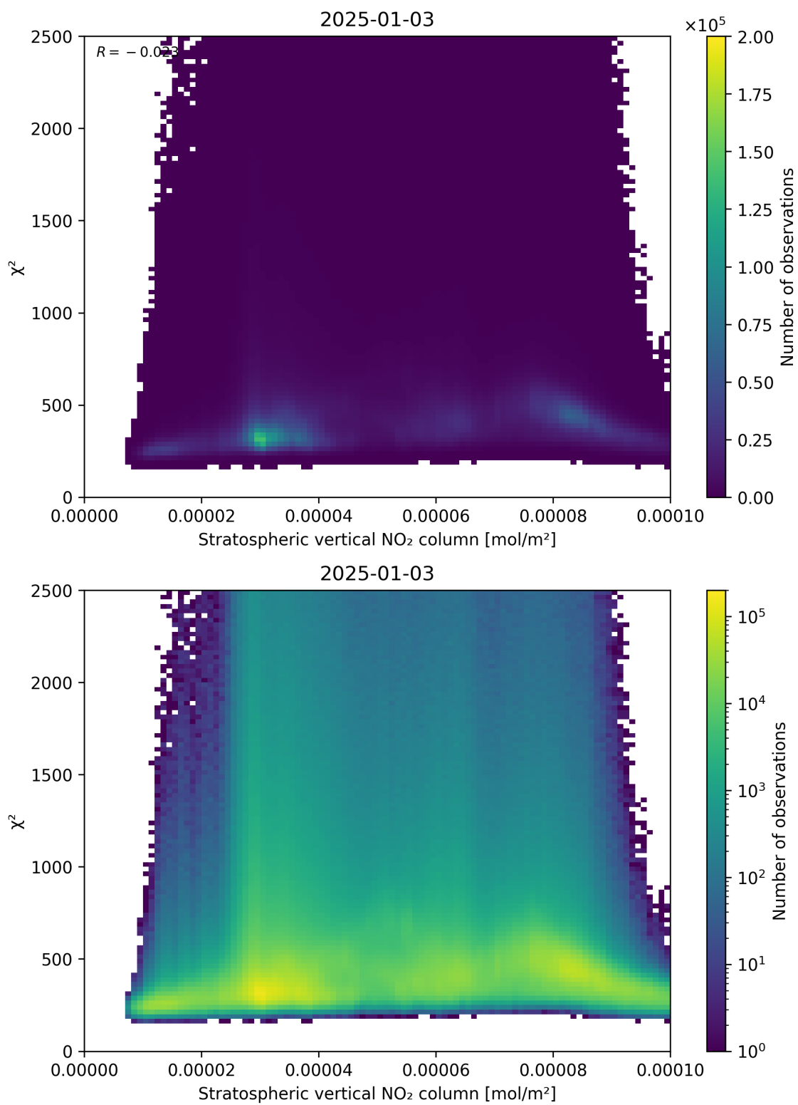
Figure 97: Scatter density plot of “Stratospheric vertical NO 2 column” against “ \chi^2 ” for 2025-01-02 to 2025-01-04.
