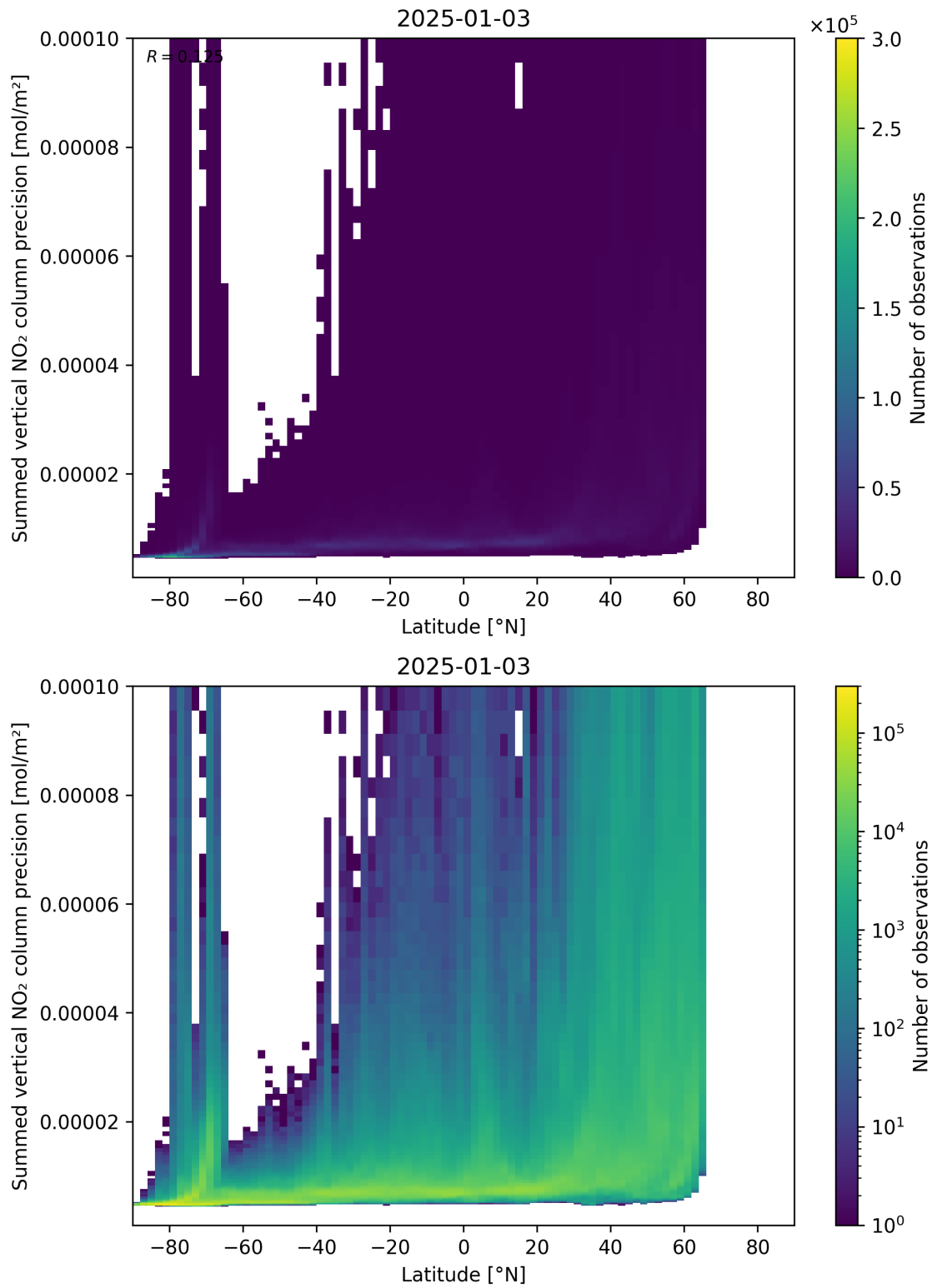
Figure 89: Scatter density plot of “Latitude” against “Summed vertical NO 2 column precision” for 2025-01-02 to 2025-01-04.
