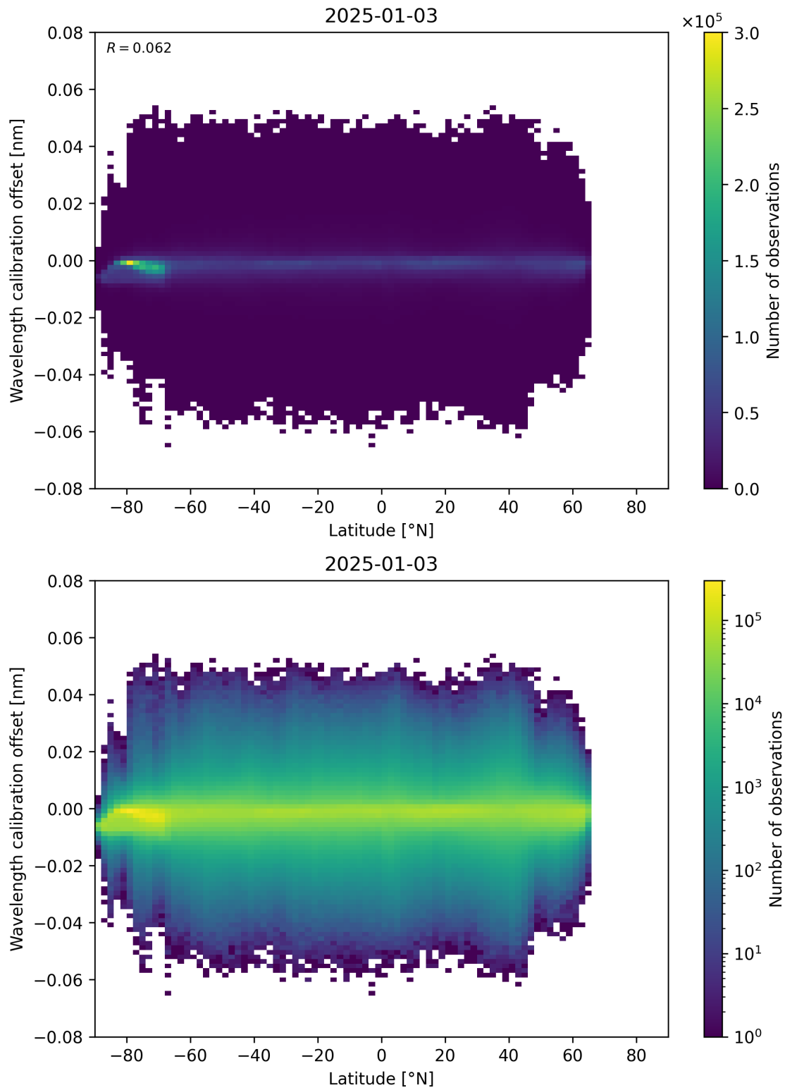
Figure 95: Scatter density plot of “Latitude” against “Wavelength calibration offset” for 2025-01-02 to 2025-01-04.
