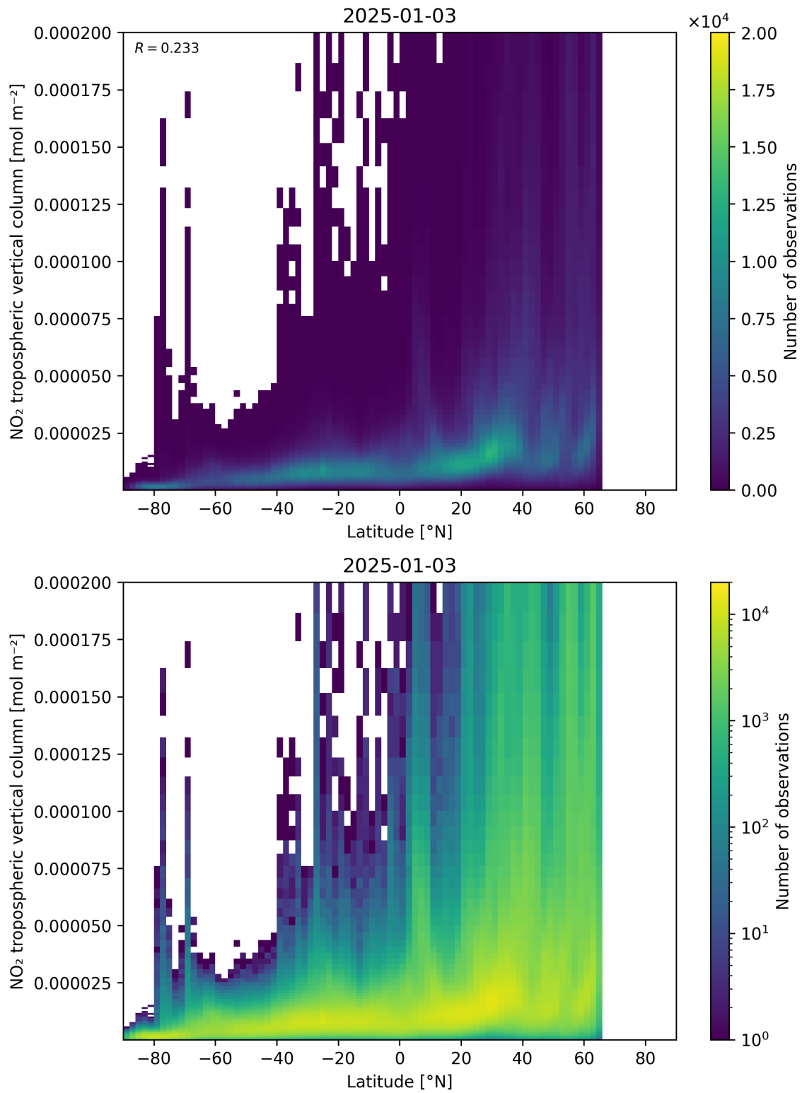
Figure 92: Scatter density plot of “Latitude” against “NO 2 tropospheric vertical column” for 2025-01-02 to 2025-01-04.
