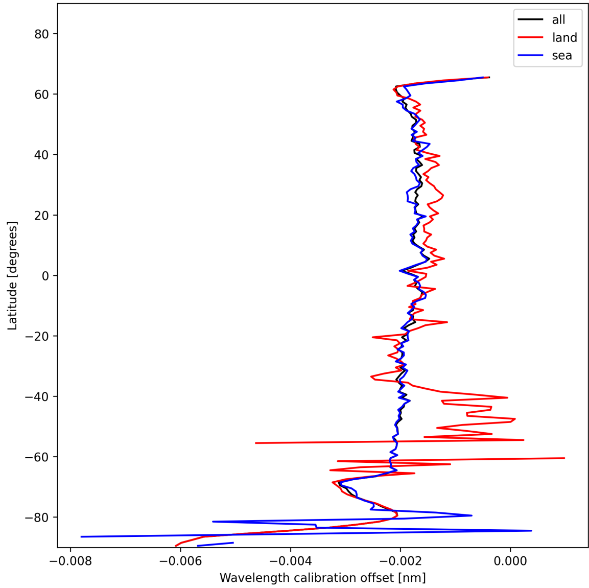
Figure 18: Zonal average of “Wavelength calibration offset” for 2025-01-02 to 2025-01-04.
