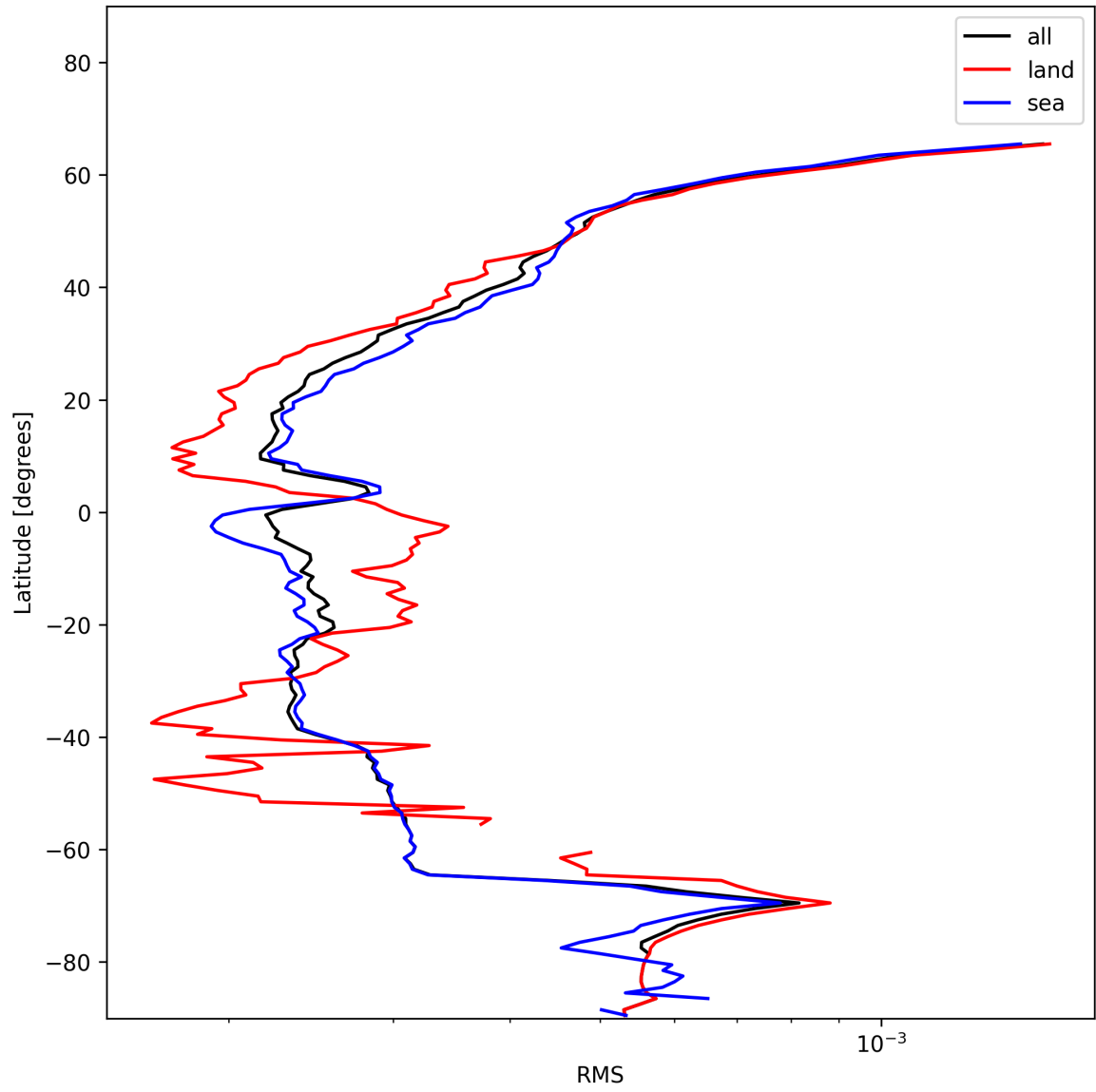
Figure 26: Zonal average of “RMS” for 2025-01-02 to 2025-01-04.
