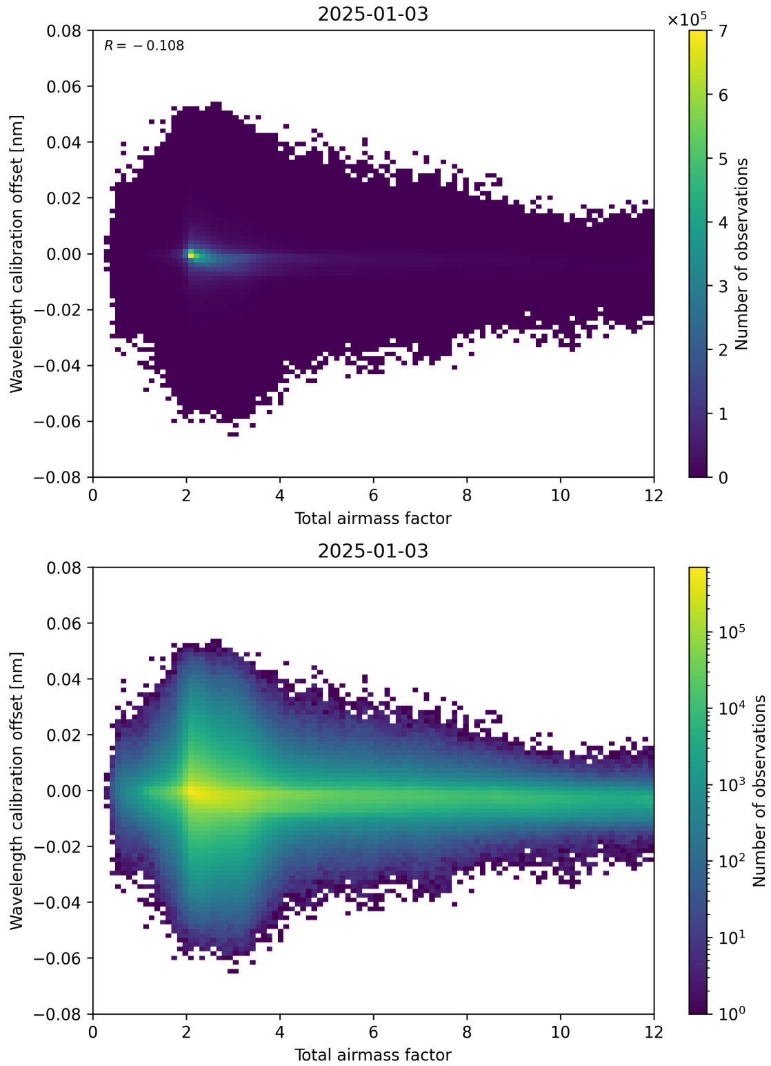
Figure 70: Scatter density plot of “Total airmass factor” against “Wavelength calibration offset” for 2025-01-02 to 2025-01-04.
