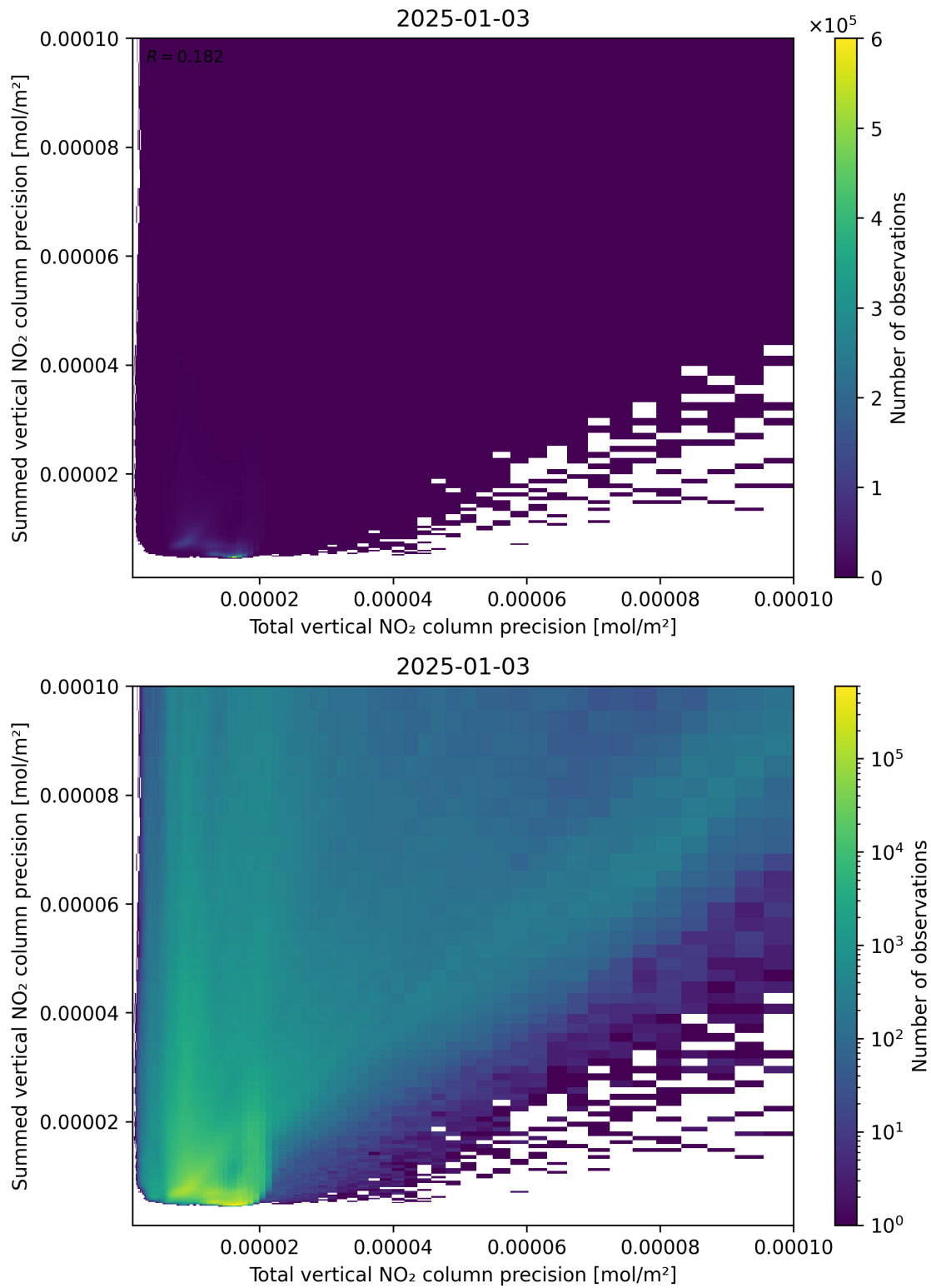
Figure 118: Scatter density plot of “Total vertical NO 2 column precision” against “Summed vertical NO 2 column precision” for 2025-01-02 to 2025-01-04.
