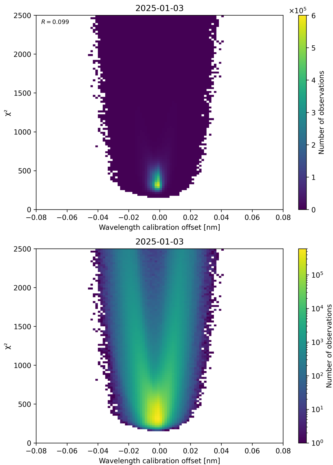
Figure 175: Scatter density plot of “Wavelength calibration offset” against “ \chi^2 ” for 2025-01-02 to 2025-01-04.
