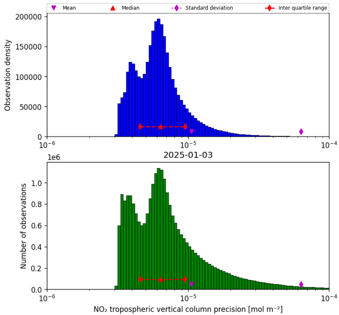
Figure 30: Histogram of “NO 2 tropospheric vertical column precision” for 2025-01-02 to 2025-01-04
