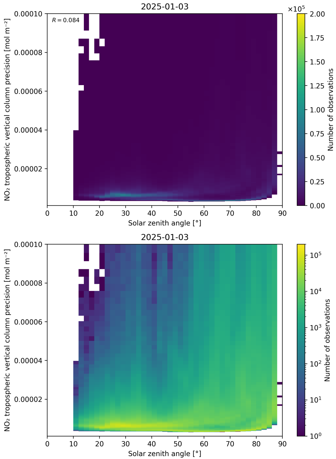
Figure 156: Scatter density plot of “Solar zenith angle” against “NO 2 tropospheric vertical column precision” for 2025-01-02 to 2025-01-04.
