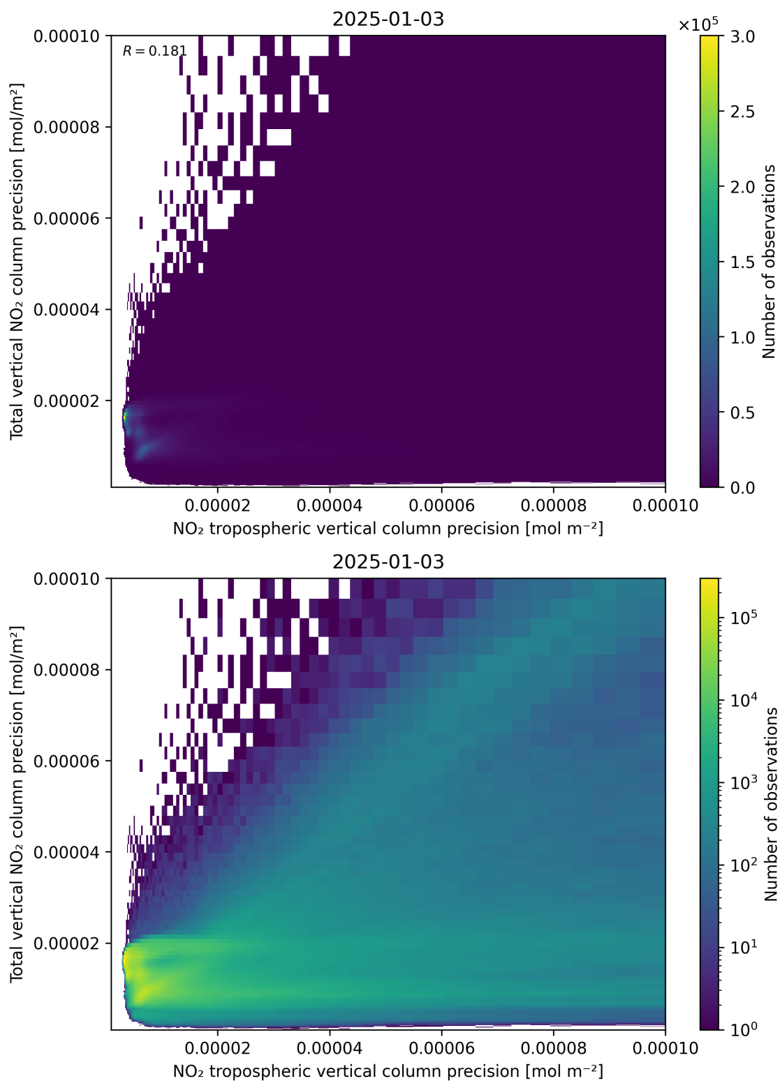
Figure 139: Scatter density plot of “NO 2 tropospheric vertical column precision” against “Total vertical NO 2 column precision” for 2025-01-02 to 2025-01-04.
