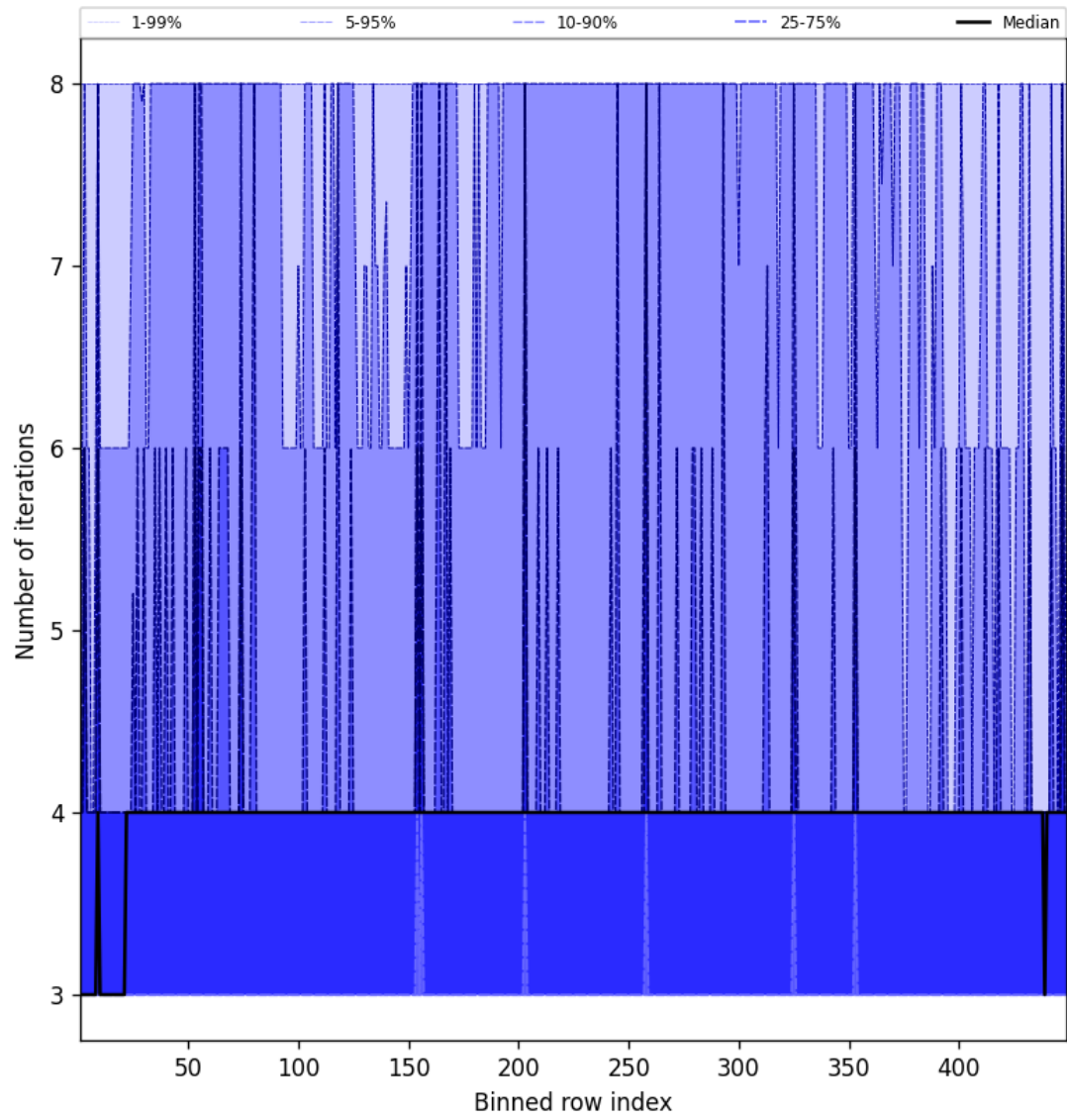
Figure 51: Along track statistics of “Number of iterations” for 2025-01-02 to 2025-01-04
