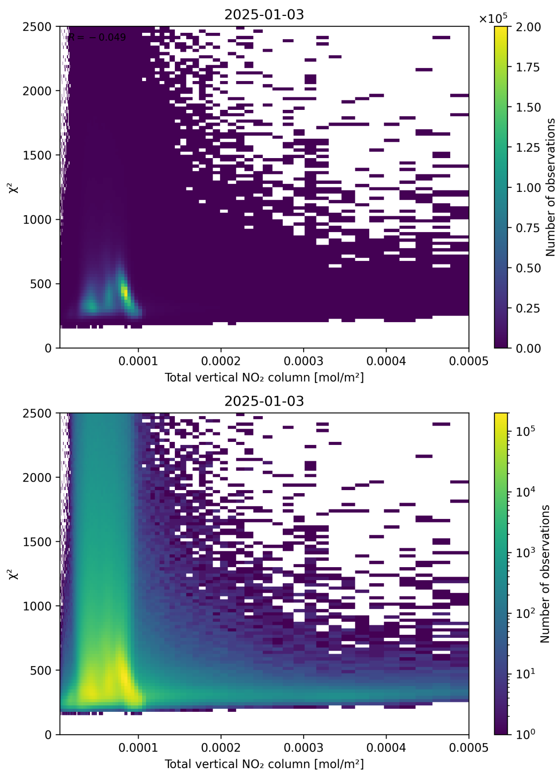
Figure 111: Scatter density plot of “Total vertical NO 2 column” against “ \chi^2 ” for 2025-01-02 to 2025-01-04.
