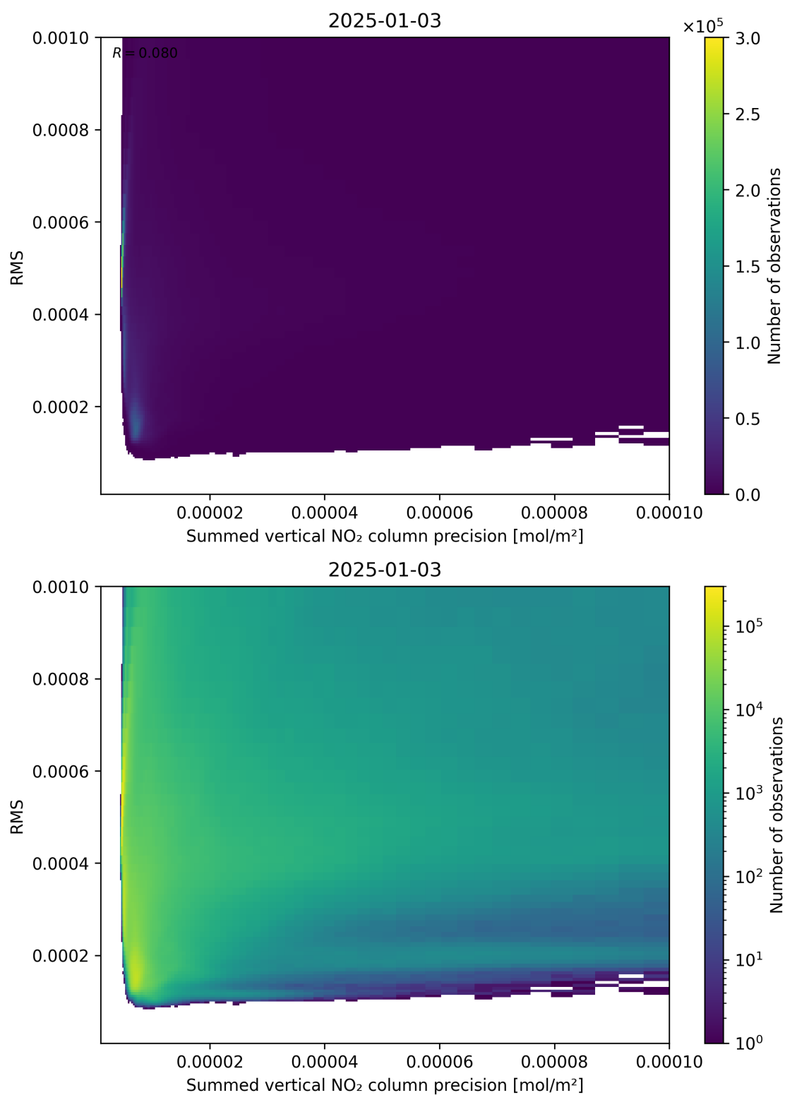
Figure 108: Scatter density plot of “Summed vertical NO 2 column precision” against “RMS” for 2025-01-02 to 2025-01-04.
