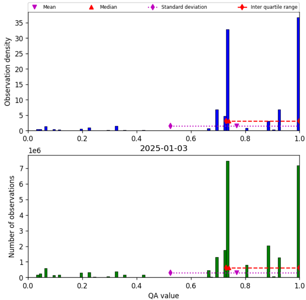
Figure 28: Histogram of “QA value” for 2025-01-02 to 2025-01-04
