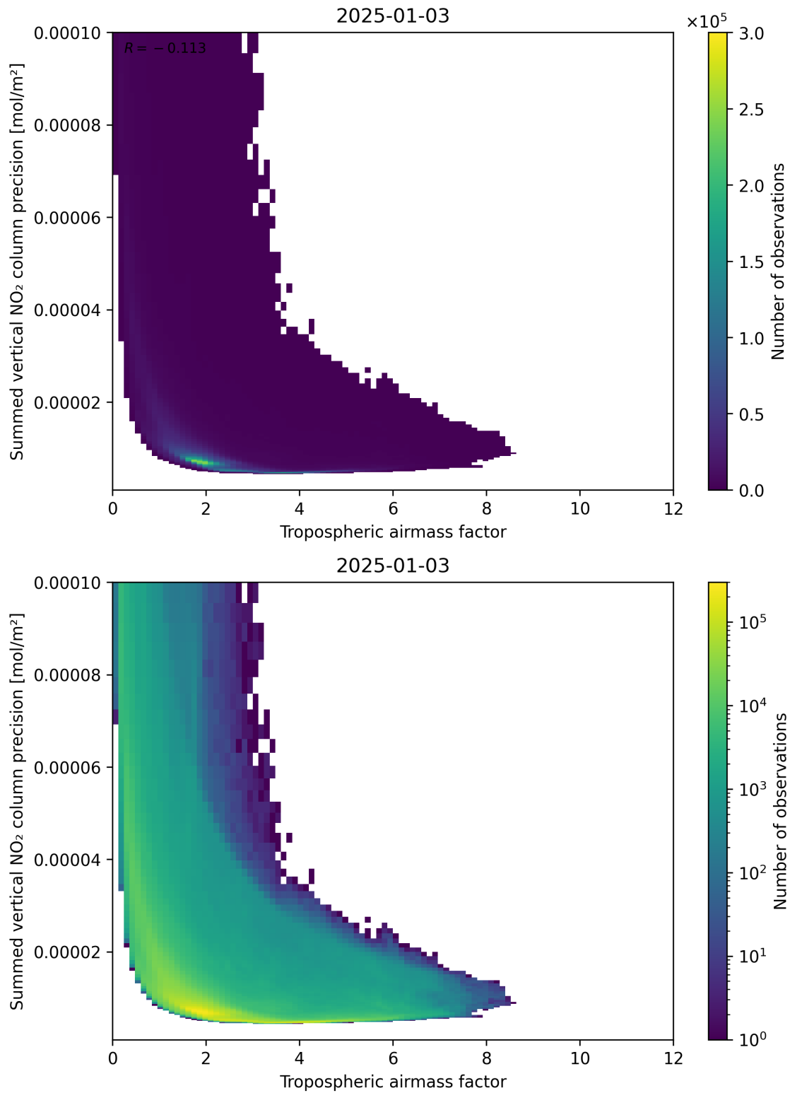
Figure 76: Scatter density plot of “Tropospheric air mass factor” against “Summed vertical NO 2 column precision” for 2025-01-02 to 2025-01-04.
