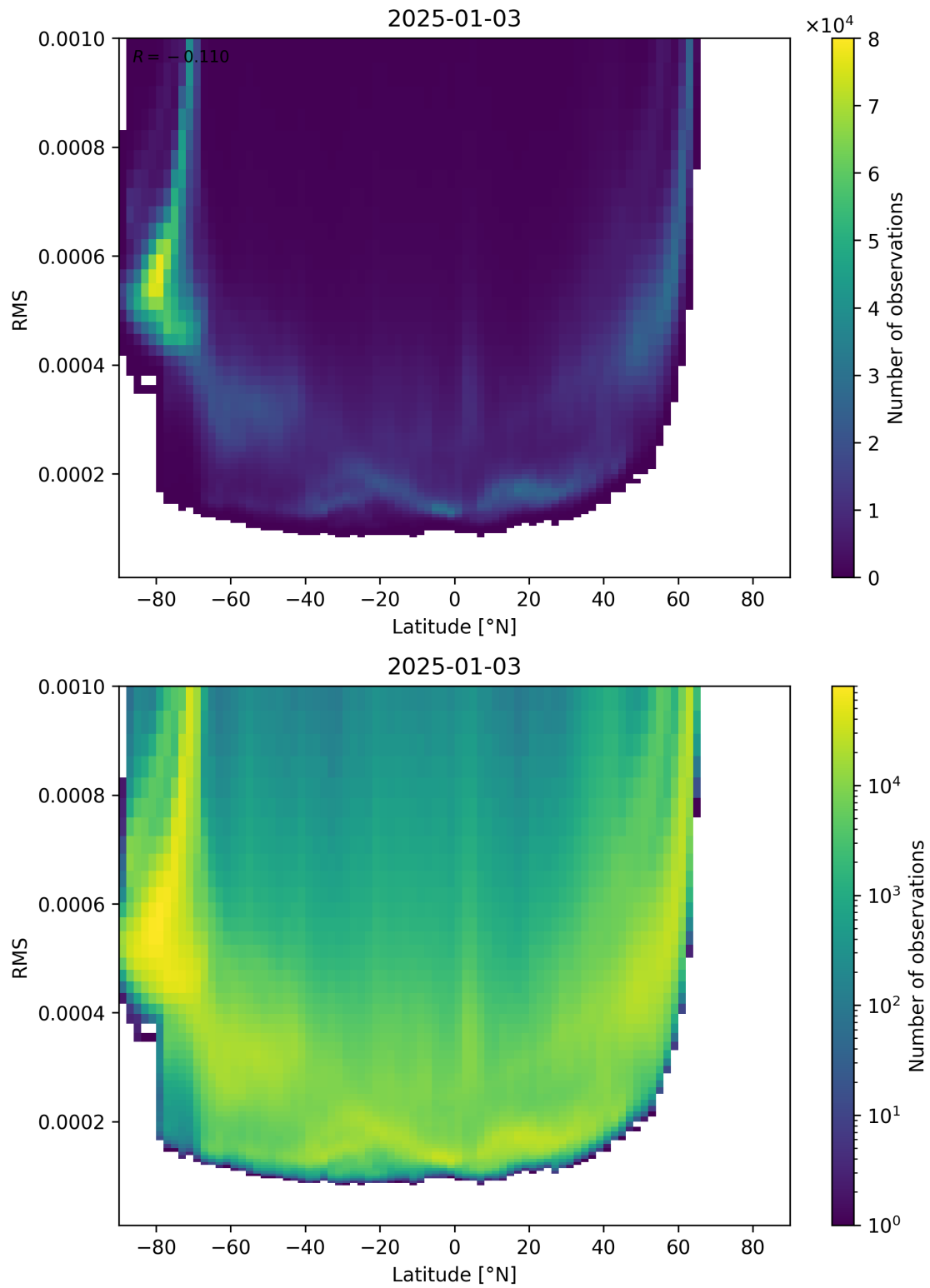
Figure 94: Scatter density plot of “Latitude” against “RMS” for 2025-01-02 to 2025-01-04.
