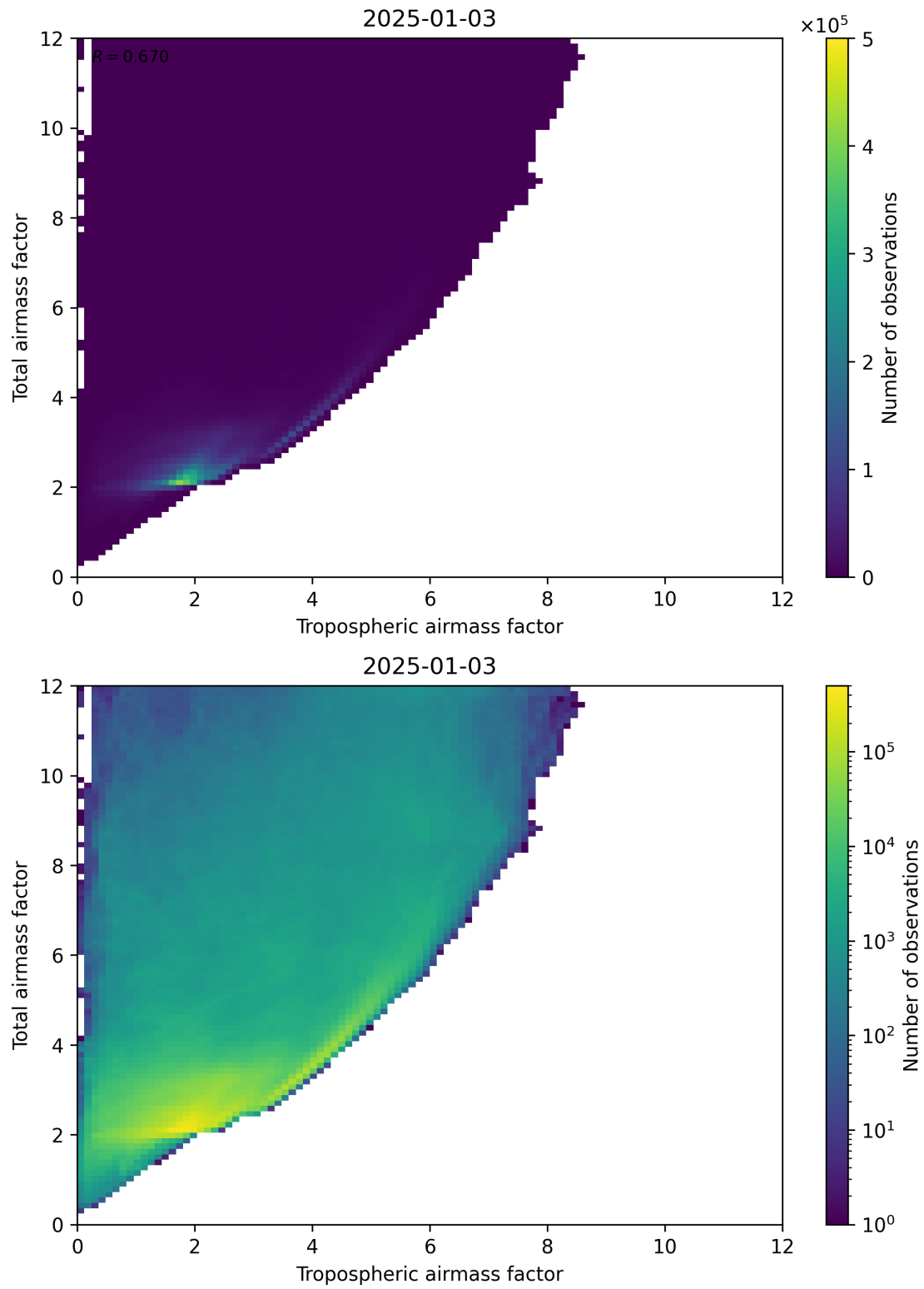
Figure 72: Scatter density plot of “Tropospheric airmass factor” against “Total airmass factor” for 2025-01-02 to 2025-01-04.
