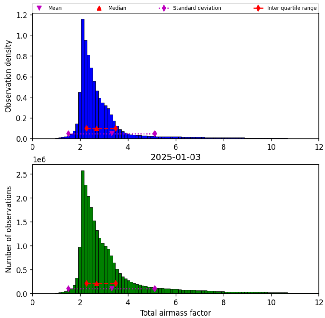
Figure 32: Histogram of “Total airmass factor” for 2025-01-02 to 2025-01-04
