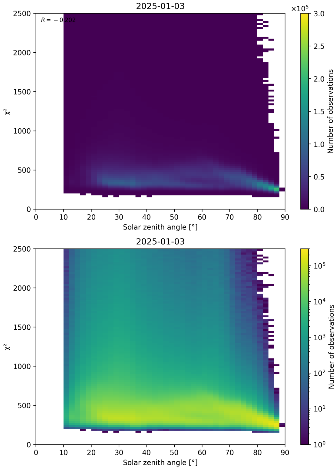
Figure 148: Scatter density plot of “Solar zenith angle” against “ \chi^2 ” for 2025-01-02 to 2025-01-04.
