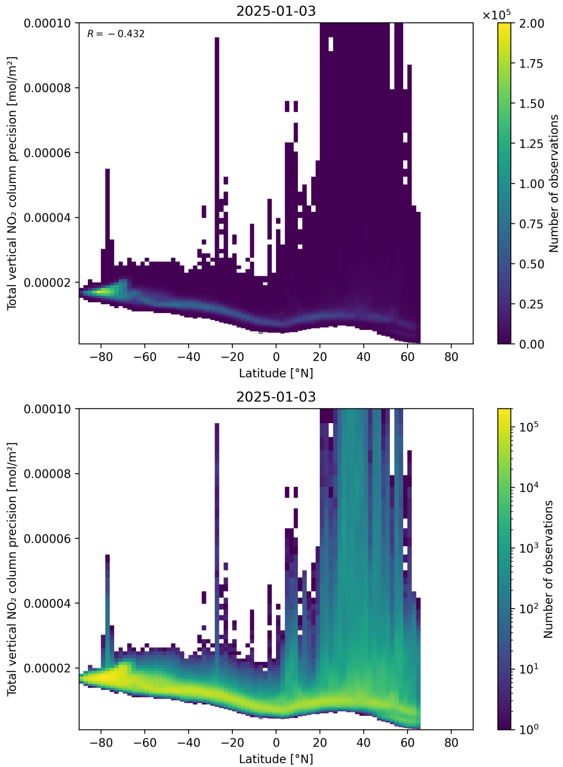
Figure 91: Scatter density plot of “Latitude” against “Total vertical NO 2 column precision” for 2025-01-02 to 2025-01-04.
