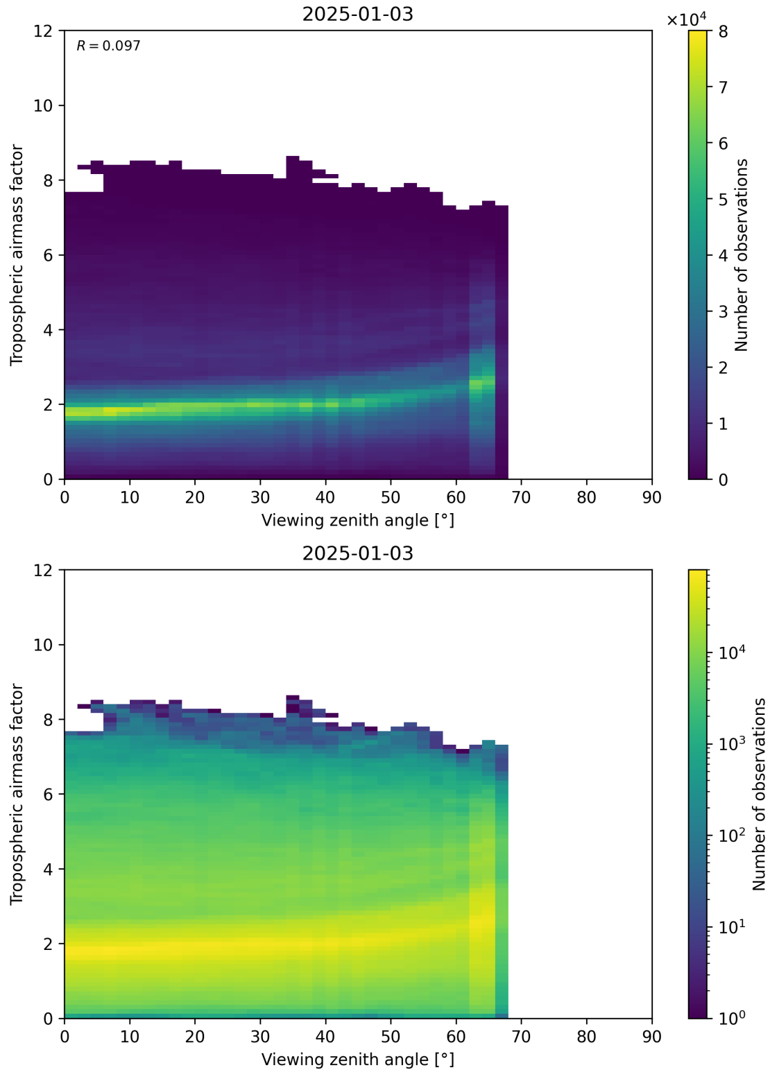
Figure 161: Scatter density plot of “Viewing zenith angle” against “Tropospheric airmass factor” for 2025-01-02 to 2025-01-04.
