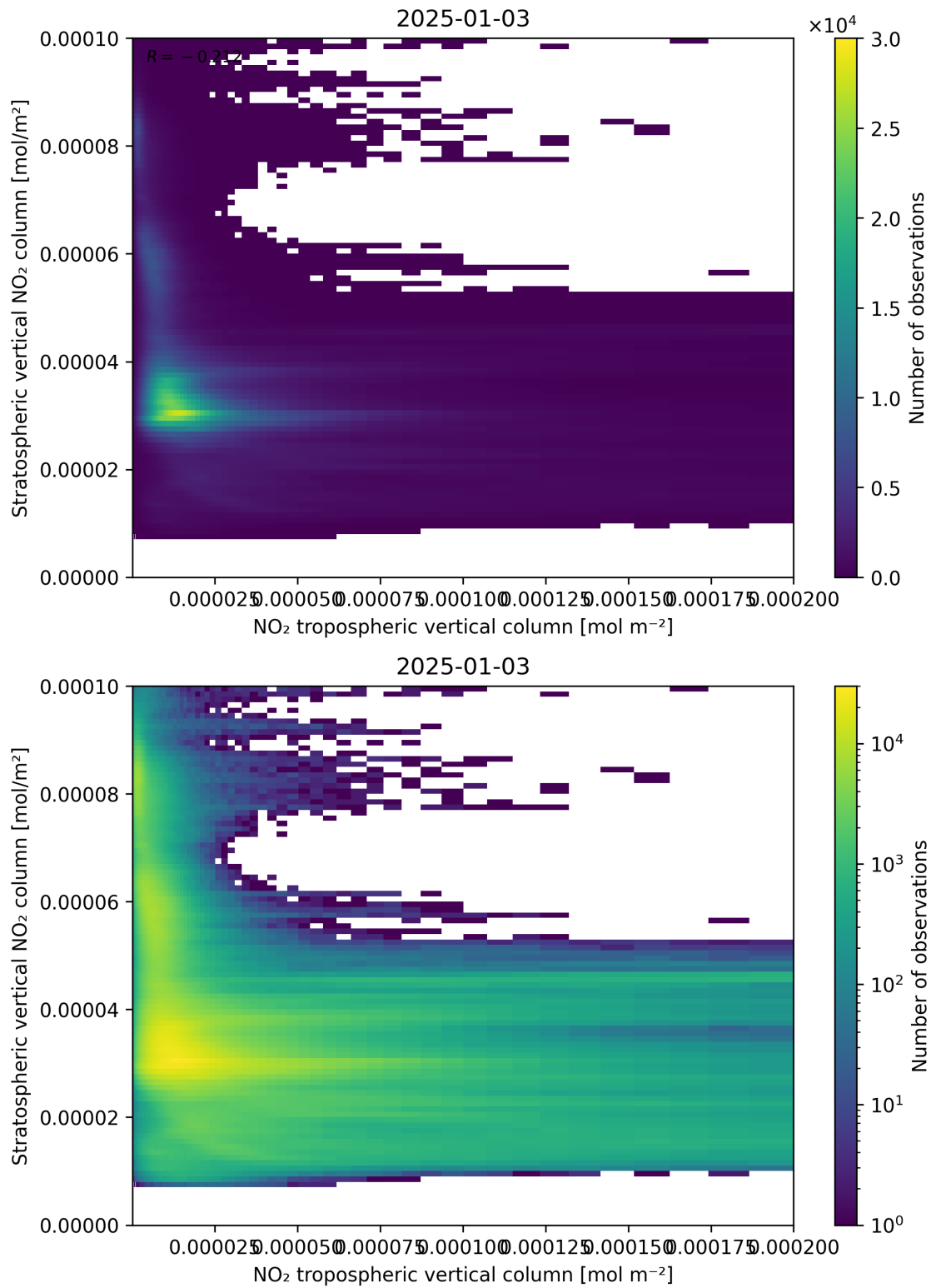
Figure 125: Scatter density plot of “NO 2 tropospheric vertical column” against “Stratospheric vertical NO 2 column” for 2025-01-02 to 2025-01-04.
