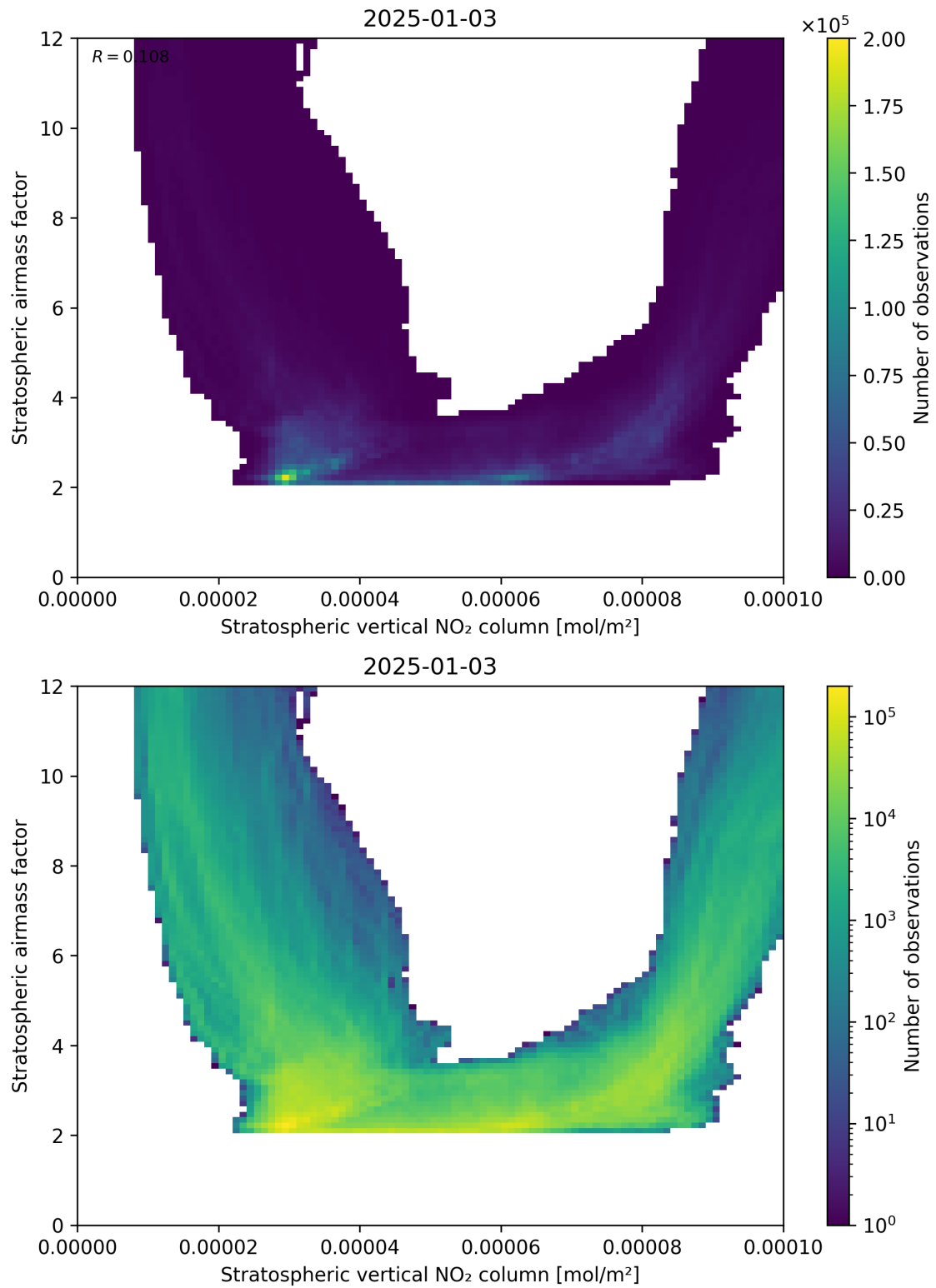
Figure 96: Scatter density plot of “Stratospheric vertical NO 2 column” against “Stratospheric airmass factor” for 2025-01-02 to 2025-01-04.
