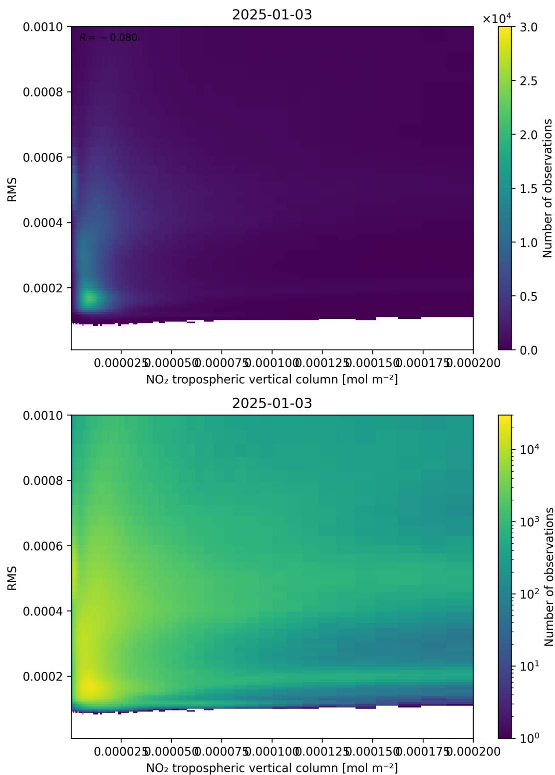
Figure 142: Scatter density plot of “NO 2 tropospheric vertical column” against “RMS” for 2025-01-02 to 2025-01-04.
