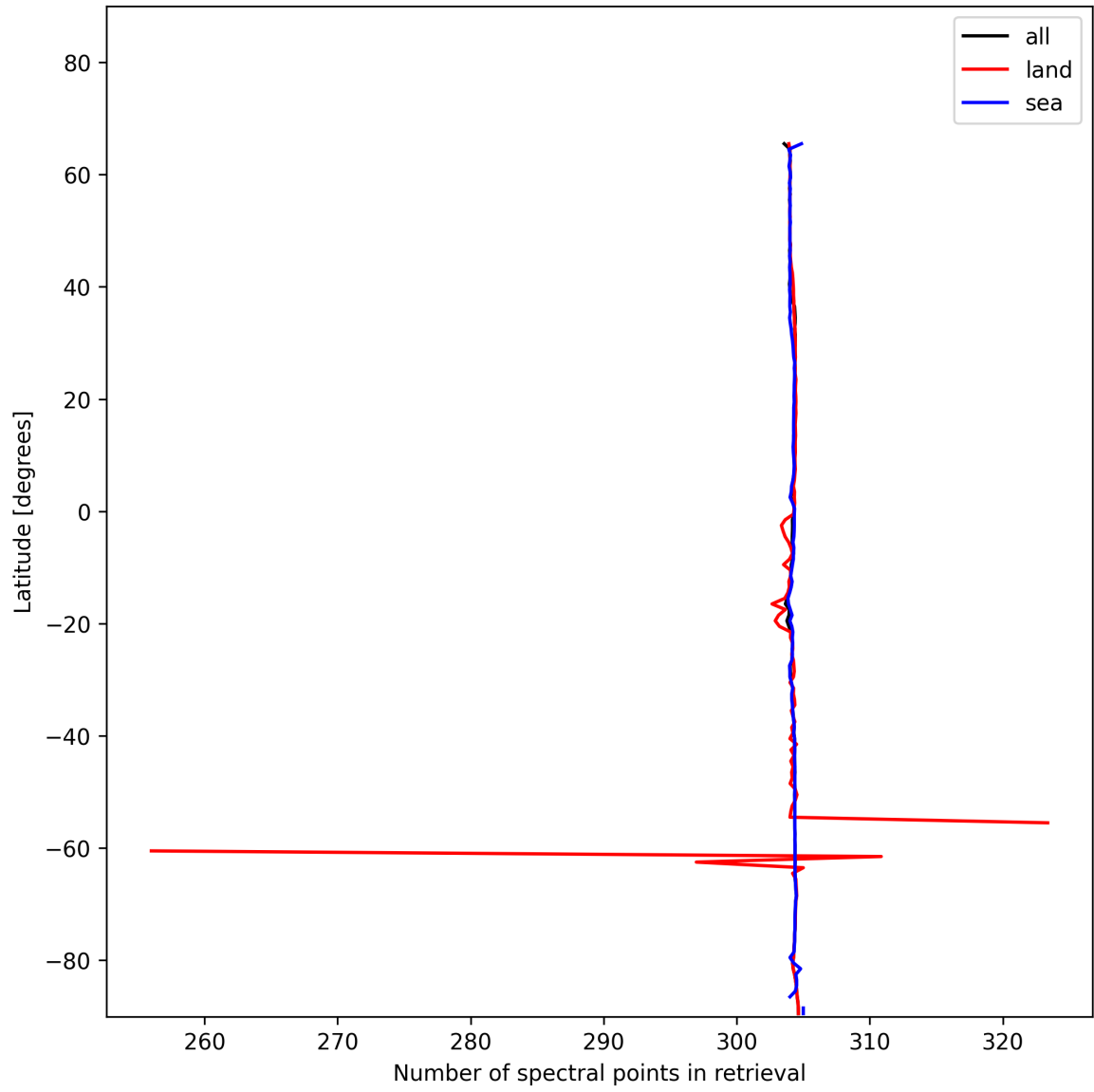
Figure 16: Zonal average of “Number of spectral points in retrieval” for 2025-01-02 to 2025-01-04.
