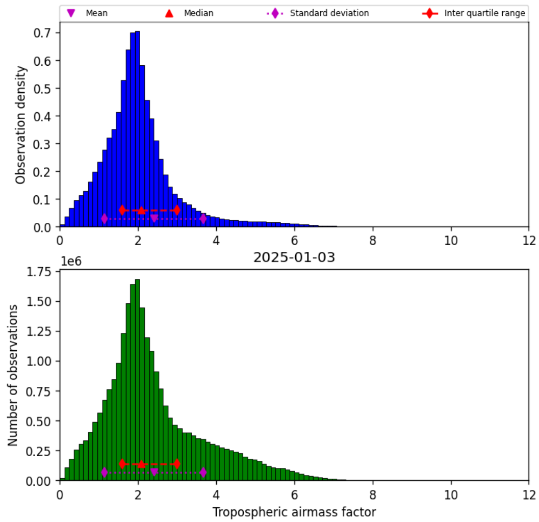
Figure 31: Histogram of “Tropospheric airmass factor” for 2025-01-02 to 2025-01-04
