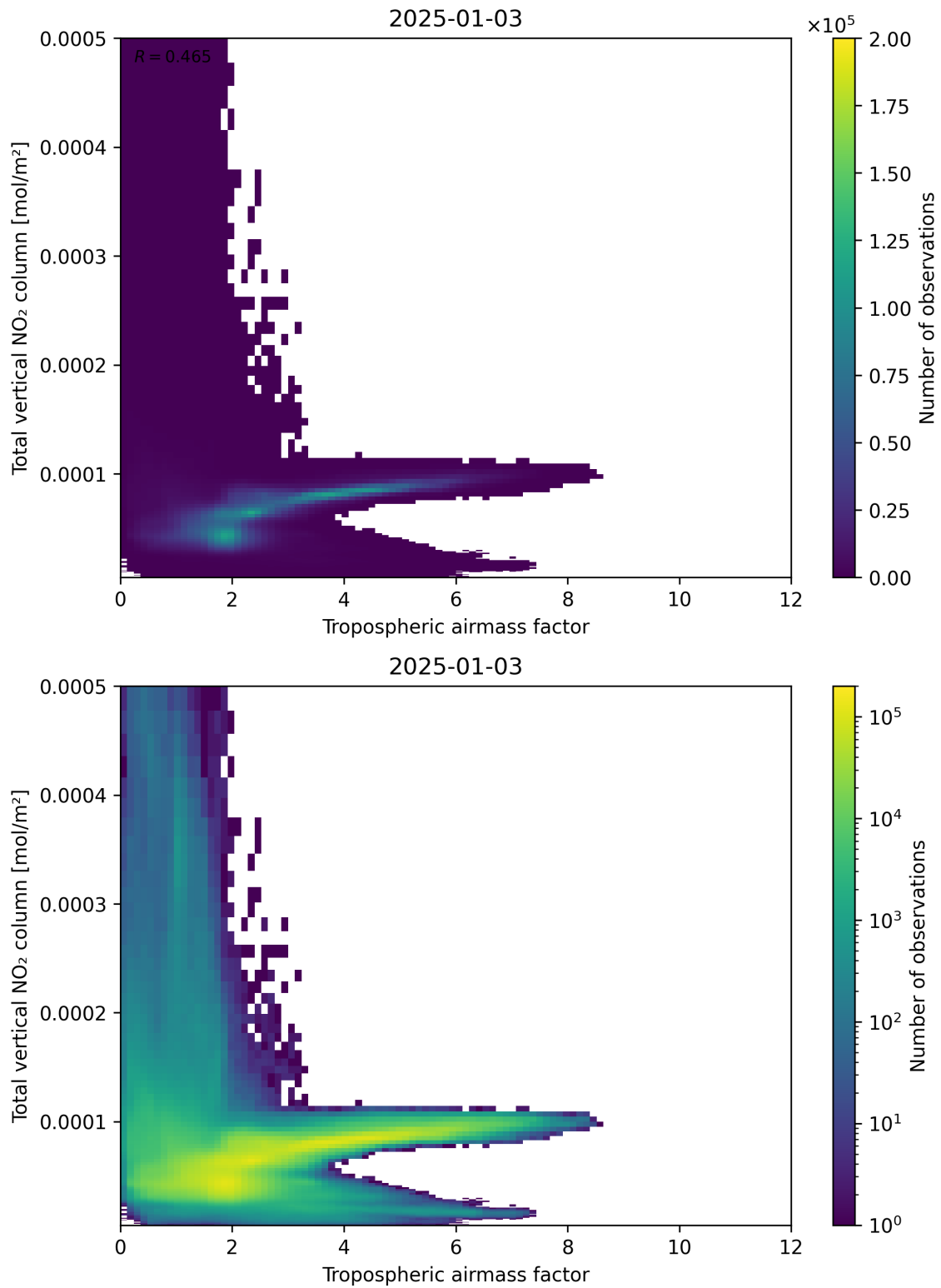
Figure 77: Scatter density plot of “Tropospheric airmass factor” against “Total vertical NO 2 column” for 2025-01-02 to 2025-01-04.
