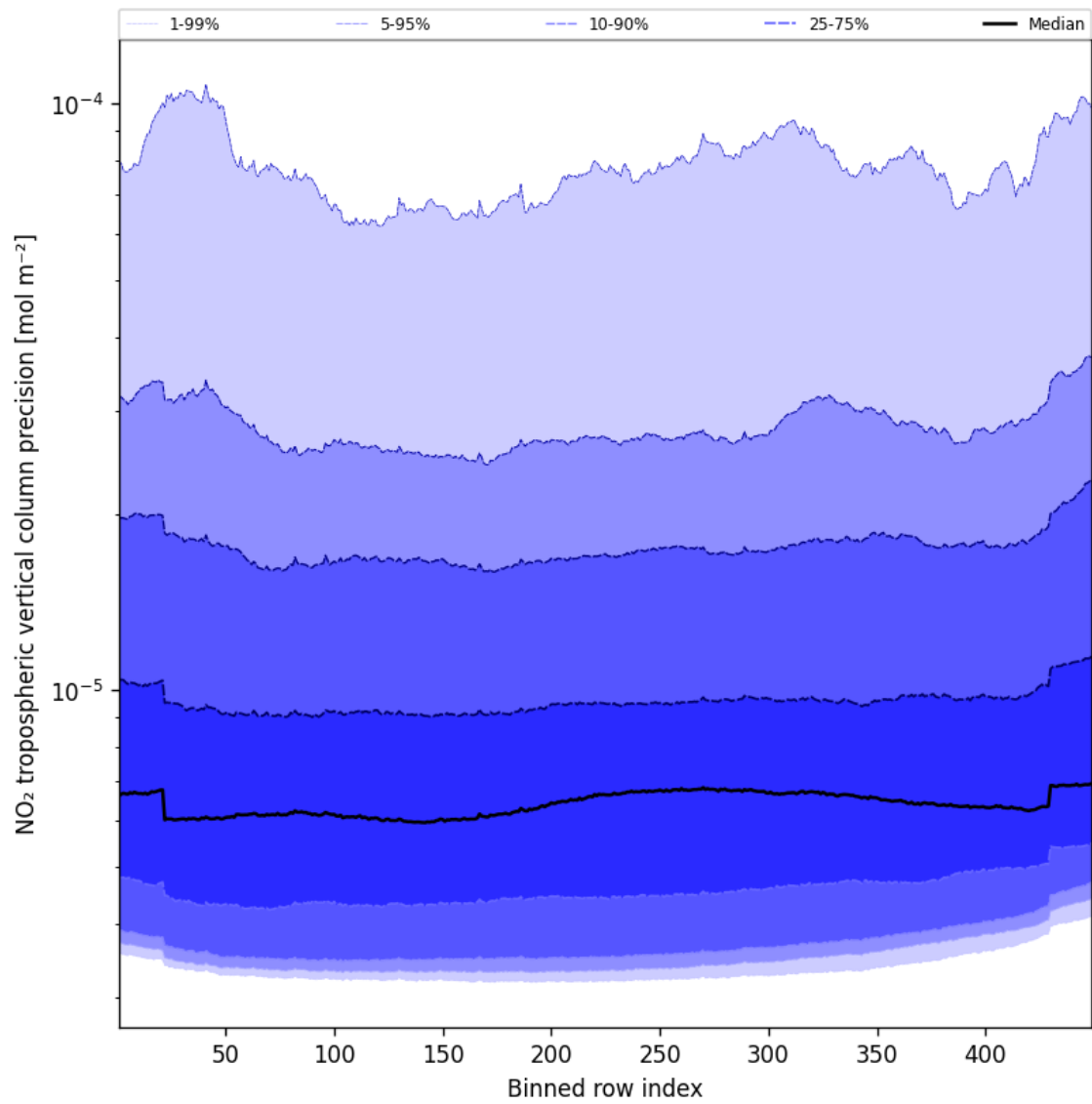
Figure 47: Along track statistics of “NO 2 tropospheric vertical column precision” for 2025-01-02 to 2025-01-04
