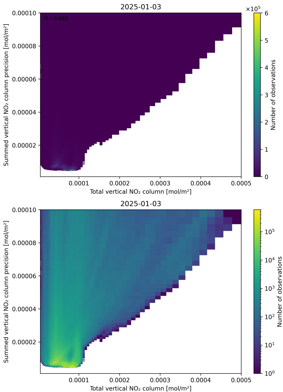
Figure 113: Scatter density plot of “Total vertical NO 2 column” against “Summed vertical NO 2 column precision” for 2025-01-02 to 2025-01-04.
