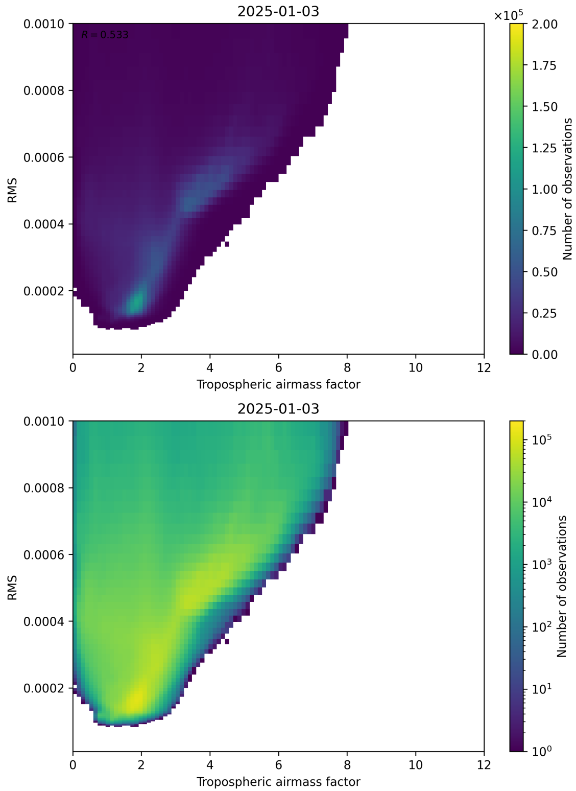
Figure 79: Scatter density plot of “Tropospheric airmass factor” against “RMS” for 2025-01-02 to 2025-01-04.
