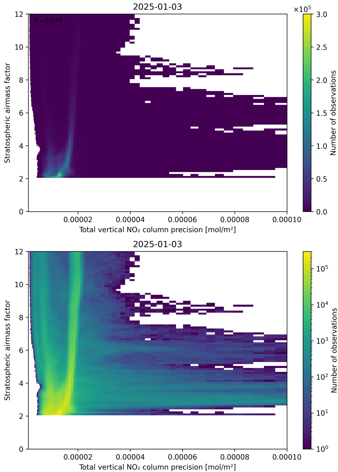
Figure 115: Scatter density plot of “Total vertical NO 2 column precision” against “Stratospheric air mass factor” for 2025-01-02 to 2025-01-04.
