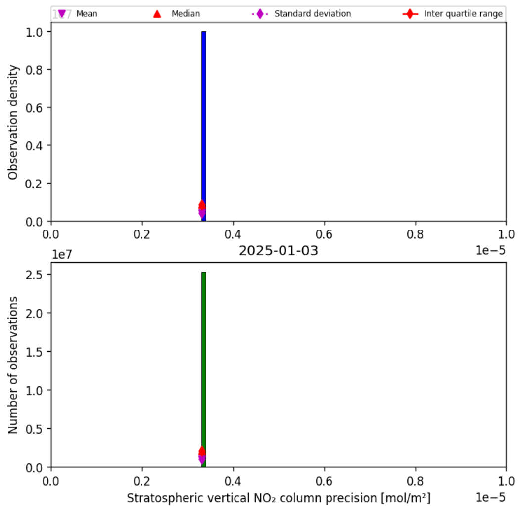
Figure 37: Histogram of “Stratospheric vertical NO 2 column precision” for 2025-01-02 to 2025-01-04
