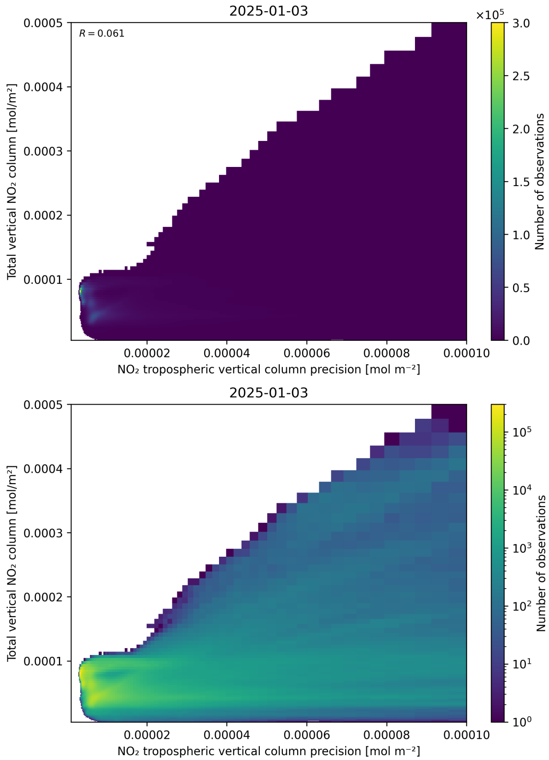
Figure 138: Scatter density plot of “NO 2 tropospheric vertical column precision” against “Total vertical NO 2 column” for 2025-01-02 to 2025-01-04.
