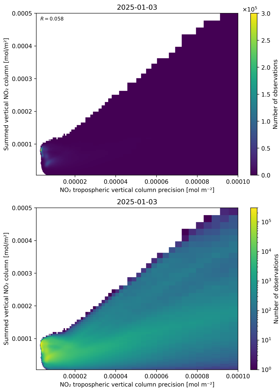
Figure 136: Scatter density plot of “NO 2 tropospheric vertical column precision” against “Summed vertical NO 2 column” for 2025-01-02 to 2025-01-04.
