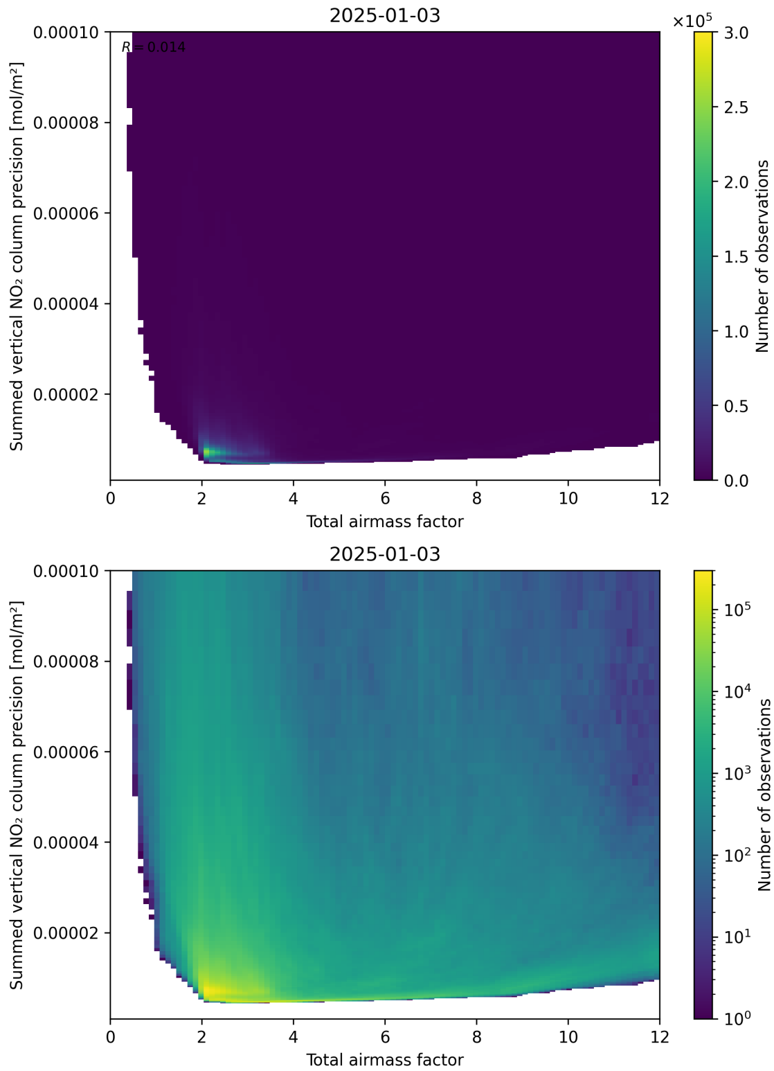
Figure 66: Scatter density plot of “Total airmass factor” against “Summed vertical NO 2 column precision” for 2025-01-02 to 2025-01-04.
