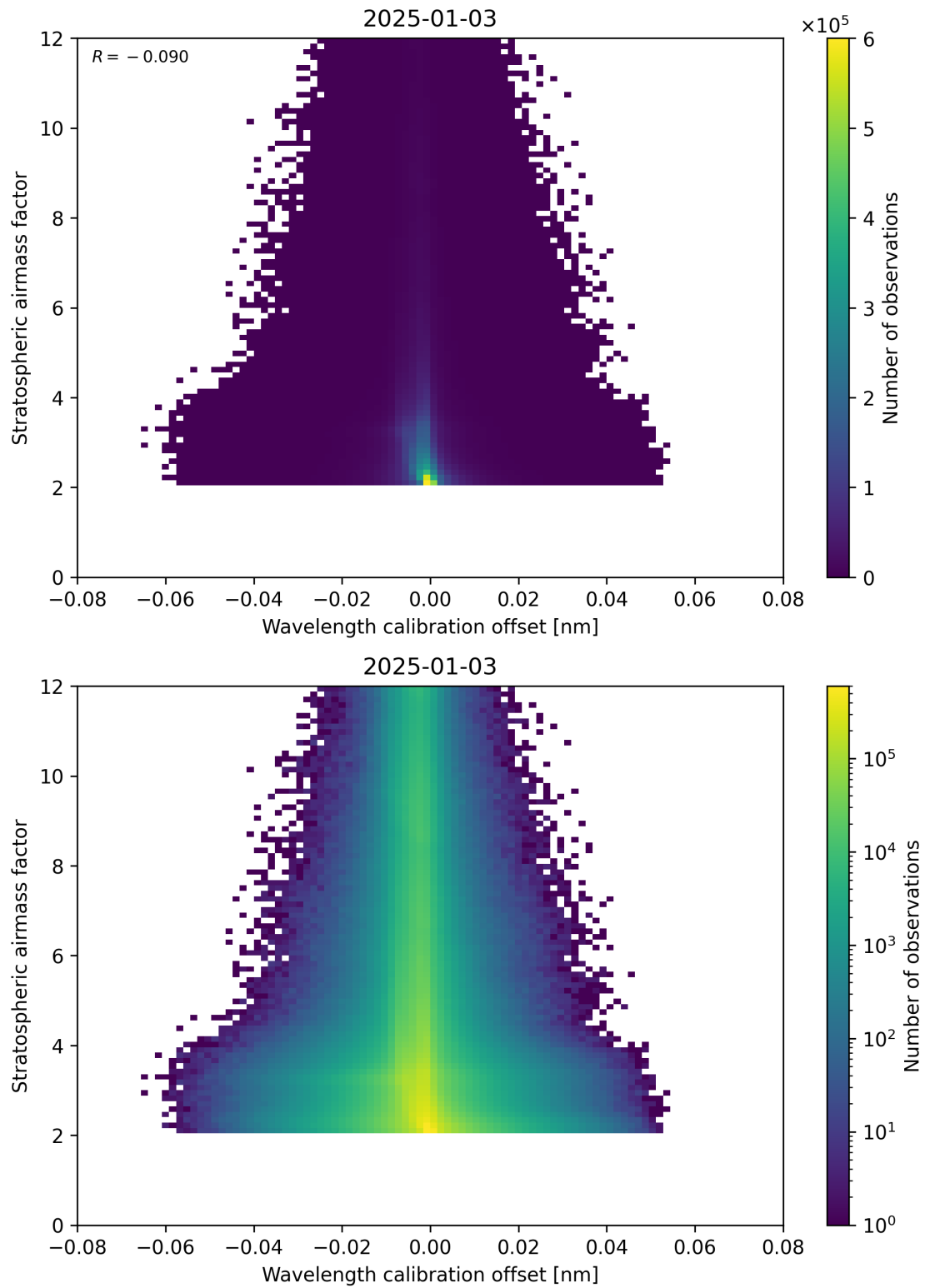
Figure 174: Scatter density plot of “Wavelength calibration offset” against “Stratospheric airmass factor” for 2025-01-02 to 2025-01-04.
