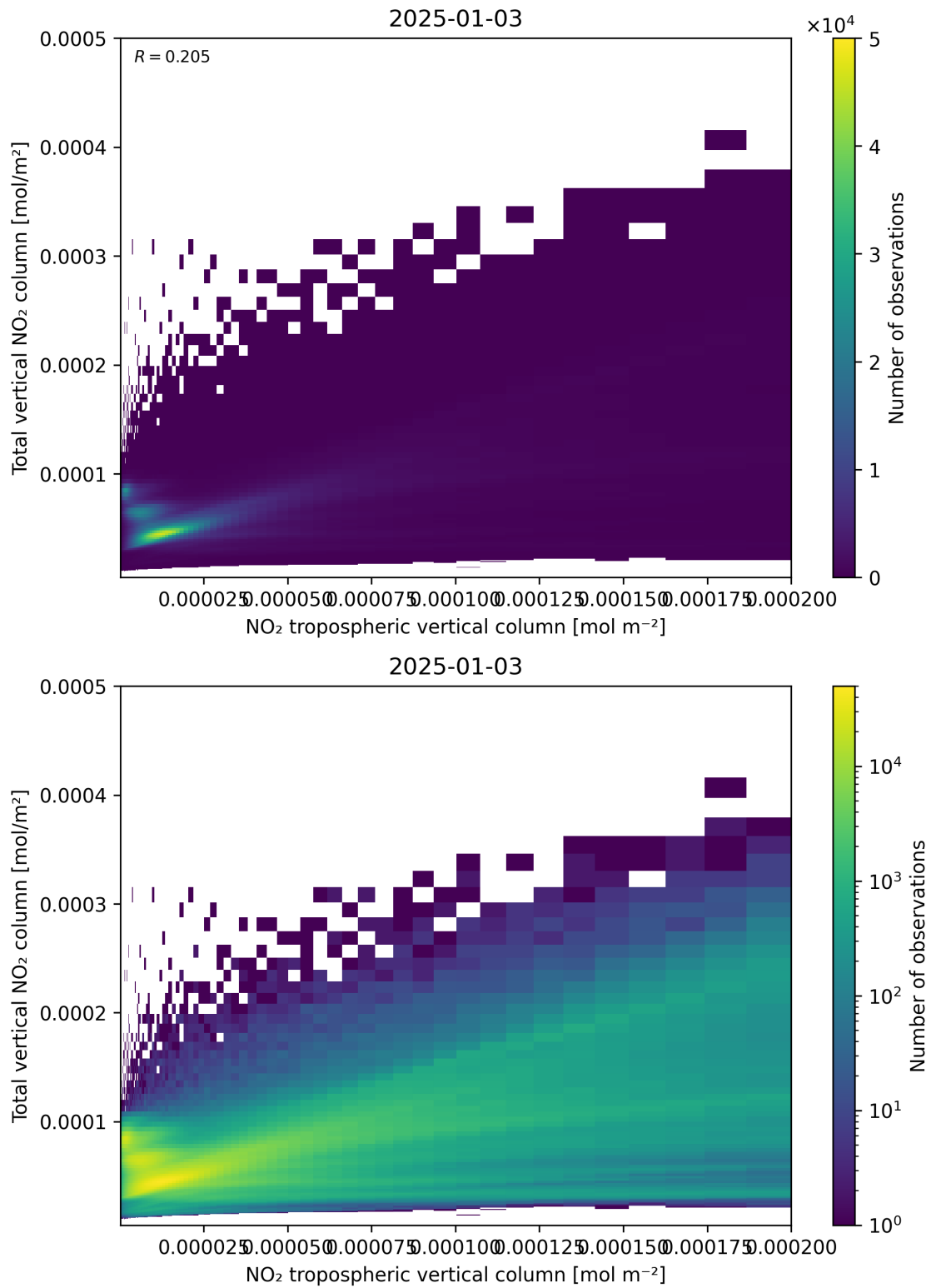
Figure 128: Scatter density plot of “NO 2 tropospheric vertical column” against “Total vertical NO 2 column” for 2025-01-02 to 2025-01-04.
