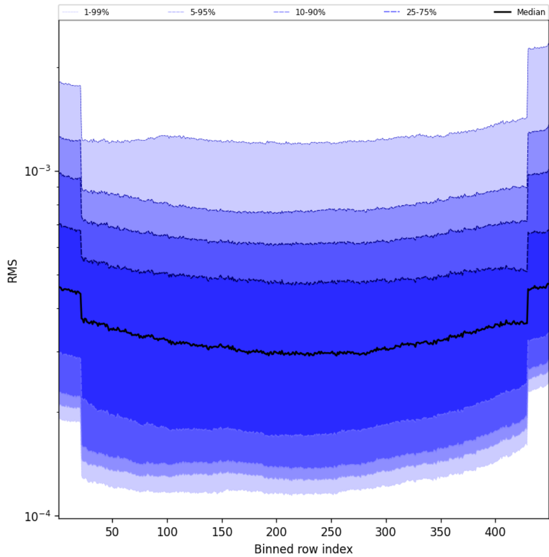
Figure 60: Along track statistics of “RMS” for 2025-01-10 to 2025-01-12
