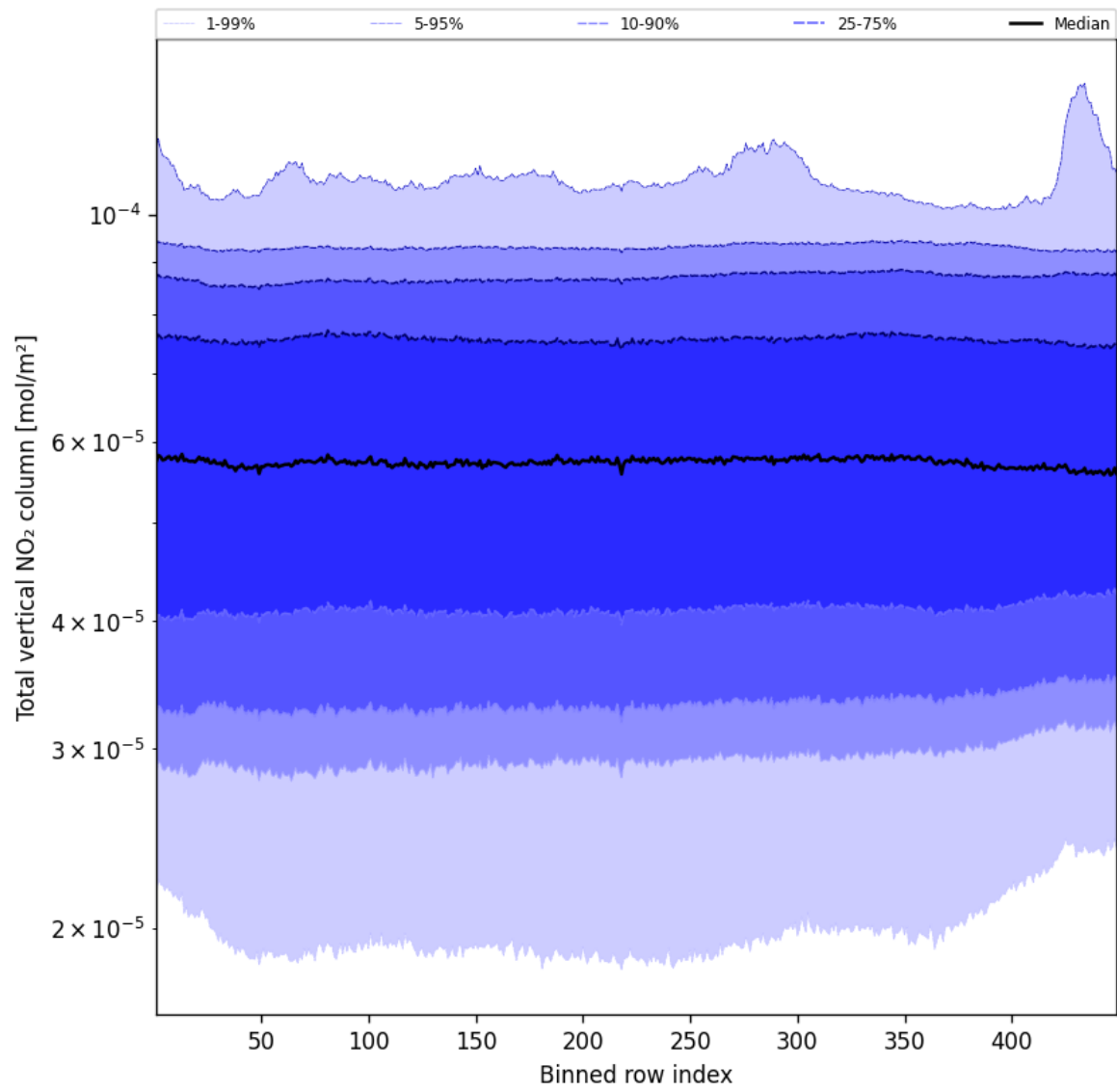
Figure 55: Along track statistics of “Total vertical NO 2 column” for 2025-01-10 to 2025-01-12
