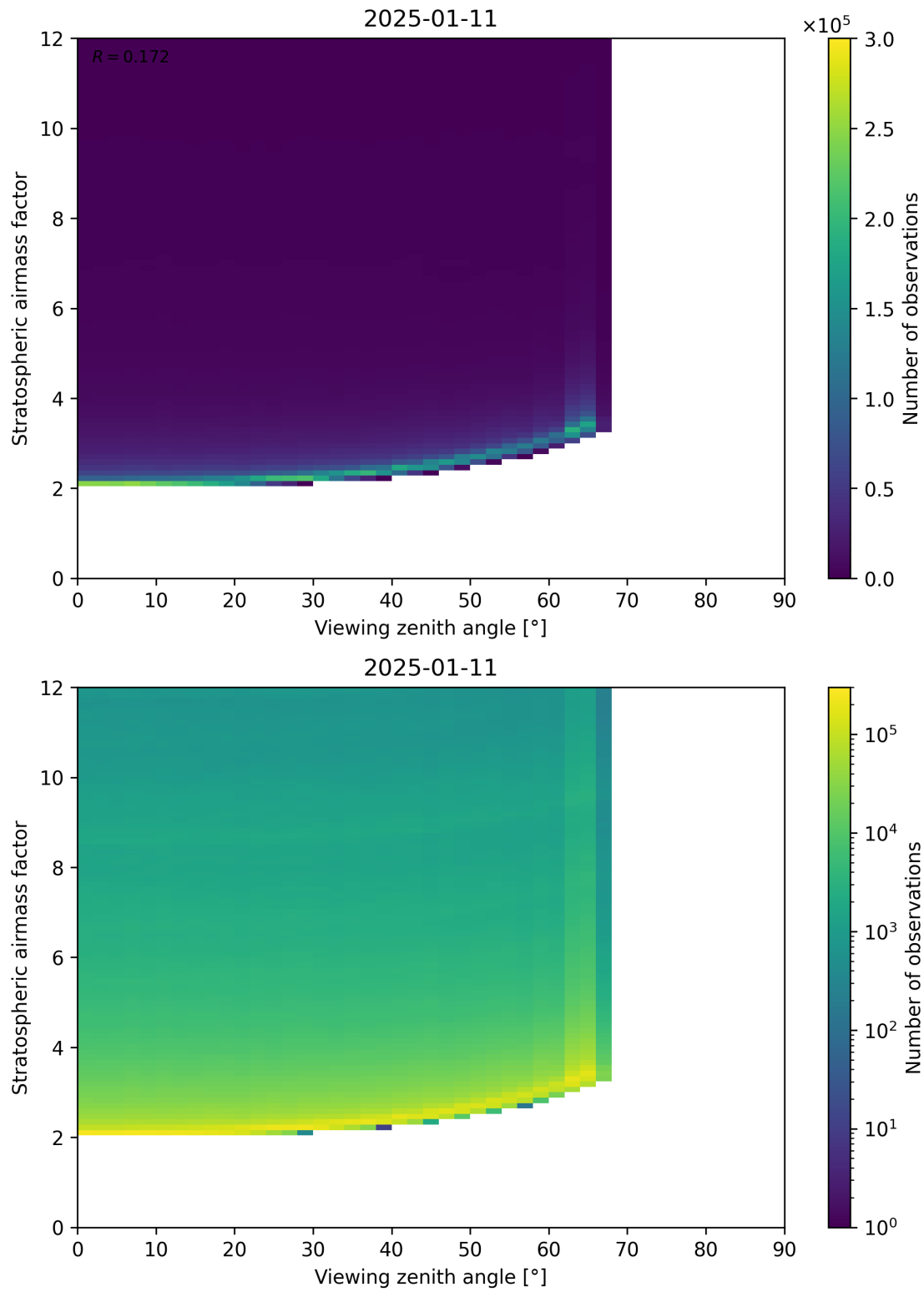
Figure 159: Scatter density plot of “Viewing zenith angle” against “Stratospheric airmass factor” for 2025-01-10 to 2025-01-12.
