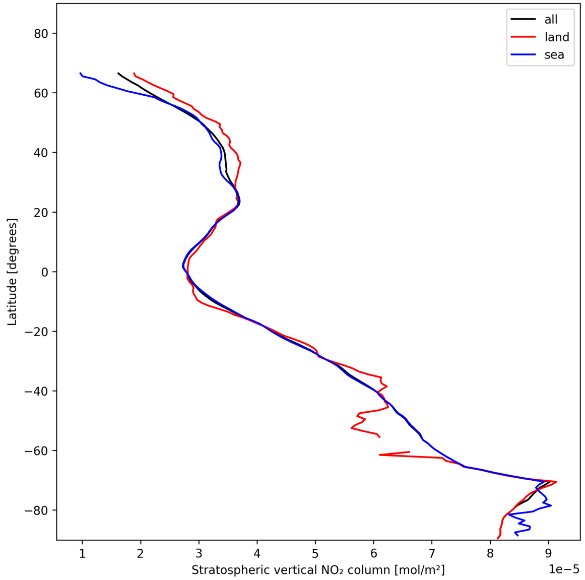
Figure 19: Zonal average of “Stratospheric vertical NO 2 column” for 2025-01-10 to 2025-01-12.
