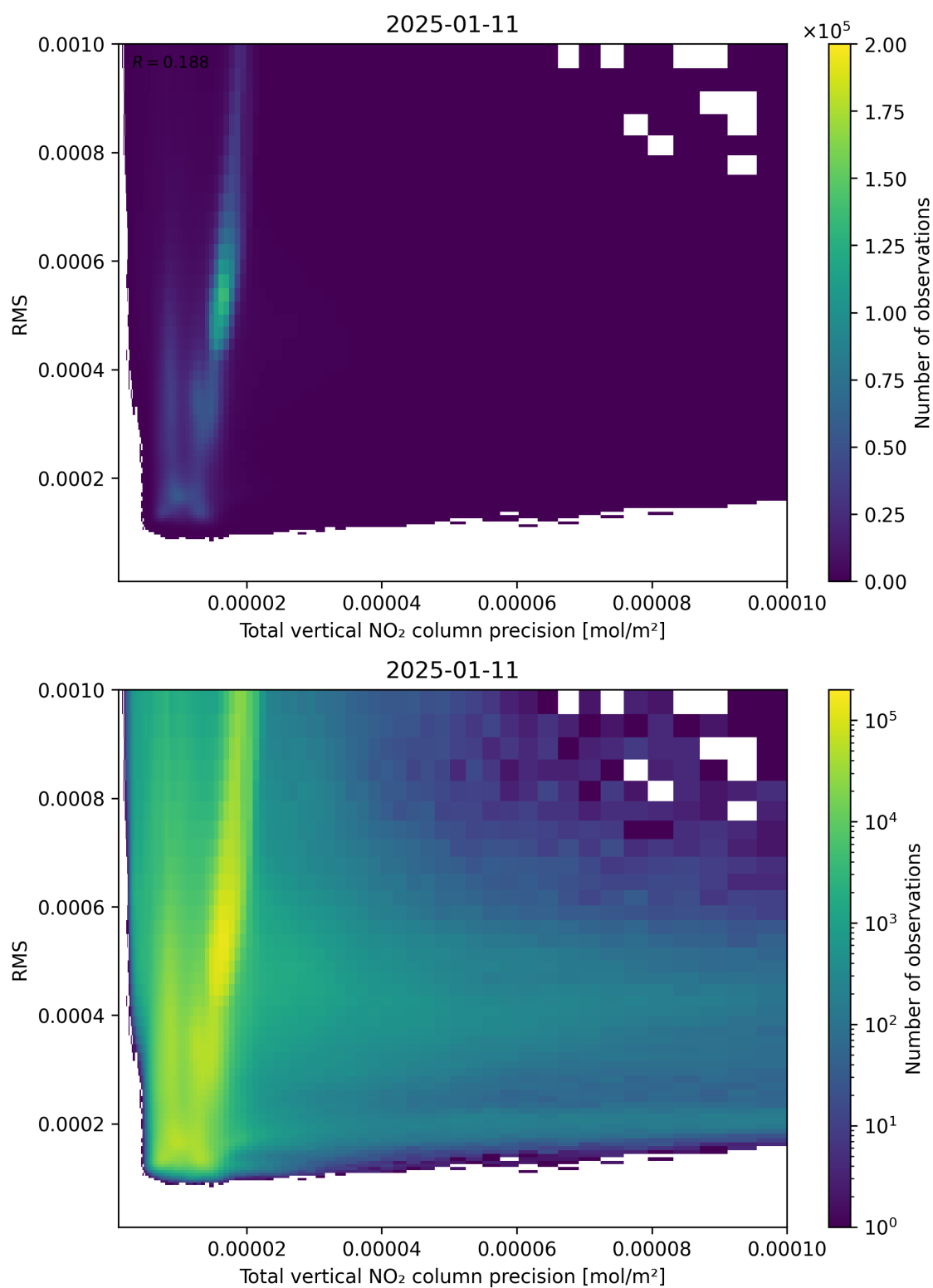
Figure 119: Scatter density plot of “Total vertical NO 2 column precision” against “RMS” for 2025-01-10 to 2025-01-12.
