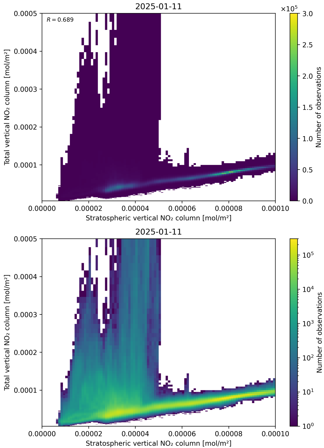
Figure 100: Scatter density plot of “Stratospheric vertical NO 2 column” against “Total vertical NO 2 column” for 2025-01-10 to 2025-01-12.
