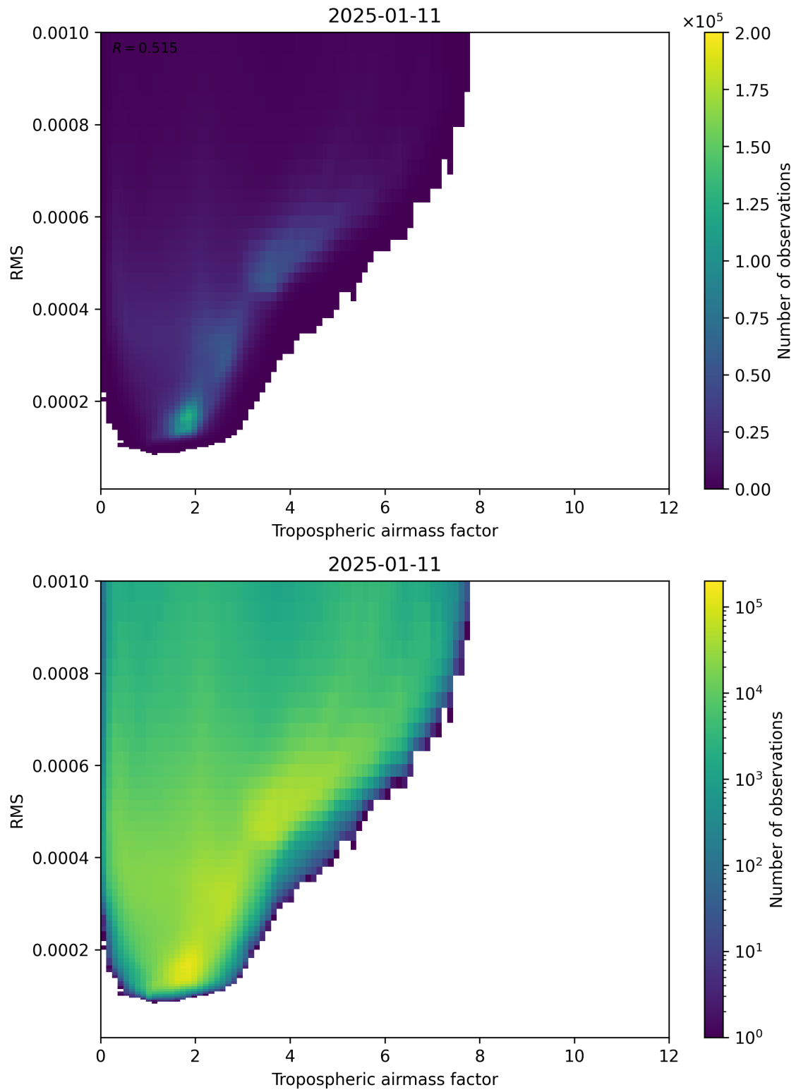
Figure 79: Scatter density plot of “Tropospheric airmass factor” against “RMS” for 2025-01-10 to 2025-01-12.
