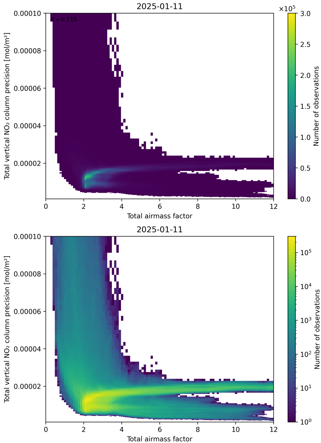
Figure 68: Scatter density plot of “Total airmass factor” against “Total vertical NO 2 column precision” for 2025-01-10 to 2025-01-12.
