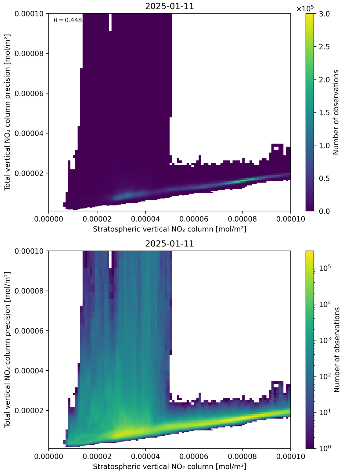
Figure 101: Scatter density plot of “Stratospheric vertical NO 2 column” against “Total vertical NO 2 column precision” for 2025-01-10 to 2025-01-12.
