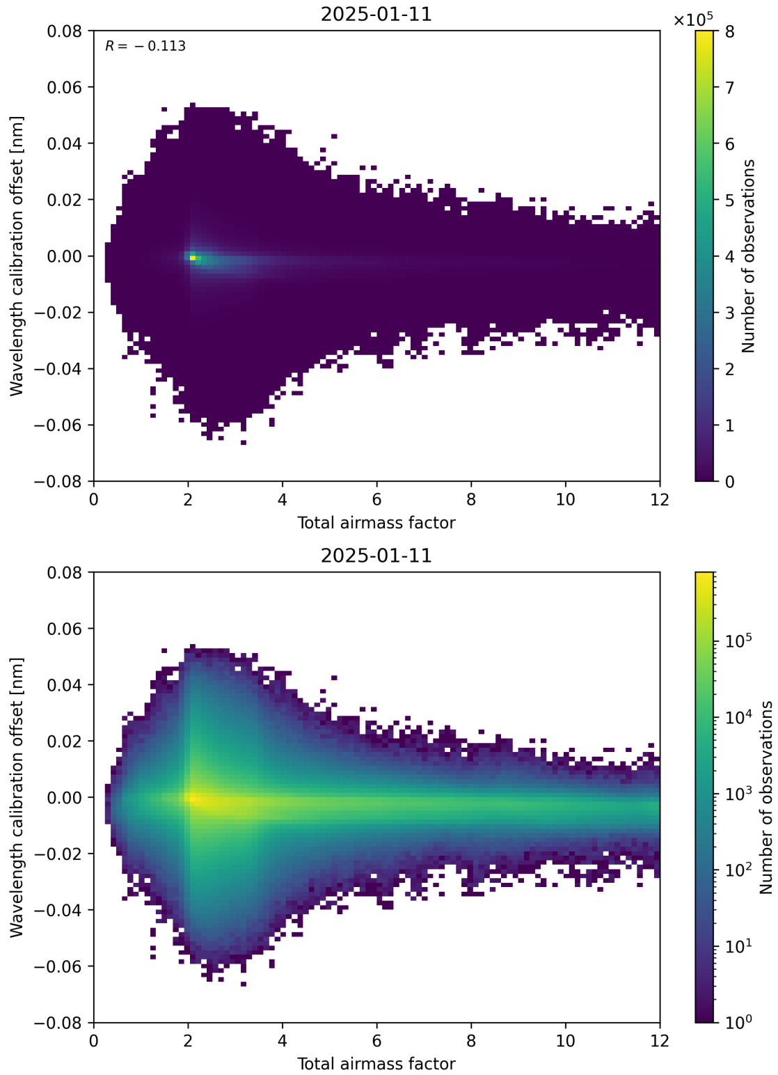
Figure 70: Scatter density plot of “Total airmass factor” against “Wavelength calibration offset” for 2025-01-10 to 2025-01-12.
