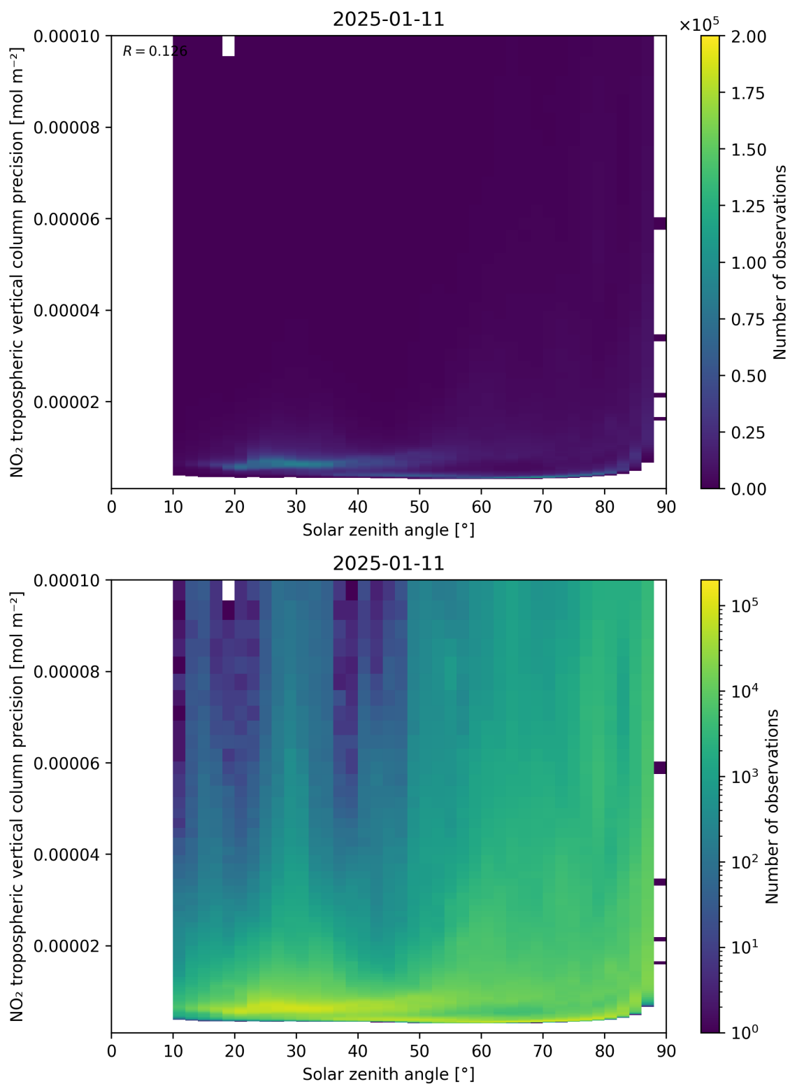
Figure 156: Scatter density plot of “Solar zenith angle” against “NO 2 tropospheric vertical column precision” for 2025-01-10 to 2025-01-12.
