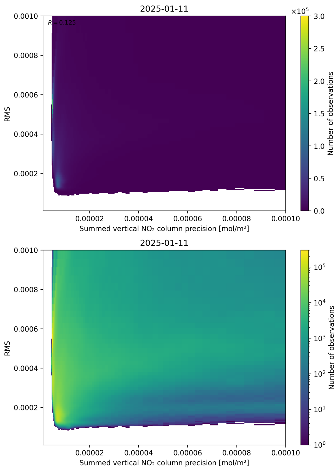
Figure 108: Scatter density plot of “Summed vertical NO 2 column precision” against “RMS” for 2025-01-10 to 2025-01-12.
