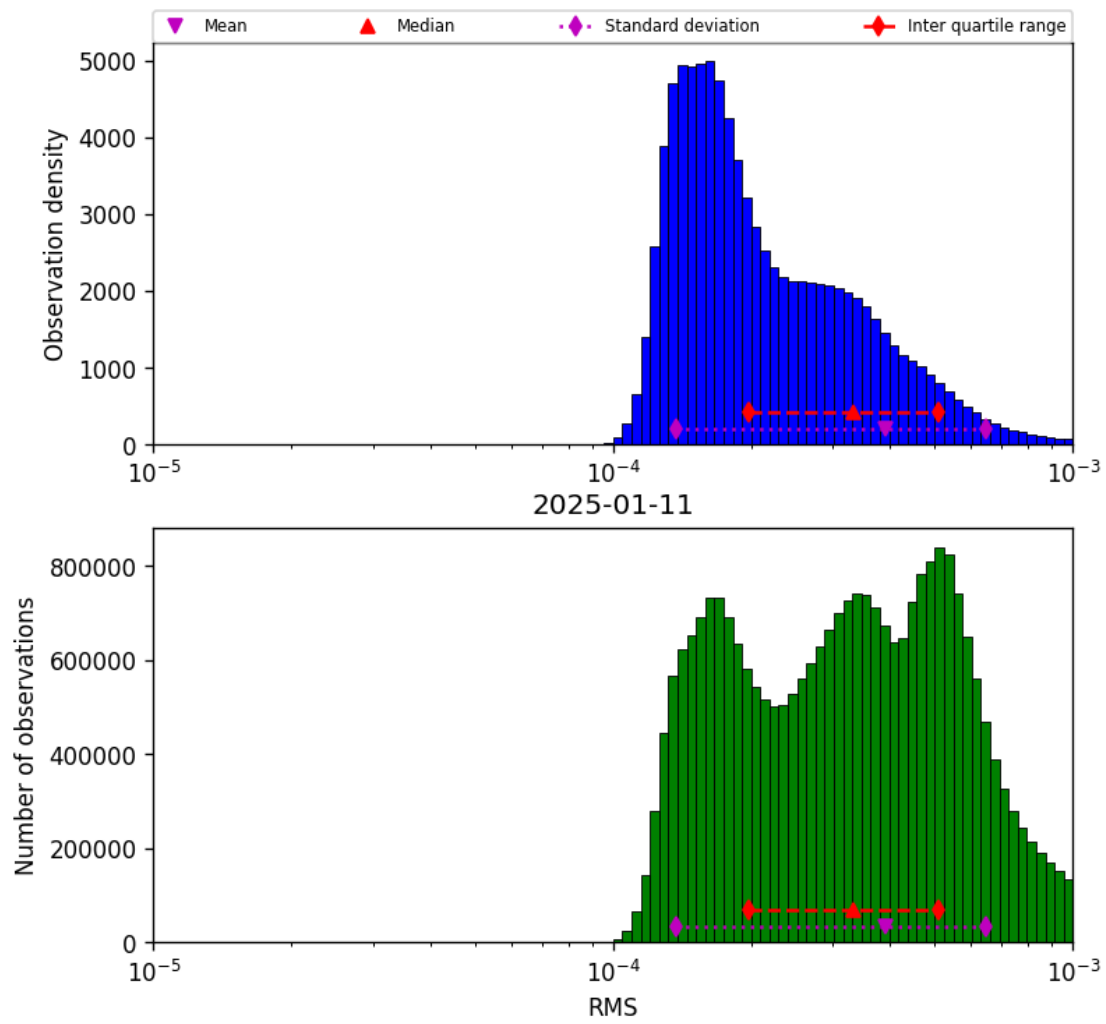
Figure 43: Histogram of “RMS” for 2025-01-10 to 2025-01-12
