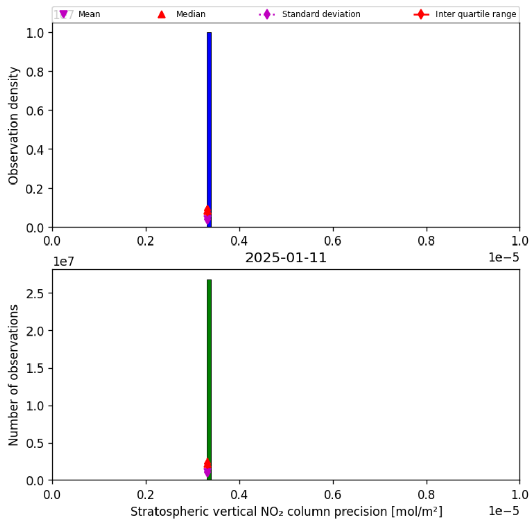
Figure 37: Histogram of “Stratospheric vertical NO 2 column precision” for 2025-01-10 to 2025-01-12
