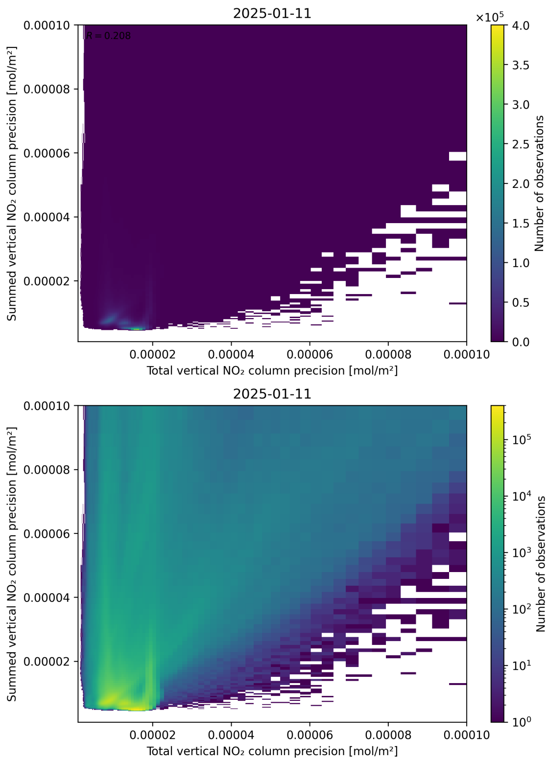
Figure 118: Scatter density plot of “Total vertical NO 2 column precision” against “Summed vertical NO 2 column precision” for 2025-01-10 to 2025-01-12.
