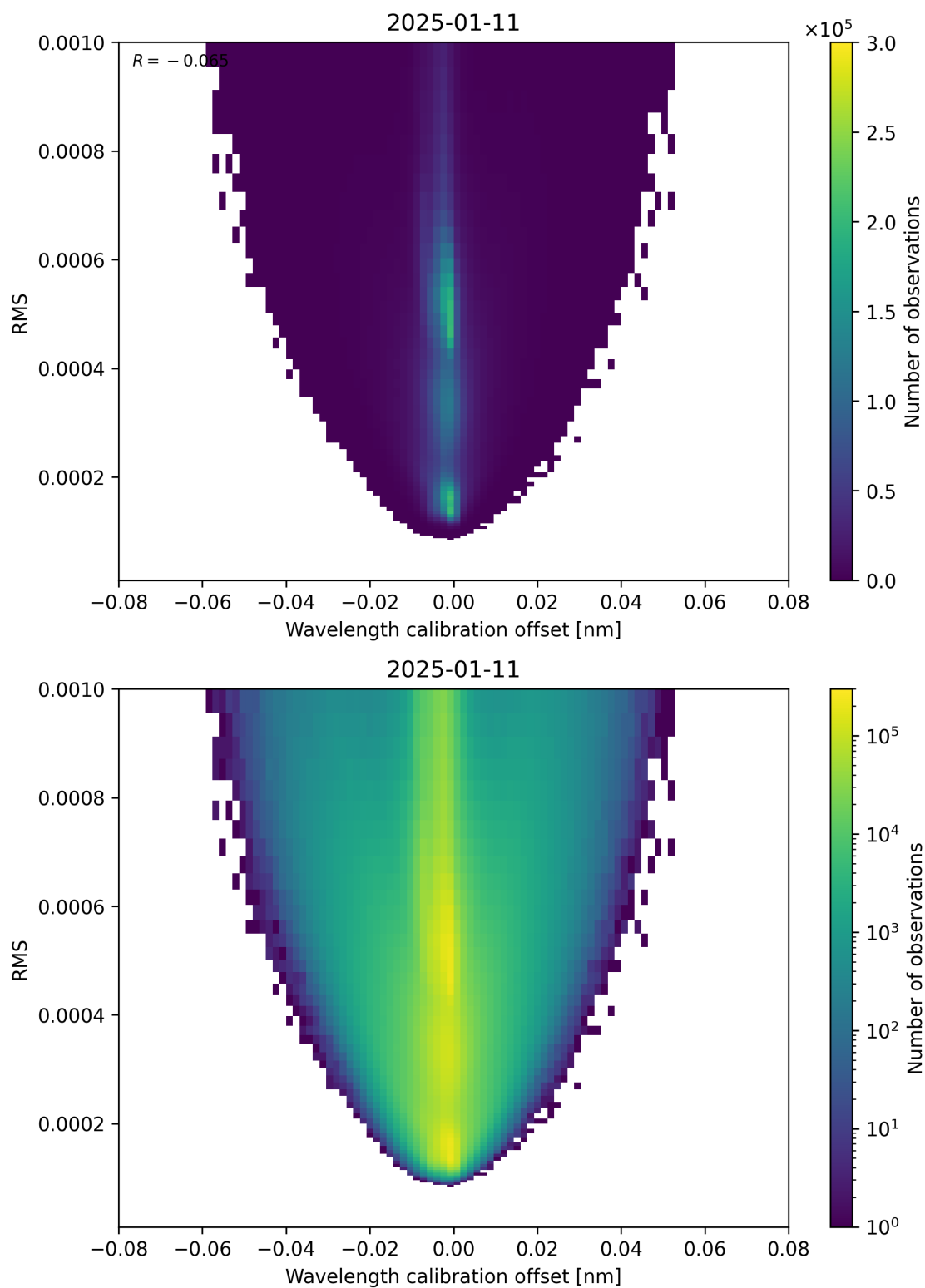
Figure 181: Scatter density plot of “Wavelength calibration offset” against “RMS” for 2025-01-10 to 2025-01-12.
