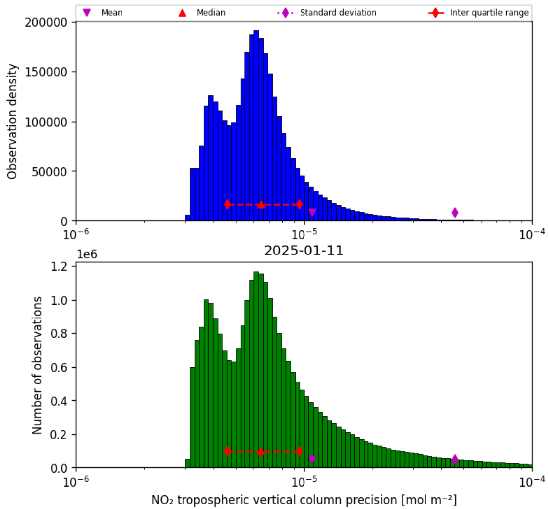
Figure 30: Histogram of “NO 2 tropospheric vertical column precision” for 2025-01-10 to 2025-01-12
