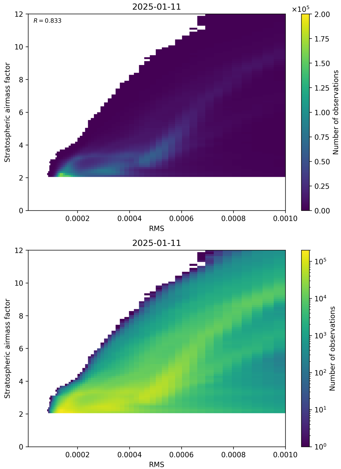
Figure 144: Scatter density plot of “RMS” against “Stratospheric airmass factor” for 2025-01-10 to 2025-01-12.
