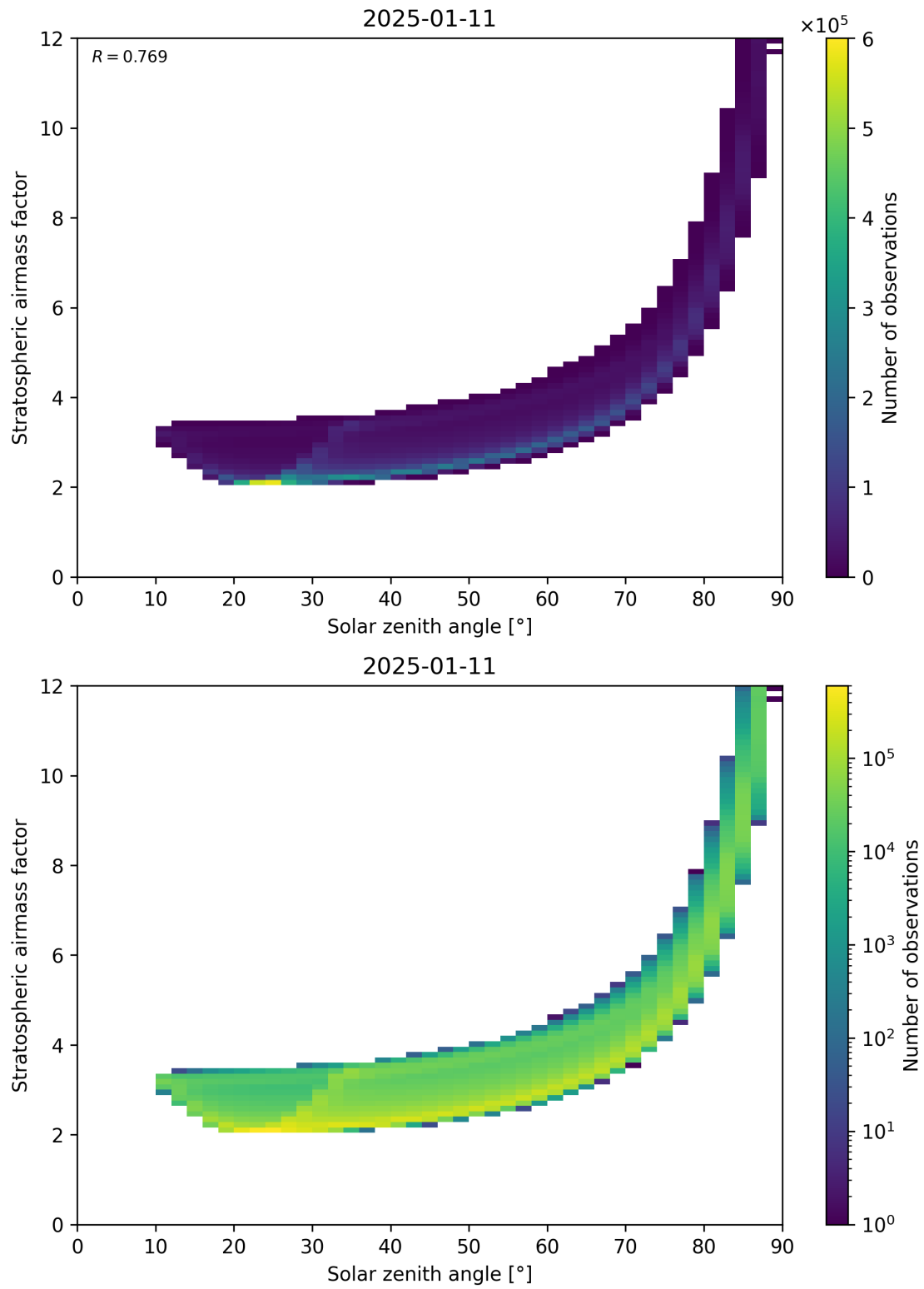
Figure 145: Scatter density plot of “Solar zenith angle” against “Stratospheric airmass factor” for 2025-01-10 to 2025-01-12.
