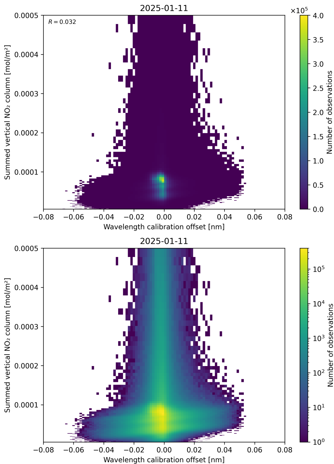
Figure 177: Scatter density plot of “Wavelength calibration offset” against “Summed vertical NO 2 column” for 2025-01-10 to 2025-01-12.
