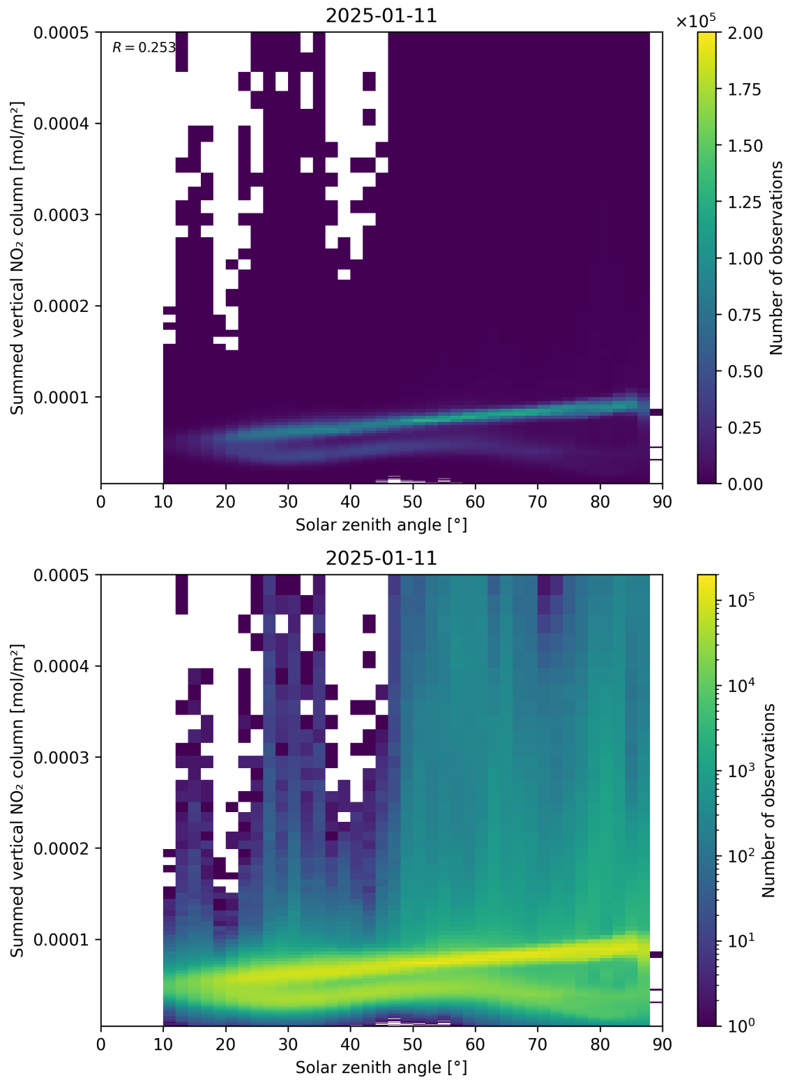
Figure 151: Scatter density plot of “Solar zenith angle” against “Summed vertical NO 2 column” for 2025-01-10 to 2025-01-12.
