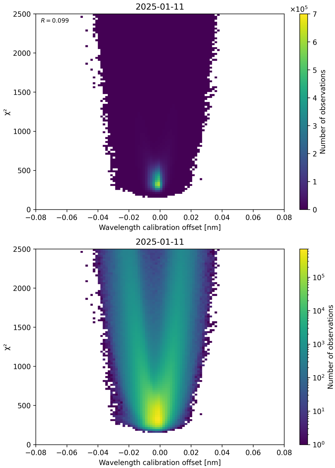
Figure 175: Scatter density plot of “Wavelength calibration offset” against “ \chi^2 ” for 2025-01-10 to 2025-01-12.
