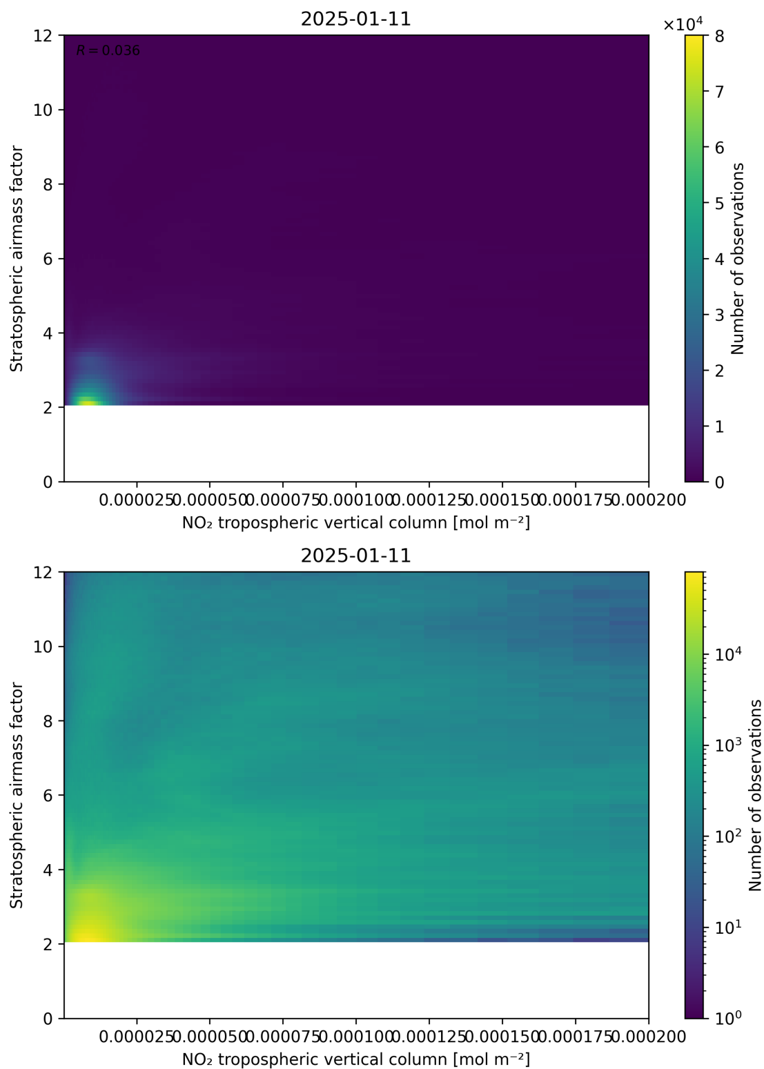
Figure 121: Scatter density plot of “NO 2 tropospheric vertical column” against “Stratospheric airmass factor” for 2025-01-10 to 2025-01-12.
