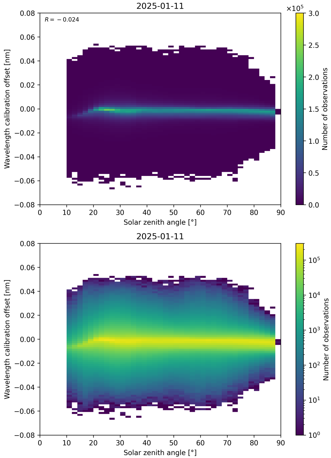
Figure 158: Scatter density plot of “Solar zenith angle” against “Wavelength calibration offset” for 2025-01-10 to 2025-01-12.
