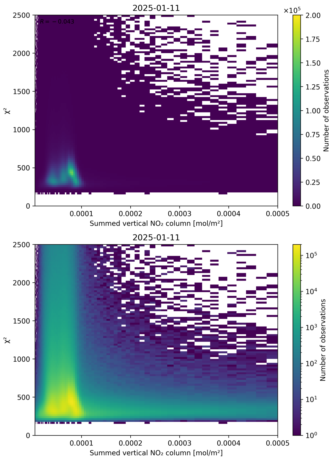
Figure 104: Scatter density plot of “Summed vertical NO 2 column” against “ \chi^2 ” for 2025-01-10 to 2025-01-12.
