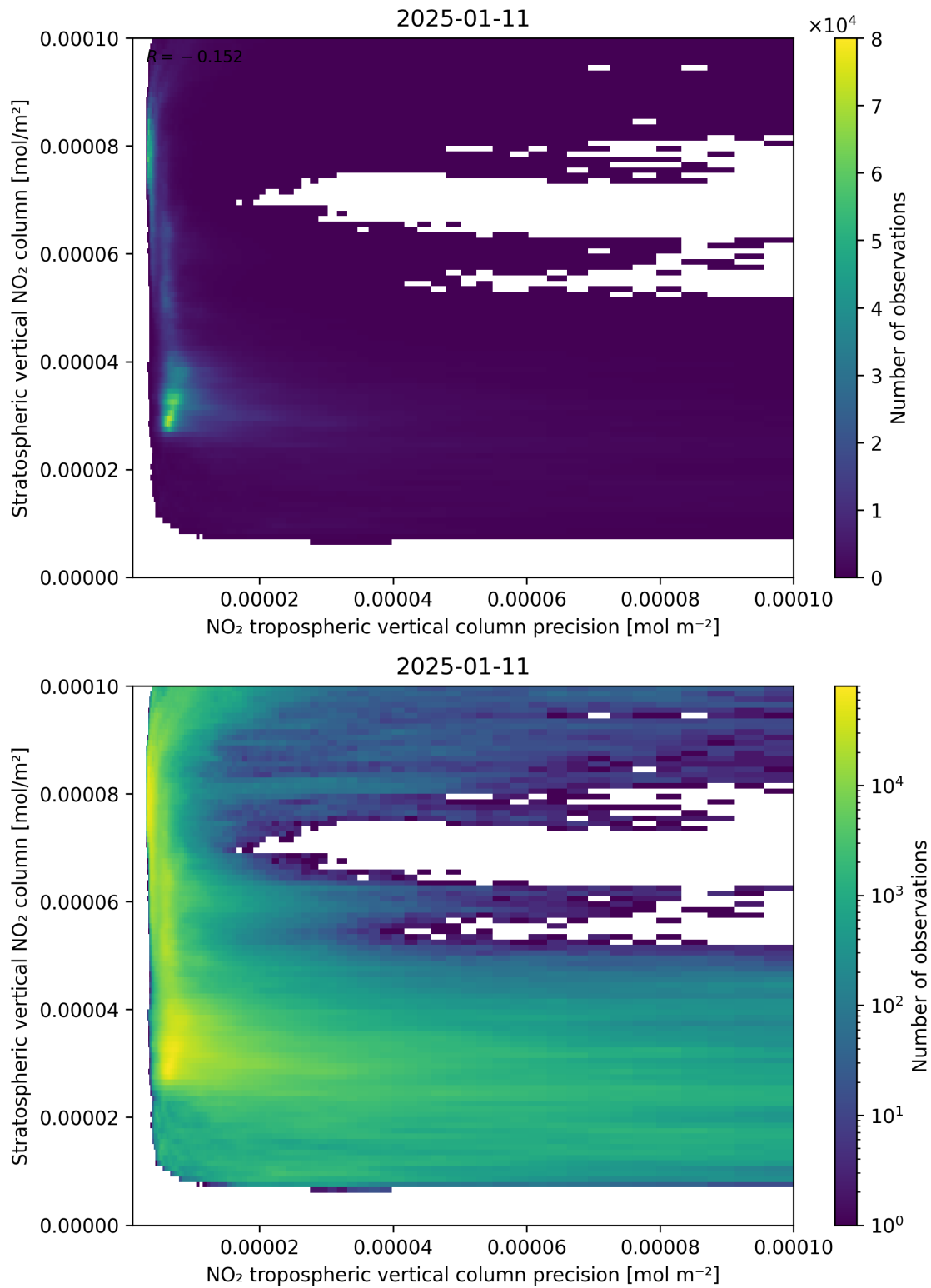
Figure 135: Scatter density plot of “NO 2 tropospheric vertical column precision” against “Stratospheric vertical NO 2 column” for 2025-01-10 to 2025-01-12.
