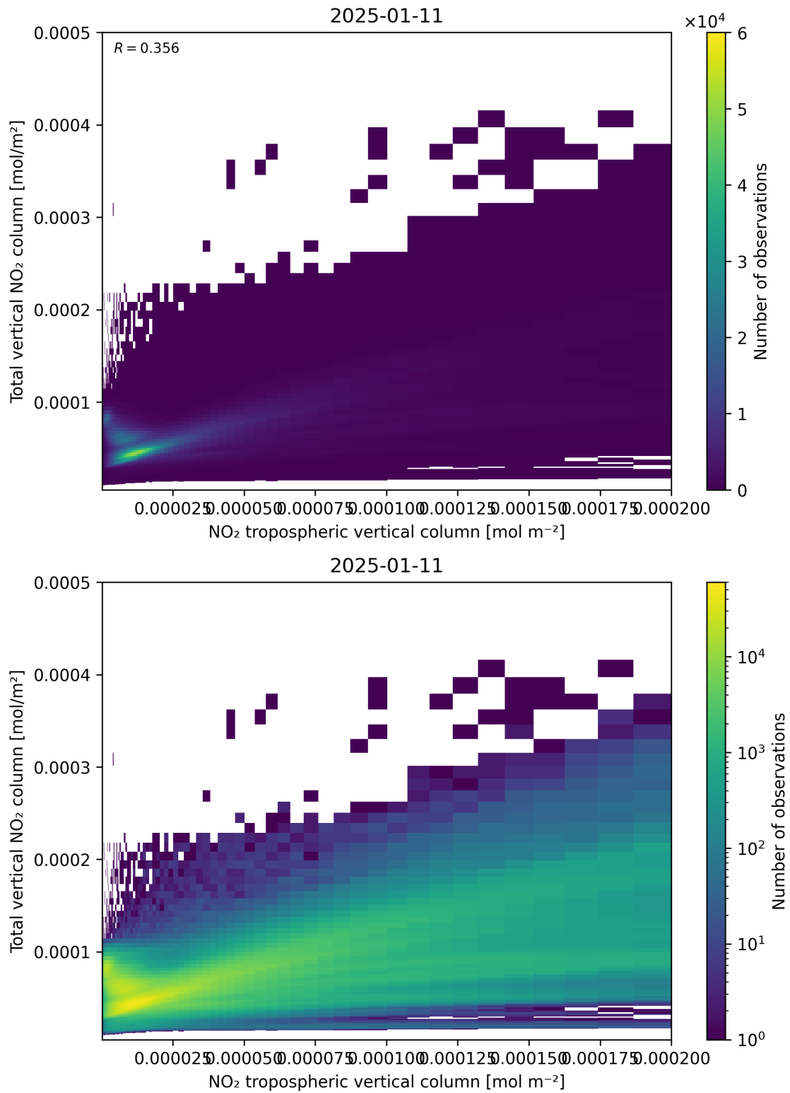
Figure 128: Scatter density plot of “NO 2 tropospheric vertical column” against “Total vertical NO 2 column” for 2025-01-10 to 2025-01-12.
