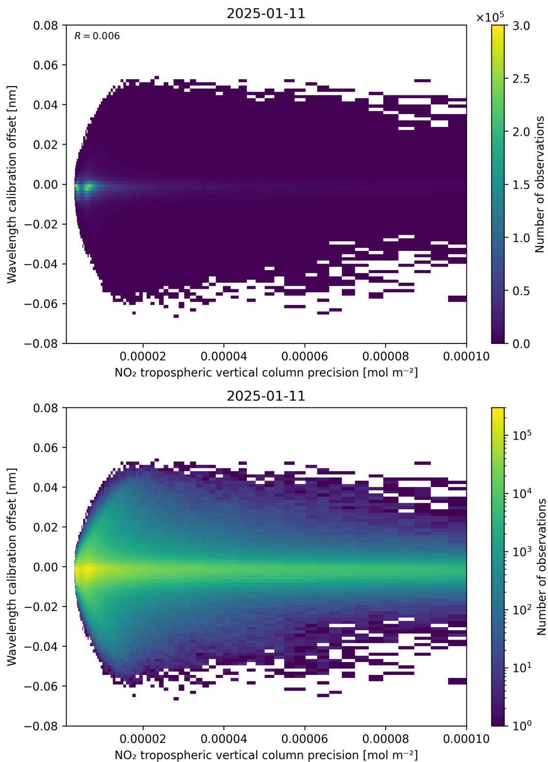
Figure 141: Scatter density plot of “NO 2 tropospheric vertical column precision” against “Wavelength calibration offset” for 2025-01-10 to 2025-01-12.
