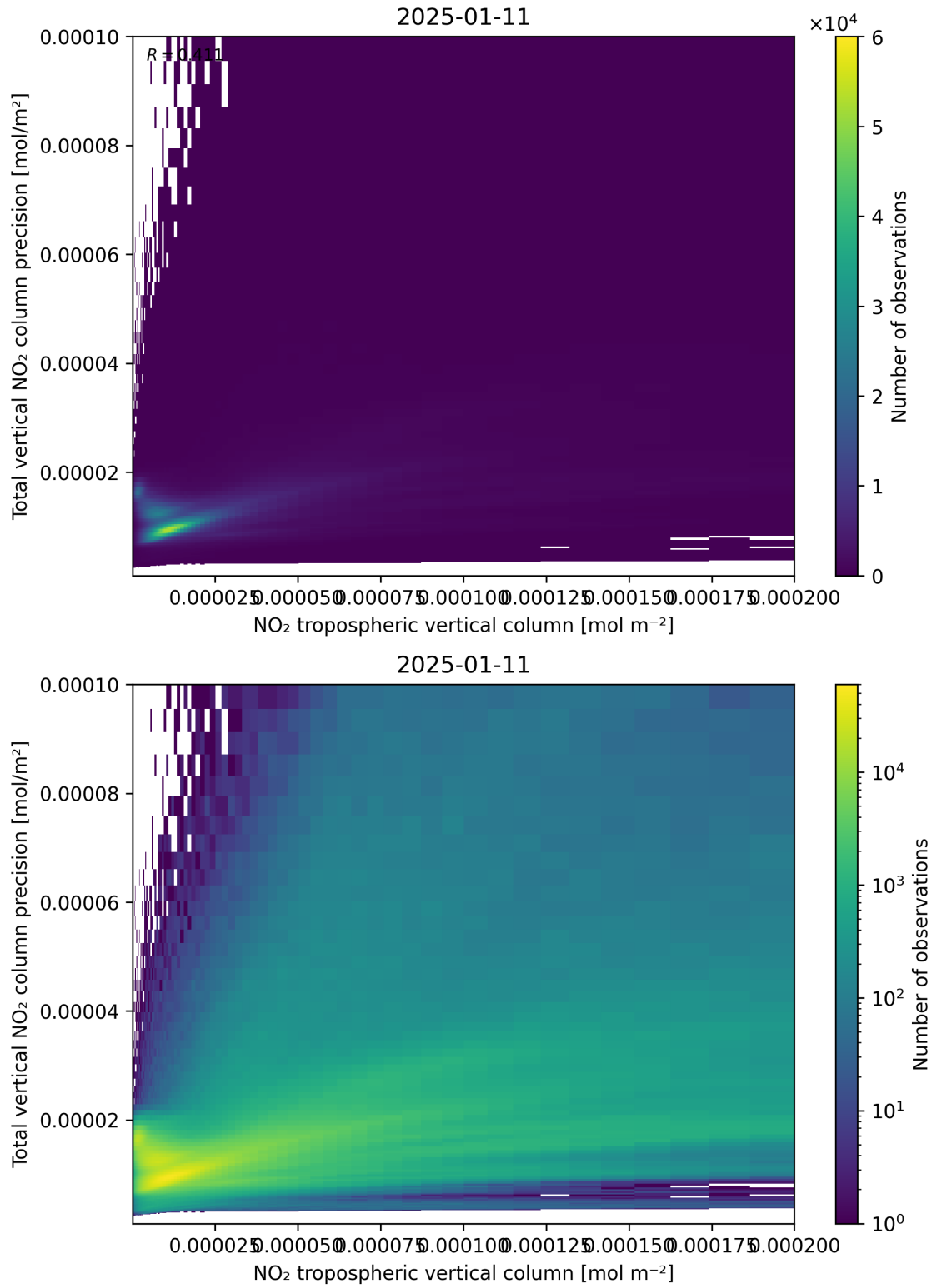
Figure 129: Scatter density plot of “NO 2 tropospheric vertical column” against “Total vertical NO 2 column precision” for 2025-01-10 to 2025-01-12.
