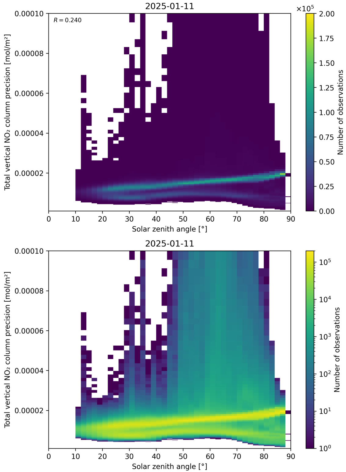
Figure 154: Scatter density plot of “Solar zenith angle” against “Total vertical NO 2 column precision” for 2025-01-10 to 2025-01-12.
