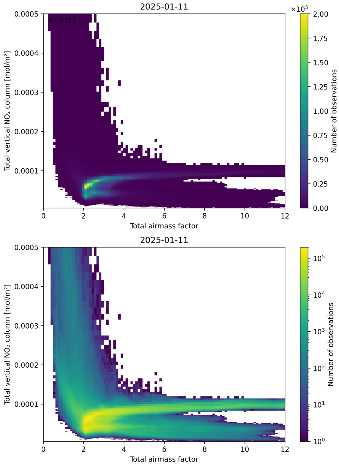
Figure 67: Scatter density plot of “Total air mass factor” against “Total vertical \text{NO}_2 column” for 2025-01-10 to 2025-01-12.
