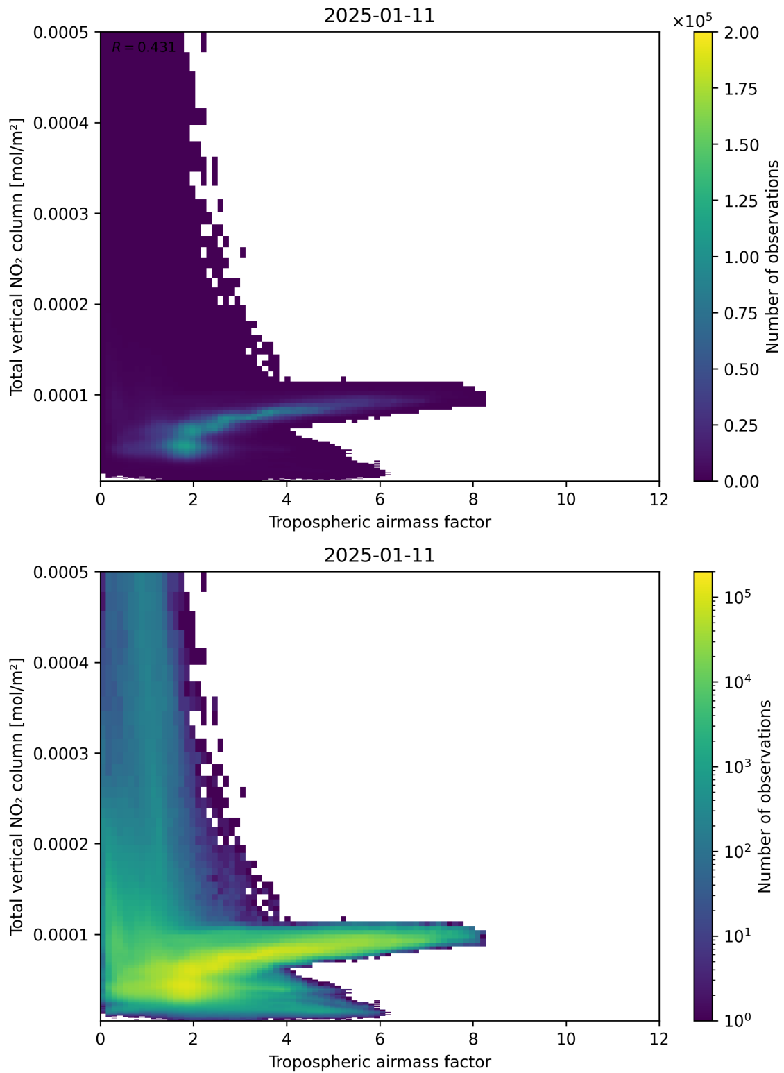
Figure 77: Scatter density plot of “Tropospheric airmass factor” against “Total vertical NO 2 column” for 2025-01-10 to 2025-01-12.
