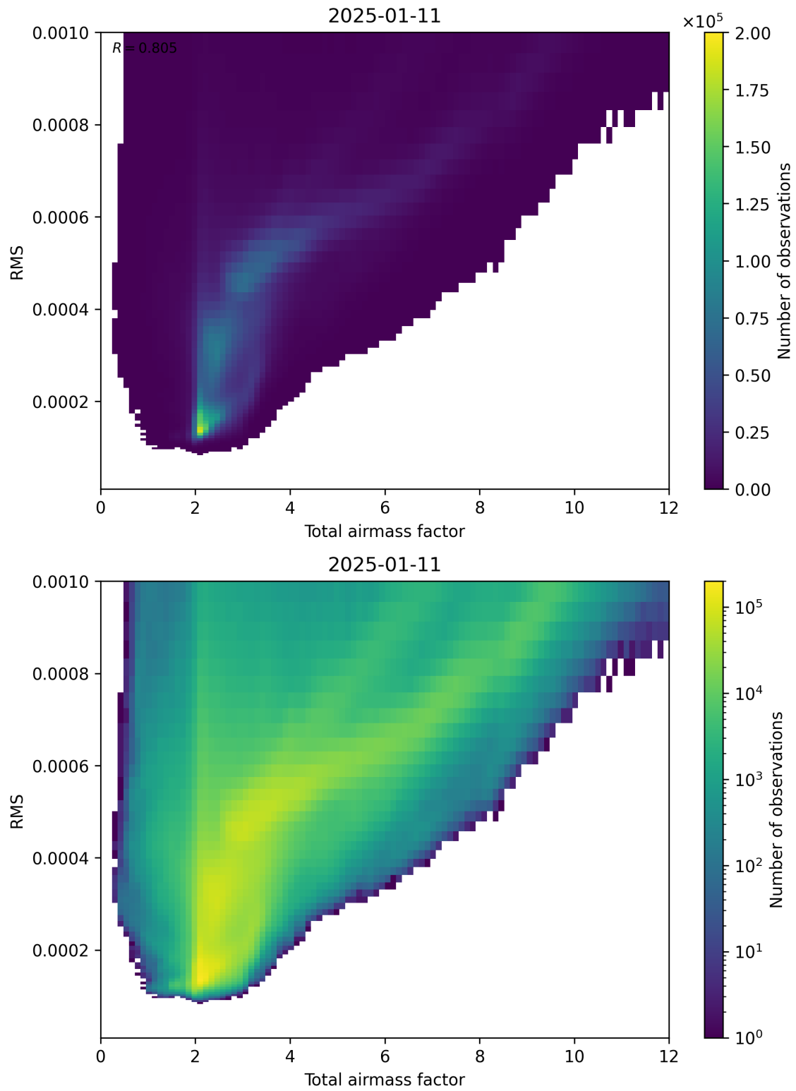
Figure 69: Scatter density plot of “Total airmass factor” against “RMS” for 2025-01-10 to 2025-01-12.
