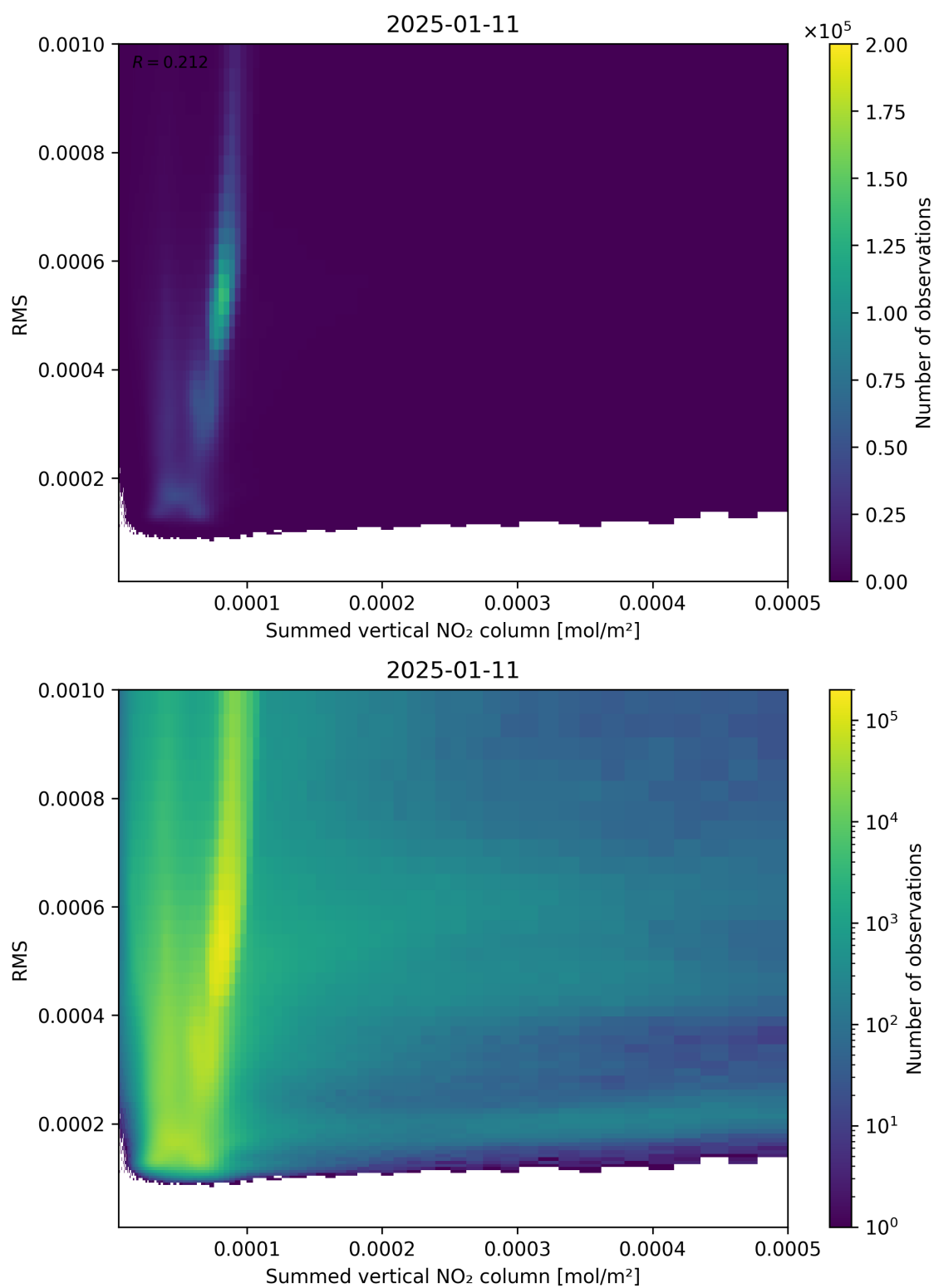
Figure 109: Scatter density plot of “Summed vertical NO 2 column” against “RMS” for 2025-01-10 to 2025-01-12.
