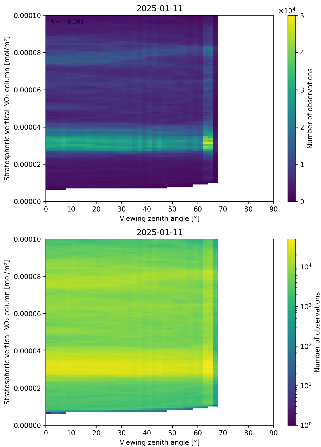
Figure 164: Scatter density plot of “Viewing zenith angle” against “Stratospheric vertical NO 2 column” for 2025-01-10 to 2025-01-12.
