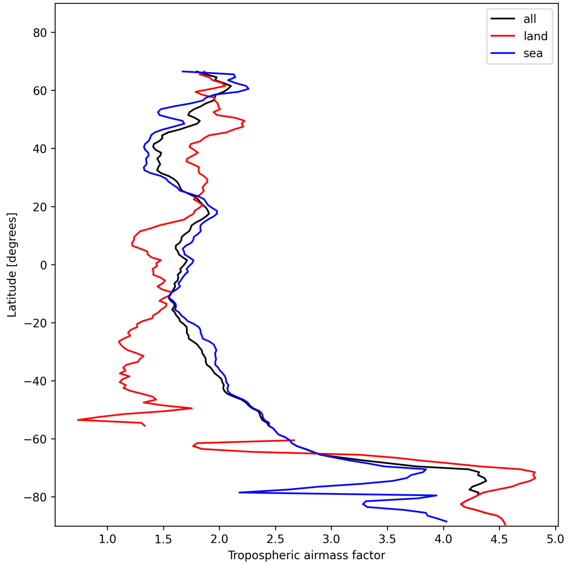
Figure 14: Zonal average of “Tropospheric airmass factor” for 2025-01-10 to 2025-01-12.
