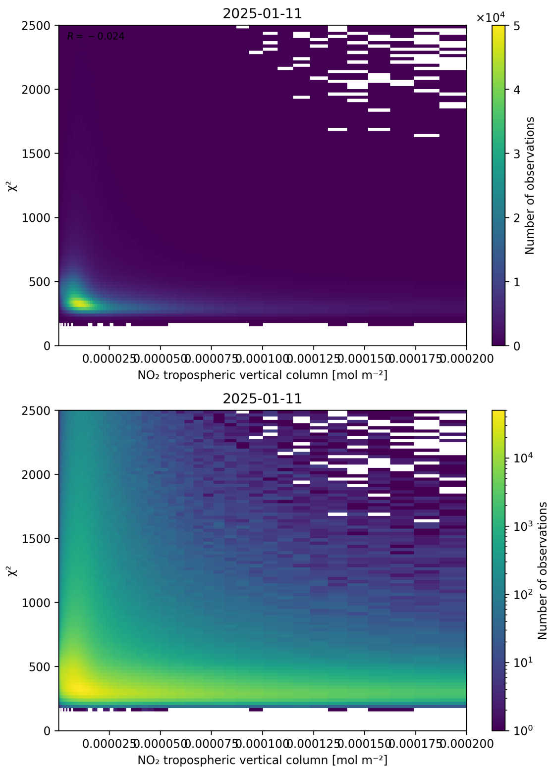
Figure 124: Scatter density plot of “NO 2 tropospheric vertical column” against “ \chi^2 ” for 2025-01-10 to 2025-01-12.
