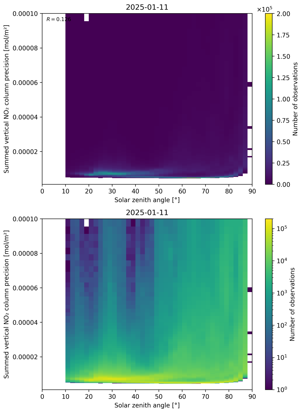
Figure 152: Scatter density plot of “Solar zenith angle” against “Summed vertical NO 2 column precision” for 2025-01-10 to 2025-01-12.
