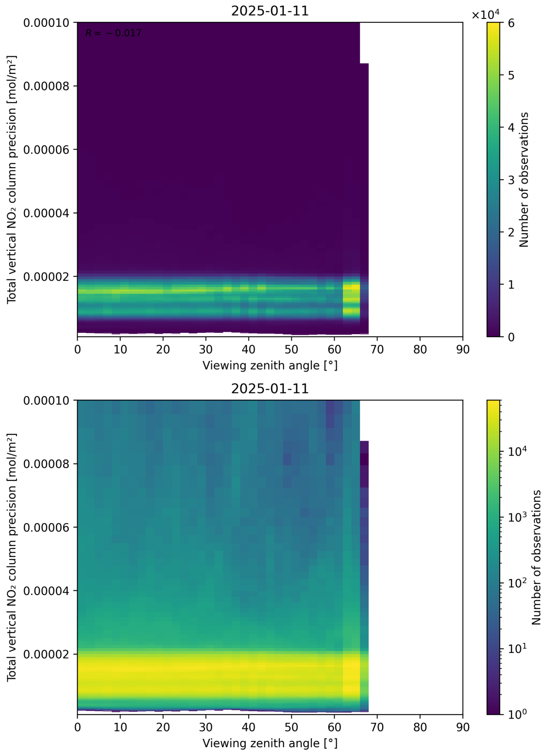
Figure 168: Scatter density plot of “Viewing zenith angle” against “Total vertical NO 2 column precision” for 2025-01-10 to 2025-01-12.
