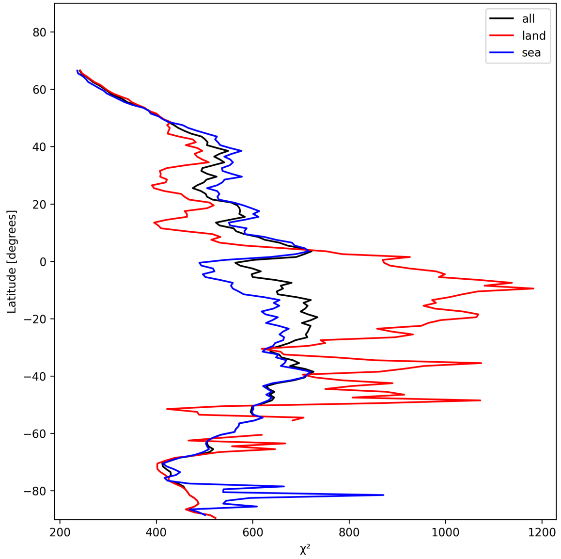
Figure 25: Zonal average of “ \chi^2 ” for 2025-01-10 to 2025-01-12.
