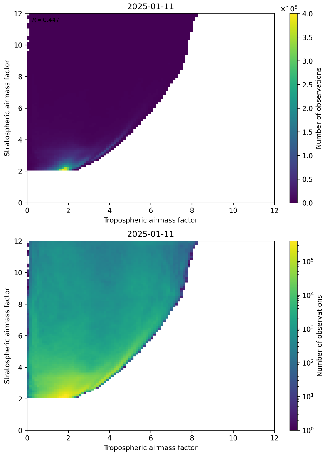
Figure 71: Scatter density plot of “Tropospheric airmass factor” against “Stratospheric airmass factor” for 2025-01-10 to 2025-01-12.
