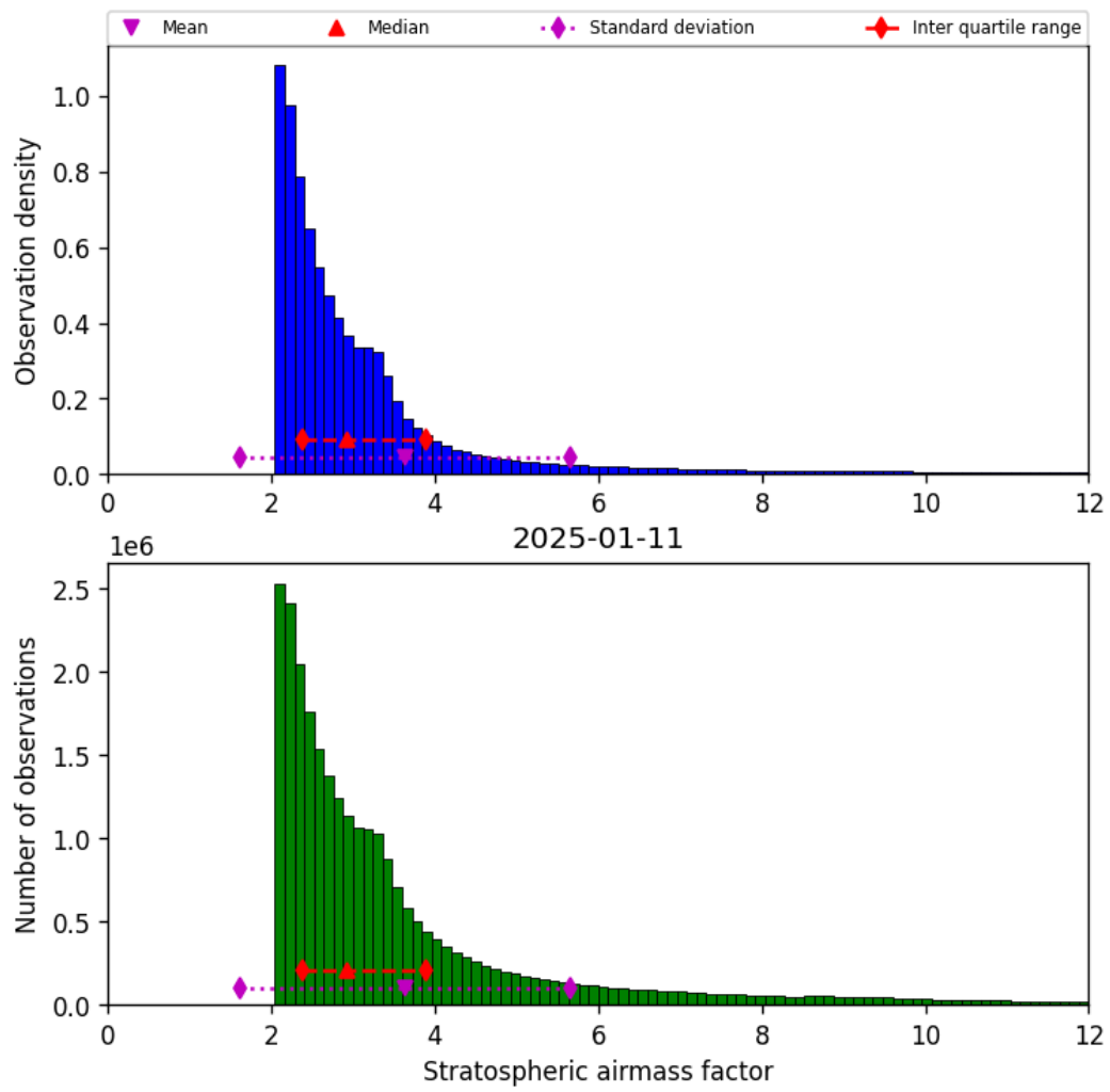
Figure 44: Histogram of “Stratospheric airmass factor” for 2025-01-10 to 2025-01-12
