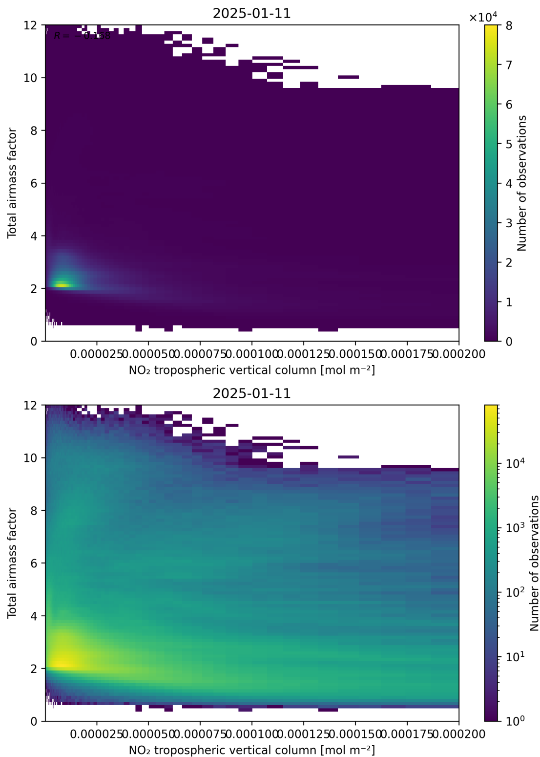
Figure 122: Scatter density plot of “NO 2 tropospheric vertical column” against “Total air mass factor” for 2025-01-10 to 2025-01-12.
