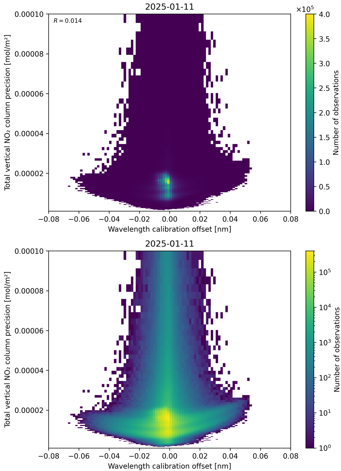
Figure 180: Scatter density plot of “Wavelength calibration offset” against “Total vertical NO 2 column precision” for 2025-01-10 to 2025-01-12.
