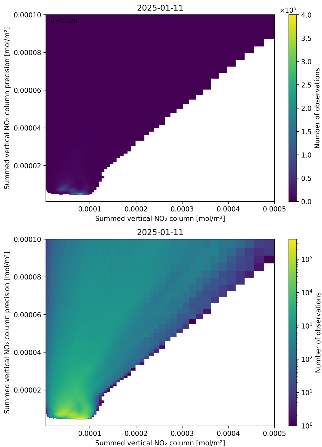
Figure 105: Scatter density plot of “Summed vertical NO 2 column” against “Summed vertical NO 2 column precision” for 2025-01-10 to 2025-01-12.
