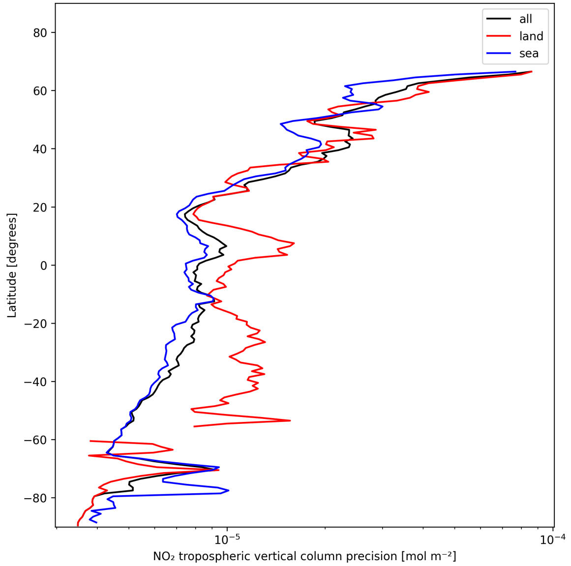
Figure 13: Zonal average of “NO 2 tropospheric vertical column precision” for 2025-01-10 to 2025-01-12.
