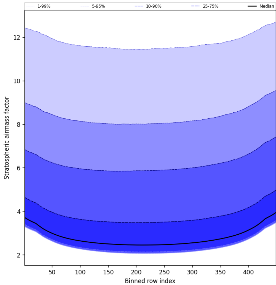
Figure 61: Along track statistics of “Stratospheric airmass factor” for 2025-01-10 to 2025-01-12
