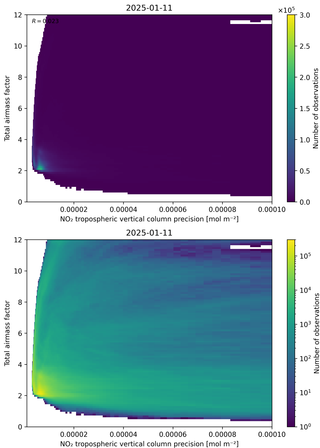
Figure 132: Scatter density plot of “NO 2 tropospheric vertical column precision” against “Total air mass factor” for 2025-01-10 to 2025-01-12.
