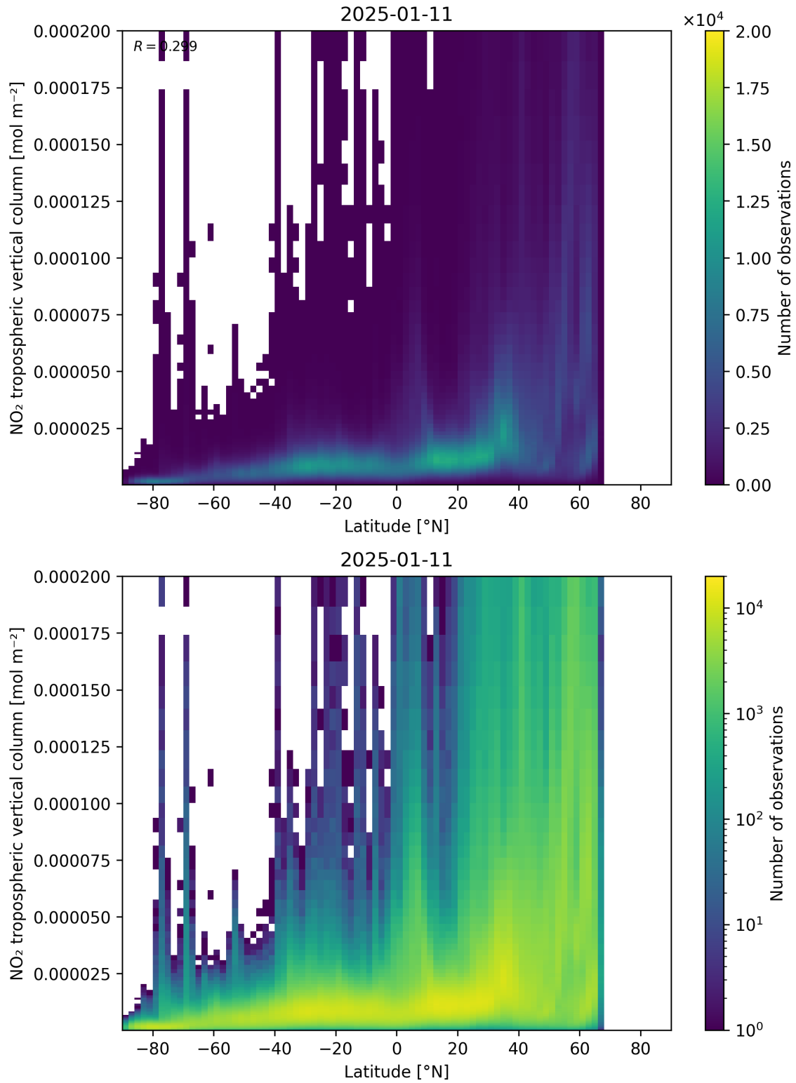
Figure 92: Scatter density plot of “Latitude” against “NO 2 tropospheric vertical column” for 2025-01-10 to 2025-01-12.
