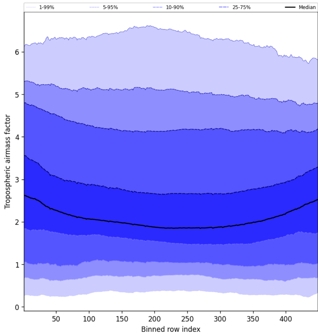
Figure 48: Along track statistics of “Tropospheric airmass factor” for 2025-01-10 to 2025-01-12
