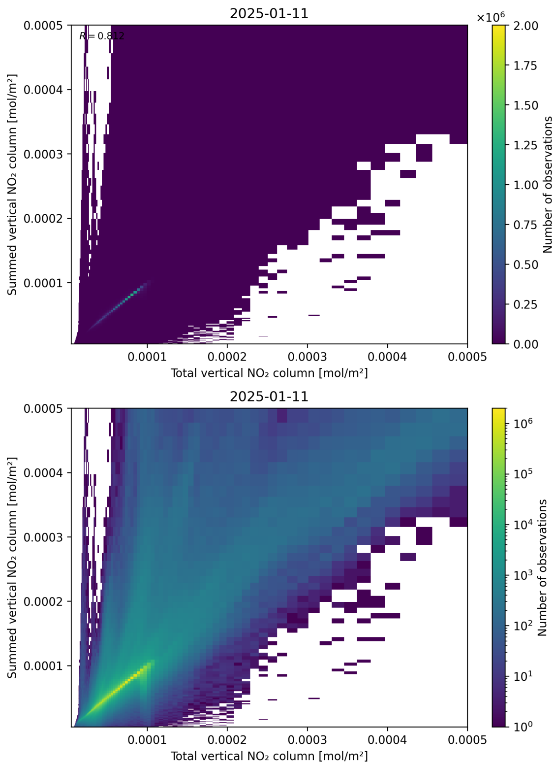
Figure 112: Scatter density plot of “Total vertical NO 2 column” against “Summed vertical NO 2 column” for 2025-01-10 to 2025-01-12.
