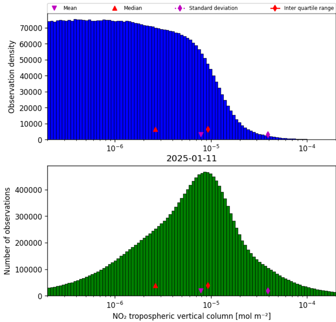
Figure 29: Histogram of “NO 2 tropospheric vertical column” for 2025-01-10 to 2025-01-12
