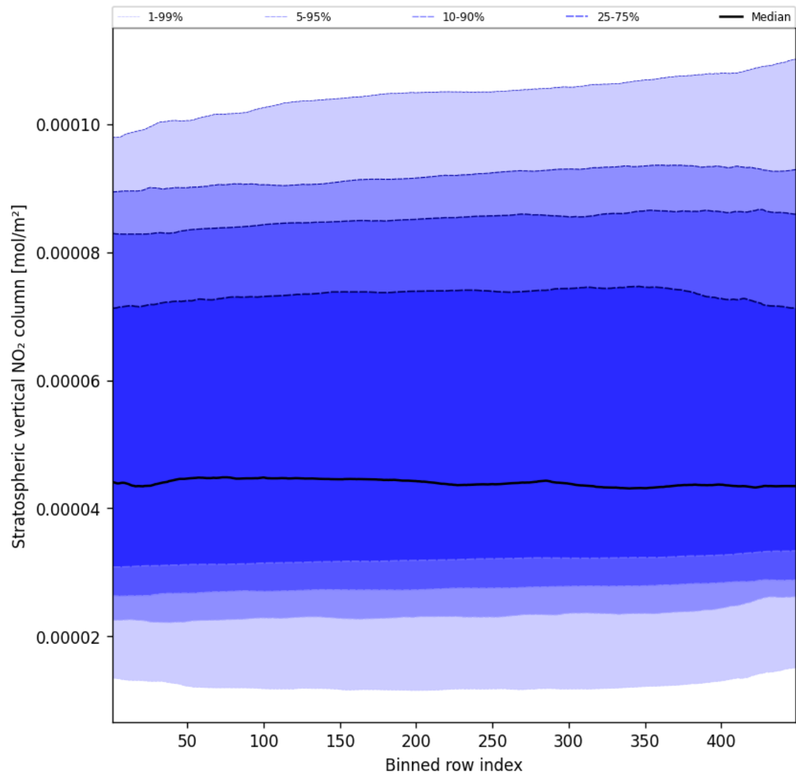
Figure 53: Along track statistics of “Stratospheric vertical NO 2 column” for 2025-01-10 to 2025-01-12
