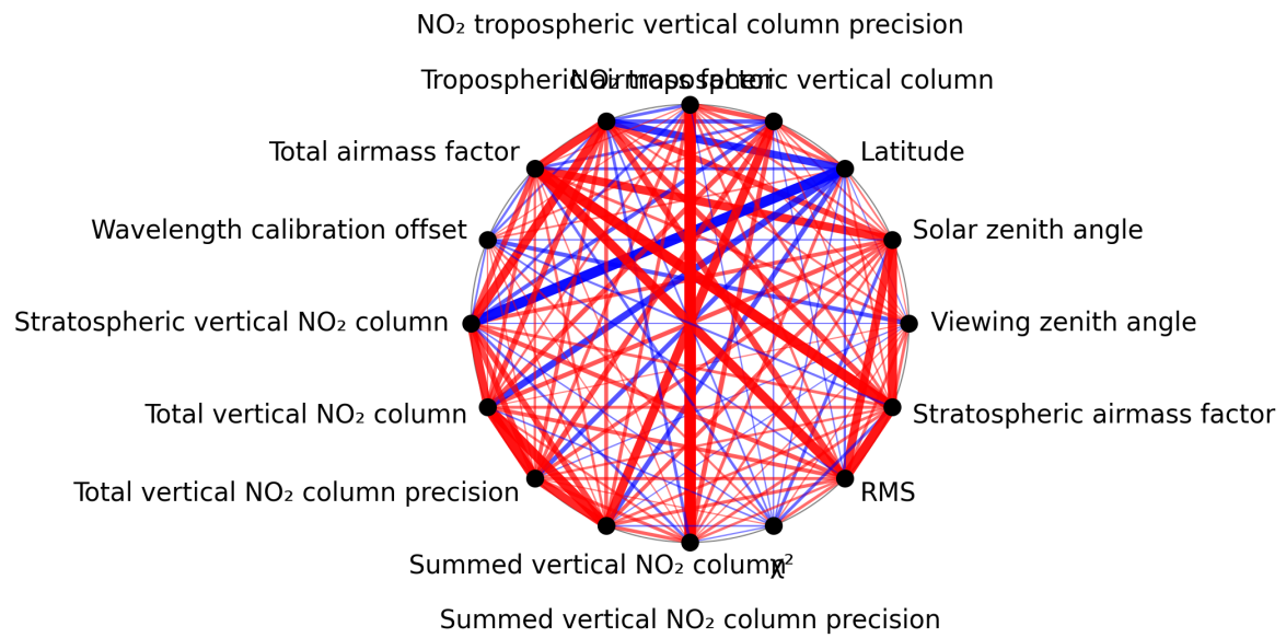
Figure 1: Map of correlation graph for 2025-01-10 to 2025-01-12.
