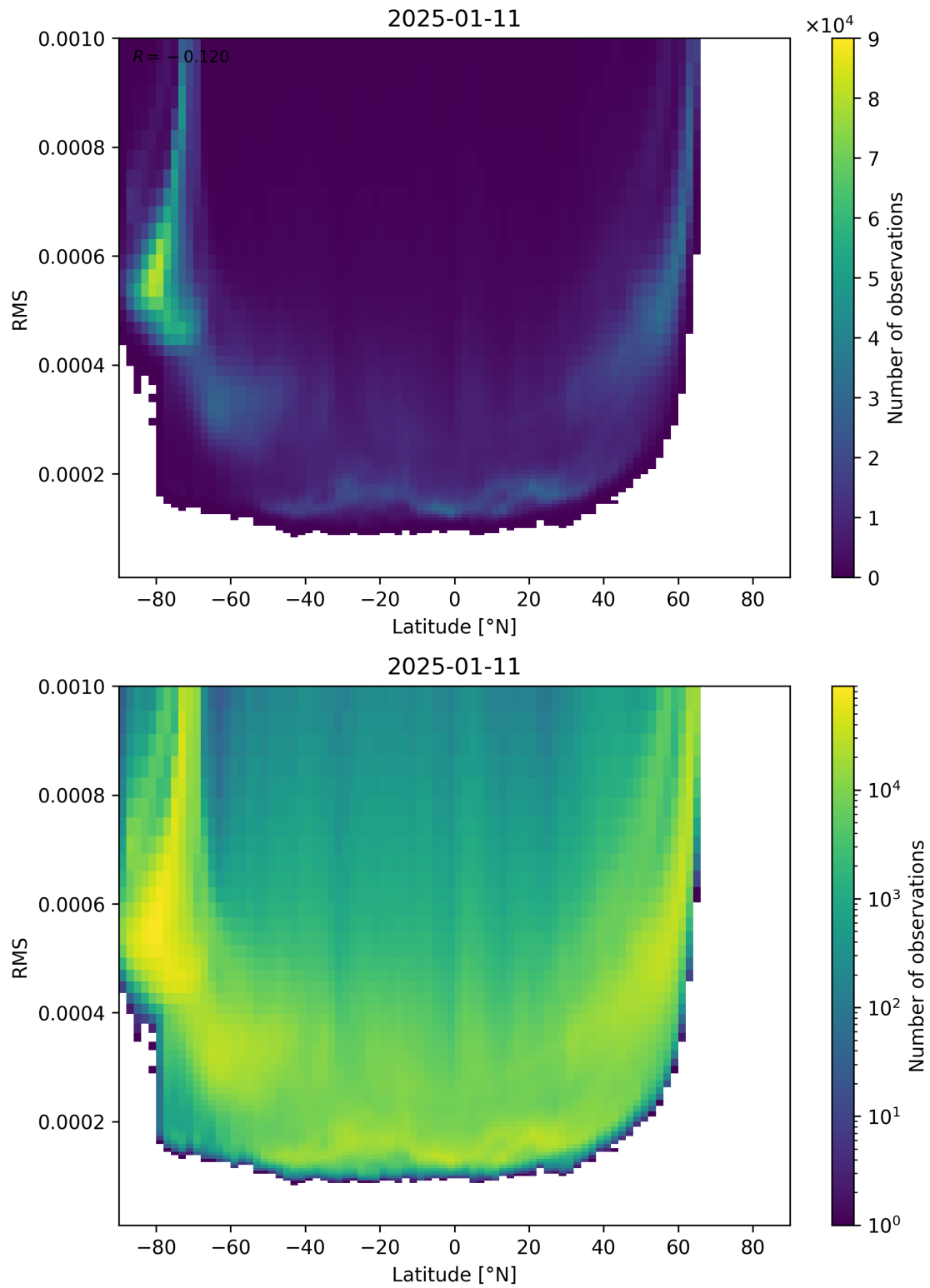
Figure 94: Scatter density plot of “Latitude” against “RMS” for 2025-01-10 to 2025-01-12.
