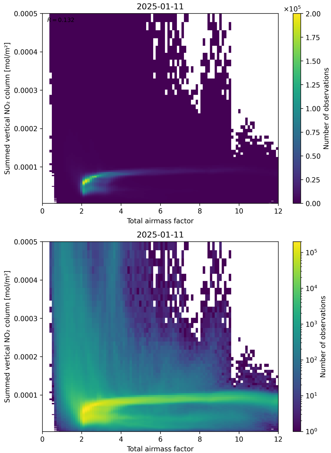
Figure 65: Scatter density plot of “Total airmass factor” against “Summed vertical NO 2 column” for 2025-01-10 to 2025-01-12.
