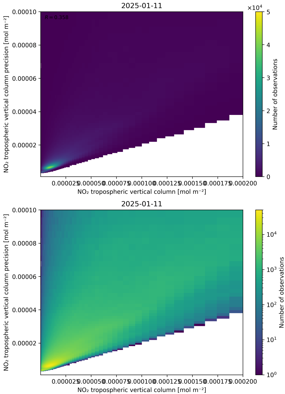
Figure 130: Scatter density plot of “NO 2 tropospheric vertical column” against “NO 2 tropospheric vertical column precision” for 2025-01-10 to 2025-01-12.
