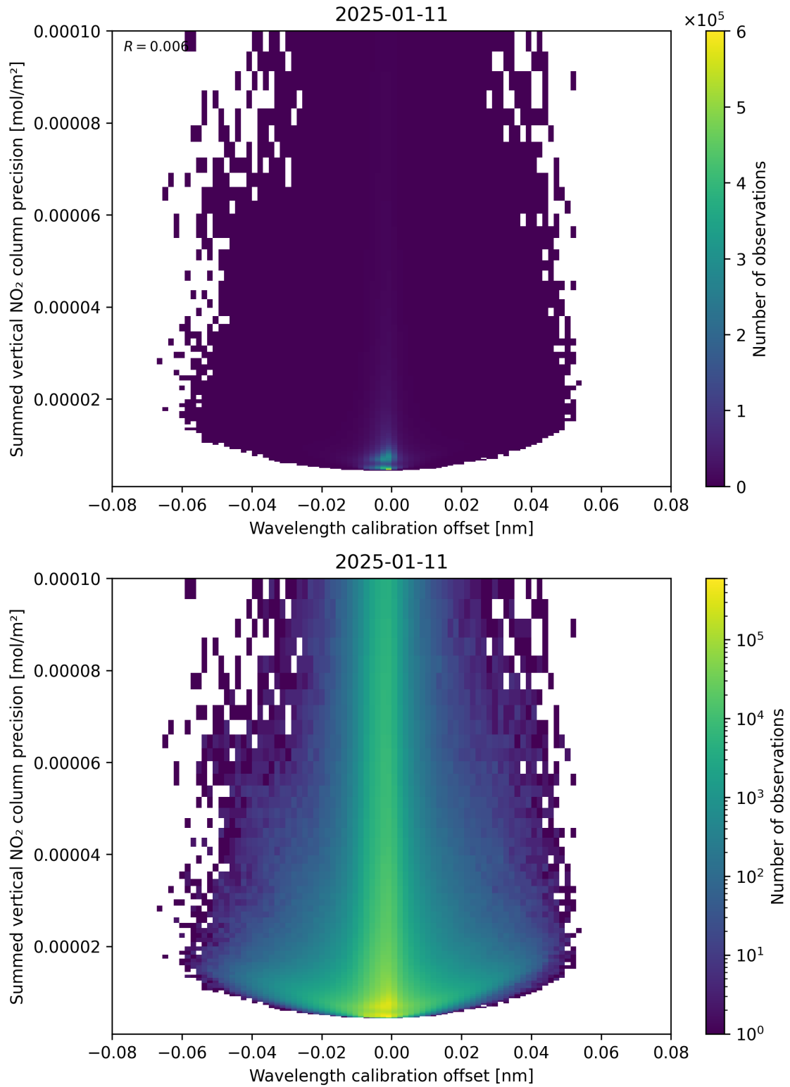
Figure 178: Scatter density plot of “Wavelength calibration offset” against “Summed vertical NO 2 column precision” for 2025-01-10 to 2025-01-12.
