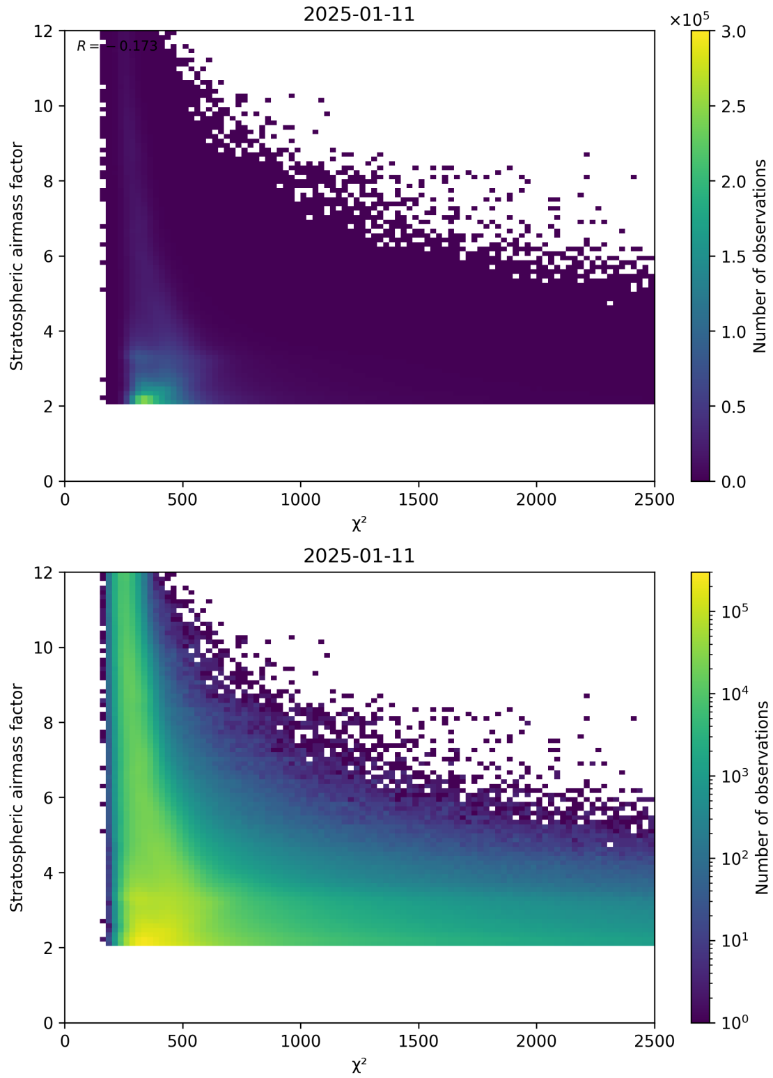
Figure 81: Scatter density plot of “ \chi^2 ” against “Stratospheric airmass factor” for 2025-01-10 to 2025-01-12.
