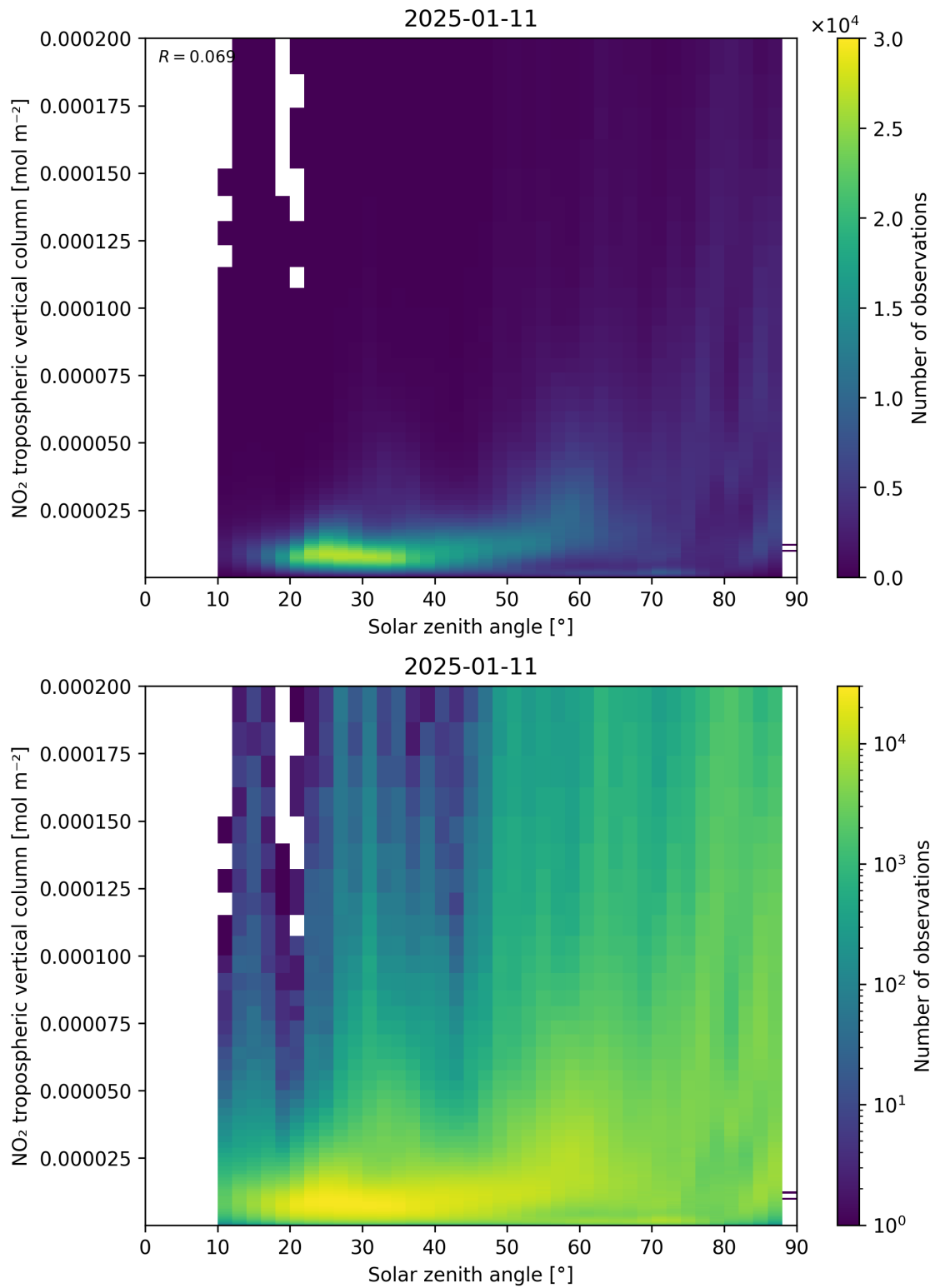
Figure 155: Scatter density plot of “Solar zenith angle” against “NO 2 tropospheric vertical column” for 2025-01-10 to 2025-01-12.
