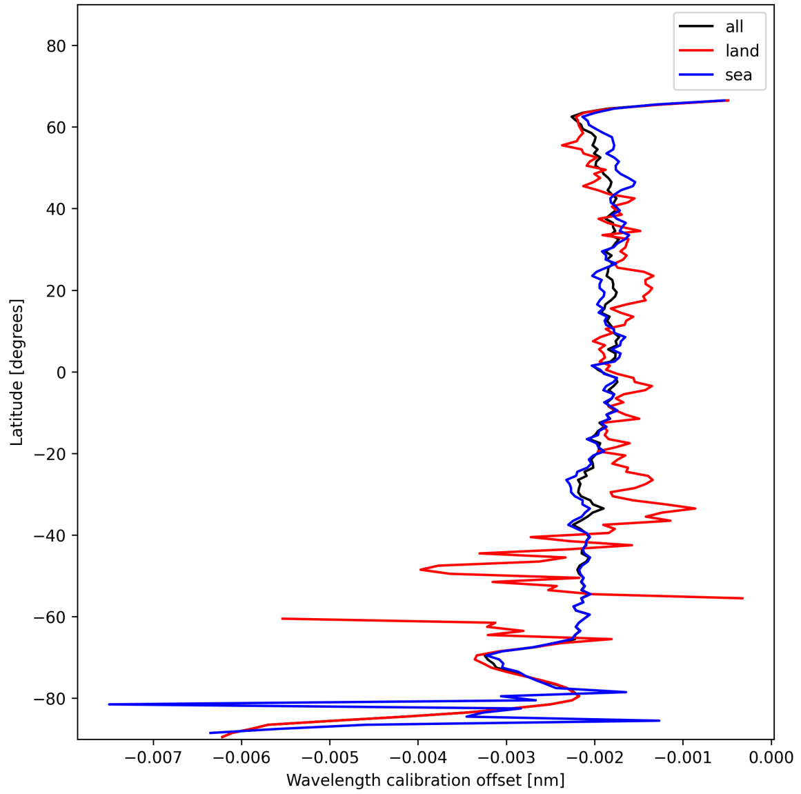
Figure 18: Zonal average of “Wavelength calibration offset” for 2025-01-10 to 2025-01-12.
