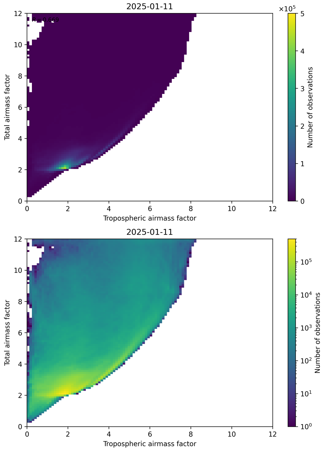
Figure 72: Scatter density plot of “Tropospheric airmass factor” against “Total airmass factor” for 2025-01-10 to 2025-01-12.
