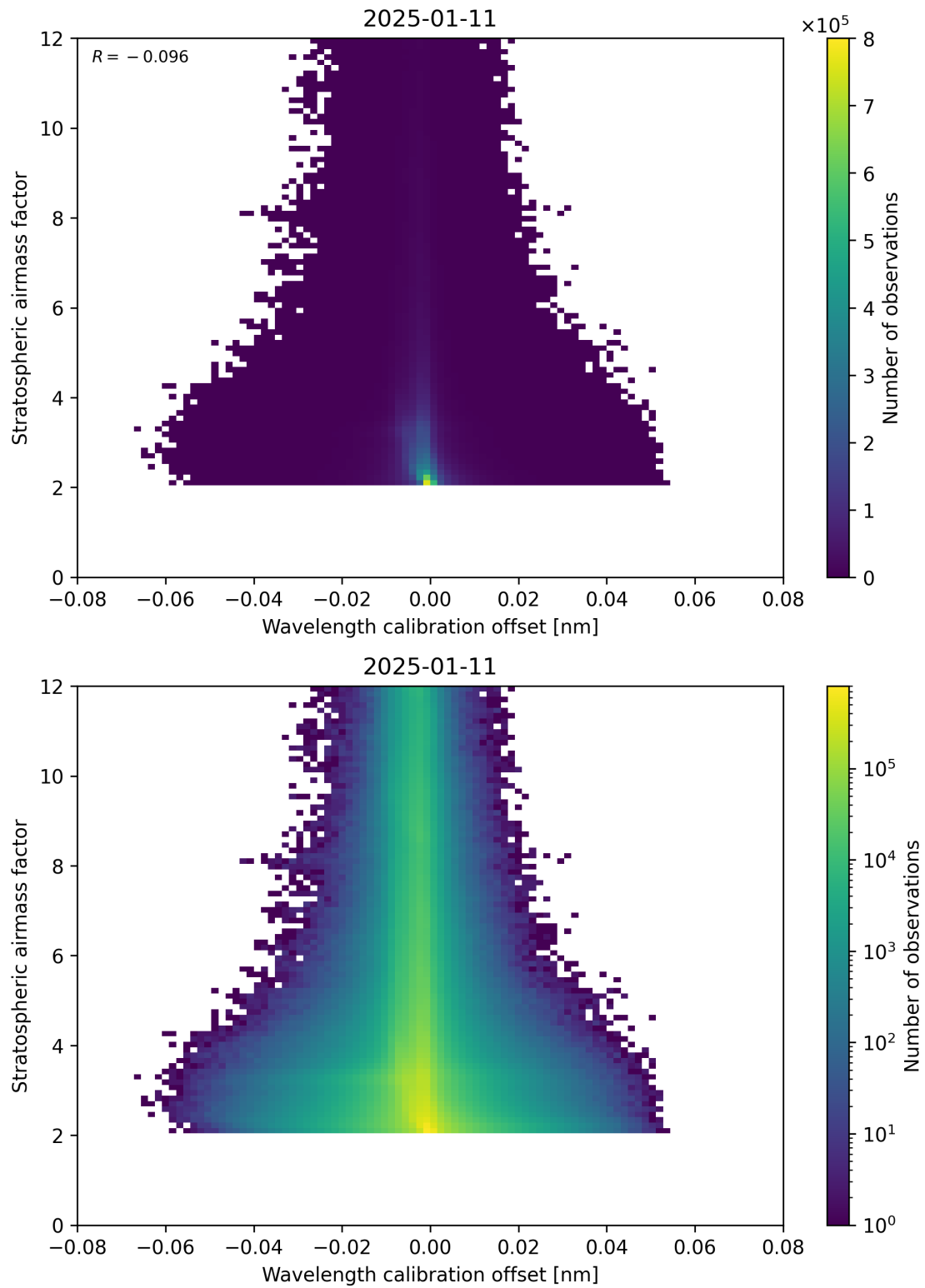
Figure 174: Scatter density plot of “Wavelength calibration offset” against “Stratospheric airmass factor” for 2025-01-10 to 2025-01-12.
