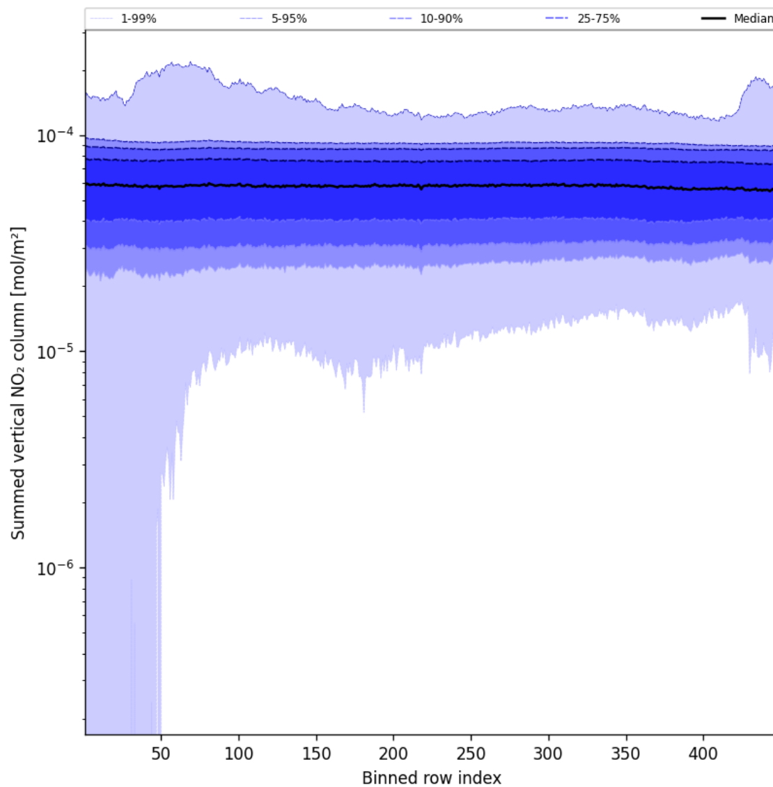
Figure 57: Along track statistics of “Summed vertical NO 2 column” for 2025-01-10 to 2025-01-12
