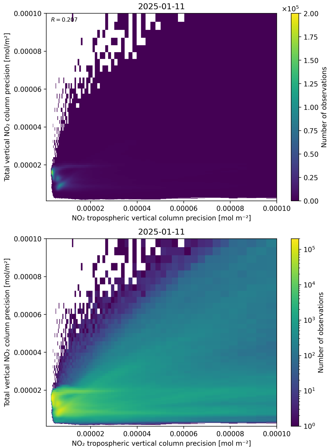
Figure 139: Scatter density plot of “NO 2 tropospheric vertical column precision” against “Total vertical NO 2 column precision” for 2025-01-10 to 2025-01-12.
