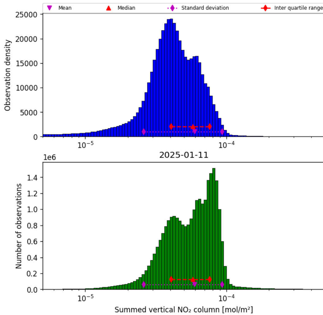
Figure 40: Histogram of “Summed vertical NO 2 column” for 2025-01-10 to 2025-01-12
