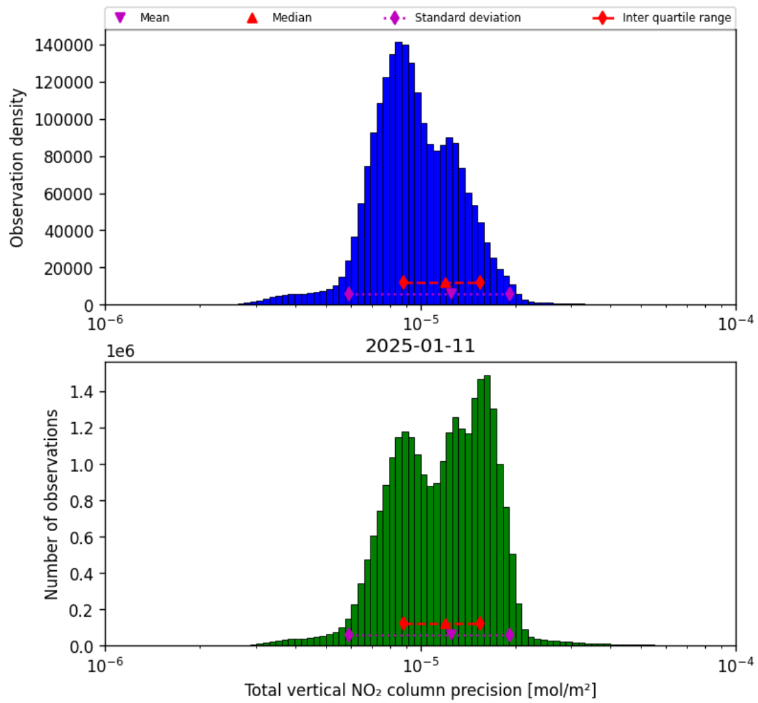
Figure 39: Histogram of “Total vertical NO 2 column precision” for 2025-01-10 to 2025-01-12
