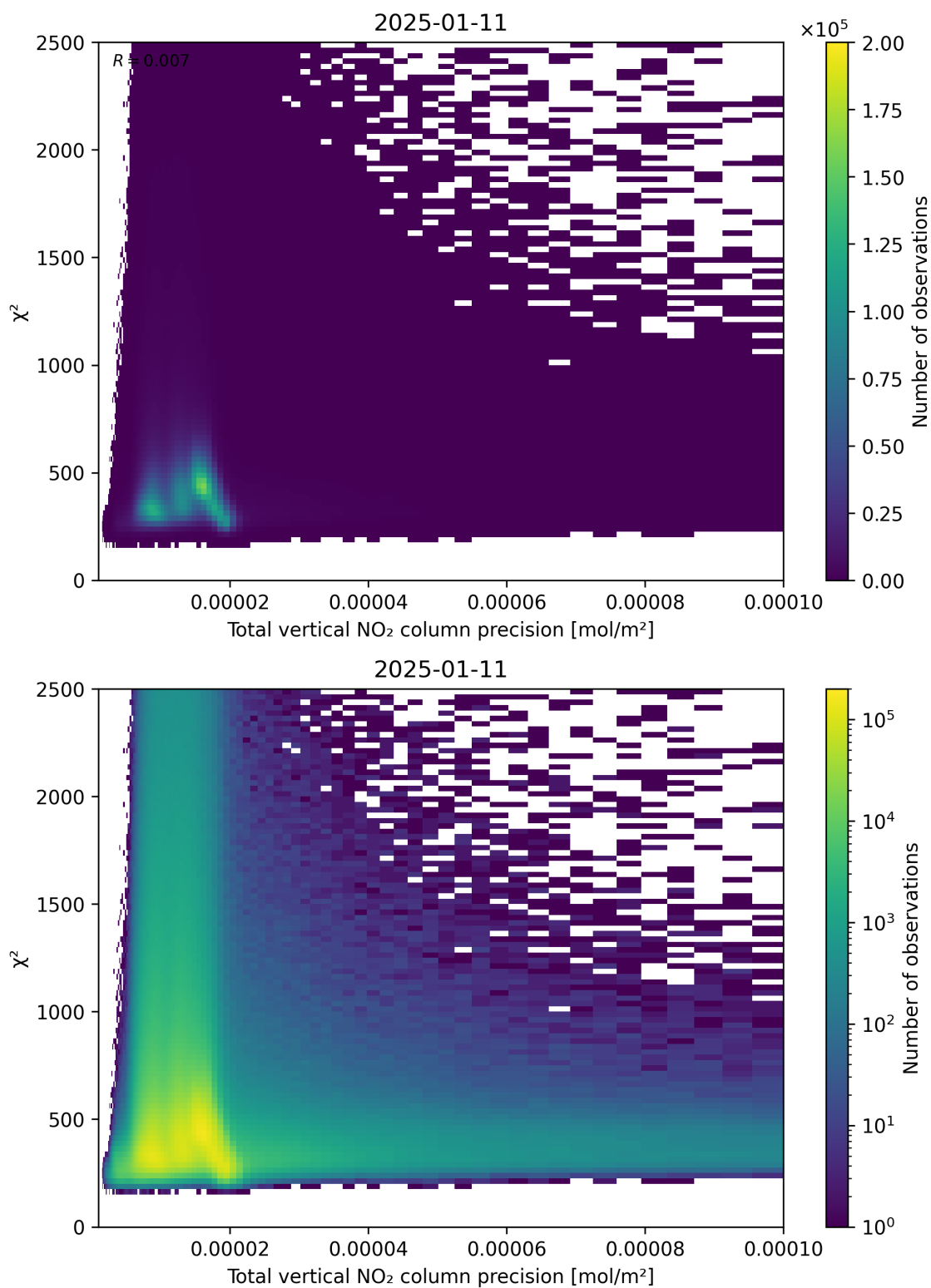
Figure 116: Scatter density plot of “Total vertical NO 2 column precision” against “ \chi^2 ” for 2025-01-10 to 2025-01-12.
