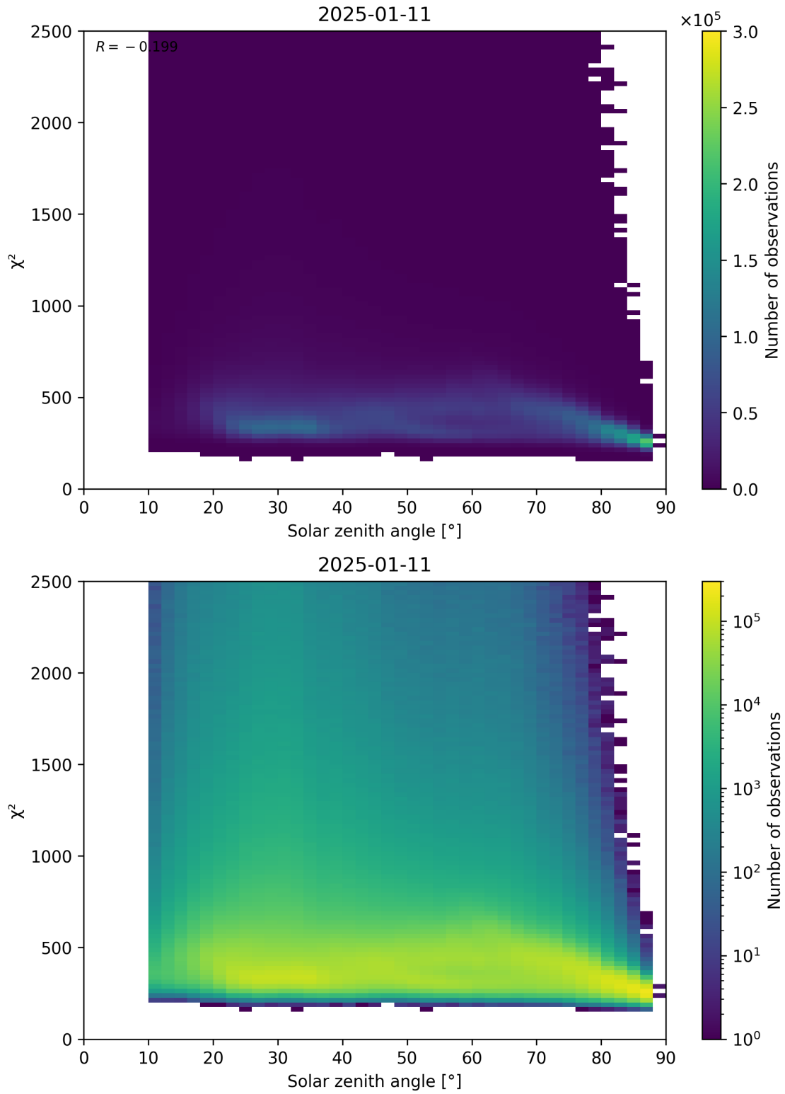
Figure 148: Scatter density plot of “Solar zenith angle” against “ \chi^2 ” for 2025-01-10 to 2025-01-12.
