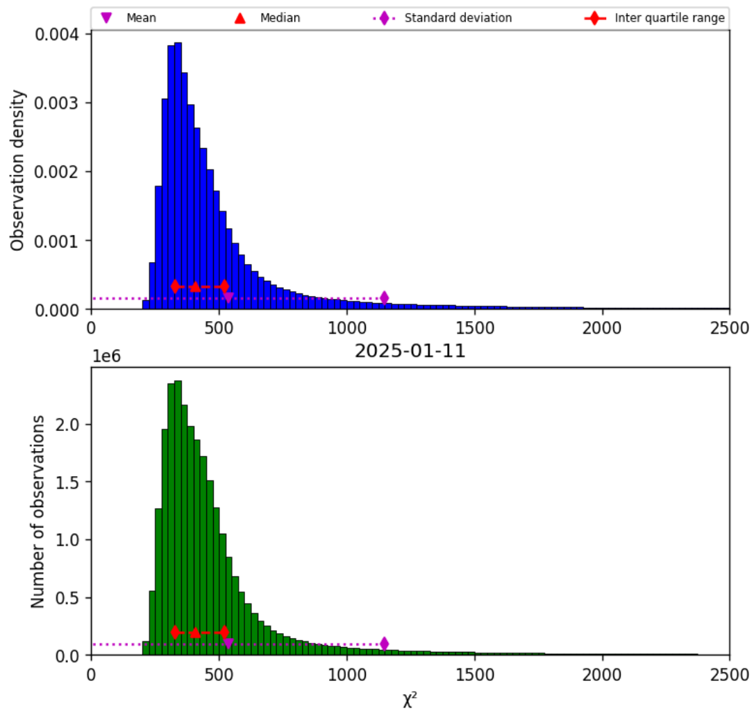
Figure 42: Histogram of “ \chi^2 ” for 2025-01-10 to 2025-01-12
