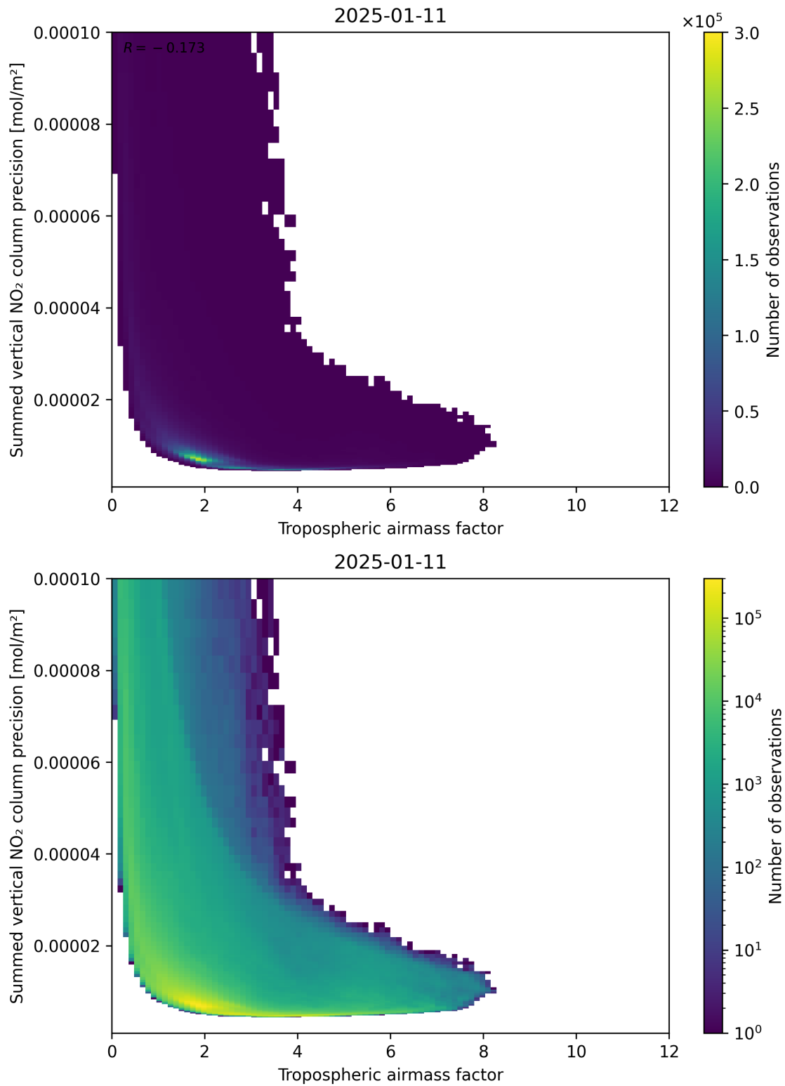
Figure 76: Scatter density plot of “Tropospheric air mass factor” against “Summed vertical NO 2 column precision” for 2025-01-10 to 2025-01-12.
