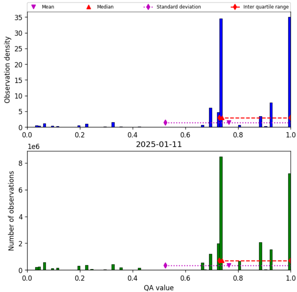
Figure 28: Histogram of “QA value” for 2025-01-10 to 2025-01-12
