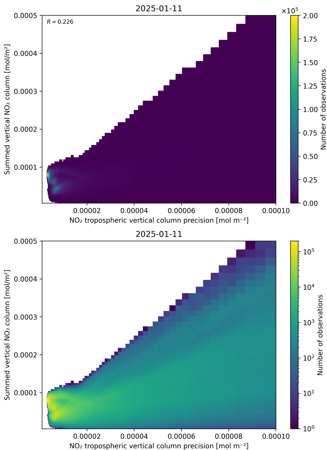
Figure 136: Scatter density plot of “NO 2 tropospheric vertical column precision” against “Summed vertical NO 2 column” for 2025-01-10 to 2025-01-12.
