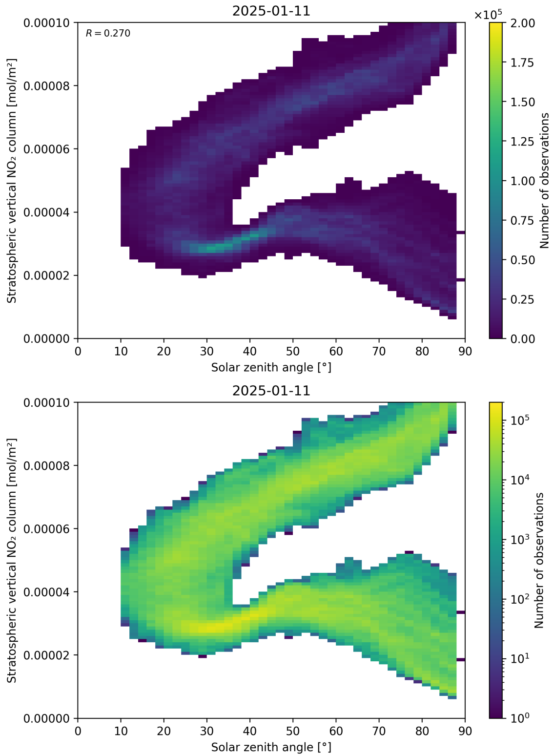
Figure 150: Scatter density plot of “Solar zenith angle” against “Stratospheric vertical NO 2 column” for 2025-01-10 to 2025-01-12.
