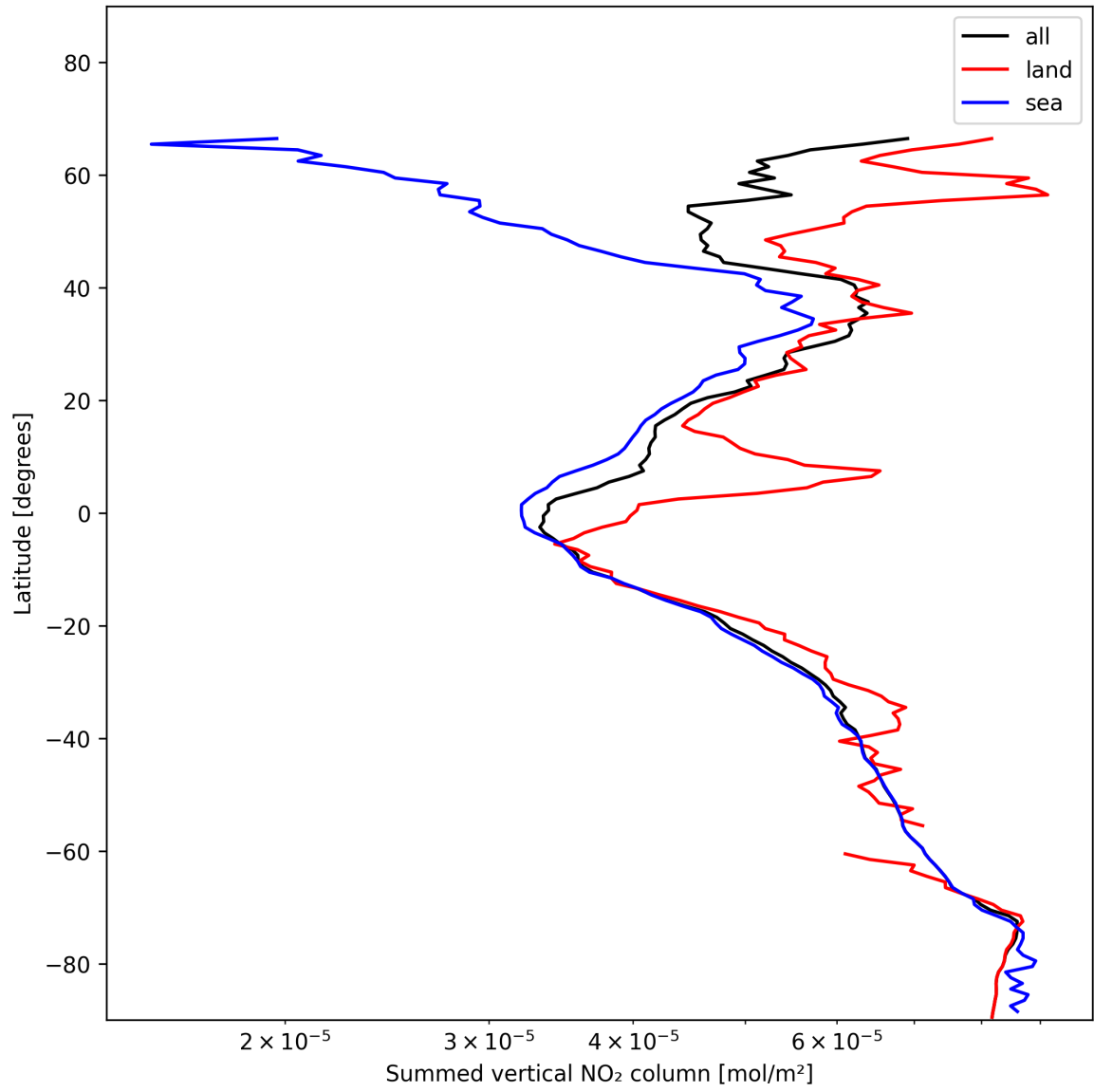
Figure 23: Zonal average of “Summed vertical NO 2 column” for 2025-01-10 to 2025-01-12.
