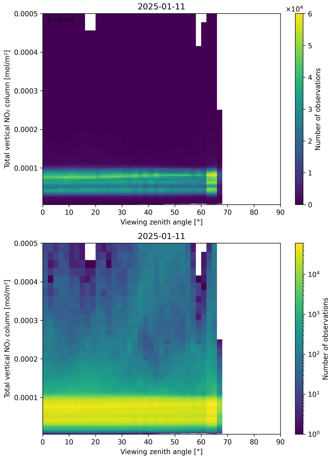
Figure 167: Scatter density plot of “Viewing zenith angle” against “Total vertical NO 2 column” for 2025-01-10 to 2025-01-12.
