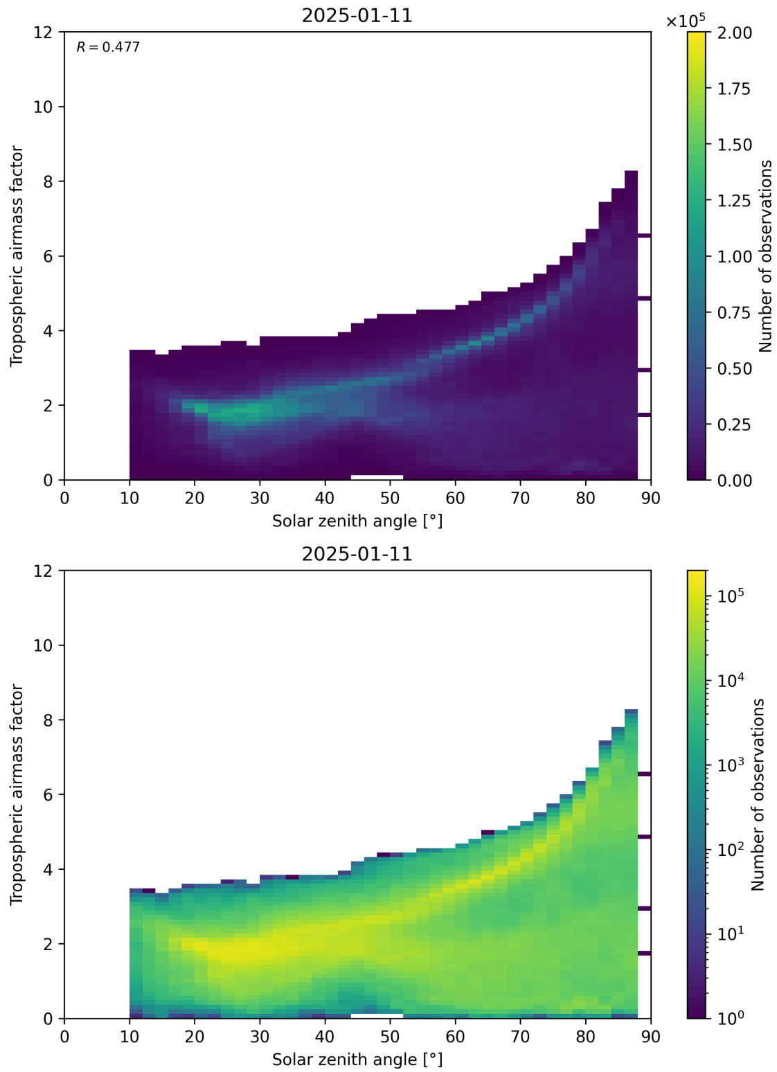
Figure 147: Scatter density plot of “Solar zenith angle” against “Tropospheric airmass factor” for 2025-01-10 to 2025-01-12.
