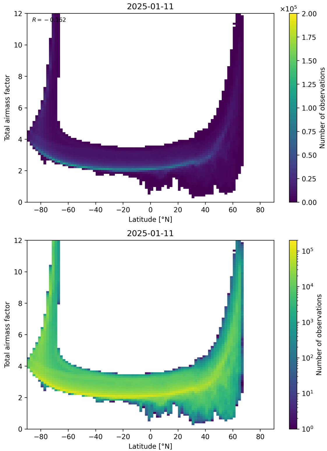
Figure 84: Scatter density plot of “Latitude” against “Total airmass factor” for 2025-01-10 to 2025-01-12.
