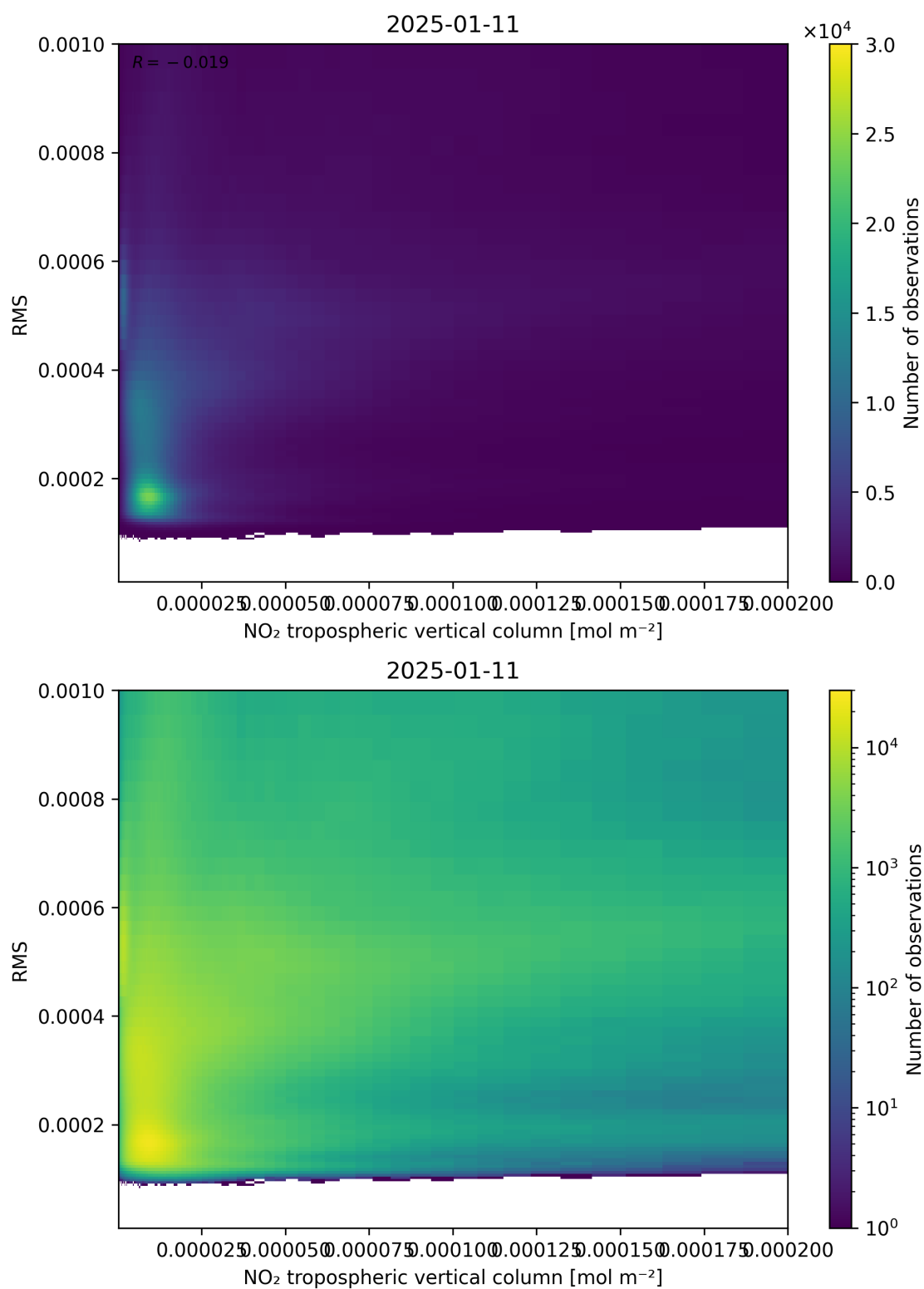
Figure 142: Scatter density plot of “NO 2 tropospheric vertical column” against “RMS” for 2025-01-10 to 2025-01-12.
