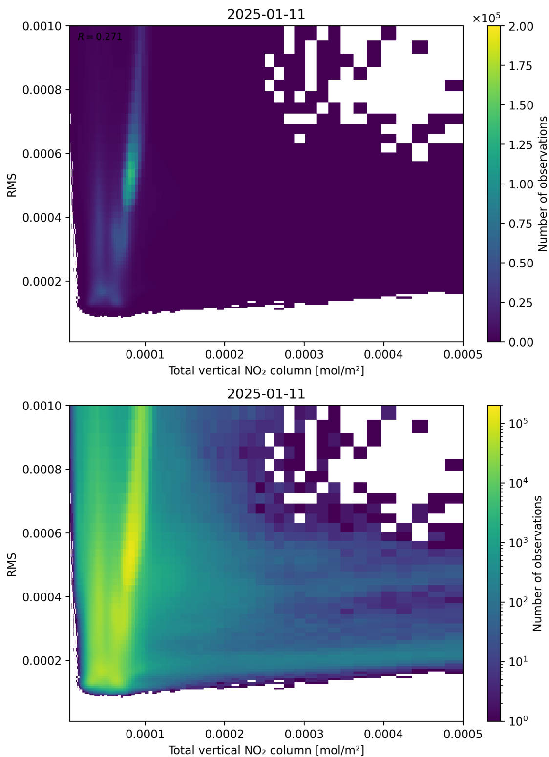
Figure 120: Scatter density plot of “Total vertical NO 2 column” against “RMS” for 2025-01-10 to 2025-01-12.
