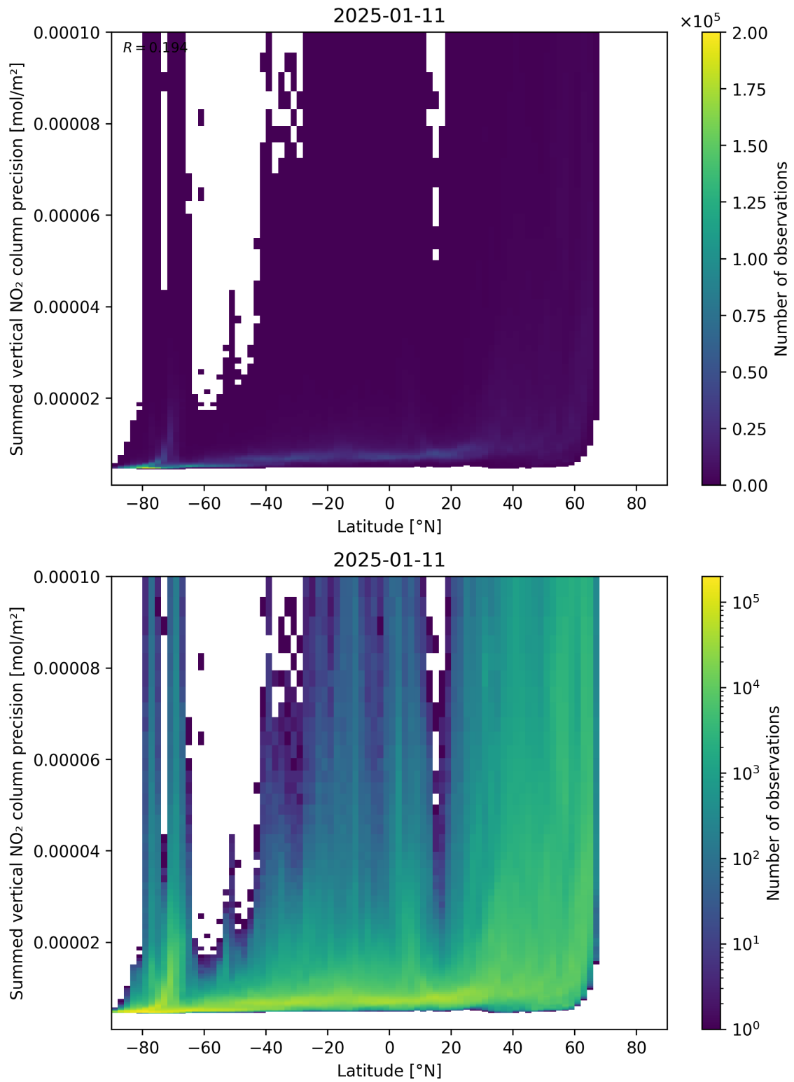
Figure 89: Scatter density plot of “Latitude” against “Summed vertical NO 2 column precision” for 2025-01-10 to 2025-01-12.
