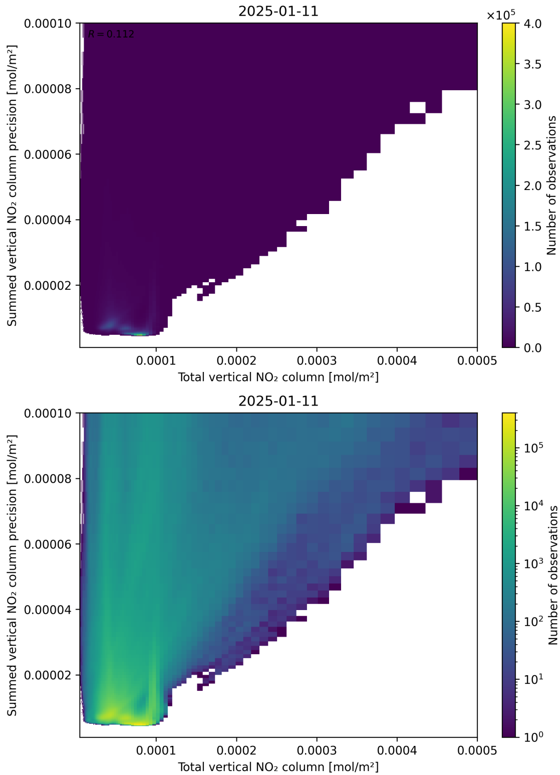
Figure 113: Scatter density plot of “Total vertical NO 2 column” against “Summed vertical NO 2 column precision” for 2025-01-10 to 2025-01-12.
