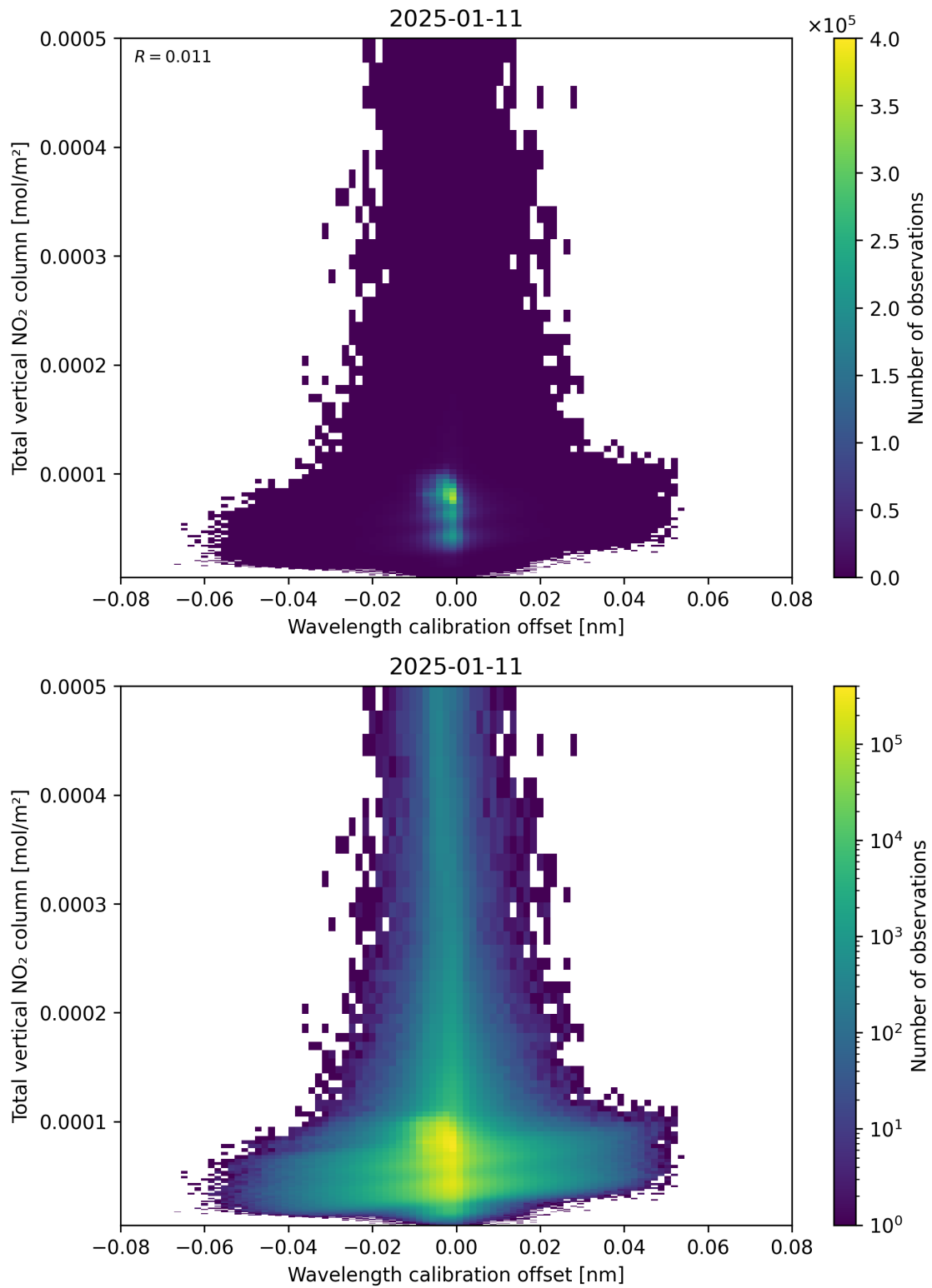
Figure 179: Scatter density plot of “Wavelength calibration offset” against “Total vertical NO 2 column” for 2025-01-10 to 2025-01-12.
