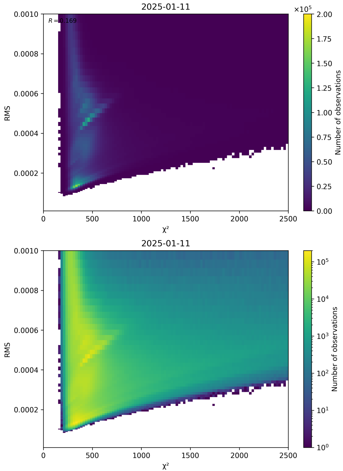
Figure 82: Scatter density plot of “ \chi^2 ” against “RMS” for 2025-01-10 to 2025-01-12.
