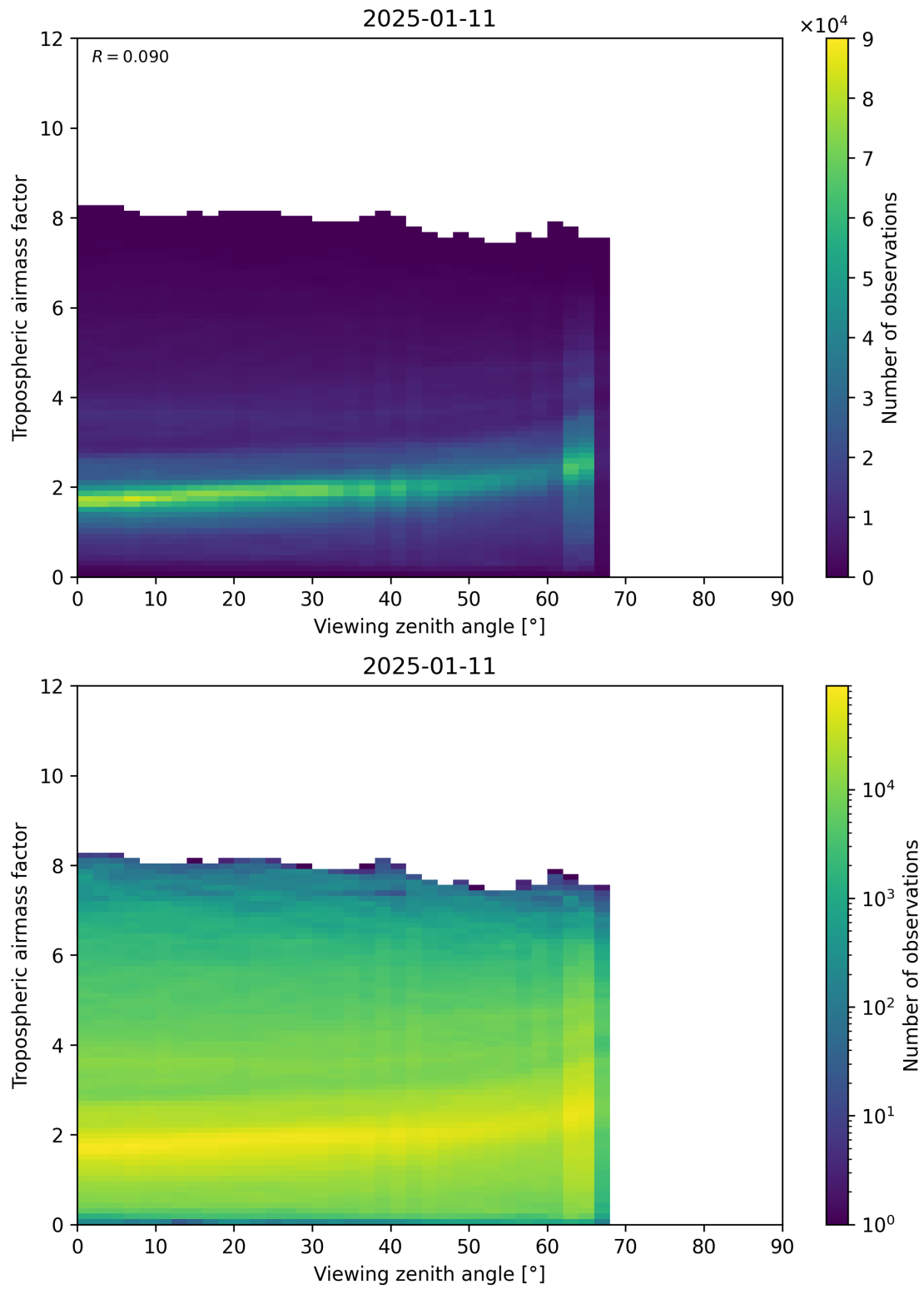
Figure 161: Scatter density plot of “Viewing zenith angle” against “Tropospheric airmass factor” for 2025-01-10 to 2025-01-12.
