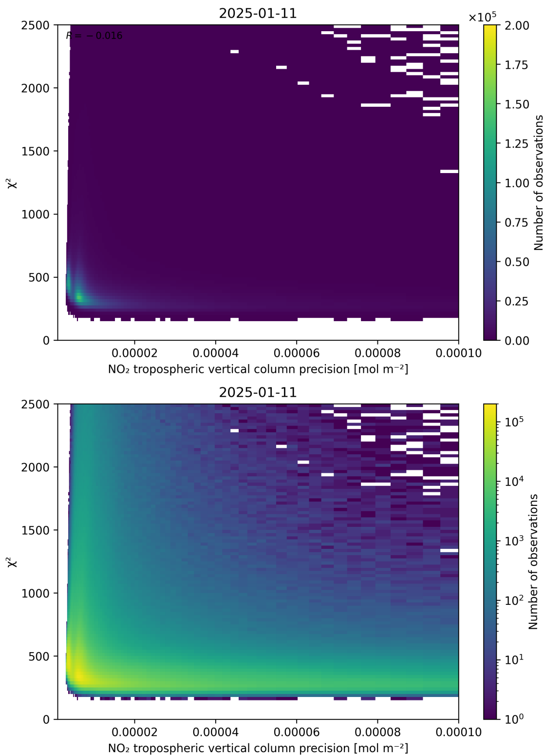
Figure 134: Scatter density plot of “NO 2 tropospheric vertical column precision” against “ \chi^2 ” for 2025-01-10 to 2025-01-12.
