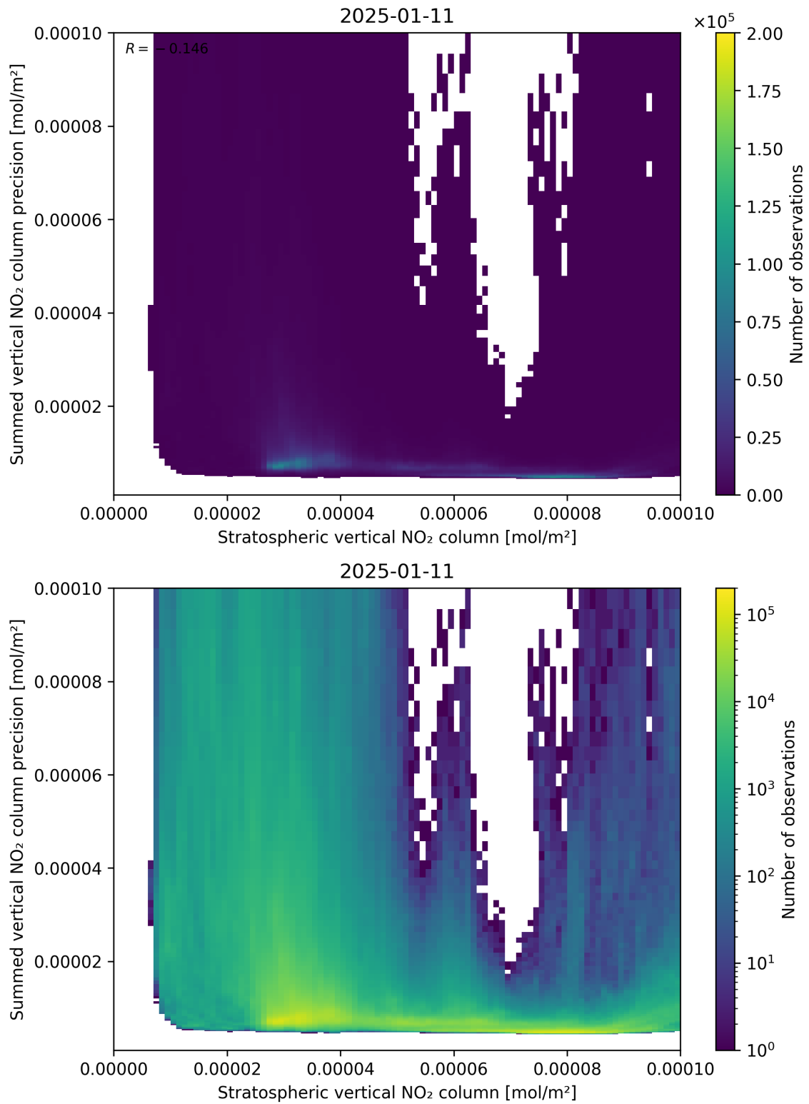
Figure 99: Scatter density plot of “Stratospheric vertical NO 2 column” against “Summed vertical NO 2 column precision” for 2025-01-10 to 2025-01-12.
