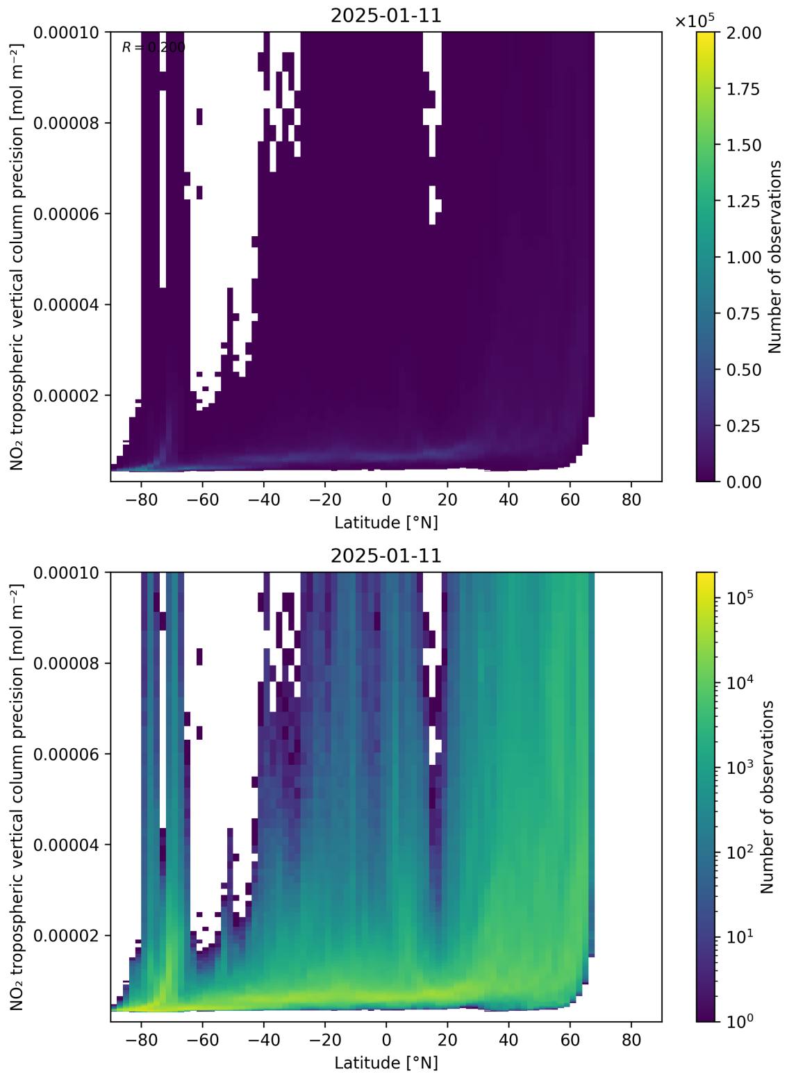
Figure 93: Scatter density plot of “Latitude” against “NO 2 tropospheric vertical column precision” for 2025-01-10 to 2025-01-12.
