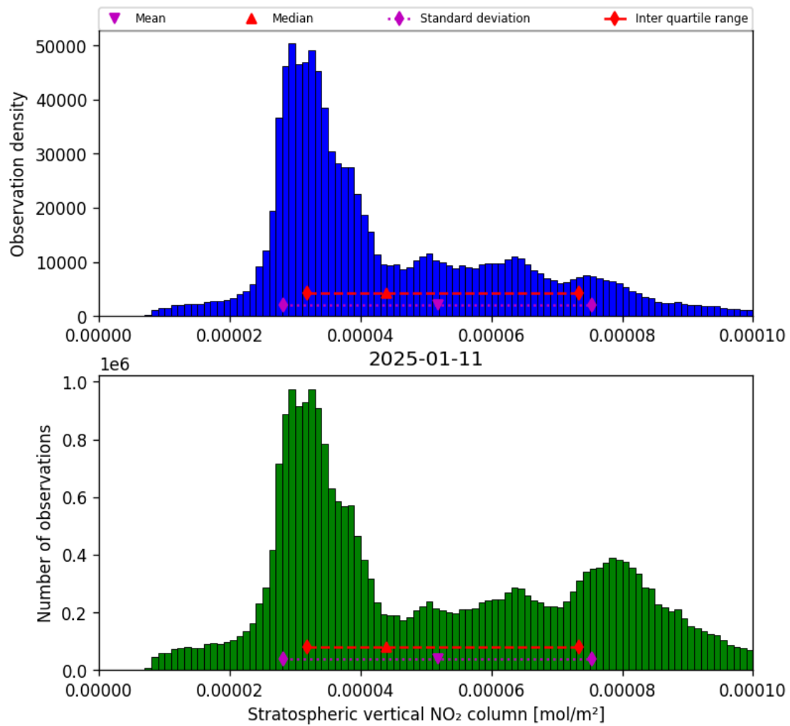
Figure 36: Histogram of “Stratospheric vertical NO 2 column” for 2025-01-10 to 2025-01-12
