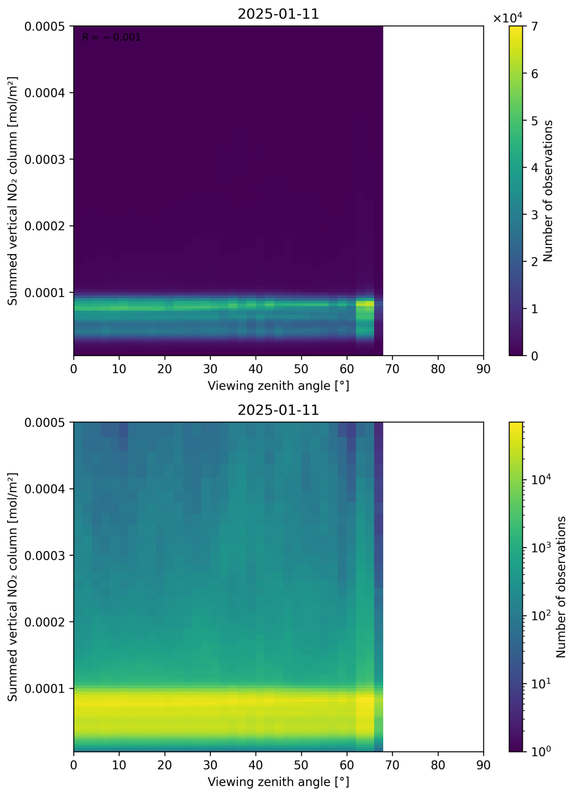
Figure 165: Scatter density plot of “Viewing zenith angle” against “Summed vertical NO 2 column” for 2025-01-10 to 2025-01-12.
