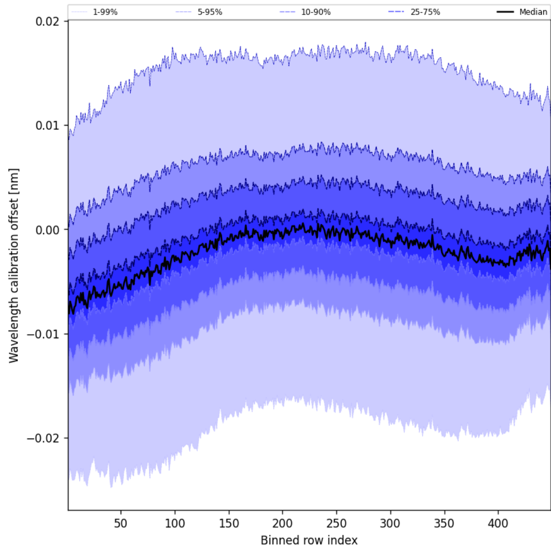
Figure 52: Along track statistics of “Wavelength calibration offset” for 2025-01-10 to 2025-01-12
