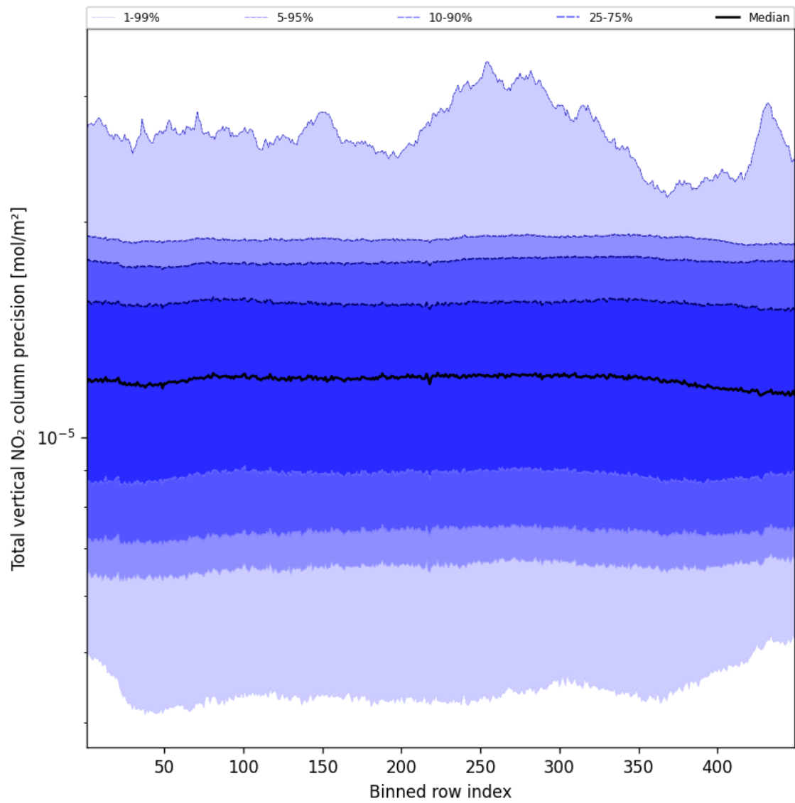
Figure 56: Along track statistics of “Total vertical NO 2 column precision” for 2025-01-10 to 2025-01-12
