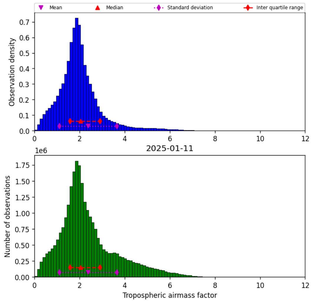
Figure 31: Histogram of “Tropospheric airmass factor” for 2025-01-10 to 2025-01-12
