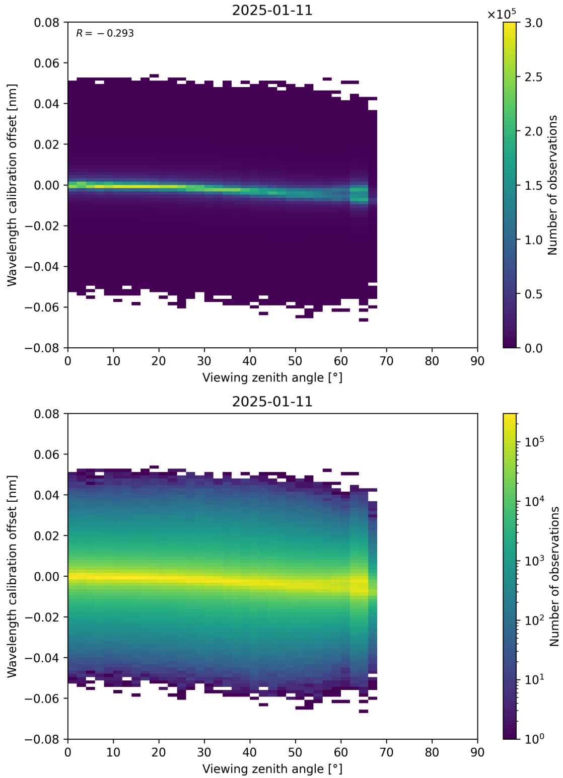
Figure 173: Scatter density plot of “Viewing zenith angle” against “Wavelength calibration offset” for 2025-01-10 to 2025-01-12.
