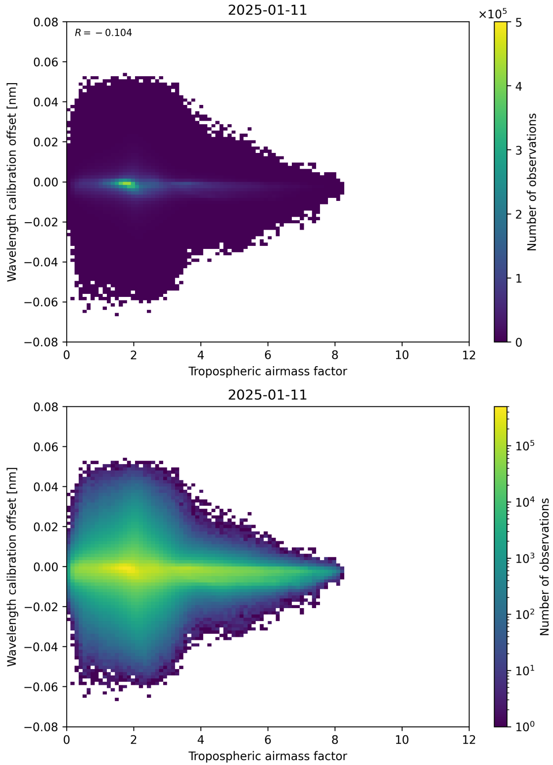
Figure 80: Scatter density plot of “Tropospheric airmass factor” against “Wavelength calibration offset” for 2025-01-10 to 2025-01-12.
