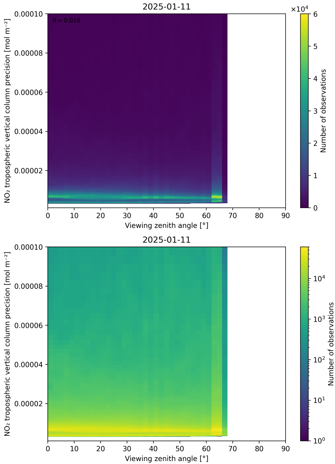
Figure 170: Scatter density plot of “Viewing zenith angle” against “NO 2 tropospheric vertical column precision” for 2025-01-10 to 2025-01-12.
