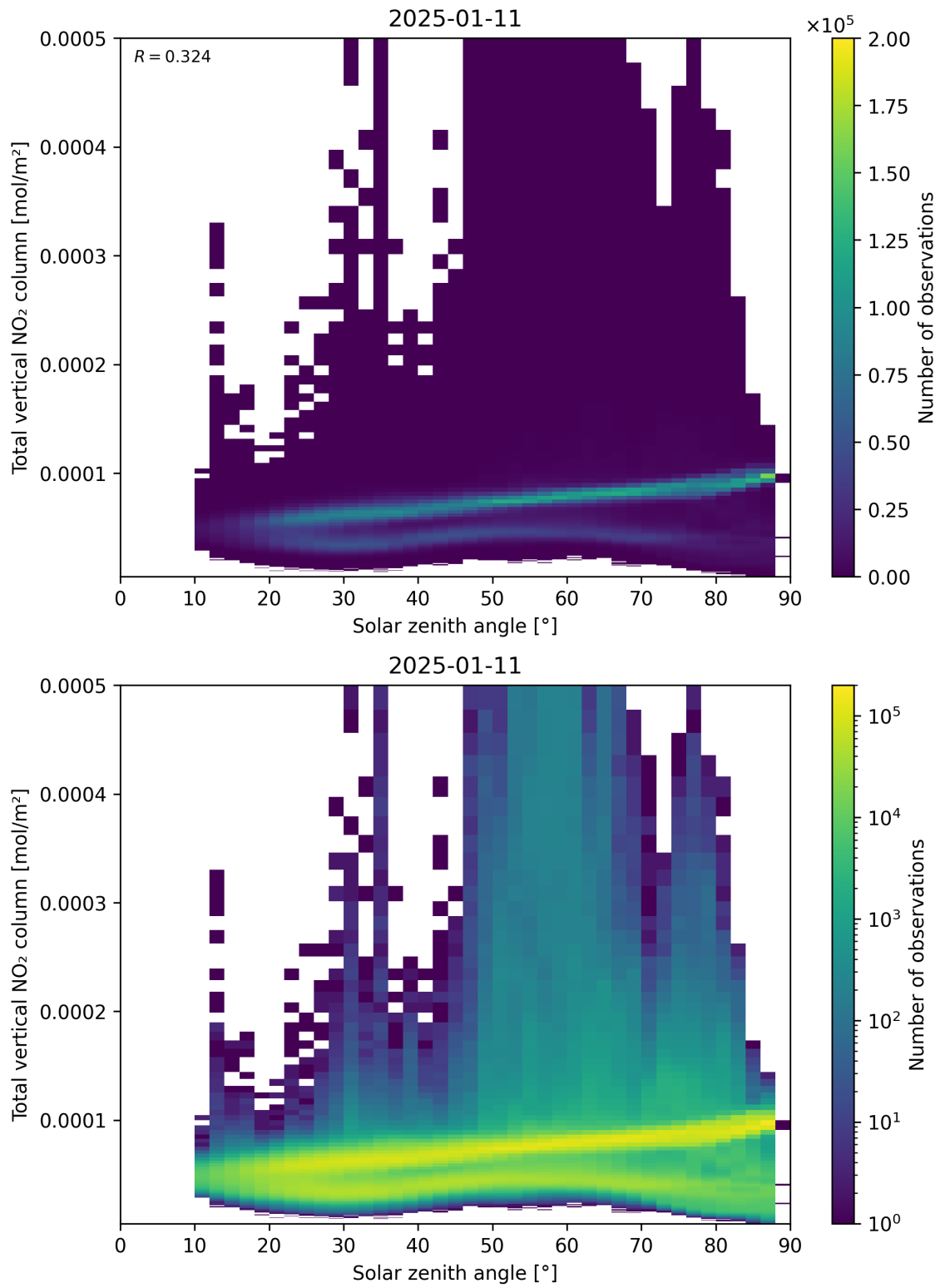
Figure 153: Scatter density plot of “Solar zenith angle” against “Total vertical NO 2 column” for 2025-01-10 to 2025-01-12.
