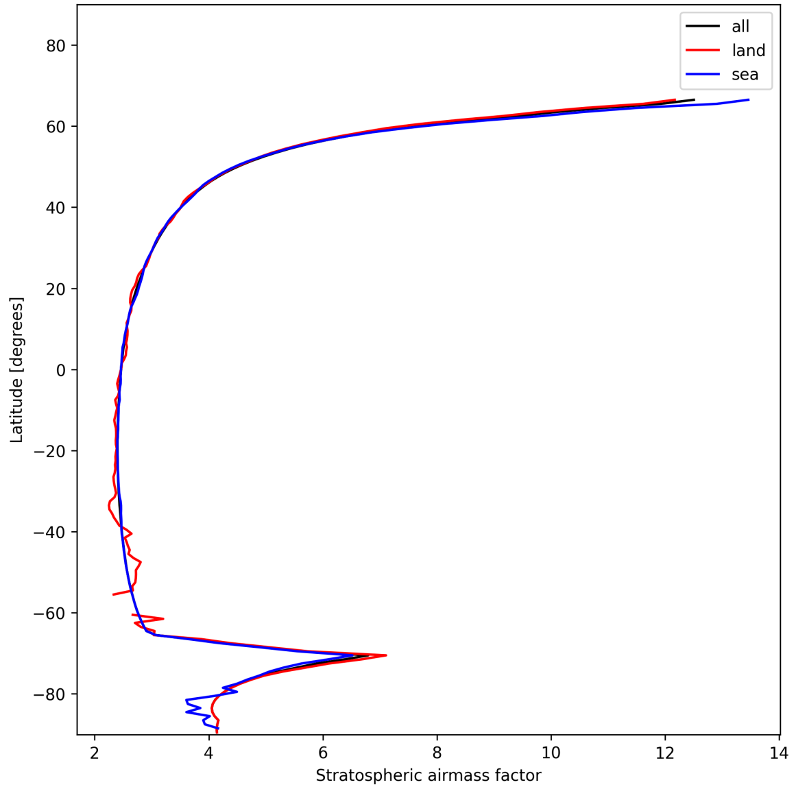
Figure 27: Zonal average of “Stratospheric airmass factor” for 2025-01-10 to 2025-01-12.
