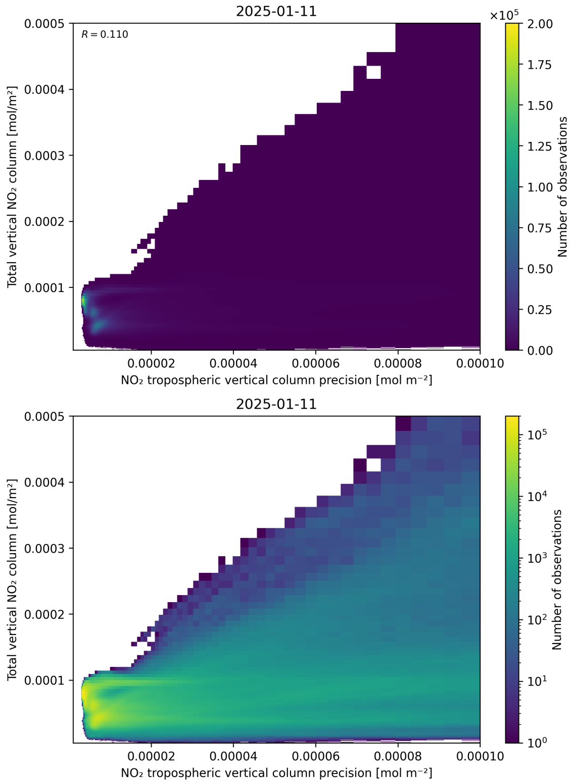
Figure 138: Scatter density plot of “NO 2 tropospheric vertical column precision” against “Total vertical NO 2 column” for 2025-01-10 to 2025-01-12.
