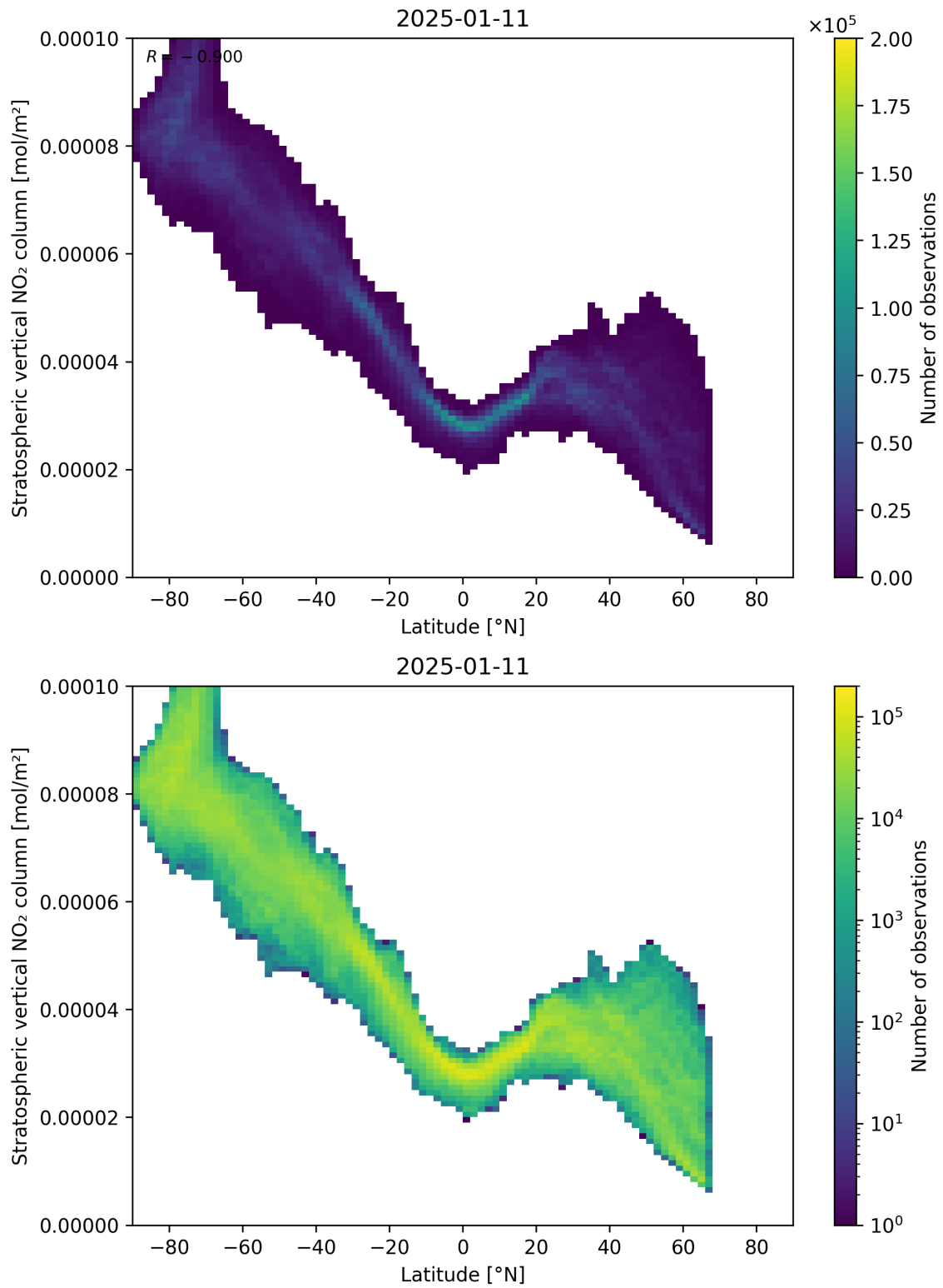
Figure 87: Scatter density plot of “Latitude” against “Stratospheric vertical NO 2 column” for 2025-01-10 to 2025-01-12.
