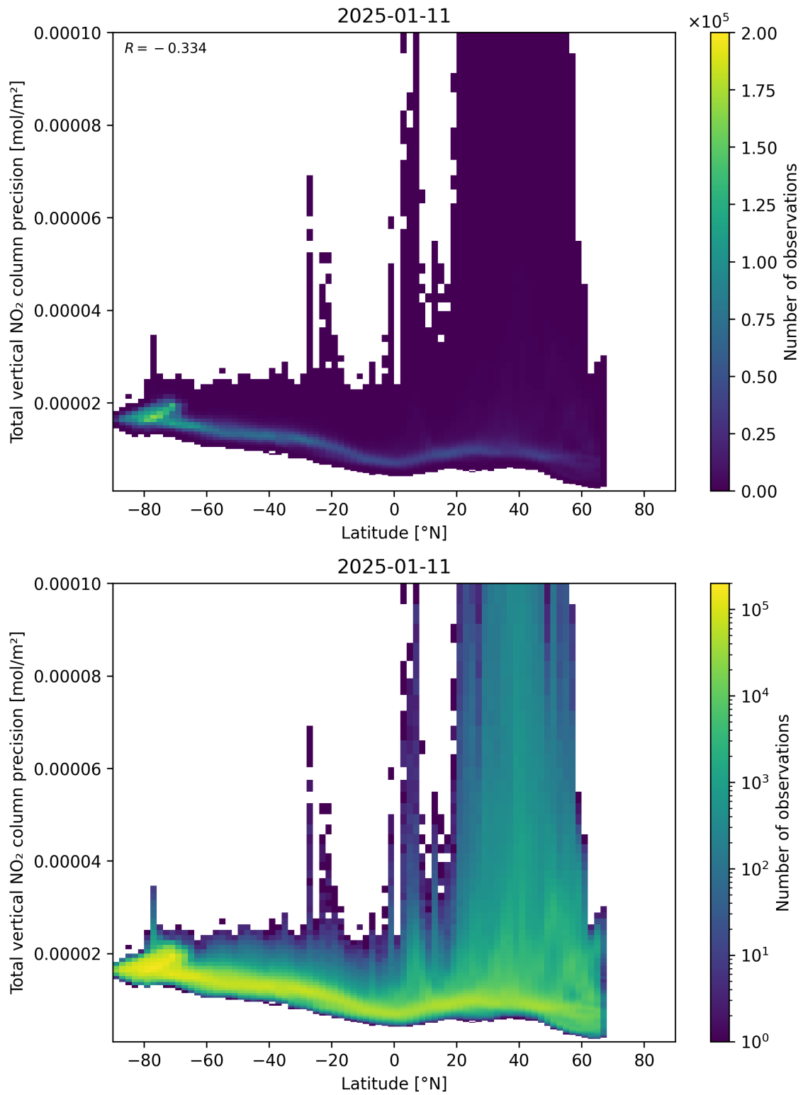
Figure 91: Scatter density plot of “Latitude” against “Total vertical NO 2 column precision” for 2025-01-10 to 2025-01-12.
