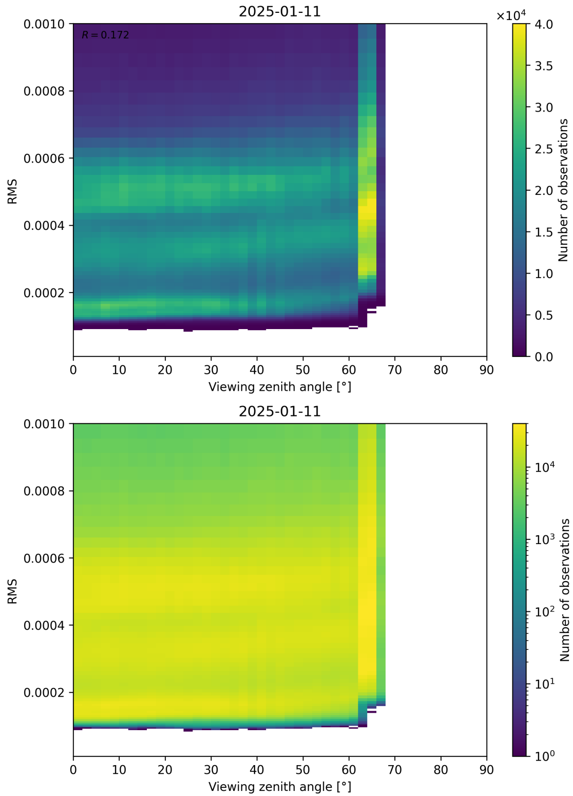
Figure 171: Scatter density plot of “Viewing zenith angle” against “RMS” for 2025-01-10 to 2025-01-12.
