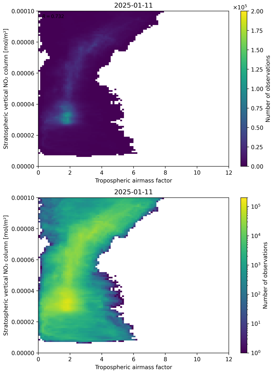
Figure 74: Scatter density plot of “Tropospheric airmass factor” against “Stratospheric vertical NO 2 column” for 2025-01-10 to 2025-01-12.
