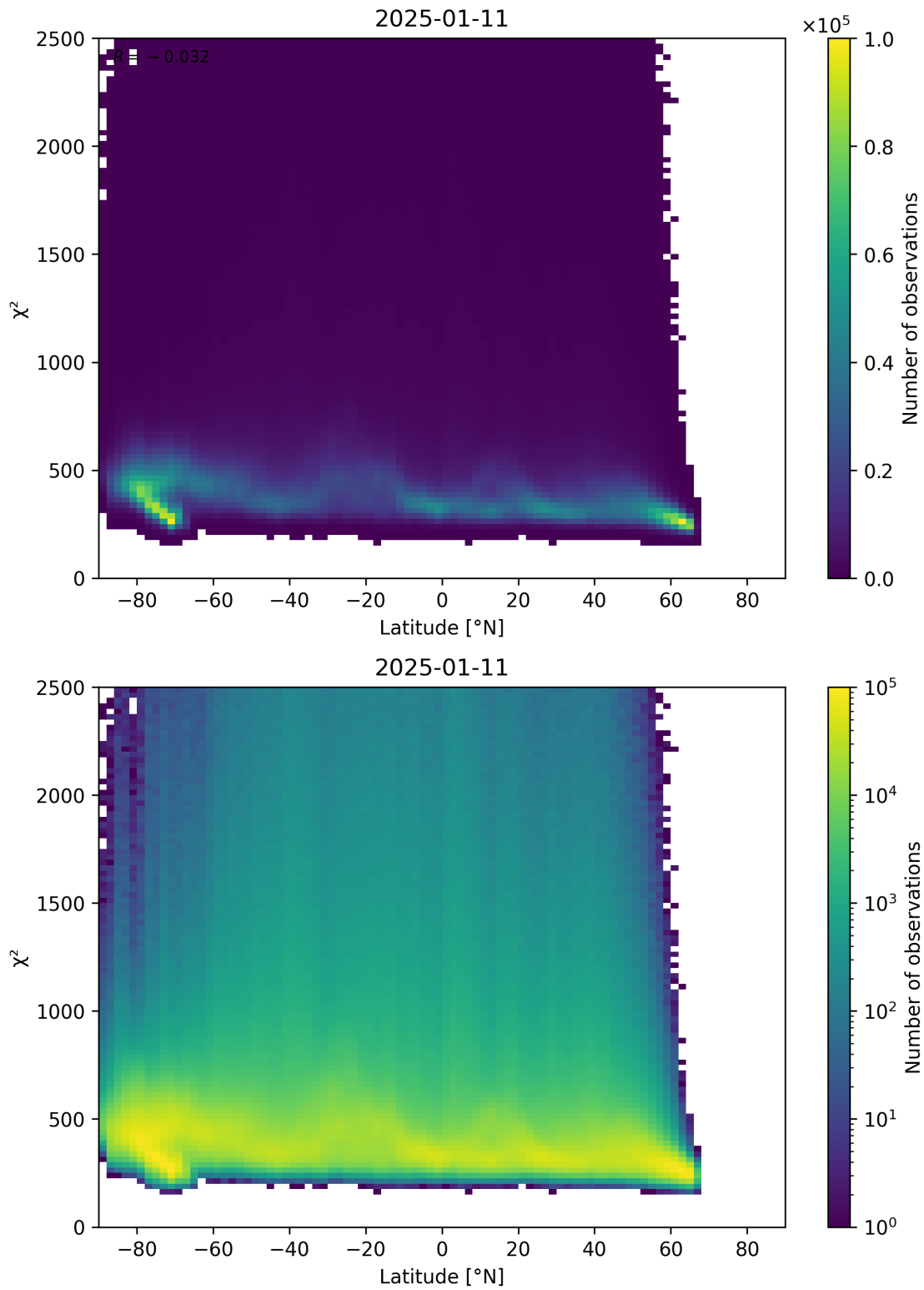
Figure 86: Scatter density plot of “Latitude” against “ \chi^2 ” for 2025-01-10 to 2025-01-12.
