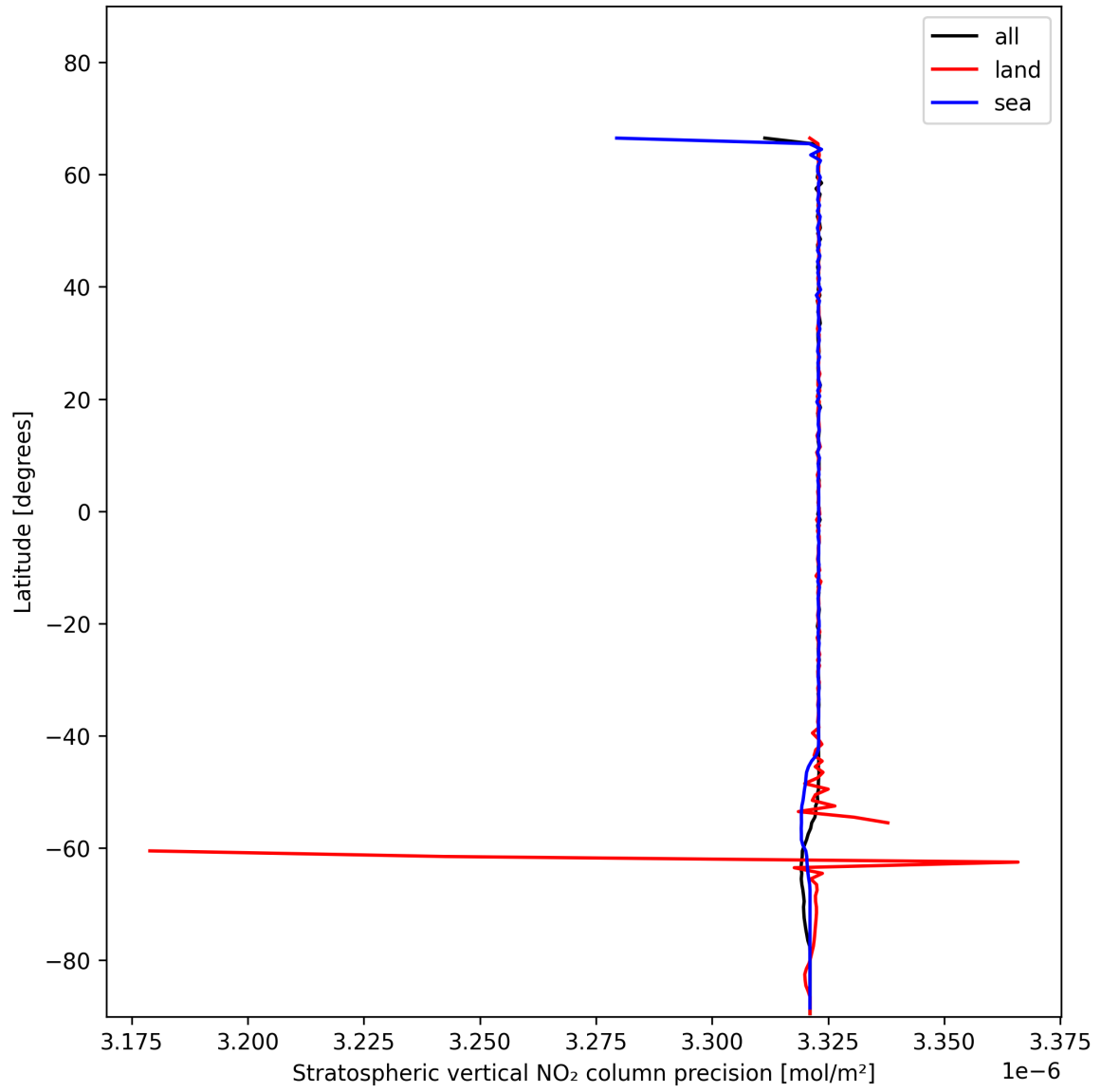
Figure 20: Zonal average of "Stratospheric vertical NO 2 column precision" for 2025-01-10 to 2025-01-12.
