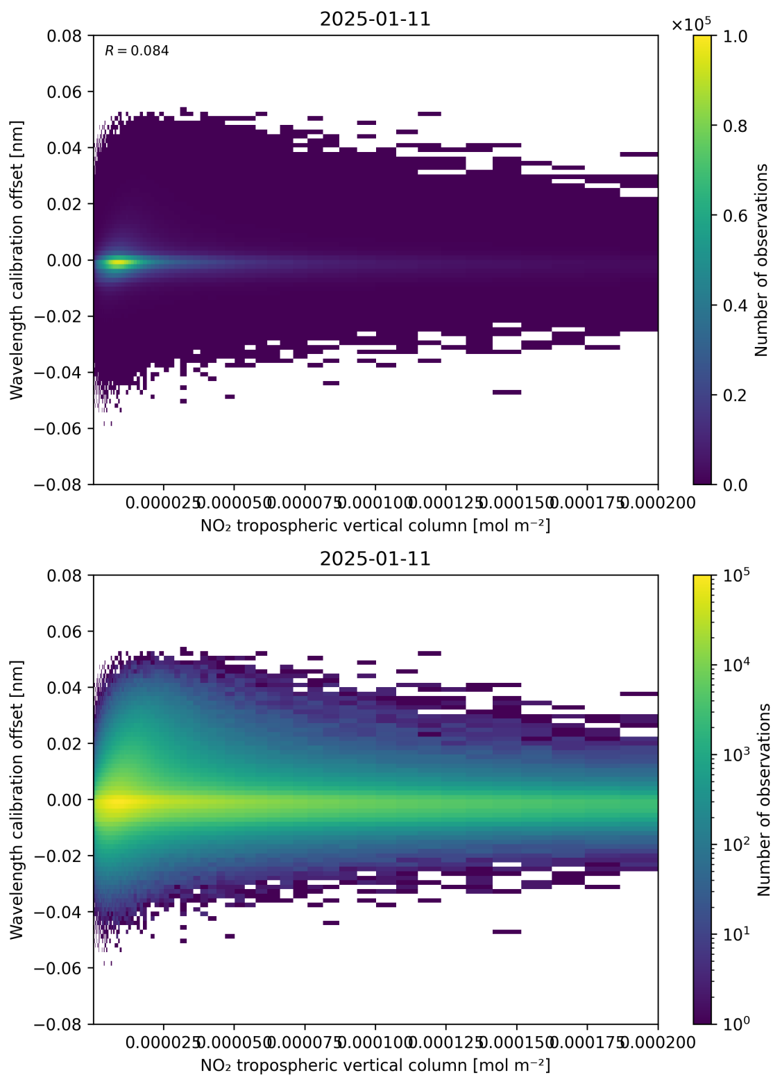
Figure 143: Scatter density plot of “NO 2 tropospheric vertical column” against “Wavelength calibration offset” for 2025-01-10 to 2025-01-12.
