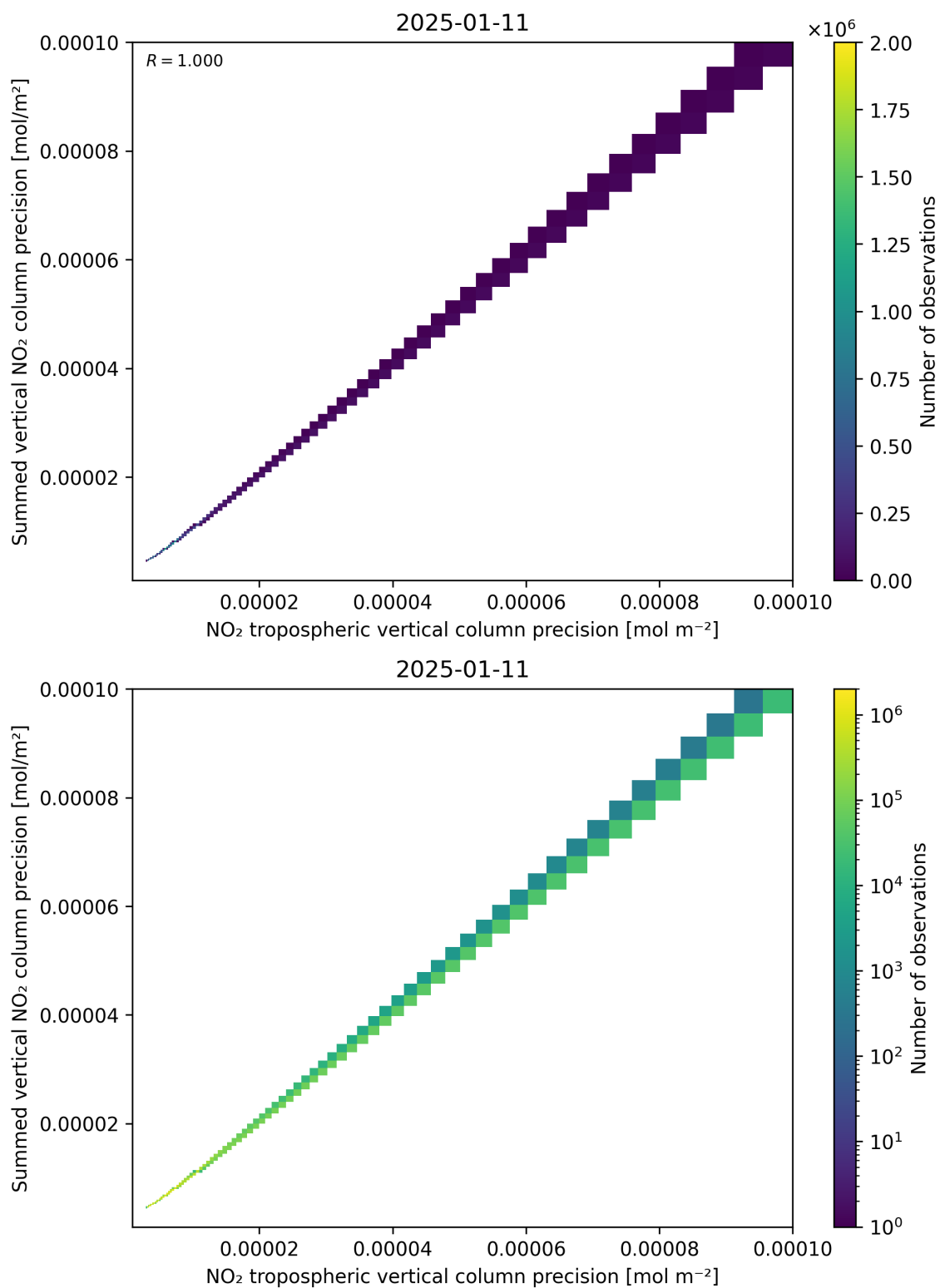
Figure 137: Scatter density plot of “NO 2 tropospheric vertical column precision” against “Summed vertical NO 2 column precision” for 2025-01-10 to 2025-01-12.
