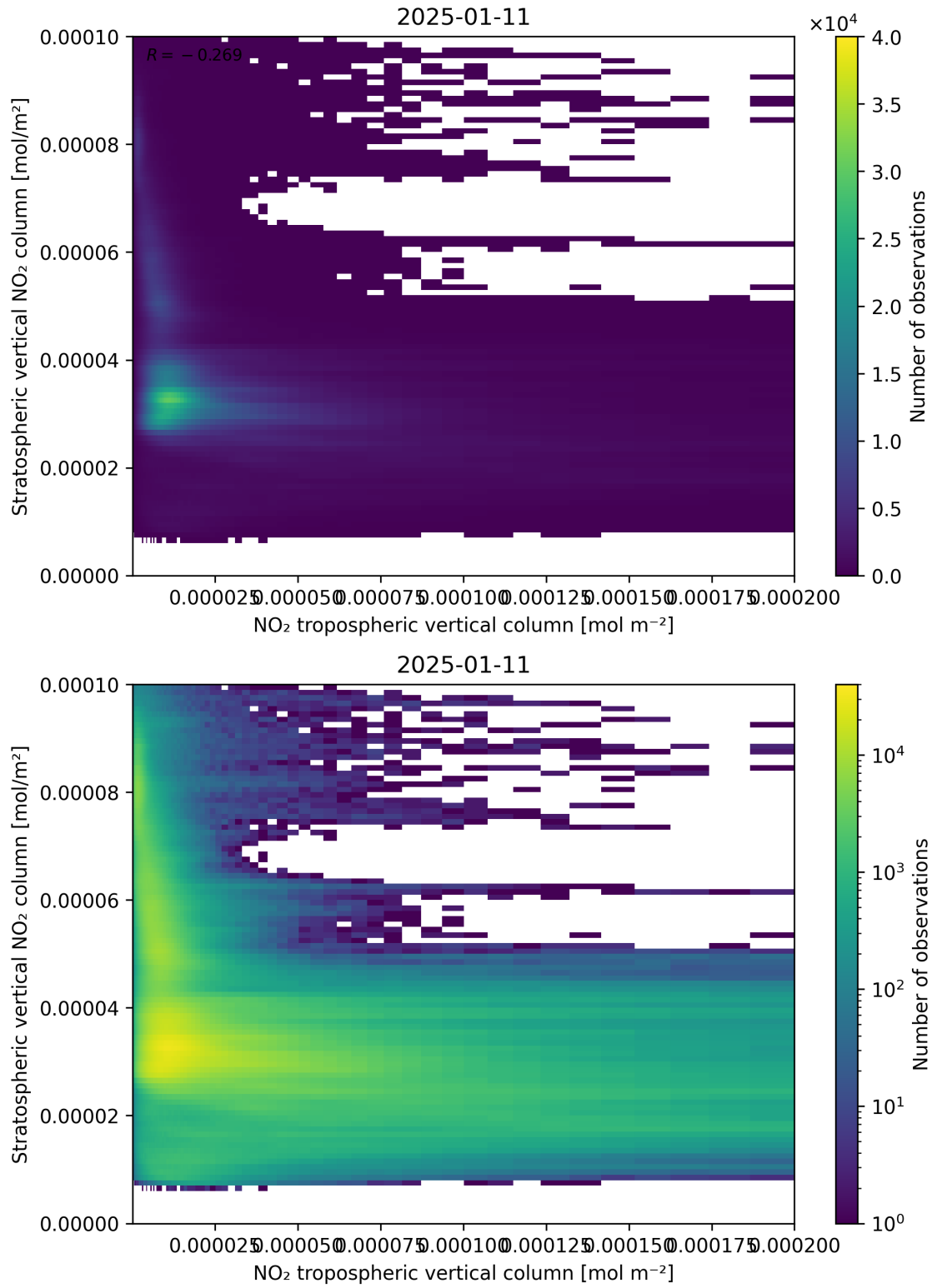
Figure 125: Scatter density plot of “NO 2 tropospheric vertical column” against “Stratospheric vertical NO 2 column” for 2025-01-10 to 2025-01-12.
