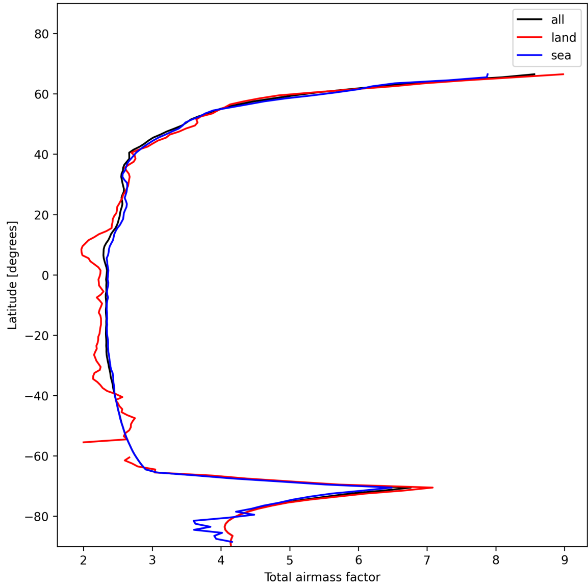
Figure 15: Zonal average of “Total airmass factor” for 2025-01-10 to 2025-01-12.
