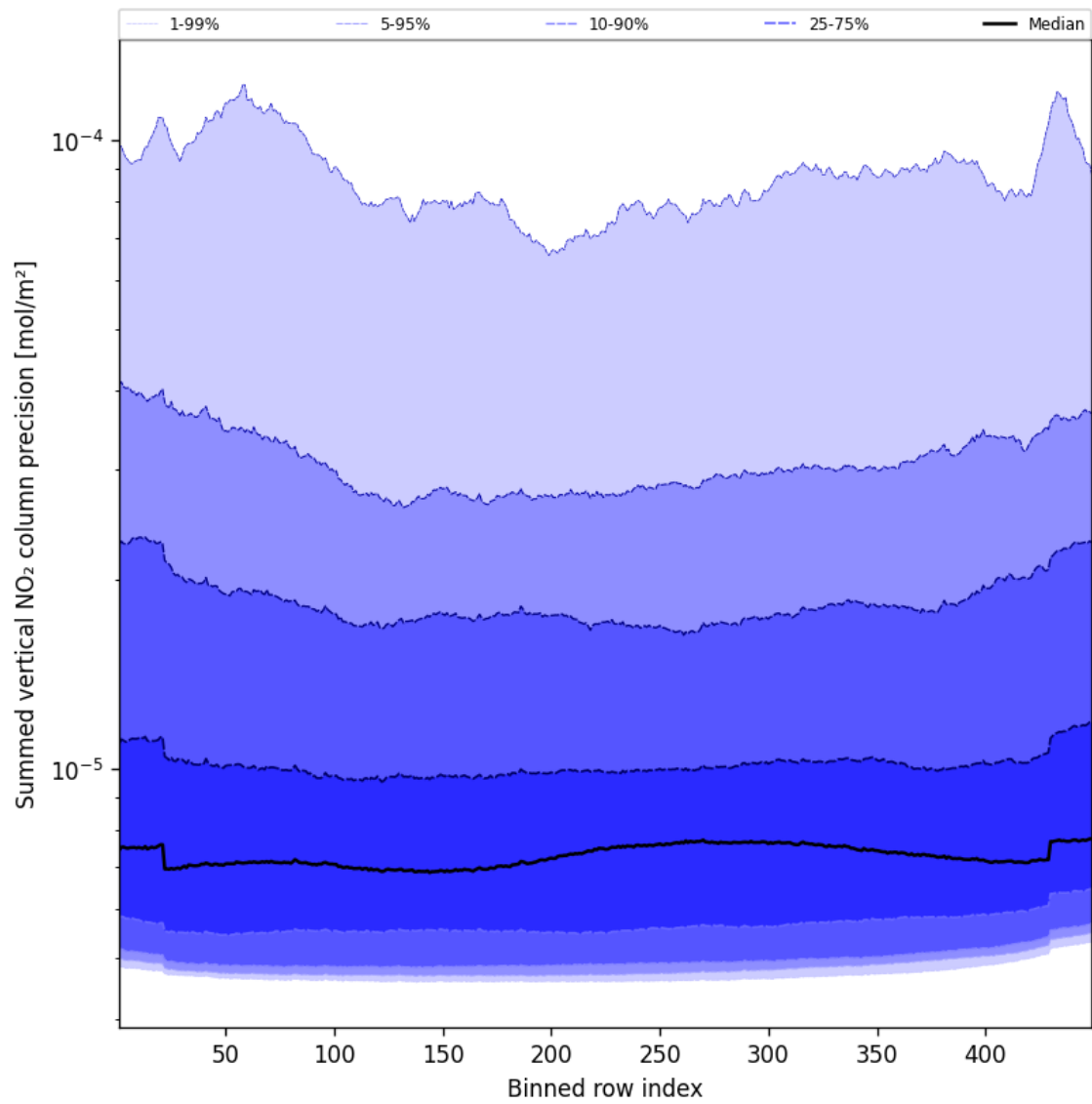
Figure 58: Along track statistics of “Summed vertical NO 2 column precision” for 2025-01-10 to 2025-01-12
