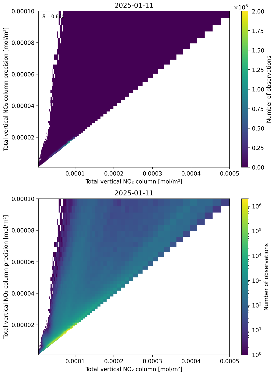
Figure 114: Scatter density plot of “Total vertical NO 2 column” against “Total vertical NO 2 column precision” for 2025-01-10 to 2025-01-12.
