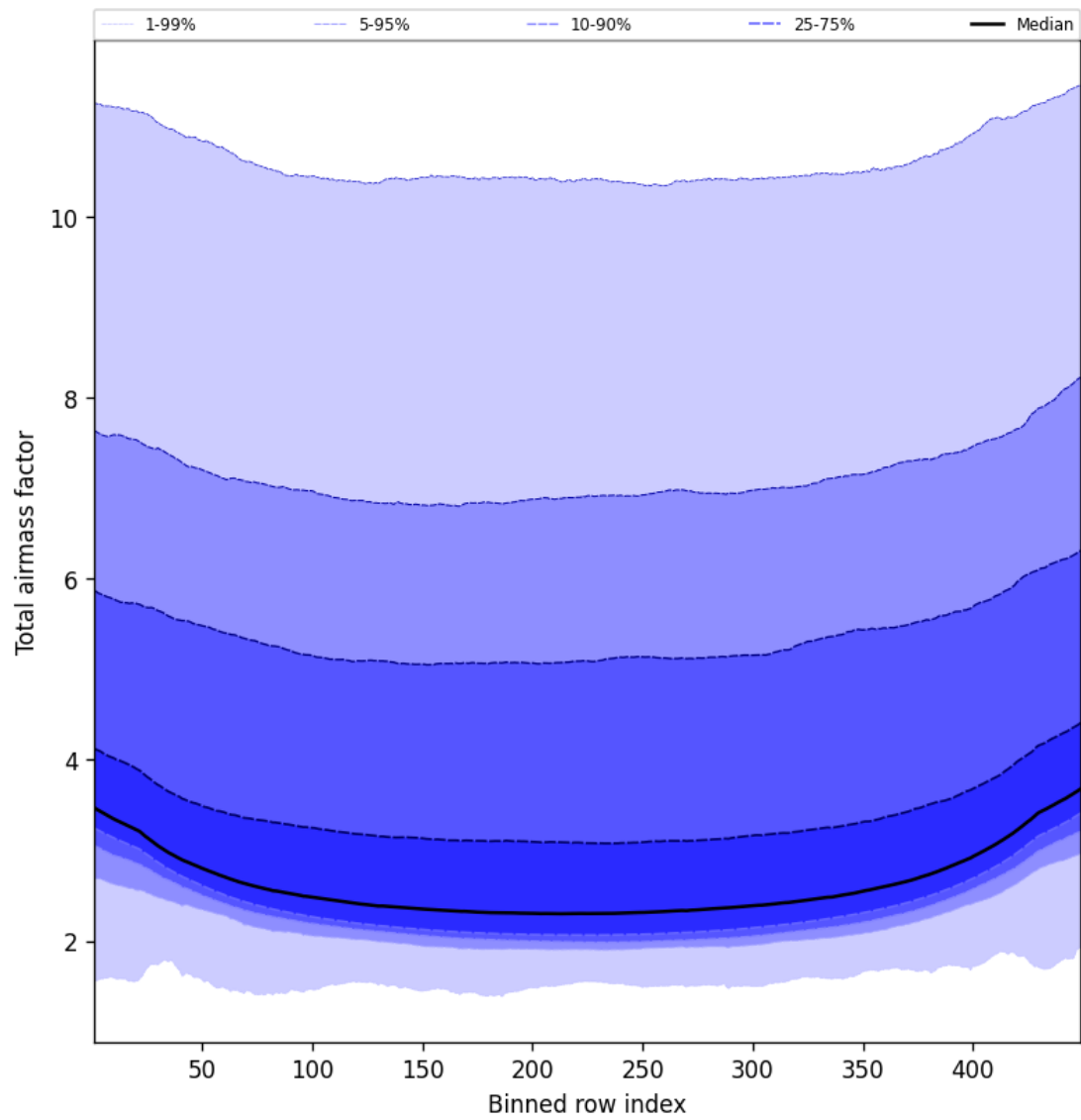
Figure 49: Along track statistics of “Total airmass factor” for 2025-01-10 to 2025-01-12
