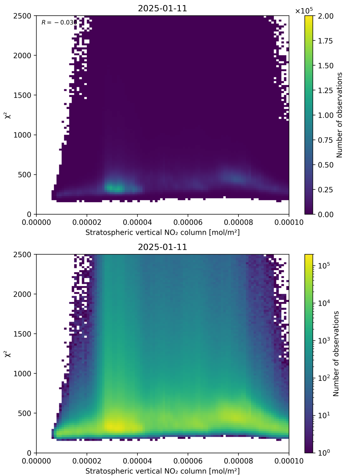
Figure 97: Scatter density plot of “Stratospheric vertical NO 2 column” against “ \chi^2 ” for 2025-01-10 to 2025-01-12.
