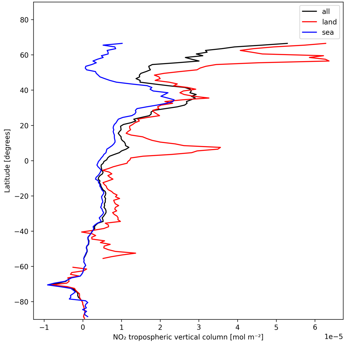
Figure 12: Zonal average of “NO 2 tropospheric vertical column” for 2025-01-10 to 2025-01-12.
