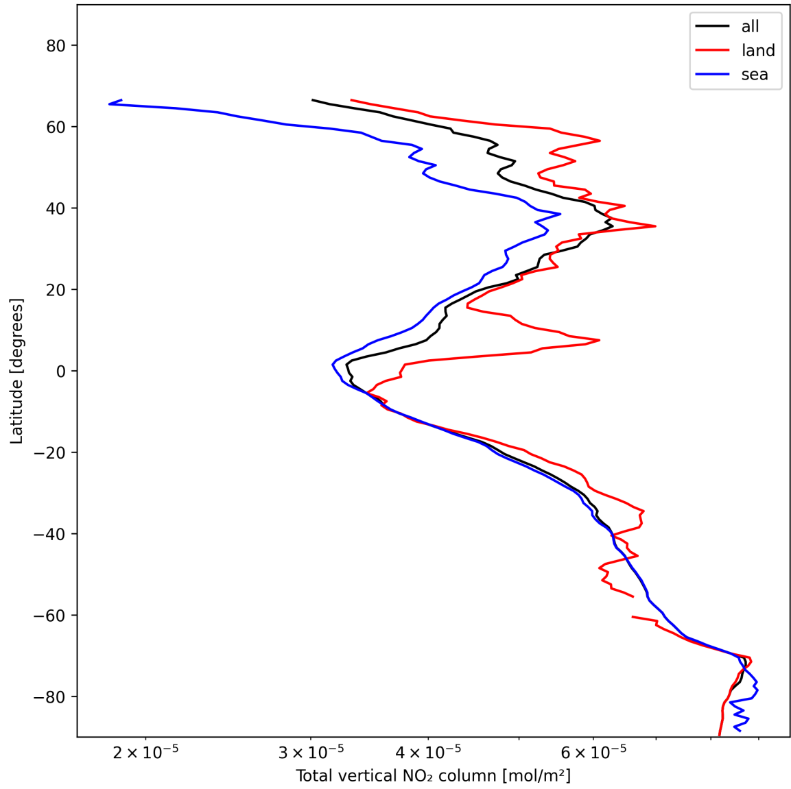
Figure 21: Zonal average of “Total vertical NO 2 column” for 2025-01-10 to 2025-01-12.
