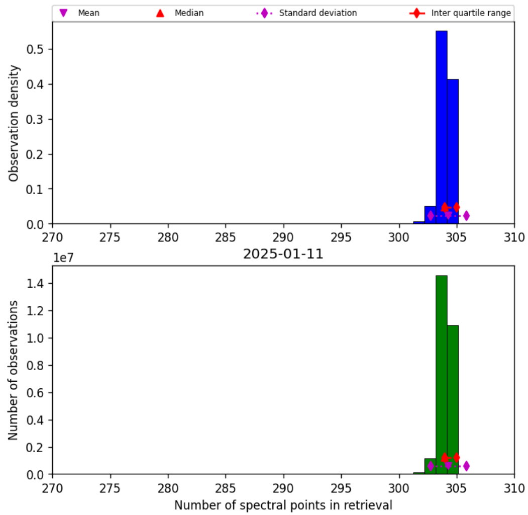
Figure 33: Histogram of “Number of spectral points in retrieval” for 2025-01-10 to 2025-01-12
