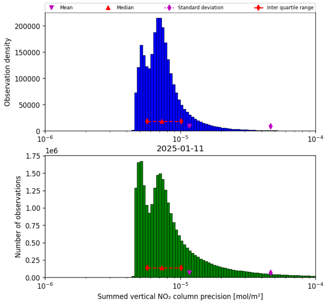
Figure 41: Histogram of “Summed vertical NO 2 column precision” for 2025-01-10 to 2025-01-12
