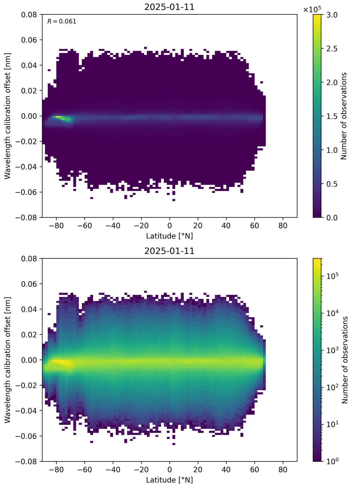
Figure 95: Scatter density plot of “Latitude” against “Wavelength calibration offset” for 2025-01-10 to 2025-01-12.
