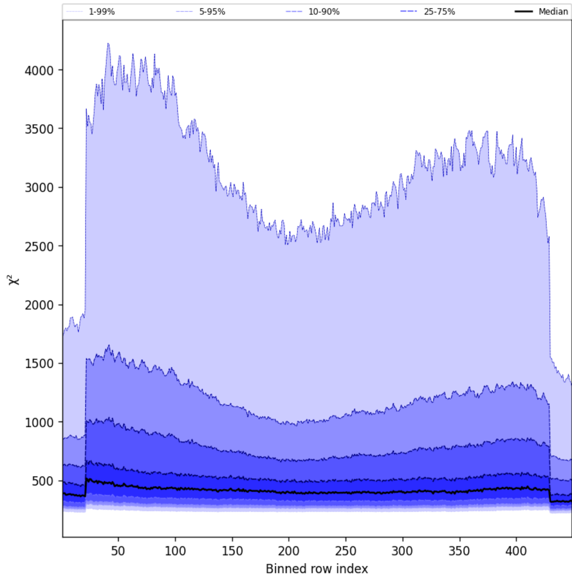
Figure 59: Along track statistics of “ \chi^2 ” for 2025-01-10 to 2025-01-12
