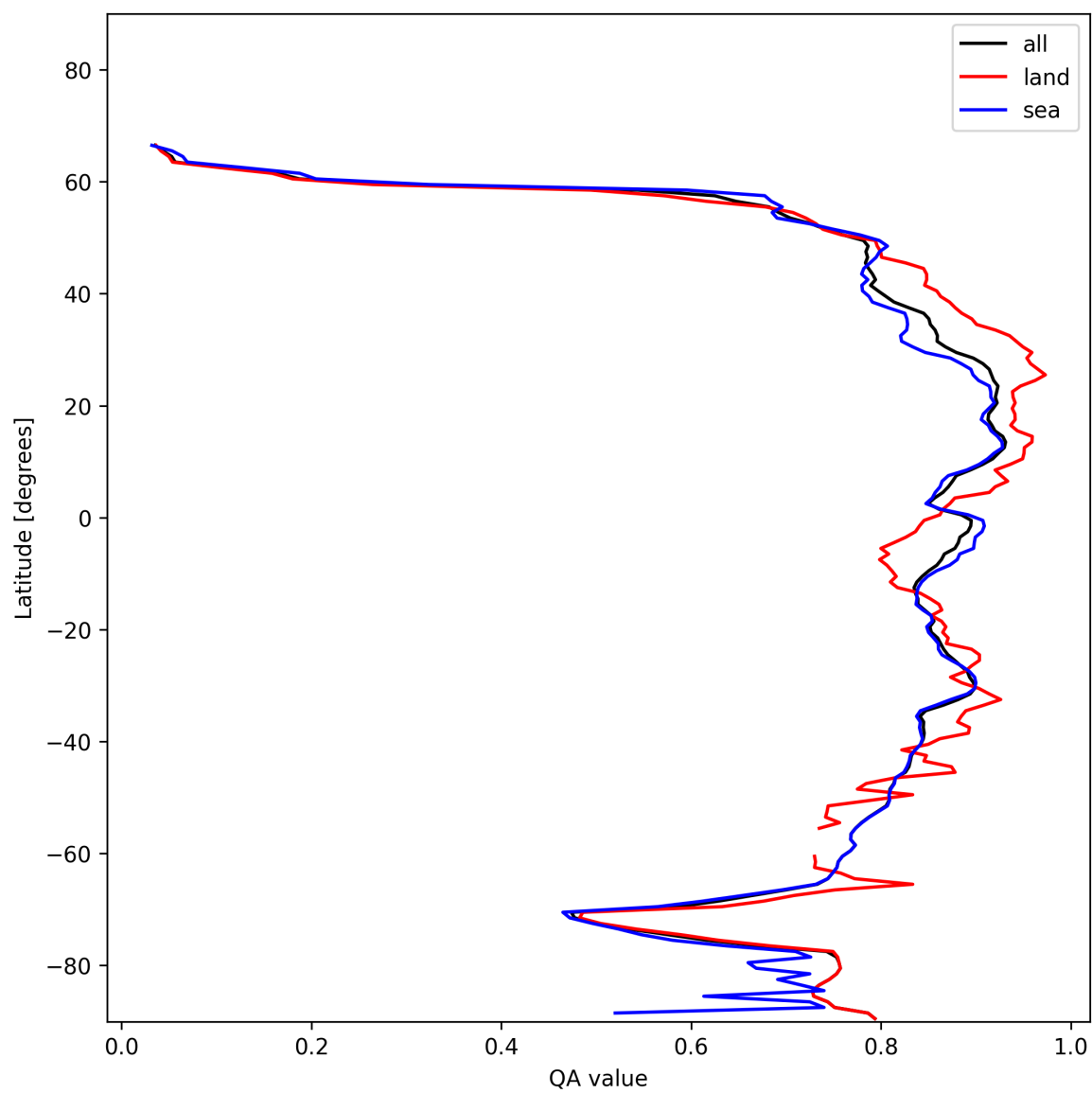
Figure 11: Zonal average of “QA value” for 2025-01-10 to 2025-01-12.
