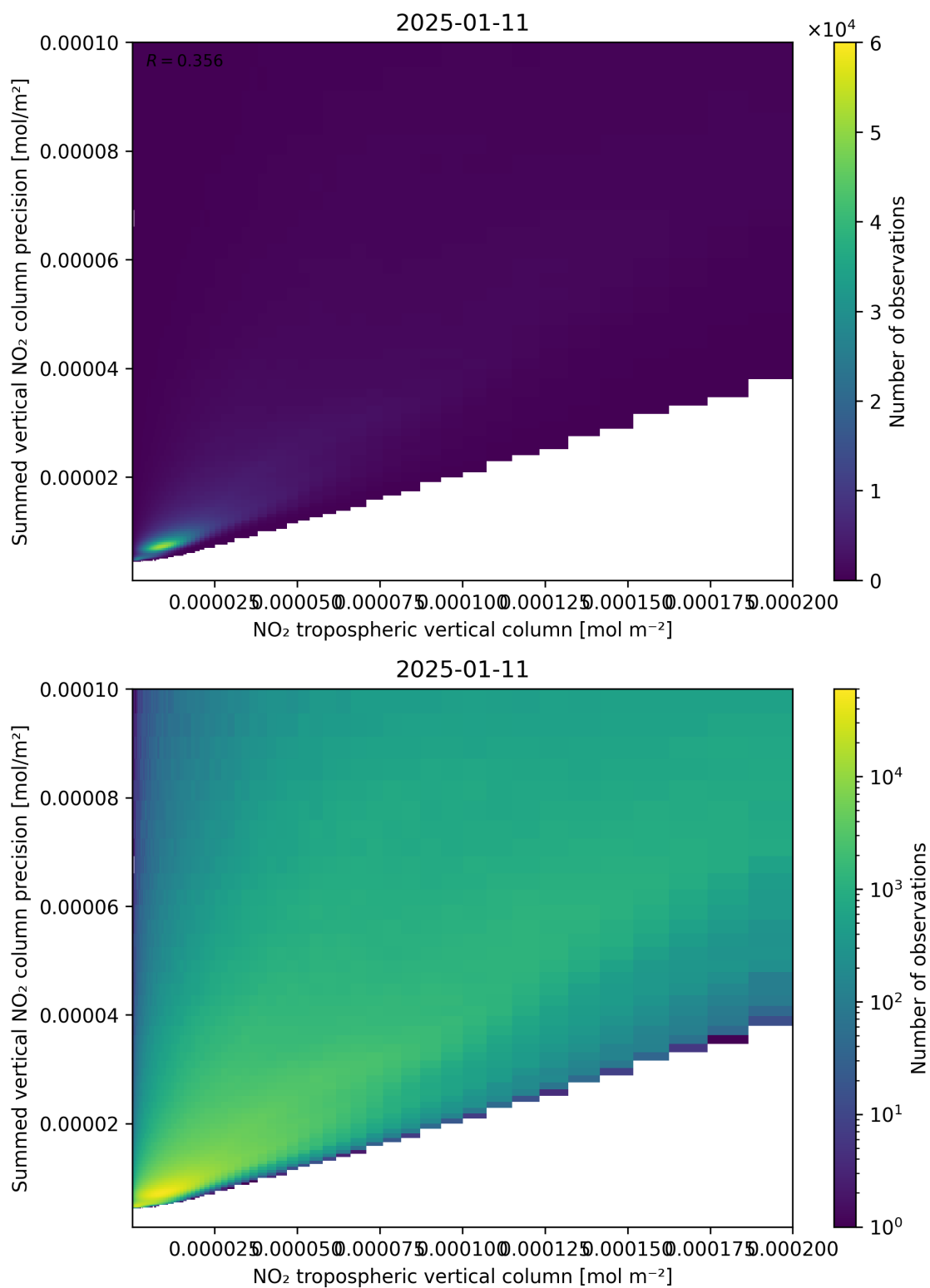
Figure 127: Scatter density plot of “NO 2 tropospheric vertical column” against “Summed vertical NO 2 column precision” for 2025-01-10 to 2025-01-12.
