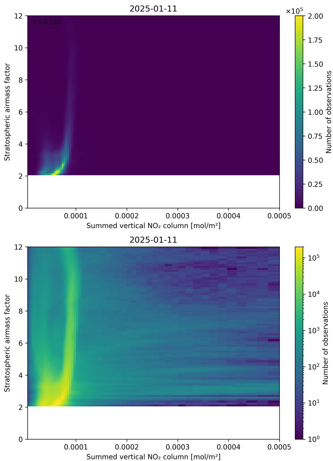
Figure 103: Scatter density plot of “Summed vertical NO 2 column” against “Stratospheric airmass factor” for 2025-01-10 to 2025-01-12.
