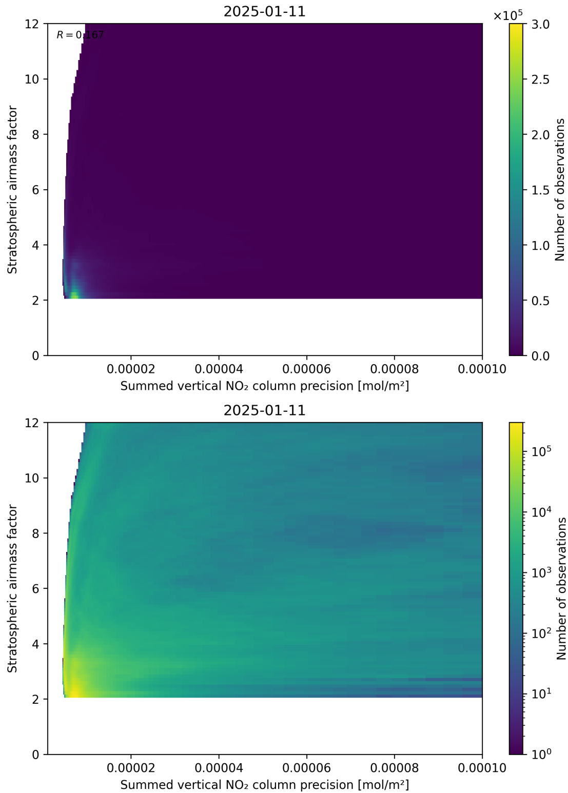
Figure 106: Scatter density plot of “Summed vertical NO 2 column precision” against “Stratospheric airmass factor” for 2025-01-10 to 2025-01-12.
