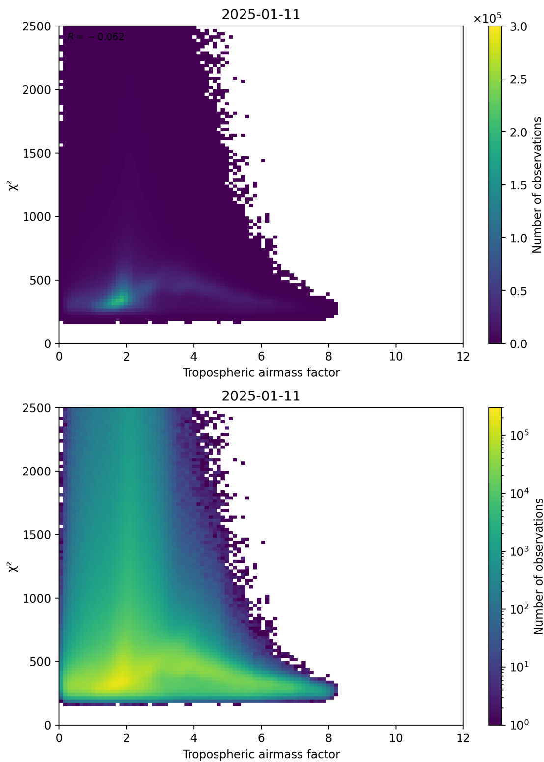
Figure 73: Scatter density plot of “Tropospheric airmass factor” against “ \chi^2 ” for 2025-01-10 to 2025-01-12.
