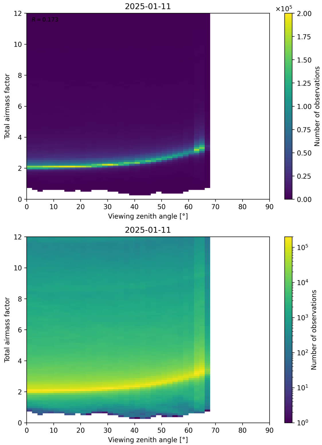
Figure 160: Scatter density plot of “Viewing zenith angle” against “Total airmass factor” for 2025-01-10 to 2025-01-12.
