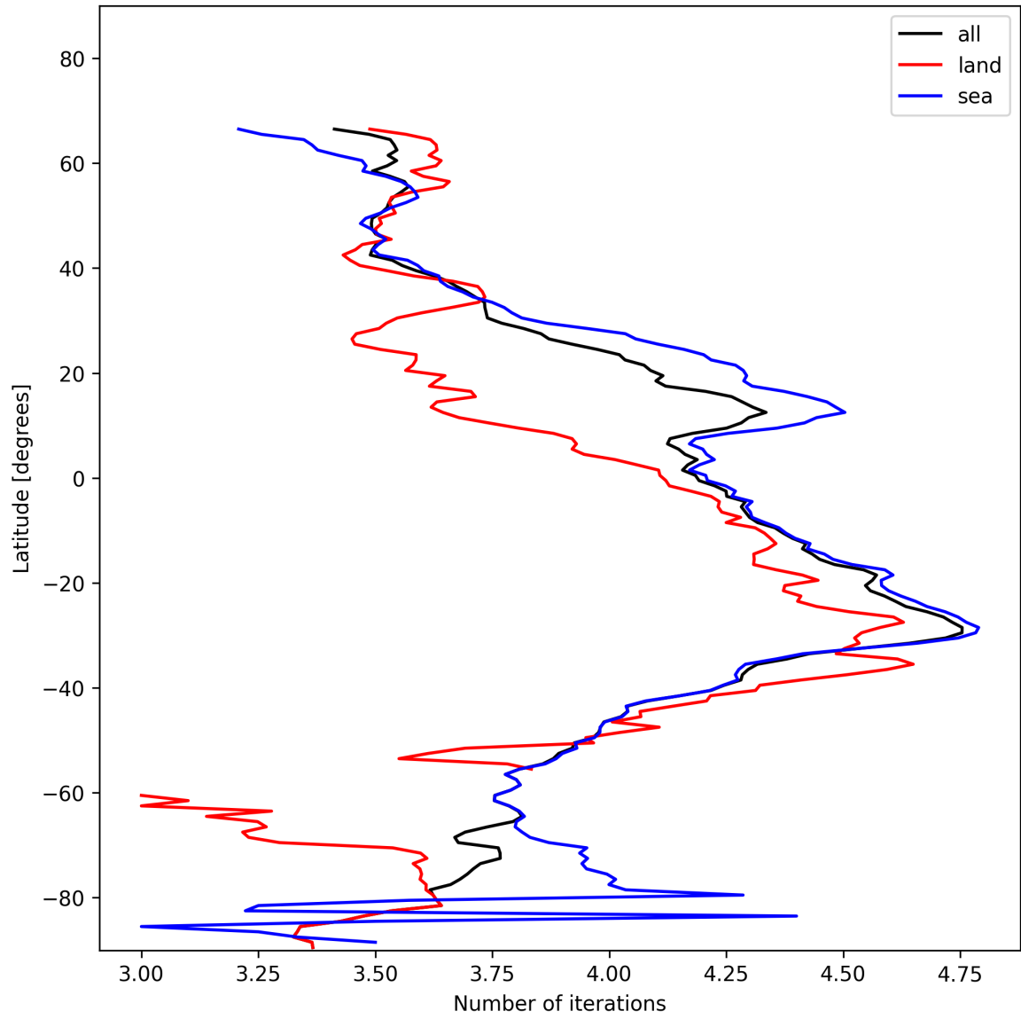
Figure 17: Zonal average of “Number of iterations” for 2025-01-10 to 2025-01-12.
