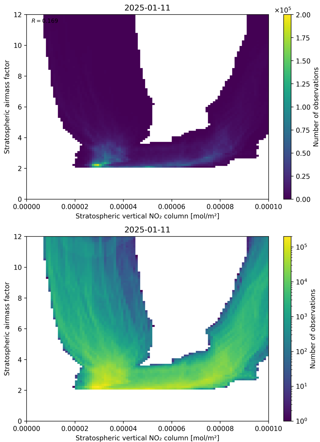
Figure 96: Scatter density plot of “Stratospheric vertical NO 2 column” against “Stratospheric airmass factor” for 2025-01-10 to 2025-01-12.
