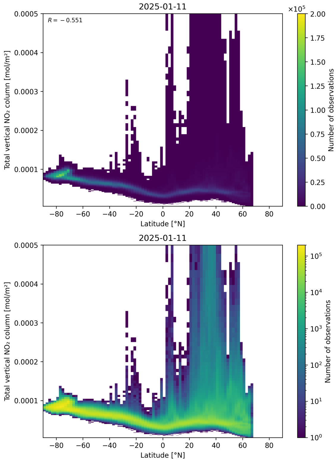
Figure 90: Scatter density plot of “Latitude” against “Total vertical NO 2 column” for 2025-01-10 to 2025-01-12.
