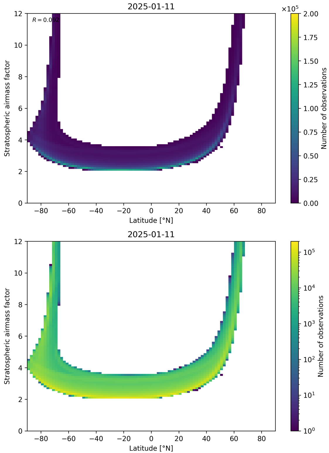
Figure 83: Scatter density plot of “Latitude” against “Stratospheric air mass factor” for 2025-01-10 to 2025-01-12.
