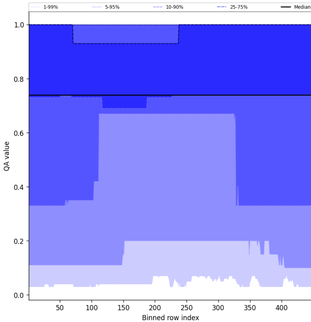
Figure 45: Along track statistics of “QA value” for 2025-01-10 to 2025-01-12
