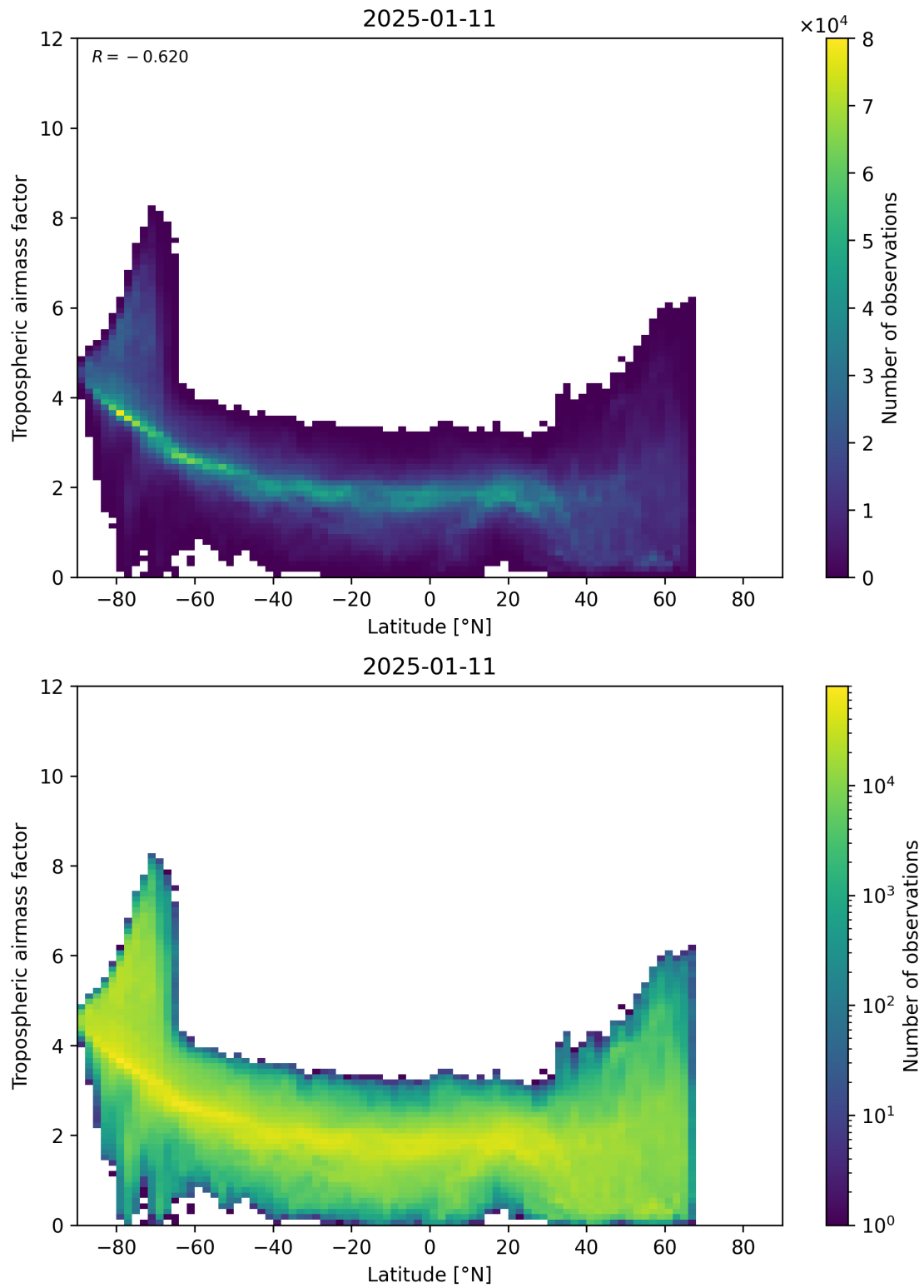
Figure 85: Scatter density plot of “Latitude” against “Tropospheric airmass factor” for 2025-01-10 to 2025-01-12.
