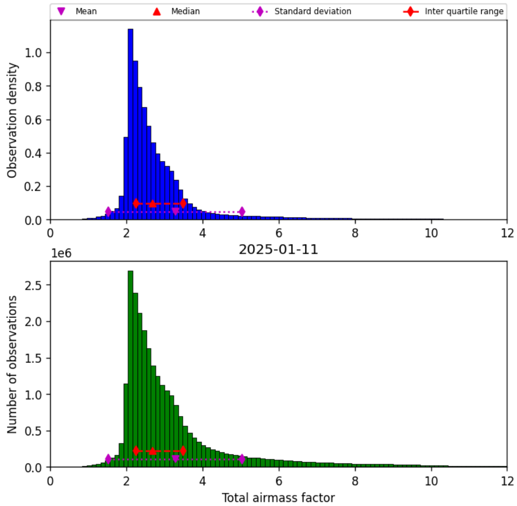
Figure 32: Histogram of “Total airmass factor” for 2025-01-10 to 2025-01-12
