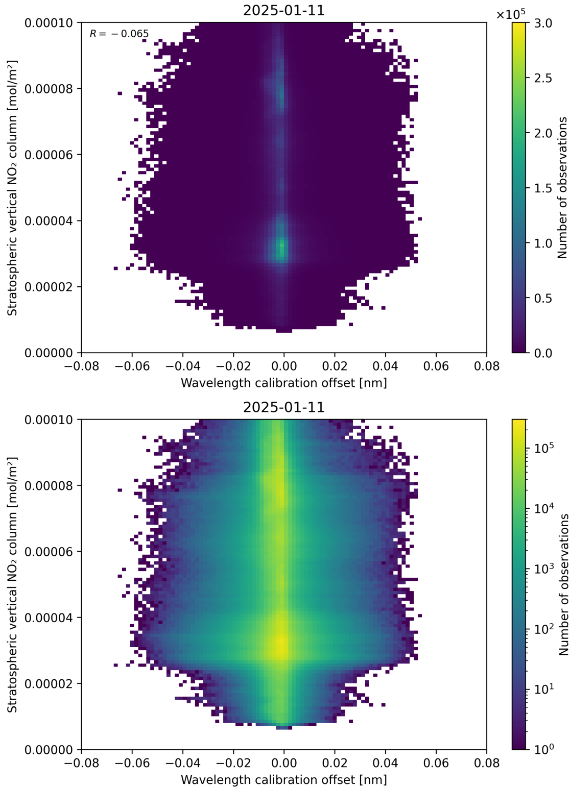
Figure 176: Scatter density plot of “Wavelength calibration offset” against “Stratospheric vertical NO 2 column” for 2025-01-10 to 2025-01-12.
