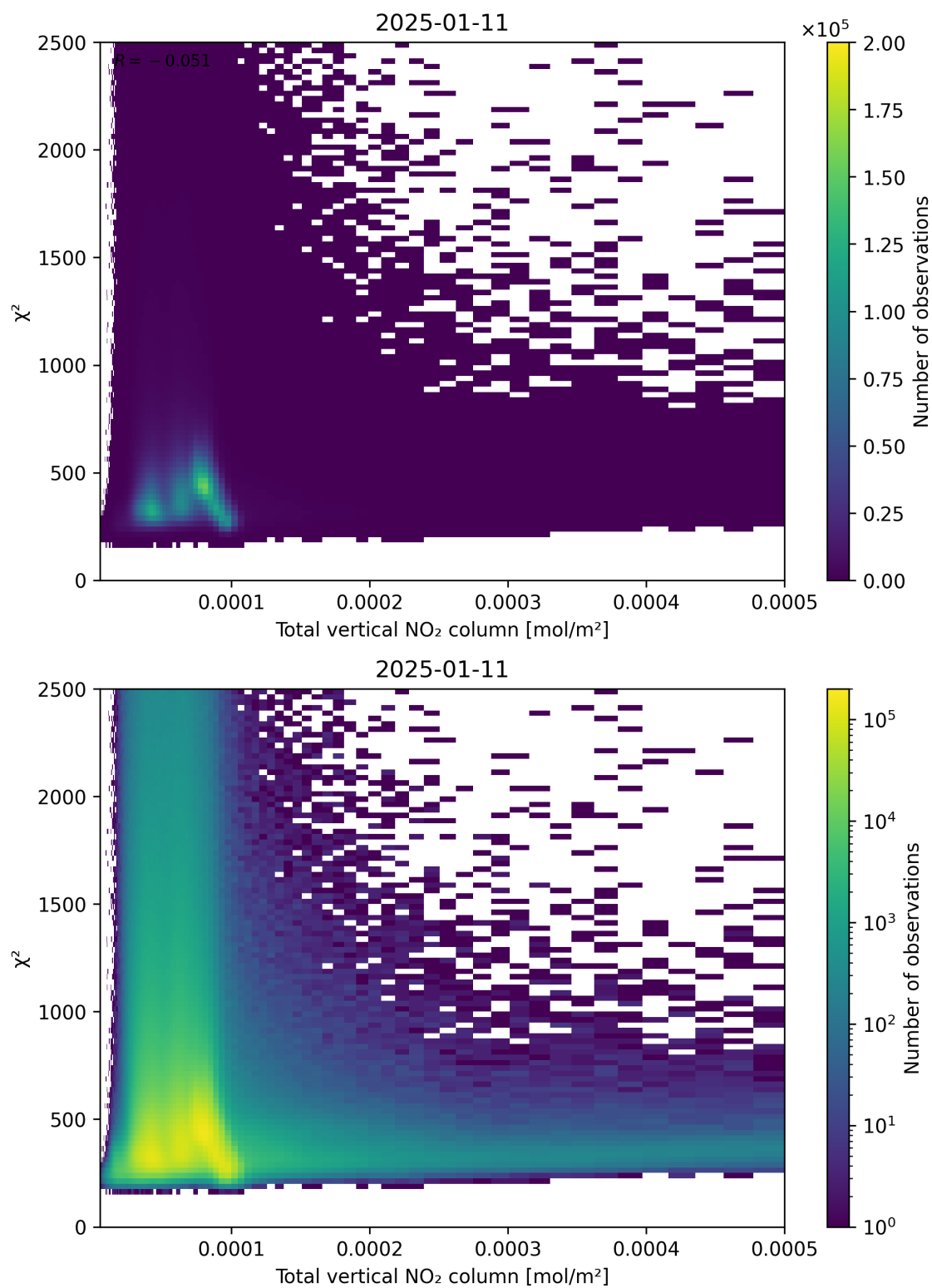
Figure 111: Scatter density plot of “Total vertical NO 2 column” against “ \chi^2 ” for 2025-01-10 to 2025-01-12.
