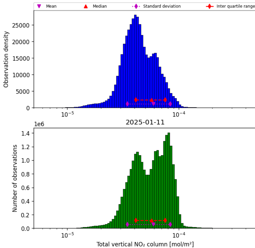
Figure 38: Histogram of “Total vertical NO 2 column” for 2025-01-10 to 2025-01-12
