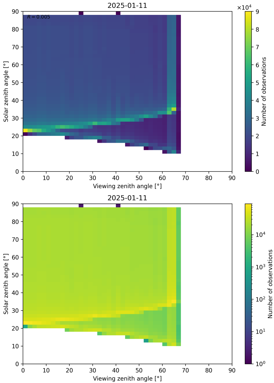
Figure 172: Scatter density plot of “Viewing zenith angle” against “Solar zenith angle” for 2025-01-10 to 2025-01-12.
