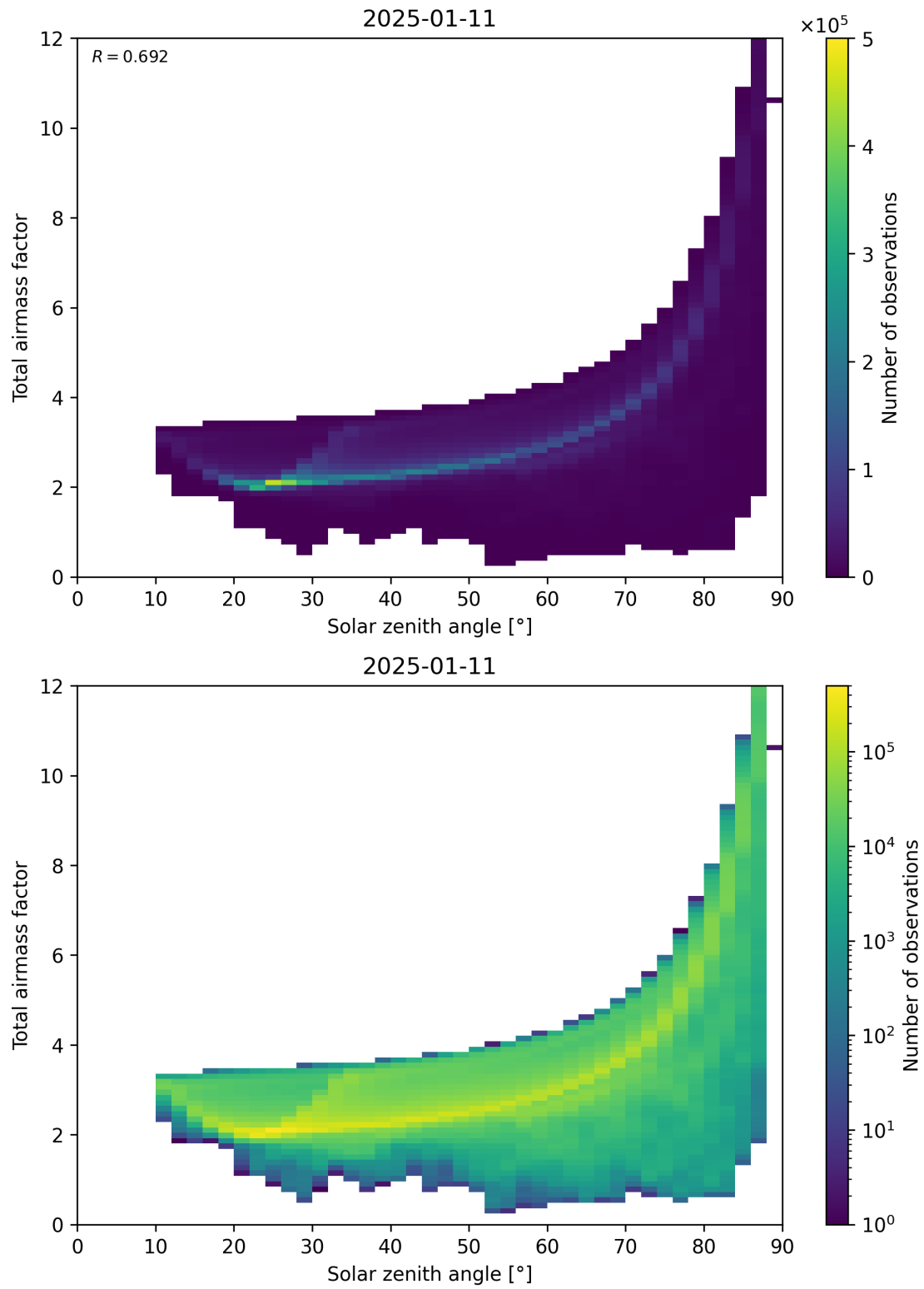
Figure 146: Scatter density plot of “Solar zenith angle” against “Total air mass factor” for 2025-01-10 to 2025-01-12.
