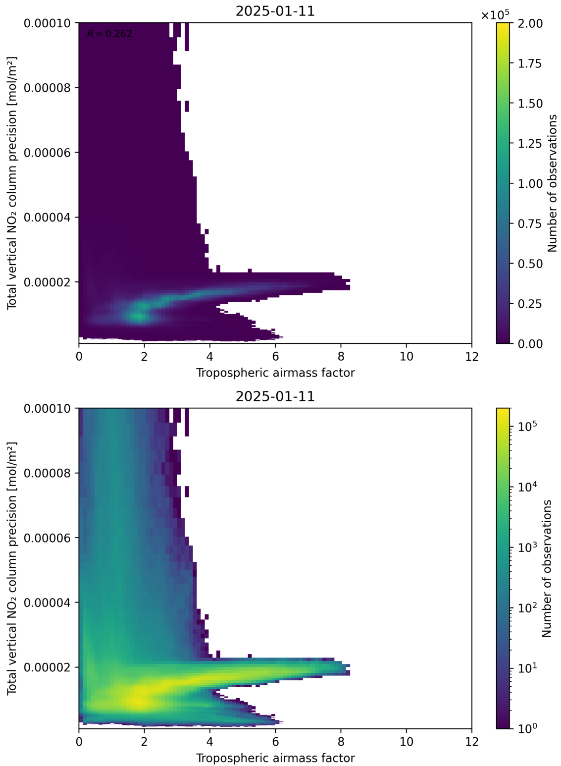
Figure 78: Scatter density plot of “Tropospheric air mass factor” against “Total vertical NO 2 column precision” for 2025-01-10 to 2025-01-12.
