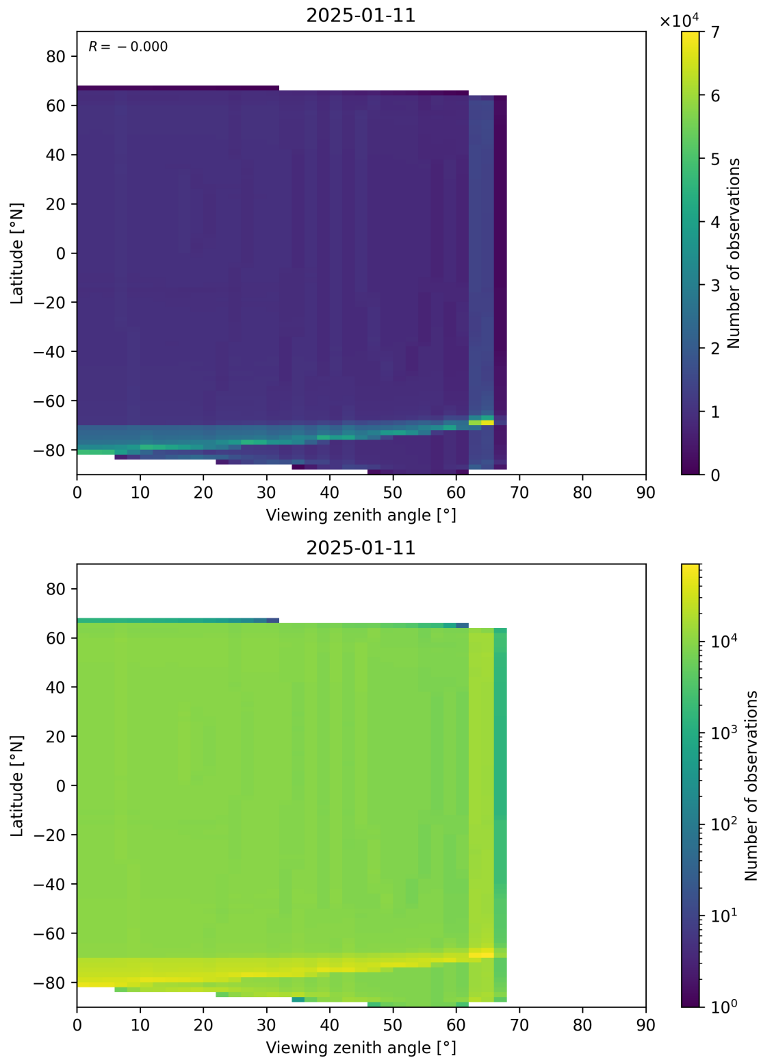
Figure 163: Scatter density plot of “Viewing zenith angle” against “Latitude” for 2025-01-10 to 2025-01-12.
