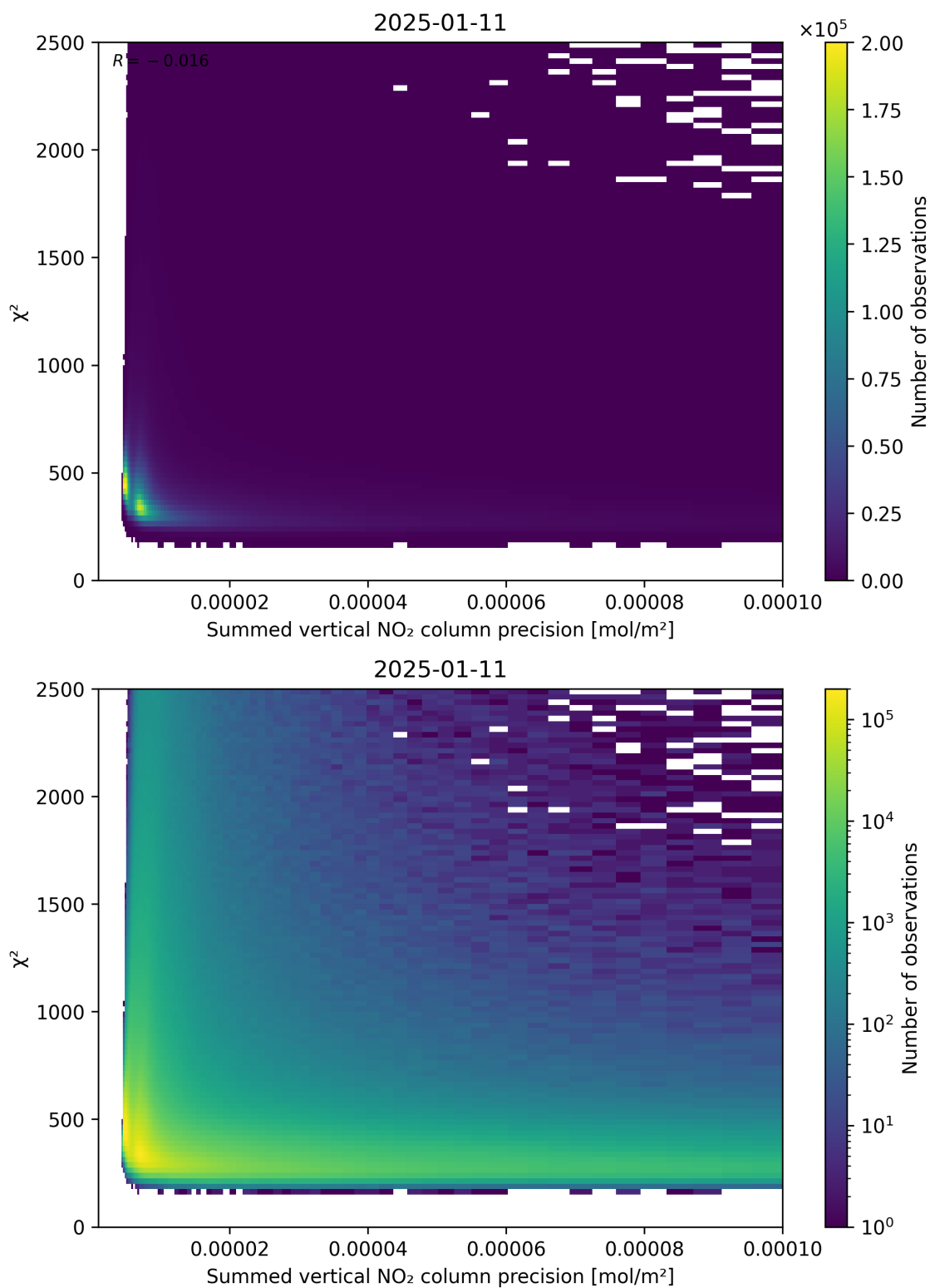
Figure 107: Scatter density plot of “Summed vertical NO 2 column precision” against “ \chi^2 ” for 2025-01-10 to 2025-01-12.
