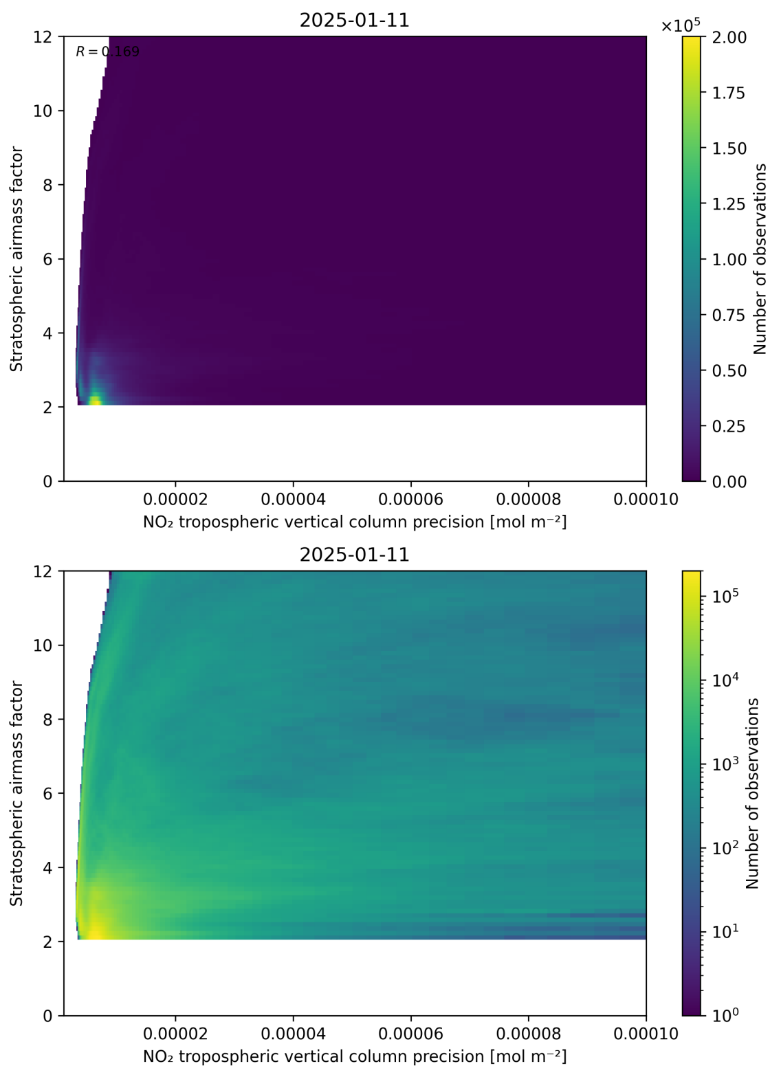
Figure 131: Scatter density plot of “NO 2 tropospheric vertical column precision” against “Stratospheric airmass factor” for 2025-01-10 to 2025-01-12.
