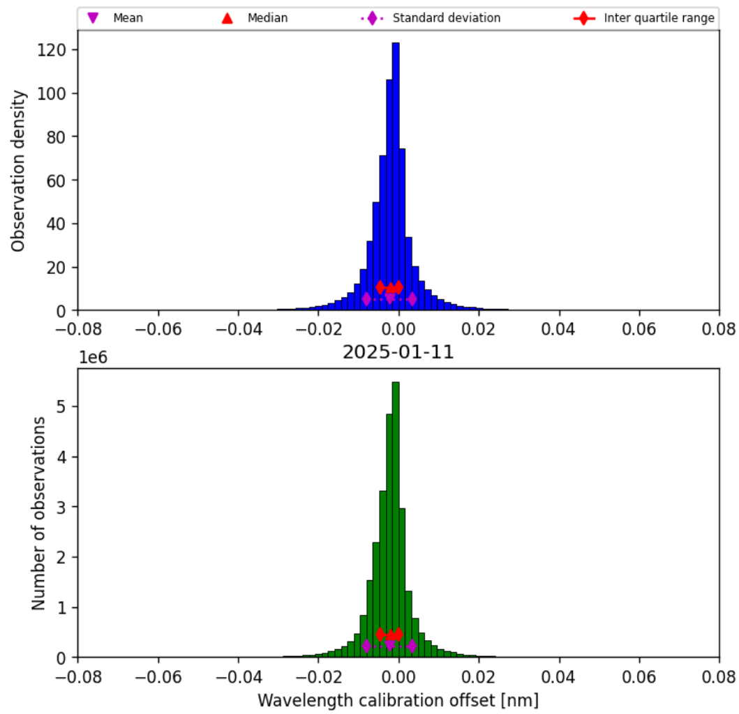
Figure 35: Histogram of “Wavelength calibration offset” for 2025-01-10 to 2025-01-12
