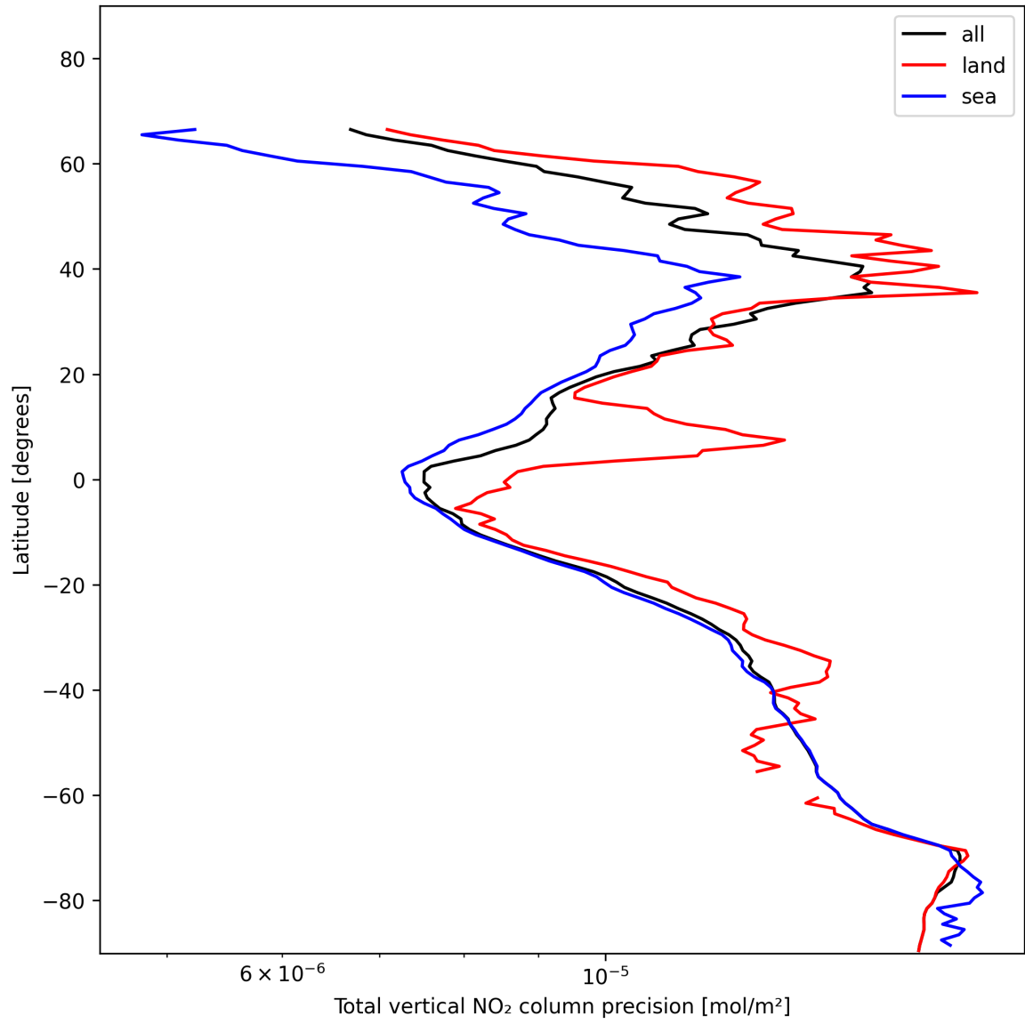
Figure 22: Zonal average of “Total vertical NO 2 column precision” for 2025-01-10 to 2025-01-12.
