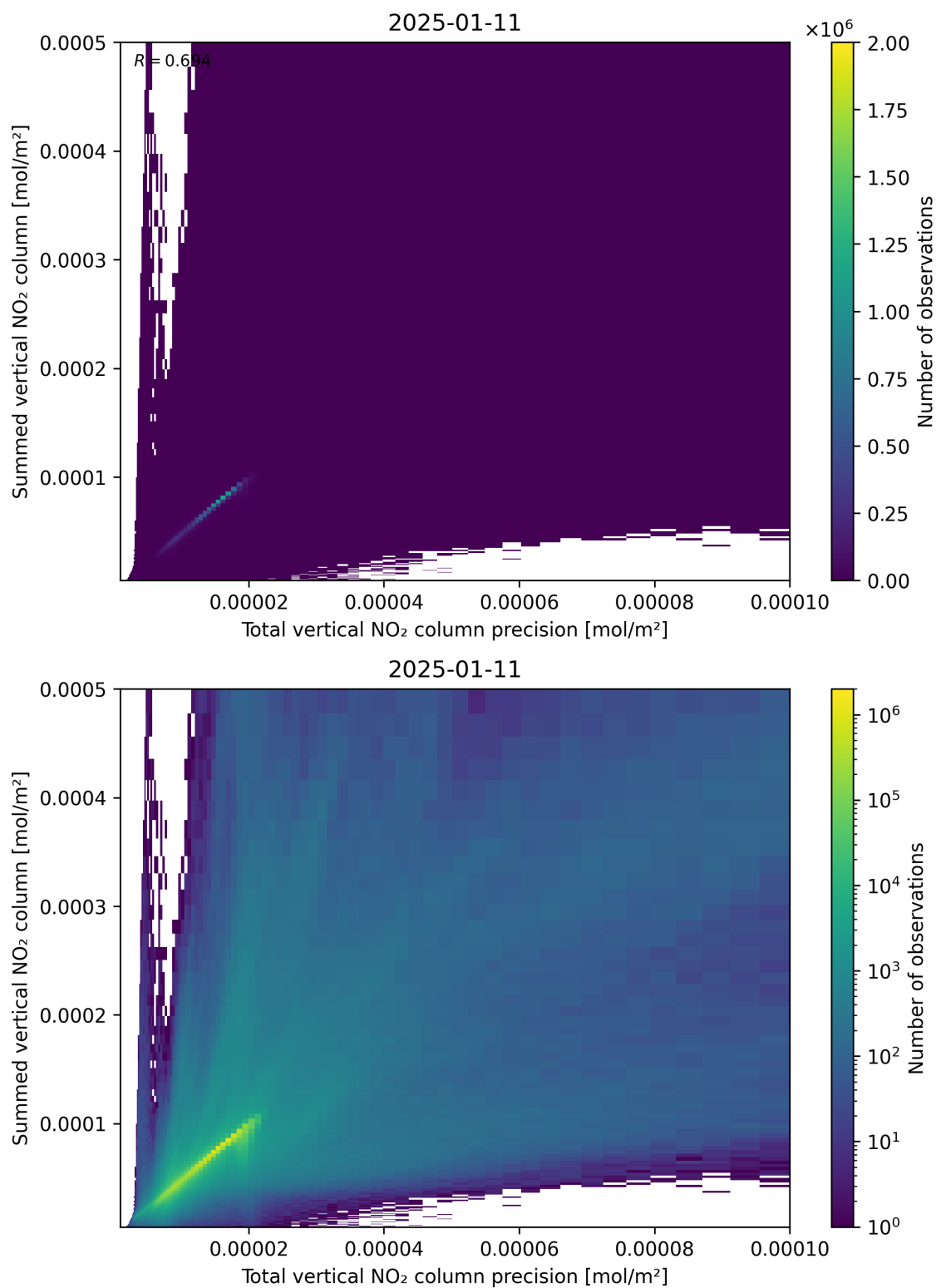
Figure 117: Scatter density plot of “Total vertical NO 2 column precision” against “Summed vertical NO 2 column” for 2025-01-10 to 2025-01-12.
