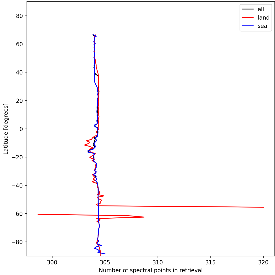
Figure 16: Zonal average of “Number of spectral points in retrieval” for 2025-01-10 to 2025-01-12.
