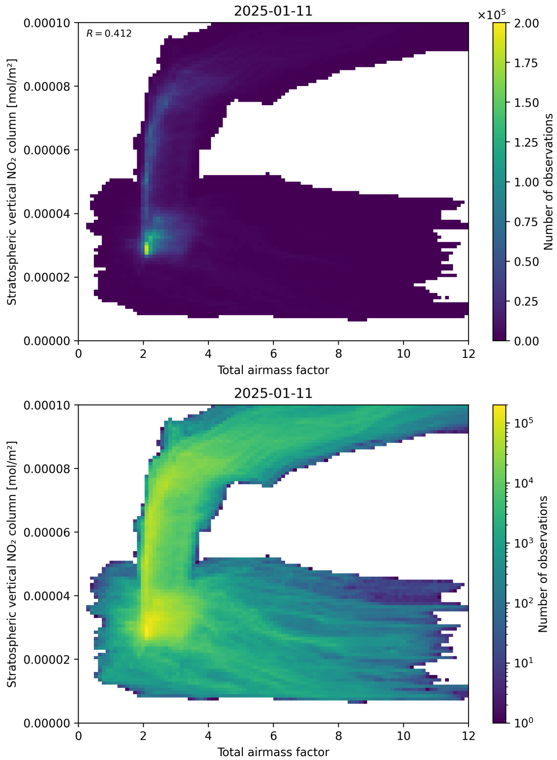
Figure 64: Scatter density plot of “Total airmass factor” against “Stratospheric vertical \text{NO}_2 column” for 2025-01-10 to 2025-01-12.
