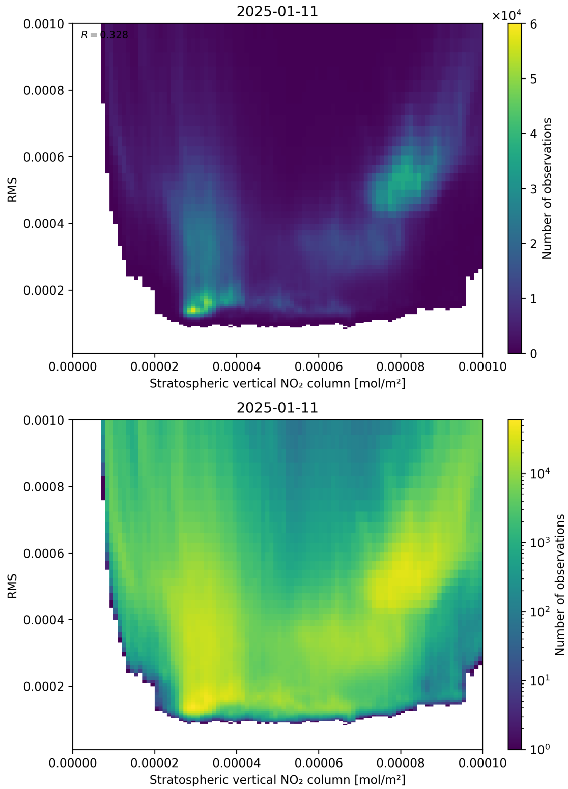
Figure 102: Scatter density plot of “Stratospheric vertical NO 2 column” against “RMS” for 2025-01-10 to 2025-01-12.
