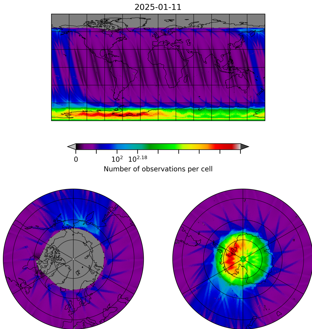
Figure 10: Map of the number of observations for 2025-01-10 to 2025-01-12
