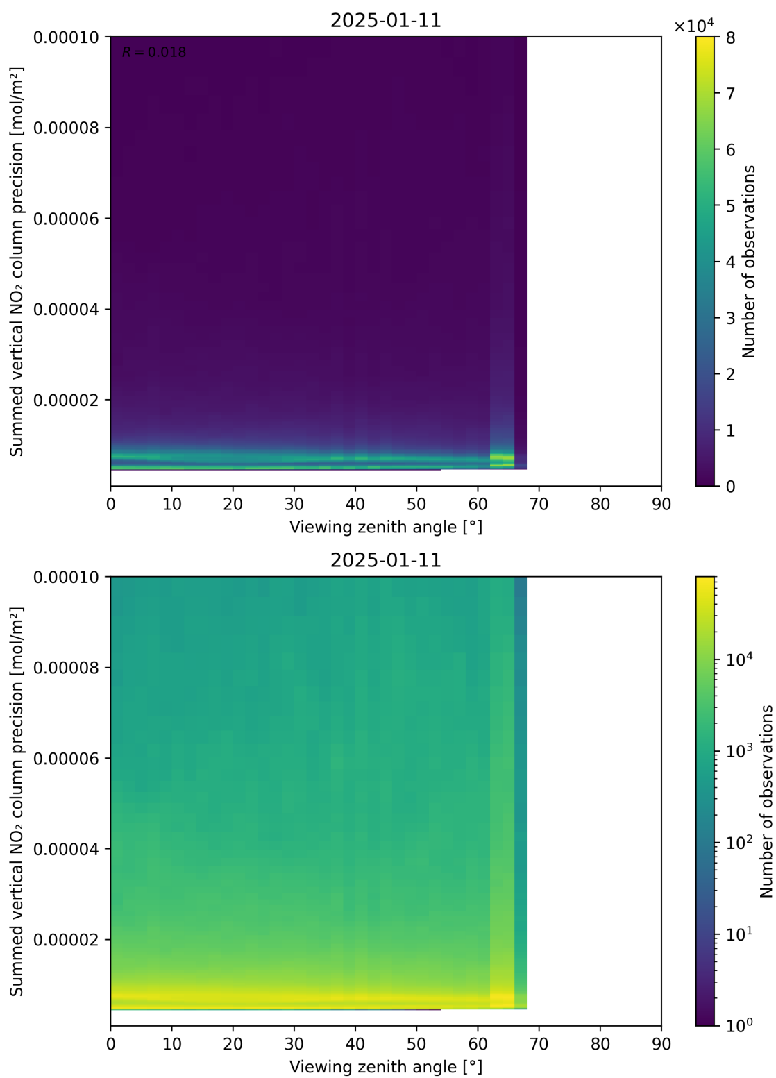
Figure 166: Scatter density plot of “Viewing zenith angle” against “Summed vertical NO 2 column precision” for 2025-01-10 to 2025-01-12.
