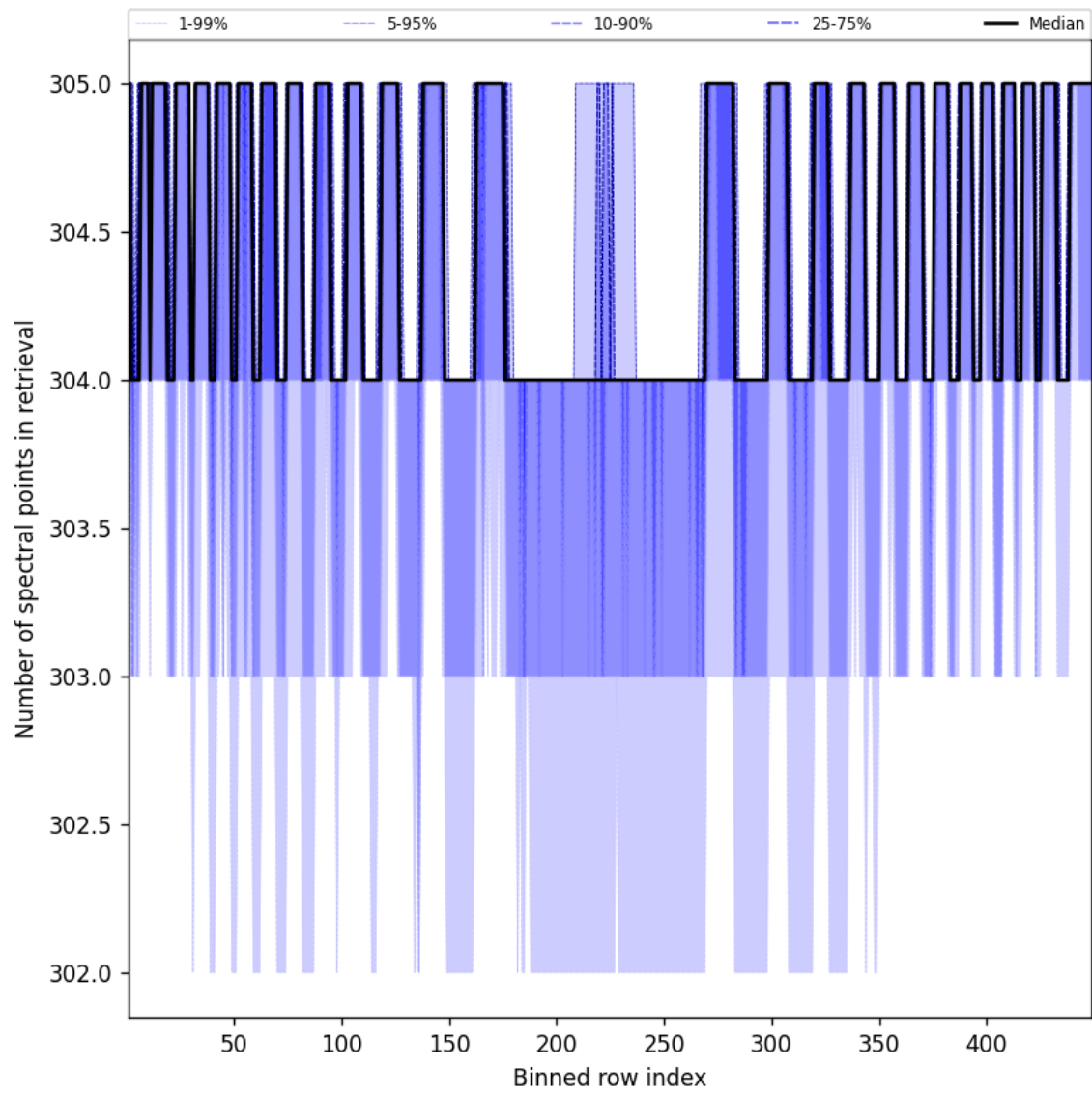
Figure 50: Along track statistics of “Number of spectral points in retrieval” for 2025-01-10 to 2025-01-12
