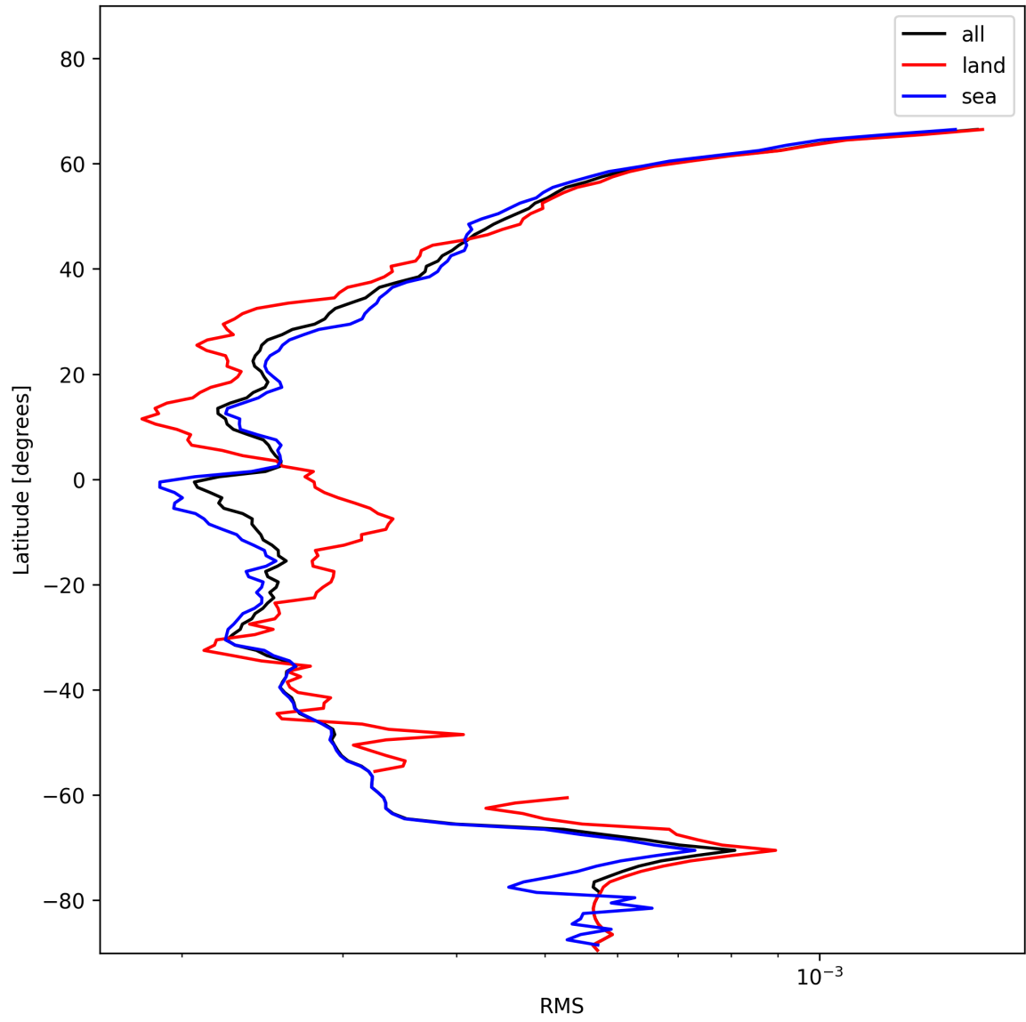
Figure 26: Zonal average of “RMS” for 2025-01-10 to 2025-01-12.
