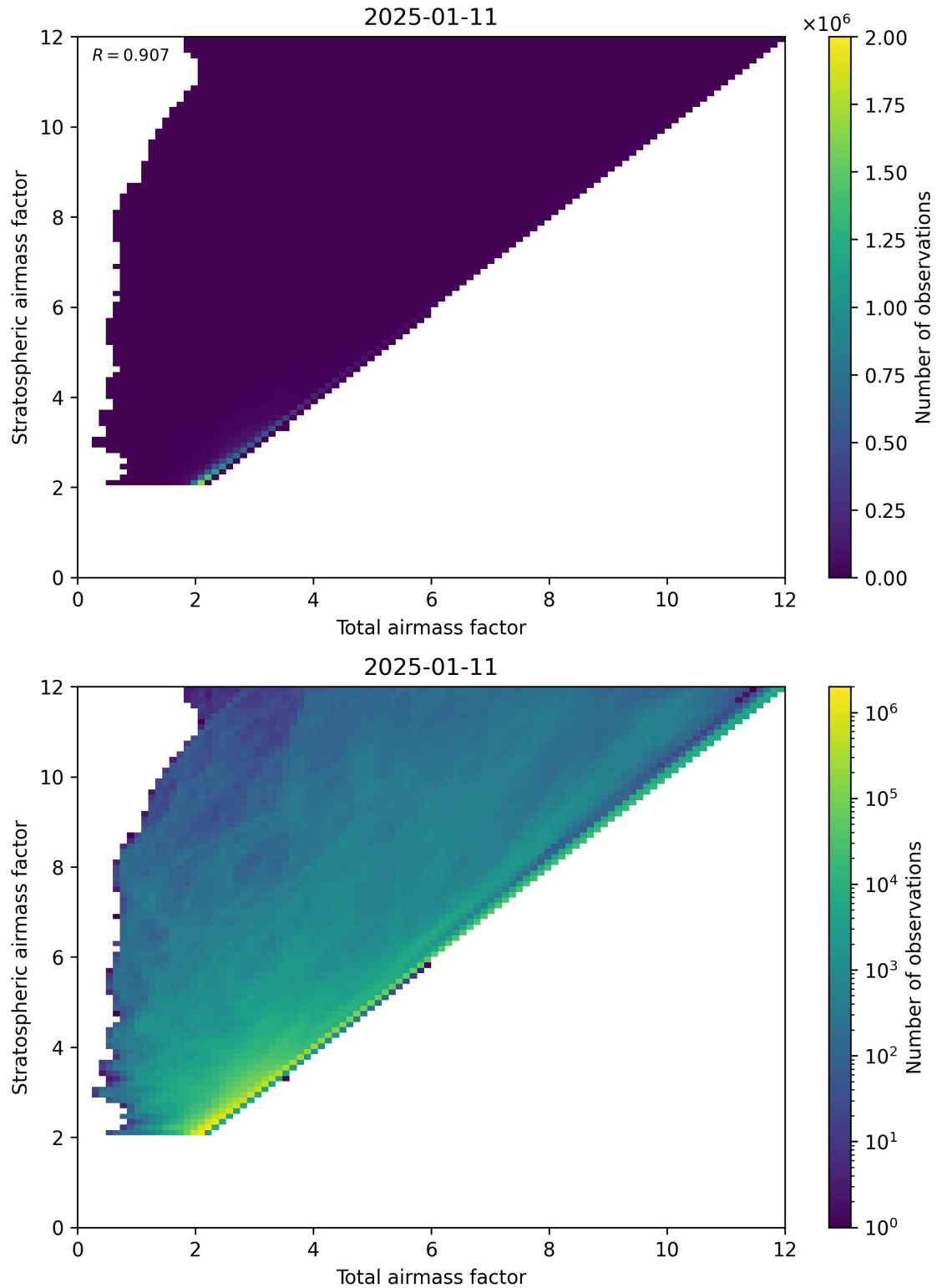
Figure 62: Scatter density plot of “Total air mass factor” against “Stratospheric air mass factor” for 2025-01-10 to 2025-01-12.
