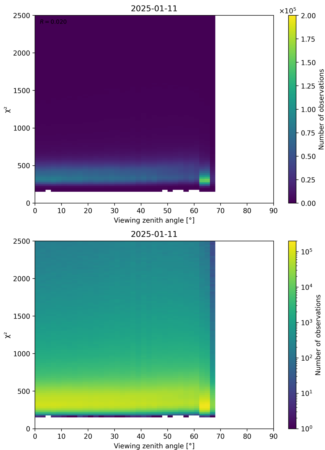
Figure 162: Scatter density plot of “Viewing zenith angle” against “ \chi^2 ” for 2025-01-10 to 2025-01-12.
