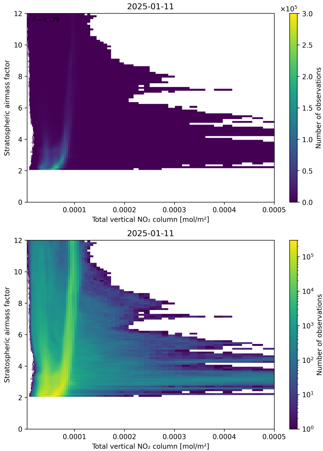
Figure 110: Scatter density plot of “Total vertical NO 2 column” against “Stratospheric airmass factor” for 2025-01-10 to 2025-01-12.
