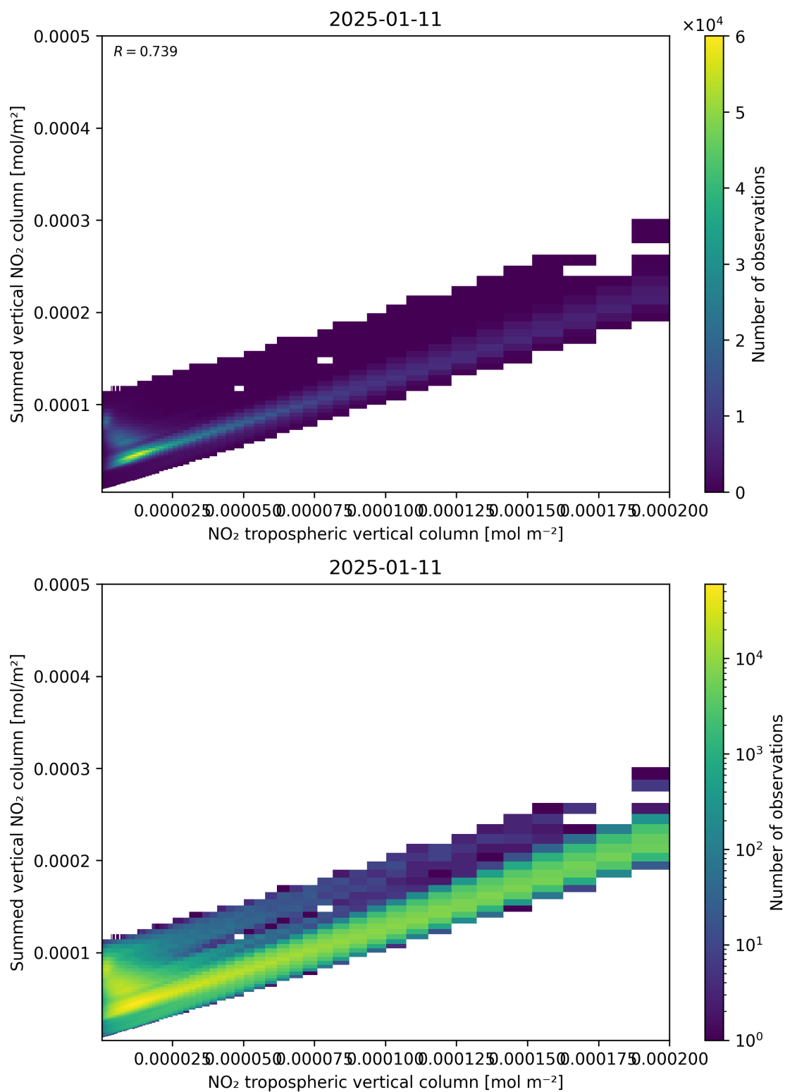
Figure 126: Scatter density plot of “NO 2 tropospheric vertical column” against “Summed vertical NO 2 column” for 2025-01-10 to 2025-01-12.
