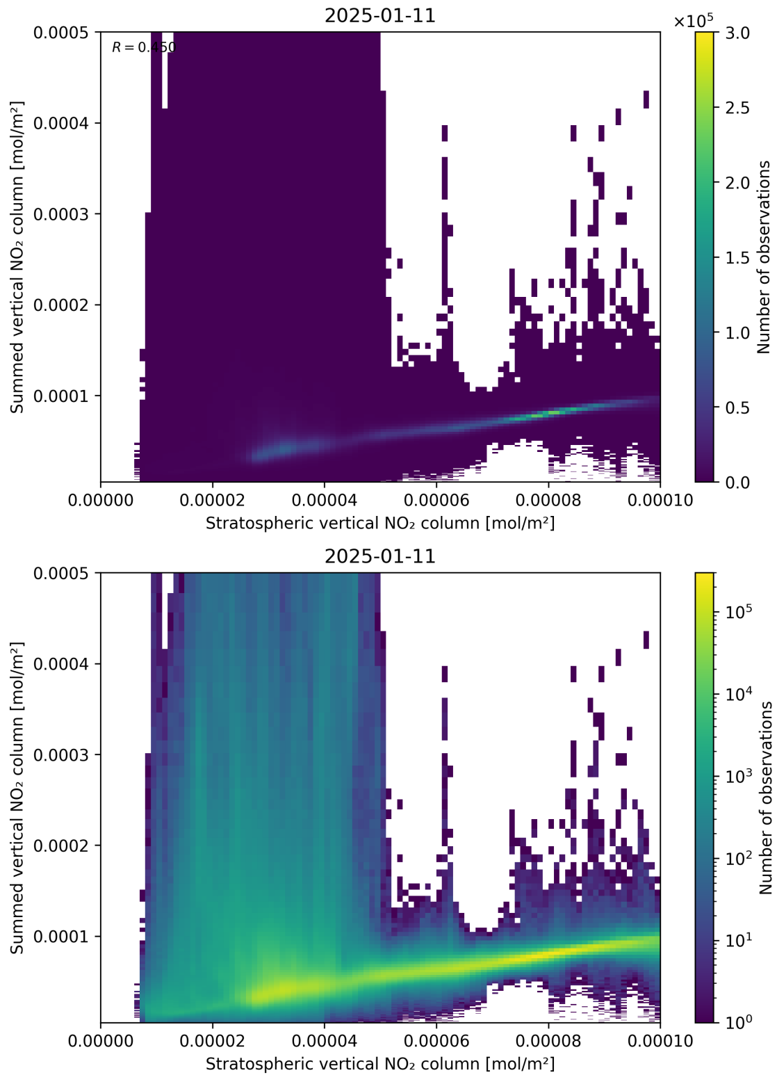
Figure 98: Scatter density plot of “Stratospheric vertical NO 2 column” against “Summed vertical NO 2 column” for 2025-01-10 to 2025-01-12.
