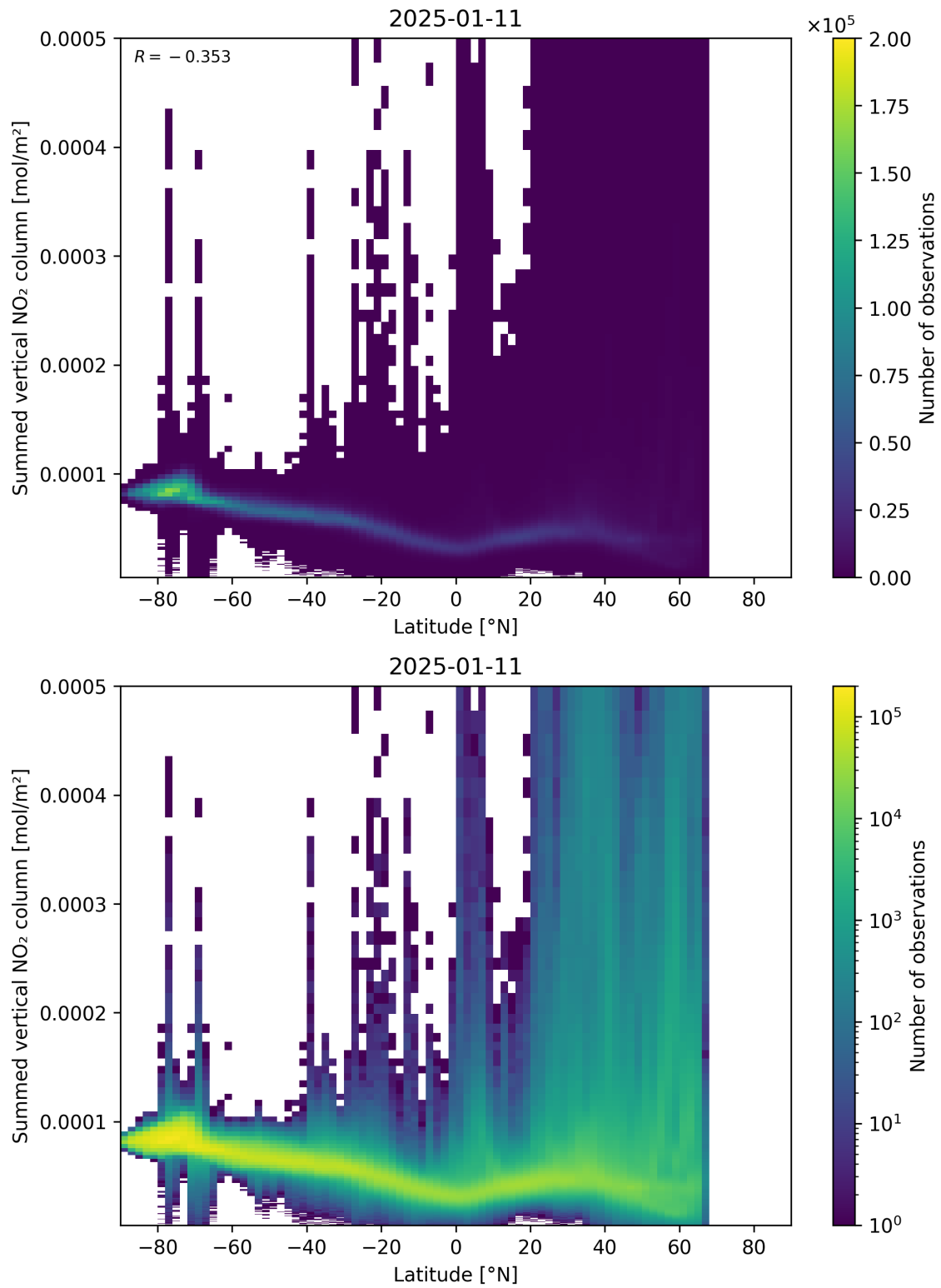
Figure 88: Scatter density plot of “Latitude” against “Summed vertical NO 2 column” for 2025-01-10 to 2025-01-12.
