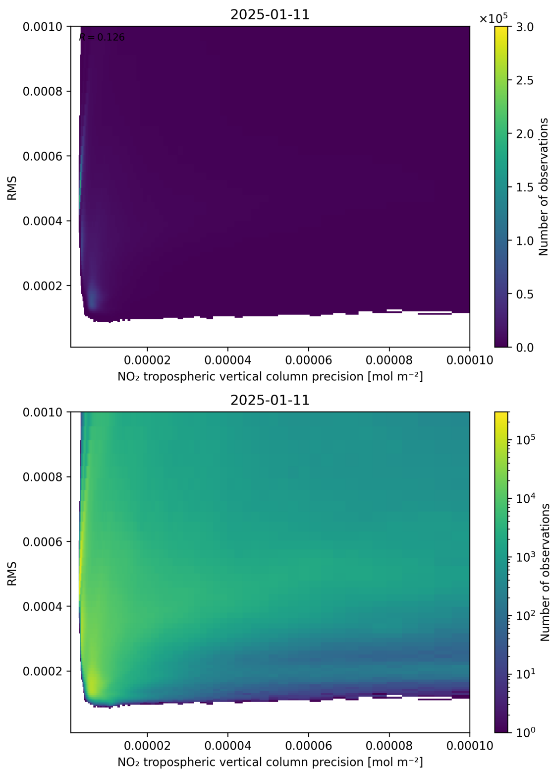
Figure 140: Scatter density plot of “NO 2 tropospheric vertical column precision” against “RMS” for 2025-01-10 to 2025-01-12.
