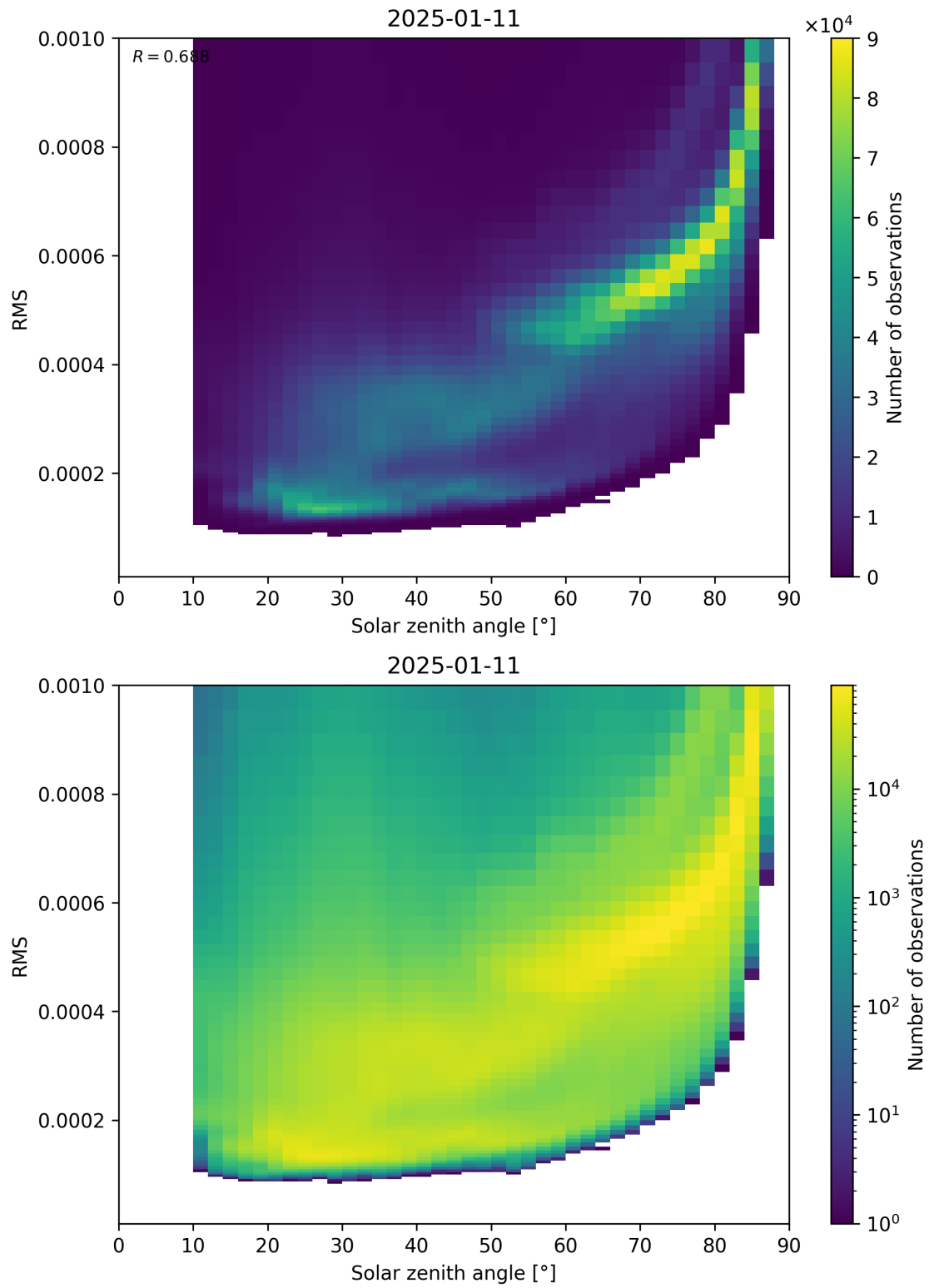
Figure 157: Scatter density plot of “Solar zenith angle” against “RMS” for 2025-01-10 to 2025-01-12.
