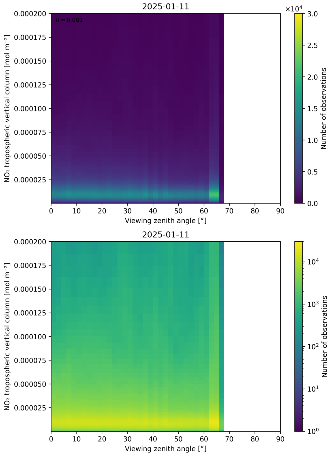
Figure 169: Scatter density plot of “Viewing zenith angle” against “NO 2 tropospheric vertical column” for 2025-01-10 to 2025-01-12.
