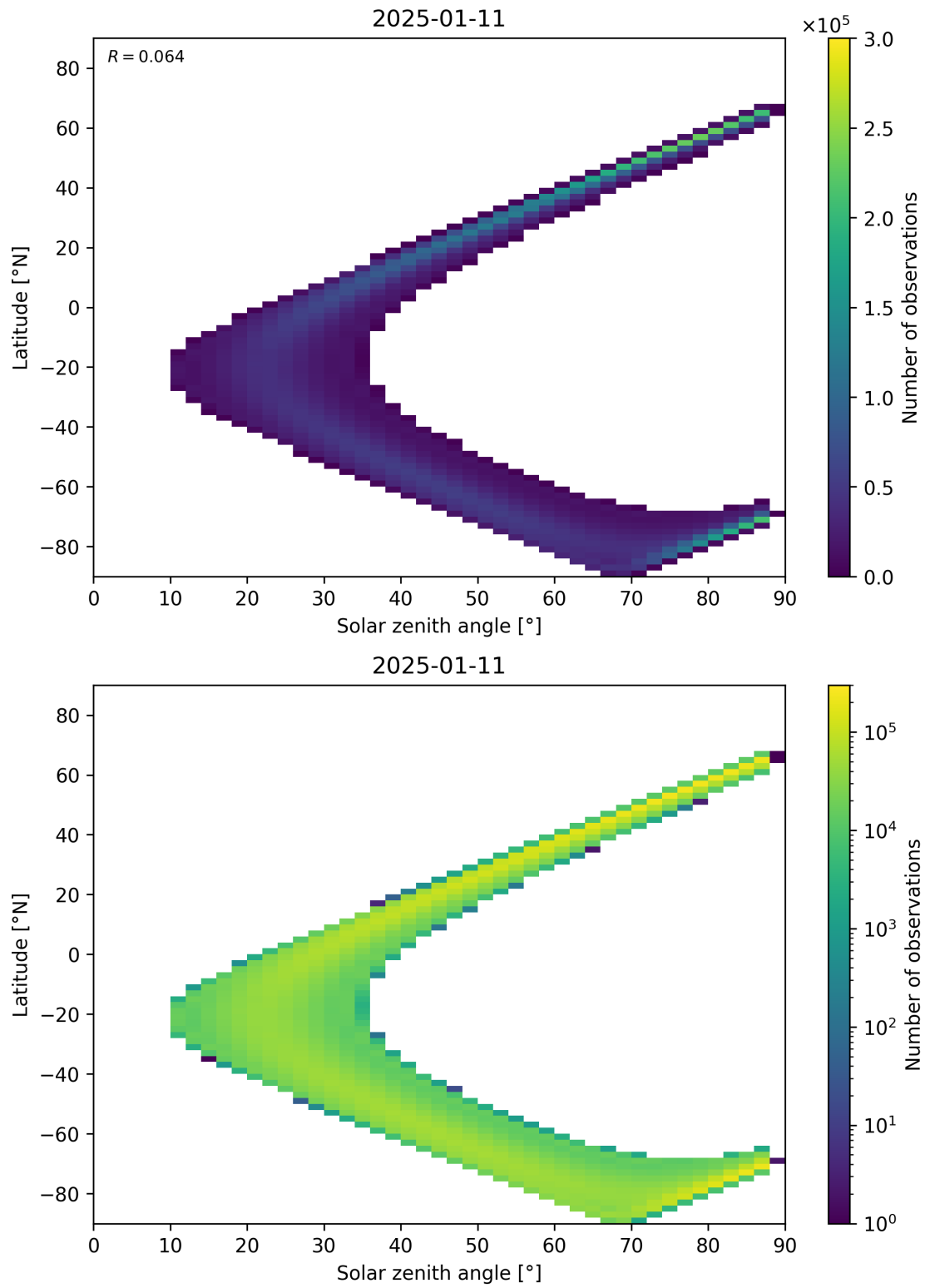
Figure 149: Scatter density plot of “Solar zenith angle” against “Latitude” for 2025-01-10 to 2025-01-12.
