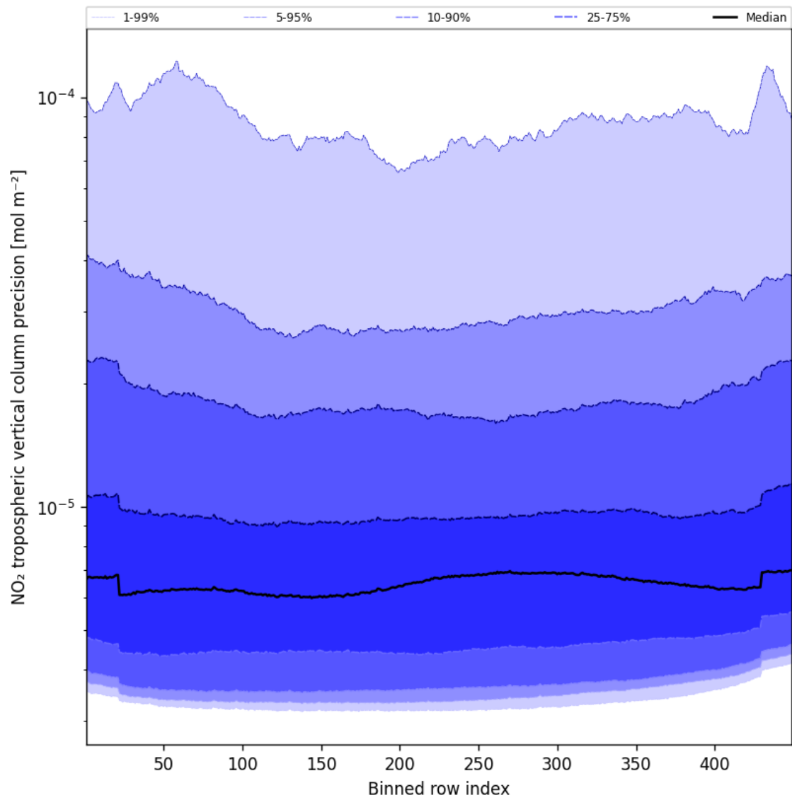
Figure 47: Along track statistics of “NO 2 tropospheric vertical column precision” for 2025-01-10 to 2025-01-12
