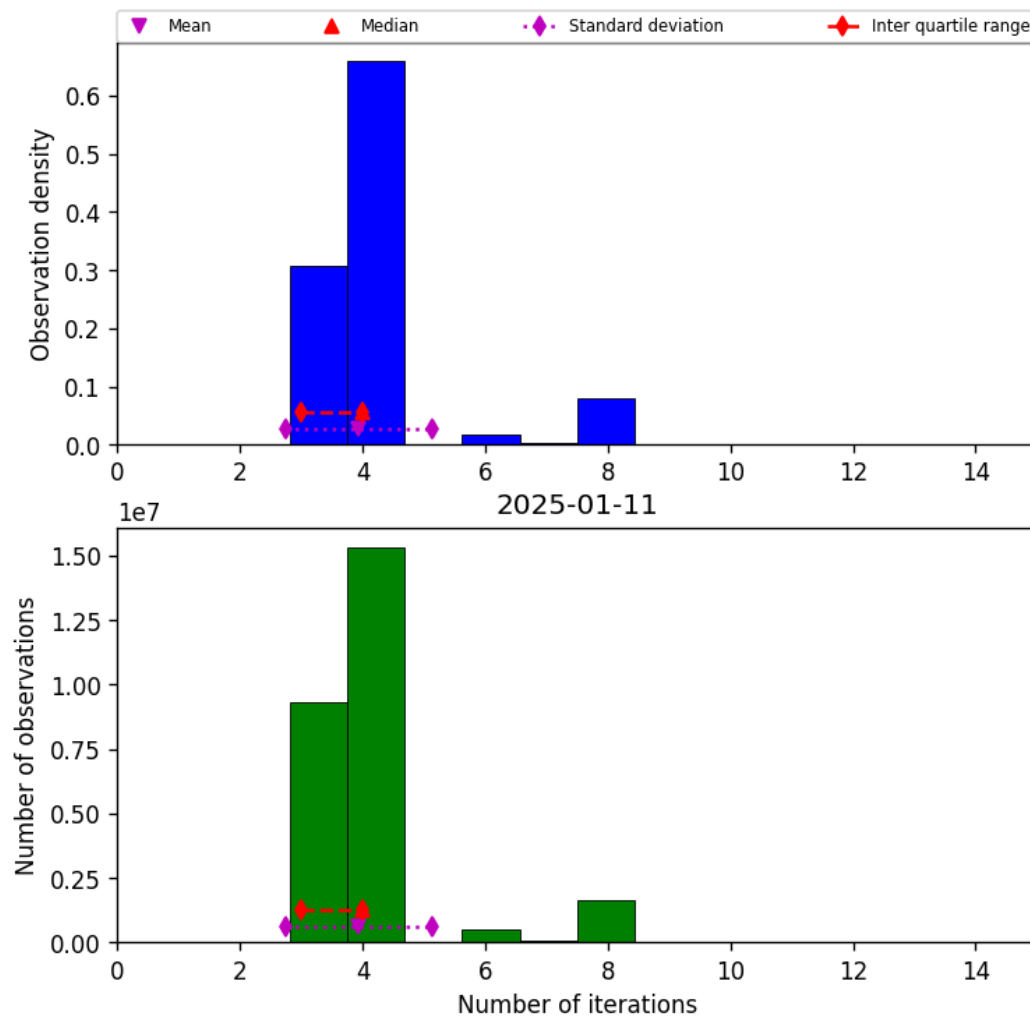
Figure 34: Histogram of “Number of iterations” for 2025-01-10 to 2025-01-12
