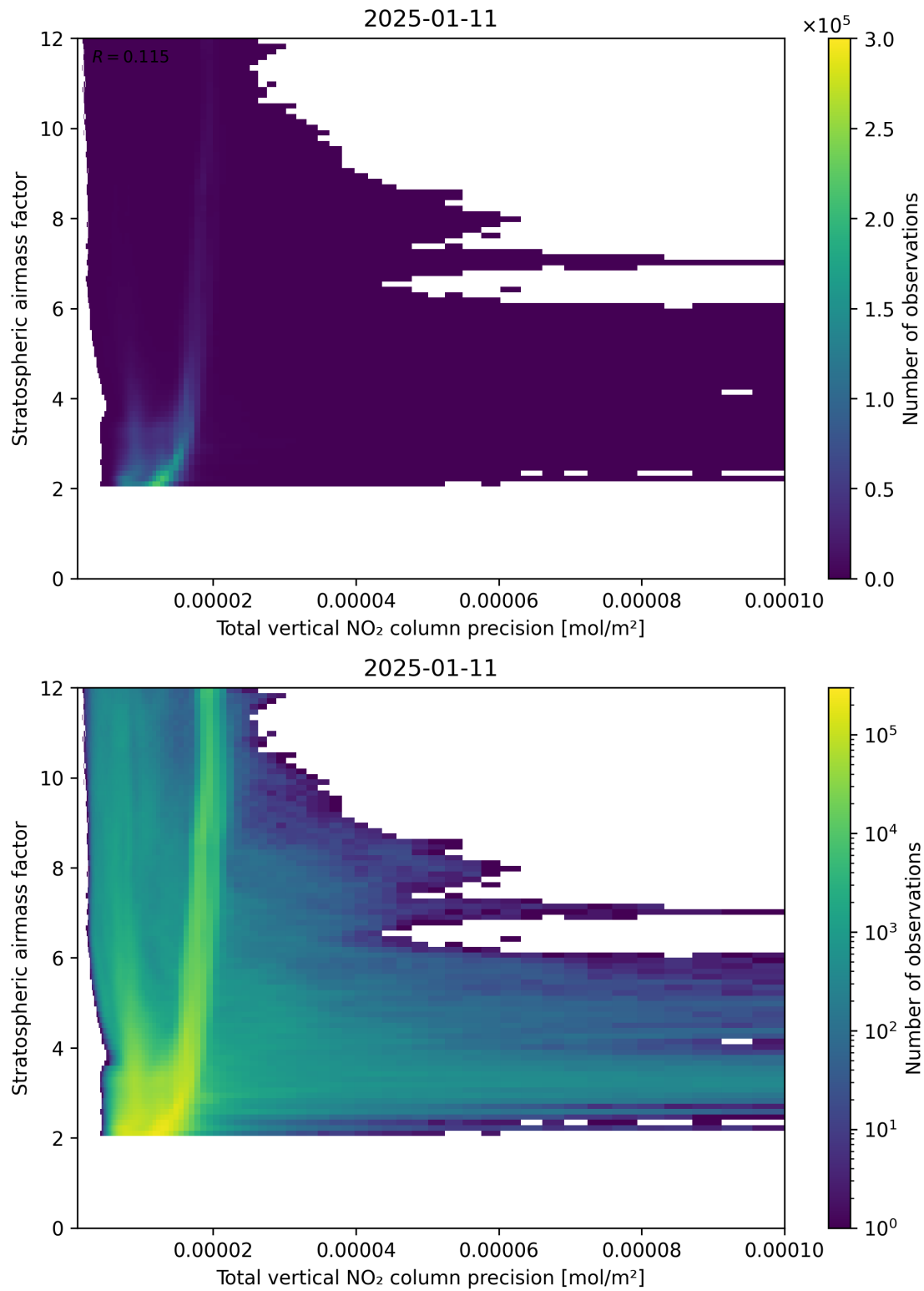
Figure 115: Scatter density plot of “Total vertical NO 2 column precision” against “Stratospheric air mass factor” for 2025-01-10 to 2025-01-12.
