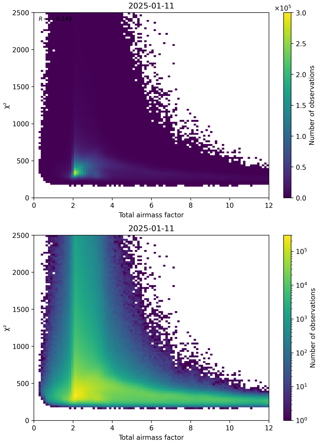
Figure 63: Scatter density plot of “Total airmass factor” against “ \chi^2 ” for 2025-01-10 to 2025-01-12.
