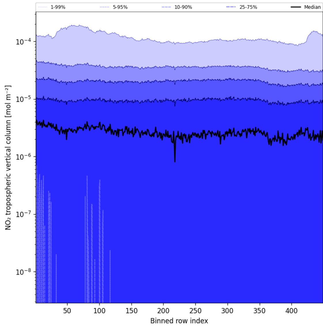
Figure 46: Along track statistics of “NO 2 tropospheric vertical column” for 2025-01-10 to 2025-01-12
