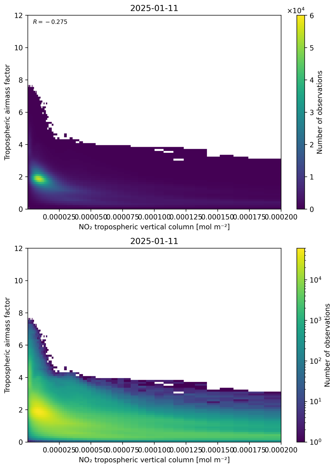
Figure 123: Scatter density plot of “NO 2 tropospheric vertical column” against “Tropospheric air mass factor” for 2025-01-10 to 2025-01-12.
