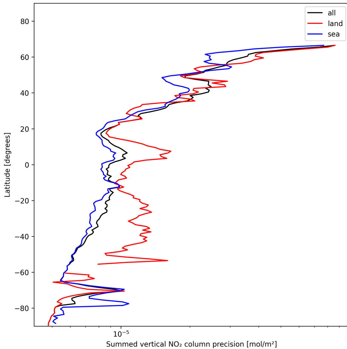
Figure 24: Zonal average of “Summed vertical NO 2 column precision” for 2025-01-10 to 2025-01-12.
