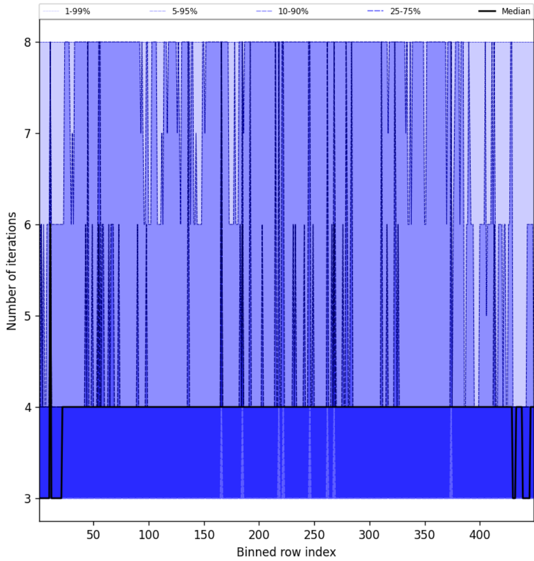
Figure 51: Along track statistics of “Number of iterations” for 2025-01-10 to 2025-01-12
