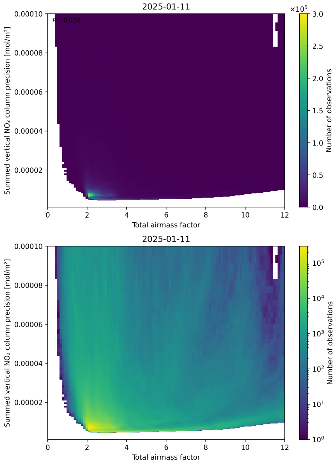
Figure 66: Scatter density plot of “Total airmass factor” against “Summed vertical NO 2 column precision” for 2025-01-10 to 2025-01-12.
