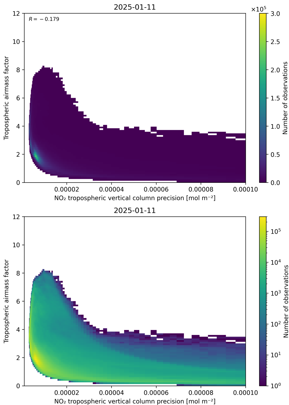
Figure 133: Scatter density plot of “NO 2 tropospheric vertical column precision” against “Tropospheric airmass factor” for 2025-01-10 to 2025-01-12.
