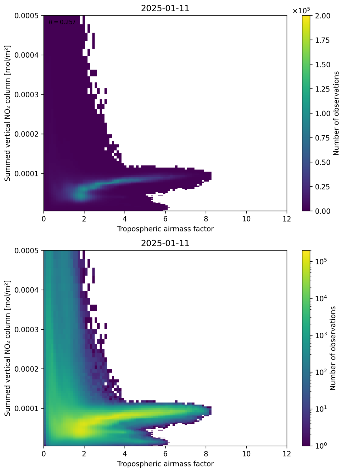
Figure 75: Scatter density plot of “Tropospheric airmass factor” against “Summed vertical NO 2 column” for 2025-01-10 to 2025-01-12.
