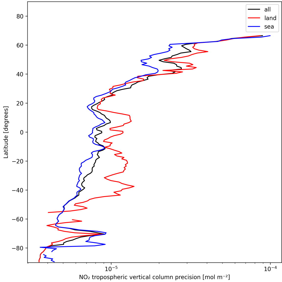
Figure 13: Zonal average of “NO 2 tropospheric vertical column precision” for 2025-01-12 to 2025-01-13.
