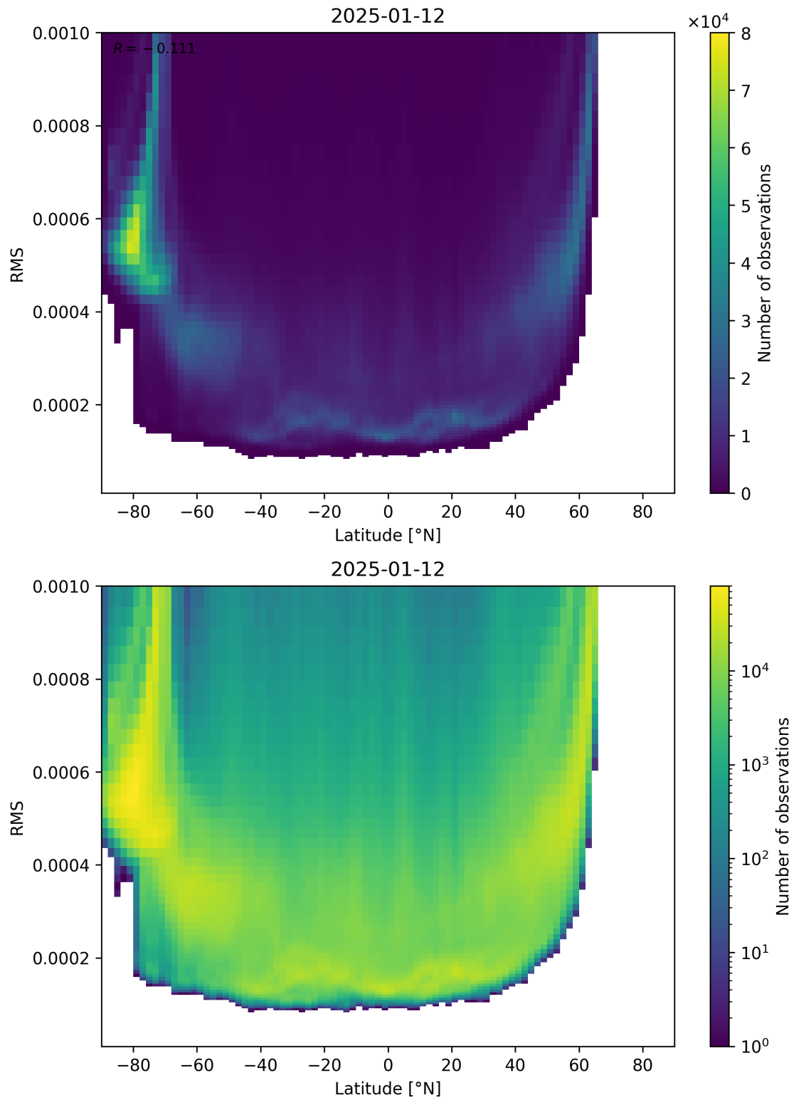
Figure 94: Scatter density plot of “Latitude” against “RMS” for 2025-01-12 to 2025-01-13.
