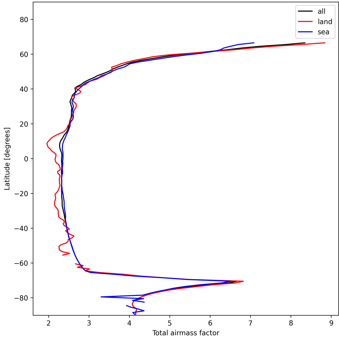
Figure 15: Zonal average of “Total airmass factor” for 2025-01-12 to 2025-01-13.
