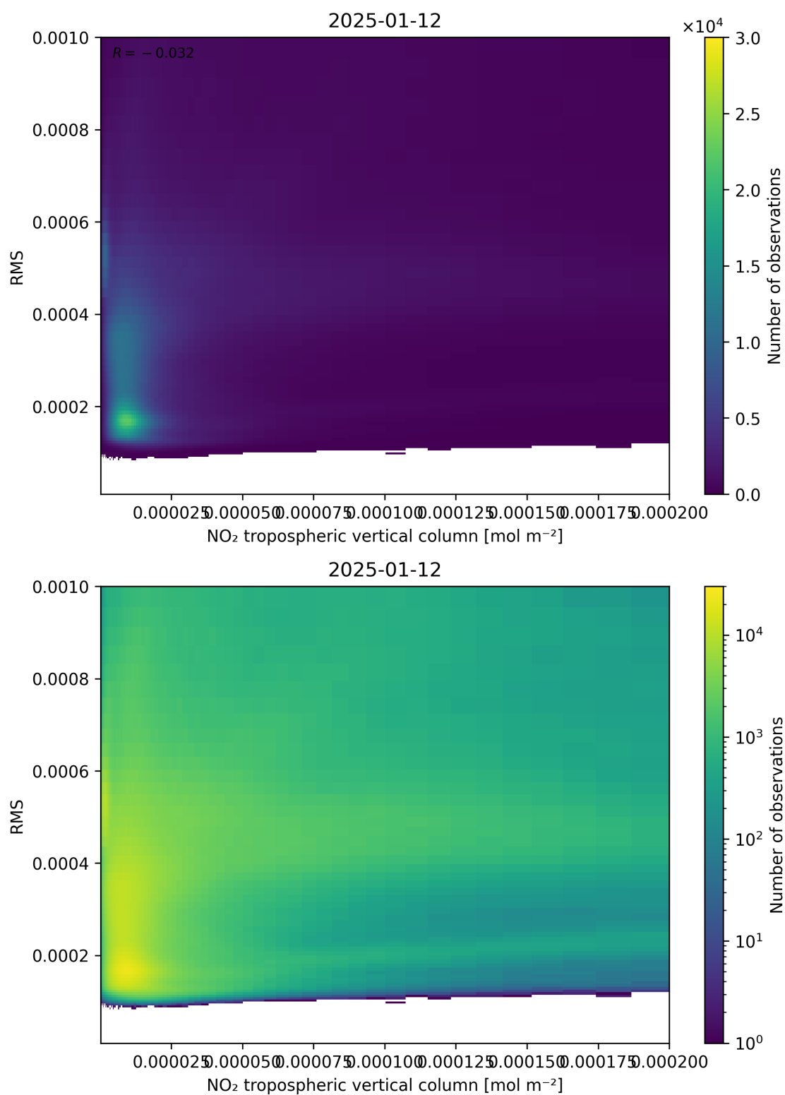
Figure 142: Scatter density plot of “NO 2 tropospheric vertical column” against “RMS” for 2025-01-12 to 2025-01-13.
