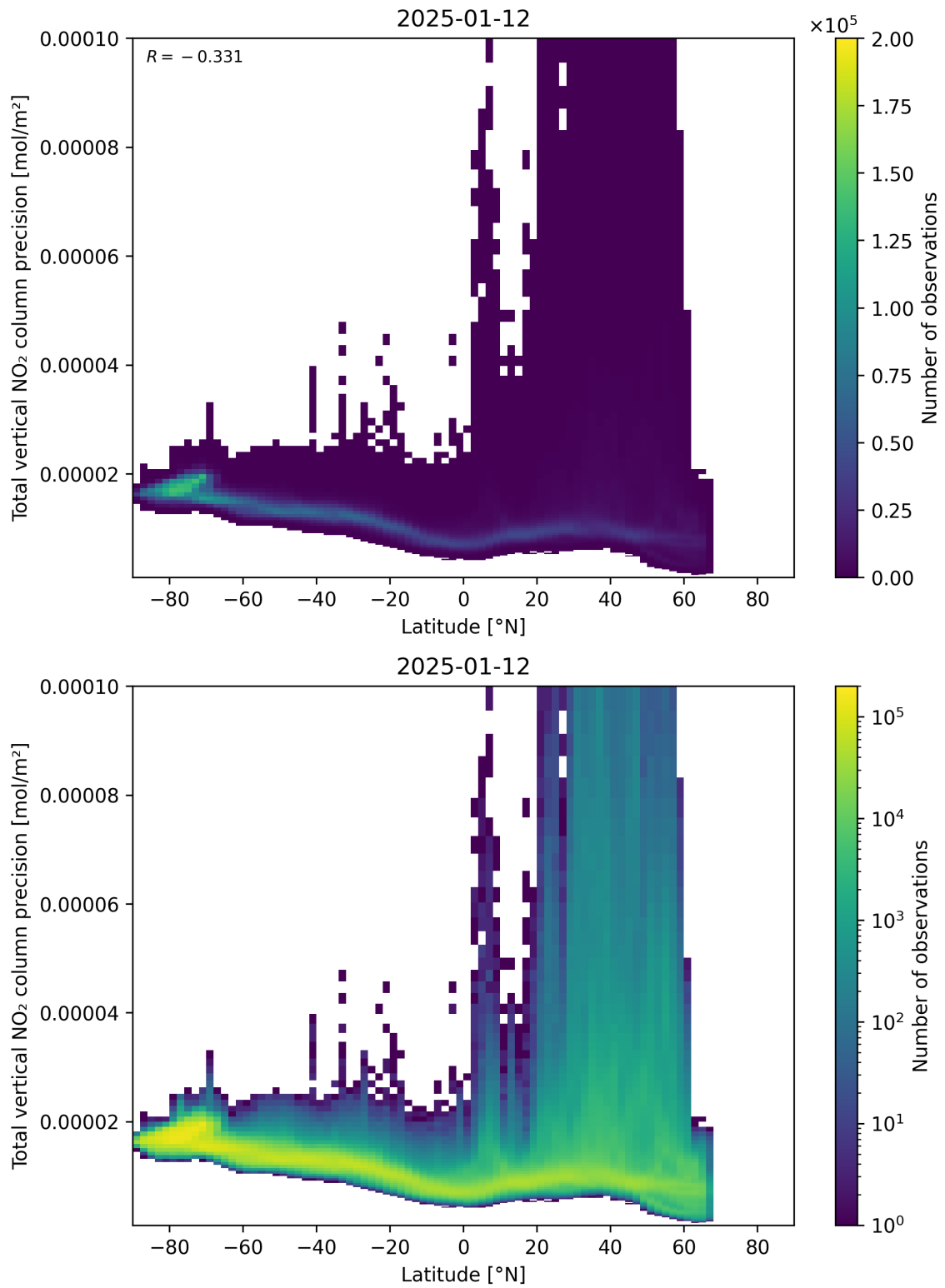
Figure 91: Scatter density plot of “Latitude” against “Total vertical NO 2 column precision” for 2025-01-12 to 2025-01-13.
