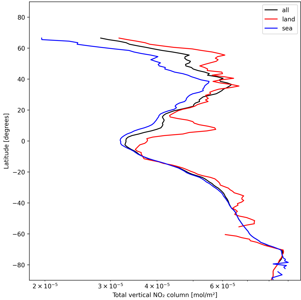
Figure 21: Zonal average of “Total vertical NO 2 column” for 2025-01-12 to 2025-01-13.
