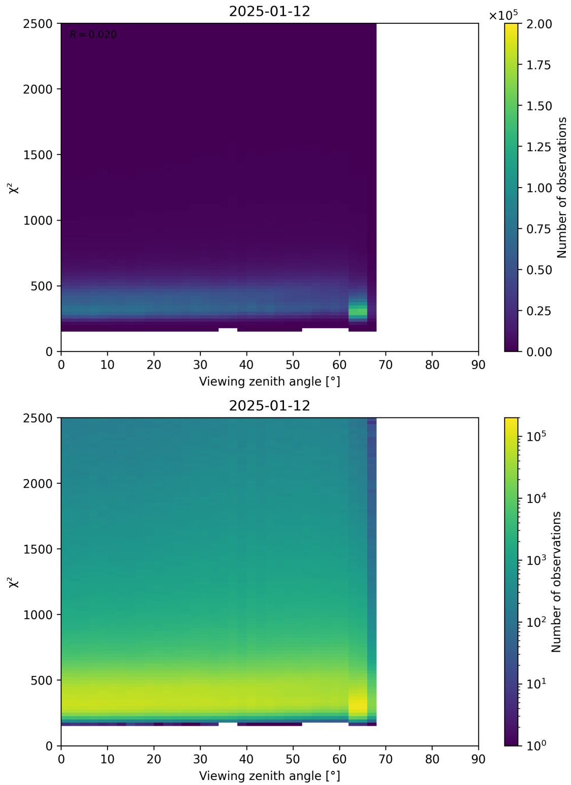
Figure 162: Scatter density plot of “Viewing zenith angle” against “ \chi^2 ” for 2025-01-12 to 2025-01-13.
