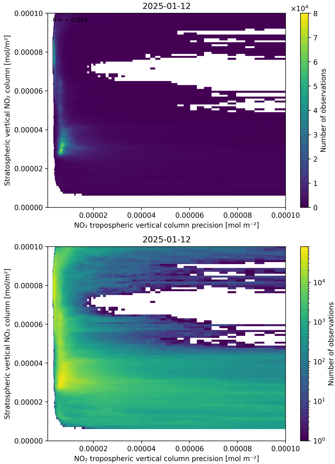
Figure 135: Scatter density plot of “NO 2 tropospheric vertical column precision” against “Stratospheric vertical NO 2 column” for 2025-01-12 to 2025-01-13.
