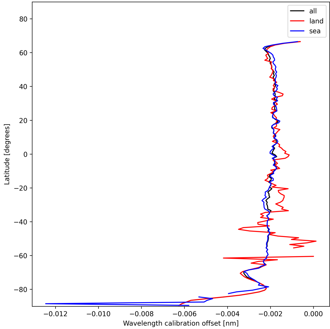
Figure 18: Zonal average of “Wavelength calibration offset” for 2025-01-12 to 2025-01-13.
