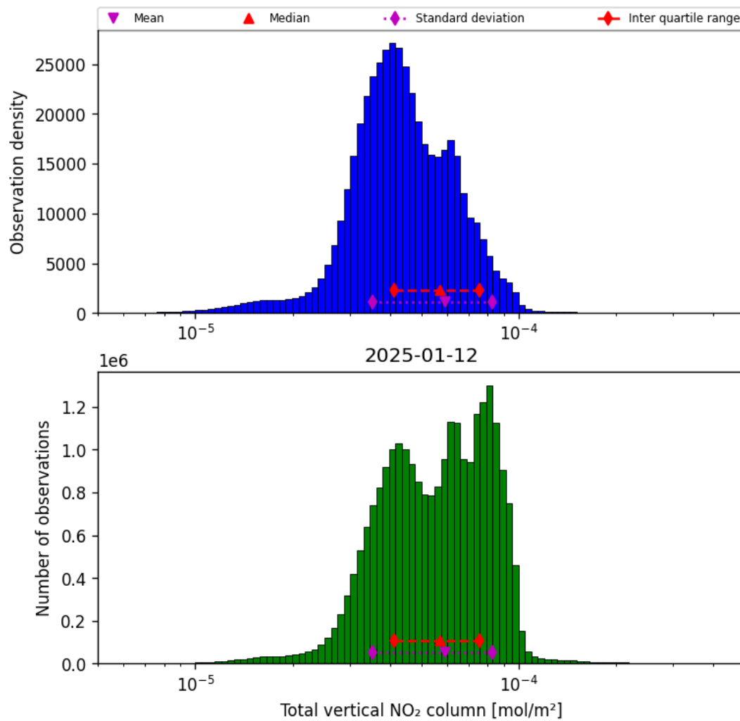
Figure 38: Histogram of “Total vertical NO 2 column” for 2025-01-12 to 2025-01-13
