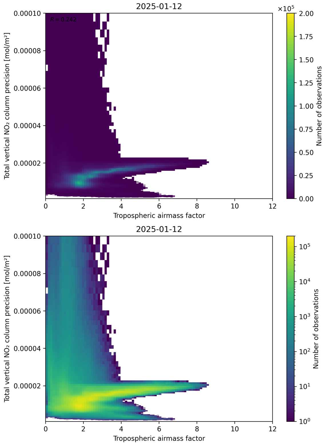
Figure 78: Scatter density plot of “Tropospheric air mass factor” against “Total vertical NO 2 column precision” for 2025-01-12 to 2025-01-13.
