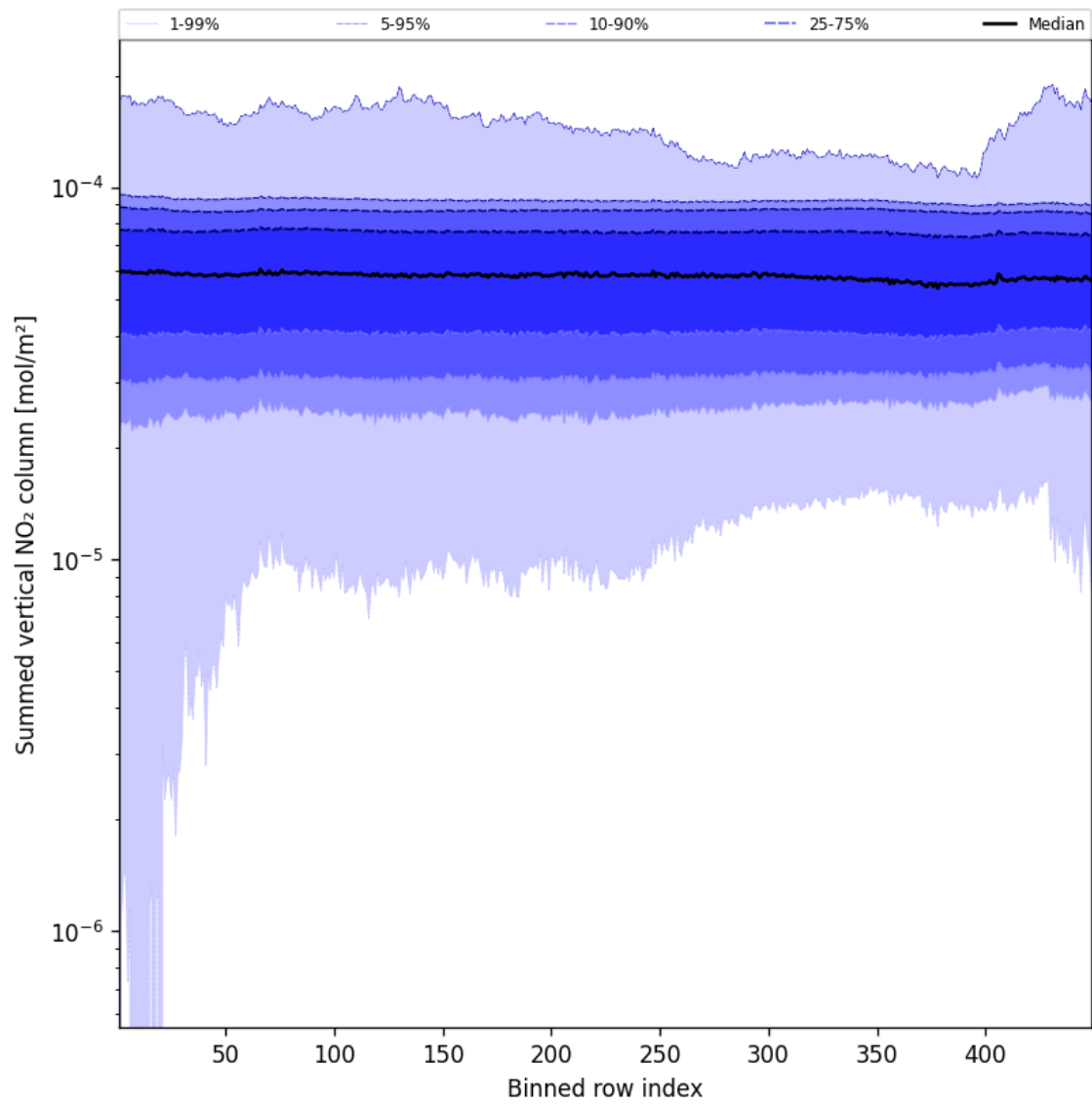
Figure 57: Along track statistics of “Summed vertical NO 2 column” for 2025-01-12 to 2025-01-13
