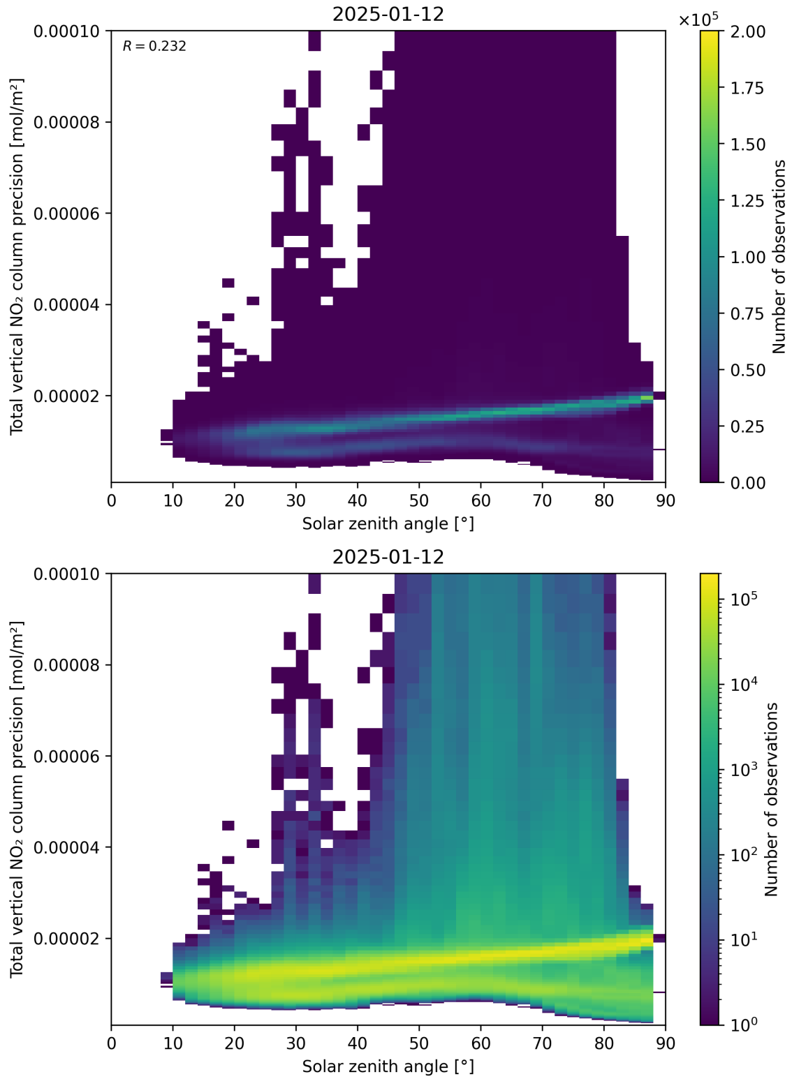
Figure 154: Scatter density plot of “Solar zenith angle” against “Total vertical NO 2 column precision” for 2025-01-12 to 2025-01-13.
