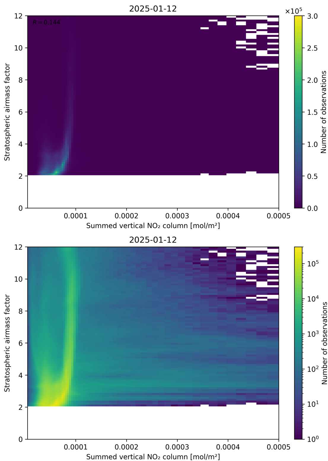
Figure 103: Scatter density plot of “Summed vertical NO 2 column” against “Stratospheric airmass factor” for 2025-01-12 to 2025-01-13.
