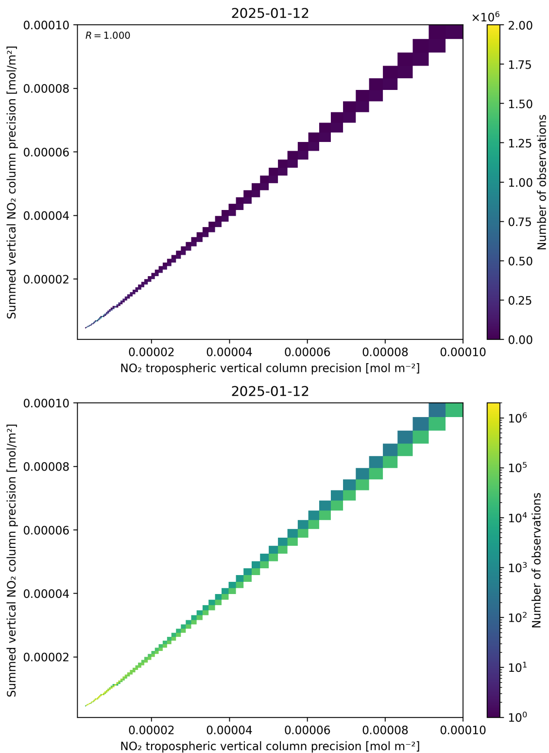
Figure 137: Scatter density plot of “NO 2 tropospheric vertical column precision” against “Summed vertical NO 2 column precision” for 2025-01-12 to 2025-01-13.
