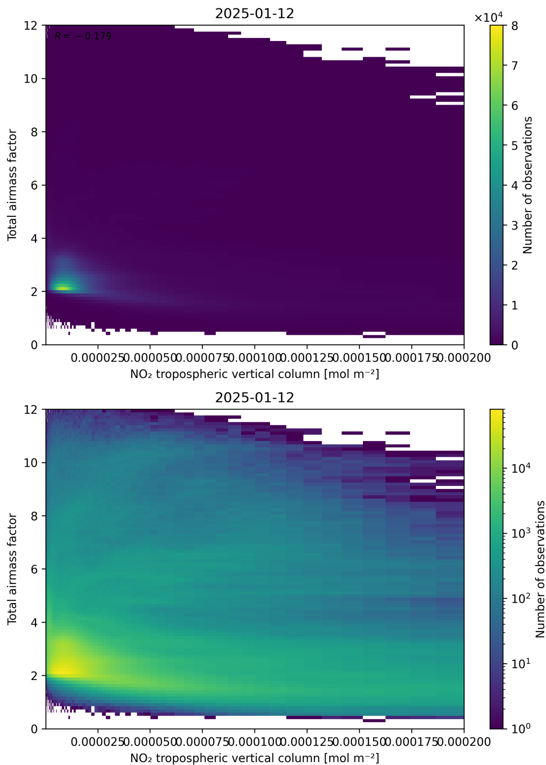
Figure 122: Scatter density plot of “NO 2 tropospheric vertical column” against “Total air mass factor” for 2025-01-12 to 2025-01-13.
