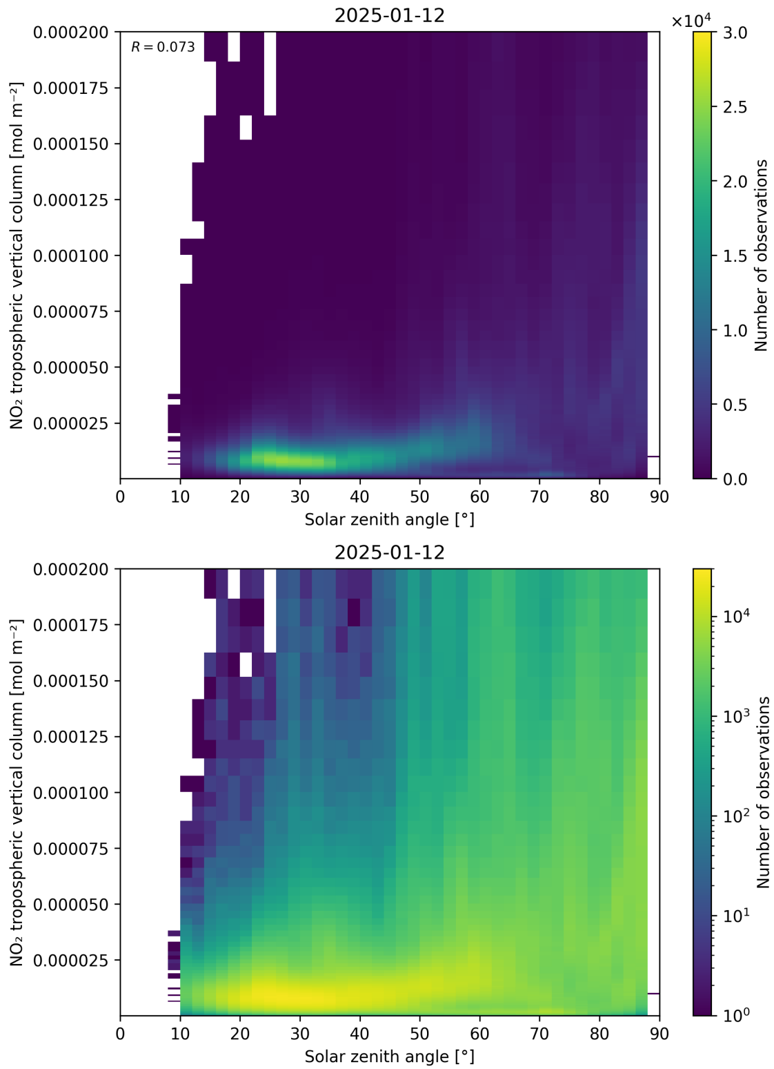
Figure 155: Scatter density plot of “Solar zenith angle” against “NO 2 tropospheric vertical column” for 2025-01-12 to 2025-01-13.
