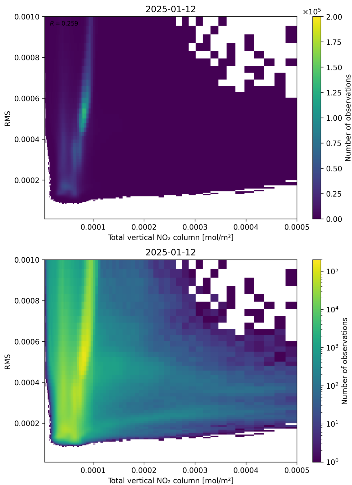
Figure 120: Scatter density plot of “Total vertical NO 2 column” against “RMS” for 2025-01-12 to 2025-01-13.
