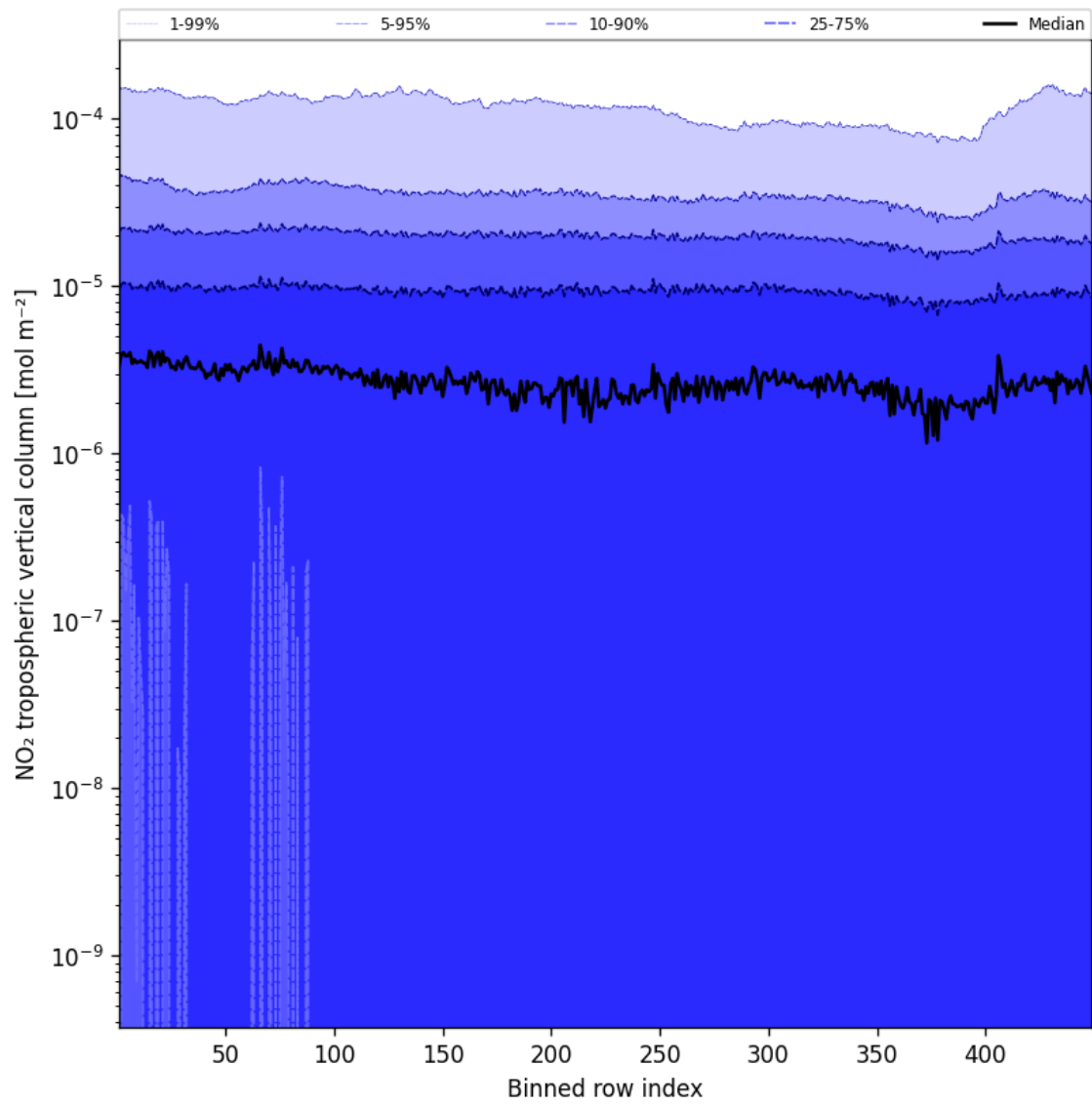
Figure 46: Along track statistics of “NO 2 tropospheric vertical column” for 2025-01-12 to 2025-01-13
