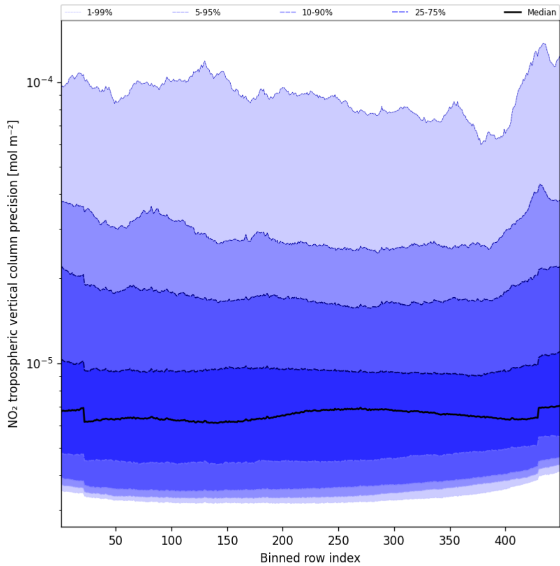
Figure 47: Along track statistics of “NO 2 tropospheric vertical column precision” for 2025-01-12 to 2025-01-13
