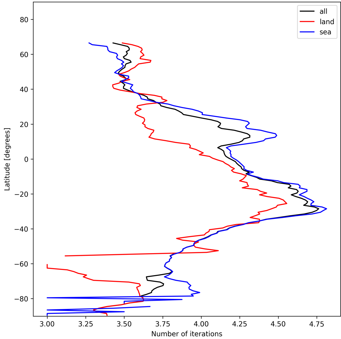
Figure 17: Zonal average of “Number of iterations” for 2025-01-12 to 2025-01-13.
