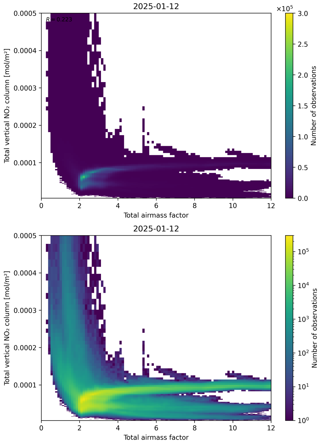
Figure 67: Scatter density plot of “Total airmass factor” against “Total vertical NO 2 column” for 2025-01-12 to 2025-01-13.
