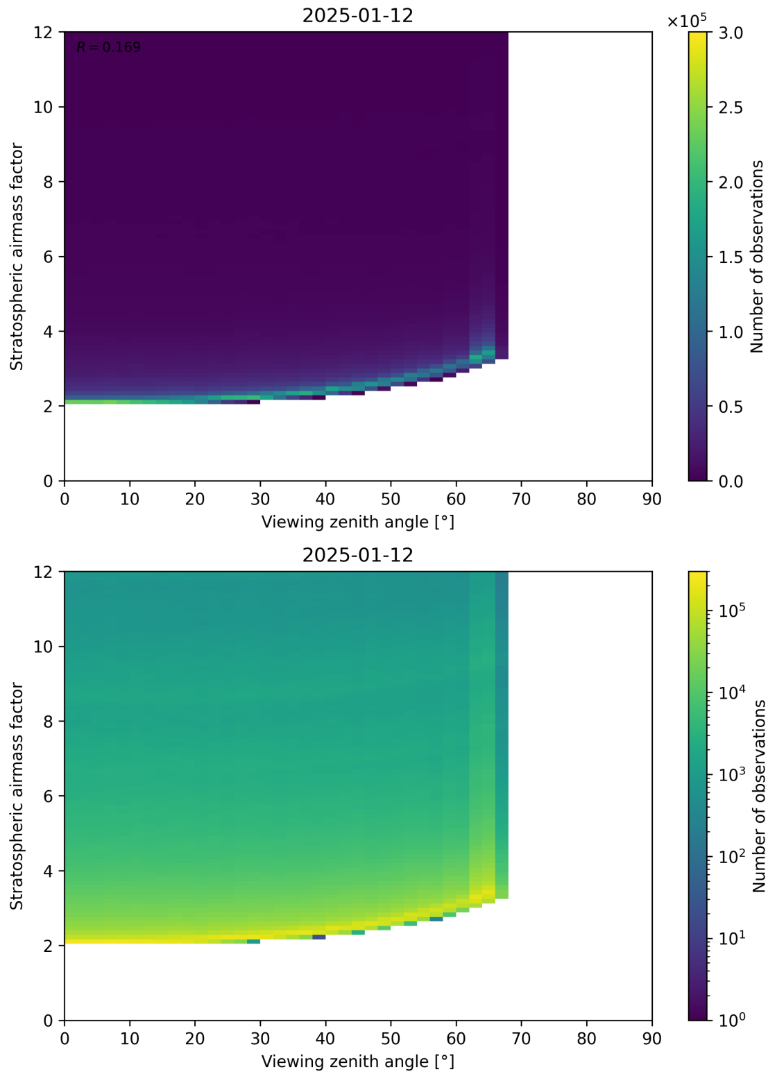
Figure 159: Scatter density plot of “Viewing zenith angle” against “Stratospheric airmass factor” for 2025-01-12 to 2025-01-13.
