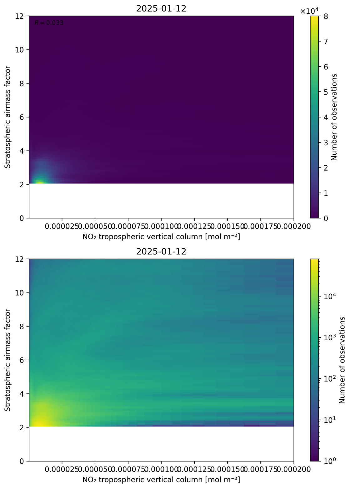
Figure 121: Scatter density plot of “NO 2 tropospheric vertical column” against “Stratospheric airmass factor” for 2025-01-12 to 2025-01-13.
