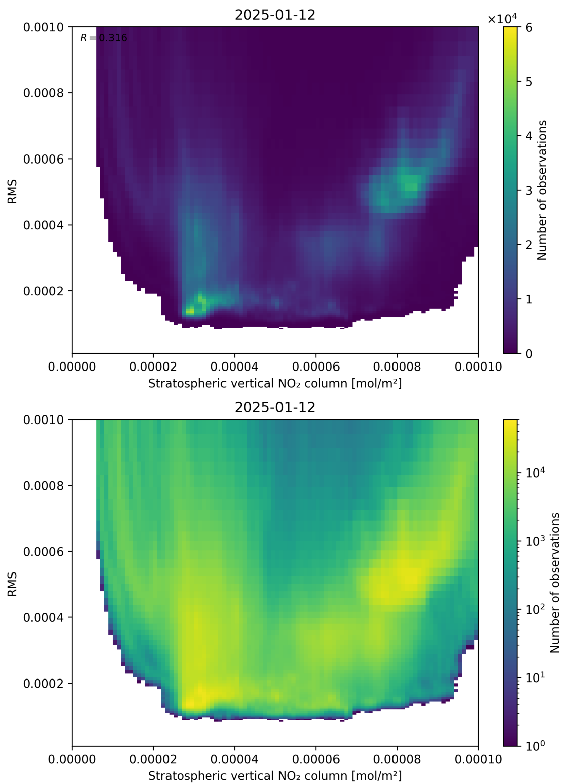
Figure 102: Scatter density plot of “Stratospheric vertical NO 2 column” against “RMS” for 2025-01-12 to 2025-01-13.
