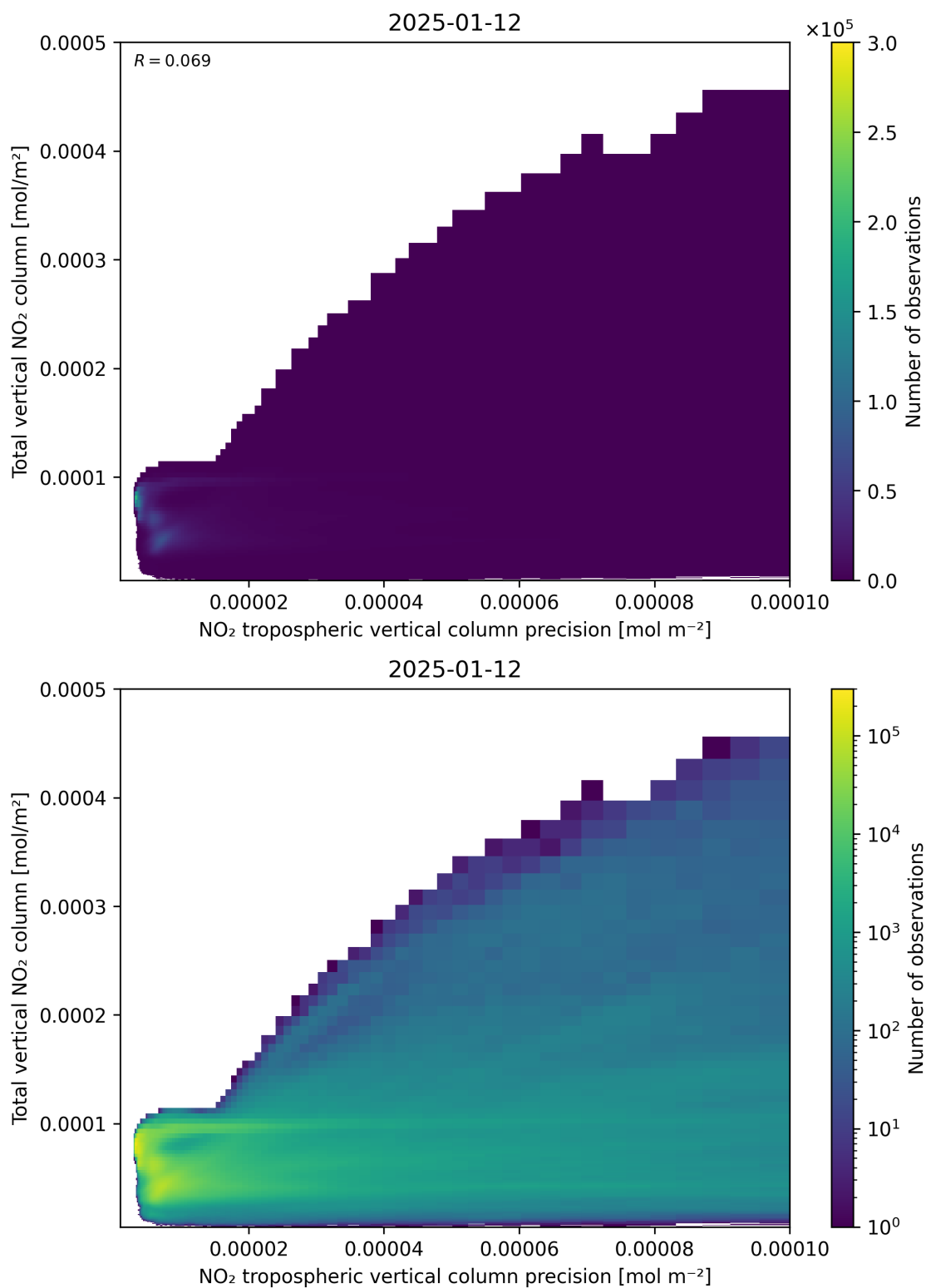
Figure 138: Scatter density plot of “NO 2 tropospheric vertical column precision” against “Total vertical NO 2 column” for 2025-01-12 to 2025-01-13.
