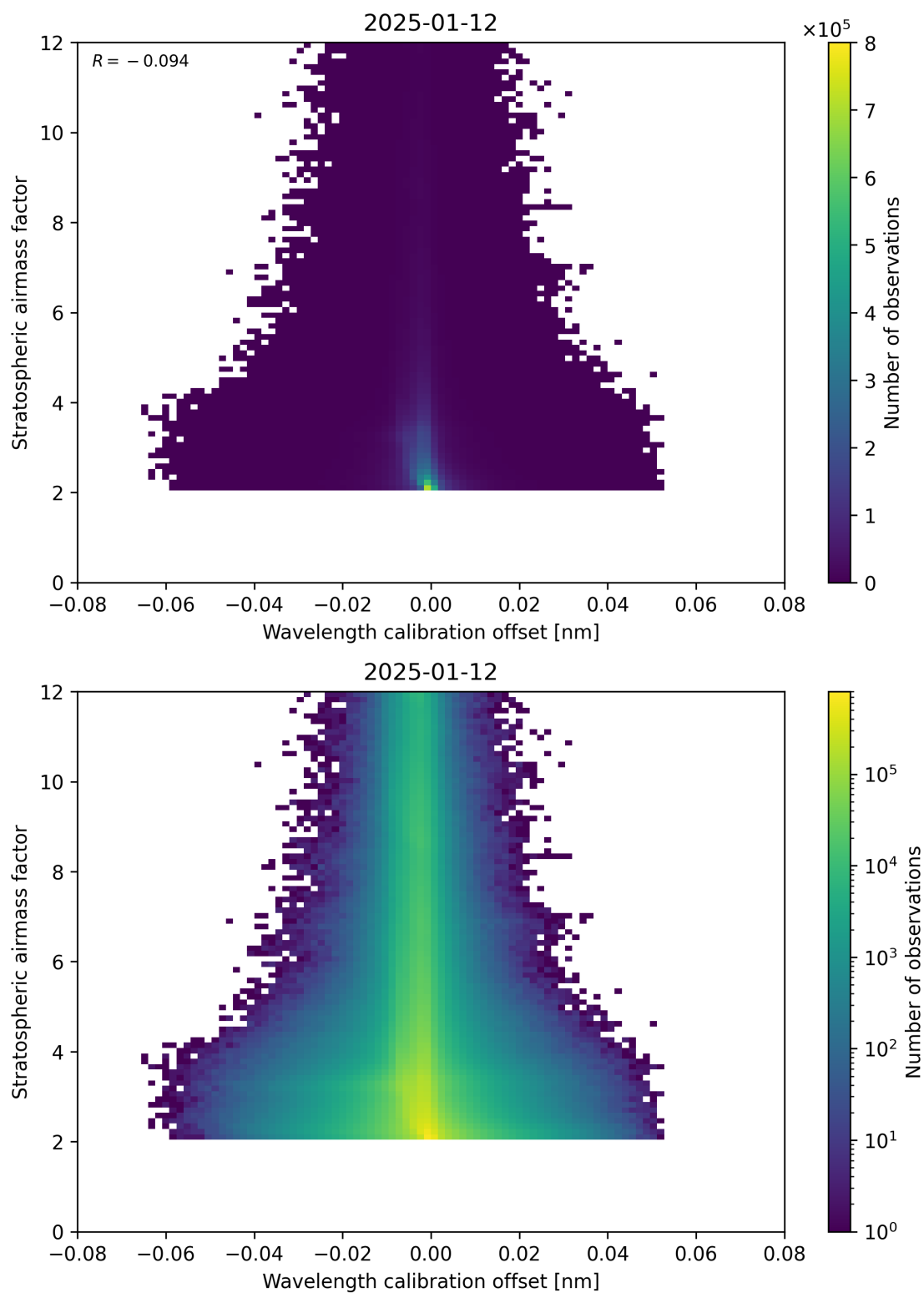
Figure 174: Scatter density plot of “Wavelength calibration offset” against “Stratospheric airmass factor” for 2025-01-12 to 2025-01-13.
