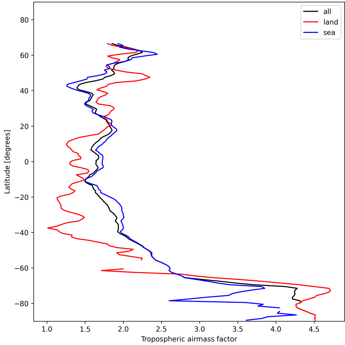
Figure 14: Zonal average of “Tropospheric airmass factor” for 2025-01-12 to 2025-01-13.
