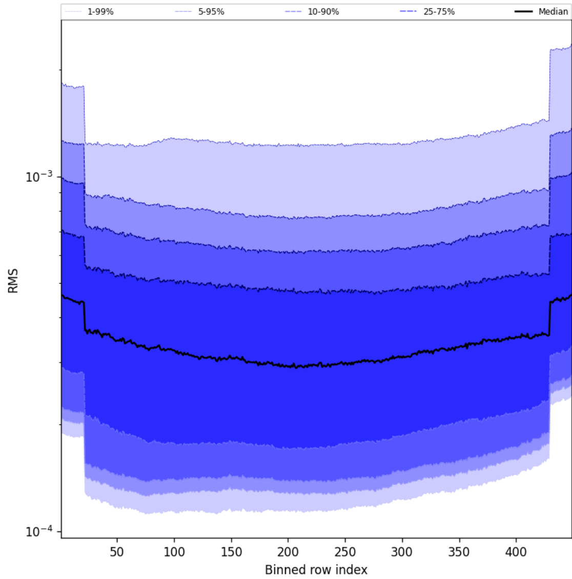
Figure 60: Along track statistics of “RMS” for 2025-01-12 to 2025-01-13
