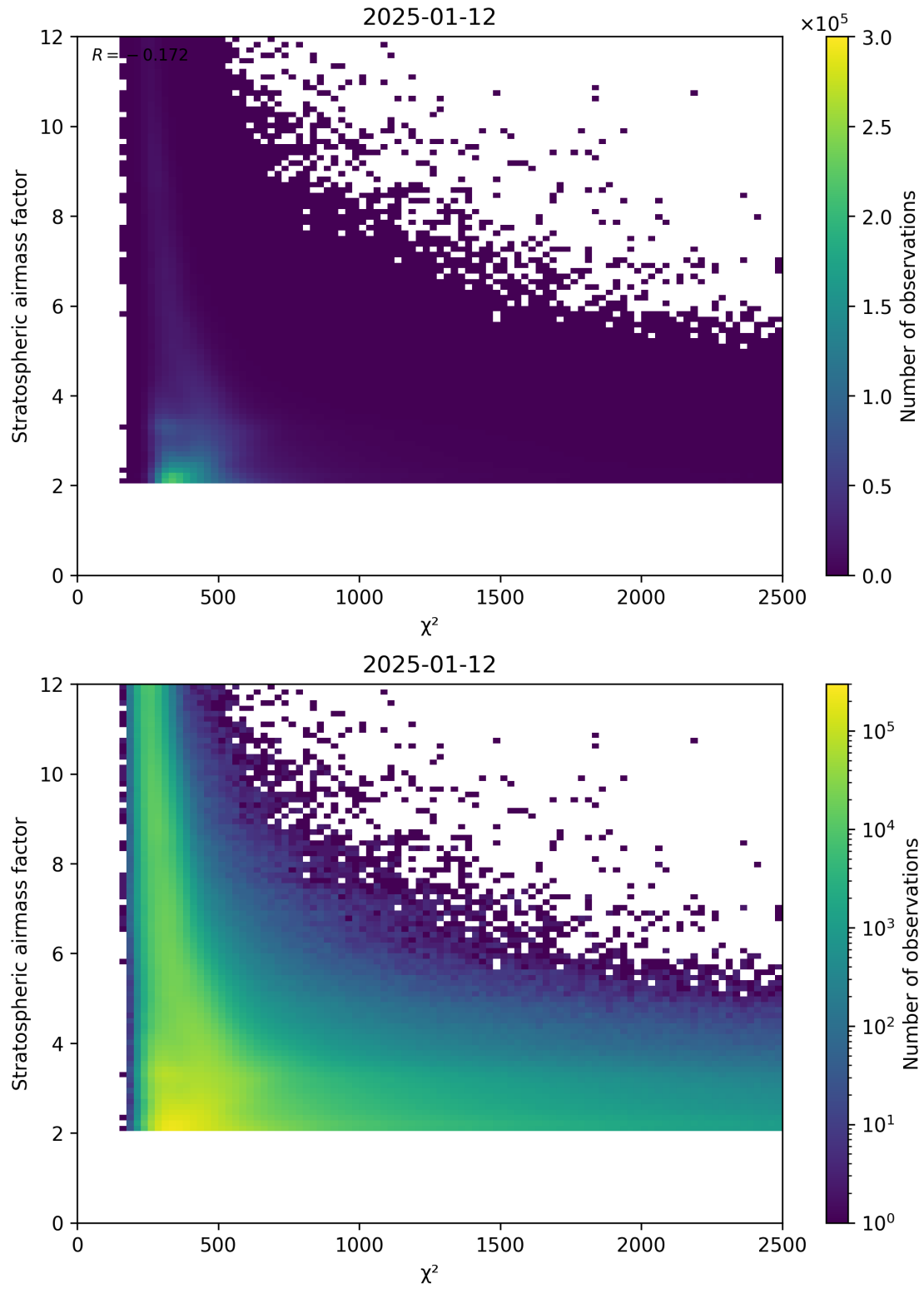
Figure 81: Scatter density plot of " \chi^2 " against "Stratospheric airmass factor" for 2025-01-12 to 2025-01-13.
