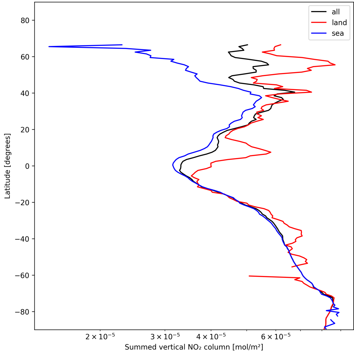
Figure 23: Zonal average of “Summed vertical NO 2 column” for 2025-01-12 to 2025-01-13.
