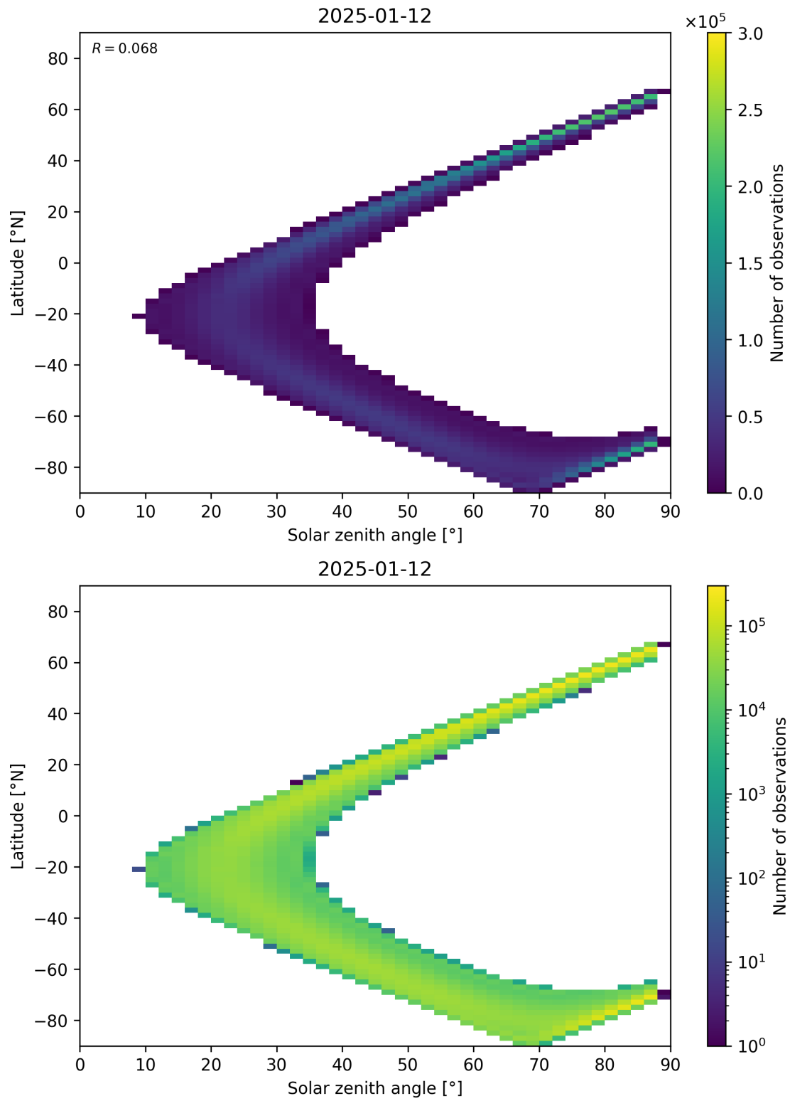
Figure 149: Scatter density plot of “Solar zenith angle” against “Latitude” for 2025-01-12 to 2025-01-13.
