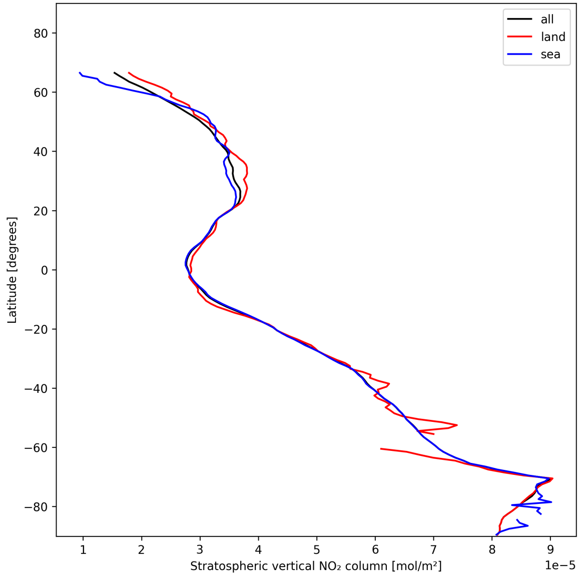
Figure 19: Zonal average of “Stratospheric vertical NO 2 column” for 2025-01-12 to 2025-01-13.
