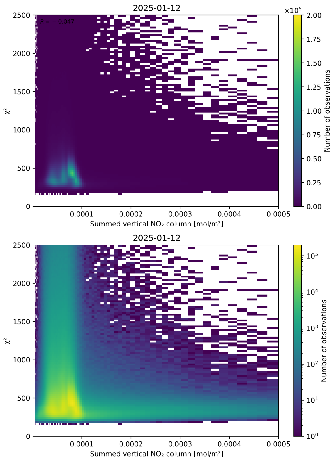
Figure 104: Scatter density plot of “Summed vertical NO 2 column” against “ \chi^2 ” for 2025-01-12 to 2025-01-13.
