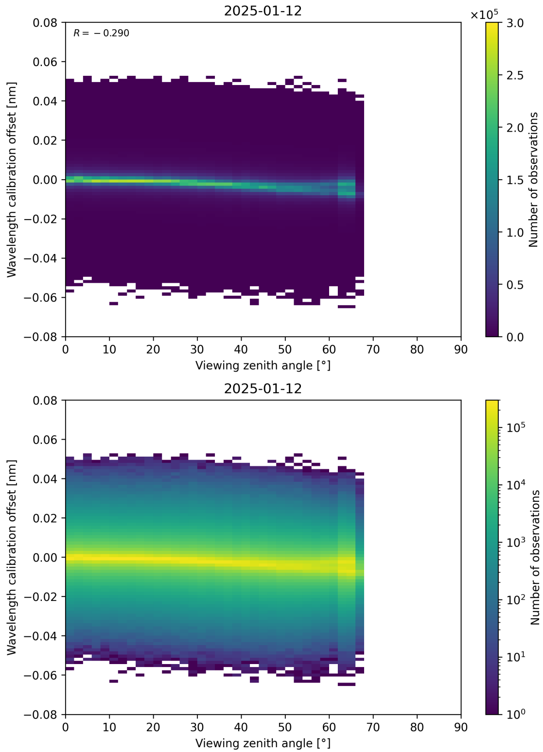
Figure 173: Scatter density plot of “Viewing zenith angle” against “Wavelength calibration offset” for 2025-01-12 to 2025-01-13.
