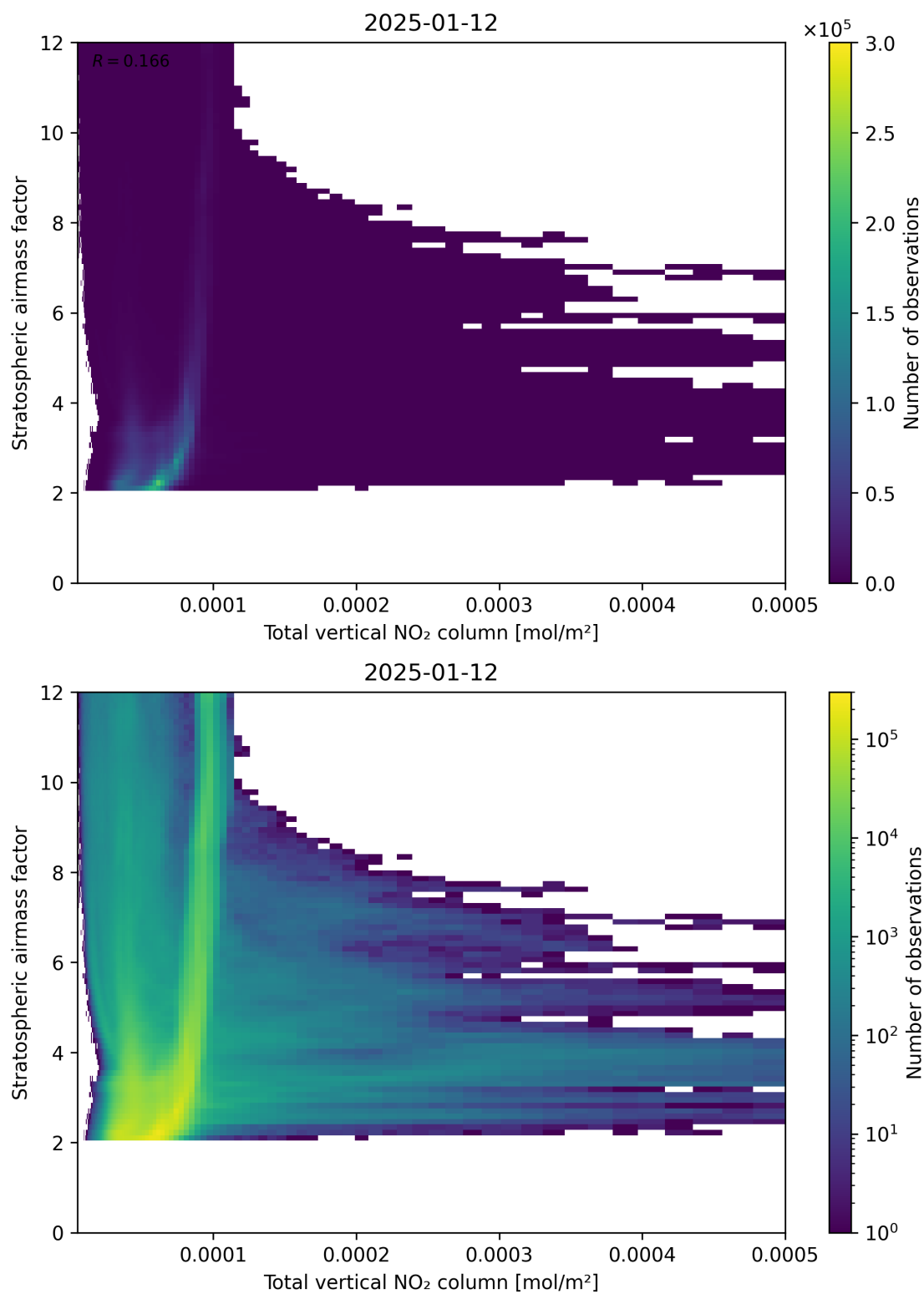
Figure 110: Scatter density plot of “Total vertical NO 2 column” against “Stratospheric airmass factor” for 2025-01-12 to 2025-01-13.
