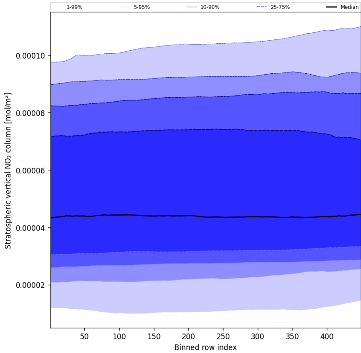
Figure 53: Along track statistics of “Stratospheric vertical NO 2 column” for 2025-01-12 to 2025-01-13
