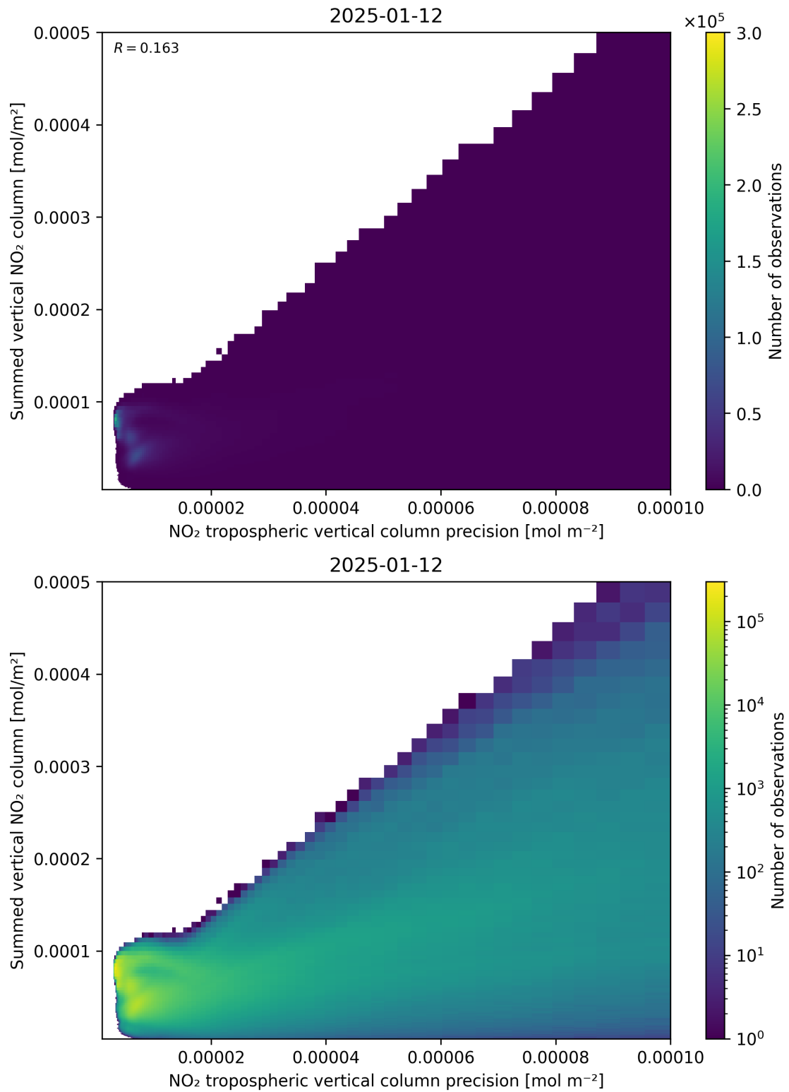
Figure 136: Scatter density plot of “NO 2 tropospheric vertical column precision” against “Summed vertical NO 2 column” for 2025-01-12 to 2025-01-13.
