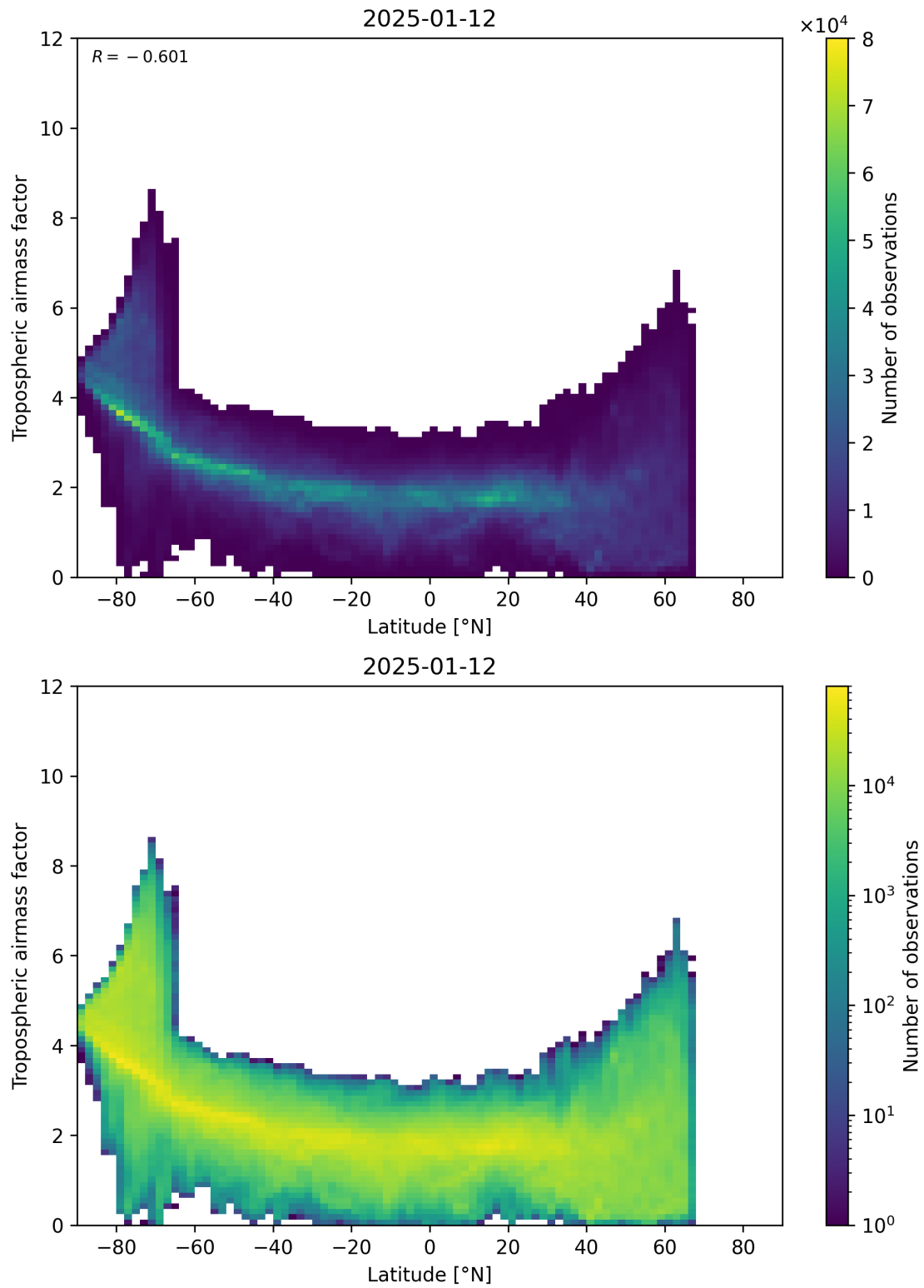
Figure 85: Scatter density plot of “Latitude” against “Tropospheric airmass factor” for 2025-01-12 to 2025-01-13.
