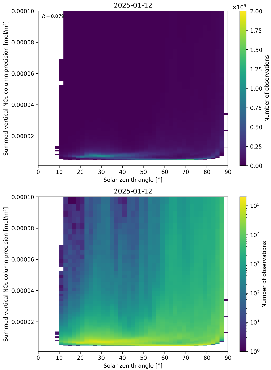
Figure 152: Scatter density plot of “Solar zenith angle” against “Summed vertical NO 2 column precision” for 2025-01-12 to 2025-01-13.
