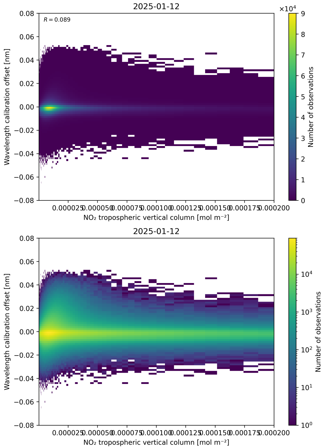
Figure 143: Scatter density plot of “NO 2 tropospheric vertical column” against “Wavelength calibration offset” for 2025-01-12 to 2025-01-13.
