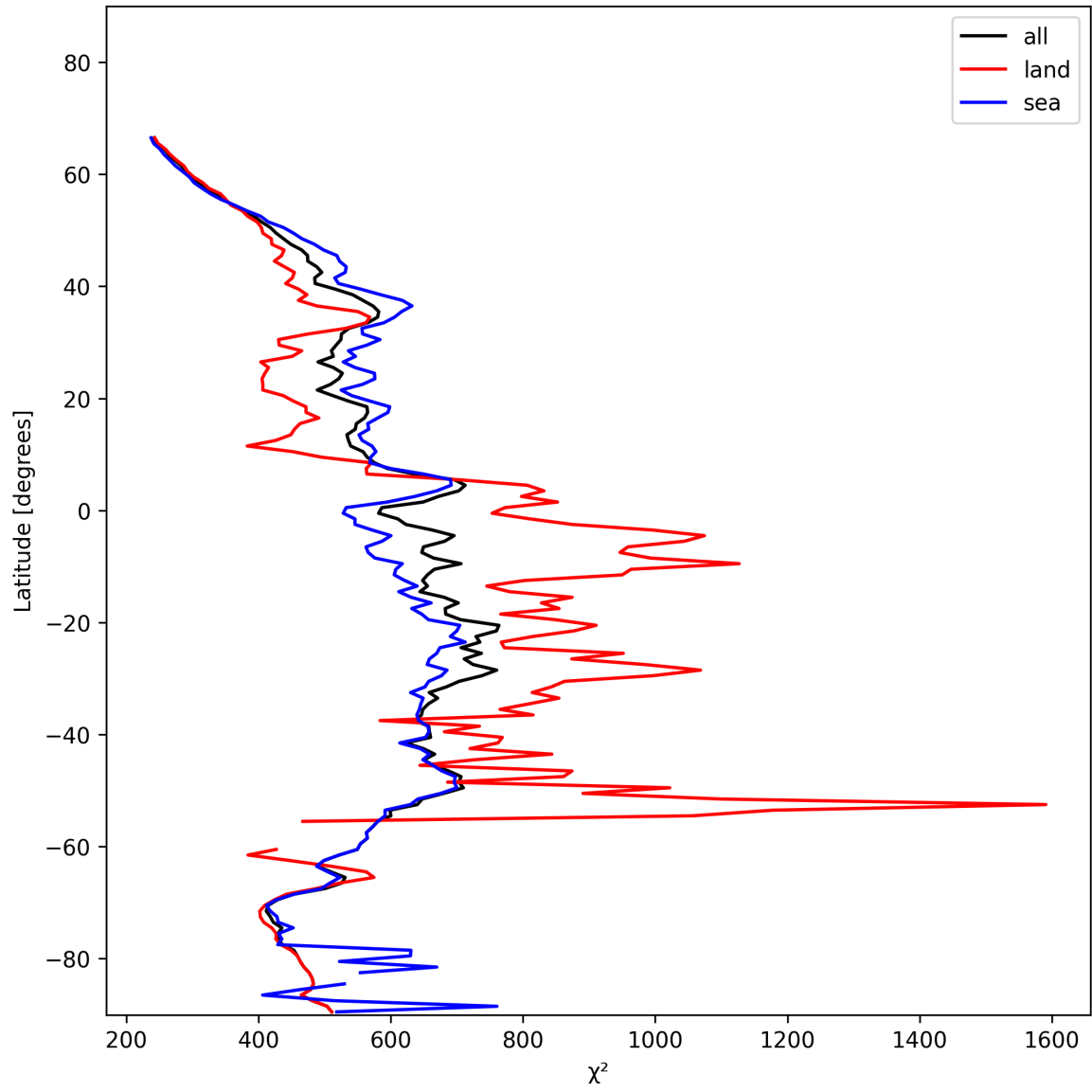
Figure 25: Zonal average of “ \chi^2 ” for 2025-01-12 to 2025-01-13.
