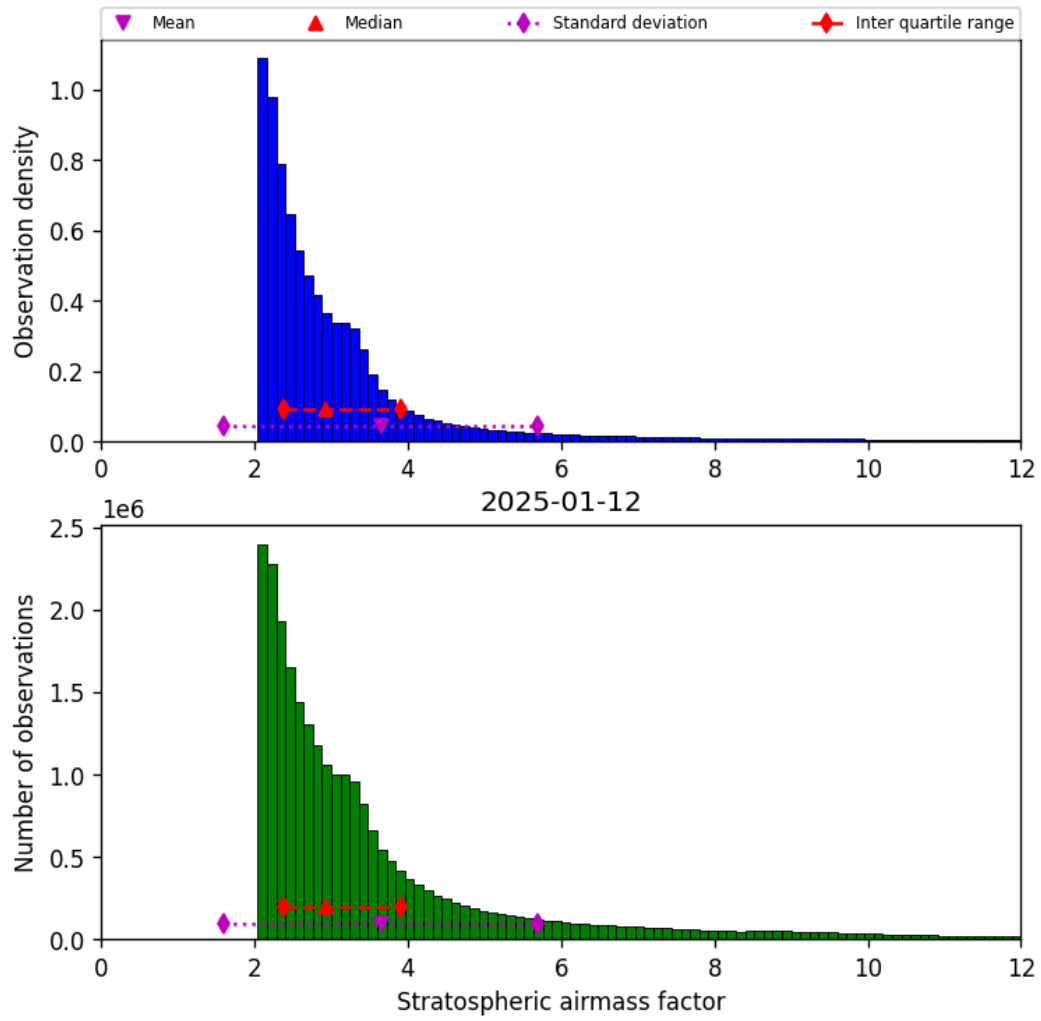
Figure 44: Histogram of “Stratospheric airmass factor” for 2025-01-12 to 2025-01-13
