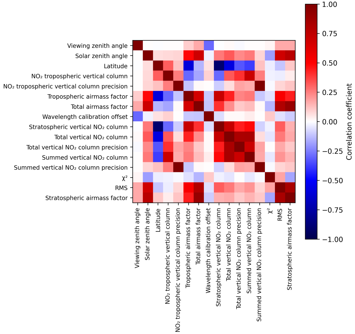
Figure 2: Map of correlation matrix for 2025-01-12 to 2025-01-13.
