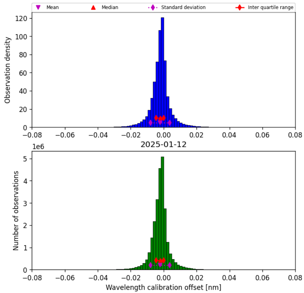
Figure 35: Histogram of “Wavelength calibration offset” for 2025-01-12 to 2025-01-13
