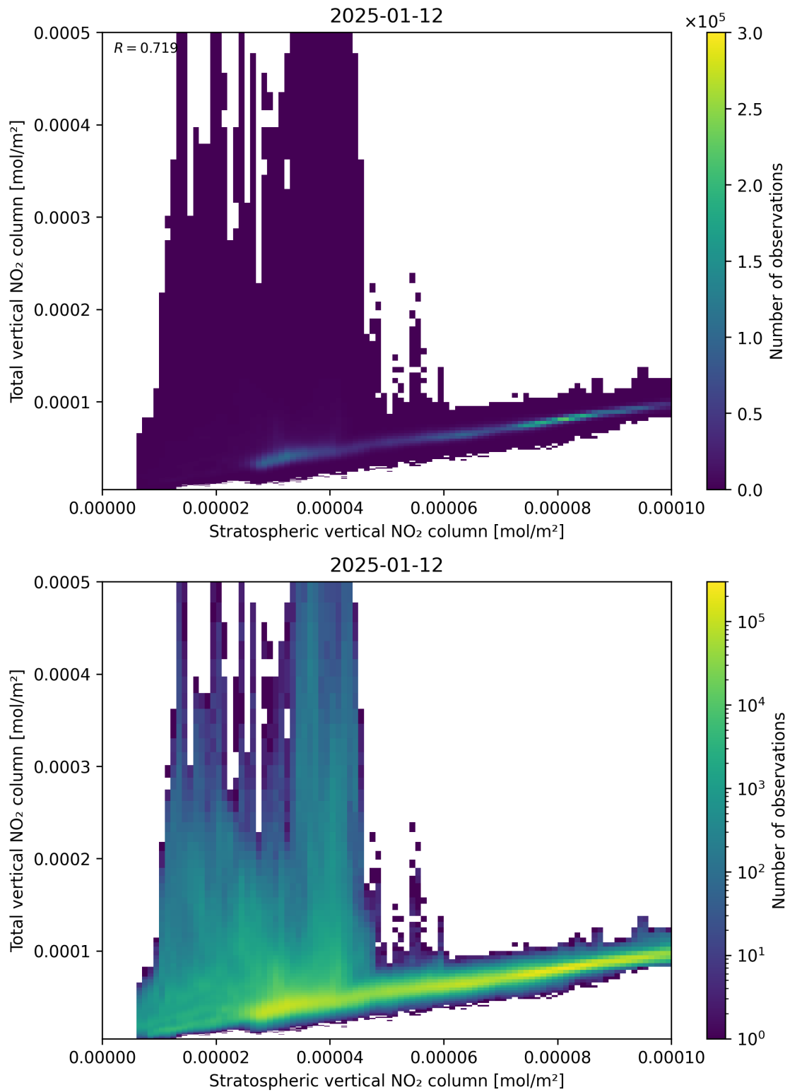
Figure 100: Scatter density plot of “Stratospheric vertical NO 2 column” against “Total vertical NO 2 column” for 2025-01-12 to 2025-01-13.
