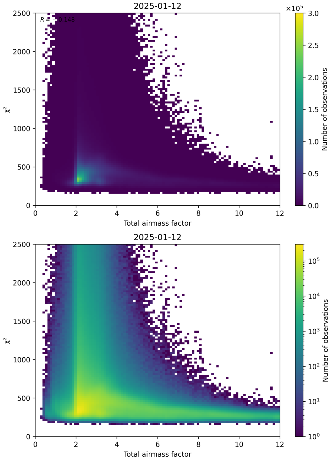
Figure 63: Scatter density plot of “Total airmass factor” against “ \chi^2 ” for 2025-01-12 to 2025-01-13.
