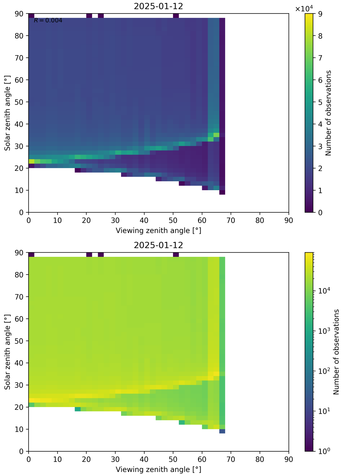
Figure 172: Scatter density plot of “Viewing zenith angle” against “Solar zenith angle” for 2025-01-12 to 2025-01-13.
