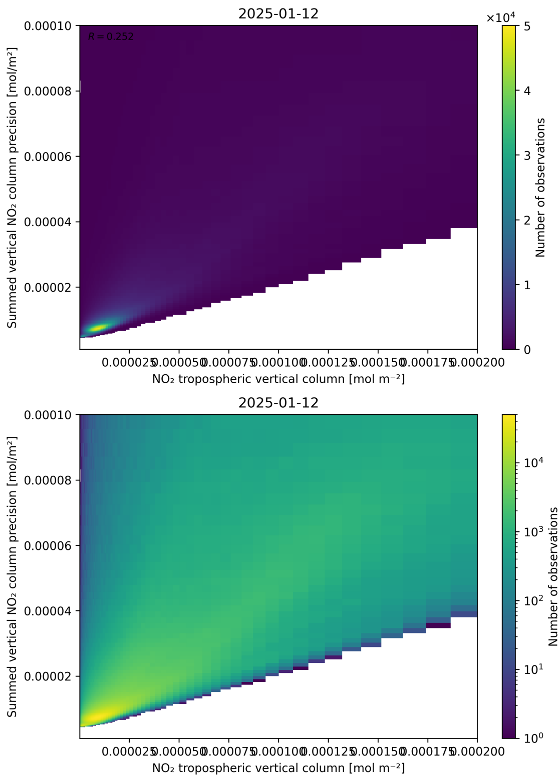
Figure 127: Scatter density plot of “NO 2 tropospheric vertical column” against “Summed vertical NO 2 column precision” for 2025-01-12 to 2025-01-13.
