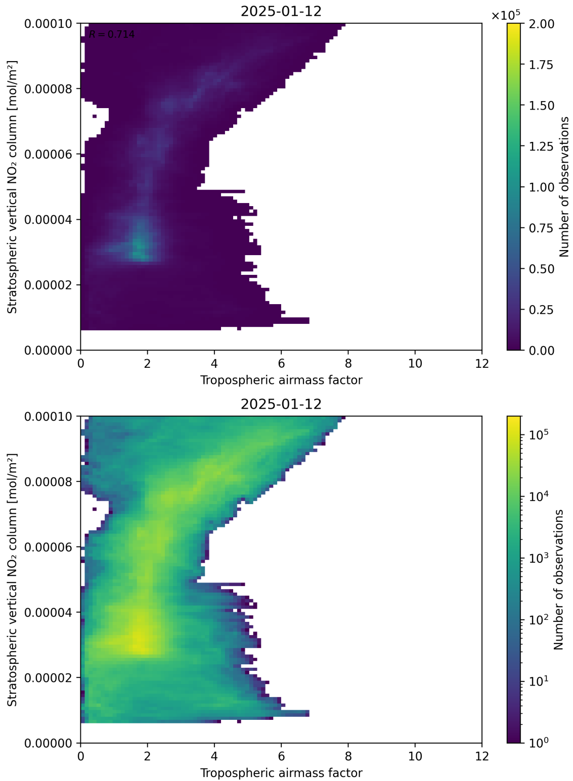
Figure 74: Scatter density plot of “Tropospheric air mass factor” against “Stratospheric vertical NO 2 column” for 2025-01-12 to 2025-01-13.
