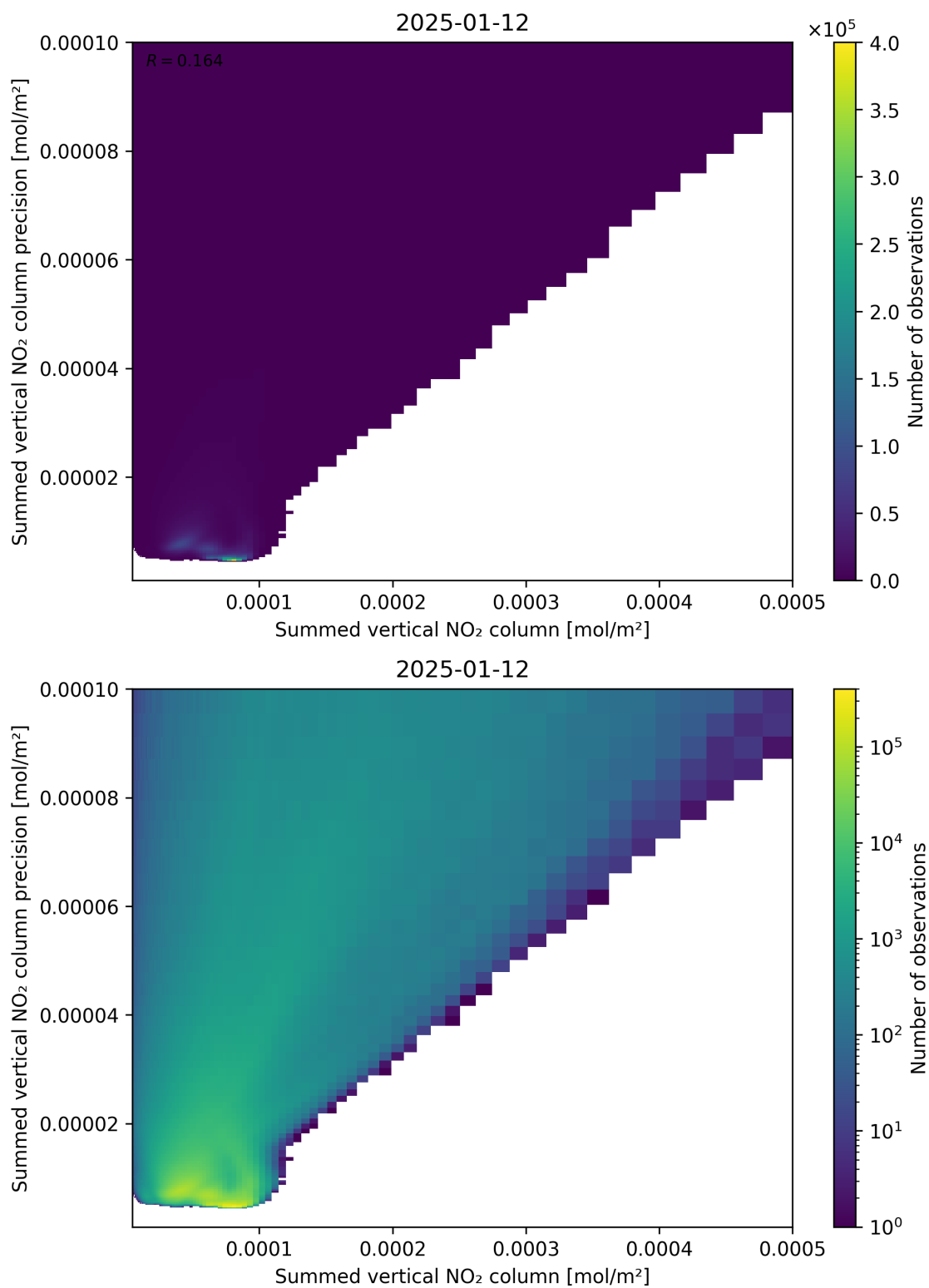
Figure 105: Scatter density plot of “Summed vertical NO 2 column” against “Summed vertical NO 2 column precision” for 2025-01-12 to 2025-01-13.
