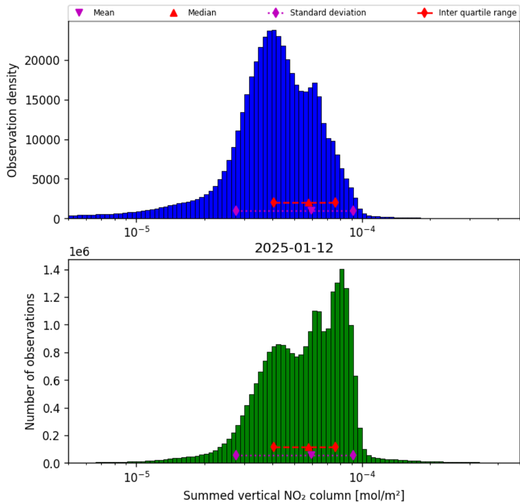
Figure 40: Histogram of “Summed vertical NO 2 column” for 2025-01-12 to 2025-01-13
