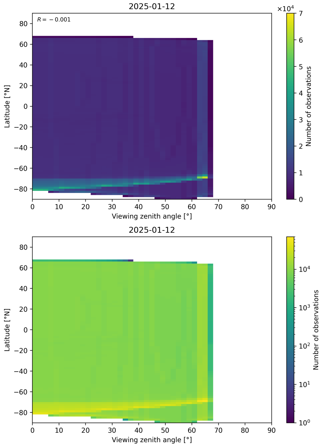
Figure 163: Scatter density plot of “Viewing zenith angle” against “Latitude” for 2025-01-12 to 2025-01-13.
