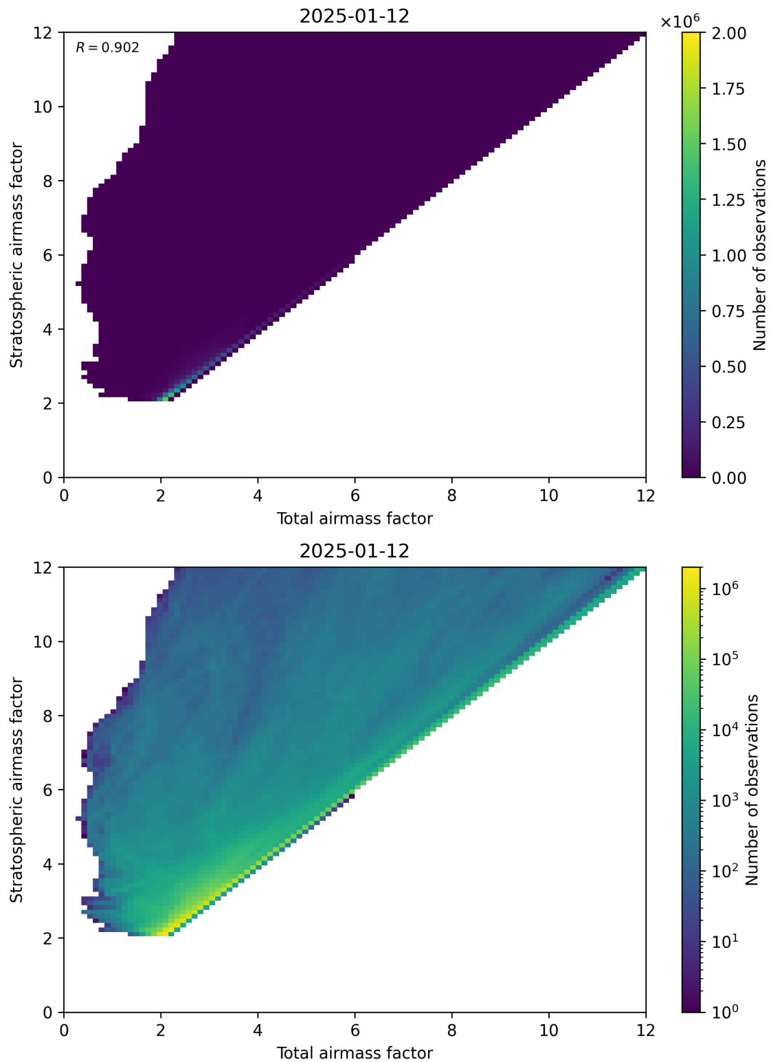
Figure 62: Scatter density plot of “Total airmass factor” against “Stratospheric airmass factor” for 2025-01-12 to 2025-01-13.
