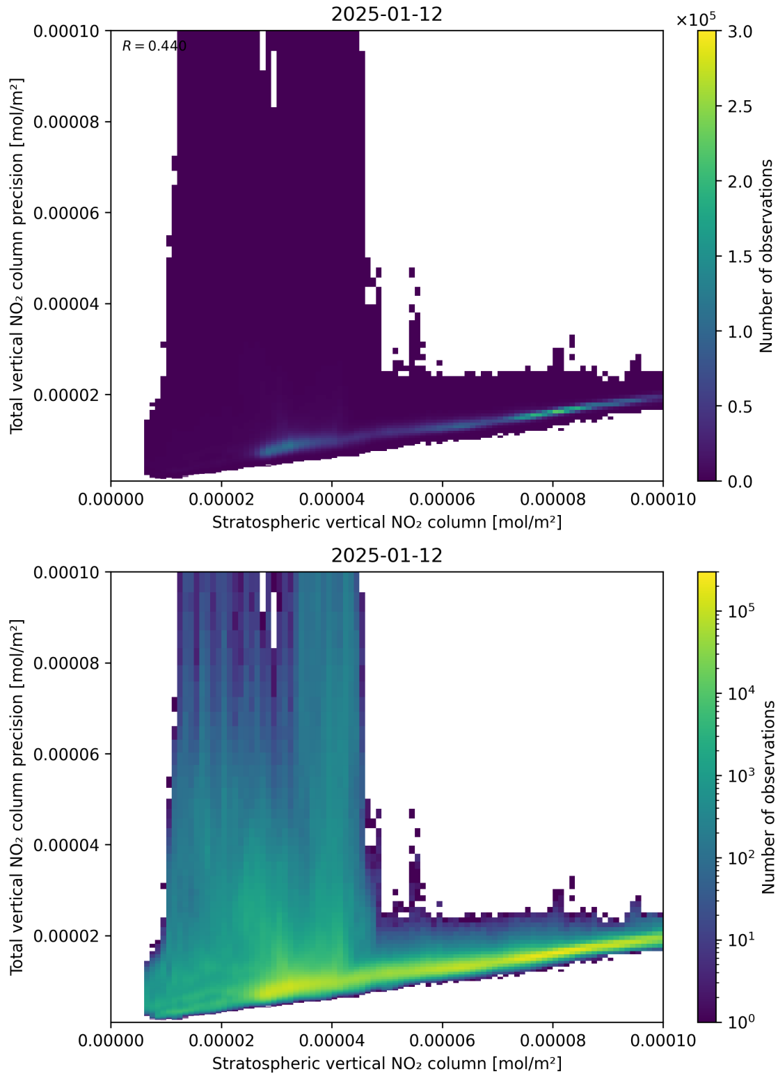
Figure 101: Scatter density plot of “Stratospheric vertical NO 2 column” against “Total vertical NO 2 column precision” for 2025-01-12 to 2025-01-13.
