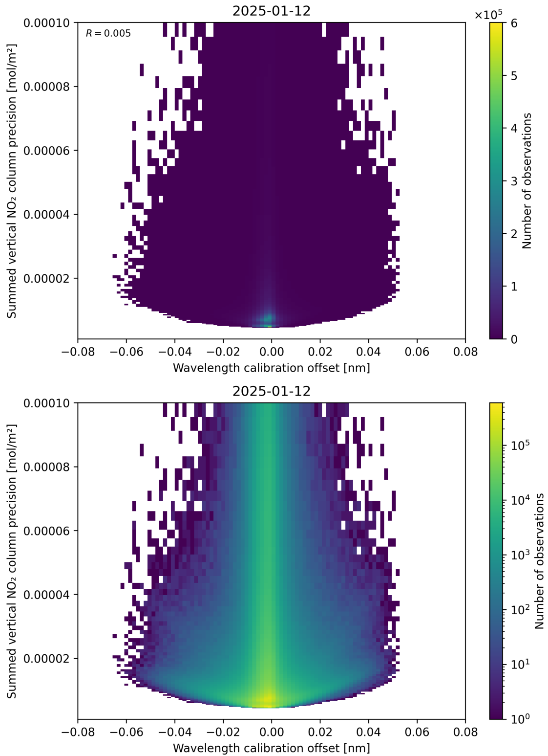
Figure 178: Scatter density plot of “Wavelength calibration offset” against “Summed vertical NO 2 column precision” for 2025-01-12 to 2025-01-13.
