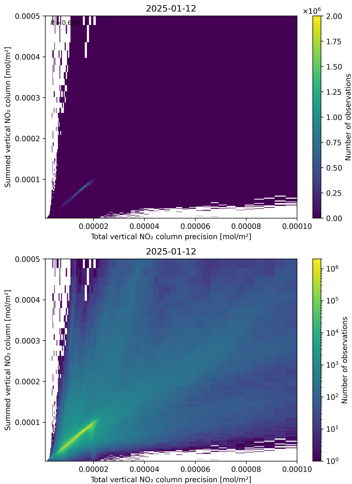
Figure 117: Scatter density plot of “Total vertical NO 2 column precision” against “Summed vertical NO 2 column” for 2025-01-12 to 2025-01-13.
