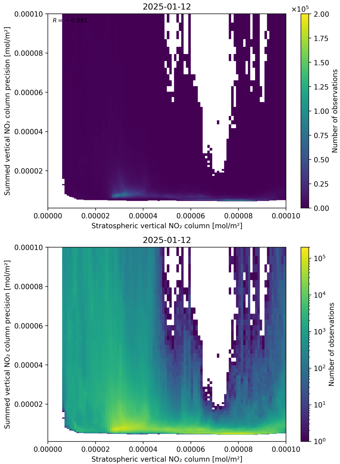
Figure 99: Scatter density plot of “Stratospheric vertical NO 2 column” against “Summed vertical NO 2 column precision” for 2025-01-12 to 2025-01-13.
