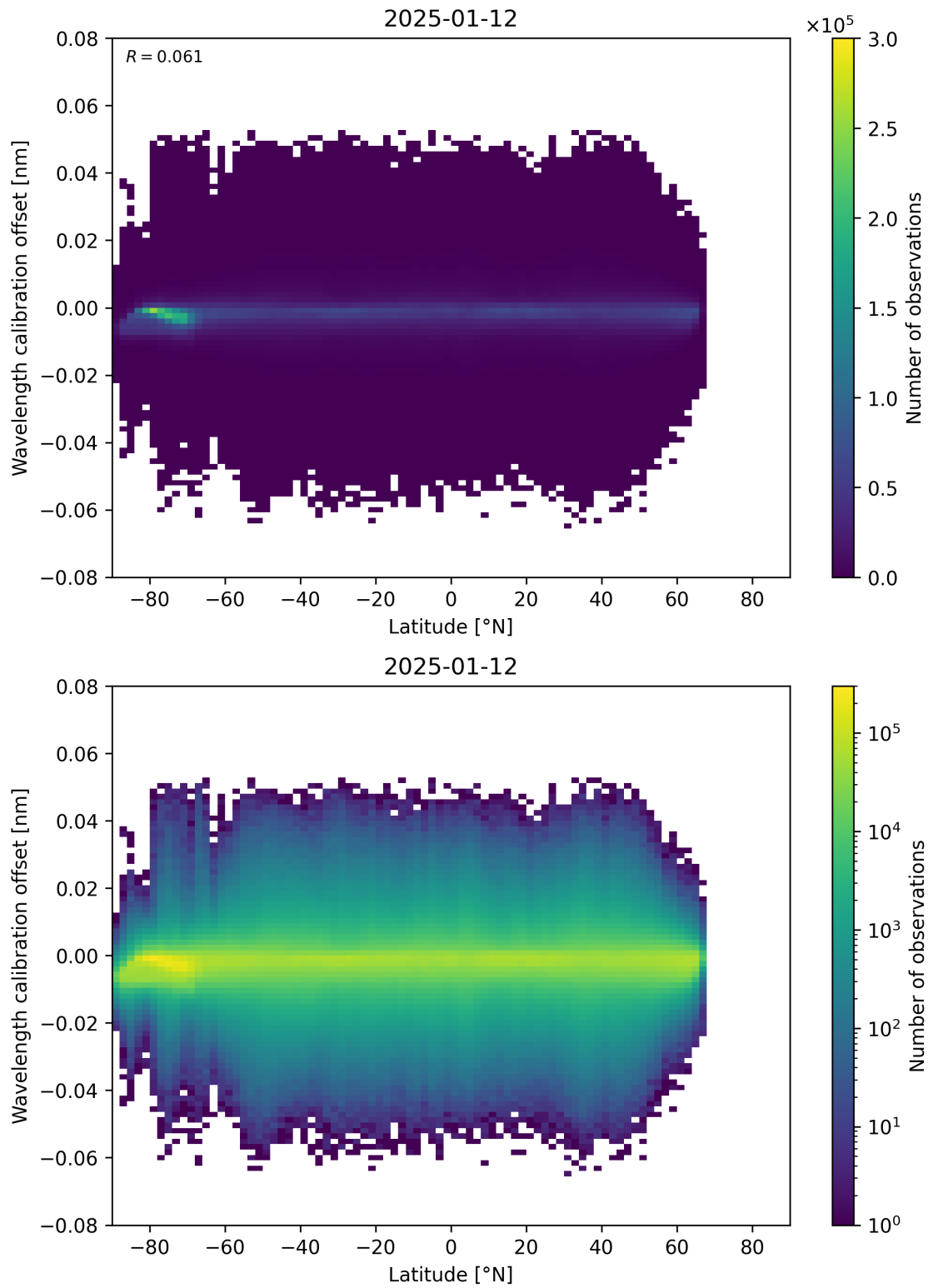
Figure 95: Scatter density plot of “Latitude” against “Wavelength calibration offset” for 2025-01-12 to 2025-01-13.
