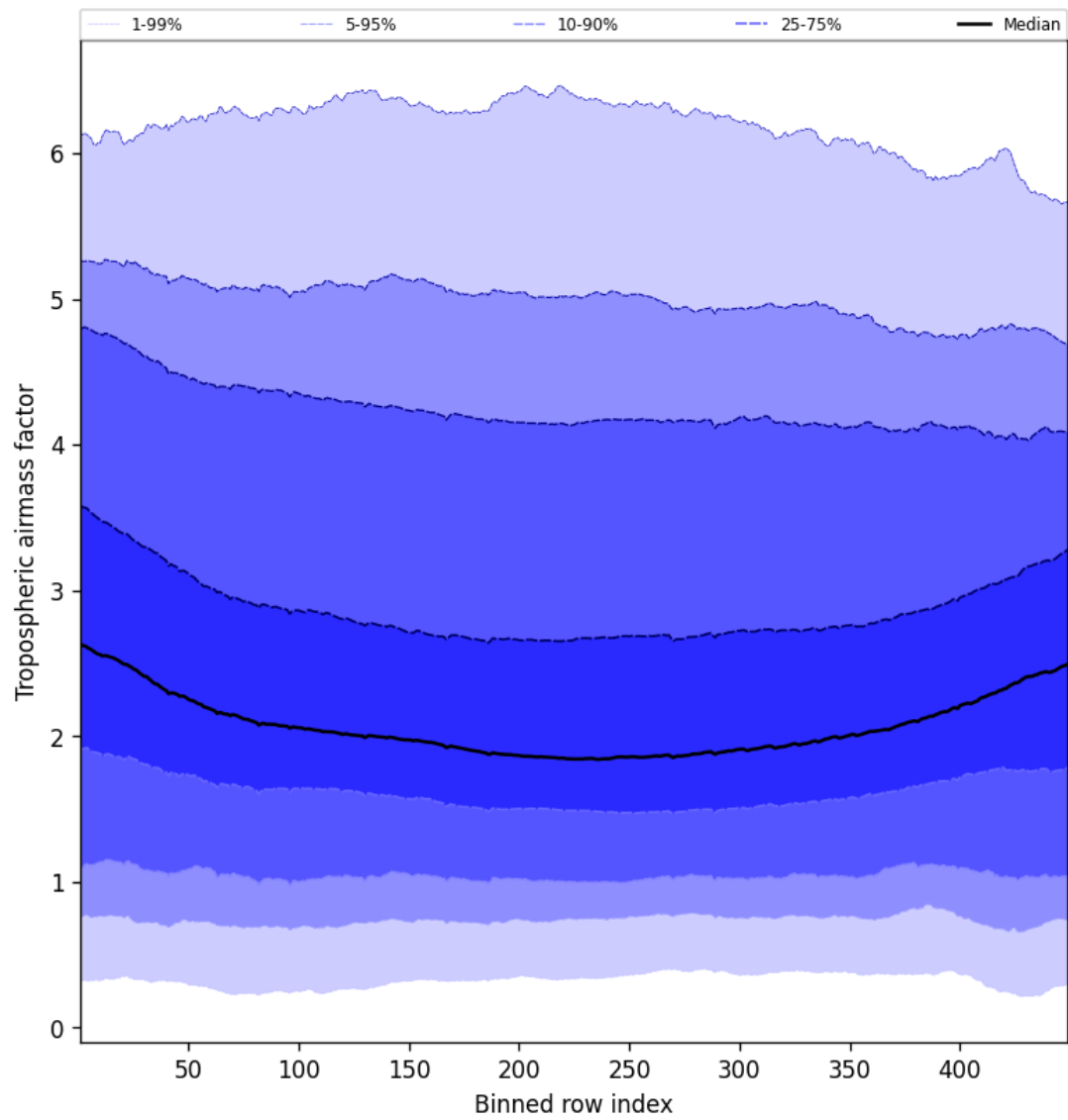
Figure 48: Along track statistics of “Tropospheric airmass factor” for 2025-01-12 to 2025-01-13
