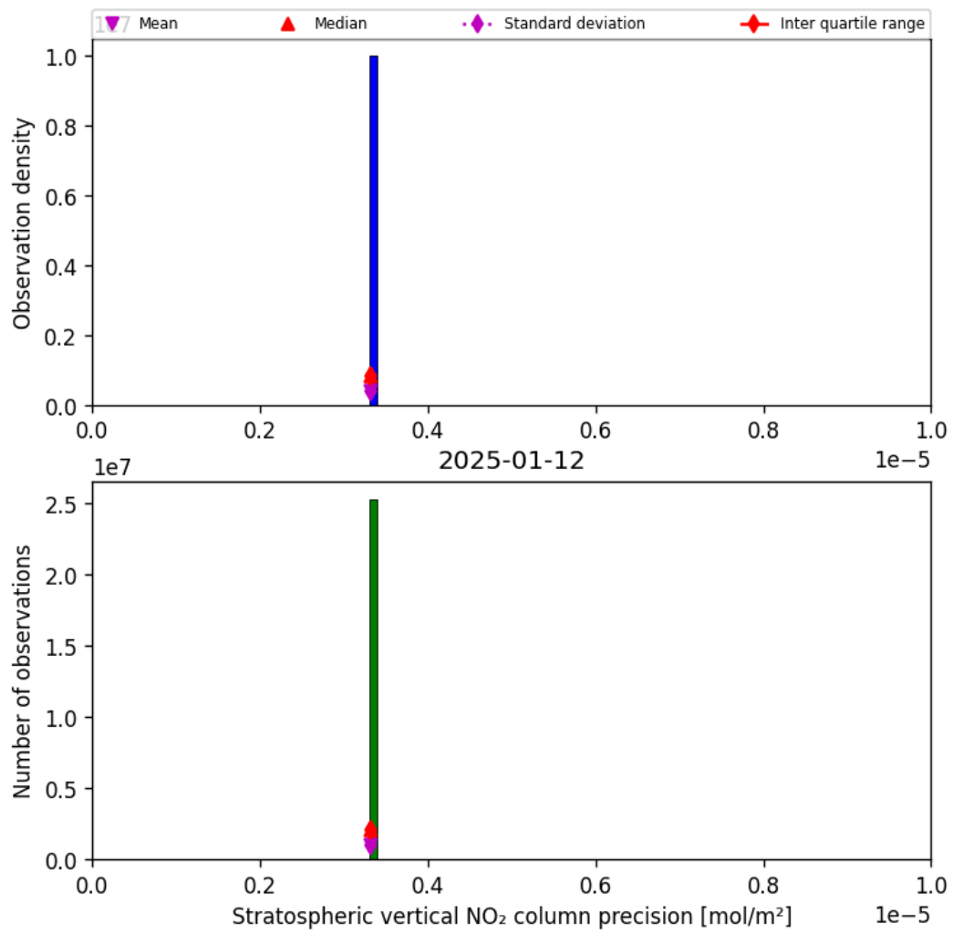
Figure 37: Histogram of “Stratospheric vertical NO 2 column precision” for 2025-01-12 to 2025-01-13
