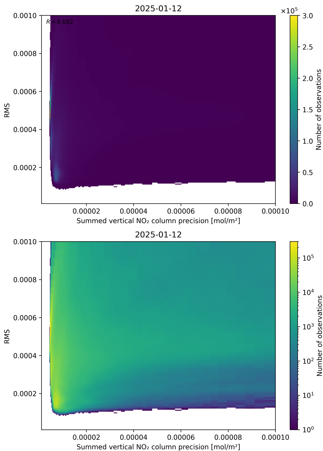
Figure 108: Scatter density plot of “Summed vertical NO 2 column precision” against “RMS” for 2025-01-12 to 2025-01-13.
