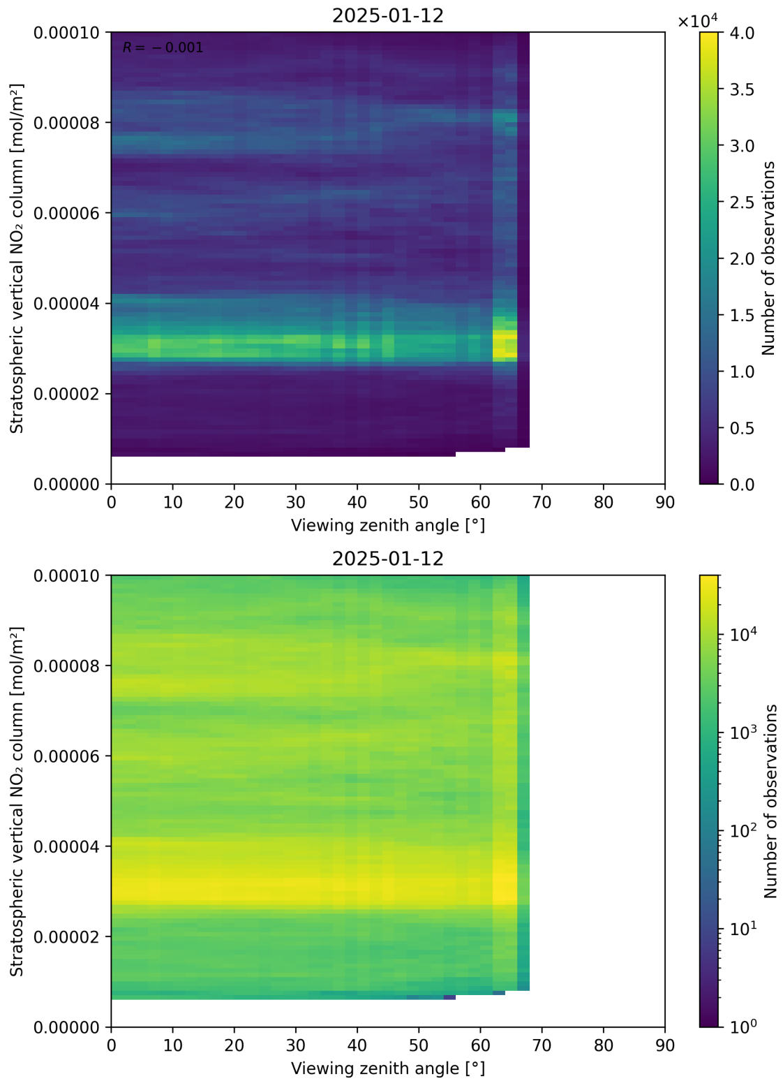
Figure 164: Scatter density plot of “Viewing zenith angle” against “Stratospheric vertical NO 2 column” for 2025-01-12 to 2025-01-13.
