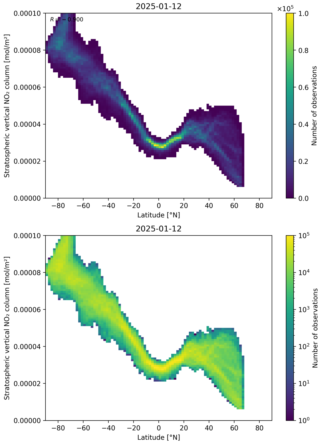
Figure 87: Scatter density plot of “Latitude” against “Stratospheric vertical NO 2 column” for 2025-01-12 to 2025-01-13.
