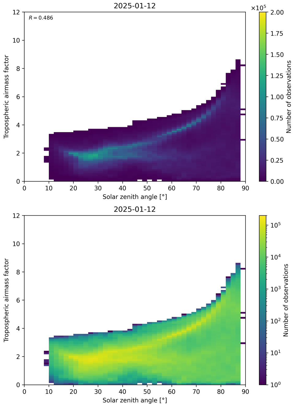
Figure 147: Scatter density plot of “Solar zenith angle” against “Tropospheric airmass factor” for 2025-01-12 to 2025-01-13.
