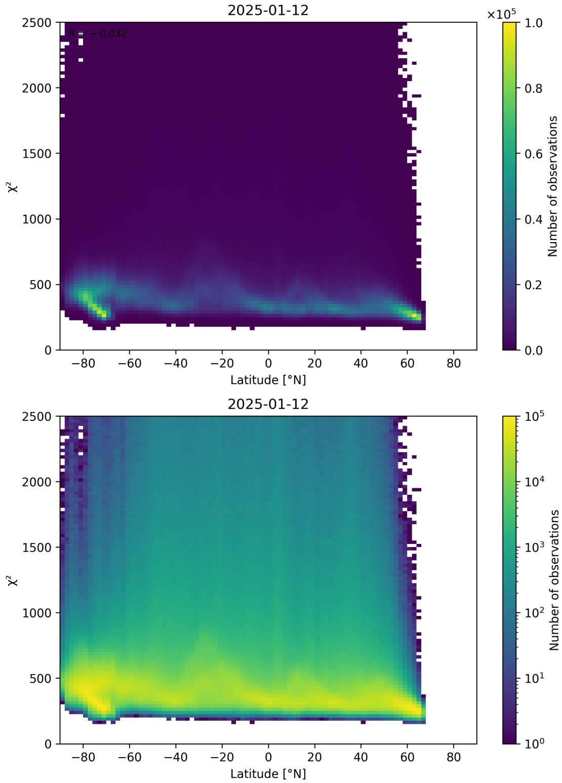
Figure 86: Scatter density plot of “Latitude” against “ \chi^2 ” for 2025-01-12 to 2025-01-13.
