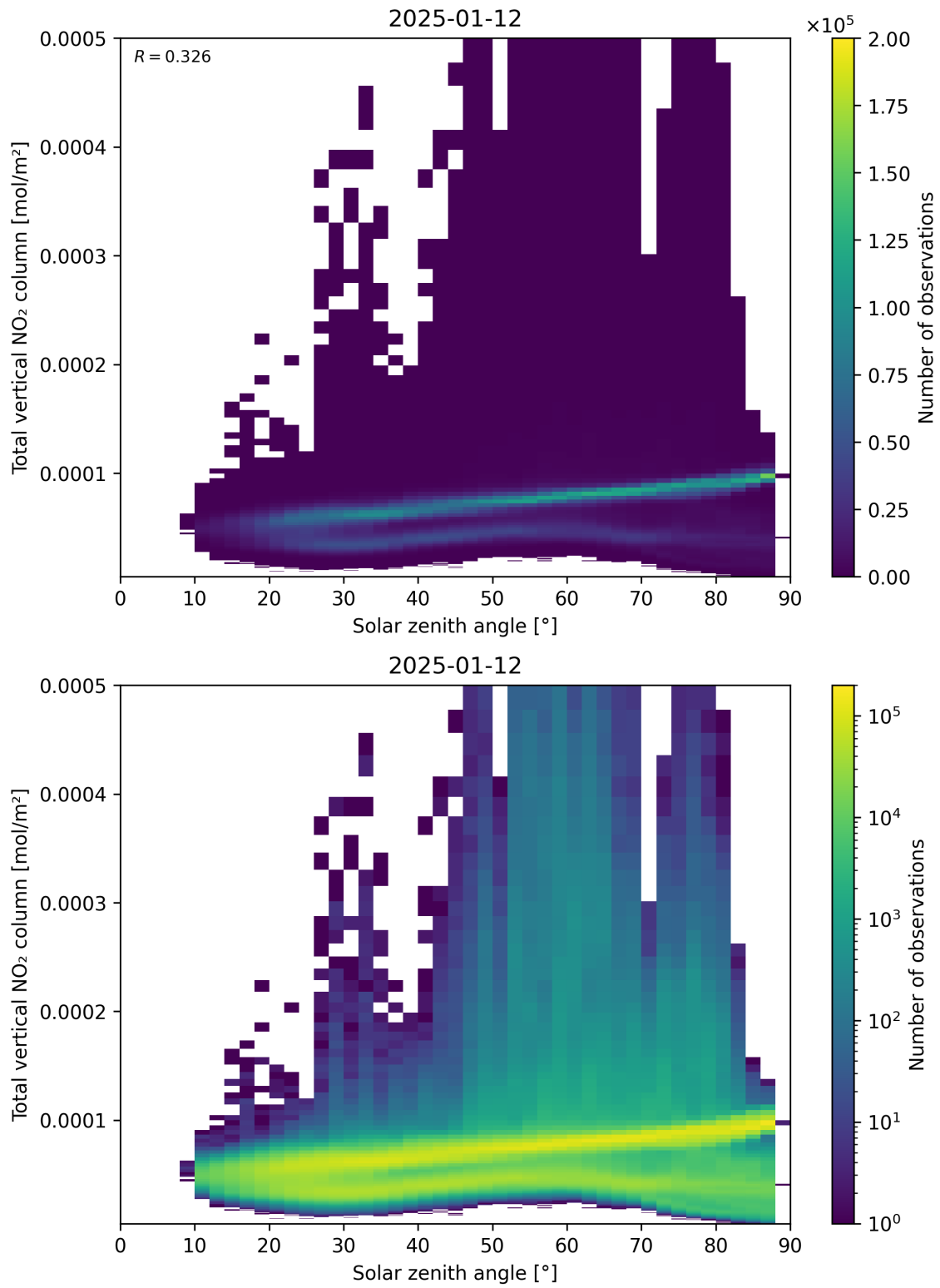
Figure 153: Scatter density plot of “Solar zenith angle” against “Total vertical NO 2 column” for 2025-01-12 to 2025-01-13.
