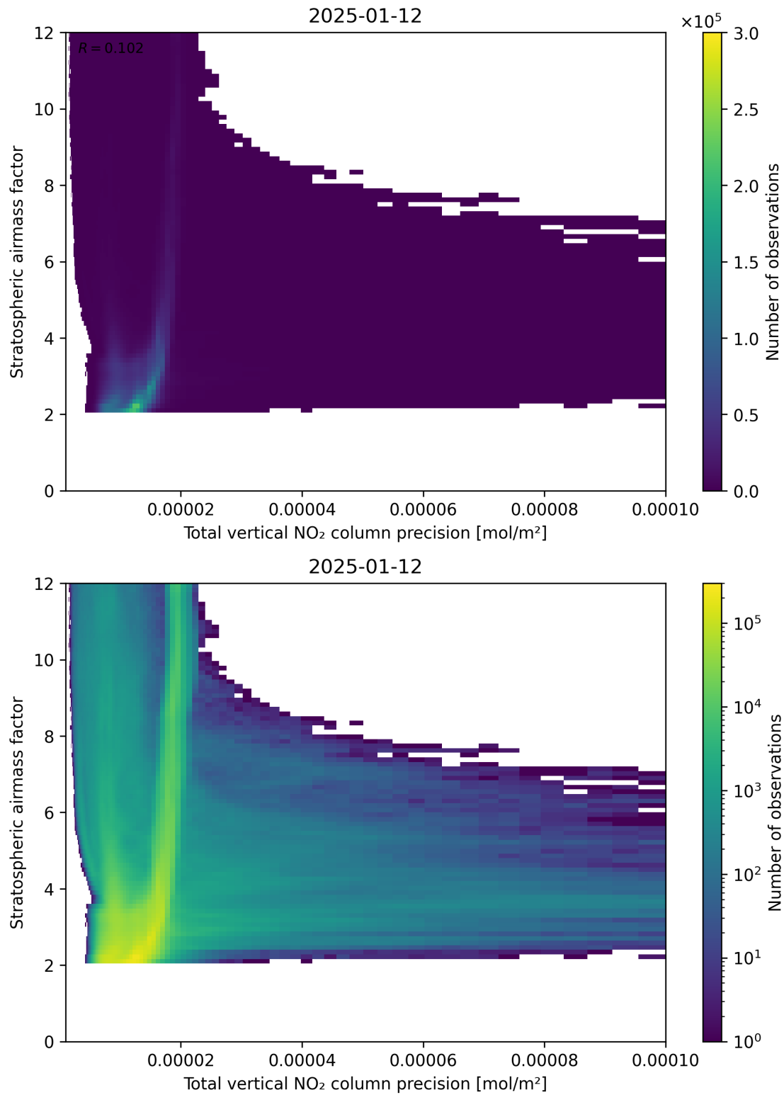
Figure 115: Scatter density plot of “Total vertical NO 2 column precision” against “Stratospheric air mass factor” for 2025-01-12 to 2025-01-13.
