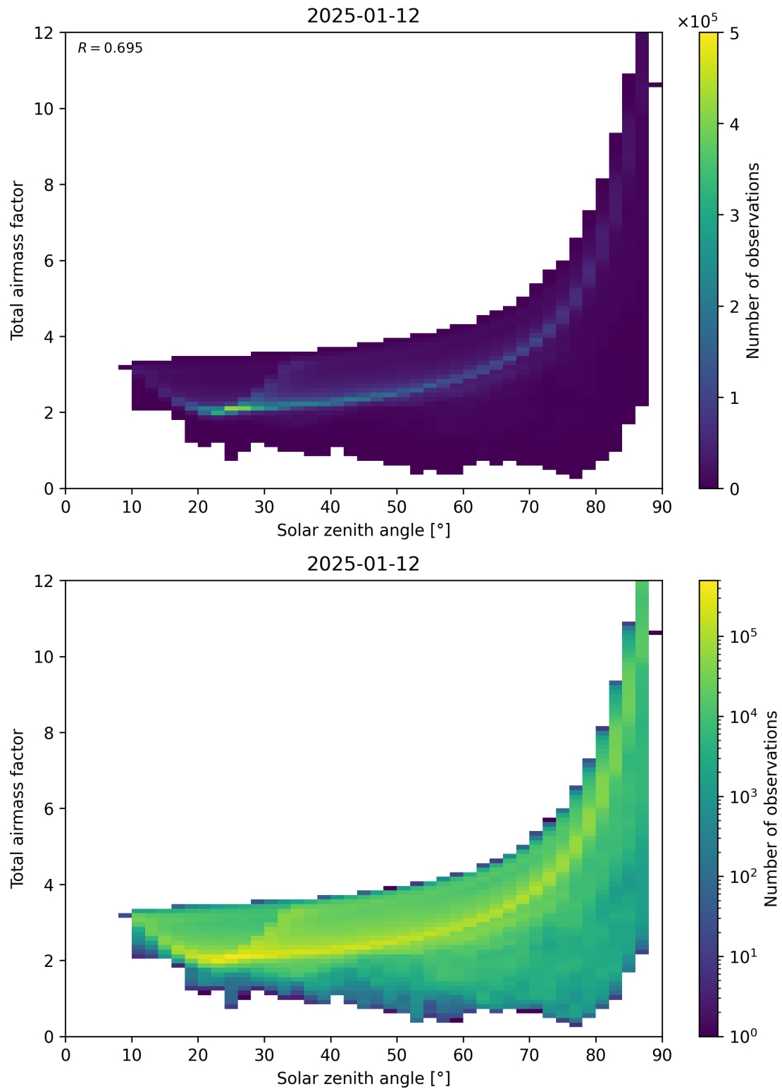
Figure 146: Scatter density plot of “Solar zenith angle” against “Total air mass factor” for 2025-01-12 to 2025-01-13.
