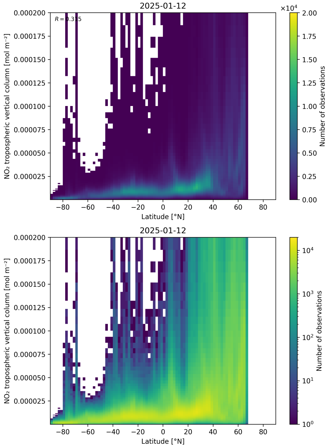
Figure 92: Scatter density plot of “Latitude” against “NO 2 tropospheric vertical column” for 2025-01-12 to 2025-01-13.
