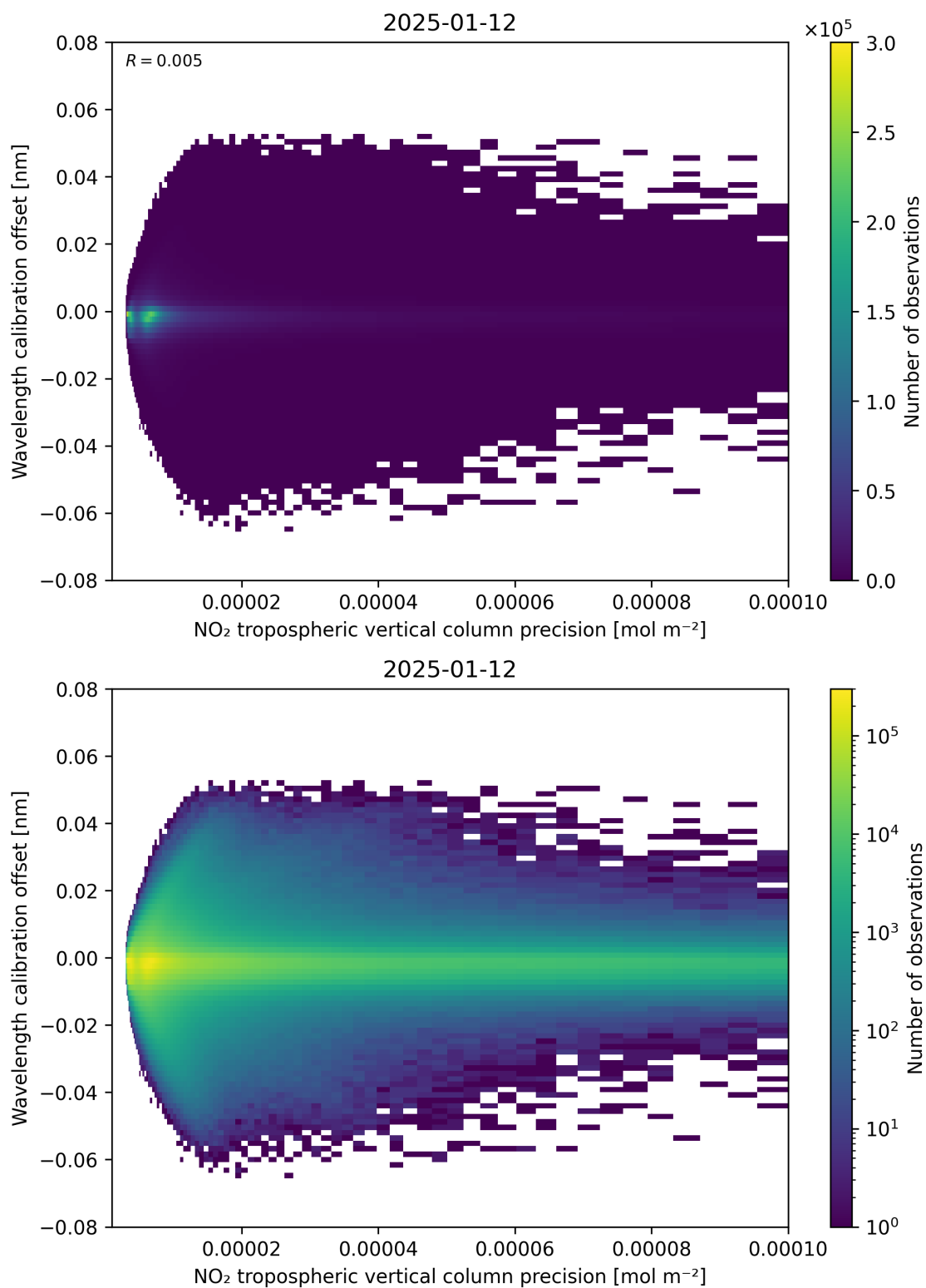
Figure 141: Scatter density plot of “NO 2 tropospheric vertical column precision” against “Wavelength calibration offset” for 2025-01-12 to 2025-01-13.
