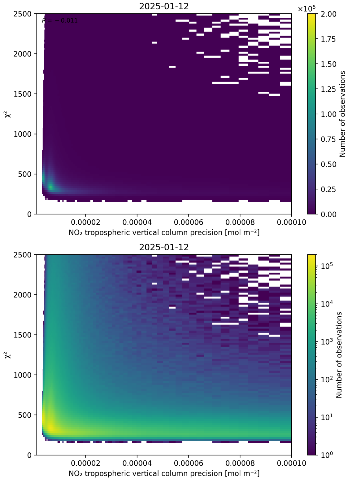
Figure 134: Scatter density plot of “NO 2 tropospheric vertical column precision” against “ \chi^2 ” for 2025-01-12 to 2025-01-13.
