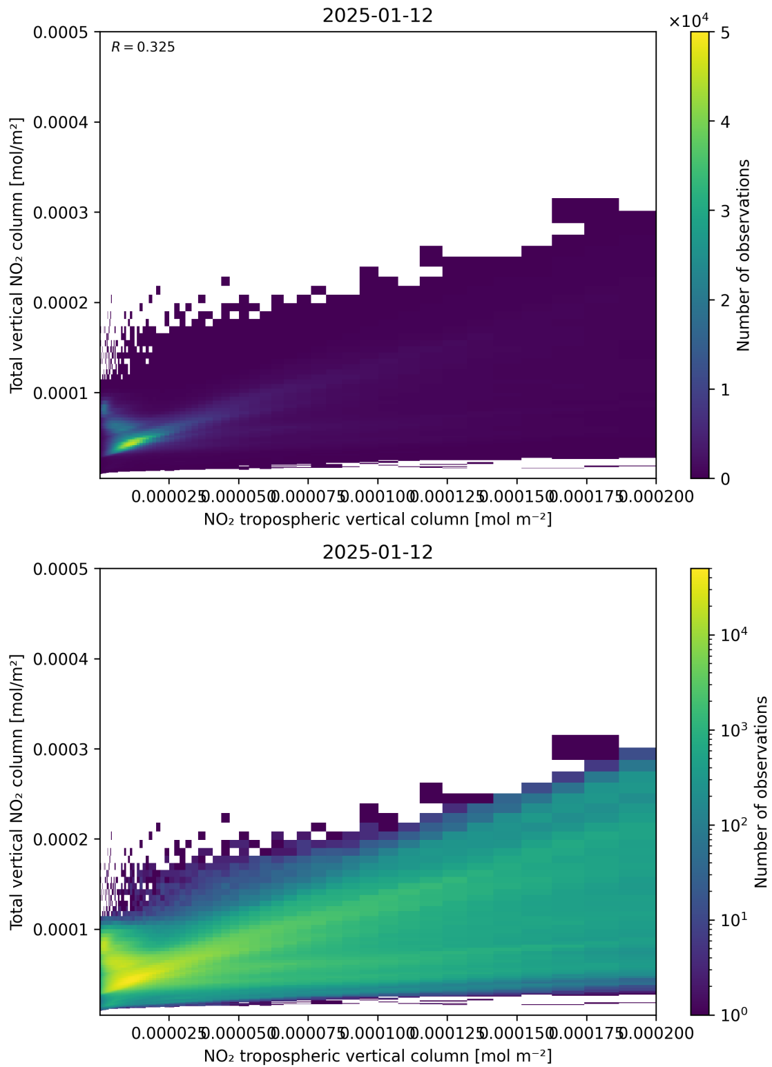
Figure 128: Scatter density plot of “NO 2 tropospheric vertical column” against “Total vertical NO 2 column” for 2025-01-12 to 2025-01-13.
