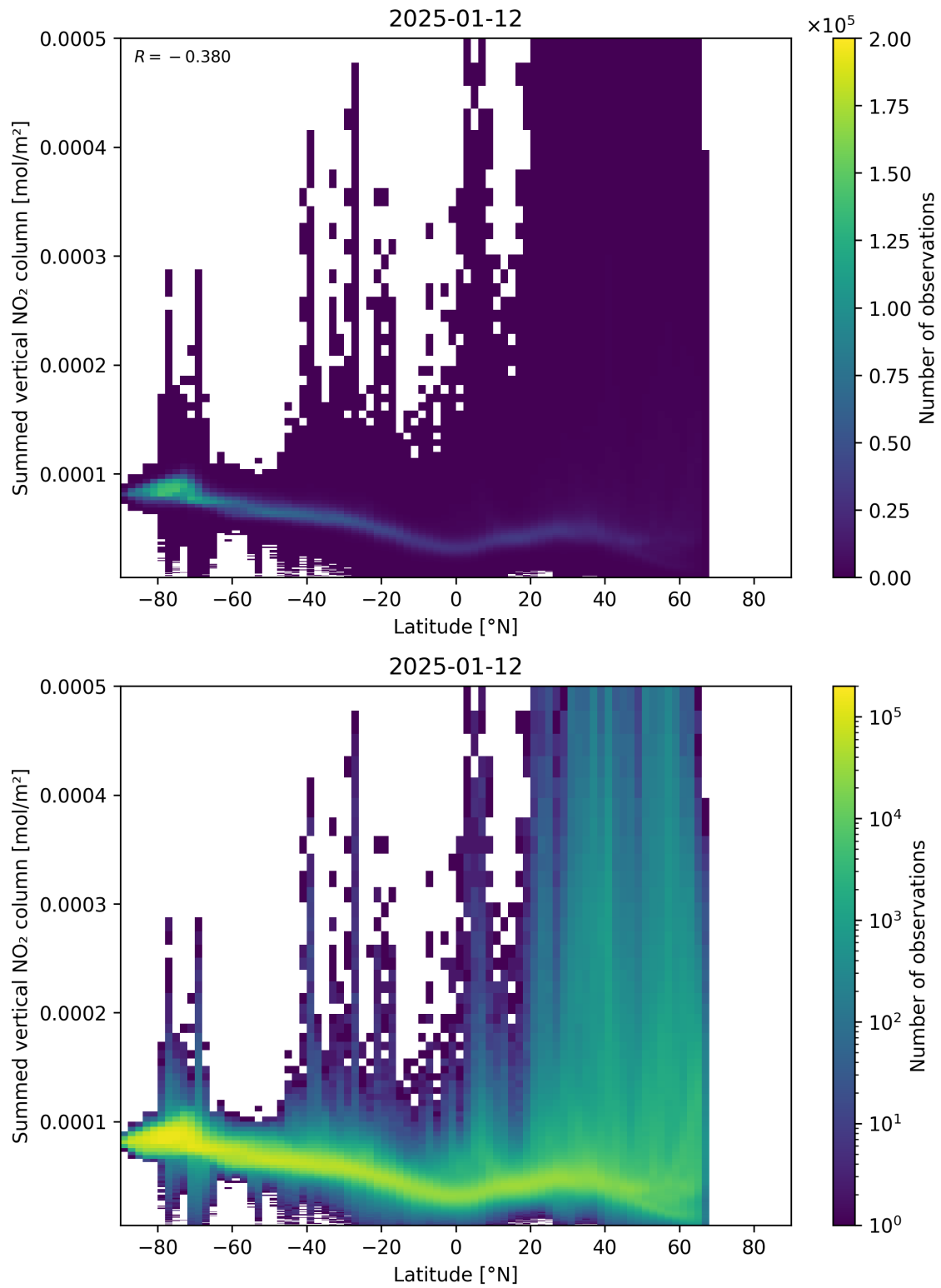
Figure 88: Scatter density plot of “Latitude” against “Summed vertical NO 2 column” for 2025-01-12 to 2025-01-13.
