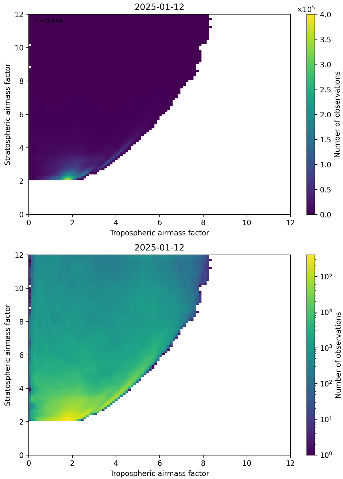
Figure 71: Scatter density plot of “Tropospheric airmass factor” against “Stratospheric airmass factor” for 2025-01-12 to 2025-01-13.
