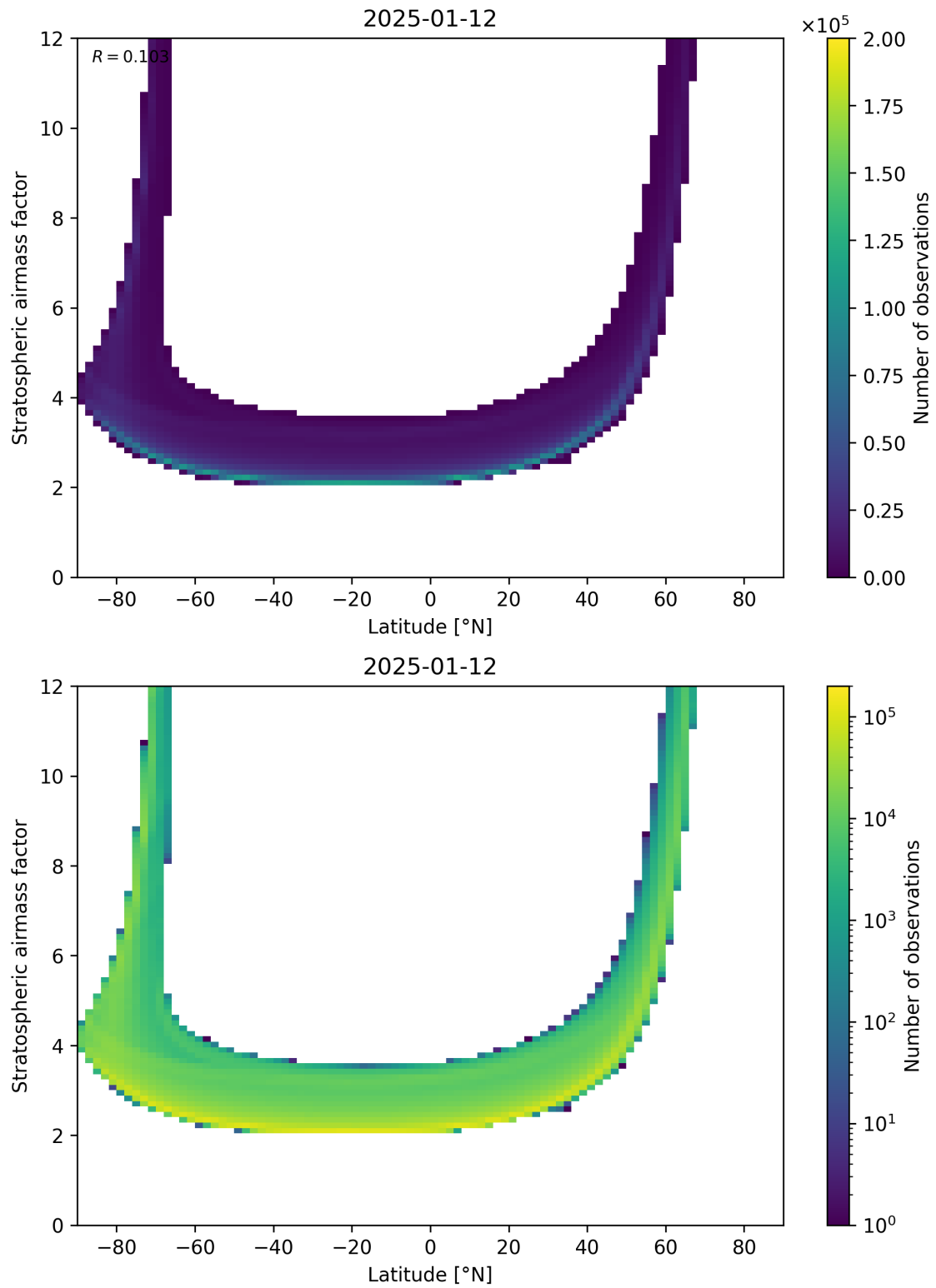
Figure 83: Scatter density plot of “Latitude” against “Stratospheric airmass factor” for 2025-01-12 to 2025-01-13.
