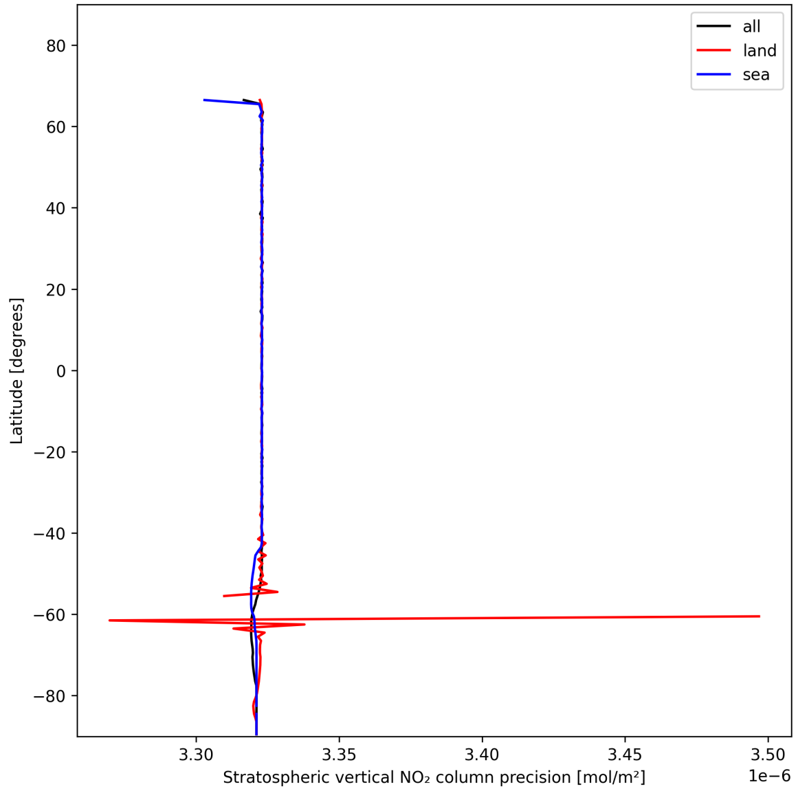
Figure 20: Zonal average of “Stratospheric vertical NO 2 column precision” for 2025-01-12 to 2025-01-13.
