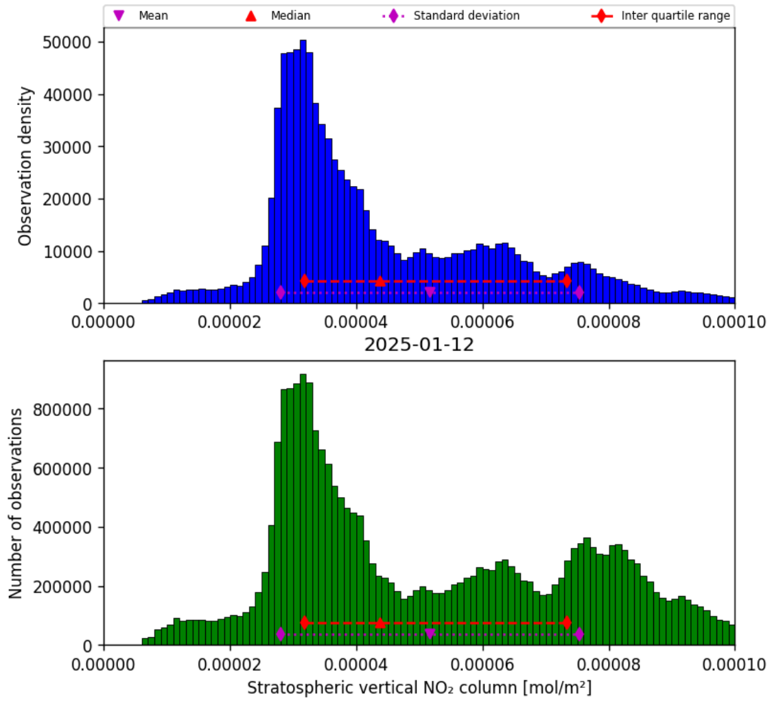
Figure 36: Histogram of “Stratospheric vertical NO 2 column” for 2025-01-12 to 2025-01-13
