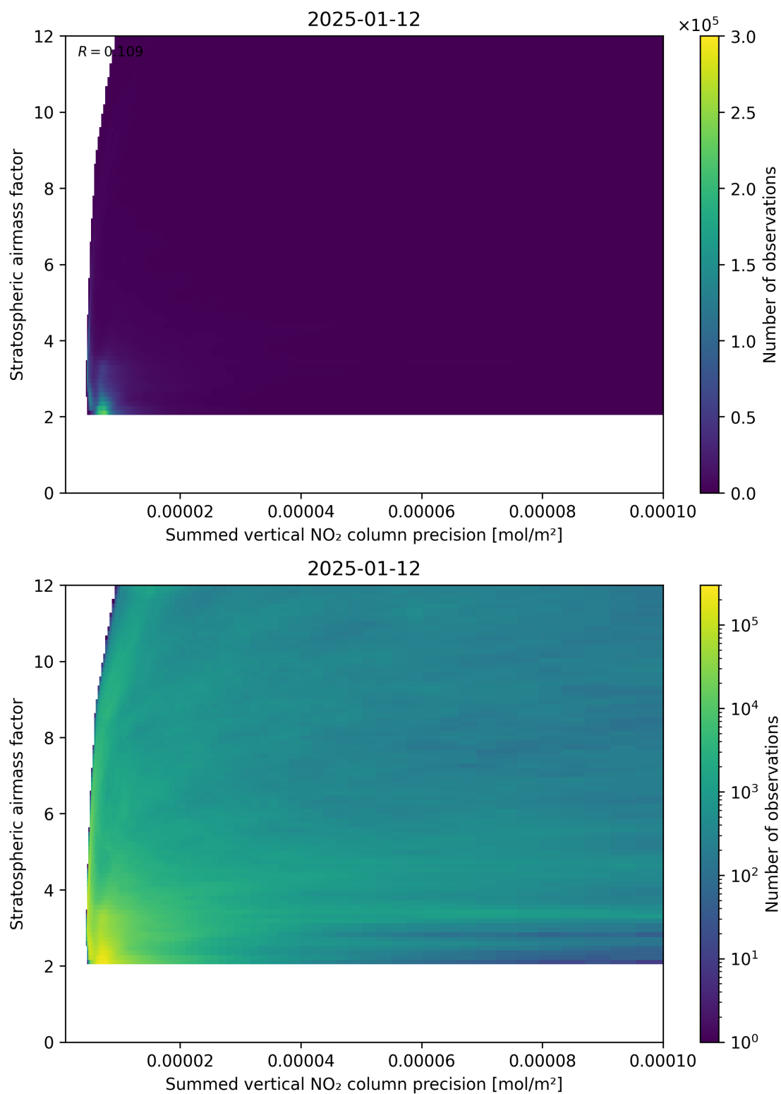
Figure 106: Scatter density plot of “Summed vertical NO 2 column precision” against “Stratospheric airmass factor” for 2025-01-12 to 2025-01-13.
