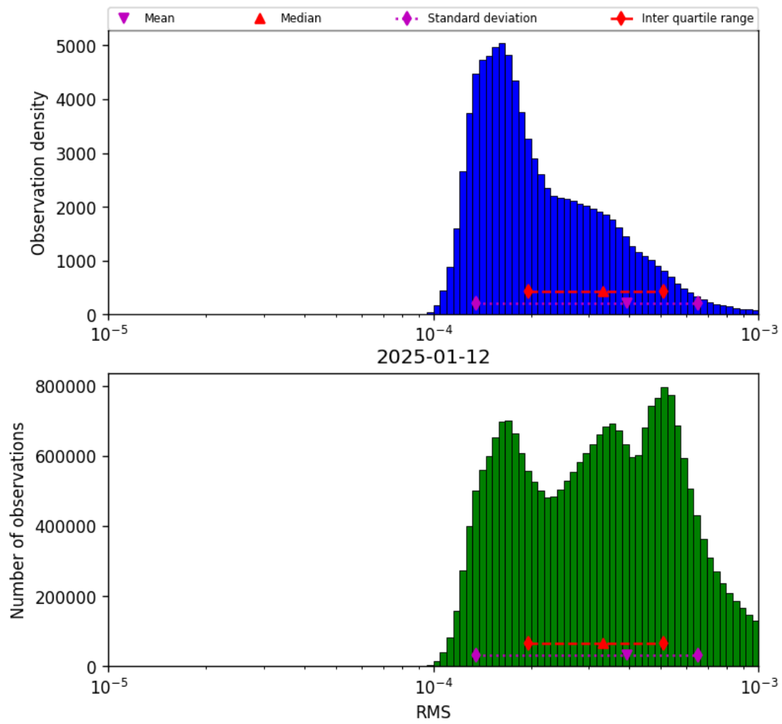
Figure 43: Histogram of “RMS” for 2025-01-12 to 2025-01-13
