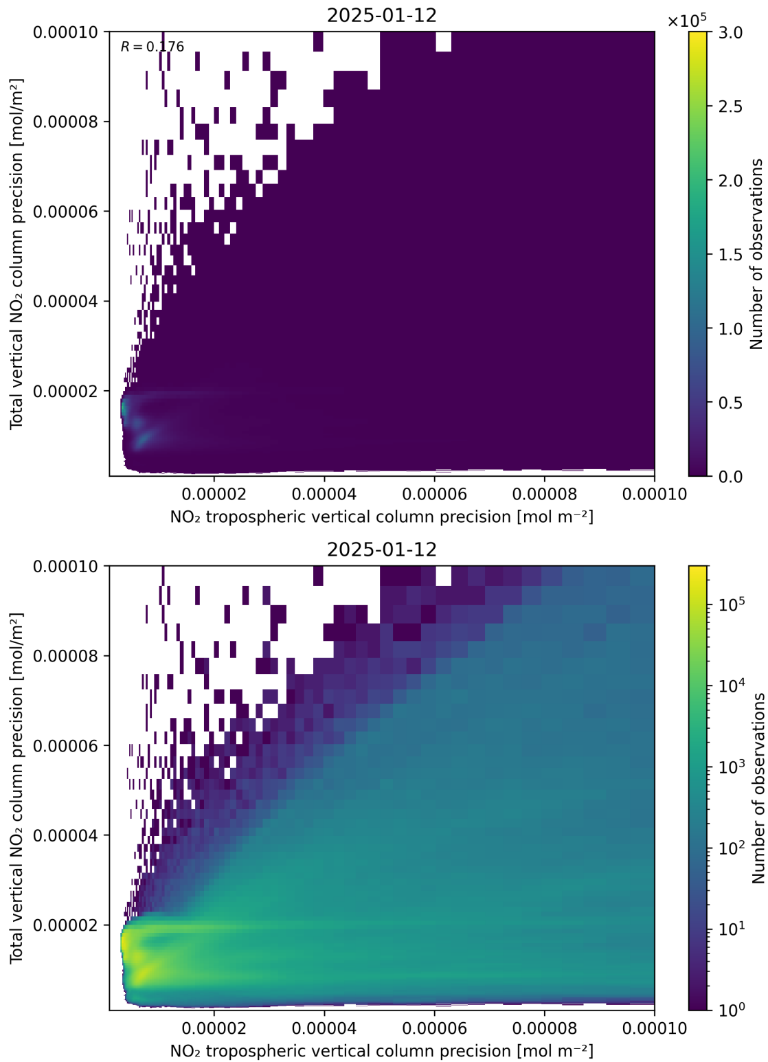
Figure 139: Scatter density plot of “NO 2 tropospheric vertical column precision” against “Total vertical NO 2 column precision” for 2025-01-12 to 2025-01-13.
