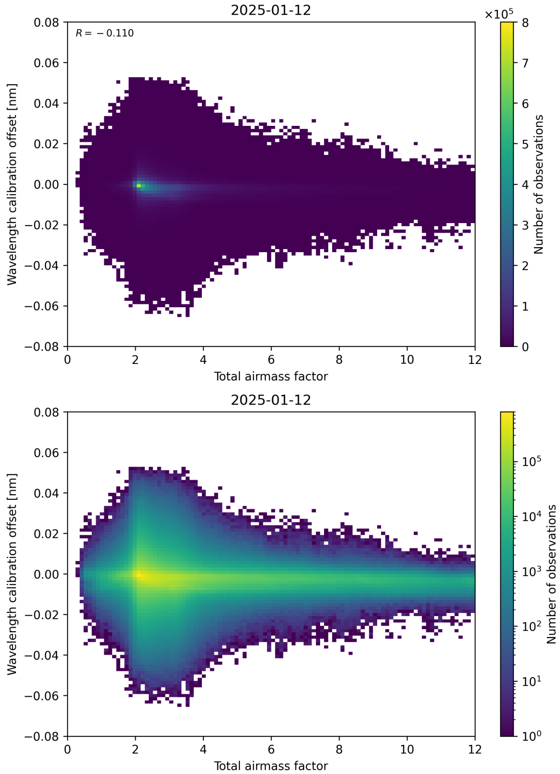
Figure 70: Scatter density plot of “Total airmass factor” against “Wavelength calibration offset” for 2025-01-12 to 2025-01-13.
