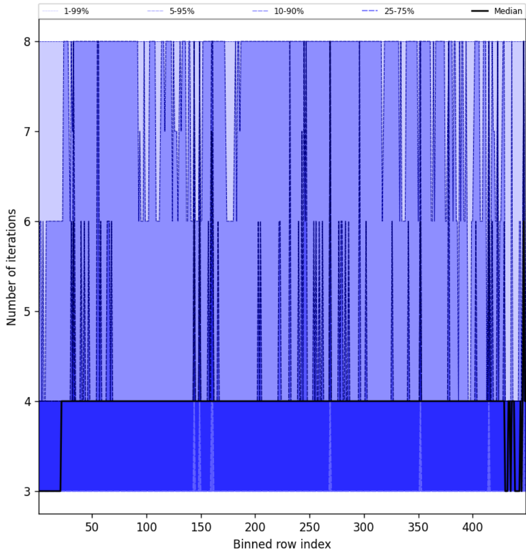
Figure 51: Along track statistics of “Number of iterations” for 2025-01-12 to 2025-01-13
