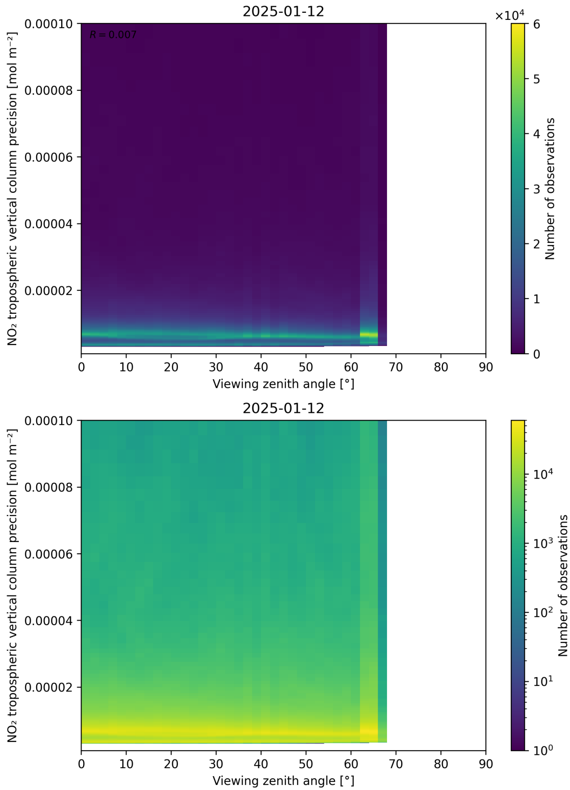
Figure 170: Scatter density plot of “Viewing zenith angle” against “NO 2 tropospheric vertical column precision” for 2025-01-12 to 2025-01-13.
