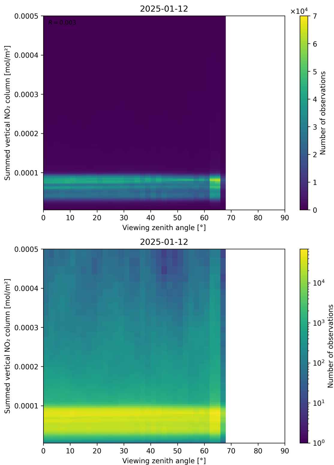
Figure 165: Scatter density plot of “Viewing zenith angle” against “Summed vertical NO 2 column” for 2025-01-12 to 2025-01-13.
