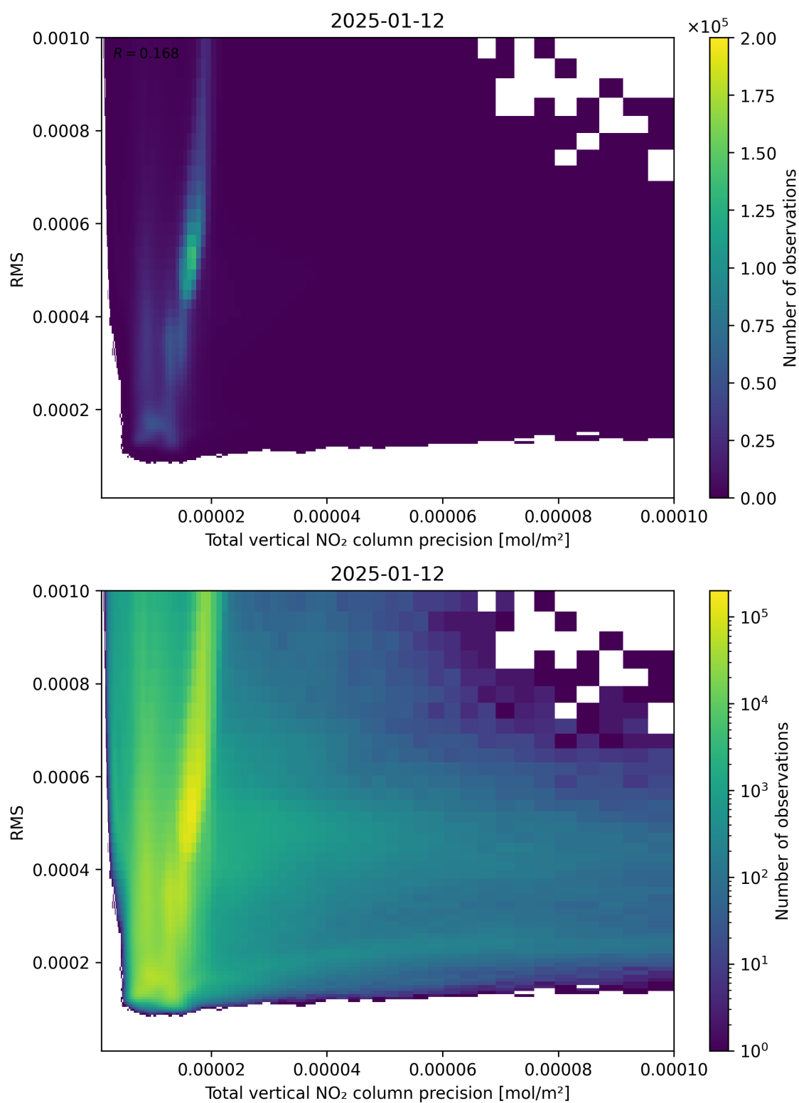
Figure 119: Scatter density plot of “Total vertical NO 2 column precision” against “RMS” for 2025-01-12 to 2025-01-13.
