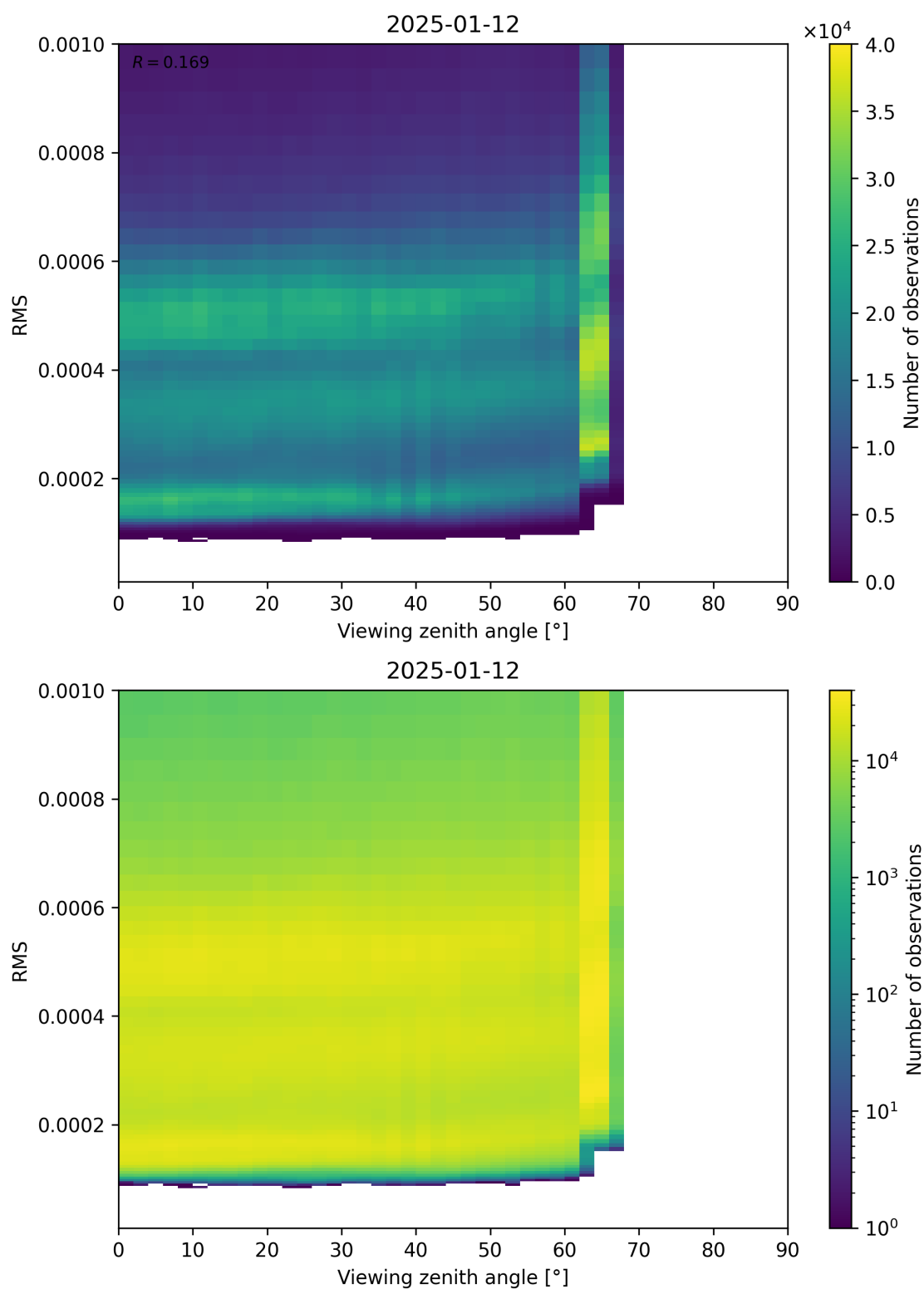
Figure 171: Scatter density plot of “Viewing zenith angle” against “RMS” for 2025-01-12 to 2025-01-13.
