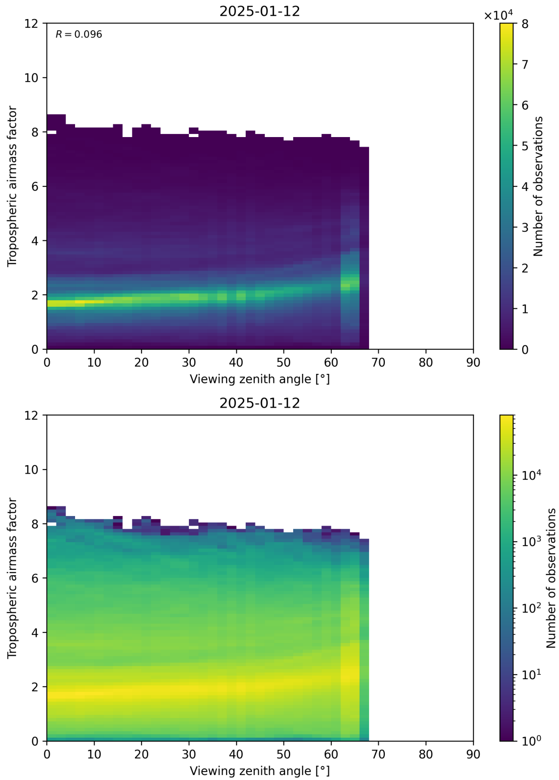
Figure 161: Scatter density plot of “Viewing zenith angle” against “Tropospheric airmass factor” for 2025-01-12 to 2025-01-13.
