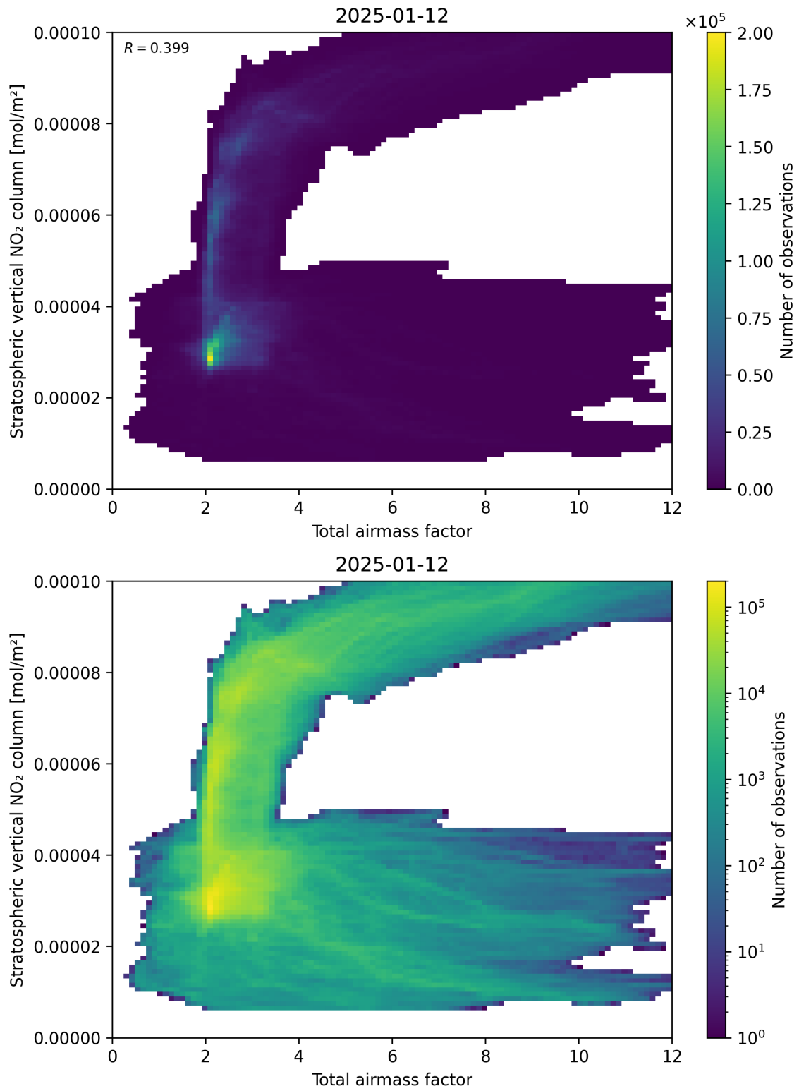
Figure 64: Scatter density plot of “Total airmass factor” against “Stratospheric vertical NO 2 column” for 2025-01-12 to 2025-01-13.
