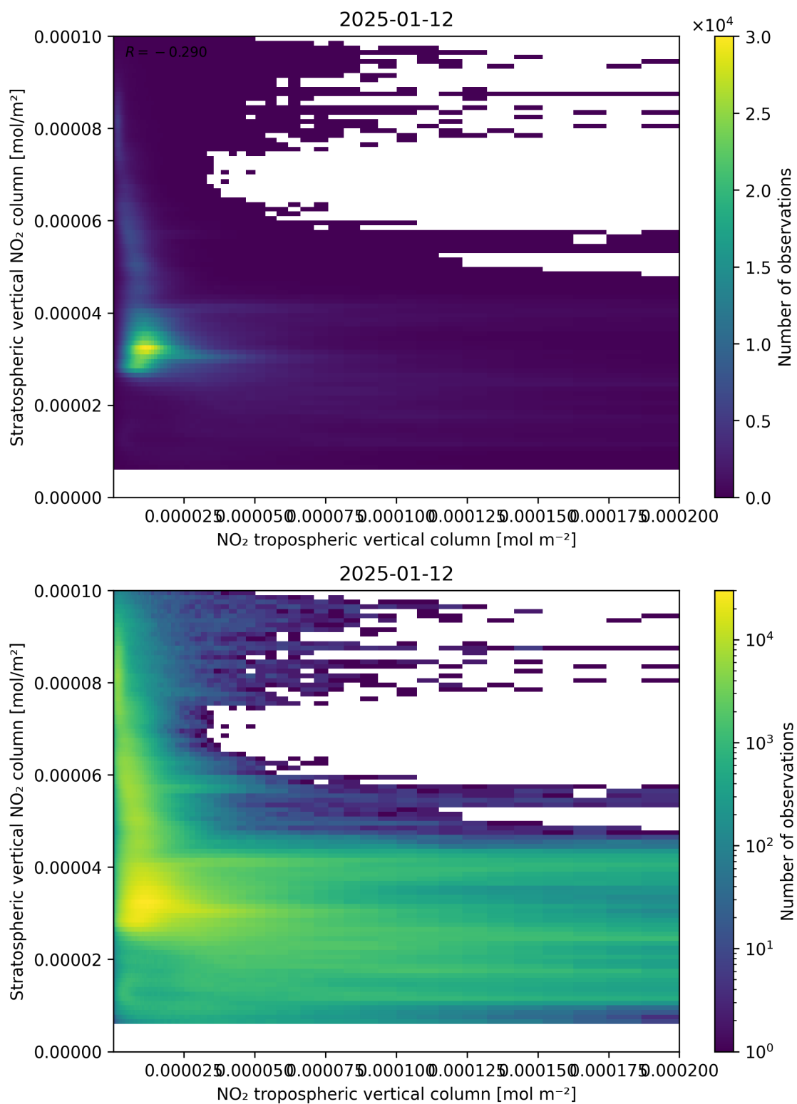
Figure 125: Scatter density plot of “NO 2 tropospheric vertical column” against “Stratospheric vertical NO 2 column” for 2025-01-12 to 2025-01-13.
