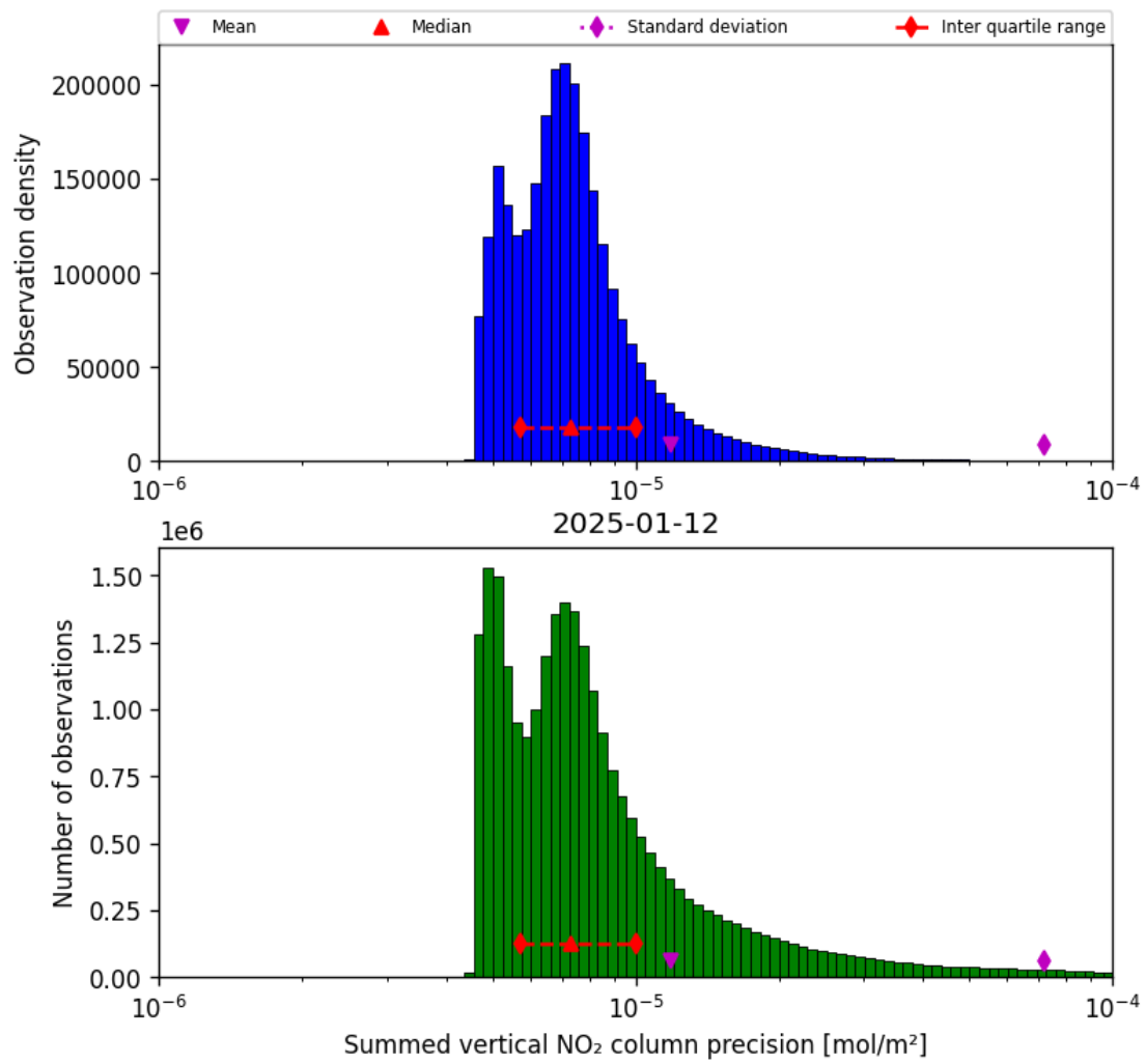
Figure 41: Histogram of “Summed vertical NO 2 column precision” for 2025-01-12 to 2025-01-13
