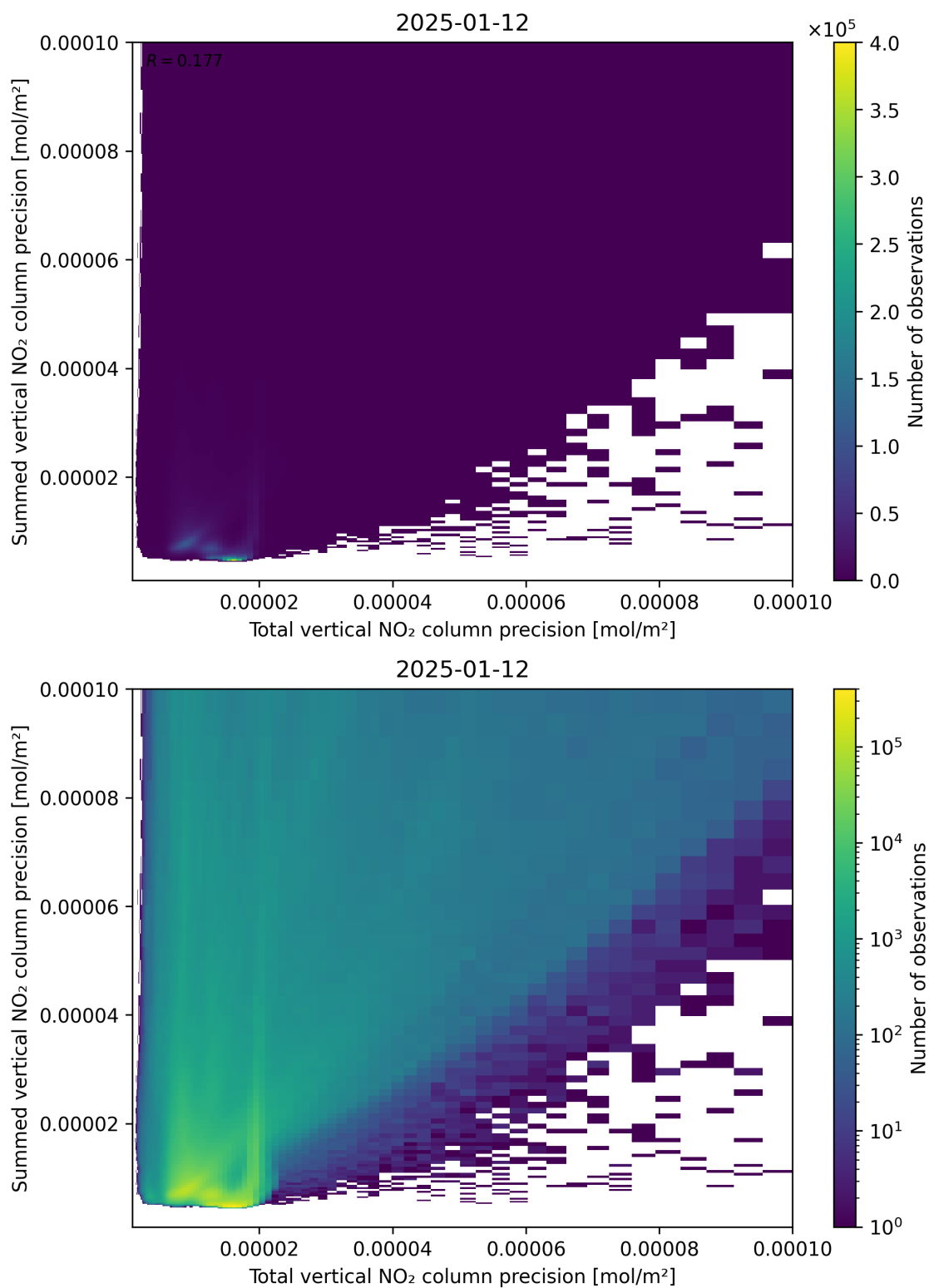
Figure 118: Scatter density plot of “Total vertical NO 2 column precision” against “Summed vertical NO 2 column precision” for 2025-01-12 to 2025-01-13.
