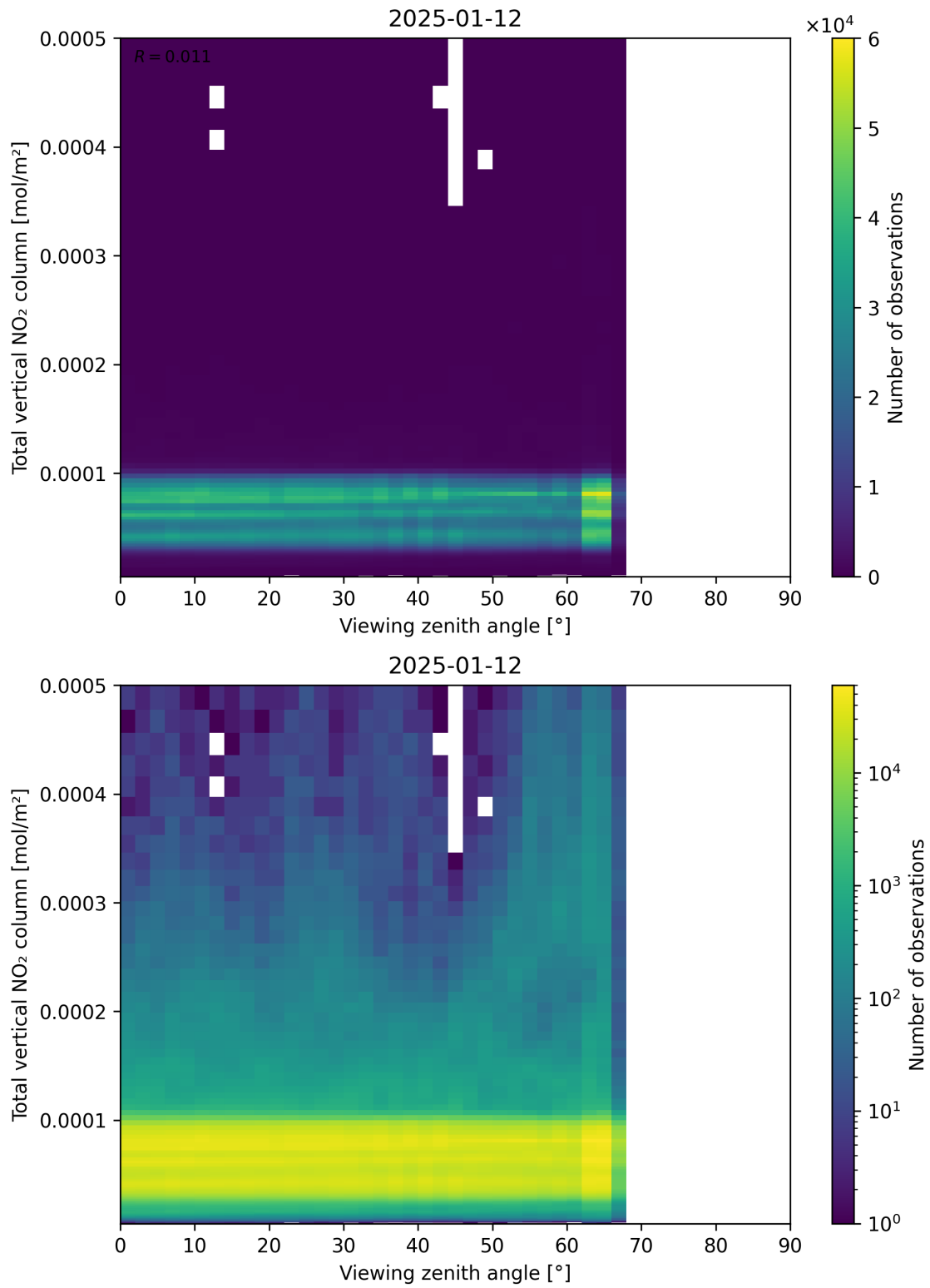
Figure 167: Scatter density plot of “Viewing zenith angle” against “Total vertical NO 2 column” for 2025-01-12 to 2025-01-13.
