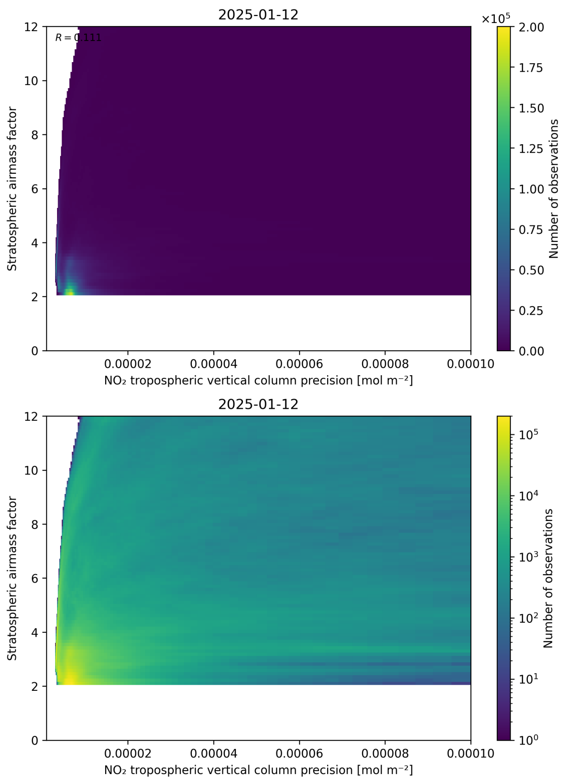
Figure 131: Scatter density plot of “NO 2 tropospheric vertical column precision” against “Stratospheric airmass factor” for 2025-01-12 to 2025-01-13.
