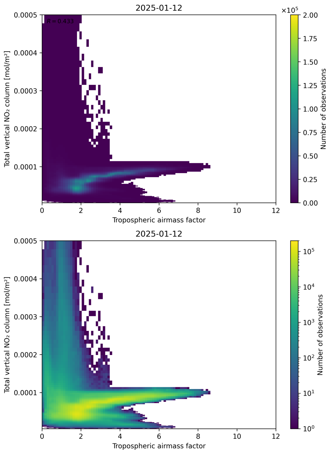
Figure 77: Scatter density plot of “Tropospheric airmass factor” against “Total vertical NO 2 column” for 2025-01-12 to 2025-01-13.
