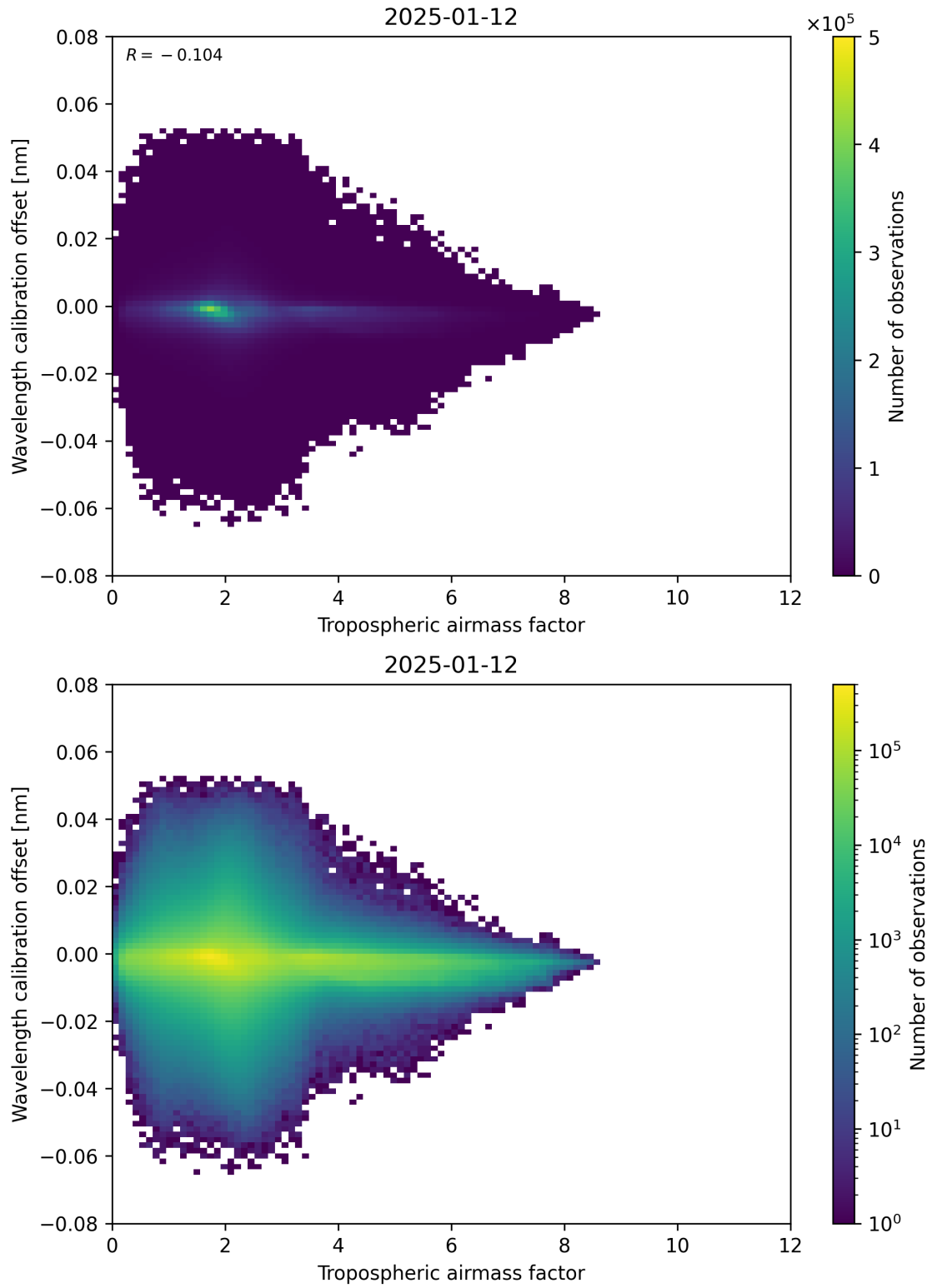
Figure 80: Scatter density plot of “Tropospheric airmass factor” against “Wavelength calibration offset” for 2025-01-12 to 2025-01-13.
