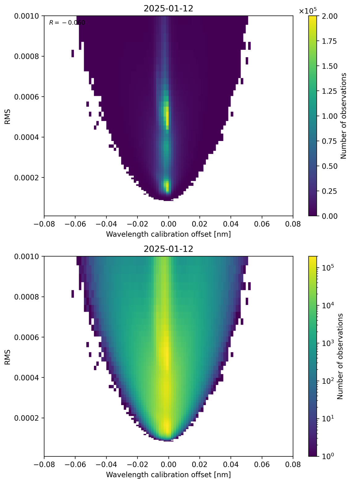
Figure 181: Scatter density plot of “Wavelength calibration offset” against “RMS” for 2025-01-12 to 2025-01-13.
