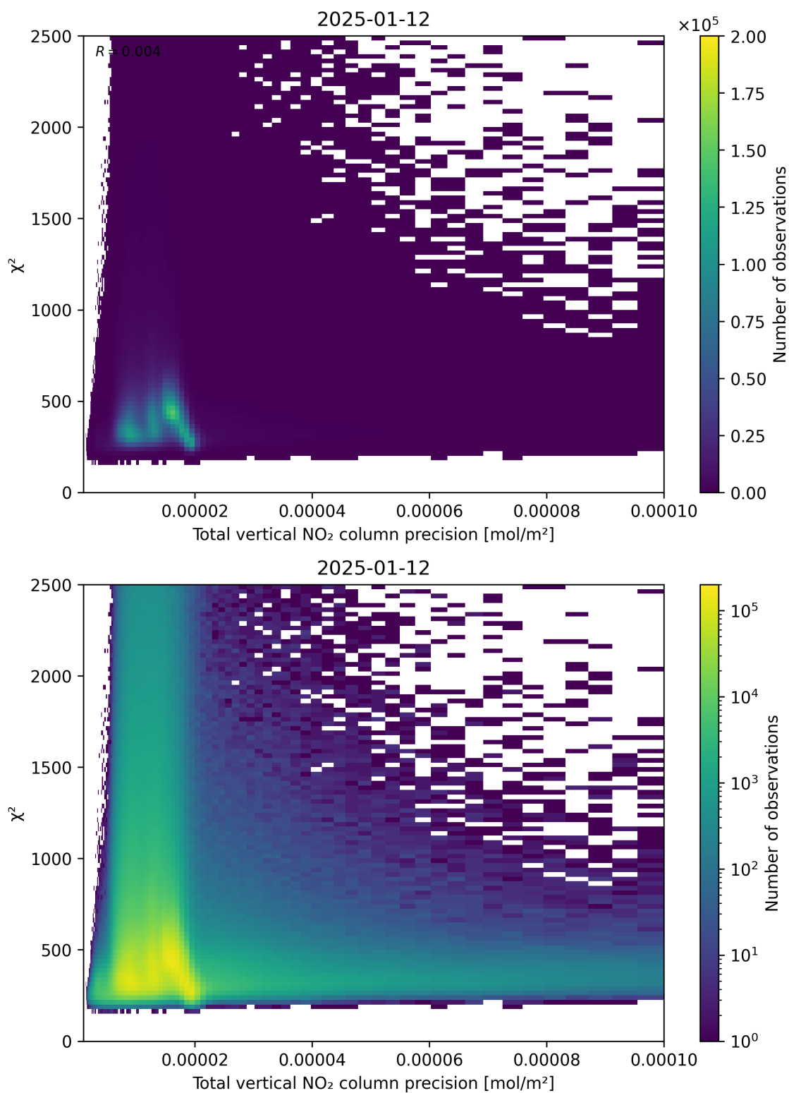
Figure 116: Scatter density plot of “Total vertical NO 2 column precision” against “ \chi^2 ” for 2025-01-12 to 2025-01-13.
