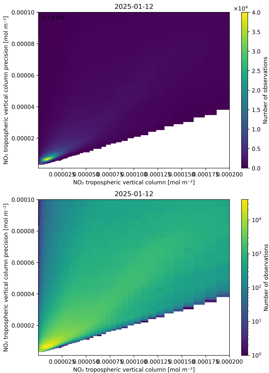
Figure 130: Scatter density plot of “NO 2 tropospheric vertical column” against “NO 2 tropospheric vertical column precision” for 2025-01-12 to 2025-01-13.
