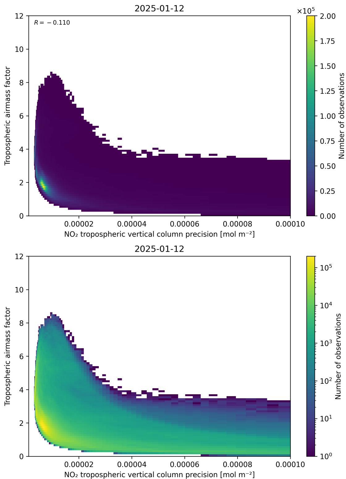
Figure 133: Scatter density plot of “NO 2 tropospheric vertical column precision” against “Tropospheric air mass factor” for 2025-01-12 to 2025-01-13.
