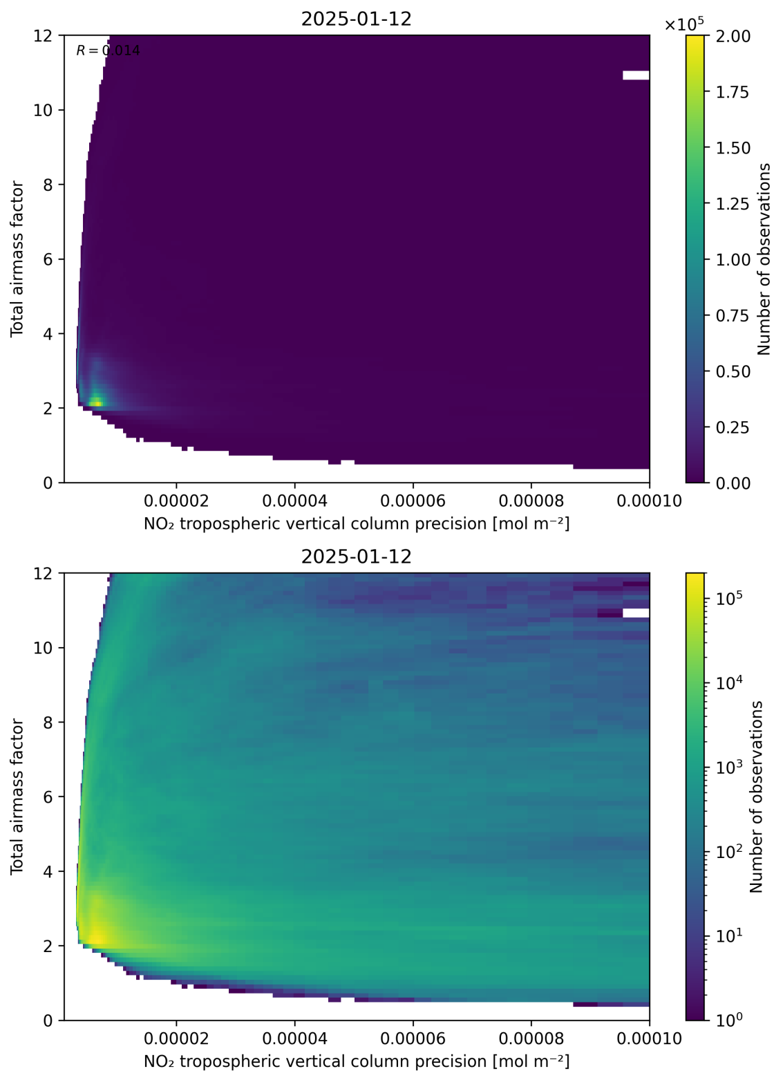
Figure 132: Scatter density plot of “NO 2 tropospheric vertical column precision” against “Total air mass factor” for 2025-01-12 to 2025-01-13.
