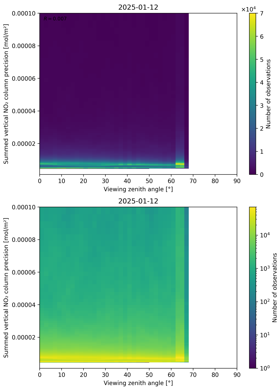
Figure 166: Scatter density plot of “Viewing zenith angle” against “Summed vertical NO 2 column precision” for 2025-01-12 to 2025-01-13.
