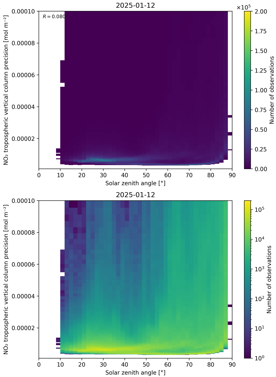
Figure 156: Scatter density plot of “Solar zenith angle” against “NO 2 tropospheric vertical column precision” for 2025-01-12 to 2025-01-13.
