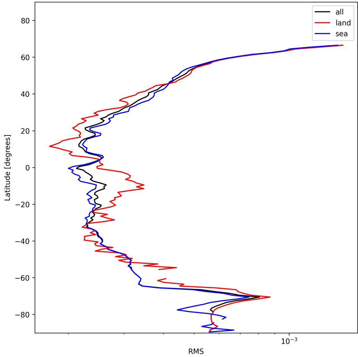
Figure 26: Zonal average of “RMS” for 2025-01-12 to 2025-01-13.
