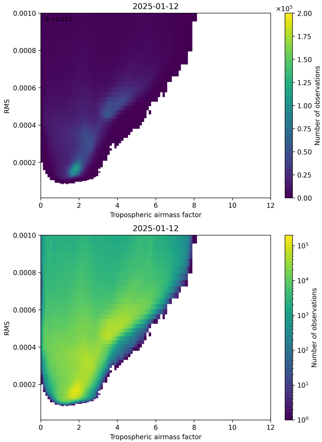
Figure 79: Scatter density plot of “Tropospheric airmass factor” against “RMS” for 2025-01-12 to 2025-01-13.
