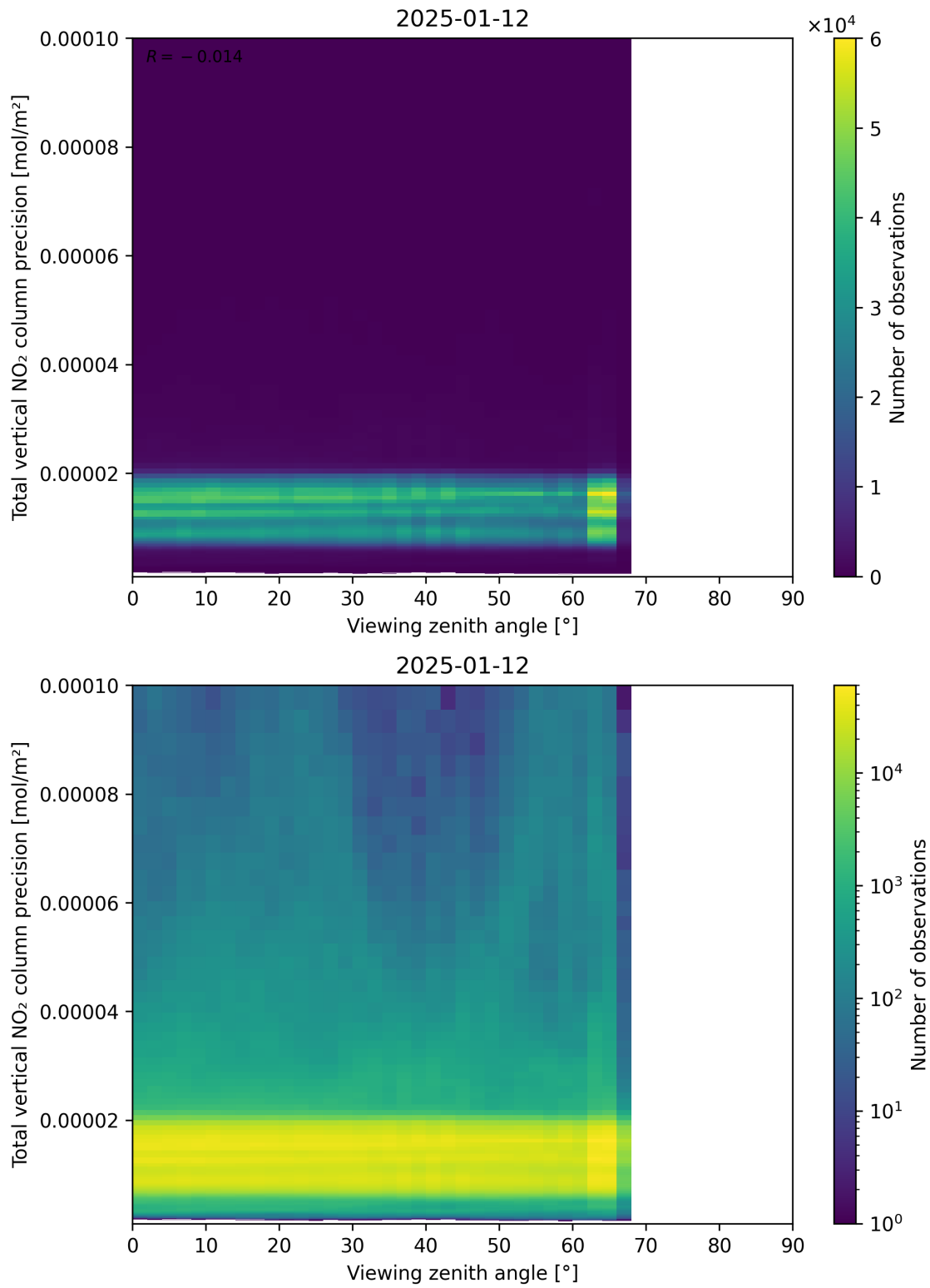
Figure 168: Scatter density plot of “Viewing zenith angle” against “Total vertical NO 2 column precision” for 2025-01-12 to 2025-01-13.
