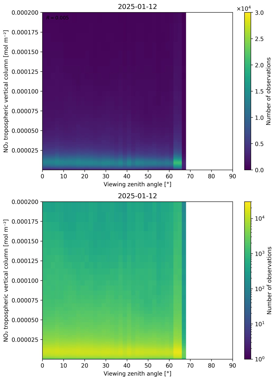
Figure 169: Scatter density plot of “Viewing zenith angle” against “NO 2 tropospheric vertical column” for 2025-01-12 to 2025-01-13.
