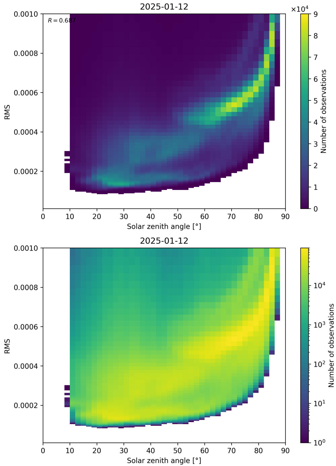
Figure 157: Scatter density plot of “Solar zenith angle” against “RMS” for 2025-01-12 to 2025-01-13.
