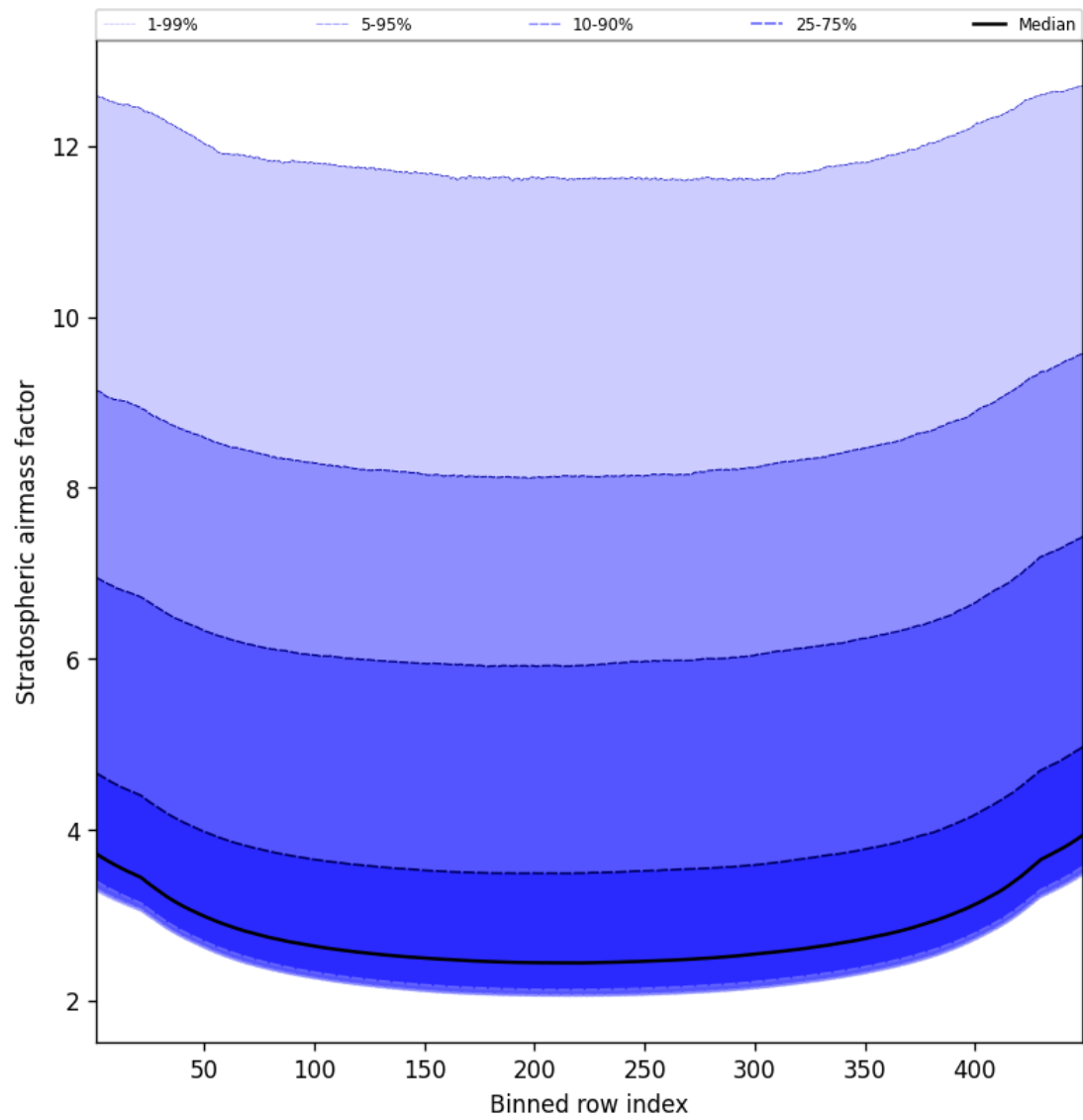
Figure 61: Along track statistics of “Stratospheric airmass factor” for 2025-01-12 to 2025-01-13
