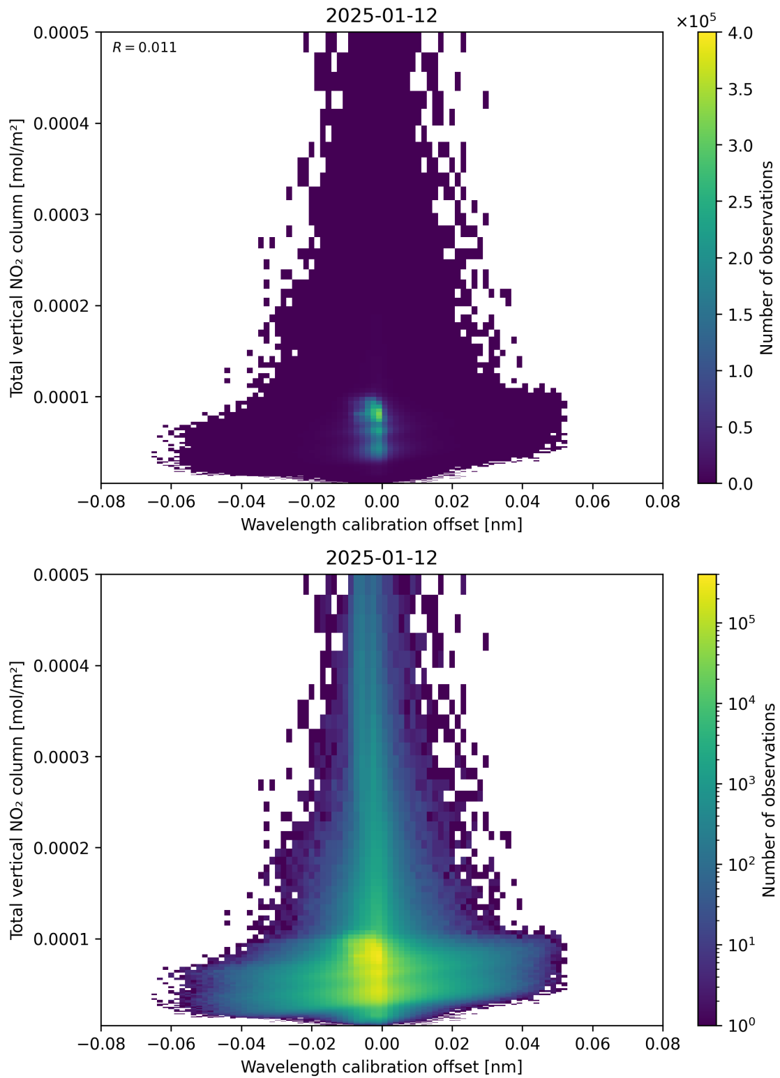
Figure 179: Scatter density plot of “Wavelength calibration offset” against “Total vertical NO 2 column” for 2025-01-12 to 2025-01-13.
