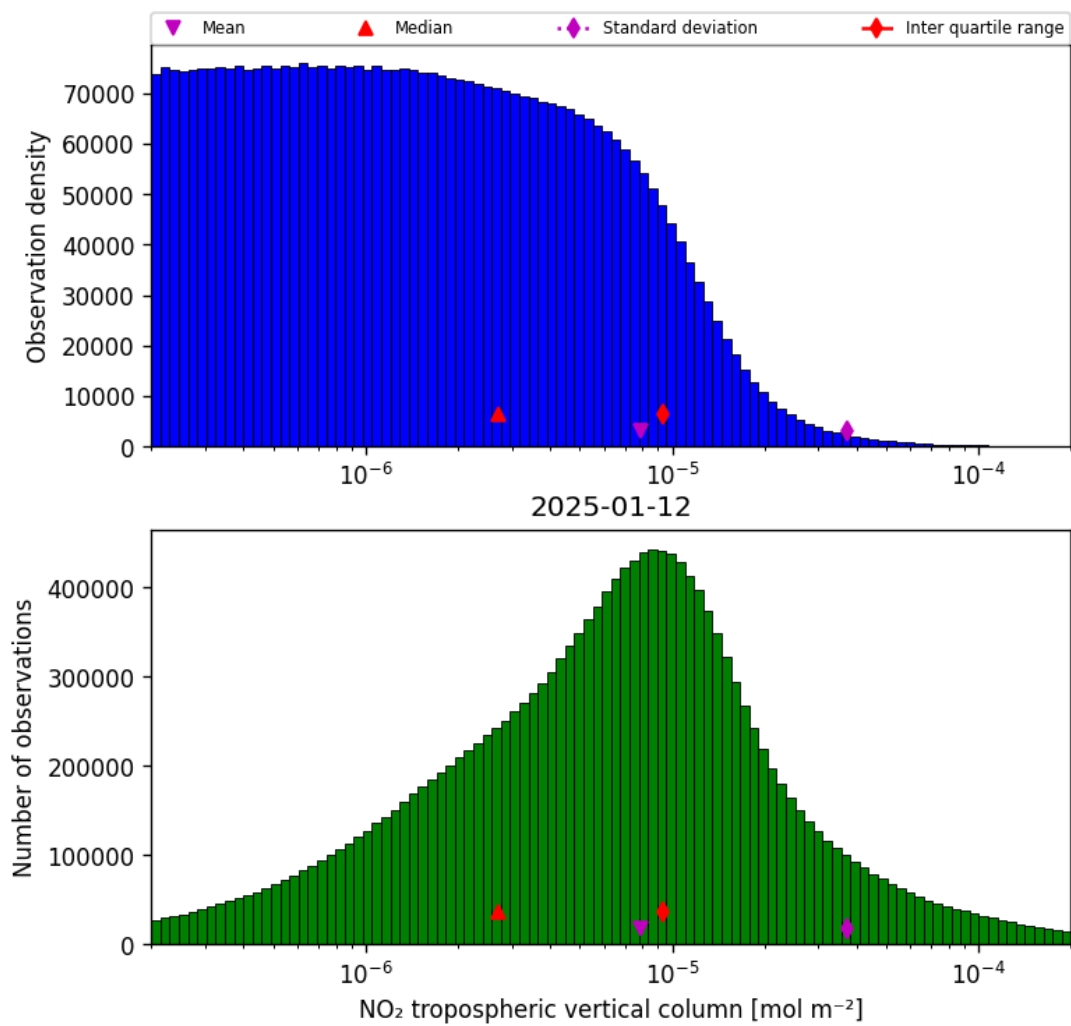
Figure 29: Histogram of “NO 2 tropospheric vertical column” for 2025-01-12 to 2025-01-13
