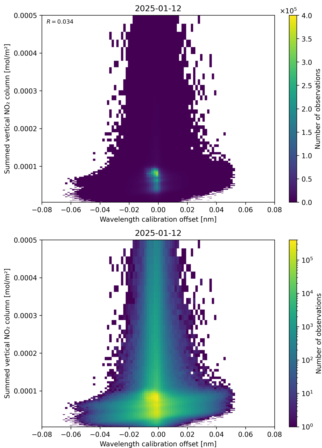
Figure 177: Scatter density plot of “Wavelength calibration offset” against “Summed vertical NO 2 column” for 2025-01-12 to 2025-01-13.
