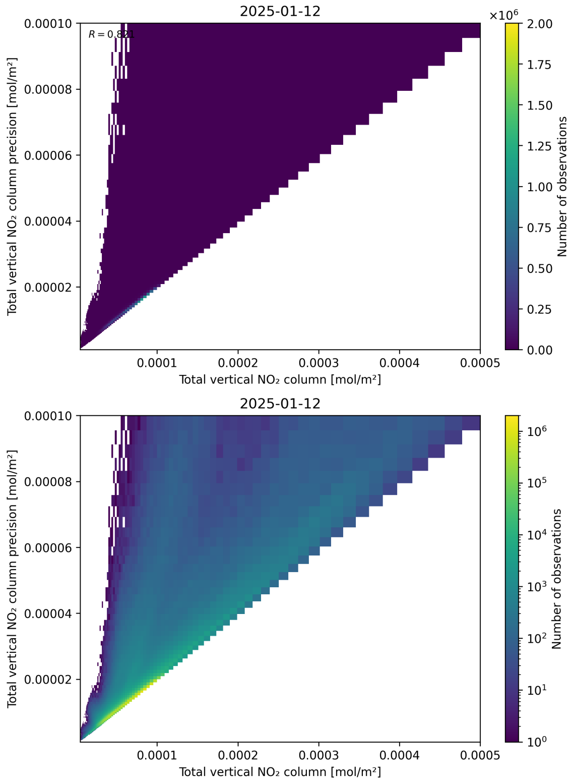
Figure 114: Scatter density plot of “Total vertical NO 2 column” against “Total vertical NO 2 column precision” for 2025-01-12 to 2025-01-13.
