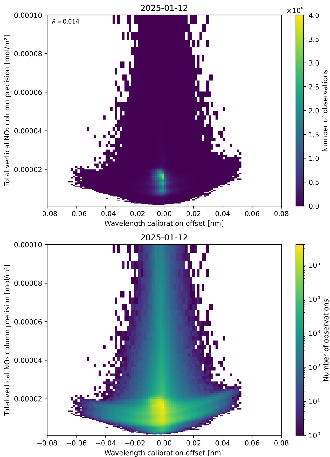
Figure 180: Scatter density plot of “Wavelength calibration offset” against “Total vertical NO 2 column precision” for 2025-01-12 to 2025-01-13.
