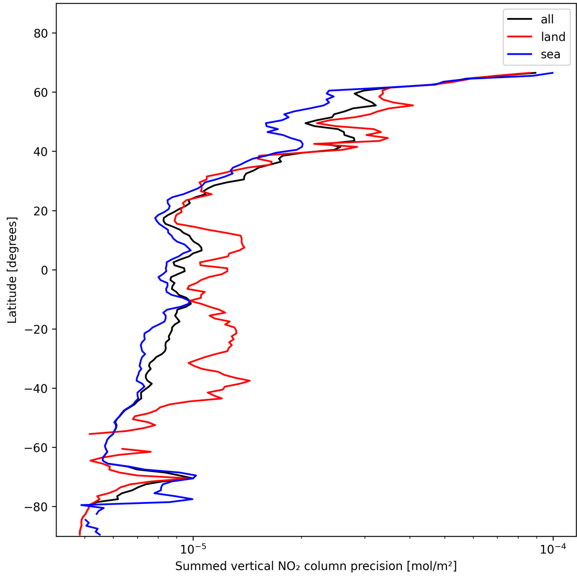
Figure 24: Zonal average of “Summed vertical NO 2 column precision” for 2025-01-12 to 2025-01-13.
