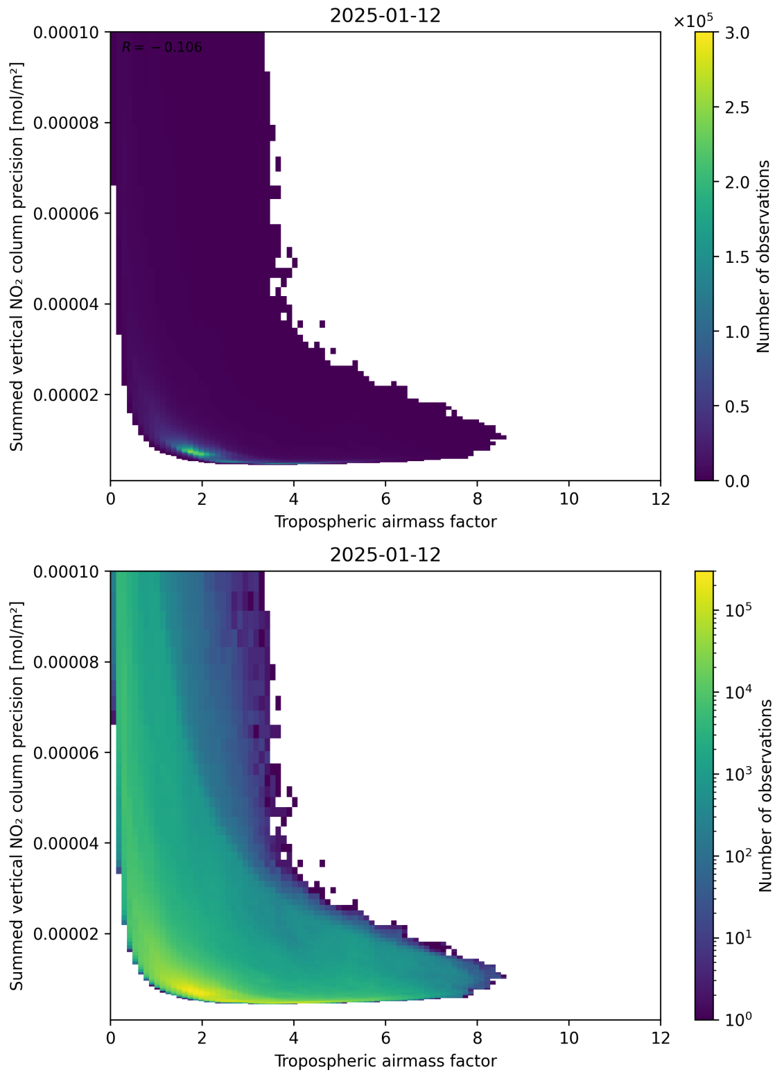
Figure 76: Scatter density plot of “Tropospheric air mass factor” against “Summed vertical NO 2 column precision” for 2025-01-12 to 2025-01-13.
