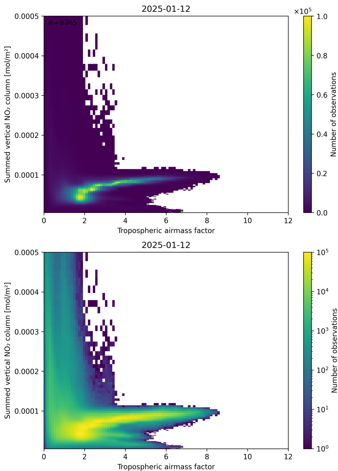
Figure 75: Scatter density plot of “Tropospheric air mass factor” against “Summed vertical NO 2 column” for 2025-01-12 to 2025-01-13.
