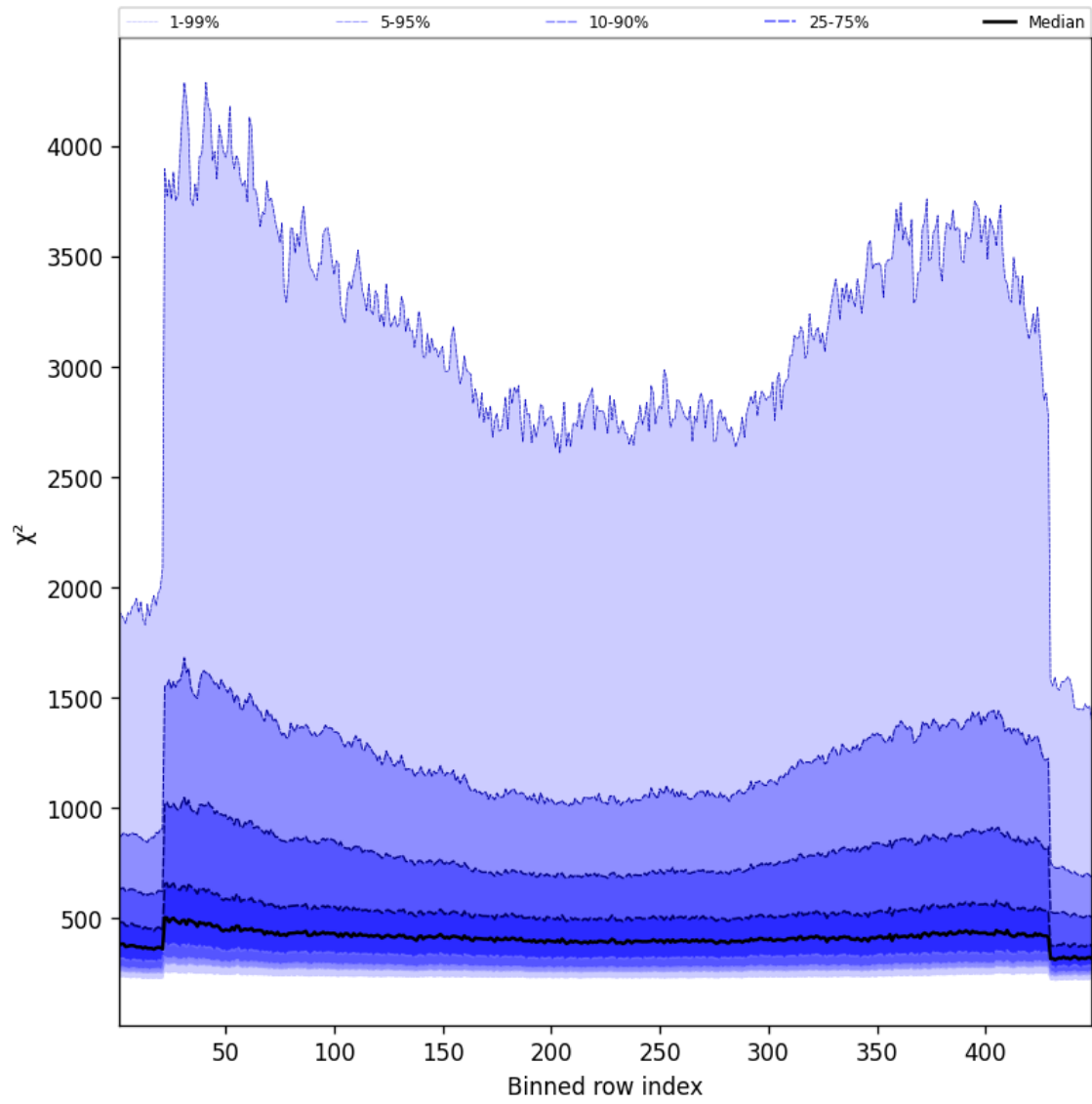
Figure 59: Along track statistics of “ \chi^2 ” for 2025-01-12 to 2025-01-13
