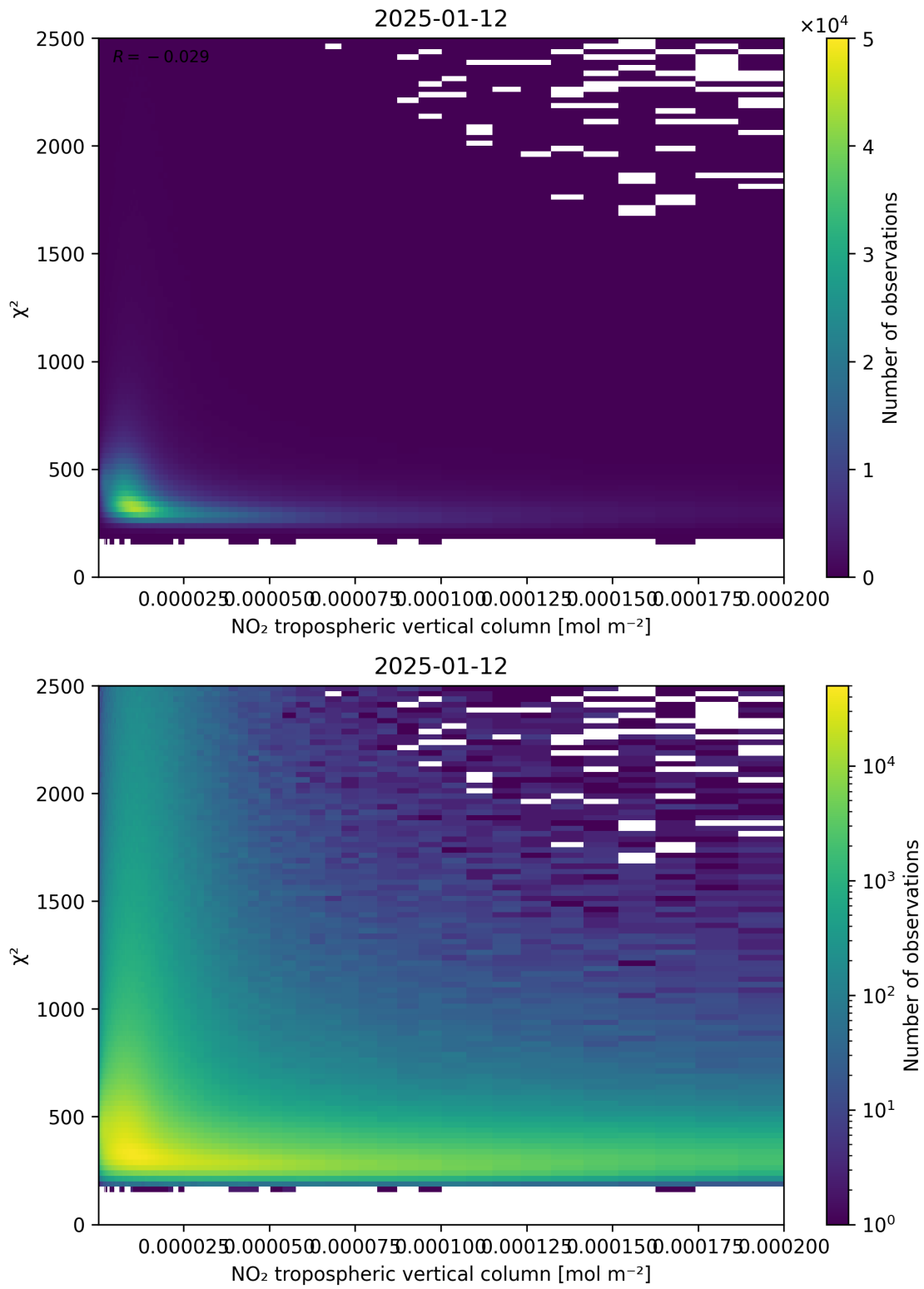
Figure 124: Scatter density plot of “NO 2 tropospheric vertical column” against “ \chi^2 ” for 2025-01-12 to 2025-01-13.
