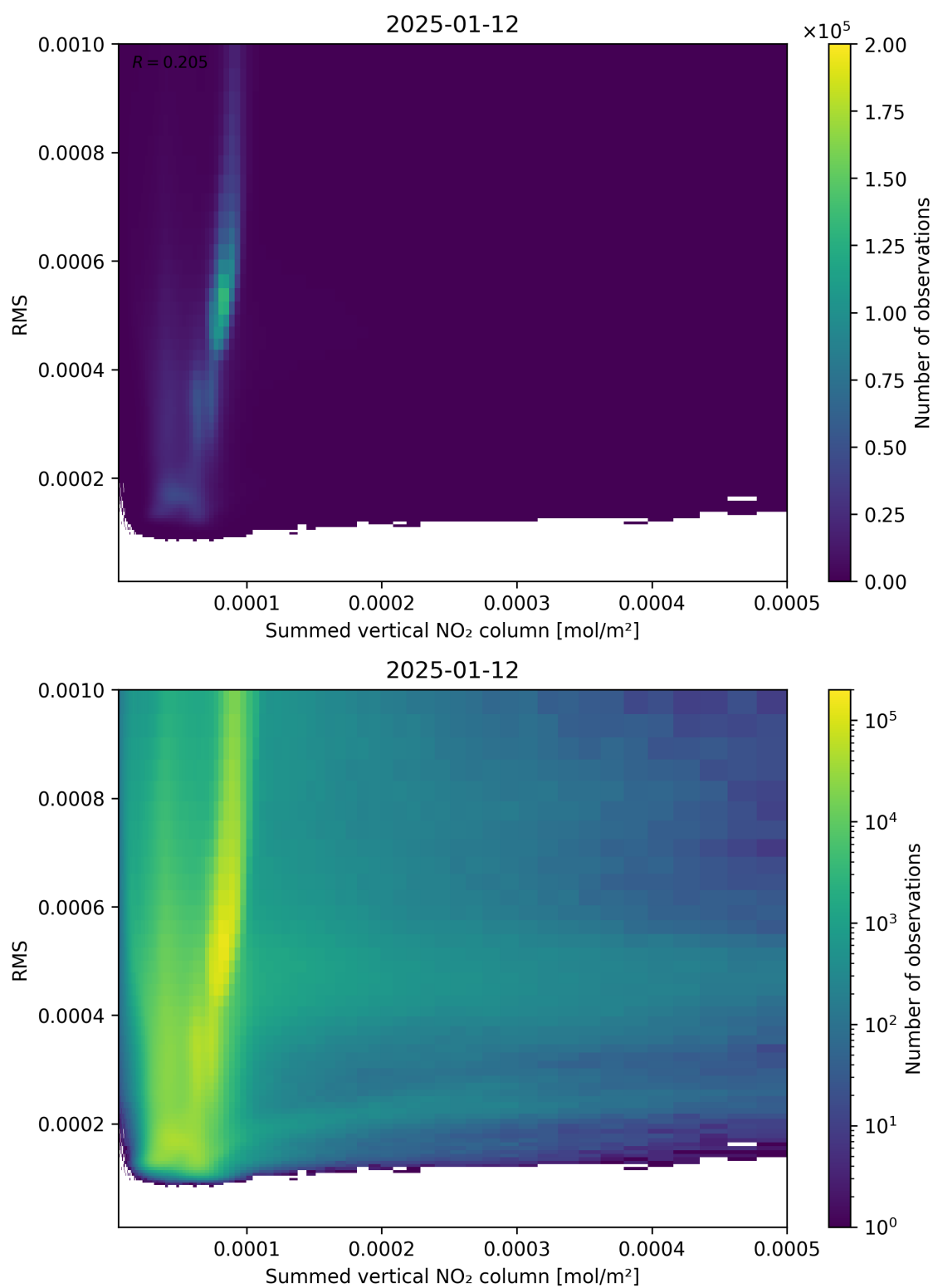
Figure 109: Scatter density plot of “Summed vertical NO 2 column” against “RMS” for 2025-01-12 to 2025-01-13.
