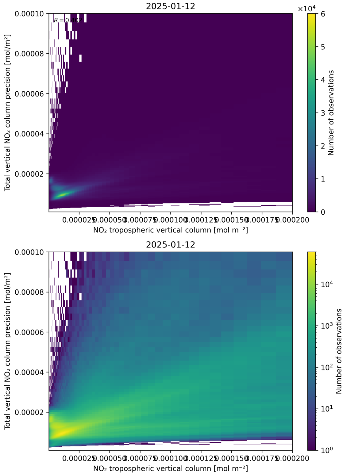
Figure 129: Scatter density plot of “NO 2 tropospheric vertical column” against “Total vertical NO 2 column precision” for 2025-01-12 to 2025-01-13.
