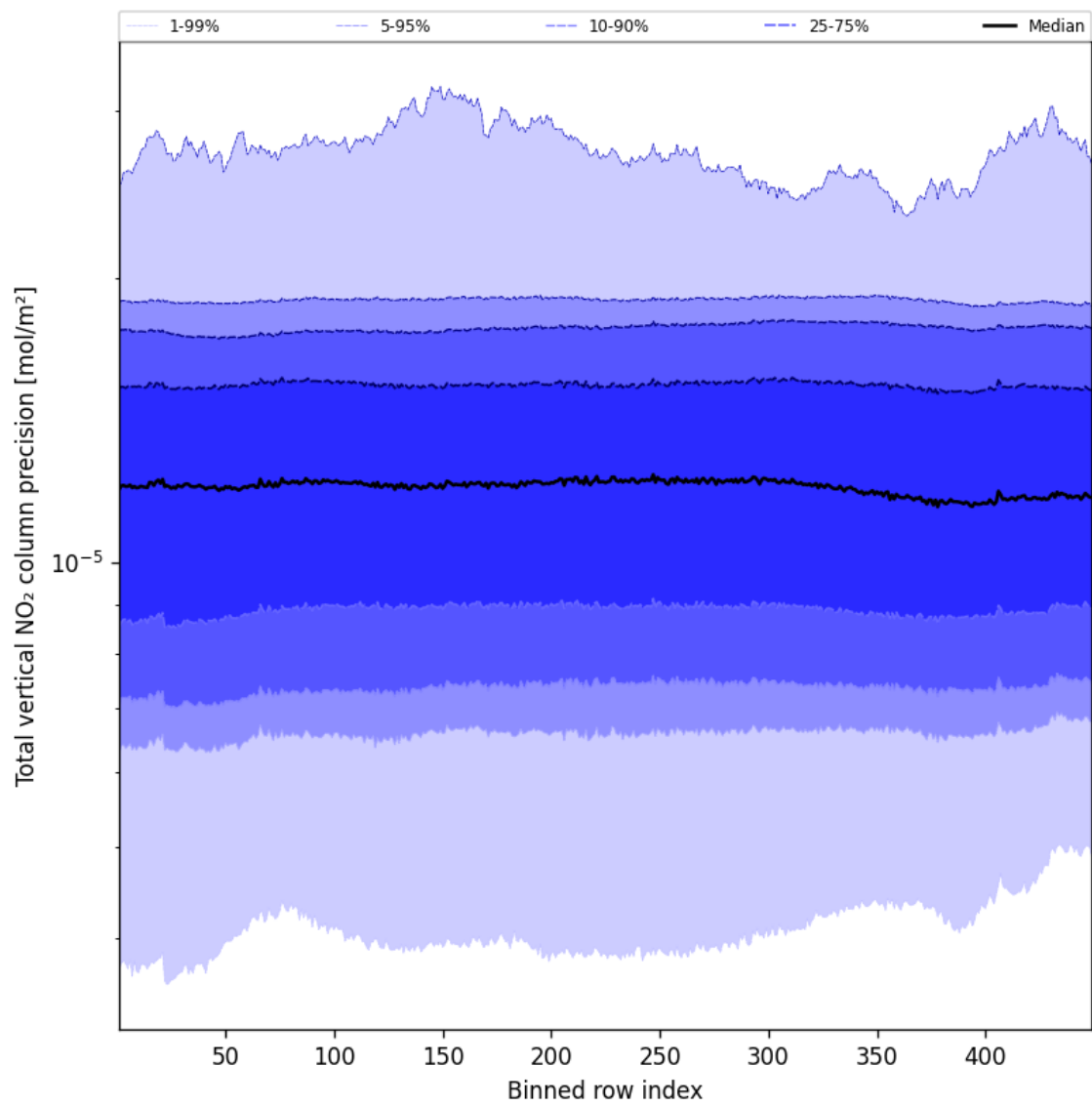
Figure 56: Along track statistics of “Total vertical NO 2 column precision” for 2025-01-12 to 2025-01-13
