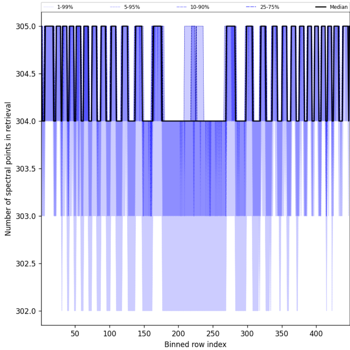
Figure 50: Along track statistics of “Number of spectral points in retrieval” for 2025-01-12 to 2025-01-13
