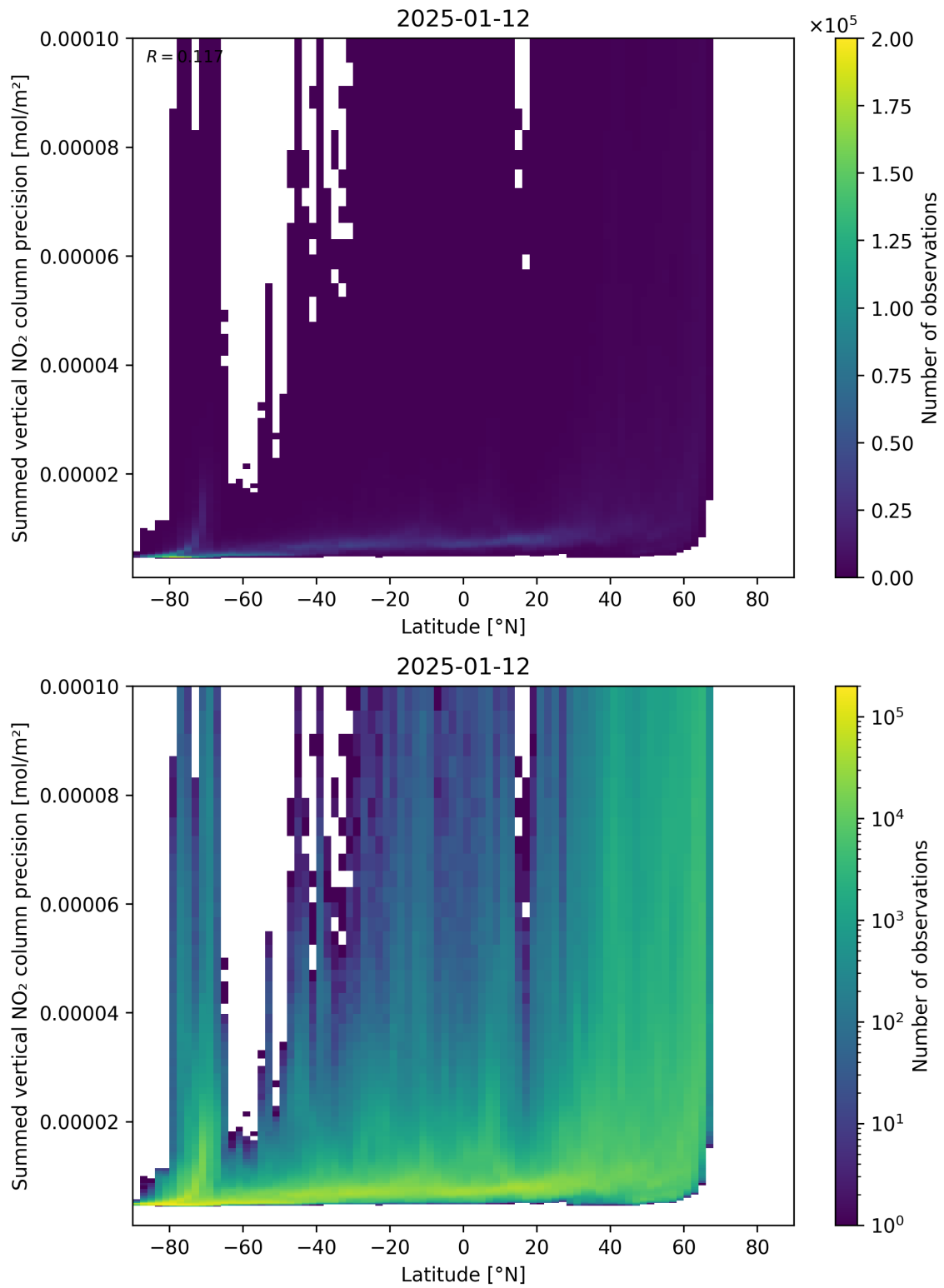
Figure 89: Scatter density plot of “Latitude” against “Summed vertical NO 2 column precision” for 2025-01-12 to 2025-01-13.
