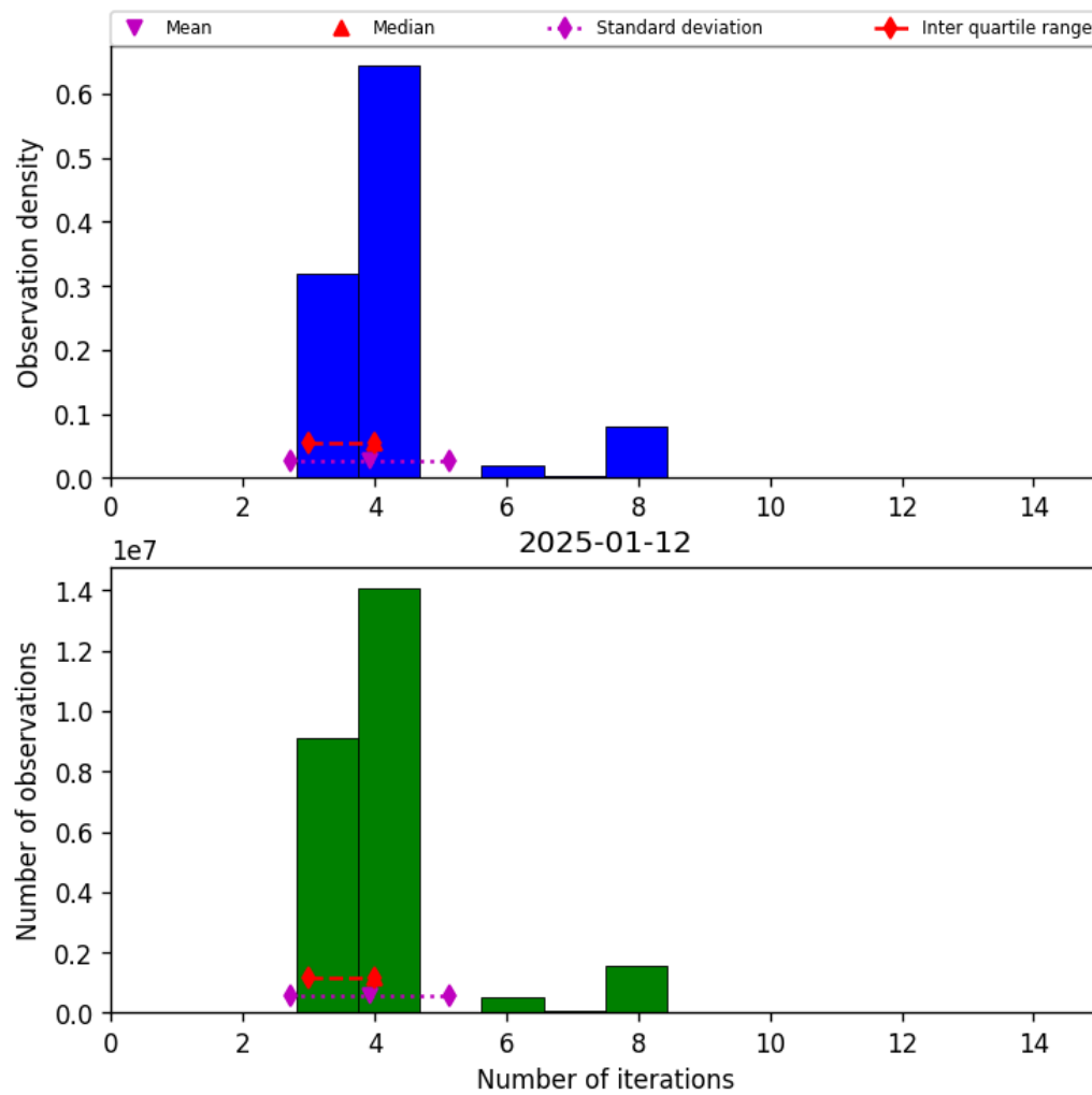
Figure 34: Histogram of “Number of iterations” for 2025-01-12 to 2025-01-13
