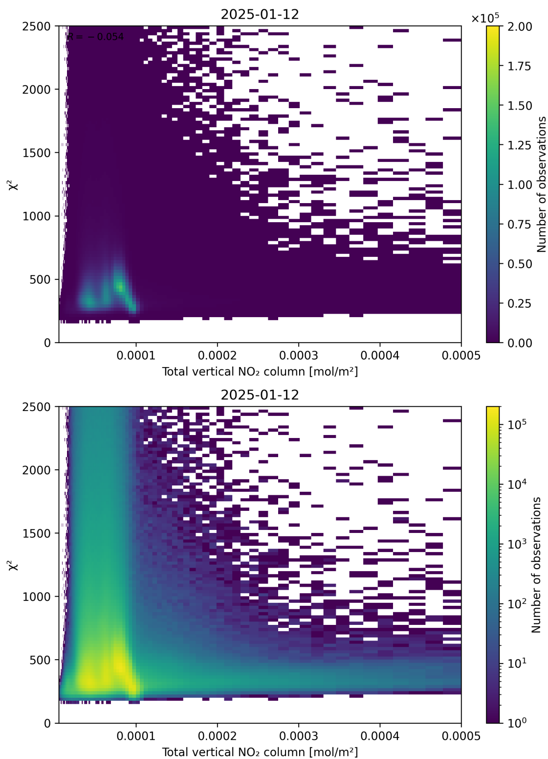
Figure 111: Scatter density plot of “Total vertical NO 2 column” against “ \chi^2 ” for 2025-01-12 to 2025-01-13.
