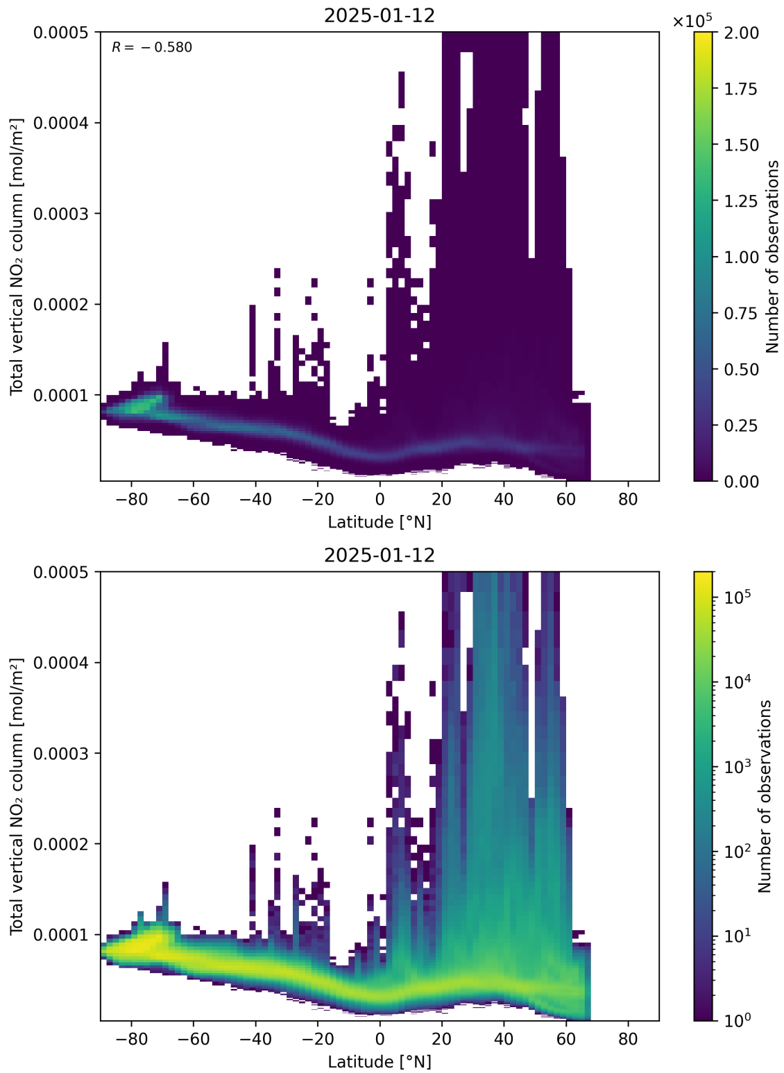
Figure 90: Scatter density plot of “Latitude” against “Total vertical NO 2 column” for 2025-01-12 to 2025-01-13.
