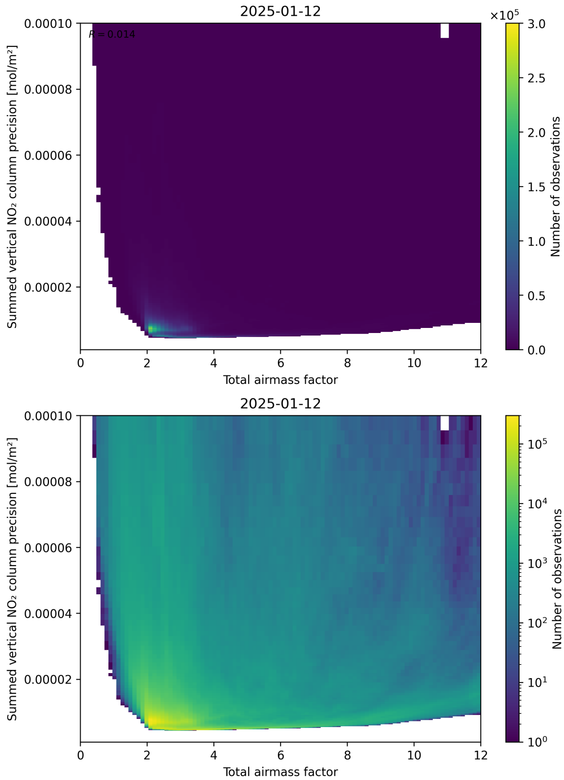
Figure 66: Scatter density plot of “Total airmass factor” against “Summed vertical NO 2 column precision” for 2025-01-12 to 2025-01-13.
