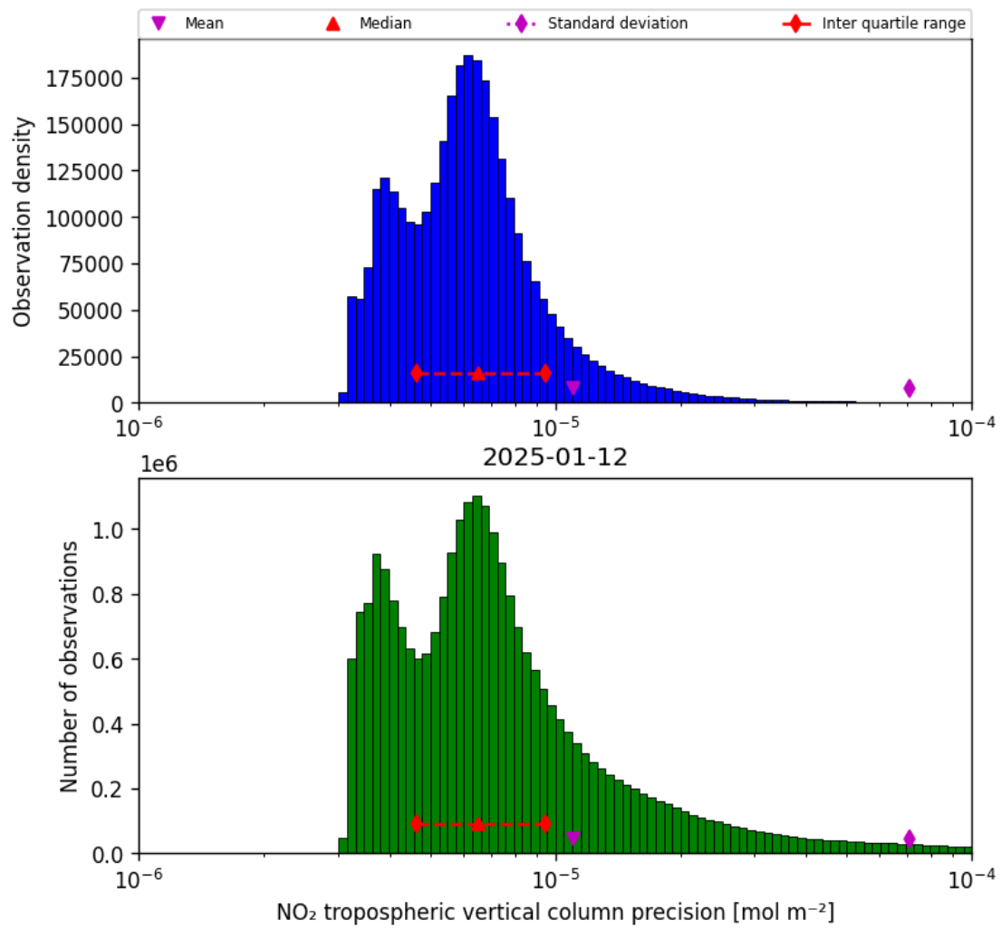
Figure 30: Histogram of “NO 2 tropospheric vertical column precision” for 2025-01-12 to 2025-01-13
