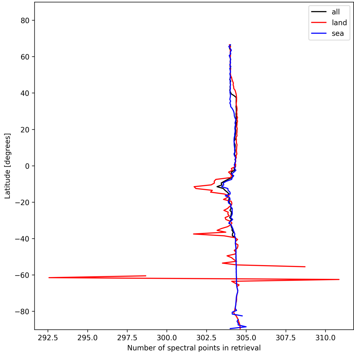
Figure 16: Zonal average of “Number of spectral points in retrieval” for 2025-01-12 to 2025-01-13.
