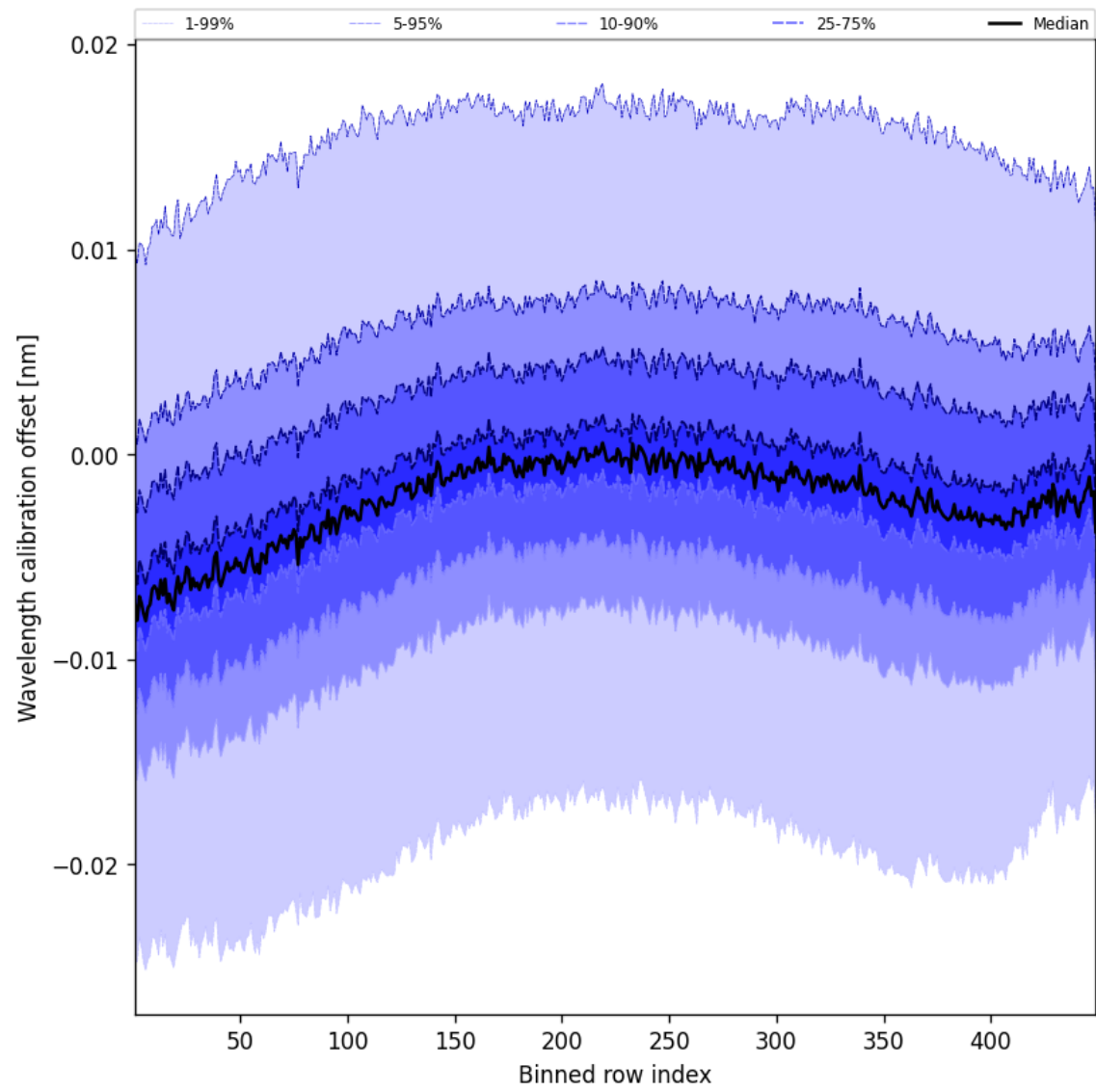
Figure 52: Along track statistics of “Wavelength calibration offset” for 2025-01-12 to 2025-01-13
