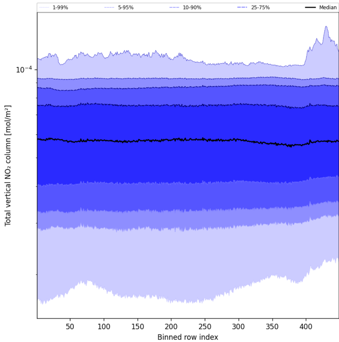
Figure 55: Along track statistics of “Total vertical NO 2 column” for 2025-01-12 to 2025-01-13
