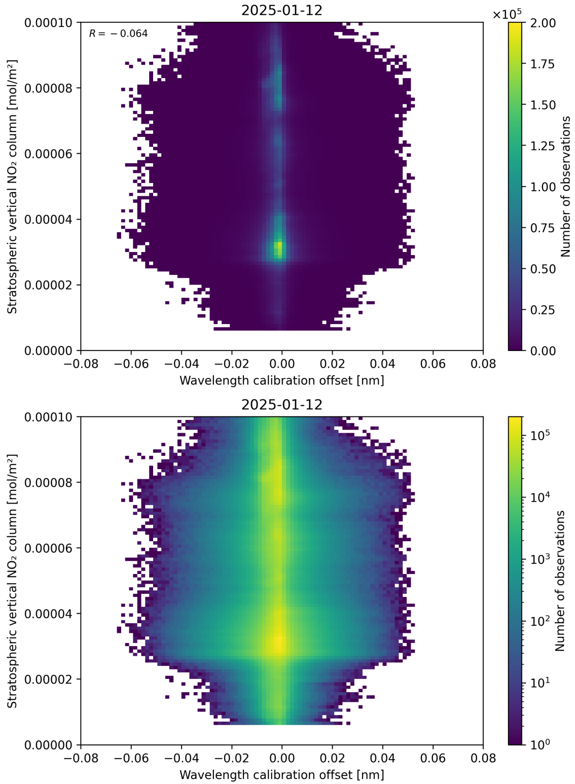
Figure 176: Scatter density plot of “Wavelength calibration offset” against “Stratospheric vertical NO 2 column” for 2025-01-12 to 2025-01-13.
