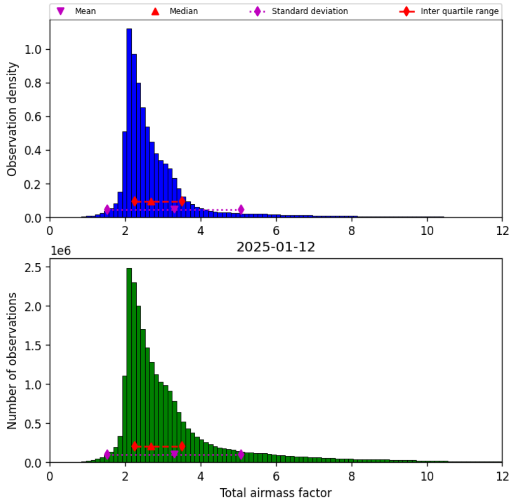
Figure 32: Histogram of “Total airmass factor” for 2025-01-12 to 2025-01-13
