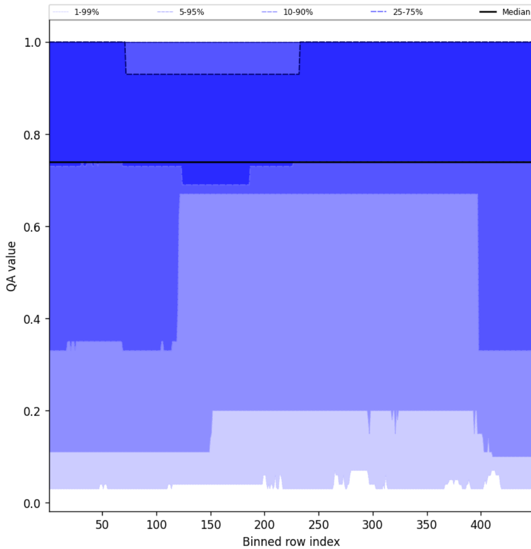
Figure 45: Along track statistics of “QA value” for 2025-01-12 to 2025-01-13
