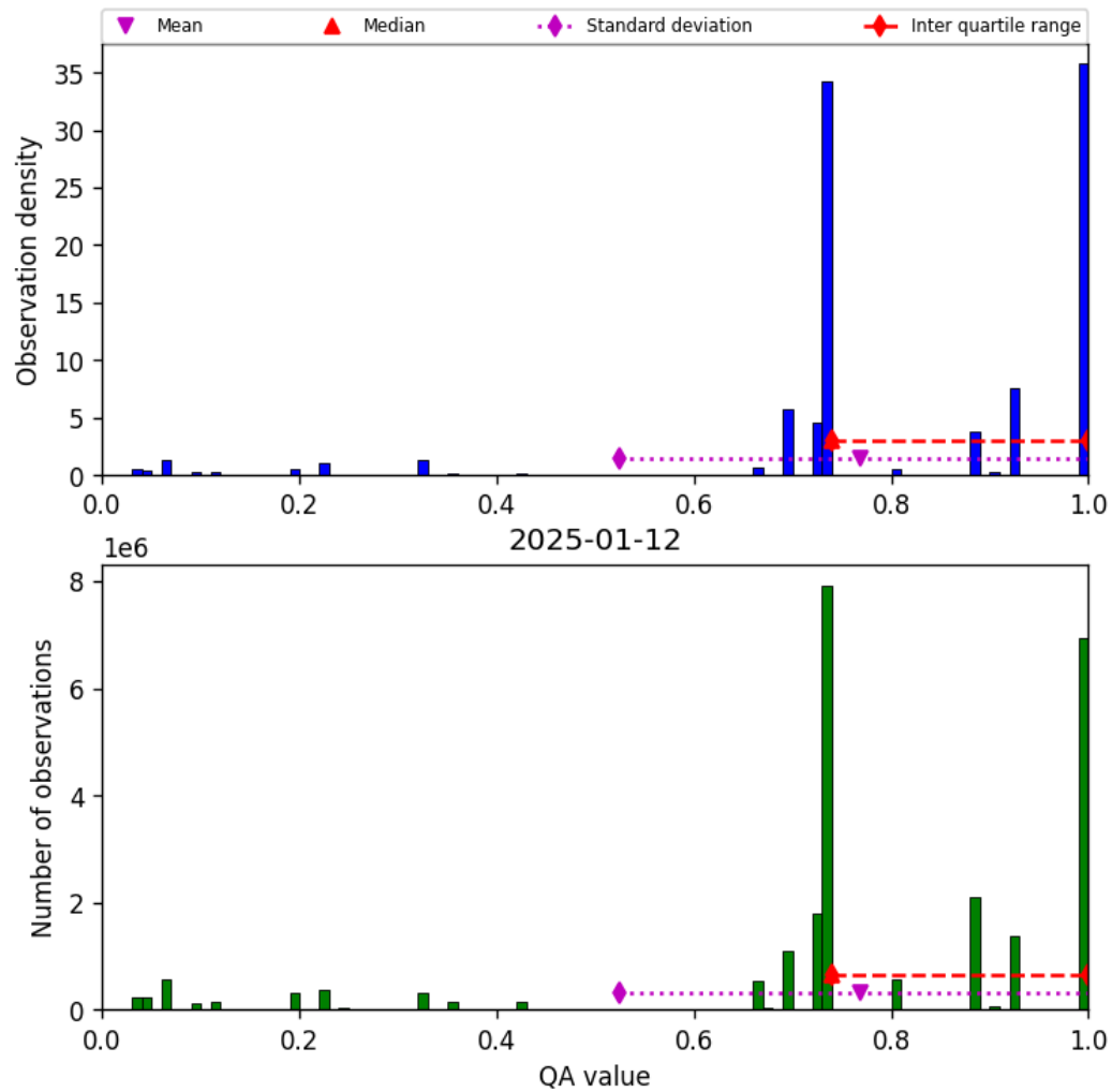
Figure 28: Histogram of “QA value” for 2025-01-12 to 2025-01-13
