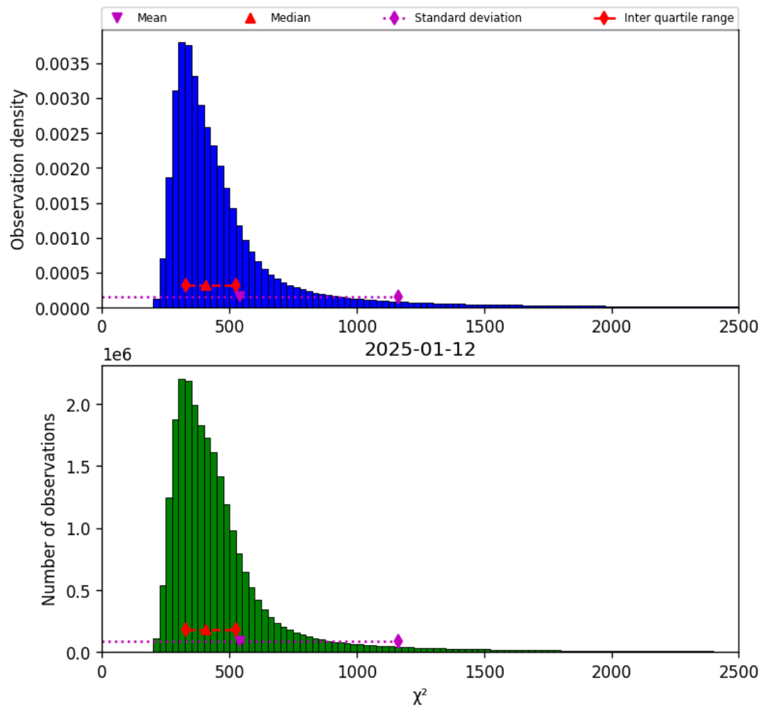
Figure 42: Histogram of “ \chi^2 ” for 2025-01-12 to 2025-01-13
