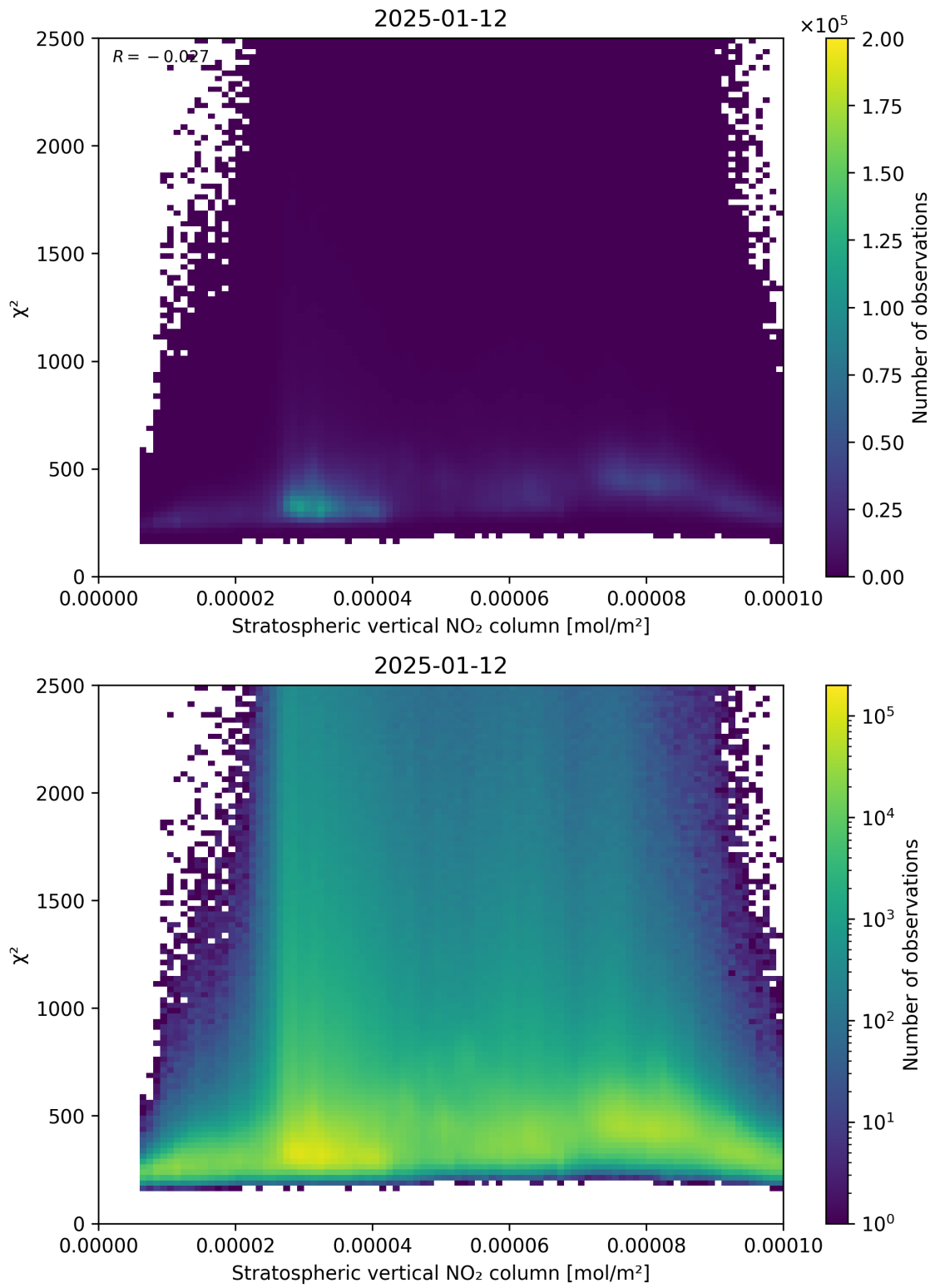
Figure 97: Scatter density plot of “Stratospheric vertical NO 2 column” against “ \chi^2 ” for 2025-01-12 to 2025-01-13.
