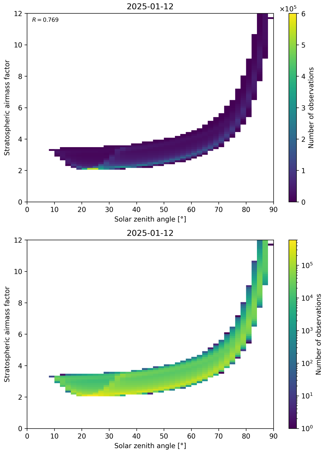
Figure 145: Scatter density plot of “Solar zenith angle” against “Stratospheric airmass factor” for 2025-01-12 to 2025-01-13.
