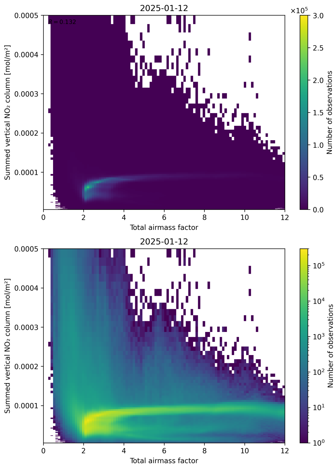
Figure 65: Scatter density plot of “Total airmass factor” against “Summed vertical NO 2 column” for 2025-01-12 to 2025-01-13.
