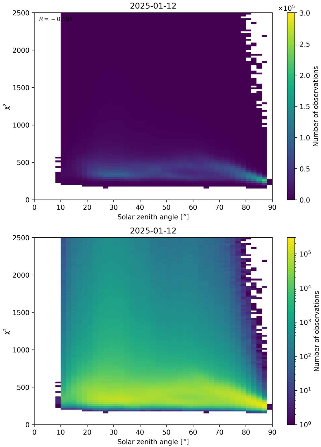
Figure 148: Scatter density plot of “Solar zenith angle” against “ \chi^2 ” for 2025-01-12 to 2025-01-13.
