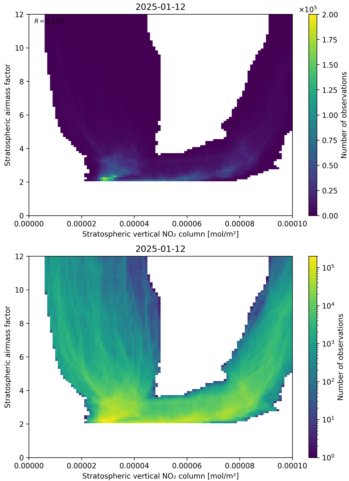
Figure 96: Scatter density plot of “Stratospheric vertical NO 2 column” against “Stratospheric airmass factor” for 2025-01-12 to 2025-01-13.
