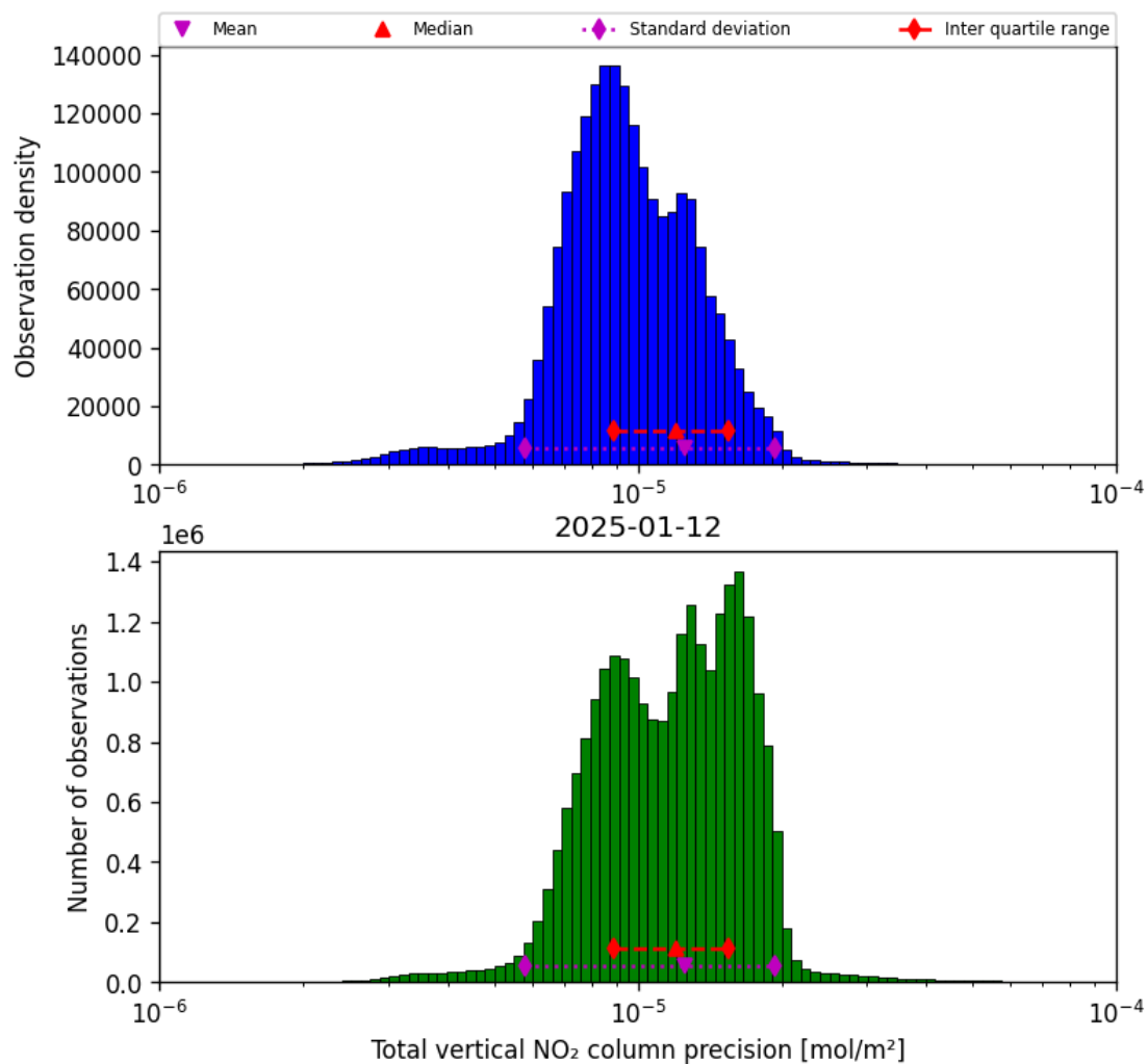
Figure 39: Histogram of “Total vertical NO 2 column precision” for 2025-01-12 to 2025-01-13
