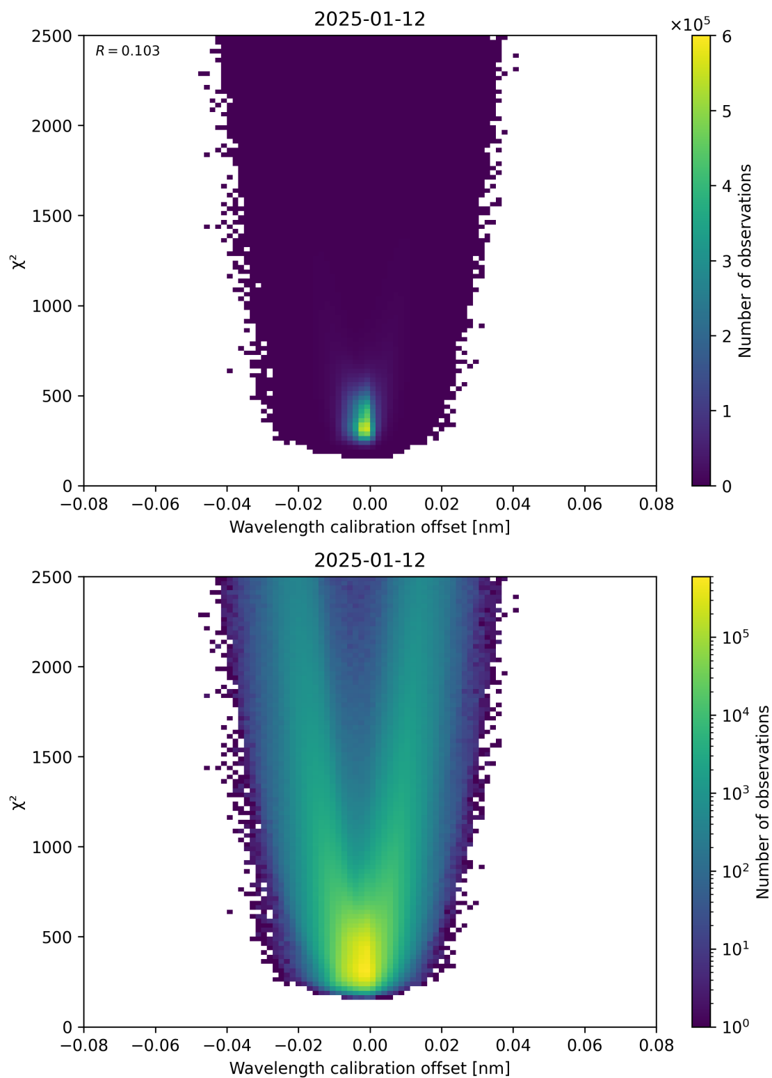
Figure 175: Scatter density plot of “Wavelength calibration offset” against “ \chi^2 ” for 2025-01-12 to 2025-01-13.
