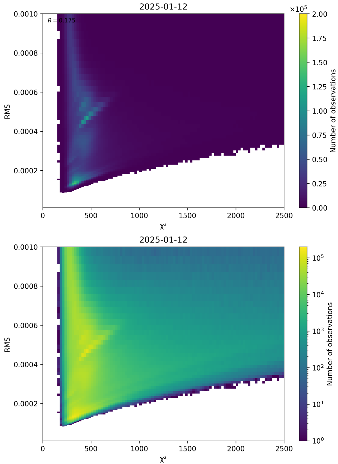
Figure 82: Scatter density plot of “ \chi^2 ” against “RMS” for 2025-01-12 to 2025-01-13.
