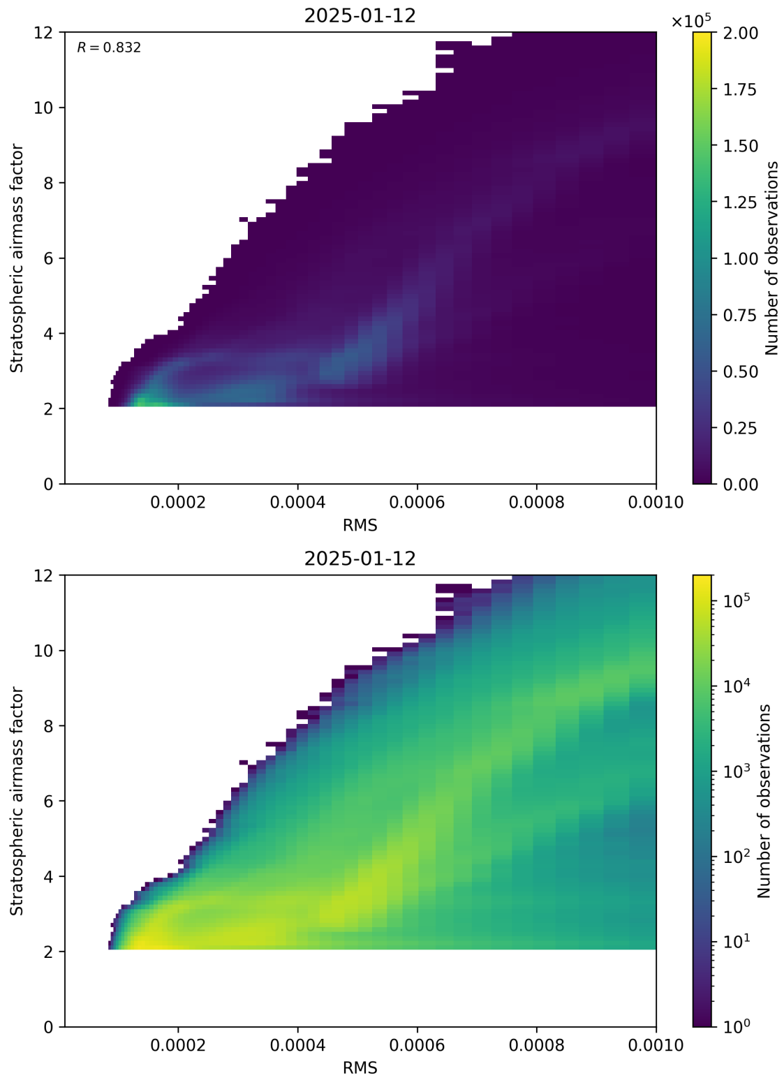
Figure 144: Scatter density plot of “RMS” against “Stratospheric airmass factor” for 2025-01-12 to 2025-01-13.
