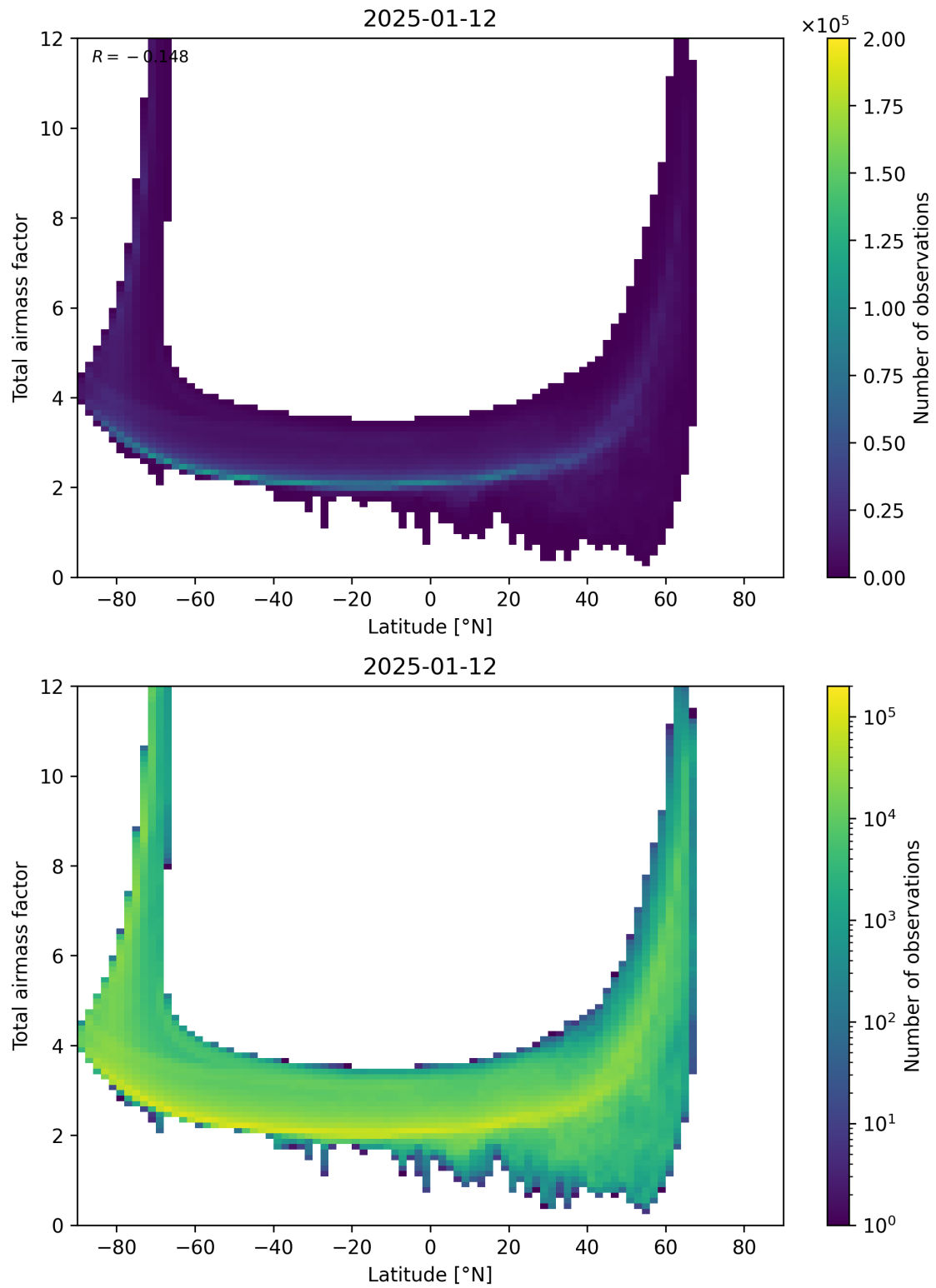
Figure 84: Scatter density plot of “Latitude” against “Total airmass factor” for 2025-01-12 to 2025-01-13.
