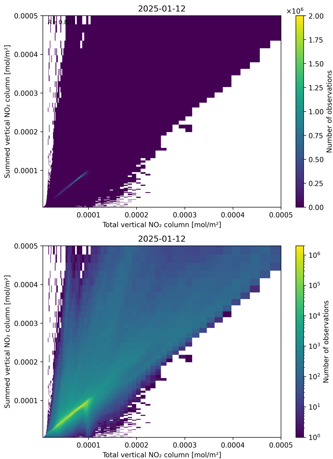
Figure 112: Scatter density plot of “Total vertical NO 2 column” against “Summed vertical NO 2 column” for 2025-01-12 to 2025-01-13.
