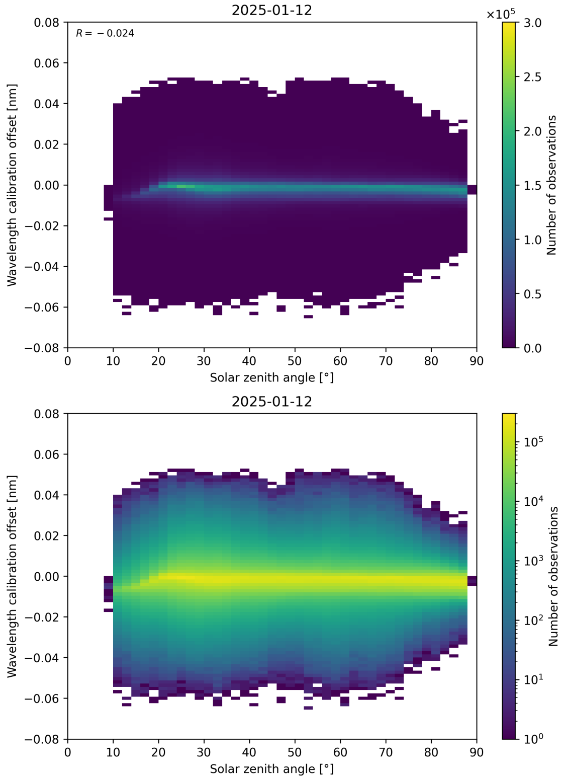
Figure 158: Scatter density plot of “Solar zenith angle” against “Wavelength calibration offset” for 2025-01-12 to 2025-01-13.
