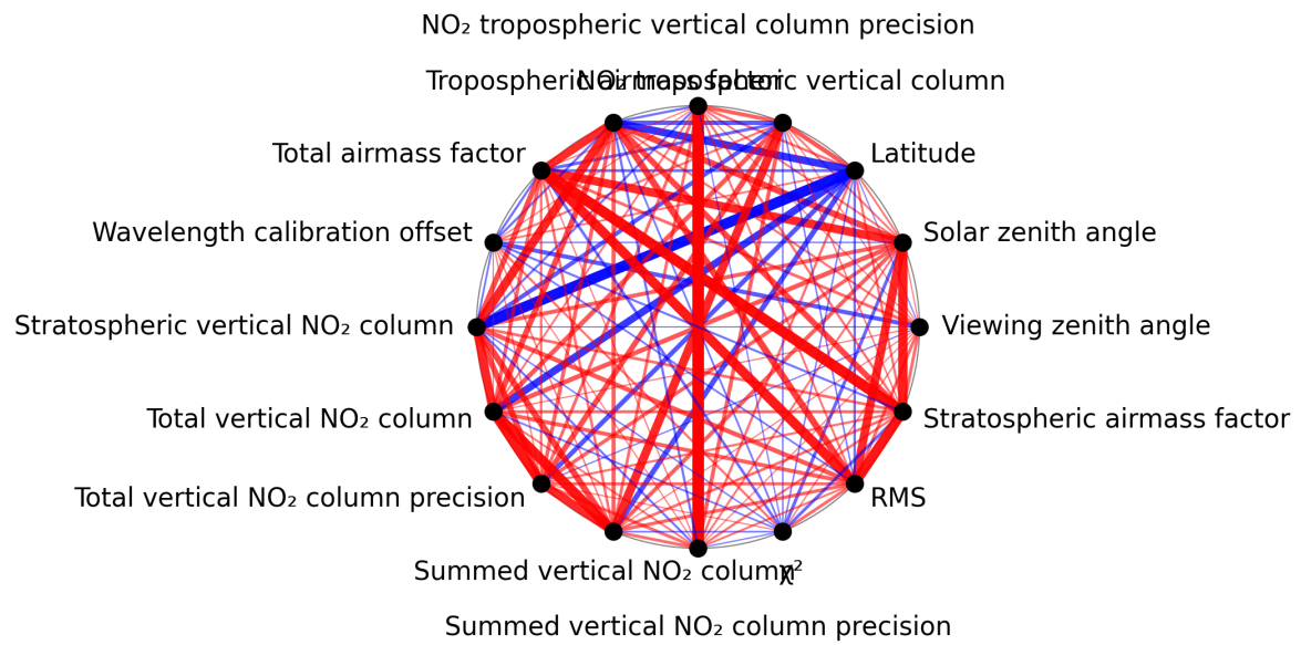
Figure 1: Map of correlation graph for 2025-01-12 to 2025-01-13.
