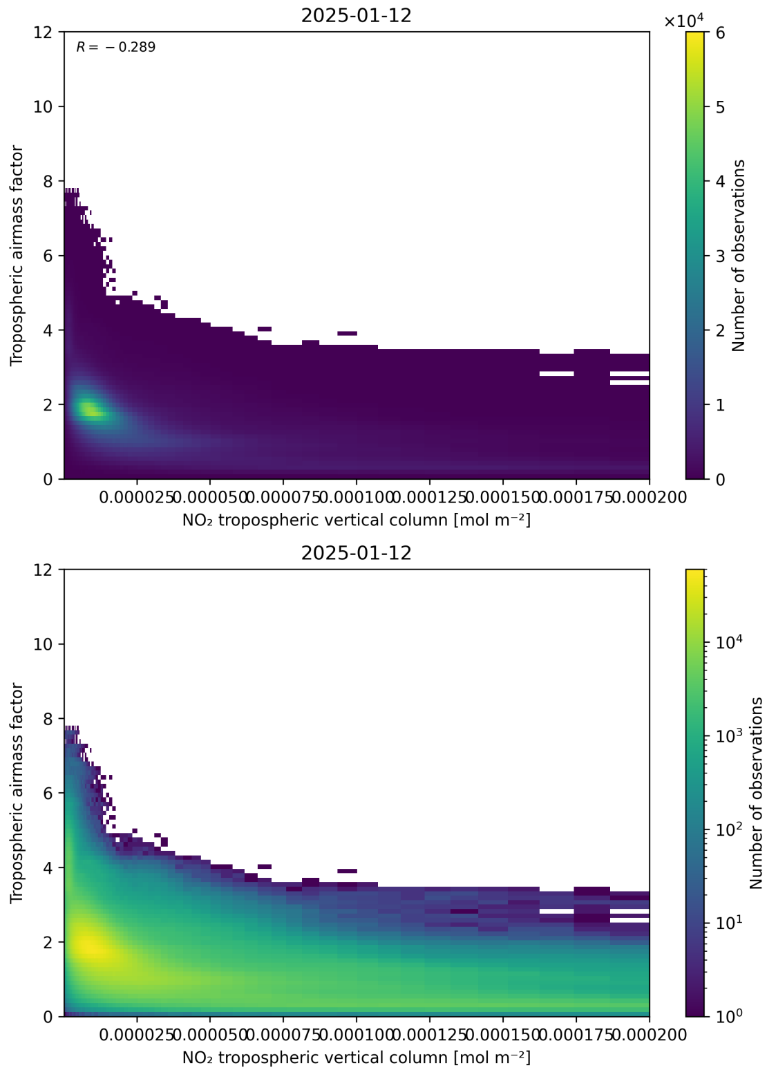
Figure 123: Scatter density plot of “NO 2 tropospheric vertical column” against “Tropospheric air mass factor” for 2025-01-12 to 2025-01-13.
