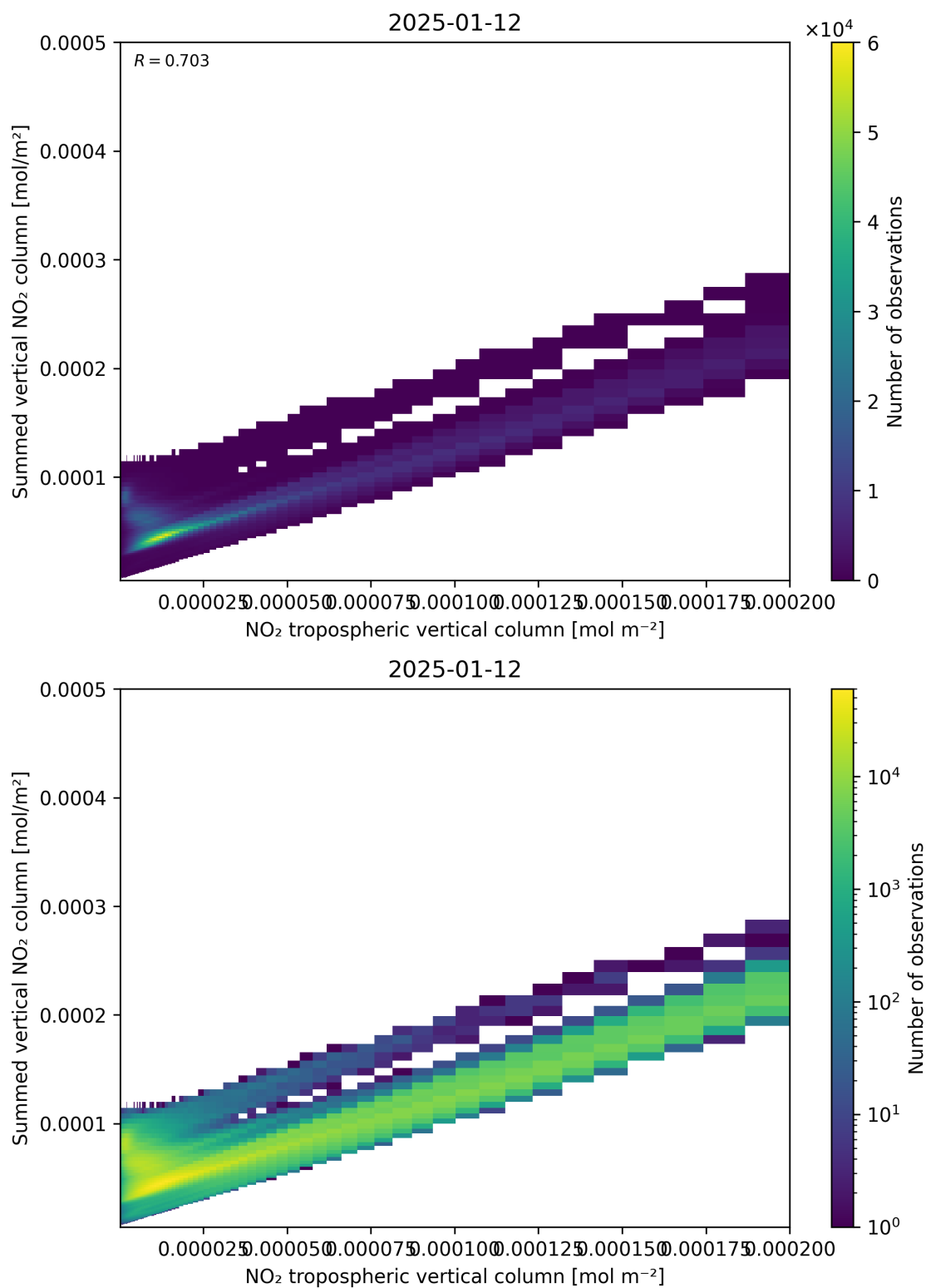
Figure 126: Scatter density plot of “NO 2 tropospheric vertical column” against “Summed vertical NO 2 column” for 2025-01-12 to 2025-01-13.
