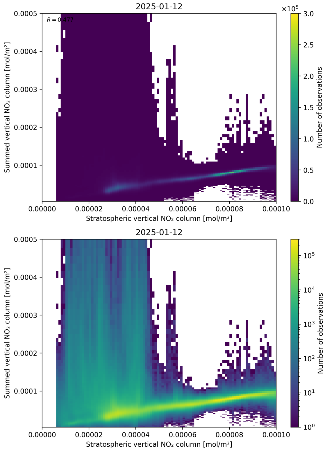
Figure 98: Scatter density plot of “Stratospheric vertical NO 2 column” against “Summed vertical NO 2 column” for 2025-01-12 to 2025-01-13.
