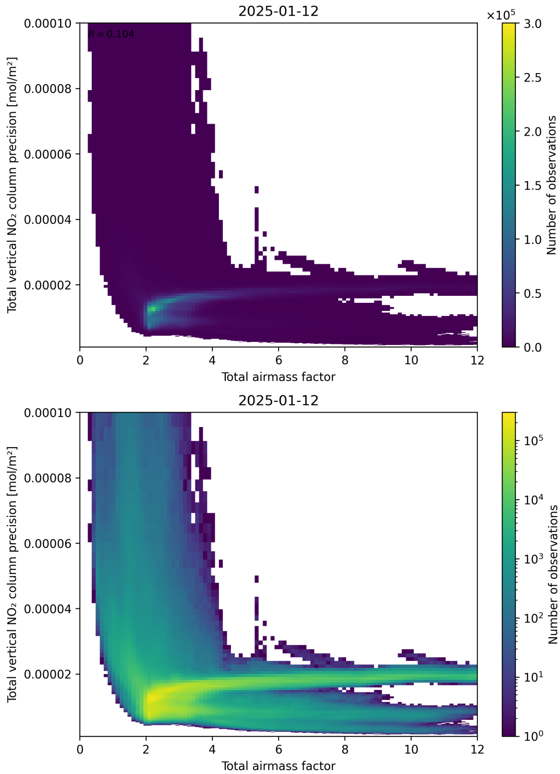
Figure 68: Scatter density plot of “Total airmass factor” against “Total vertical NO 2 column precision” for 2025-01-12 to 2025-01-13.
