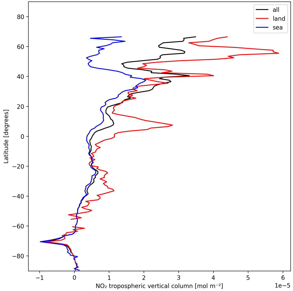
Figure 12: Zonal average of “NO 2 tropospheric vertical column” for 2025-01-12 to 2025-01-13.
