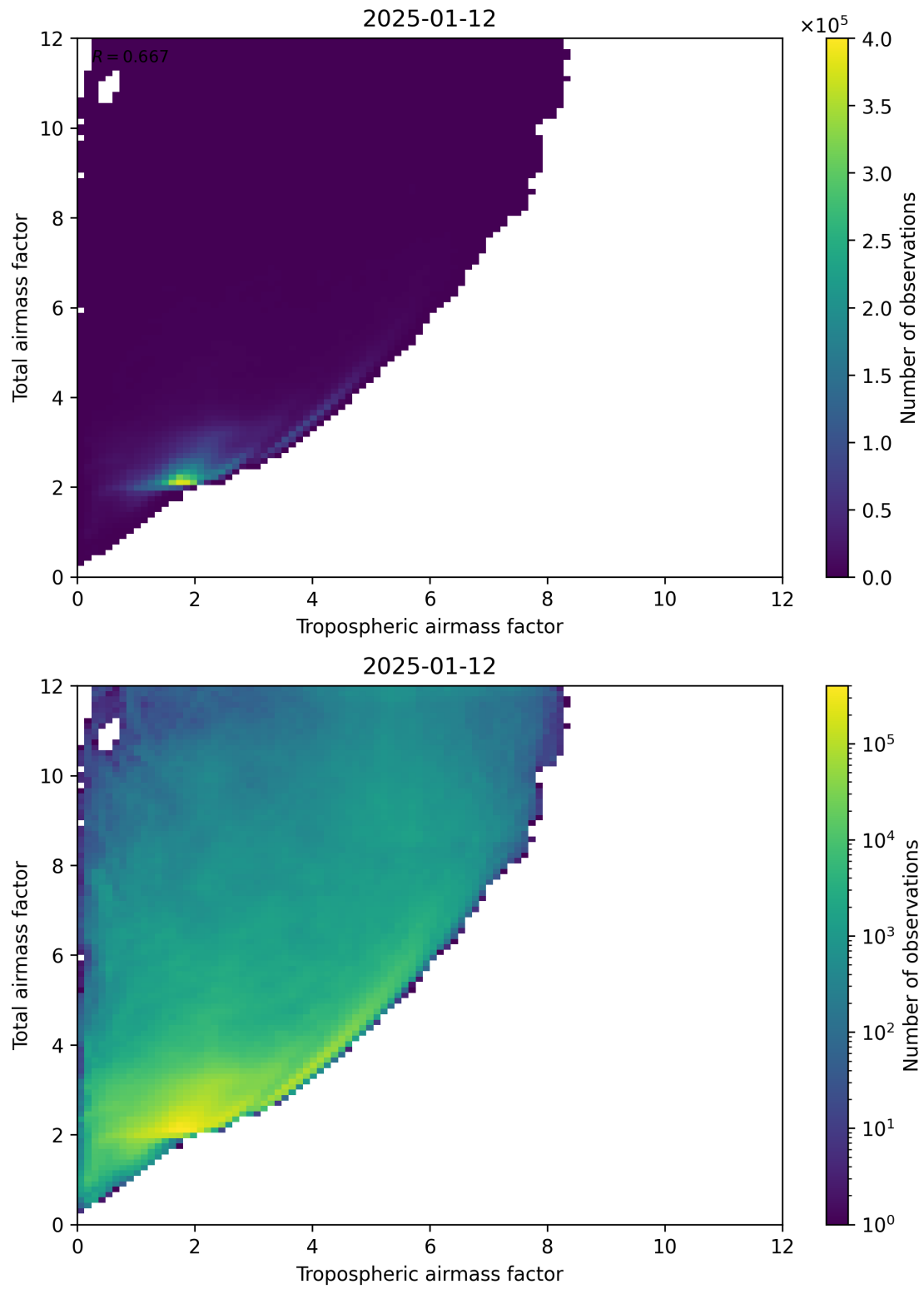
Figure 72: Scatter density plot of “Tropospheric airmass factor” against “Total airmass factor” for 2025-01-12 to 2025-01-13.
