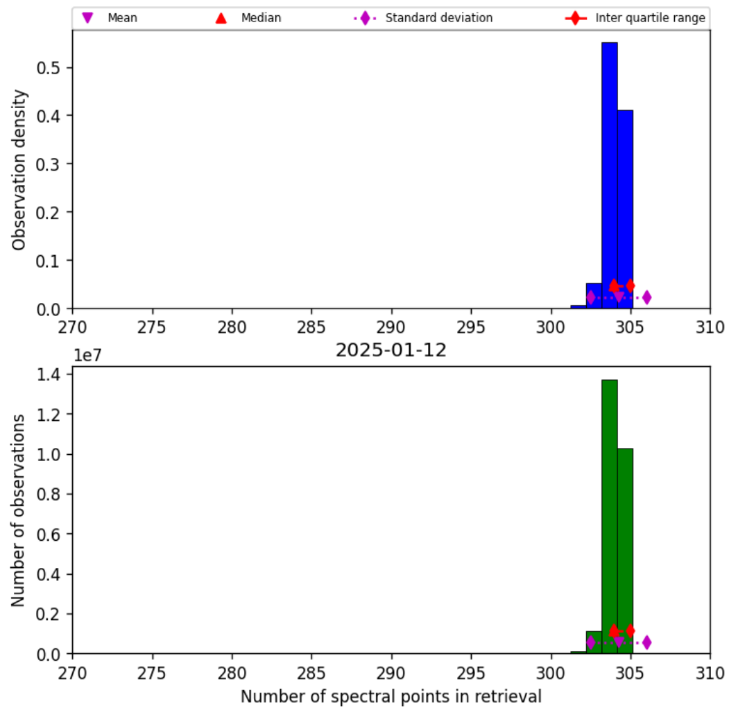
Figure 33: Histogram of “Number of spectral points in retrieval” for 2025-01-12 to 2025-01-13
