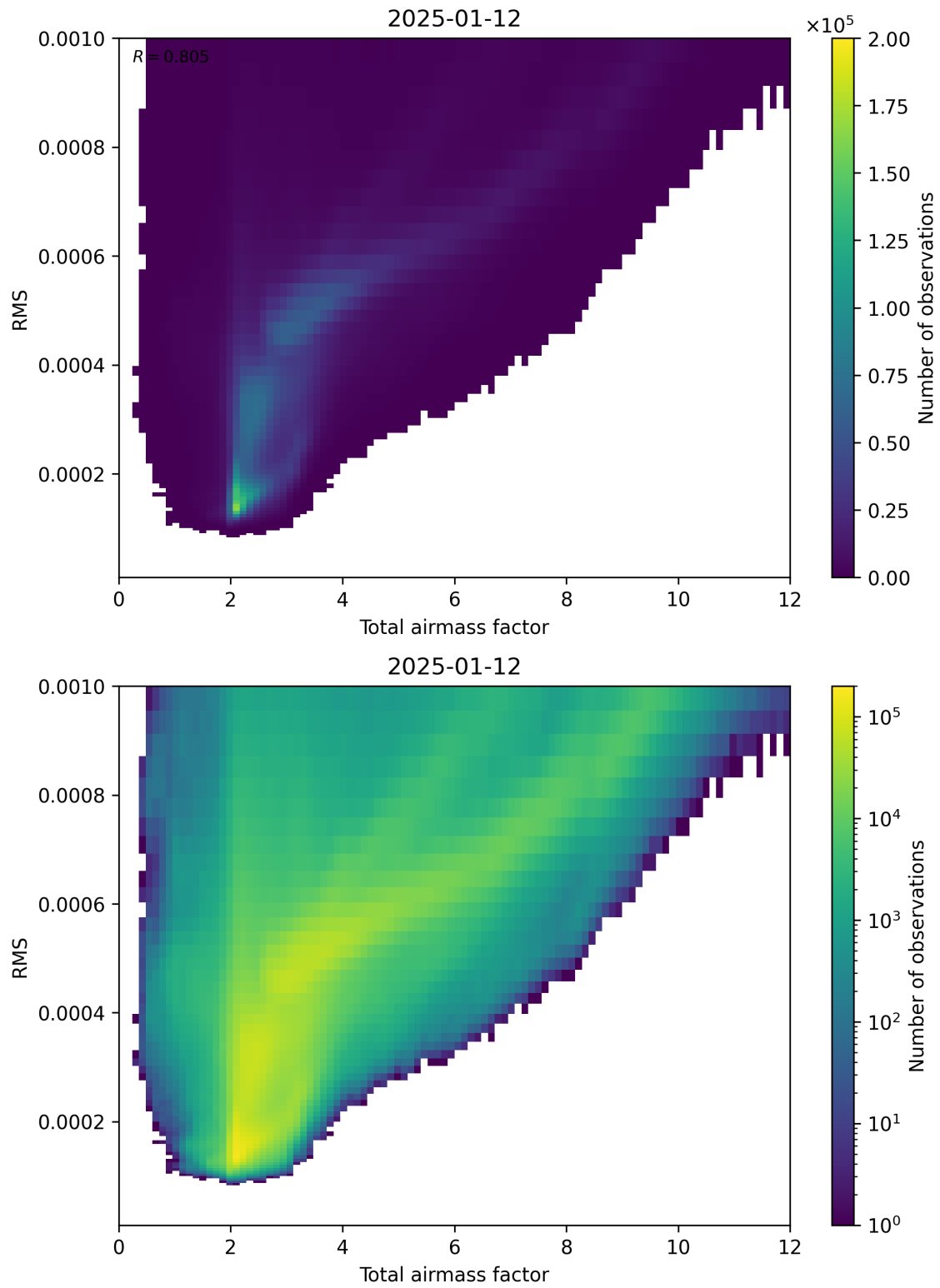
Figure 69: Scatter density plot of “Total airmass factor” against “RMS” for 2025-01-12 to 2025-01-13.
