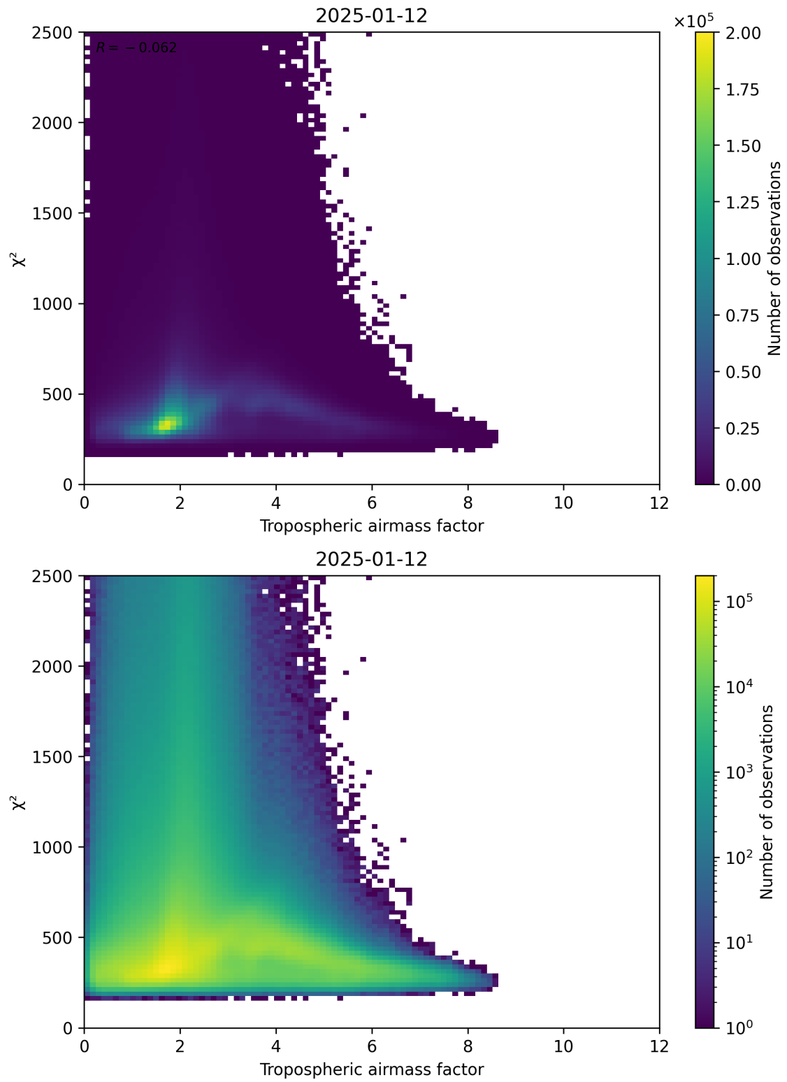
Figure 73: Scatter density plot of “Tropospheric airmass factor” against “ \chi^2 ” for 2025-01-12 to 2025-01-13.
