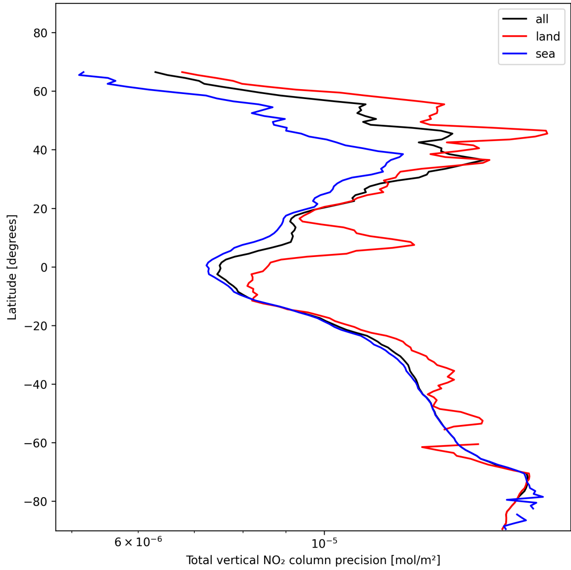
Figure 22: Zonal average of “Total vertical NO 2 column precision” for 2025-01-12 to 2025-01-13.
