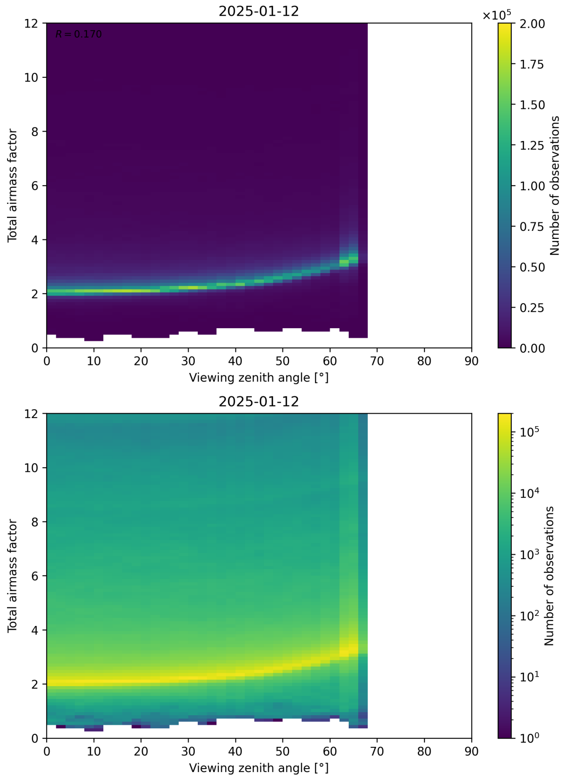
Figure 160: Scatter density plot of “Viewing zenith angle” against “Total airmass factor” for 2025-01-12 to 2025-01-13.
