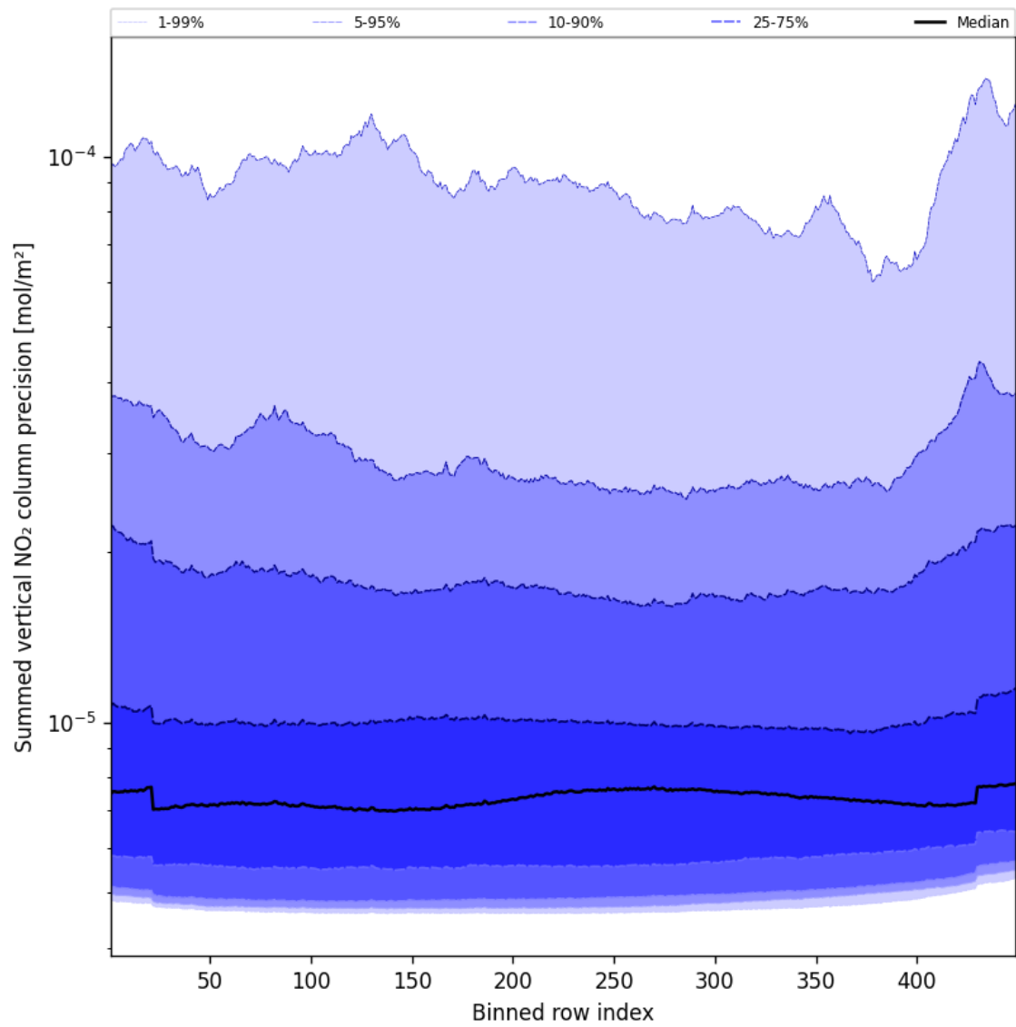
Figure 58: Along track statistics of “Summed vertical NO 2 column precision” for 2025-01-12 to 2025-01-13
