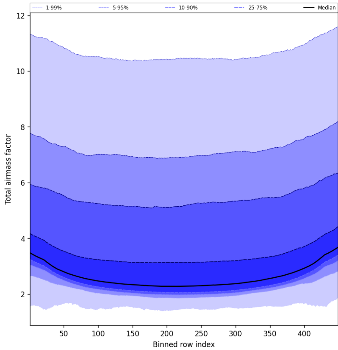
Figure 49: Along track statistics of “Total airmass factor” for 2025-01-12 to 2025-01-13
