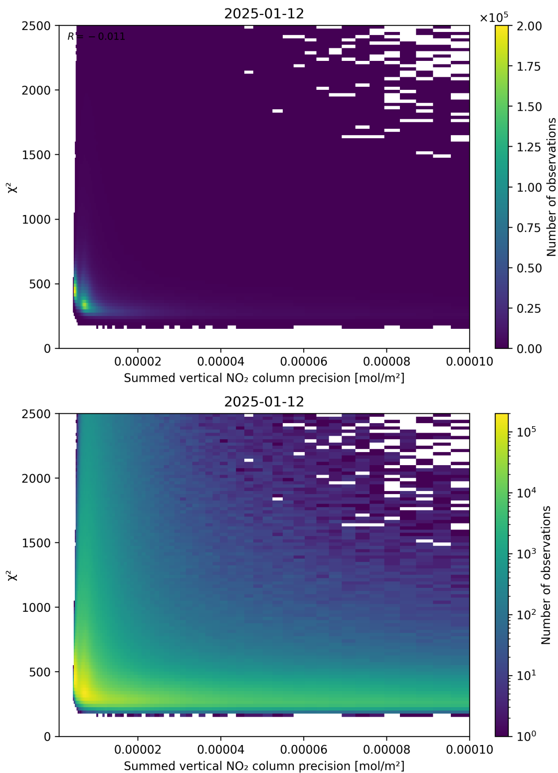
Figure 107: Scatter density plot of “Summed vertical NO 2 column precision” against “ \chi^2 ” for 2025-01-12 to 2025-01-13.
