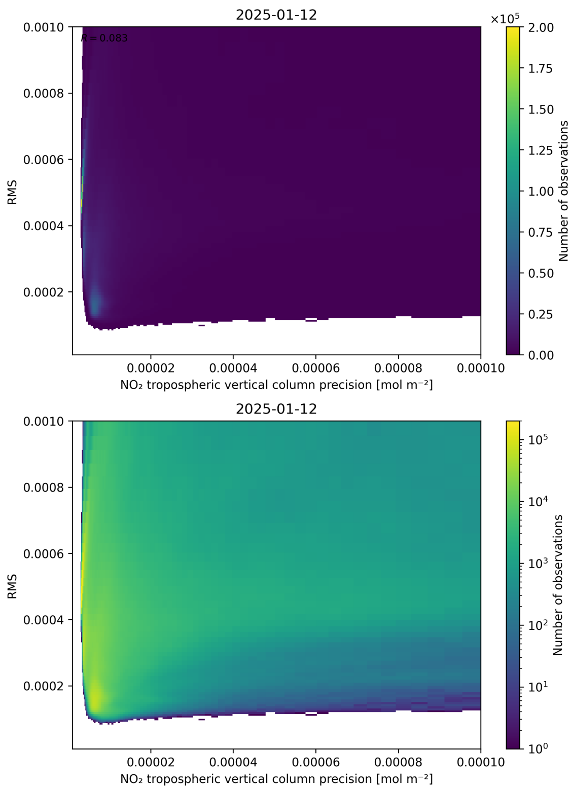
Figure 140: Scatter density plot of “NO 2 tropospheric vertical column precision” against “RMS” for 2025-01-12 to 2025-01-13.
