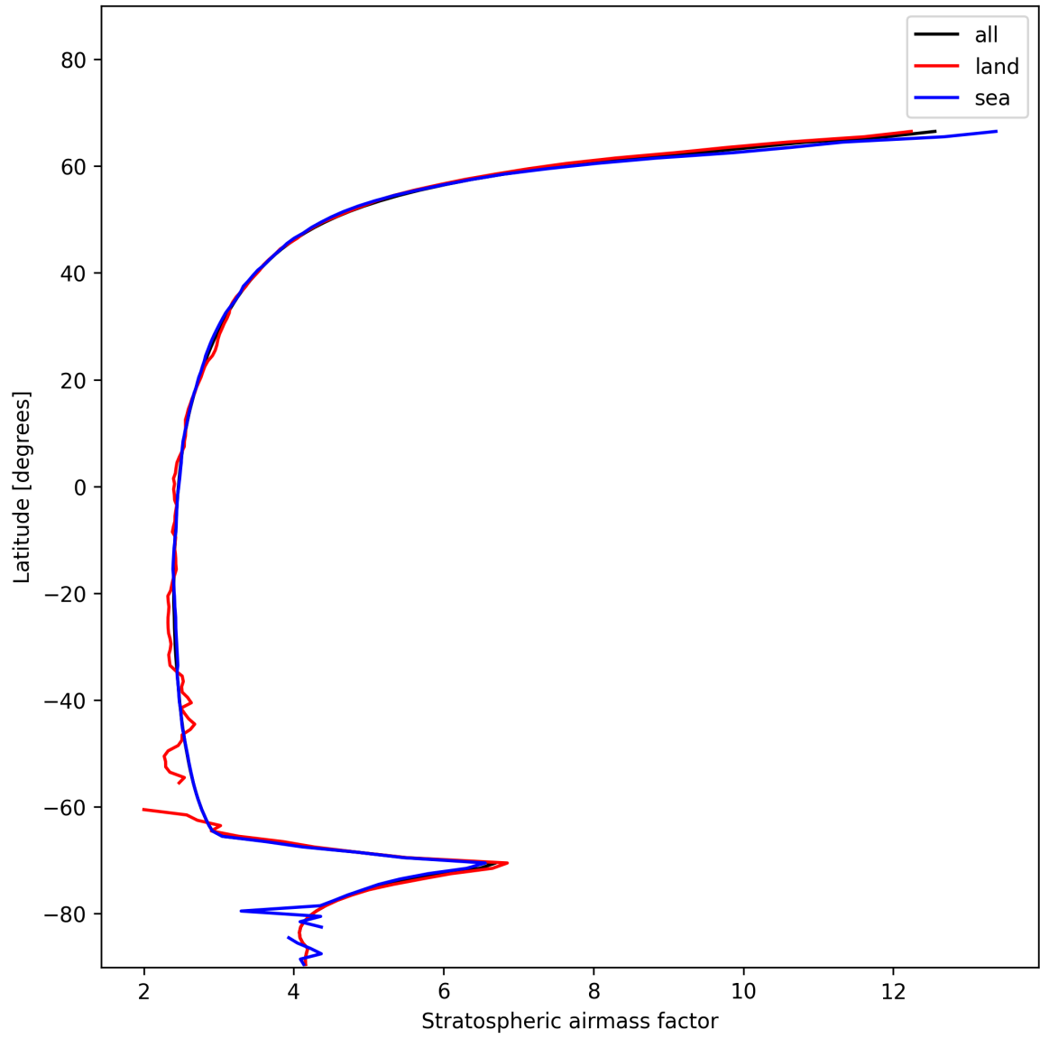
Figure 27: Zonal average of “Stratospheric airmass factor” for 2025-01-12 to 2025-01-13.
