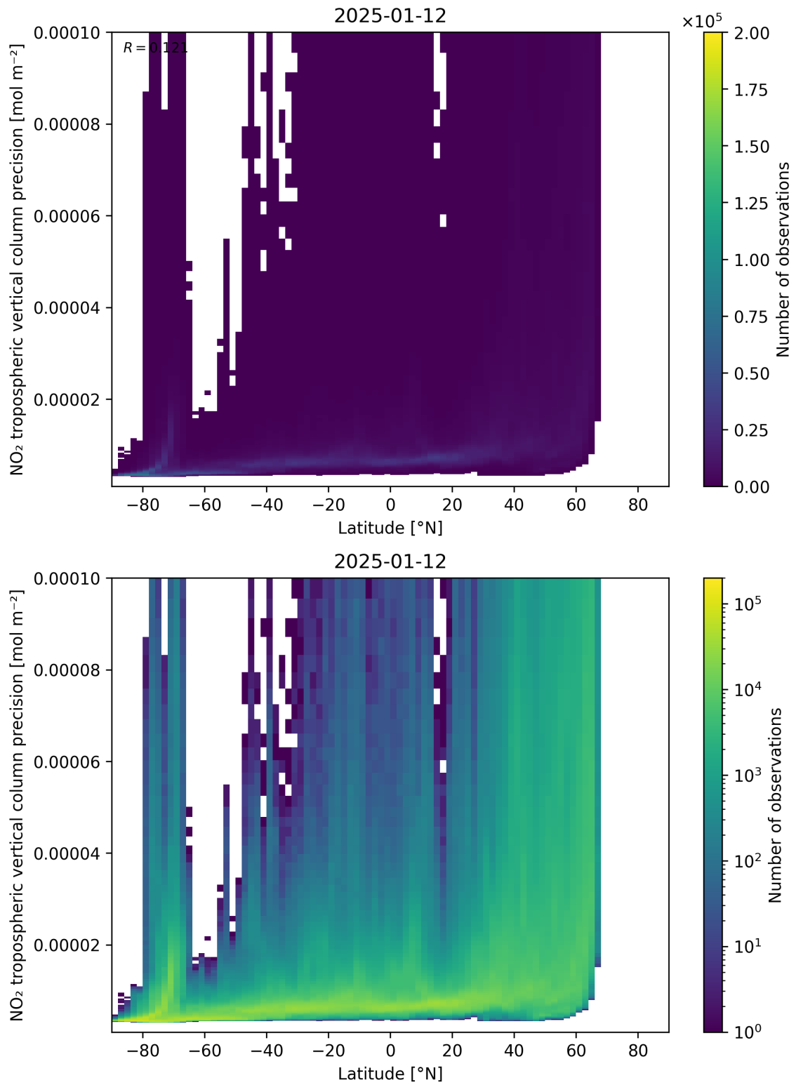
Figure 93: Scatter density plot of “Latitude” against “NO 2 tropospheric vertical column precision” for 2025-01-12 to 2025-01-13.
