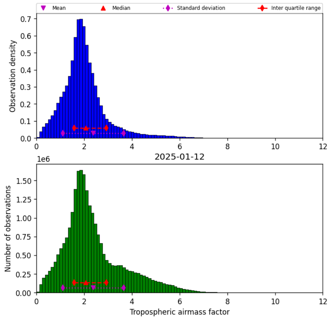
Figure 31: Histogram of “Tropospheric airmass factor” for 2025-01-12 to 2025-01-13
