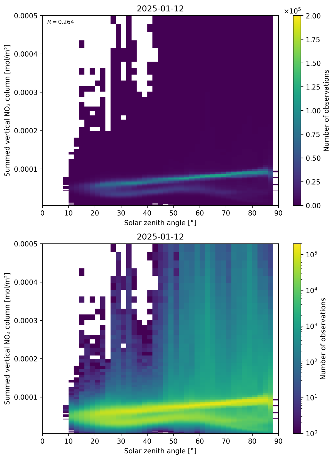
Figure 151: Scatter density plot of “Solar zenith angle” against “Summed vertical NO 2 column” for 2025-01-12 to 2025-01-13.
