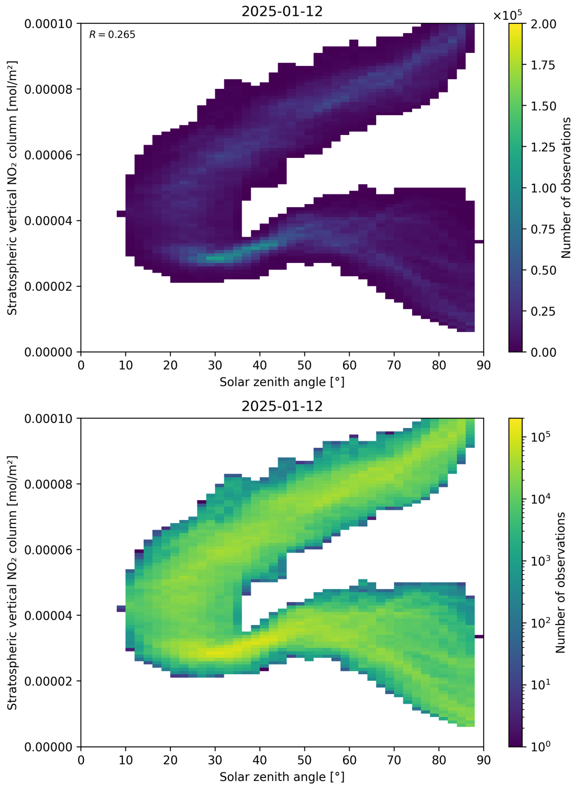
Figure 150: Scatter density plot of “Solar zenith angle” against “Stratospheric vertical NO 2 column” for 2025-01-12 to 2025-01-13.
