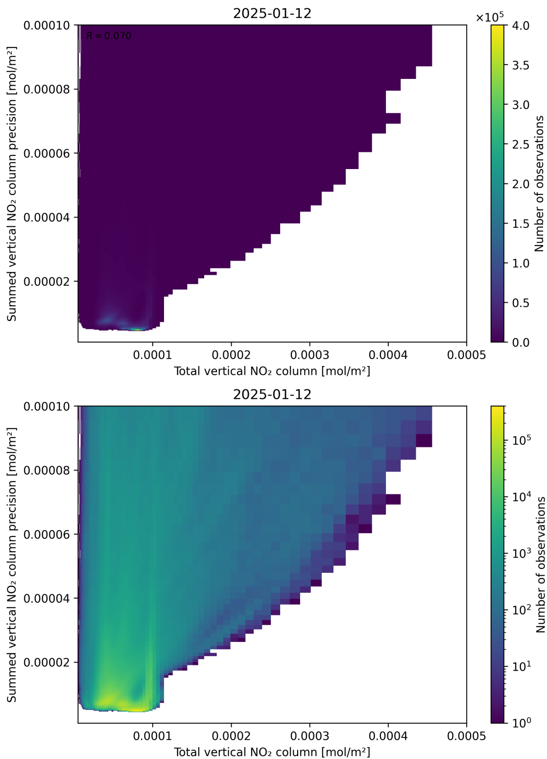
Figure 113: Scatter density plot of “Total vertical NO 2 column” against “Summed vertical NO 2 column precision” for 2025-01-12 to 2025-01-13.
