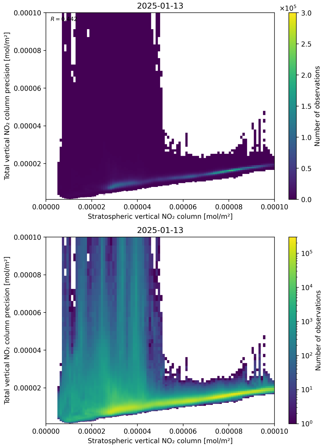
Figure 101: Scatter density plot of “Stratospheric vertical NO 2 column” against “Total vertical NO 2 column precision” for 2025-01-12 to 2025-01-14.
