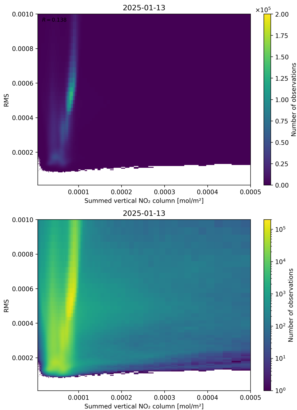
Figure 109: Scatter density plot of “Summed vertical NO 2 column” against “RMS” for 2025-01-12 to 2025-01-14.
