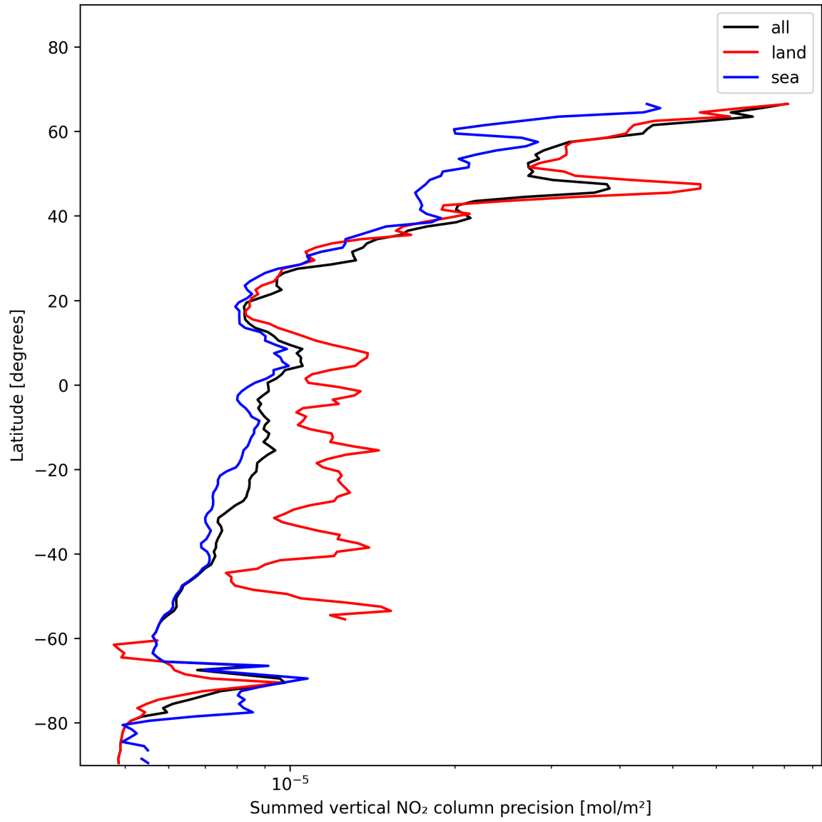
Figure 24: Zonal average of “Summed vertical NO 2 column precision” for 2025-01-12 to 2025-01-14.
