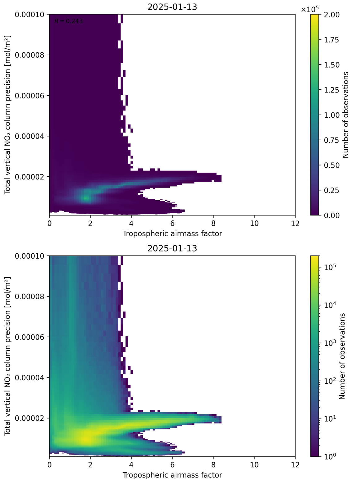
Figure 78: Scatter density plot of “Tropospheric air mass factor” against “Total vertical NO 2 column precision” for 2025-01-12 to 2025-01-14.
