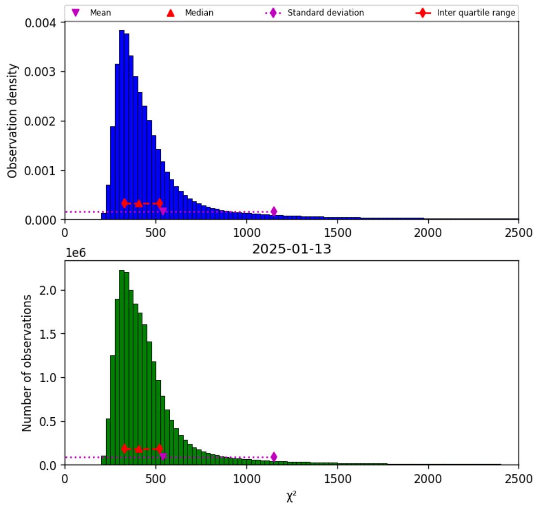
Figure 42: Histogram of “ \chi^2 ” for 2025-01-12 to 2025-01-14
