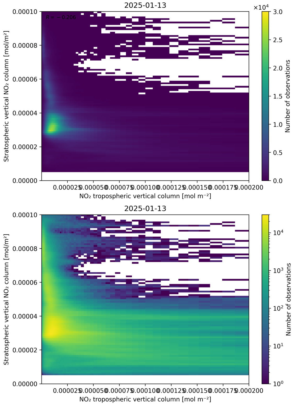
Figure 125: Scatter density plot of “NO 2 tropospheric vertical column” against “Stratospheric vertical NO 2 column” for 2025-01-12 to 2025-01-14.
