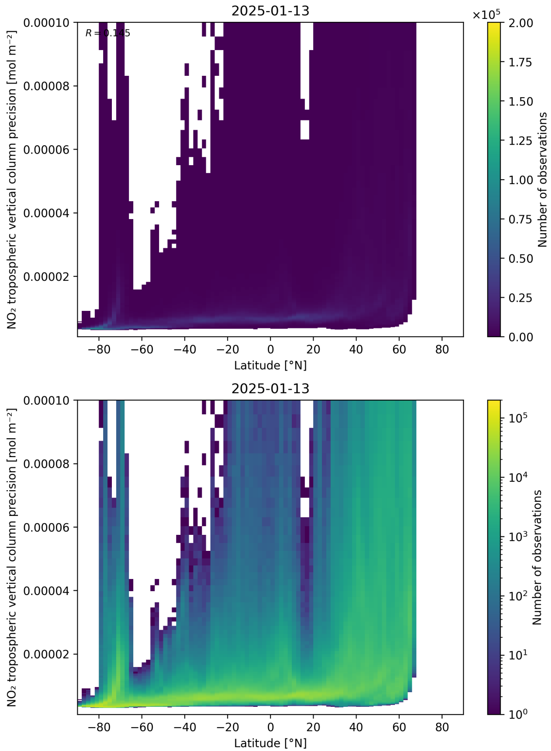
Figure 93: Scatter density plot of “Latitude” against “NO 2 tropospheric vertical column precision” for 2025-01-12 to 2025-01-14.
