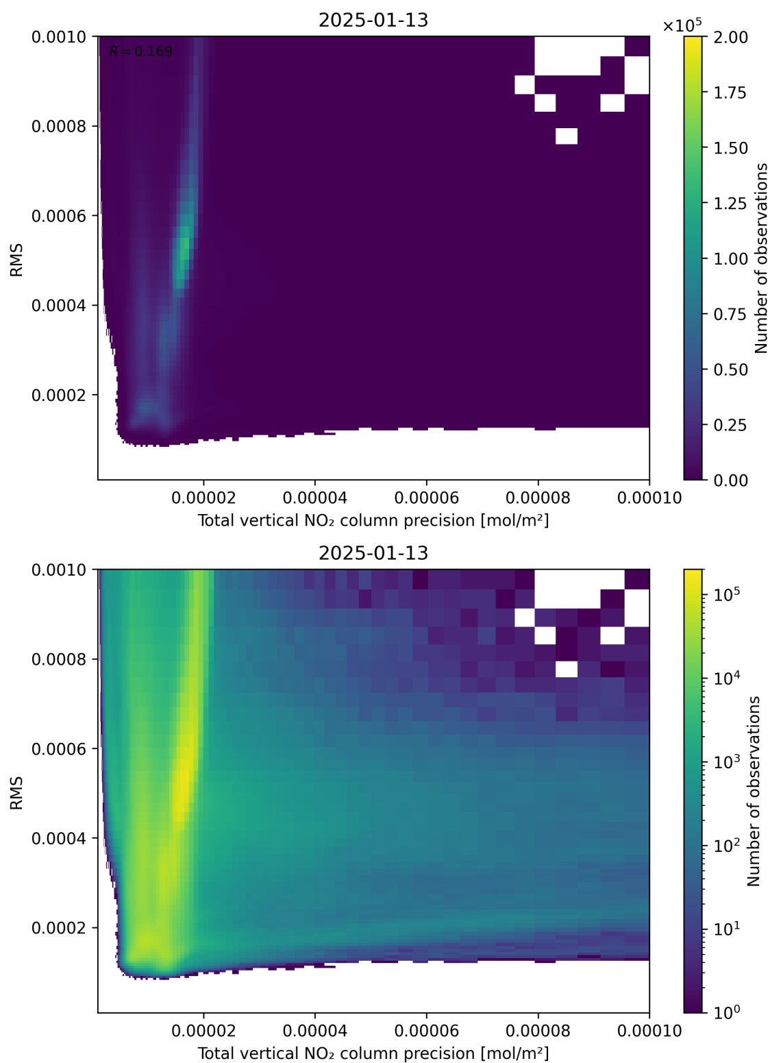
Figure 119: Scatter density plot of “Total vertical NO 2 column precision” against “RMS” for 2025-01-12 to 2025-01-14.
