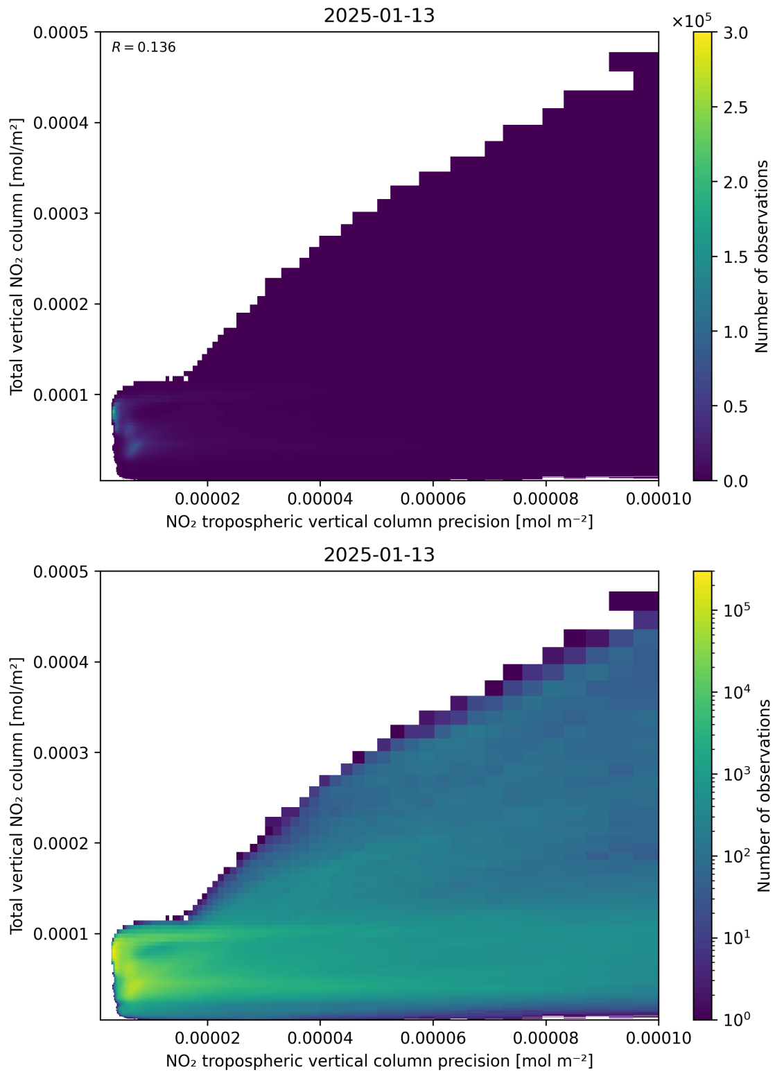
Figure 138: Scatter density plot of “NO 2 tropospheric vertical column precision” against “Total vertical NO 2 column” for 2025-01-12 to 2025-01-14.
