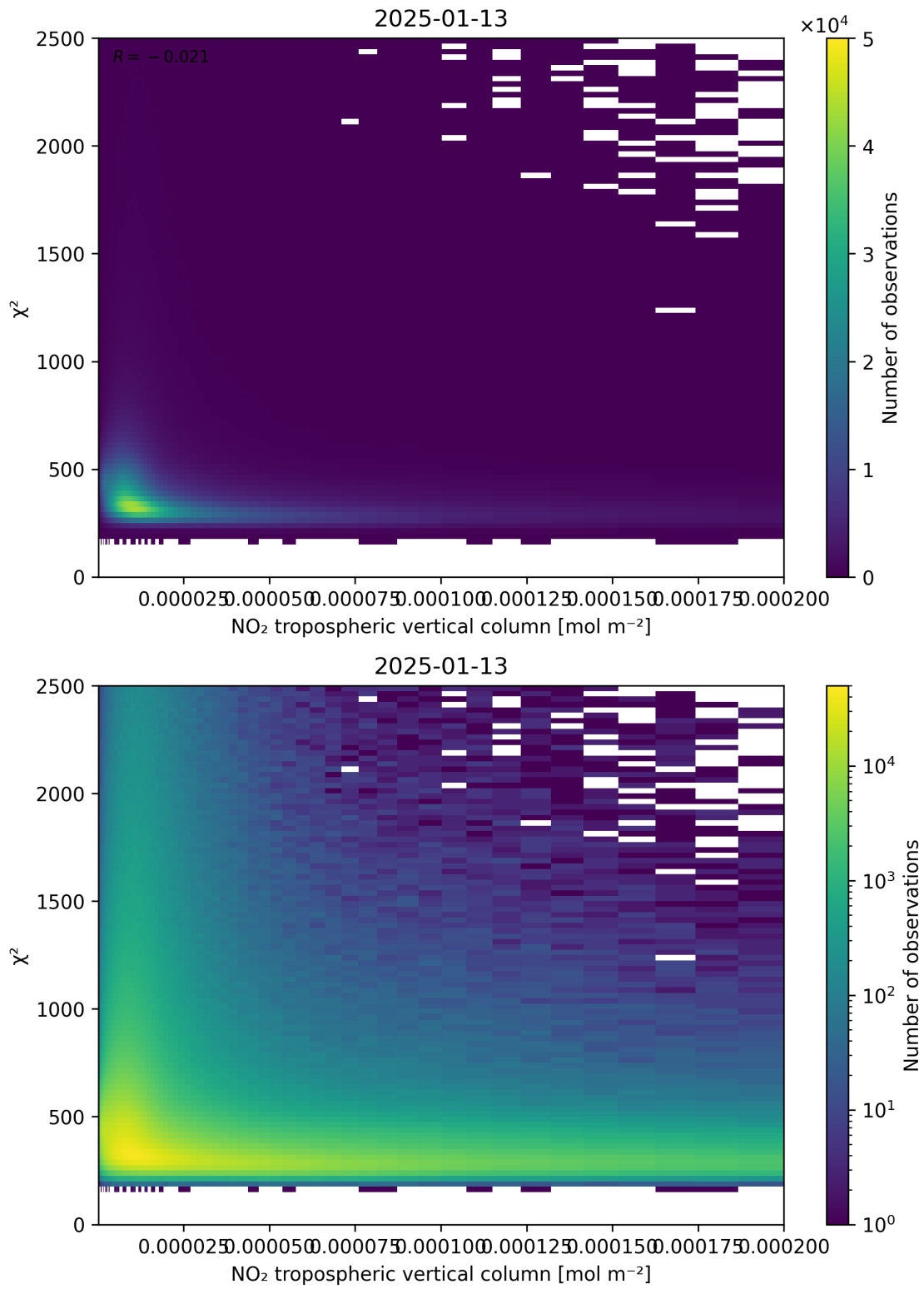
Figure 124: Scatter density plot of “NO 2 tropospheric vertical column” against “ \chi^2 ” for 2025-01-12 to 2025-01-14.
