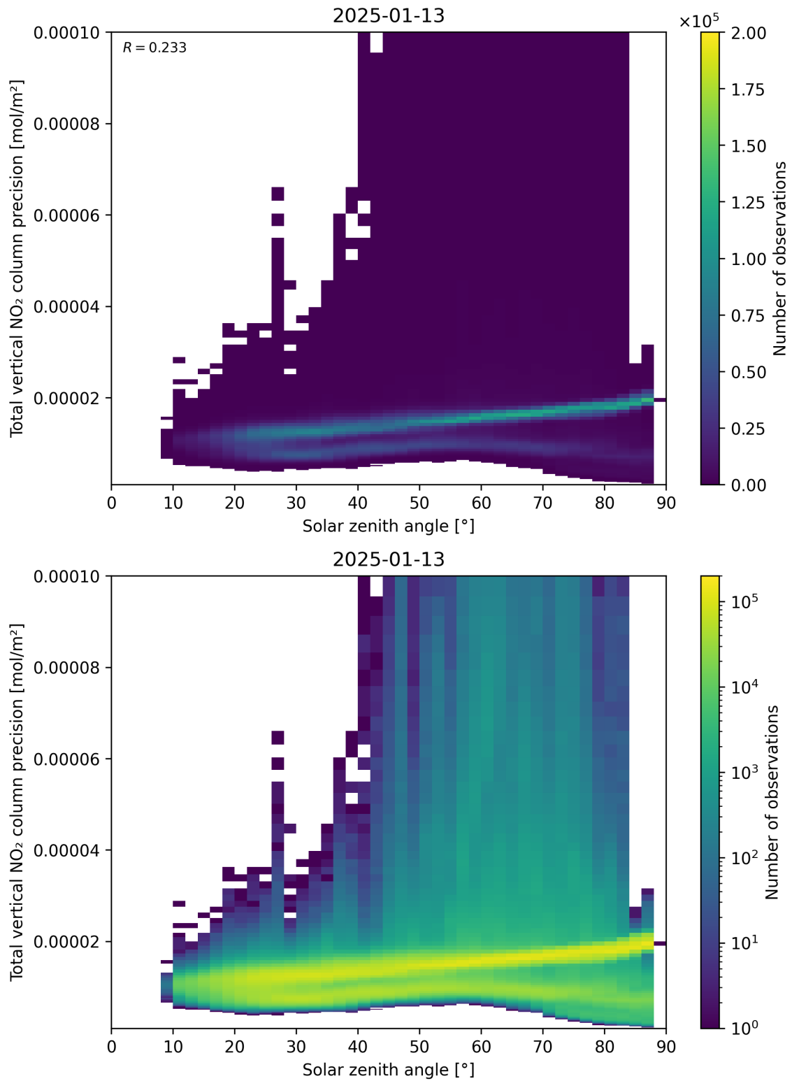
Figure 154: Scatter density plot of “Solar zenith angle” against “Total vertical NO 2 column precision” for 2025-01-12 to 2025-01-14.
