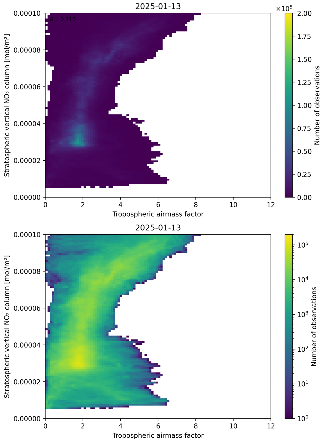
Figure 74: Scatter density plot of “Tropospheric air mass factor” against “Stratospheric vertical NO 2 column” for 2025-01-12 to 2025-01-14.
