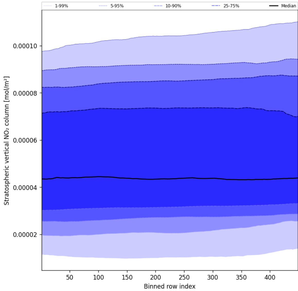
Figure 53: Along track statistics of “Stratospheric vertical NO 2 column” for 2025-01-12 to 2025-01-14
