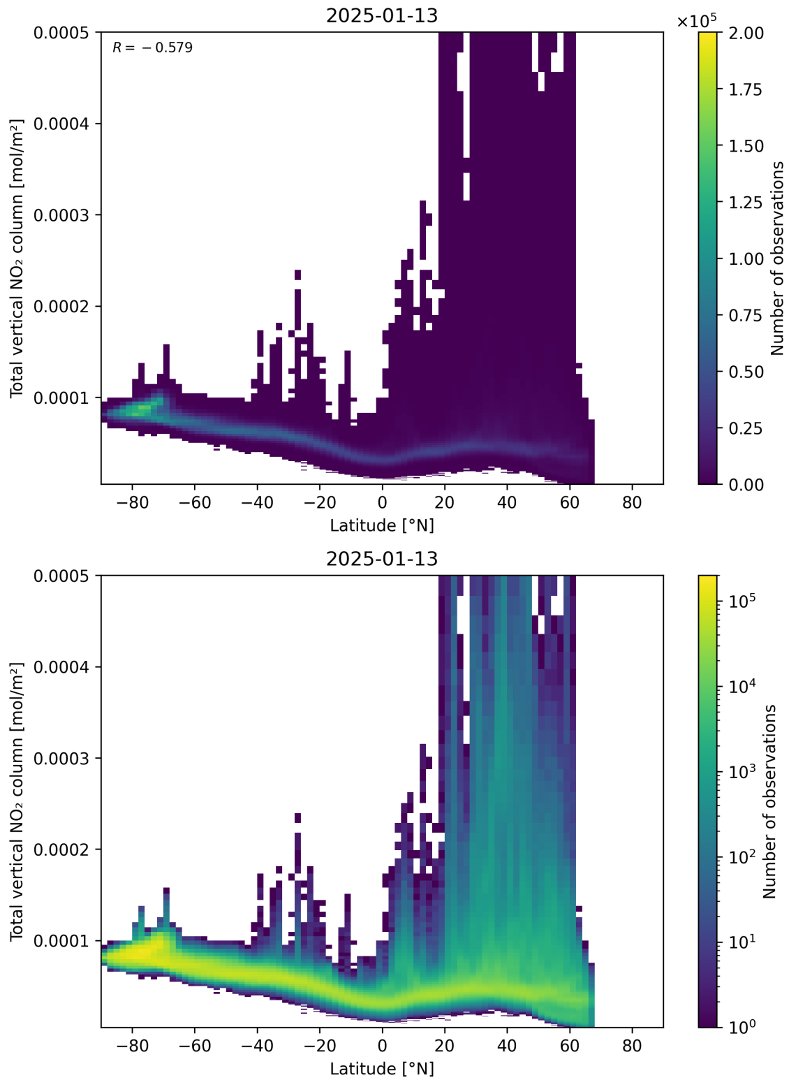
Figure 90: Scatter density plot of “Latitude” against “Total vertical NO 2 column” for 2025-01-12 to 2025-01-14.
