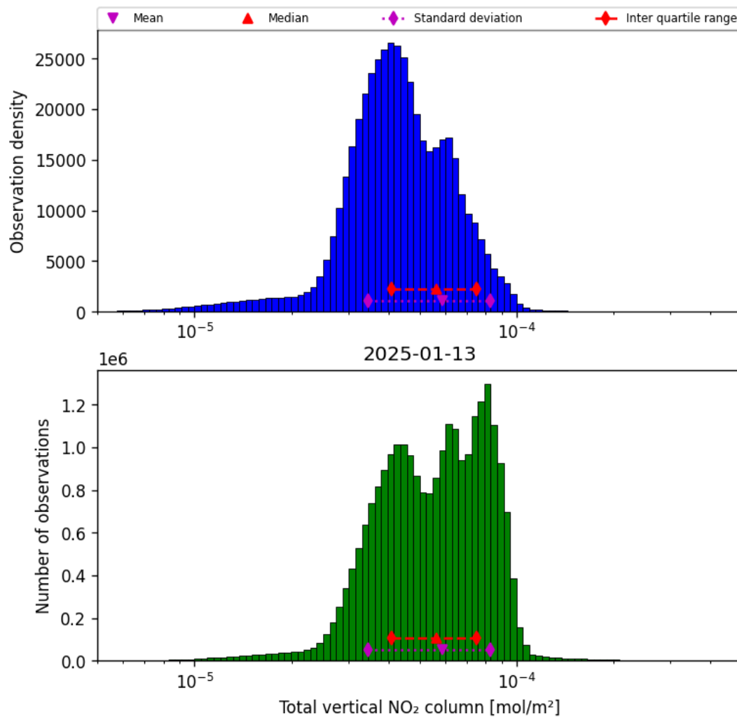
Figure 38: Histogram of “Total vertical NO 2 column” for 2025-01-12 to 2025-01-14
