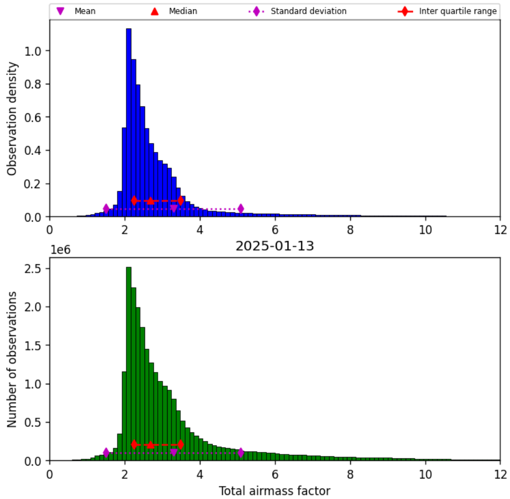
Figure 32: Histogram of “Total airmass factor” for 2025-01-12 to 2025-01-14
