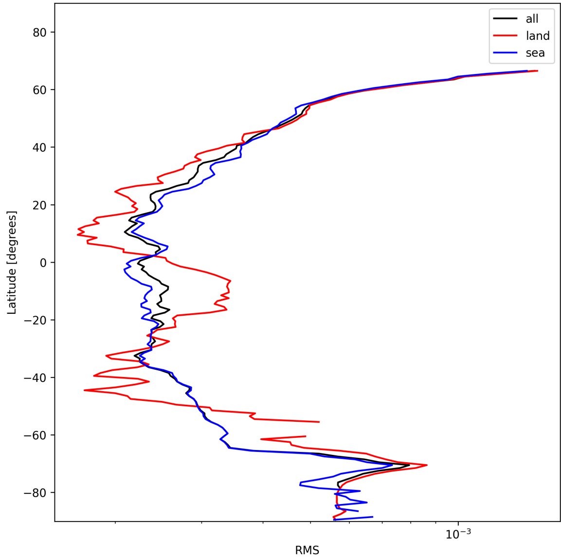
Figure 26: Zonal average of “RMS” for 2025-01-12 to 2025-01-14.
