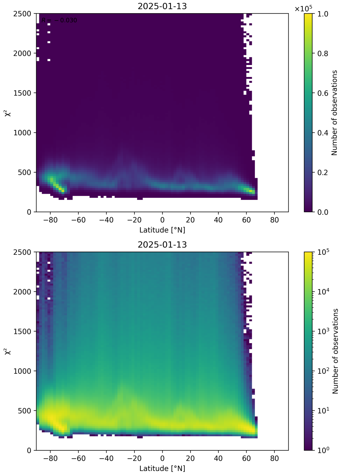
Figure 86: Scatter density plot of “Latitude” against “ \chi^2 ” for 2025-01-12 to 2025-01-14.
