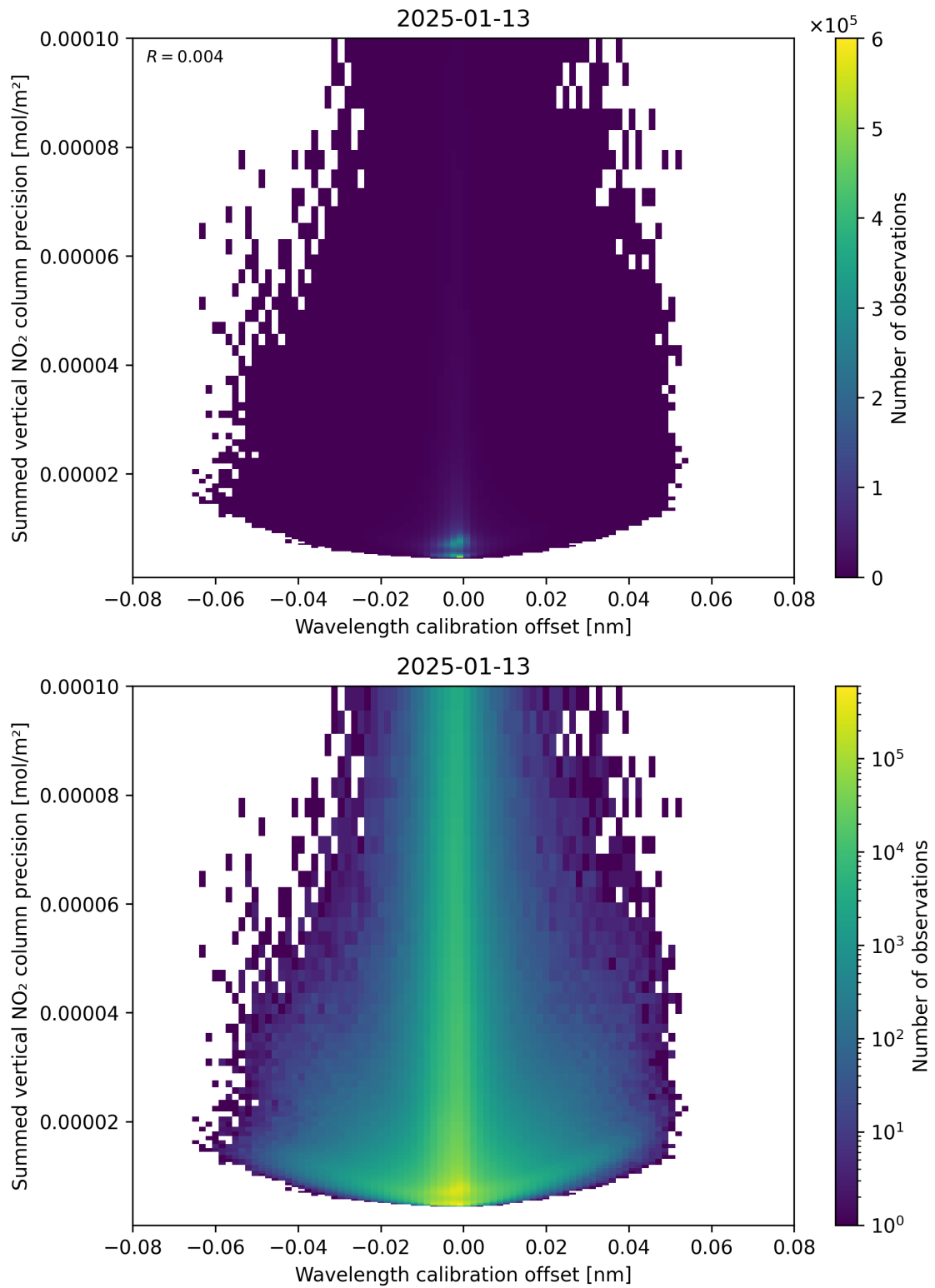
Figure 178: Scatter density plot of “Wavelength calibration offset” against “Summed vertical NO 2 column precision” for 2025-01-12 to 2025-01-14.
