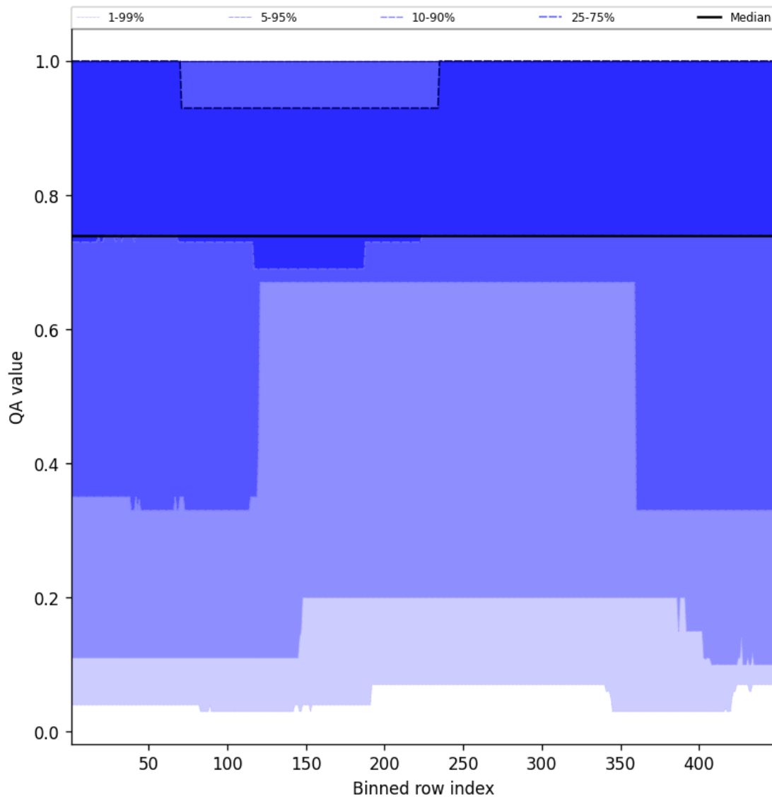
Figure 45: Along track statistics of “QA value” for 2025-01-12 to 2025-01-14
