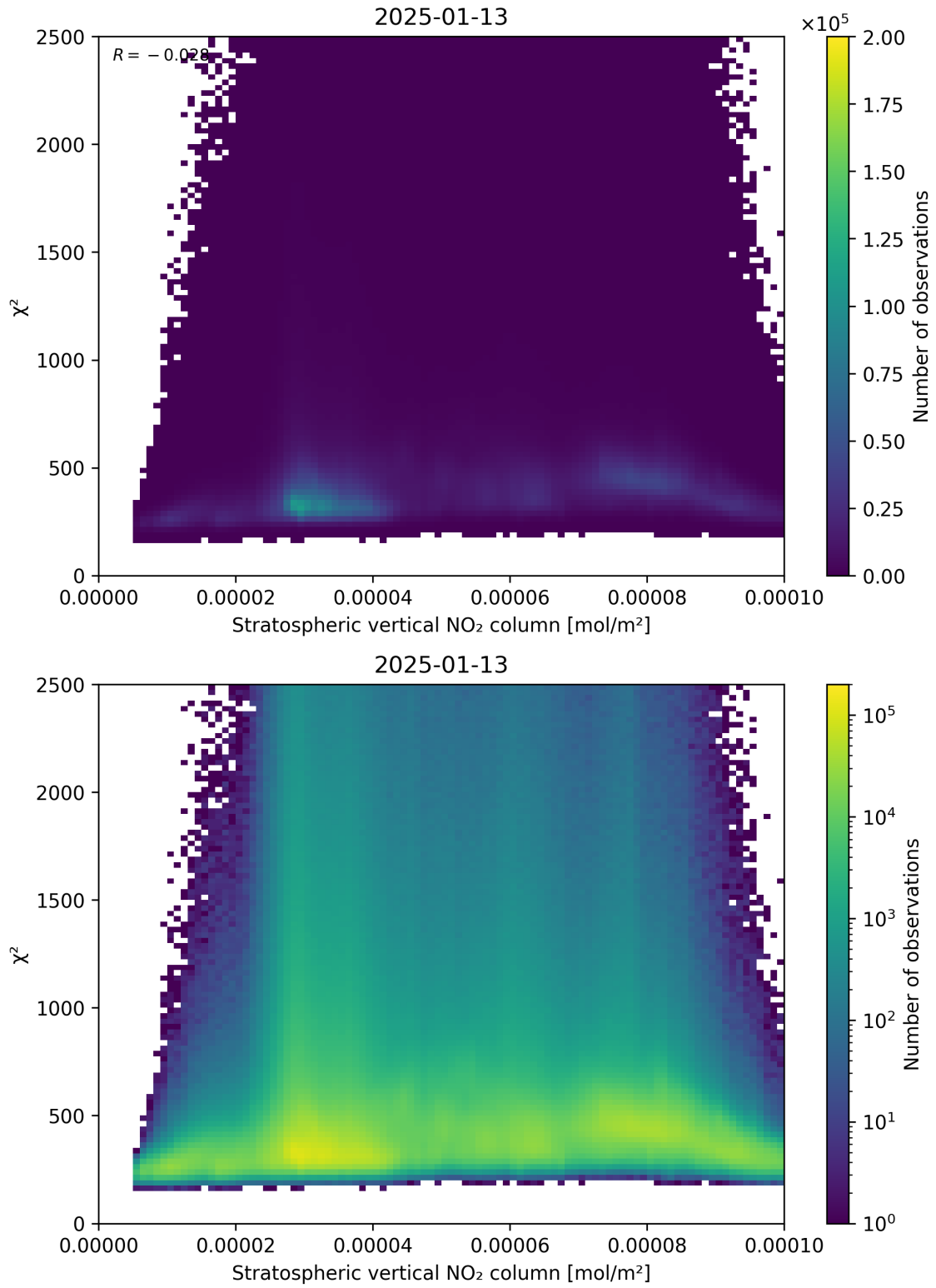
Figure 97: Scatter density plot of “Stratospheric vertical NO 2 column” against “ \chi^2 ” for 2025-01-12 to 2025-01-14.
