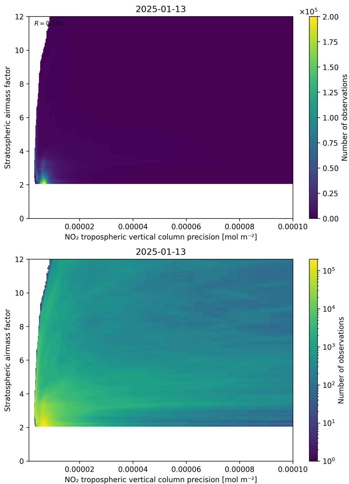
Figure 131: Scatter density plot of “NO 2 tropospheric vertical column precision” against “Stratospheric airmass factor” for 2025-01-12 to 2025-01-14.
