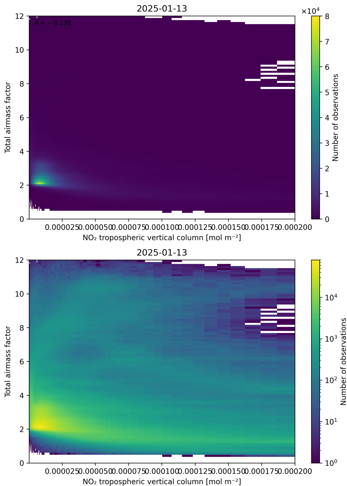
Figure 122: Scatter density plot of “NO 2 tropospheric vertical column” against “Total air mass factor” for 2025-01-12 to 2025-01-14.
