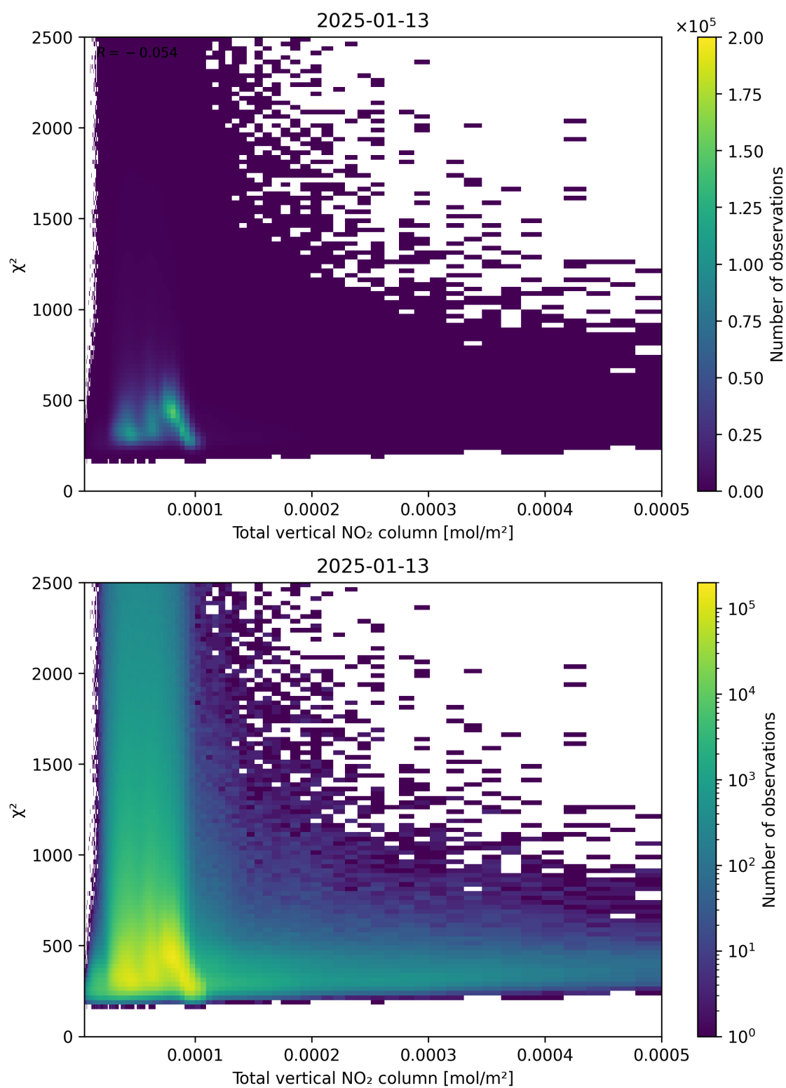
Figure 111: Scatter density plot of “Total vertical NO 2 column” against “ \chi^2 ” for 2025-01-12 to 2025-01-14.
