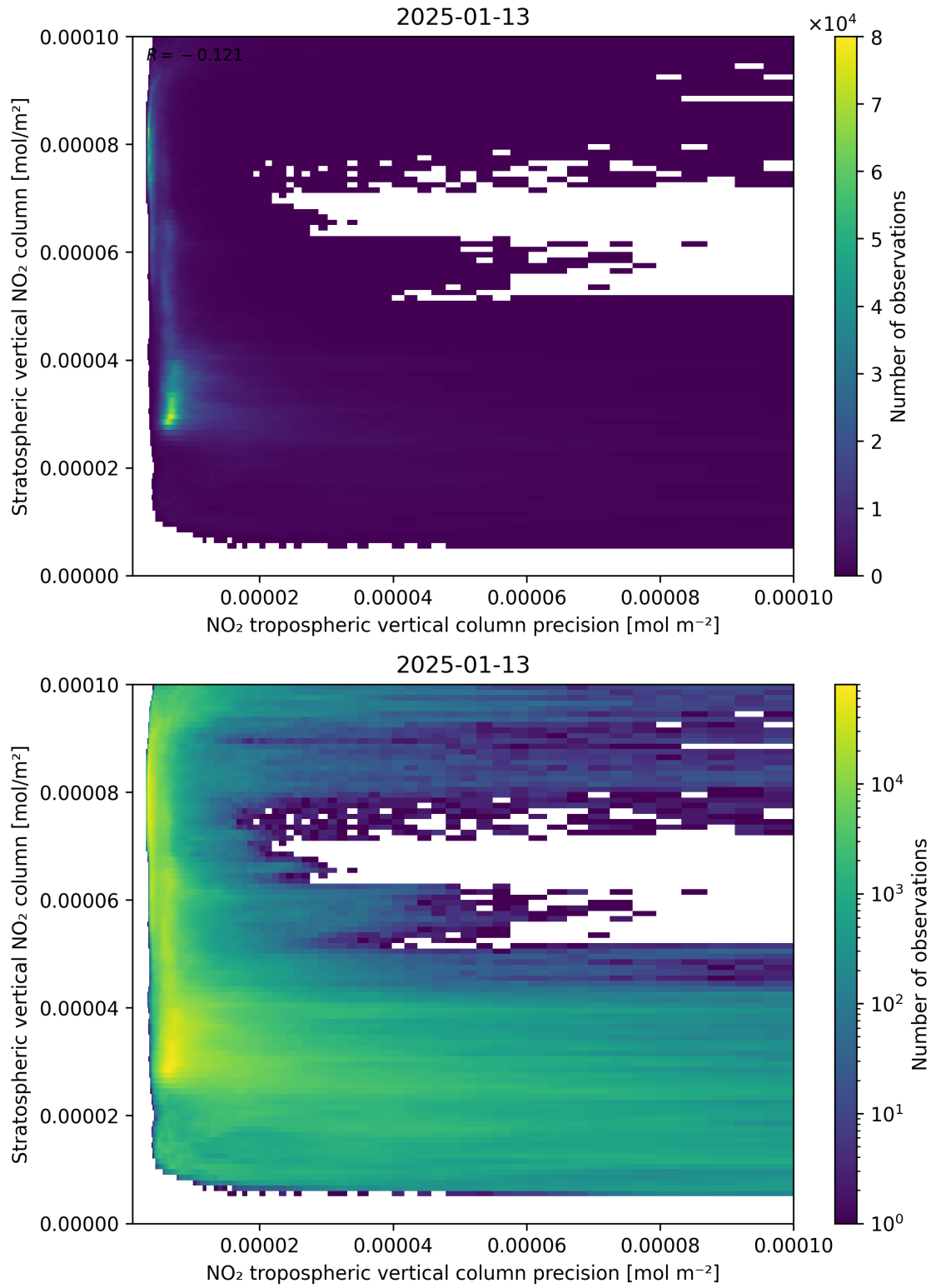
Figure 135: Scatter density plot of “NO 2 tropospheric vertical column precision” against “Stratospheric vertical NO 2 column” for 2025-01-12 to 2025-01-14.
