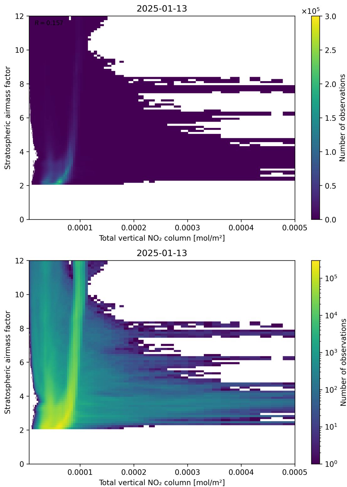
Figure 110: Scatter density plot of “Total vertical NO 2 column” against “Stratospheric airmass factor” for 2025-01-12 to 2025-01-14.
