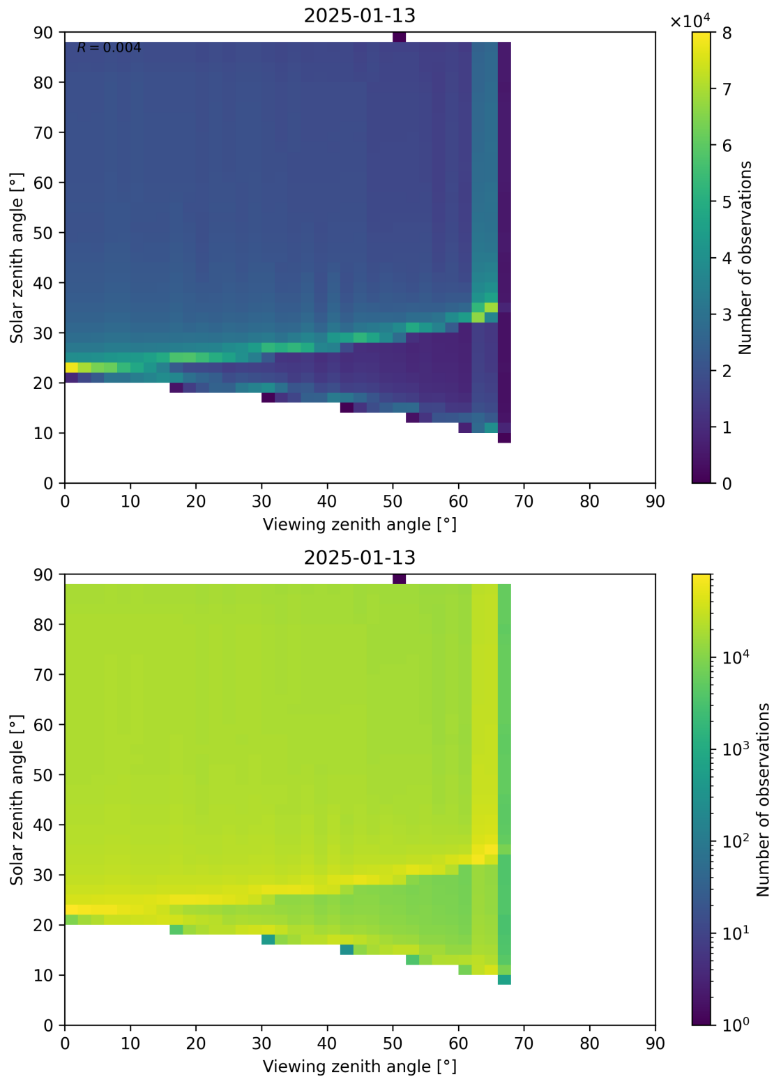
Figure 172: Scatter density plot of “Viewing zenith angle” against “Solar zenith angle” for 2025-01-12 to 2025-01-14.
