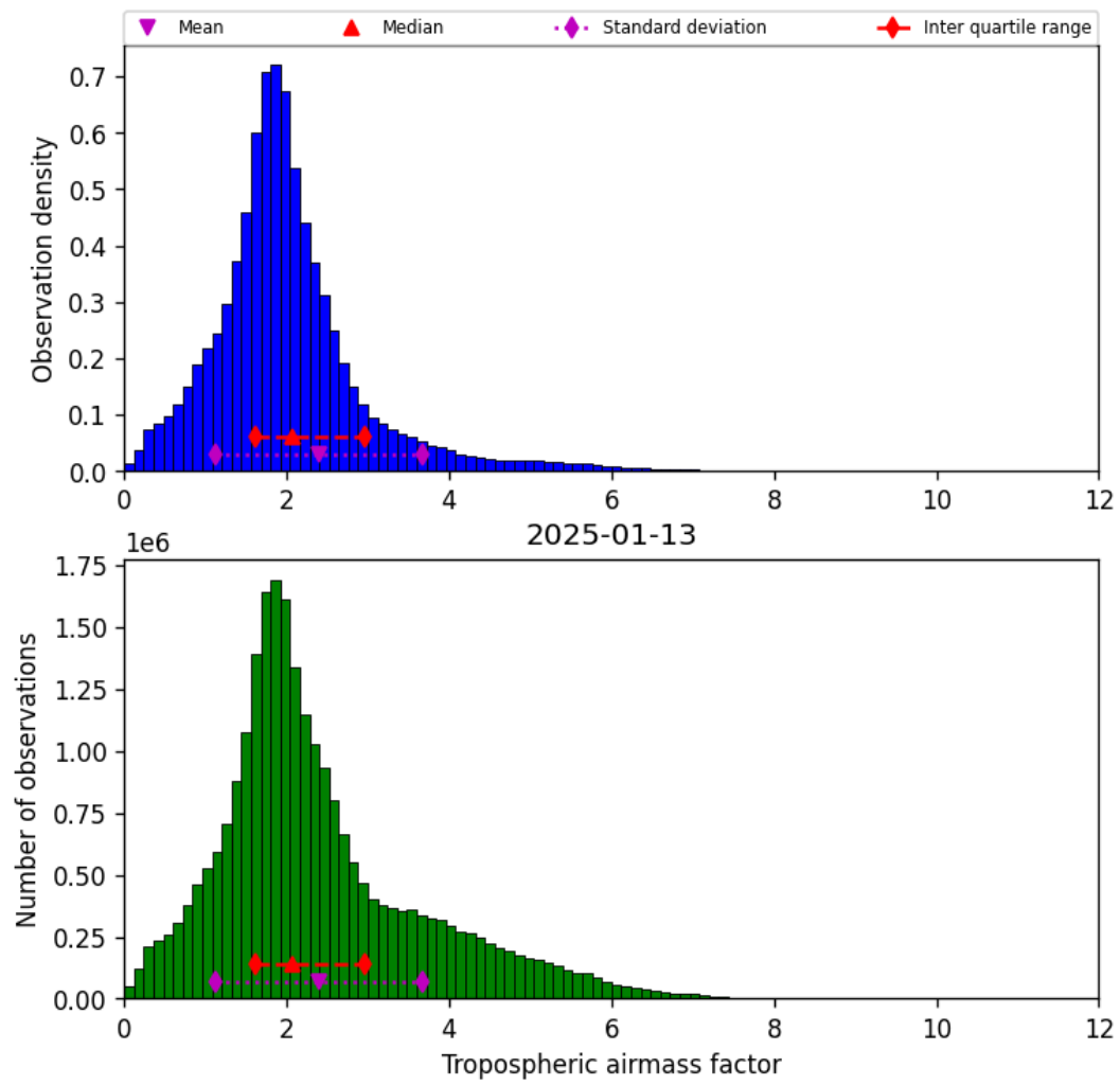
Figure 31: Histogram of “Tropospheric airmass factor” for 2025-01-12 to 2025-01-14
