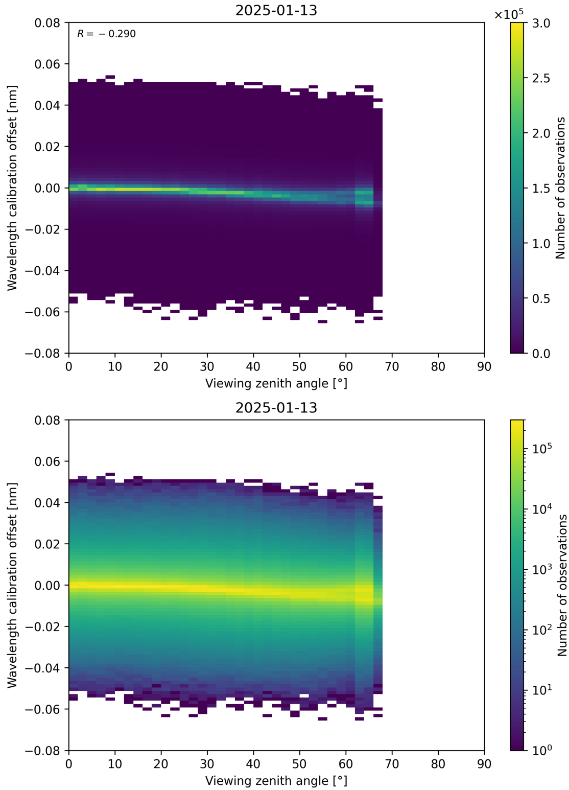
Figure 173: Scatter density plot of “Viewing zenith angle” against “Wavelength calibration offset” for 2025-01-12 to 2025-01-14.
