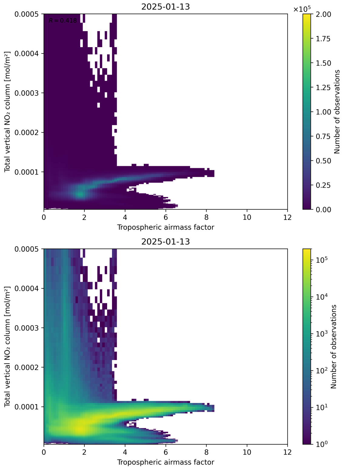
Figure 77: Scatter density plot of “Tropospheric airmass factor” against “Total vertical NO 2 column” for 2025-01-12 to 2025-01-14.
