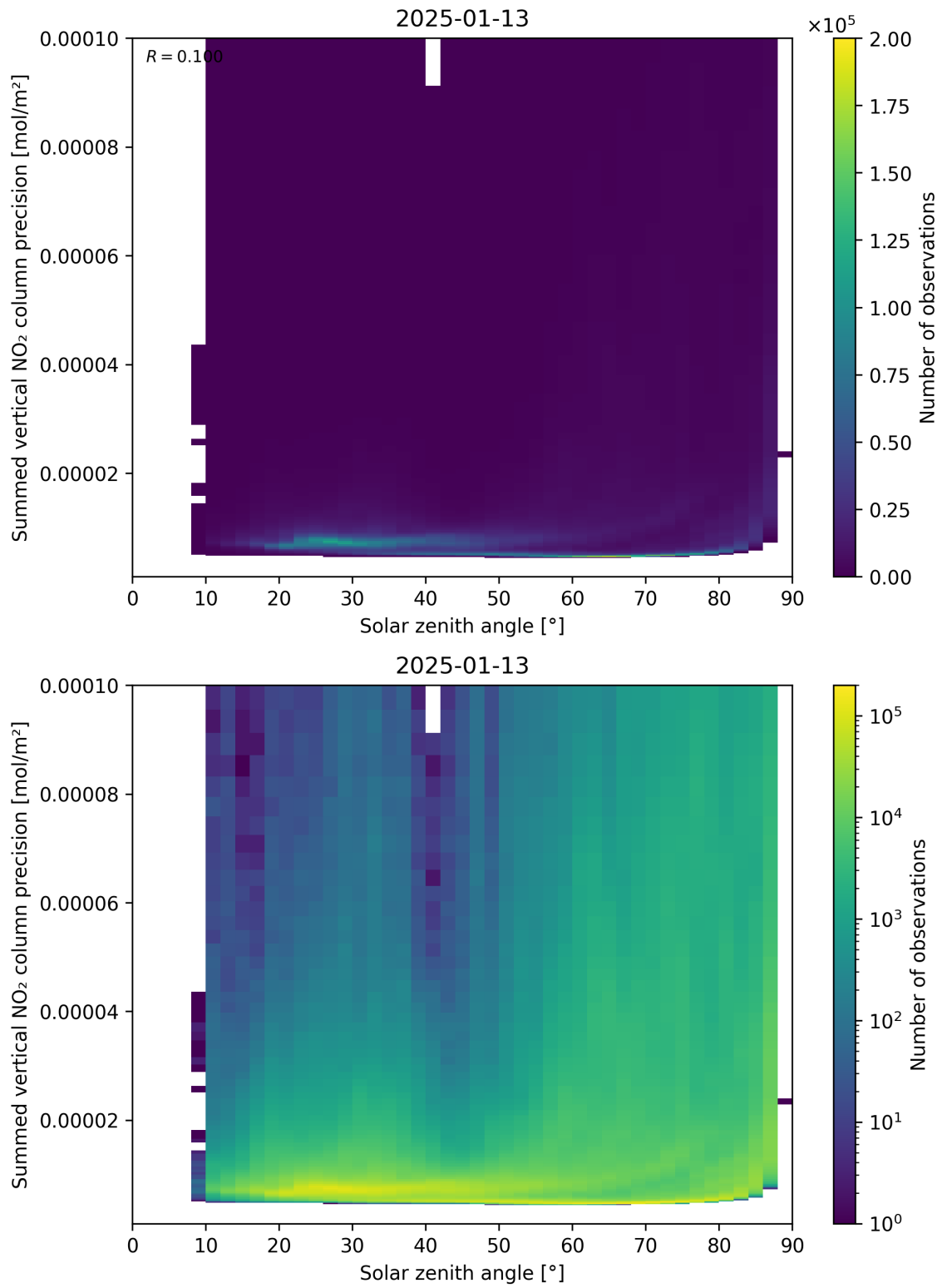
Figure 152: Scatter density plot of “Solar zenith angle” against “Summed vertical NO 2 column precision” for 2025-01-12 to 2025-01-14.
