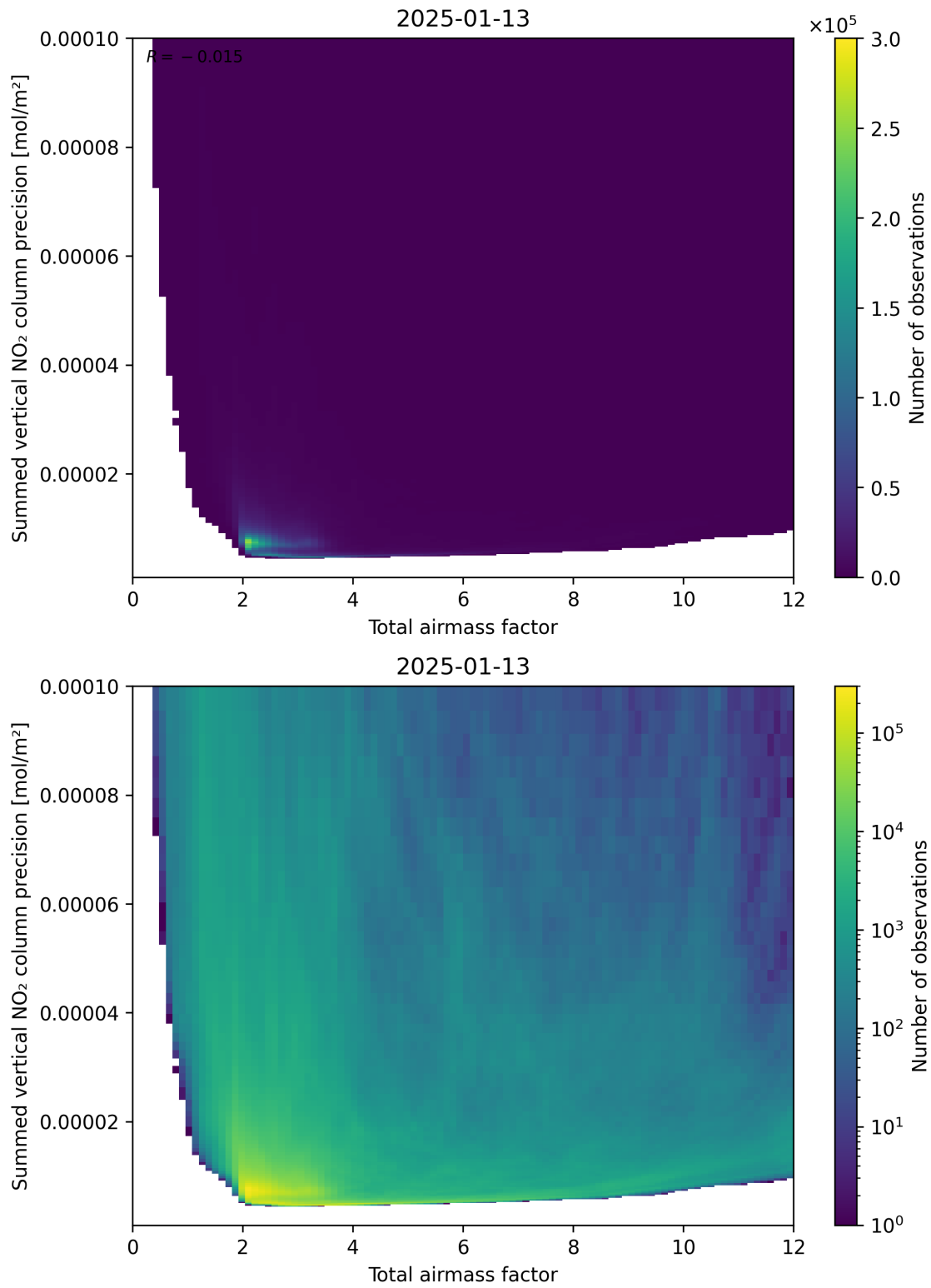
Figure 66: Scatter density plot of “Total airmass factor” against “Summed vertical NO 2 column precision” for 2025-01-12 to 2025-01-14.
