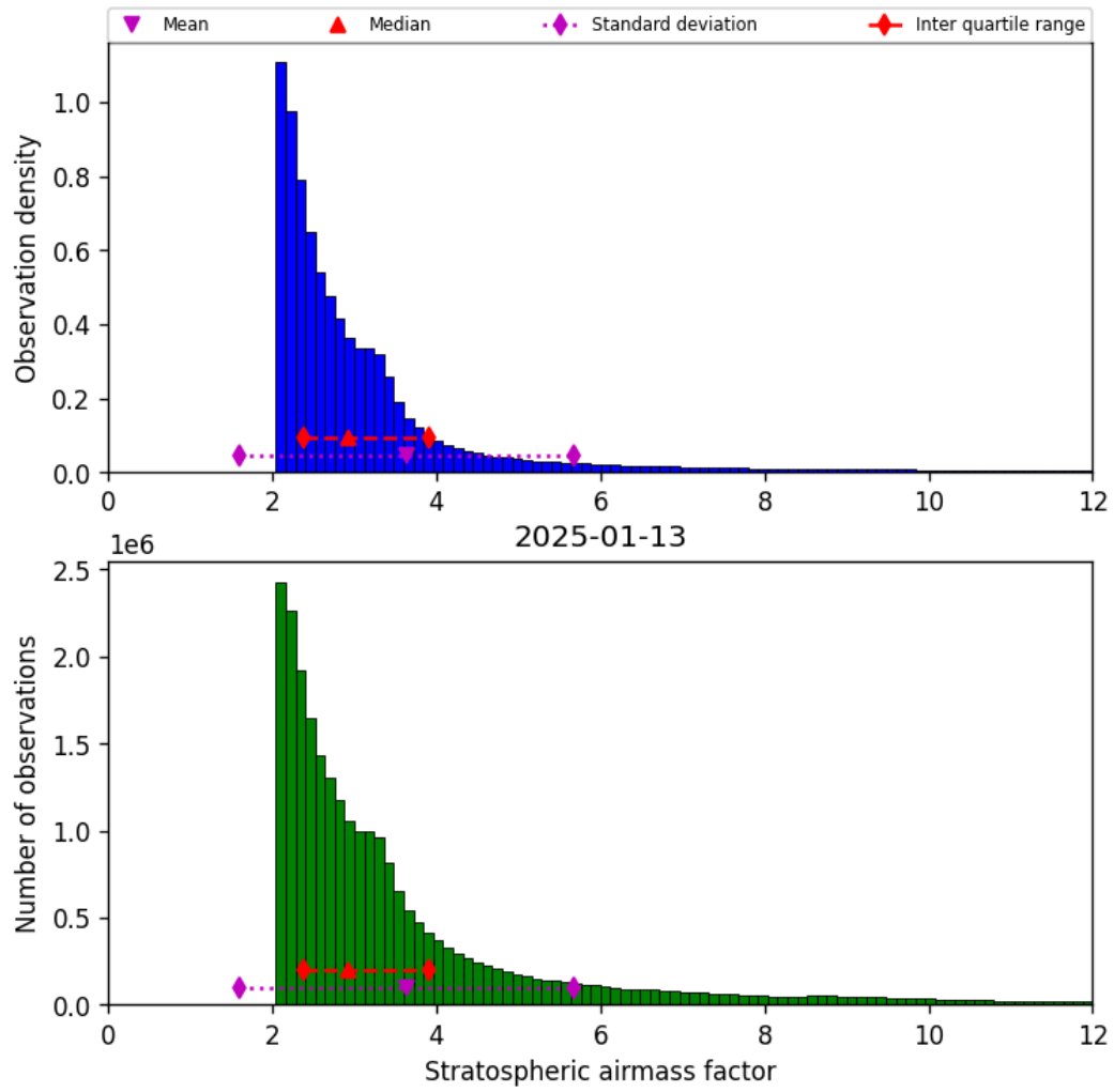
Figure 44: Histogram of “Stratospheric airmass factor” for 2025-01-12 to 2025-01-14
