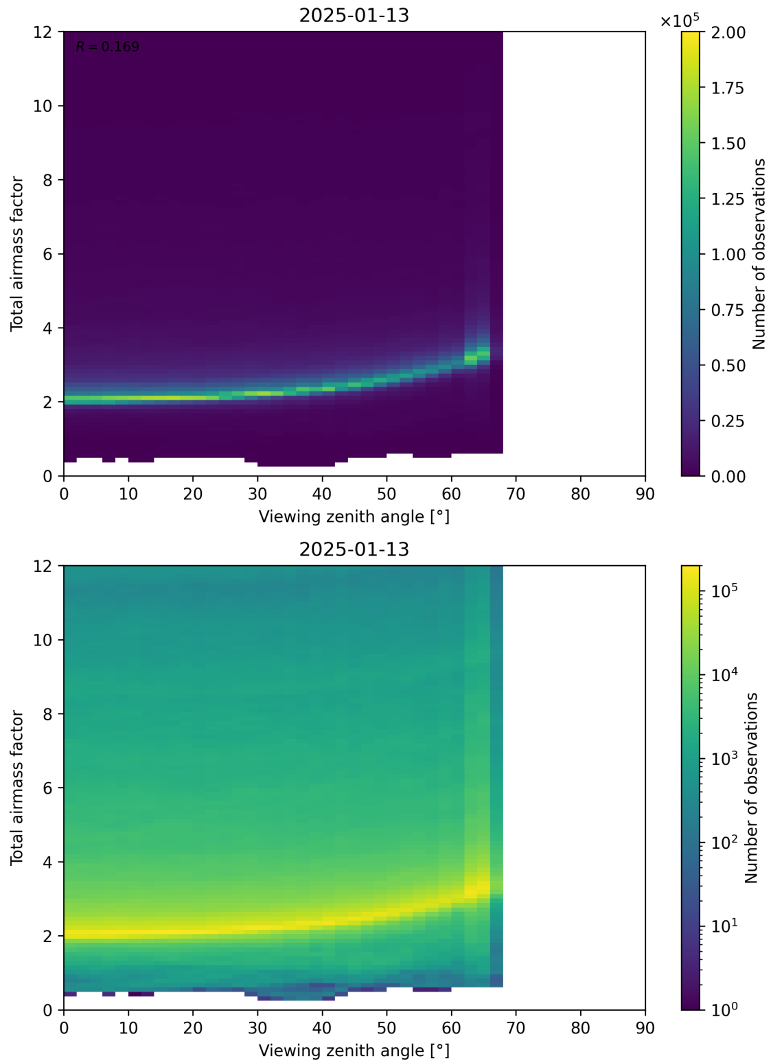
Figure 160: Scatter density plot of “Viewing zenith angle” against “Total airmass factor” for 2025-01-12 to 2025-01-14.
