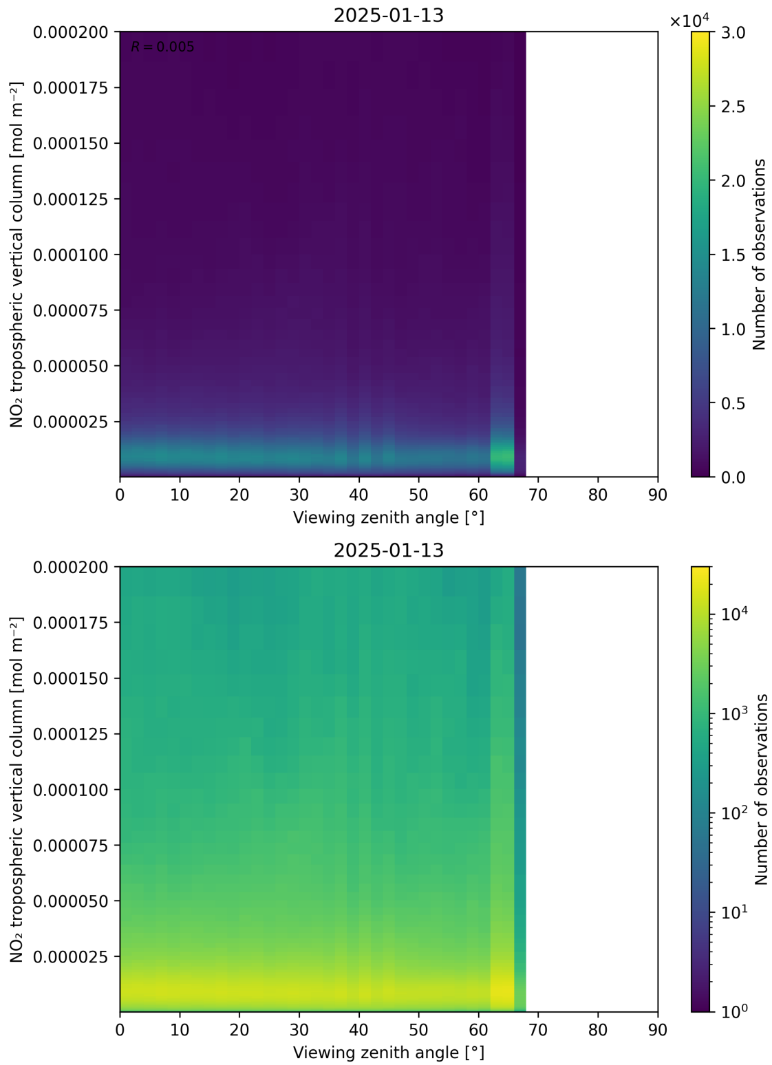
Figure 169: Scatter density plot of “Viewing zenith angle” against “NO 2 tropospheric vertical column” for 2025-01-12 to 2025-01-14.
