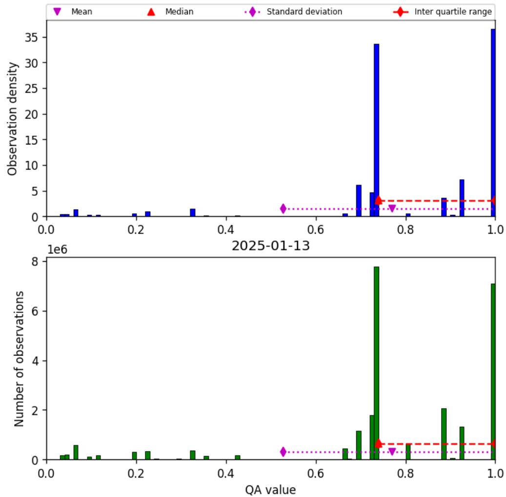
Figure 28: Histogram of “QA value” for 2025-01-12 to 2025-01-14
