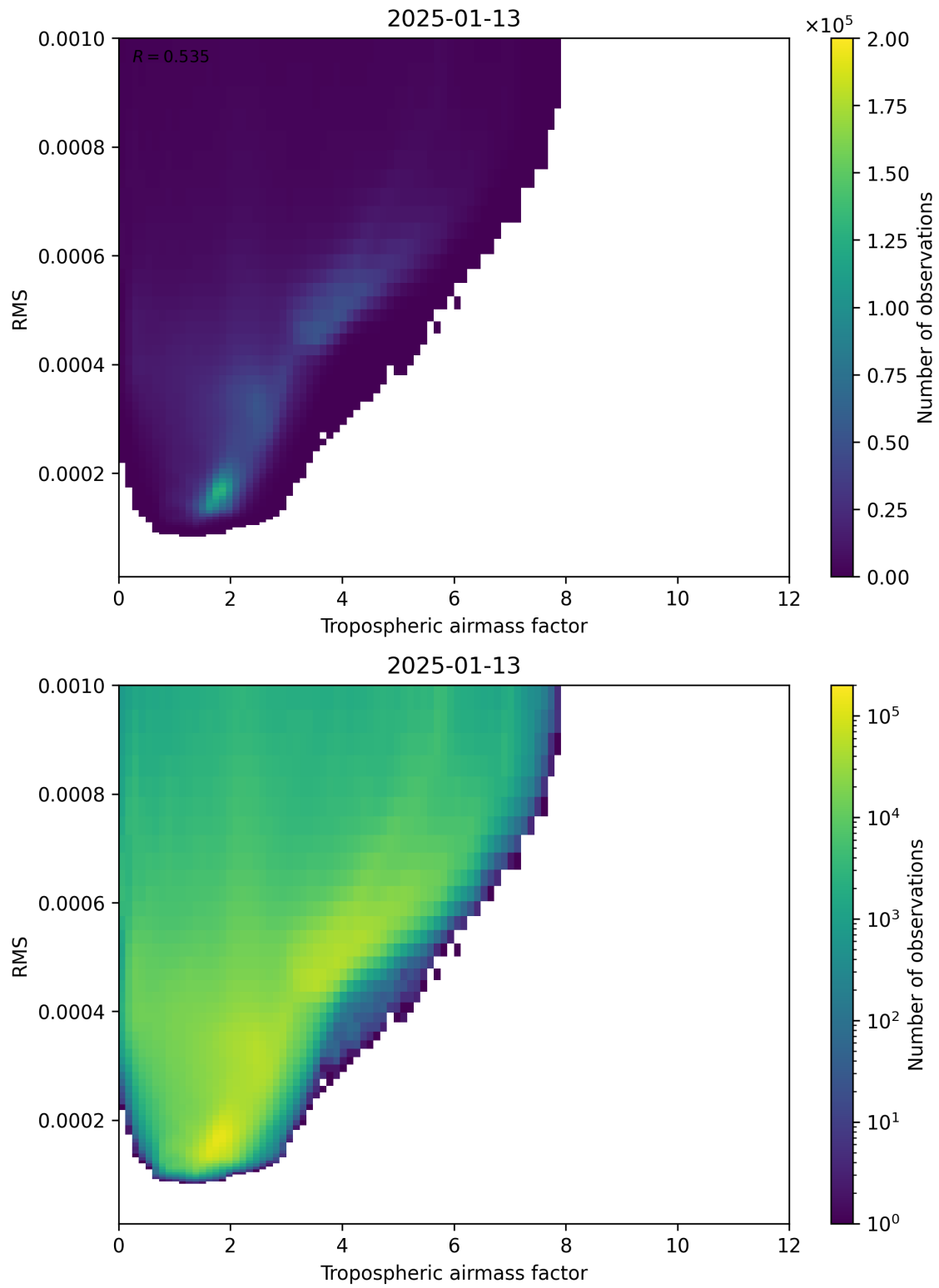
Figure 79: Scatter density plot of “Tropospheric airmass factor” against “RMS” for 2025-01-12 to 2025-01-14.
