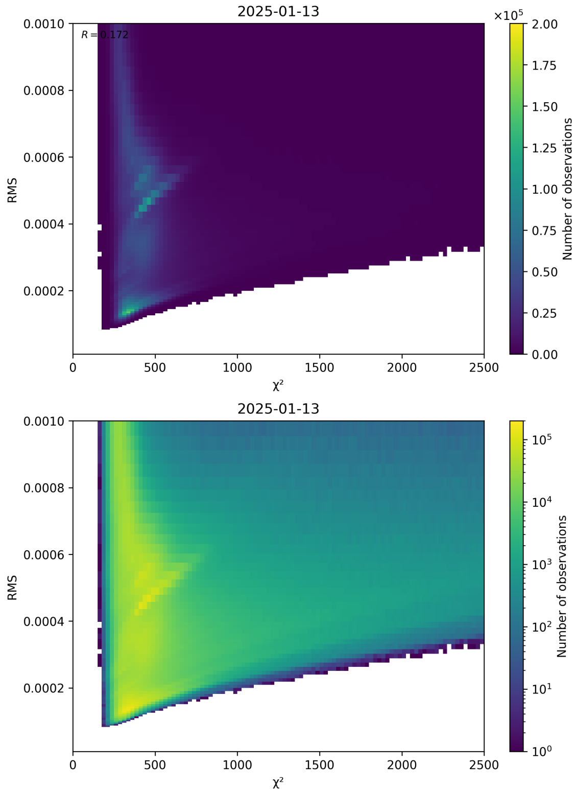
Figure 82: Scatter density plot of “ \chi^2 ” against “RMS” for 2025-01-12 to 2025-01-14.
