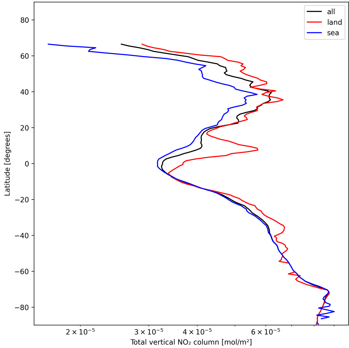
Figure 21: Zonal average of “Total vertical NO 2 column” for 2025-01-12 to 2025-01-14.
