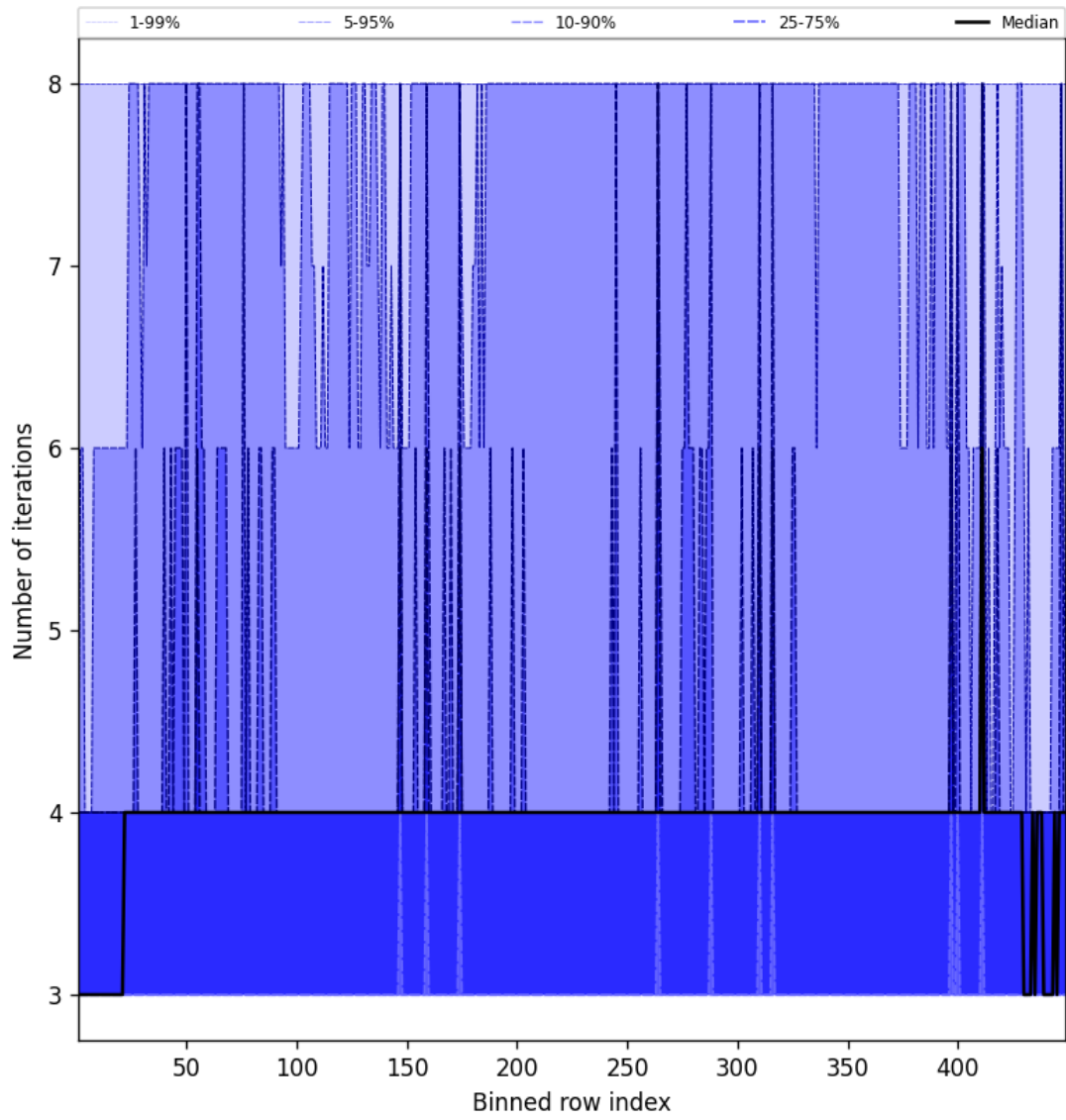
Figure 51: Along track statistics of “Number of iterations” for 2025-01-12 to 2025-01-14
