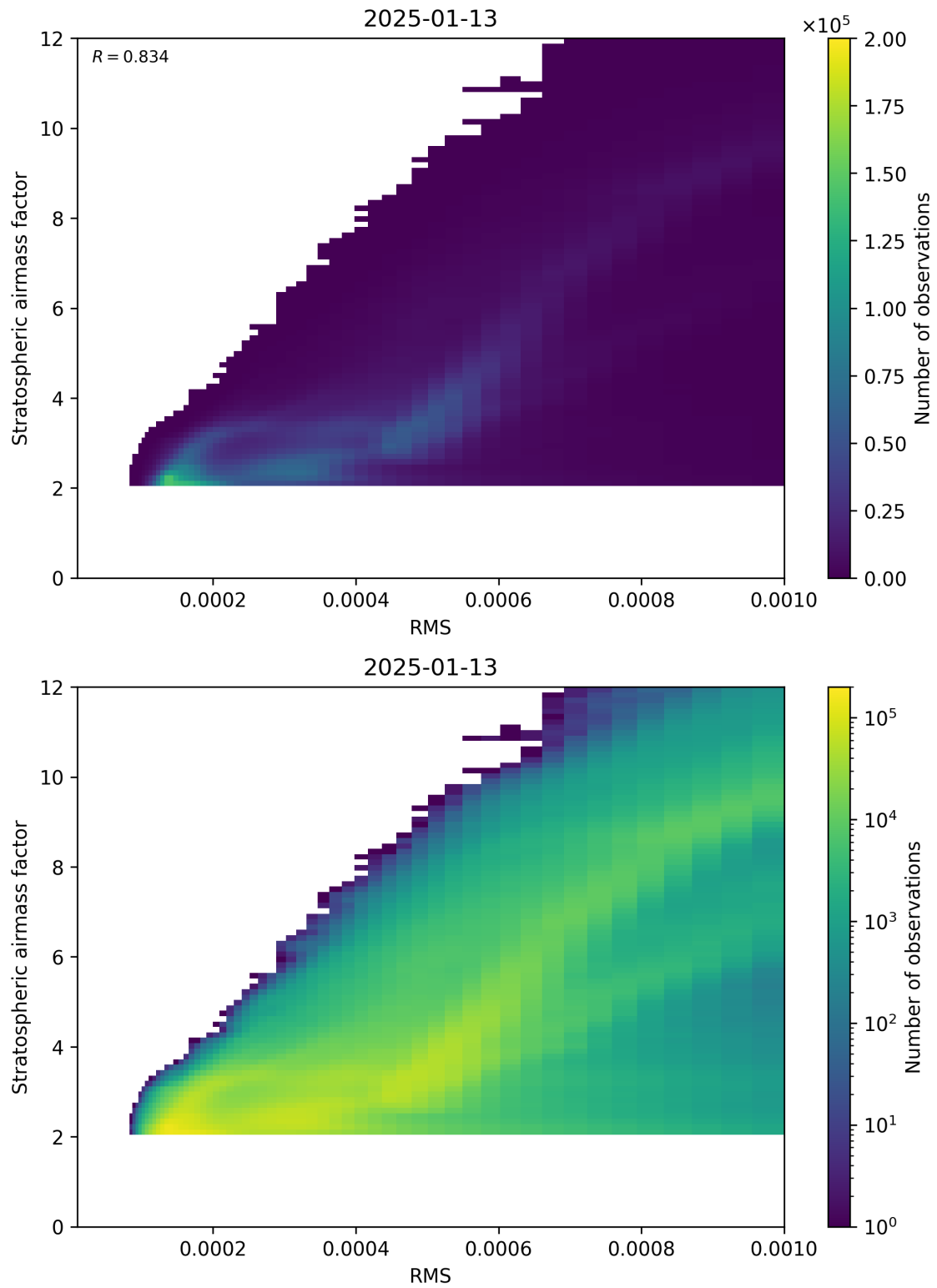
Figure 144: Scatter density plot of “RMS” against “Stratospheric airmass factor” for 2025-01-12 to 2025-01-14.
