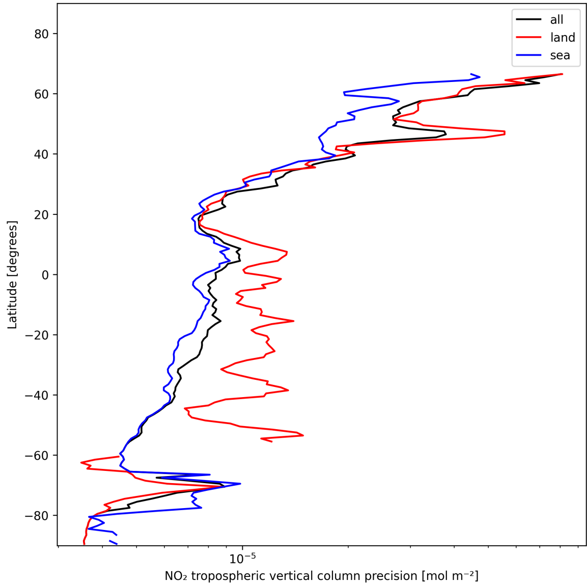
Figure 13: Zonal average of “NO 2 tropospheric vertical column precision” for 2025-01-12 to 2025-01-14.
