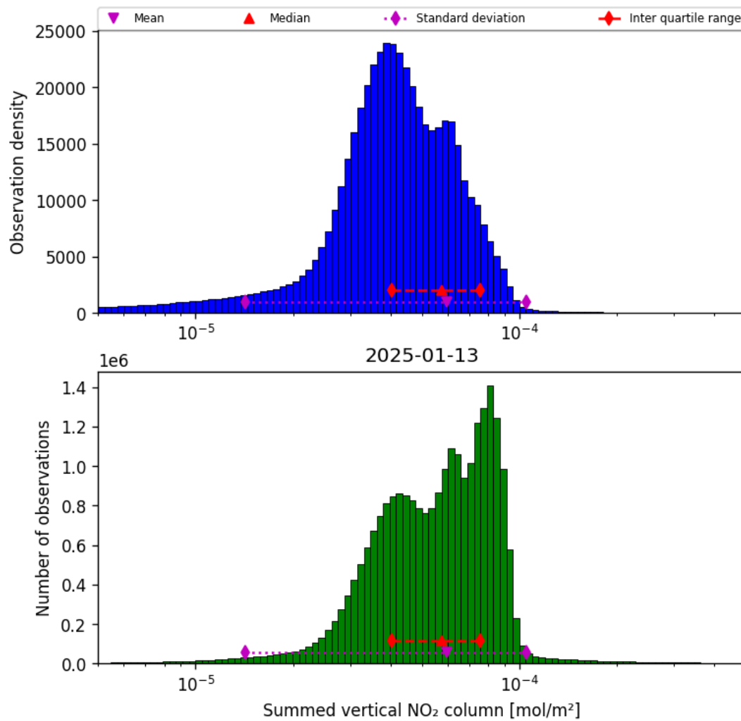
Figure 40: Histogram of “Summed vertical NO 2 column” for 2025-01-12 to 2025-01-14
