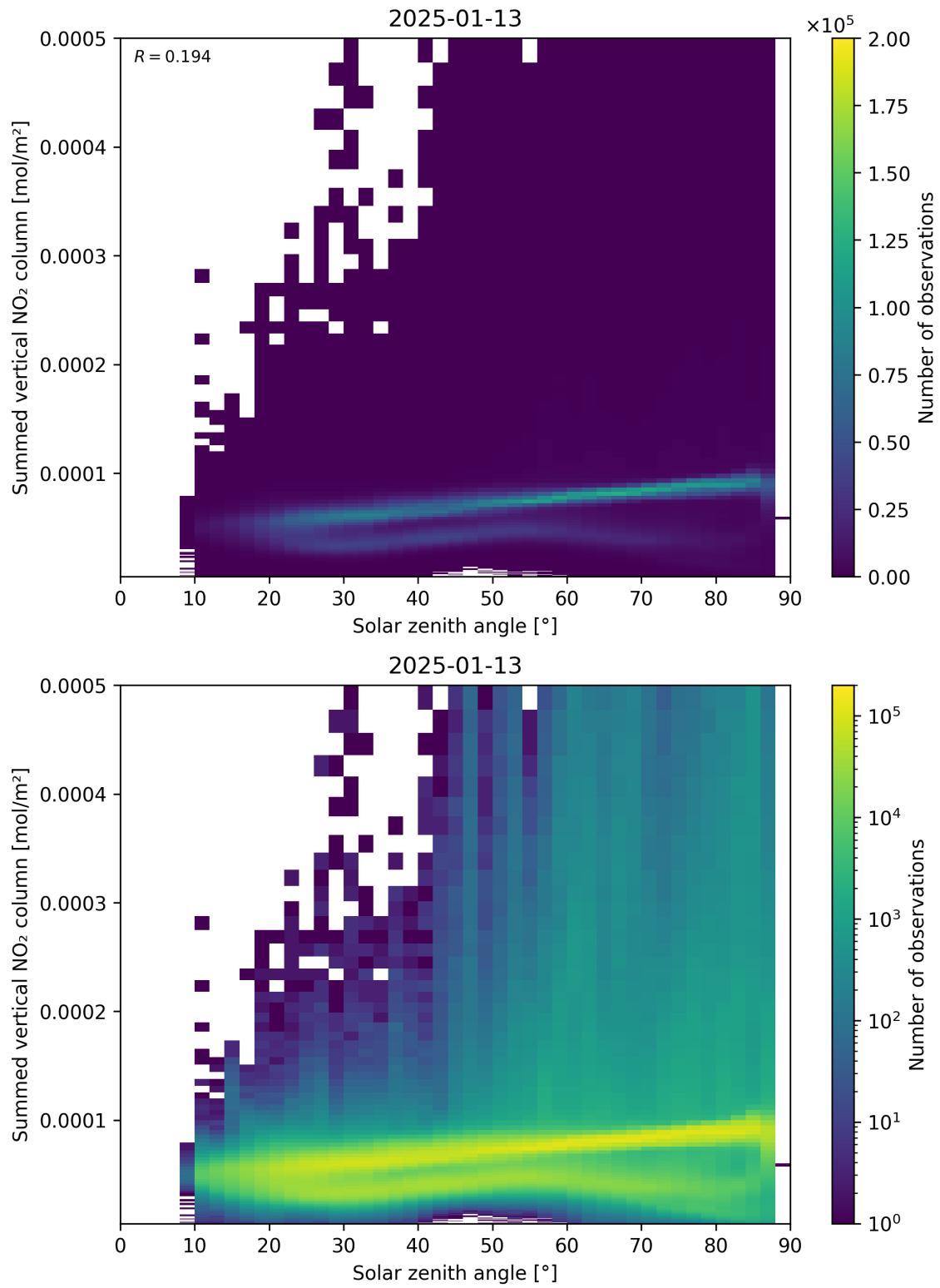
Figure 151: Scatter density plot of “Solar zenith angle” against “Summed vertical NO 2 column” for 2025-01-12 to 2025-01-14.
