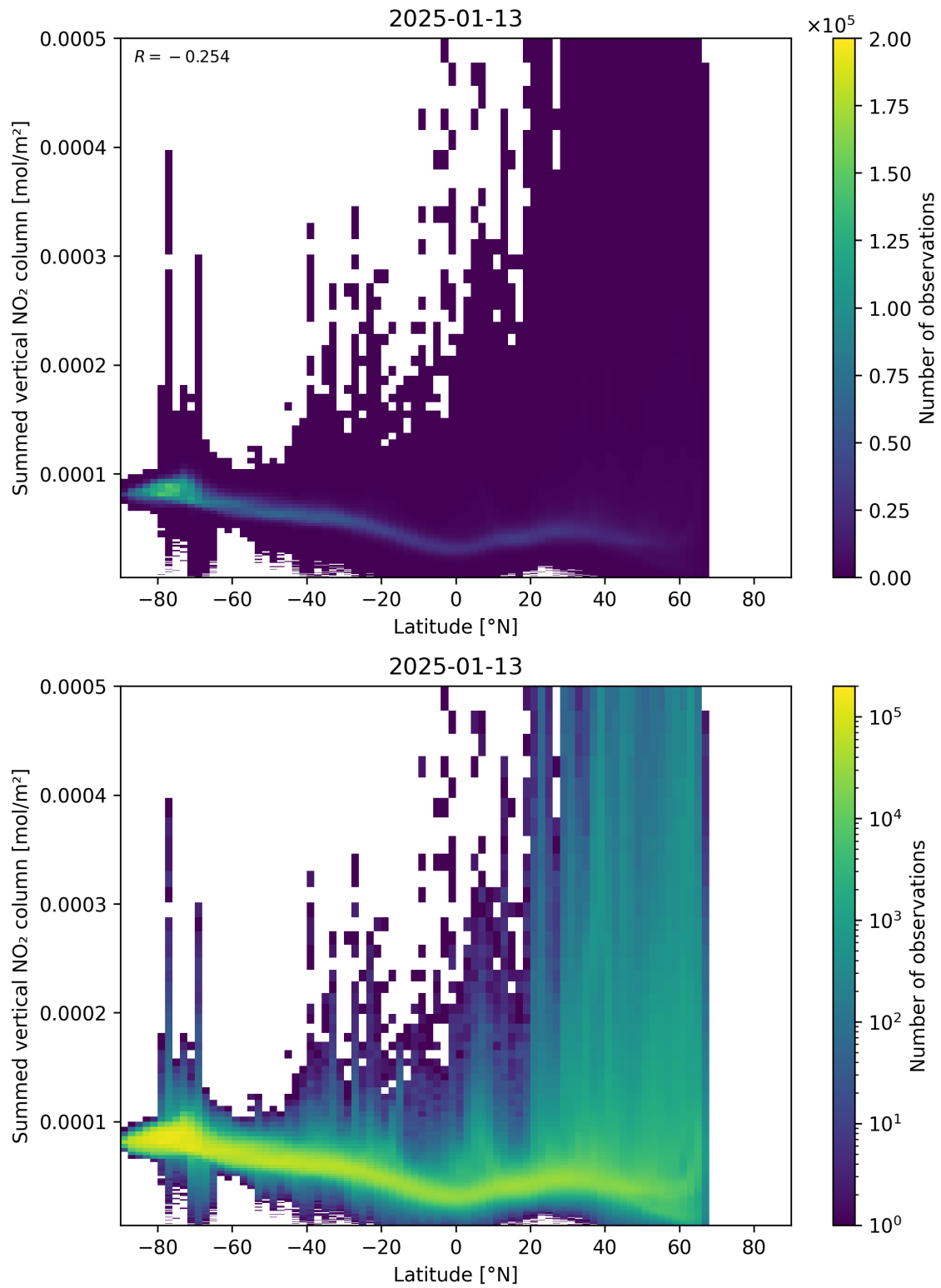
Figure 88: Scatter density plot of “Latitude” against “Summed vertical NO 2 column” for 2025-01-12 to 2025-01-14.
