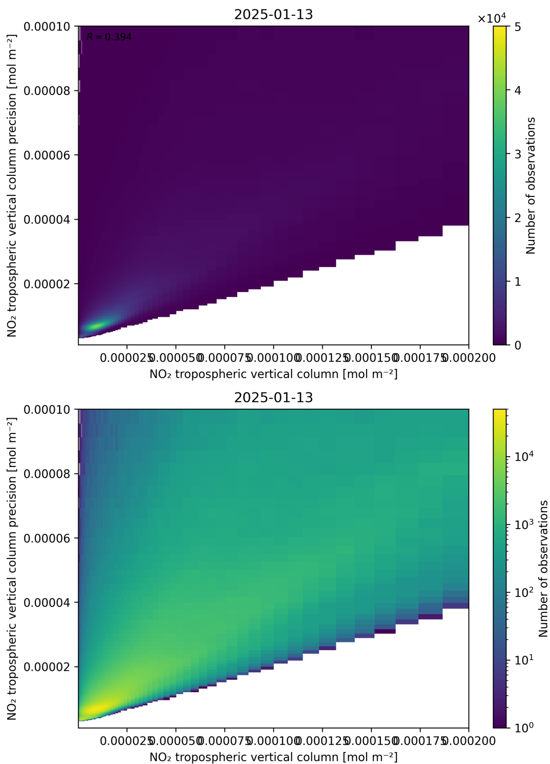
Figure 130: Scatter density plot of “NO 2 tropospheric vertical column” against “NO 2 tropospheric vertical column precision” for 2025-01-12 to 2025-01-14.
