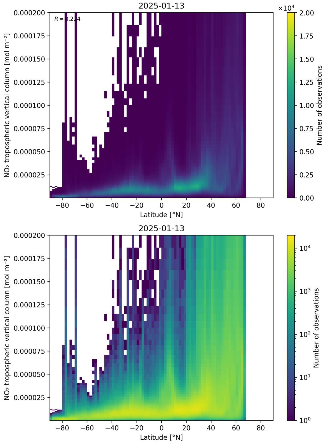
Figure 92: Scatter density plot of “Latitude” against “NO 2 tropospheric vertical column” for 2025-01-12 to 2025-01-14.
