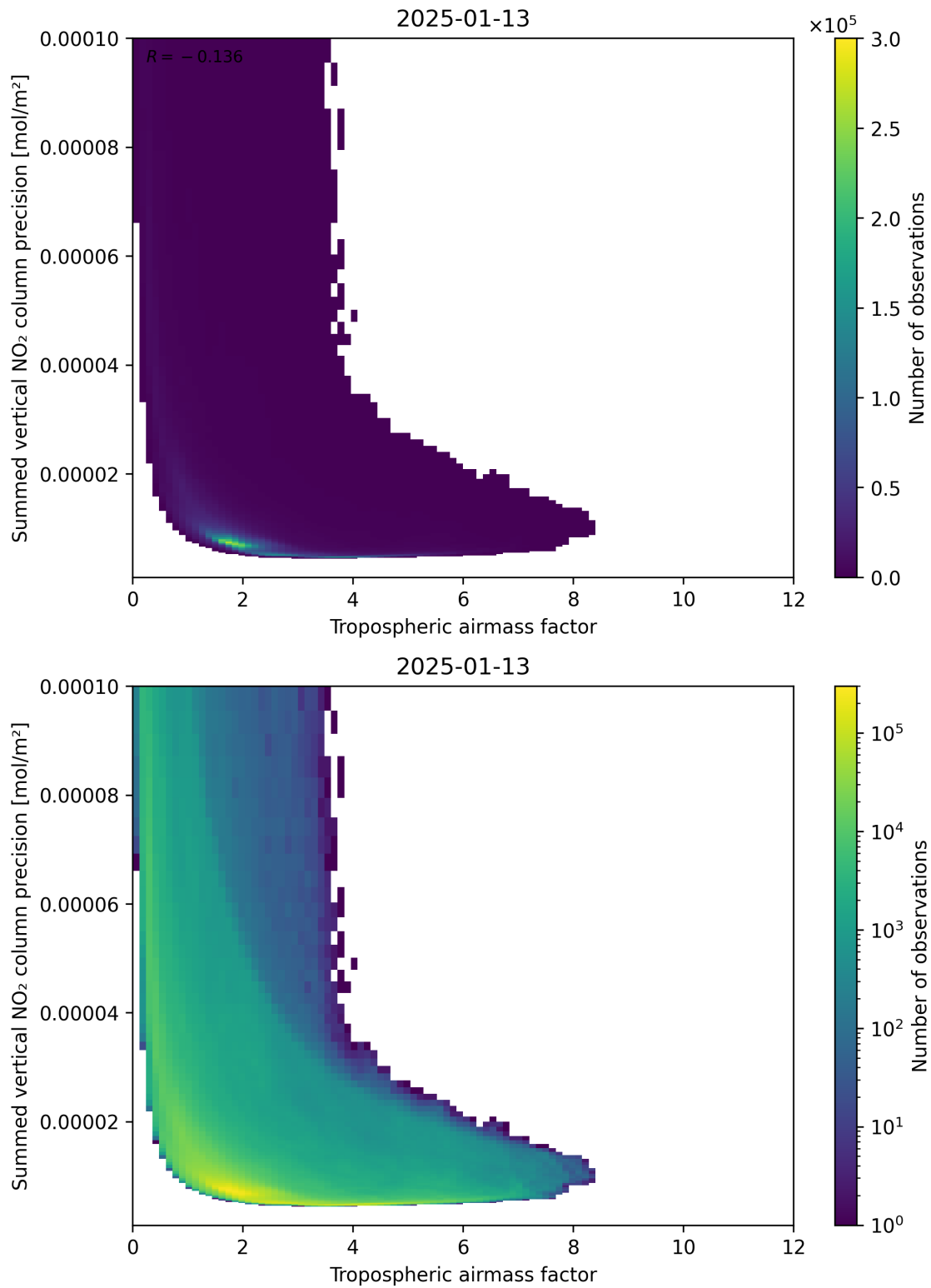
Figure 76: Scatter density plot of “Tropospheric air mass factor” against “Summed vertical NO 2 column precision” for 2025-01-12 to 2025-01-14.
