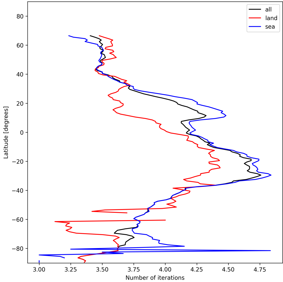
Figure 17: Zonal average of “Number of iterations” for 2025-01-12 to 2025-01-14.
