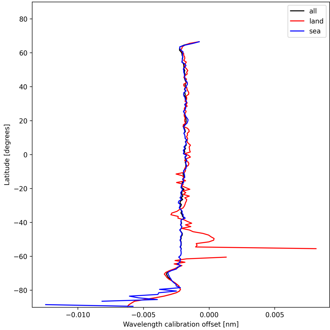
Figure 18: Zonal average of “Wavelength calibration offset” for 2025-01-12 to 2025-01-14.
