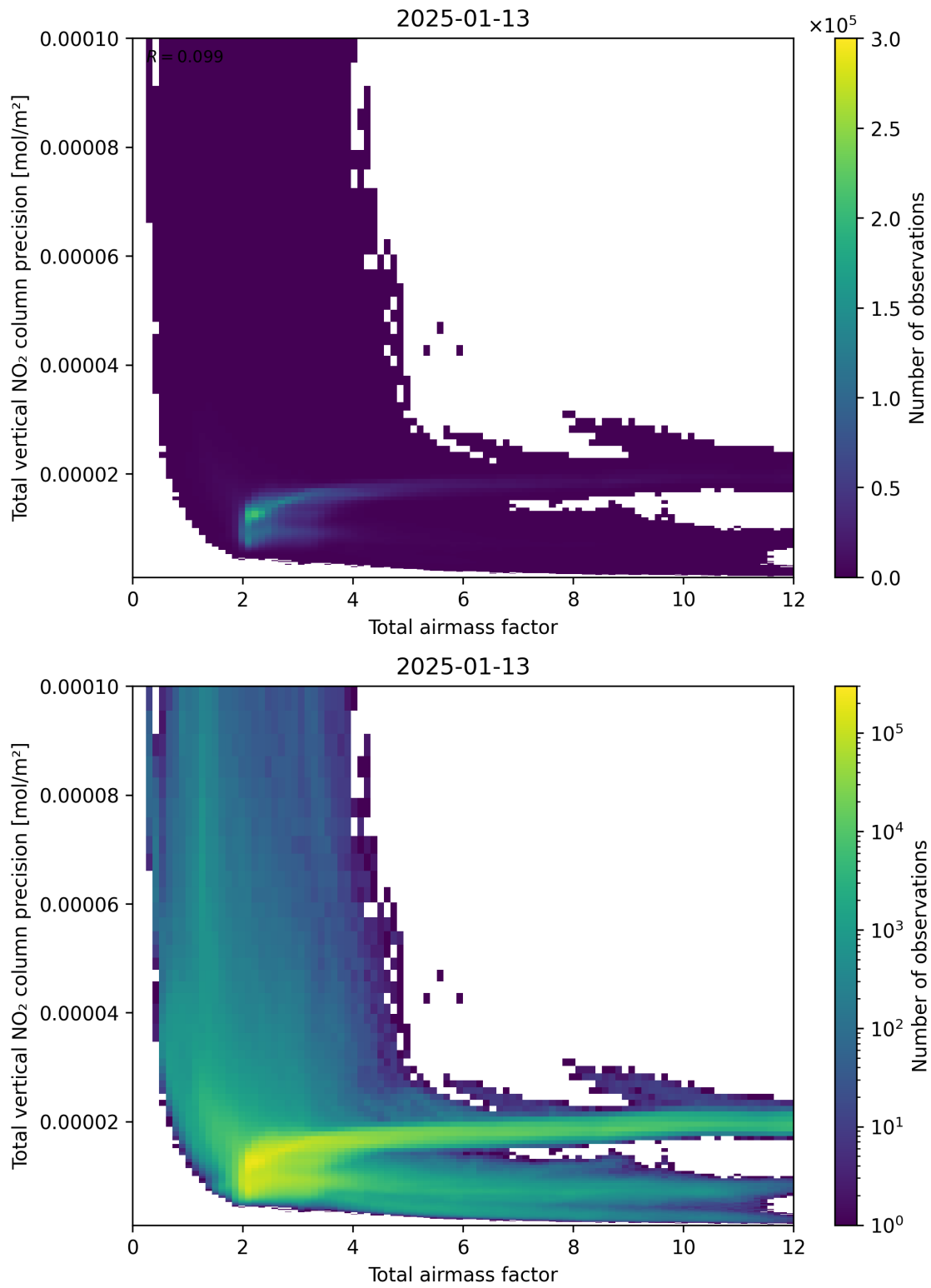
Figure 68: Scatter density plot of “Total airmass factor” against “Total vertical NO 2 column precision” for 2025-01-12 to 2025-01-14.
