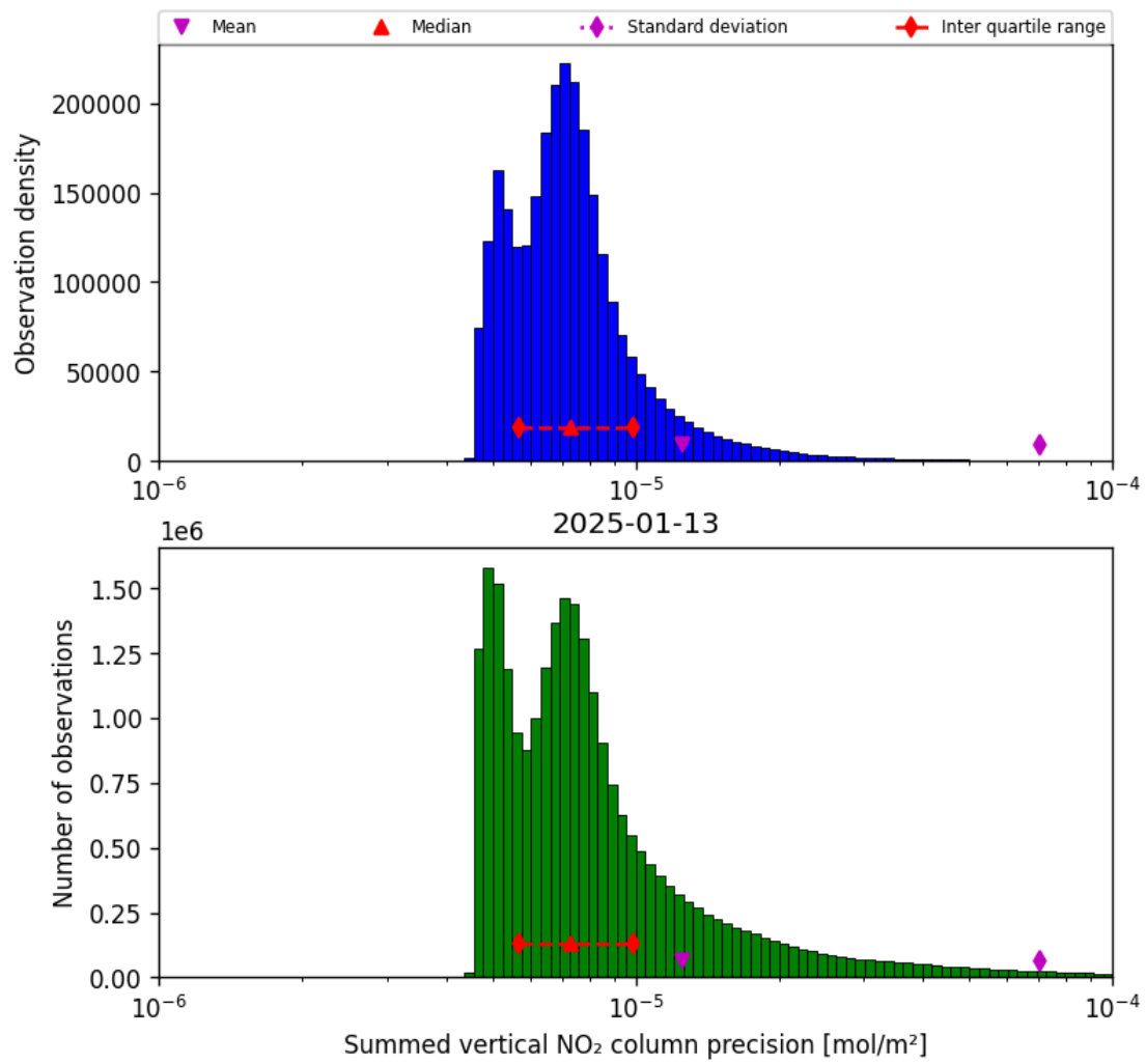
Figure 41: Histogram of “Summed vertical NO 2 column precision” for 2025-01-12 to 2025-01-14
