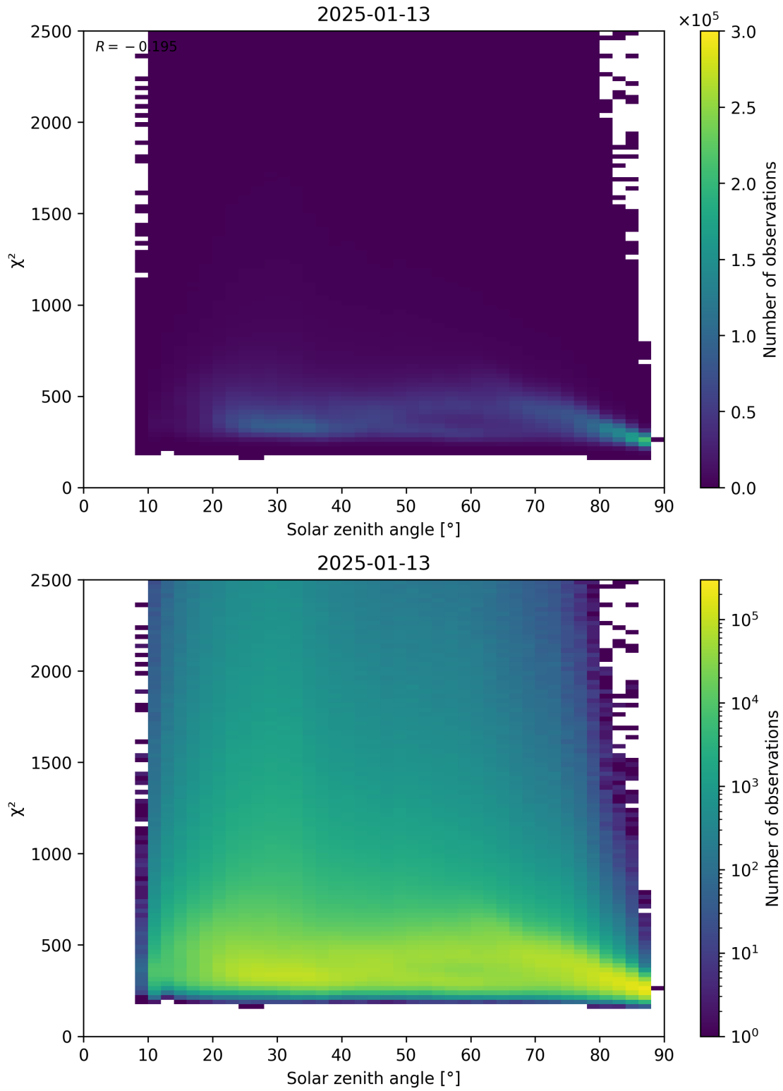
Figure 148: Scatter density plot of “Solar zenith angle” against “ \chi^2 ” for 2025-01-12 to 2025-01-14.
