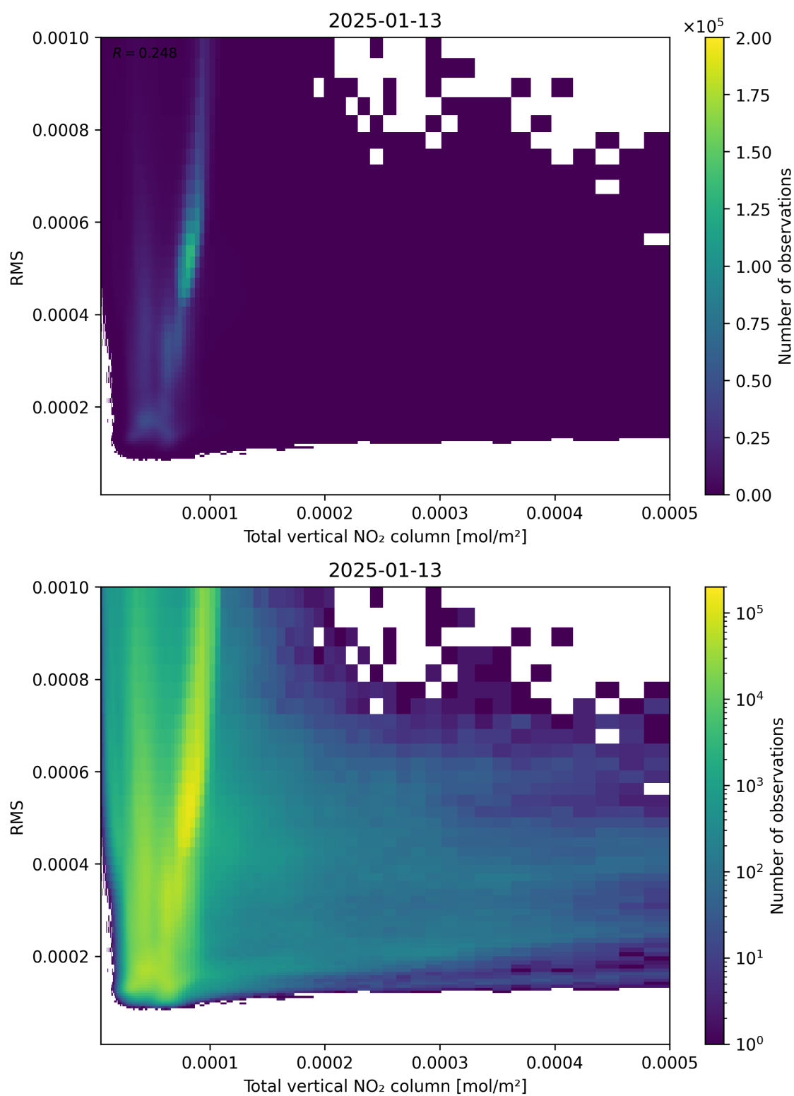
Figure 120: Scatter density plot of “Total vertical NO 2 column” against “RMS” for 2025-01-12 to 2025-01-14.
