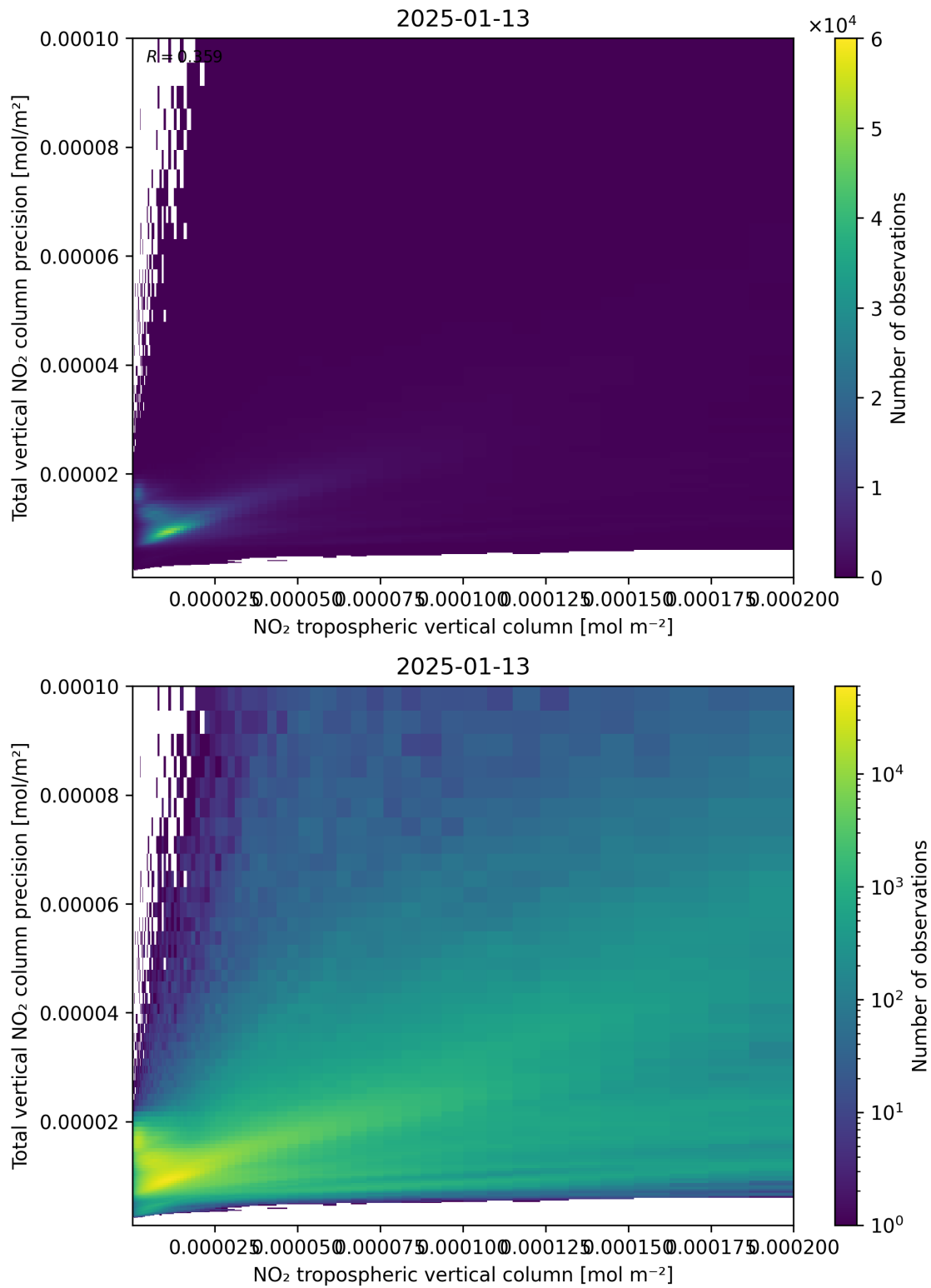
Figure 129: Scatter density plot of “NO 2 tropospheric vertical column” against “Total vertical NO 2 column precision” for 2025-01-12 to 2025-01-14.
