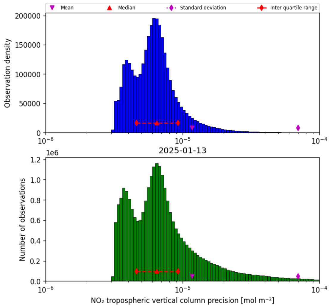
Figure 30: Histogram of “NO 2 tropospheric vertical column precision” for 2025-01-12 to 2025-01-14
