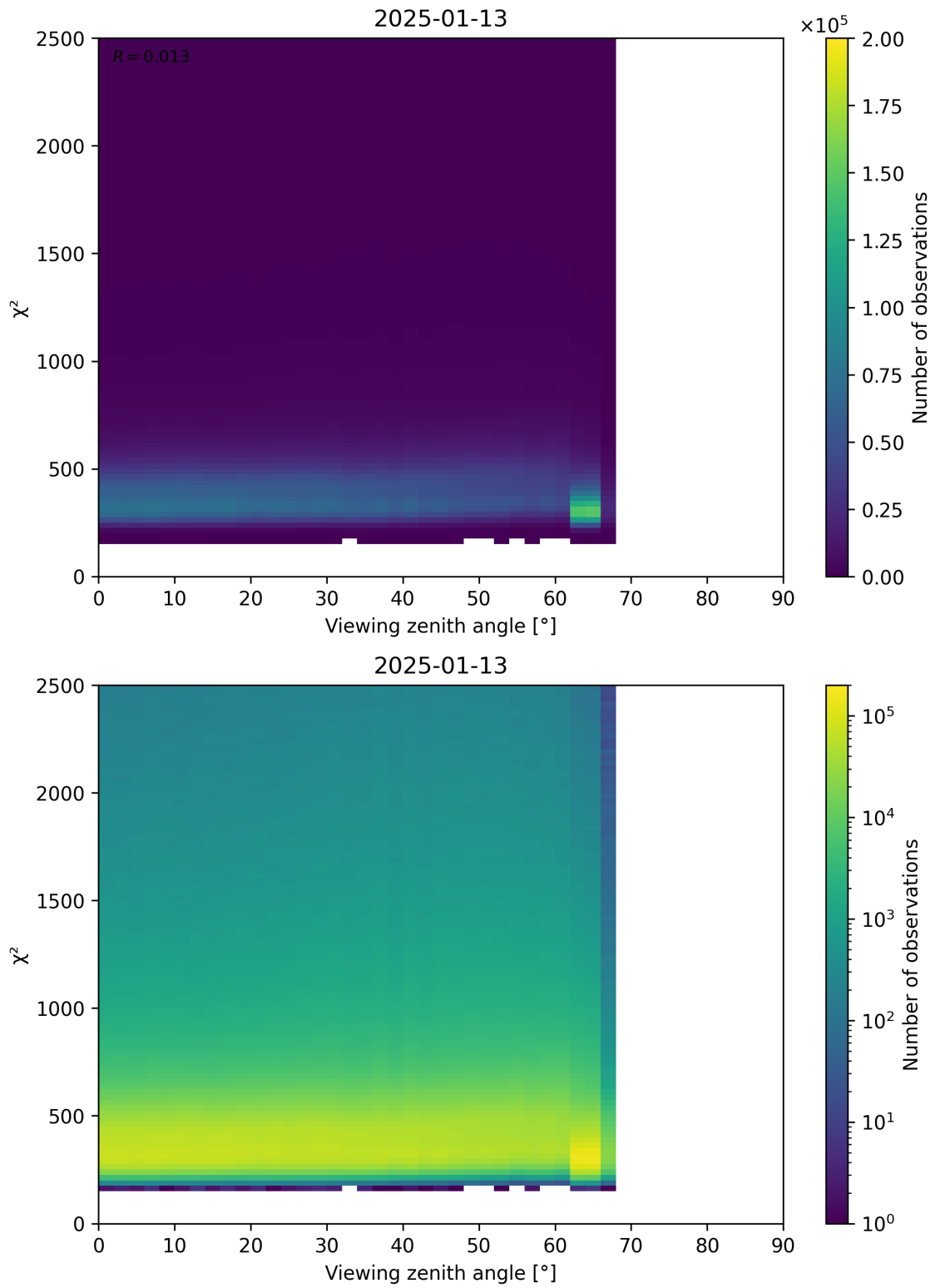
Figure 162: Scatter density plot of “Viewing zenith angle” against “ \chi^2 ” for 2025-01-12 to 2025-01-14.
