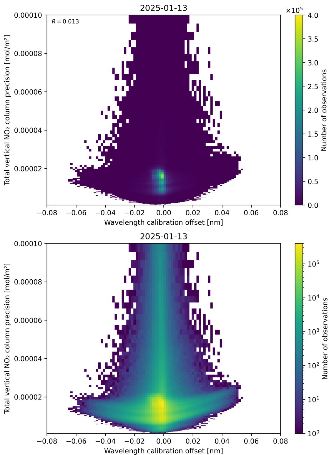
Figure 180: Scatter density plot of “Wavelength calibration offset” against “Total vertical NO 2 column precision” for 2025-01-12 to 2025-01-14.
