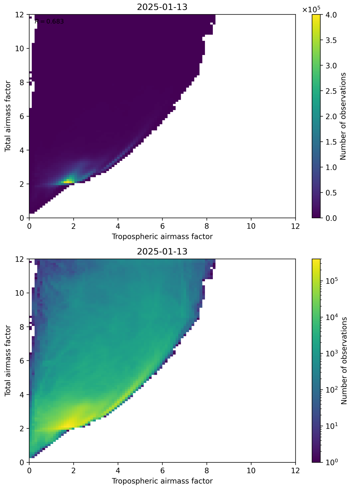
Figure 72: Scatter density plot of “Tropospheric airmass factor” against “Total airmass factor” for 2025-01-12 to 2025-01-14.
