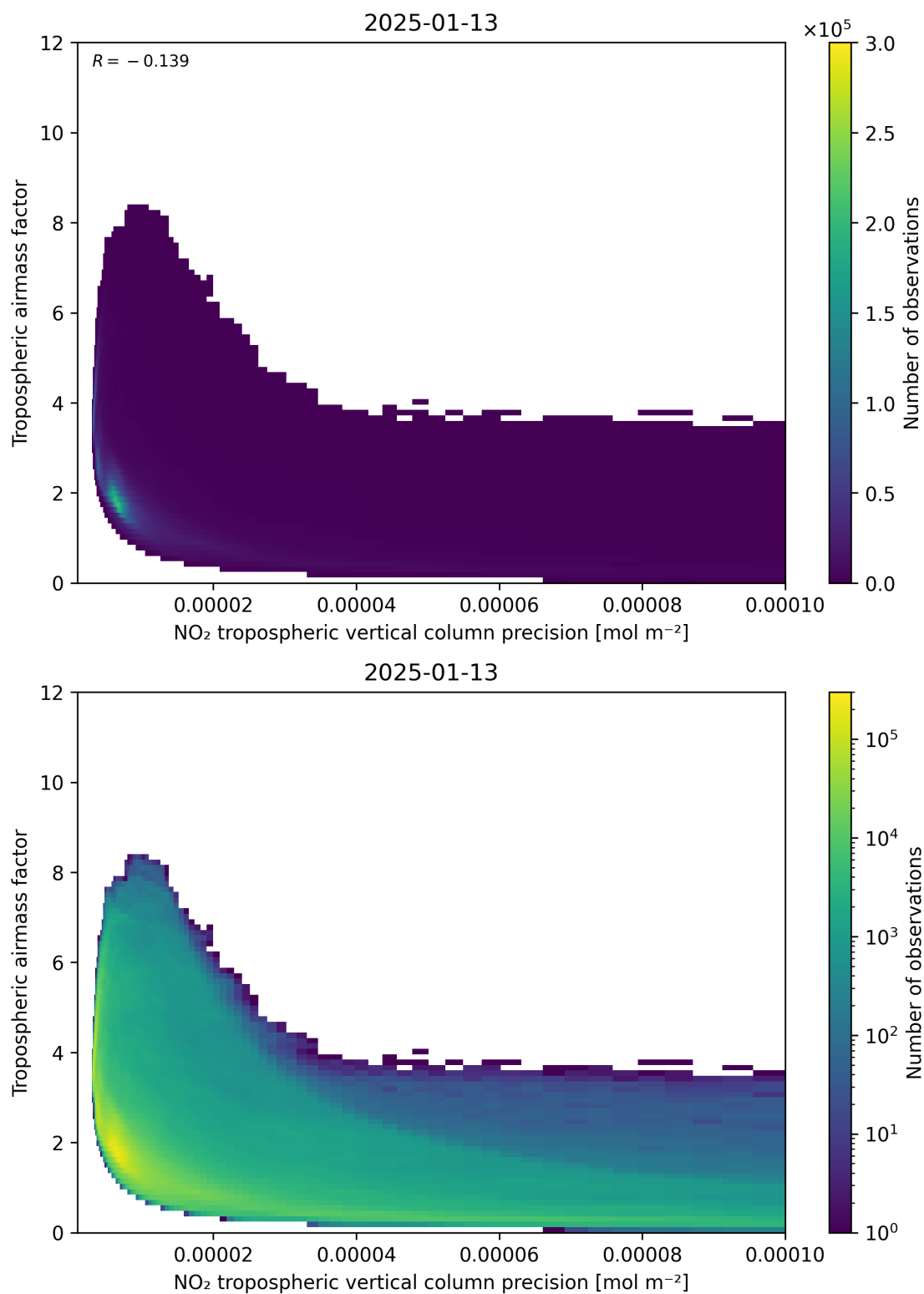
Figure 133: Scatter density plot of “NO 2 tropospheric vertical column precision” against “Tropospheric air mass factor” for 2025-01-12 to 2025-01-14.
