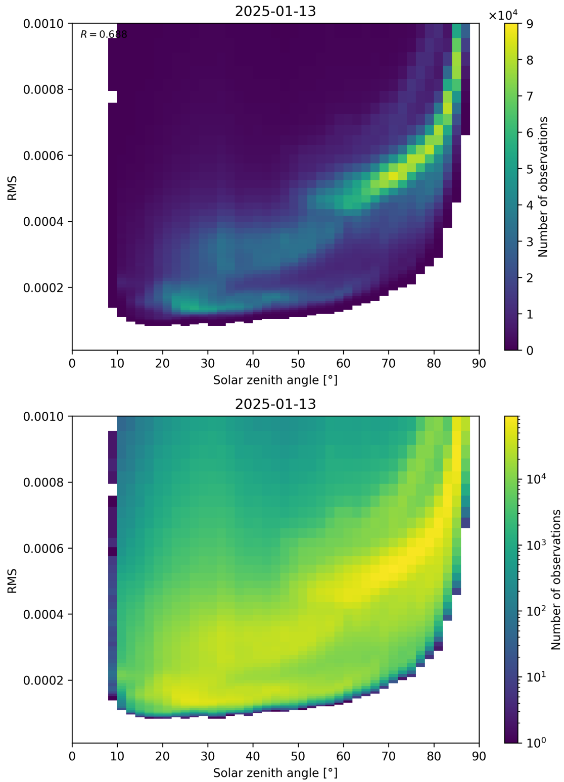
Figure 157: Scatter density plot of “Solar zenith angle” against “RMS” for 2025-01-12 to 2025-01-14.
