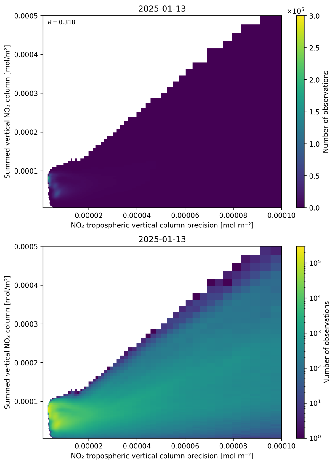
Figure 136: Scatter density plot of “NO 2 tropospheric vertical column precision” against “Summed vertical NO 2 column” for 2025-01-12 to 2025-01-14.
