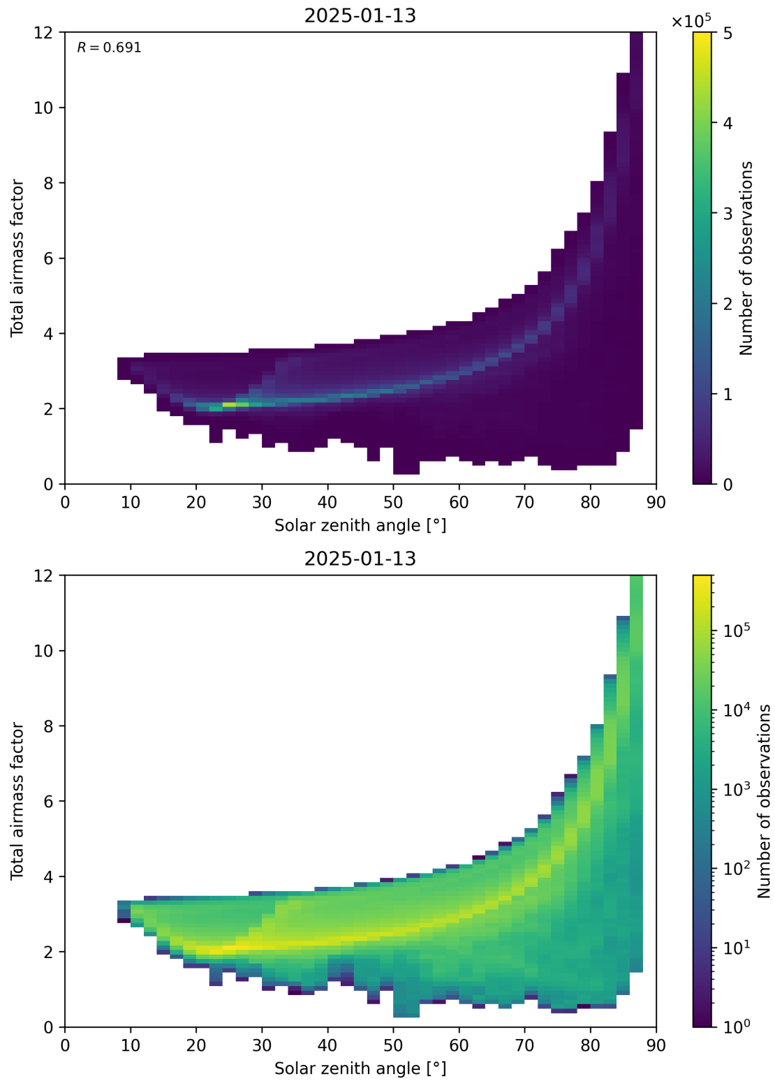
Figure 146: Scatter density plot of “Solar zenith angle” against “Total air mass factor” for 2025-01-12 to 2025-01-14.
