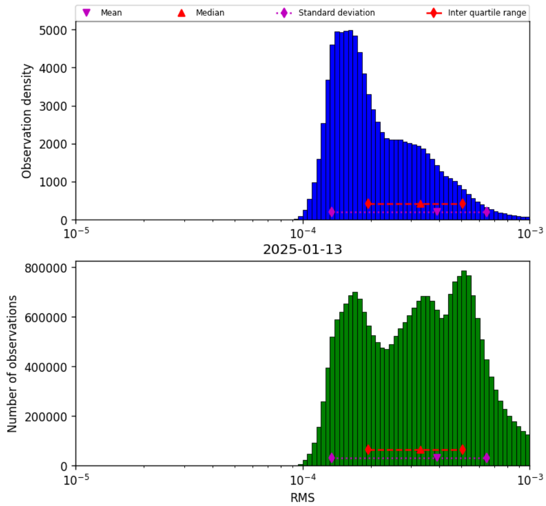
Figure 43: Histogram of “RMS” for 2025-01-12 to 2025-01-14
