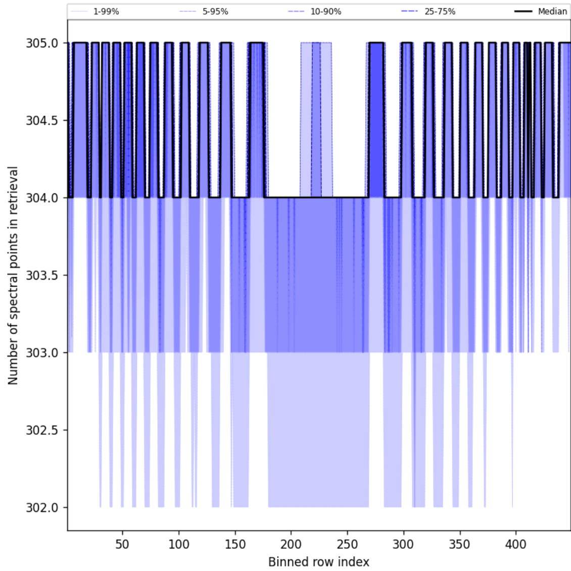
Figure 50: Along track statistics of “Number of spectral points in retrieval” for 2025-01-12 to 2025-01-14
