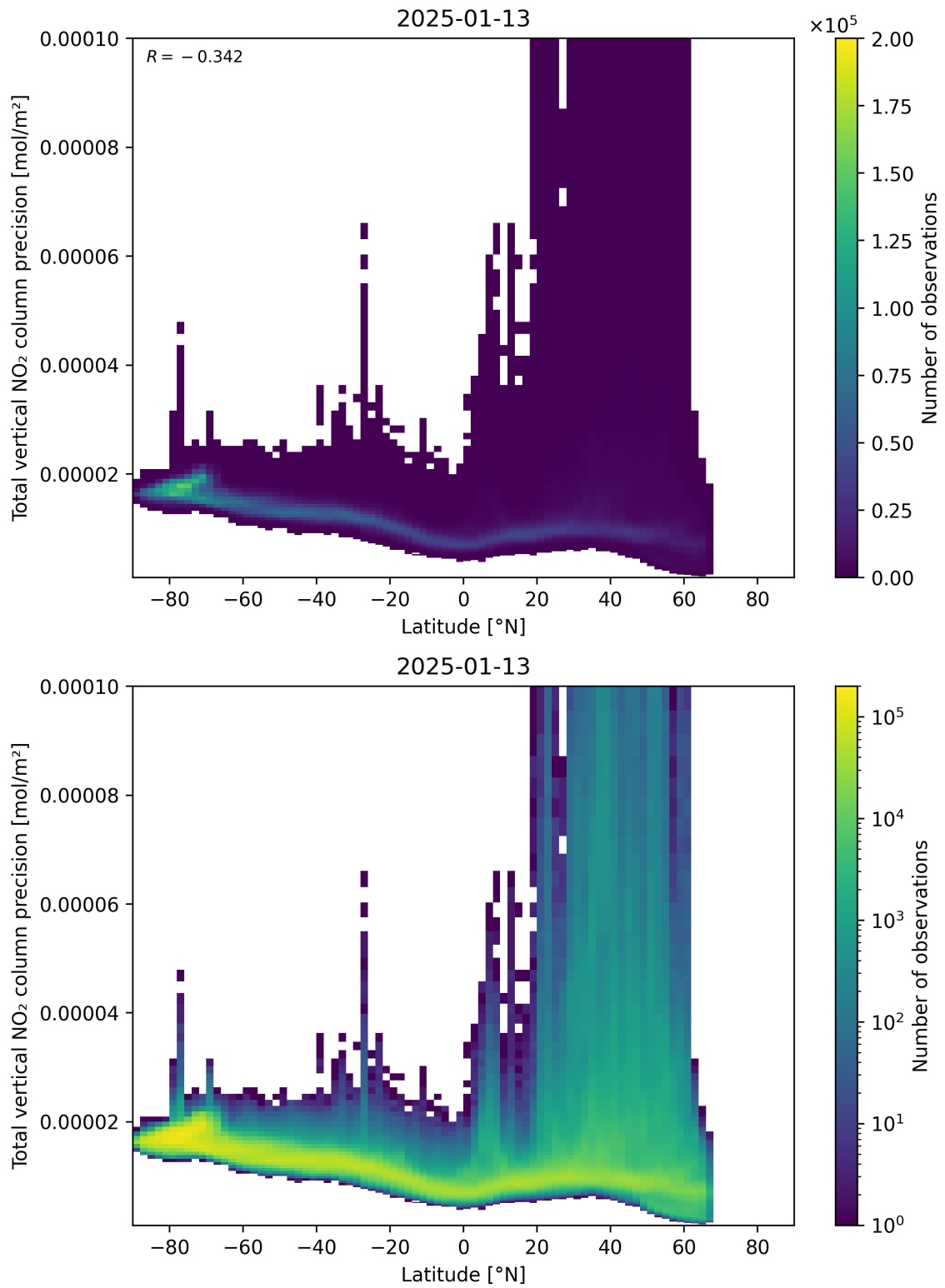
Figure 91: Scatter density plot of “Latitude” against “Total vertical NO 2 column precision” for 2025-01-12 to 2025-01-14.
