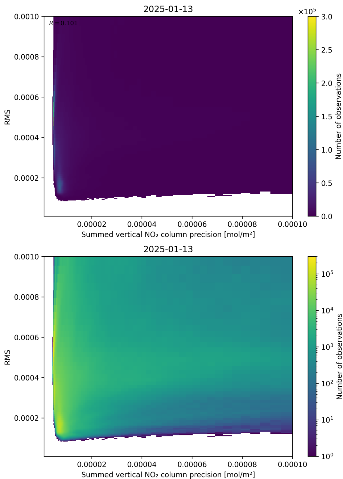
Figure 108: Scatter density plot of “Summed vertical NO 2 column precision” against “RMS” for 2025-01-12 to 2025-01-14.
