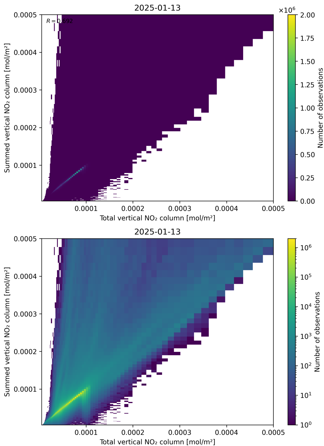
Figure 112: Scatter density plot of “Total vertical NO 2 column” against “Summed vertical NO 2 column” for 2025-01-12 to 2025-01-14.
