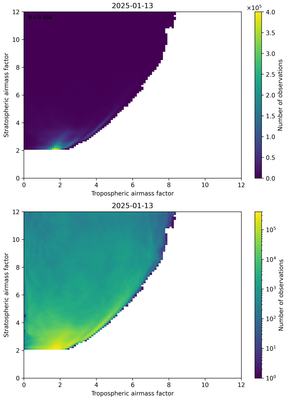
Figure 71: Scatter density plot of “Tropospheric airmass factor” against “Stratospheric airmass factor” for 2025-01-12 to 2025-01-14.
