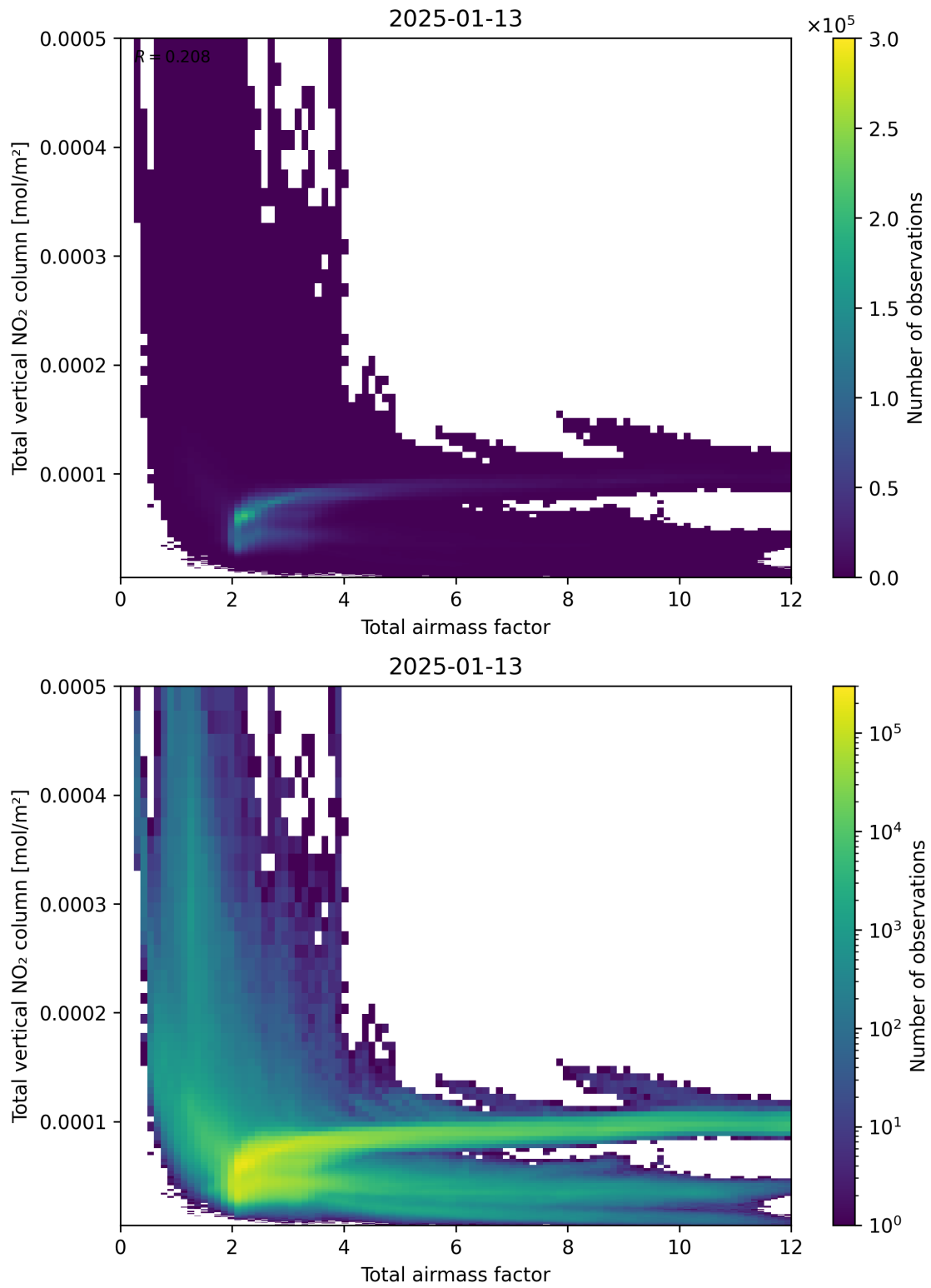
Figure 67: Scatter density plot of “Total air mass factor” against “Total vertical NO 2 column” for 2025-01-12 to 2025-01-14.
