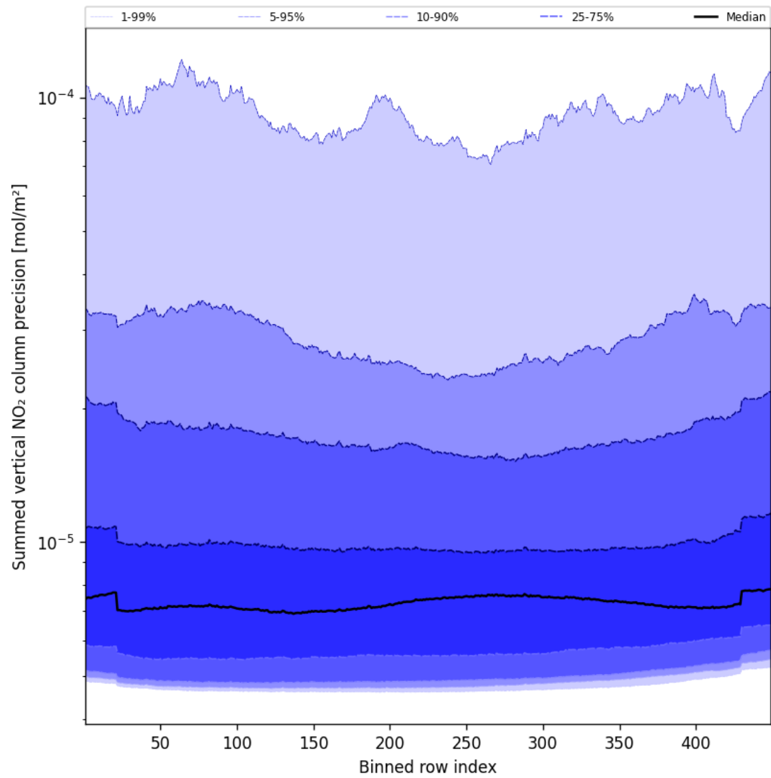
Figure 58: Along track statistics of “Summed vertical NO 2 column precision” for 2025-01-12 to 2025-01-14
