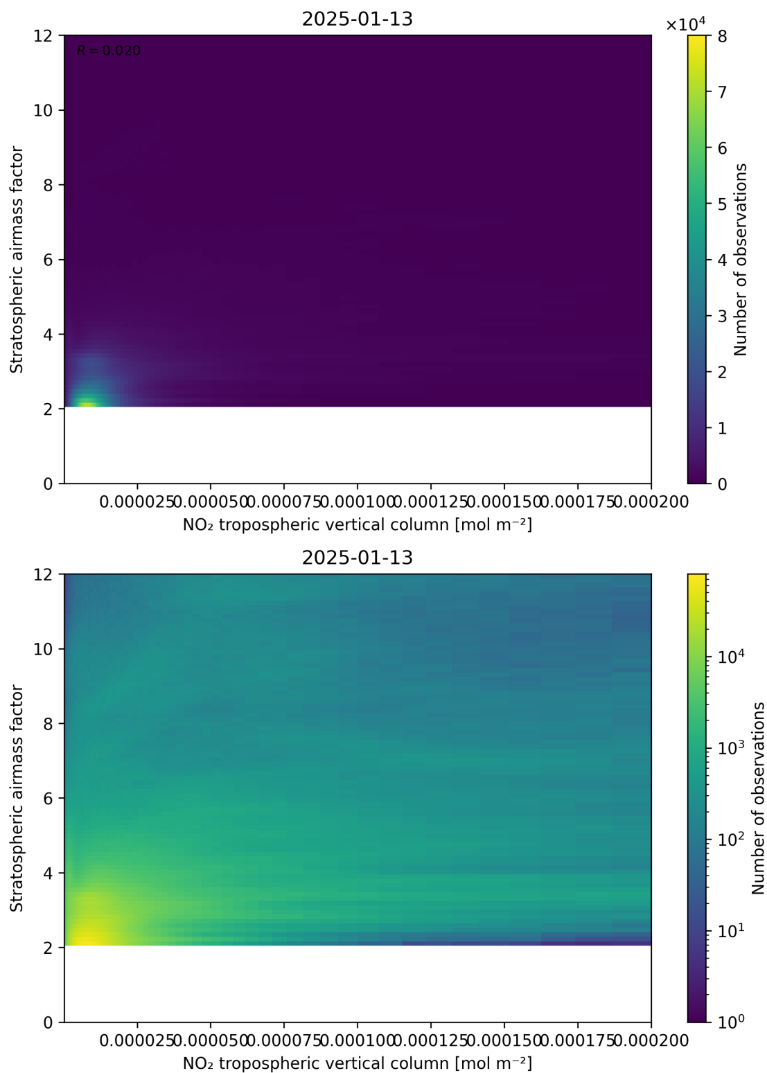
Figure 121: Scatter density plot of “NO 2 tropospheric vertical column” against “Stratospheric airmass factor” for 2025-01-12 to 2025-01-14.
