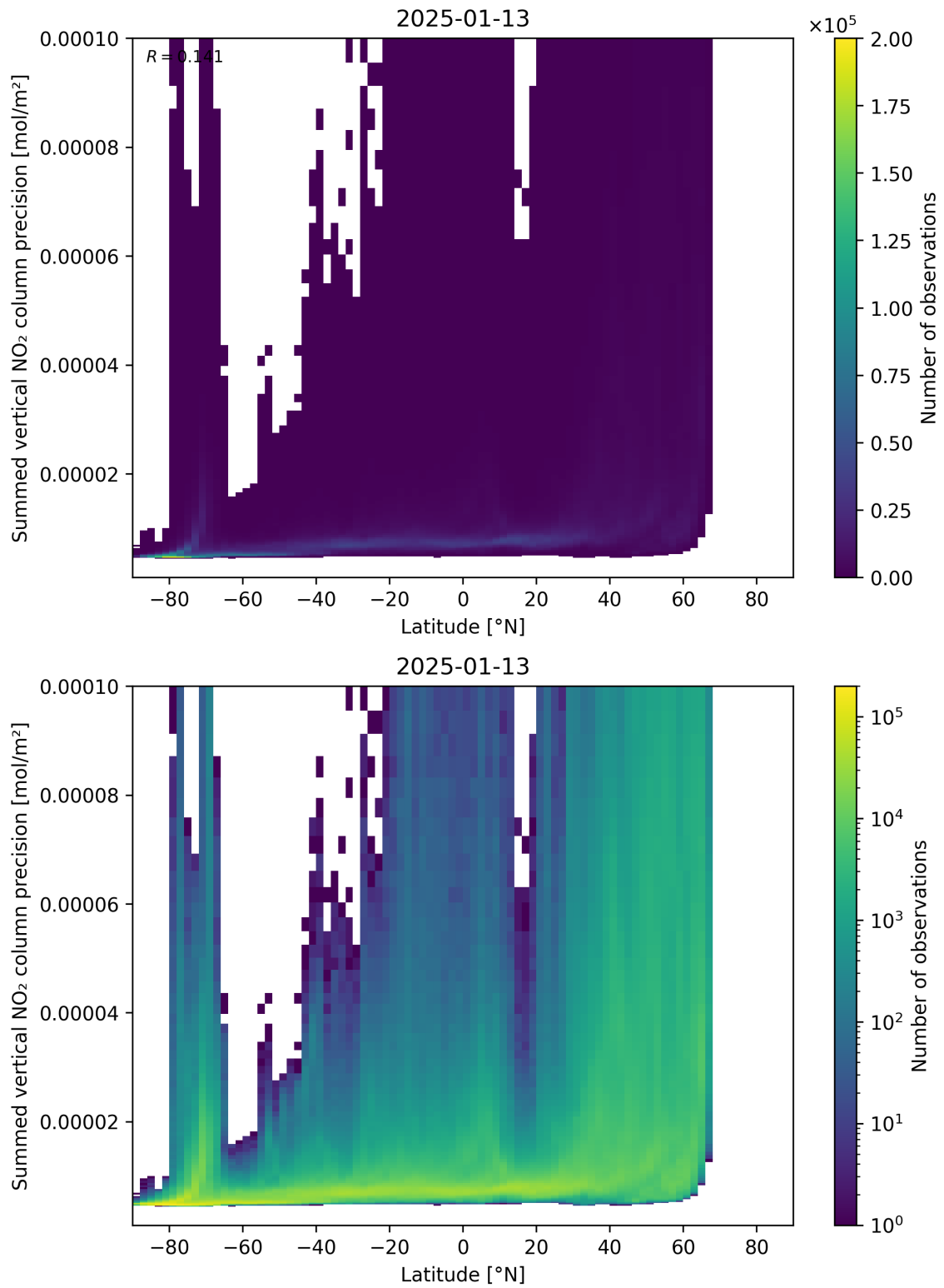
Figure 89: Scatter density plot of “Latitude” against “Summed vertical NO 2 column precision” for 2025-01-12 to 2025-01-14.
