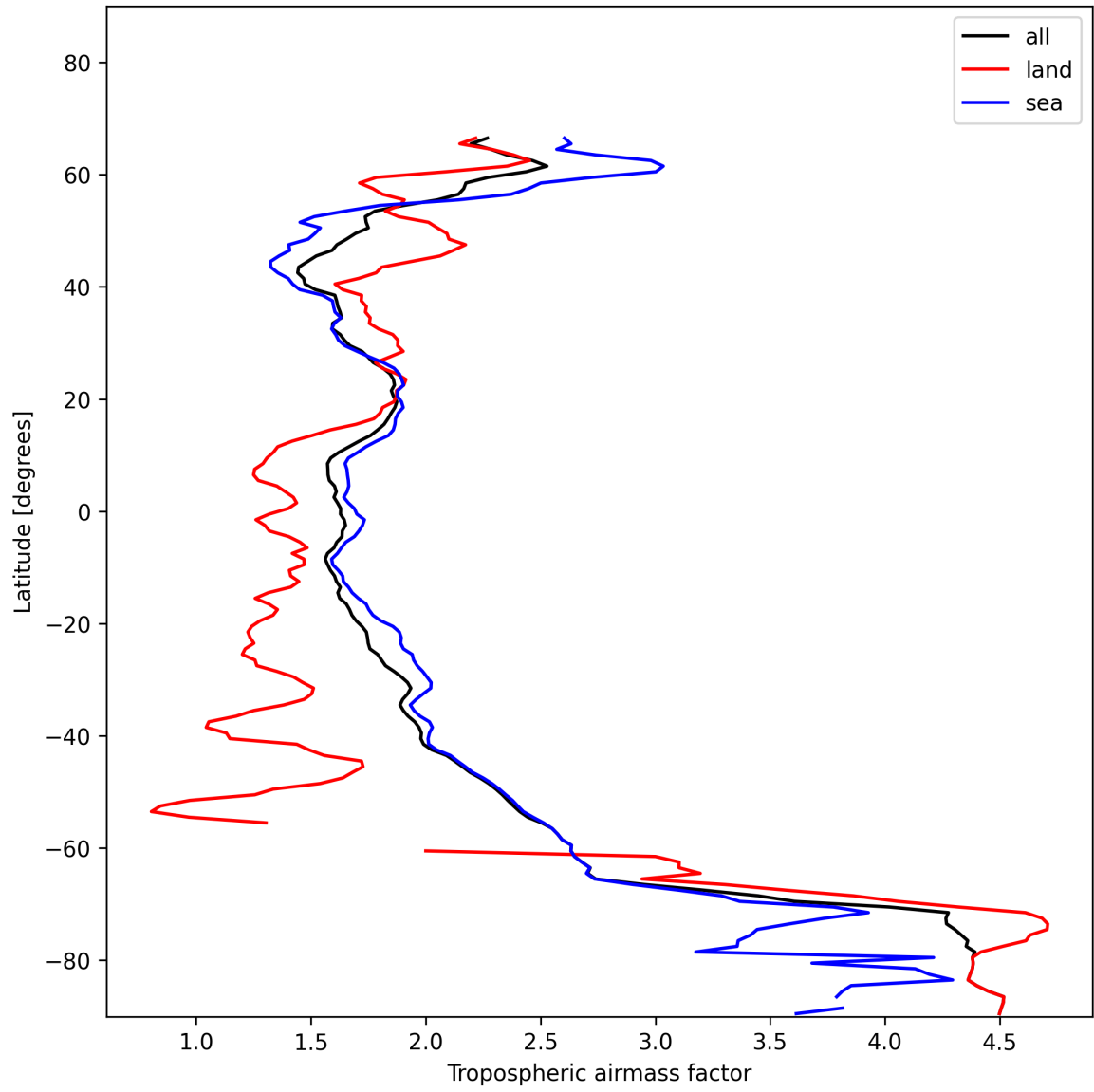
Figure 14: Zonal average of “Tropospheric airmass factor” for 2025-01-12 to 2025-01-14.
