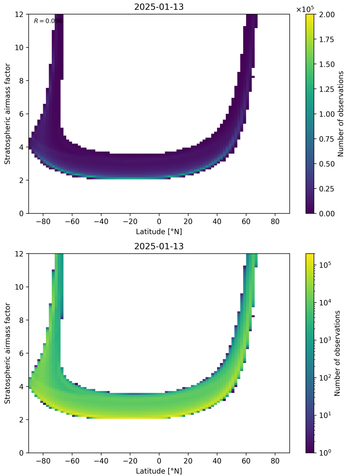
Figure 83: Scatter density plot of “Latitude” against “Stratospheric airmass factor” for 2025-01-12 to 2025-01-14.
