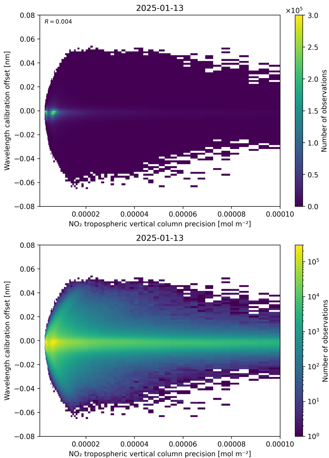
Figure 141: Scatter density plot of “NO 2 tropospheric vertical column precision” against “Wavelength calibration offset” for 2025-01-12 to 2025-01-14.
