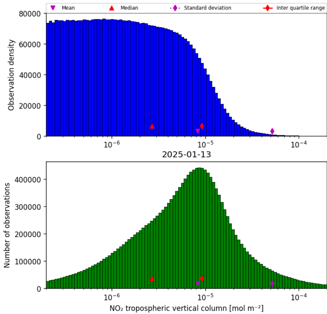
Figure 29: Histogram of “NO 2 tropospheric vertical column” for 2025-01-12 to 2025-01-14
