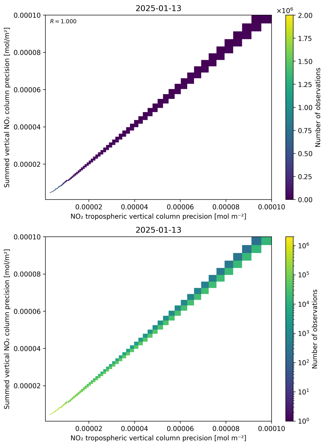
Figure 137: Scatter density plot of “NO 2 tropospheric vertical column precision” against “Summed vertical NO 2 column precision” for 2025-01-12 to 2025-01-14.
