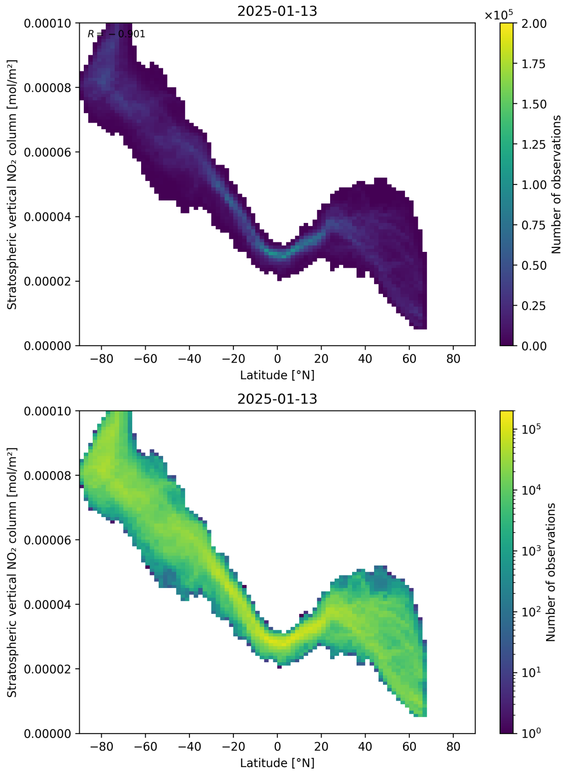
Figure 87: Scatter density plot of “Latitude” against “Stratospheric vertical NO 2 column” for 2025-01-12 to 2025-01-14.
