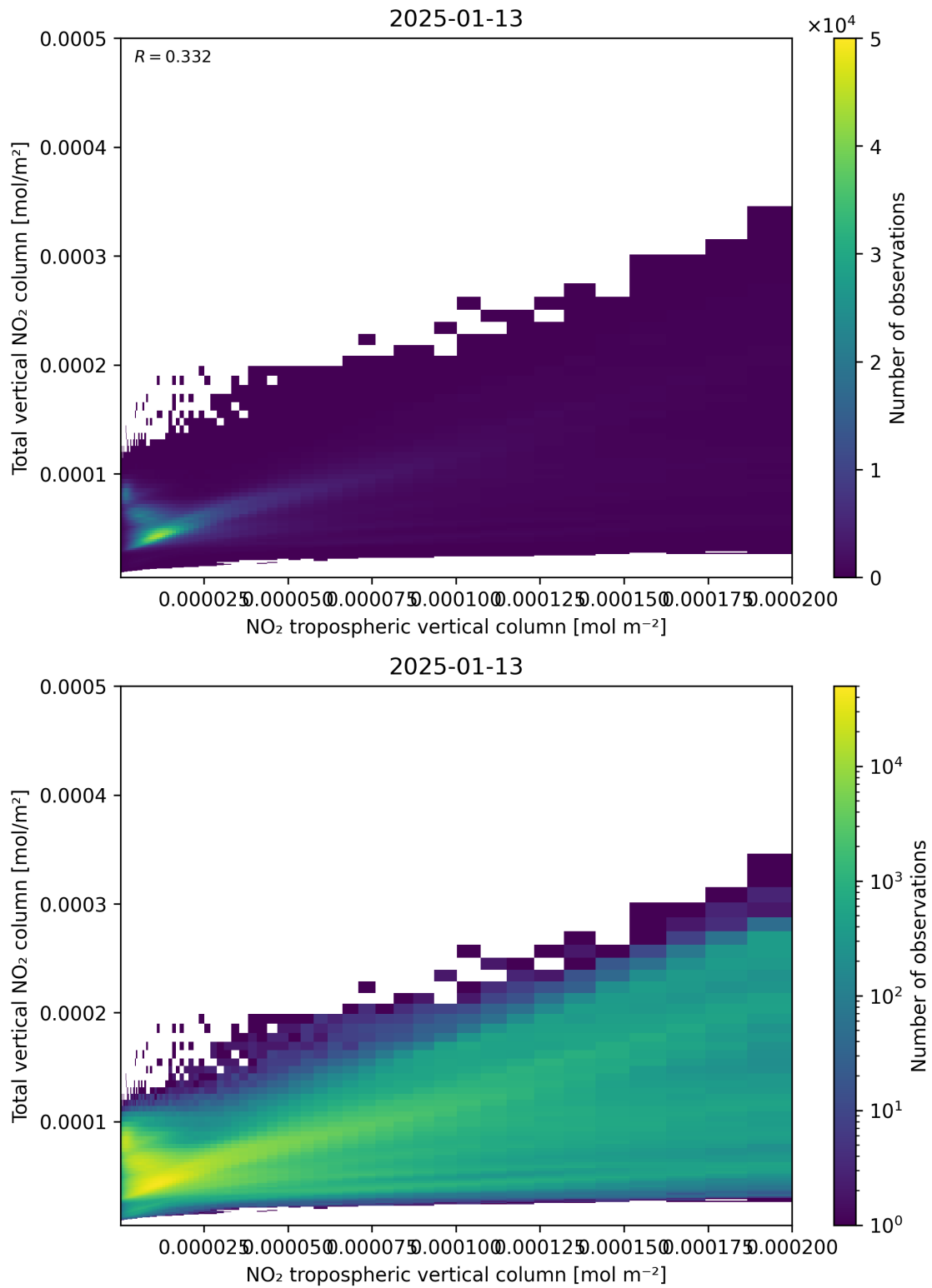
Figure 128: Scatter density plot of “NO 2 tropospheric vertical column” against “Total vertical NO 2 column” for 2025-01-12 to 2025-01-14.
