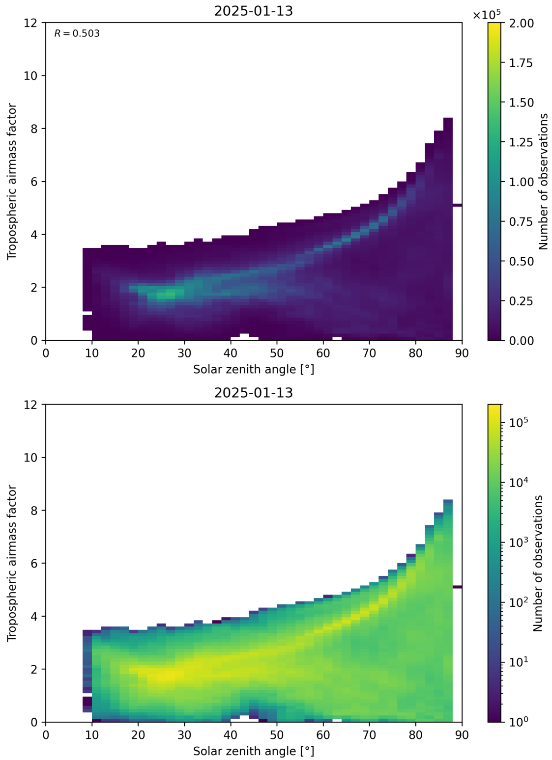
Figure 147: Scatter density plot of “Solar zenith angle” against “Tropospheric airmass factor” for 2025-01-12 to 2025-01-14.
