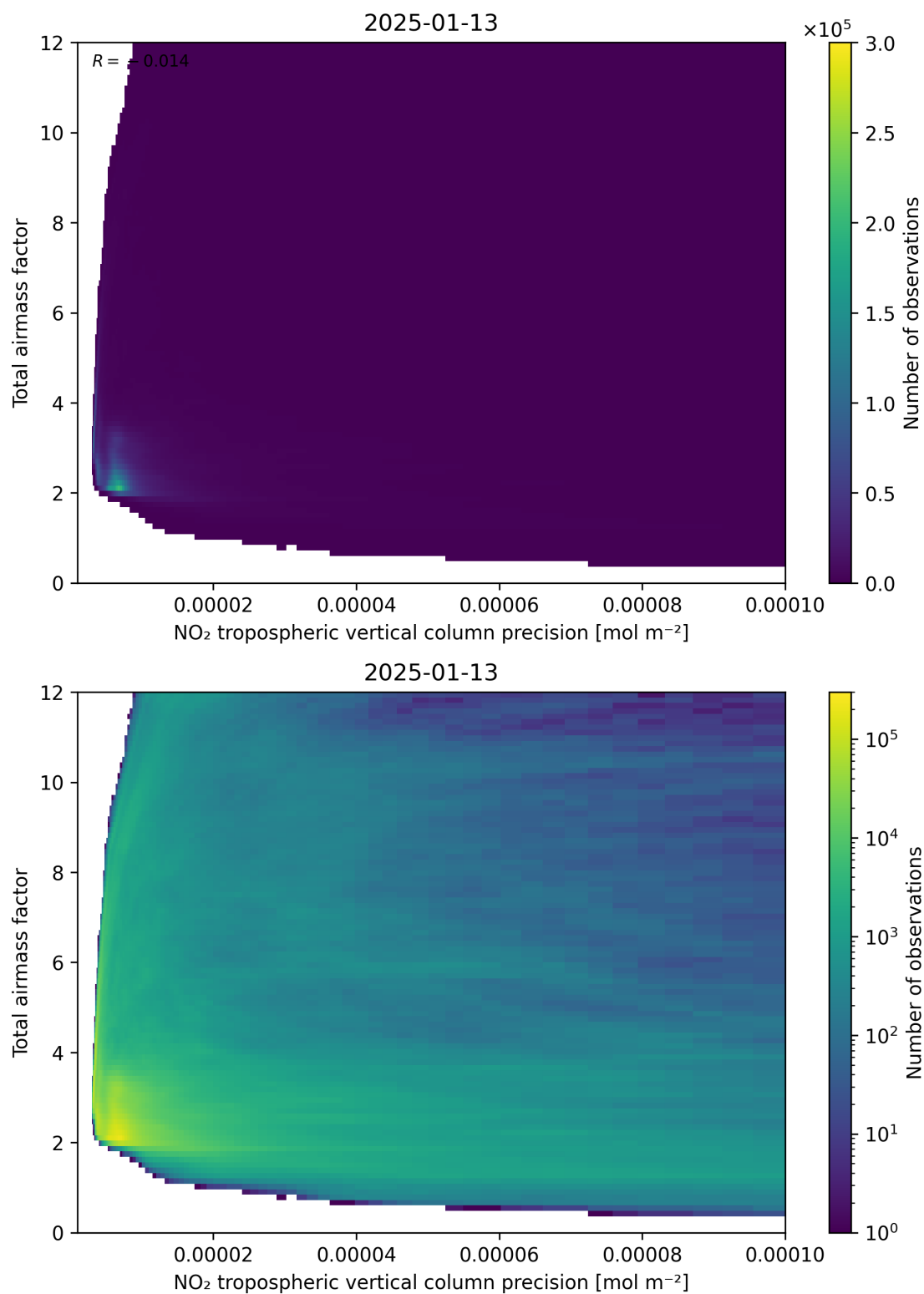
Figure 132: Scatter density plot of “NO 2 tropospheric vertical column precision” against “Total air mass factor” for 2025-01-12 to 2025-01-14.
