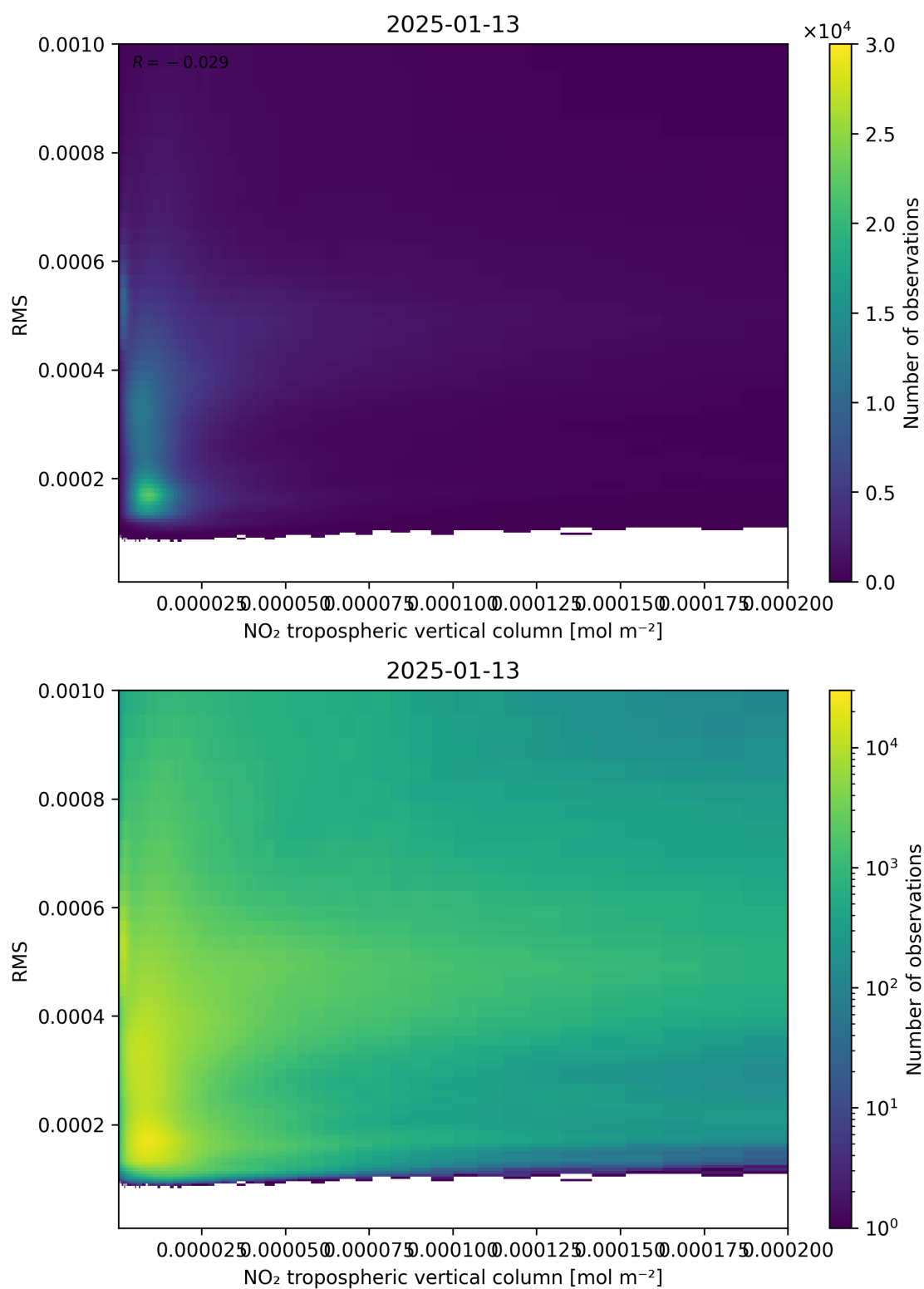
Figure 142: Scatter density plot of “NO 2 tropospheric vertical column” against “RMS” for 2025-01-12 to 2025-01-14.
