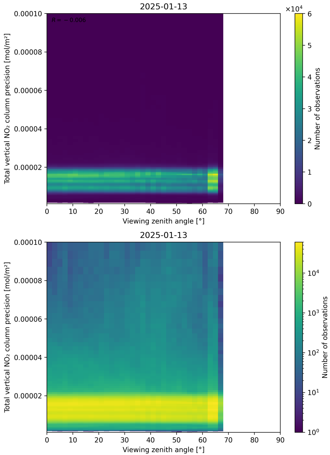
Figure 168: Scatter density plot of “Viewing zenith angle” against “Total vertical NO 2 column precision” for 2025-01-12 to 2025-01-14.
