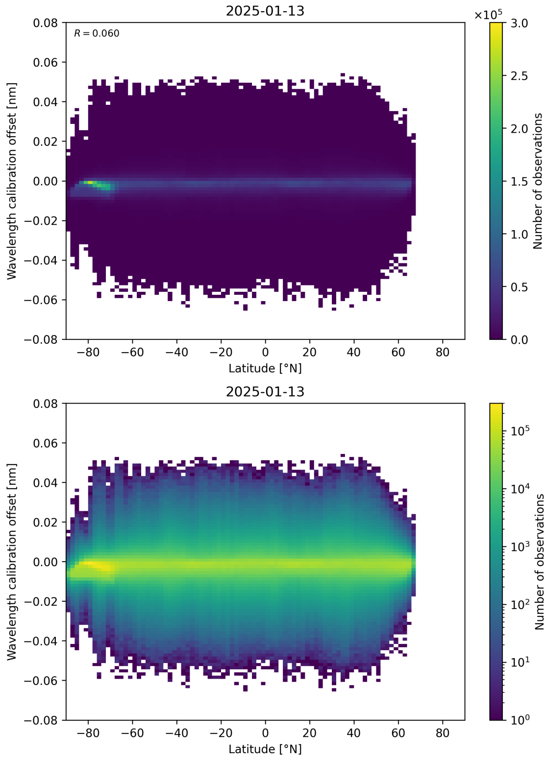
Figure 95: Scatter density plot of “Latitude” against “Wavelength calibration offset” for 2025-01-12 to 2025-01-14.
