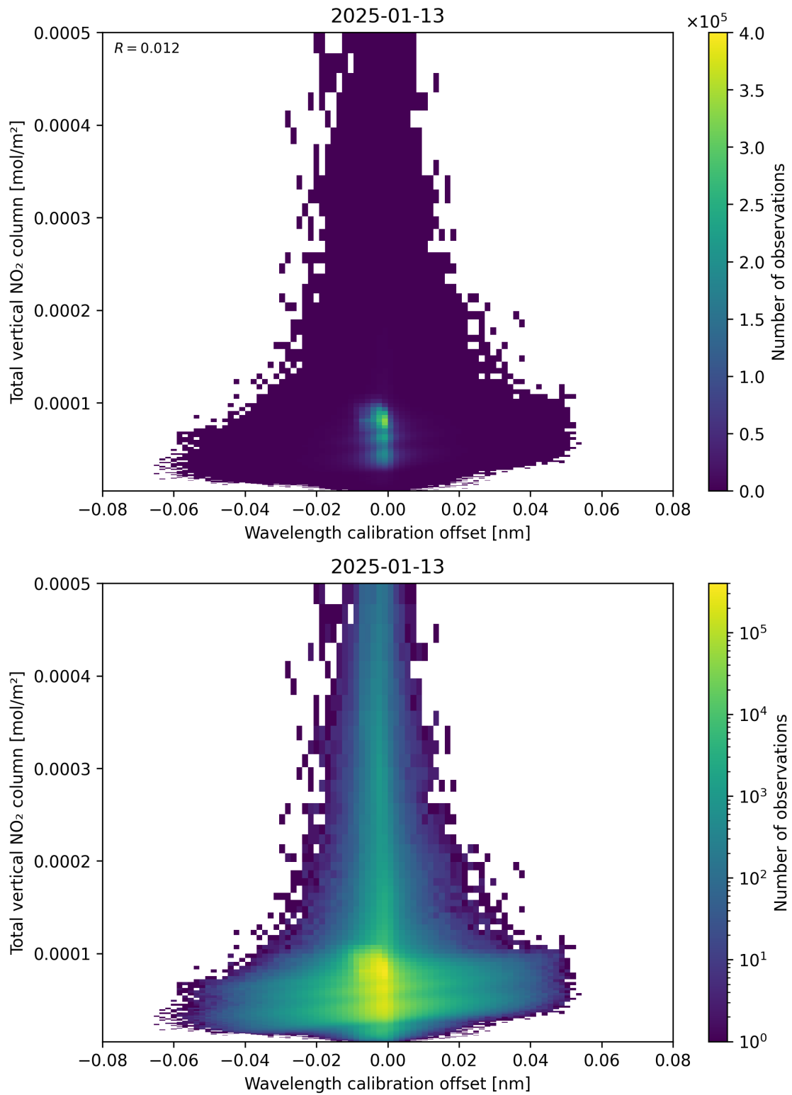
Figure 179: Scatter density plot of “Wavelength calibration offset” against “Total vertical NO 2 column” for 2025-01-12 to 2025-01-14.
