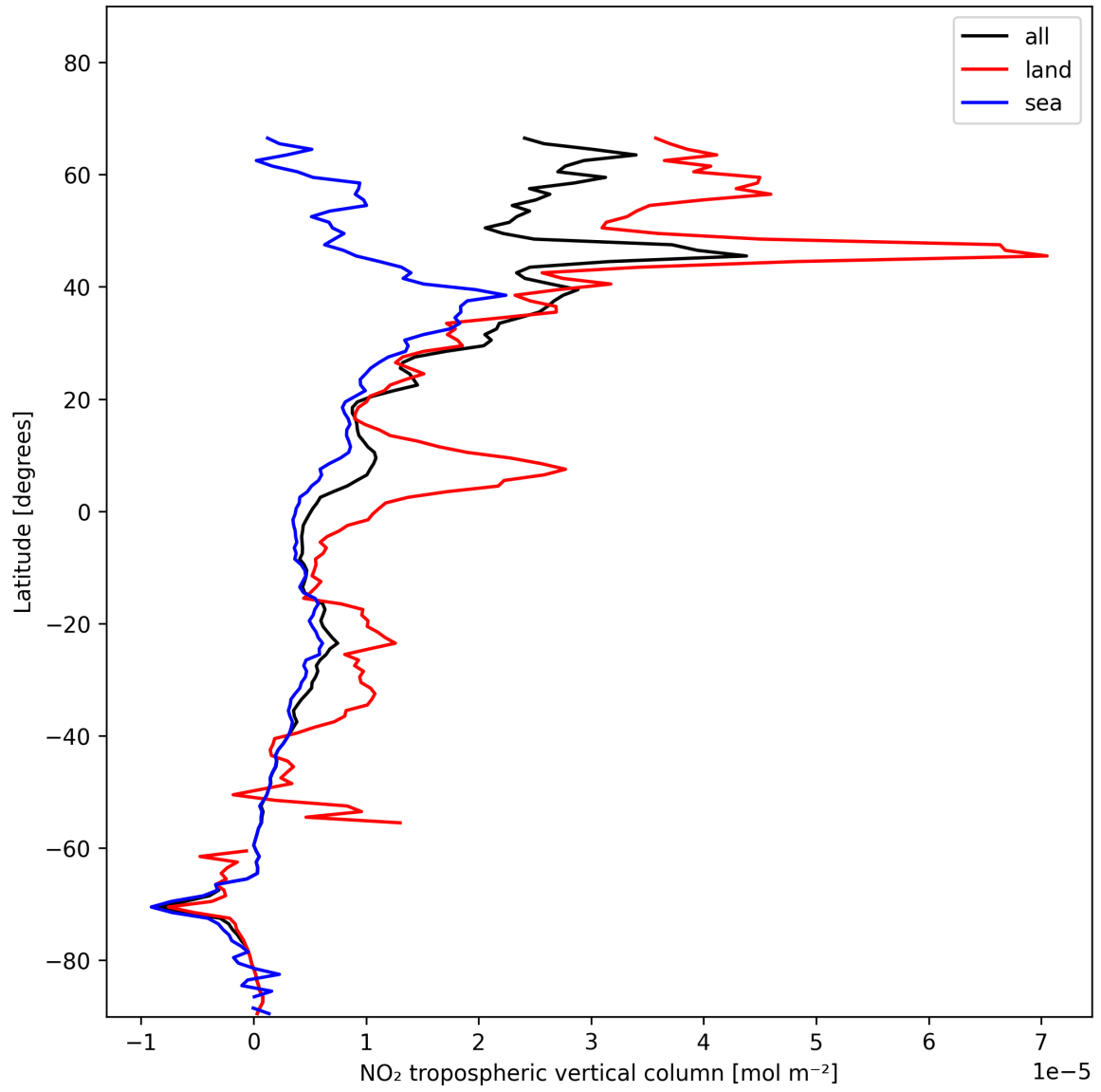
Figure 12: Zonal average of “NO 2 tropospheric vertical column” for 2025-01-12 to 2025-01-14.
