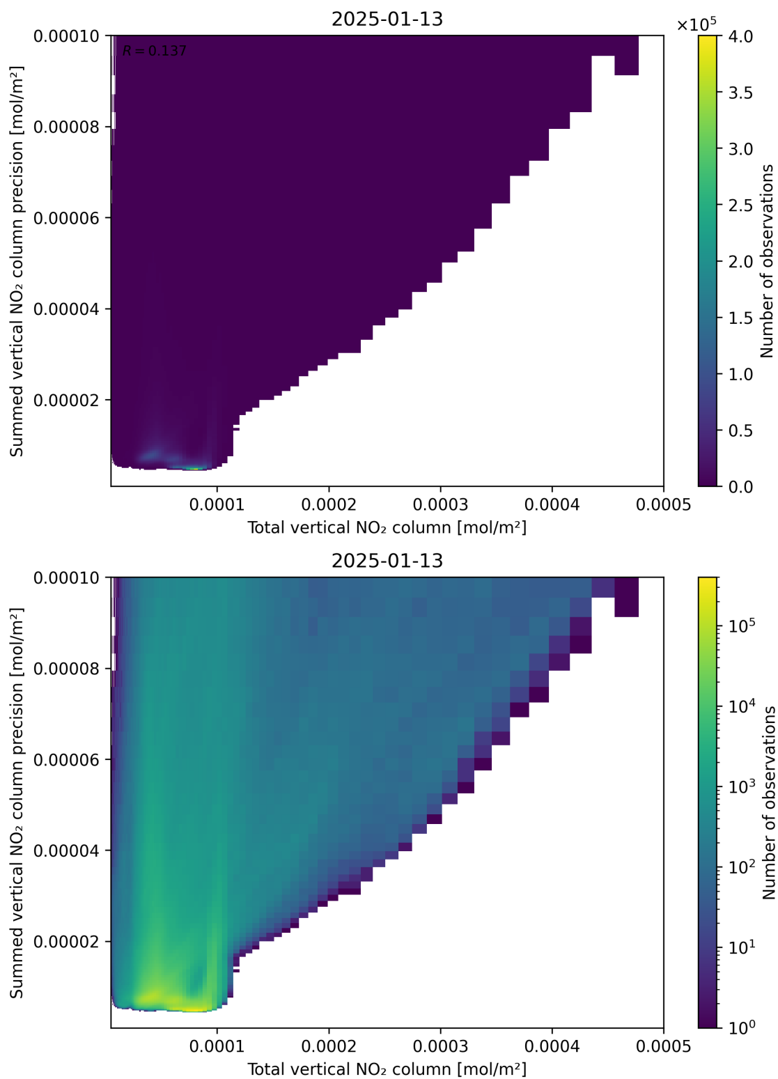
Figure 113: Scatter density plot of “Total vertical NO 2 column” against “Summed vertical NO 2 column precision” for 2025-01-12 to 2025-01-14.
