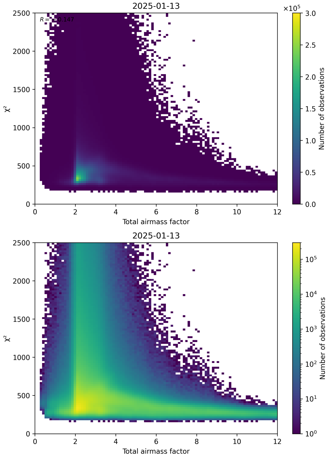
Figure 63: Scatter density plot of “Total airmass factor” against “ \chi^2 ” for 2025-01-12 to 2025-01-14.
