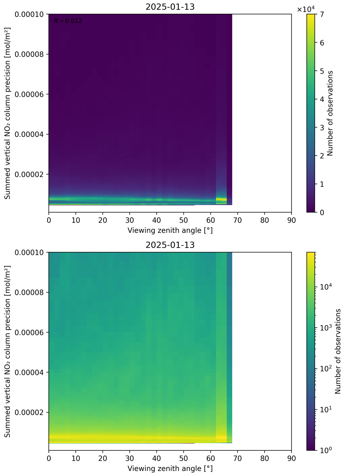
Figure 166: Scatter density plot of “Viewing zenith angle” against “Summed vertical NO 2 column precision” for 2025-01-12 to 2025-01-14.
