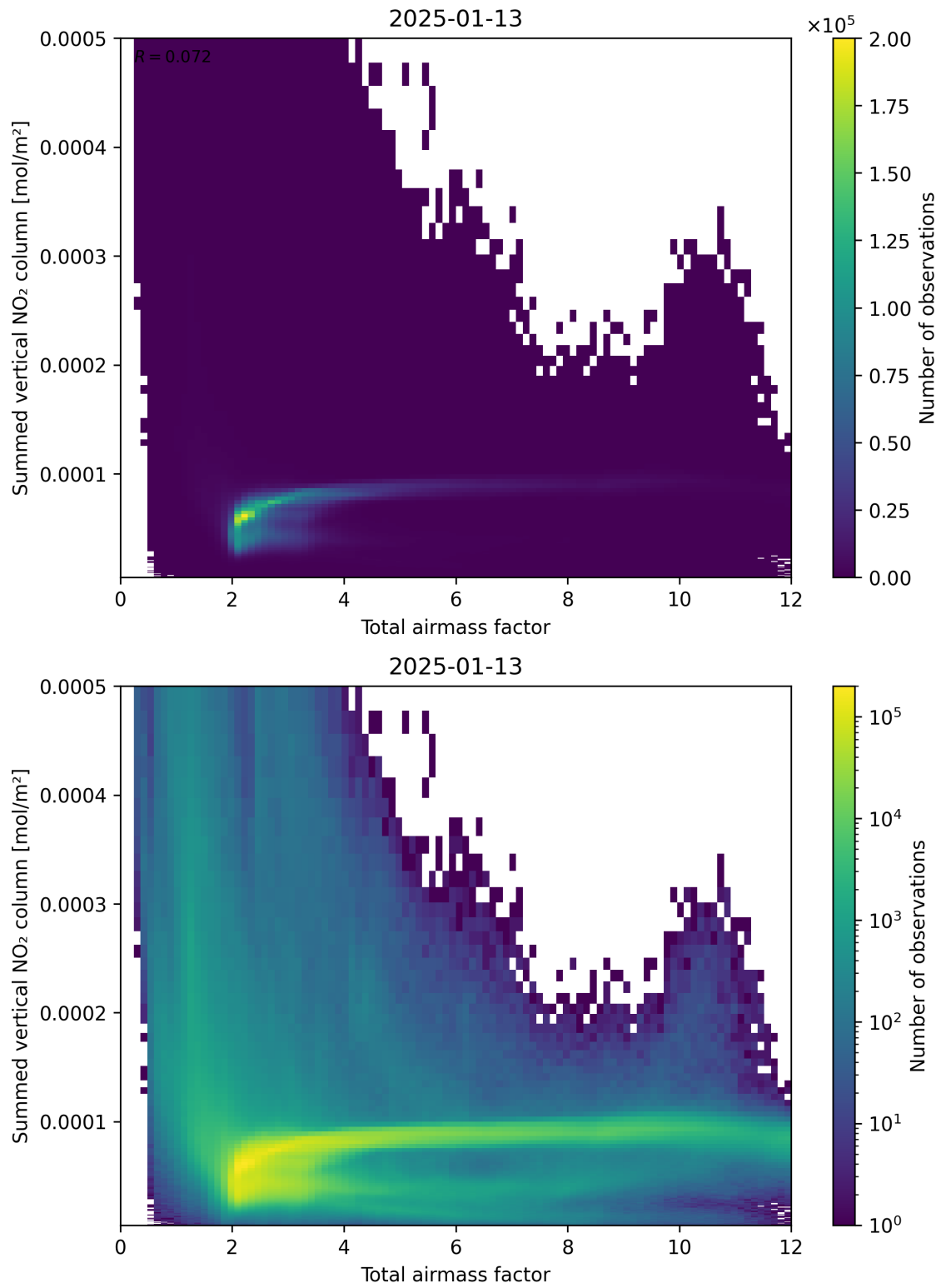
Figure 65: Scatter density plot of “Total airmass factor” against “Summed vertical NO 2 column” for 2025-01-12 to 2025-01-14.
