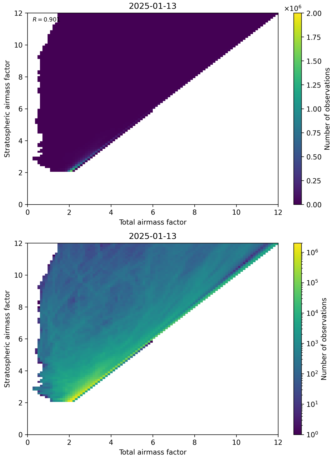
Figure 62: Scatter density plot of “Total airmass factor” against “Stratospheric airmass factor” for 2025-01-12 to 2025-01-14.
