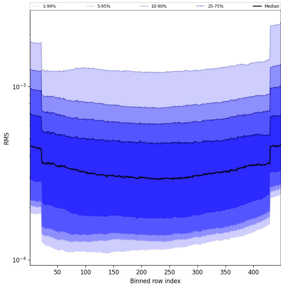
Figure 60: Along track statistics of “RMS” for 2025-01-12 to 2025-01-14
