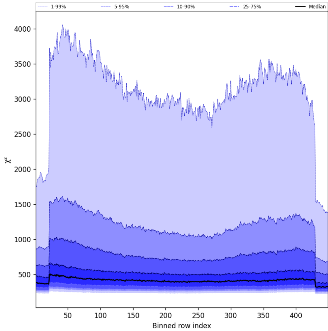
Figure 59: Along track statistics of “ \chi^2 ” for 2025-01-12 to 2025-01-14
