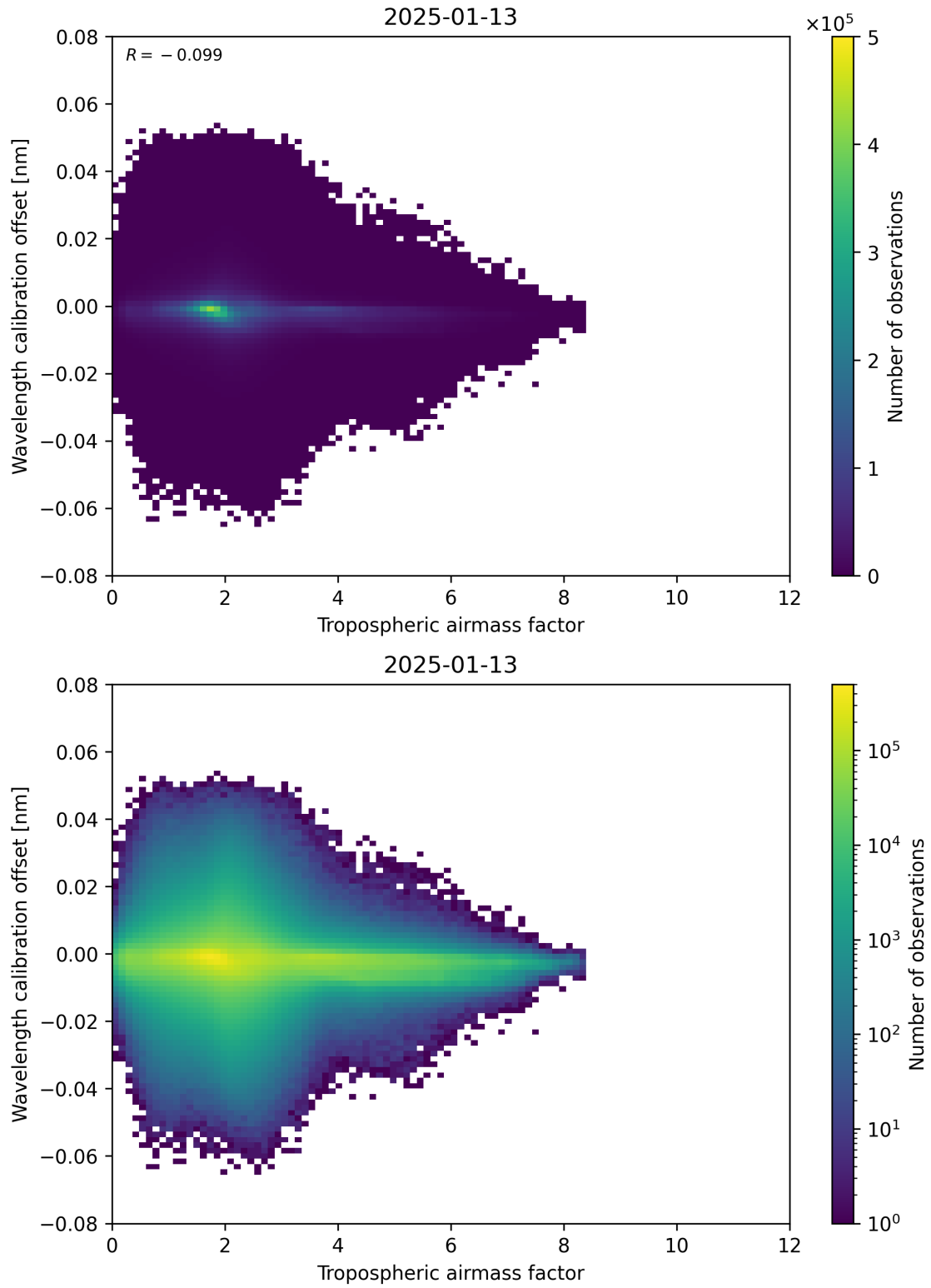
Figure 80: Scatter density plot of “Tropospheric airmass factor” against “Wavelength calibration offset” for 2025-01-12 to 2025-01-14.
