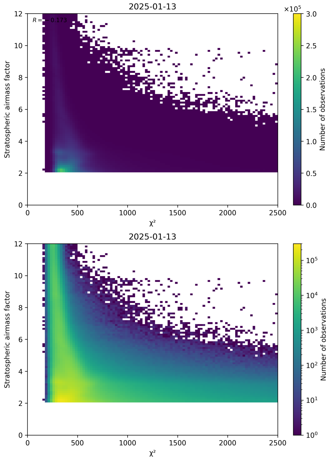
Figure 81: Scatter density plot of “ \chi^2 ” against “Stratospheric airmass factor” for 2025-01-12 to 2025-01-14.
