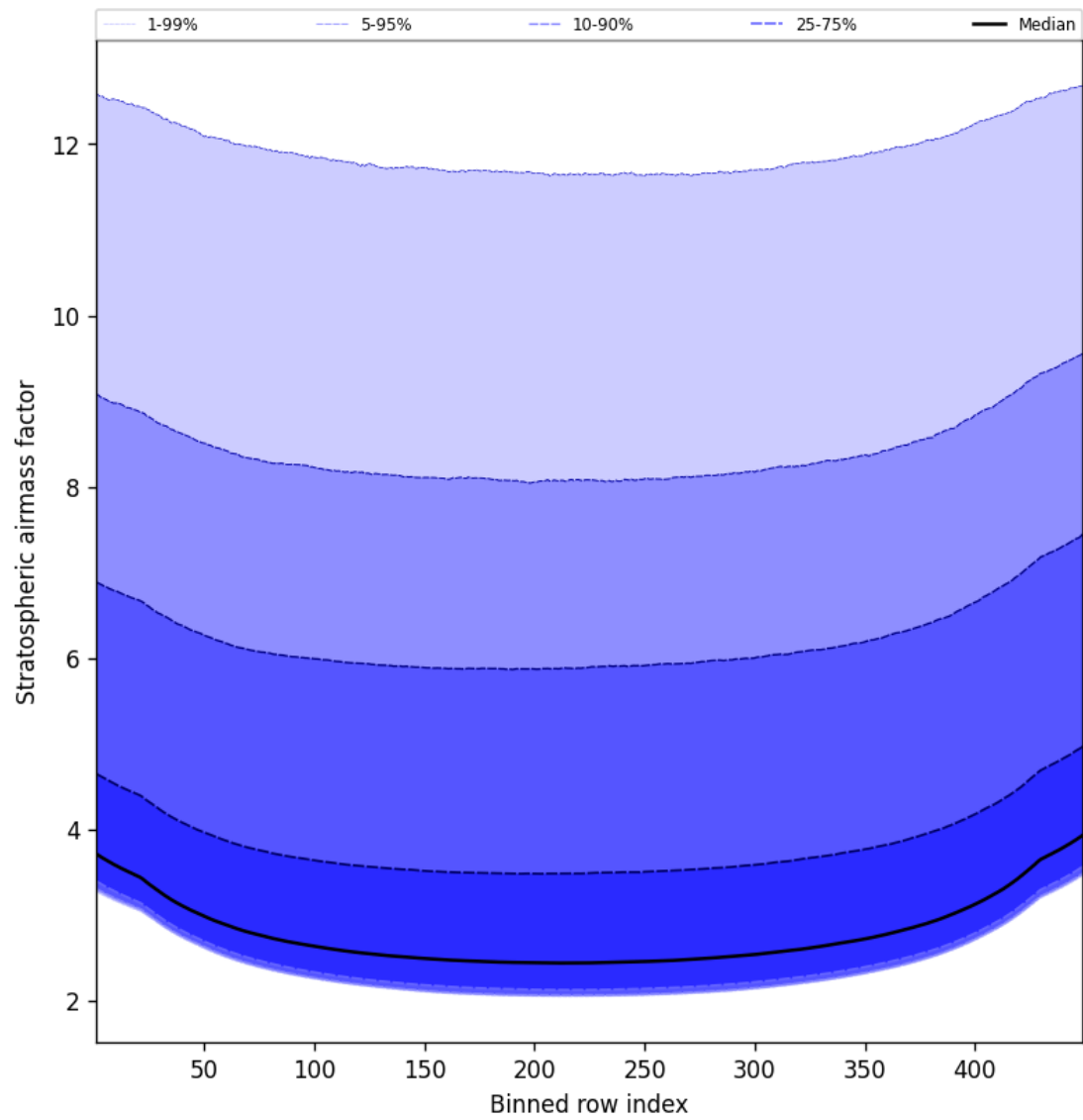
Figure 61: Along track statistics of “Stratospheric airmass factor” for 2025-01-12 to 2025-01-14
