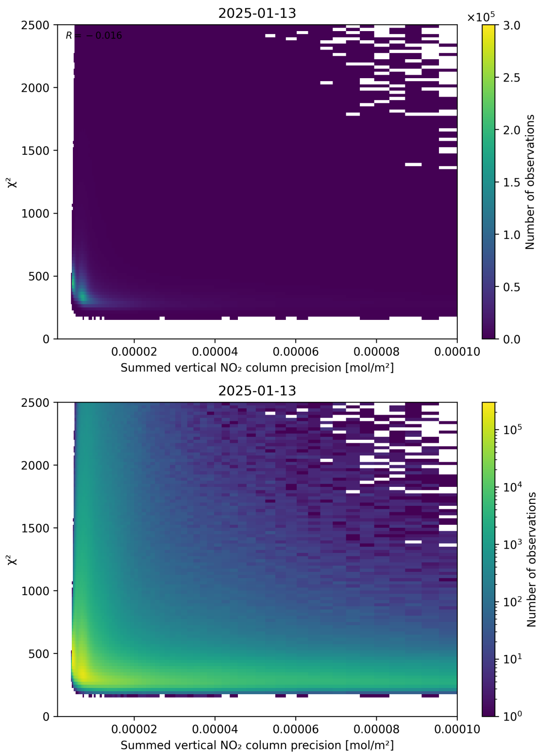
Figure 107: Scatter density plot of “Summed vertical NO 2 column precision” against “ \chi^2 ” for 2025-01-12 to 2025-01-14.
