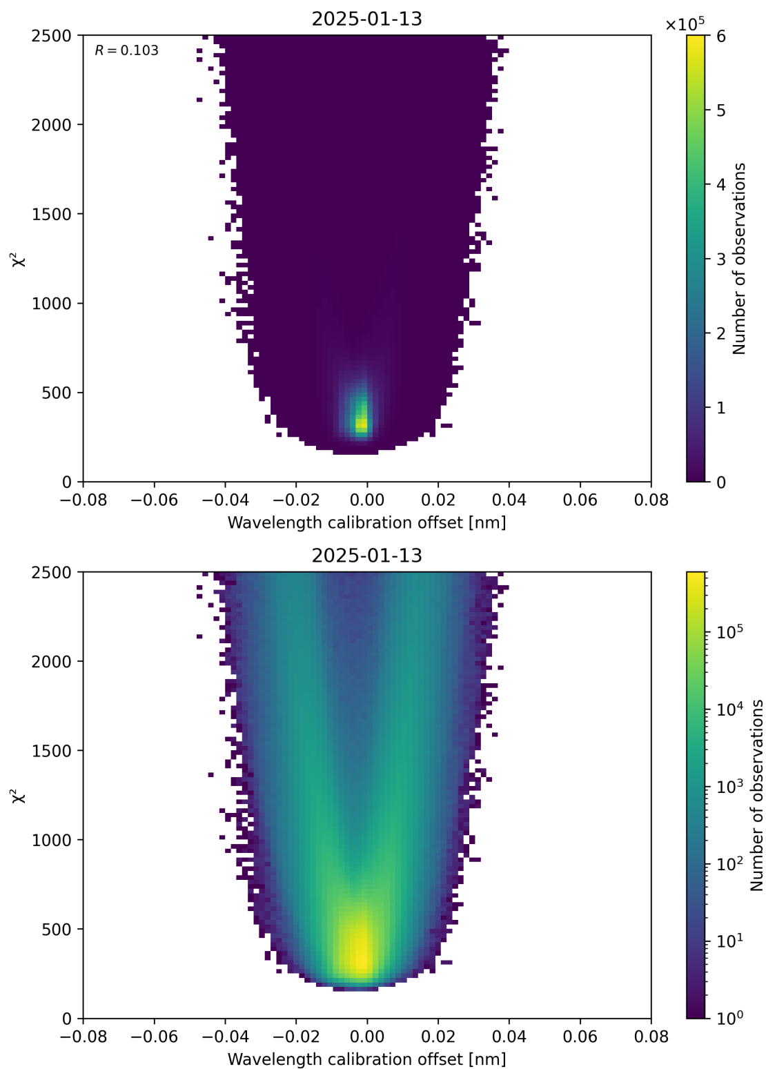
Figure 175: Scatter density plot of “Wavelength calibration offset” against “ \chi^2 ” for 2025-01-12 to 2025-01-14.
