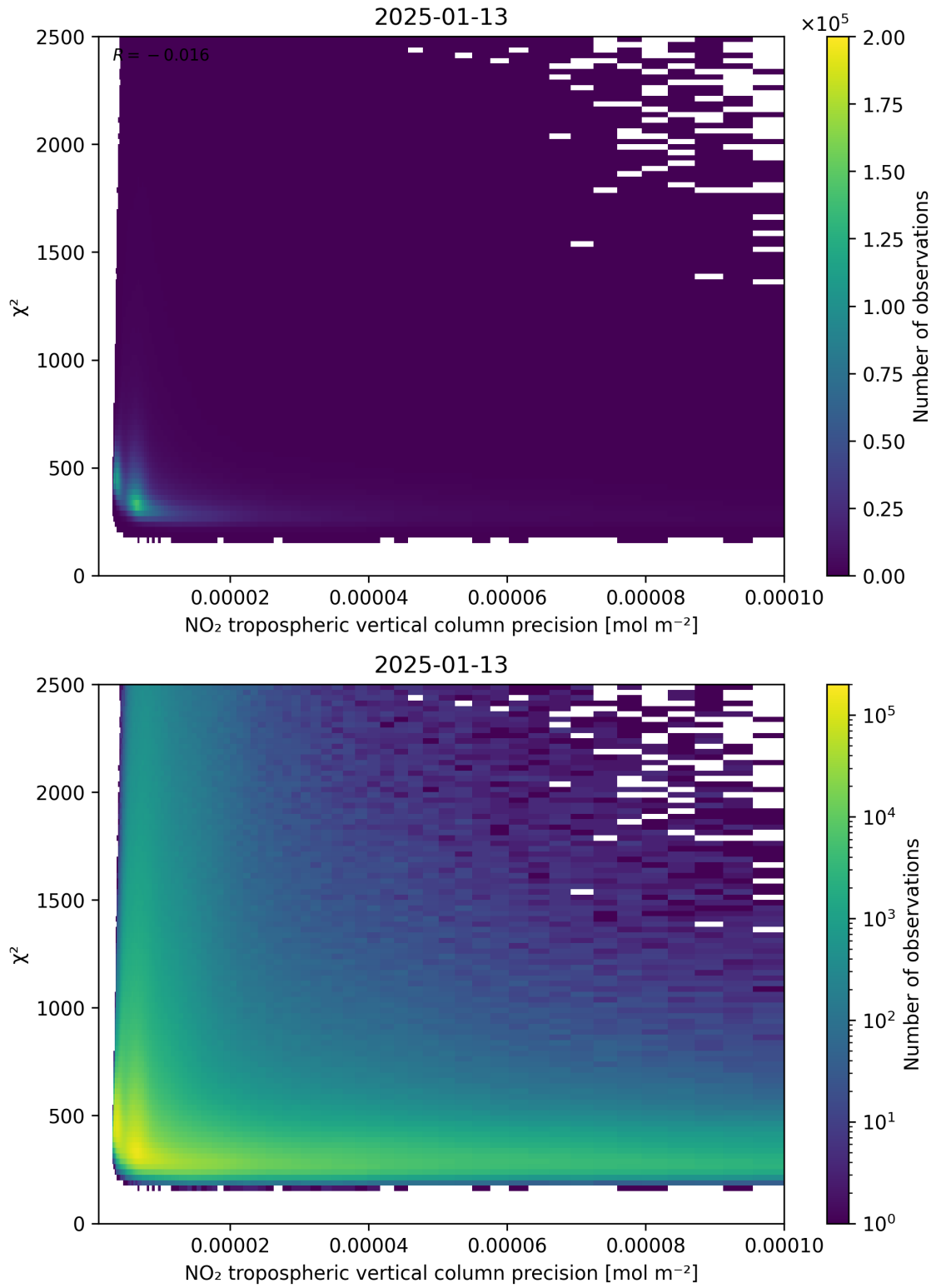
Figure 134: Scatter density plot of “NO 2 tropospheric vertical column precision” against “ \chi^2 ” for 2025-01-12 to 2025-01-14.
