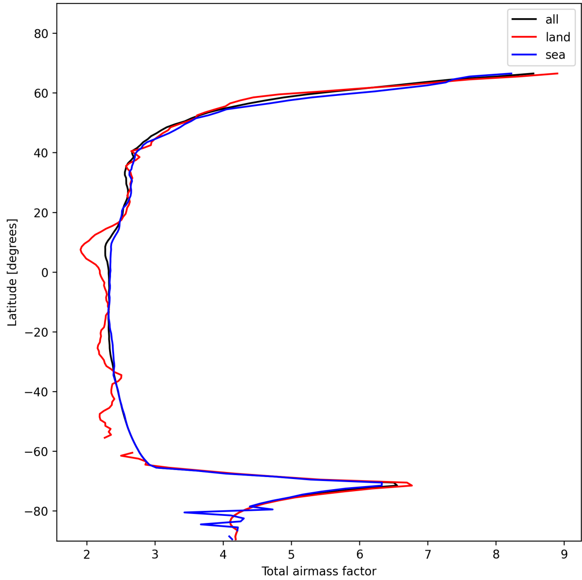
Figure 15: Zonal average of “Total airmass factor” for 2025-01-12 to 2025-01-14.
