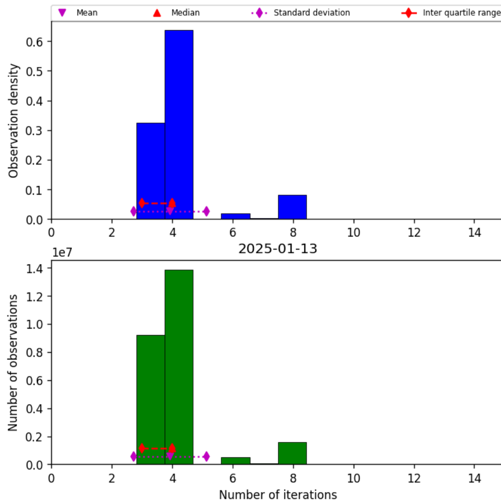
Figure 34: Histogram of “Number of iterations” for 2025-01-12 to 2025-01-14
