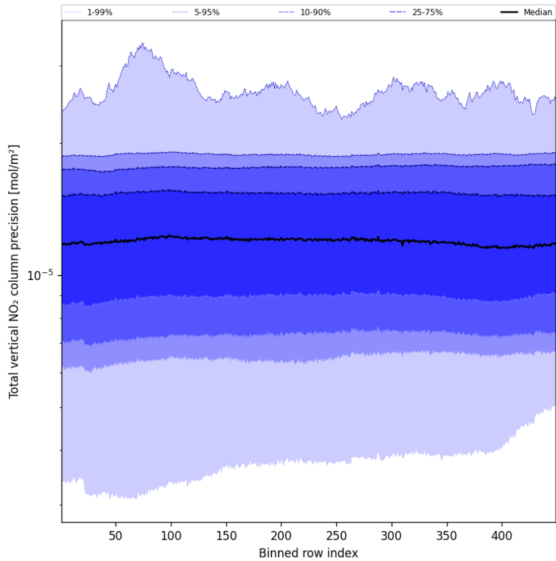
Figure 56: Along track statistics of “Total vertical NO 2 column precision” for 2025-01-12 to 2025-01-14
