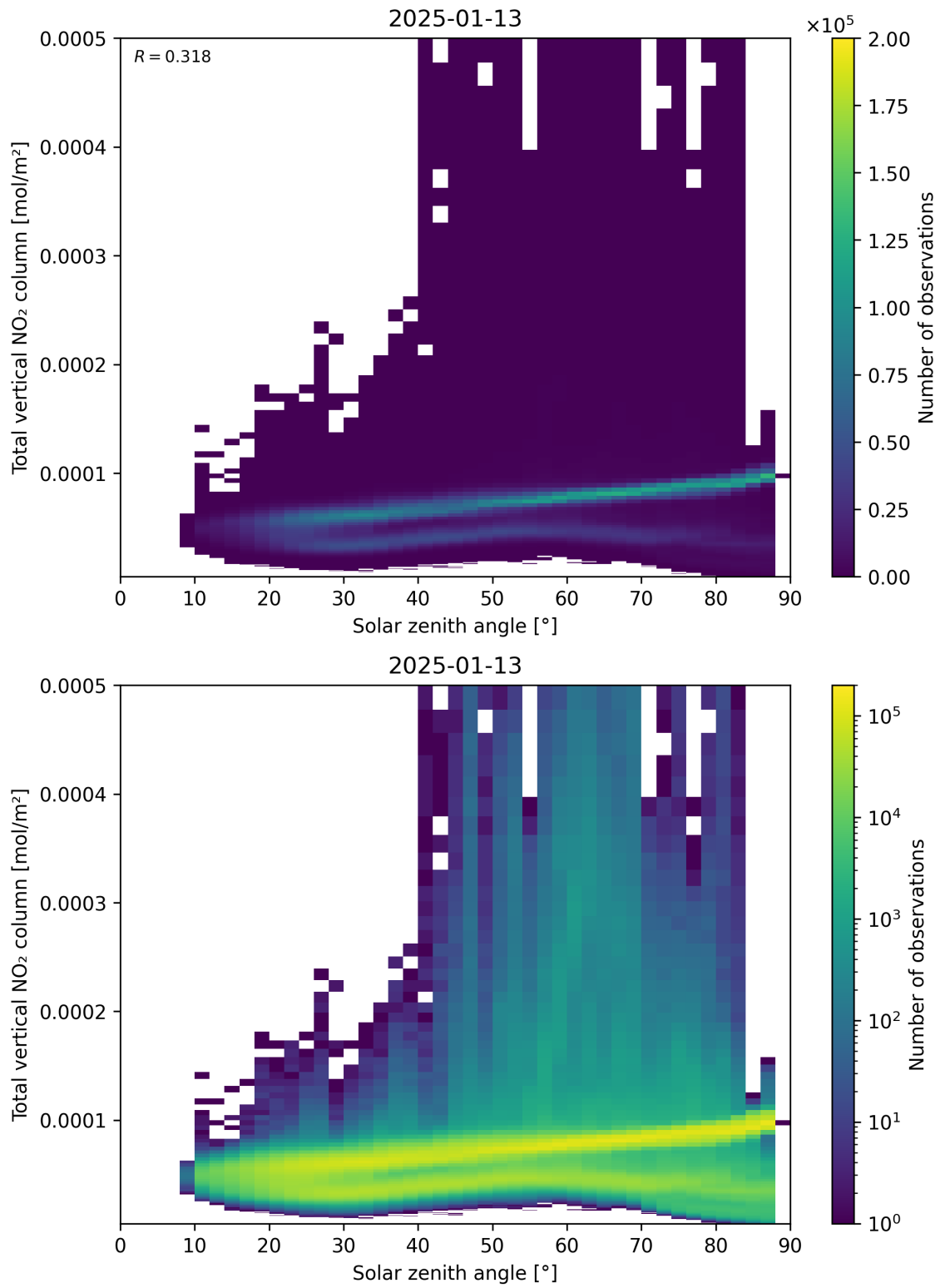
Figure 153: Scatter density plot of “Solar zenith angle” against “Total vertical NO 2 column” for 2025-01-12 to 2025-01-14.
