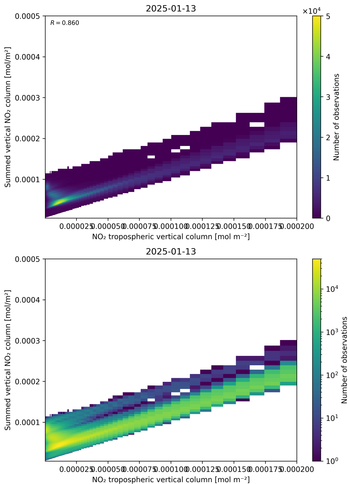
Figure 126: Scatter density plot of “NO 2 tropospheric vertical column” against “Summed vertical NO 2 column” for 2025-01-12 to 2025-01-14.
