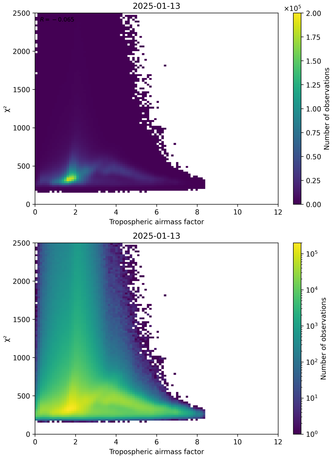
Figure 73: Scatter density plot of “Tropospheric airmass factor” against “ \chi^2 ” for 2025-01-12 to 2025-01-14.
