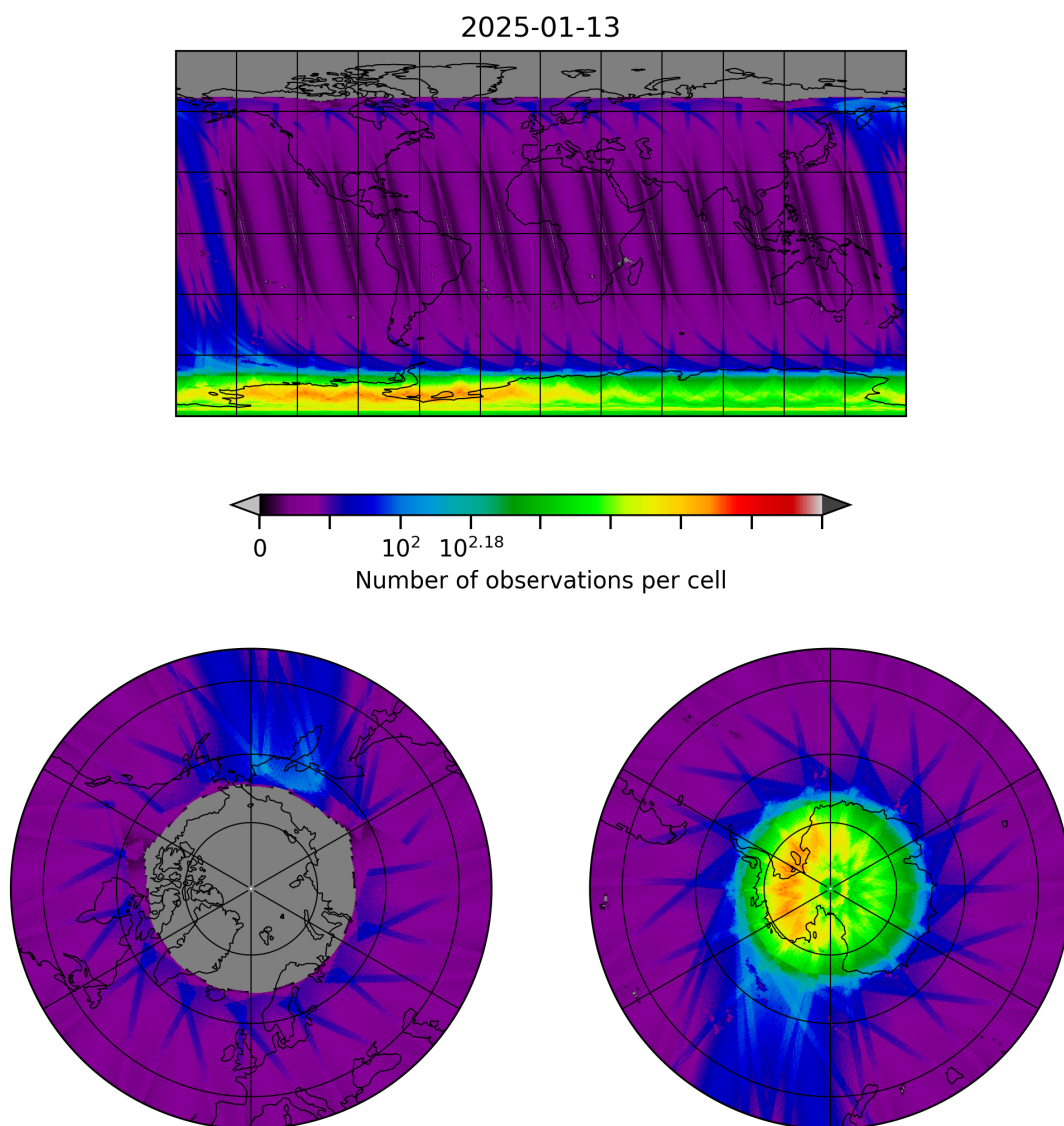
Figure 10: Map of the number of observations for 2025-01-12 to 2025-01-14
