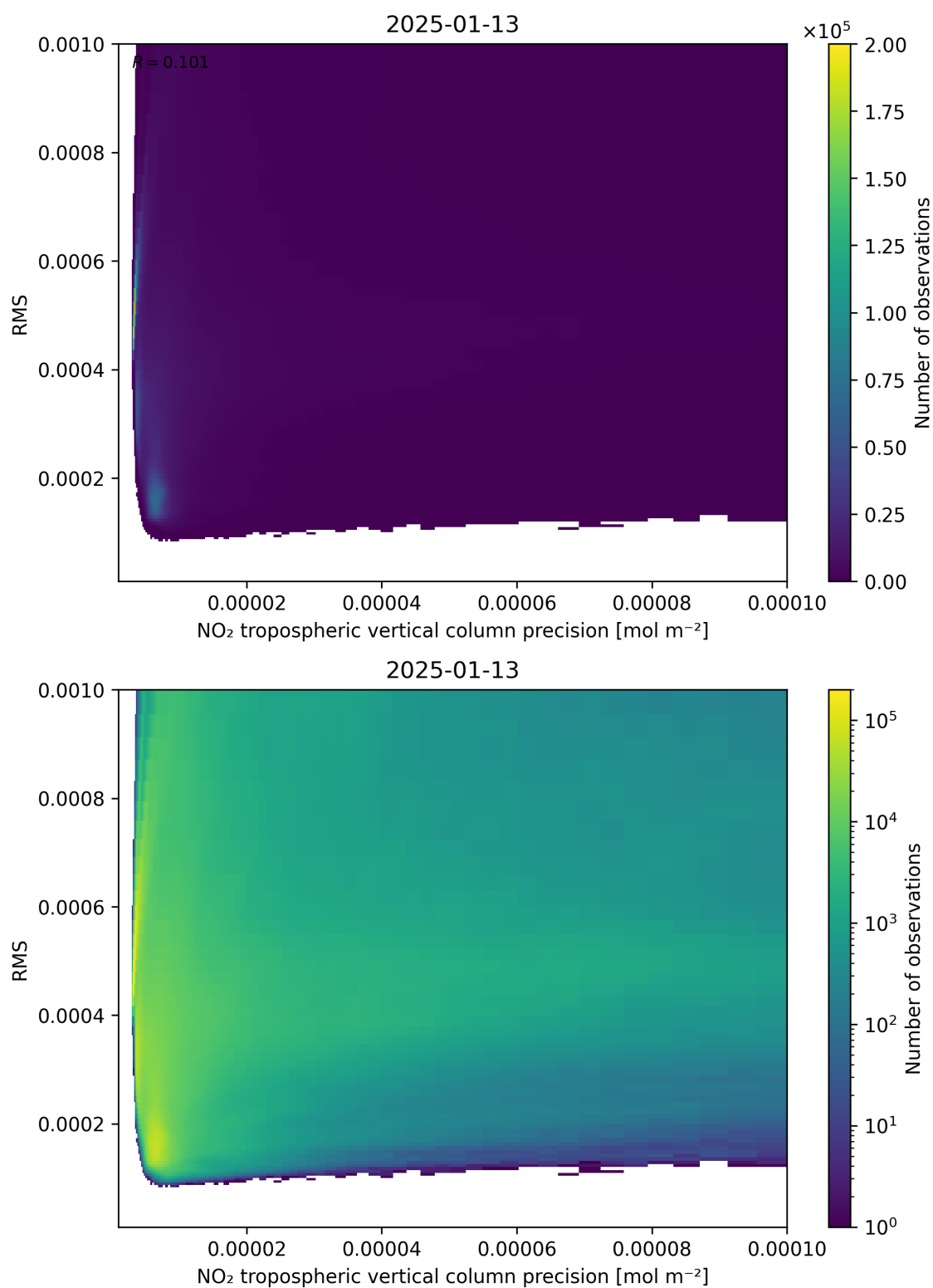
Figure 140: Scatter density plot of “NO 2 tropospheric vertical column precision” against “RMS” for 2025-01-12 to 2025-01-14.
