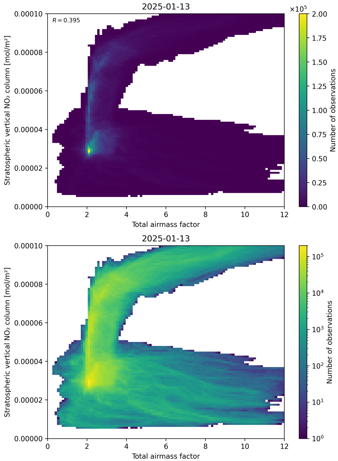
Figure 64: Scatter density plot of “Total airmass factor” against “Stratospheric vertical \text{NO}_2 column” for 2025-01-12 to 2025-01-14.
