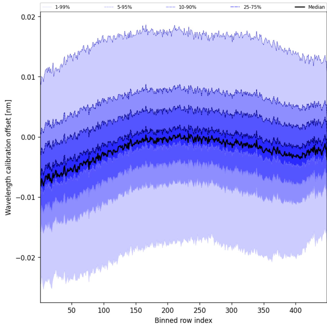
Figure 52: Along track statistics of “Wavelength calibration offset” for 2025-01-12 to 2025-01-14
