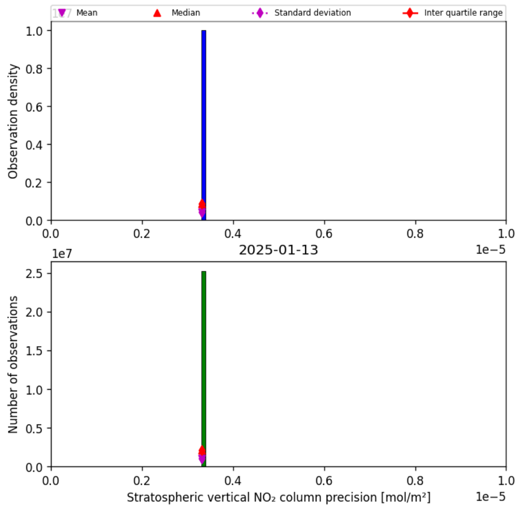
Figure 37: Histogram of “Stratospheric vertical NO 2 column precision” for 2025-01-12 to 2025-01-14
