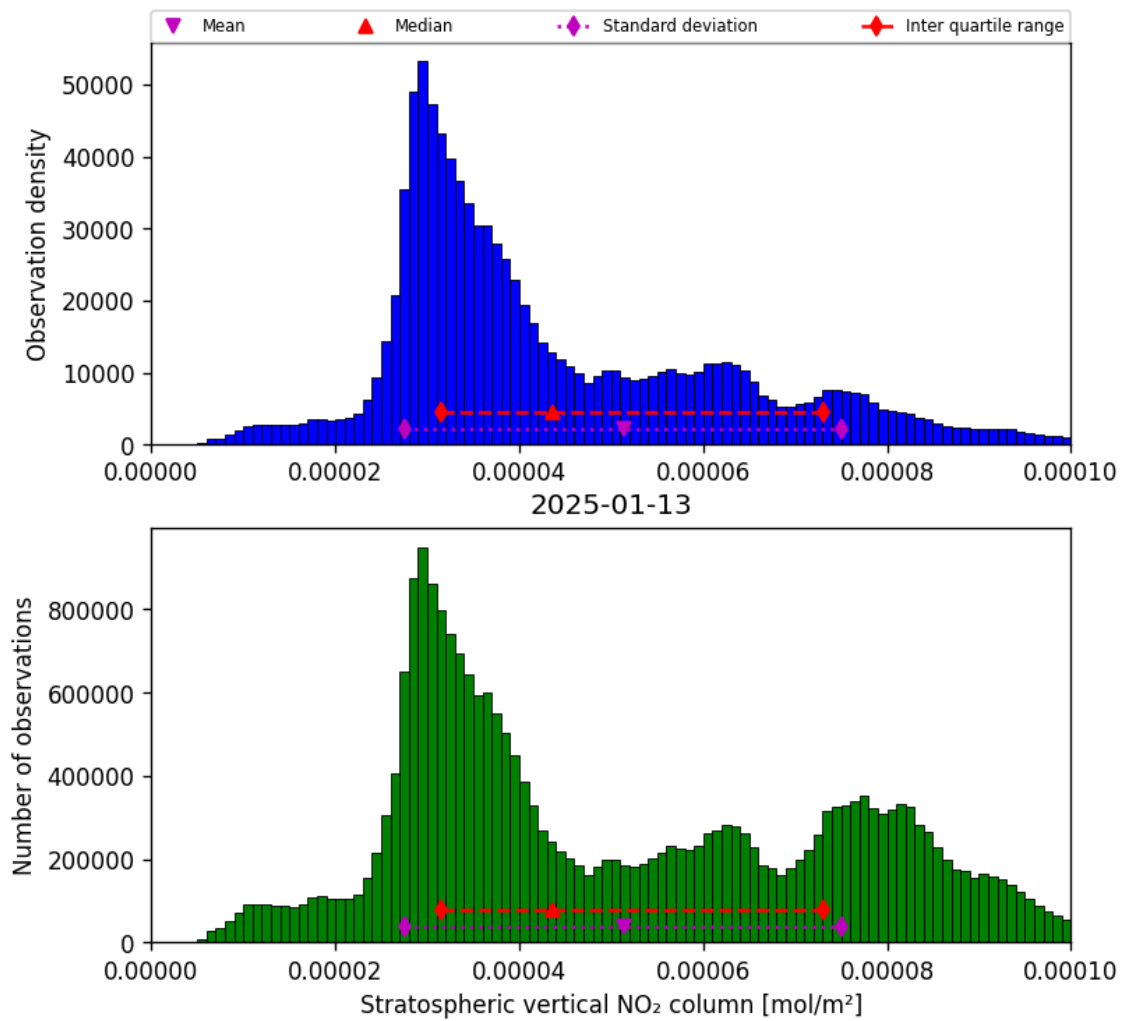
Figure 36: Histogram of “Stratospheric vertical NO 2 column” for 2025-01-12 to 2025-01-14
