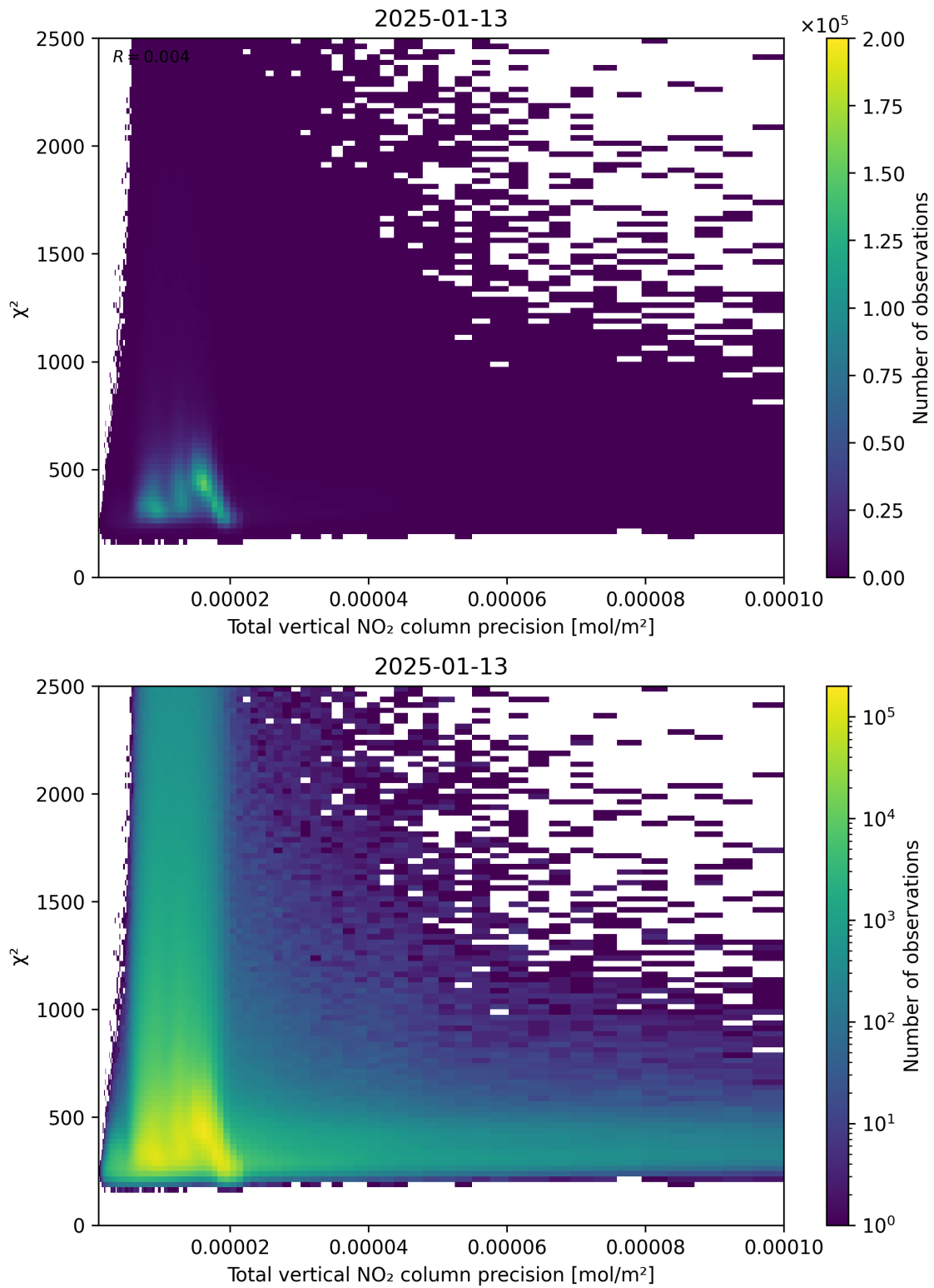
Figure 116: Scatter density plot of “Total vertical NO 2 column precision” against “ \chi^2 ” for 2025-01-12 to 2025-01-14.
