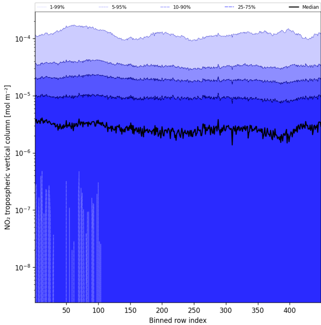
Figure 46: Along track statistics of “NO 2 tropospheric vertical column” for 2025-01-12 to 2025-01-14
