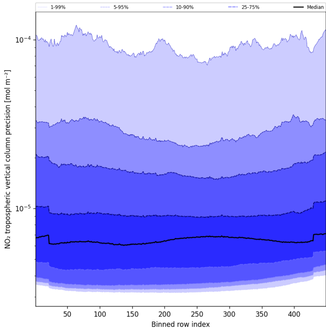
Figure 47: Along track statistics of “NO 2 tropospheric vertical column precision” for 2025-01-12 to 2025-01-14
