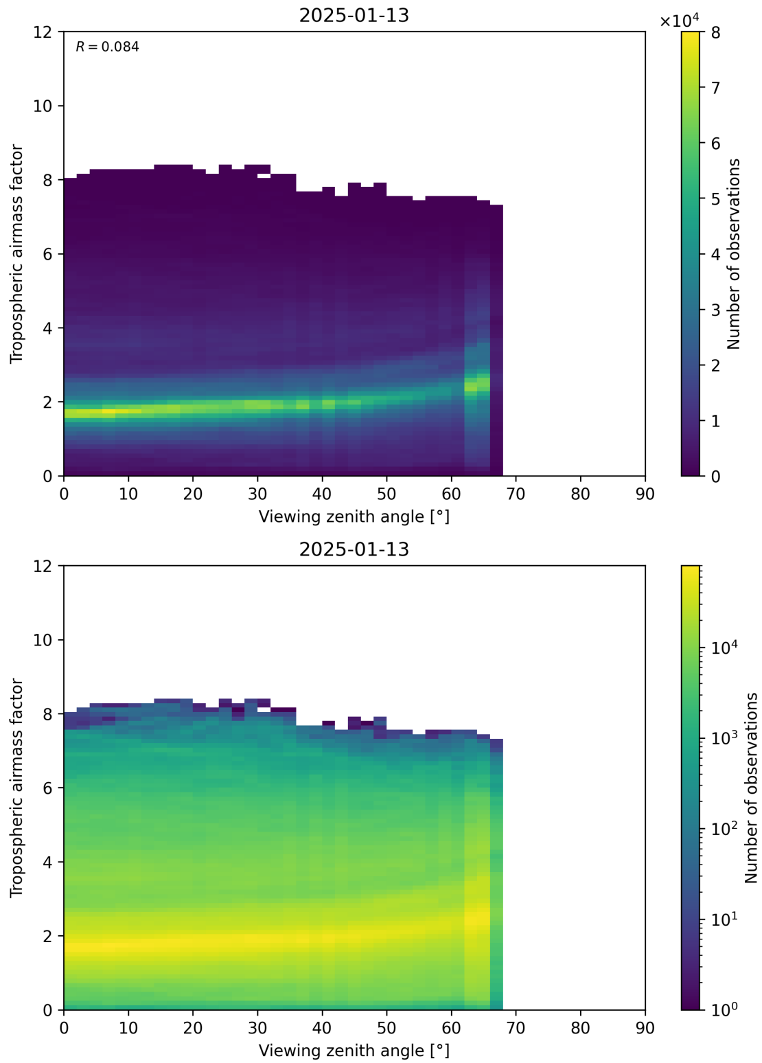
Figure 161: Scatter density plot of “Viewing zenith angle” against “Tropospheric airmass factor” for 2025-01-12 to 2025-01-14.
