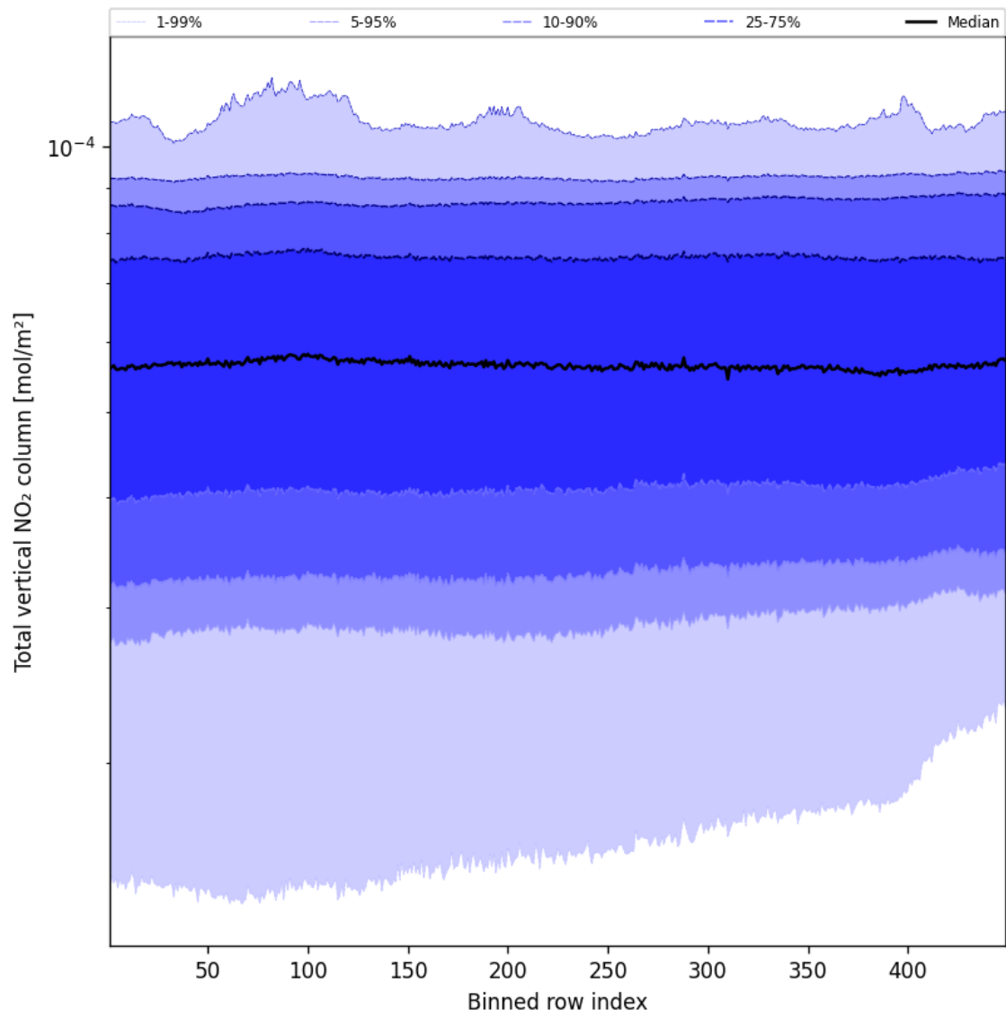
Figure 55: Along track statistics of “Total vertical NO 2 column” for 2025-01-12 to 2025-01-14
