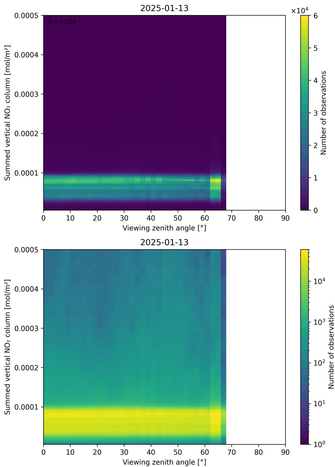
Figure 165: Scatter density plot of “Viewing zenith angle” against “Summed vertical NO 2 column” for 2025-01-12 to 2025-01-14.
