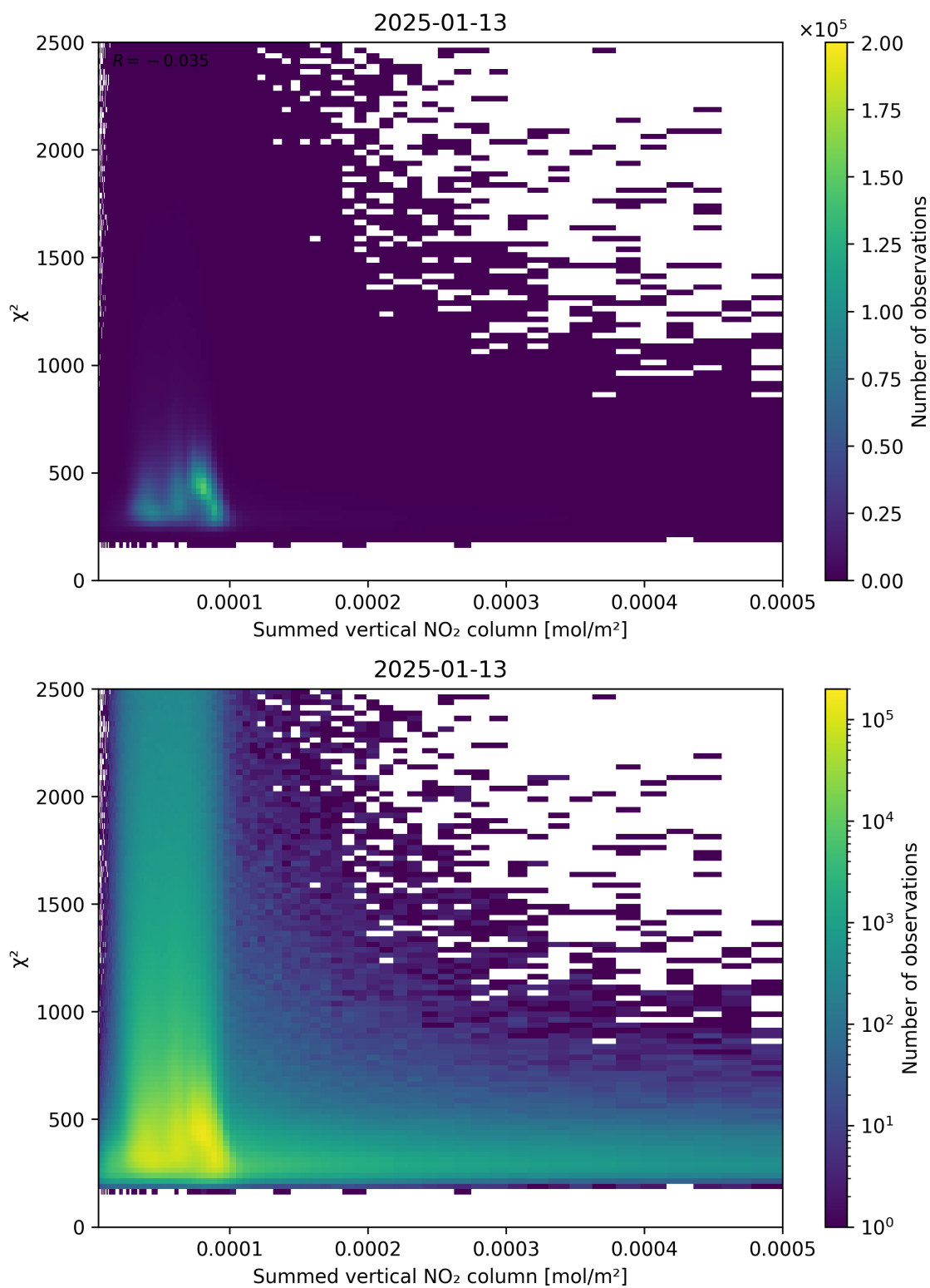
Figure 104: Scatter density plot of “Summed vertical NO 2 column” against “ \chi^2 ” for 2025-01-12 to 2025-01-14.
