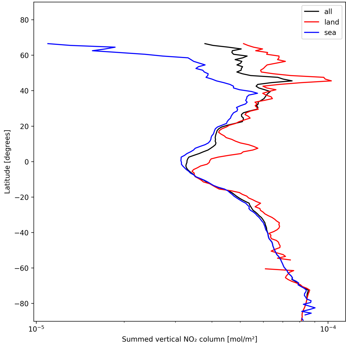
Figure 23: Zonal average of “Summed vertical NO 2 column” for 2025-01-12 to 2025-01-14.
