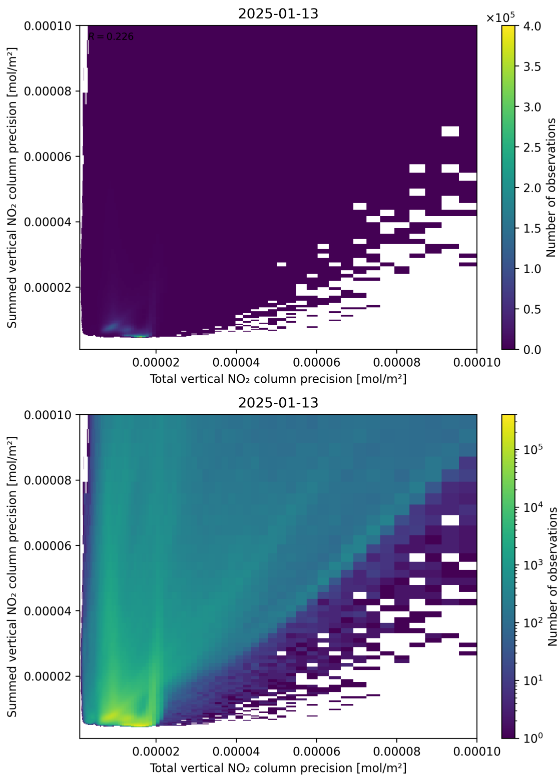
Figure 118: Scatter density plot of “Total vertical NO 2 column precision” against “Summed vertical NO 2 column precision” for 2025-01-12 to 2025-01-14.
