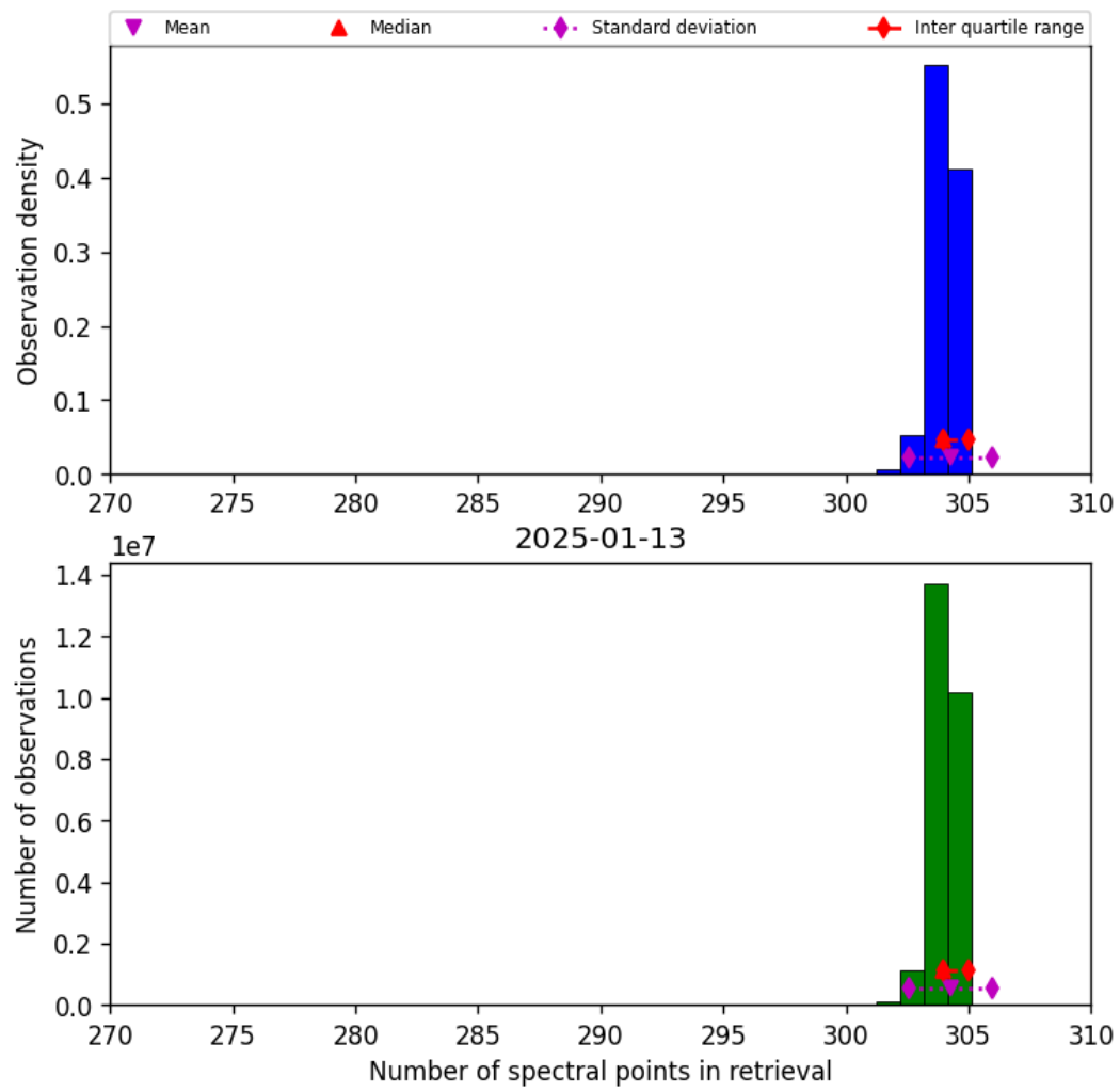
Figure 33: Histogram of “Number of spectral points in retrieval” for 2025-01-12 to 2025-01-14
