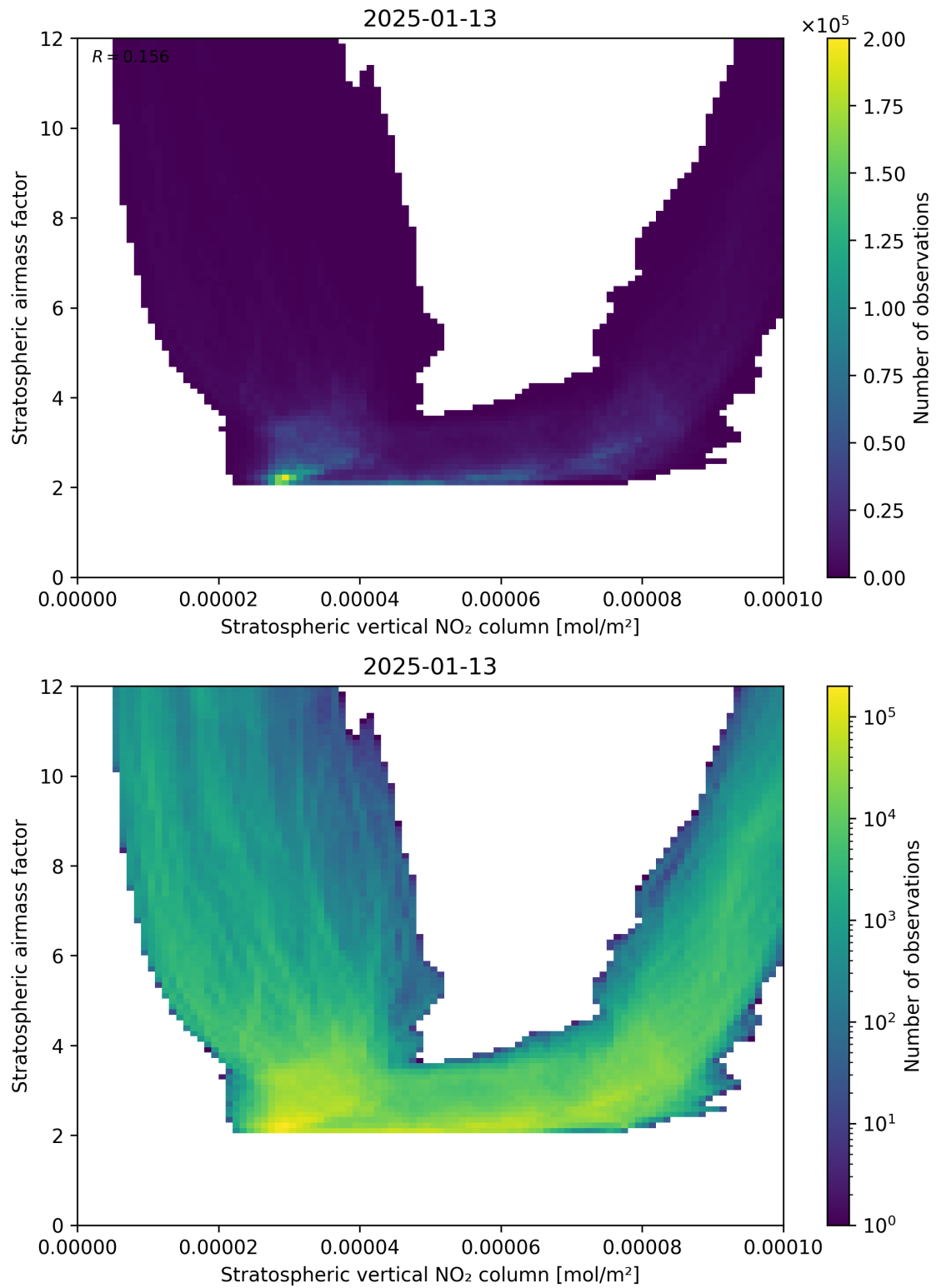
Figure 96: Scatter density plot of “Stratospheric vertical NO 2 column” against “Stratospheric airmass factor” for 2025-01-12 to 2025-01-14.
