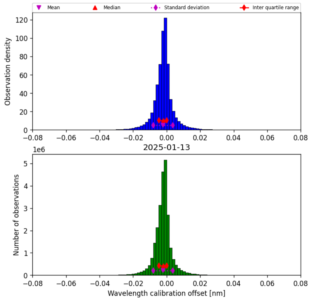
Figure 35: Histogram of “Wavelength calibration offset” for 2025-01-12 to 2025-01-14
