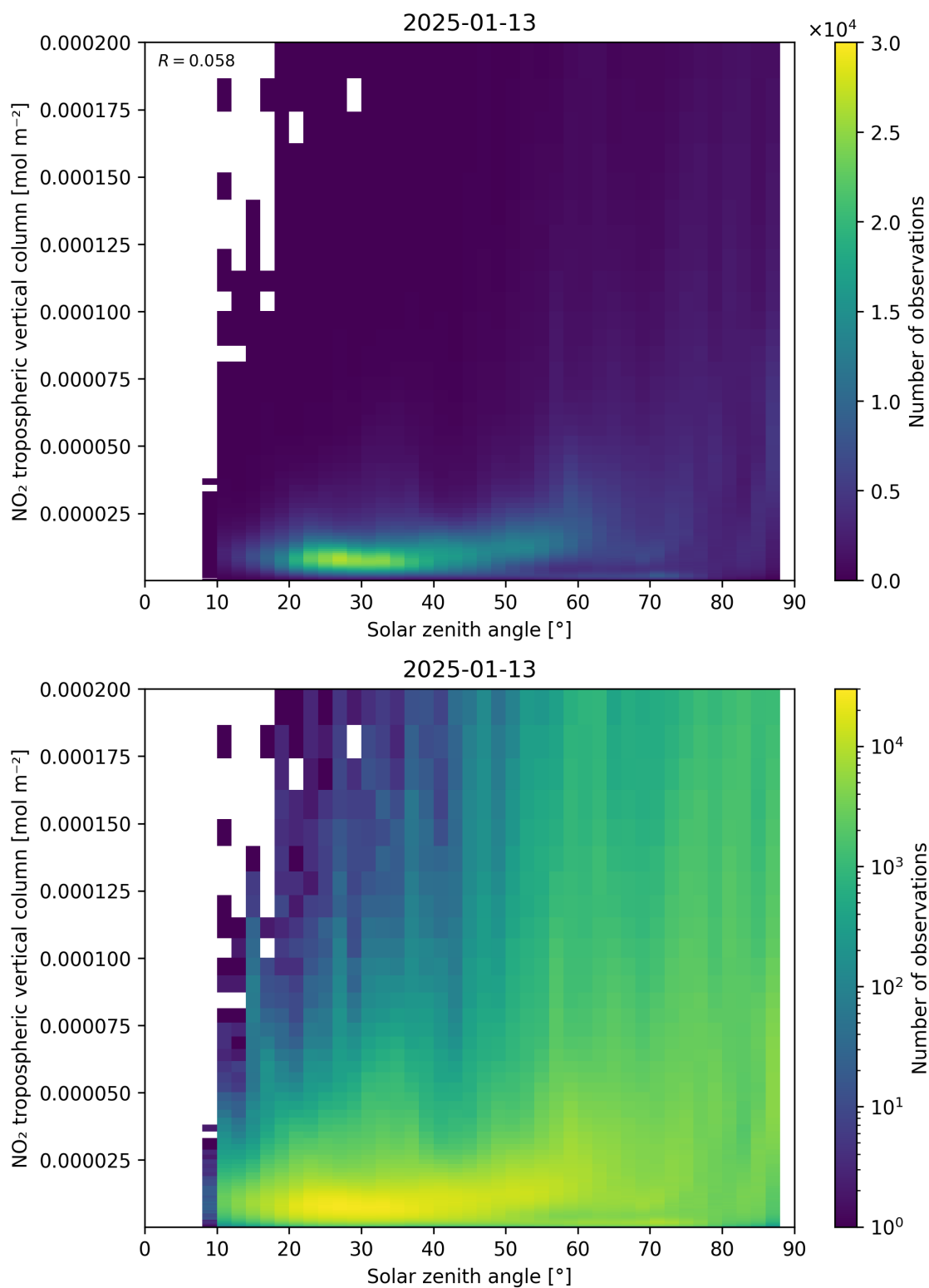
Figure 155: Scatter density plot of “Solar zenith angle” against “NO 2 tropospheric vertical column” for 2025-01-12 to 2025-01-14.
