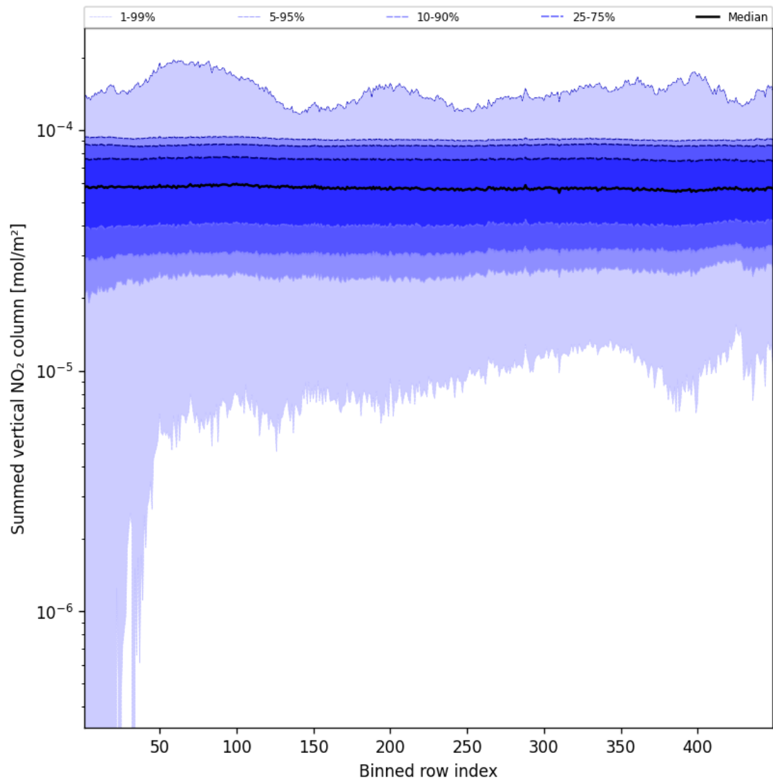
Figure 57: Along track statistics of “Summed vertical NO 2 column” for 2025-01-12 to 2025-01-14
