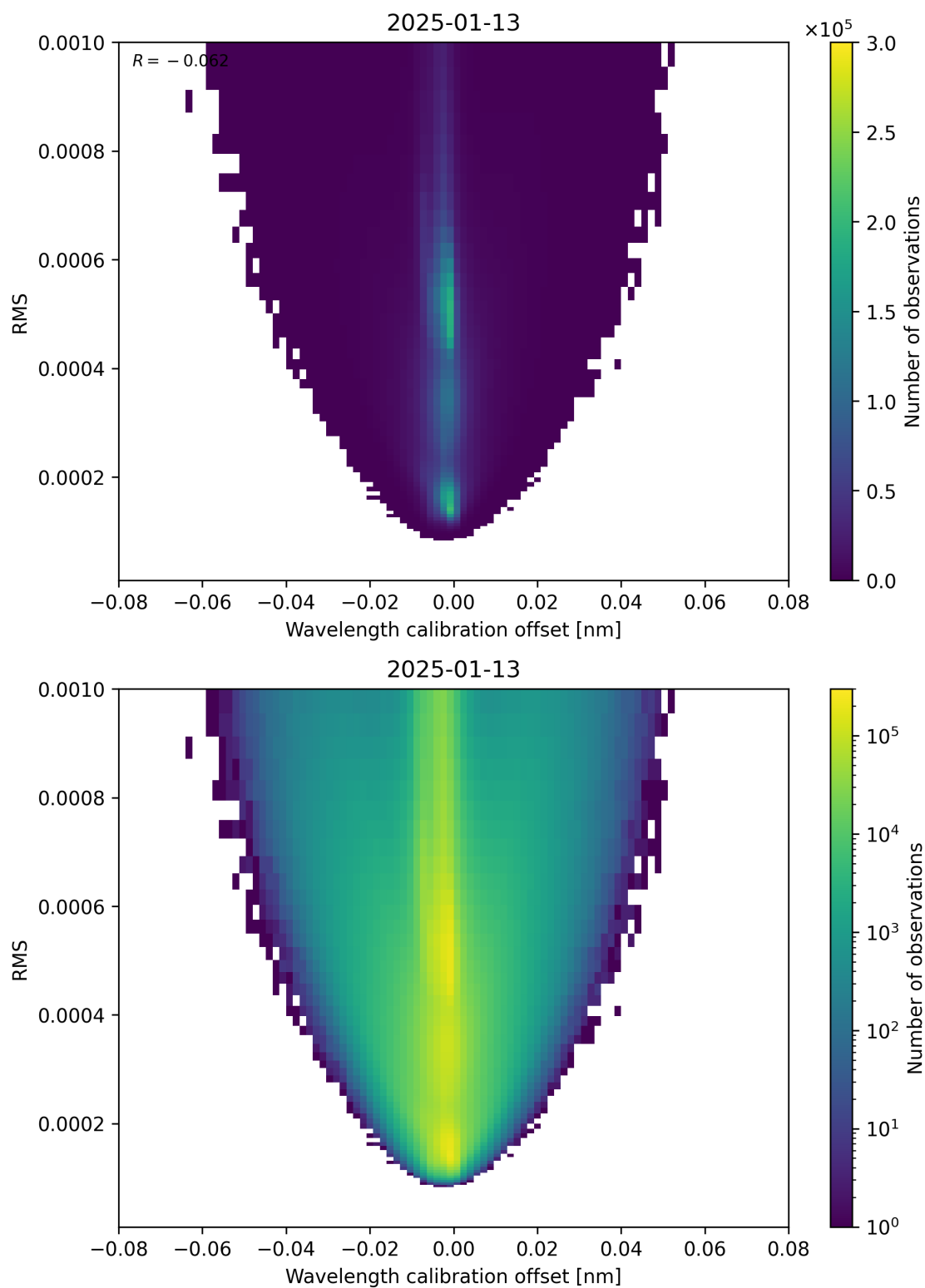
Figure 181: Scatter density plot of “Wavelength calibration offset” against “RMS” for 2025-01-12 to 2025-01-14.
