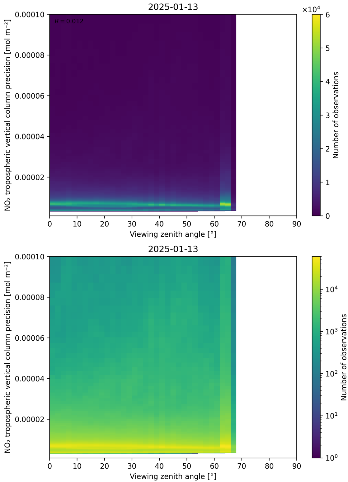
Figure 170: Scatter density plot of “Viewing zenith angle” against “NO 2 tropospheric vertical column precision” for 2025-01-12 to 2025-01-14.
