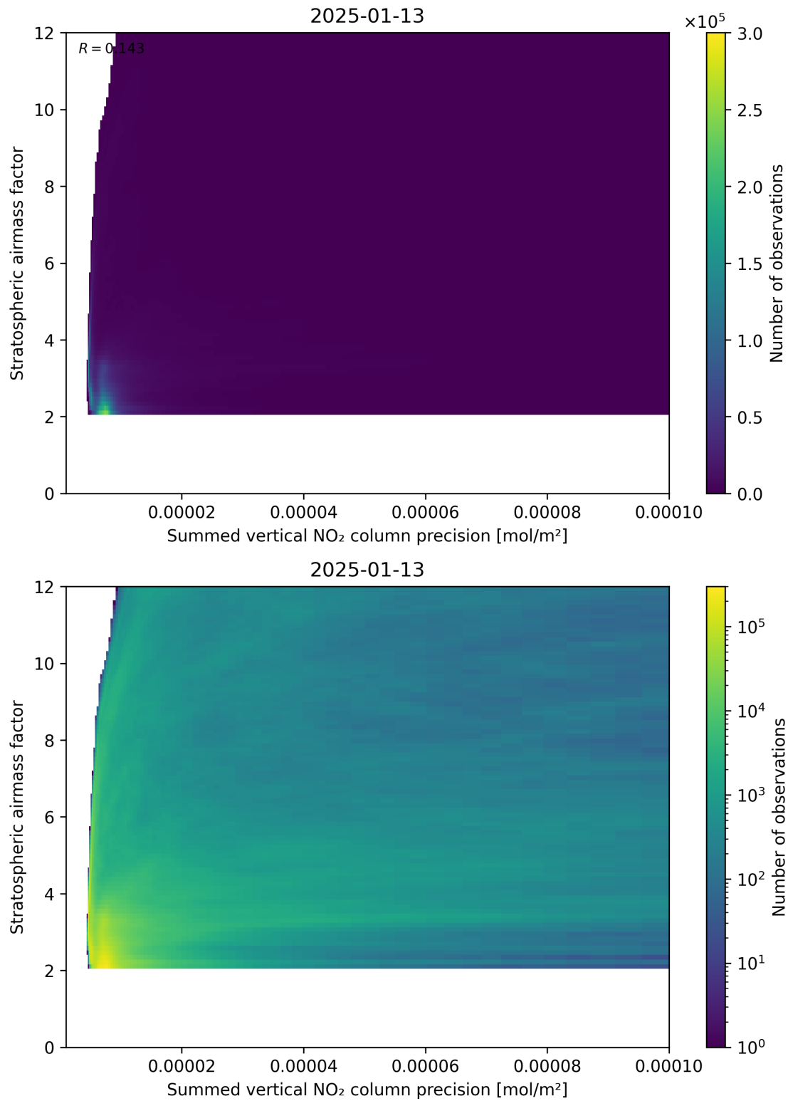
Figure 106: Scatter density plot of “Summed vertical NO 2 column precision” against “Stratospheric airmass factor” for 2025-01-12 to 2025-01-14.
