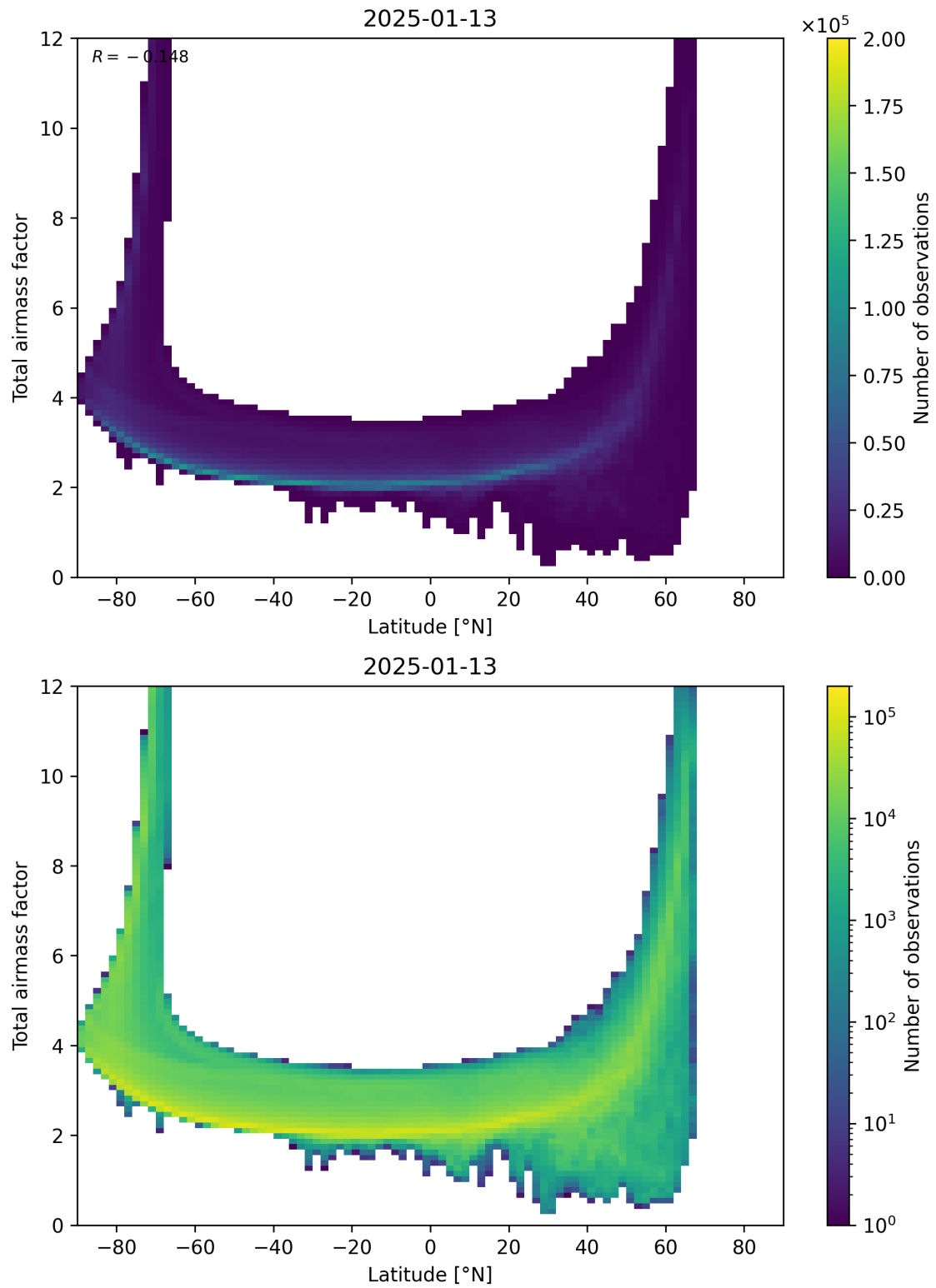
Figure 84: Scatter density plot of “Latitude” against “Total airmass factor” for 2025-01-12 to 2025-01-14.
