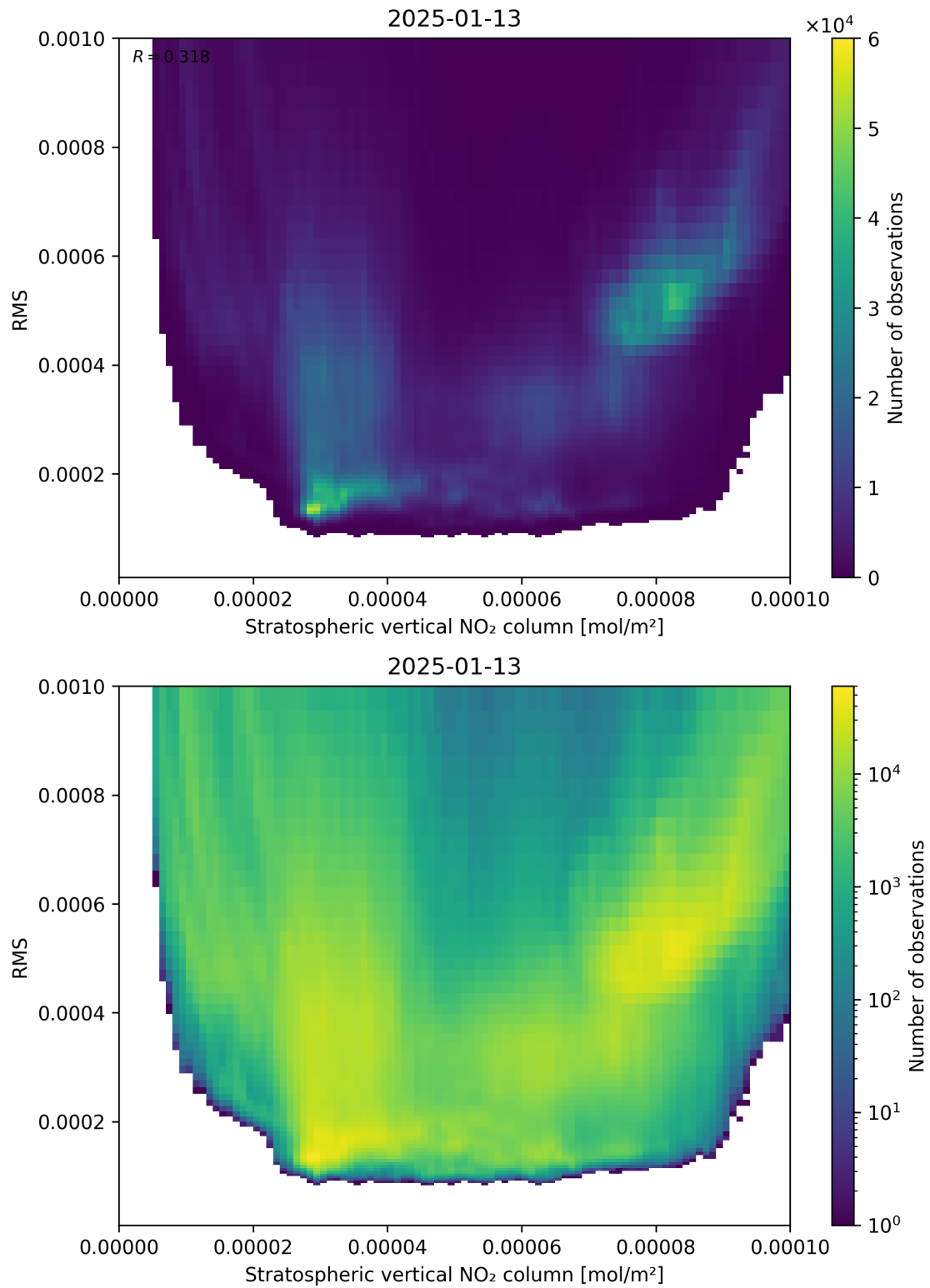
Figure 102: Scatter density plot of “Stratospheric vertical NO 2 column” against “RMS” for 2025-01-12 to 2025-01-14.
