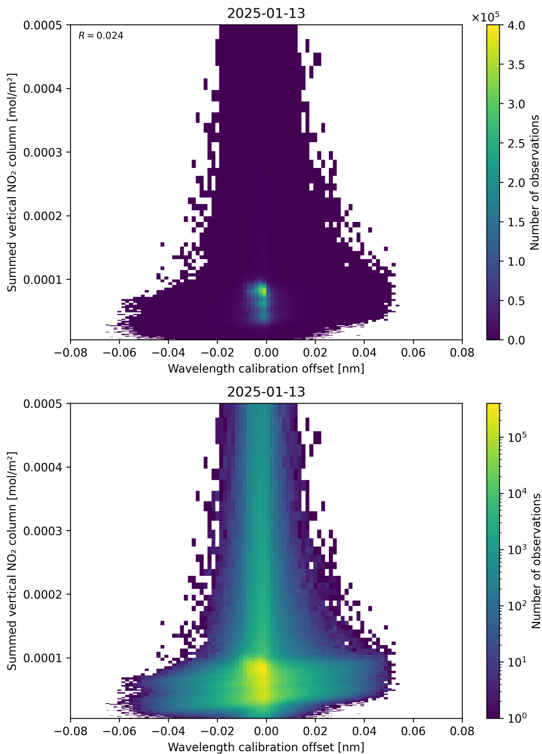
Figure 177: Scatter density plot of “Wavelength calibration offset” against “Summed vertical NO 2 column” for 2025-01-12 to 2025-01-14.
