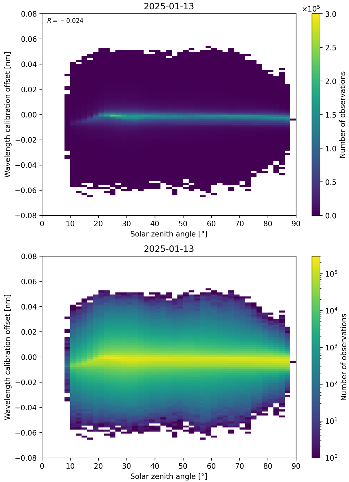
Figure 158: Scatter density plot of “Solar zenith angle” against “Wavelength calibration offset” for 2025-01-12 to 2025-01-14.
