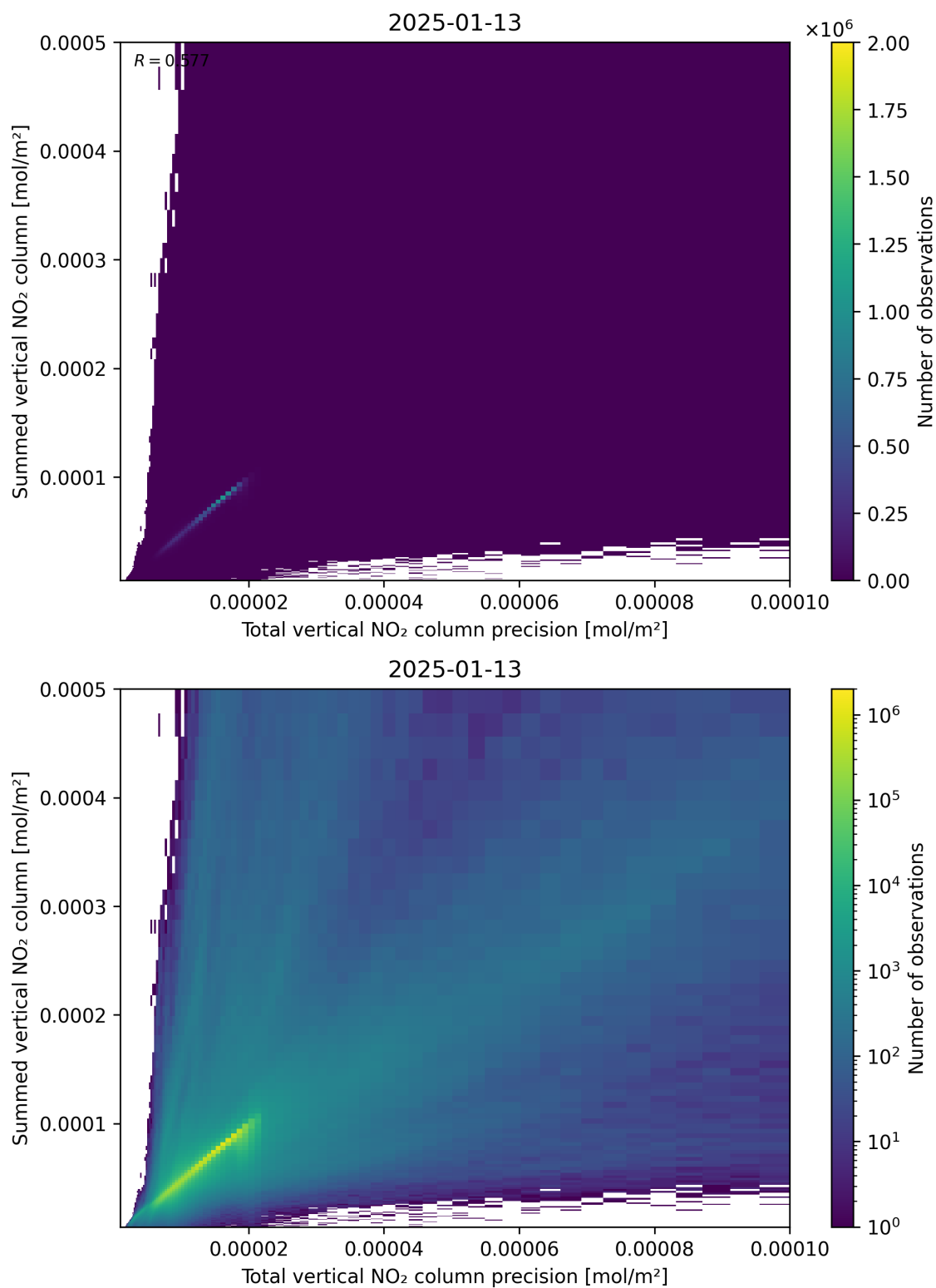
Figure 117: Scatter density plot of “Total vertical NO 2 column precision” against “Summed vertical NO 2 column” for 2025-01-12 to 2025-01-14.
