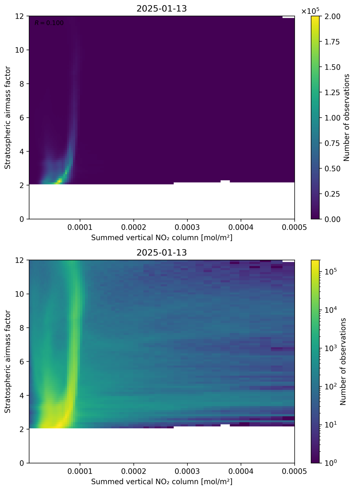
Figure 103: Scatter density plot of “Summed vertical NO 2 column” against “Stratospheric airmass factor” for 2025-01-12 to 2025-01-14.
