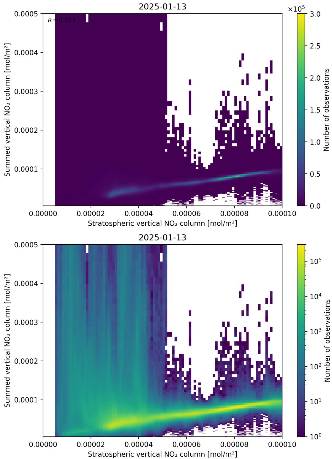
Figure 98: Scatter density plot of “Stratospheric vertical NO 2 column” against “Summed vertical NO 2 column” for 2025-01-12 to 2025-01-14.
