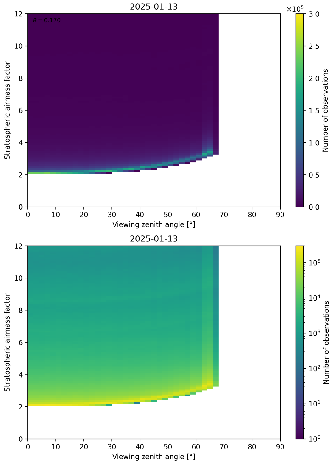
Figure 159: Scatter density plot of “Viewing zenith angle” against “Stratospheric airmass factor” for 2025-01-12 to 2025-01-14.
