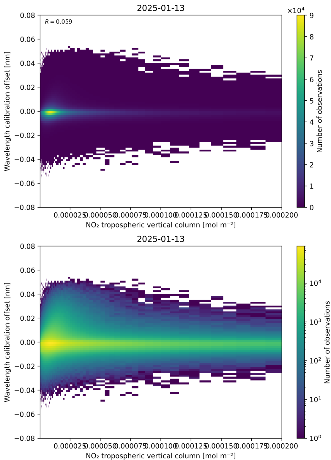
Figure 143: Scatter density plot of “NO 2 tropospheric vertical column” against “Wavelength calibration offset” for 2025-01-12 to 2025-01-14.
