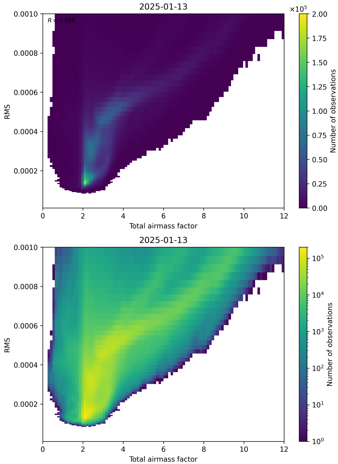
Figure 69: Scatter density plot of “Total airmass factor” against “RMS” for 2025-01-12 to 2025-01-14.
