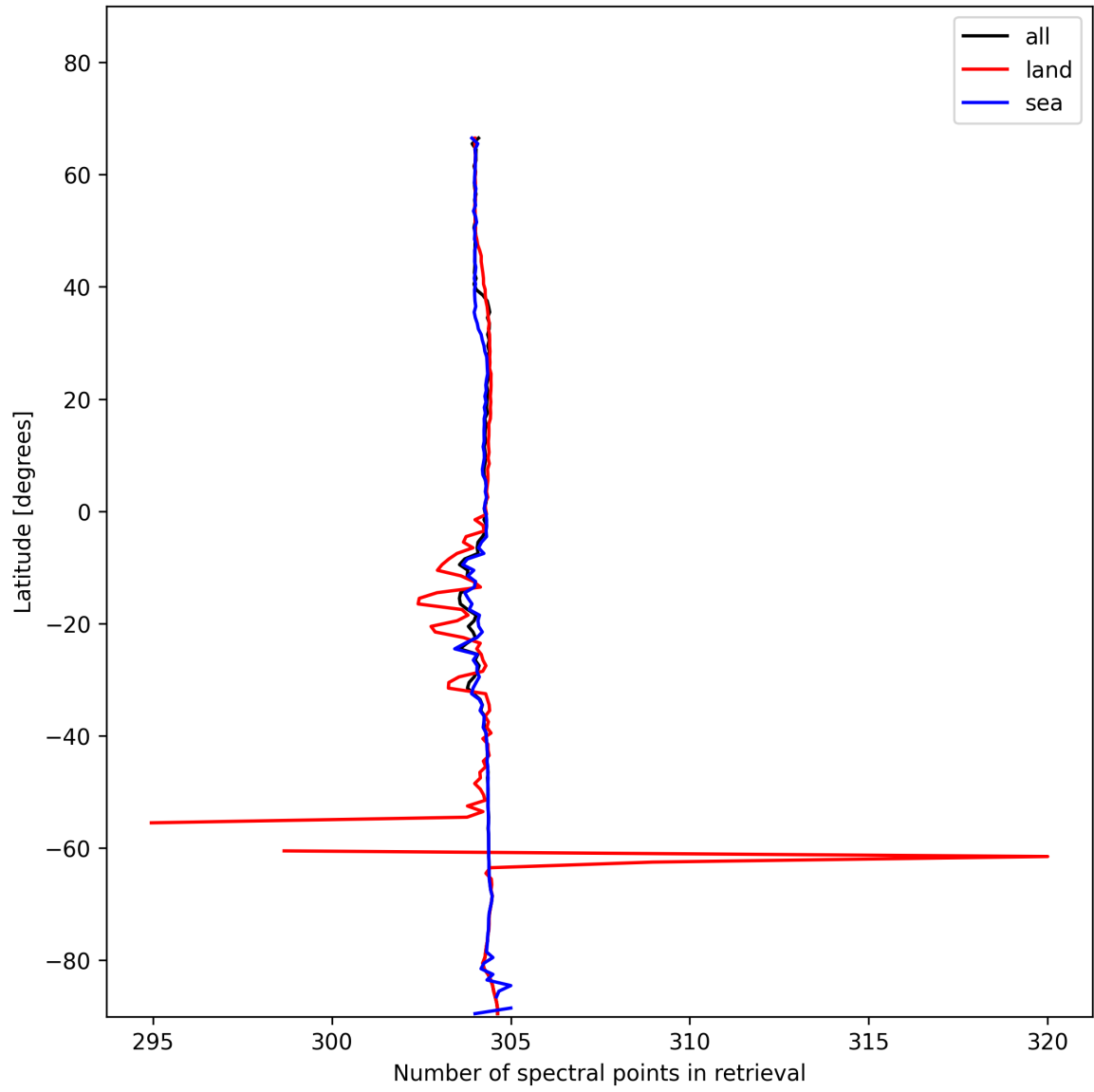
Figure 16: Zonal average of “Number of spectral points in retrieval” for 2025-01-12 to 2025-01-14.
