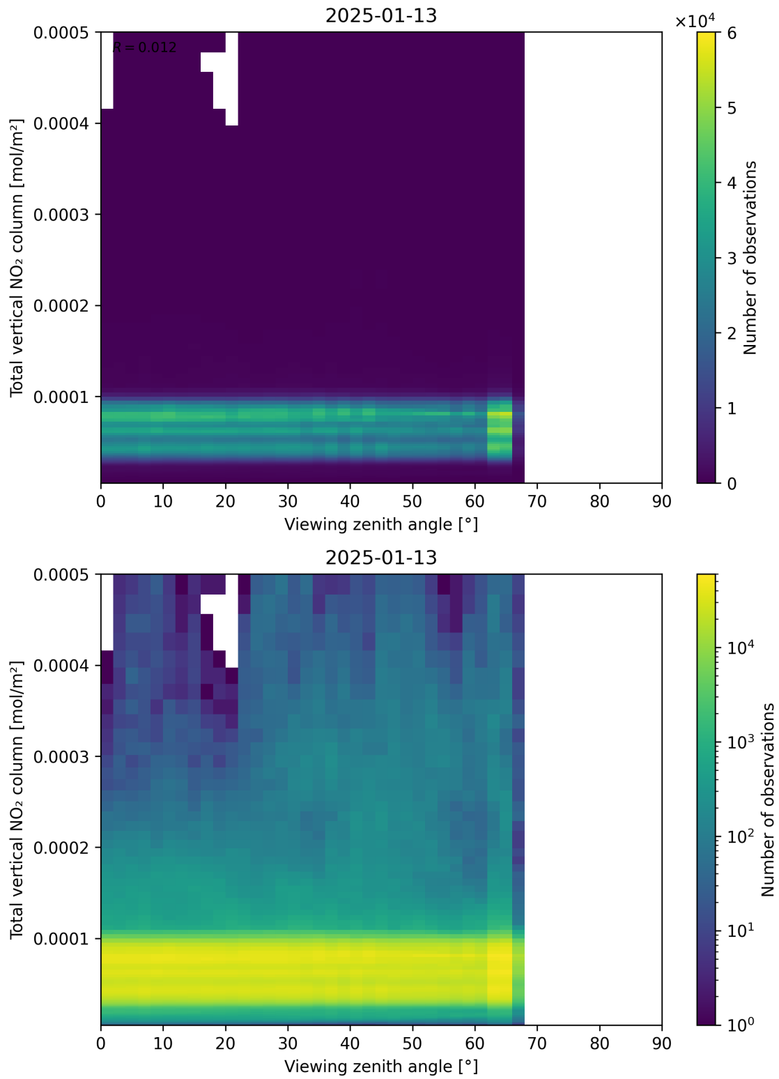
Figure 167: Scatter density plot of “Viewing zenith angle” against “Total vertical NO 2 column” for 2025-01-12 to 2025-01-14.
