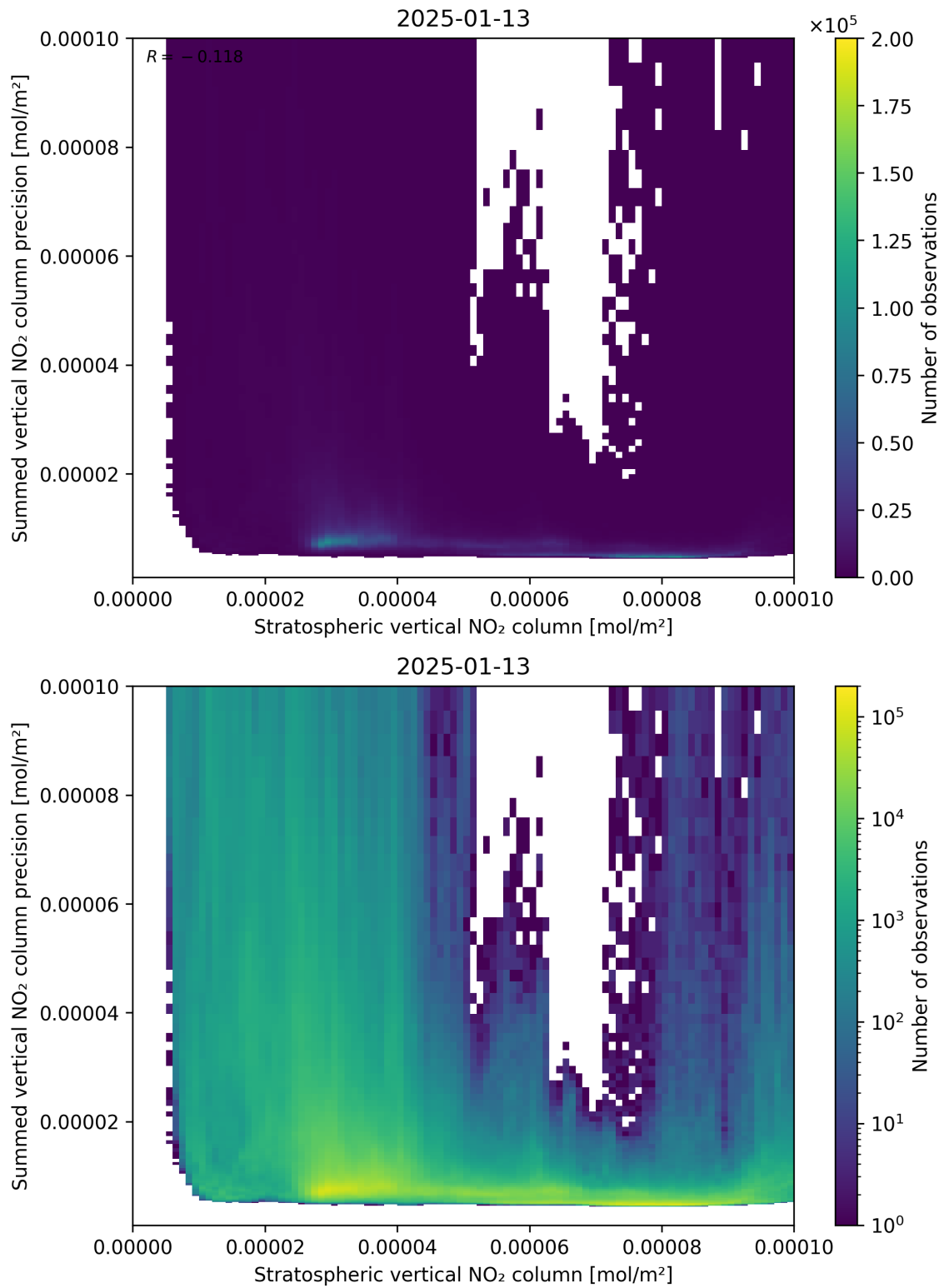
Figure 99: Scatter density plot of “Stratospheric vertical NO 2 column” against “Summed vertical NO 2 column precision” for 2025-01-12 to 2025-01-14.
