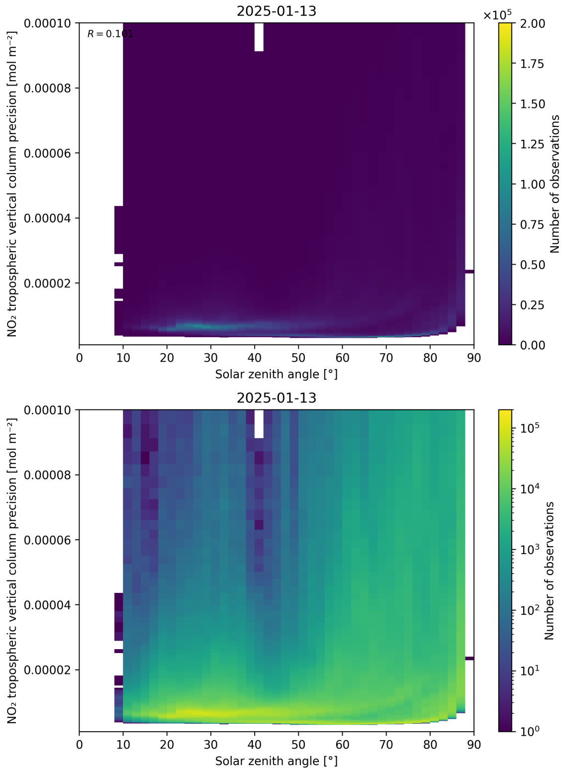
Figure 156: Scatter density plot of “Solar zenith angle” against “NO 2 tropospheric vertical column precision” for 2025-01-12 to 2025-01-14.
