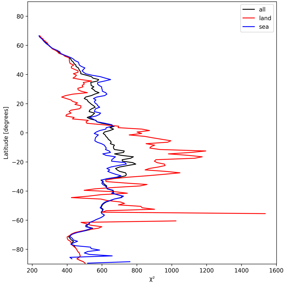
Figure 25: Zonal average of “ \chi^2 ” for 2025-01-12 to 2025-01-14.
