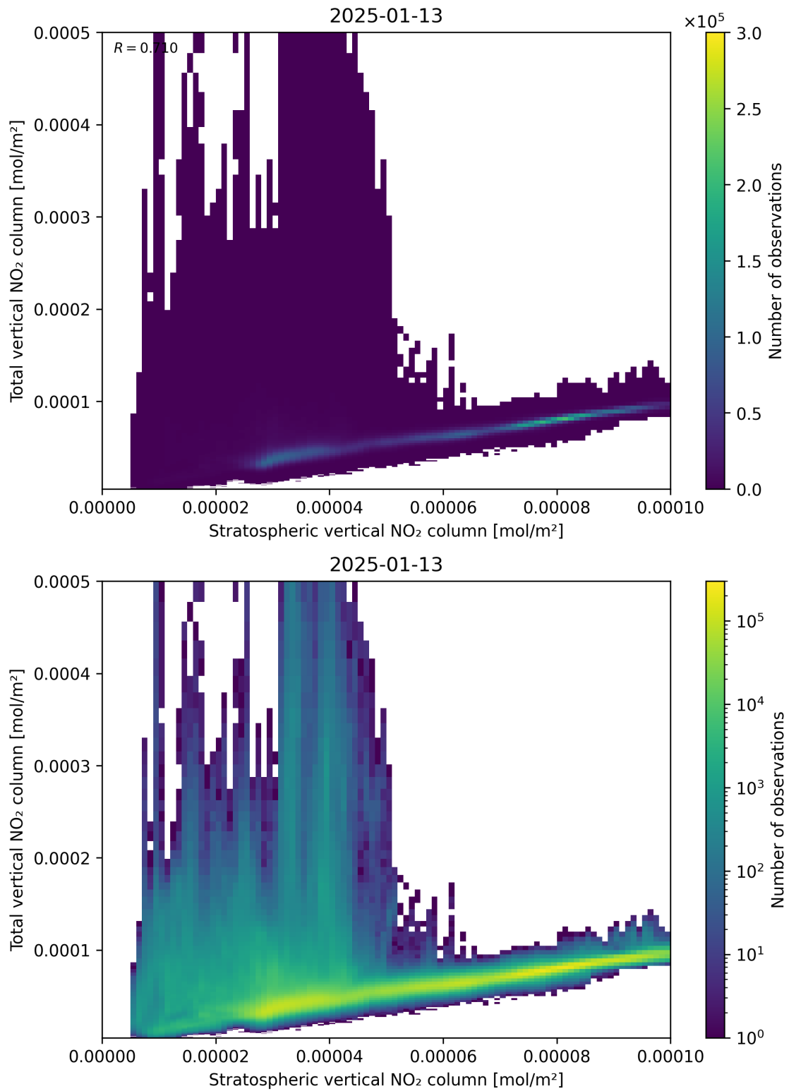
Figure 100: Scatter density plot of “Stratospheric vertical NO 2 column” against “Total vertical NO 2 column” for 2025-01-12 to 2025-01-14.
