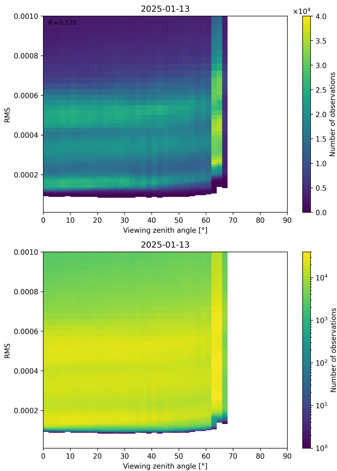
Figure 171: Scatter density plot of “Viewing zenith angle” against “RMS” for 2025-01-12 to 2025-01-14.
