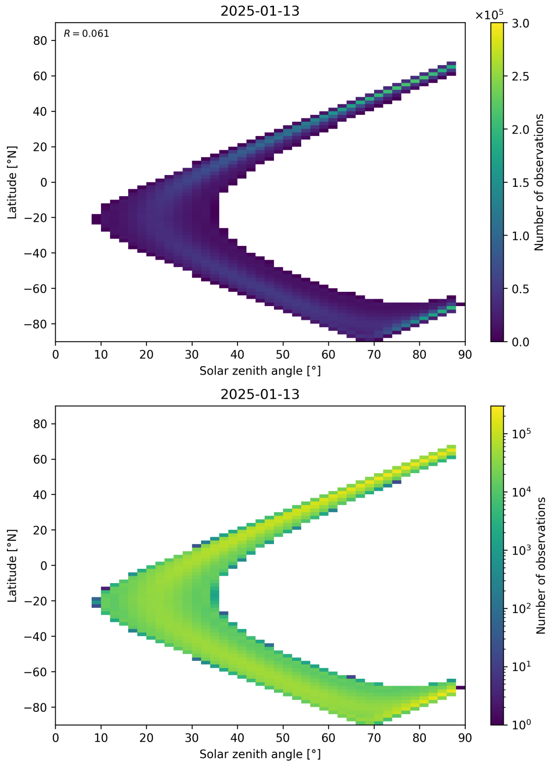
Figure 149: Scatter density plot of “Solar zenith angle” against “Latitude” for 2025-01-12 to 2025-01-14.
