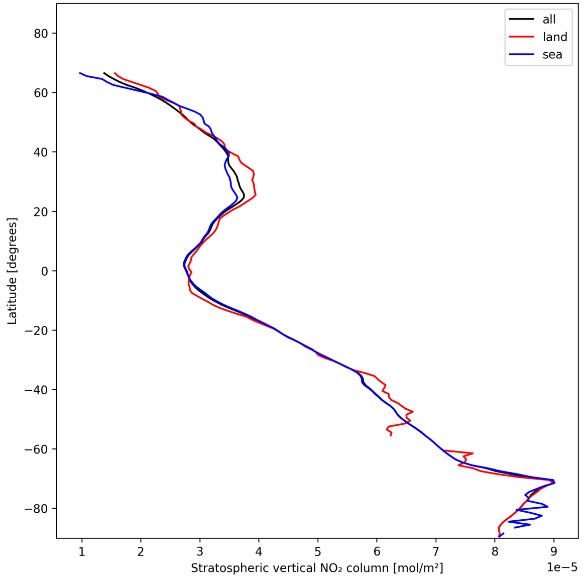
Figure 19: Zonal average of “Stratospheric vertical NO 2 column” for 2025-01-12 to 2025-01-14.
