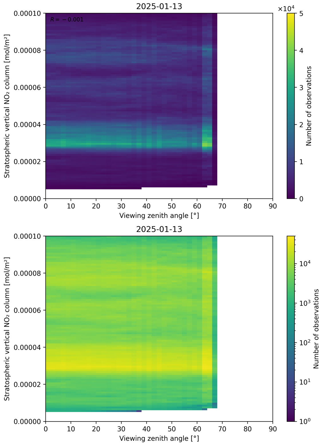
Figure 164: Scatter density plot of “Viewing zenith angle” against “Stratospheric vertical NO 2 column” for 2025-01-12 to 2025-01-14.
