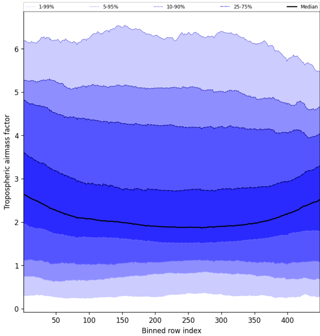
Figure 48: Along track statistics of “Tropospheric air mass factor” for 2025-01-12 to 2025-01-14
