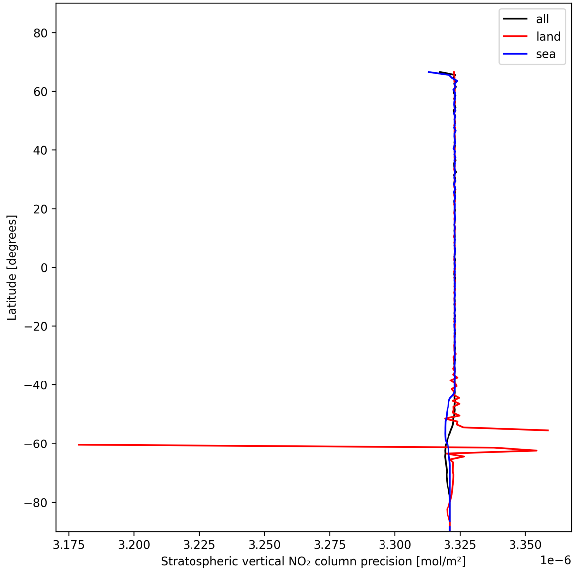
Figure 20: Zonal average of “Stratospheric vertical NO 2 column precision” for 2025-01-12 to 2025-01-14.
