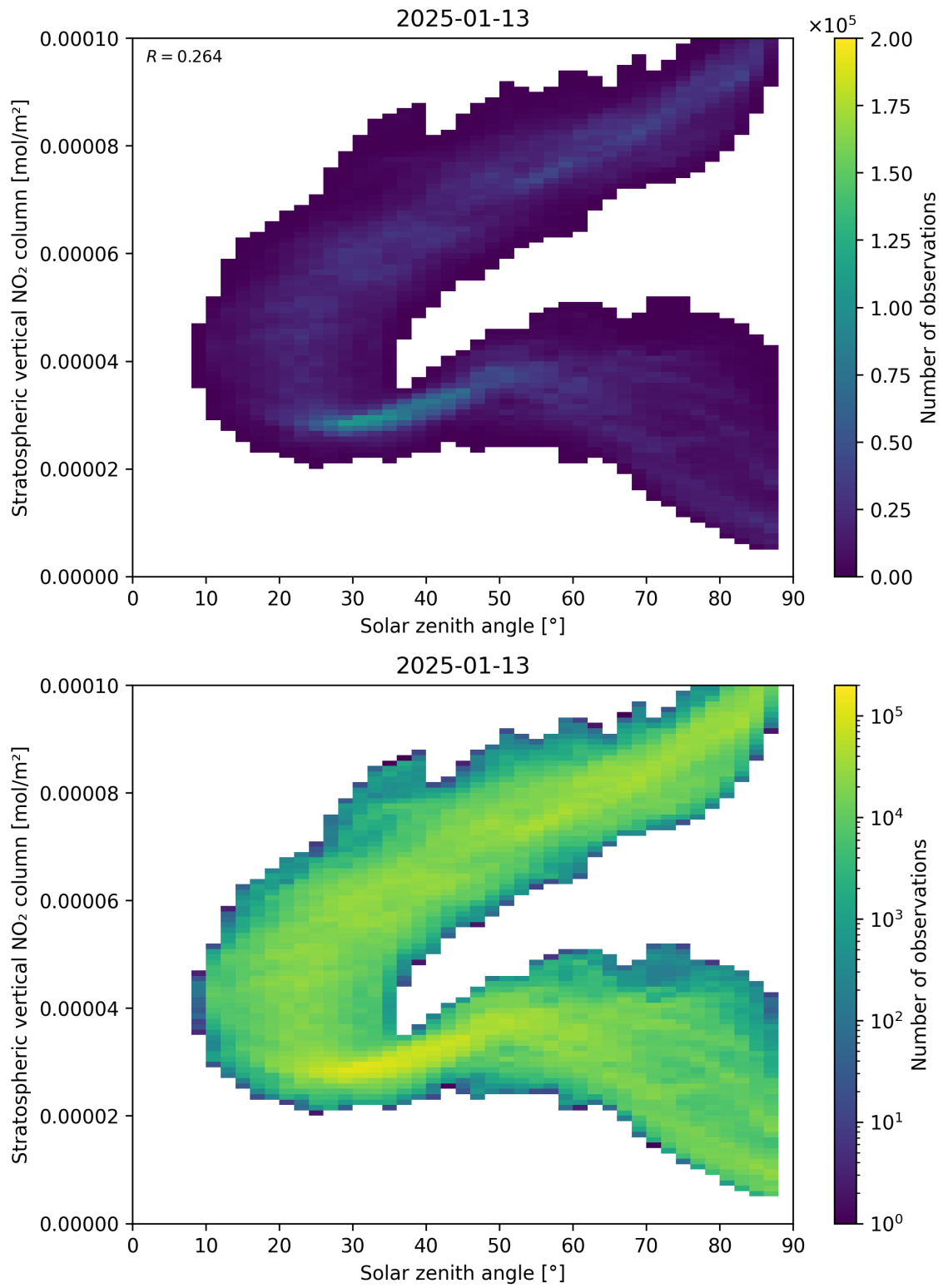
Figure 150: Scatter density plot of “Solar zenith angle” against “Stratospheric vertical NO 2 column” for 2025-01-12 to 2025-01-14.
