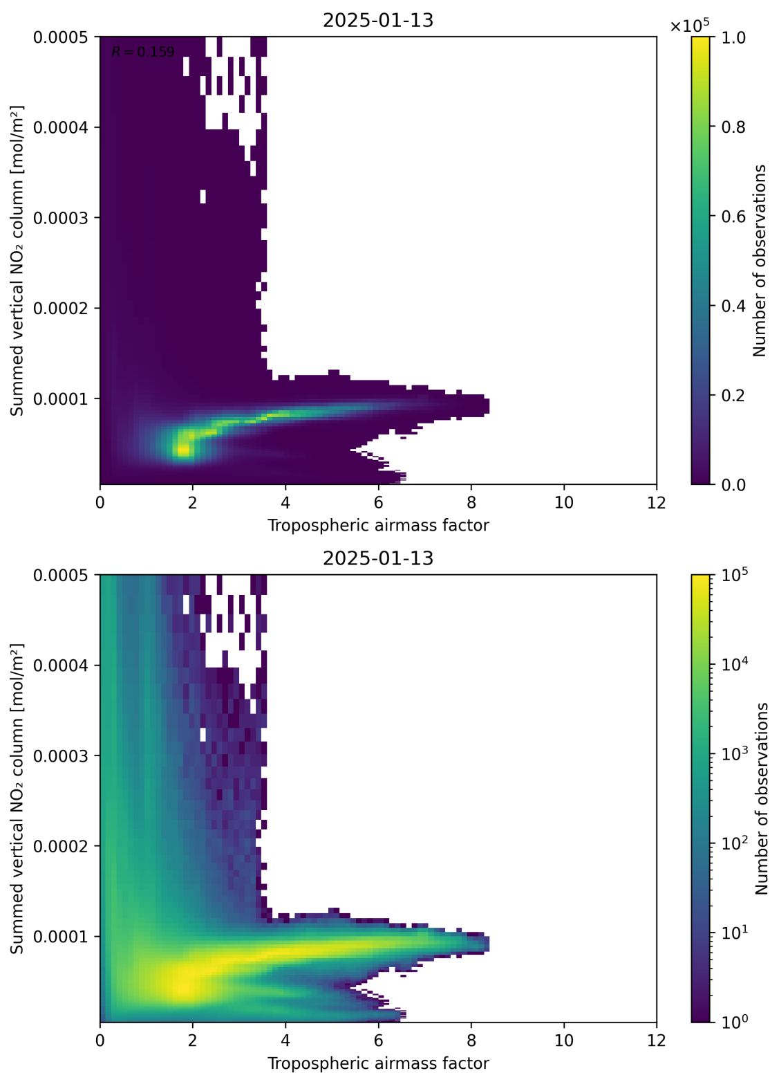
Figure 75: Scatter density plot of “Tropospheric airmass factor” against “Summed vertical NO 2 column” for 2025-01-12 to 2025-01-14.
