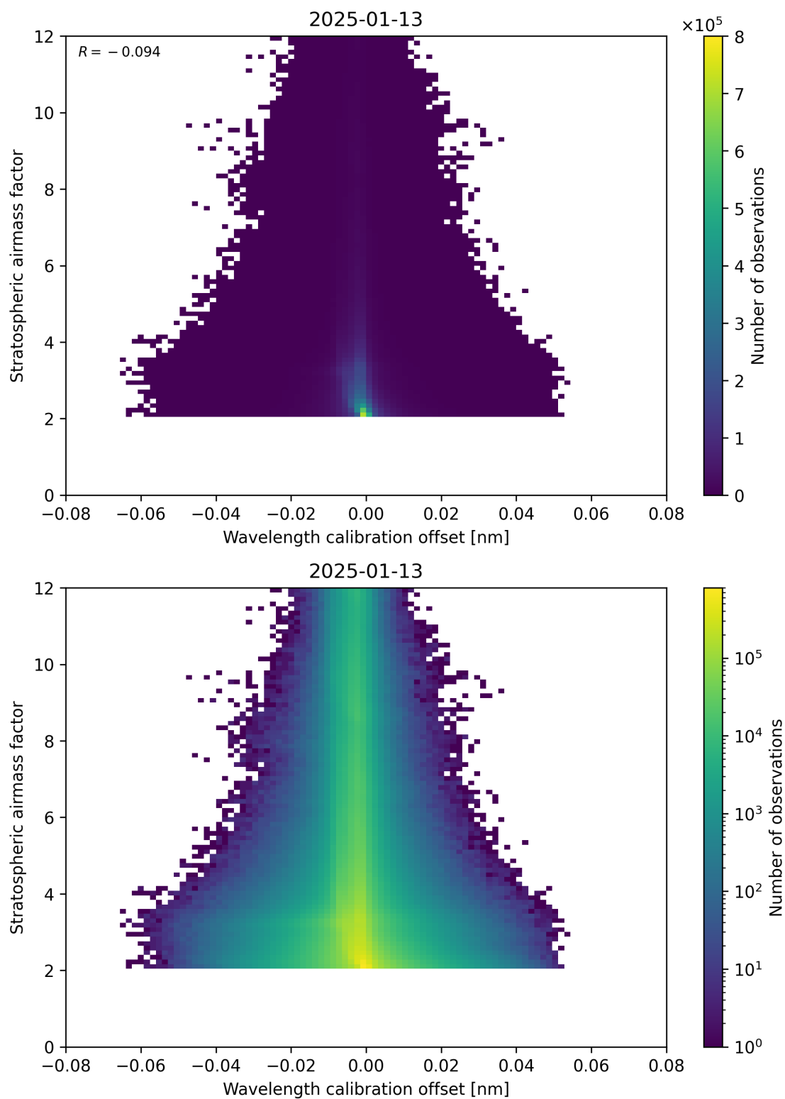
Figure 174: Scatter density plot of “Wavelength calibration offset” against “Stratospheric airmass factor” for 2025-01-12 to 2025-01-14.
