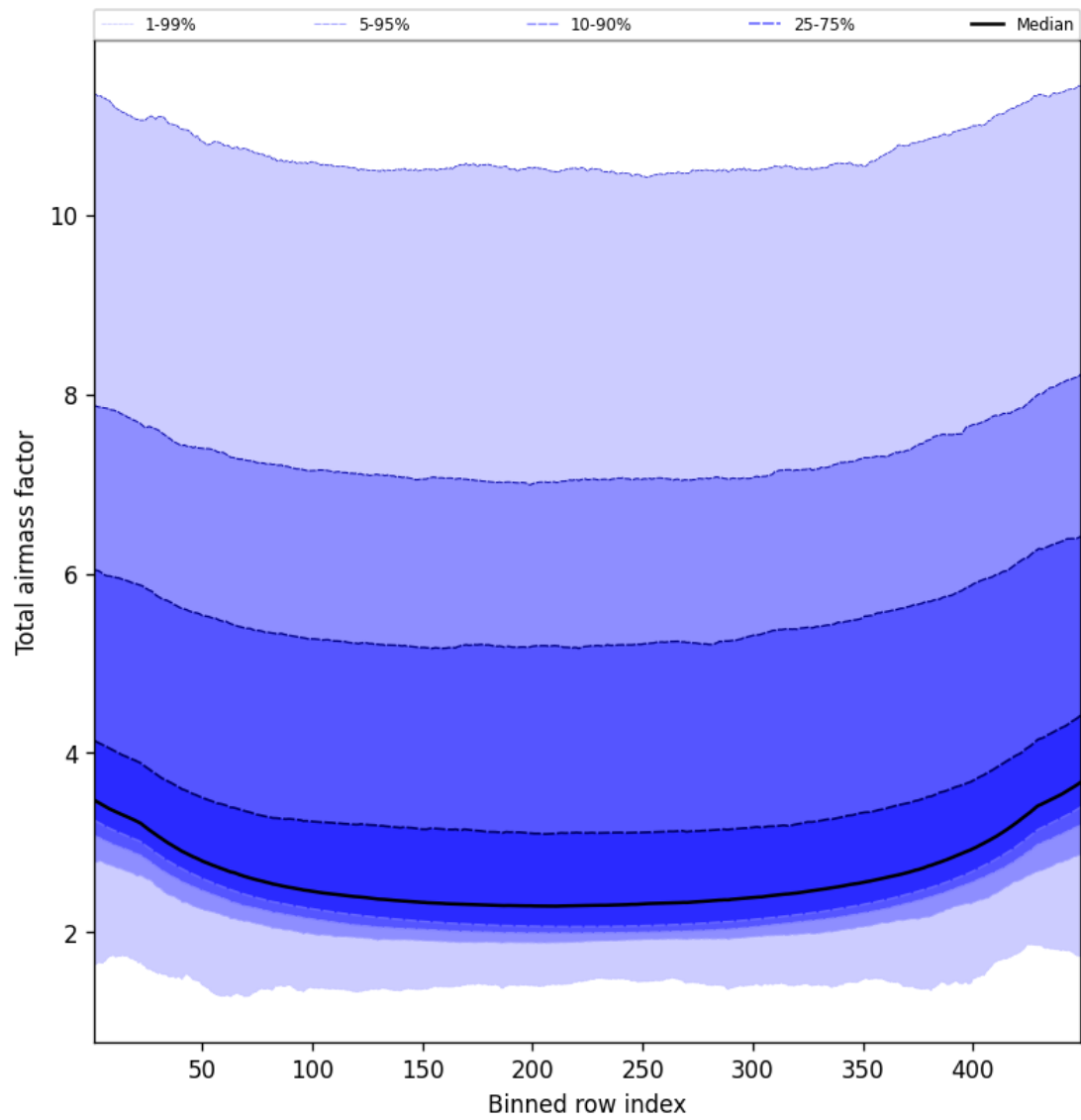
Figure 49: Along track statistics of “Total airmass factor” for 2025-01-12 to 2025-01-14
