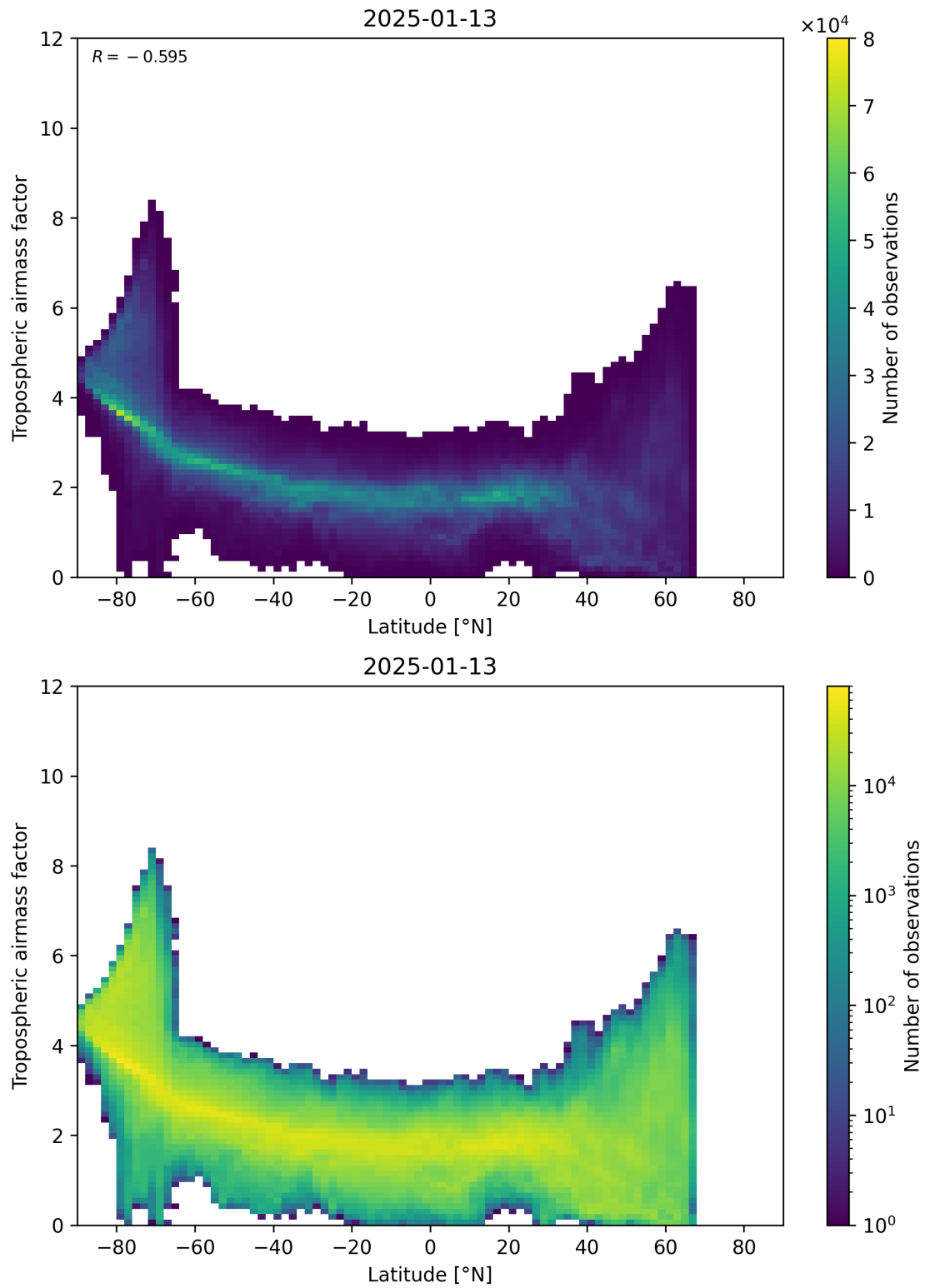
Figure 85: Scatter density plot of “Latitude” against “Tropospheric airmass factor” for 2025-01-12 to 2025-01-14.
