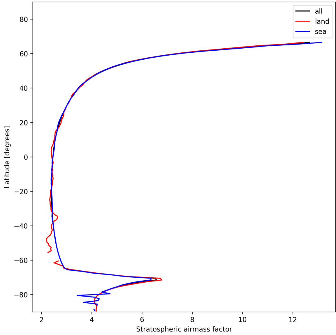
Figure 27: Zonal average of “Stratospheric airmass factor” for 2025-01-12 to 2025-01-14.
