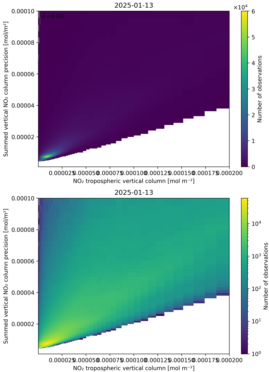
Figure 127: Scatter density plot of “NO 2 tropospheric vertical column” against “Summed vertical NO 2 column precision” for 2025-01-12 to 2025-01-14.
