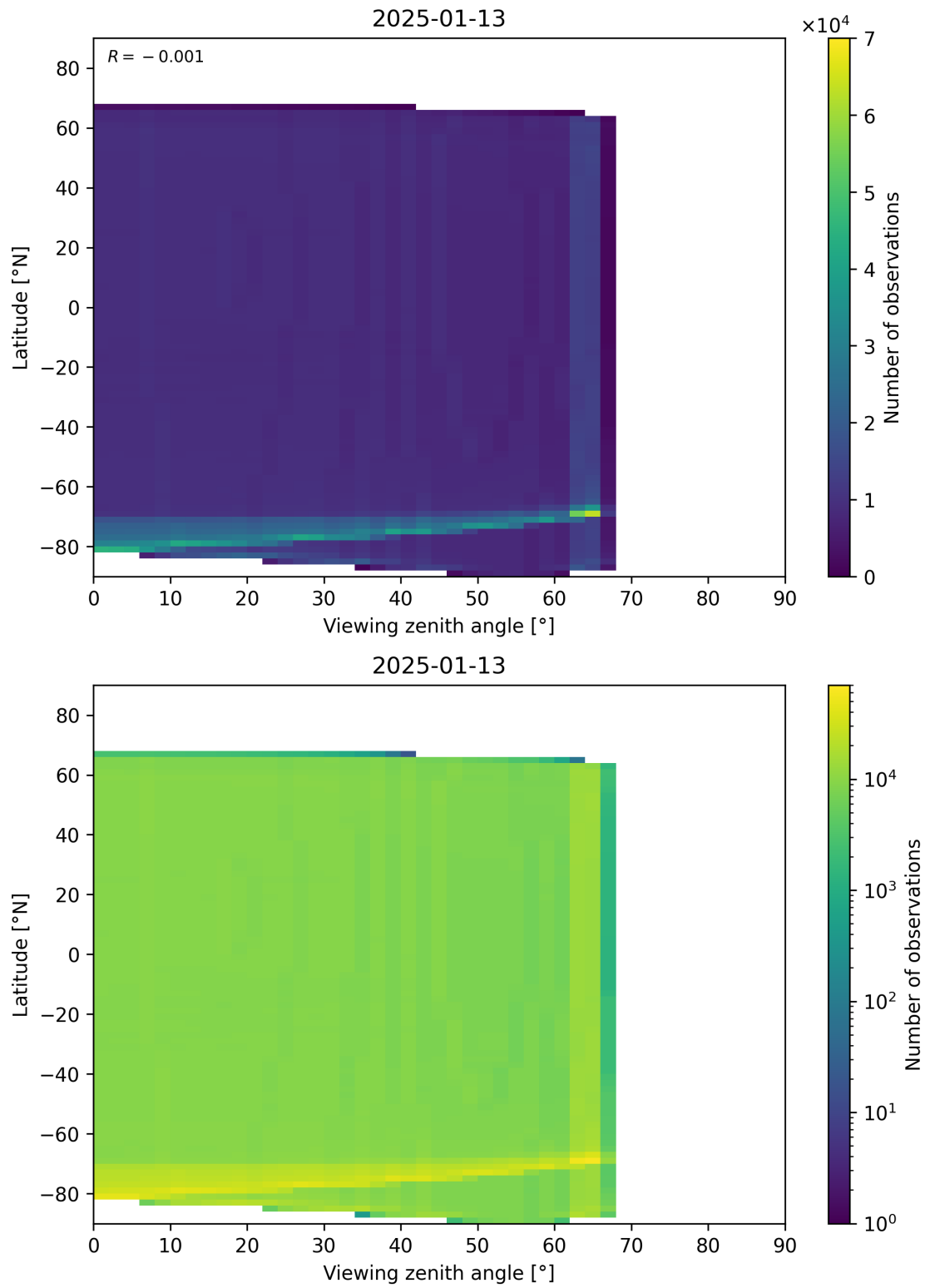
Figure 163: Scatter density plot of “Viewing zenith angle” against “Latitude” for 2025-01-12 to 2025-01-14.
