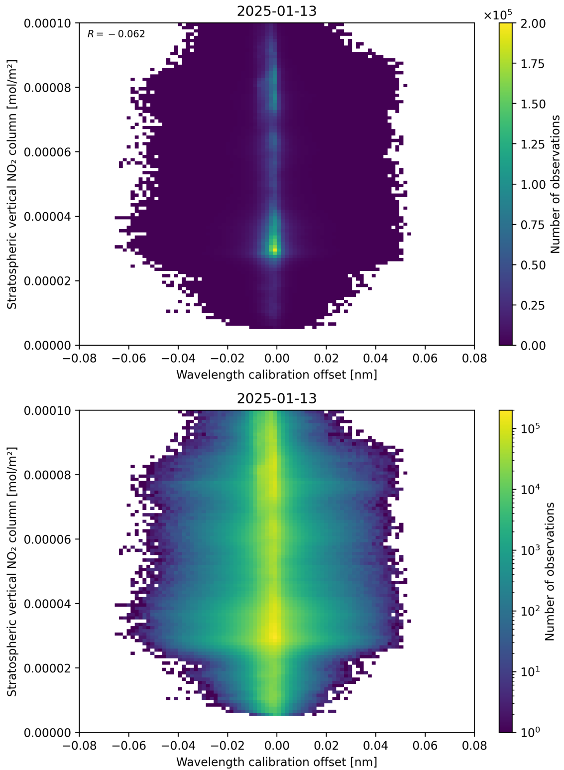
Figure 176: Scatter density plot of “Wavelength calibration offset” against “Stratospheric vertical NO 2 column” for 2025-01-12 to 2025-01-14.
