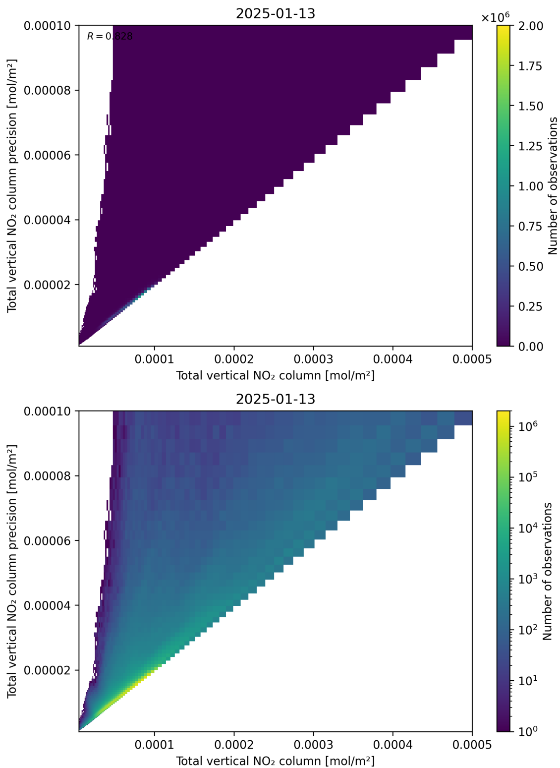
Figure 114: Scatter density plot of “Total vertical NO 2 column” against “Total vertical NO 2 column precision” for 2025-01-12 to 2025-01-14.
