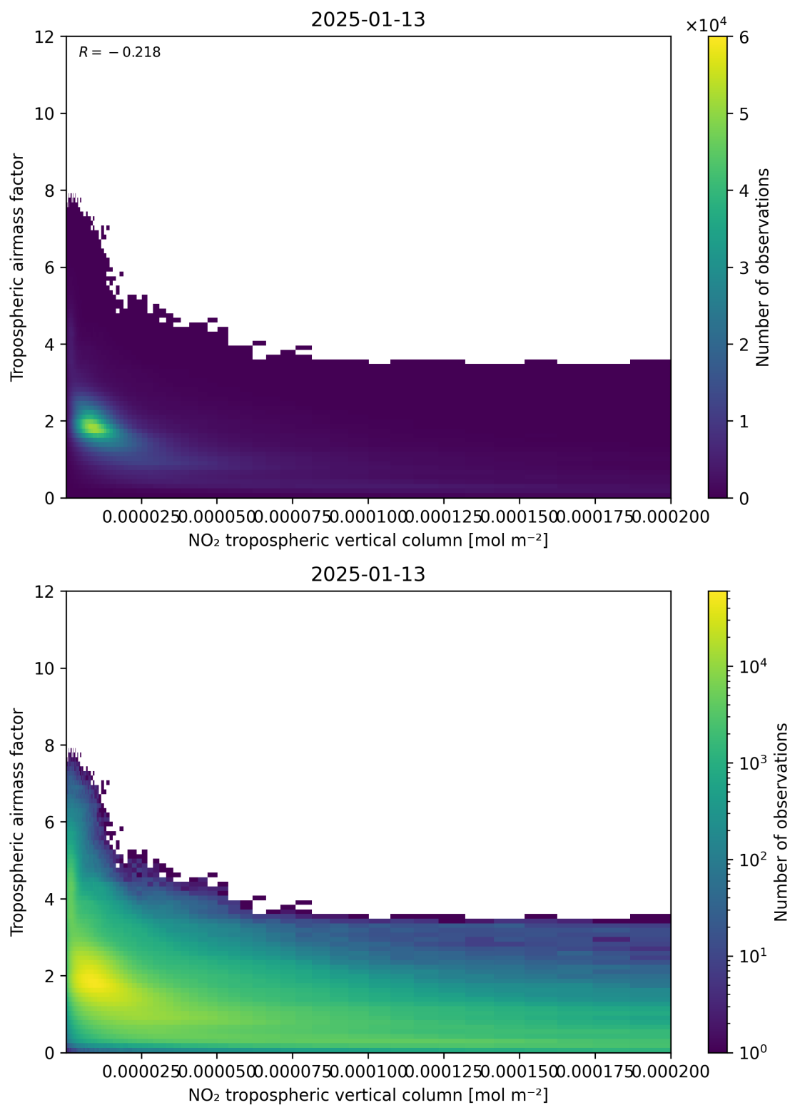
Figure 123: Scatter density plot of “NO 2 tropospheric vertical column” against “Tropospheric air mass factor” for 2025-01-12 to 2025-01-14.
