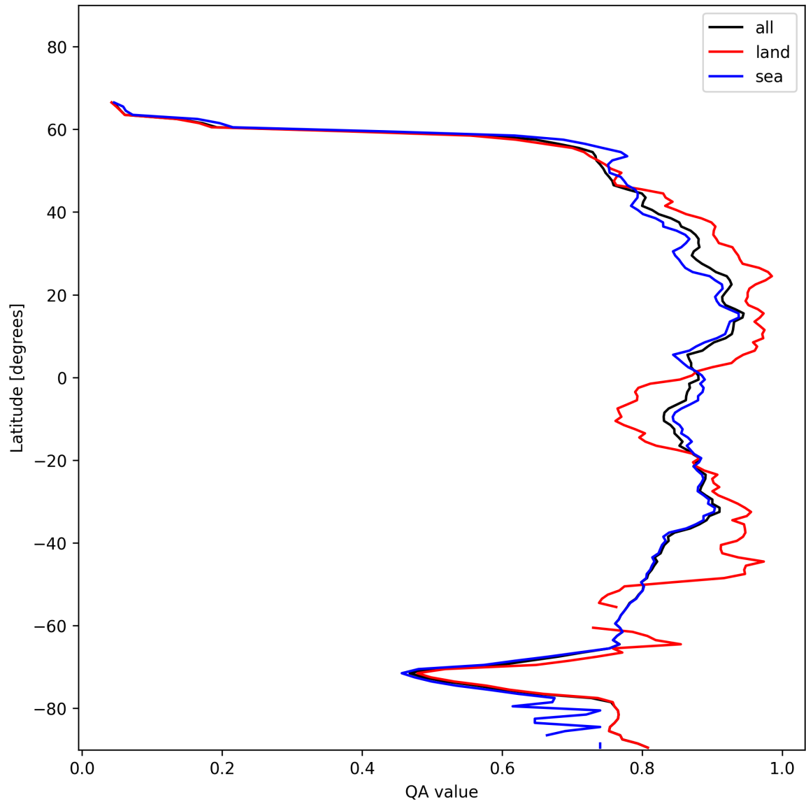
Figure 11: Zonal average of “QA value” for 2025-01-12 to 2025-01-14.
