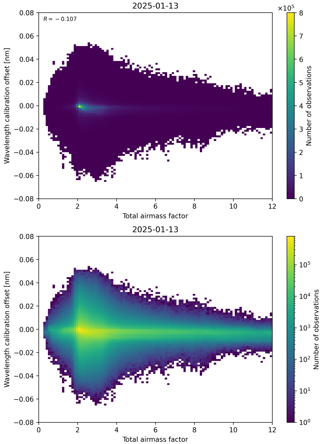
Figure 70: Scatter density plot of “Total airmass factor” against “Wavelength calibration offset” for 2025-01-12 to 2025-01-14.
