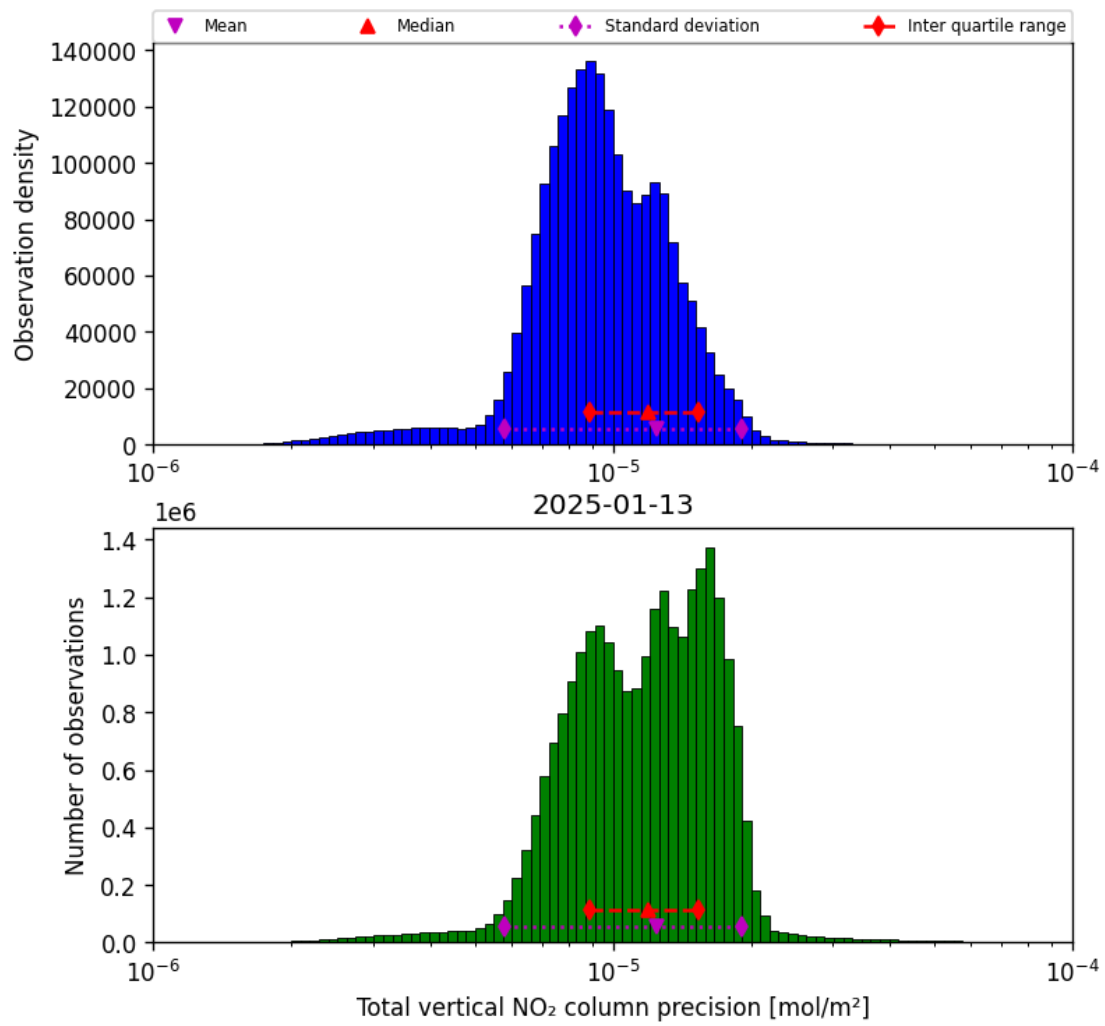
Figure 39: Histogram of “Total vertical NO 2 column precision” for 2025-01-12 to 2025-01-14
