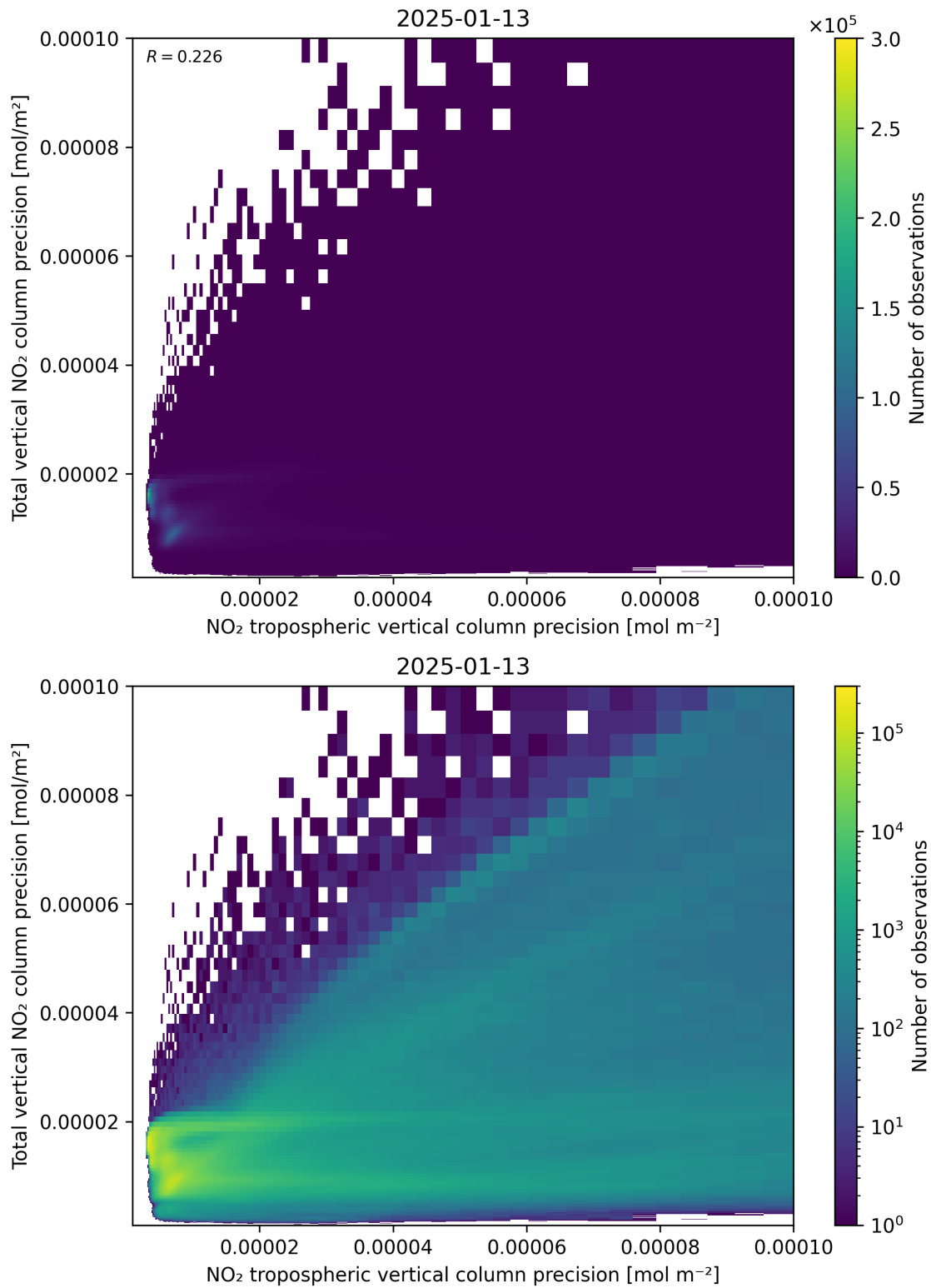
Figure 139: Scatter density plot of “NO 2 tropospheric vertical column precision” against “Total vertical NO 2 column precision” for 2025-01-12 to 2025-01-14.
