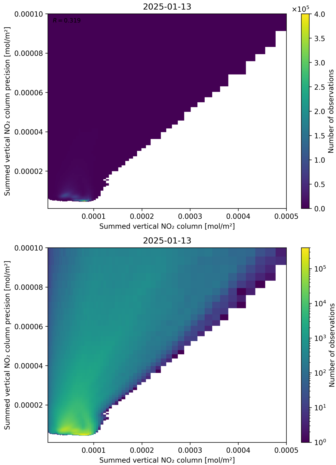
Figure 105: Scatter density plot of “Summed vertical NO 2 column” against “Summed vertical NO 2 column precision” for 2025-01-12 to 2025-01-14.
