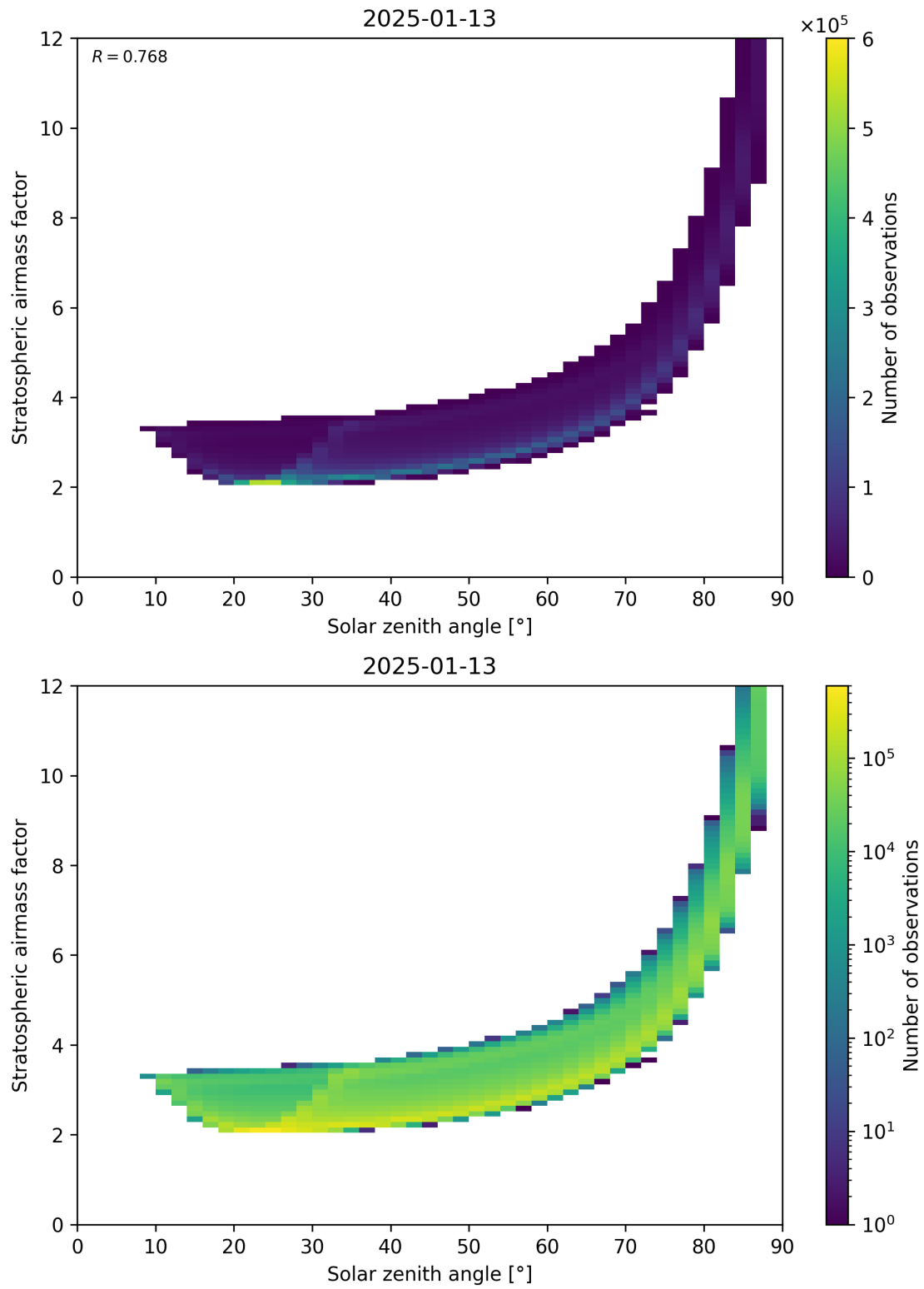
Figure 145: Scatter density plot of “Solar zenith angle” against “Stratospheric airmass factor” for 2025-01-12 to 2025-01-14.
