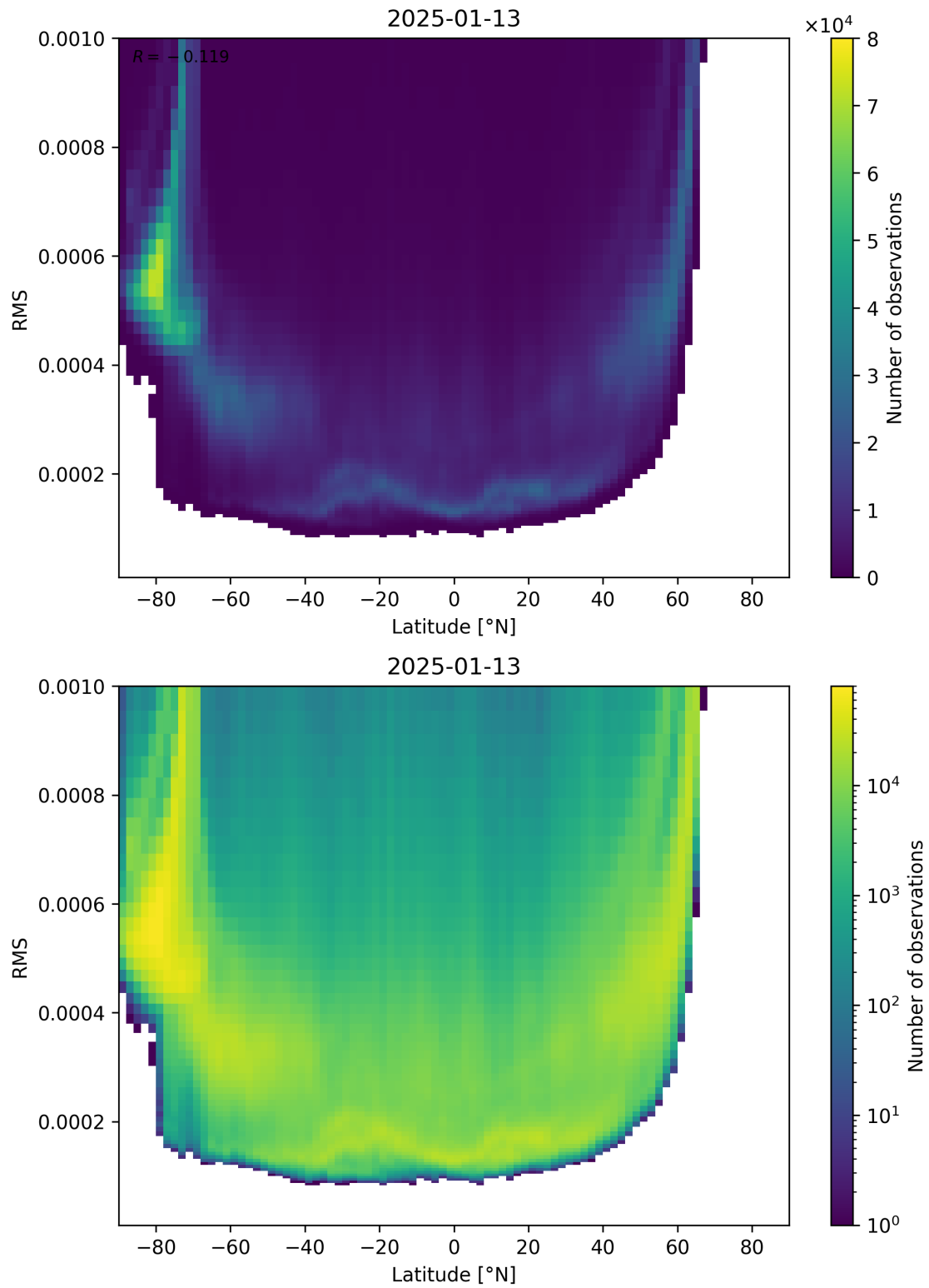
Figure 94: Scatter density plot of “Latitude” against “RMS” for 2025-01-12 to 2025-01-14.
