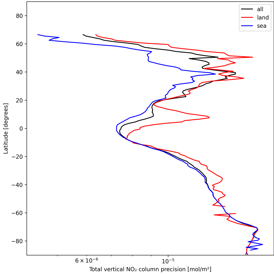
Figure 22: Zonal average of “Total vertical NO 2 column precision” for 2025-01-12 to 2025-01-14.
