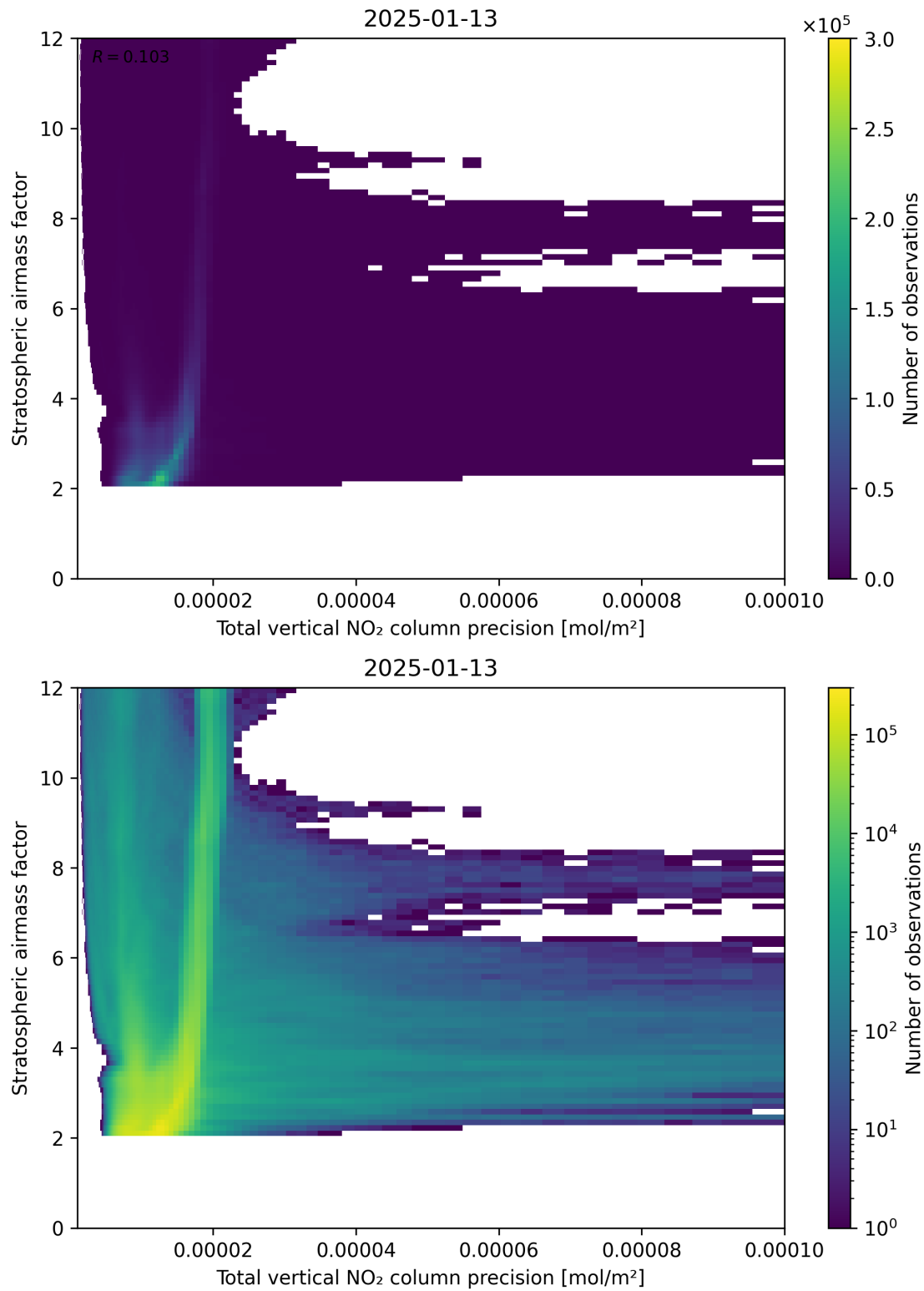
Figure 115: Scatter density plot of “Total vertical NO 2 column precision” against “Stratospheric air mass factor” for 2025-01-12 to 2025-01-14.
