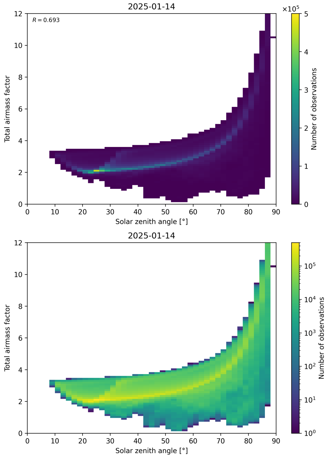
Figure 146: Scatter density plot of “Solar zenith angle” against “Total airmass factor” for 2025-01-13 to 2025-01-15.
