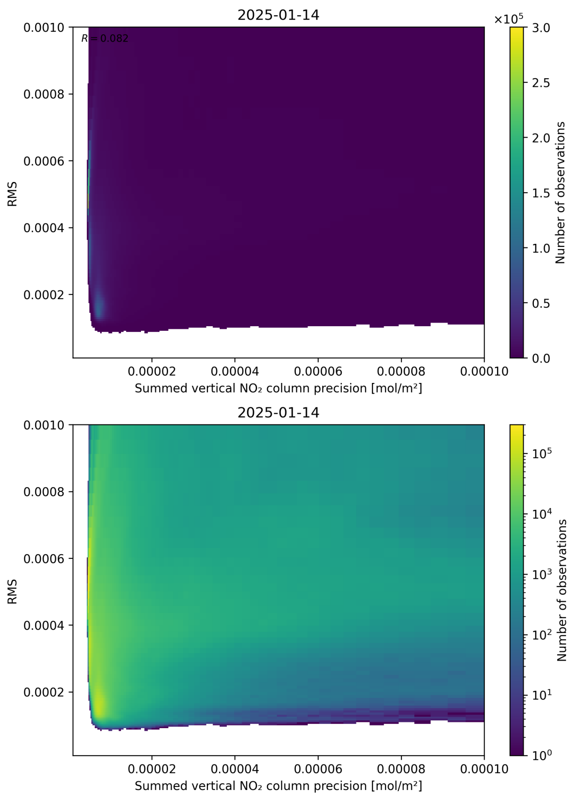
Figure 108: Scatter density plot of “Summed vertical NO 2 column precision” against “RMS” for 2025-01-13 to 2025-01-15.
