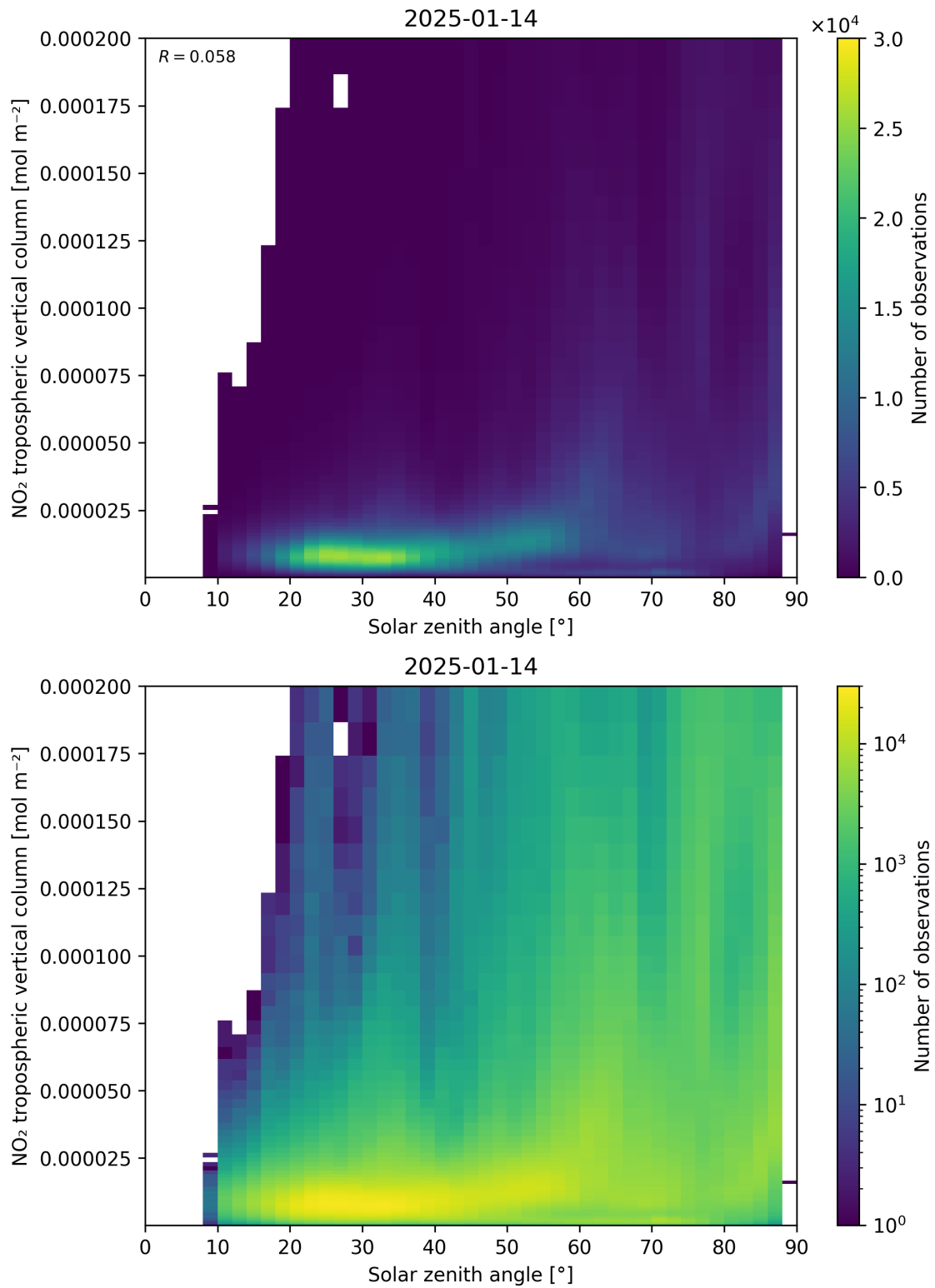
Figure 155: Scatter density plot of “Solar zenith angle” against “NO 2 tropospheric vertical column” for 2025-01-13 to 2025-01-15.
