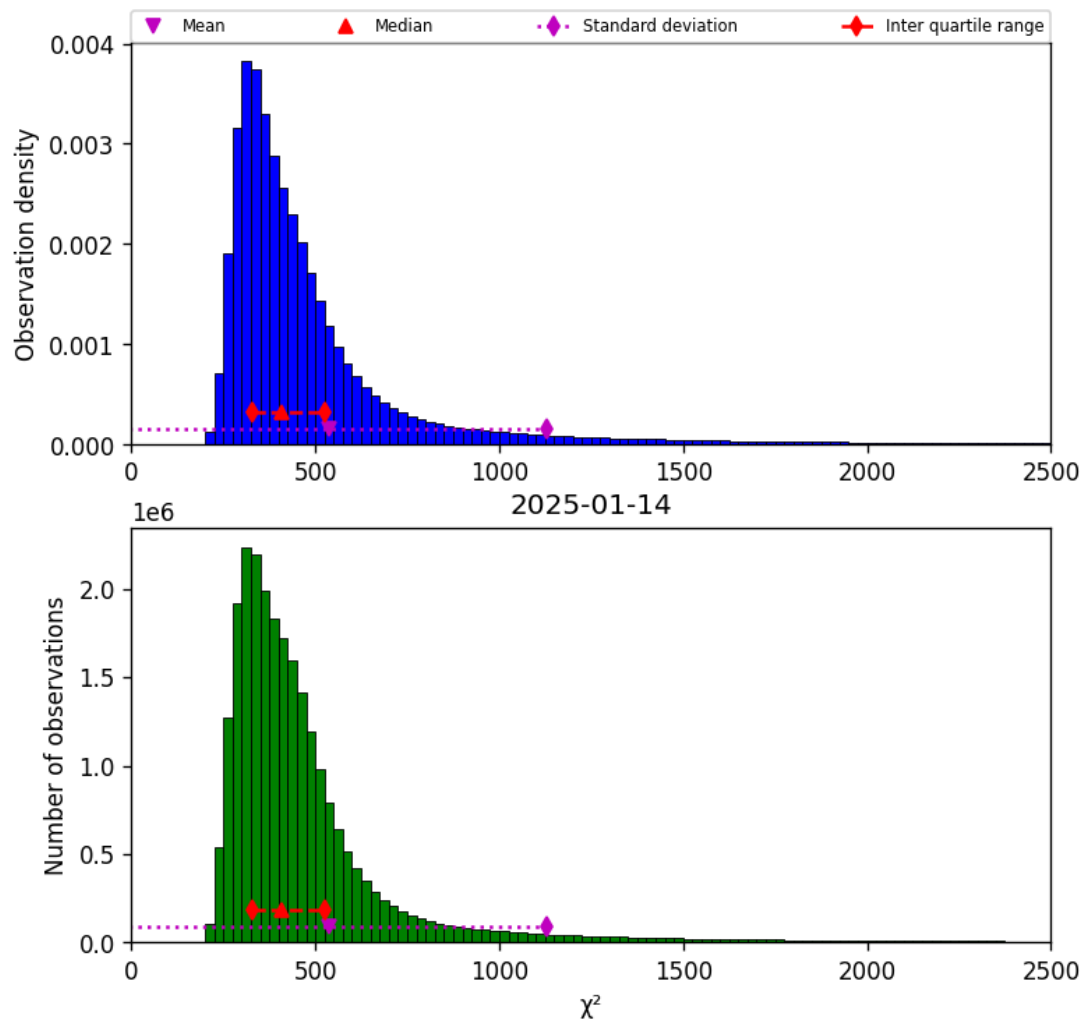
Figure 42: Histogram of “ \chi^2 ” for 2025-01-13 to 2025-01-15
