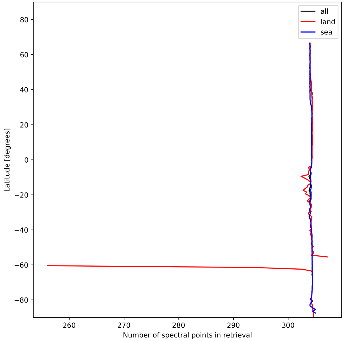
Figure 16: Zonal average of “Number of spectral points in retrieval” for 2025-01-13 to 2025-01-15.
