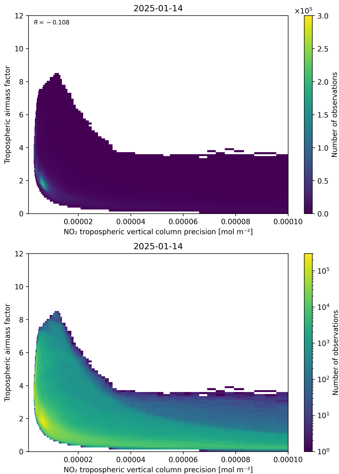
Figure 133: Scatter density plot of “NO 2 tropospheric vertical column precision” against “Tropospheric airmass factor” for 2025-01-13 to 2025-01-15.
