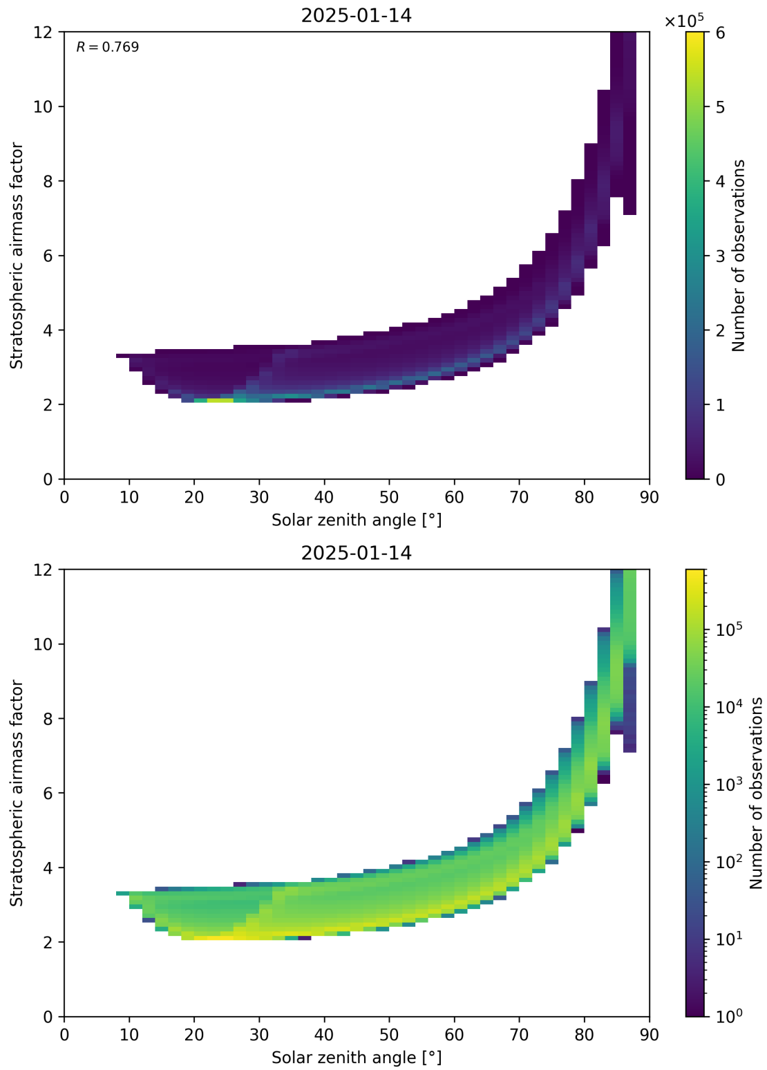
Figure 145: Scatter density plot of “Solar zenith angle” against “Stratospheric airmass factor” for 2025-01-13 to 2025-01-15.
