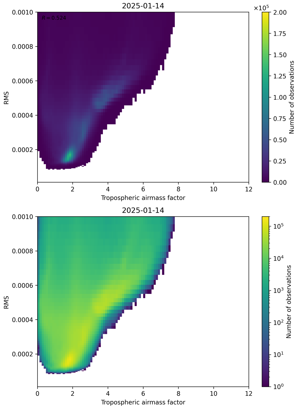
Figure 79: Scatter density plot of “Tropospheric airmass factor” against “RMS” for 2025-01-13 to 2025-01-15.
