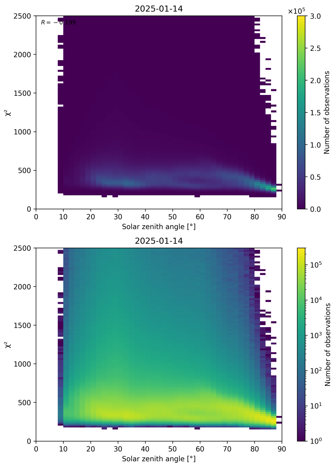
Figure 148: Scatter density plot of “Solar zenith angle” against “ \chi^2 ” for 2025-01-13 to 2025-01-15.
