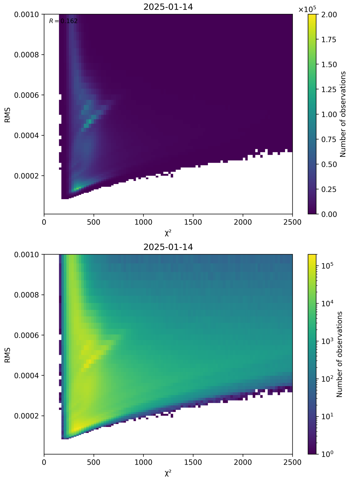
Figure 82: Scatter density plot of “ \chi^2 ” against “RMS” for 2025-01-13 to 2025-01-15.
