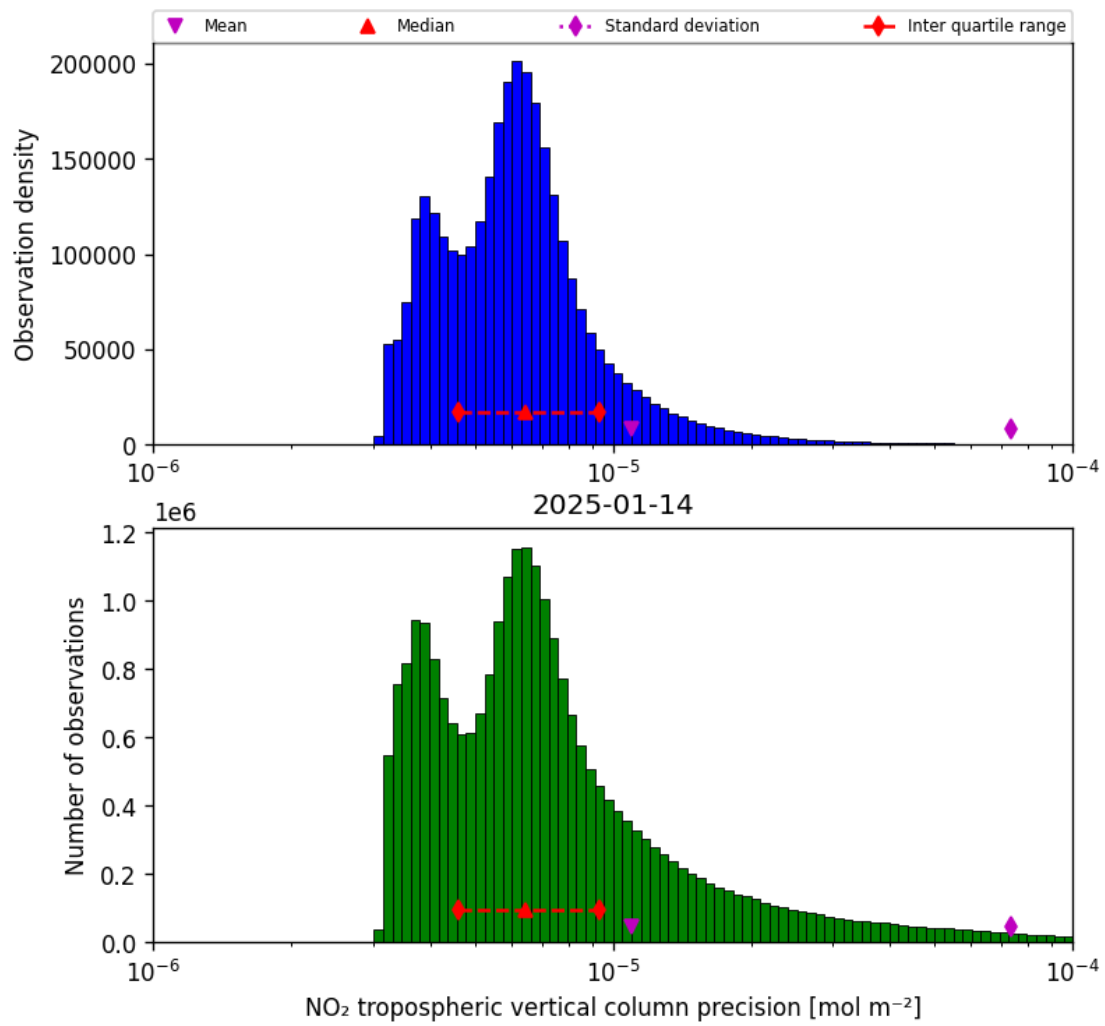
Figure 30: Histogram of “NO 2 tropospheric vertical column precision” for 2025-01-13 to 2025-01-15
