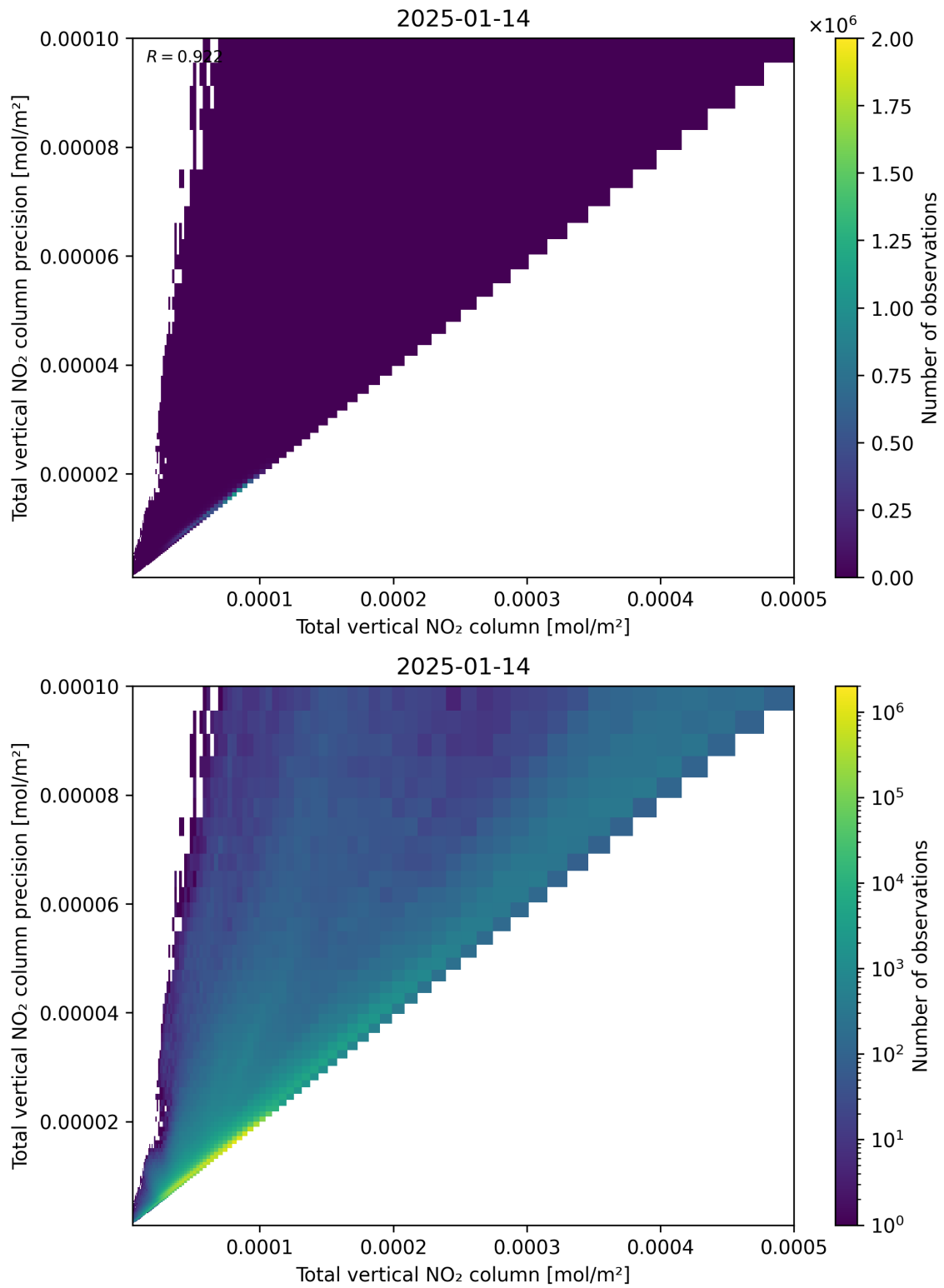
Figure 114: Scatter density plot of “Total vertical NO 2 column” against “Total vertical NO 2 column precision” for 2025-01-13 to 2025-01-15.
