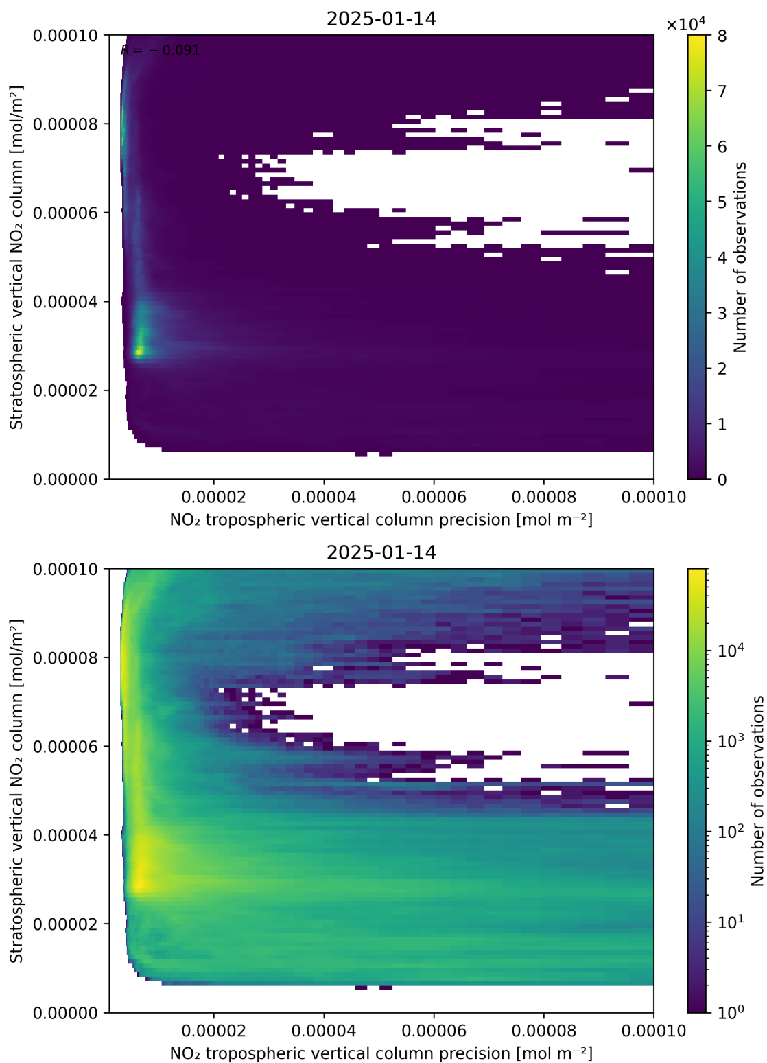
Figure 135: Scatter density plot of “NO 2 tropospheric vertical column precision” against “Stratospheric vertical NO 2 column” for 2025-01-13 to 2025-01-15.
