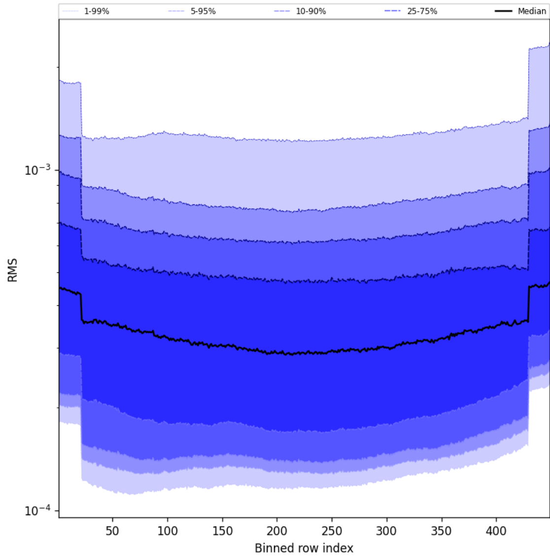
Figure 60: Along track statistics of “RMS” for 2025-01-13 to 2025-01-15
