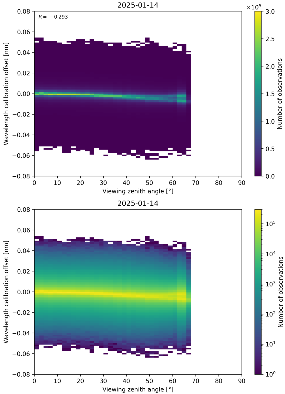
Figure 173: Scatter density plot of “Viewing zenith angle” against “Wavelength calibration offset” for 2025-01-13 to 2025-01-15.
