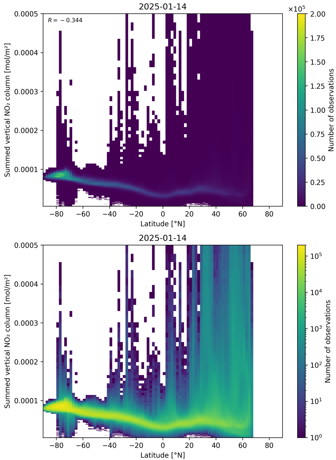
Figure 88: Scatter density plot of “Latitude” against “Summed vertical NO 2 column” for 2025-01-13 to 2025-01-15.
