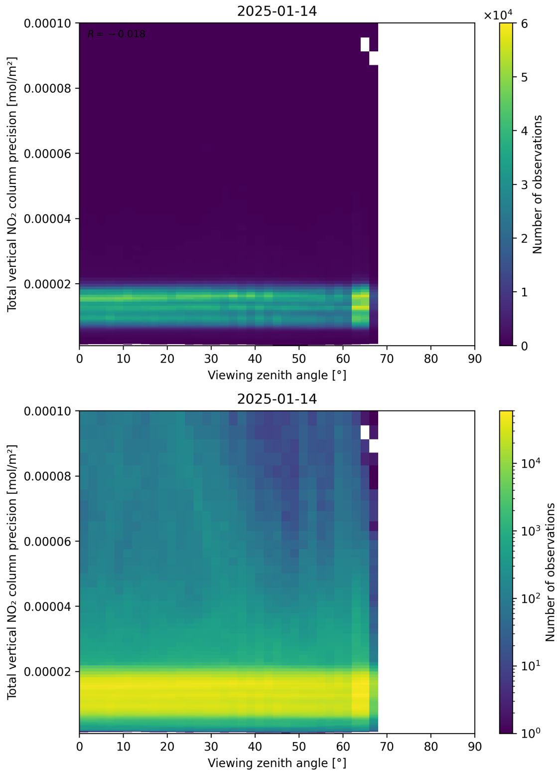
Figure 168: Scatter density plot of “Viewing zenith angle” against “Total vertical NO 2 column precision” for 2025-01-13 to 2025-01-15.
