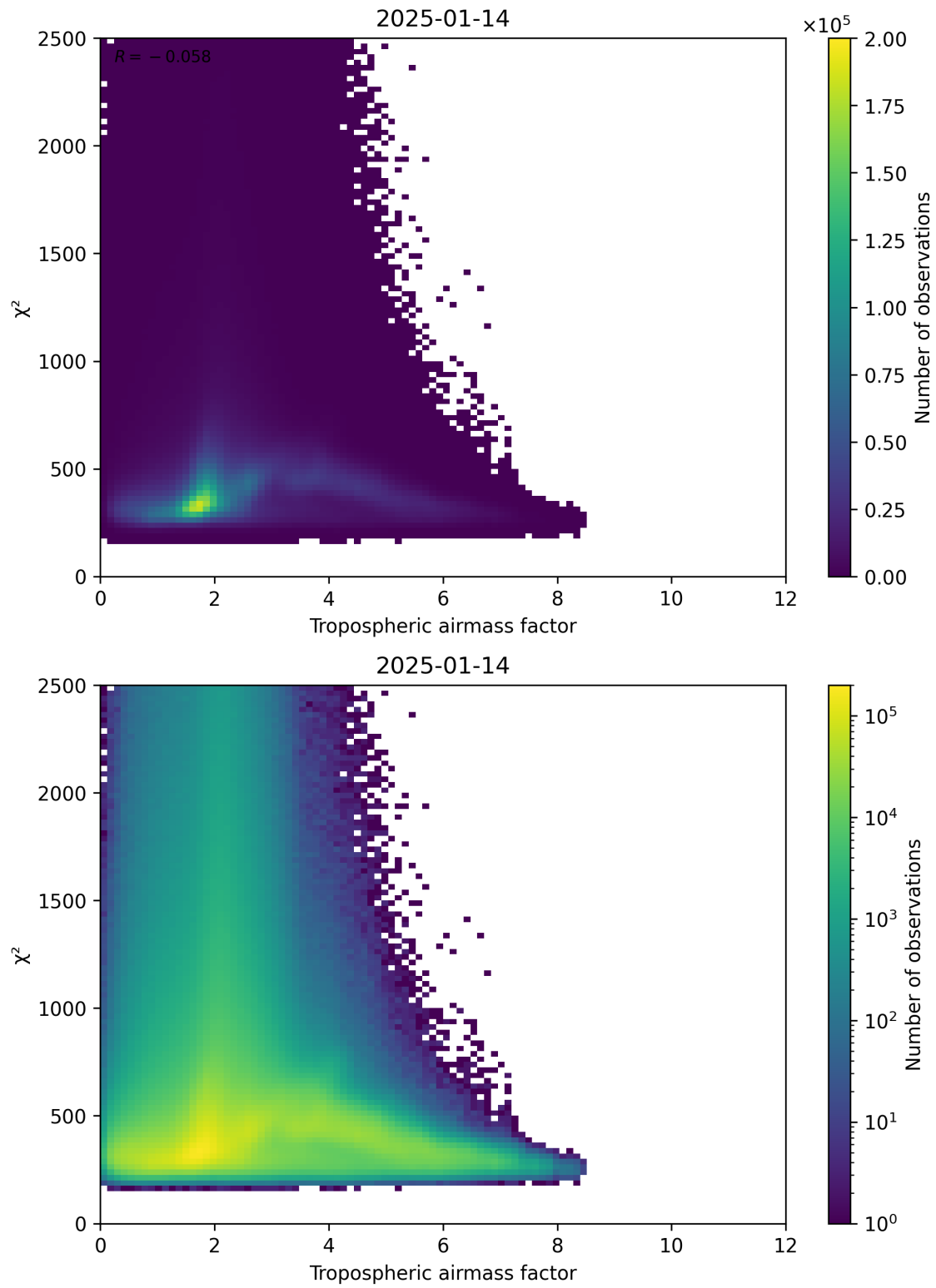
Figure 73: Scatter density plot of “Tropospheric airmass factor” against “ \chi^2 ” for 2025-01-13 to 2025-01-15.
