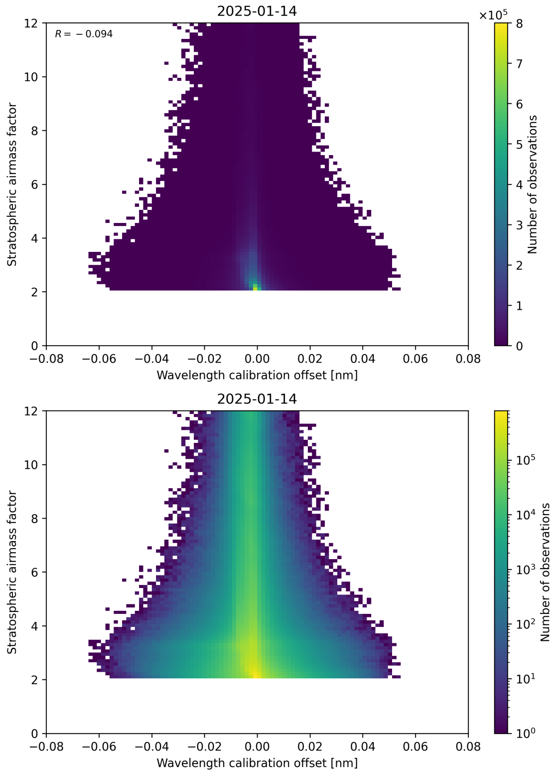
Figure 174: Scatter density plot of “Wavelength calibration offset” against “Stratospheric airmass factor” for 2025-01-13 to 2025-01-15.
