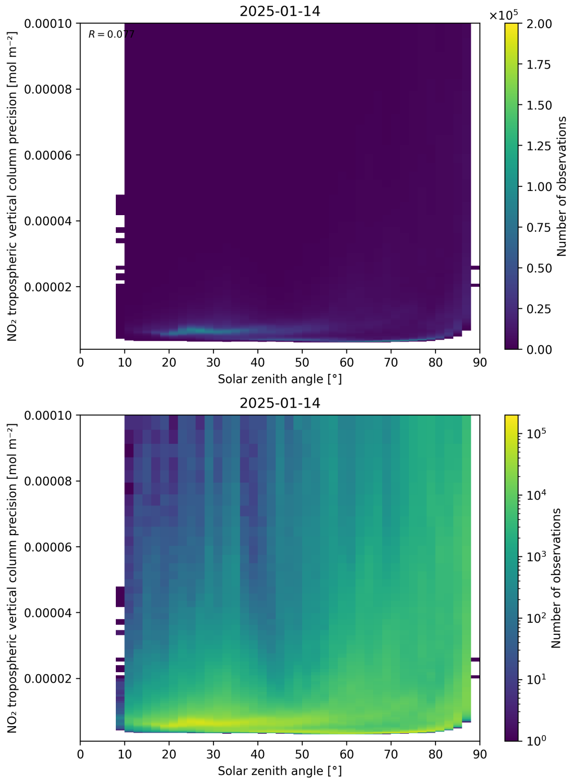
Figure 156: Scatter density plot of “Solar zenith angle” against “NO 2 tropospheric vertical column precision” for 2025-01-13 to 2025-01-15.
