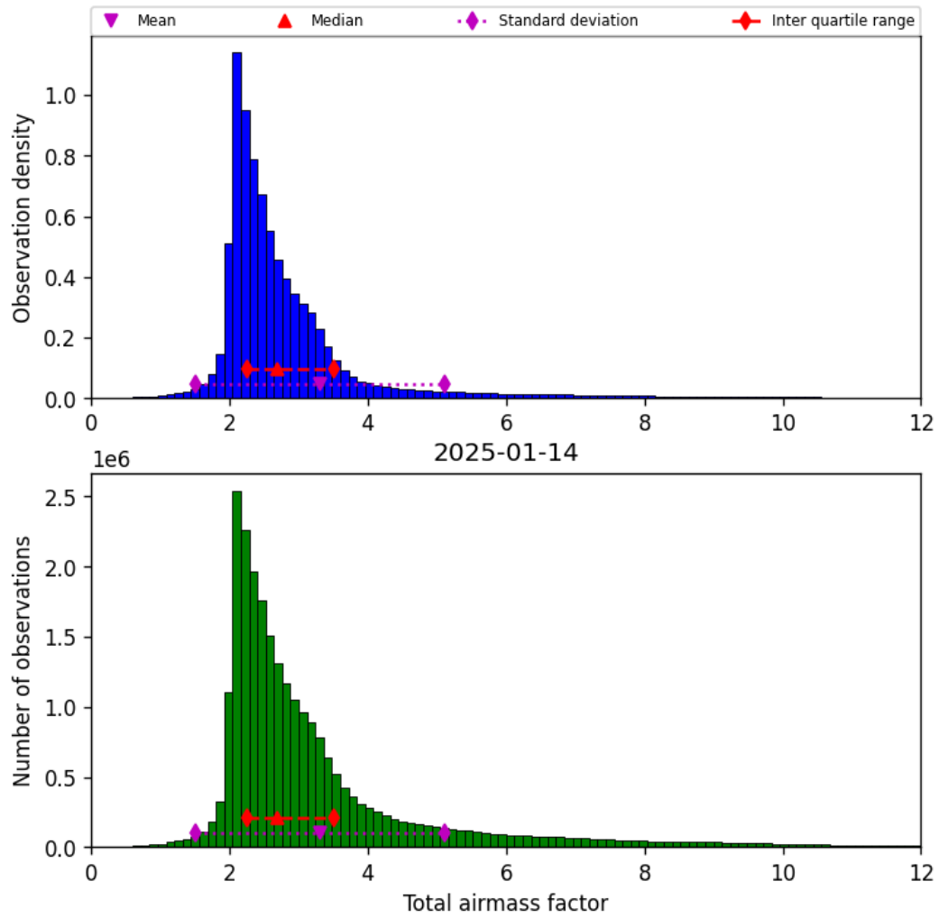
Figure 32: Histogram of “Total airmass factor” for 2025-01-13 to 2025-01-15
