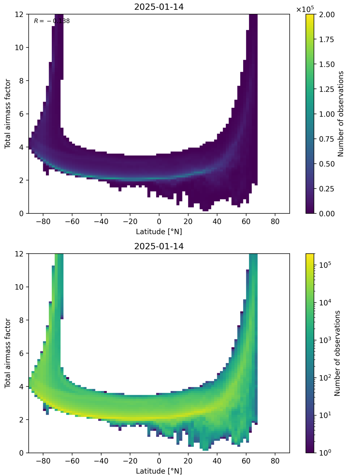
Figure 84: Scatter density plot of “Latitude” against “Total airmass factor” for 2025-01-13 to 2025-01-15.
