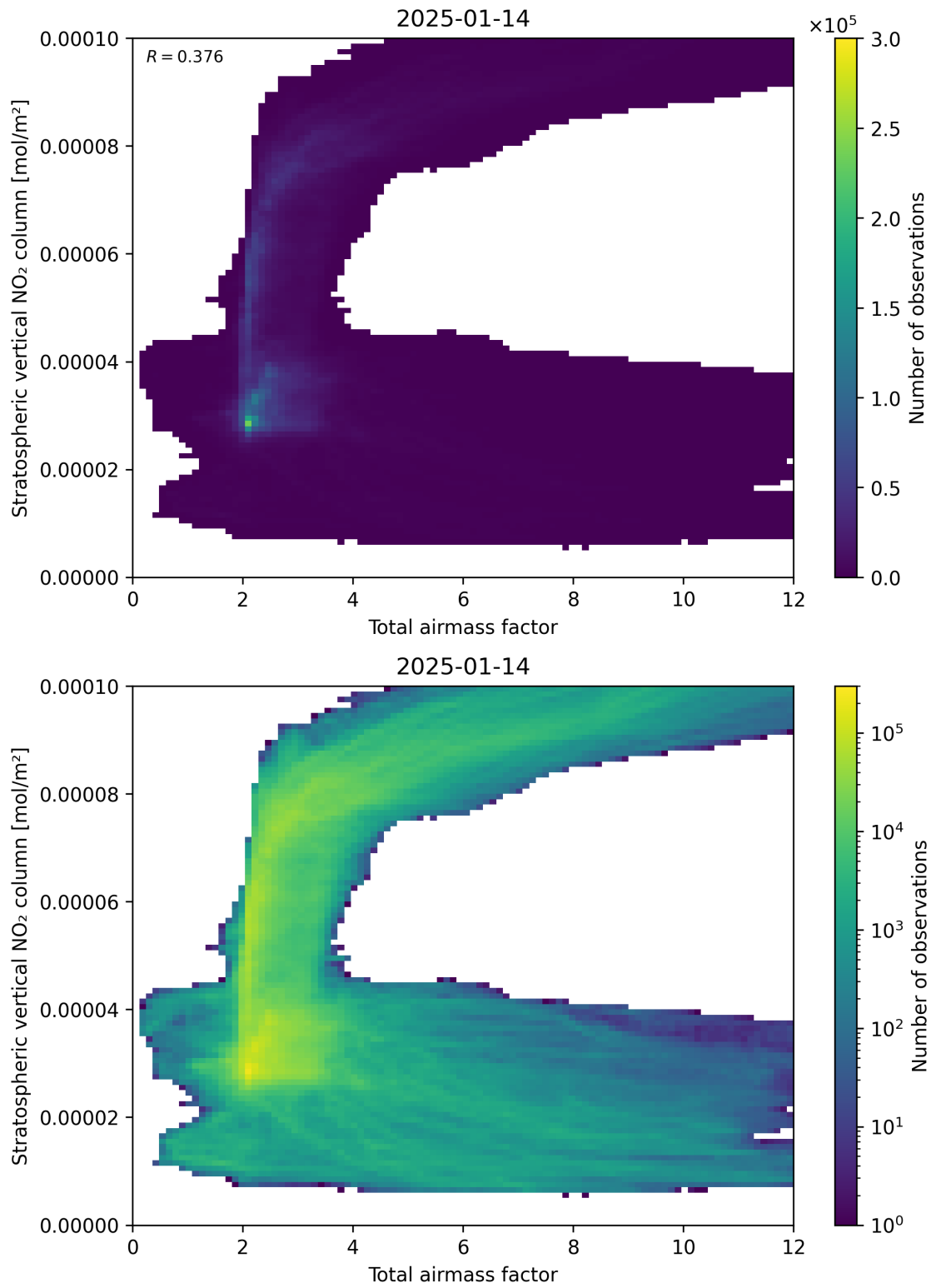
Figure 64: Scatter density plot of “Total airmass factor” against “Stratospheric vertical NO 2 column” for 2025-01-13 to 2025-01-15.
