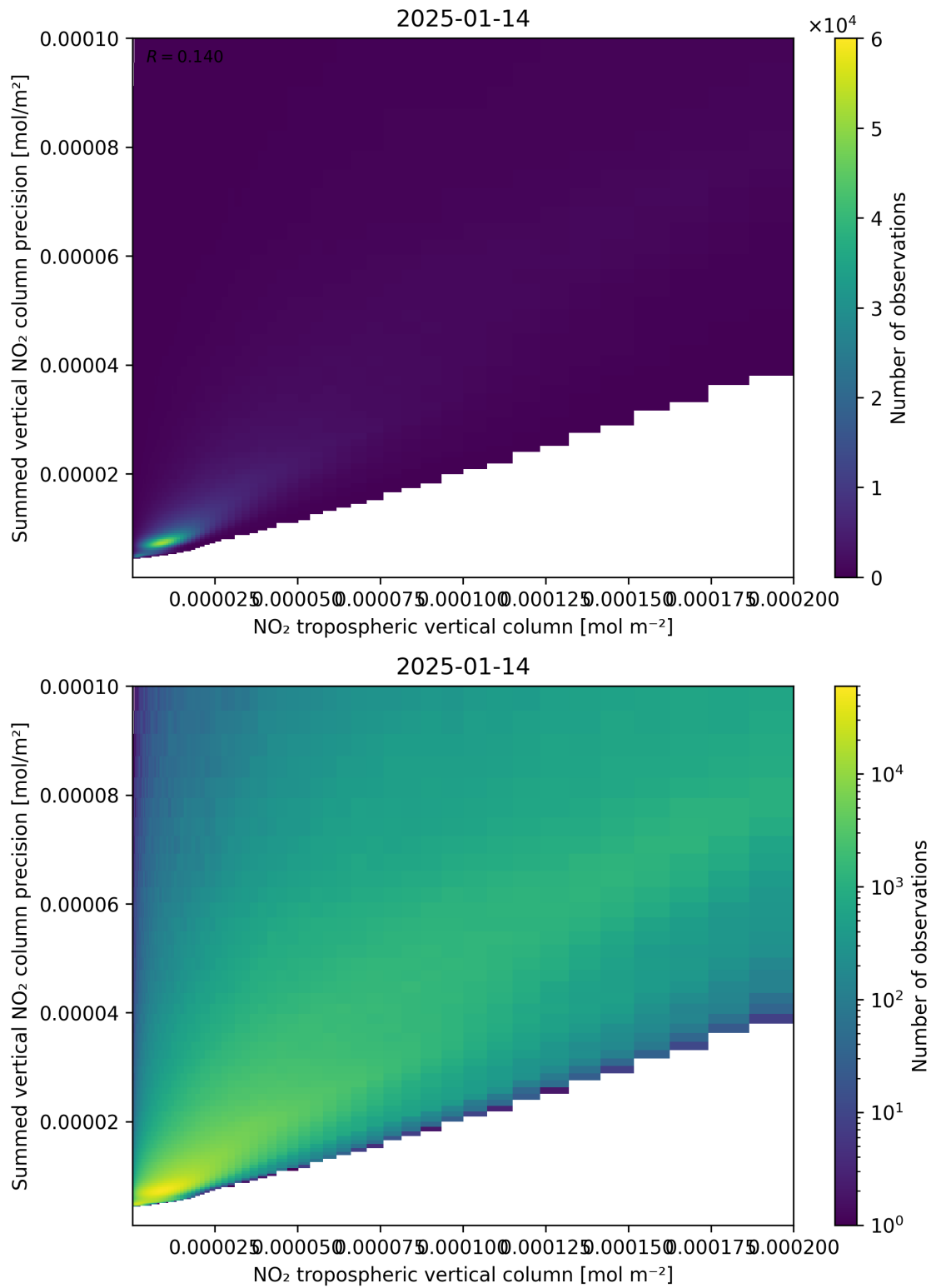
Figure 127: Scatter density plot of “NO 2 tropospheric vertical column” against “Summed vertical NO 2 column precision” for 2025-01-13 to 2025-01-15.
