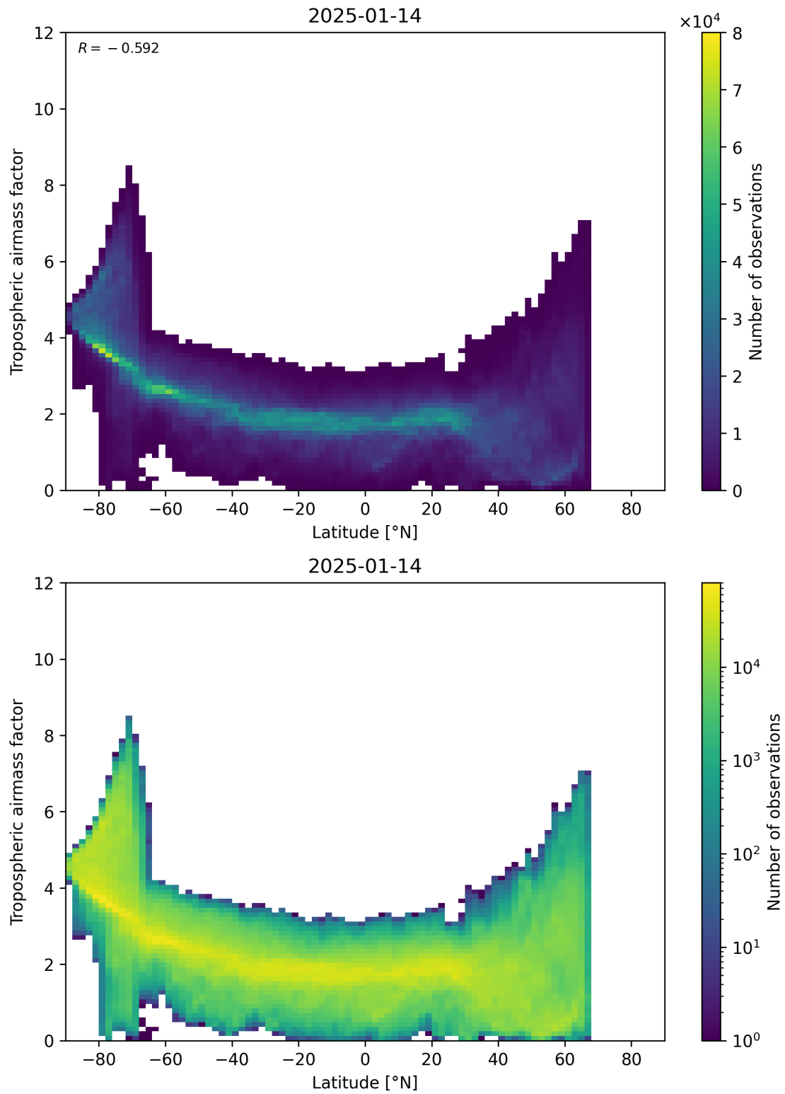
Figure 85: Scatter density plot of “Latitude” against “Tropospheric airmass factor” for 2025-01-13 to 2025-01-15.
