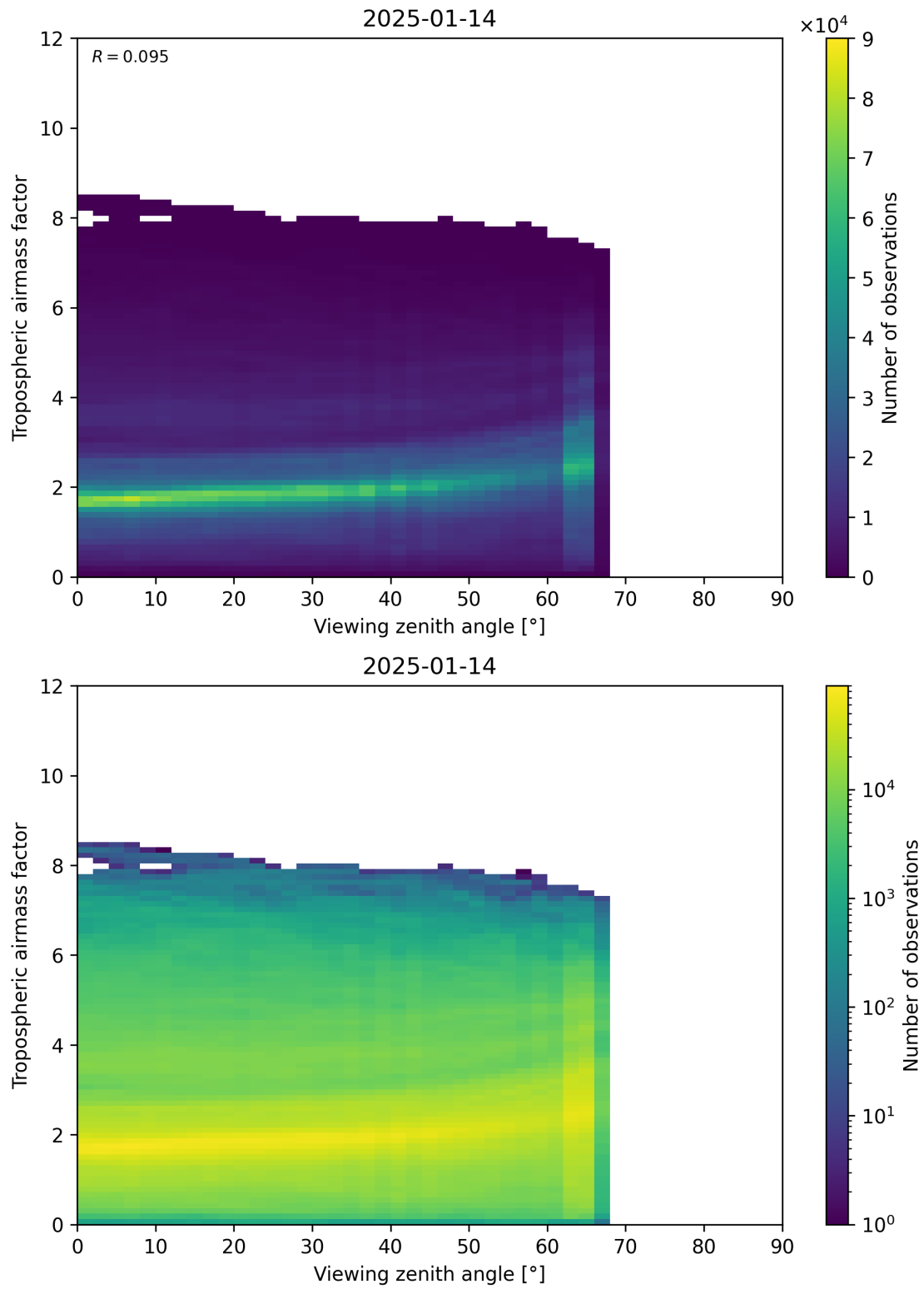
Figure 161: Scatter density plot of “Viewing zenith angle” against “Tropospheric airmass factor” for 2025-01-13 to 2025-01-15.
