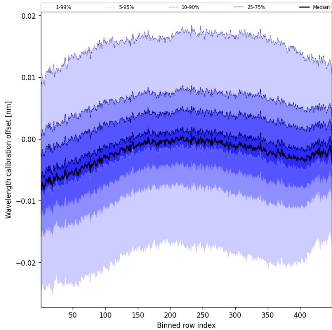
Figure 52: Along track statistics of “Wavelength calibration offset” for 2025-01-13 to 2025-01-15
