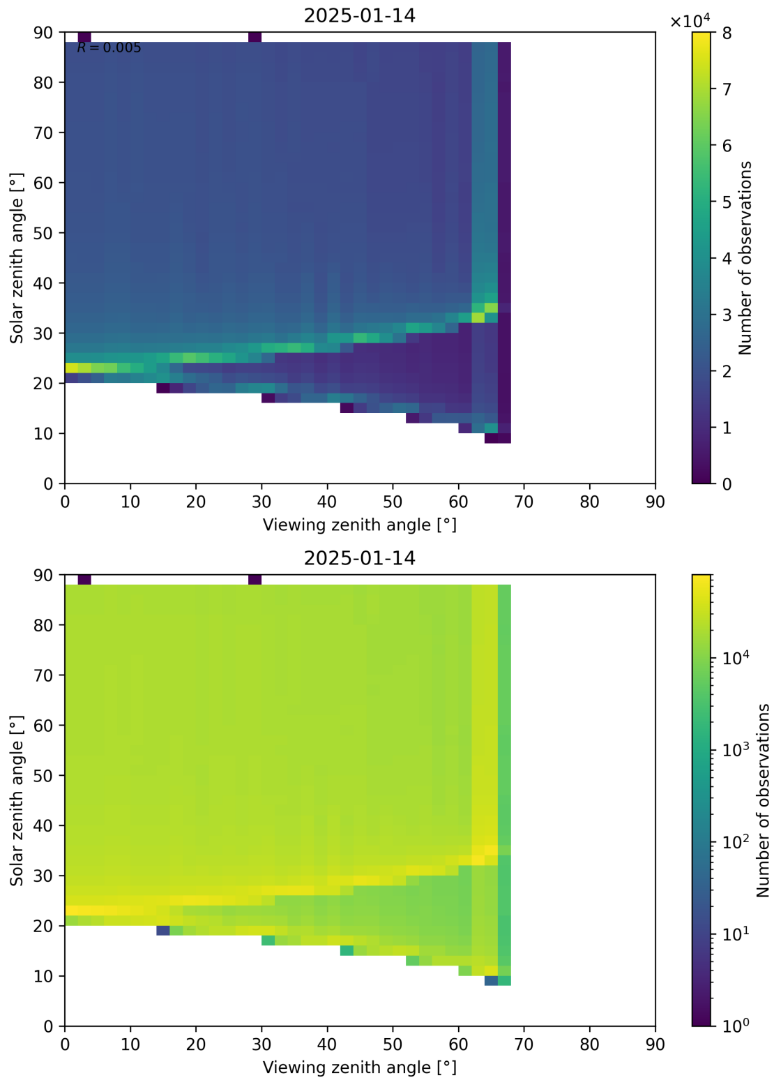
Figure 172: Scatter density plot of “Viewing zenith angle” against “Solar zenith angle” for 2025-01-13 to 2025-01-15.
