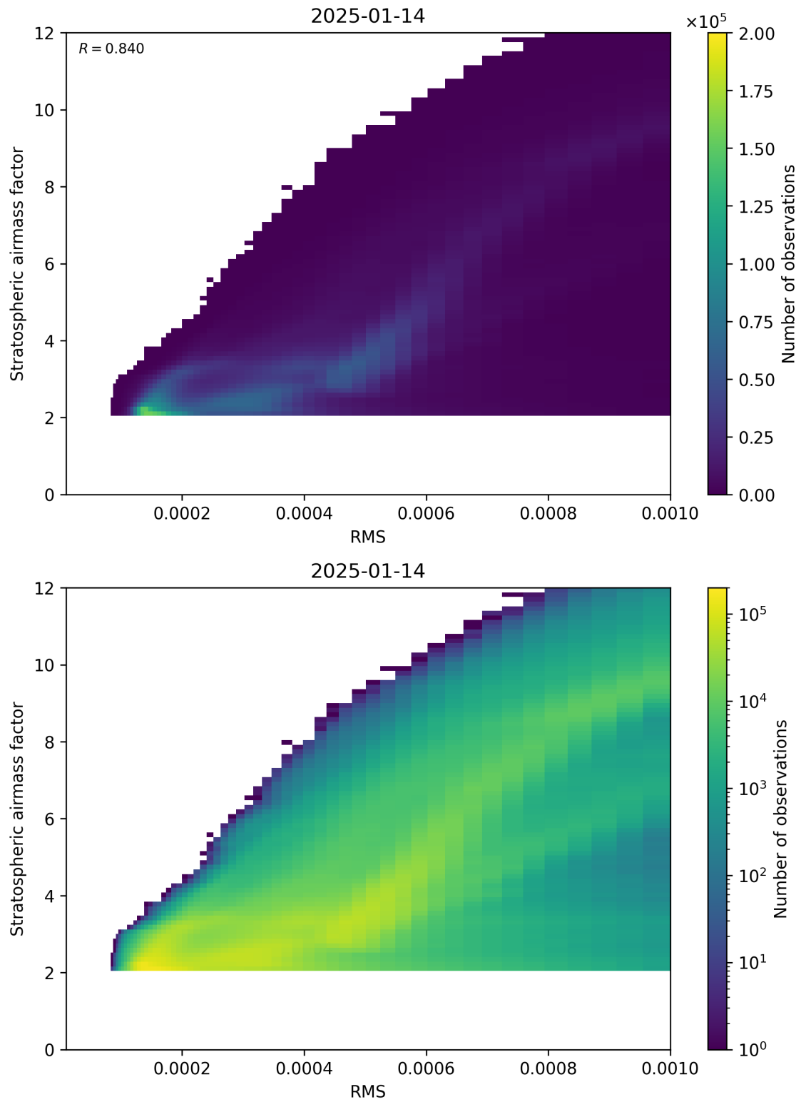
Figure 144: Scatter density plot of “RMS” against “Stratospheric airmass factor” for 2025-01-13 to 2025-01-15.
