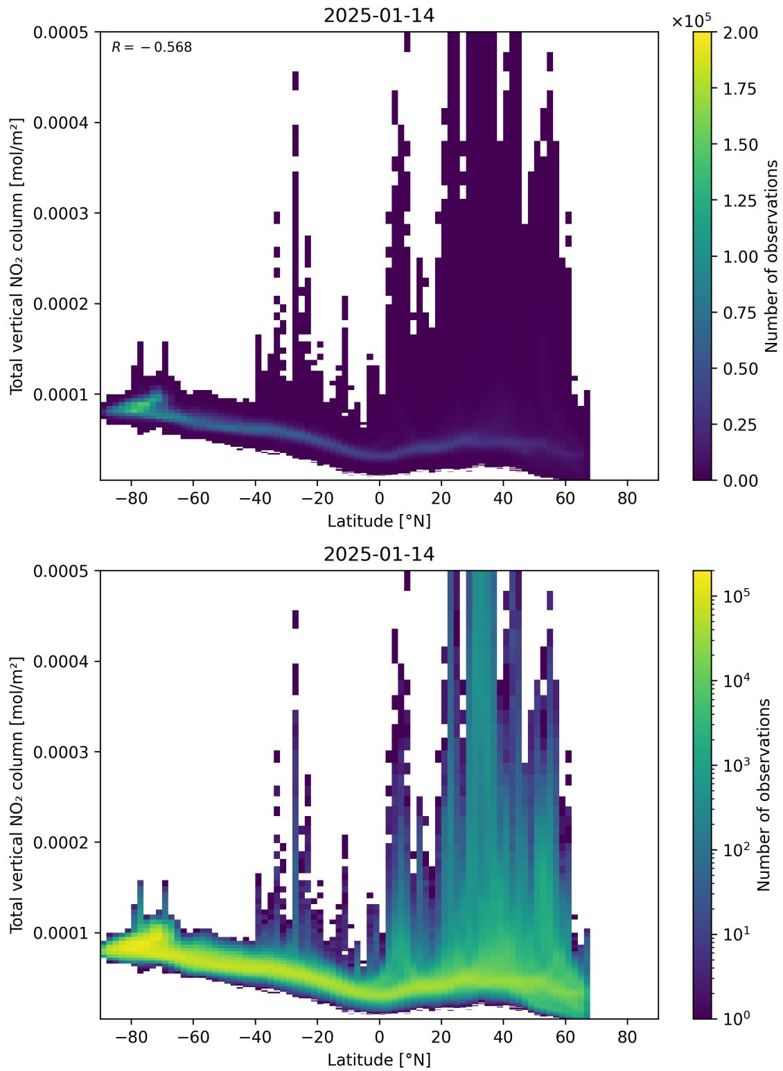
Figure 90: Scatter density plot of “Latitude” against “Total vertical NO 2 column” for 2025-01-13 to 2025-01-15.
