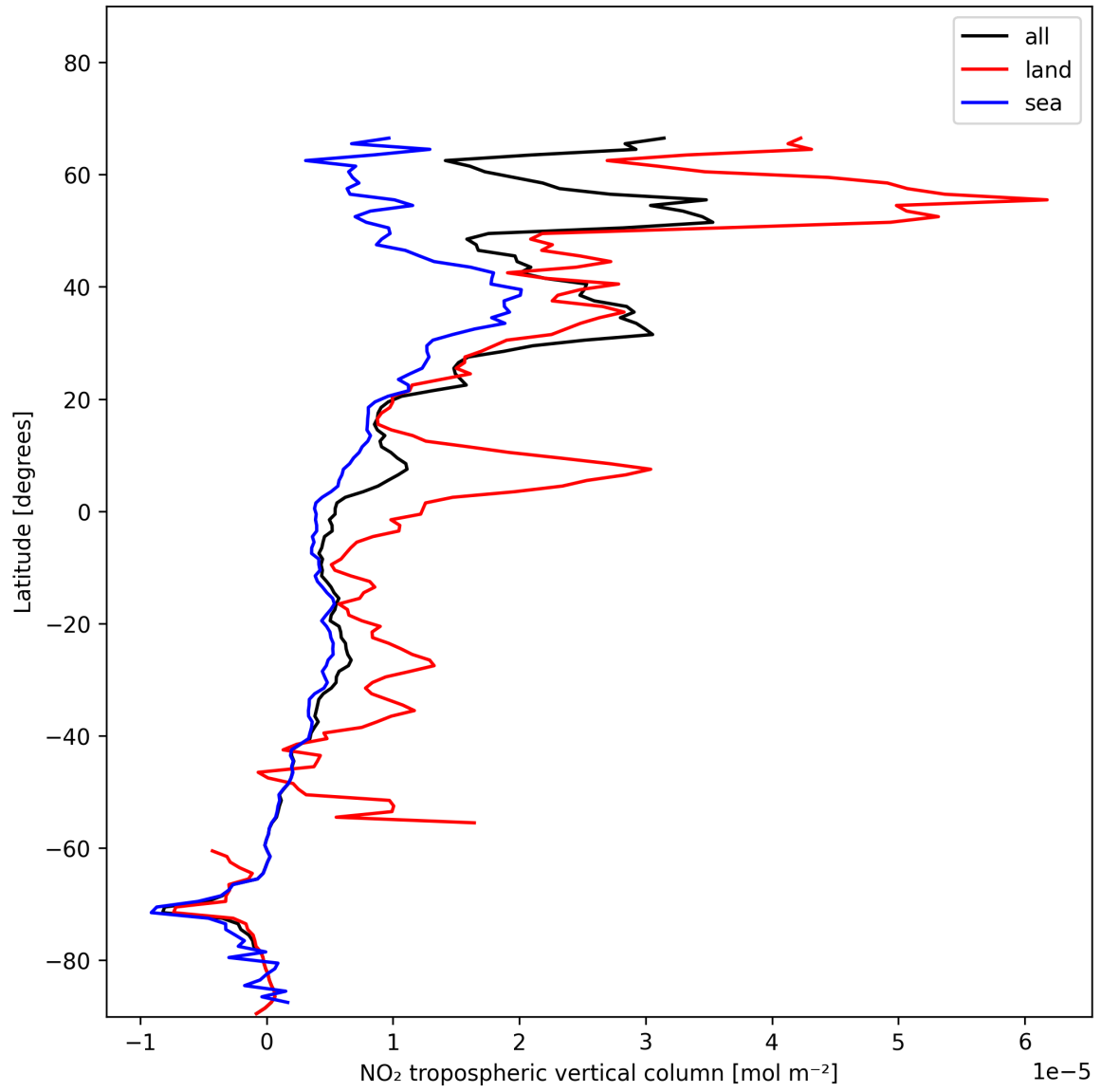
Figure 12: Zonal average of “NO 2 tropospheric vertical column” for 2025-01-13 to 2025-01-15.
