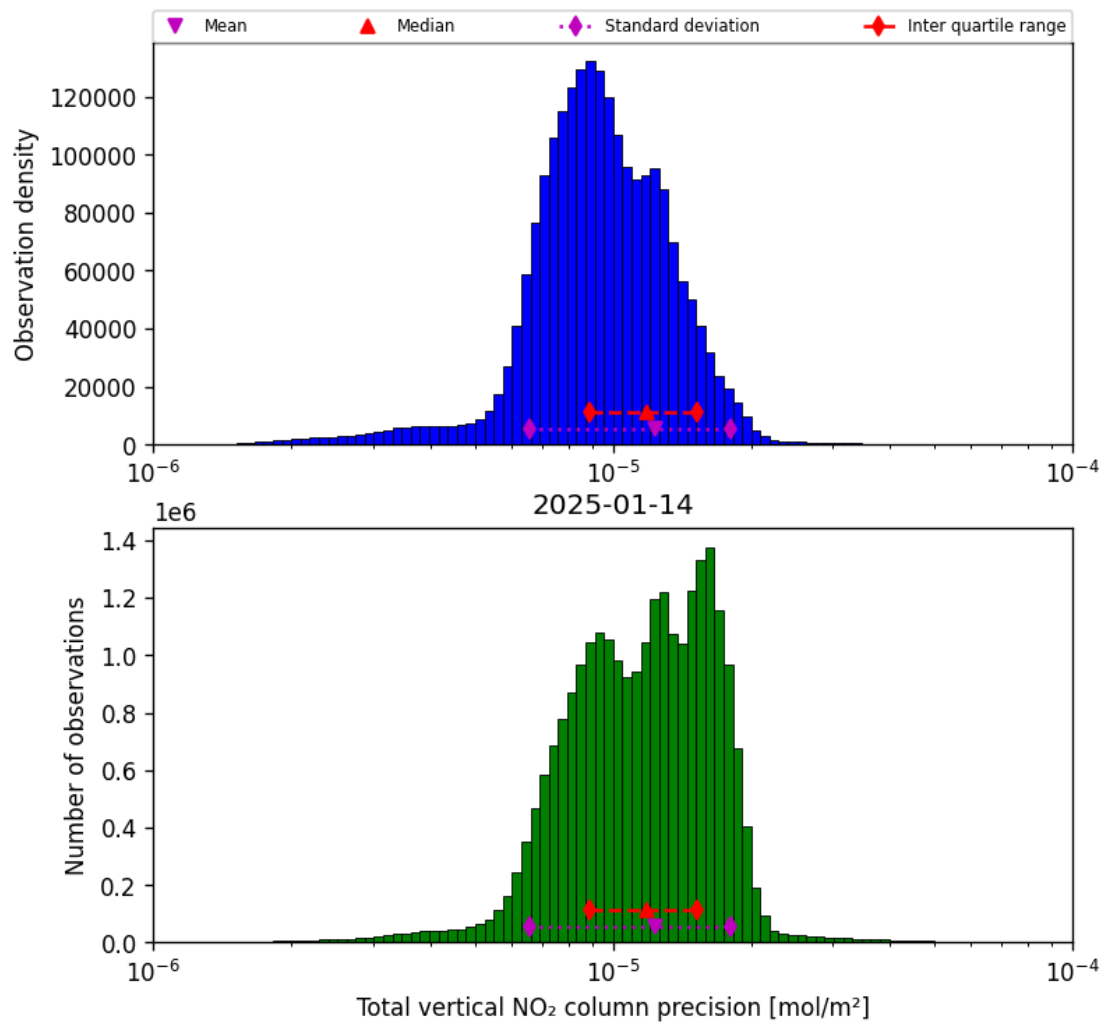
Figure 39: Histogram of “Total vertical NO 2 column precision” for 2025-01-13 to 2025-01-15
