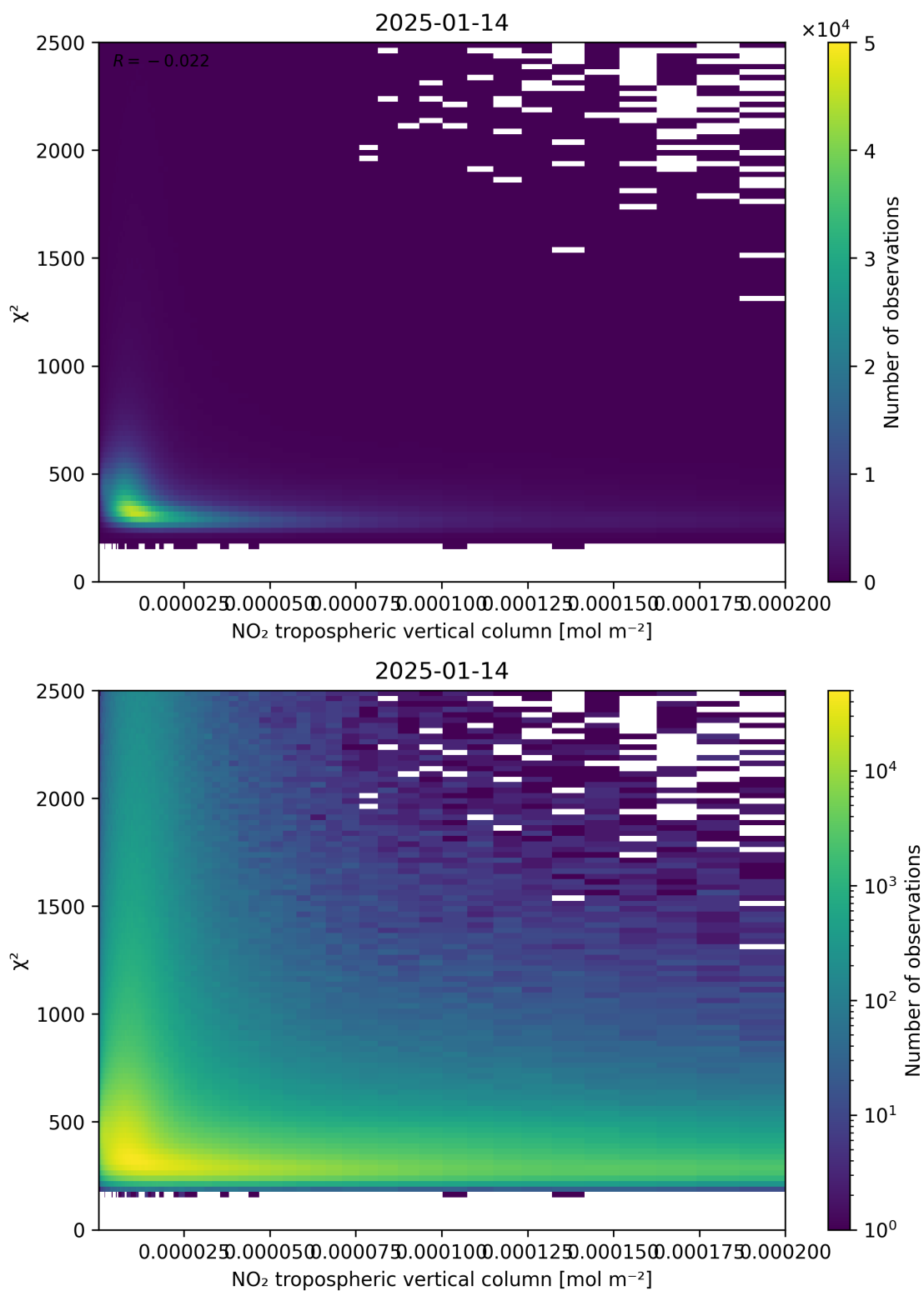
Figure 124: Scatter density plot of “NO 2 tropospheric vertical column” against “ \chi^2 ” for 2025-01-13 to 2025-01-15.
