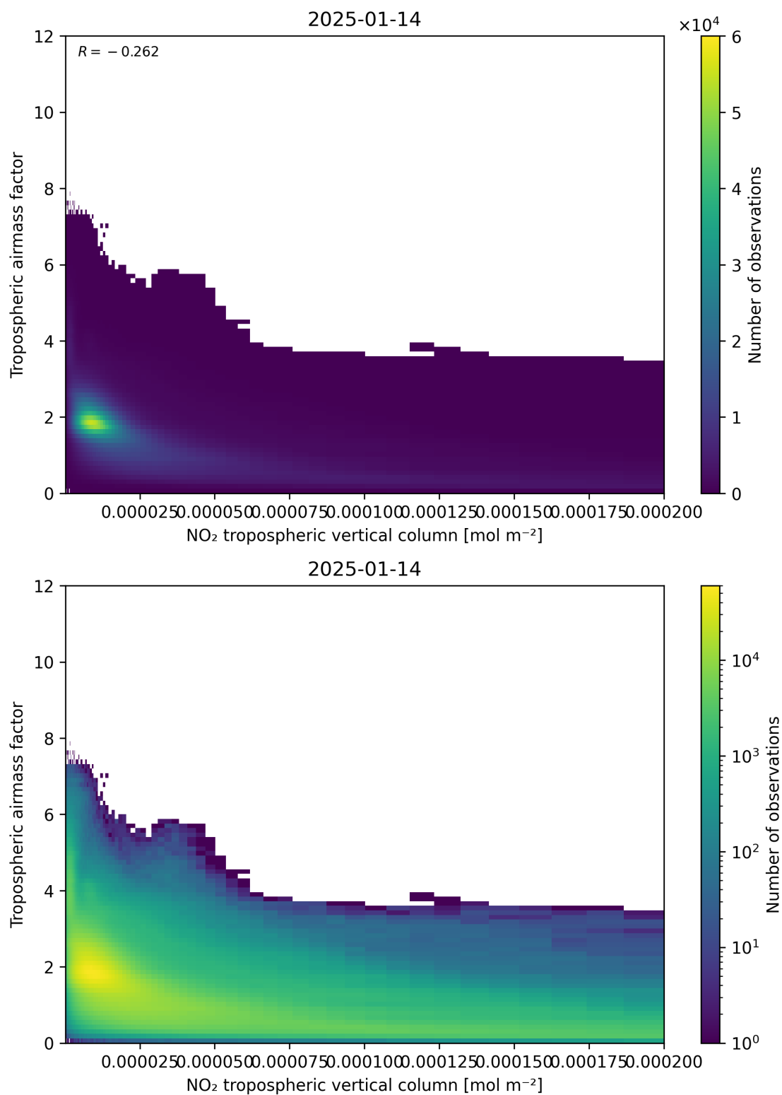
Figure 123: Scatter density plot of “NO 2 tropospheric vertical column” against “Tropospheric air mass factor” for 2025-01-13 to 2025-01-15.
