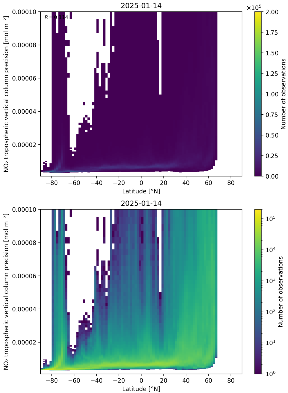
Figure 93: Scatter density plot of “Latitude” against “NO 2 tropospheric vertical column precision” for 2025-01-13 to 2025-01-15.
