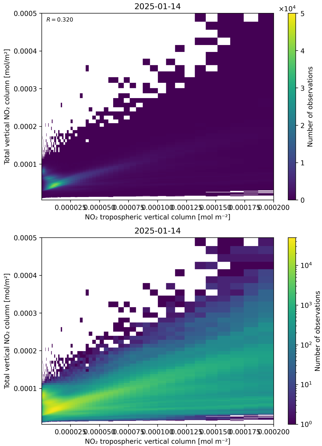
Figure 128: Scatter density plot of “NO 2 tropospheric vertical column” against “Total vertical NO 2 column” for 2025-01-13 to 2025-01-15.
