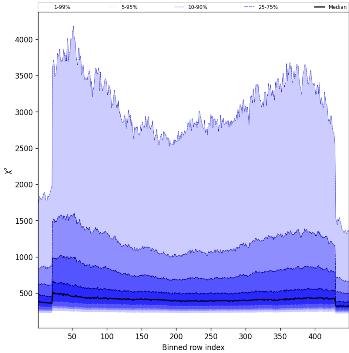
Figure 59: Along track statistics of “ \chi^2 ” for 2025-01-13 to 2025-01-15
