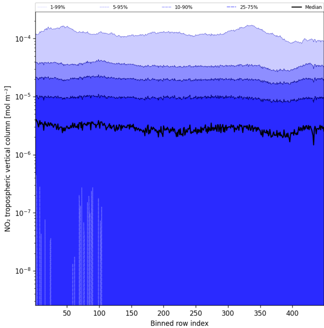
Figure 46: Along track statistics of “NO 2 tropospheric vertical column” for 2025-01-13 to 2025-01-15
