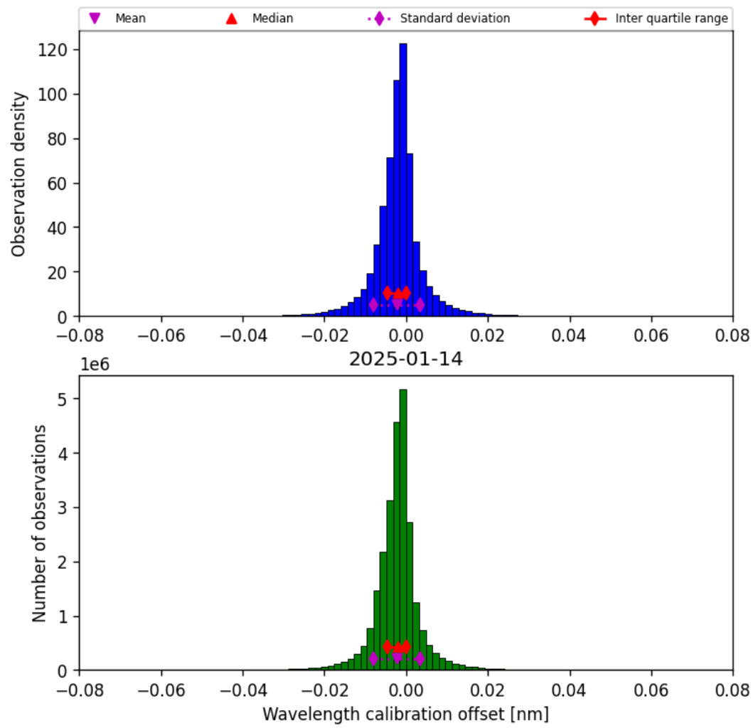
Figure 35: Histogram of “Wavelength calibration offset” for 2025-01-13 to 2025-01-15
