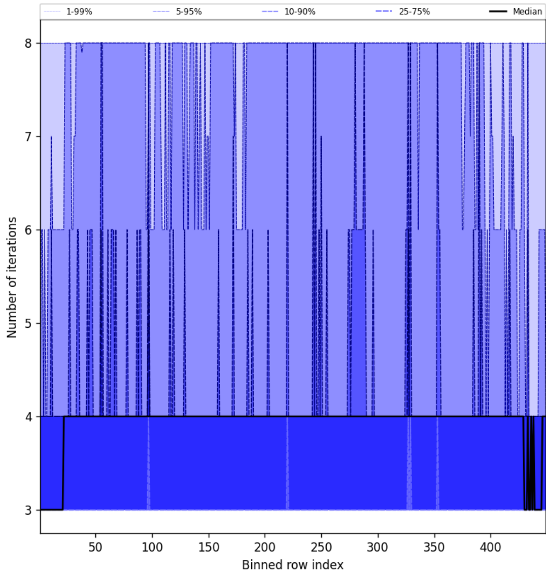
Figure 51: Along track statistics of “Number of iterations” for 2025-01-13 to 2025-01-15
