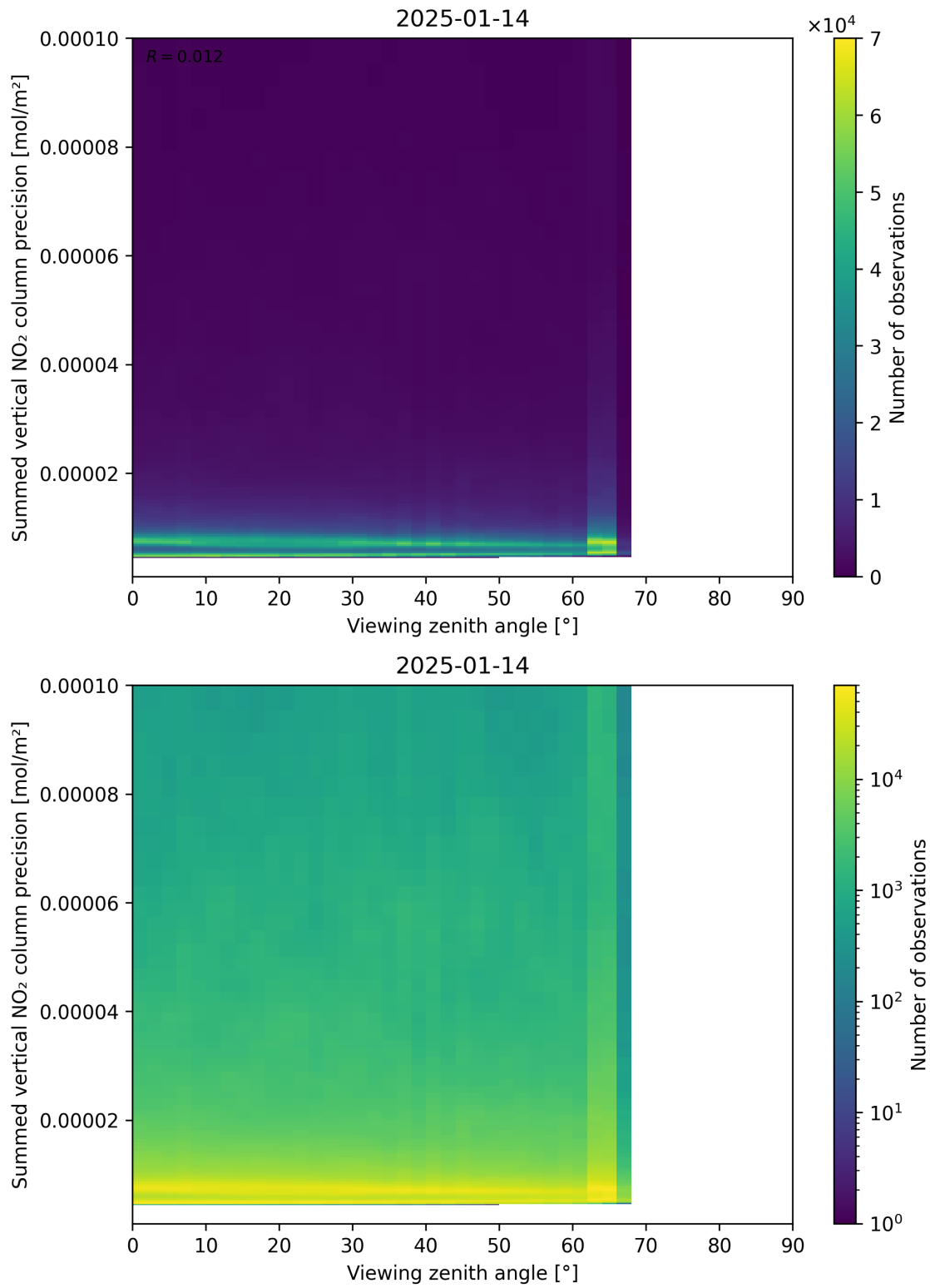
Figure 166: Scatter density plot of “Viewing zenith angle” against “Summed vertical NO 2 column precision” for 2025-01-13 to 2025-01-15.
