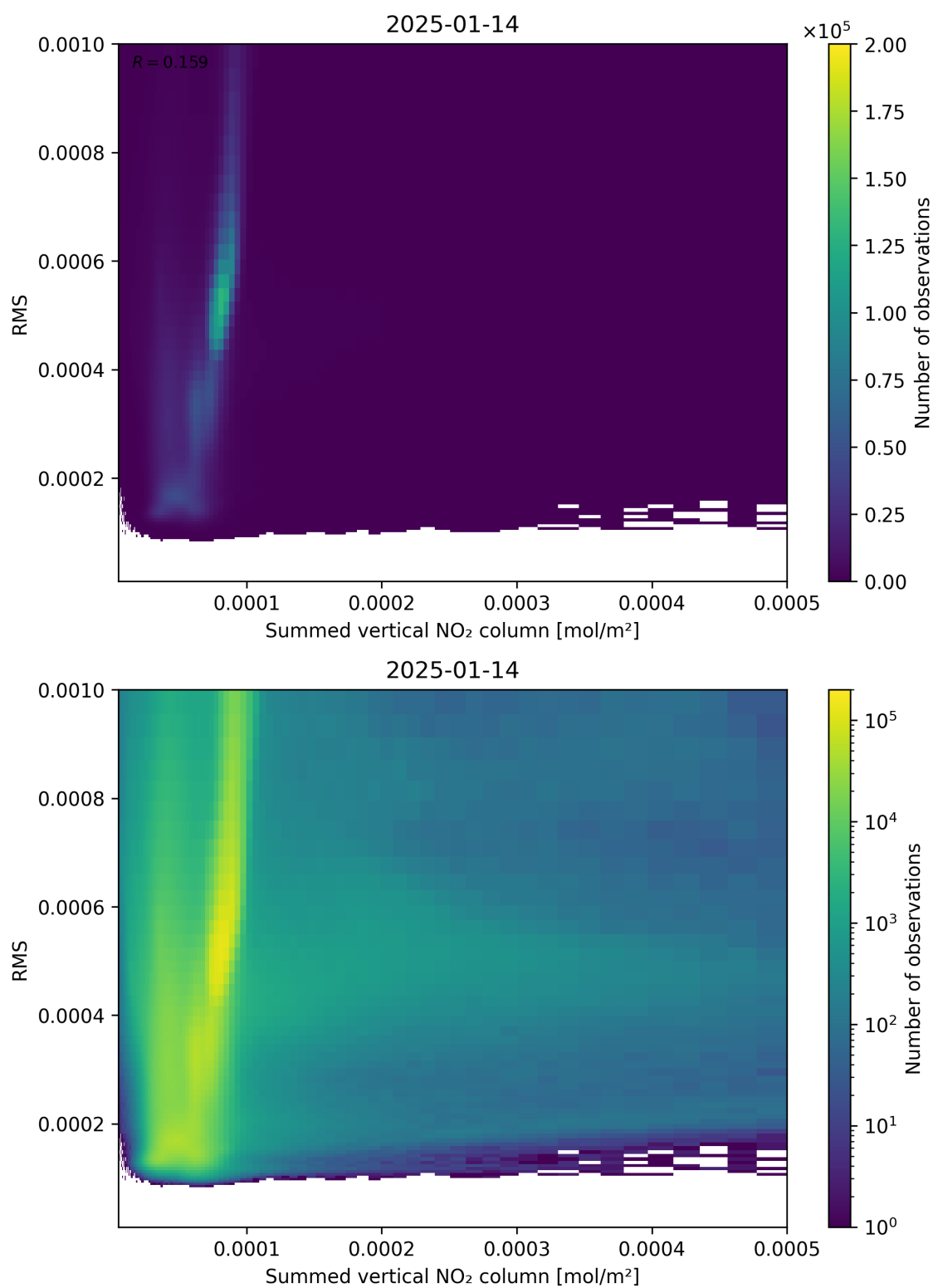
Figure 109: Scatter density plot of “Summed vertical NO 2 column” against “RMS” for 2025-01-13 to 2025-01-15.
