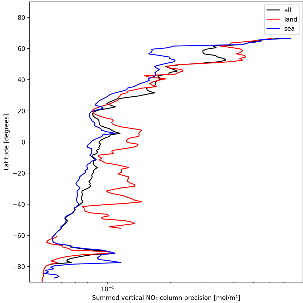
Figure 24: Zonal average of “Summed vertical NO 2 column precision” for 2025-01-13 to 2025-01-15.
