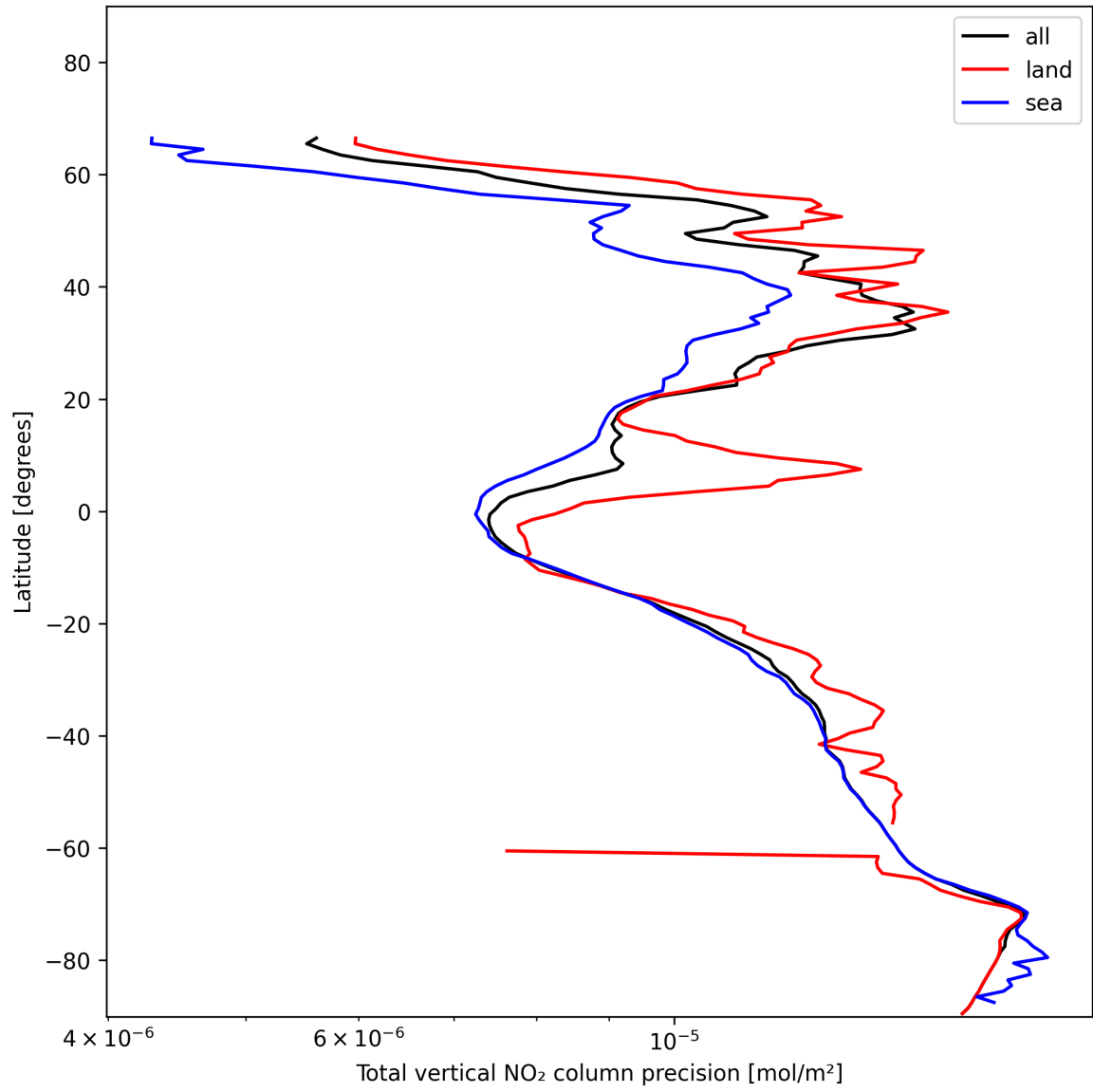
Figure 22: Zonal average of “Total vertical NO 2 column precision” for 2025-01-13 to 2025-01-15.
