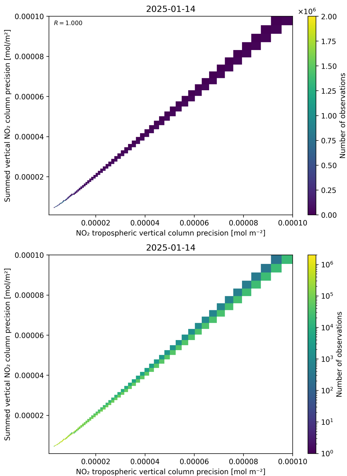
Figure 137: Scatter density plot of “NO 2 tropospheric vertical column precision” against “Summed vertical NO 2 column precision” for 2025-01-13 to 2025-01-15.
