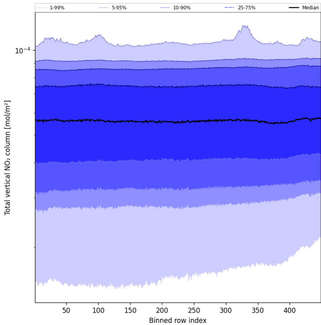
Figure 55: Along track statistics of “Total vertical NO 2 column” for 2025-01-13 to 2025-01-15
