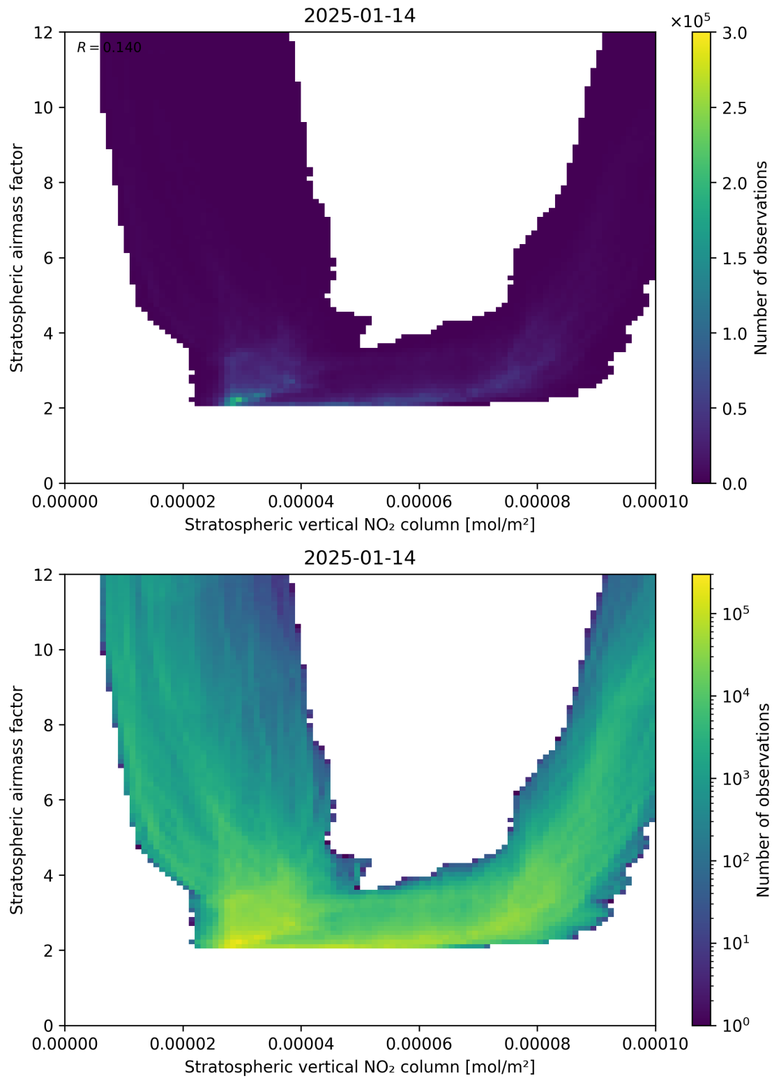
Figure 96: Scatter density plot of “Stratospheric vertical NO 2 column” against “Stratospheric airmass factor” for 2025-01-13 to 2025-01-15.
