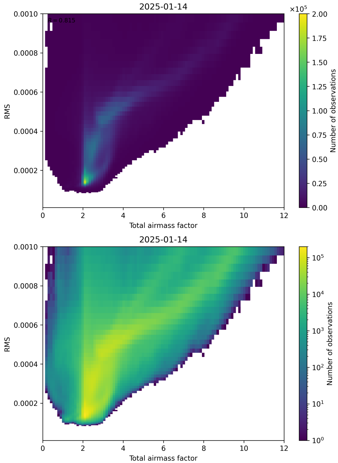
Figure 69: Scatter density plot of “Total airmass factor” against “RMS” for 2025-01-13 to 2025-01-15.
