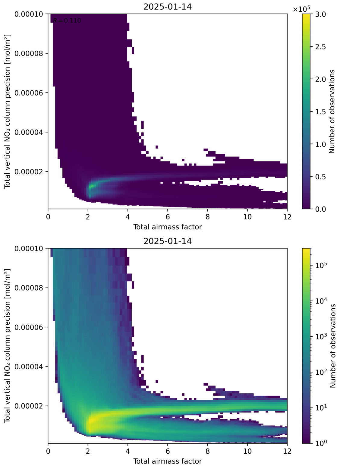
Figure 68: Scatter density plot of “Total airmass factor” against “Total vertical NO 2 column precision” for 2025-01-13 to 2025-01-15.
