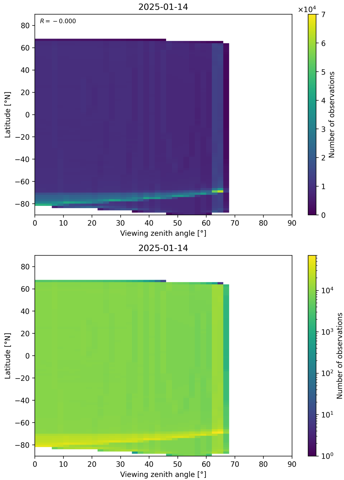
Figure 163: Scatter density plot of “Viewing zenith angle” against “Latitude” for 2025-01-13 to 2025-01-15.
