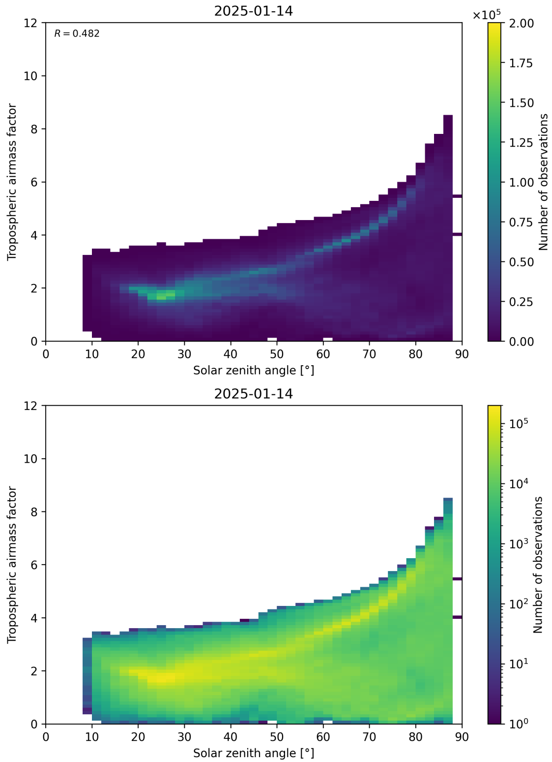
Figure 147: Scatter density plot of “Solar zenith angle” against “Tropospheric airmass factor” for 2025-01-13 to 2025-01-15.
