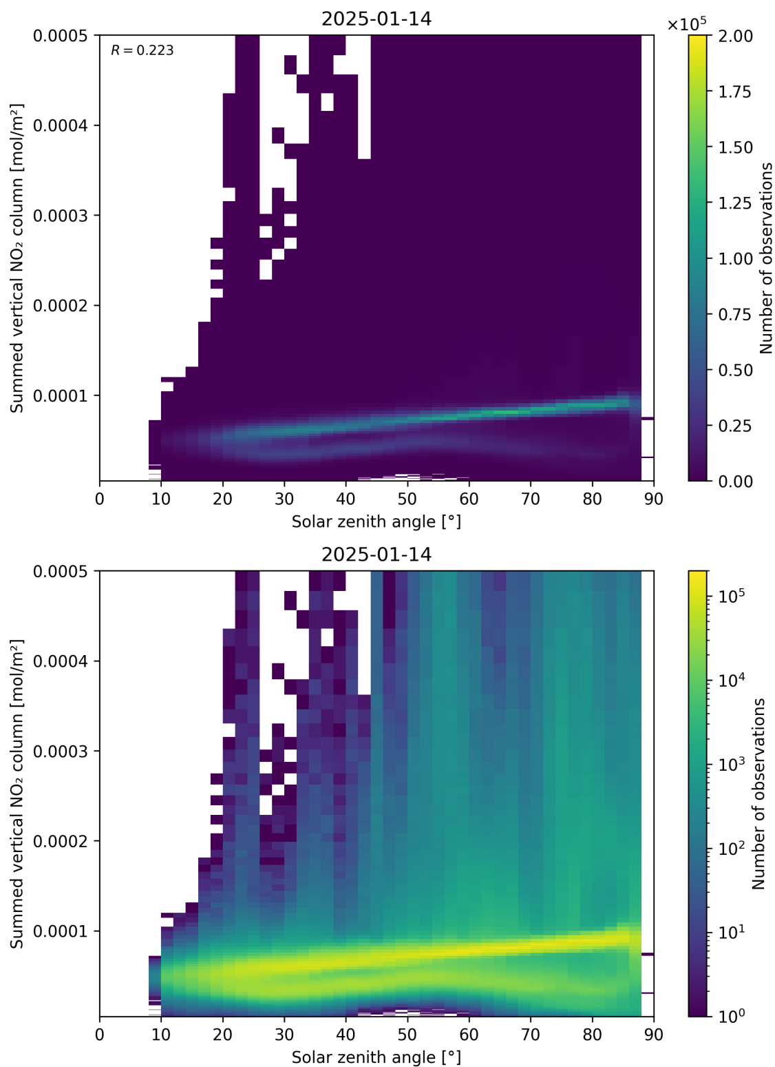
Figure 151: Scatter density plot of “Solar zenith angle” against “Summed vertical NO 2 column” for 2025-01-13 to 2025-01-15.
