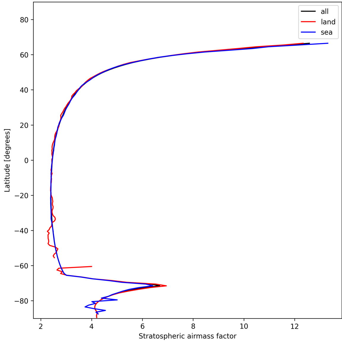
Figure 27: Zonal average of “Stratospheric air mass factor” for 2025-01-13 to 2025-01-15.
