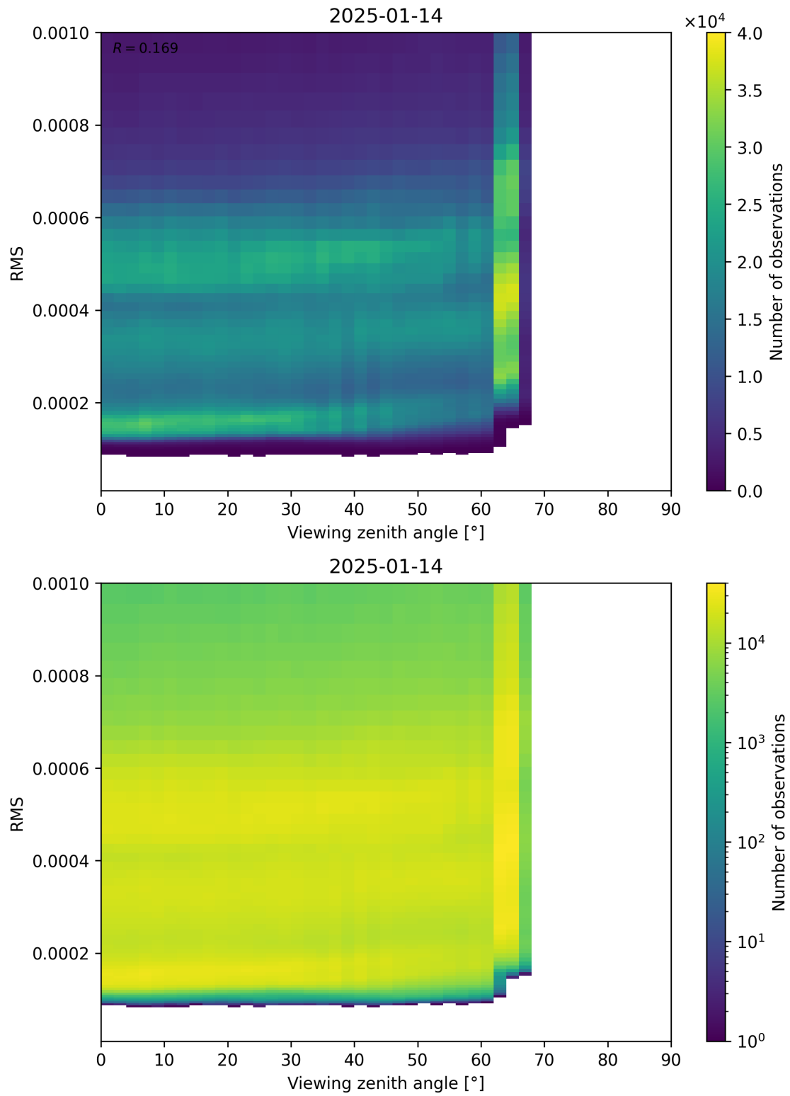
Figure 171: Scatter density plot of “Viewing zenith angle” against “RMS” for 2025-01-13 to 2025-01-15.
