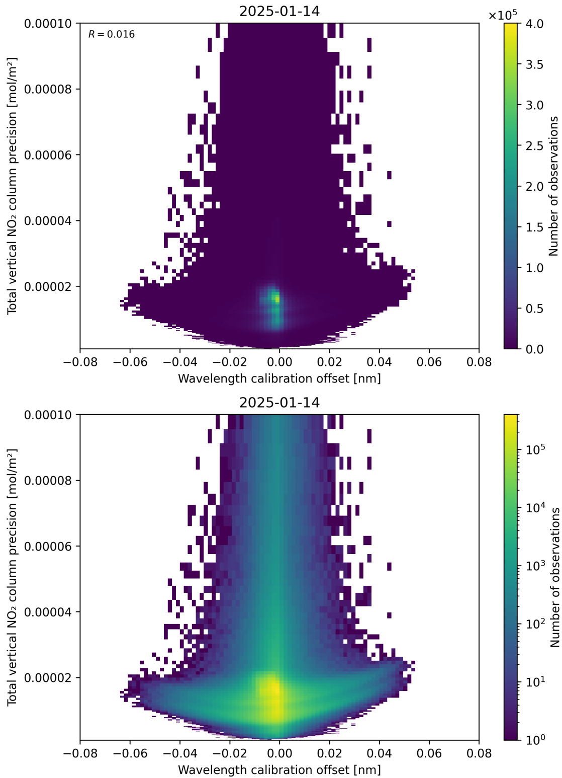
Figure 180: Scatter density plot of “Wavelength calibration offset” against “Total vertical NO 2 column precision” for 2025-01-13 to 2025-01-15.
