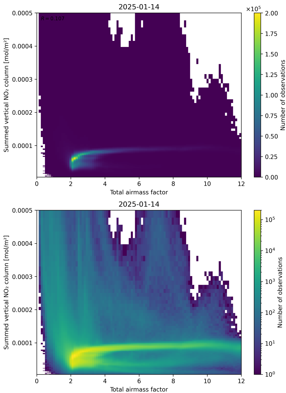
Figure 65: Scatter density plot of “Total airmass factor” against “Summed vertical NO 2 column” for 2025-01-13 to 2025-01-15.
