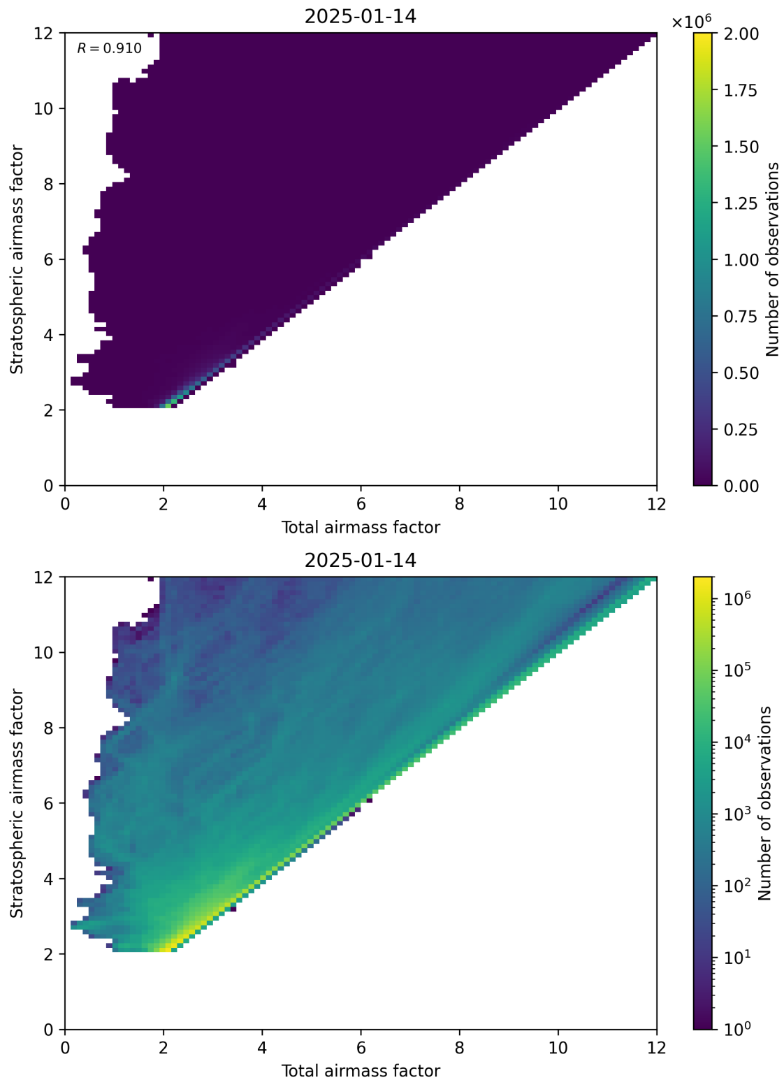
Figure 62: Scatter density plot of “Total airmass factor” against “Stratospheric airmass factor” for 2025-01-13 to 2025-01-15.
