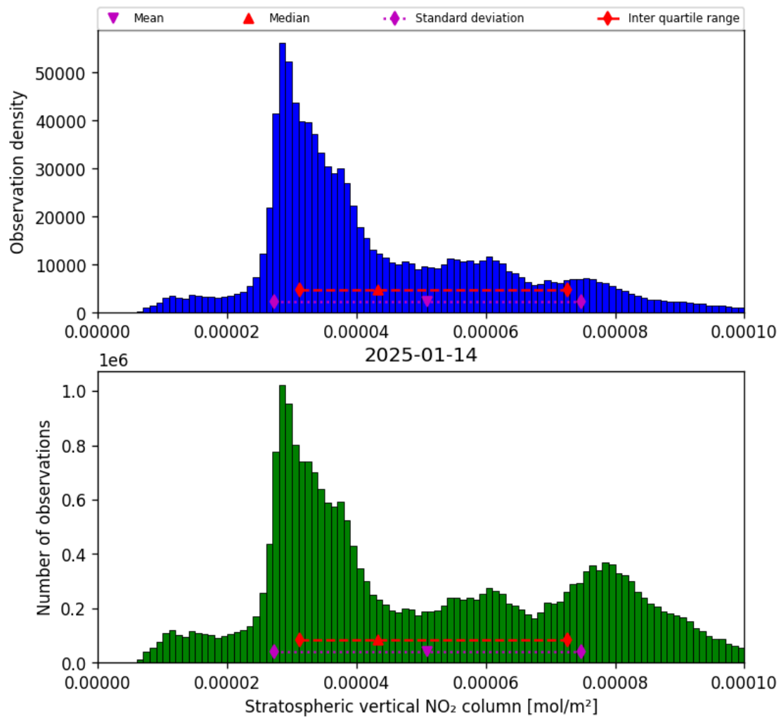
Figure 36: Histogram of “Stratospheric vertical NO 2 column” for 2025-01-13 to 2025-01-15
