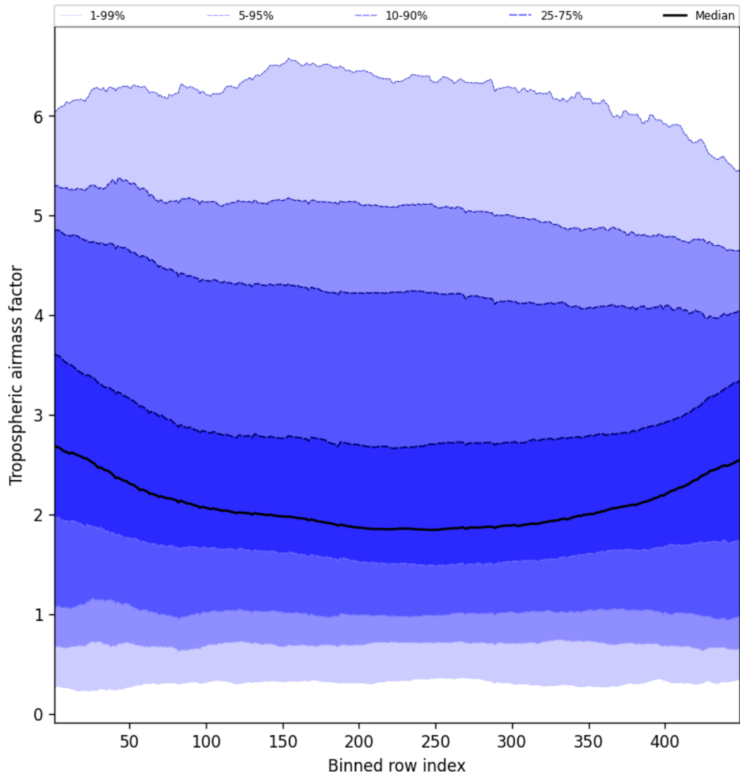
Figure 48: Along track statistics of “Tropospheric air mass factor” for 2025-01-13 to 2025-01-15
