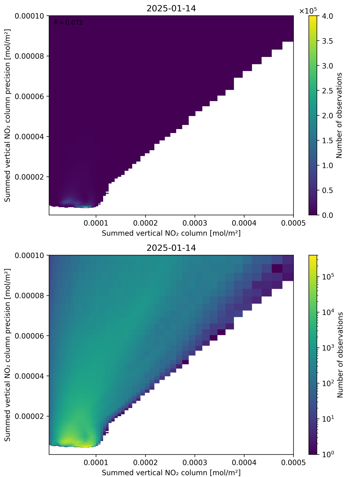
Figure 105: Scatter density plot of “Summed vertical NO 2 column” against “Summed vertical NO 2 column precision” for 2025-01-13 to 2025-01-15.
