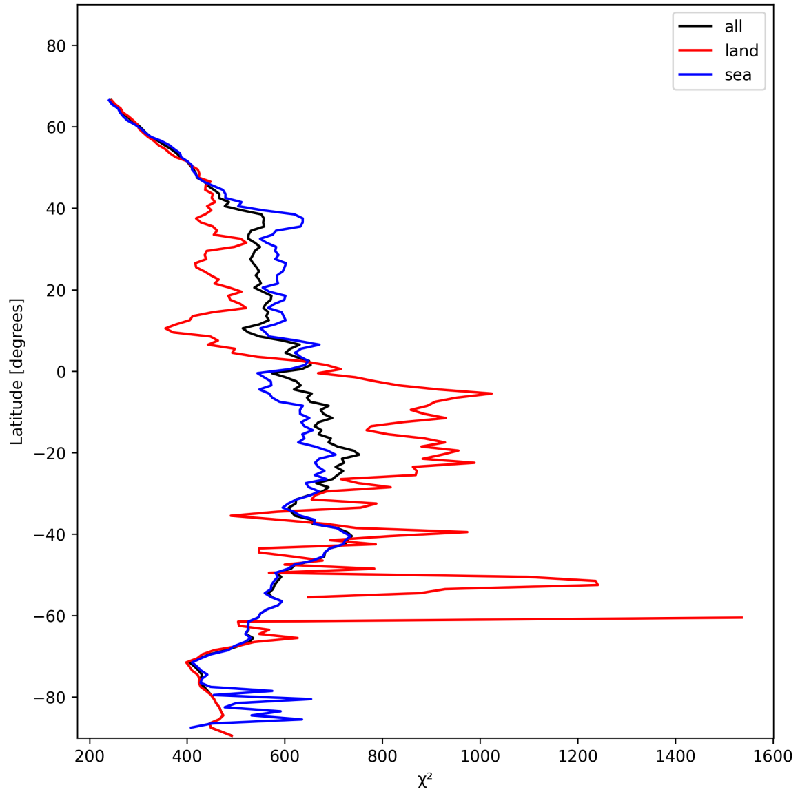
Figure 25: Zonal average of “ \chi^2 ” for 2025-01-13 to 2025-01-15.
