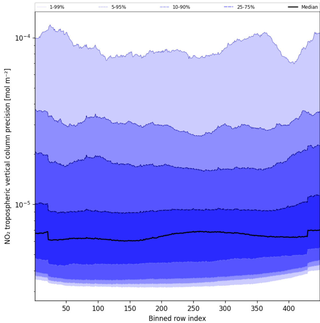
Figure 47: Along track statistics of “NO 2 tropospheric vertical column precision” for 2025-01-13 to 2025-01-15
