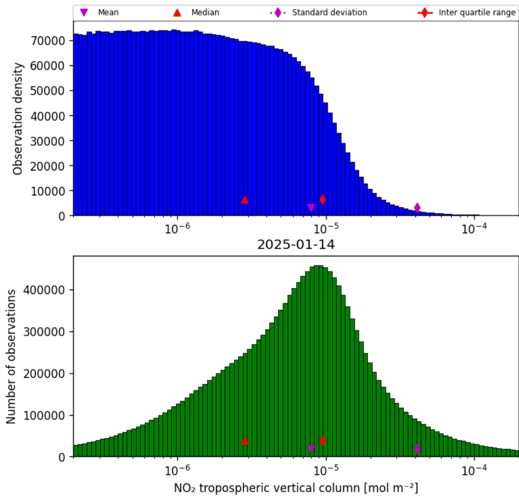
Figure 29: Histogram of “NO 2 tropospheric vertical column” for 2025-01-13 to 2025-01-15
