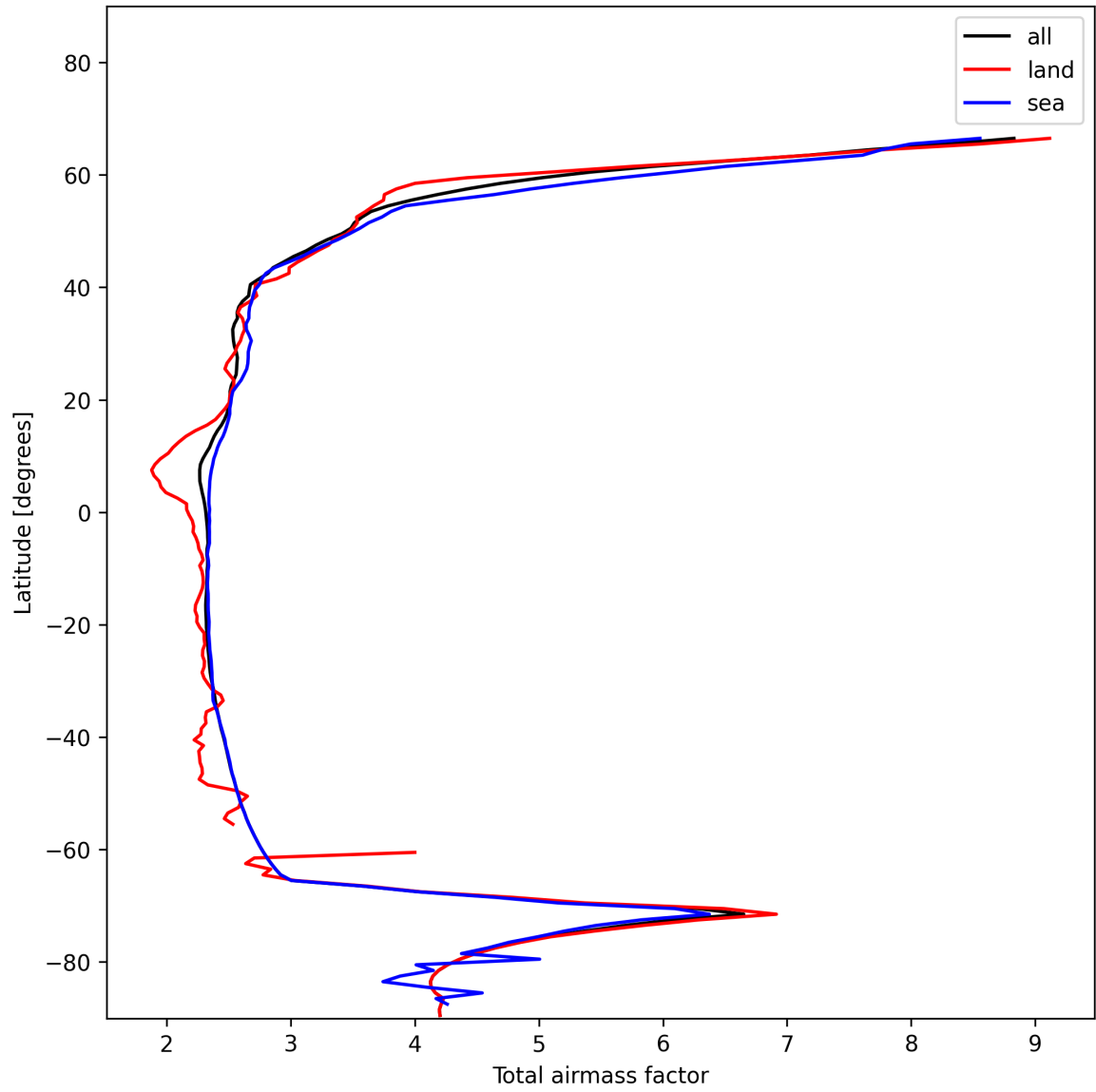
Figure 15: Zonal average of “Total airmass factor” for 2025-01-13 to 2025-01-15.
