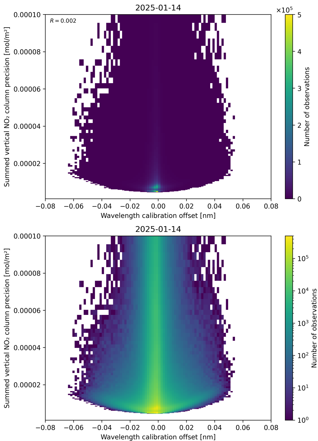
Figure 178: Scatter density plot of “Wavelength calibration offset” against “Summed vertical NO 2 column precision” for 2025-01-13 to 2025-01-15.
