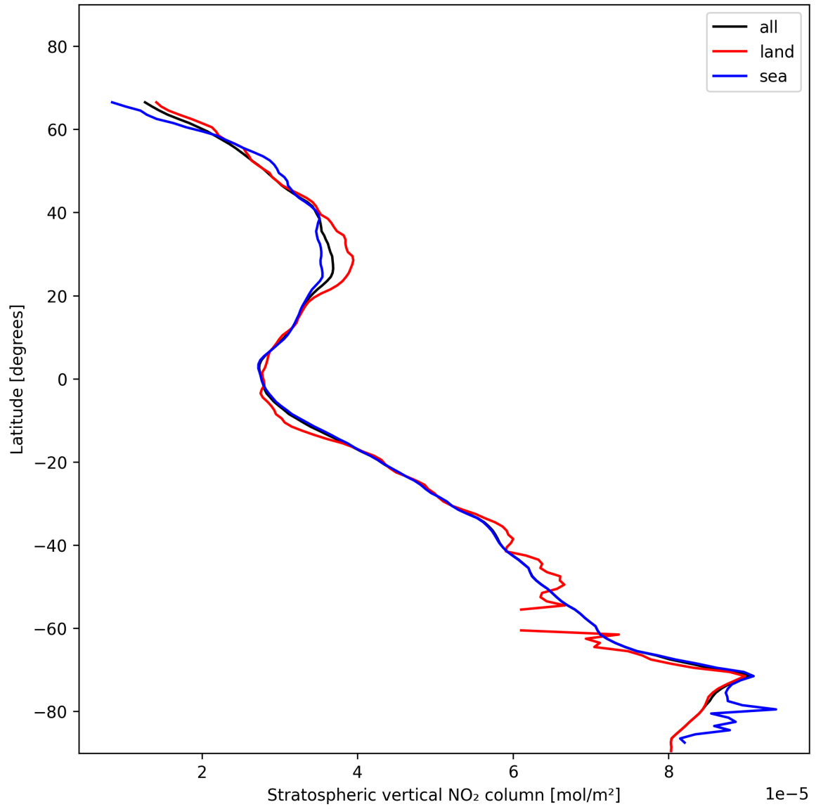
Figure 19: Zonal average of “Stratospheric vertical NO 2 column” for 2025-01-13 to 2025-01-15.
