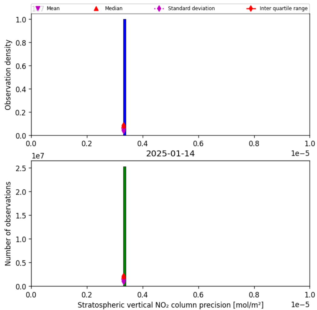
Figure 37: Histogram of “Stratospheric vertical NO 2 column precision” for 2025-01-13 to 2025-01-15
