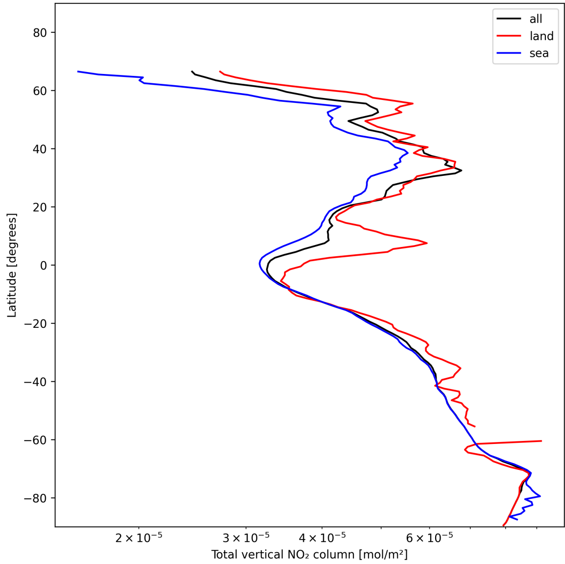
Figure 21: Zonal average of “Total vertical NO 2 column” for 2025-01-13 to 2025-01-15.
