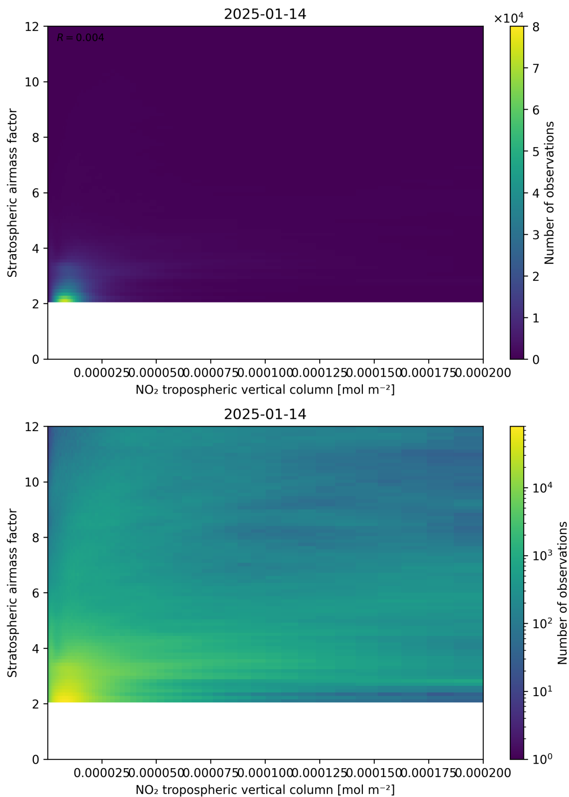
Figure 121: Scatter density plot of “NO 2 tropospheric vertical column” against “Stratospheric airmass factor” for 2025-01-13 to 2025-01-15.
