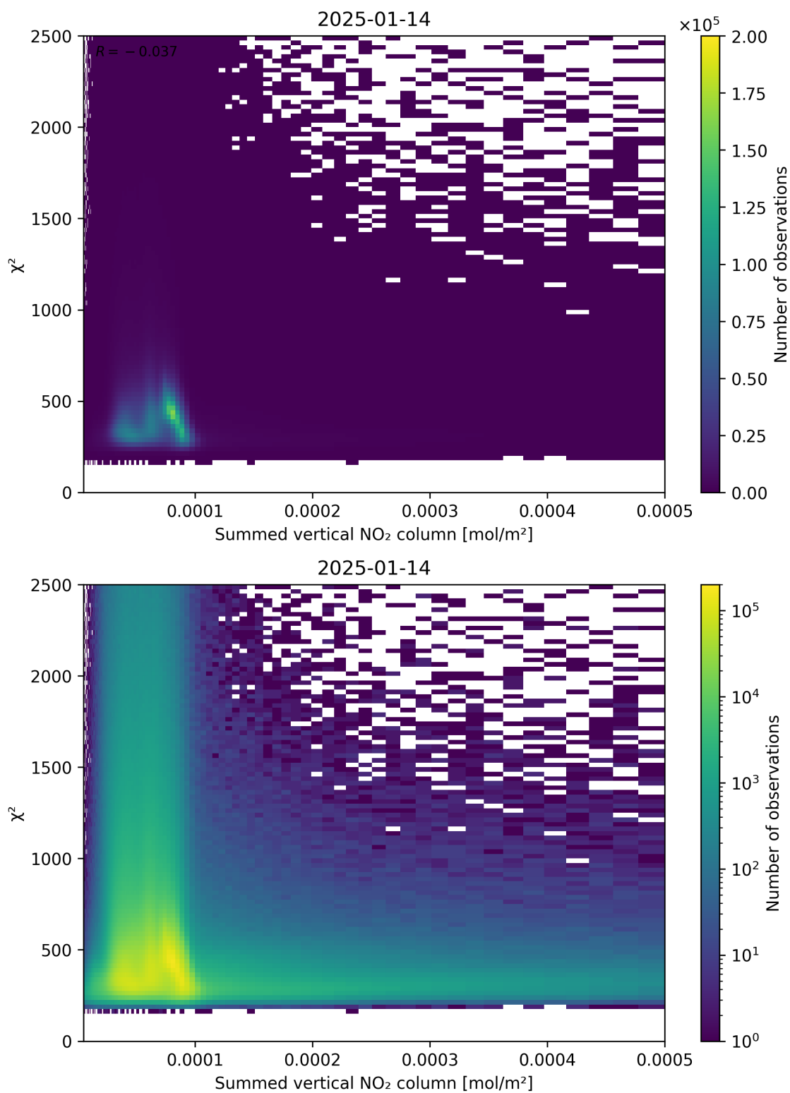
Figure 104: Scatter density plot of “Summed vertical NO 2 column” against “ \chi^2 ” for 2025-01-13 to 2025-01-15.
