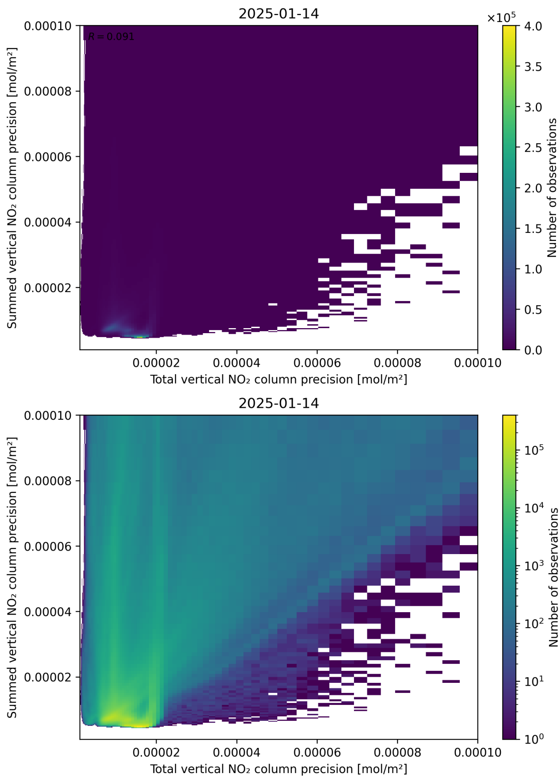
Figure 118: Scatter density plot of “Total vertical NO 2 column precision” against “Summed vertical NO 2 column precision” for 2025-01-13 to 2025-01-15.
