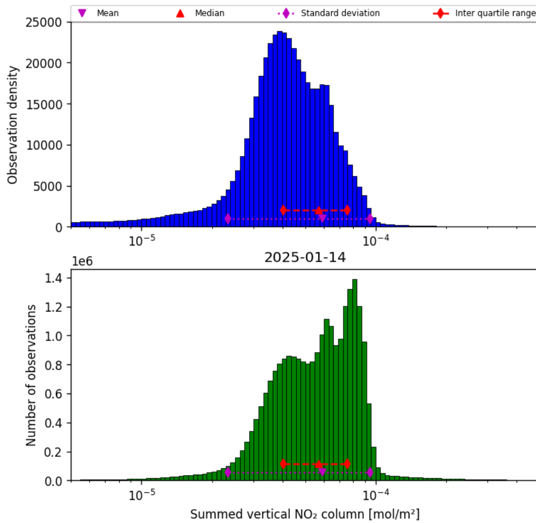
Figure 40: Histogram of “Summed vertical NO 2 column” for 2025-01-13 to 2025-01-15
