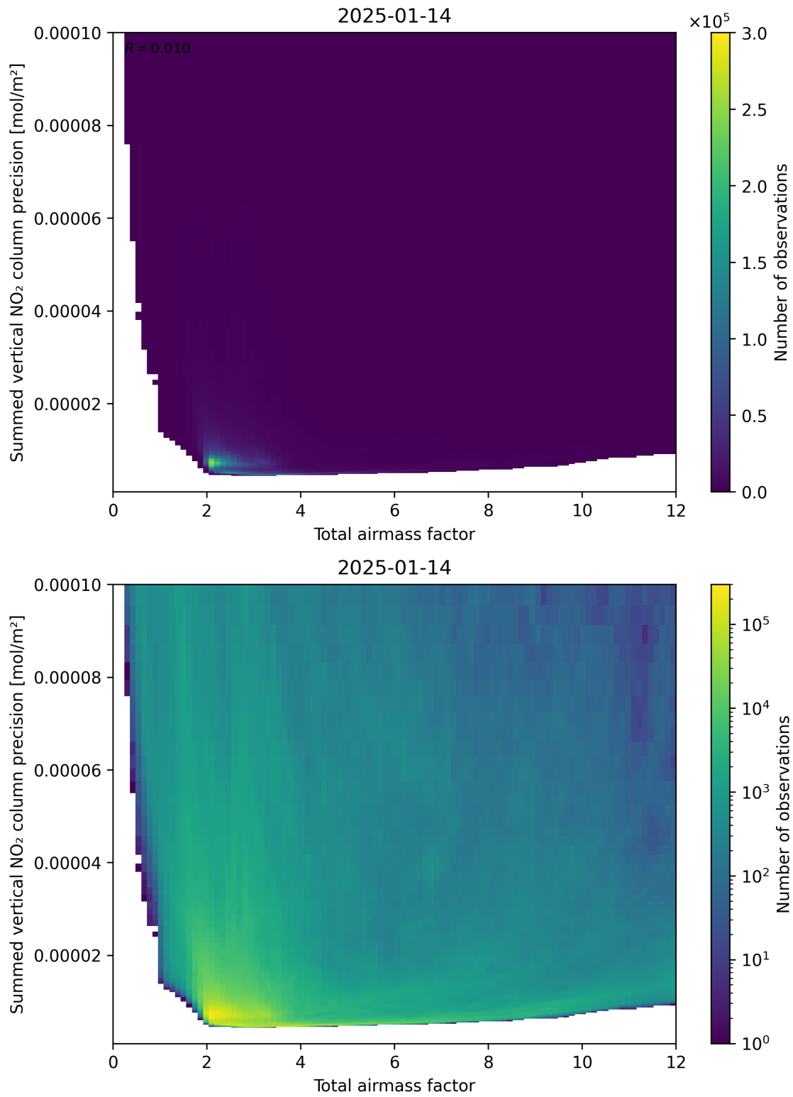
Figure 66: Scatter density plot of “Total airmass factor” against “Summed vertical NO 2 column precision” for 2025-01-13 to 2025-01-15.
