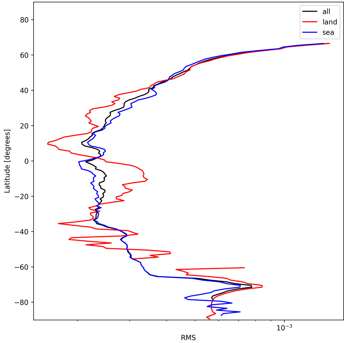
Figure 26: Zonal average of “RMS” for 2025-01-13 to 2025-01-15.
