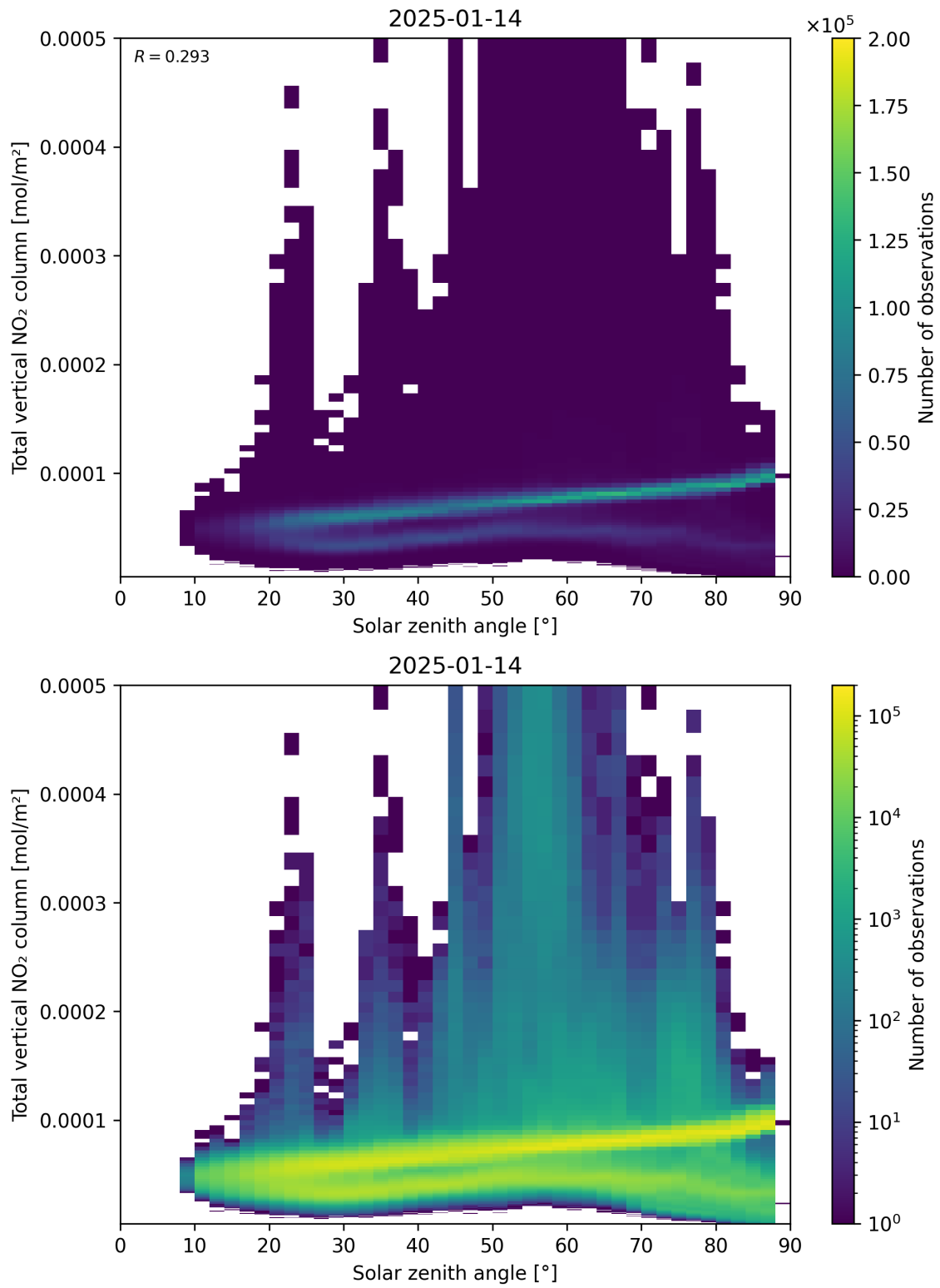
Figure 153: Scatter density plot of “Solar zenith angle” against “Total vertical NO 2 column” for 2025-01-13 to 2025-01-15.
