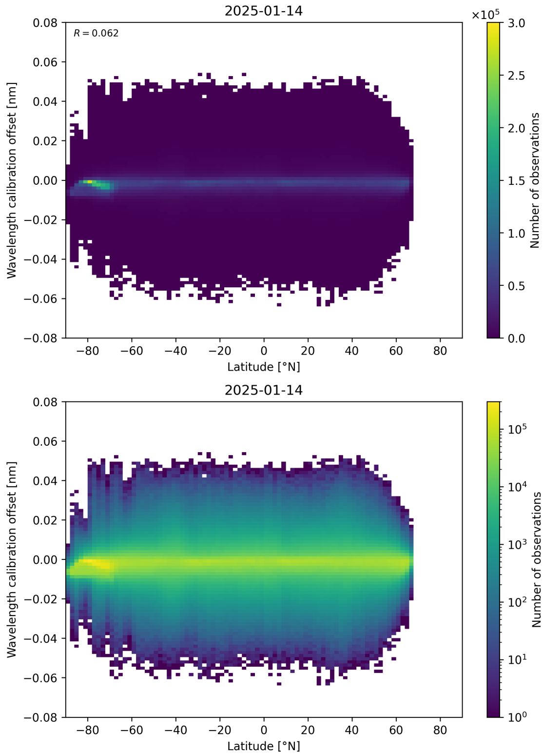
Figure 95: Scatter density plot of “Latitude” against “Wavelength calibration offset” for 2025-01-13 to 2025-01-15.
