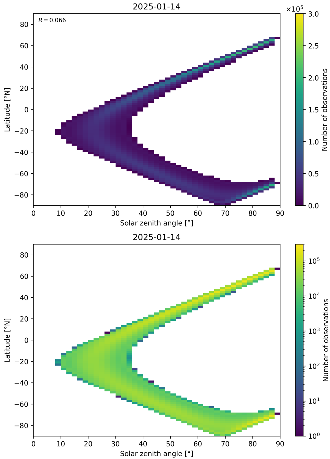
Figure 149: Scatter density plot of “Solar zenith angle” against “Latitude” for 2025-01-13 to 2025-01-15.
