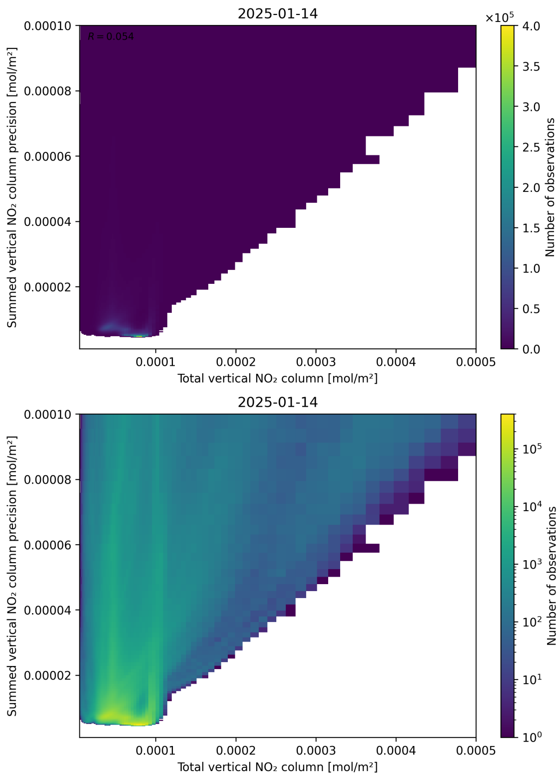
Figure 113: Scatter density plot of “Total vertical NO 2 column” against “Summed vertical NO 2 column precision” for 2025-01-13 to 2025-01-15.
