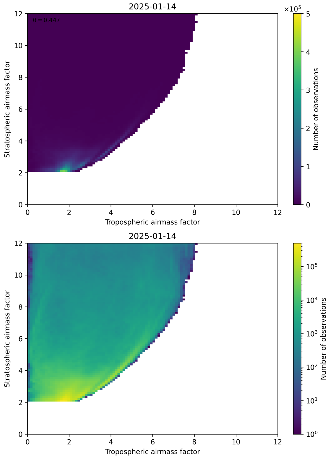
Figure 71: Scatter density plot of “Tropospheric airmass factor” against “Stratospheric airmass factor” for 2025-01-13 to 2025-01-15.
