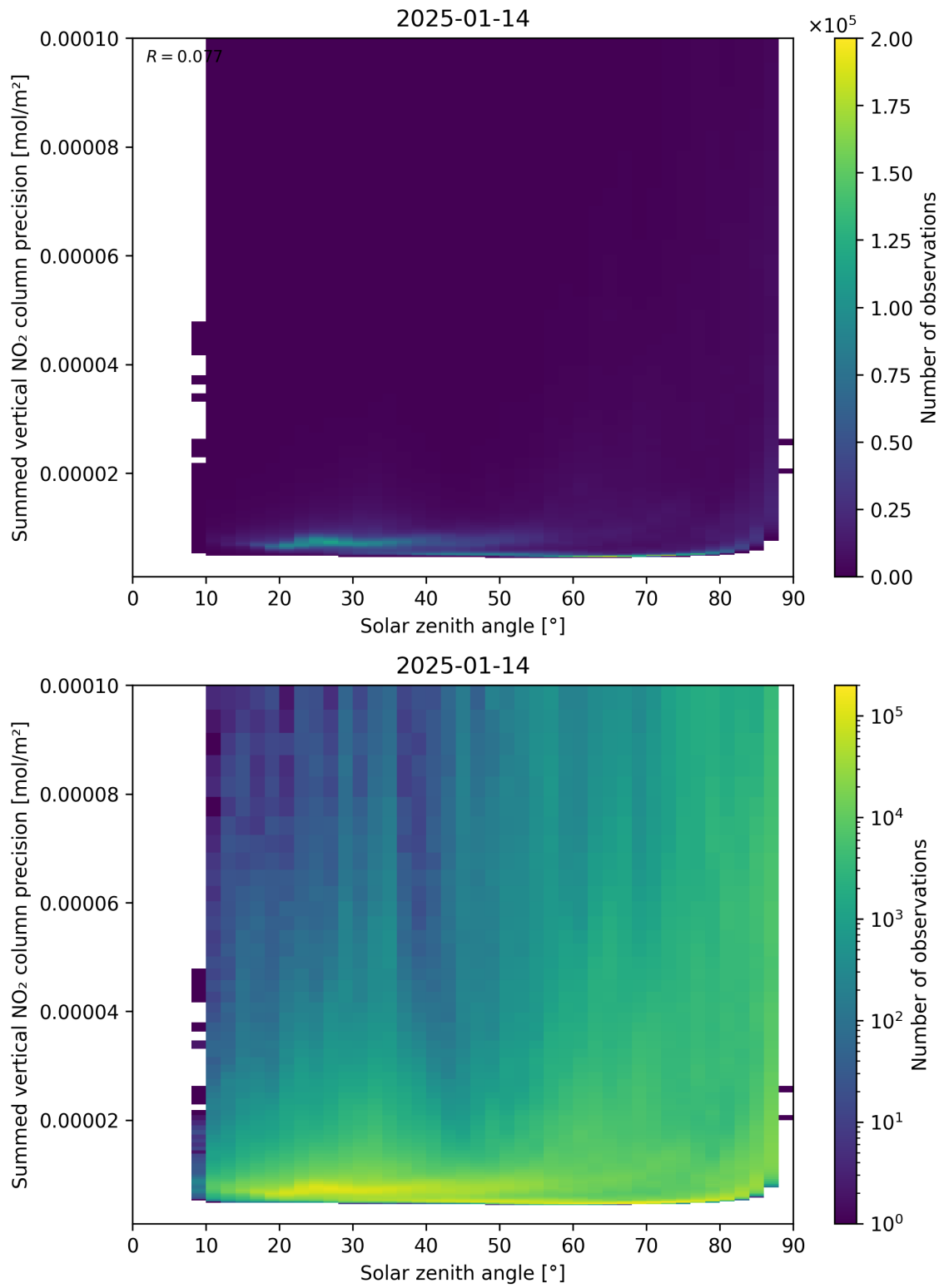
Figure 152: Scatter density plot of “Solar zenith angle” against “Summed vertical NO 2 column precision” for 2025-01-13 to 2025-01-15.
