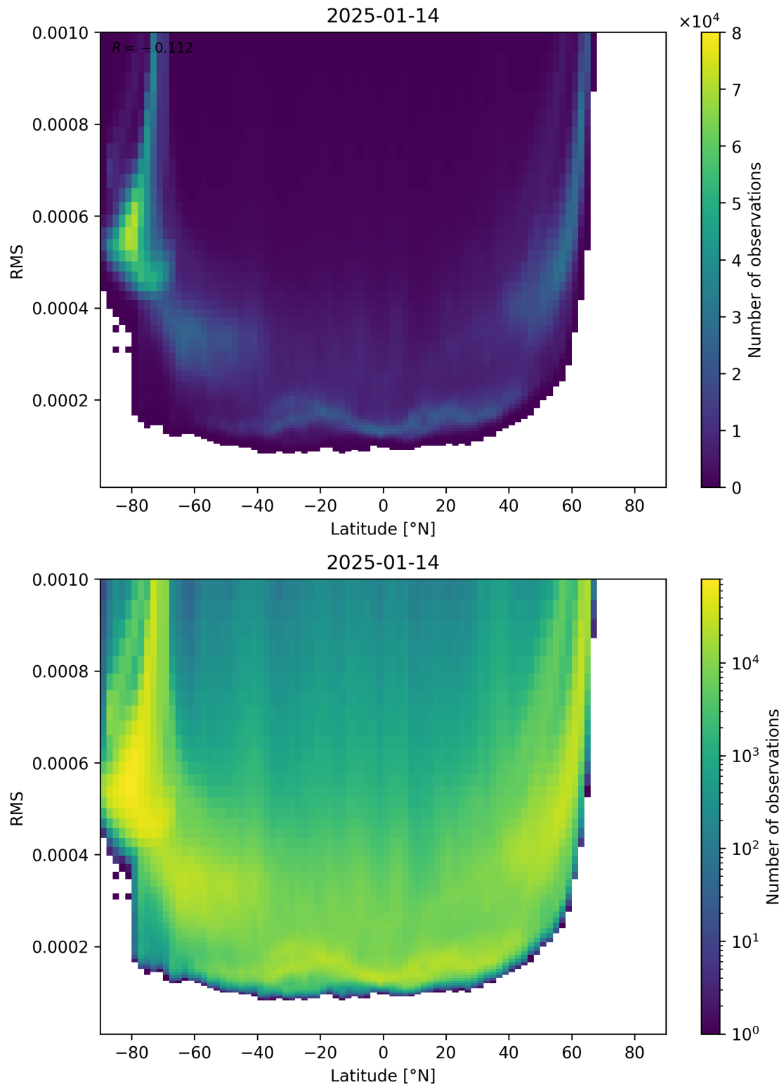
Figure 94: Scatter density plot of “Latitude” against “RMS” for 2025-01-13 to 2025-01-15.
