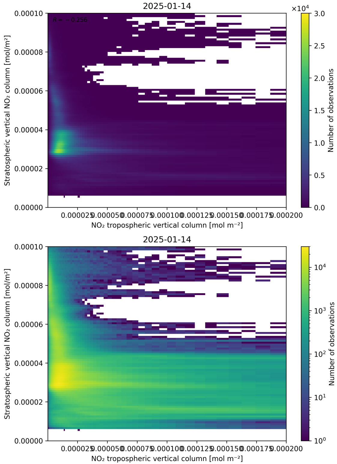
Figure 125: Scatter density plot of “NO 2 tropospheric vertical column” against “Stratospheric vertical NO 2 column” for 2025-01-13 to 2025-01-15.
