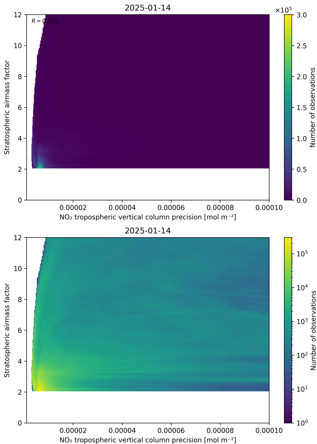
Figure 131: Scatter density plot of “NO 2 tropospheric vertical column precision” against “Stratospheric airmass factor” for 2025-01-13 to 2025-01-15.
