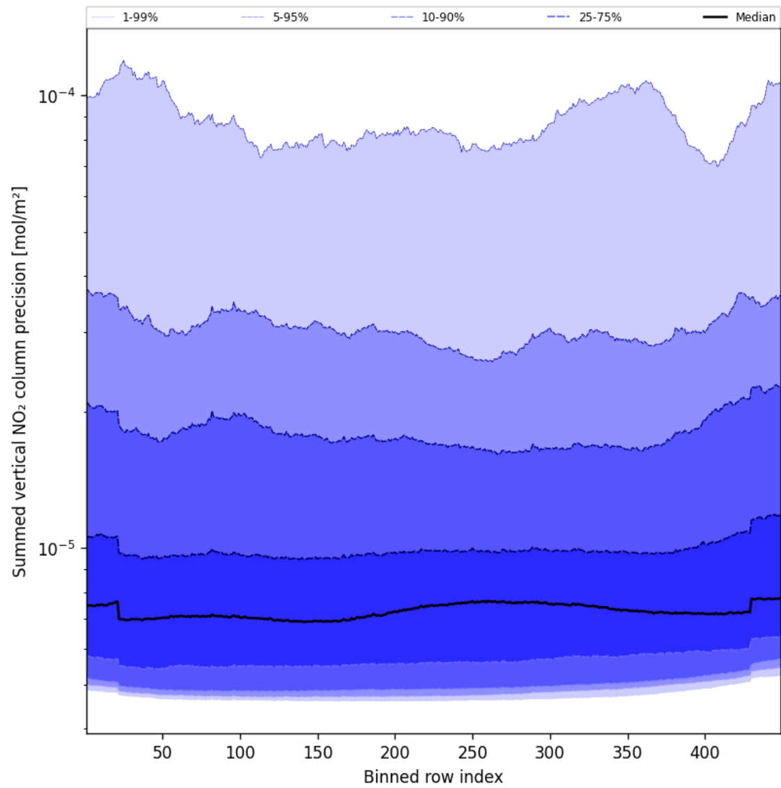
Figure 58: Along track statistics of “Summed vertical NO 2 column precision” for 2025-01-13 to 2025-01-15
