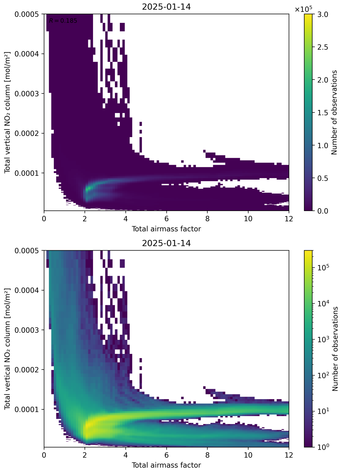
Figure 67: Scatter density plot of “Total airmass factor” against “Total vertical NO 2 column” for 2025-01-13 to 2025-01-15.
