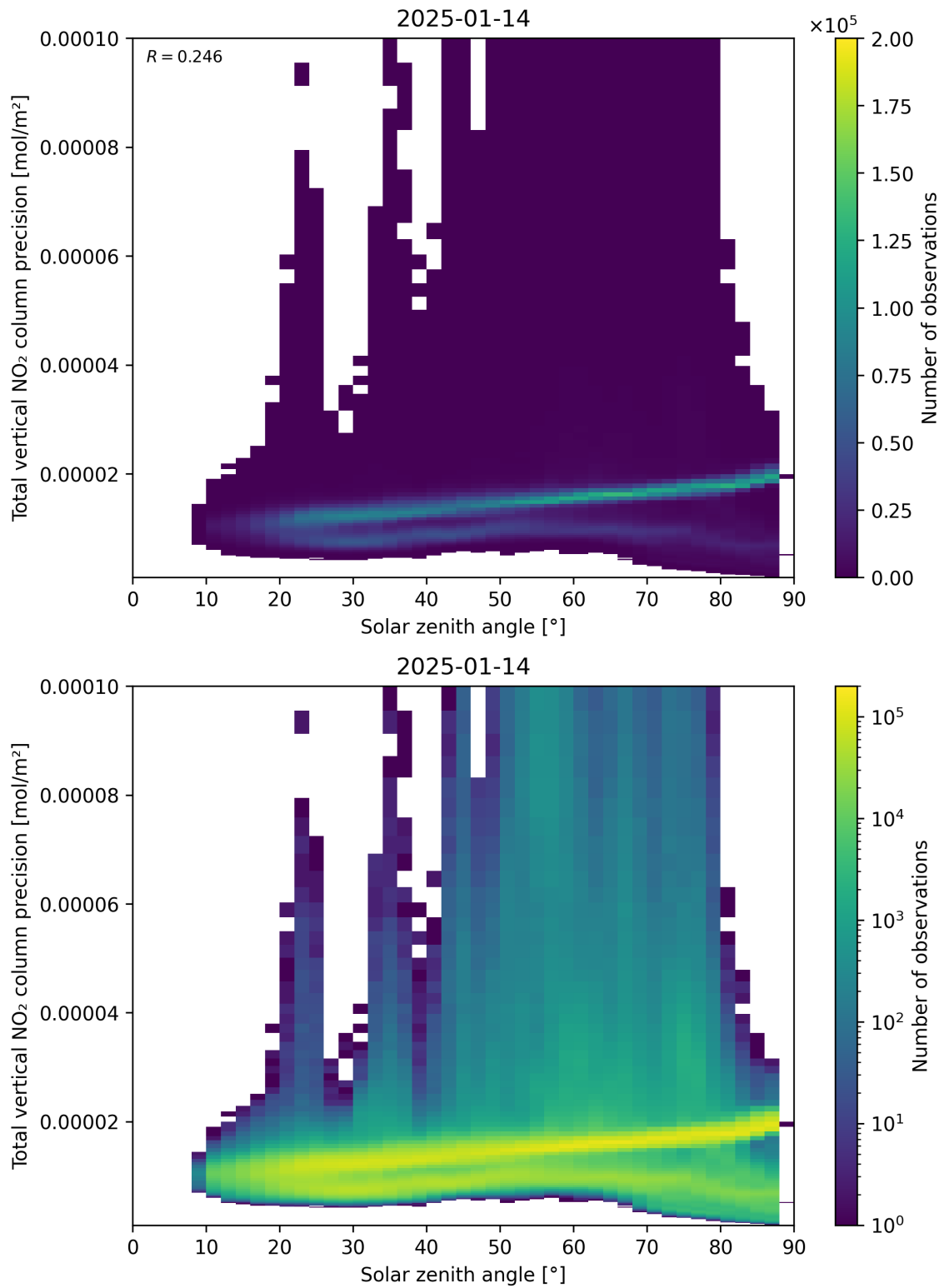
Figure 154: Scatter density plot of “Solar zenith angle” against “Total vertical NO 2 column precision” for 2025-01-13 to 2025-01-15.
