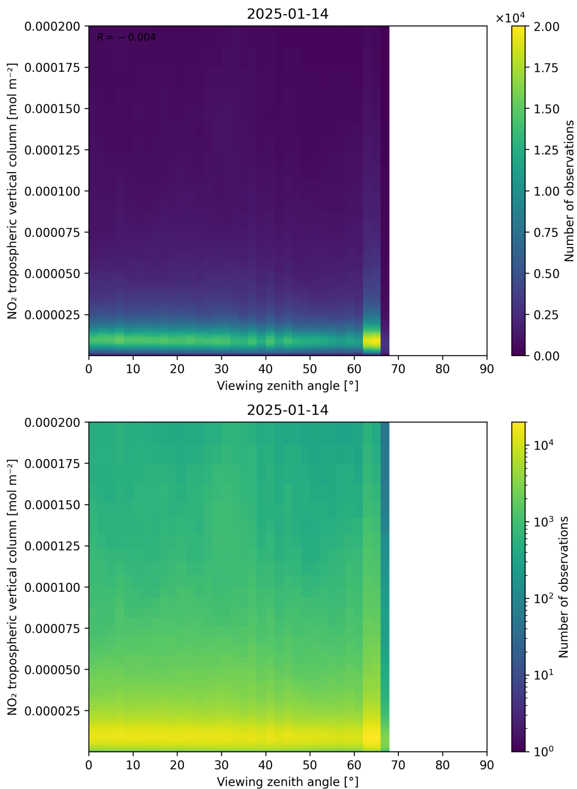
Figure 169: Scatter density plot of “Viewing zenith angle” against “NO 2 tropospheric vertical column” for 2025-01-13 to 2025-01-15.
