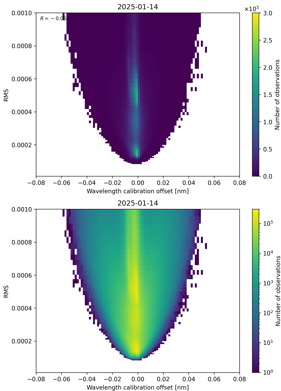
Figure 181: Scatter density plot of “Wavelength calibration offset” against “RMS” for 2025-01-13 to 2025-01-15.
