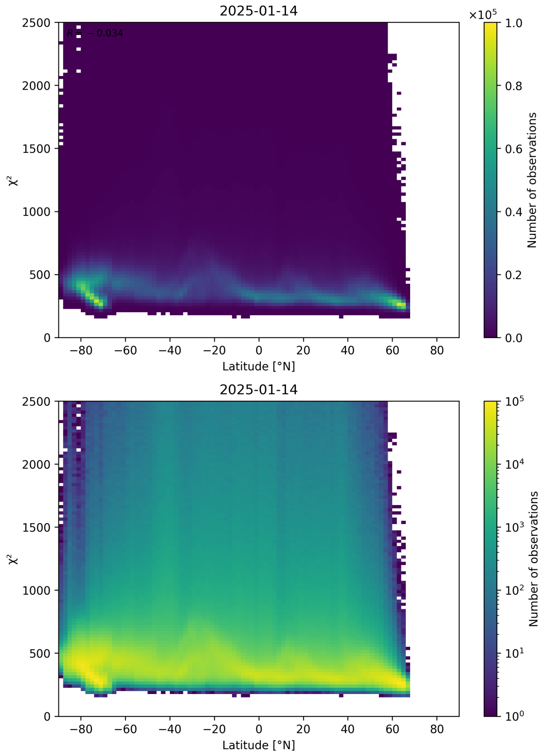
Figure 86: Scatter density plot of “Latitude” against “ \chi^2 ” for 2025-01-13 to 2025-01-15.
