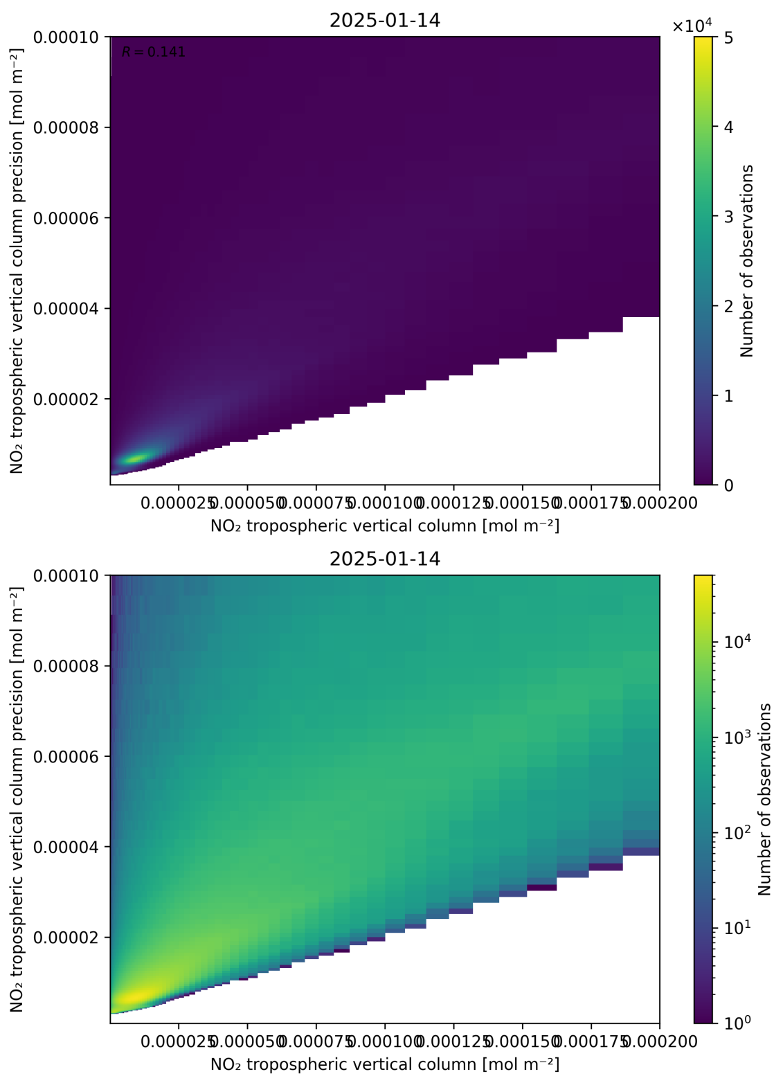
Figure 130: Scatter density plot of “NO 2 tropospheric vertical column” against “NO 2 tropospheric vertical column precision” for 2025-01-13 to 2025-01-15.
