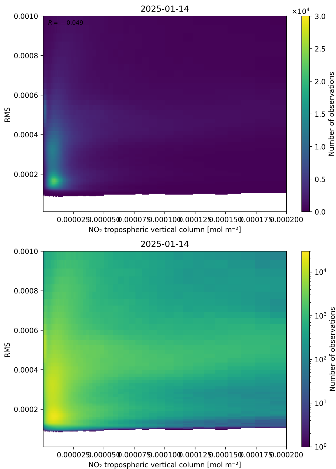
Figure 142: Scatter density plot of “NO 2 tropospheric vertical column” against “RMS” for 2025-01-13 to 2025-01-15.
