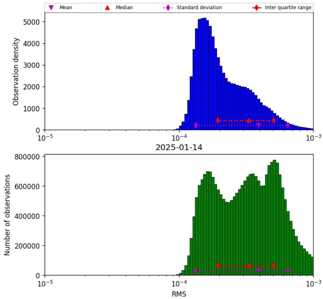
Figure 43: Histogram of “RMS” for 2025-01-13 to 2025-01-15
