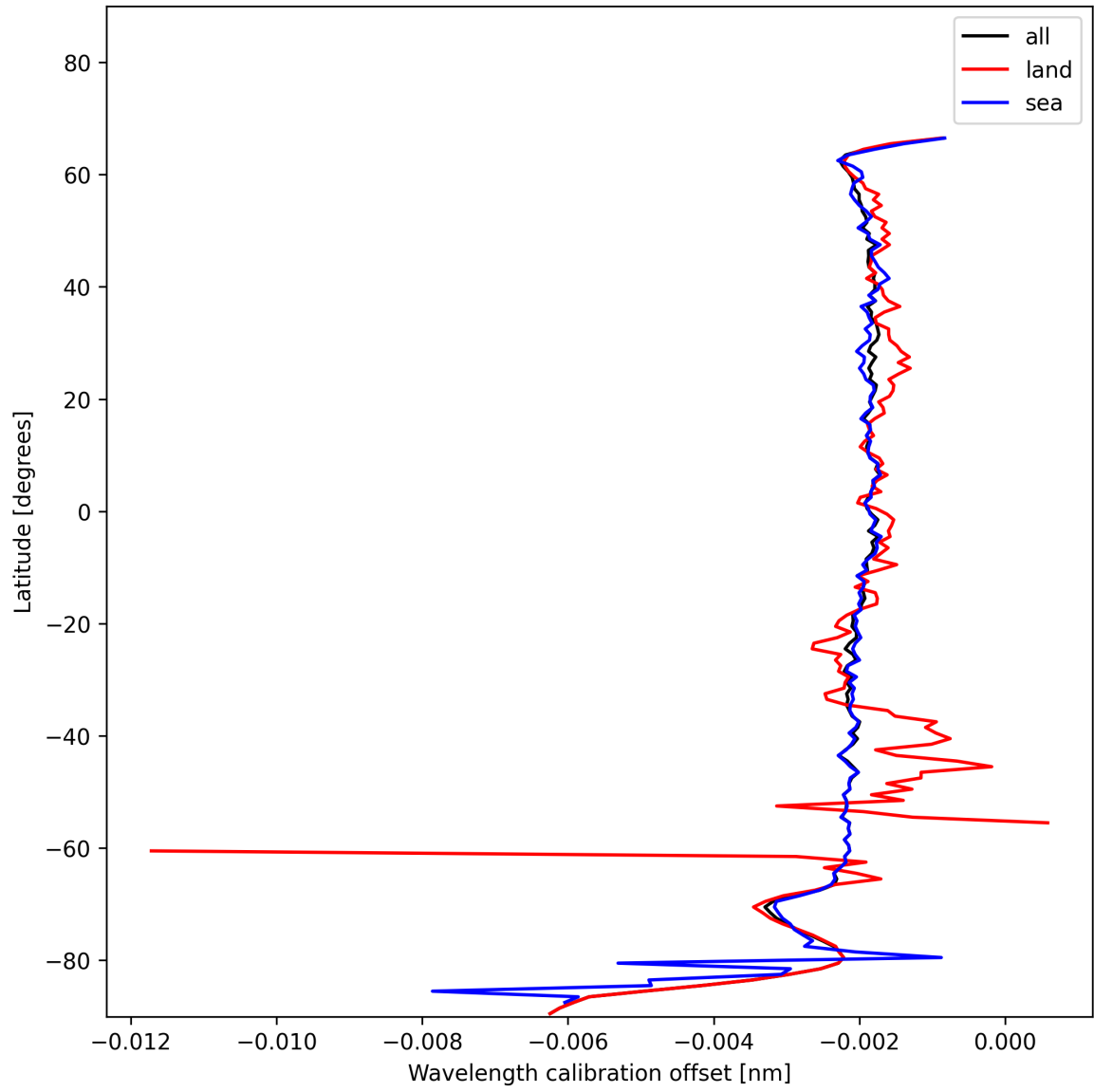
Figure 18: Zonal average of “Wavelength calibration offset” for 2025-01-13 to 2025-01-15.
