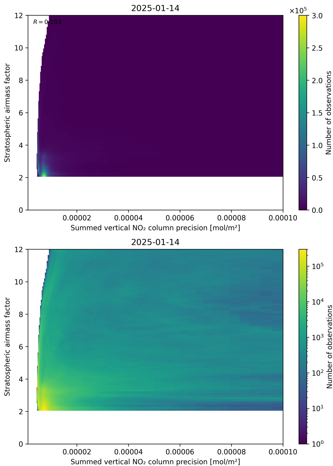
Figure 106: Scatter density plot of “Summed vertical NO 2 column precision” against “Stratospheric airmass factor” for 2025-01-13 to 2025-01-15.
