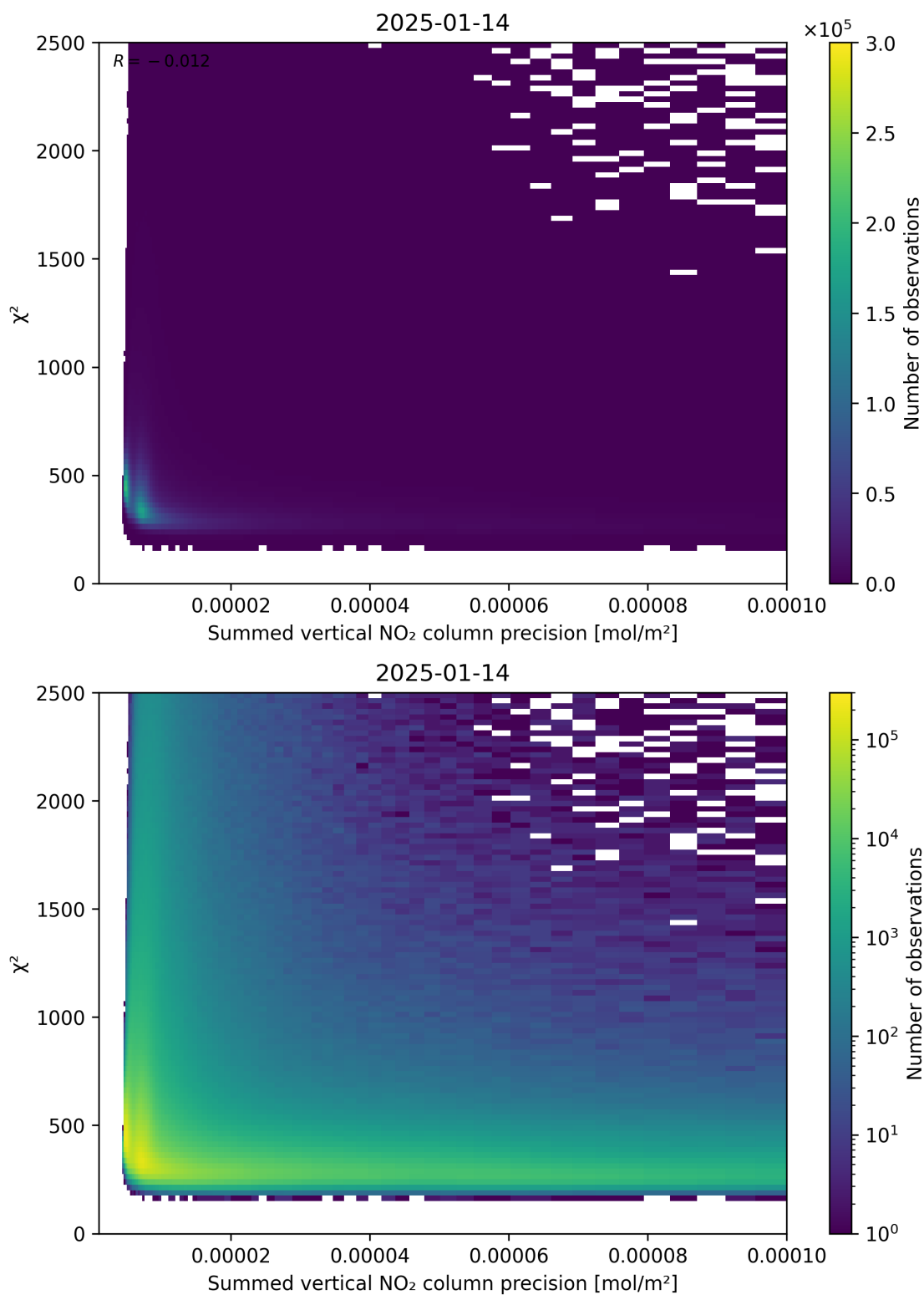
Figure 107: Scatter density plot of “Summed vertical NO 2 column precision” against “ \chi^2 ” for 2025-01-13 to 2025-01-15.
