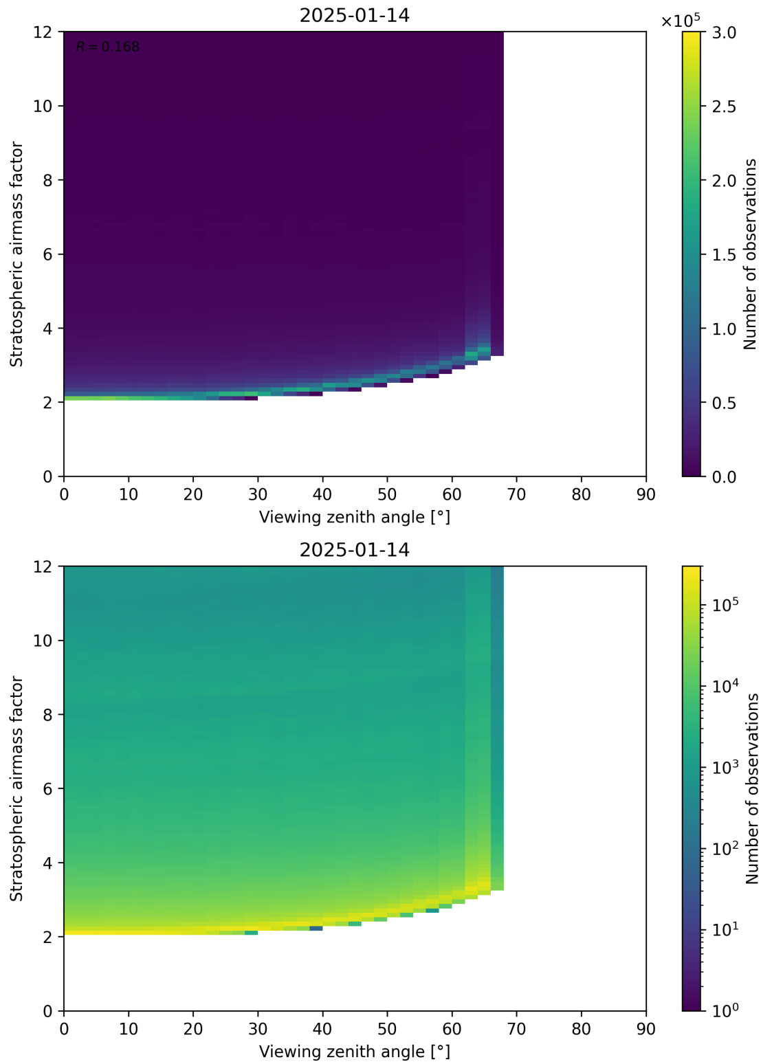
Figure 159: Scatter density plot of “Viewing zenith angle” against “Stratospheric airmass factor” for 2025-01-13 to 2025-01-15.
