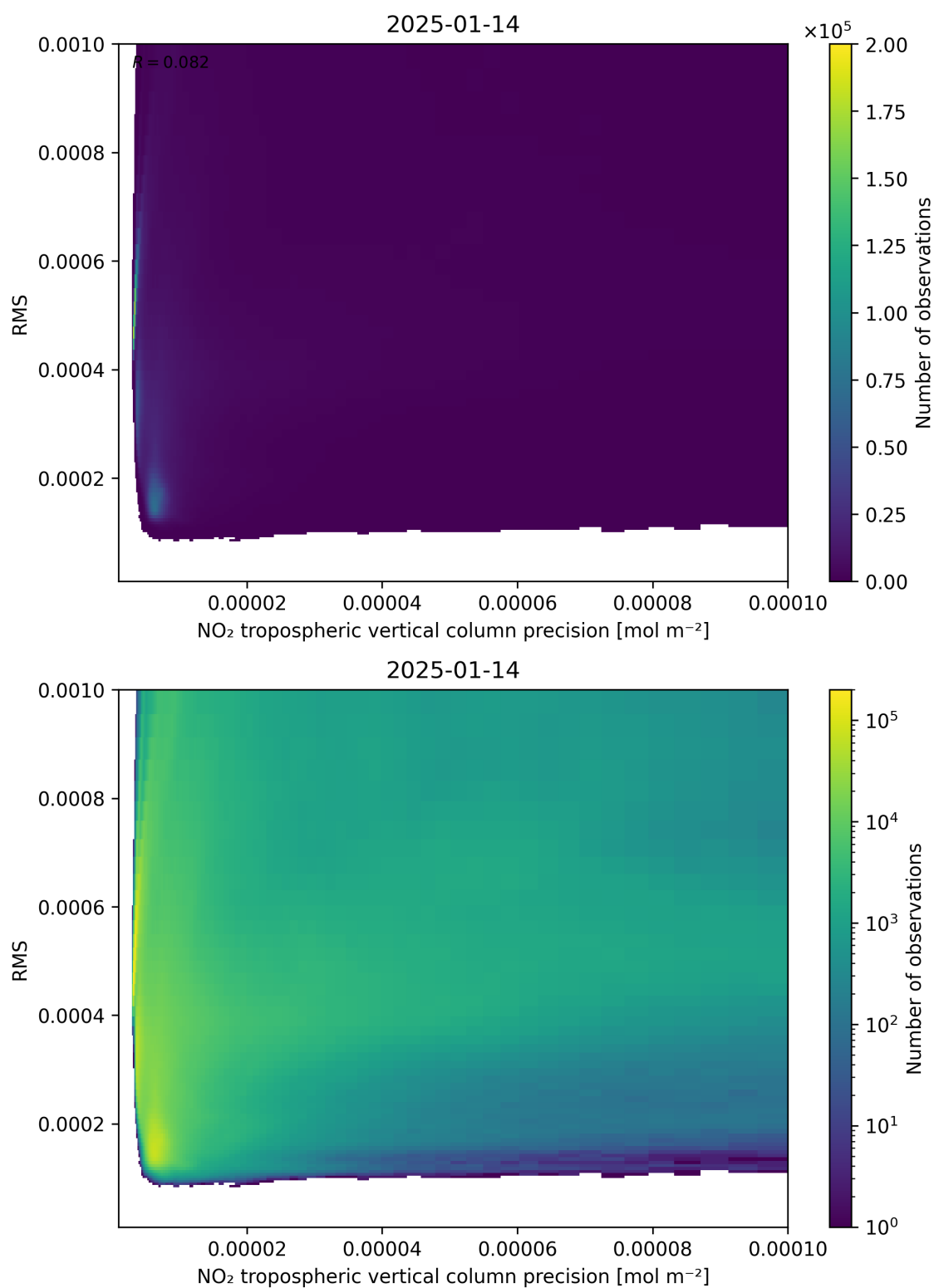
Figure 140: Scatter density plot of “NO 2 tropospheric vertical column precision” against “RMS” for 2025-01-13 to 2025-01-15.
