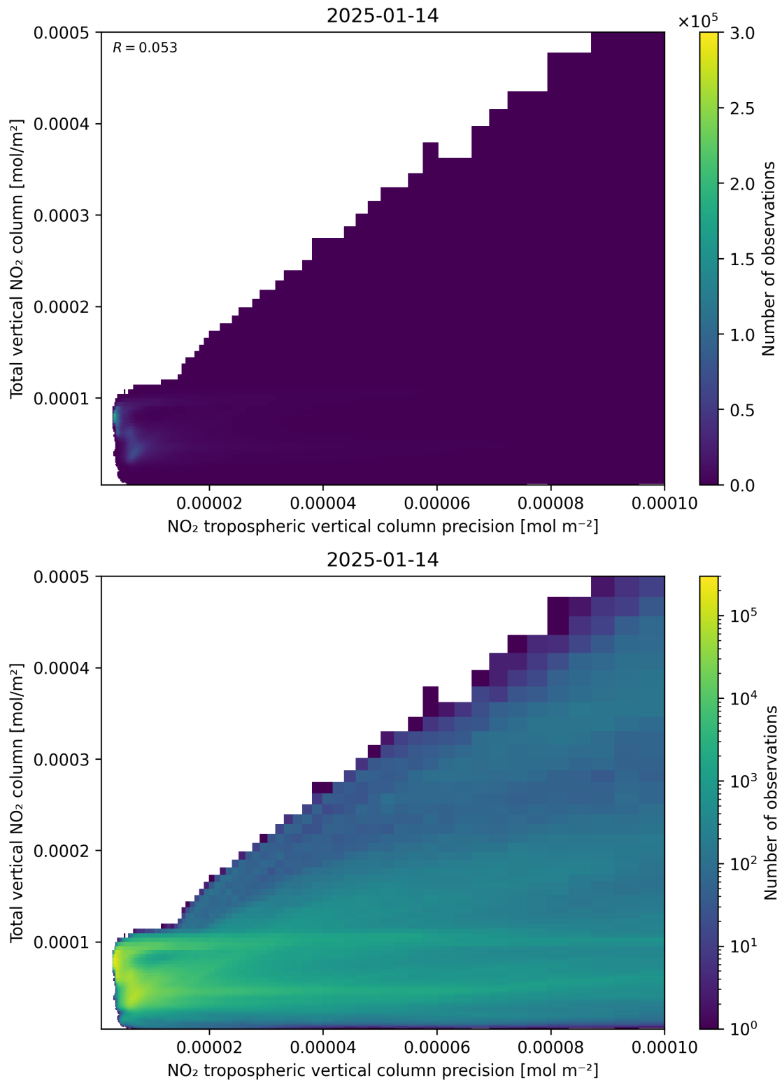
Figure 138: Scatter density plot of “NO 2 tropospheric vertical column precision” against “Total vertical NO 2 column” for 2025-01-13 to 2025-01-15.
