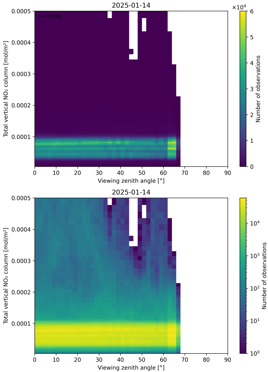
Figure 167: Scatter density plot of “Viewing zenith angle” against “Total vertical NO 2 column” for 2025-01-13 to 2025-01-15.
