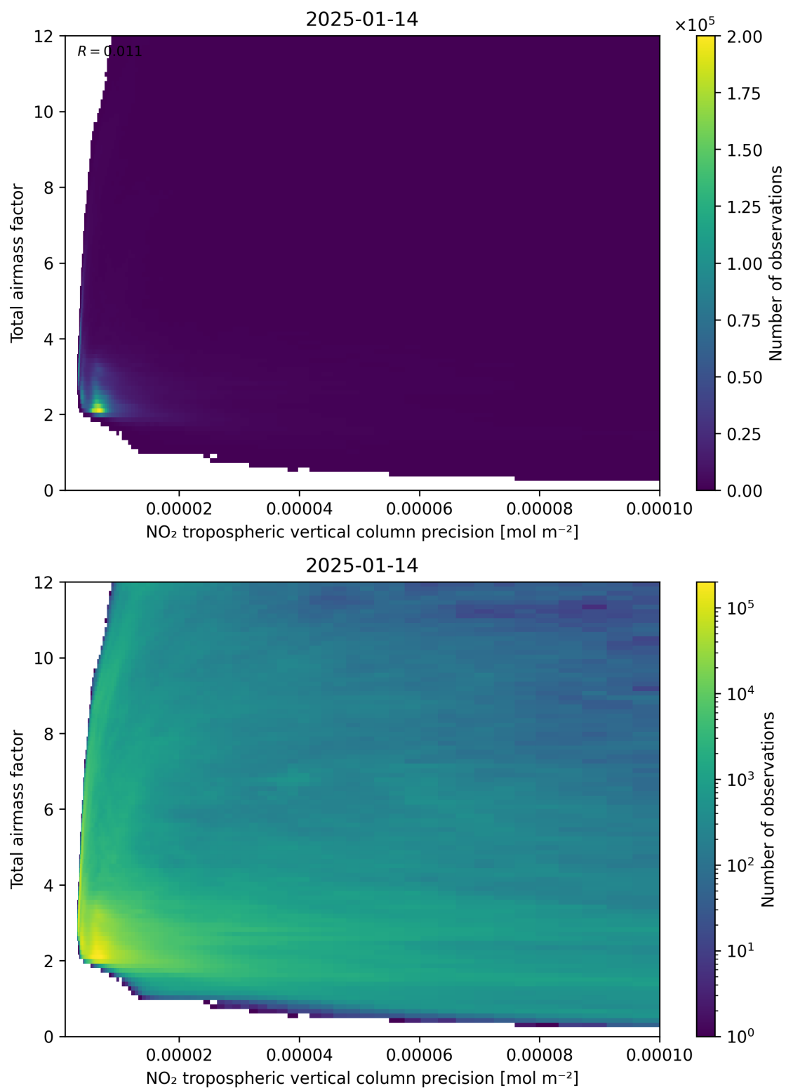
Figure 132: Scatter density plot of “NO 2 tropospheric vertical column precision” against “Total air mass factor” for 2025-01-13 to 2025-01-15.
