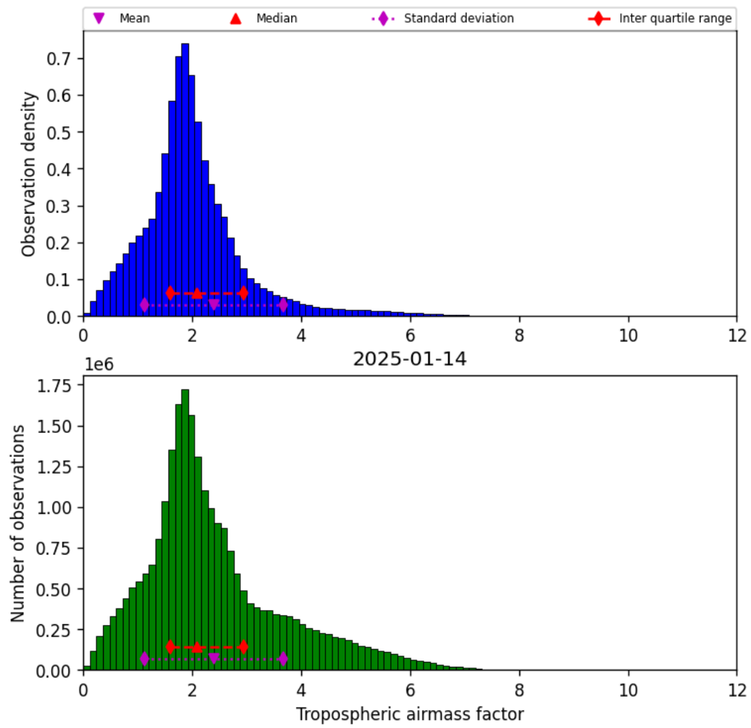
Figure 31: Histogram of “Tropospheric airmass factor” for 2025-01-13 to 2025-01-15
