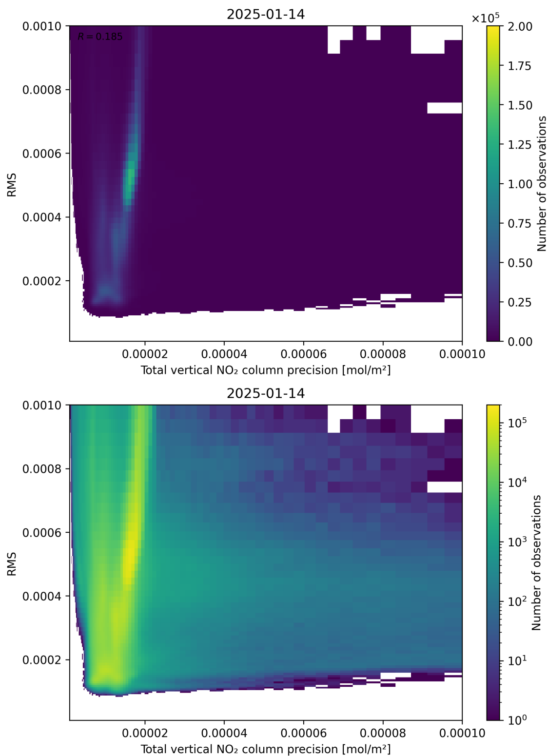
Figure 119: Scatter density plot of “Total vertical NO 2 column precision” against “RMS” for 2025-01-13 to 2025-01-15.
