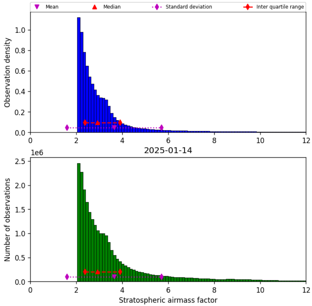
Figure 44: Histogram of “Stratospheric airmass factor” for 2025-01-13 to 2025-01-15
