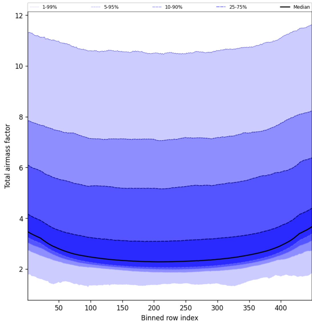
Figure 49: Along track statistics of “Total airmass factor” for 2025-01-13 to 2025-01-15
