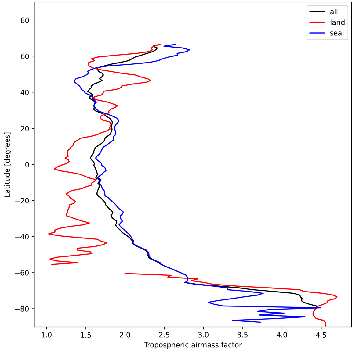
Figure 14: Zonal average of “Tropospheric airmass factor” for 2025-01-13 to 2025-01-15.
