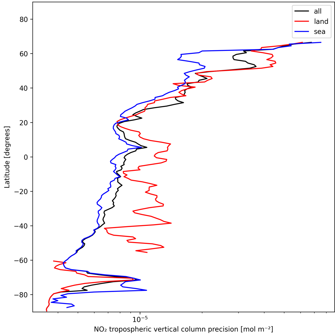
Figure 13: Zonal average of “NO 2 tropospheric vertical column precision” for 2025-01-13 to 2025-01-15.
