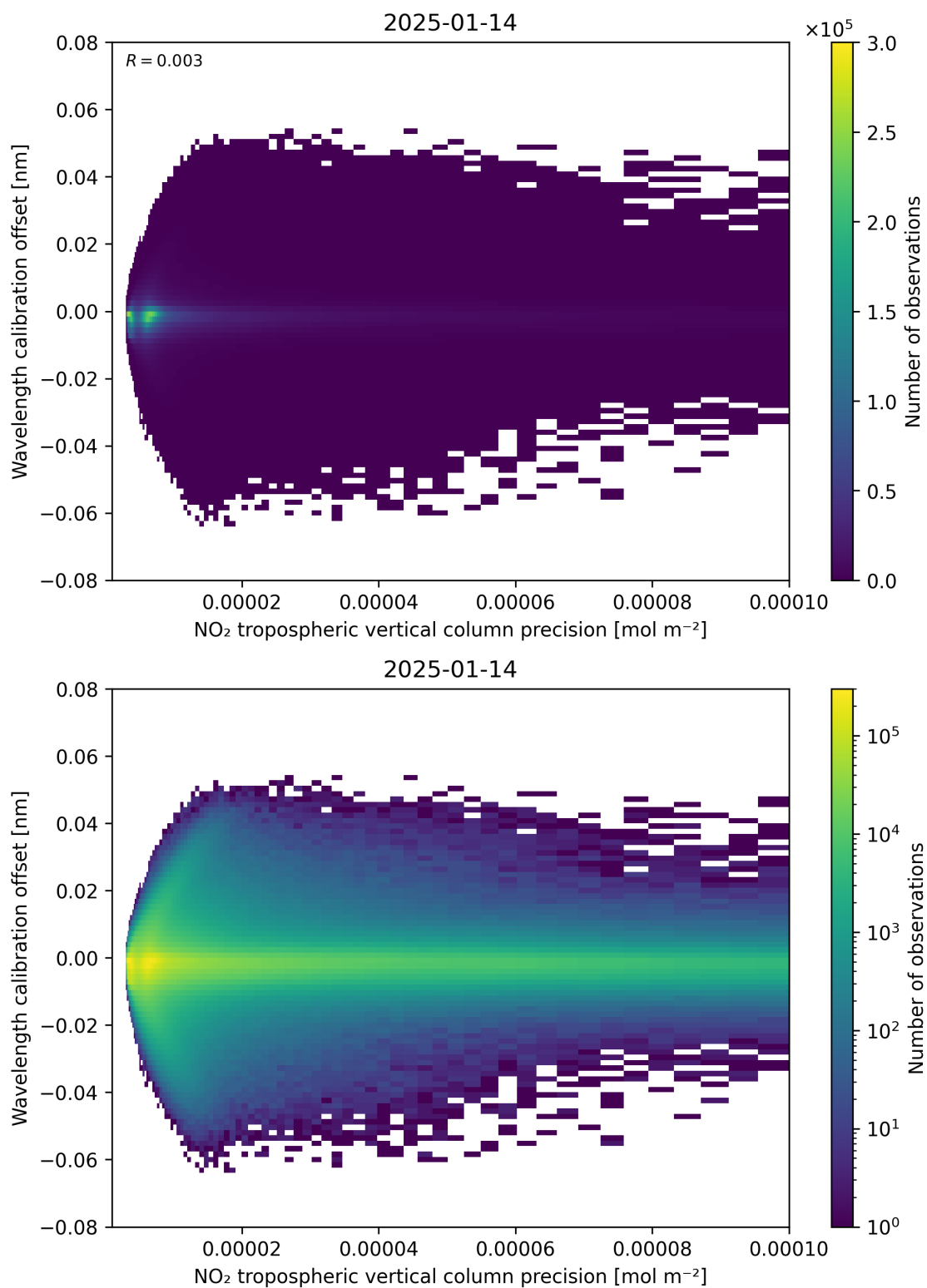
Figure 141: Scatter density plot of “NO 2 tropospheric vertical column precision” against “Wavelength calibration offset” for 2025-01-13 to 2025-01-15.
