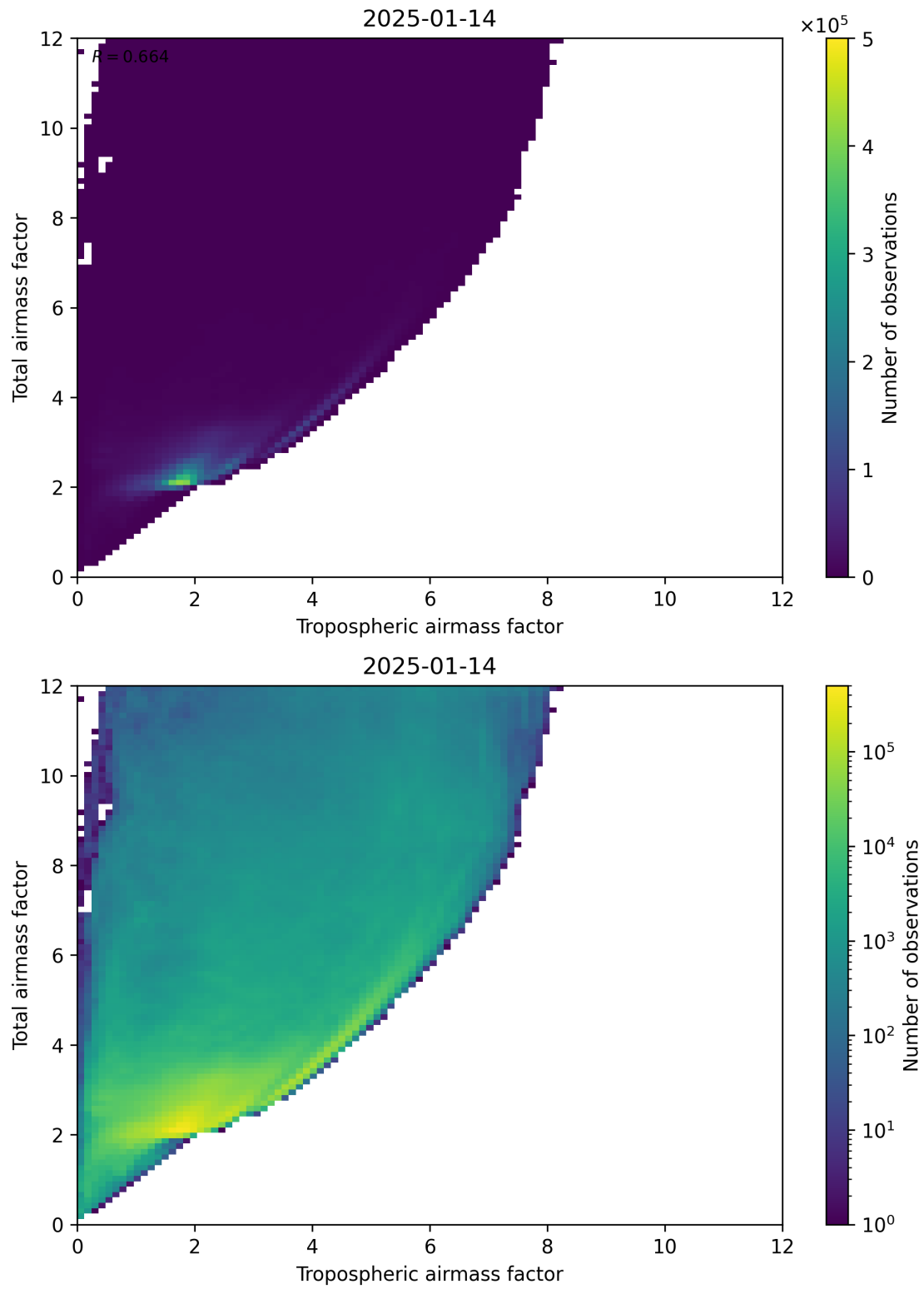
Figure 72: Scatter density plot of “Tropospheric airmass factor” against “Total airmass factor” for 2025-01-13 to 2025-01-15.
