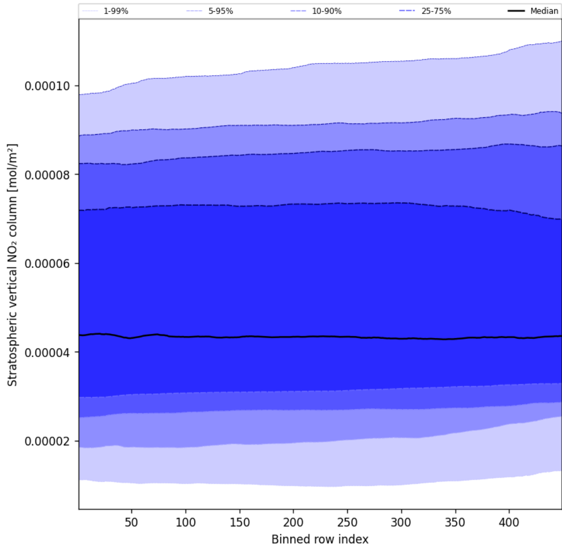
Figure 53: Along track statistics of “Stratospheric vertical NO 2 column” for 2025-01-13 to 2025-01-15
