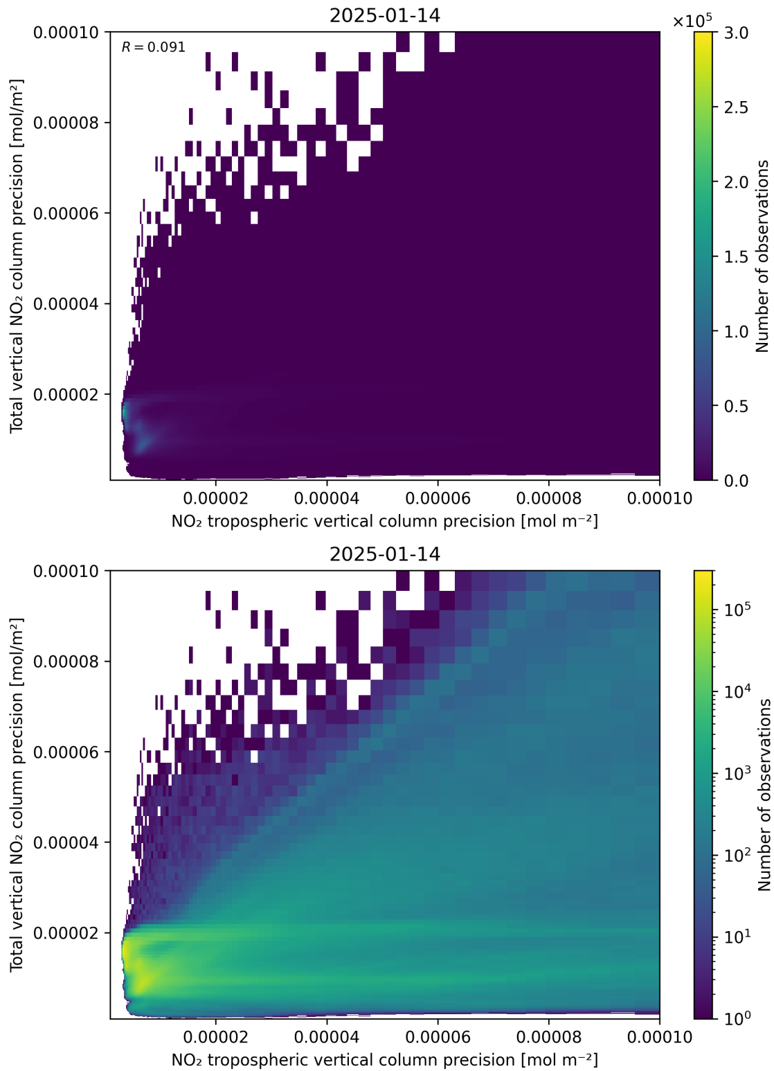
Figure 139: Scatter density plot of “NO 2 tropospheric vertical column precision” against “Total vertical NO 2 column precision” for 2025-01-13 to 2025-01-15.
