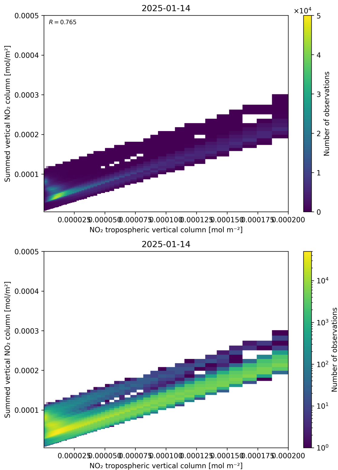
Figure 126: Scatter density plot of “NO 2 tropospheric vertical column” against “Summed vertical NO 2 column” for 2025-01-13 to 2025-01-15.
