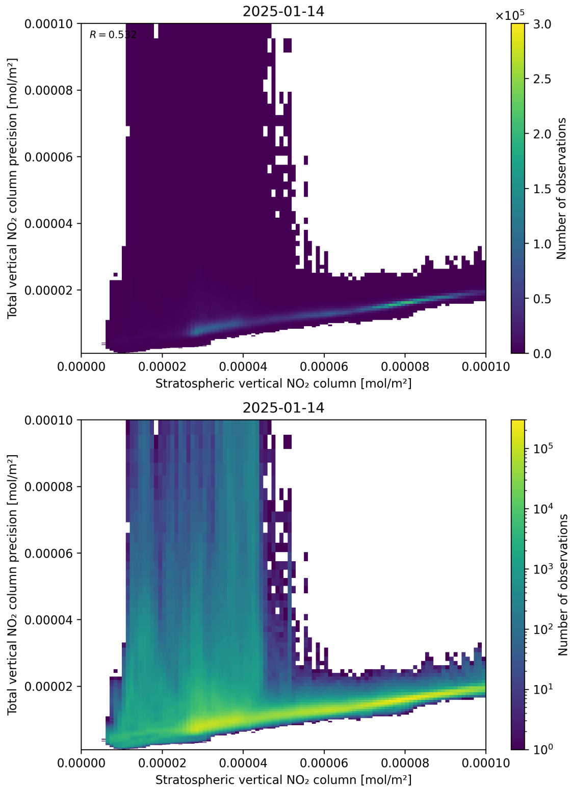
Figure 101: Scatter density plot of “Stratospheric vertical NO 2 column” against “Total vertical NO 2 column precision” for 2025-01-13 to 2025-01-15.
