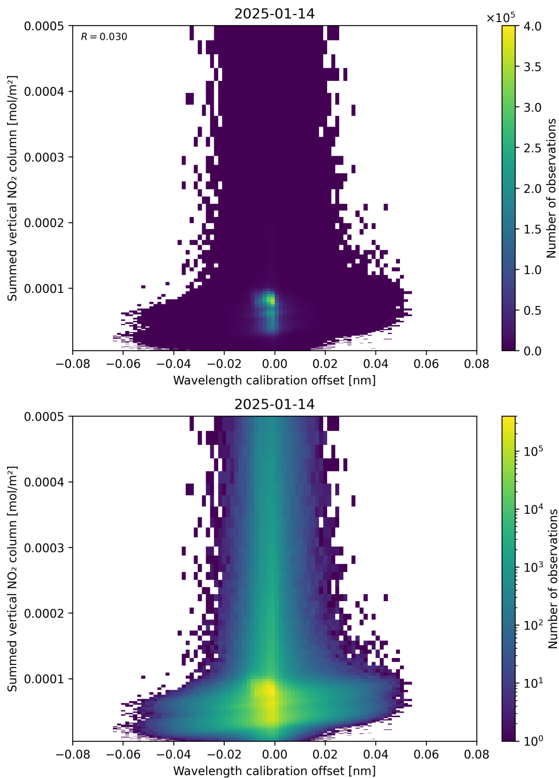
Figure 177: Scatter density plot of “Wavelength calibration offset” against “Summed vertical NO 2 column” for 2025-01-13 to 2025-01-15.
