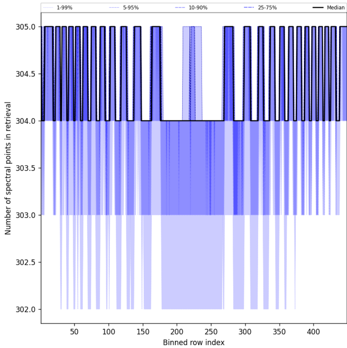
Figure 50: Along track statistics of “Number of spectral points in retrieval” for 2025-01-13 to 2025-01-15
