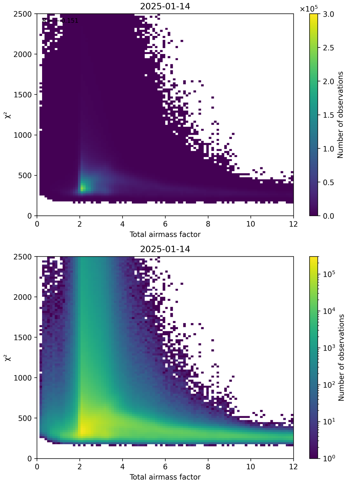
Figure 63: Scatter density plot of “Total airmass factor” against “ \chi^2 ” for 2025-01-13 to 2025-01-15.
