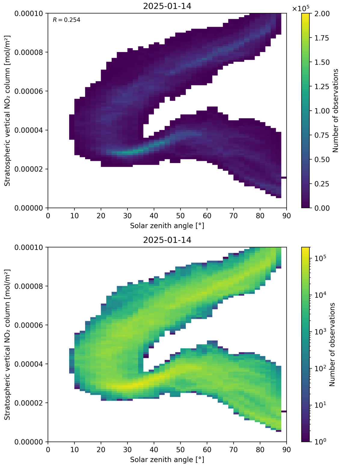
Figure 150: Scatter density plot of “Solar zenith angle” against “Stratospheric vertical NO 2 column” for 2025-01-13 to 2025-01-15.
