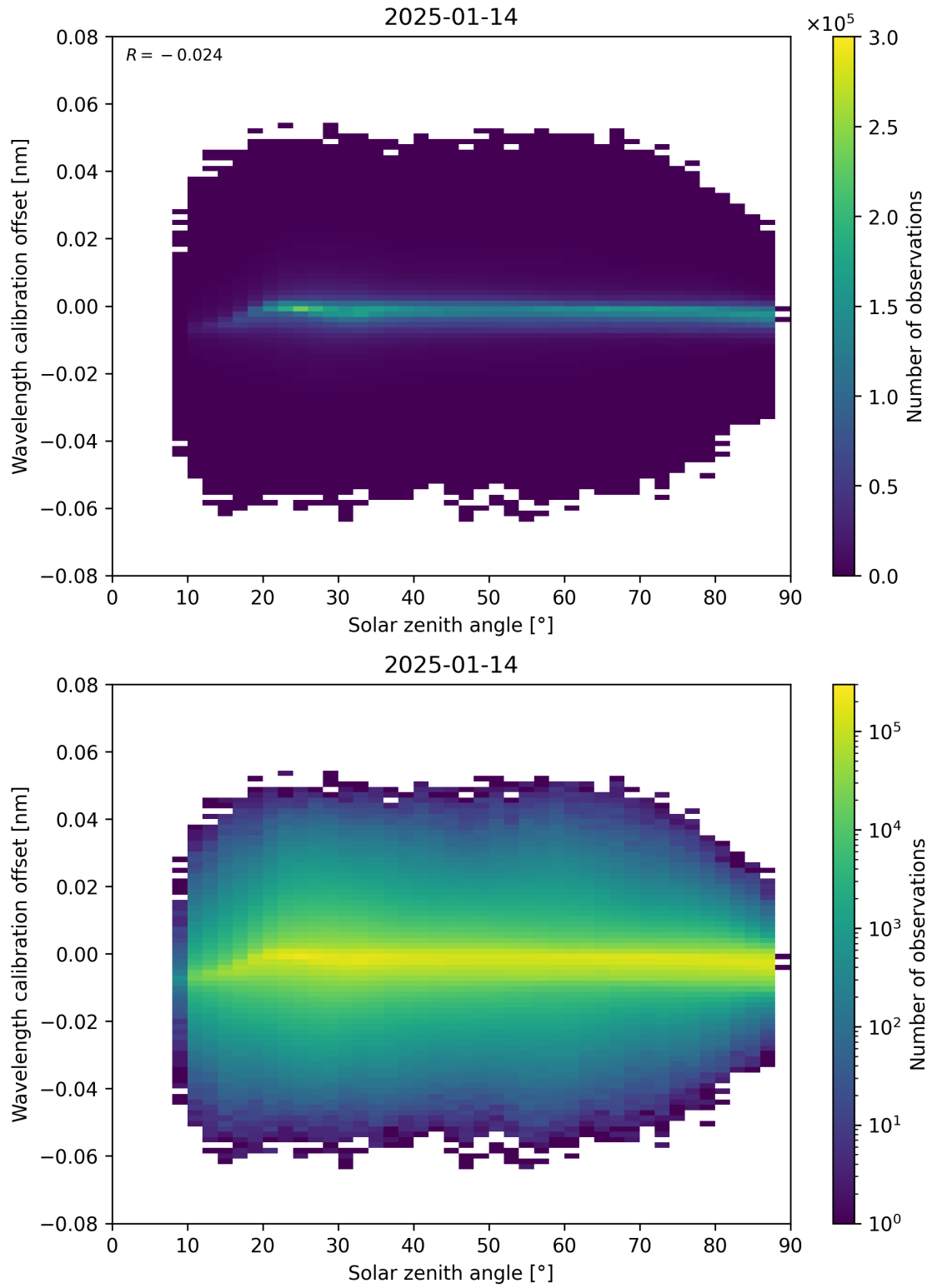
Figure 158: Scatter density plot of “Solar zenith angle” against “Wavelength calibration offset” for 2025-01-13 to 2025-01-15.
