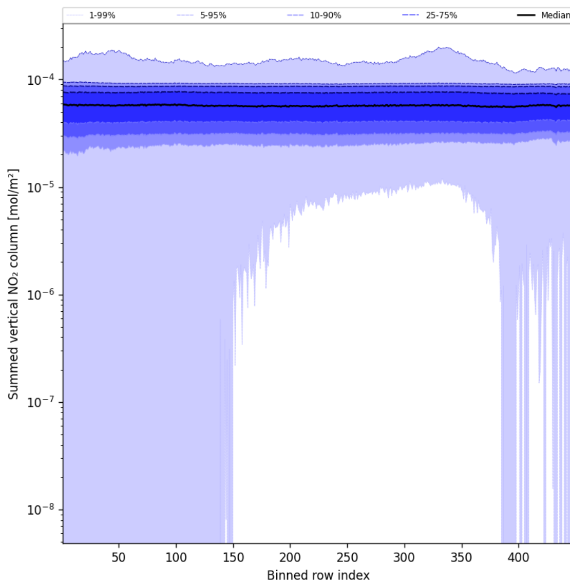
Figure 57: Along track statistics of “Summed vertical NO 2 column” for 2025-01-13 to 2025-01-15
