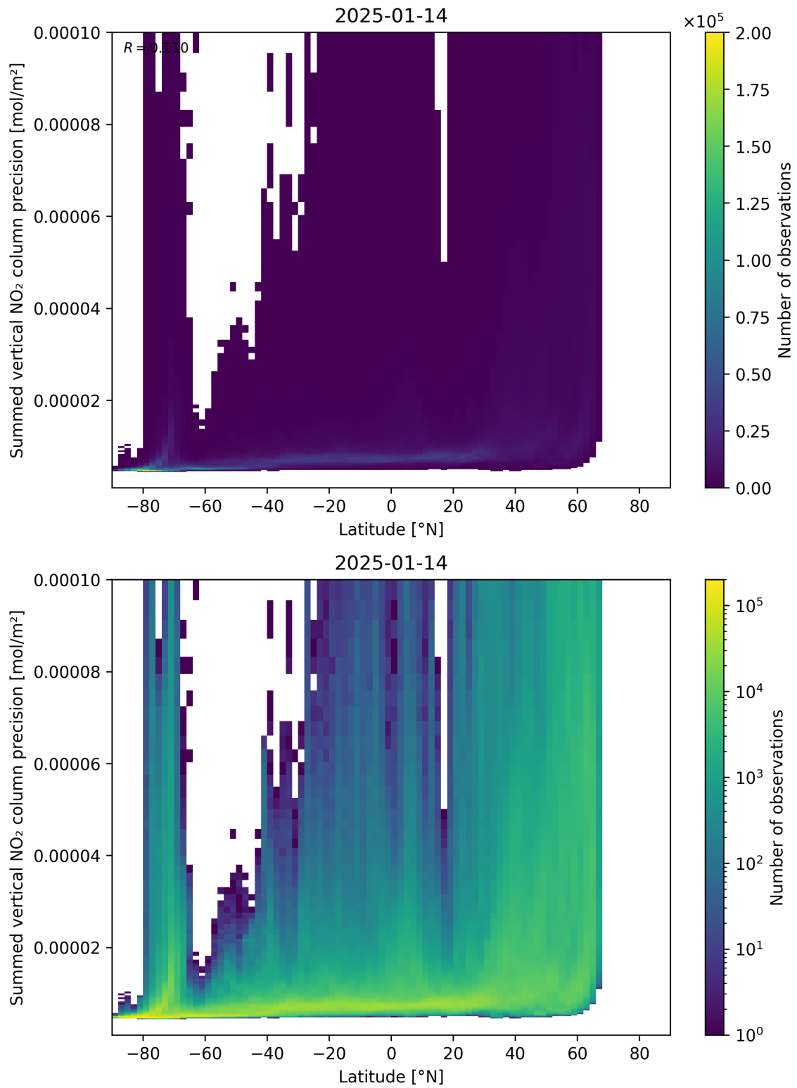
Figure 89: Scatter density plot of “Latitude” against “Summed vertical NO 2 column precision” for 2025-01-13 to 2025-01-15.
