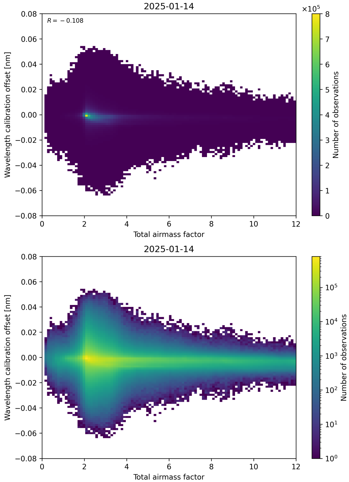
Figure 70: Scatter density plot of “Total airmass factor” against “Wavelength calibration offset” for 2025-01-13 to 2025-01-15.
