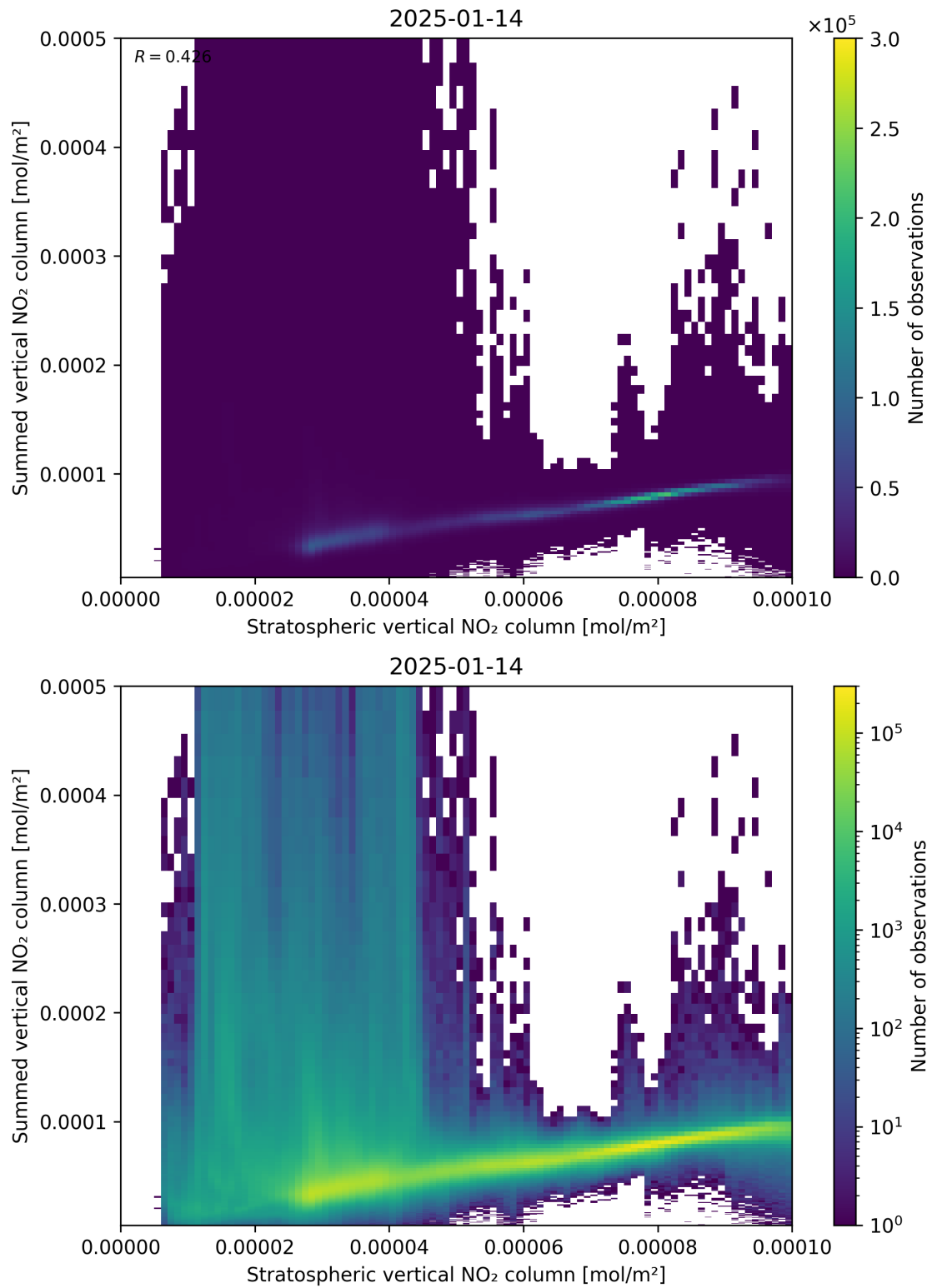
Figure 98: Scatter density plot of “Stratospheric vertical NO 2 column” against “Summed vertical NO 2 column” for 2025-01-13 to 2025-01-15.
