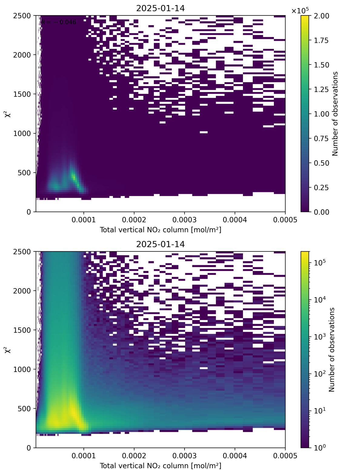
Figure 111: Scatter density plot of “Total vertical NO 2 column” against “ \chi^2 ” for 2025-01-13 to 2025-01-15.
