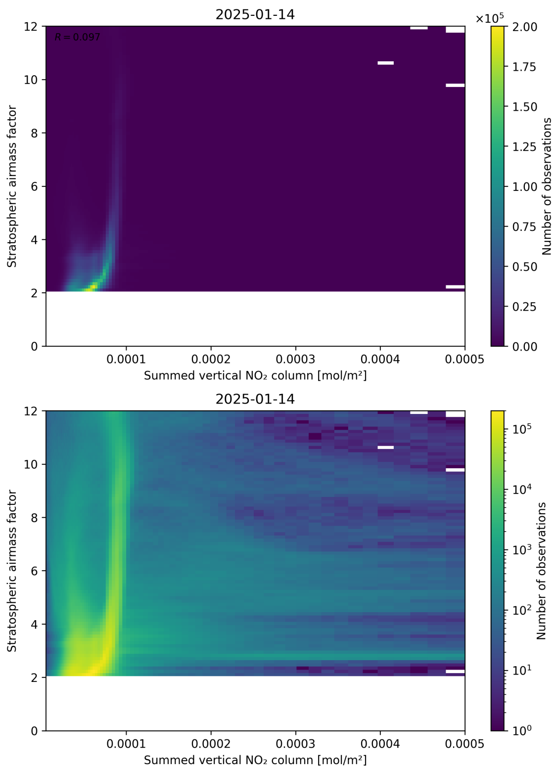
Figure 103: Scatter density plot of “Summed vertical NO 2 column” against “Stratospheric airmass factor” for 2025-01-13 to 2025-01-15.
