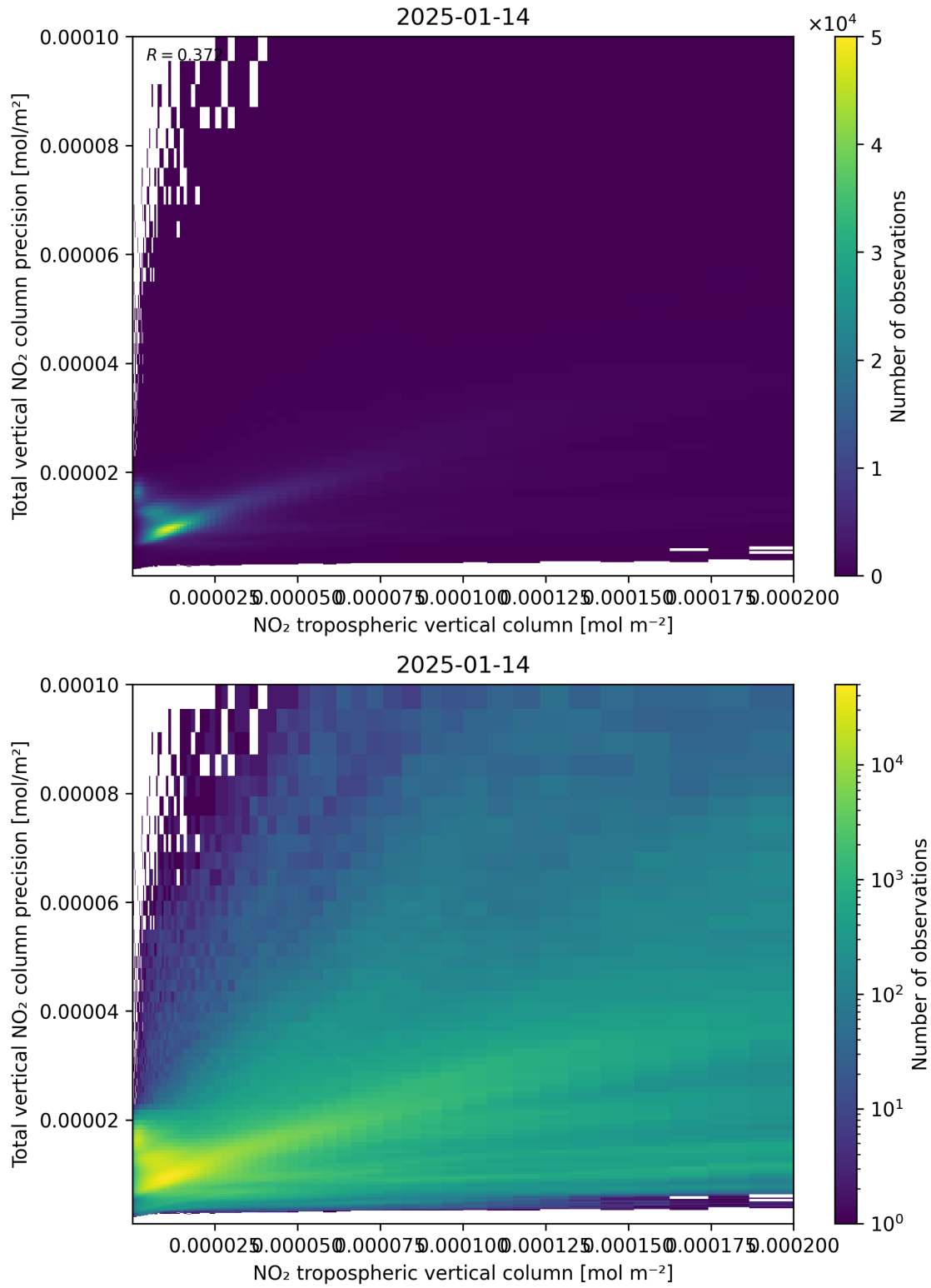
Figure 129: Scatter density plot of “NO 2 tropospheric vertical column” against “Total vertical NO 2 column precision” for 2025-01-13 to 2025-01-15.
