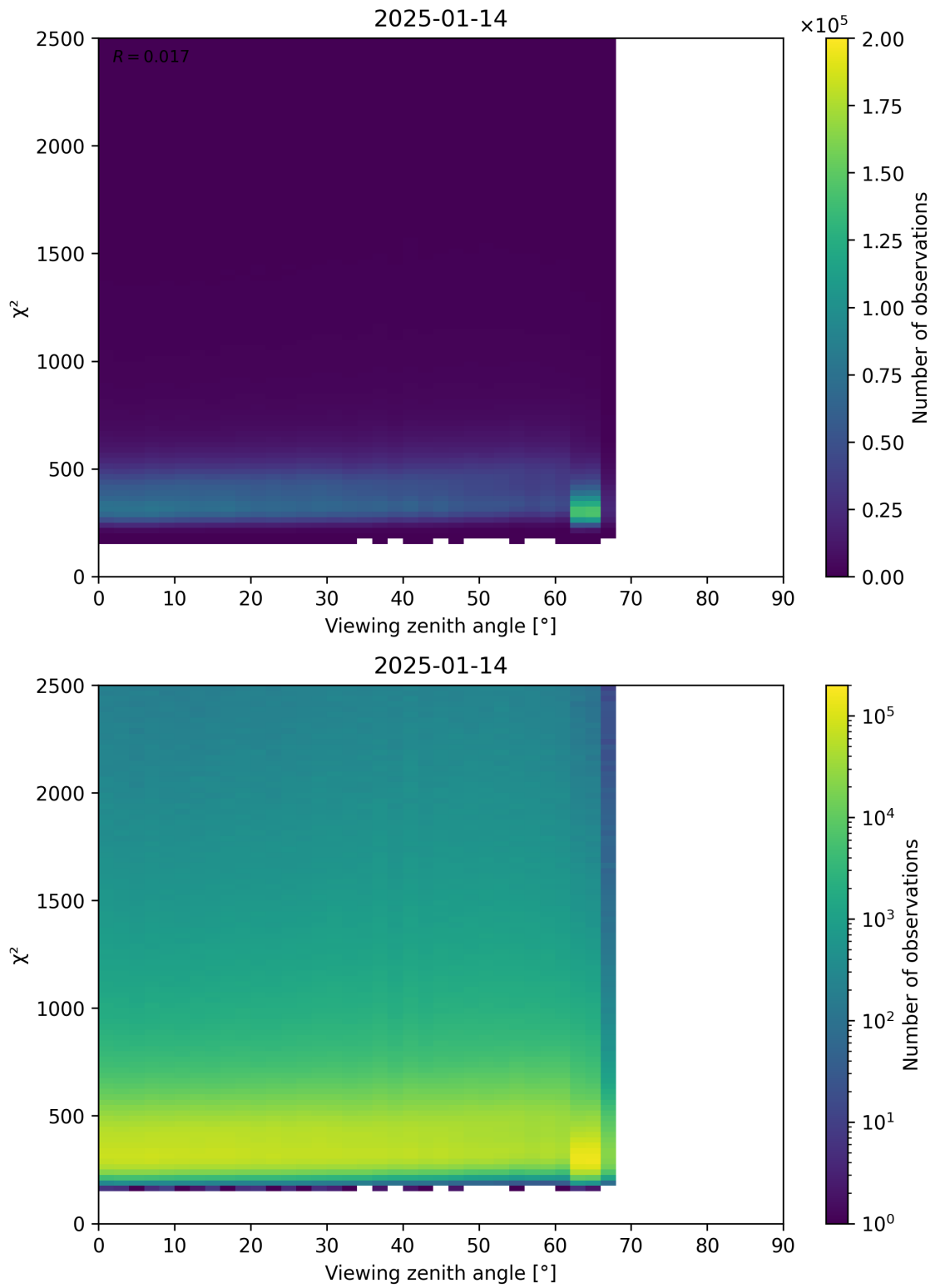
Figure 162: Scatter density plot of “Viewing zenith angle” against “ \chi^2 ” for 2025-01-13 to 2025-01-15.
