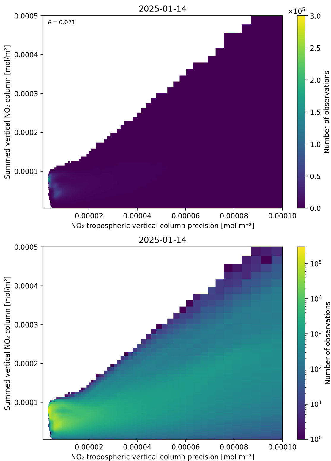
Figure 136: Scatter density plot of “NO 2 tropospheric vertical column precision” against “Summed vertical NO 2 column” for 2025-01-13 to 2025-01-15.
