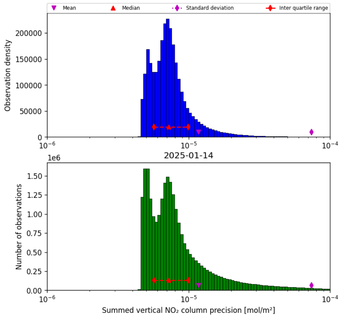
Figure 41: Histogram of “Summed vertical NO 2 column precision” for 2025-01-13 to 2025-01-15
