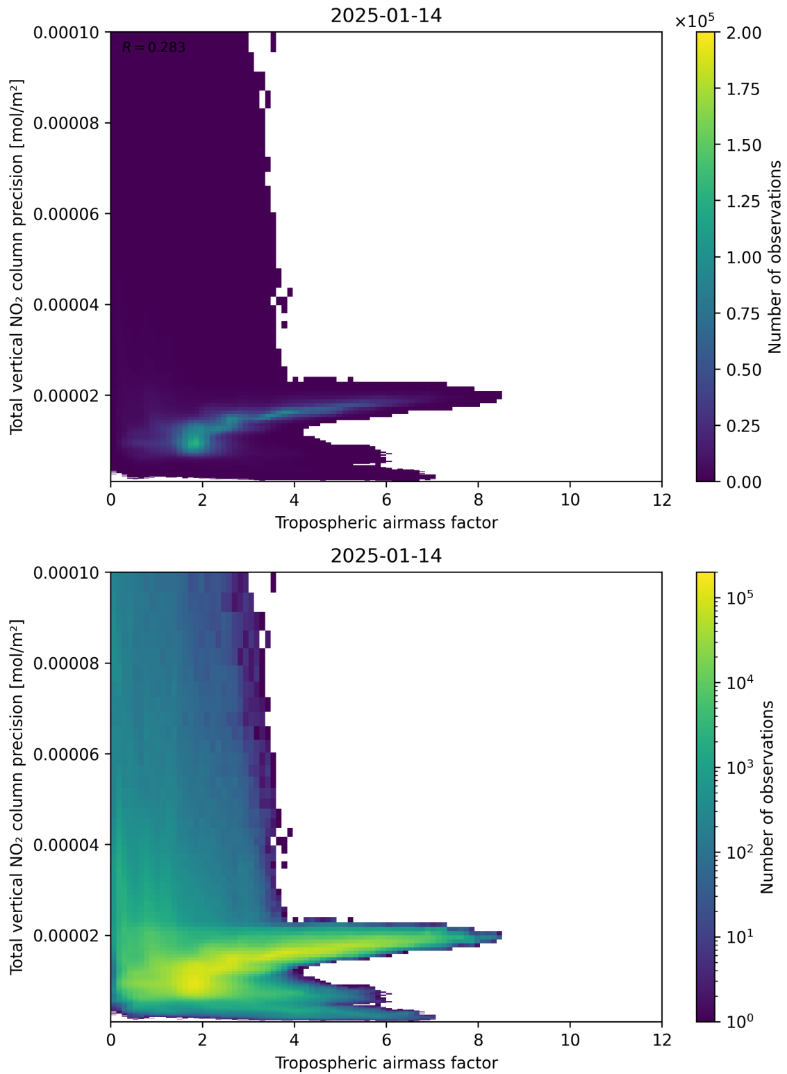
Figure 78: Scatter density plot of “Tropospheric air mass factor” against “Total vertical NO 2 column precision” for 2025-01-13 to 2025-01-15.
