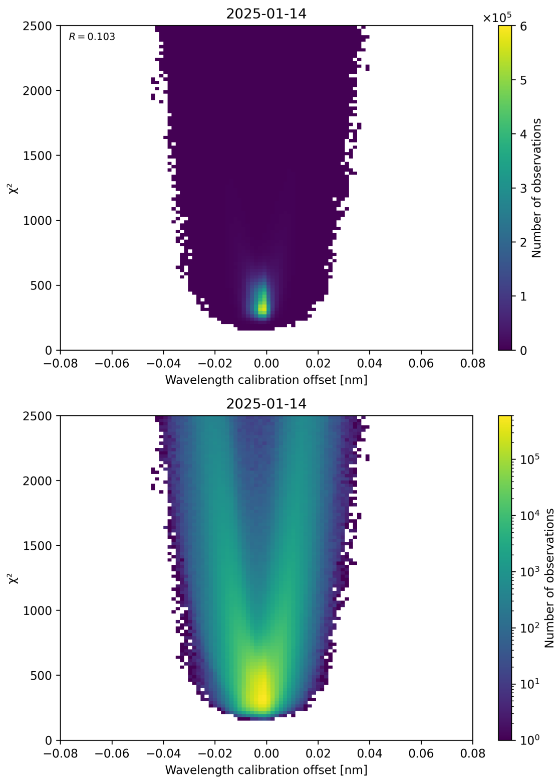
Figure 175: Scatter density plot of “Wavelength calibration offset” against “ \chi^2 ” for 2025-01-13 to 2025-01-15.
