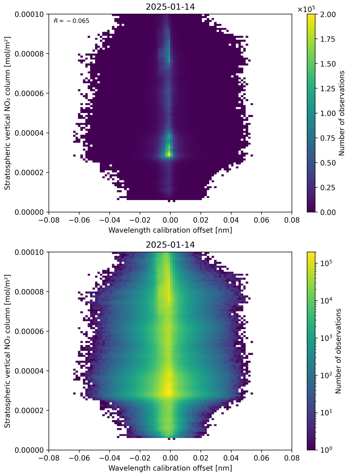
Figure 176: Scatter density plot of “Wavelength calibration offset” against “Stratospheric vertical NO 2 column” for 2025-01-13 to 2025-01-15.
