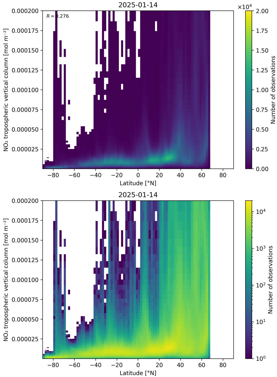
Figure 92: Scatter density plot of “Latitude” against “NO 2 tropospheric vertical column” for 2025-01-13 to 2025-01-15.
