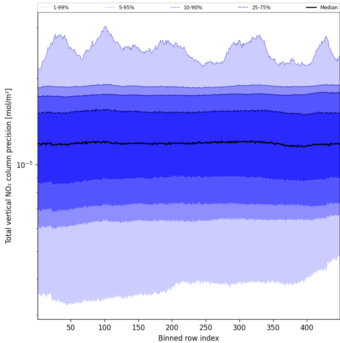
Figure 56: Along track statistics of “Total vertical NO 2 column precision” for 2025-01-13 to 2025-01-15
