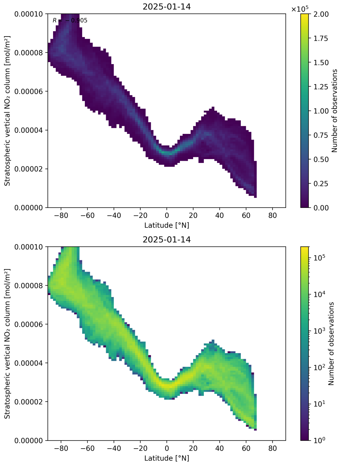
Figure 87: Scatter density plot of “Latitude” against “Stratospheric vertical NO 2 column” for 2025-01-13 to 2025-01-15.
