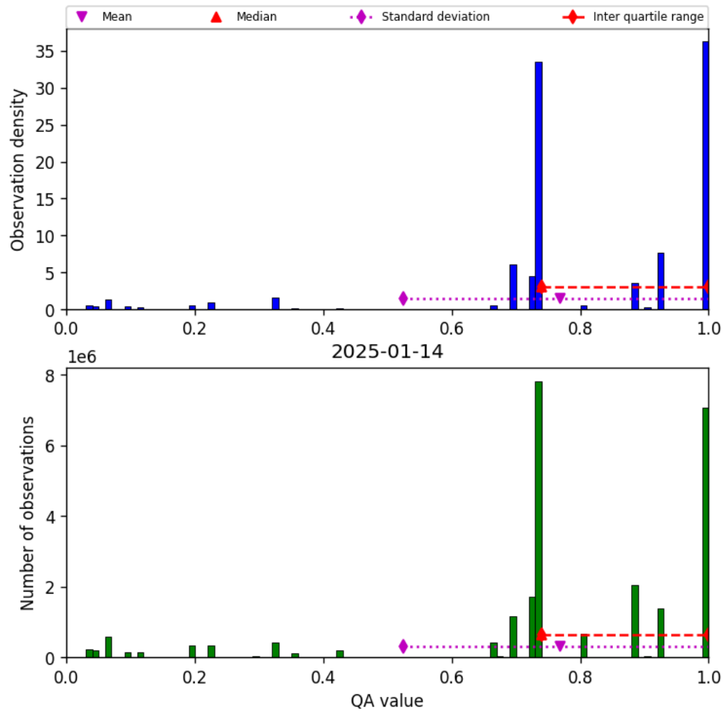
Figure 28: Histogram of “QA value” for 2025-01-13 to 2025-01-15
