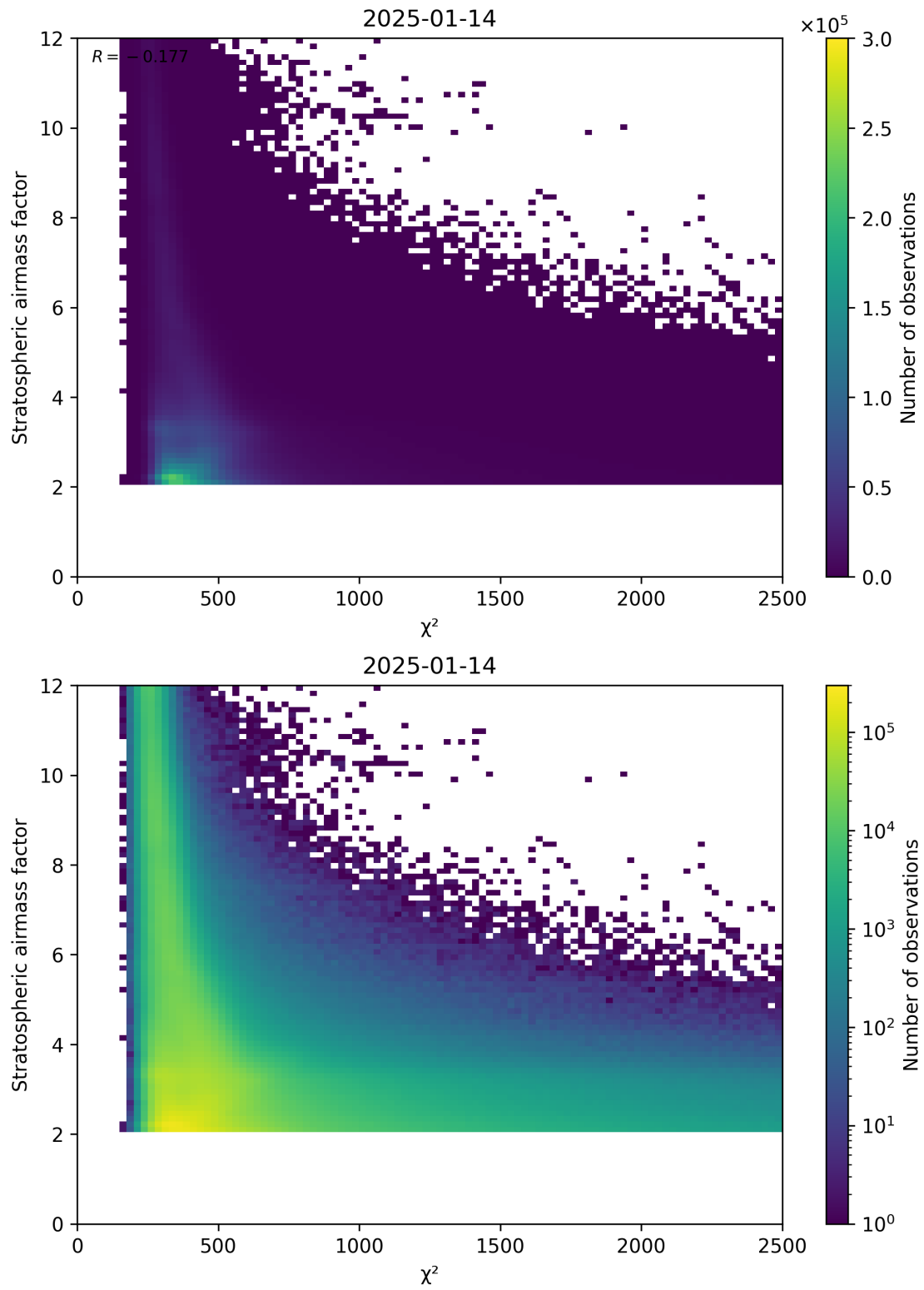
Figure 81: Scatter density plot of “ \chi^2 ” against “Stratospheric airmass factor” for 2025-01-13 to 2025-01-15.
