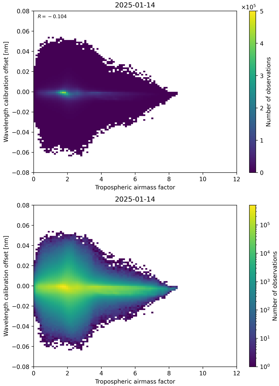
Figure 80: Scatter density plot of “Tropospheric airmass factor” against “Wavelength calibration offset” for 2025-01-13 to 2025-01-15.
