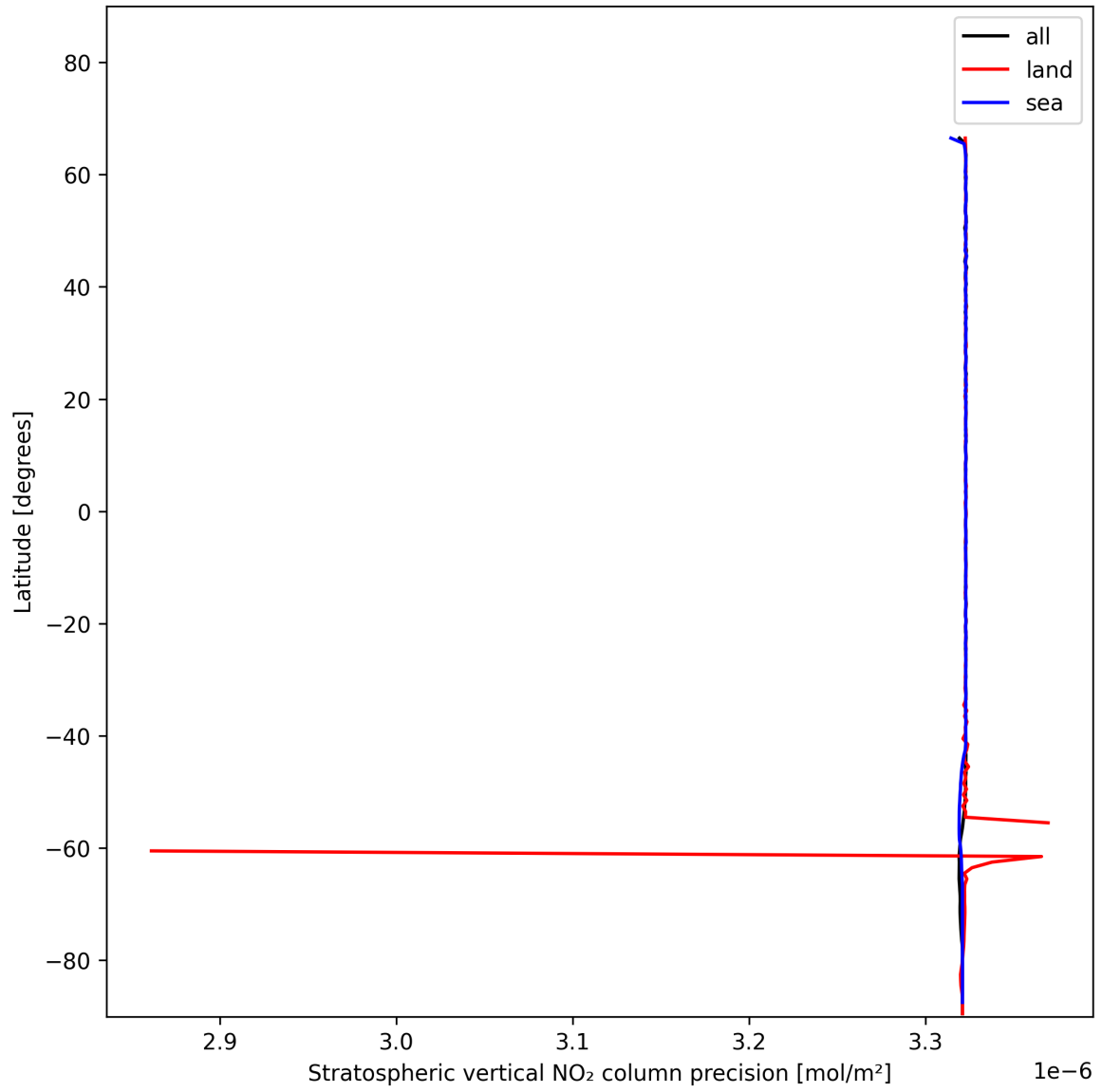
Figure 20: Zonal average of “Stratospheric vertical NO 2 column precision” for 2025-01-13 to 2025-01-15.
