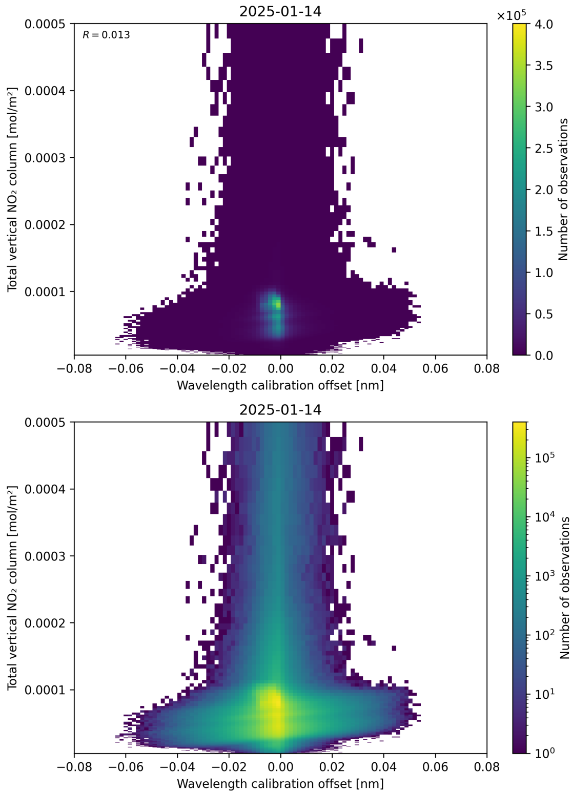
Figure 179: Scatter density plot of “Wavelength calibration offset” against “Total vertical NO 2 column” for 2025-01-13 to 2025-01-15.
