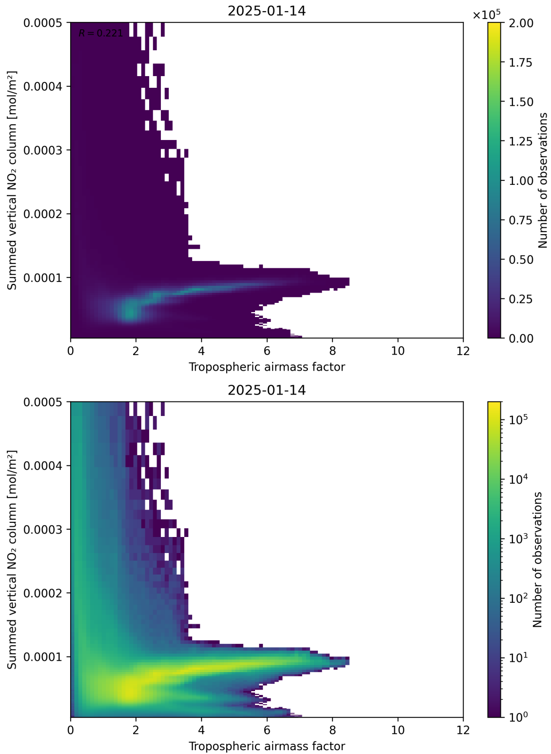
Figure 75: Scatter density plot of “Tropospheric airmass factor” against “Summed vertical NO 2 column” for 2025-01-13 to 2025-01-15.
