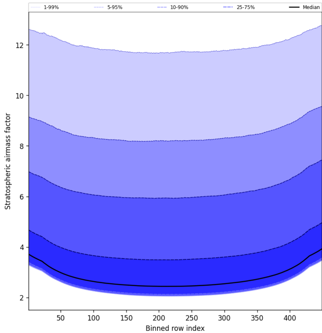
Figure 61: Along track statistics of “Stratospheric air mass factor” for 2025-01-13 to 2025-01-15
