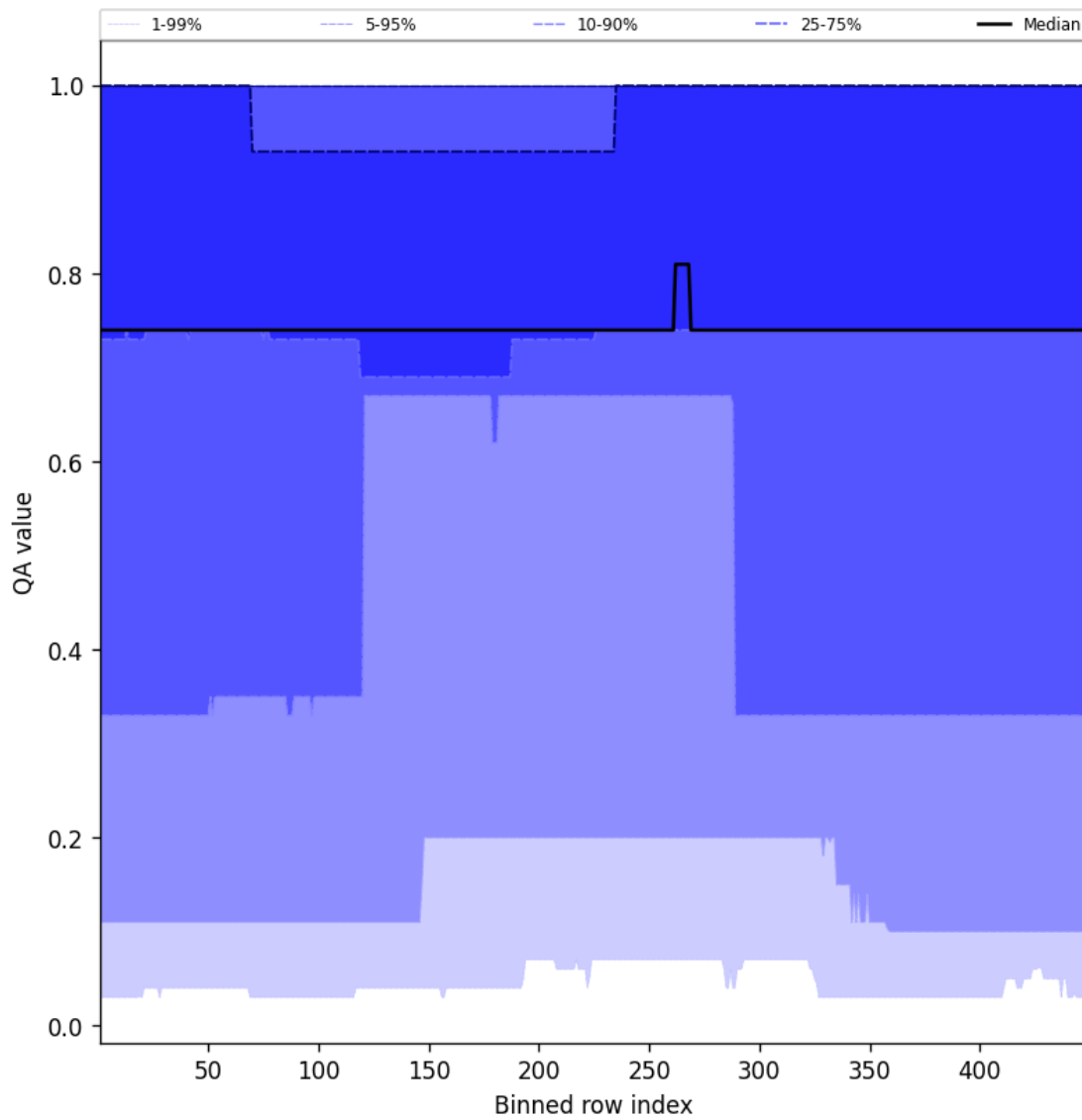
Figure 45: Along track statistics of “QA value” for 2025-01-13 to 2025-01-15
