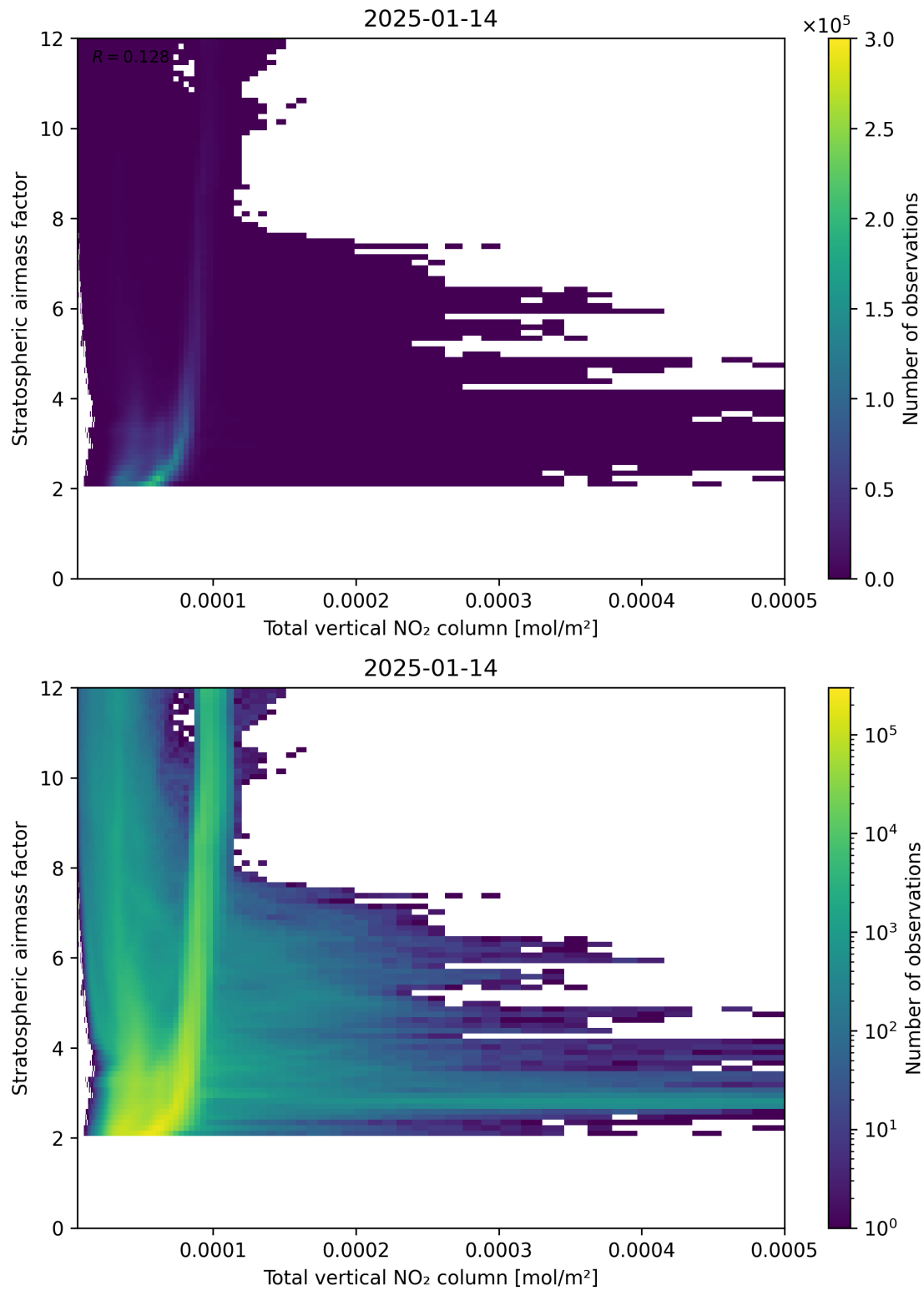
Figure 110: Scatter density plot of “Total vertical NO 2 column” against “Stratospheric airmass factor” for 2025-01-13 to 2025-01-15.
