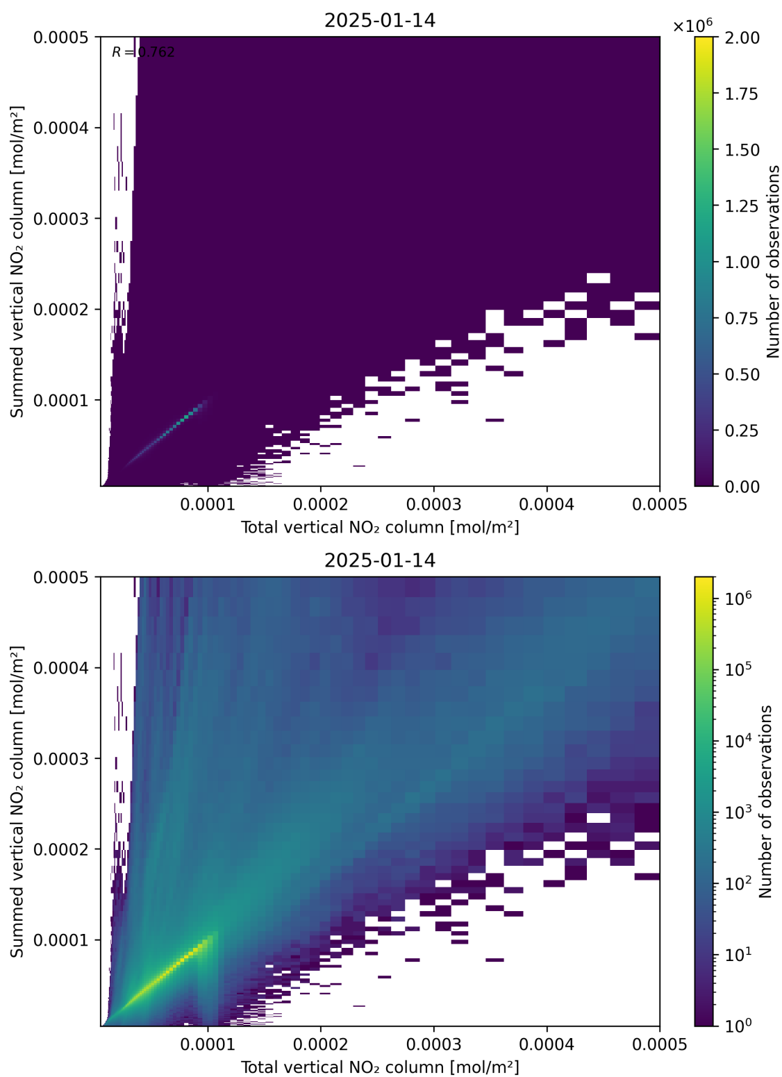
Figure 112: Scatter density plot of “Total vertical NO 2 column” against “Summed vertical NO 2 column” for 2025-01-13 to 2025-01-15.
