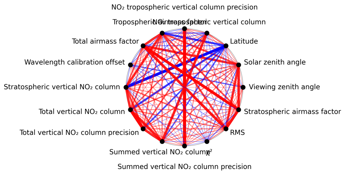
Figure 1: Map of correlation graph for 2025-01-13 to 2025-01-15.
