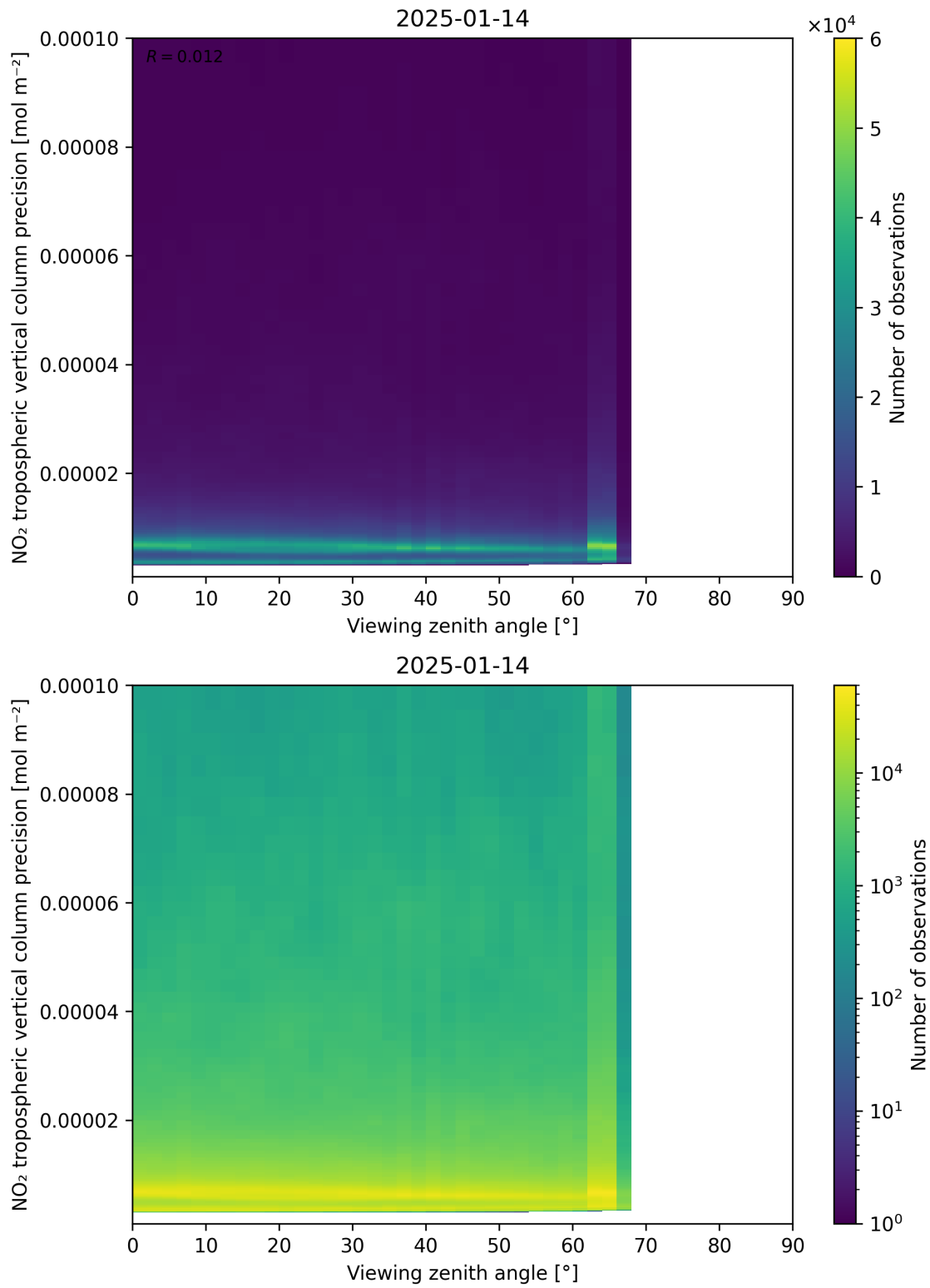
Figure 170: Scatter density plot of “Viewing zenith angle” against “NO 2 tropospheric vertical column precision” for 2025-01-13 to 2025-01-15.
