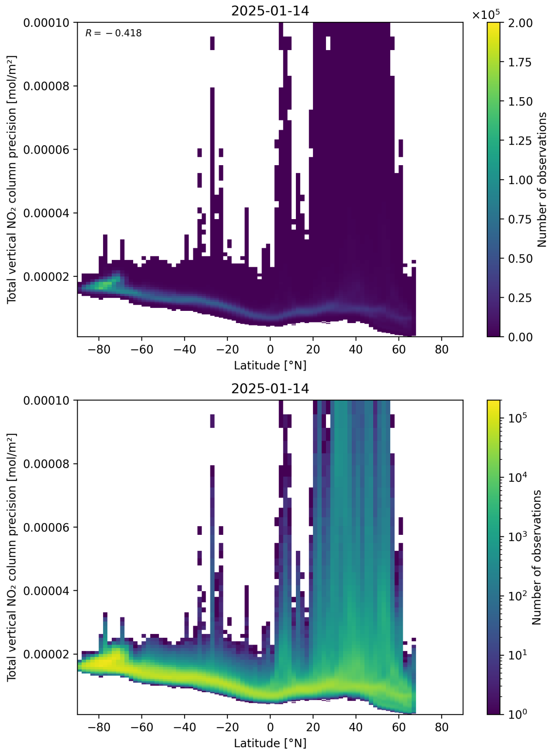
Figure 91: Scatter density plot of “Latitude” against “Total vertical NO 2 column precision” for 2025-01-13 to 2025-01-15.
