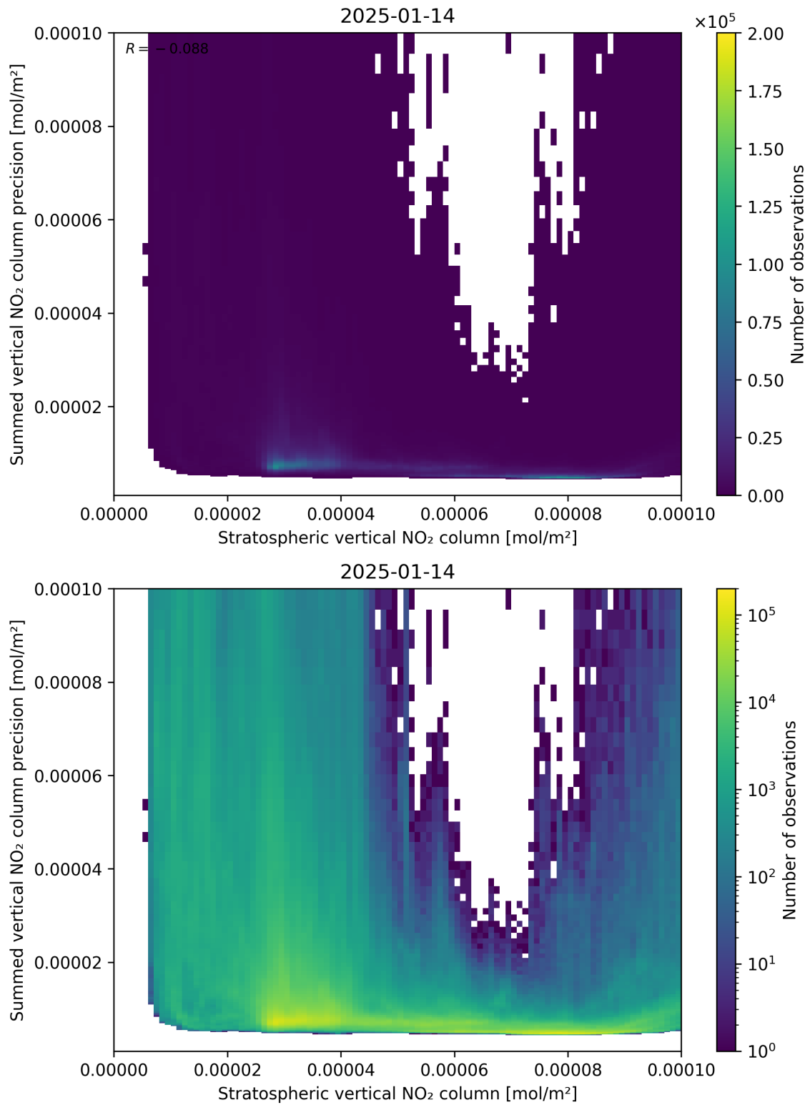
Figure 99: Scatter density plot of “Stratospheric vertical NO 2 column” against “Summed vertical NO 2 column precision” for 2025-01-13 to 2025-01-15.
