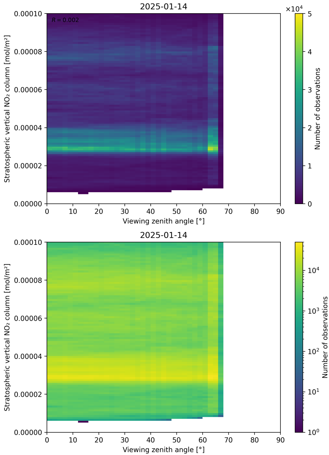
Figure 164: Scatter density plot of “Viewing zenith angle” against “Stratospheric vertical NO 2 column” for 2025-01-13 to 2025-01-15.
