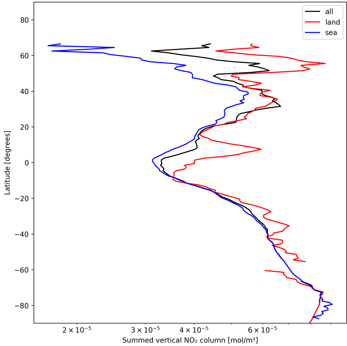
Figure 23: Zonal average of “Summed vertical NO 2 column” for 2025-01-13 to 2025-01-15.
