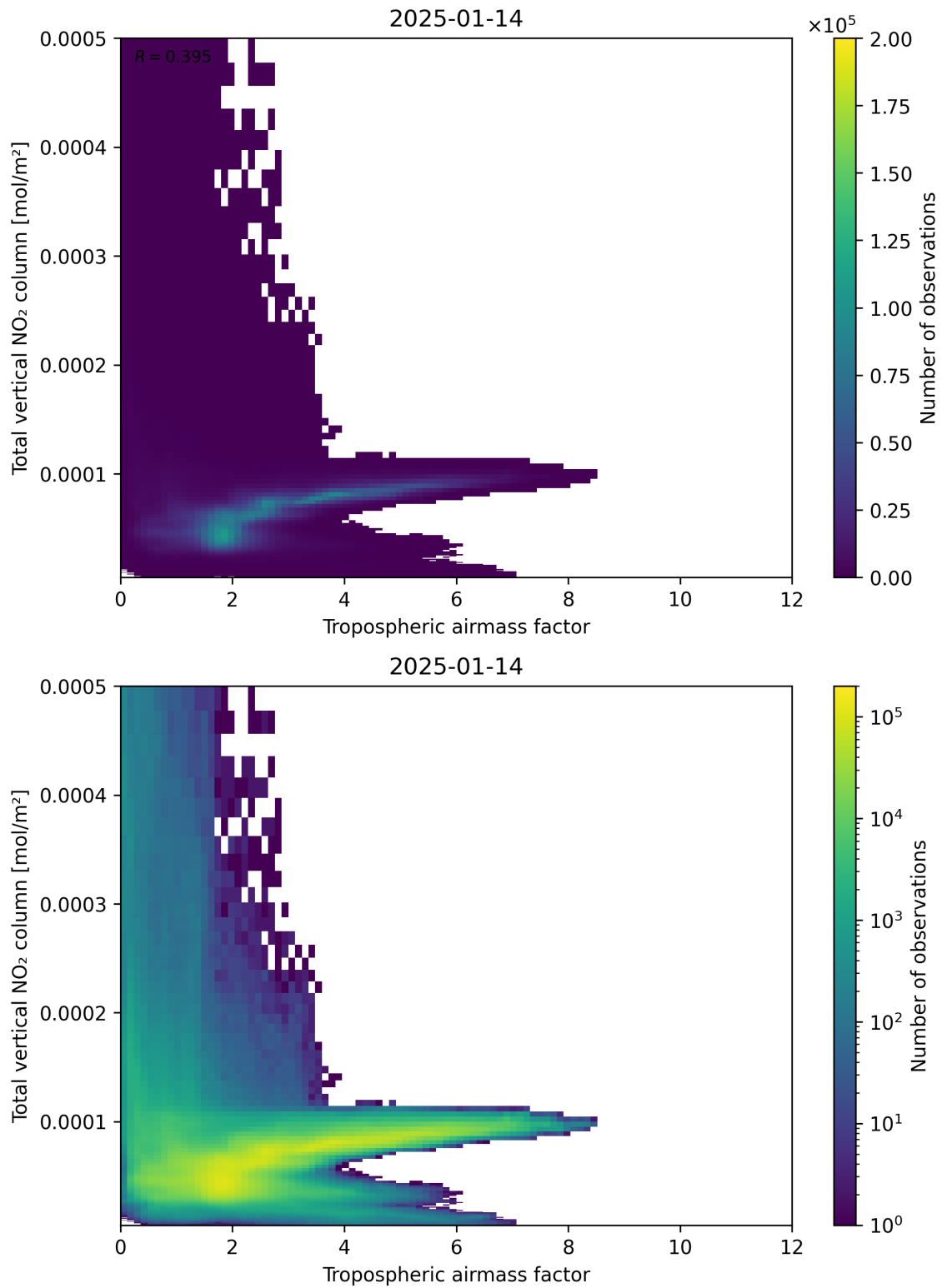
Figure 77: Scatter density plot of “Tropospheric airmass factor” against “Total vertical NO 2 column” for 2025-01-13 to 2025-01-15.
