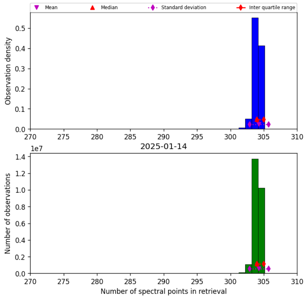
Figure 33: Histogram of “Number of spectral points in retrieval” for 2025-01-13 to 2025-01-15
