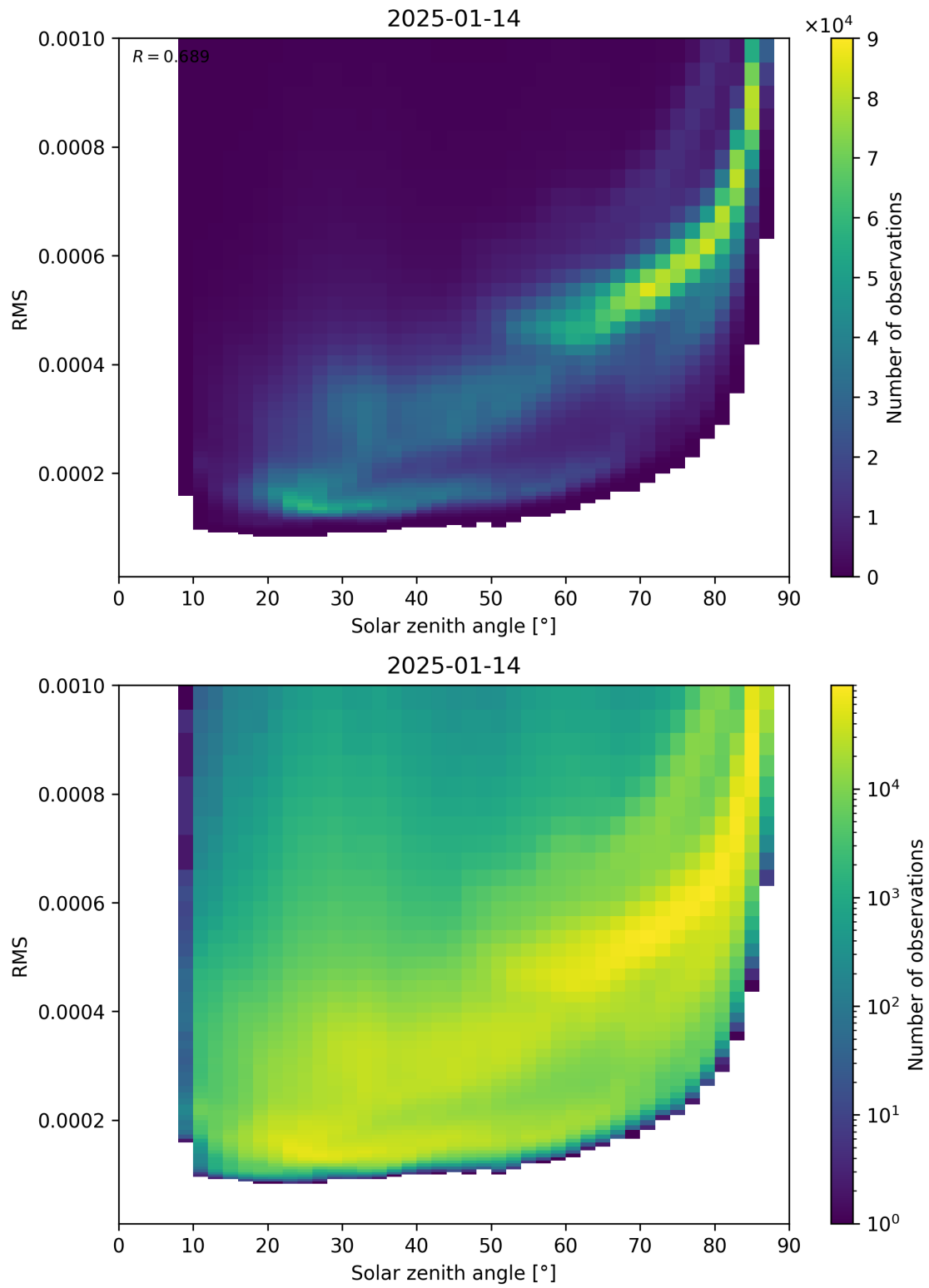
Figure 157: Scatter density plot of “Solar zenith angle” against “RMS” for 2025-01-13 to 2025-01-15.
