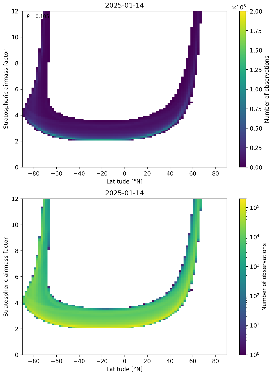
Figure 83: Scatter density plot of “Latitude” against “Stratospheric air mass factor” for 2025-01-13 to 2025-01-15.
