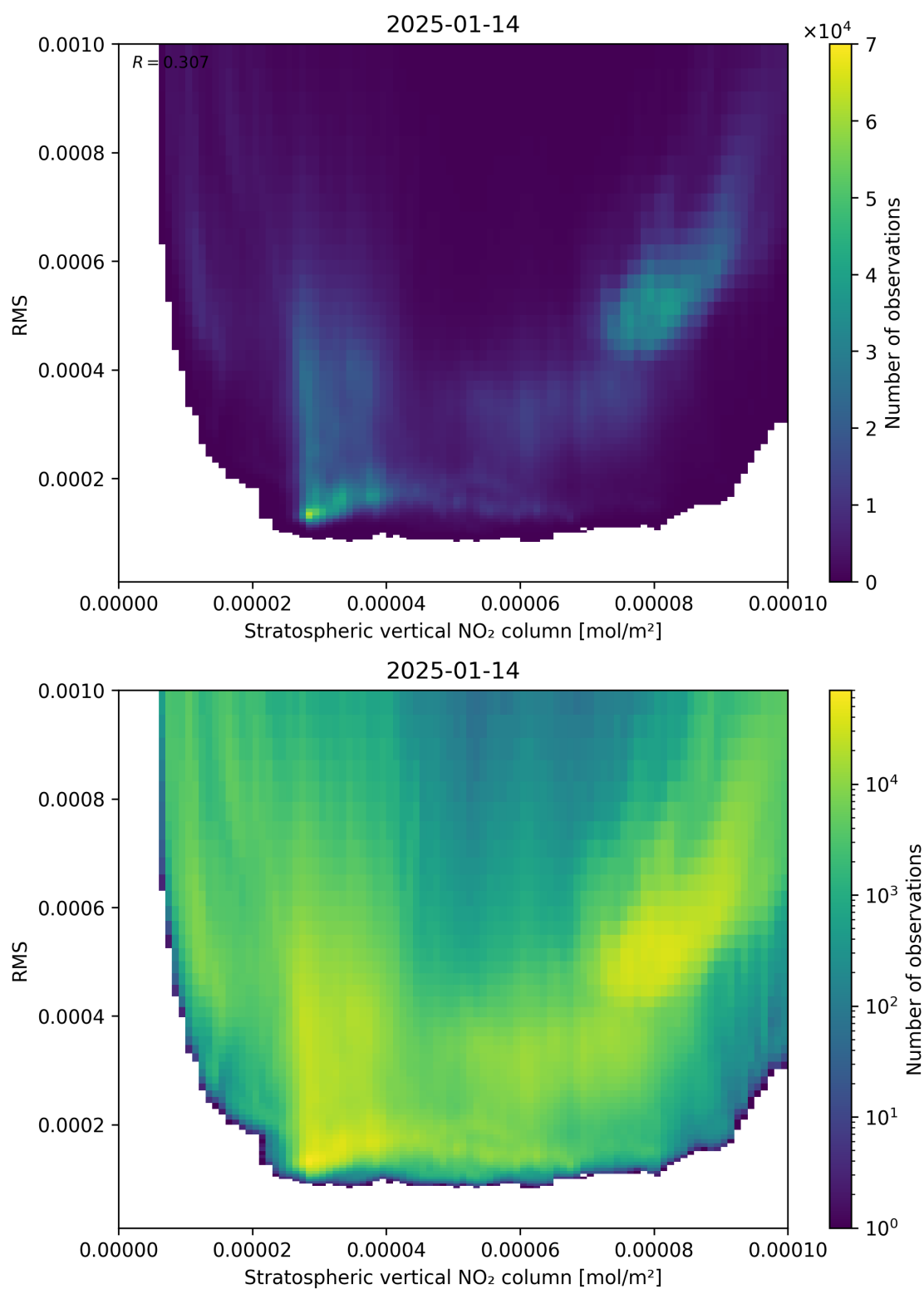
Figure 102: Scatter density plot of “Stratospheric vertical NO 2 column” against “RMS” for 2025-01-13 to 2025-01-15.
