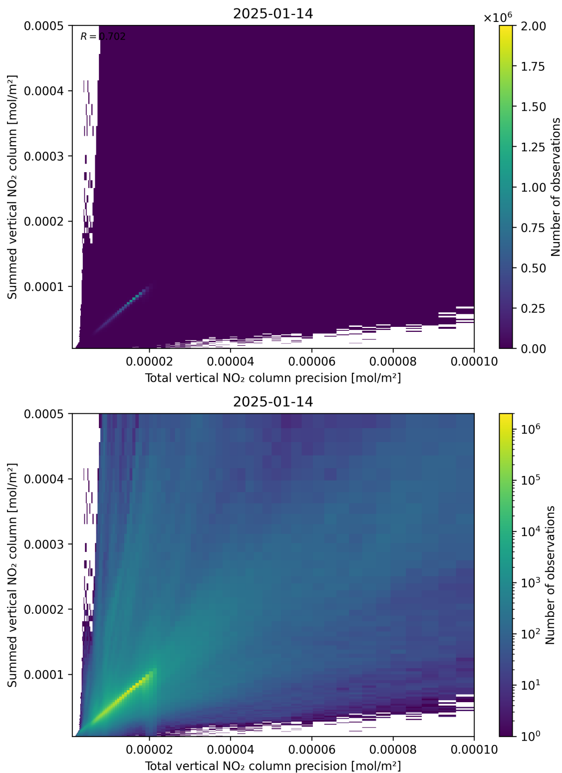
Figure 117: Scatter density plot of “Total vertical NO 2 column precision” against “Summed vertical NO 2 column” for 2025-01-13 to 2025-01-15.
