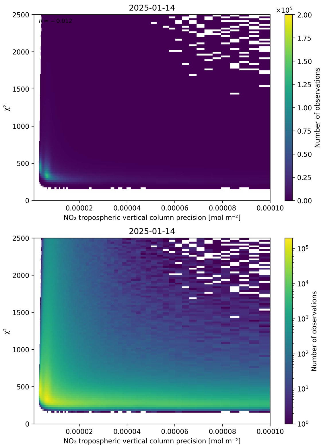
Figure 134: Scatter density plot of “NO 2 tropospheric vertical column precision” against “ \chi^2 ” for 2025-01-13 to 2025-01-15.
