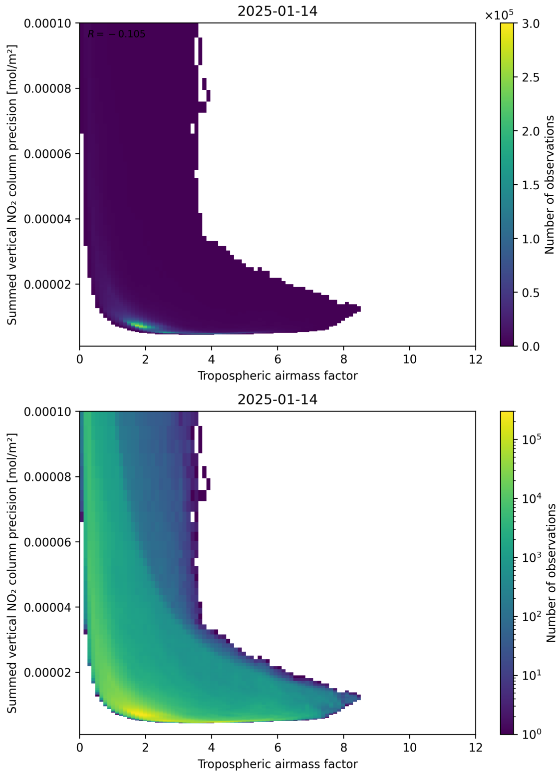
Figure 76: Scatter density plot of “Tropospheric air mass factor” against “Summed vertical NO 2 column precision” for 2025-01-13 to 2025-01-15.
