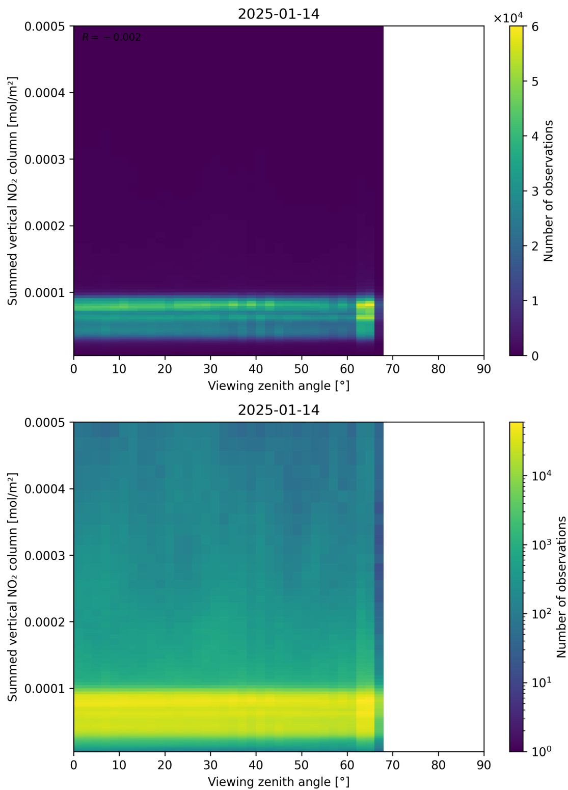
Figure 165: Scatter density plot of “Viewing zenith angle” against “Summed vertical NO 2 column” for 2025-01-13 to 2025-01-15.
