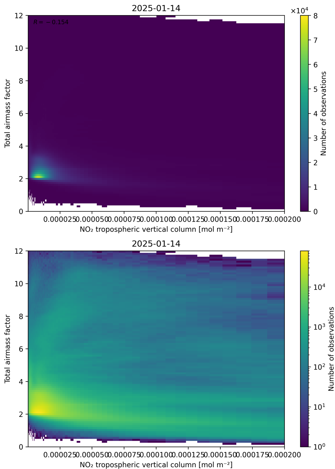
Figure 122: Scatter density plot of “NO 2 tropospheric vertical column” against “Total air mass factor” for 2025-01-13 to 2025-01-15.
