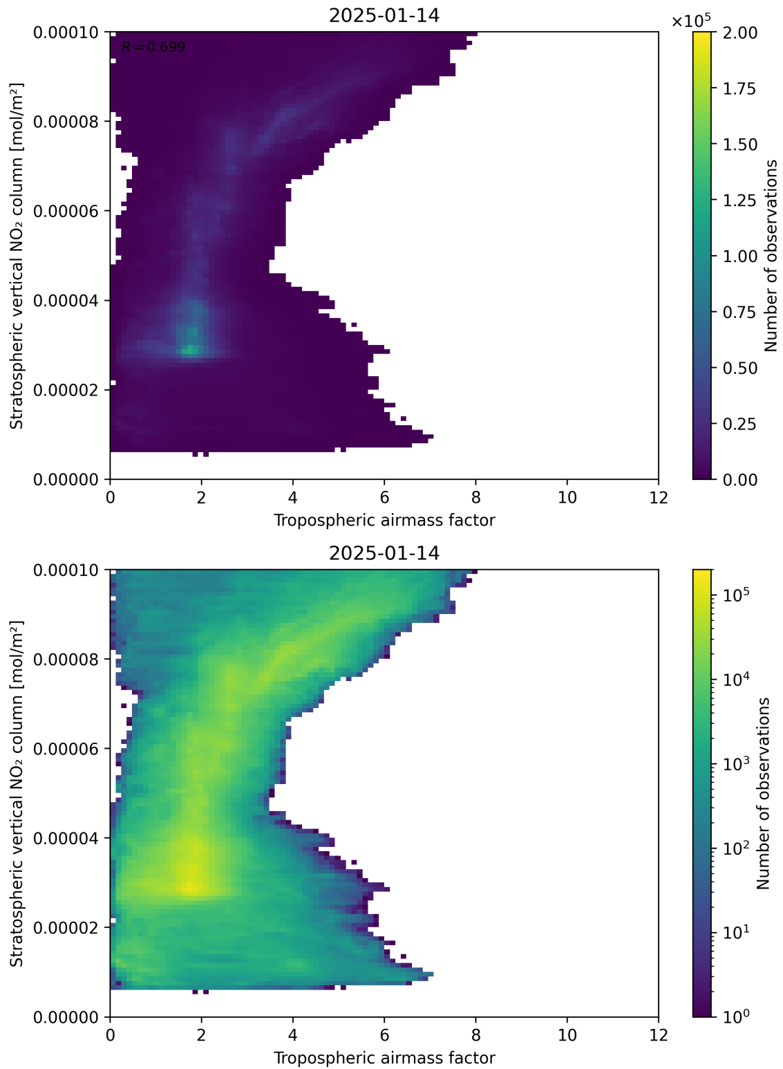
Figure 74: Scatter density plot of “Tropospheric air mass factor” against “Stratospheric vertical NO 2 column” for 2025-01-13 to 2025-01-15.
