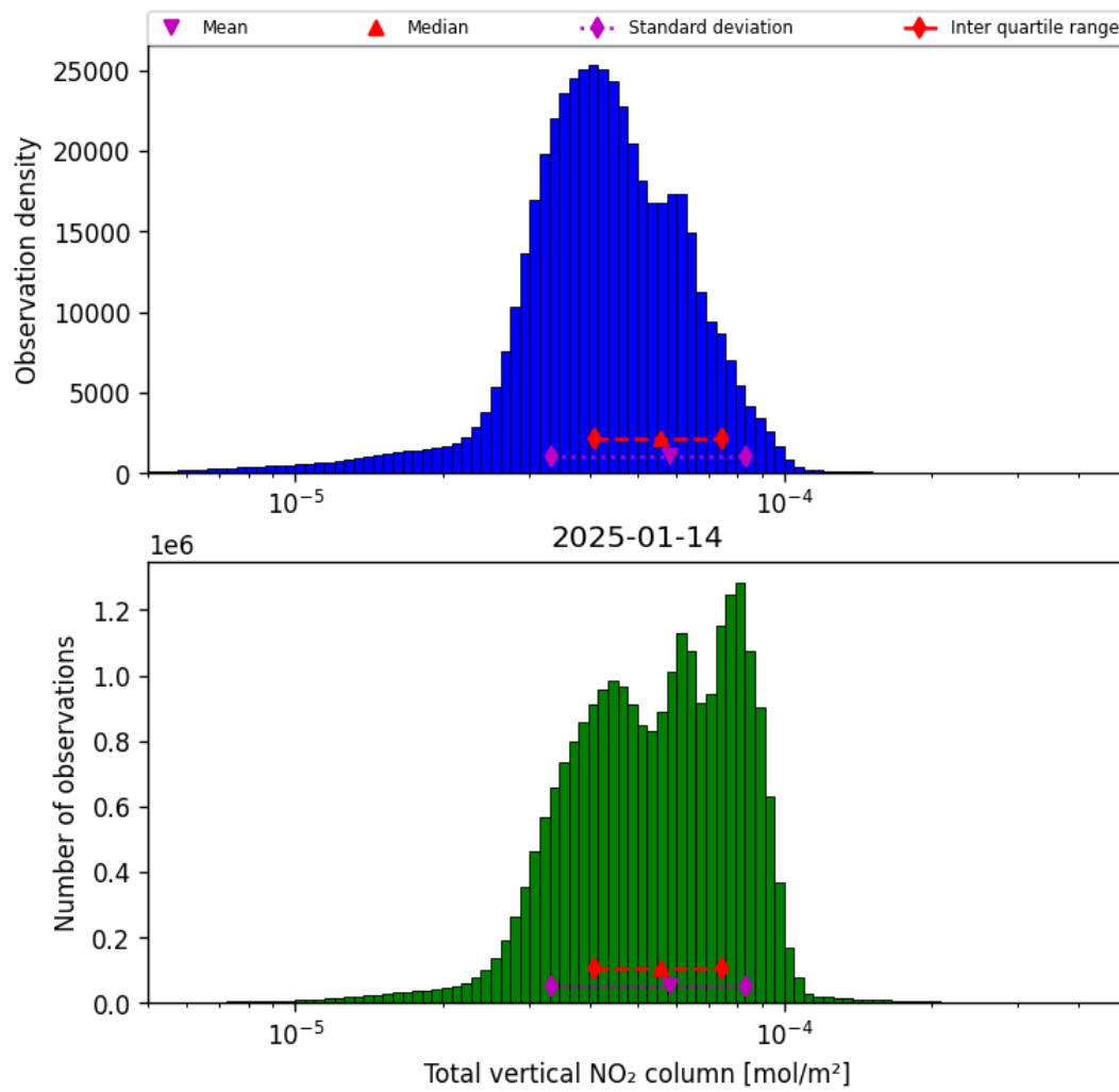
Figure 38: Histogram of “Total vertical NO 2 column” for 2025-01-13 to 2025-01-15
