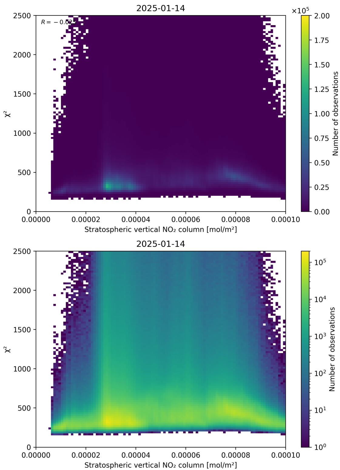
Figure 97: Scatter density plot of “Stratospheric vertical NO 2 column” against “ \chi^2 ” for 2025-01-13 to 2025-01-15.
