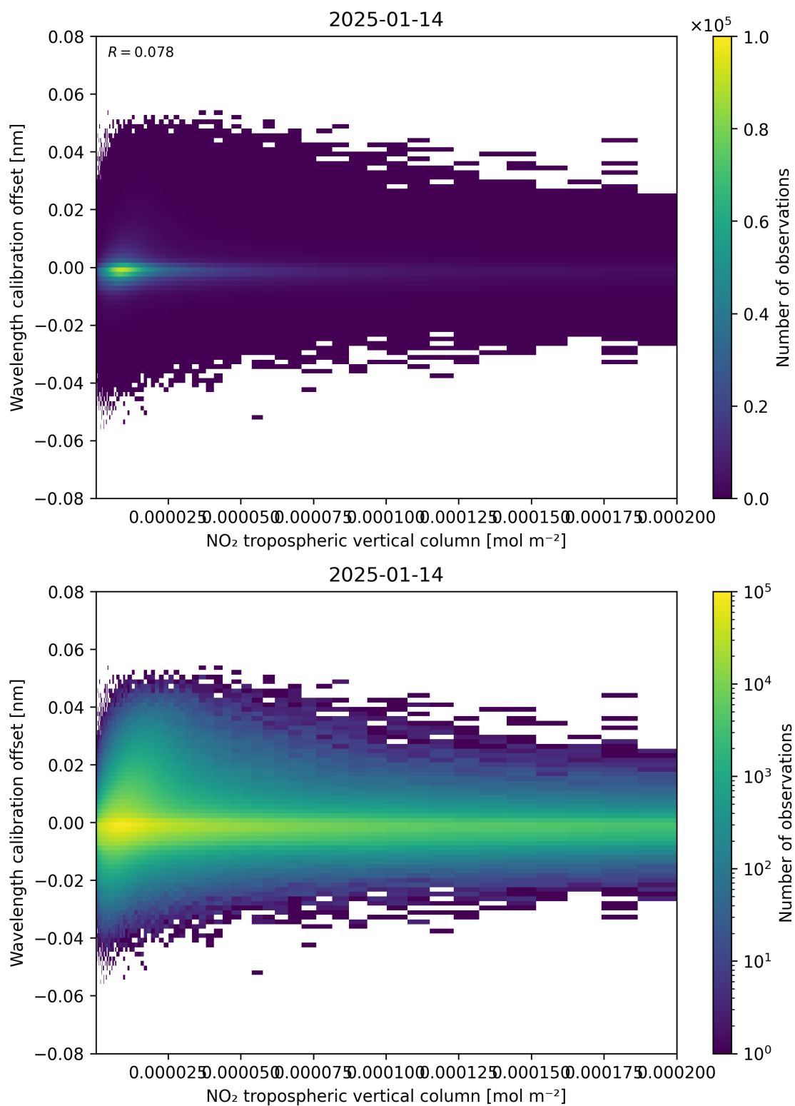
Figure 143: Scatter density plot of “NO 2 tropospheric vertical column” against “Wavelength calibration offset” for 2025-01-13 to 2025-01-15.
