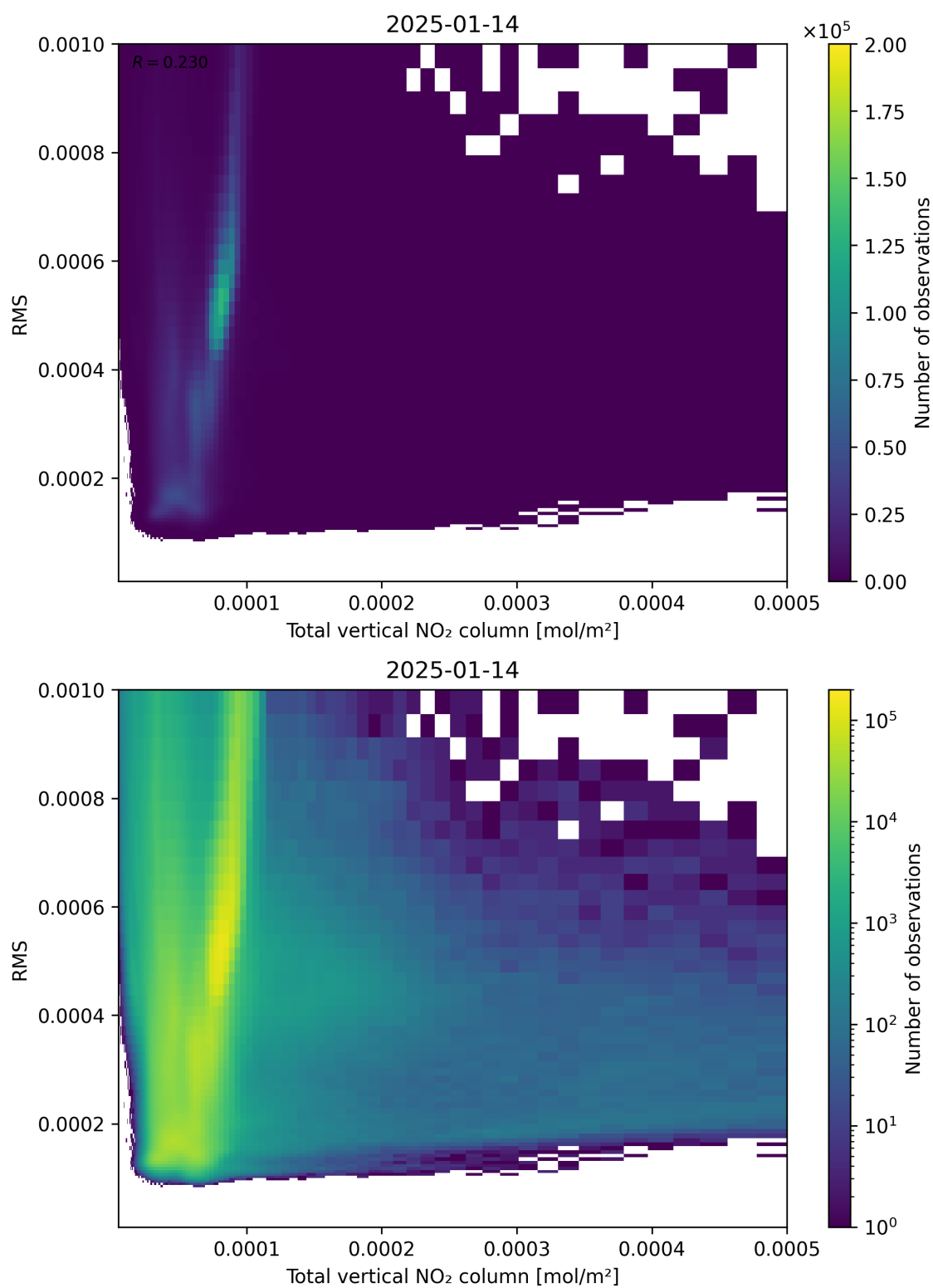
Figure 120: Scatter density plot of “Total vertical NO 2 column” against “RMS” for 2025-01-13 to 2025-01-15.
