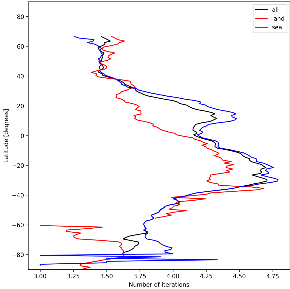
Figure 17: Zonal average of “Number of iterations” for 2025-01-13 to 2025-01-15.
