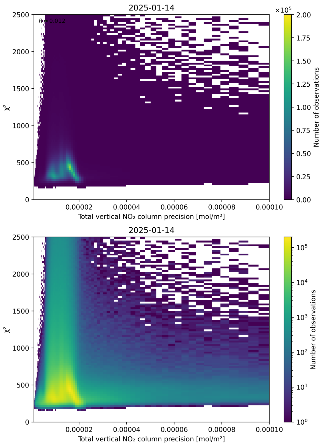
Figure 116: Scatter density plot of “Total vertical NO 2 column precision” against “ \chi^2 ” for 2025-01-13 to 2025-01-15.
