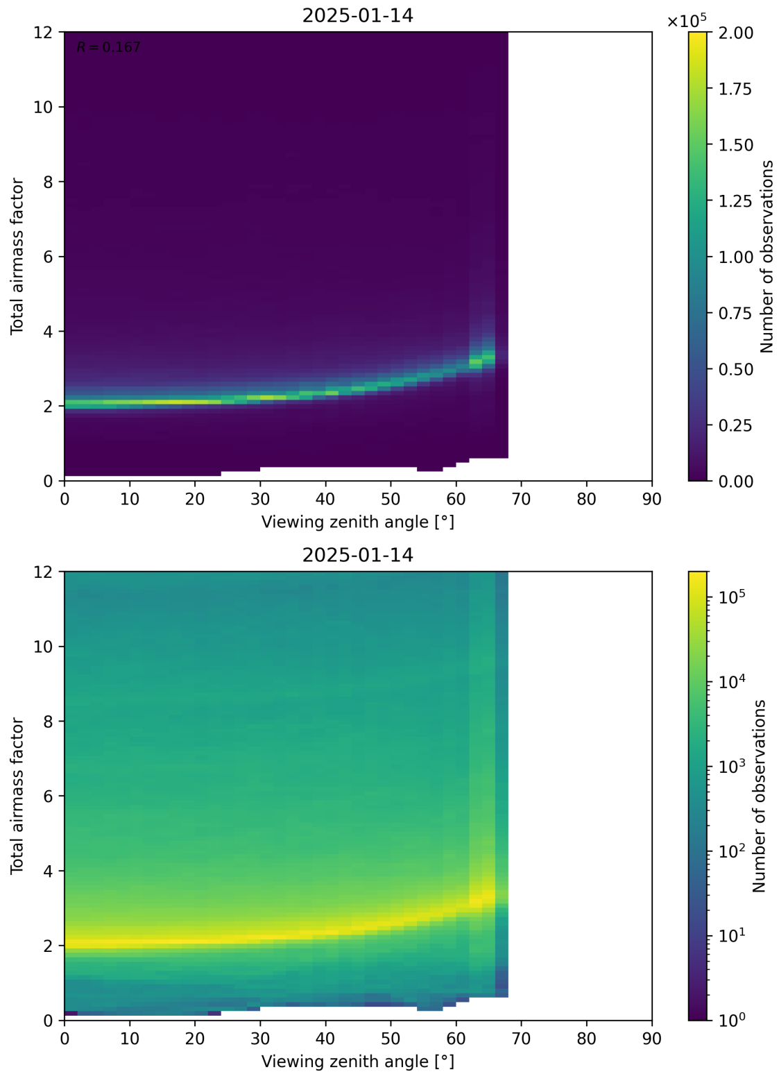
Figure 160: Scatter density plot of “Viewing zenith angle” against “Total airmass factor” for 2025-01-13 to 2025-01-15.
