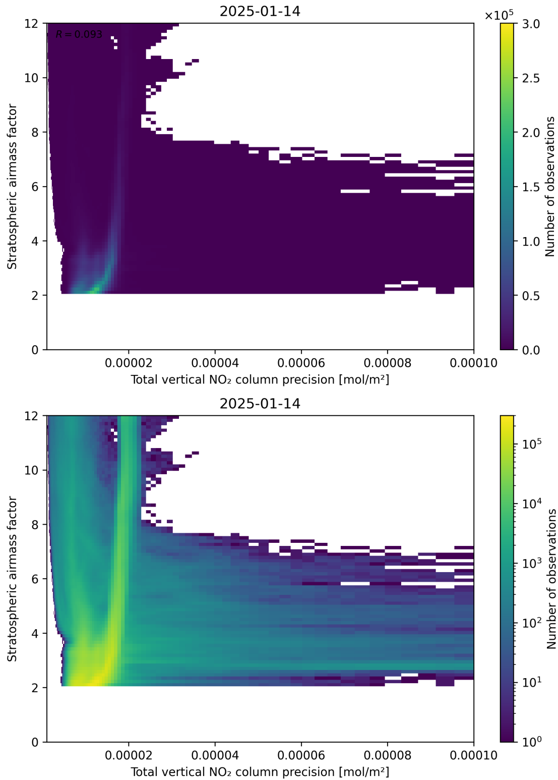
Figure 115: Scatter density plot of “Total vertical NO 2 column precision” against “Stratospheric airmass factor” for 2025-01-13 to 2025-01-15.
