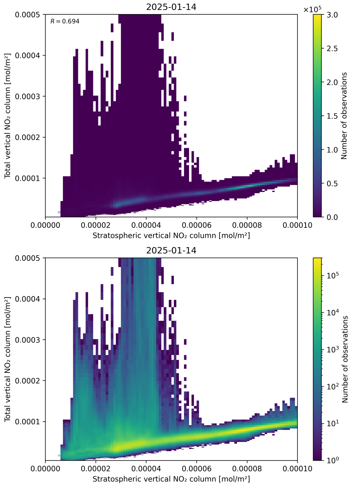
Figure 100: Scatter density plot of “Stratospheric vertical NO 2 column” against “Total vertical NO 2 column” for 2025-01-13 to 2025-01-15.
