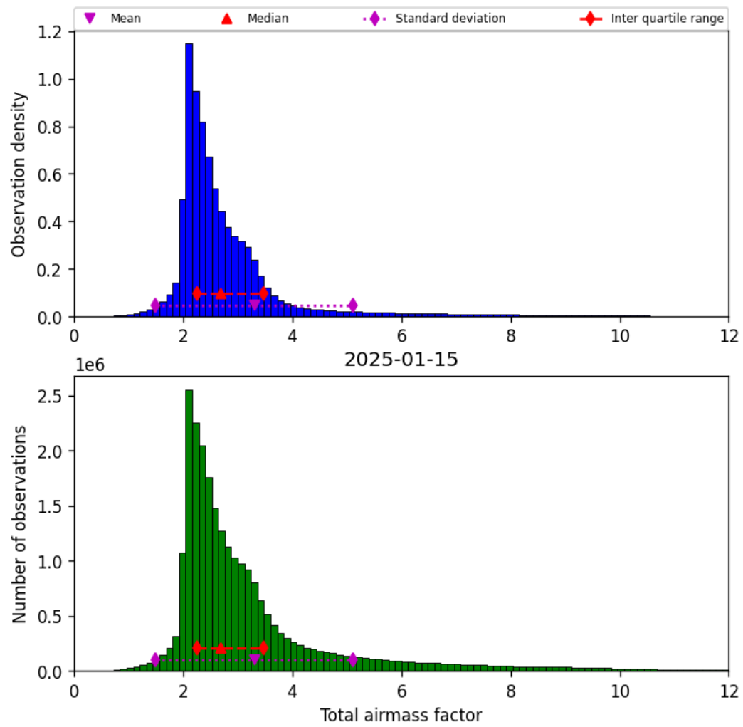
Figure 32: Histogram of “Total airmass factor” for 2025-01-14 to 2025-01-16
