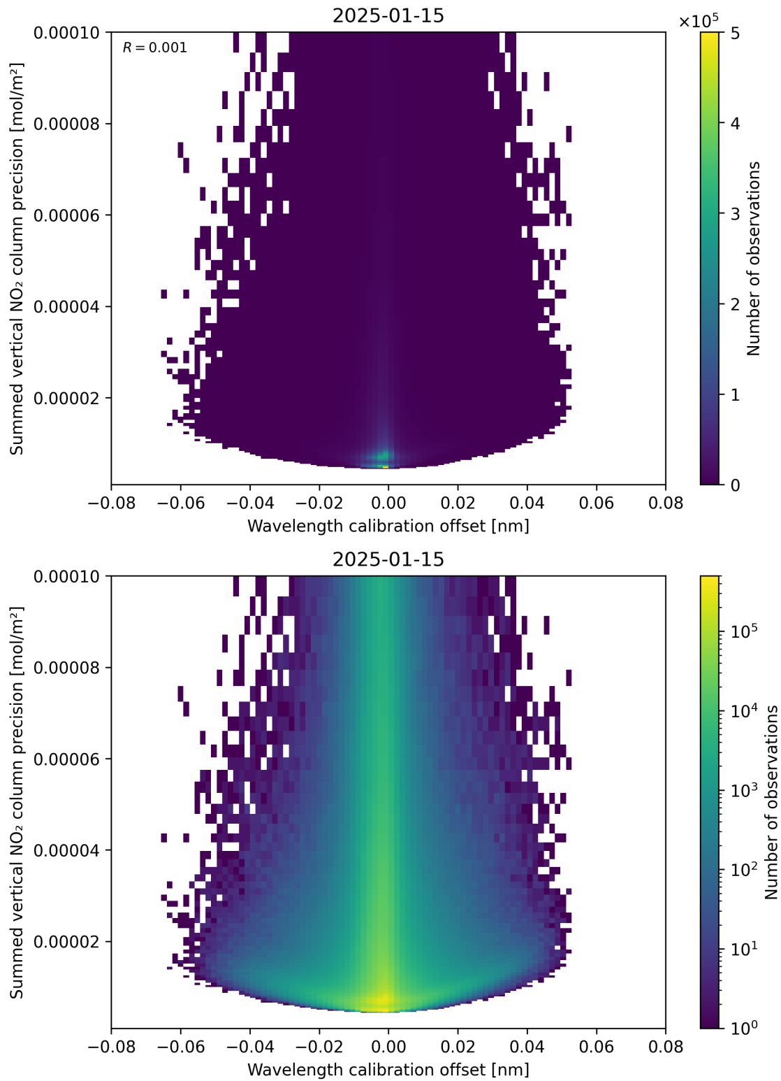
Figure 178: Scatter density plot of “Wavelength calibration offset” against “Summed vertical NO 2 column precision” for 2025-01-14 to 2025-01-16.
