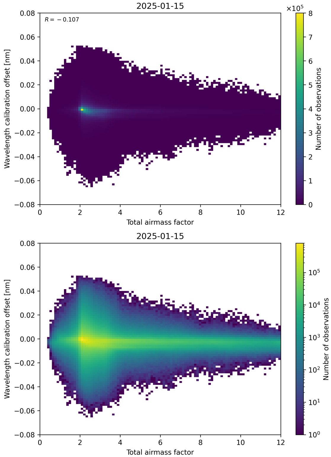
Figure 70: Scatter density plot of “Total airmass factor” against “Wavelength calibration offset” for 2025-01-14 to 2025-01-16.
