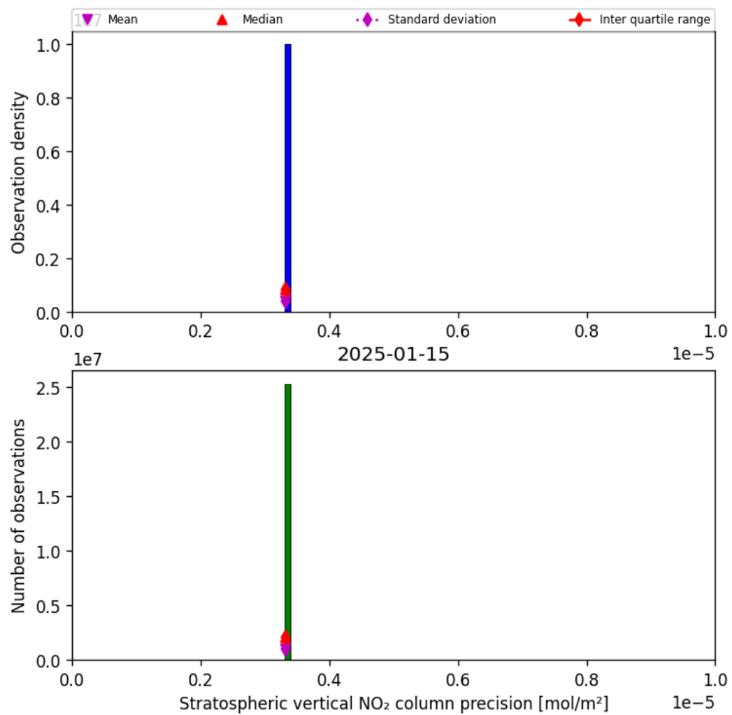
Figure 37: Histogram of “Stratospheric vertical NO 2 column precision” for 2025-01-14 to 2025-01-16
