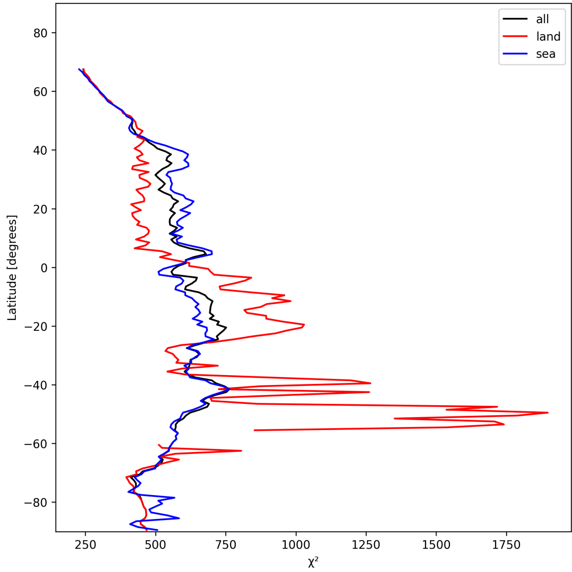
Figure 25: Zonal average of “ \chi^2 ” for 2025-01-14 to 2025-01-16.
