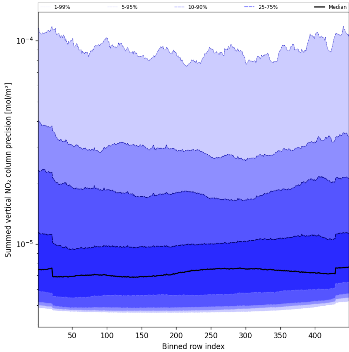
Figure 58: Along track statistics of “Summed vertical NO 2 column precision” for 2025-01-14 to 2025-01-16
