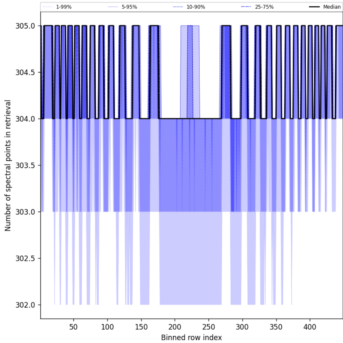
Figure 50: Along track statistics of “Number of spectral points in retrieval” for 2025-01-14 to 2025-01-16
