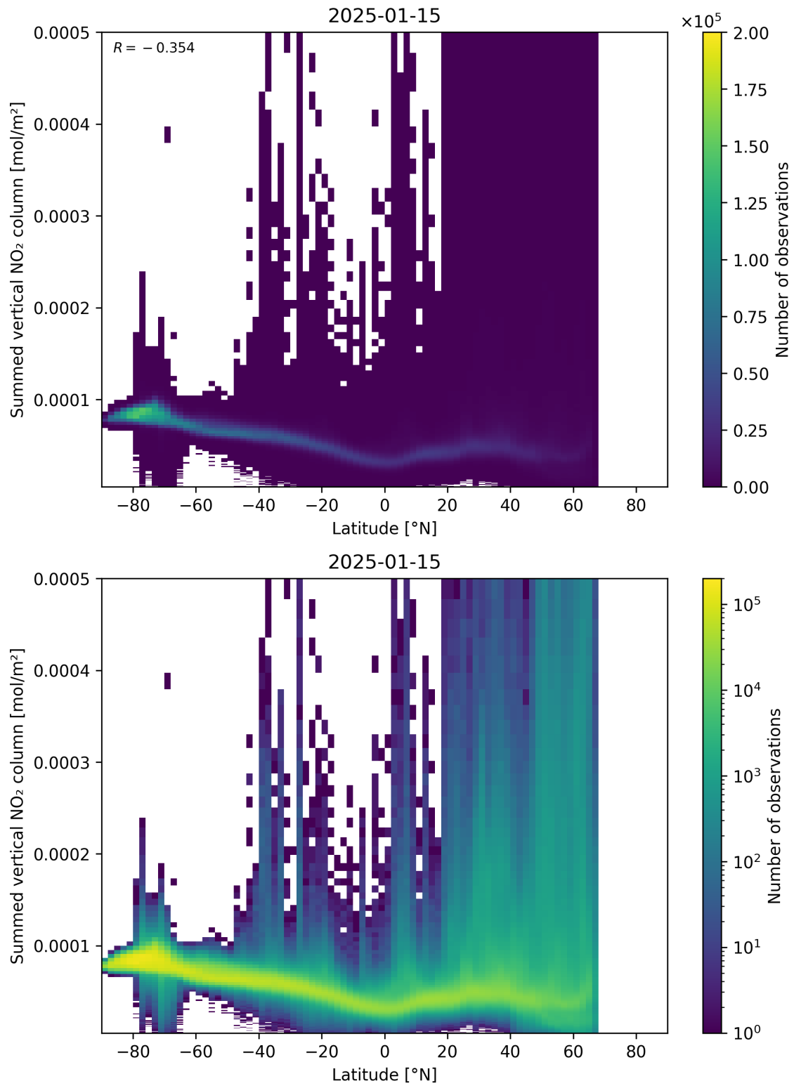
Figure 88: Scatter density plot of “Latitude” against “Summed vertical NO 2 column” for 2025-01-14 to 2025-01-16.
