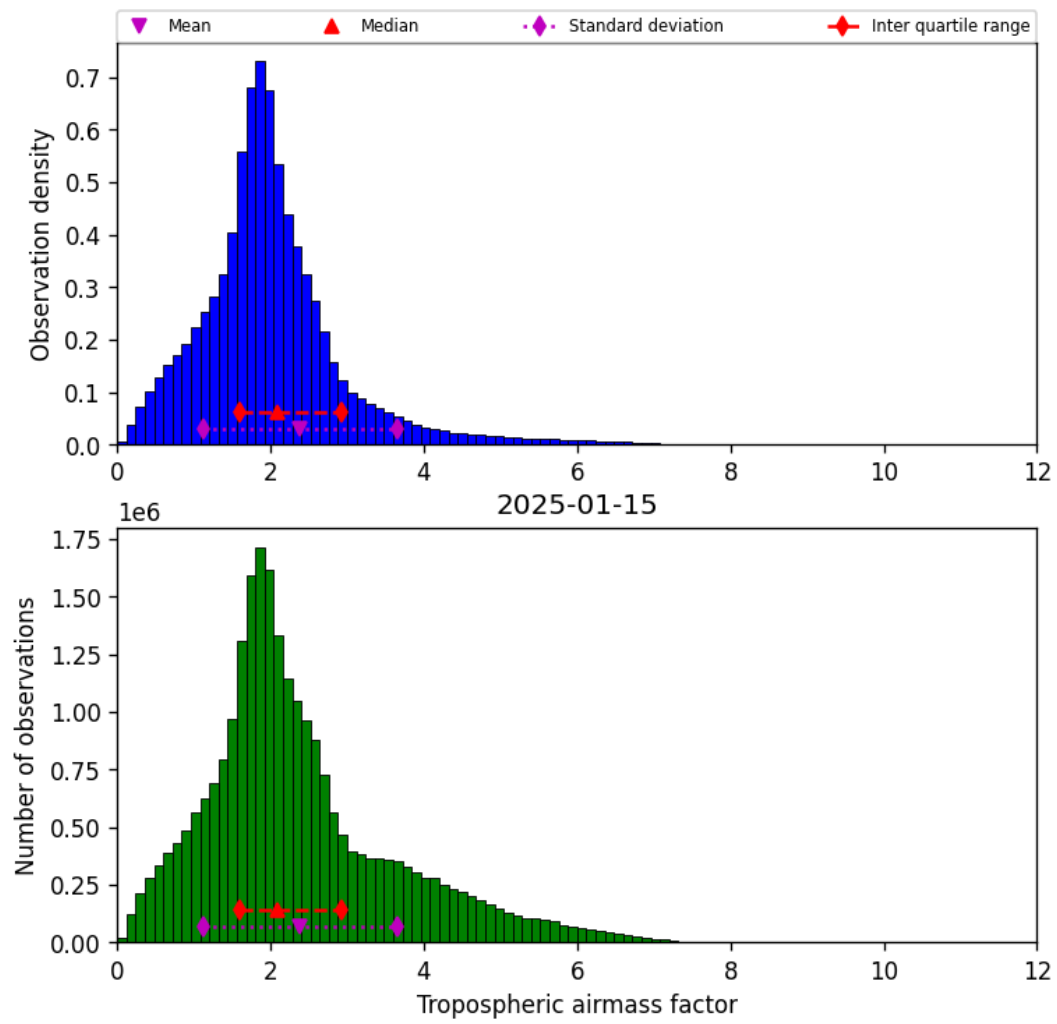
Figure 31: Histogram of “Tropospheric airmass factor” for 2025-01-14 to 2025-01-16
