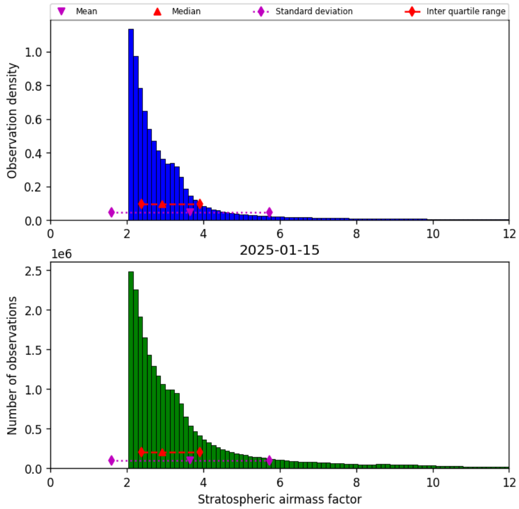
Figure 44: Histogram of “Stratospheric airmass factor” for 2025-01-14 to 2025-01-16
