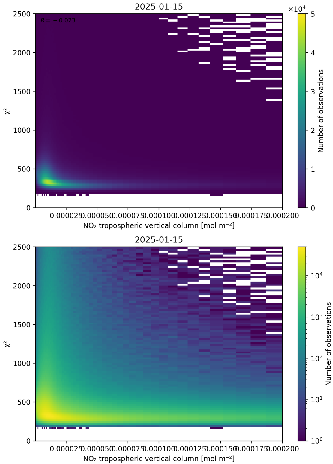
Figure 124: Scatter density plot of “NO 2 tropospheric vertical column” against “ \chi^2 ” for 2025-01-14 to 2025-01-16.
