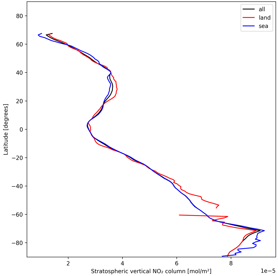
Figure 19: Zonal average of “Stratospheric vertical NO 2 column” for 2025-01-14 to 2025-01-16.
