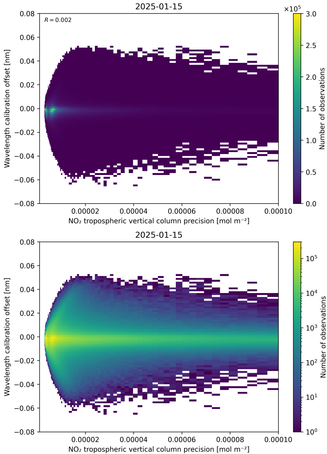
Figure 141: Scatter density plot of “NO 2 tropospheric vertical column precision” against “Wavelength calibration offset” for 2025-01-14 to 2025-01-16.
