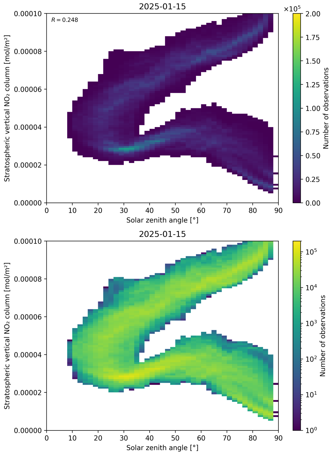
Figure 150: Scatter density plot of “Solar zenith angle” against “Stratospheric vertical \text{NO}_2 column” for 2025-01-14 to 2025-01-16.
