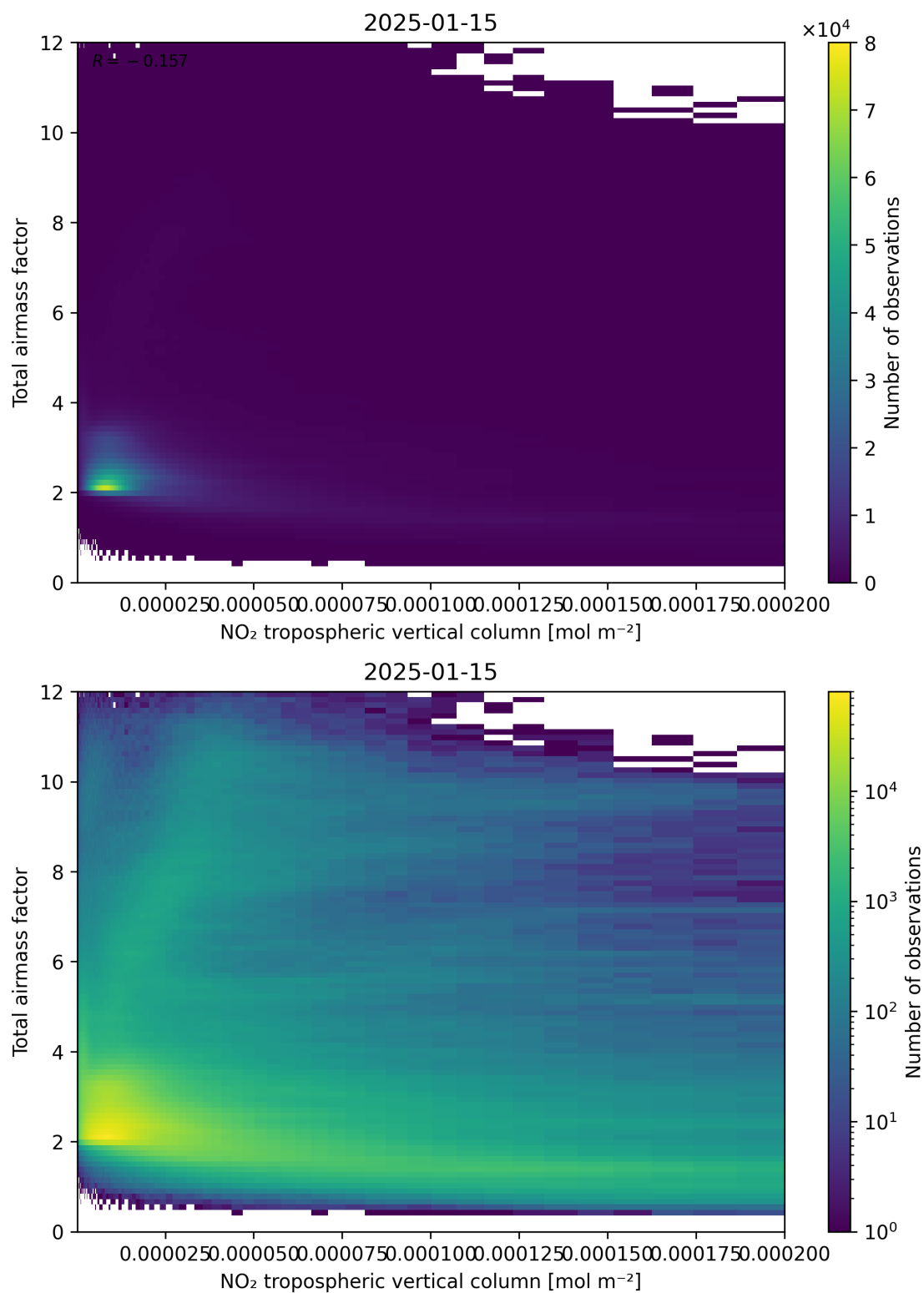
Figure 122: Scatter density plot of “NO 2 tropospheric vertical column” against “Total air mass factor” for 2025-01-14 to 2025-01-16.
