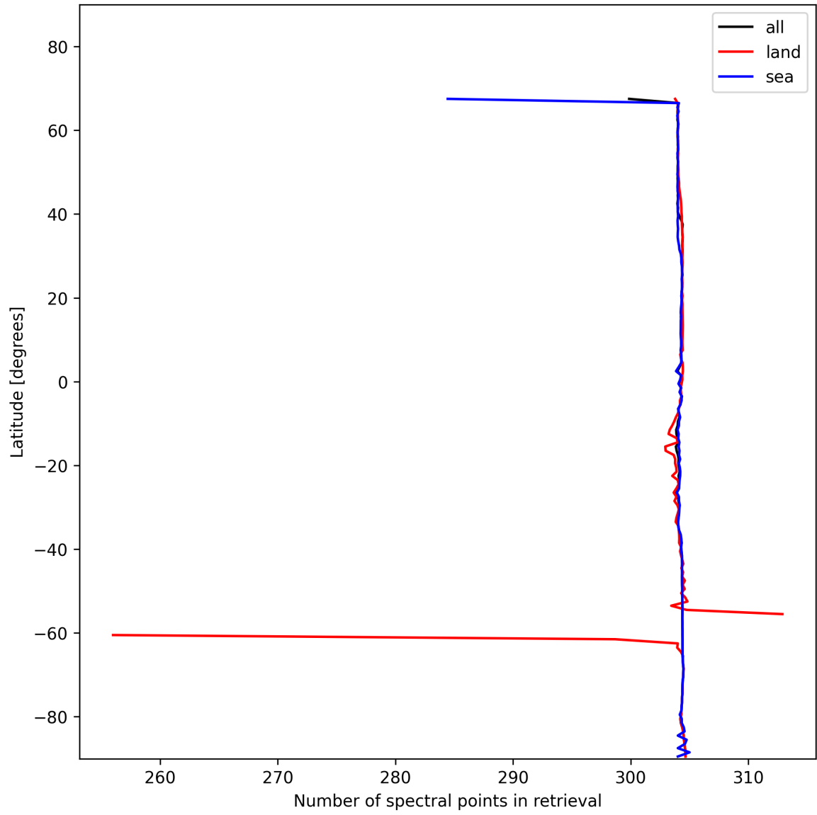
Figure 16: Zonal average of “Number of spectral points in retrieval” for 2025-01-14 to 2025-01-16.
