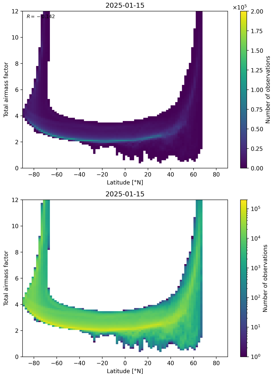
Figure 84: Scatter density plot of “Latitude” against “Total airmass factor” for 2025-01-14 to 2025-01-16.
