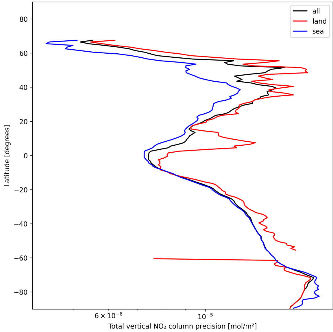
Figure 22: Zonal average of “Total vertical NO 2 column precision” for 2025-01-14 to 2025-01-16.
