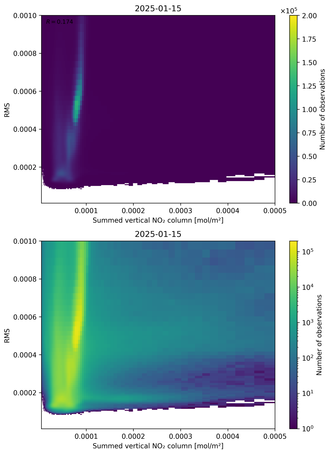
Figure 109: Scatter density plot of “Summed vertical NO 2 column” against “RMS” for 2025-01-14 to 2025-01-16.
