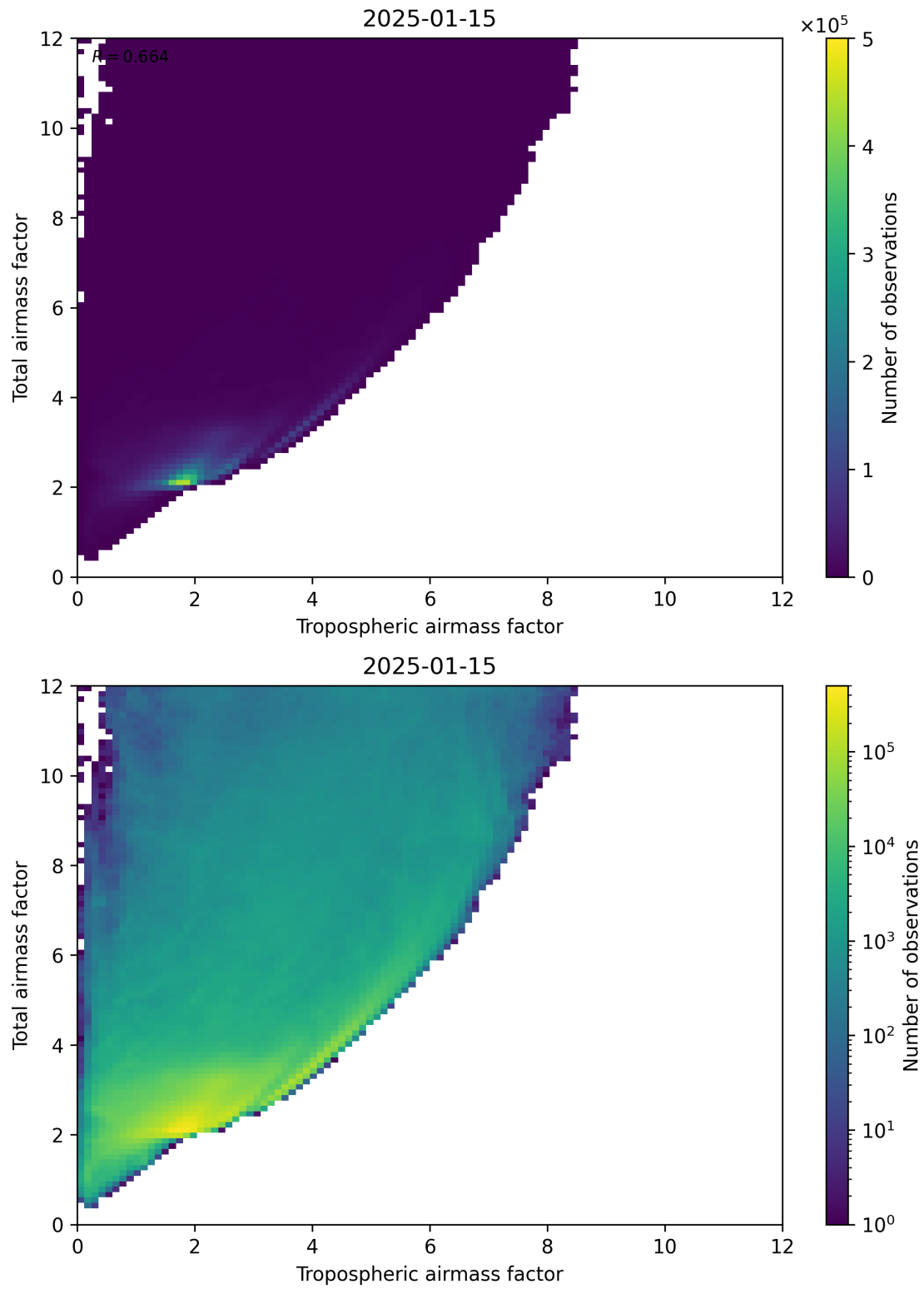
Figure 72: Scatter density plot of “Tropospheric airmass factor” against “Total airmass factor” for 2025-01-14 to 2025-01-16.
