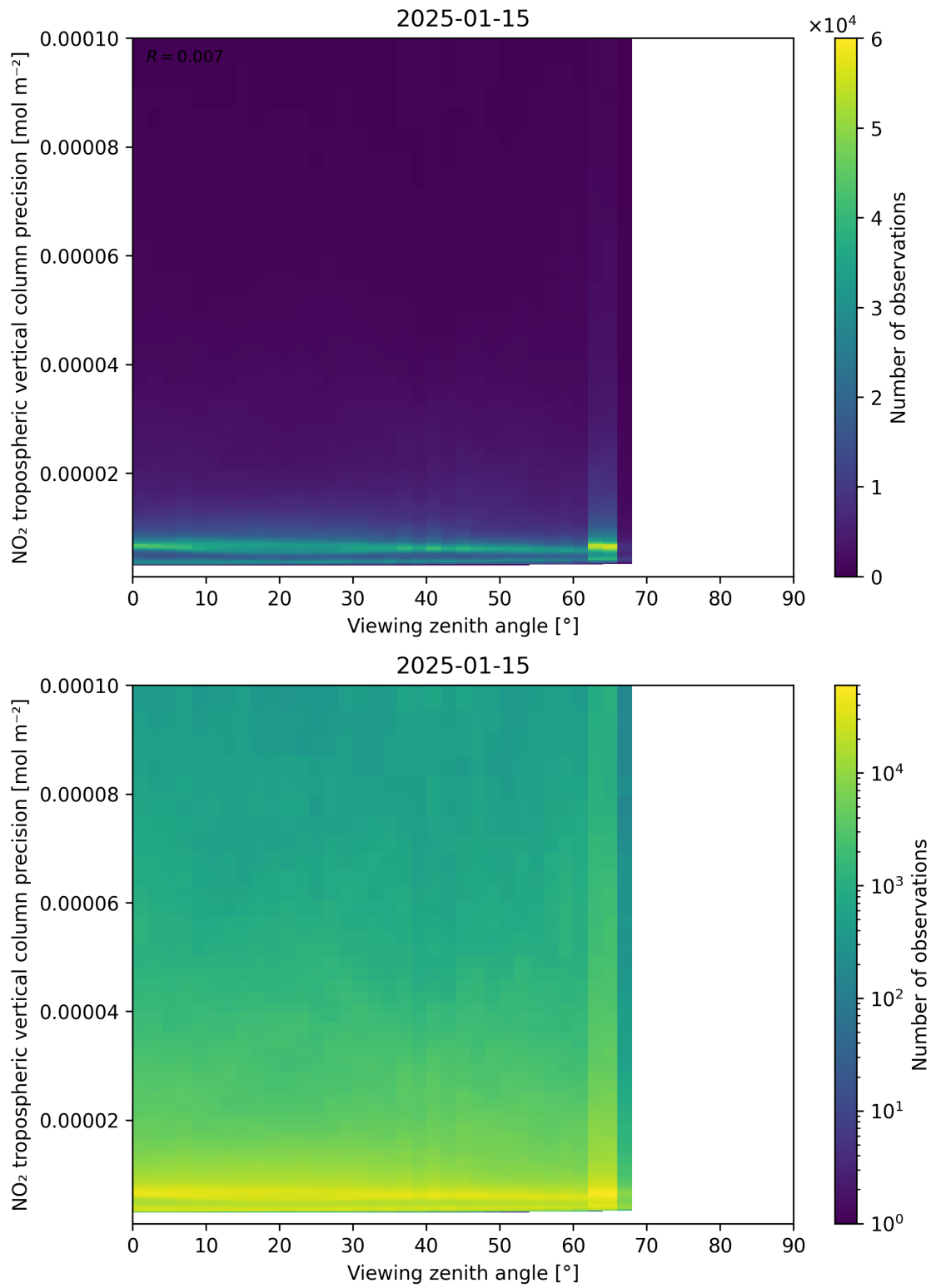
Figure 170: Scatter density plot of “Viewing zenith angle” against “NO 2 tropospheric vertical column precision” for 2025-01-14 to 2025-01-16.
