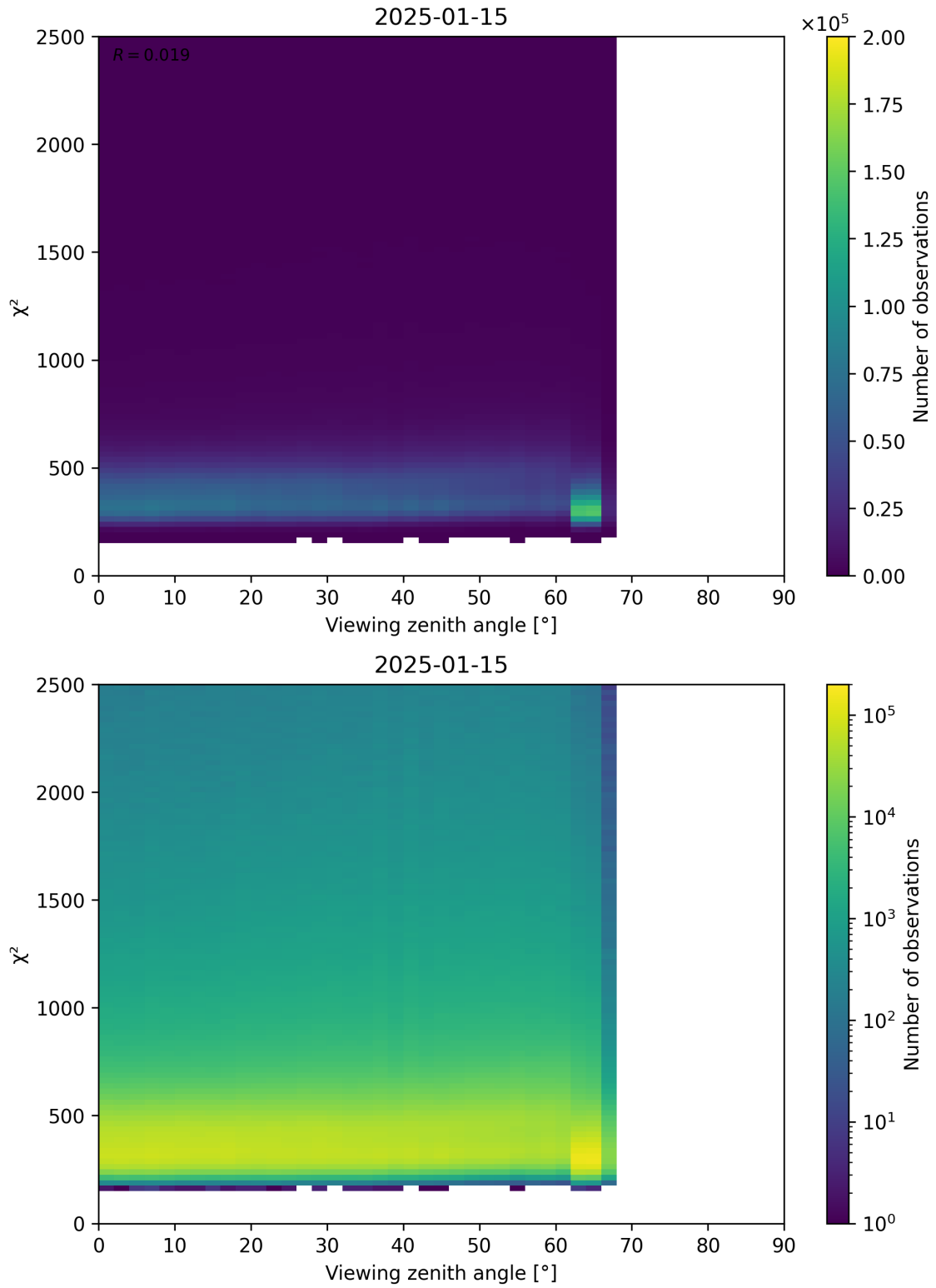
Figure 162: Scatter density plot of “Viewing zenith angle” against “ \chi^2 ” for 2025-01-14 to 2025-01-16.
