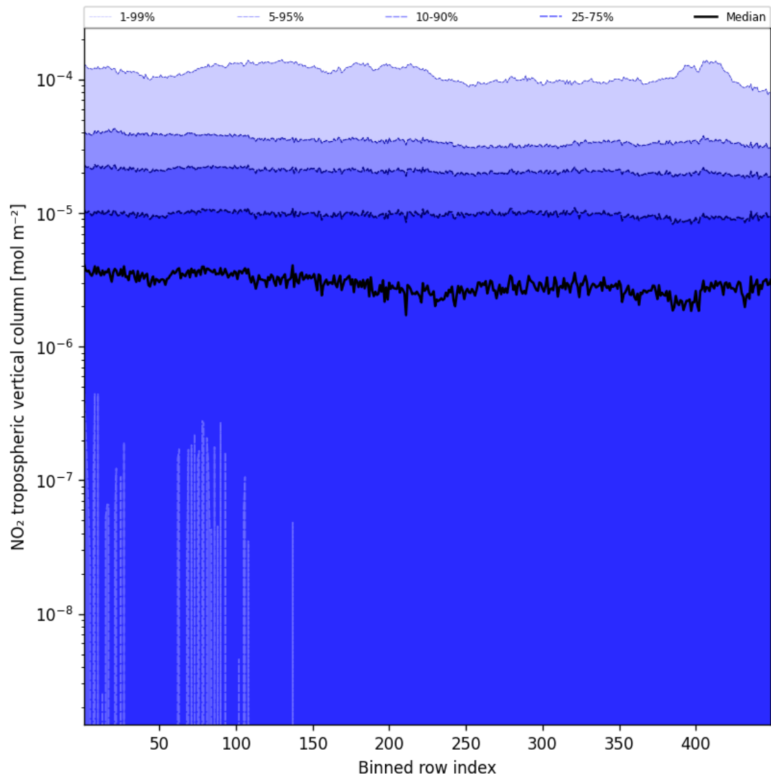
Figure 46: Along track statistics of “NO 2 tropospheric vertical column” for 2025-01-14 to 2025-01-16
