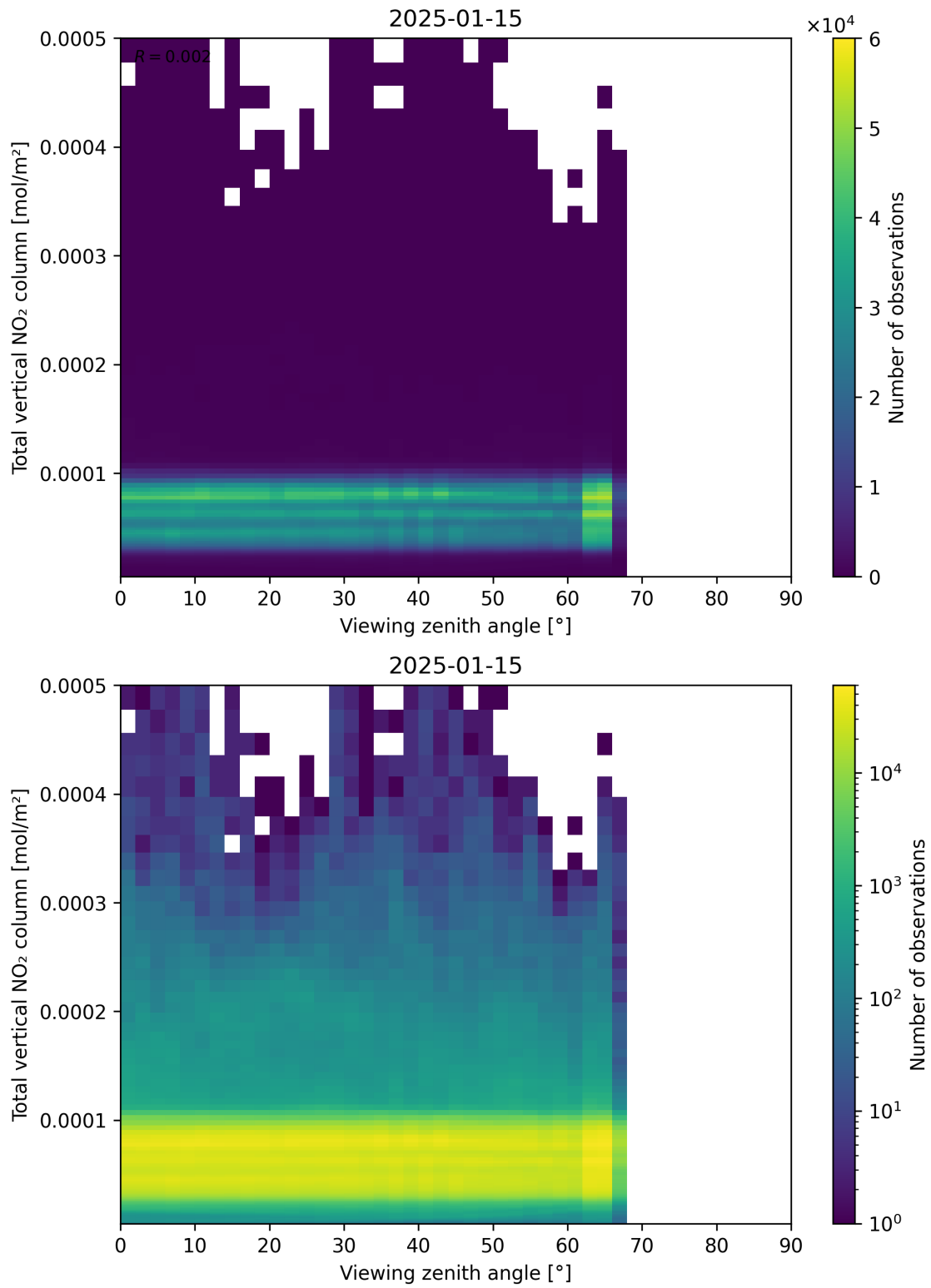
Figure 167: Scatter density plot of “Viewing zenith angle” against “Total vertical NO 2 column” for 2025-01-14 to 2025-01-16.
