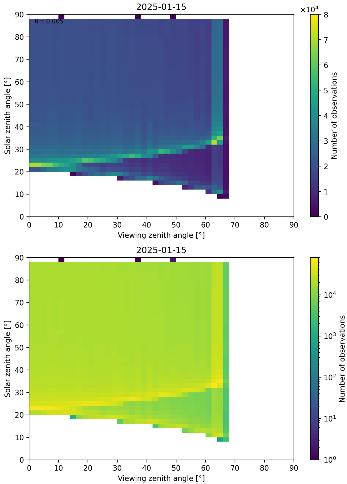
Figure 172: Scatter density plot of “Viewing zenith angle” against “Solar zenith angle” for 2025-01-14 to 2025-01-16.
