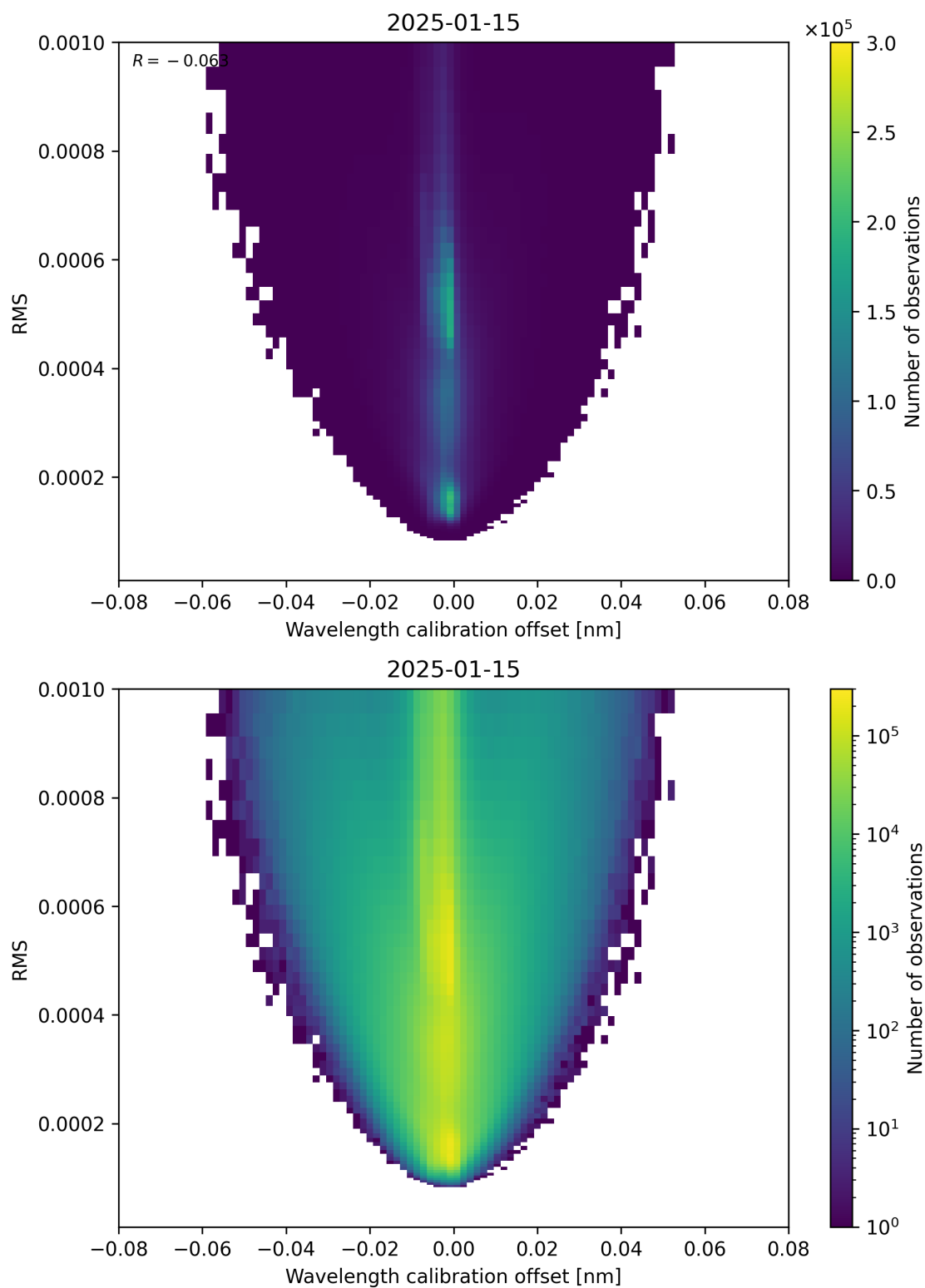
Figure 181: Scatter density plot of “Wavelength calibration offset” against “RMS” for 2025-01-14 to 2025-01-16.
