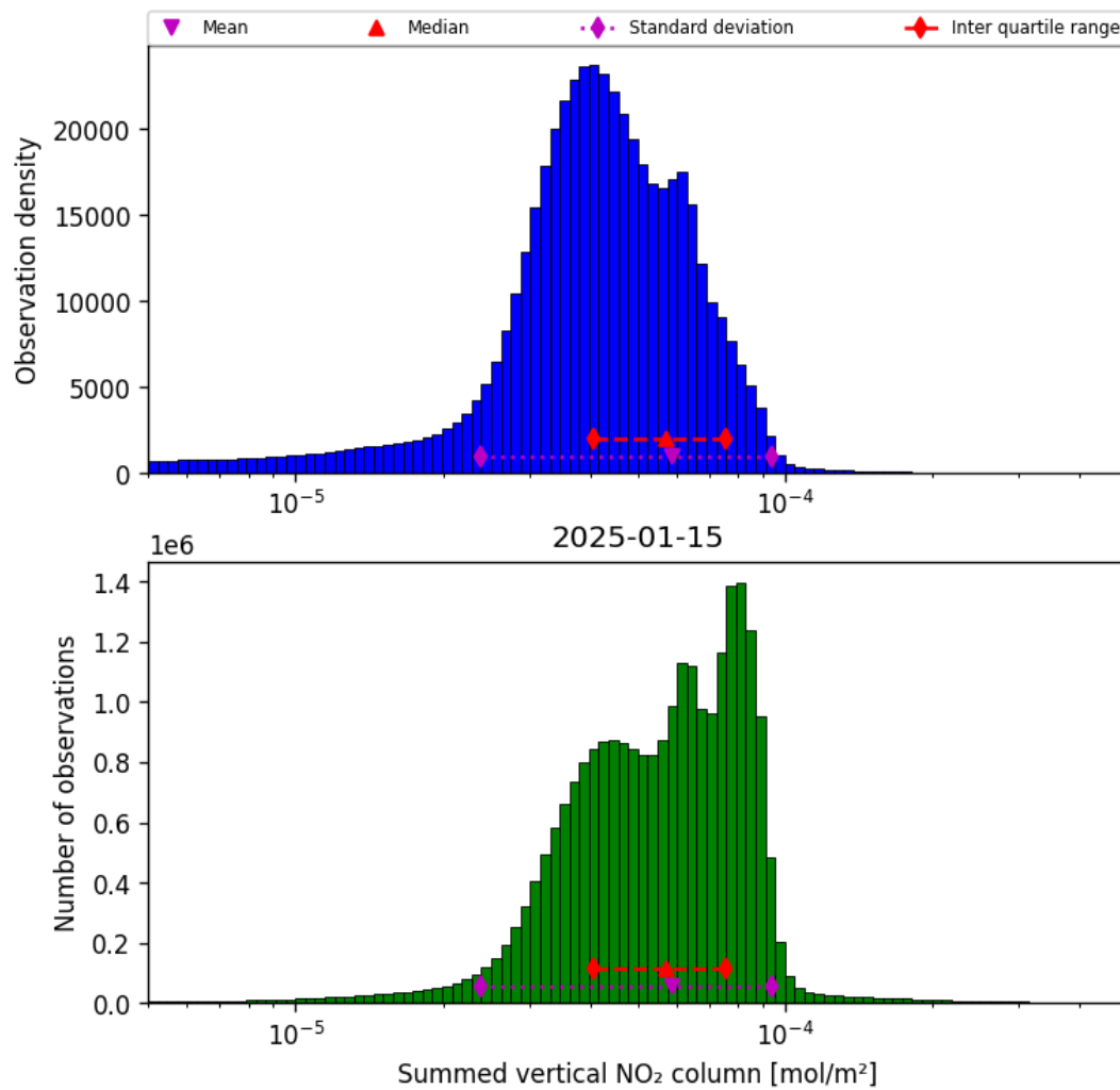
Figure 40: Histogram of “Summed vertical NO 2 column” for 2025-01-14 to 2025-01-16
