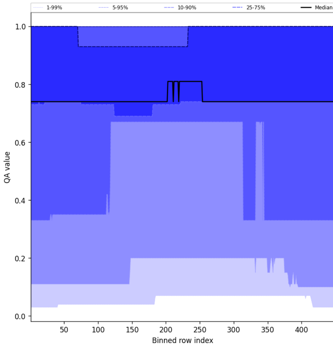
Figure 45: Along track statistics of “QA value” for 2025-01-14 to 2025-01-16
