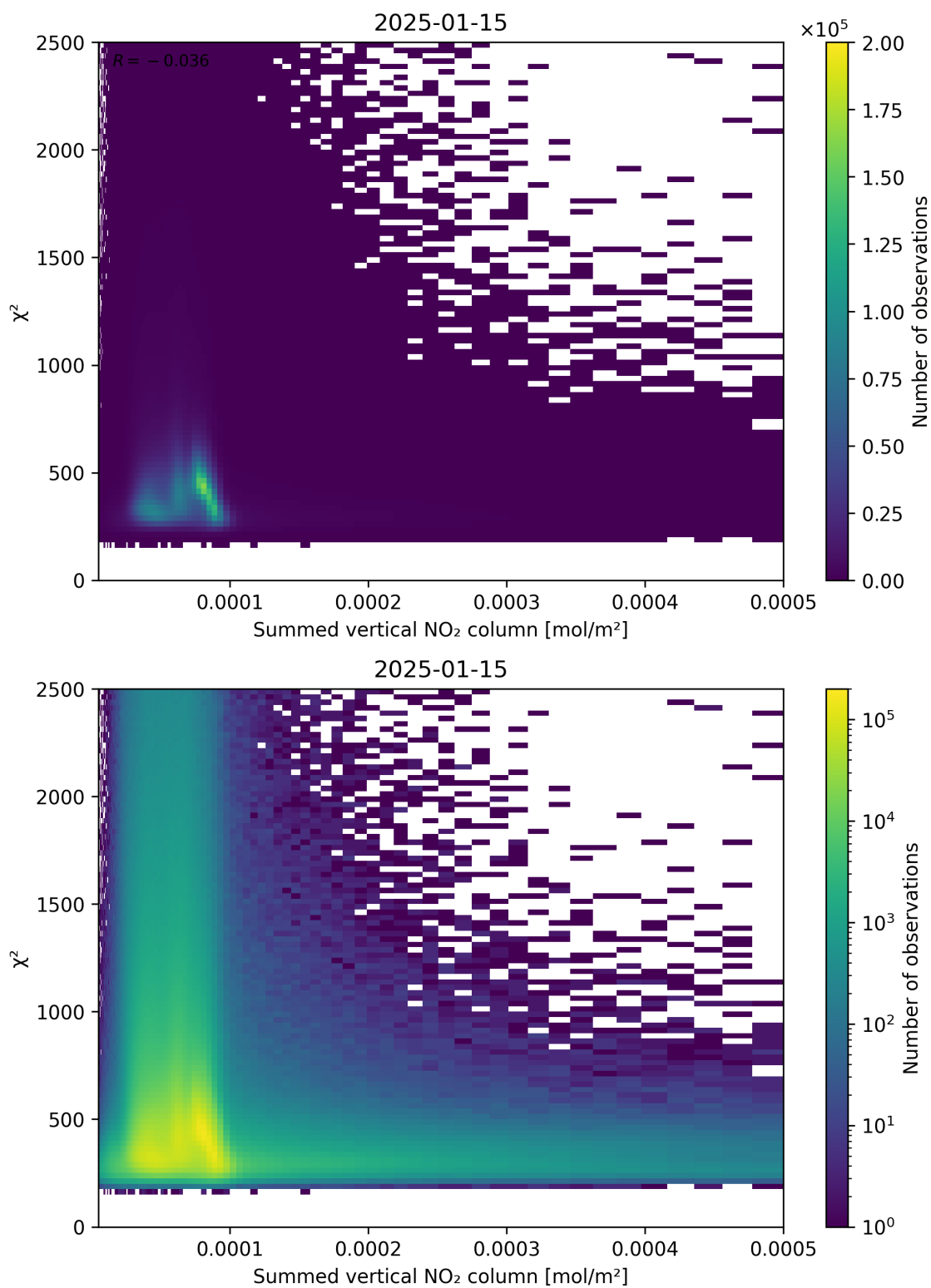
Figure 104: Scatter density plot of “Summed vertical NO 2 column” against “ \chi^2 ” for 2025-01-14 to 2025-01-16.
