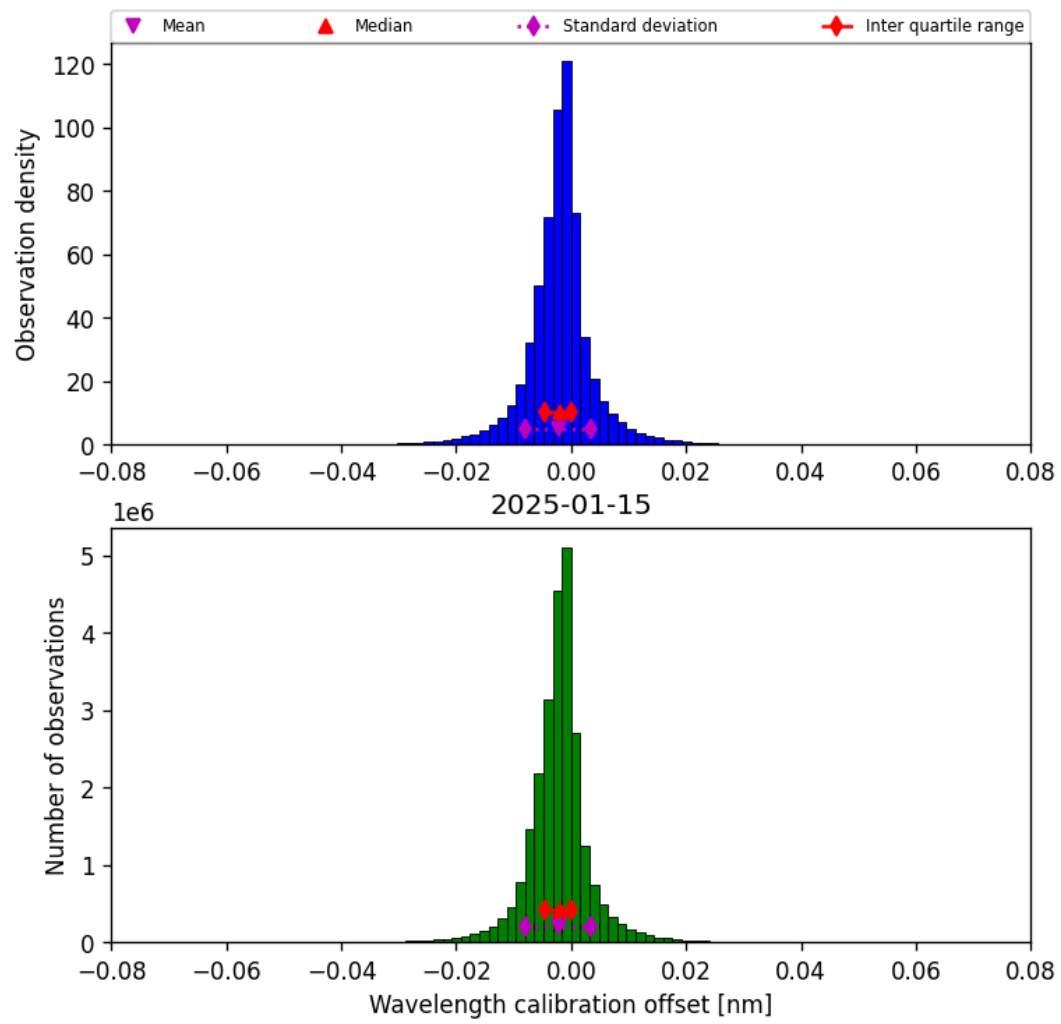
Figure 35: Histogram of “Wavelength calibration offset” for 2025-01-14 to 2025-01-16
