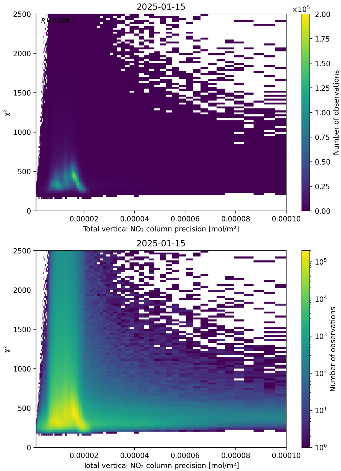
Figure 116: Scatter density plot of “Total vertical NO 2 column precision” against “ \chi^2 ” for 2025-01-14 to 2025-01-16.
