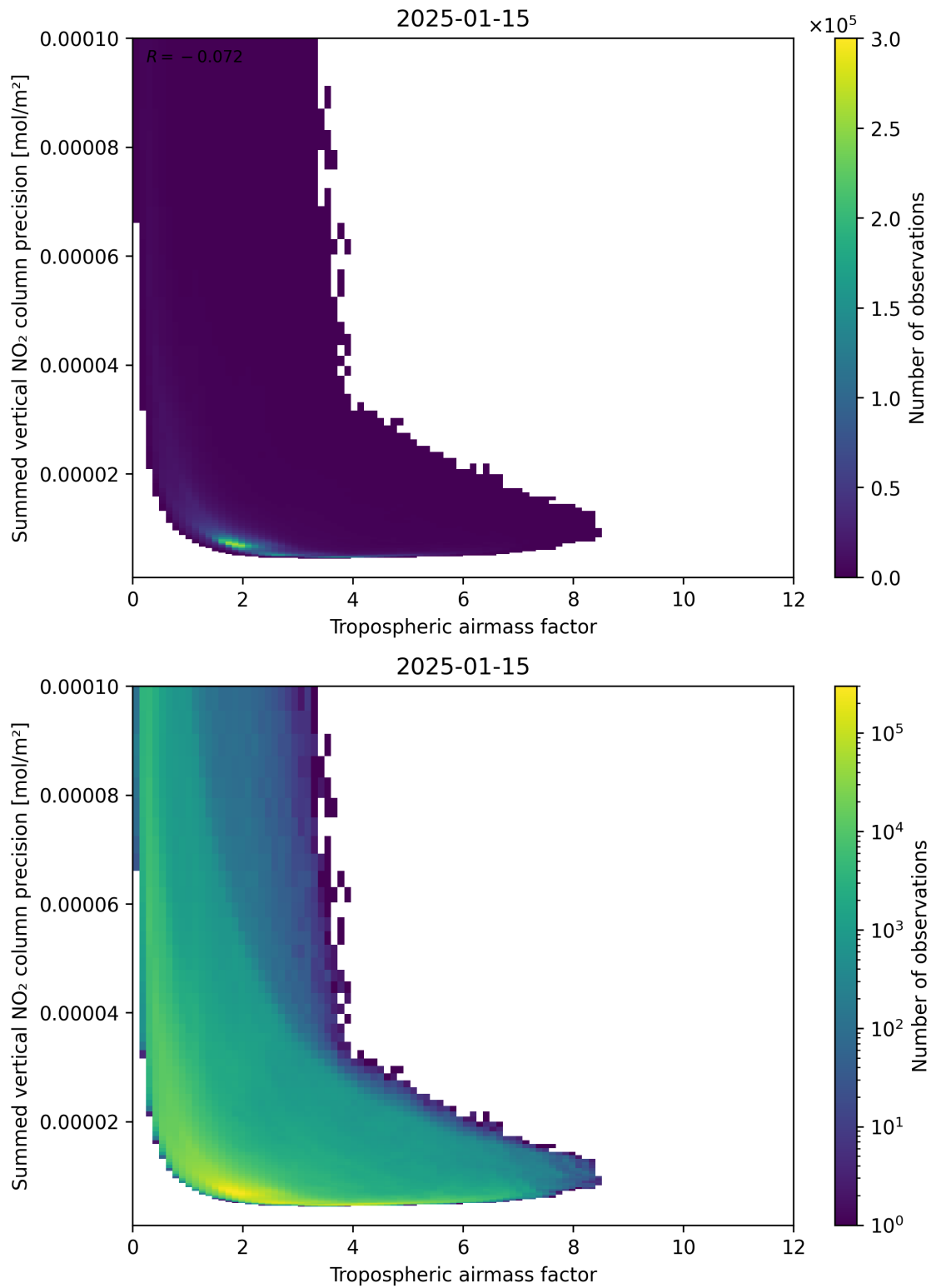
Figure 76: Scatter density plot of “Tropospheric air mass factor” against “Summed vertical NO 2 column precision” for 2025-01-14 to 2025-01-16.
