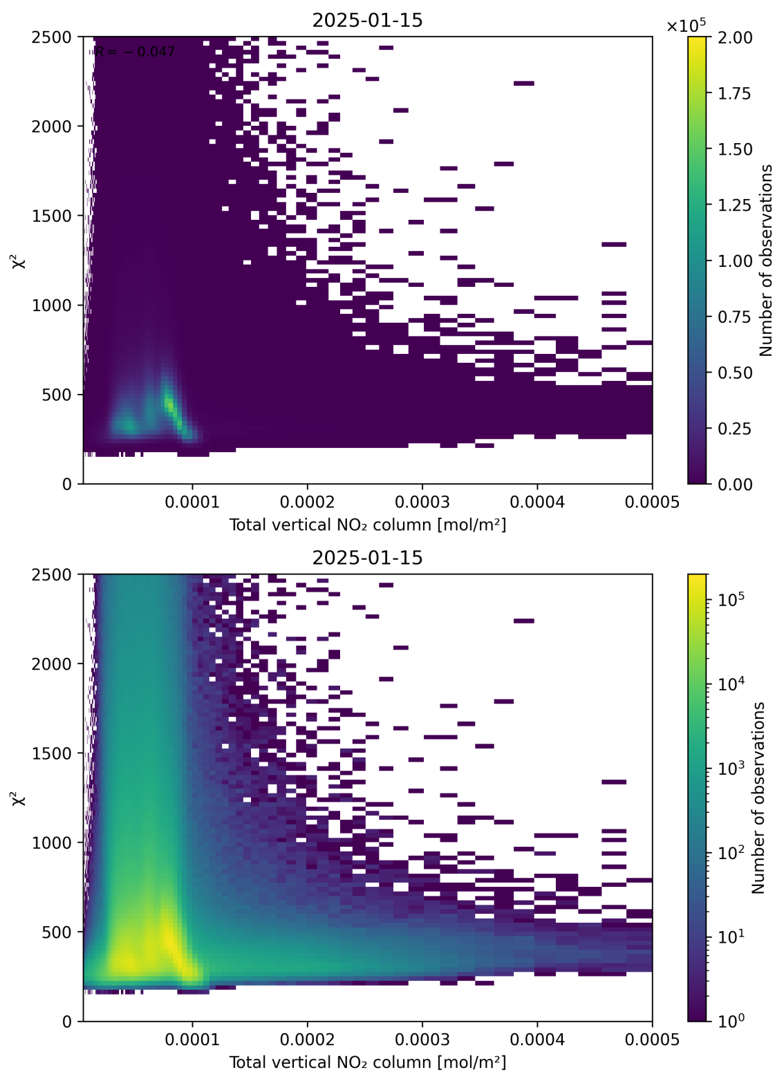
Figure 111: Scatter density plot of “Total vertical NO 2 column” against “ \chi^2 ” for 2025-01-14 to 2025-01-16.
