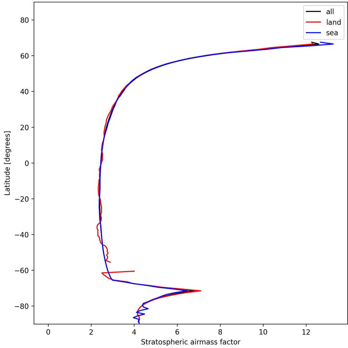
Figure 27: Zonal average of “Stratospheric air mass factor” for 2025-01-14 to 2025-01-16.
