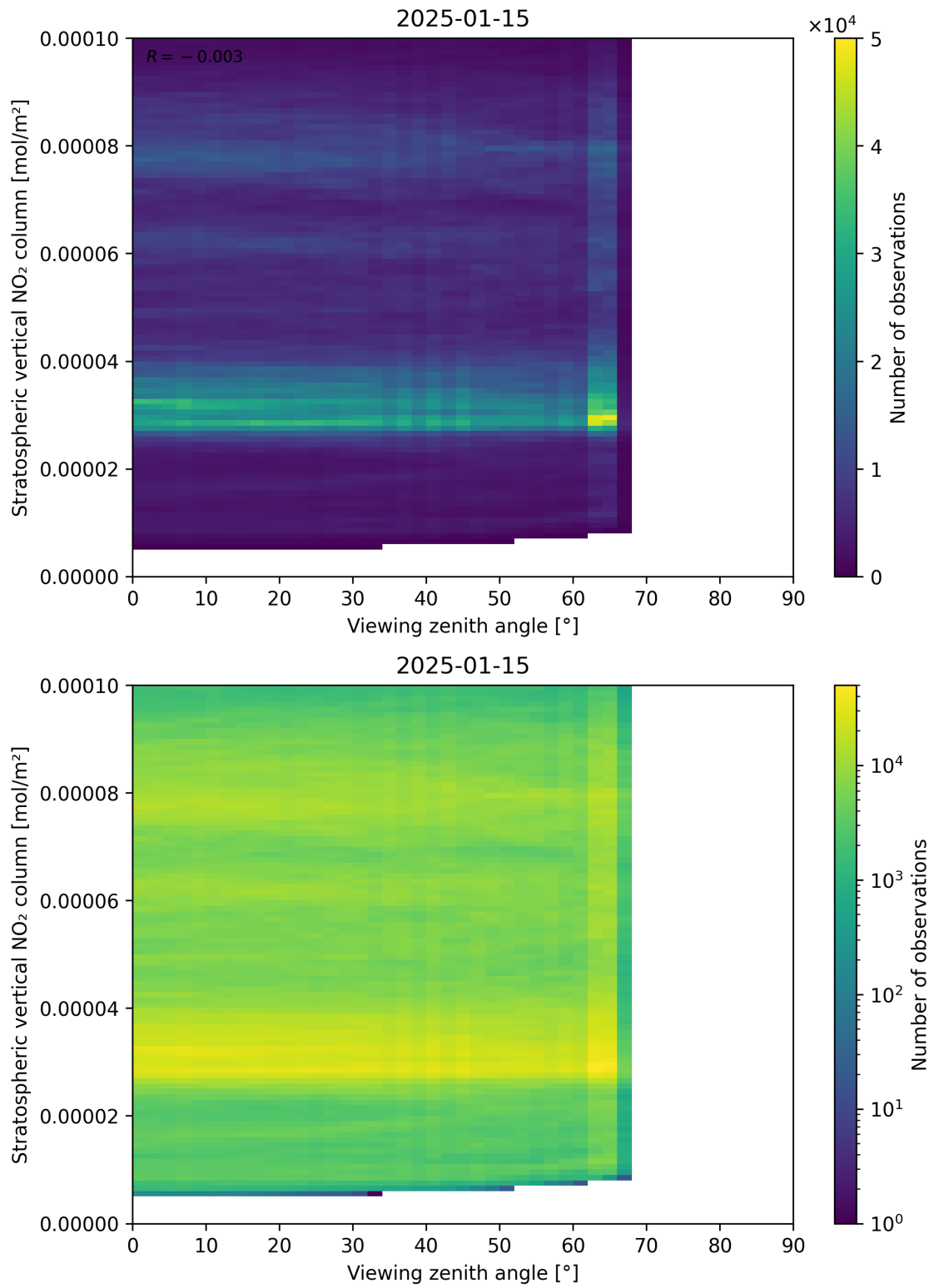
Figure 164: Scatter density plot of “Viewing zenith angle” against “Stratospheric vertical NO 2 column” for 2025-01-14 to 2025-01-16.
