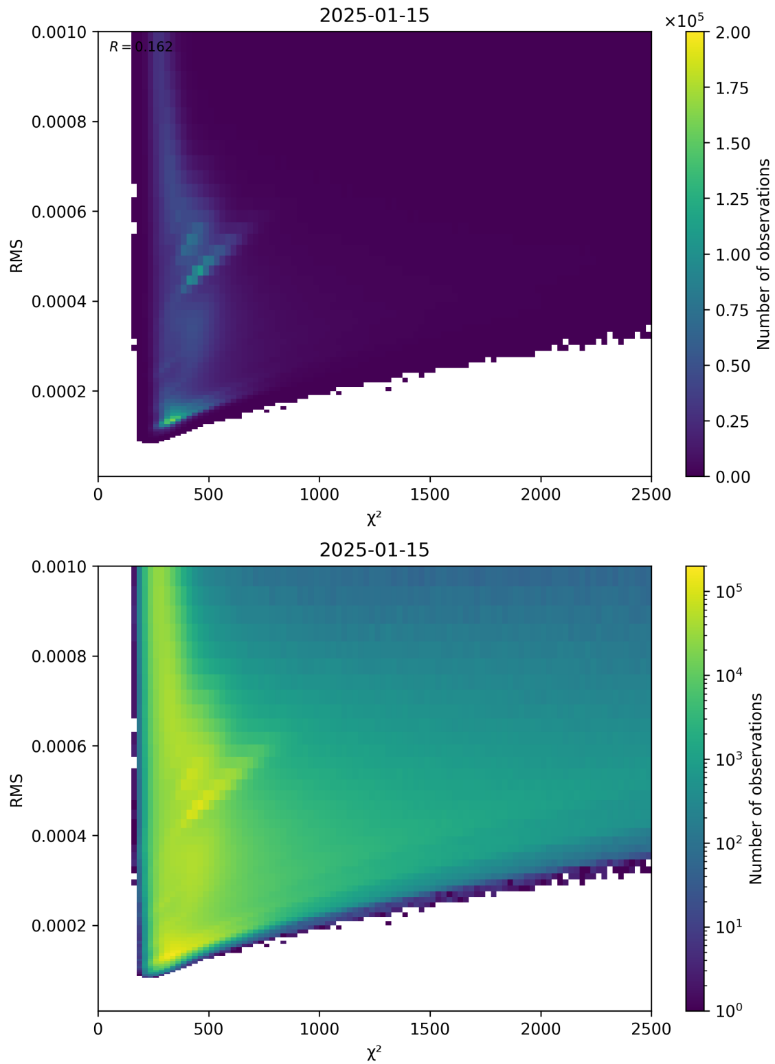
Figure 82: Scatter density plot of “ \chi^2 ” against “RMS” for 2025-01-14 to 2025-01-16.
