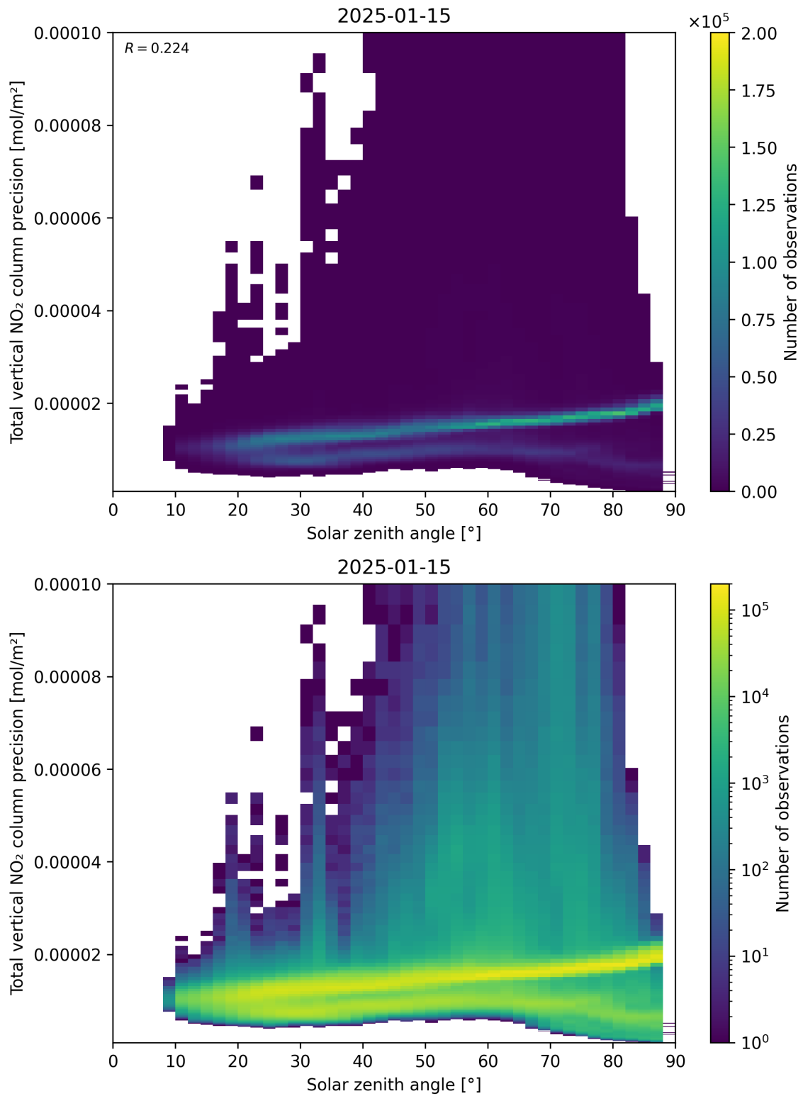
Figure 154: Scatter density plot of “Solar zenith angle” against “Total vertical NO 2 column precision” for 2025-01-14 to 2025-01-16.
