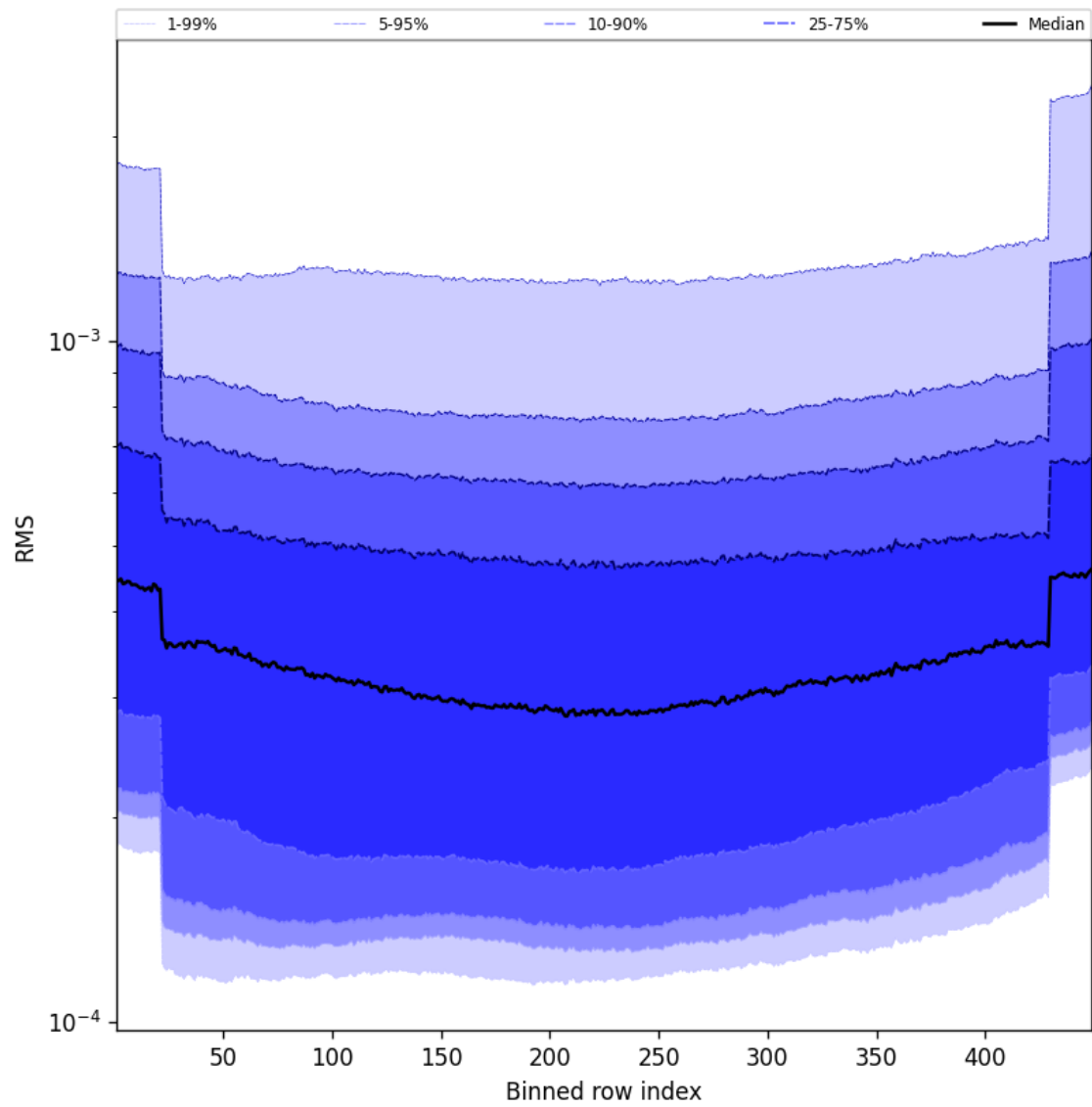
Figure 60: Along track statistics of “RMS” for 2025-01-14 to 2025-01-16
