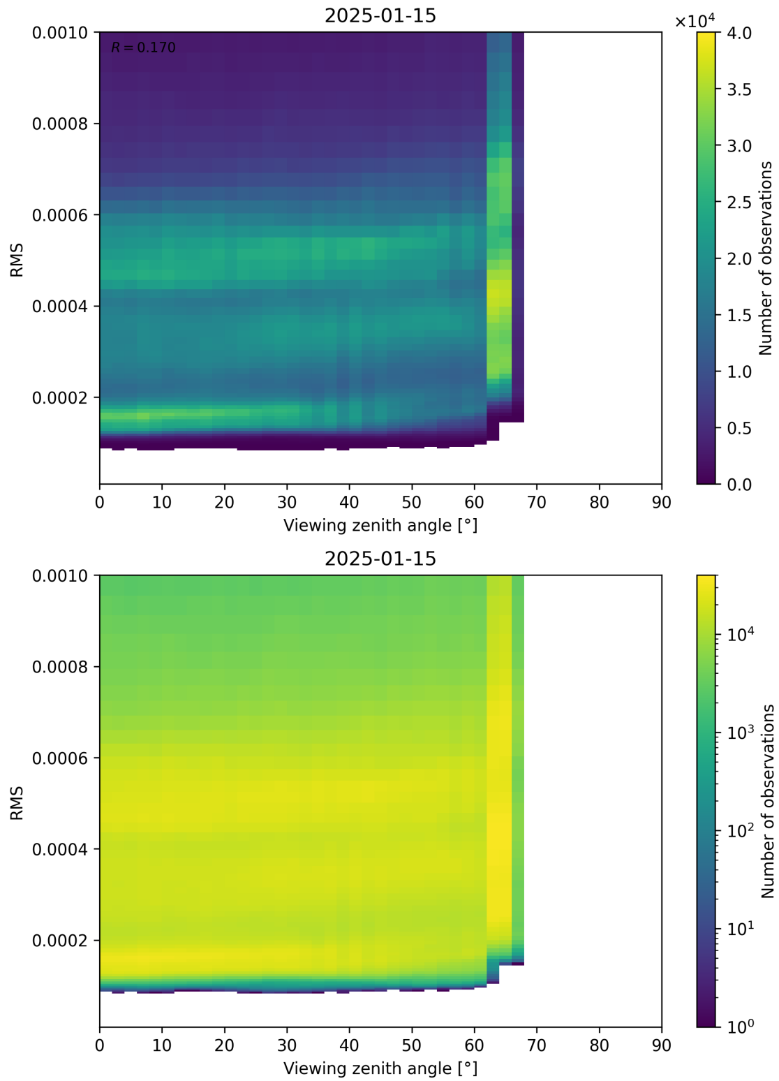
Figure 171: Scatter density plot of “Viewing zenith angle” against “RMS” for 2025-01-14 to 2025-01-16.
