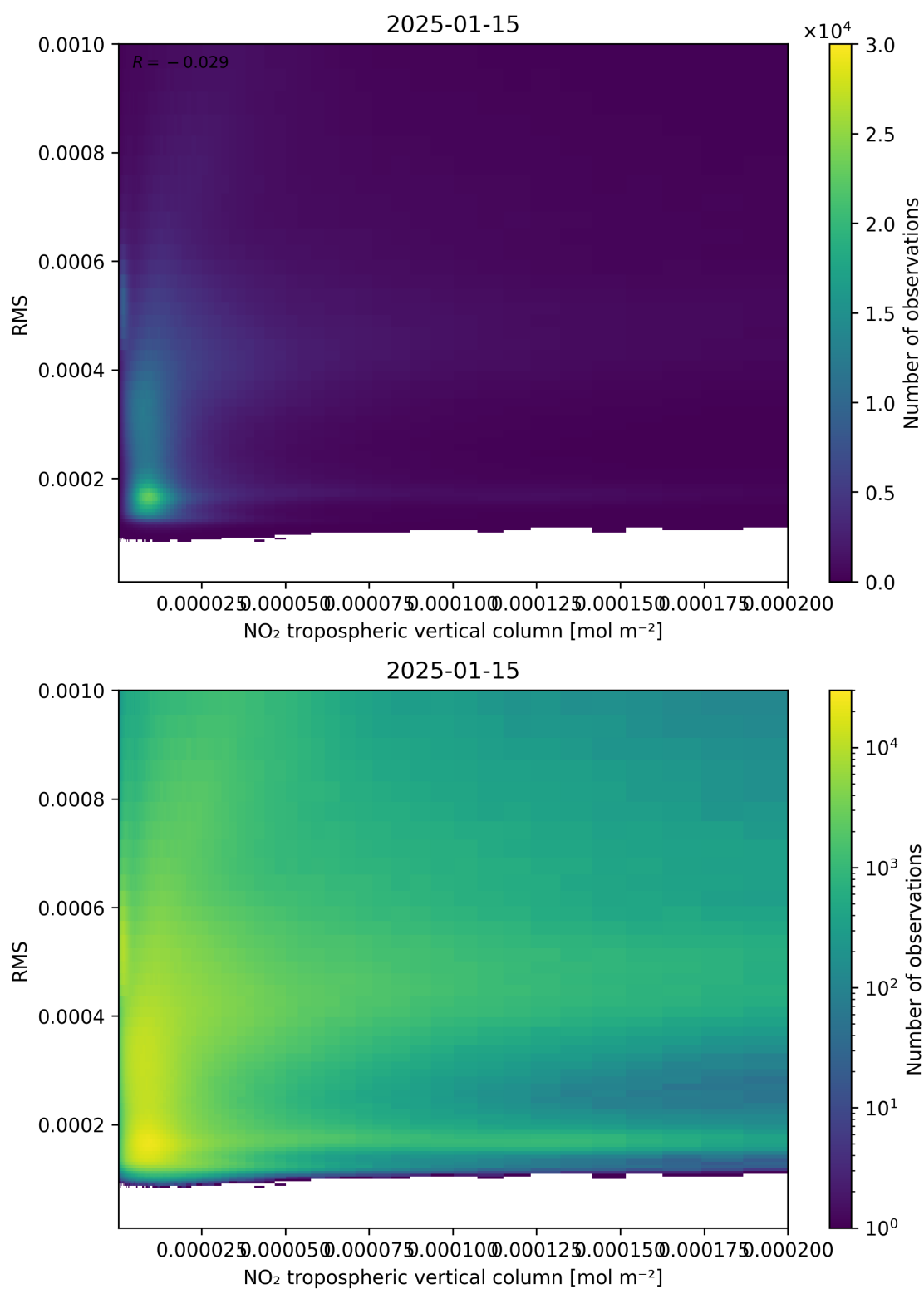
Figure 142: Scatter density plot of “NO 2 tropospheric vertical column” against “RMS” for 2025-01-14 to 2025-01-16.
