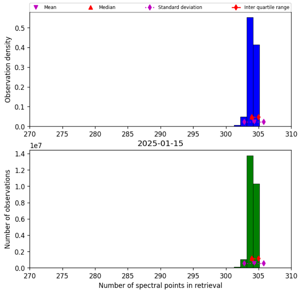
Figure 33: Histogram of “Number of spectral points in retrieval” for 2025-01-14 to 2025-01-16
