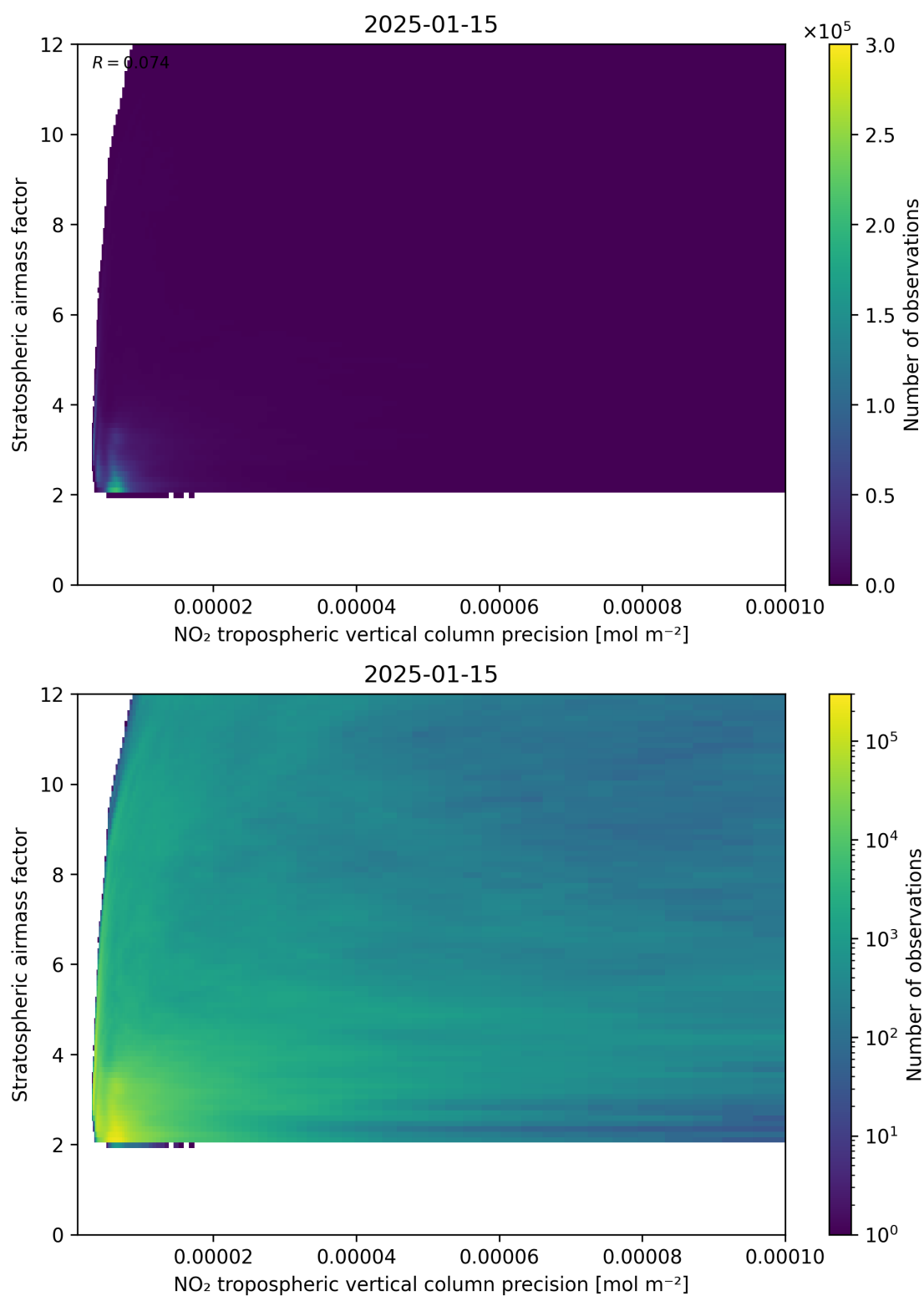
Figure 131: Scatter density plot of “NO 2 tropospheric vertical column precision” against “Stratospheric airmass factor” for 2025-01-14 to 2025-01-16.
