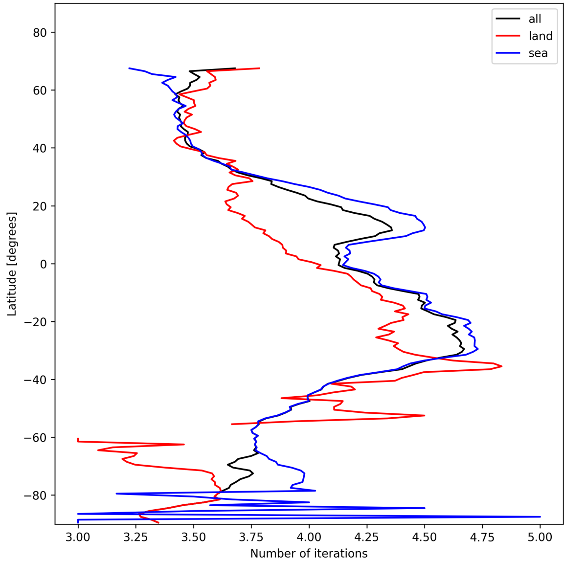
Figure 17: Zonal average of “Number of iterations” for 2025-01-14 to 2025-01-16.
