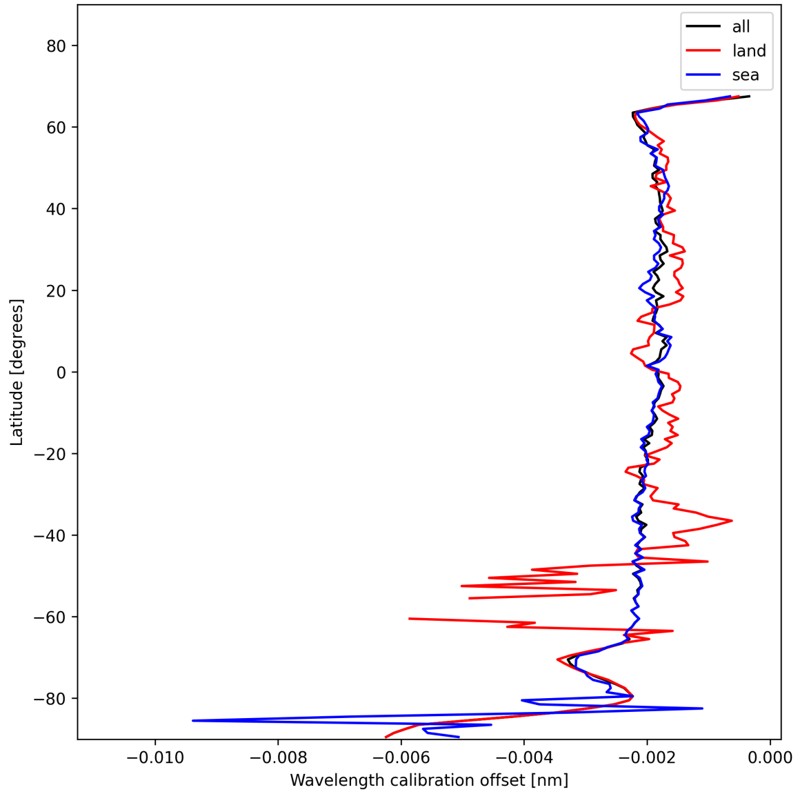
Figure 18: Zonal average of “Wavelength calibration offset” for 2025-01-14 to 2025-01-16.
