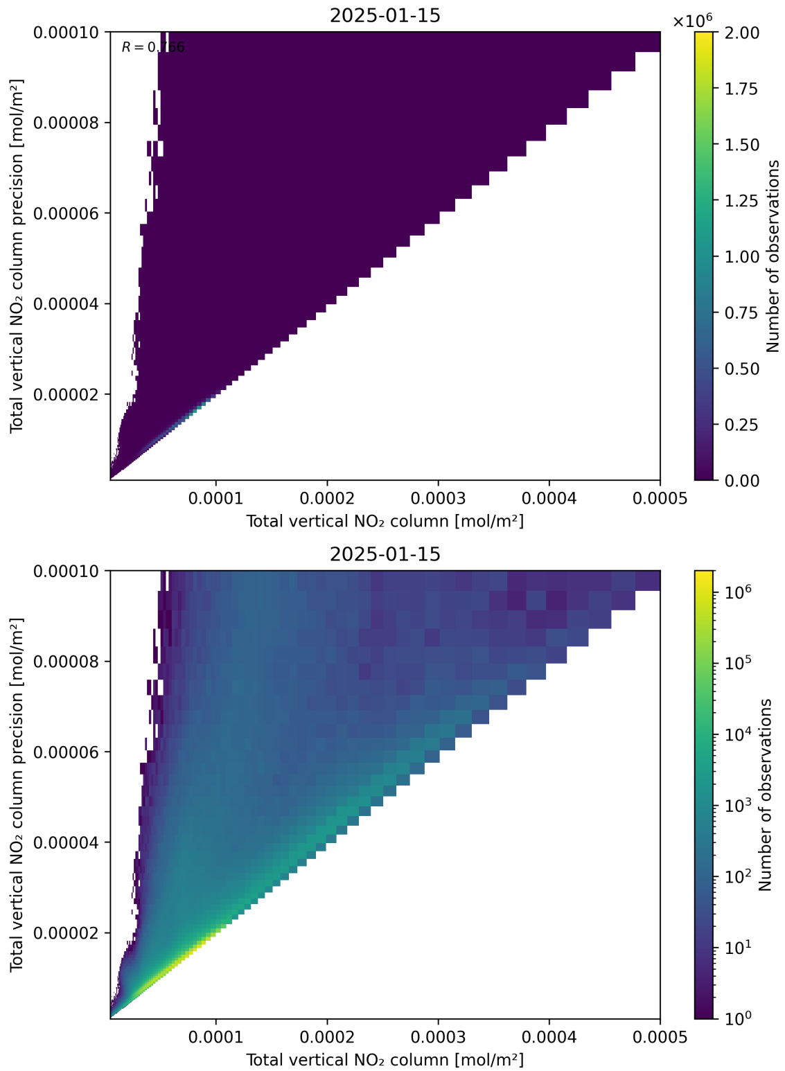
Figure 114: Scatter density plot of “Total vertical NO 2 column” against “Total vertical NO 2 column precision” for 2025-01-14 to 2025-01-16.
