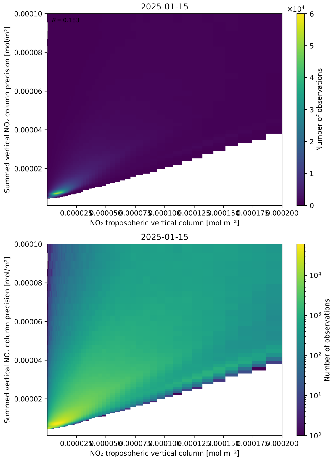
Figure 127: Scatter density plot of “NO 2 tropospheric vertical column” against “Summed vertical NO 2 column precision” for 2025-01-14 to 2025-01-16.
