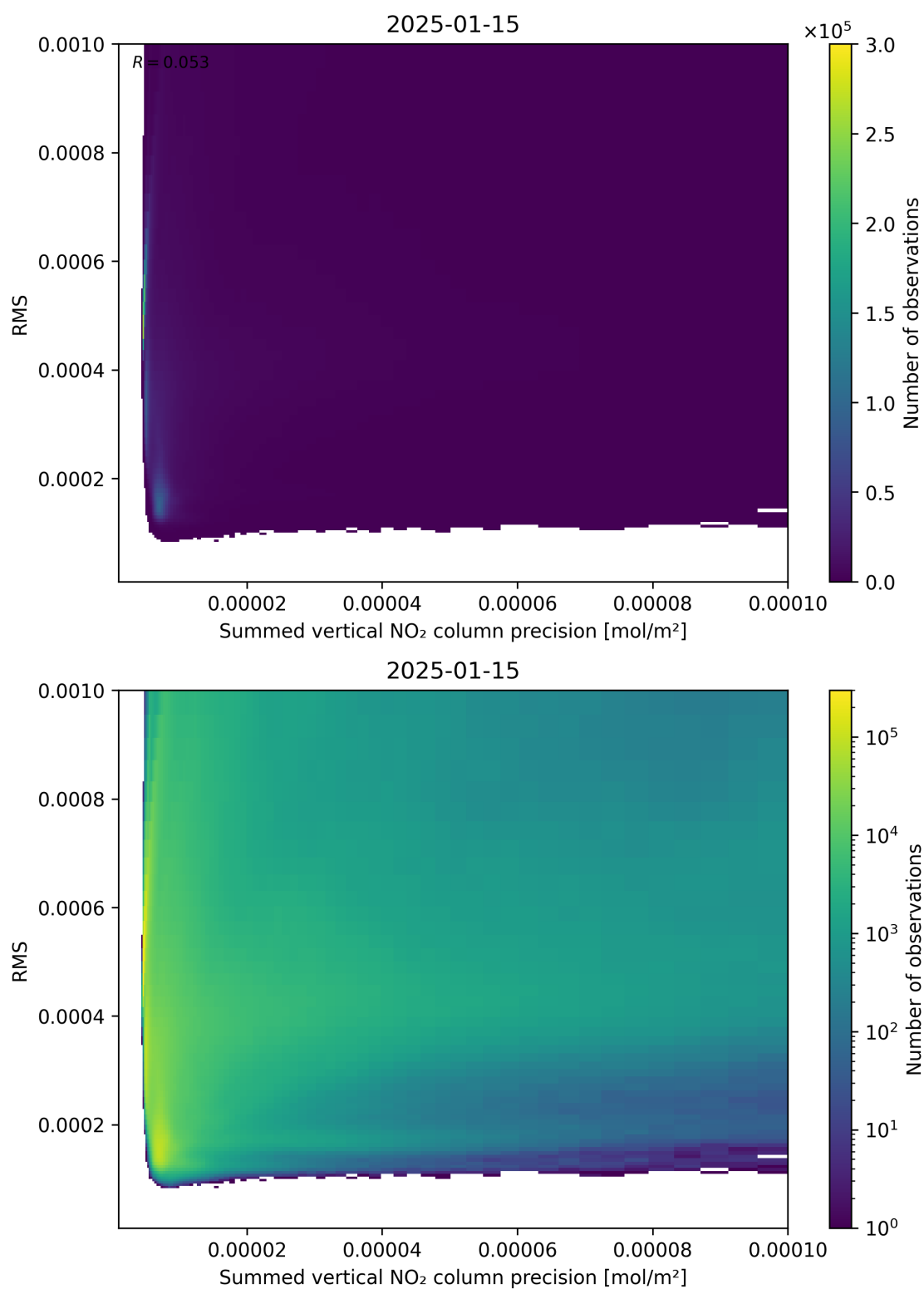
Figure 108: Scatter density plot of “Summed vertical NO 2 column precision” against “RMS” for 2025-01-14 to 2025-01-16.
