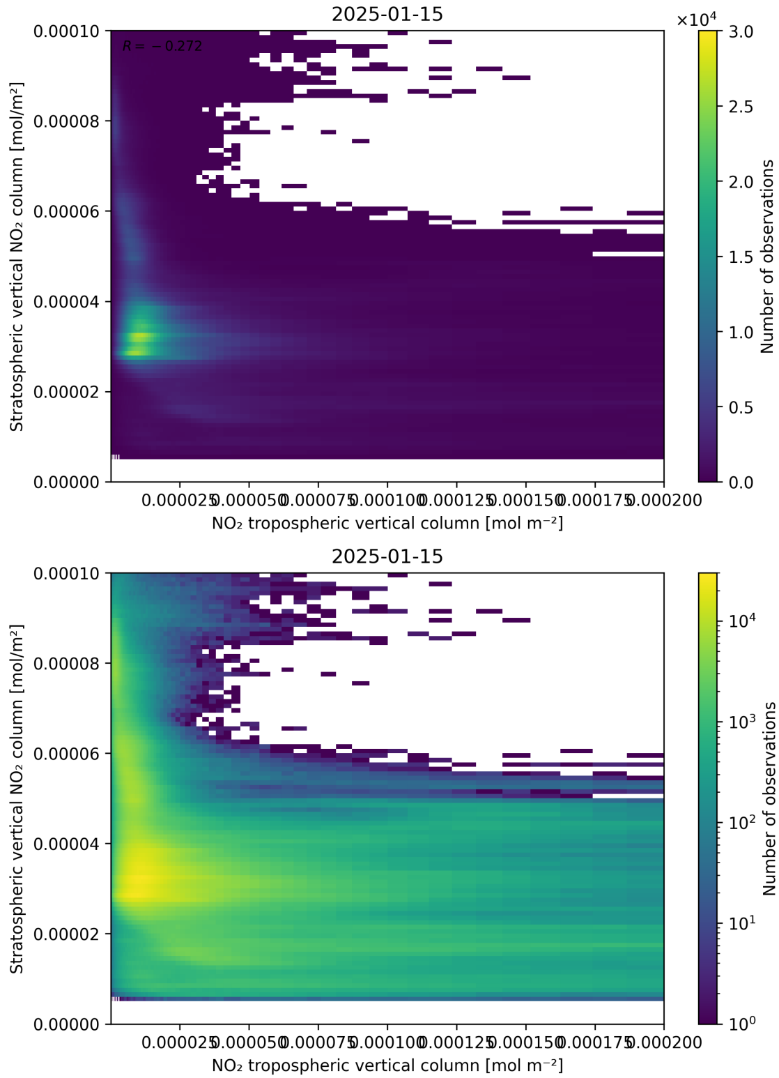
Figure 125: Scatter density plot of “NO 2 tropospheric vertical column” against “Stratospheric vertical NO 2 column” for 2025-01-14 to 2025-01-16.
