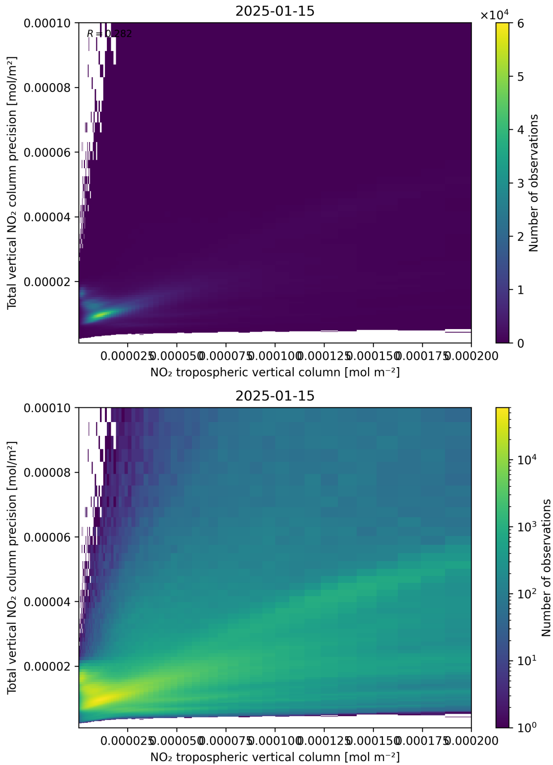
Figure 129: Scatter density plot of “NO 2 tropospheric vertical column” against “Total vertical NO 2 column precision” for 2025-01-14 to 2025-01-16.
