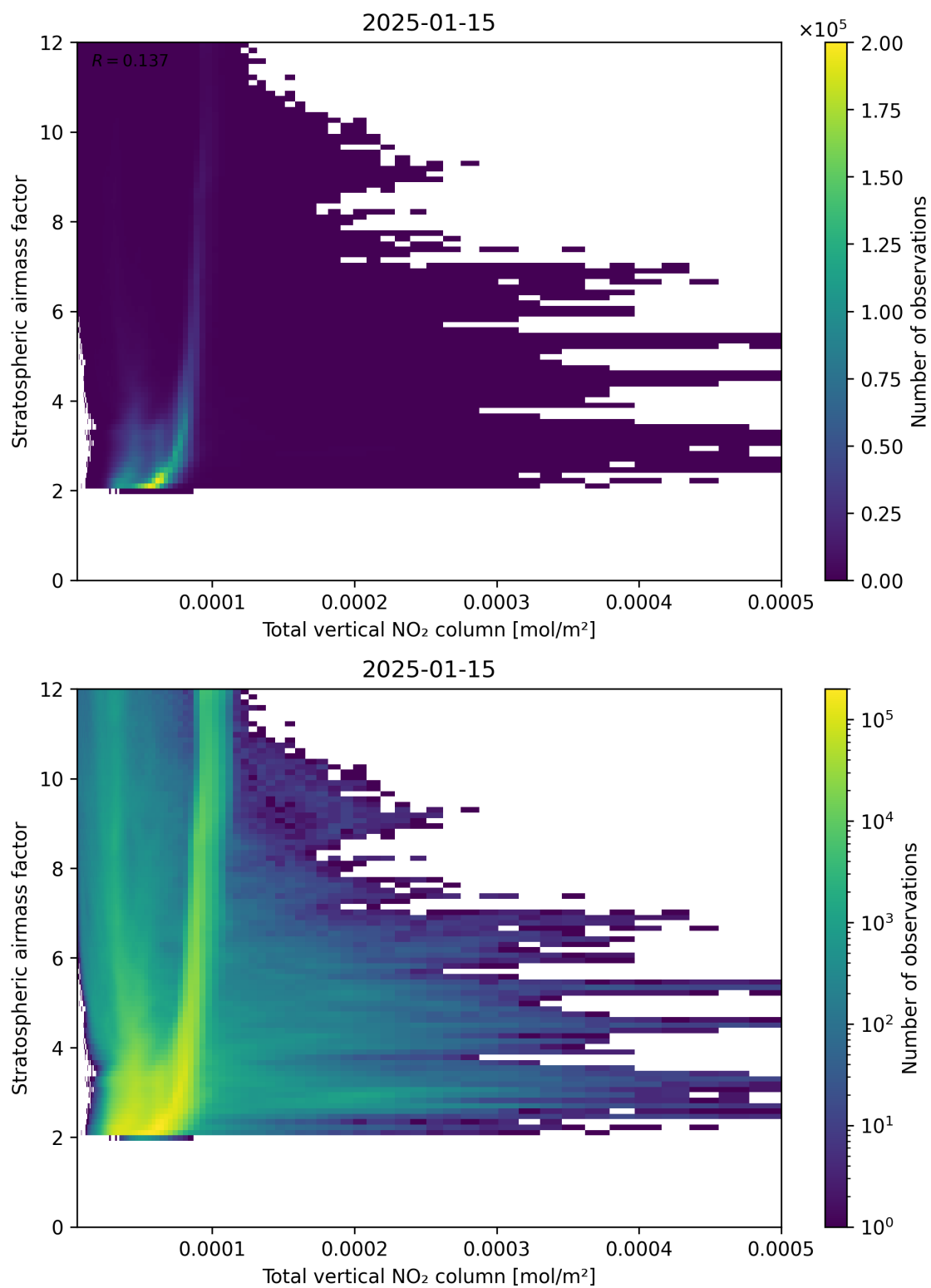
Figure 110: Scatter density plot of “Total vertical NO 2 column” against “Stratospheric airmass factor” for 2025-01-14 to 2025-01-16.
