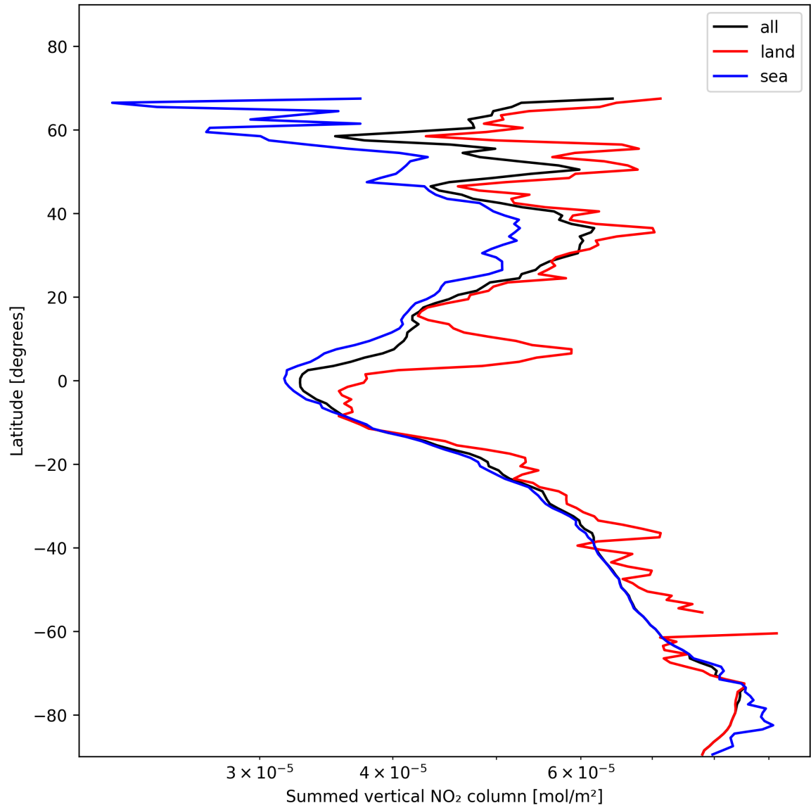
Figure 23: Zonal average of “Summed vertical NO 2 column” for 2025-01-14 to 2025-01-16.
