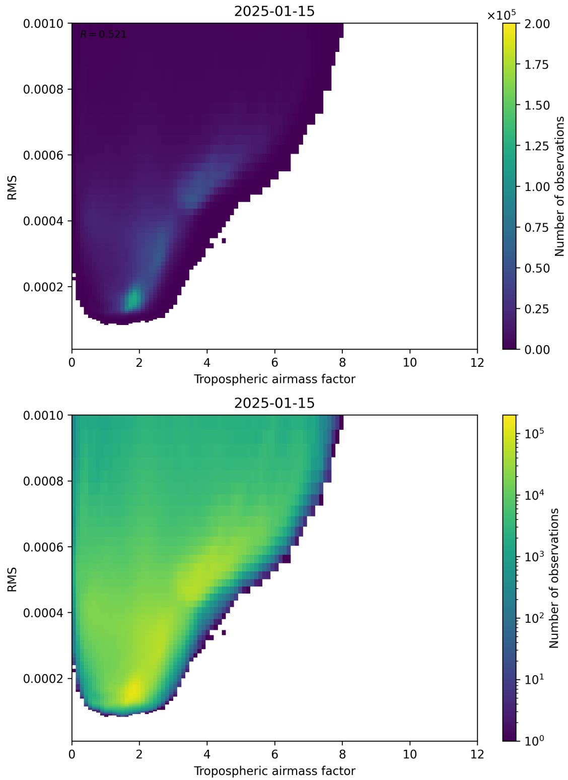
Figure 79: Scatter density plot of “Tropospheric airmass factor” against “RMS” for 2025-01-14 to 2025-01-16.
