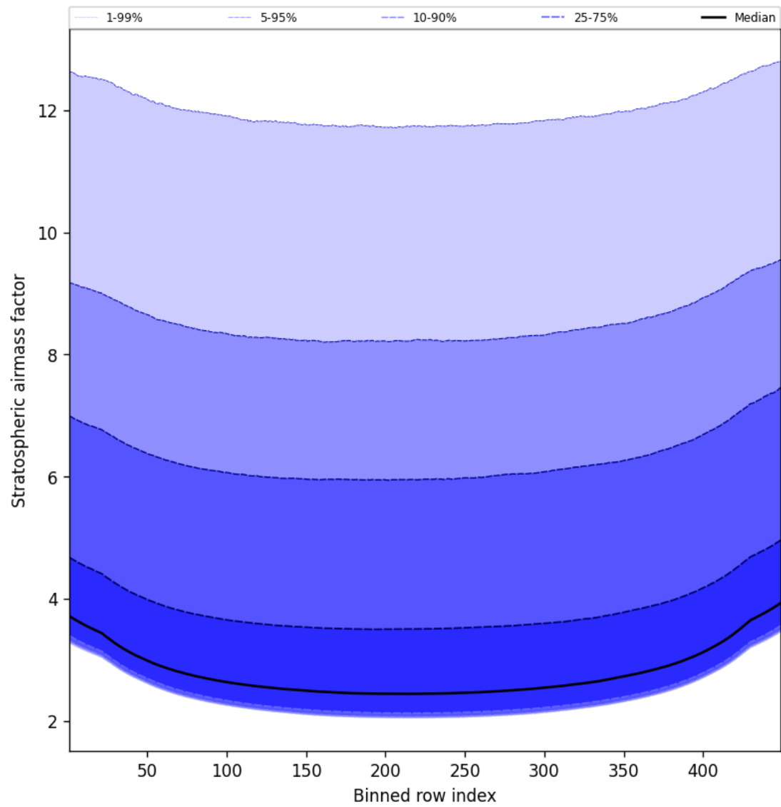
Figure 61: Along track statistics of “Stratospheric air mass factor” for 2025-01-14 to 2025-01-16
