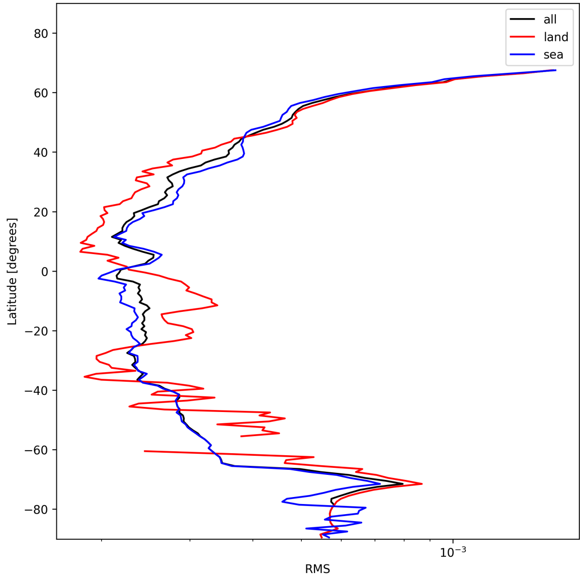
Figure 26: Zonal average of “RMS” for 2025-01-14 to 2025-01-16.
