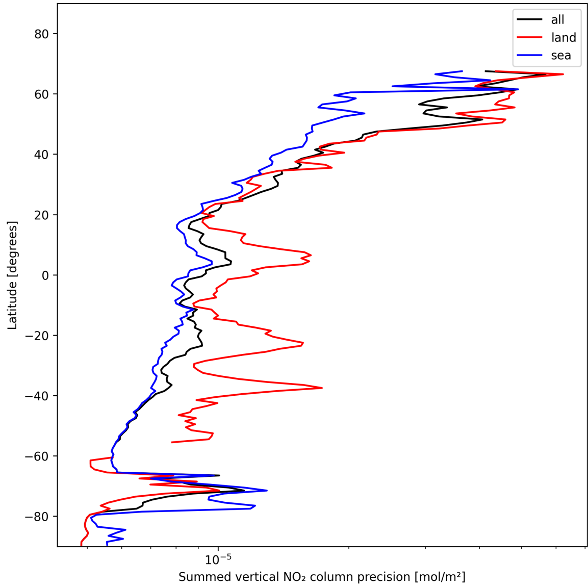
Figure 24: Zonal average of “Summed vertical NO 2 column precision” for 2025-01-14 to 2025-01-16.
