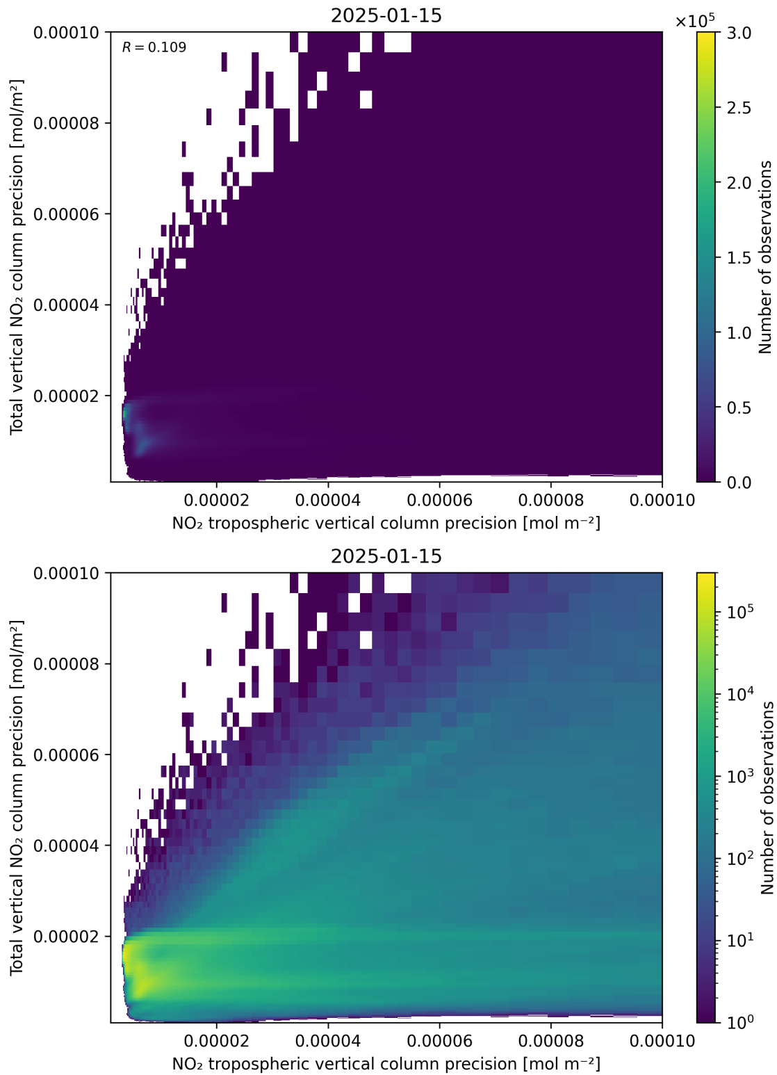
Figure 139: Scatter density plot of “NO 2 tropospheric vertical column precision” against “Total vertical NO 2 column precision” for 2025-01-14 to 2025-01-16.
