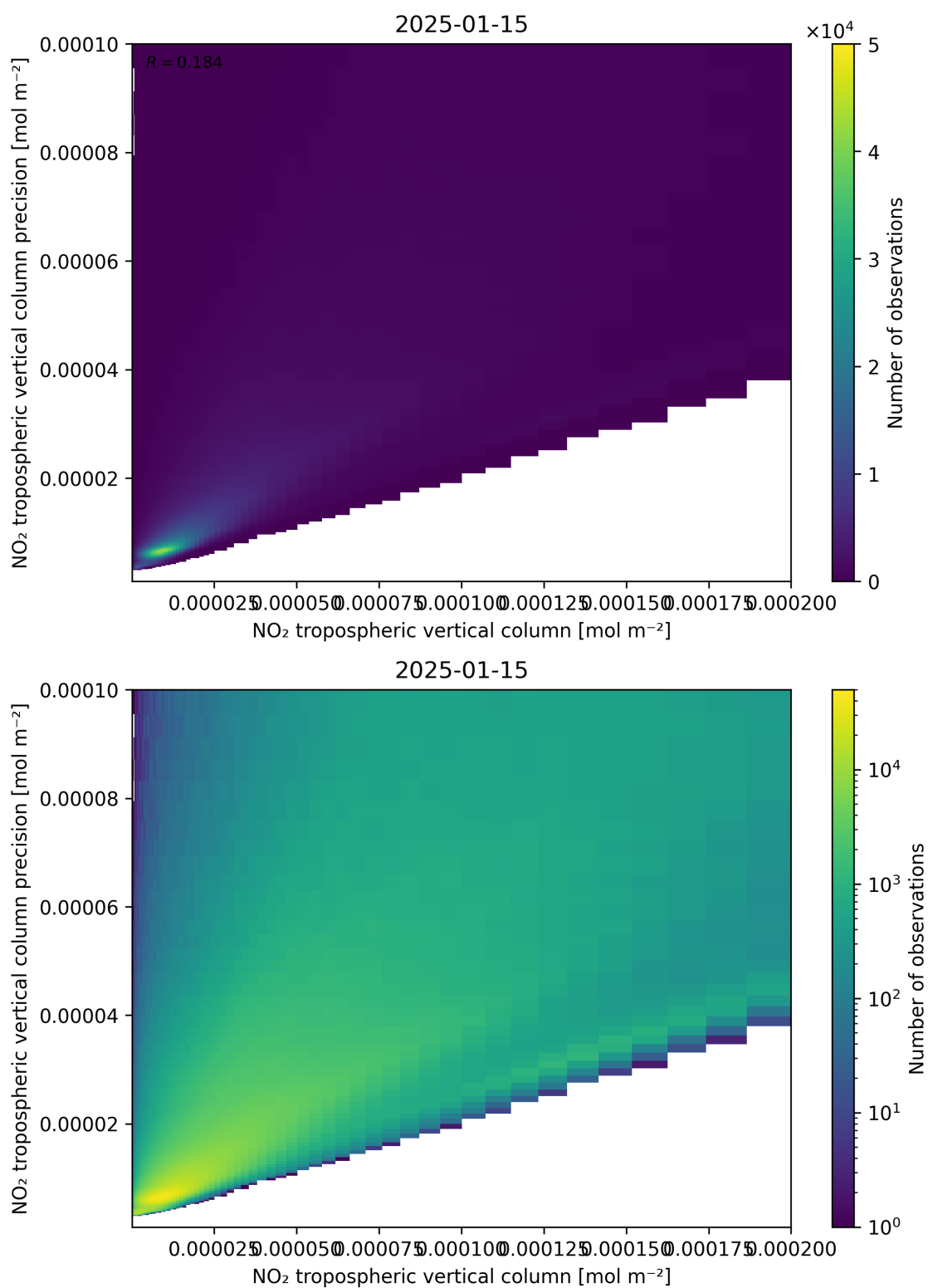
Figure 130: Scatter density plot of “NO 2 tropospheric vertical column” against “NO 2 tropospheric vertical column precision” for 2025-01-14 to 2025-01-16.
