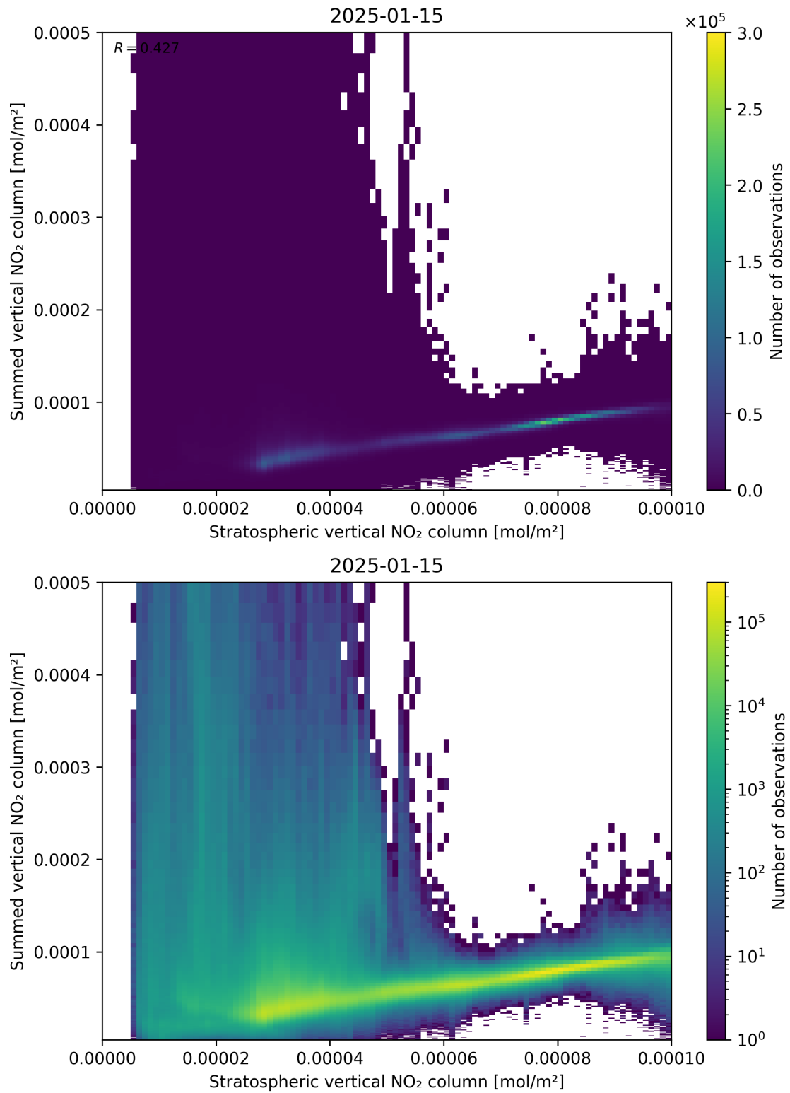
Figure 98: Scatter density plot of “Stratospheric vertical NO 2 column” against “Summed vertical NO 2 column” for 2025-01-14 to 2025-01-16.
