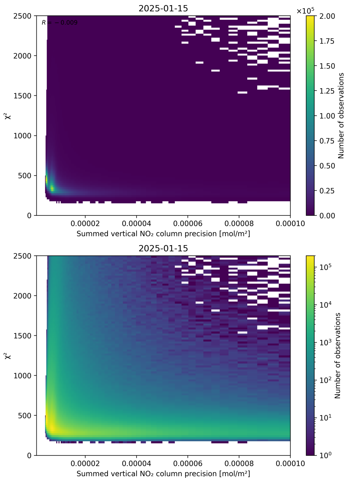
Figure 107: Scatter density plot of “Summed vertical NO 2 column precision” against “ \chi^2 ” for 2025-01-14 to 2025-01-16.
