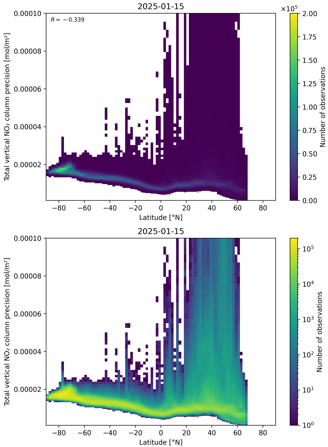
Figure 91: Scatter density plot of “Latitude” against “Total vertical NO 2 column precision” for 2025-01-14 to 2025-01-16.
