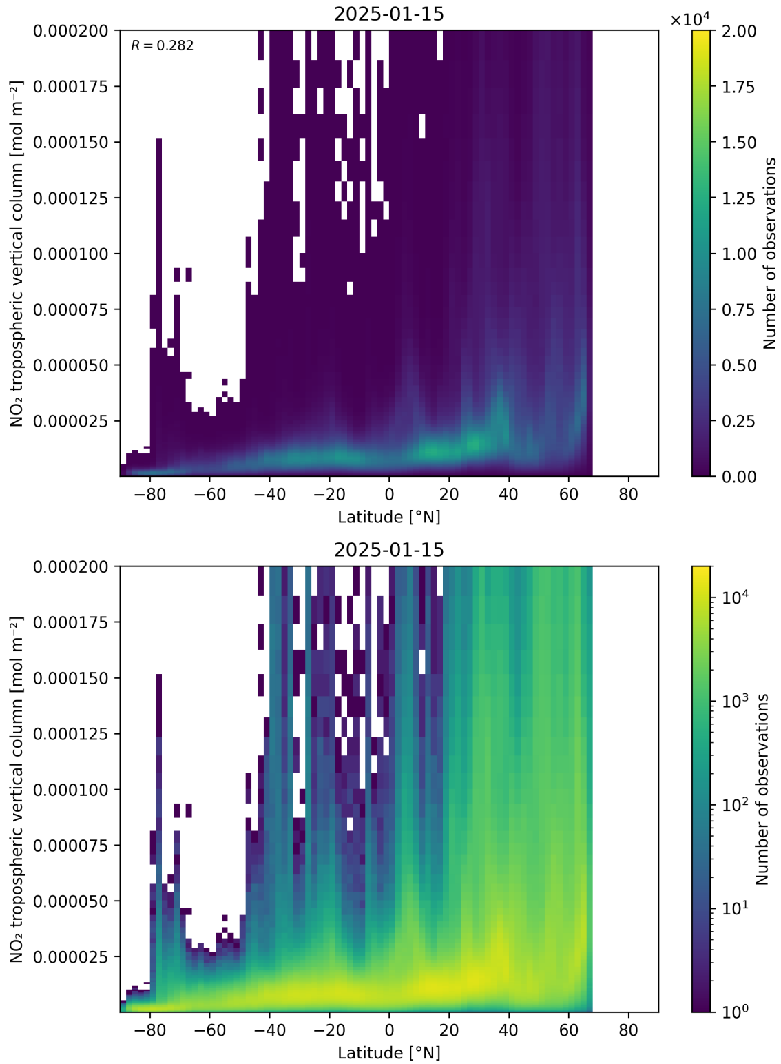
Figure 92: Scatter density plot of “Latitude” against “NO 2 tropospheric vertical column” for 2025-01-14 to 2025-01-16.
