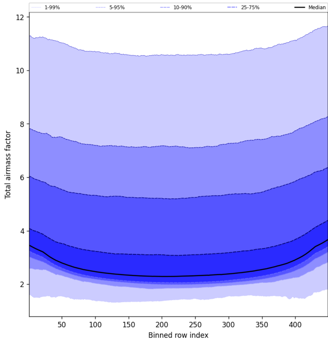
Figure 49: Along track statistics of “Total airmass factor” for 2025-01-14 to 2025-01-16
