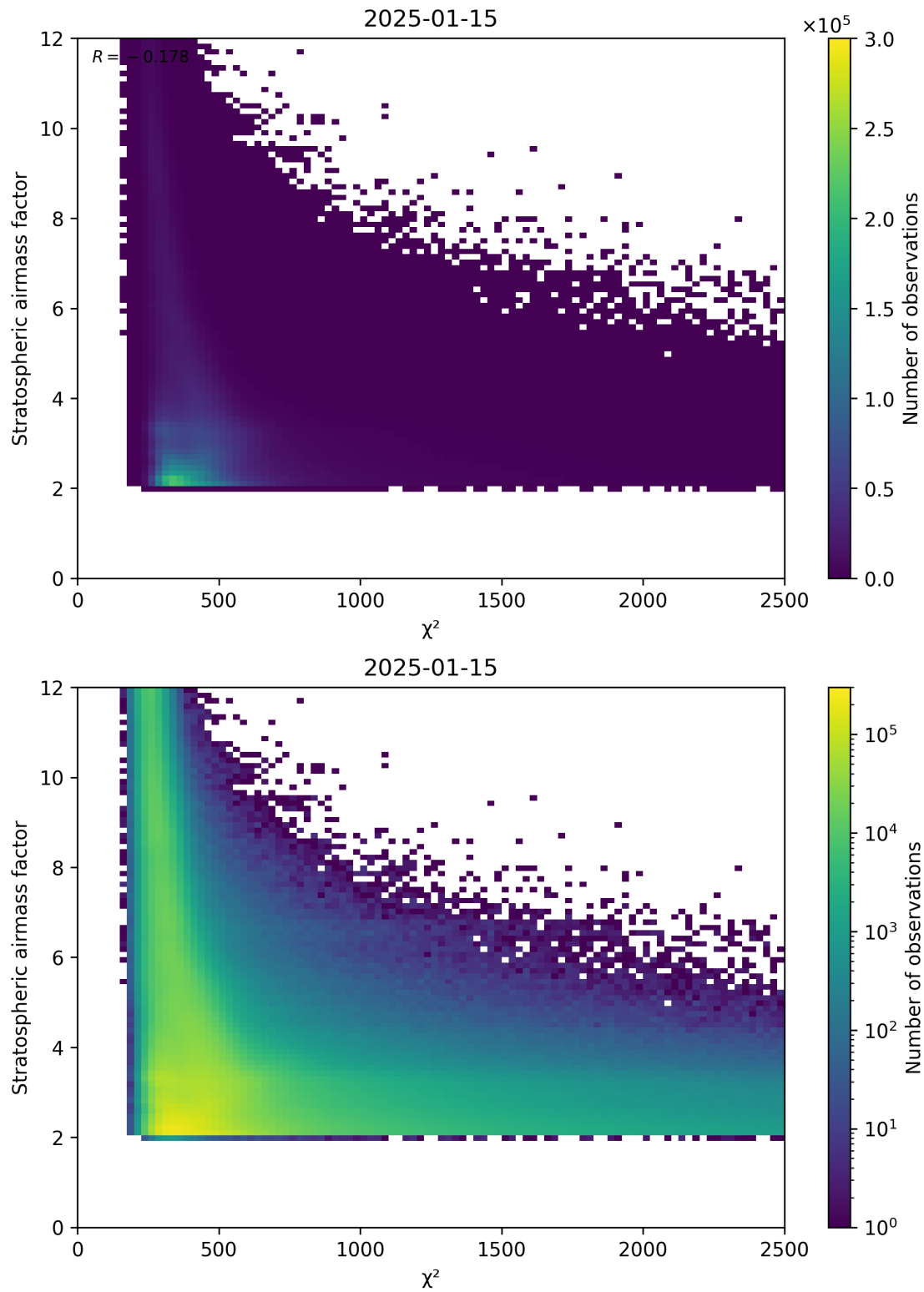
Figure 81: Scatter density plot of “ \chi^2 ” against “Stratospheric airmass factor” for 2025-01-14 to 2025-01-16.
