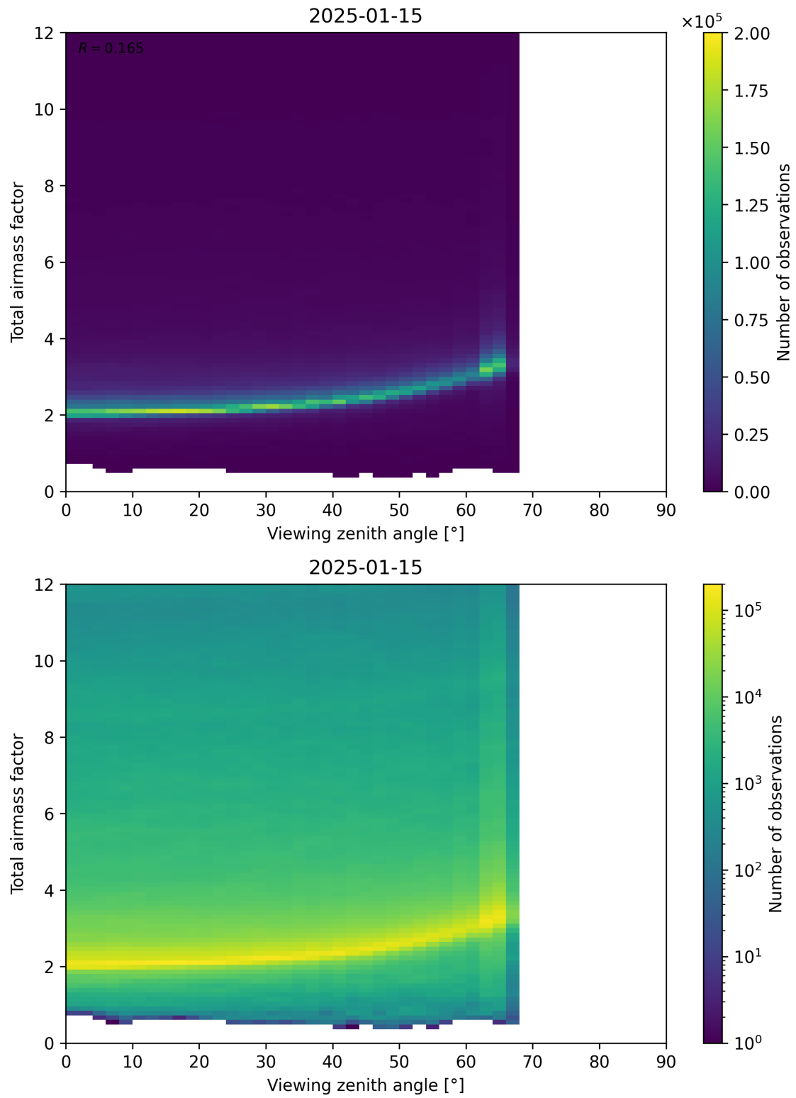
Figure 160: Scatter density plot of “Viewing zenith angle” against “Total airmass factor” for 2025-01-14 to 2025-01-16.
