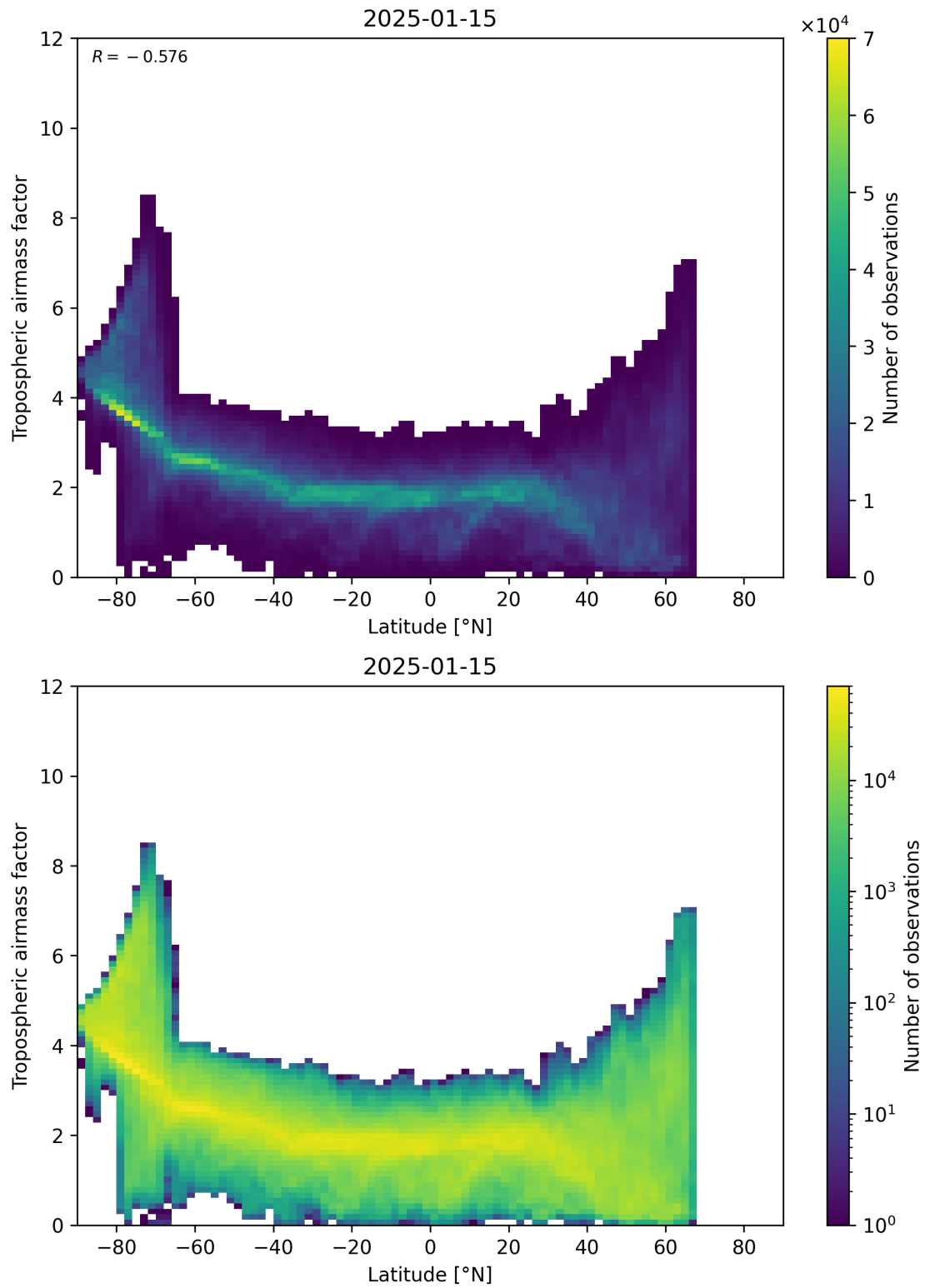
Figure 85: Scatter density plot of “Latitude” against “Tropospheric airmass factor” for 2025-01-14 to 2025-01-16.
