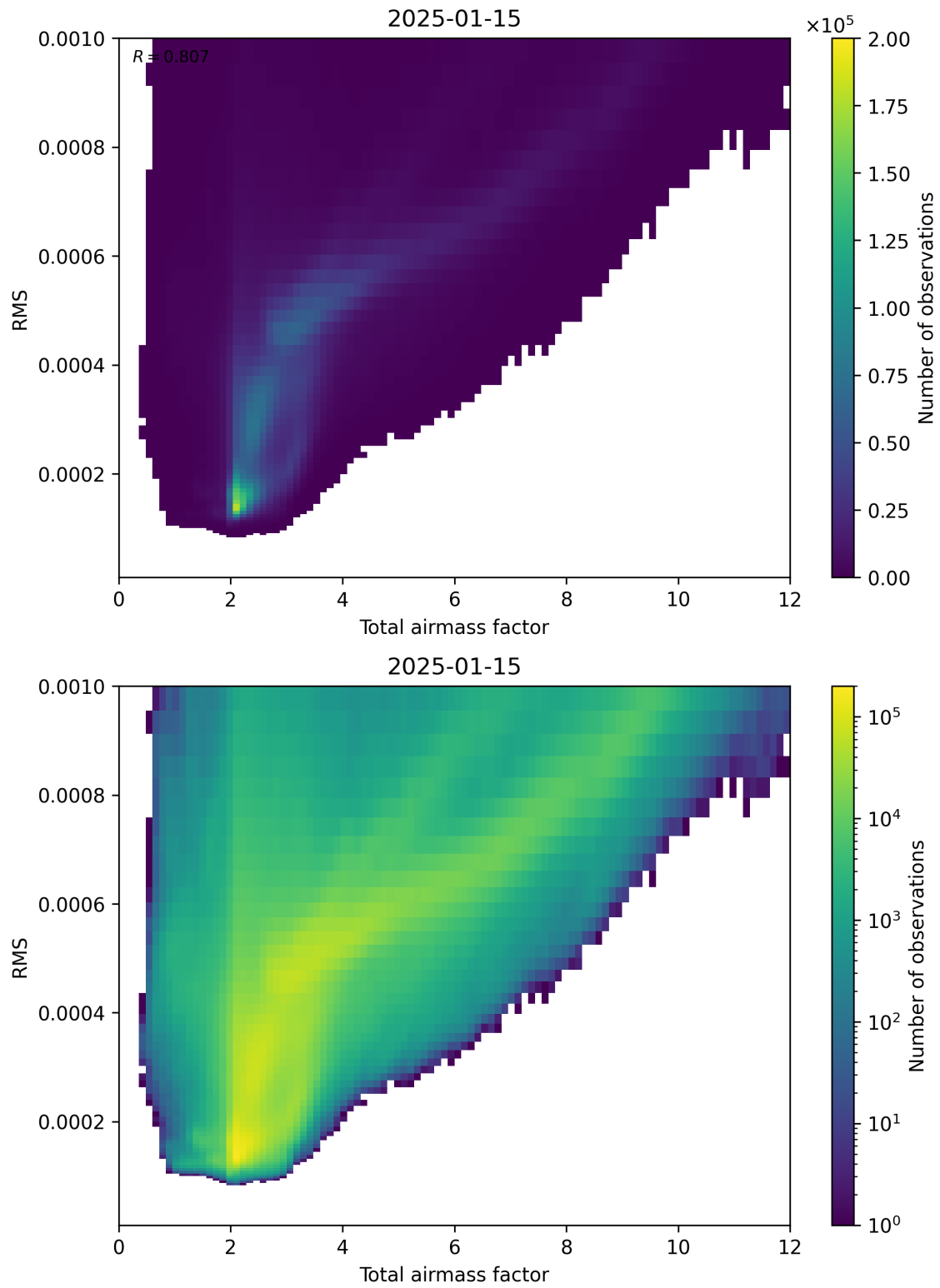
Figure 69: Scatter density plot of “Total airmass factor” against “RMS” for 2025-01-14 to 2025-01-16.
