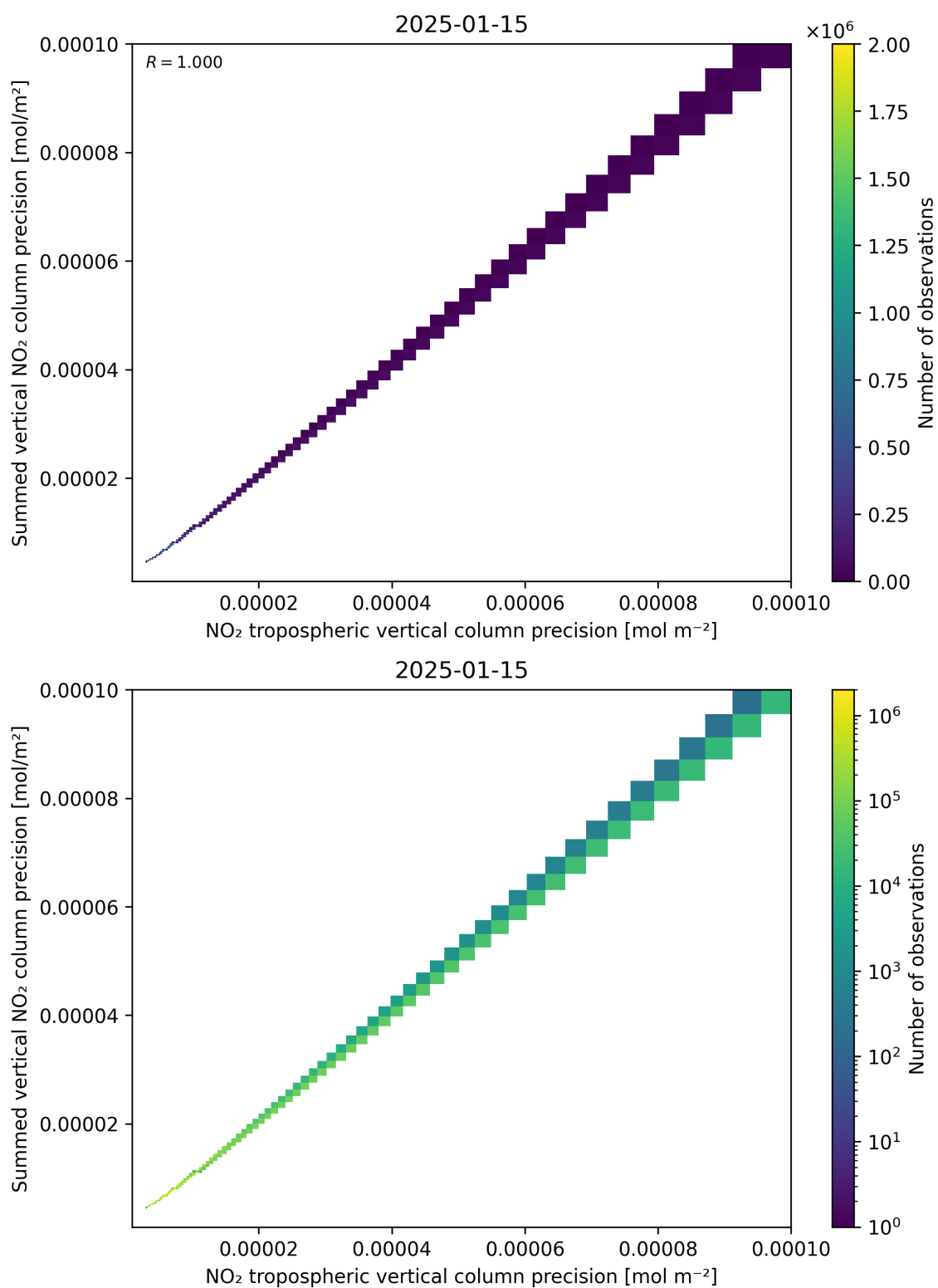
Figure 137: Scatter density plot of “NO 2 tropospheric vertical column precision” against “Summed vertical NO 2 column precision” for 2025-01-14 to 2025-01-16.
