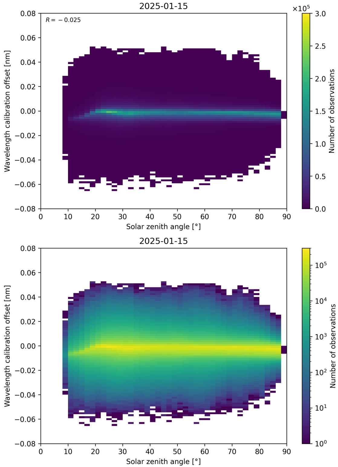
Figure 158: Scatter density plot of “Solar zenith angle” against “Wavelength calibration offset” for 2025-01-14 to 2025-01-16.
