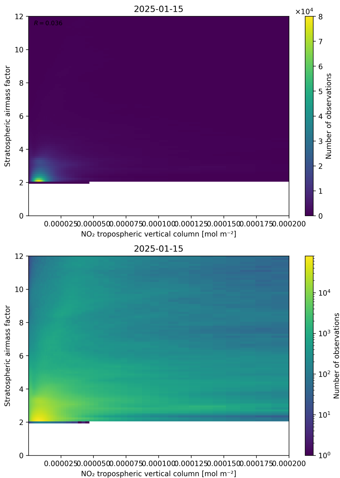
Figure 121: Scatter density plot of “NO 2 tropospheric vertical column” against “Stratospheric airmass factor” for 2025-01-14 to 2025-01-16.
