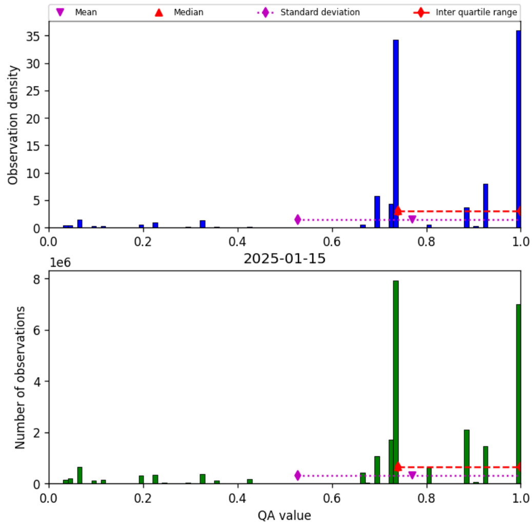
Figure 28: Histogram of “QA value” for 2025-01-14 to 2025-01-16
