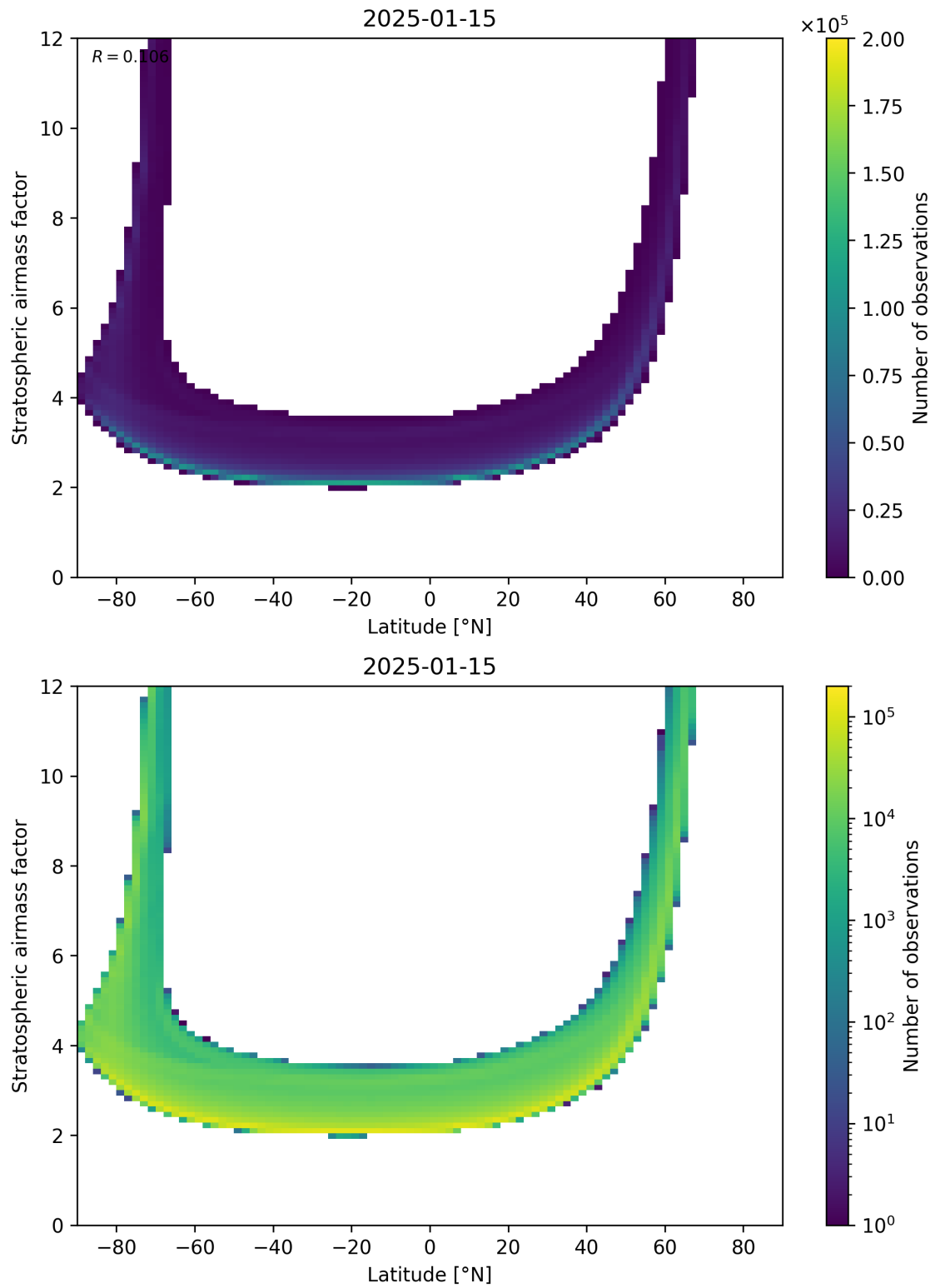
Figure 83: Scatter density plot of “Latitude” against “Stratospheric air mass factor” for 2025-01-14 to 2025-01-16.
