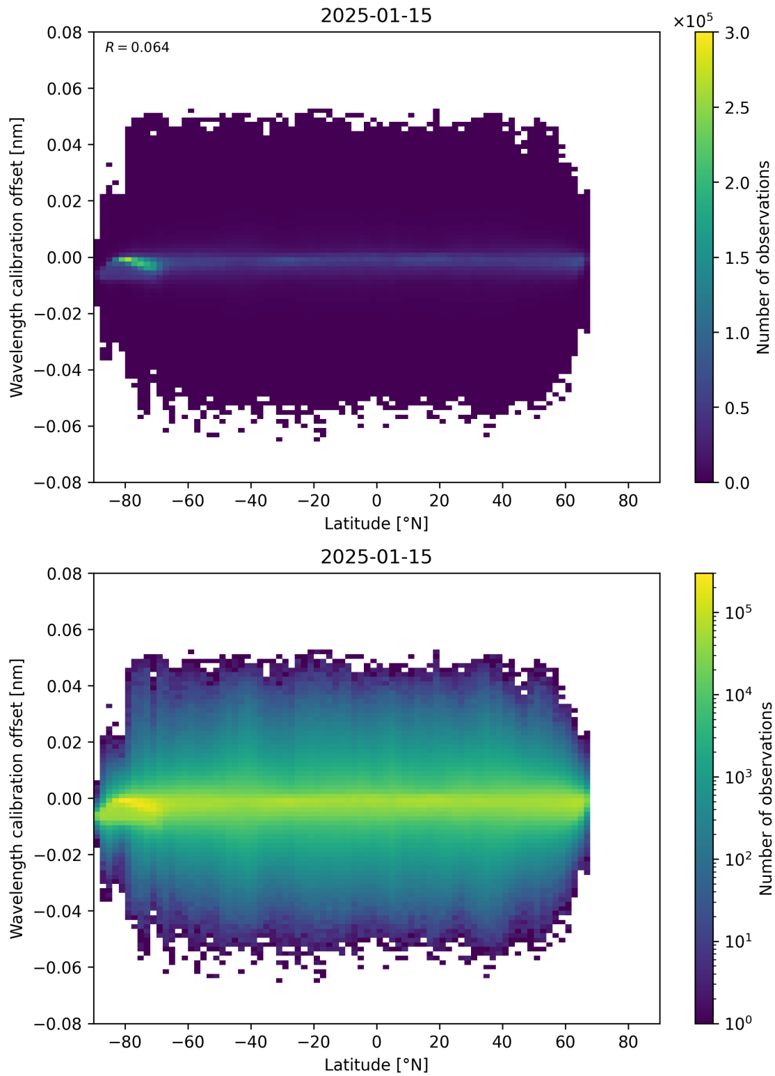
Figure 95: Scatter density plot of “Latitude” against “Wavelength calibration offset” for 2025-01-14 to 2025-01-16.
