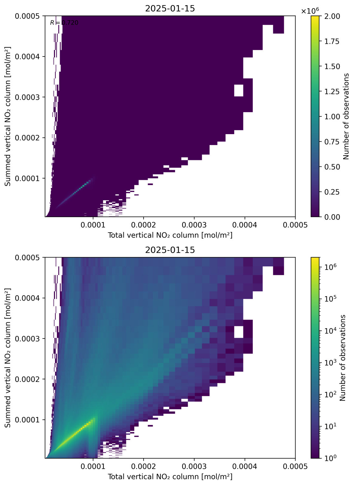
Figure 112: Scatter density plot of “Total vertical NO 2 column” against “Summed vertical NO 2 column” for 2025-01-14 to 2025-01-16.
