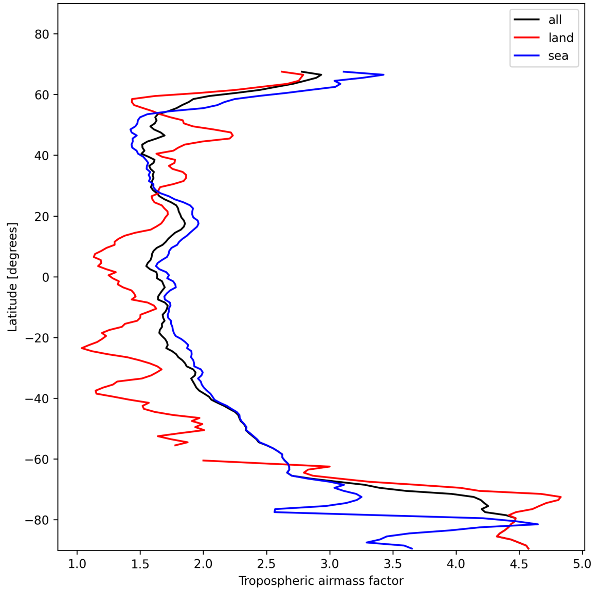
Figure 14: Zonal average of “Tropospheric airmass factor” for 2025-01-14 to 2025-01-16.
