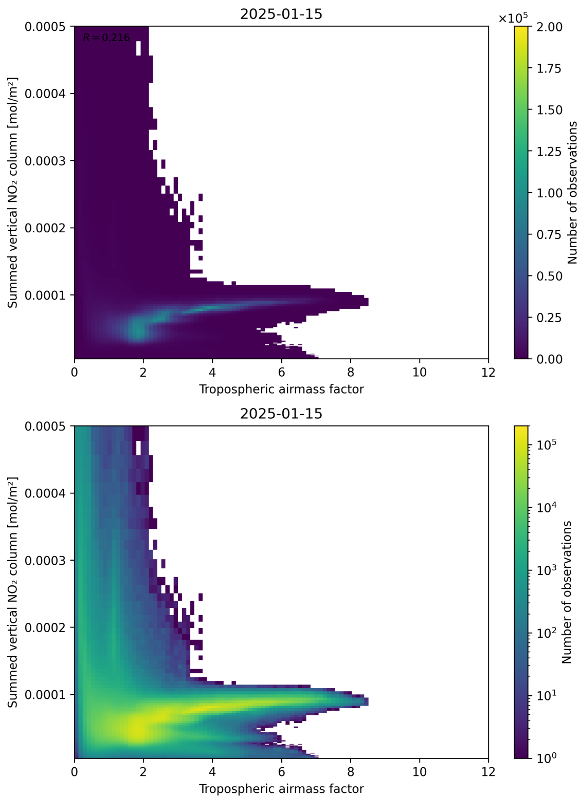
Figure 75: Scatter density plot of “Tropospheric air mass factor” against “Summed vertical NO 2 column” for 2025-01-14 to 2025-01-16.
