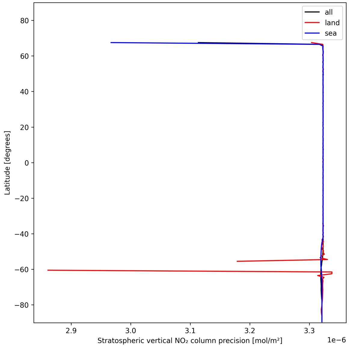
Figure 20: Zonal average of “Stratospheric vertical NO 2 column precision” for 2025-01-14 to 2025-01-16.
