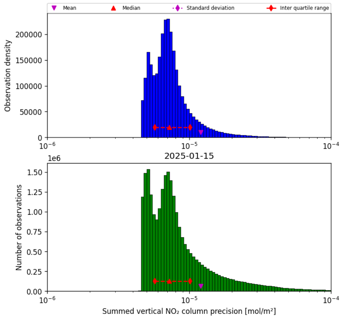
Figure 41: Histogram of "Summed vertical NO 2 column precision" for 2025-01-14 to 2025-01-16
