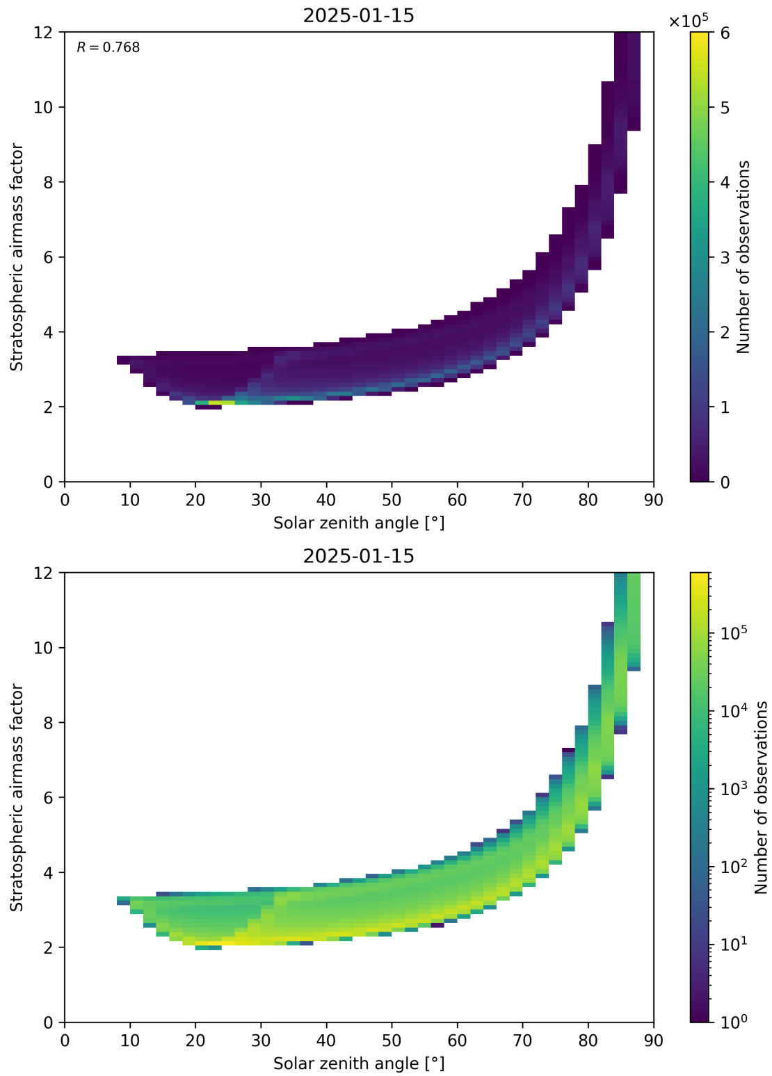
Figure 145: Scatter density plot of “Solar zenith angle” against “Stratospheric airmass factor” for 2025-01-14 to 2025-01-16.
