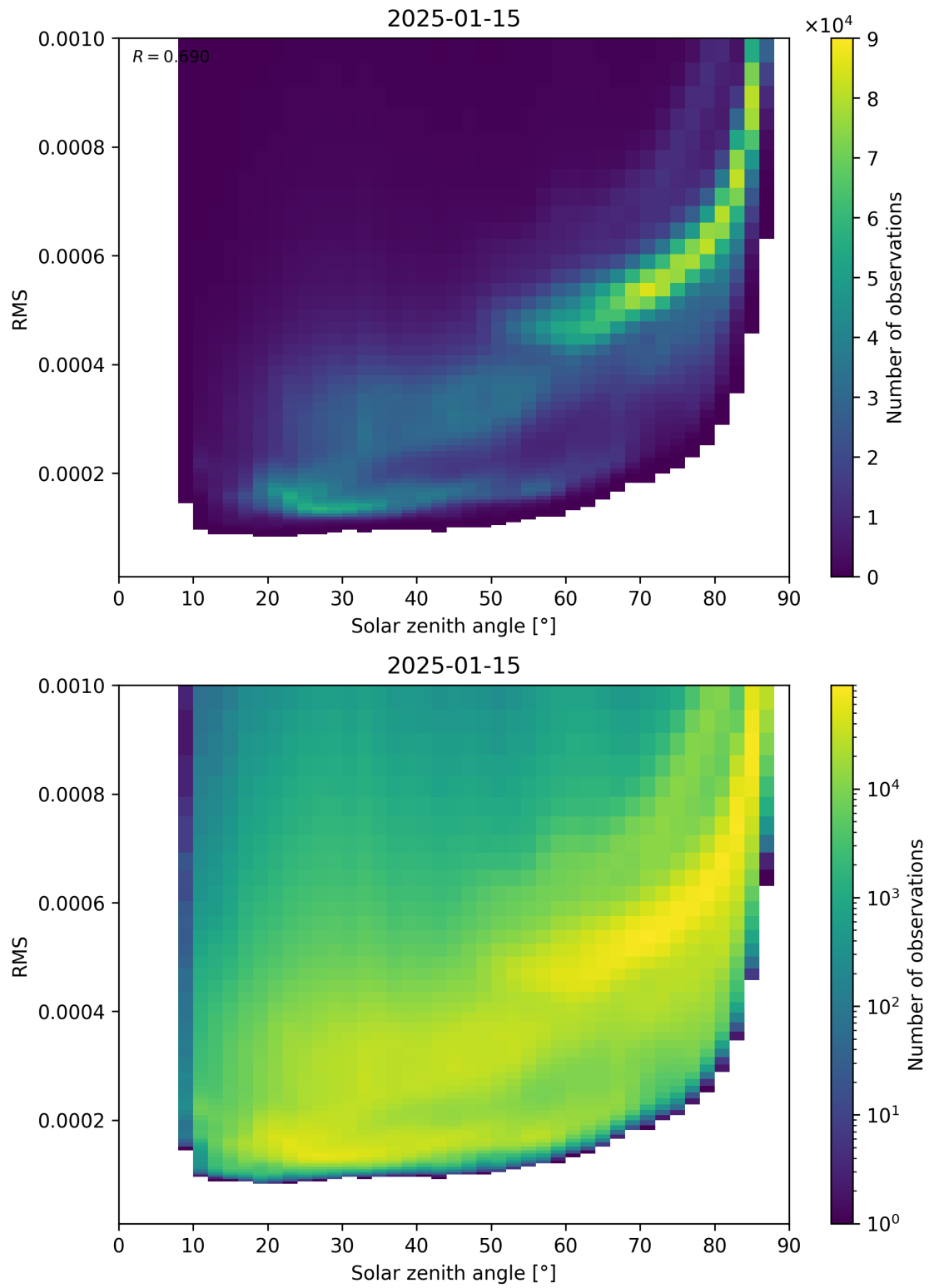
Figure 157: Scatter density plot of “Solar zenith angle” against “RMS” for 2025-01-14 to 2025-01-16.
