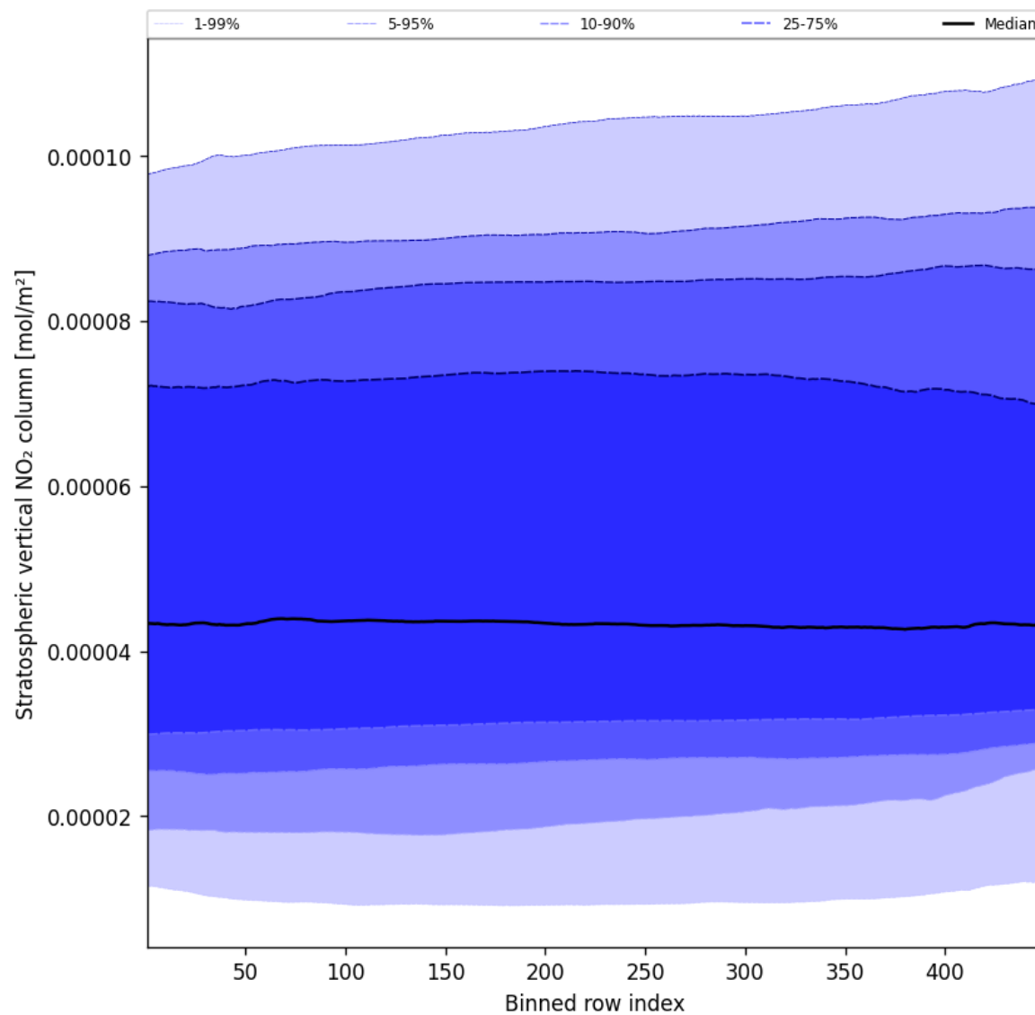
Figure 53: Along track statistics of “Stratospheric vertical NO 2 column” for 2025-01-14 to 2025-01-16
