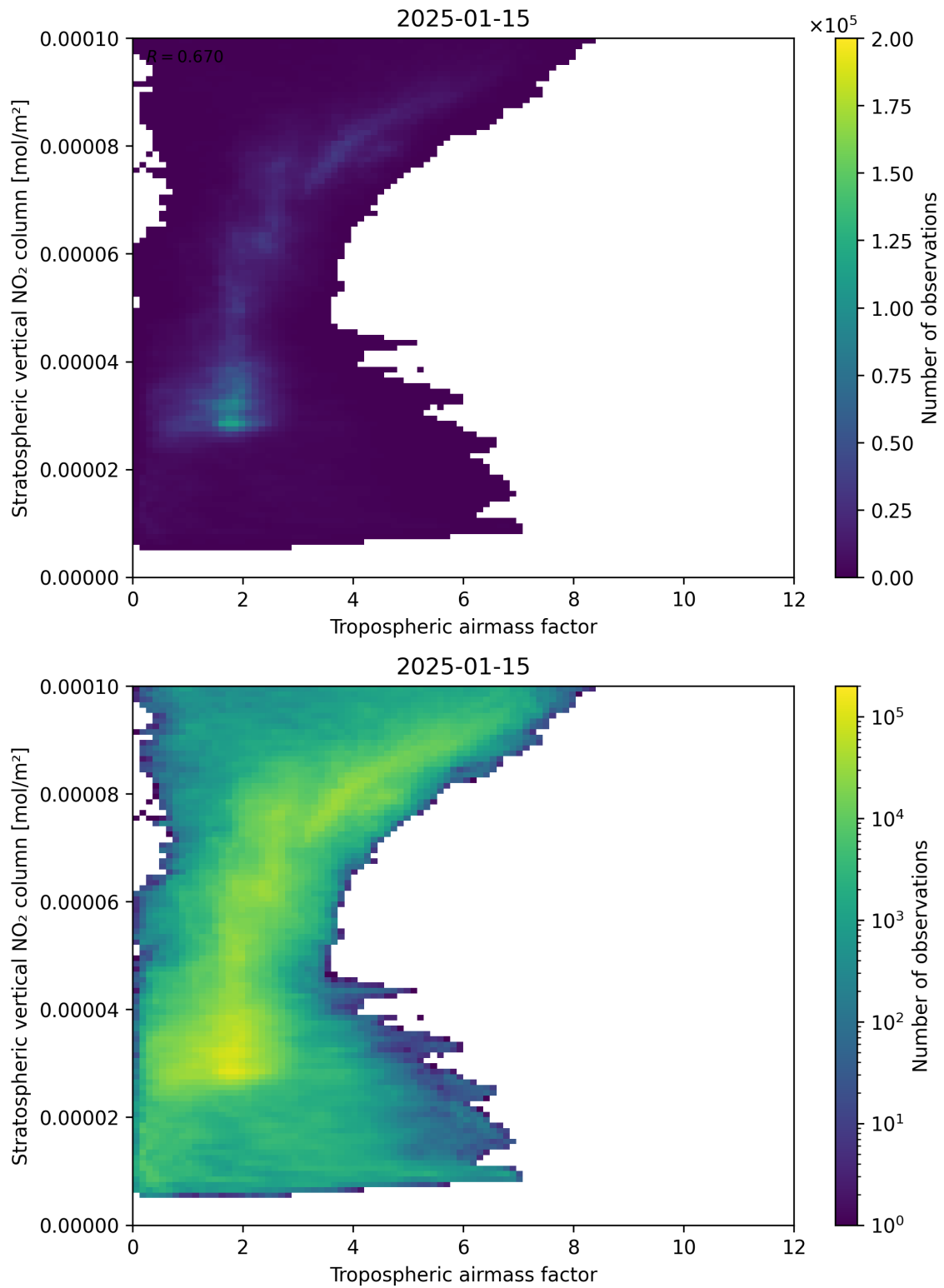
Figure 74: Scatter density plot of “Tropospheric air mass factor” against “Stratospheric vertical NO 2 column” for 2025-01-14 to 2025-01-16.
