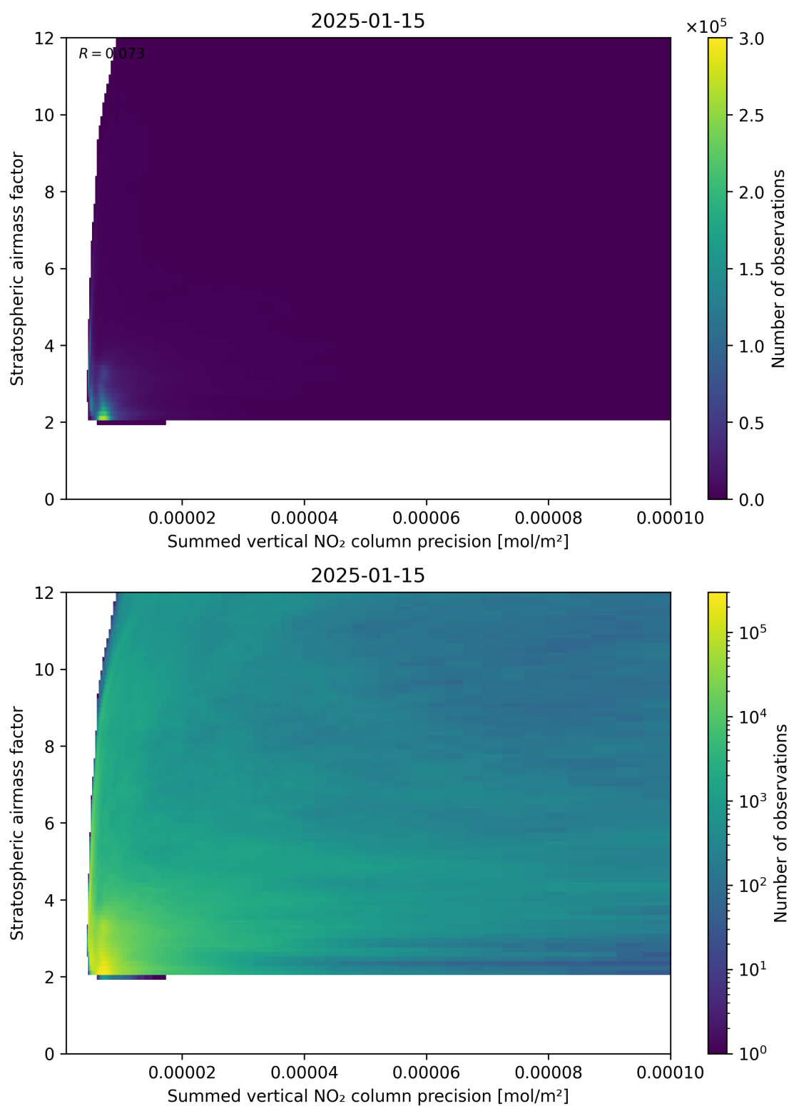
Figure 106: Scatter density plot of “Summed vertical NO 2 column precision” against “Stratospheric airmass factor” for 2025-01-14 to 2025-01-16.
