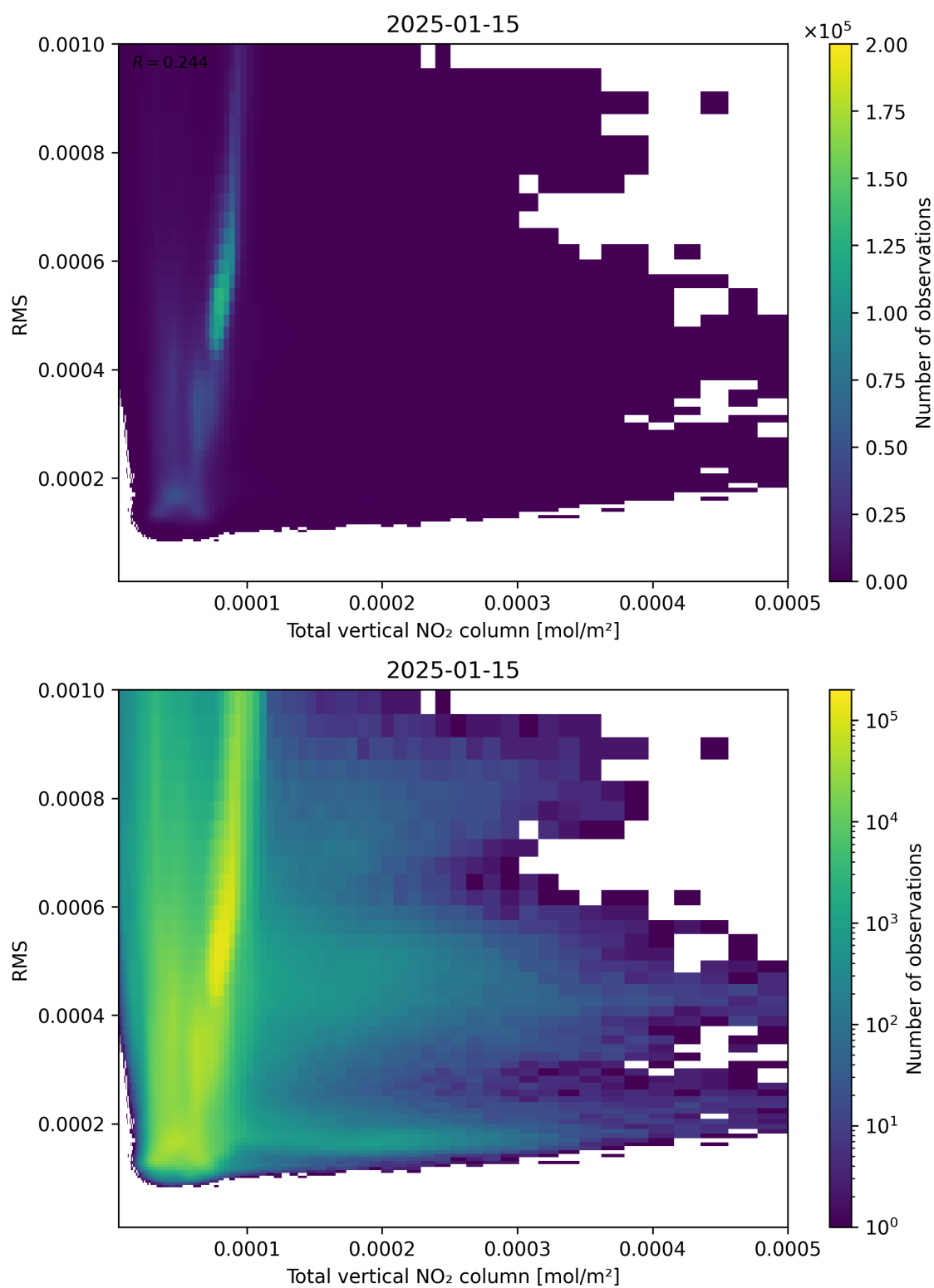
Figure 120: Scatter density plot of “Total vertical NO 2 column” against “RMS” for 2025-01-14 to 2025-01-16.
