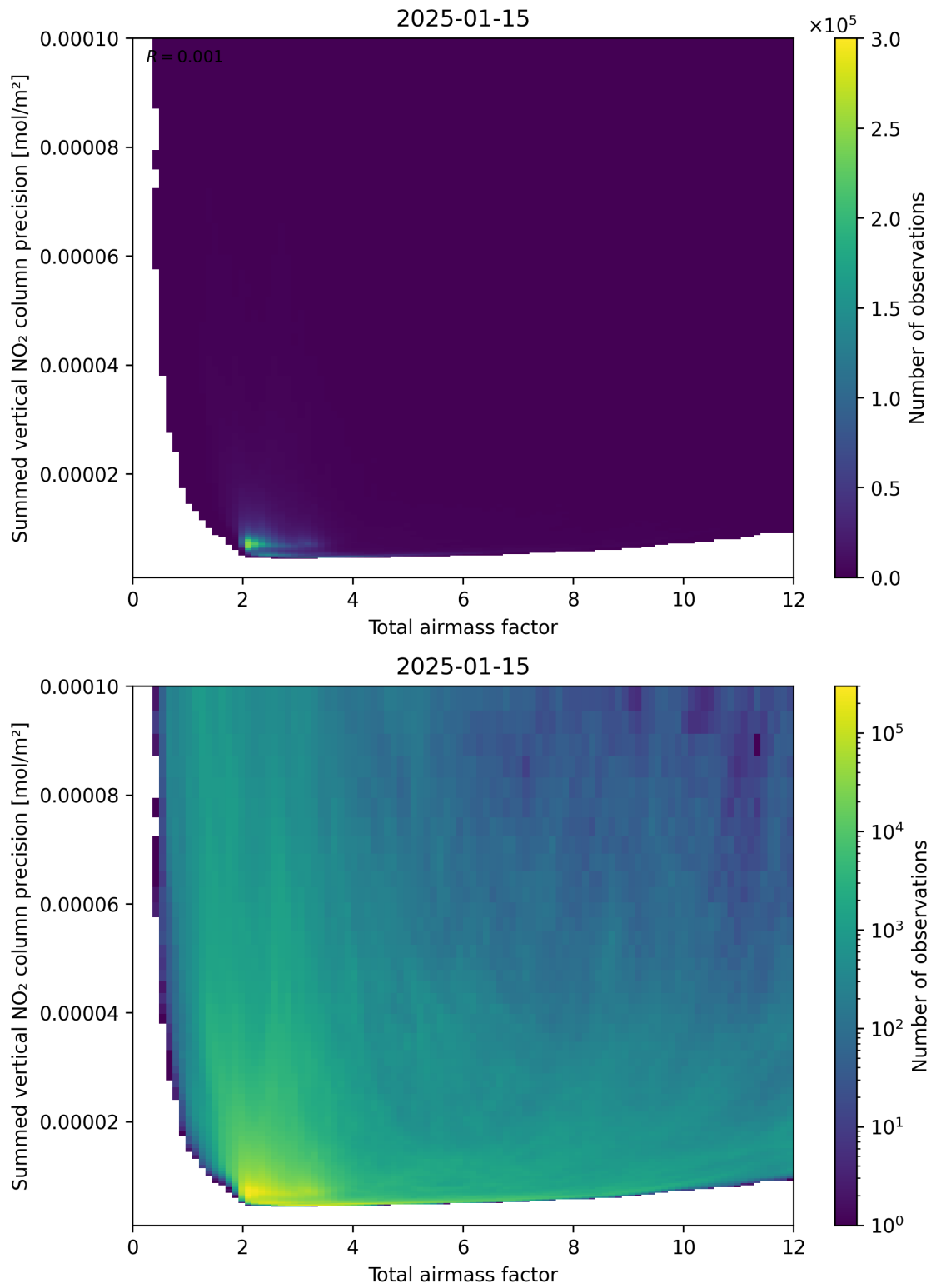
Figure 66: Scatter density plot of “Total airmass factor” against “Summed vertical NO 2 column precision” for 2025-01-14 to 2025-01-16.
