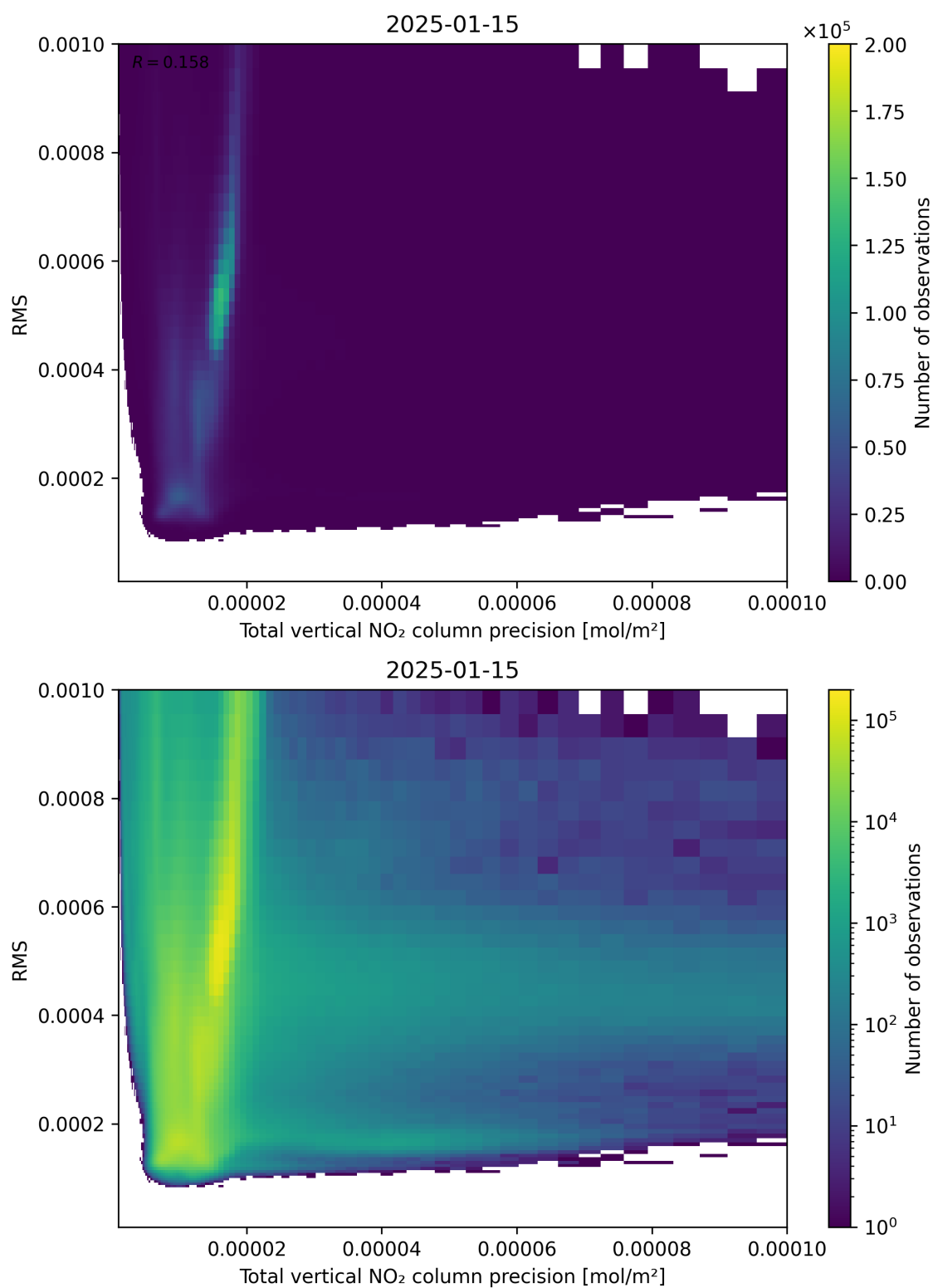
Figure 119: Scatter density plot of “Total vertical NO 2 column precision” against “RMS” for 2025-01-14 to 2025-01-16.
