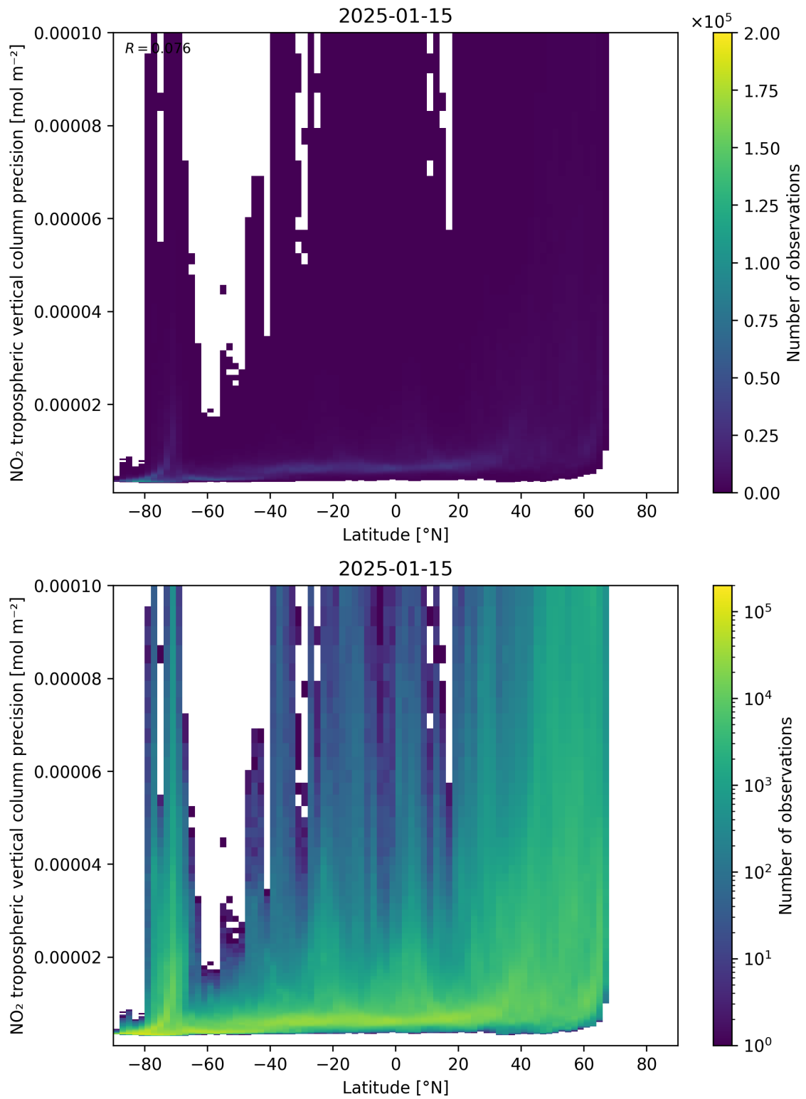
Figure 93: Scatter density plot of “Latitude” against “NO 2 tropospheric vertical column precision” for 2025-01-14 to 2025-01-16.
