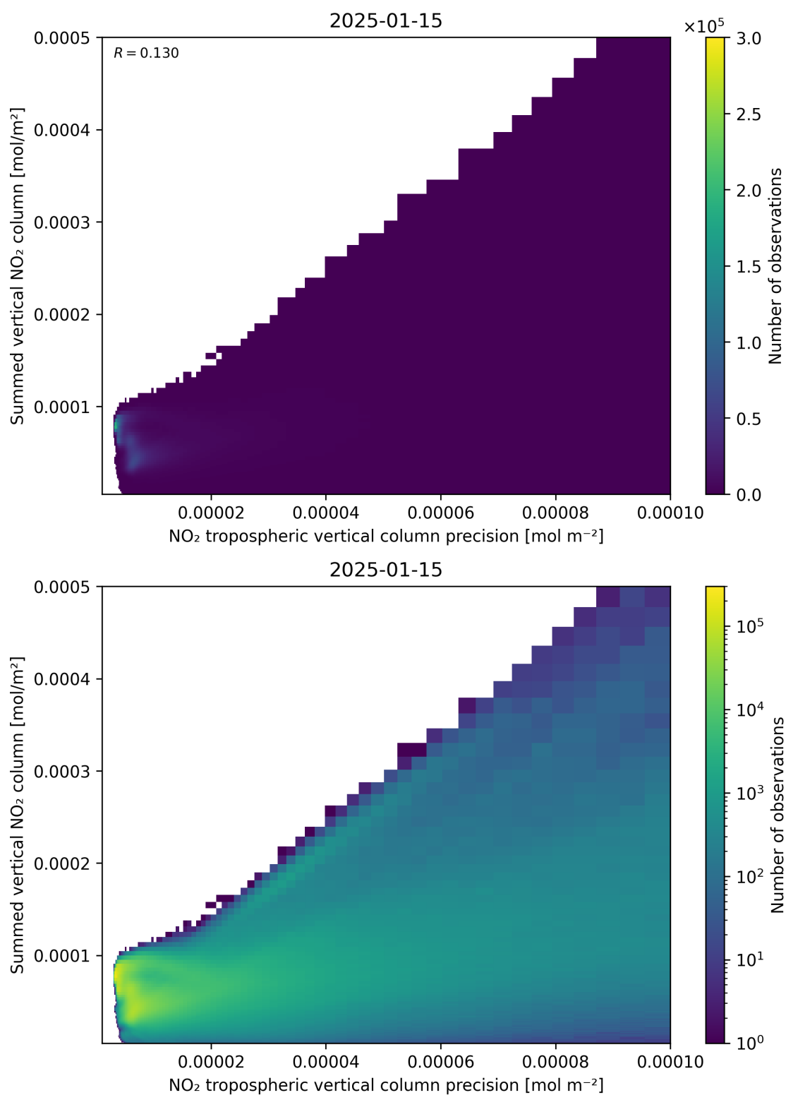
Figure 136: Scatter density plot of “NO 2 tropospheric vertical column precision” against “Summed vertical NO 2 column” for 2025-01-14 to 2025-01-16.
