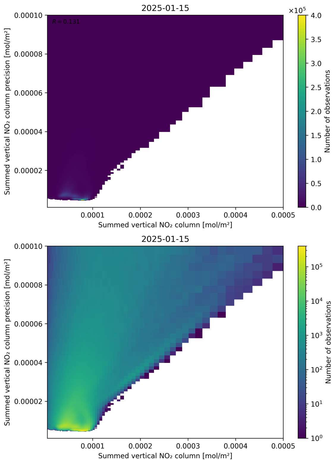
Figure 105: Scatter density plot of “Summed vertical NO 2 column” against “Summed vertical NO 2 column precision” for 2025-01-14 to 2025-01-16.
