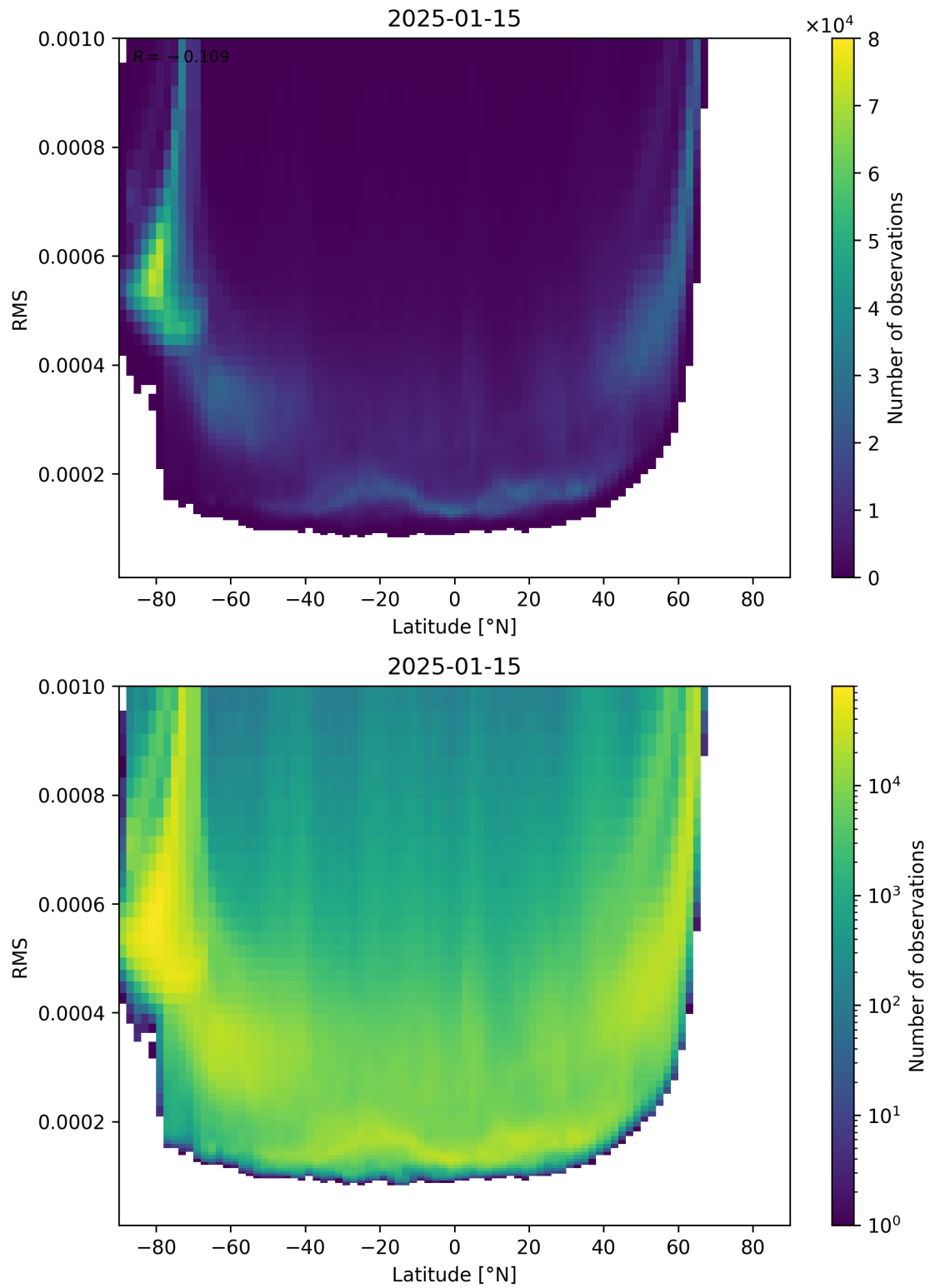
Figure 94: Scatter density plot of “Latitude” against “RMS” for 2025-01-14 to 2025-01-16.
