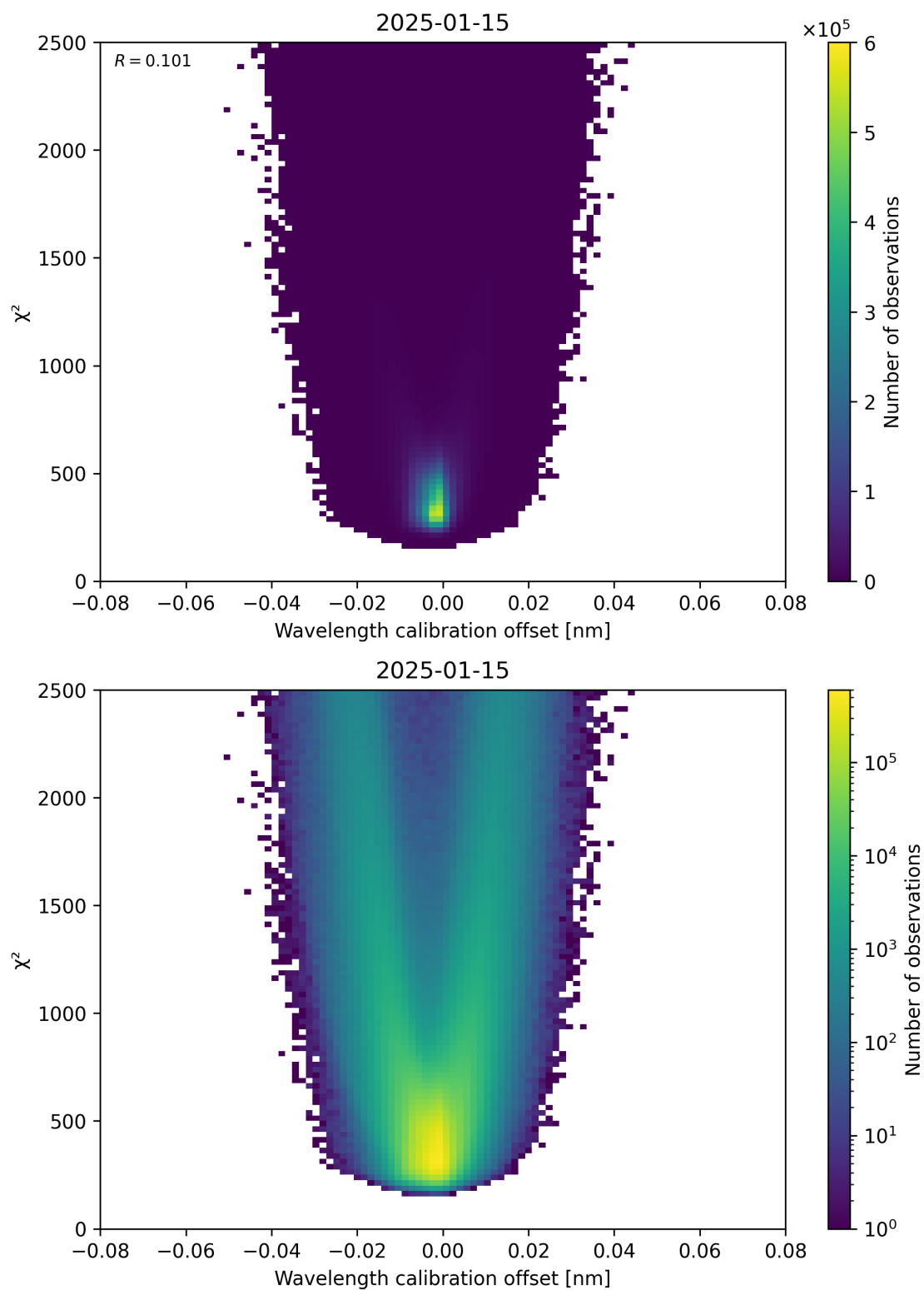
Figure 175: Scatter density plot of “Wavelength calibration offset” against “ \chi^2 ” for 2025-01-14 to 2025-01-16.
