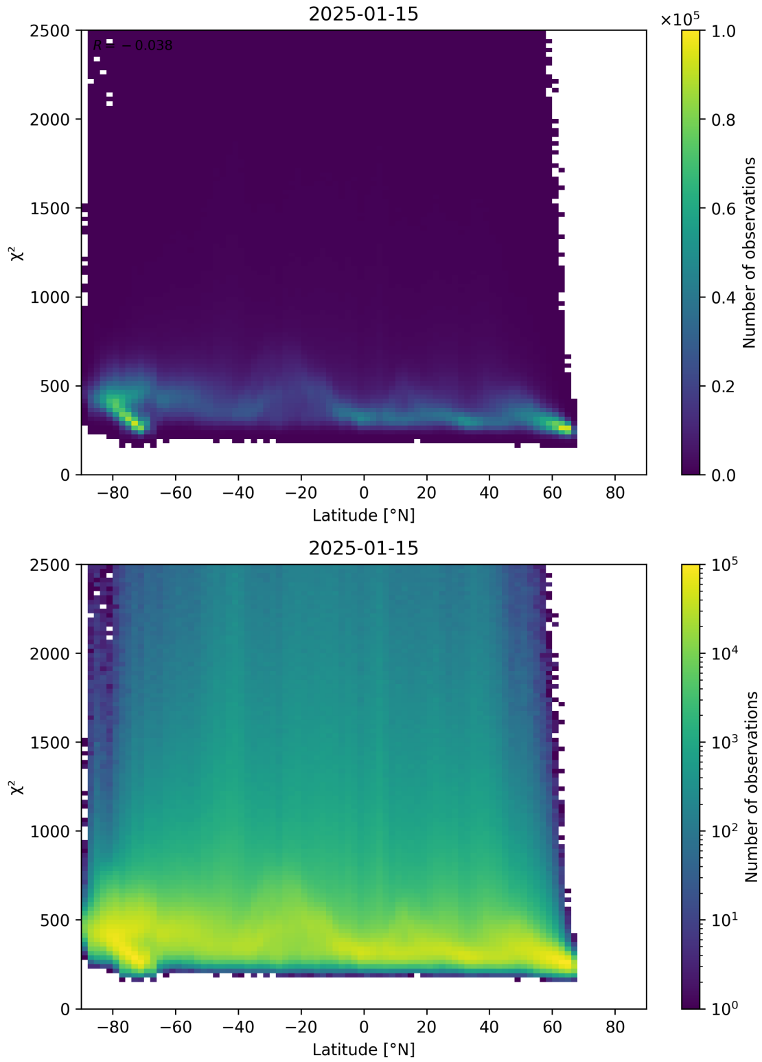
Figure 86: Scatter density plot of “Latitude” against “ \chi^2 ” for 2025-01-14 to 2025-01-16.
