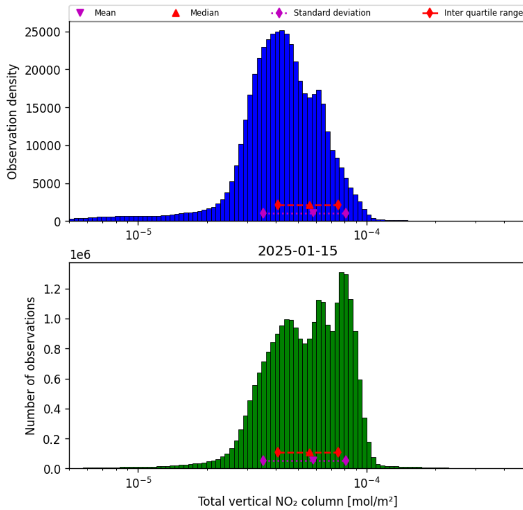
Figure 38: Histogram of “Total vertical NO 2 column” for 2025-01-14 to 2025-01-16
