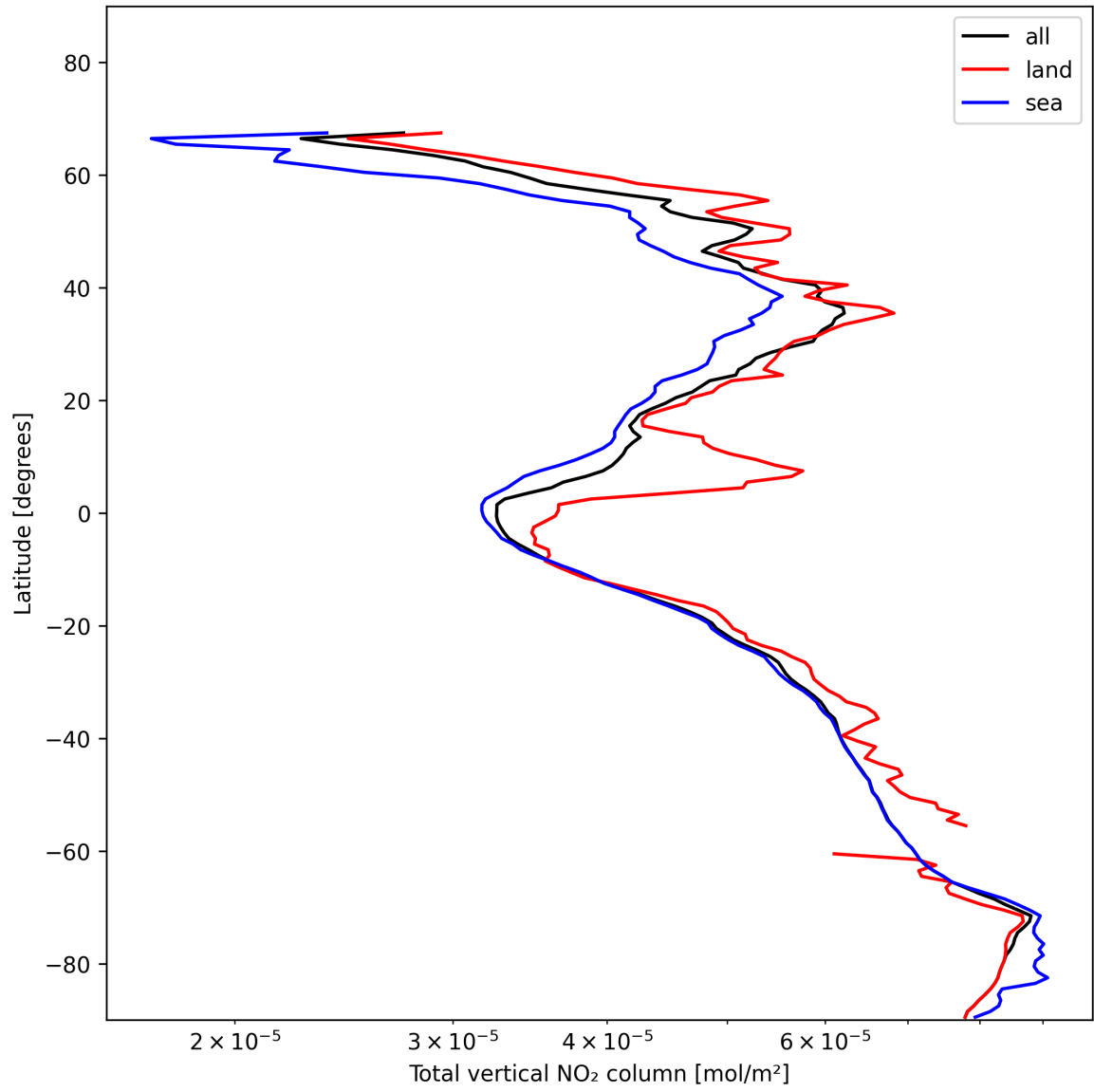
Figure 21: Zonal average of “Total vertical NO 2 column” for 2025-01-14 to 2025-01-16.
