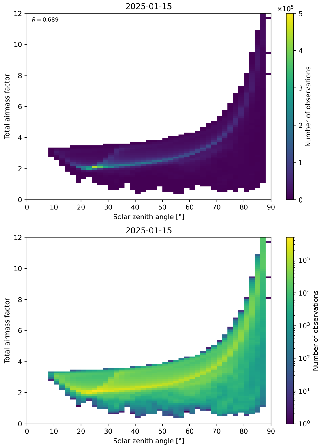
Figure 146: Scatter density plot of “Solar zenith angle” against “Total airmass factor” for 2025-01-14 to 2025-01-16.
