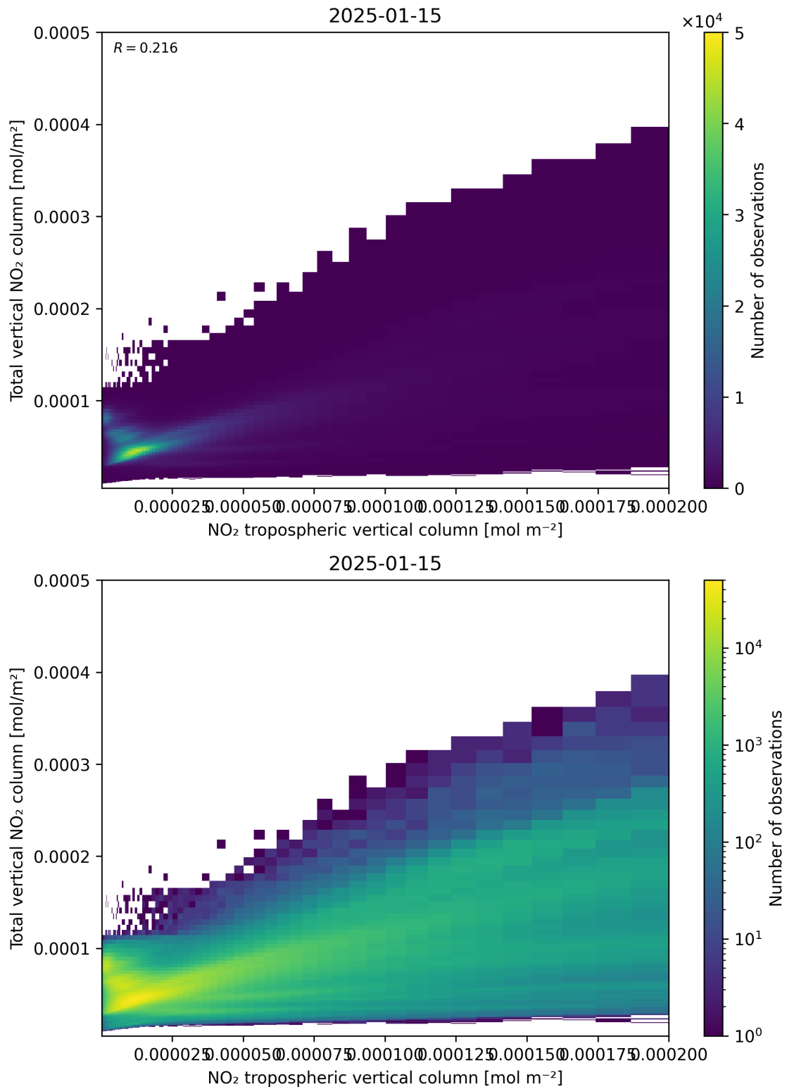
Figure 128: Scatter density plot of “NO 2 tropospheric vertical column” against “Total vertical NO 2 column” for 2025-01-14 to 2025-01-16.
