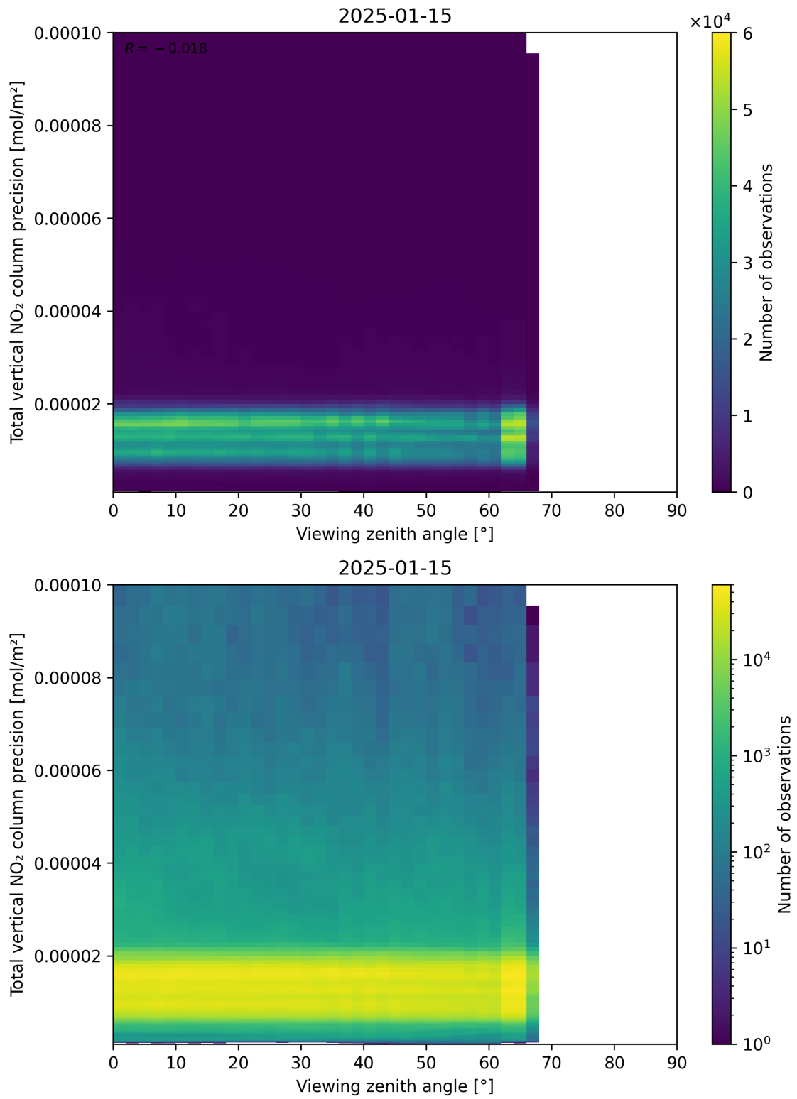
Figure 168: Scatter density plot of “Viewing zenith angle” against “Total vertical NO 2 column precision” for 2025-01-14 to 2025-01-16.
