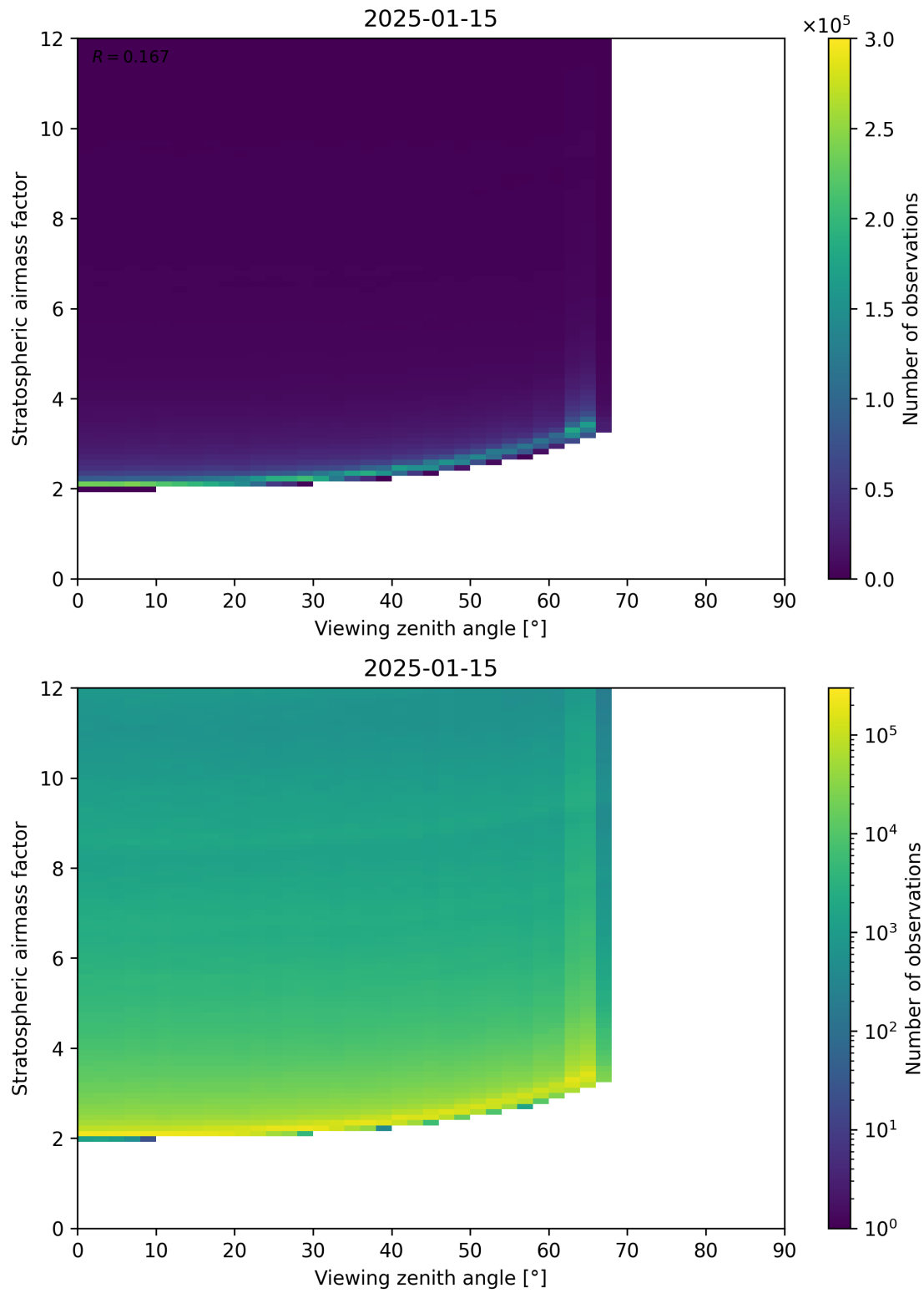
Figure 159: Scatter density plot of “Viewing zenith angle” against “Stratospheric airmass factor” for 2025-01-14 to 2025-01-16.
