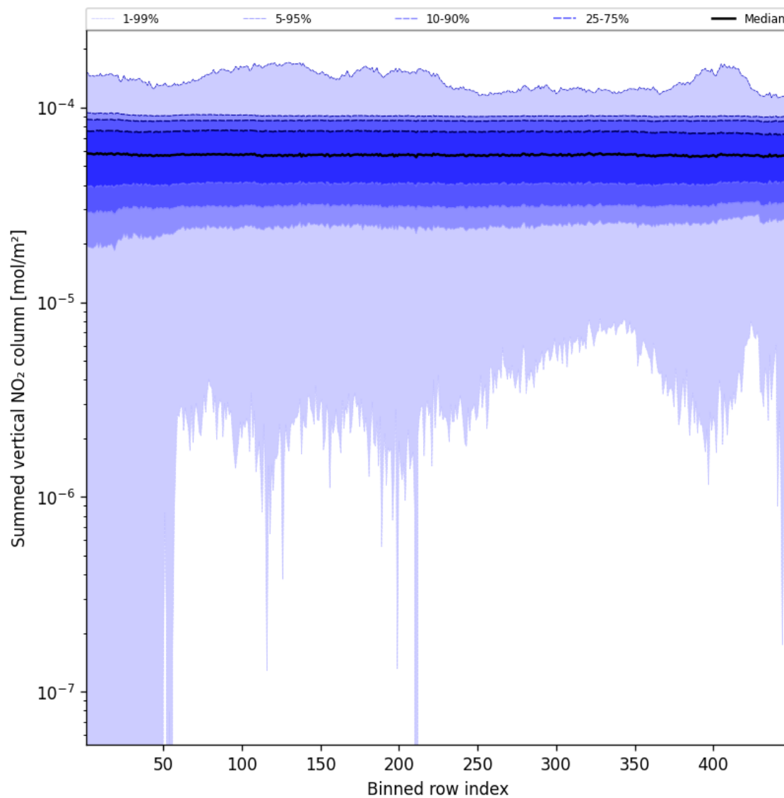
Figure 57: Along track statistics of “Summed vertical NO 2 column” for 2025-01-14 to 2025-01-16
