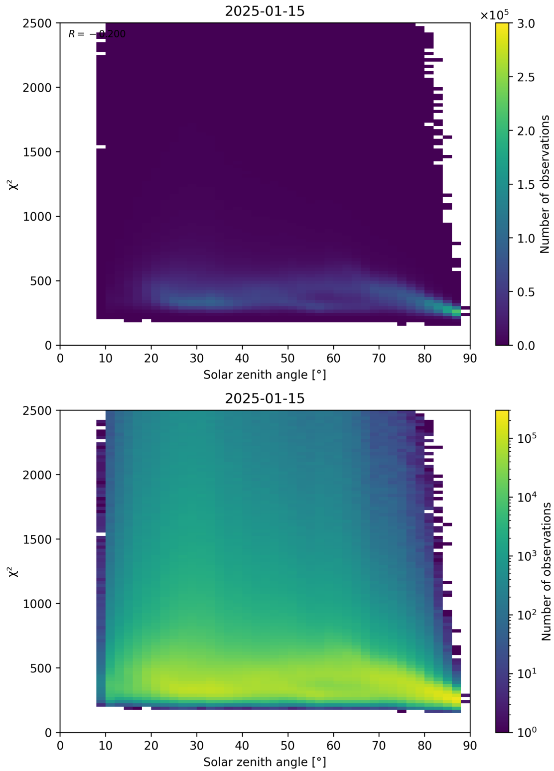
Figure 148: Scatter density plot of “Solar zenith angle” against “ \chi^2 ” for 2025-01-14 to 2025-01-16.
