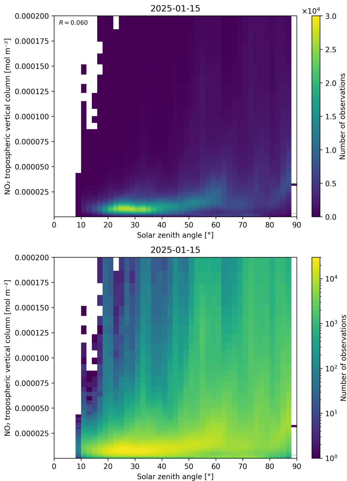
Figure 155: Scatter density plot of “Solar zenith angle” against “NO 2 tropospheric vertical column” for 2025-01-14 to 2025-01-16.
