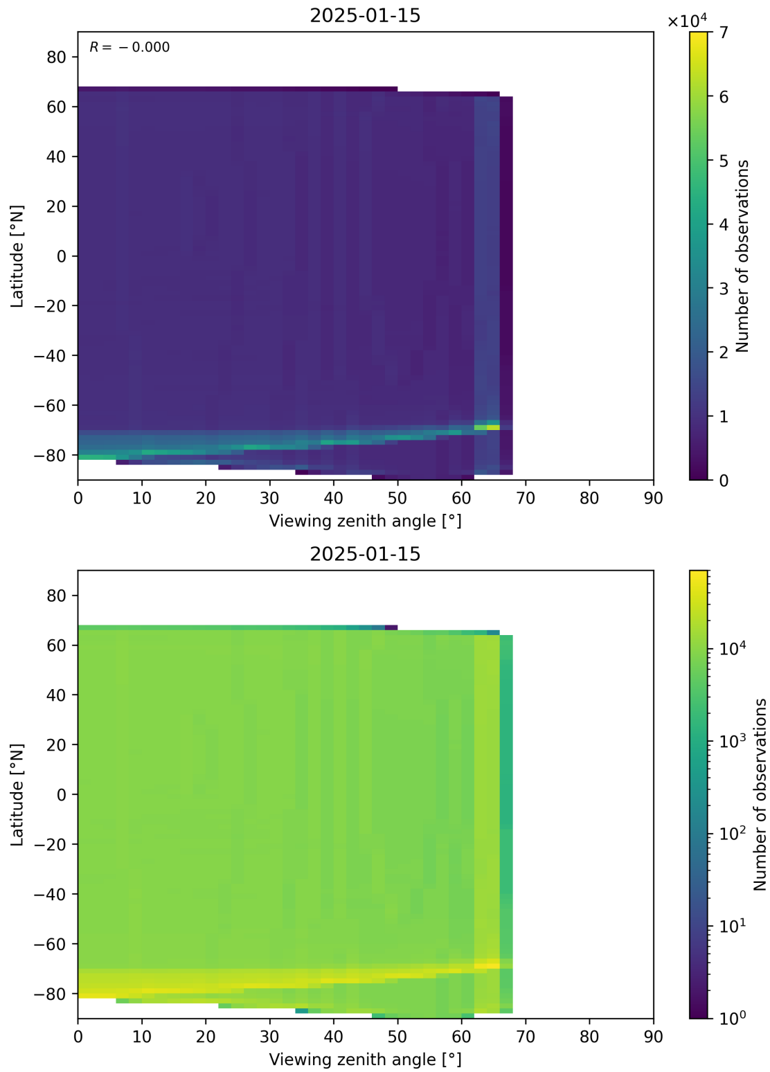
Figure 163: Scatter density plot of “Viewing zenith angle” against “Latitude” for 2025-01-14 to 2025-01-16.
