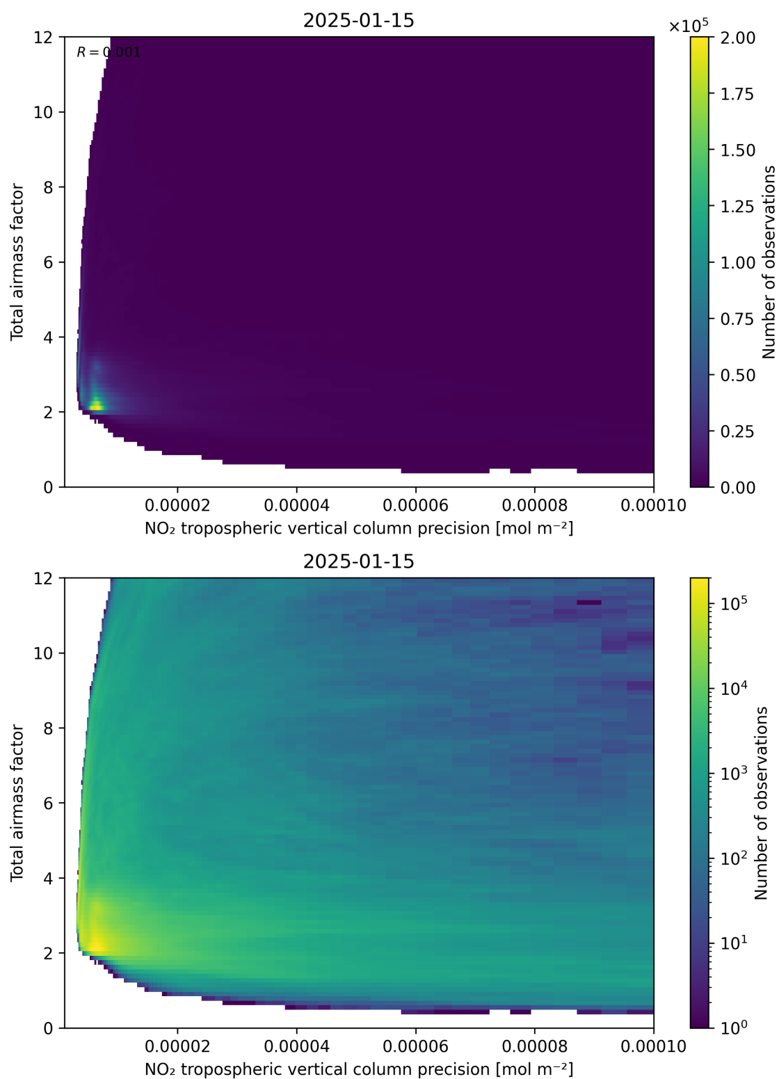
Figure 132: Scatter density plot of “NO 2 tropospheric vertical column precision” against “Total air mass factor” for 2025-01-14 to 2025-01-16.
