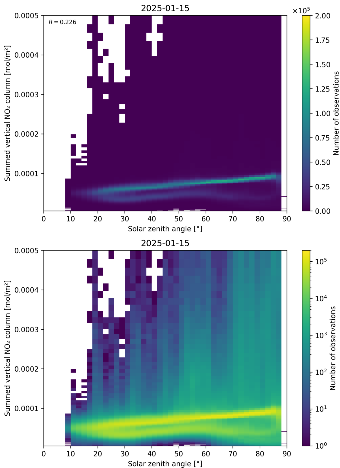
Figure 151: Scatter density plot of “Solar zenith angle” against “Summed vertical NO 2 column” for 2025-01-14 to 2025-01-16.
