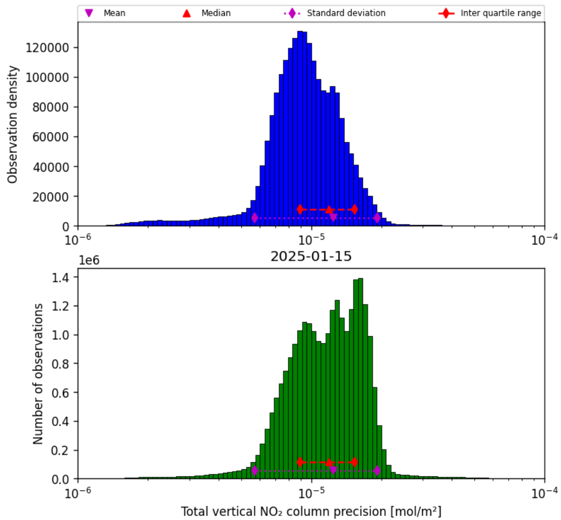
Figure 39: Histogram of “Total vertical NO 2 column precision” for 2025-01-14 to 2025-01-16
