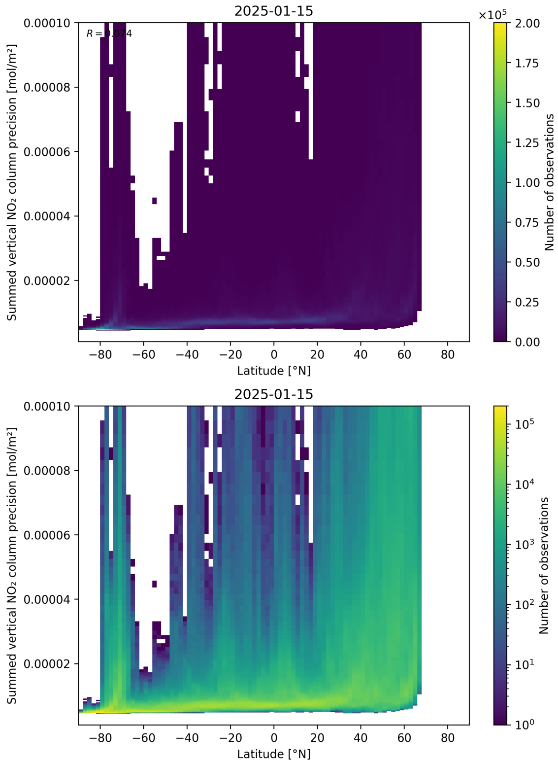
Figure 89: Scatter density plot of “Latitude” against “Summed vertical NO 2 column precision” for 2025-01-14 to 2025-01-16.
