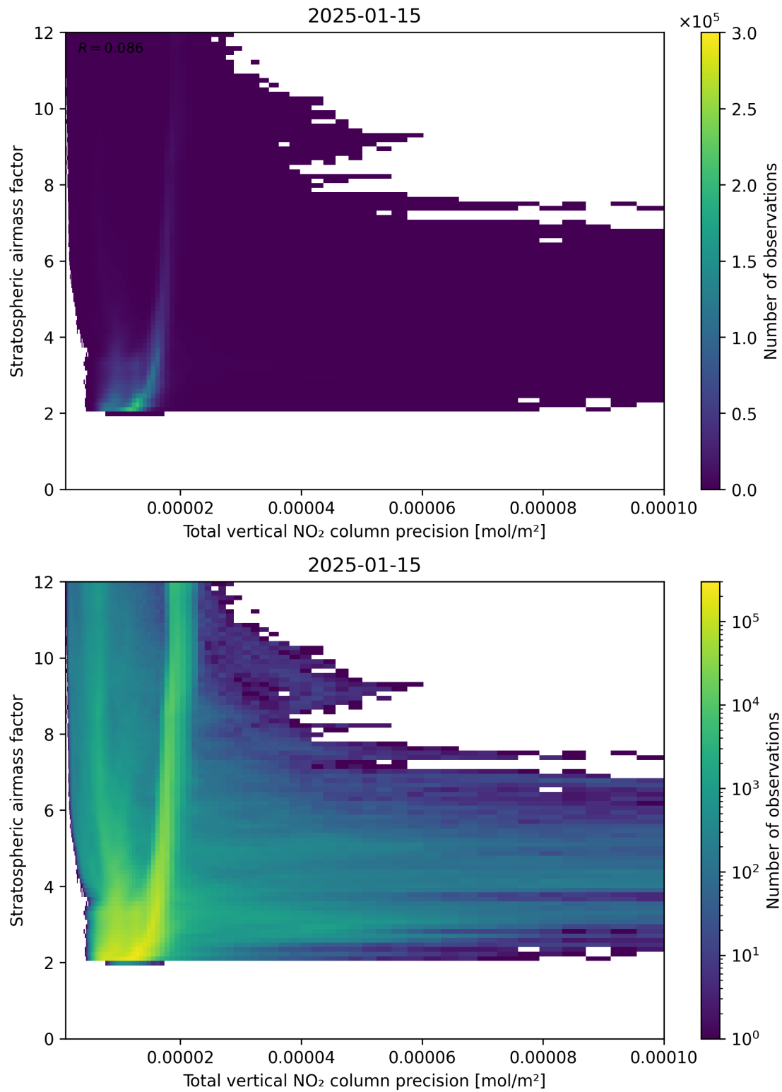
Figure 115: Scatter density plot of “Total vertical NO 2 column precision” against “Stratospheric air mass factor” for 2025-01-14 to 2025-01-16.
