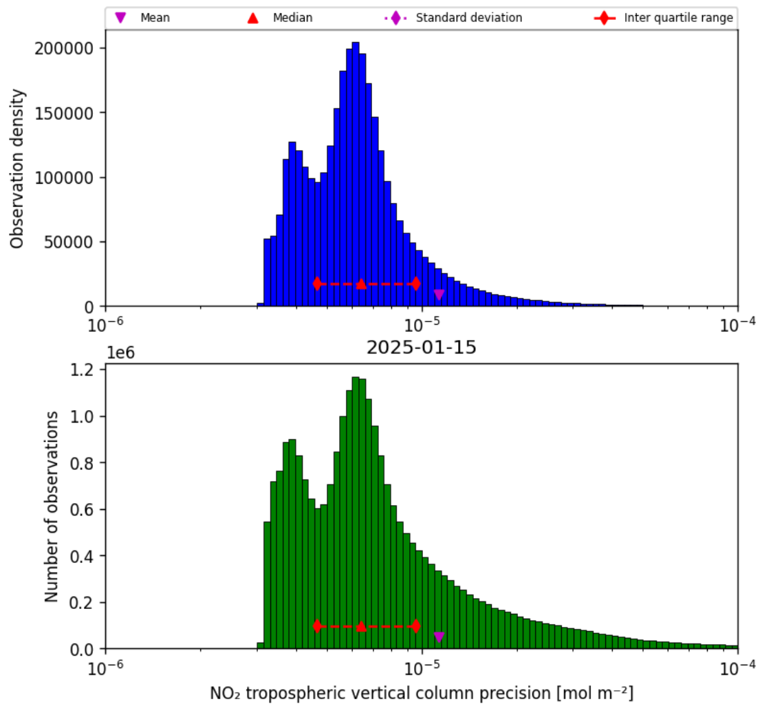
Figure 30: Histogram of “NO 2 tropospheric vertical column precision” for 2025-01-14 to 2025-01-16
