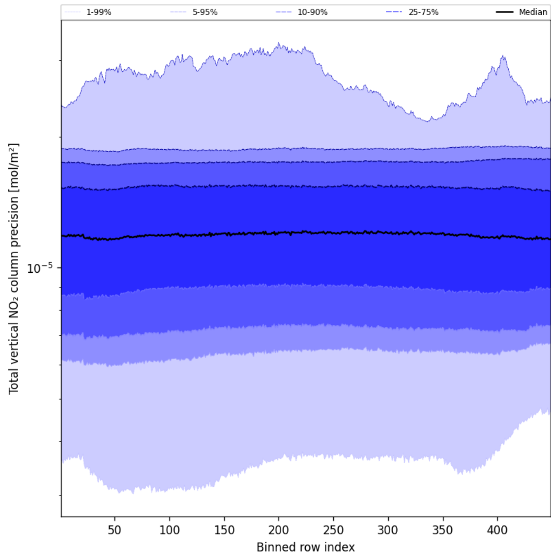
Figure 56: Along track statistics of “Total vertical NO 2 column precision” for 2025-01-14 to 2025-01-16
