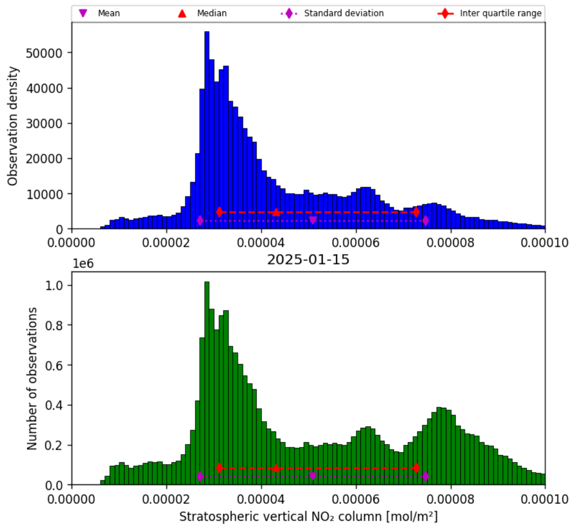
Figure 36: Histogram of “Stratospheric vertical NO 2 column” for 2025-01-14 to 2025-01-16
