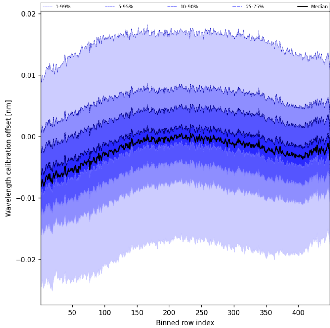
Figure 52: Along track statistics of “Wavelength calibration offset” for 2025-01-14 to 2025-01-16
