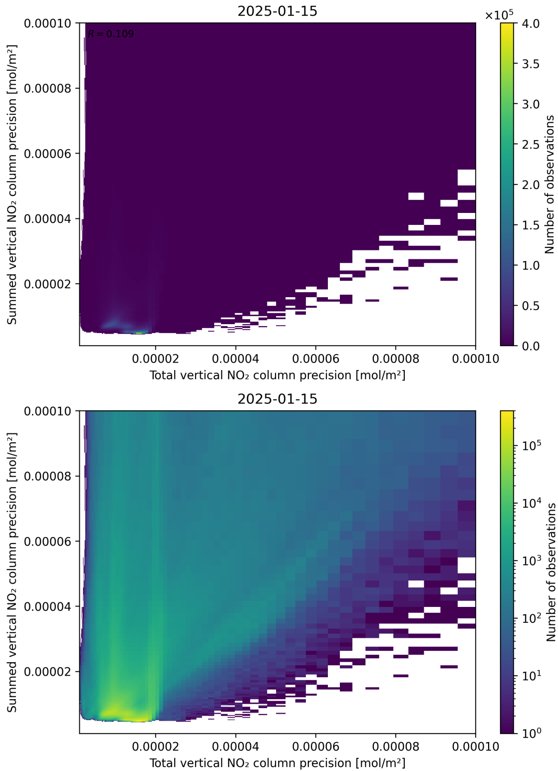
Figure 118: Scatter density plot of “Total vertical NO 2 column precision” against “Summed vertical NO 2 column precision” for 2025-01-14 to 2025-01-16.
