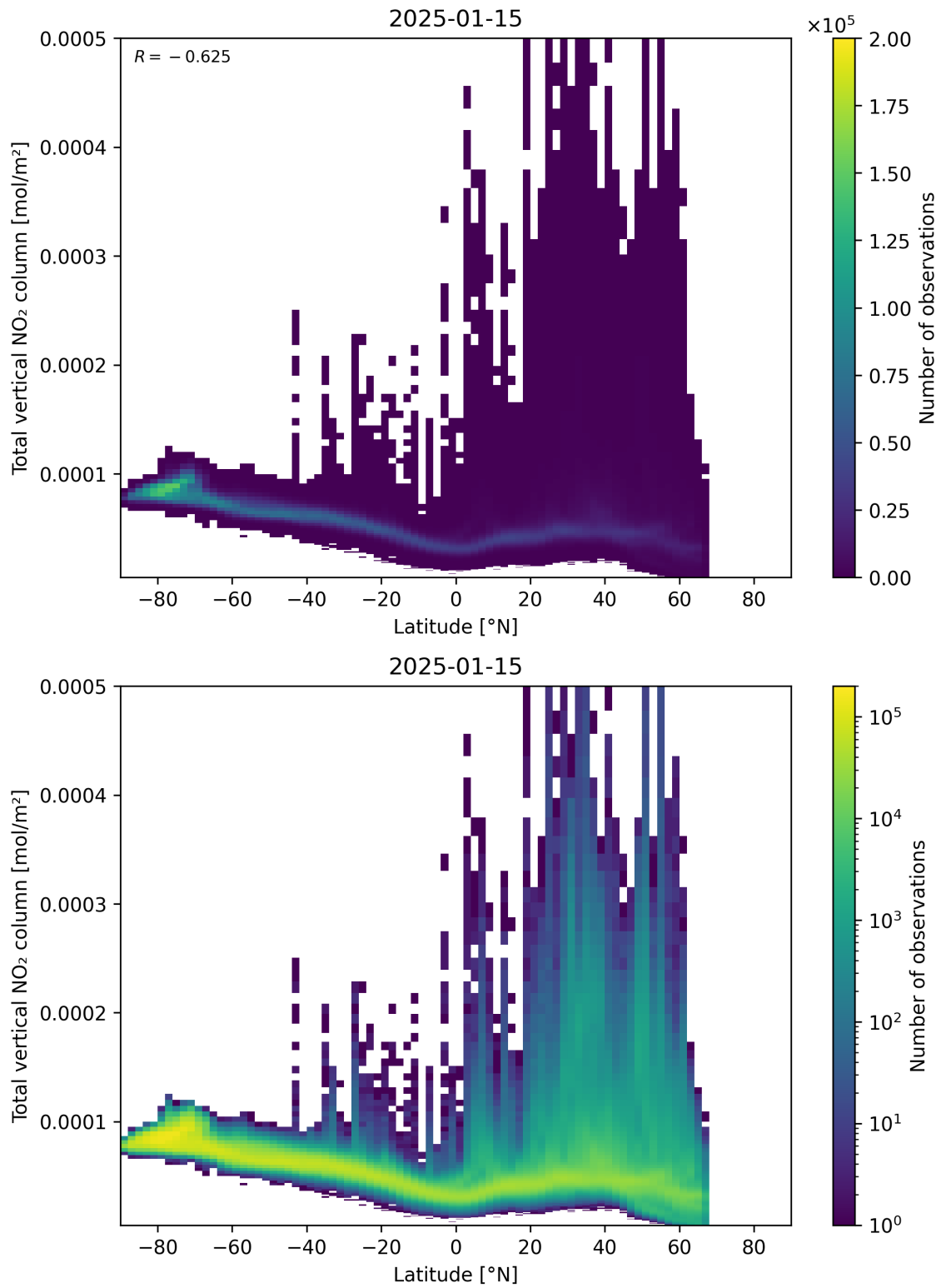
Figure 90: Scatter density plot of “Latitude” against “Total vertical NO 2 column” for 2025-01-14 to 2025-01-16.
