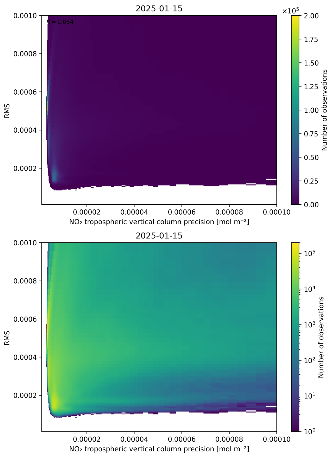
Figure 140: Scatter density plot of “NO 2 tropospheric vertical column precision” against “RMS” for 2025-01-14 to 2025-01-16.
