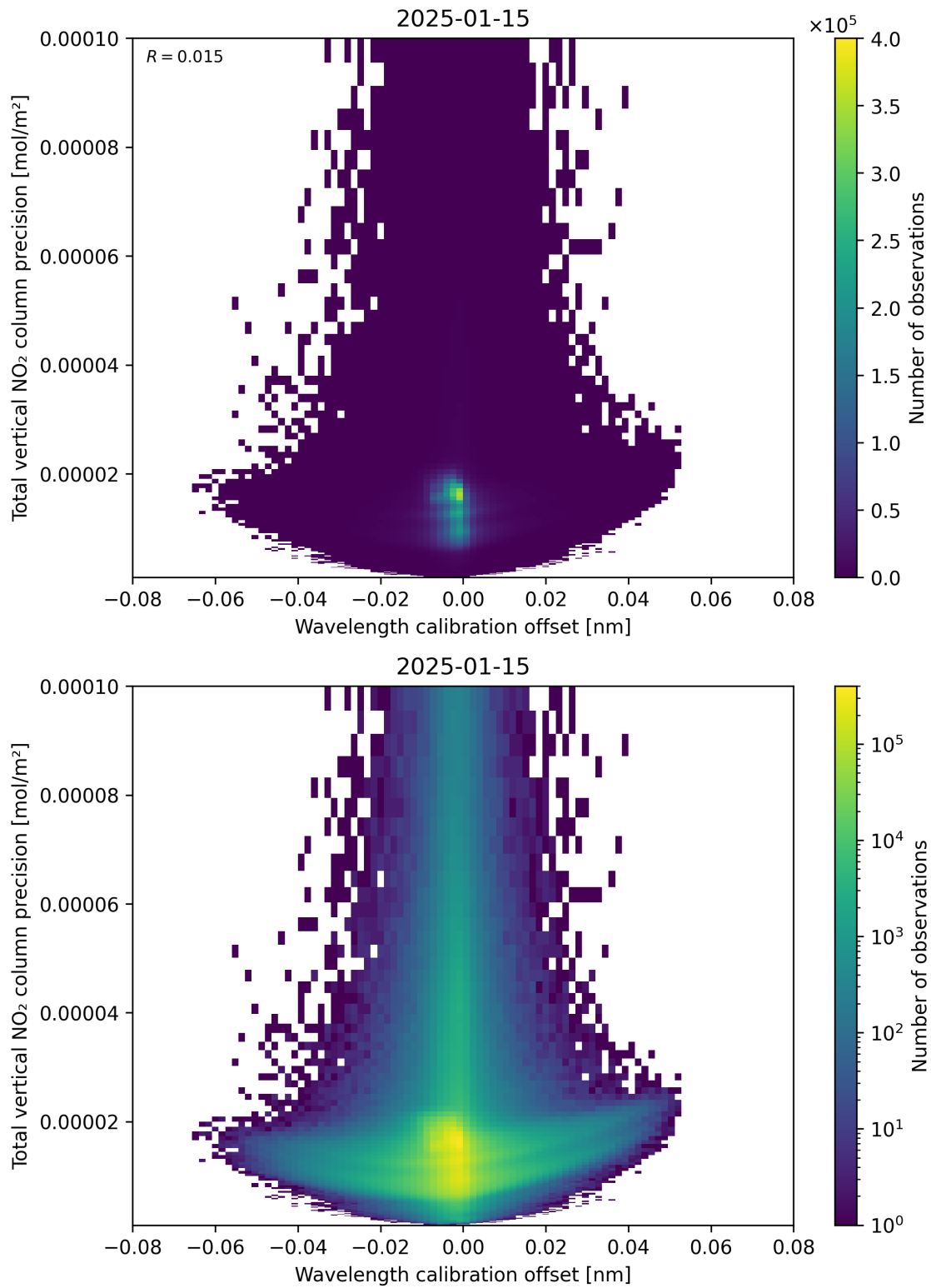
Figure 180: Scatter density plot of “Wavelength calibration offset” against “Total vertical NO 2 column precision” for 2025-01-14 to 2025-01-16.
