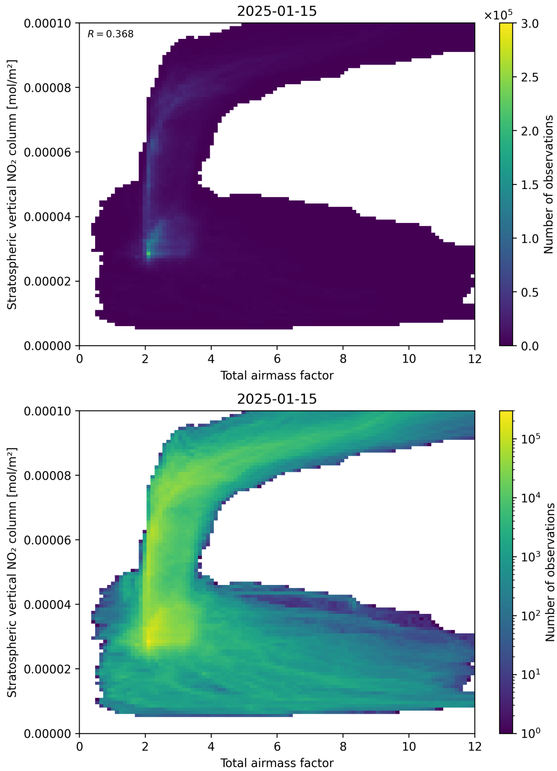
Figure 64: Scatter density plot of “Total airmass factor” against “Stratospheric vertical NO 2 column” for 2025-01-14 to 2025-01-16.
