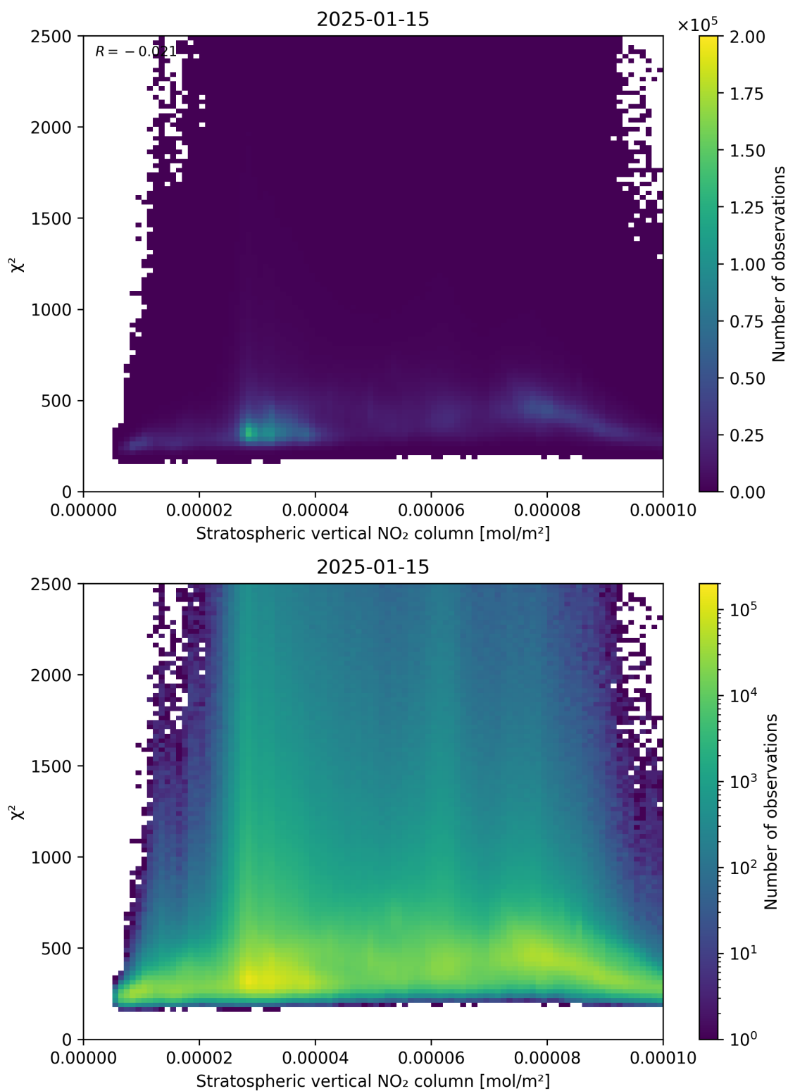
Figure 97: Scatter density plot of “Stratospheric vertical NO 2 column” against “ \chi^2 ” for 2025-01-14 to 2025-01-16.
