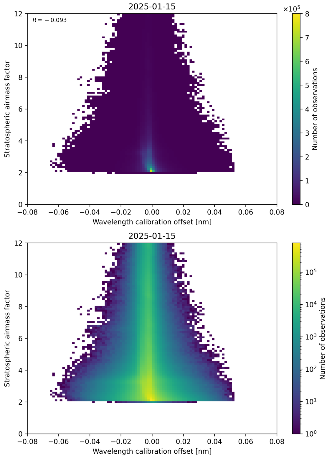
Figure 174: Scatter density plot of “Wavelength calibration offset” against “Stratospheric airmass factor” for 2025-01-14 to 2025-01-16.
