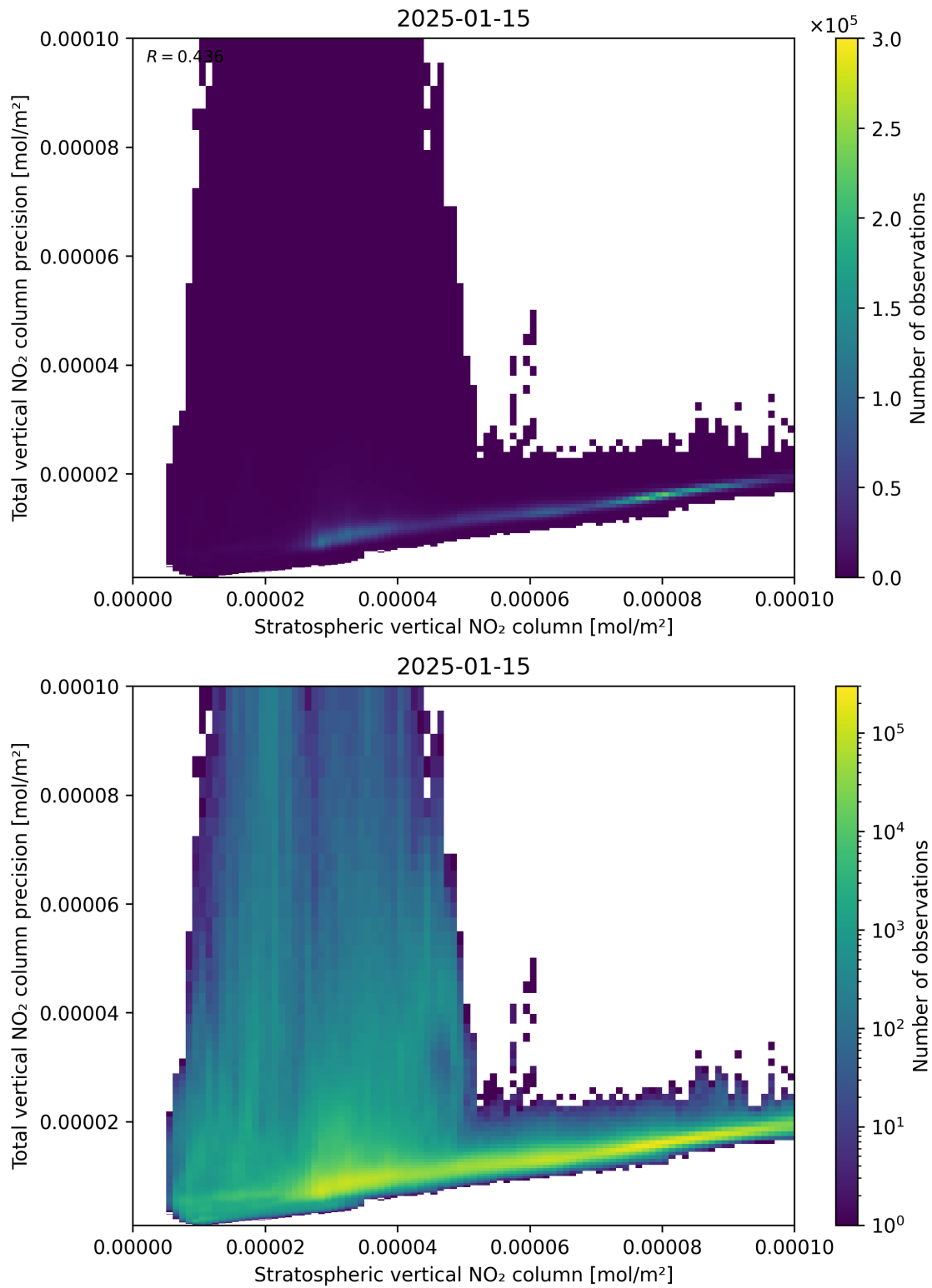
Figure 101: Scatter density plot of “Stratospheric vertical NO 2 column” against “Total vertical NO 2 column precision” for 2025-01-14 to 2025-01-16.
