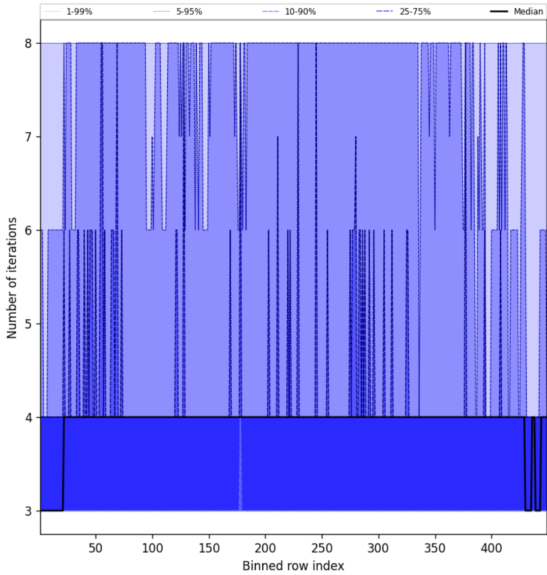
Figure 51: Along track statistics of “Number of iterations” for 2025-01-14 to 2025-01-16
