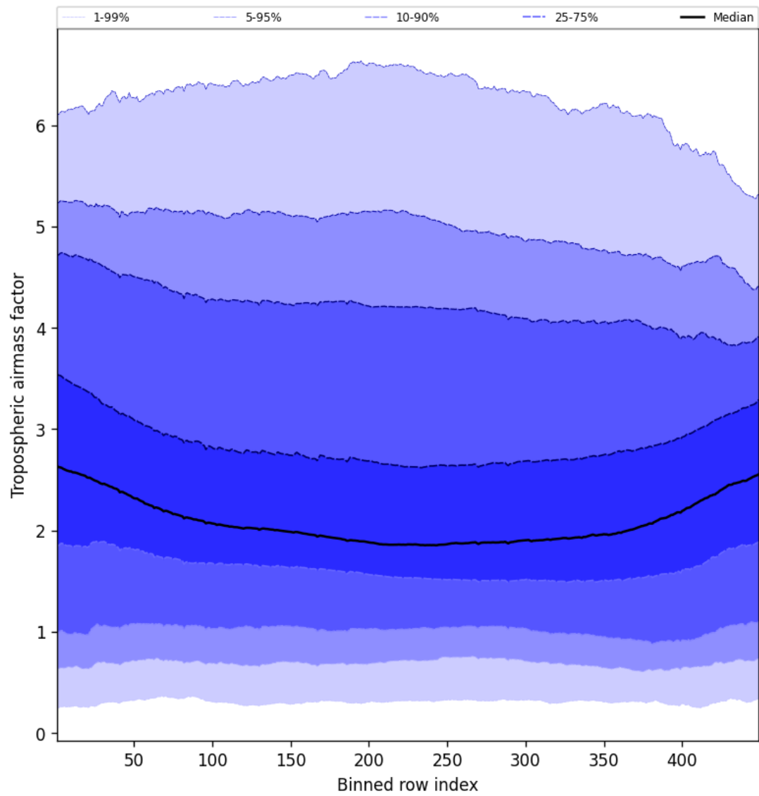
Figure 48: Along track statistics of “Tropospheric airmass factor” for 2025-01-14 to 2025-01-16
