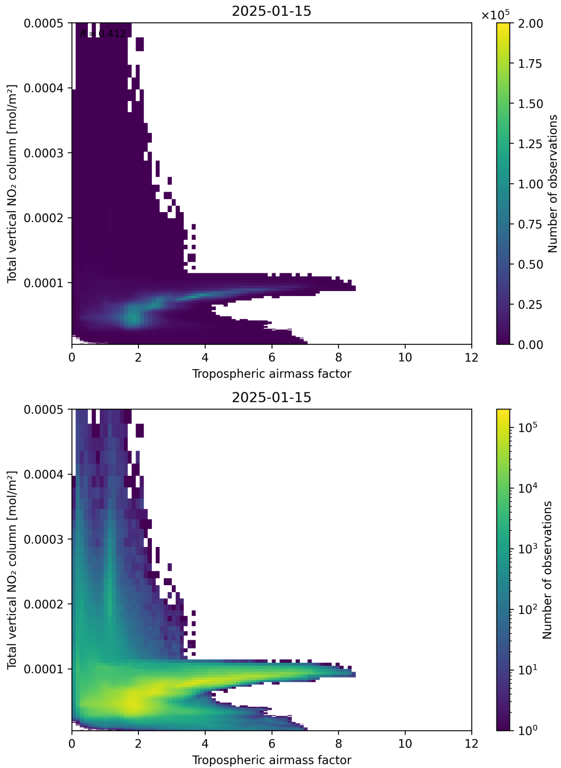
Figure 77: Scatter density plot of “Tropospheric airmass factor” against “Total vertical NO 2 column” for 2025-01-14 to 2025-01-16.
