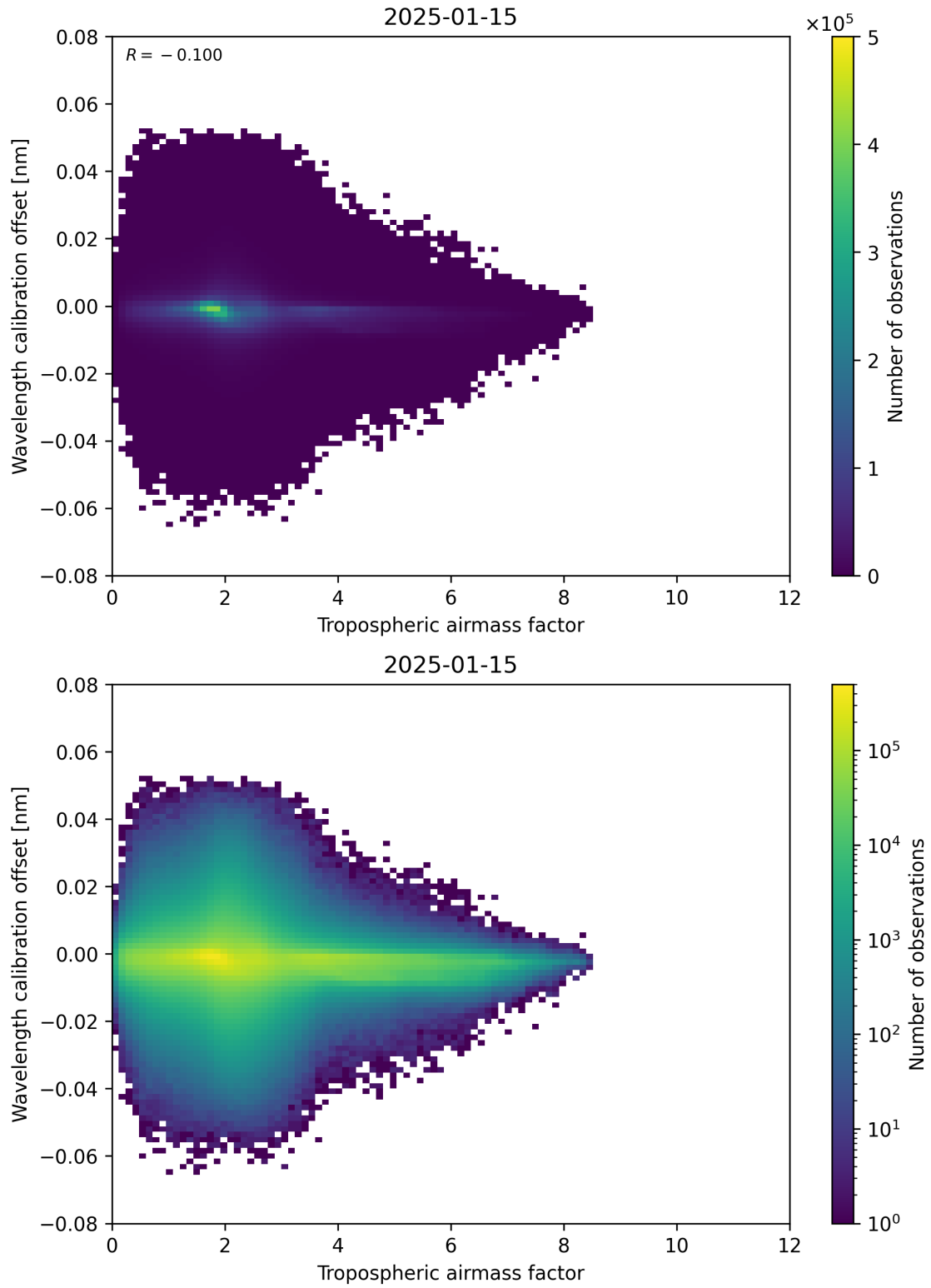
Figure 80: Scatter density plot of “Tropospheric airmass factor” against “Wavelength calibration offset” for 2025-01-14 to 2025-01-16.
