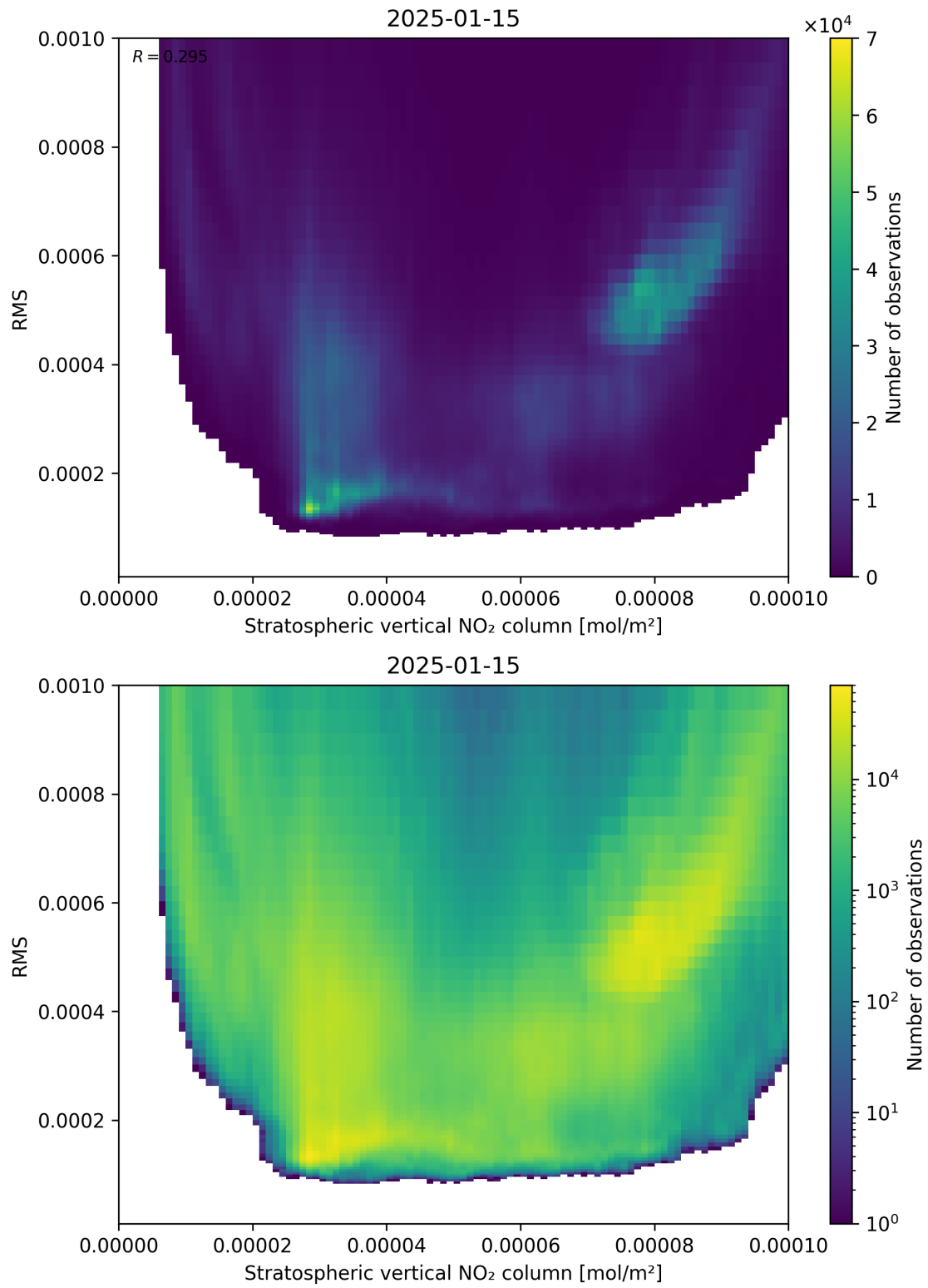
Figure 102: Scatter density plot of “Stratospheric vertical NO 2 column” against “RMS” for 2025-01-14 to 2025-01-16.
