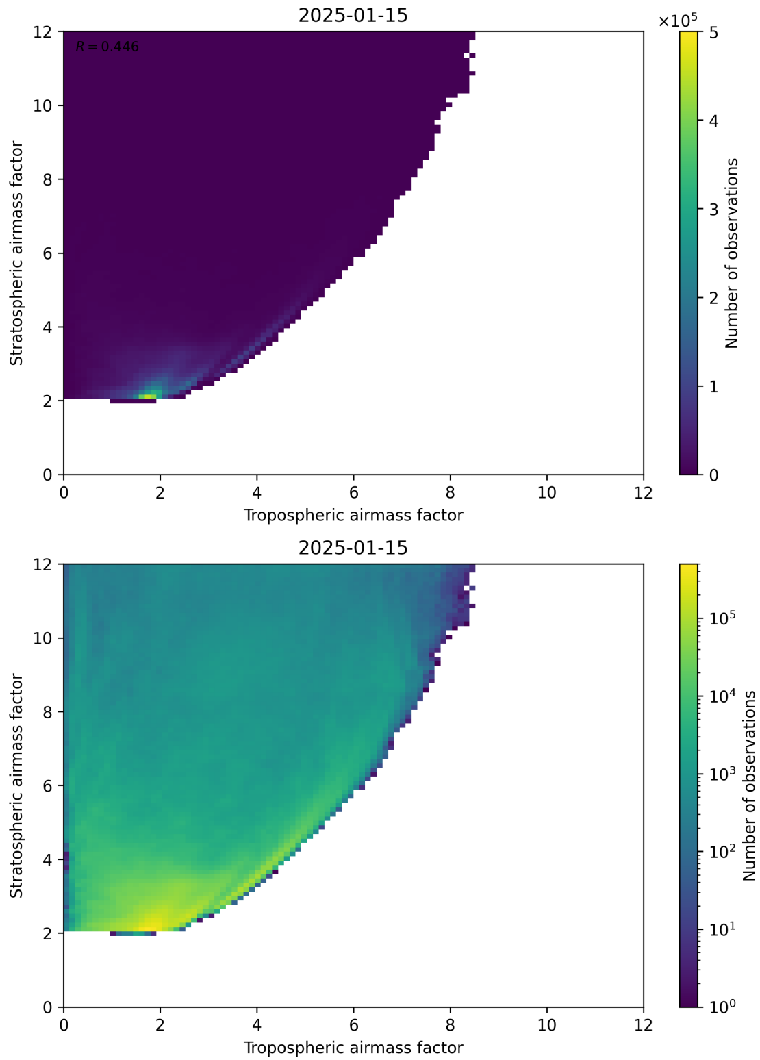
Figure 71: Scatter density plot of “Tropospheric airmass factor” against “Stratospheric airmass factor” for 2025-01-14 to 2025-01-16.
