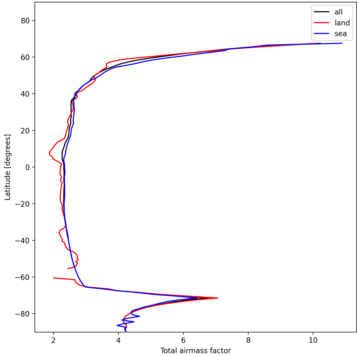
Figure 15: Zonal average of “Total airmass factor” for 2025-01-14 to 2025-01-16.
