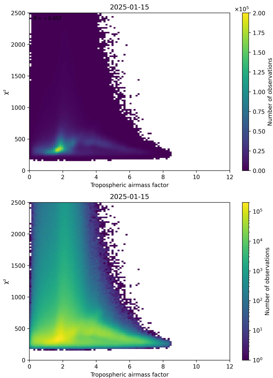
Figure 73: Scatter density plot of “Tropospheric airmass factor” against “ \chi^2 ” for 2025-01-14 to 2025-01-16.
