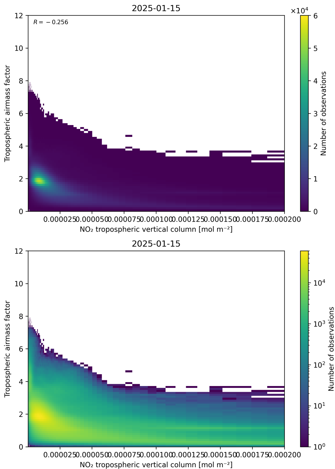
Figure 123: Scatter density plot of “NO 2 tropospheric vertical column” against “Tropospheric air mass factor” for 2025-01-14 to 2025-01-16.
