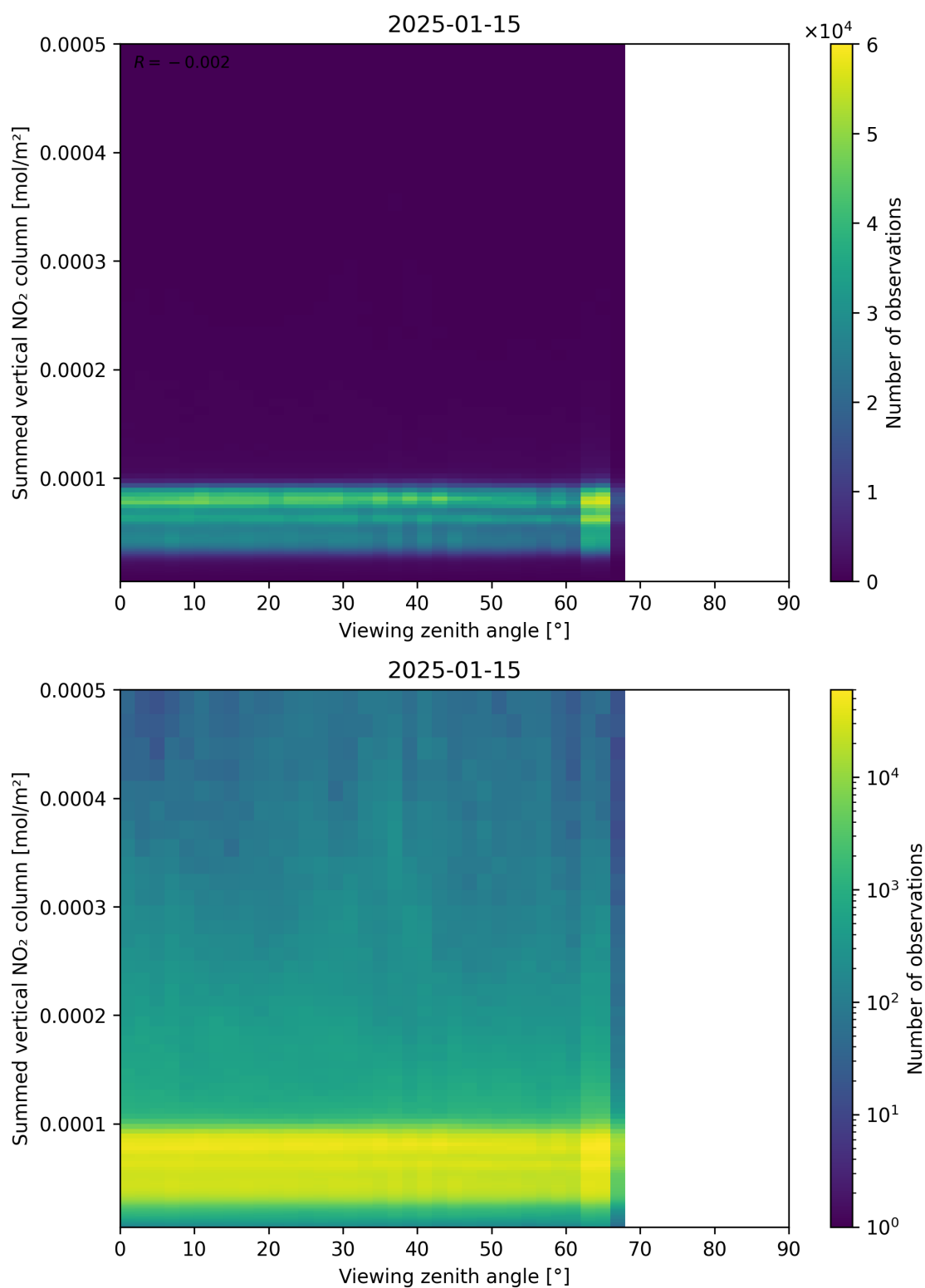
Figure 165: Scatter density plot of “Viewing zenith angle” against “Summed vertical NO 2 column” for 2025-01-14 to 2025-01-16.
