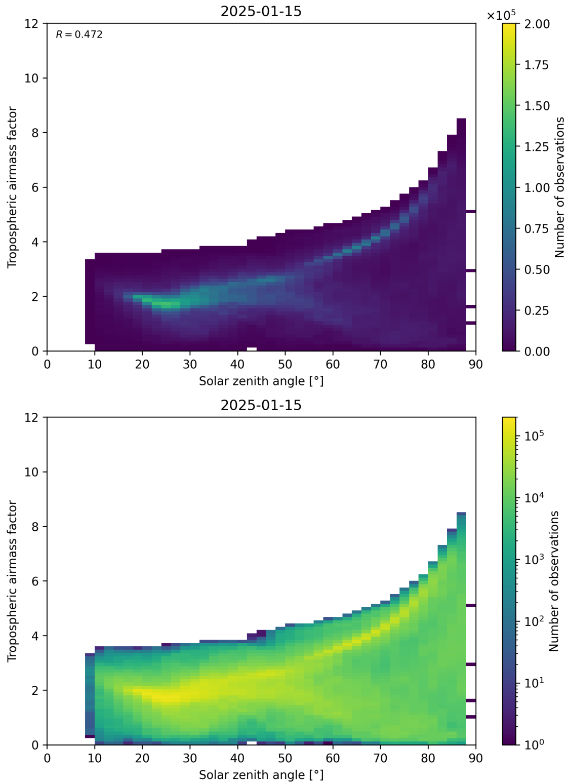
Figure 147: Scatter density plot of “Solar zenith angle” against “Tropospheric airmass factor” for 2025-01-14 to 2025-01-16.
