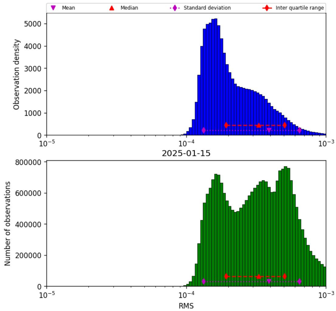
Figure 43: Histogram of “RMS” for 2025-01-14 to 2025-01-16
