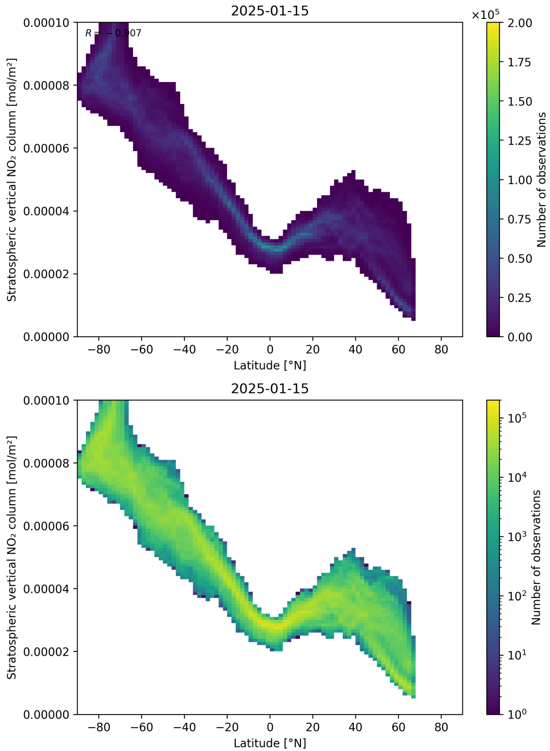
Figure 87: Scatter density plot of “Latitude” against “Stratospheric vertical NO 2 column” for 2025-01-14 to 2025-01-16.
