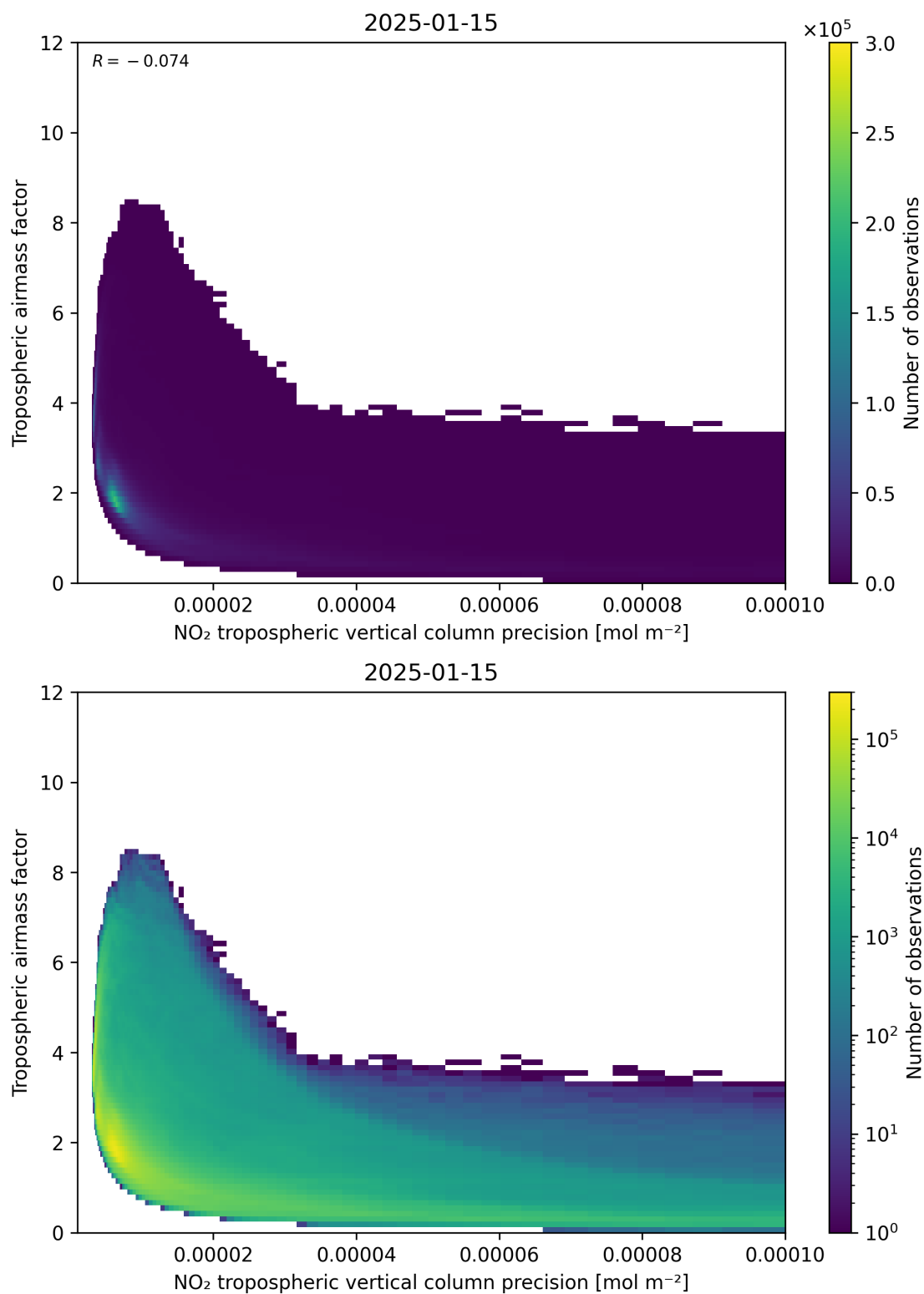
Figure 133: Scatter density plot of “NO 2 tropospheric vertical column precision” against “Tropospheric air mass factor” for 2025-01-14 to 2025-01-16.
