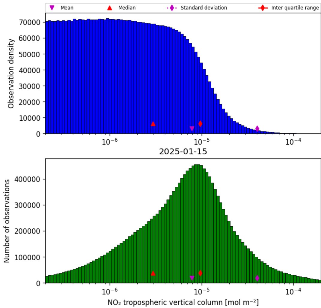
Figure 29: Histogram of “NO 2 tropospheric vertical column” for 2025-01-14 to 2025-01-16
