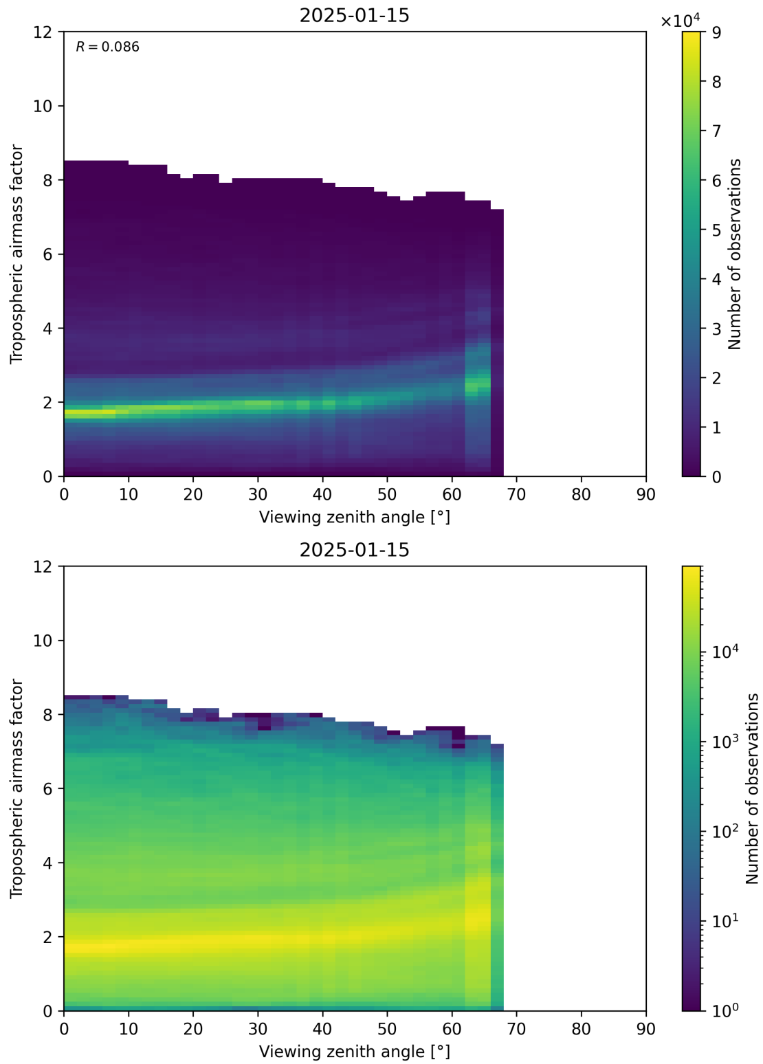
Figure 161: Scatter density plot of “Viewing zenith angle” against “Tropospheric airmass factor” for 2025-01-14 to 2025-01-16.
