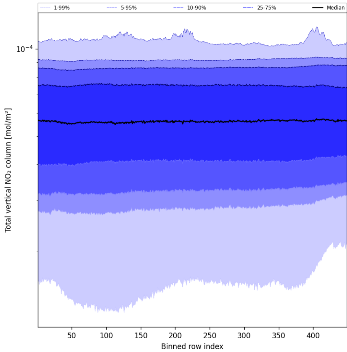
Figure 55: Along track statistics of “Total vertical NO 2 column” for 2025-01-14 to 2025-01-16
