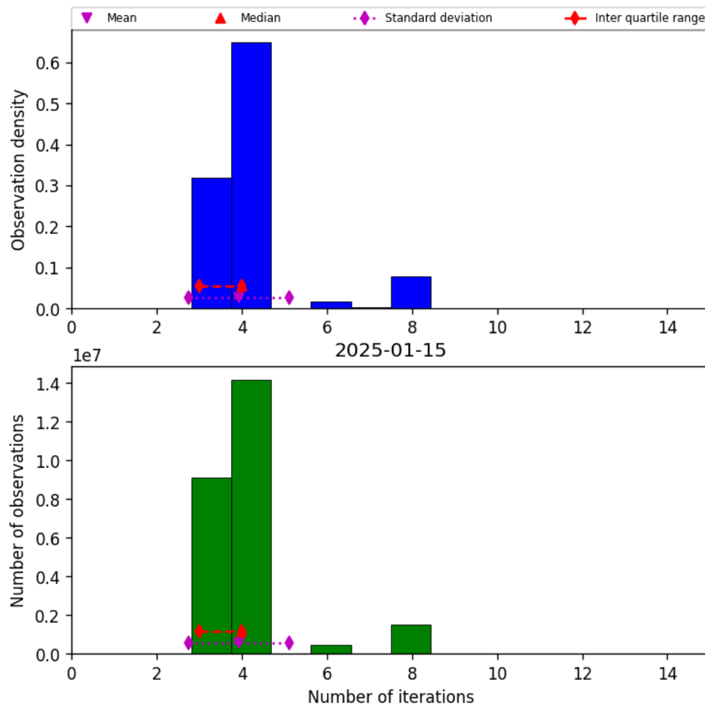
Figure 34: Histogram of “Number of iterations” for 2025-01-14 to 2025-01-16
