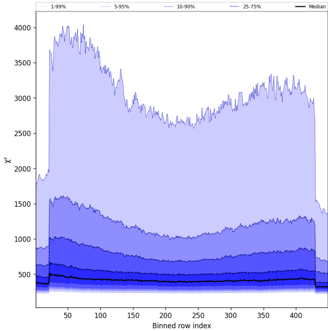
Figure 59: Along track statistics of “ \chi^2 ” for 2025-01-14 to 2025-01-16
