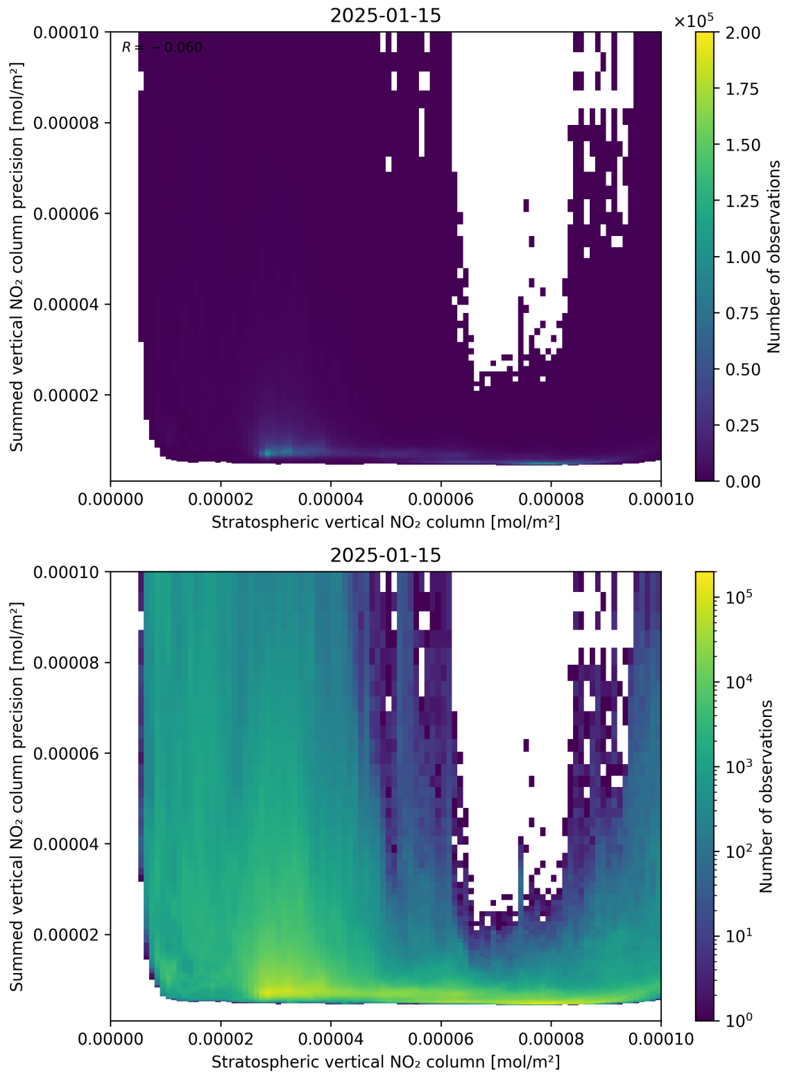
Figure 99: Scatter density plot of “Stratospheric vertical NO 2 column” against “Summed vertical NO 2 column precision” for 2025-01-14 to 2025-01-16.
