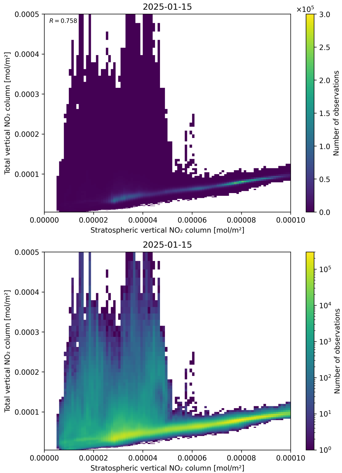
Figure 100: Scatter density plot of “Stratospheric vertical NO 2 column” against “Total vertical NO 2 column” for 2025-01-14 to 2025-01-16.
