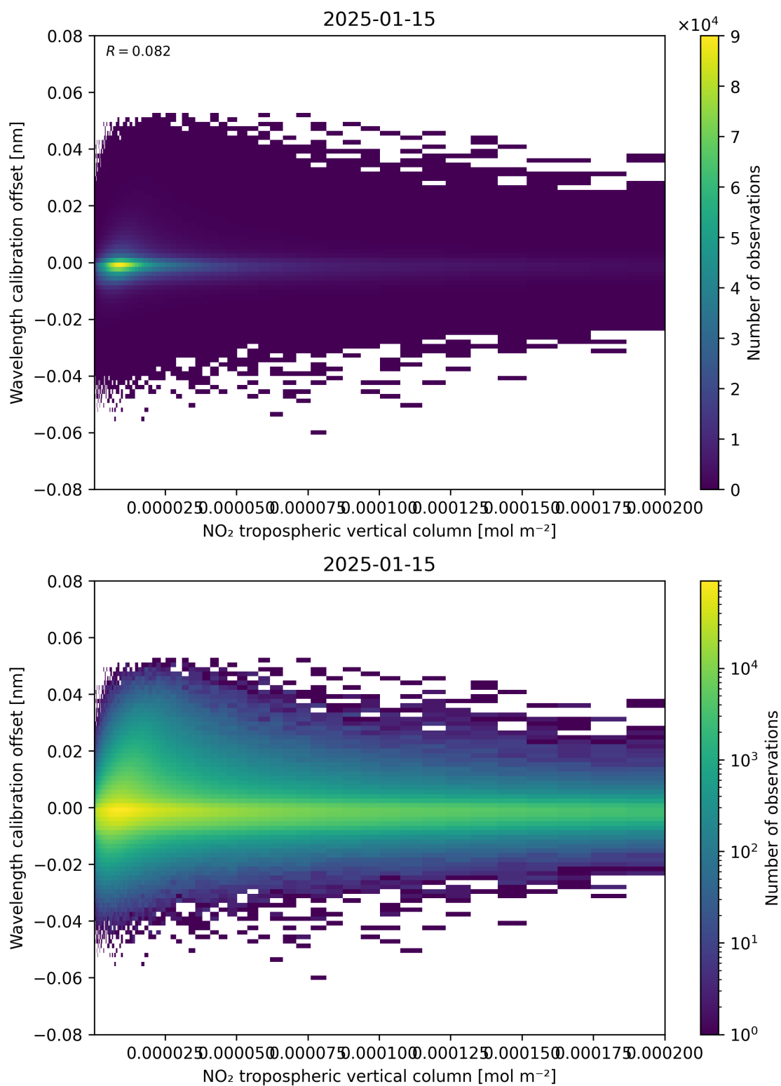
Figure 143: Scatter density plot of “NO 2 tropospheric vertical column” against “Wavelength calibration offset” for 2025-01-14 to 2025-01-16.
