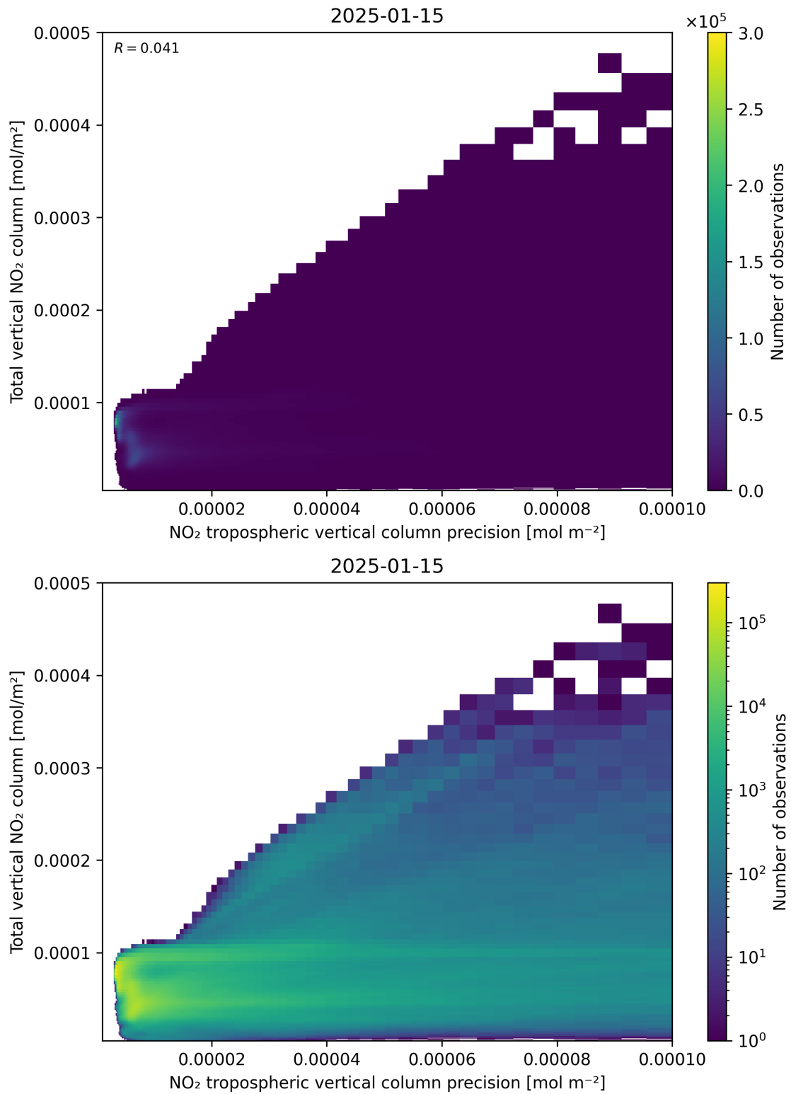
Figure 138: Scatter density plot of “NO 2 tropospheric vertical column precision” against “Total vertical NO 2 column” for 2025-01-14 to 2025-01-16.
