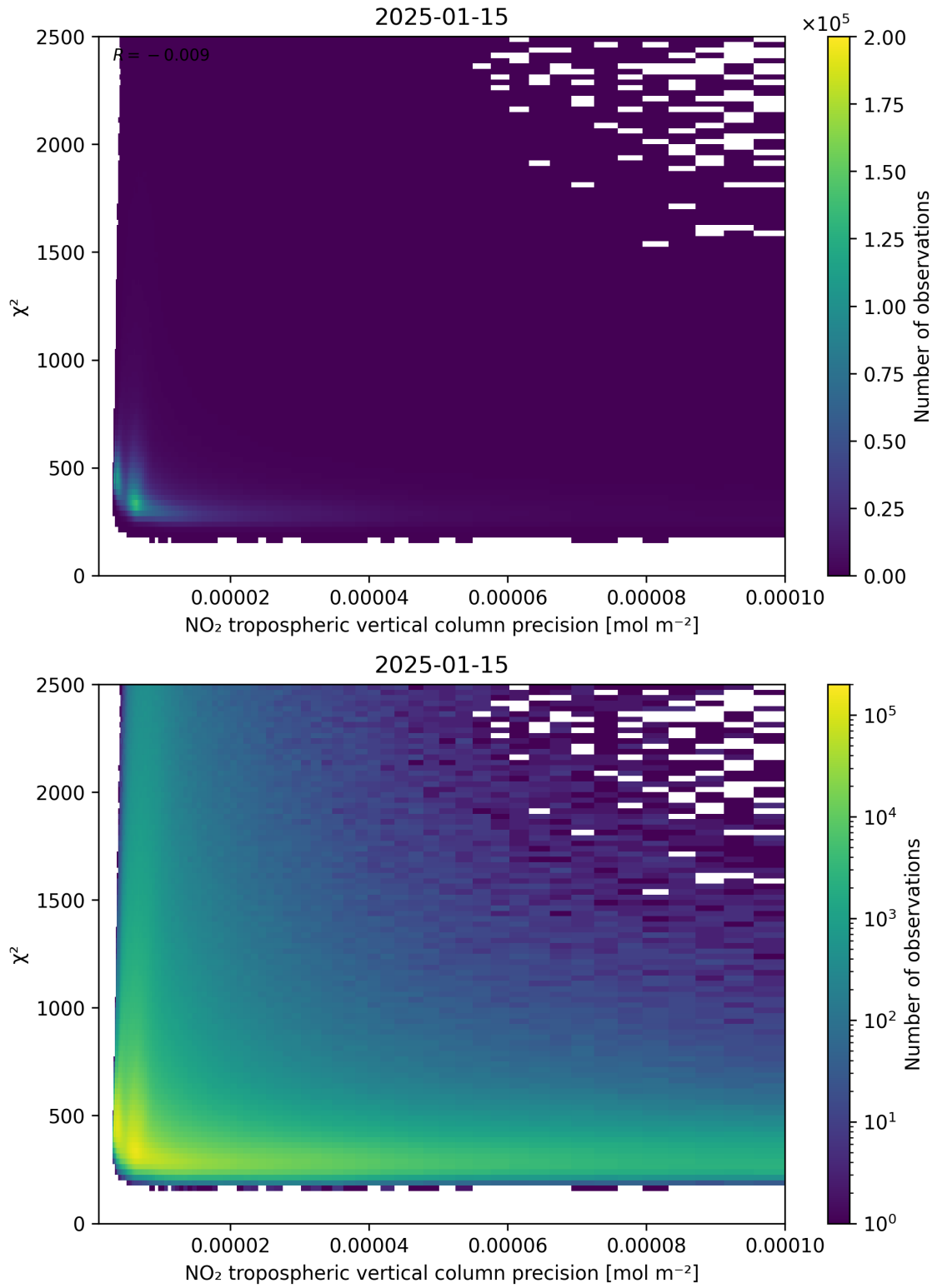
Figure 134: Scatter density plot of “NO 2 tropospheric vertical column precision” against “ \chi^2 ” for 2025-01-14 to 2025-01-16.
