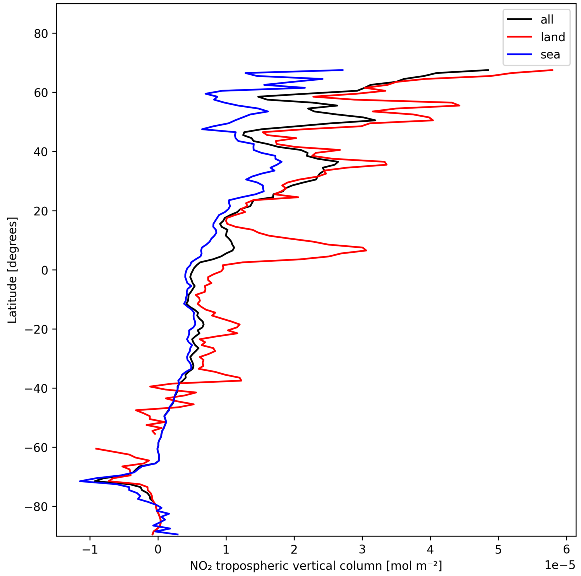
Figure 12: Zonal average of “NO 2 tropospheric vertical column” for 2025-01-14 to 2025-01-16.
