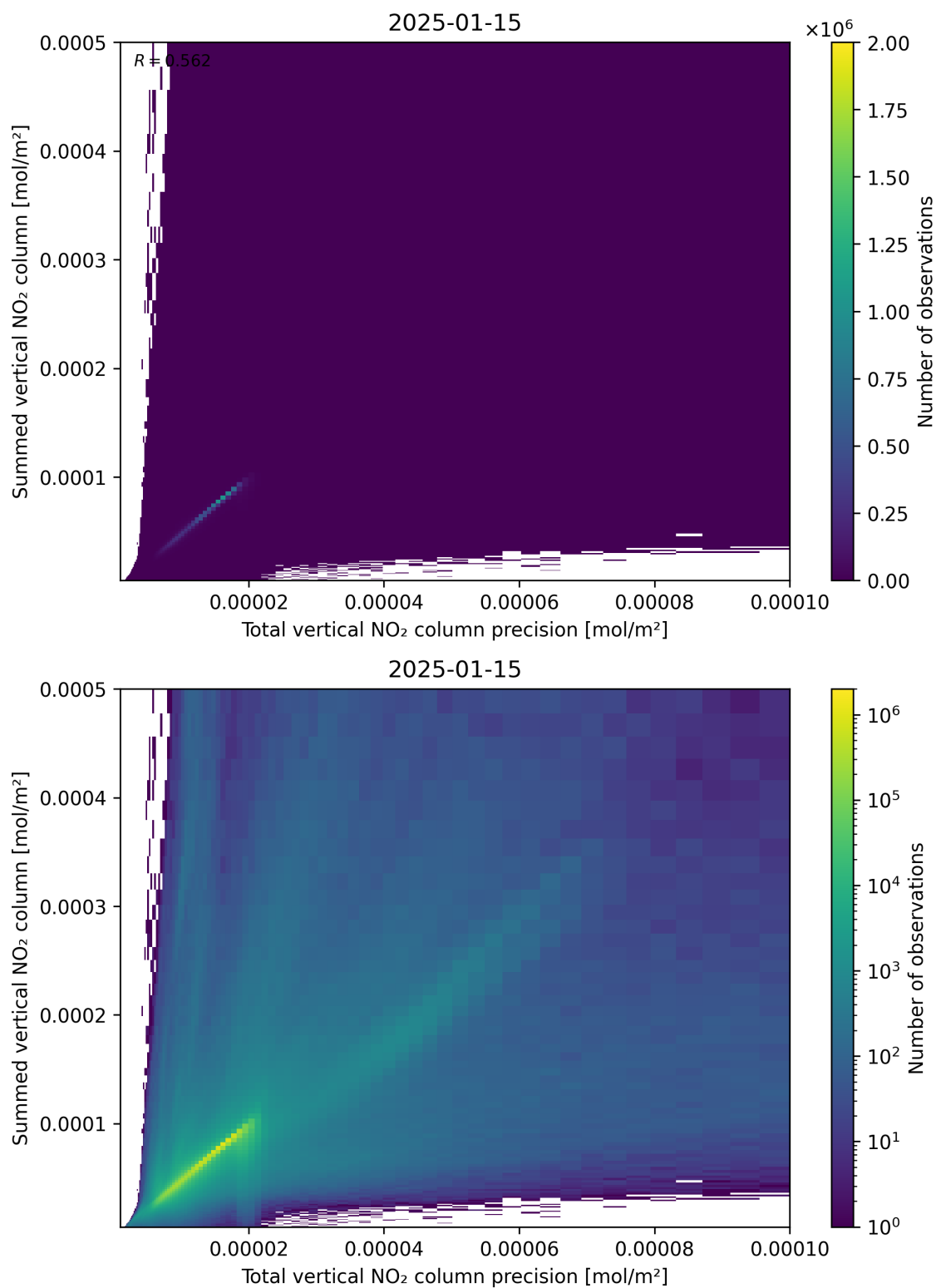
Figure 117: Scatter density plot of “Total vertical NO 2 column precision” against “Summed vertical NO 2 column” for 2025-01-14 to 2025-01-16.
