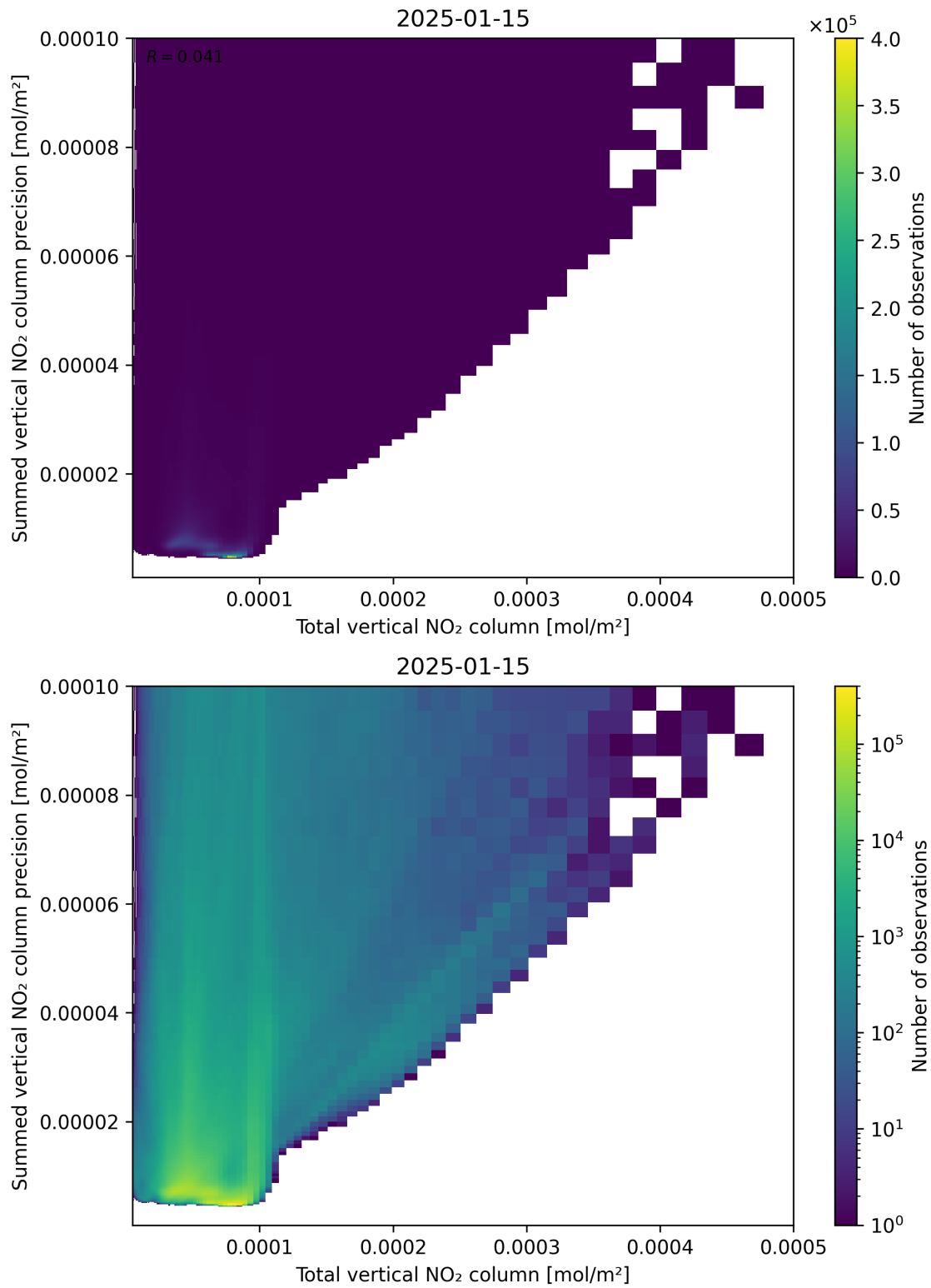
Figure 113: Scatter density plot of “Total vertical NO 2 column” against “Summed vertical NO 2 column precision” for 2025-01-14 to 2025-01-16.
