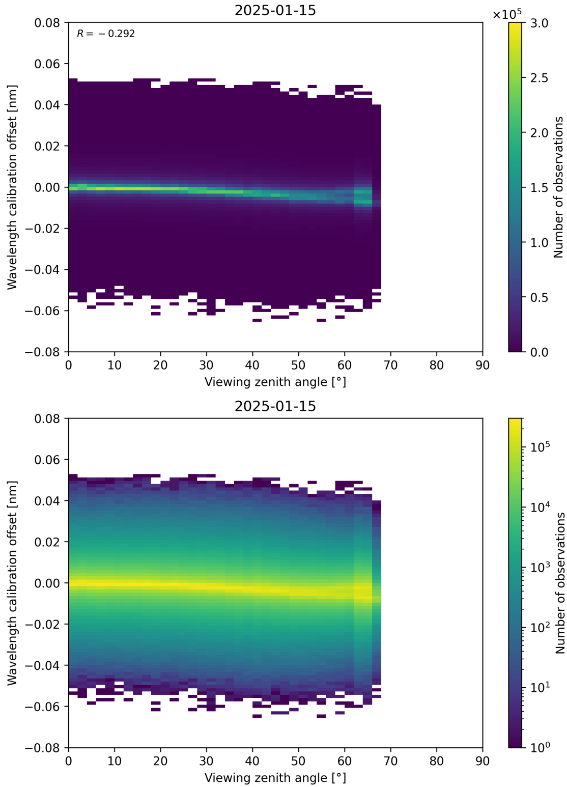
Figure 173: Scatter density plot of “Viewing zenith angle” against “Wavelength calibration offset” for 2025-01-14 to 2025-01-16.
