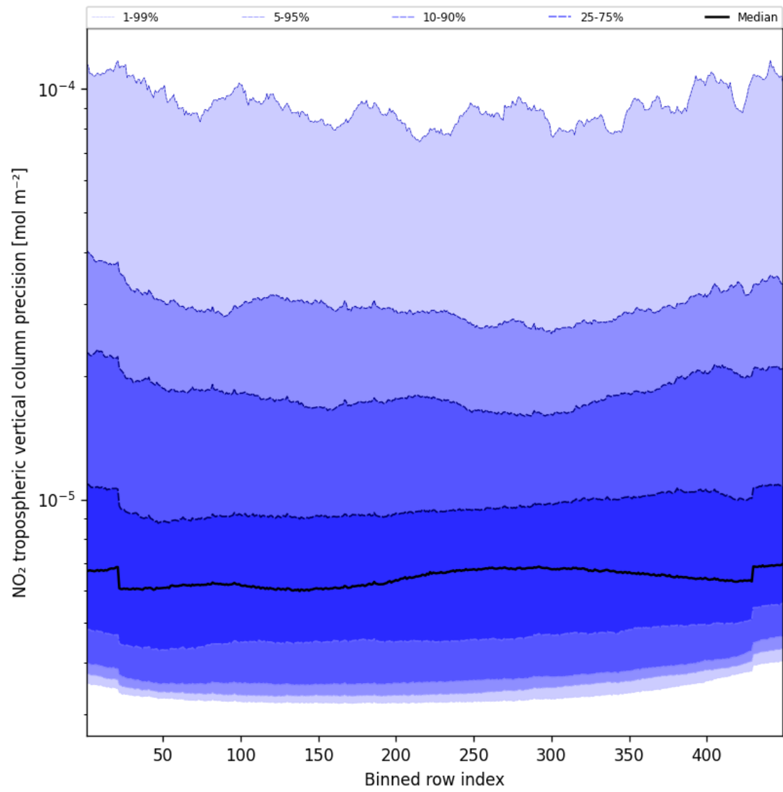
Figure 47: Along track statistics of “NO 2 tropospheric vertical column precision” for 2025-01-14 to 2025-01-16
