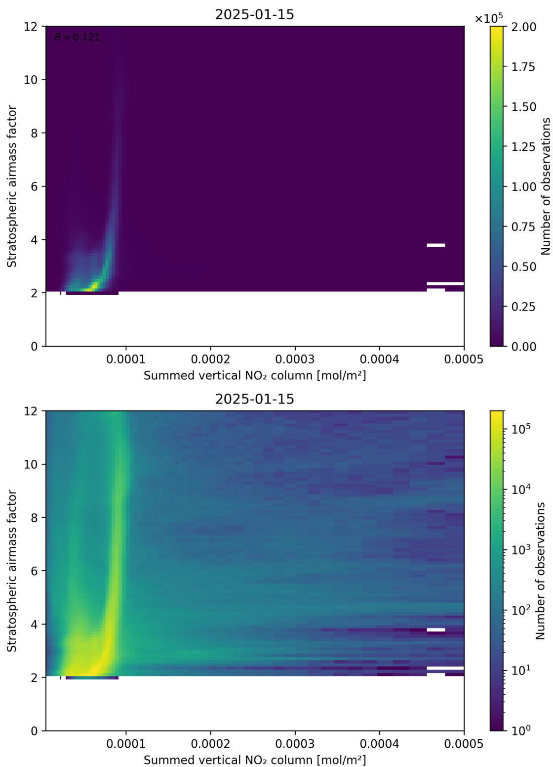
Figure 103: Scatter density plot of “Summed vertical NO 2 column” against “Stratospheric airmass factor” for 2025-01-14 to 2025-01-16.
