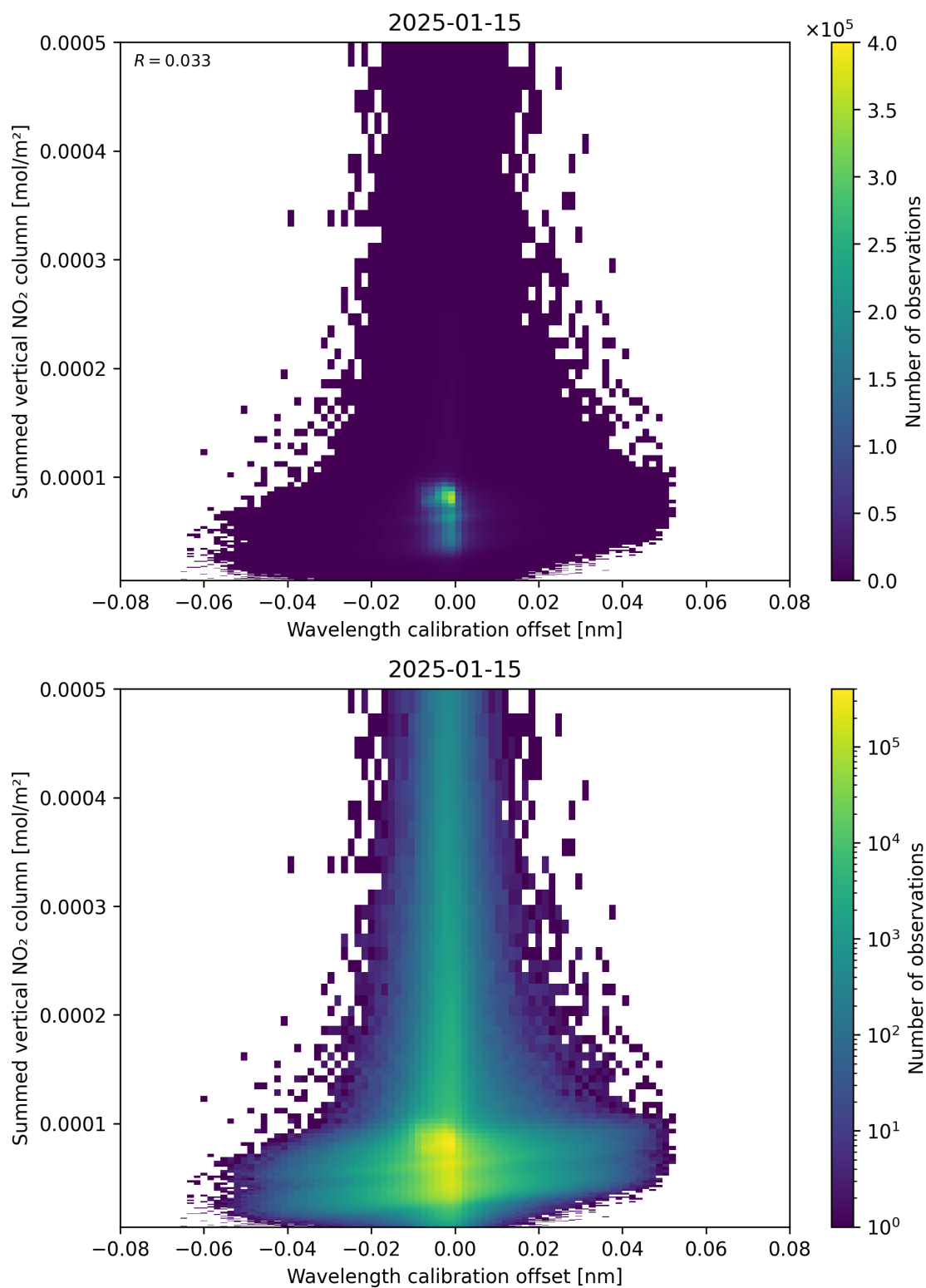
Figure 177: Scatter density plot of “Wavelength calibration offset” against “Summed vertical NO 2 column” for 2025-01-14 to 2025-01-16.
