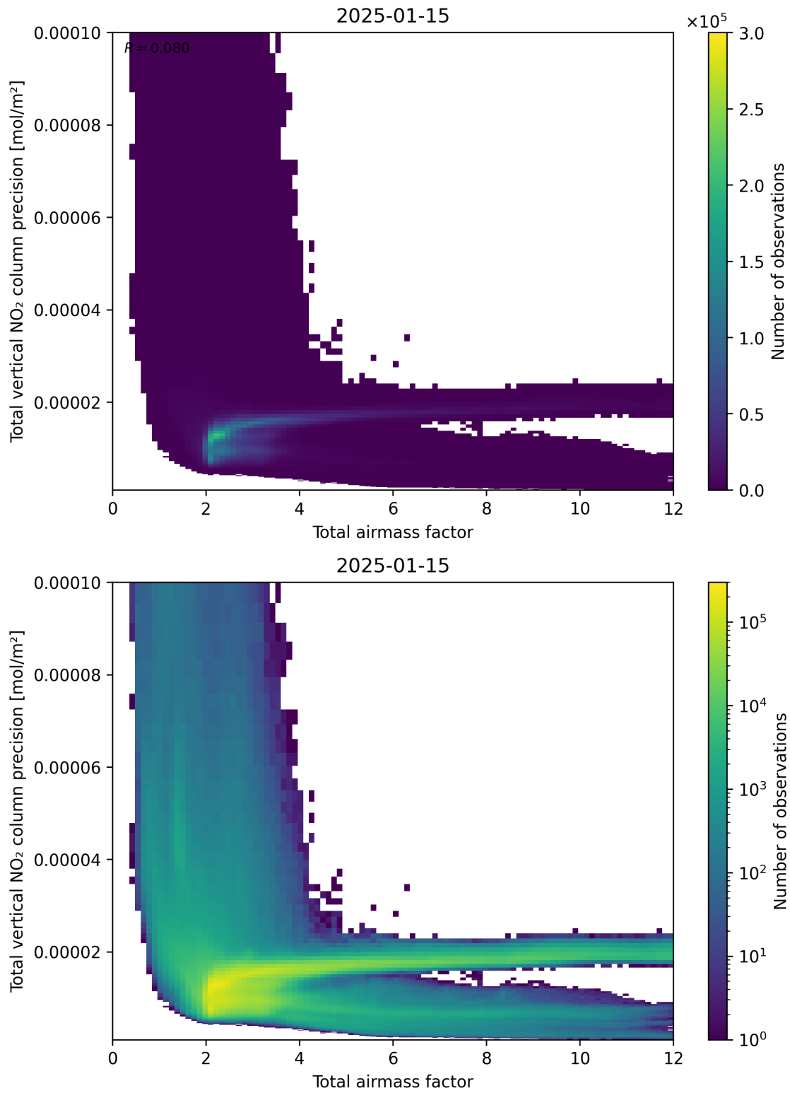
Figure 68: Scatter density plot of “Total airmass factor” against “Total vertical NO 2 column precision” for 2025-01-14 to 2025-01-16.
