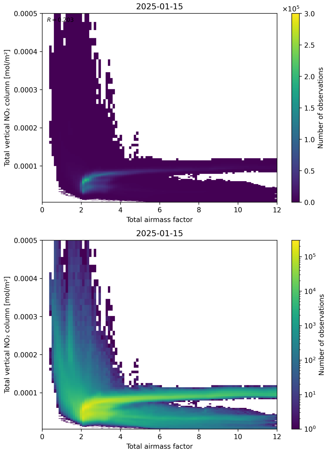
Figure 67: Scatter density plot of “Total airmass factor” against “Total vertical NO 2 column” for 2025-01-14 to 2025-01-16.
