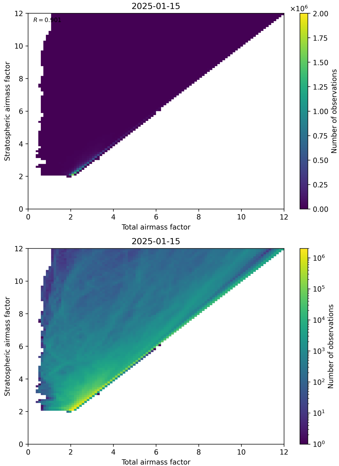
Figure 62: Scatter density plot of “Total air mass factor” against “Stratospheric air mass factor” for 2025-01-14 to 2025-01-16.
