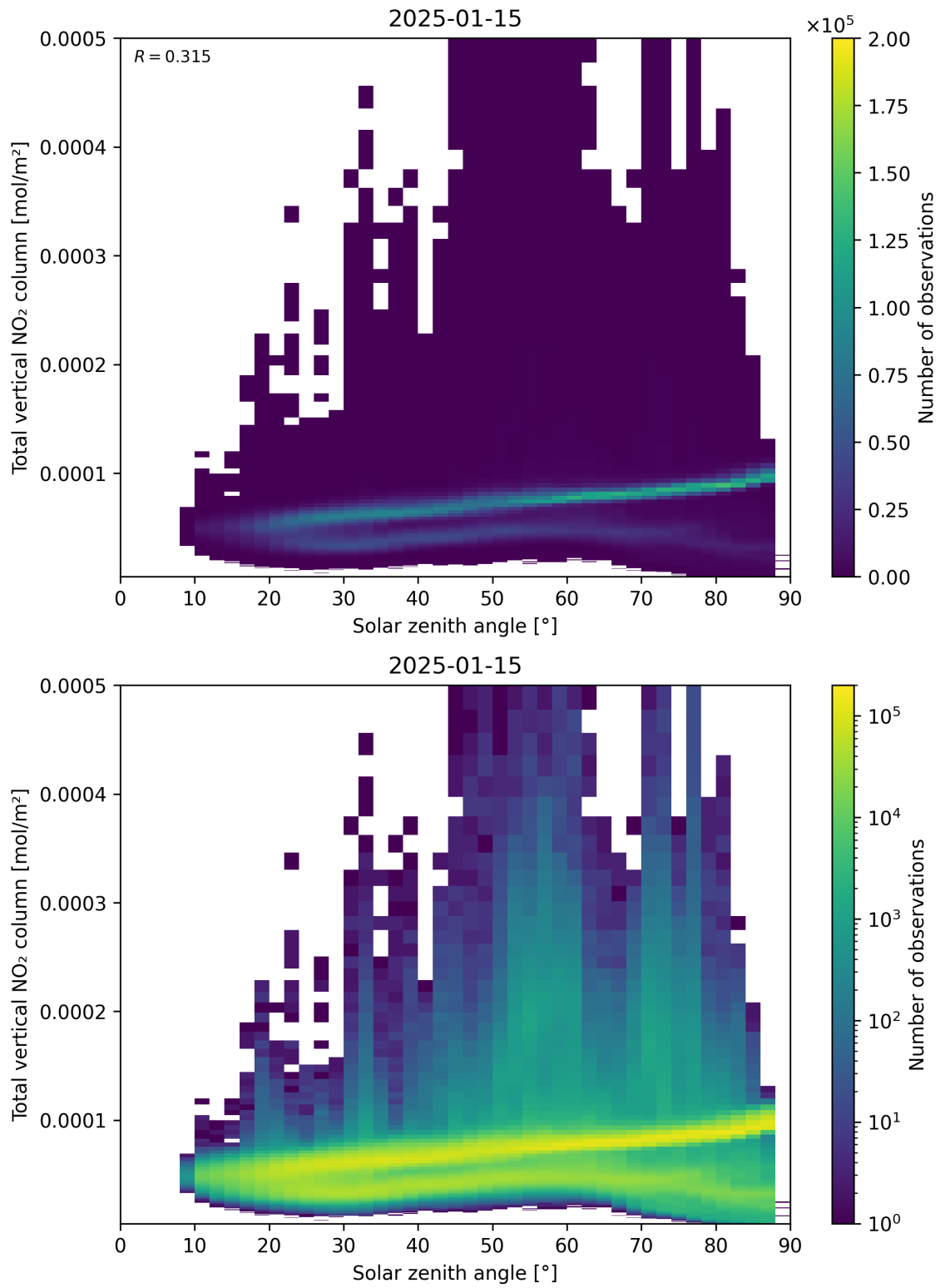
Figure 153: Scatter density plot of “Solar zenith angle” against “Total vertical NO 2 column” for 2025-01-14 to 2025-01-16.
