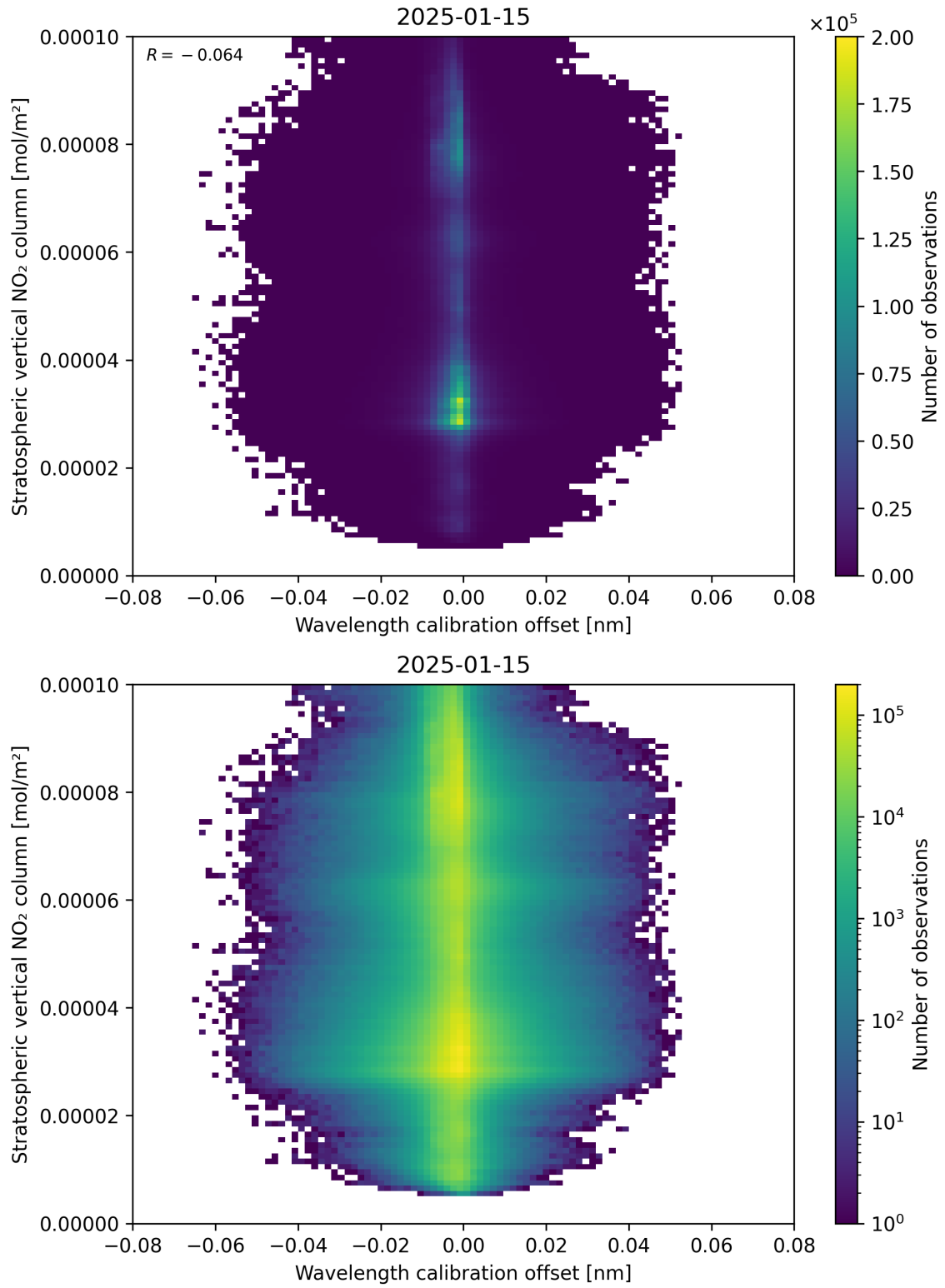
Figure 176: Scatter density plot of “Wavelength calibration offset” against “Stratospheric vertical NO 2 column” for 2025-01-14 to 2025-01-16.
