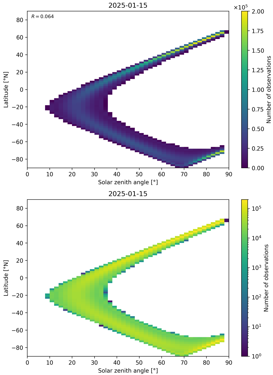
Figure 149: Scatter density plot of “Solar zenith angle” against “Latitude” for 2025-01-14 to 2025-01-16.
