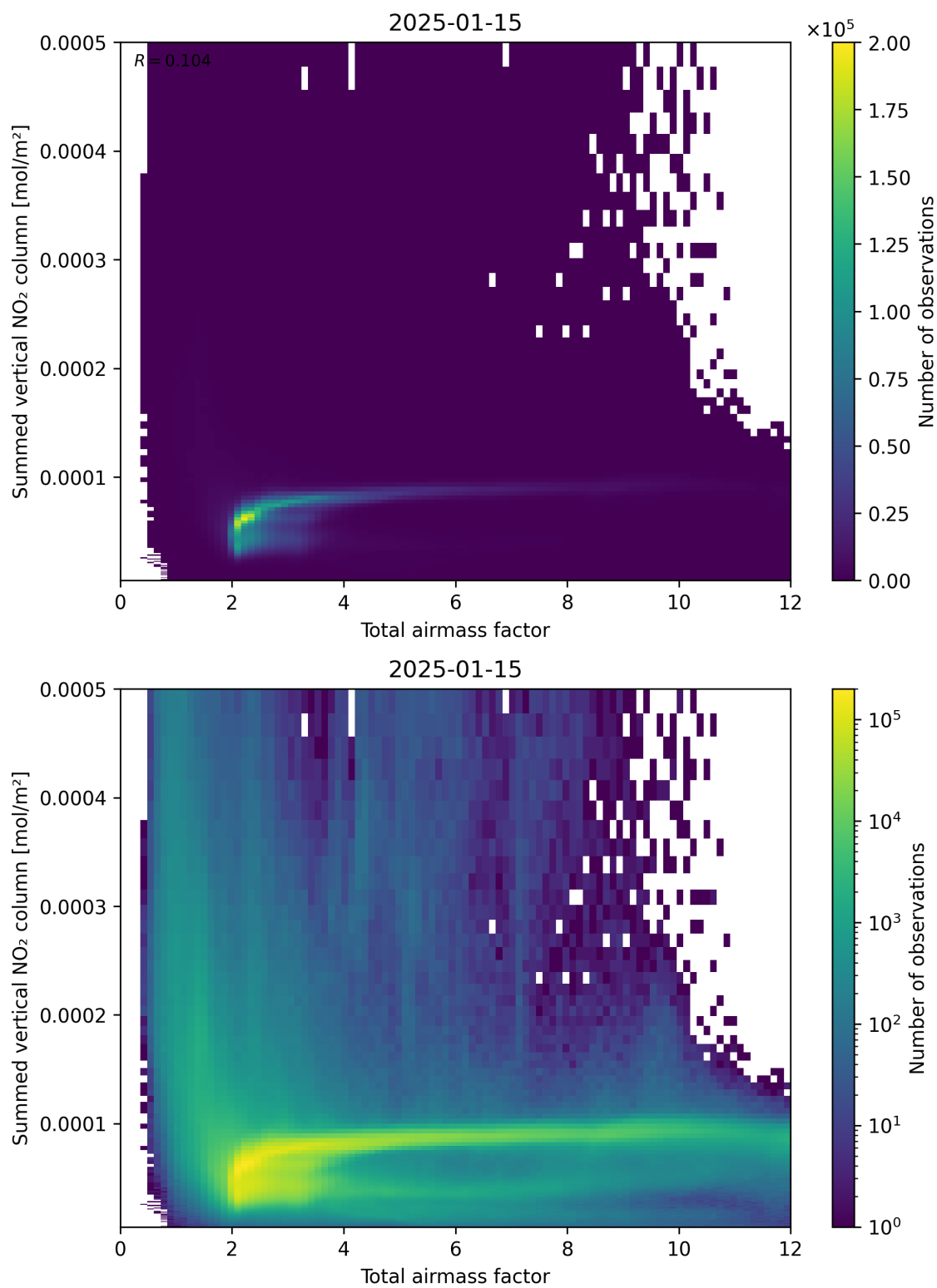
Figure 65: Scatter density plot of “Total airmass factor” against “Summed vertical NO 2 column” for 2025-01-14 to 2025-01-16.
