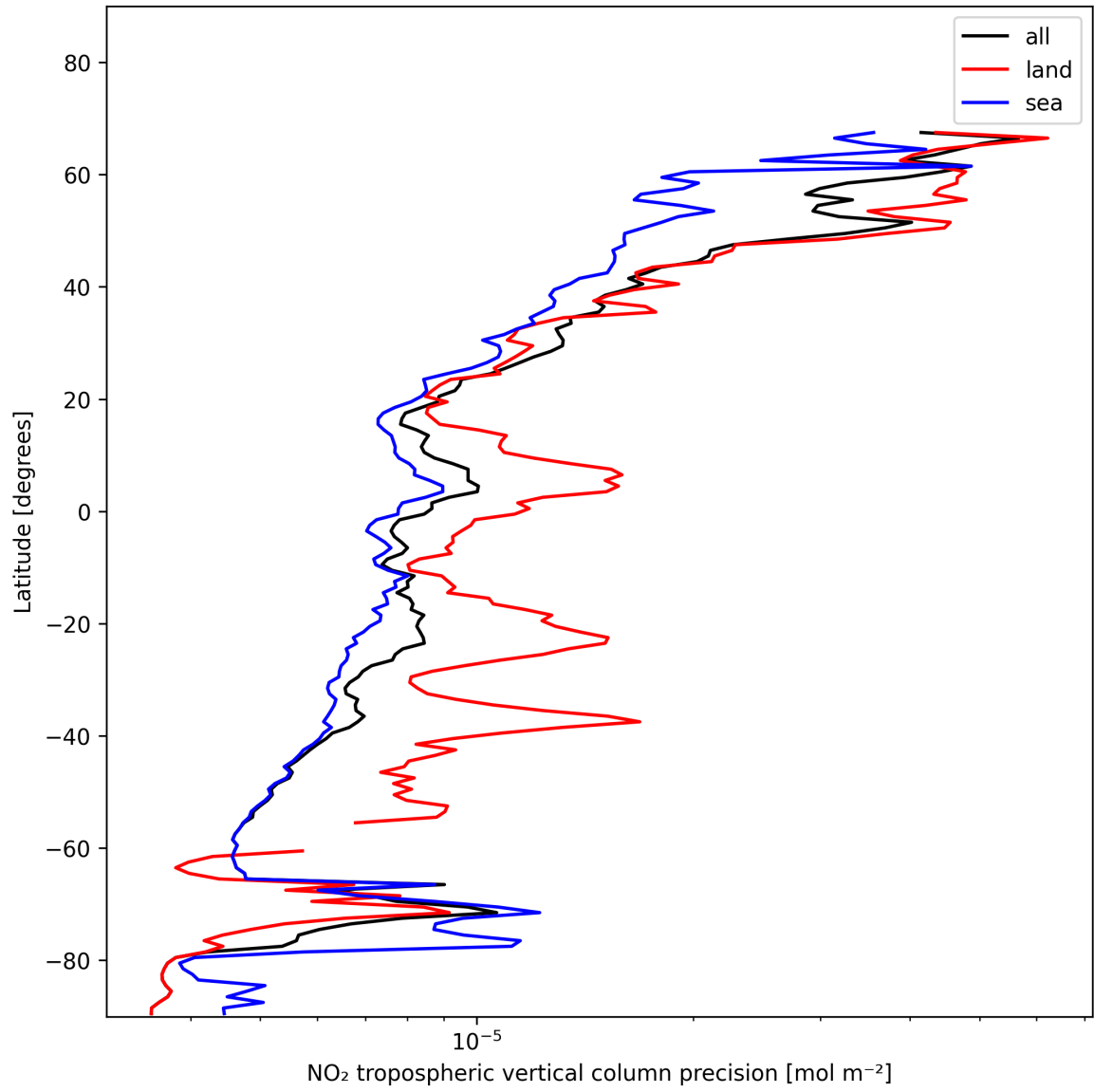
Figure 13: Zonal average of “NO 2 tropospheric vertical column precision” for 2025-01-14 to 2025-01-16.
