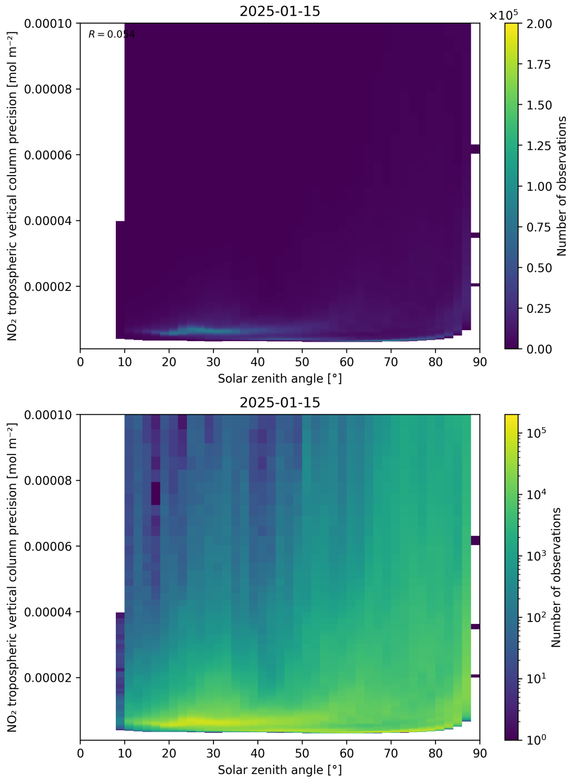
Figure 156: Scatter density plot of “Solar zenith angle” against “NO 2 tropospheric vertical column precision” for 2025-01-14 to 2025-01-16.
