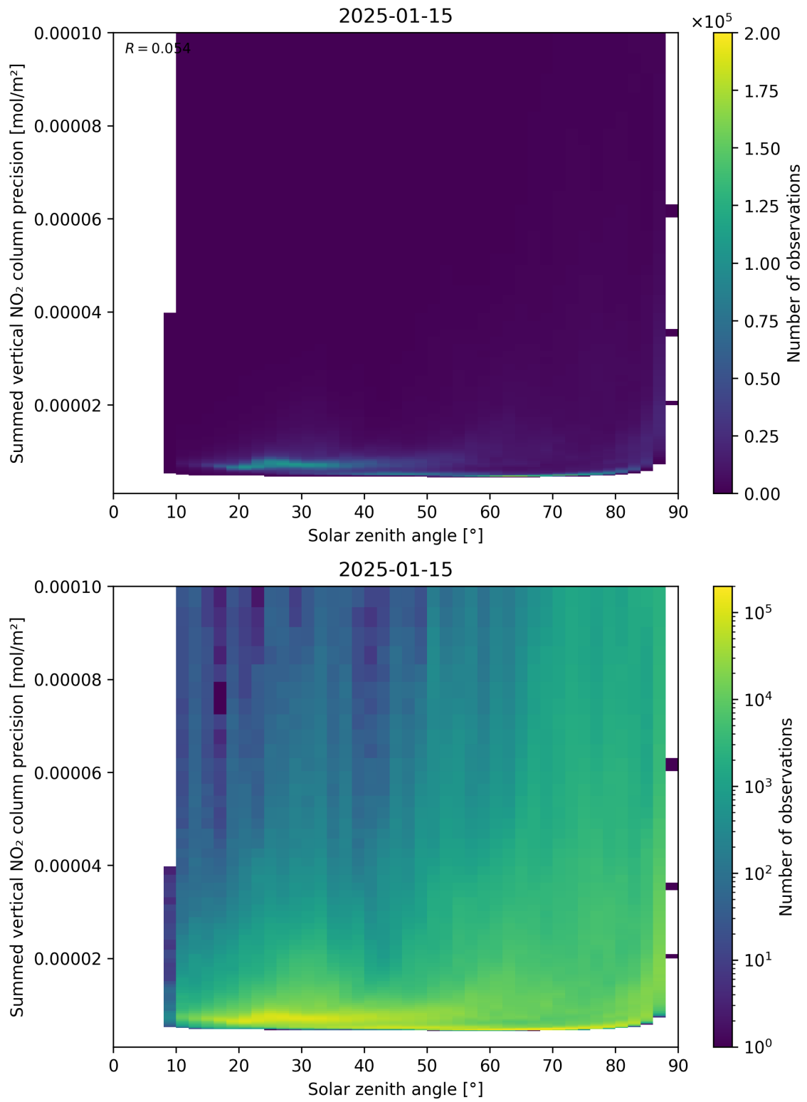
Figure 152: Scatter density plot of “Solar zenith angle” against “Summed vertical NO 2 column precision” for 2025-01-14 to 2025-01-16.
