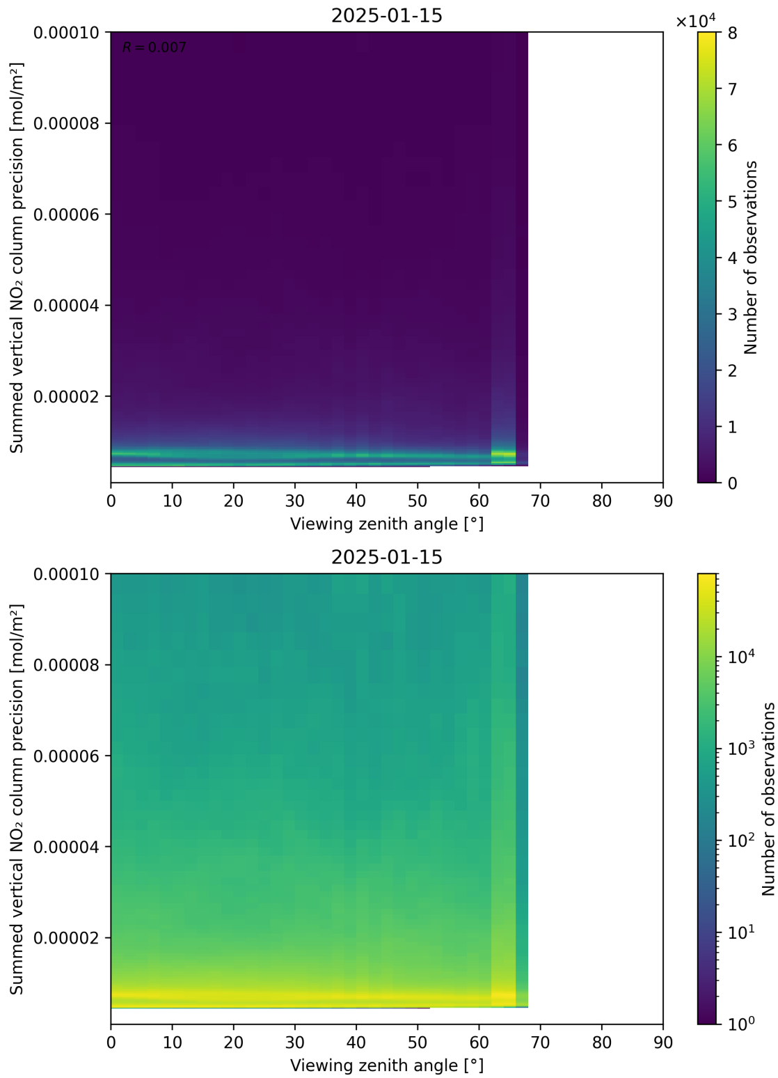
Figure 166: Scatter density plot of “Viewing zenith angle” against “Summed vertical NO 2 column precision” for 2025-01-14 to 2025-01-16.
