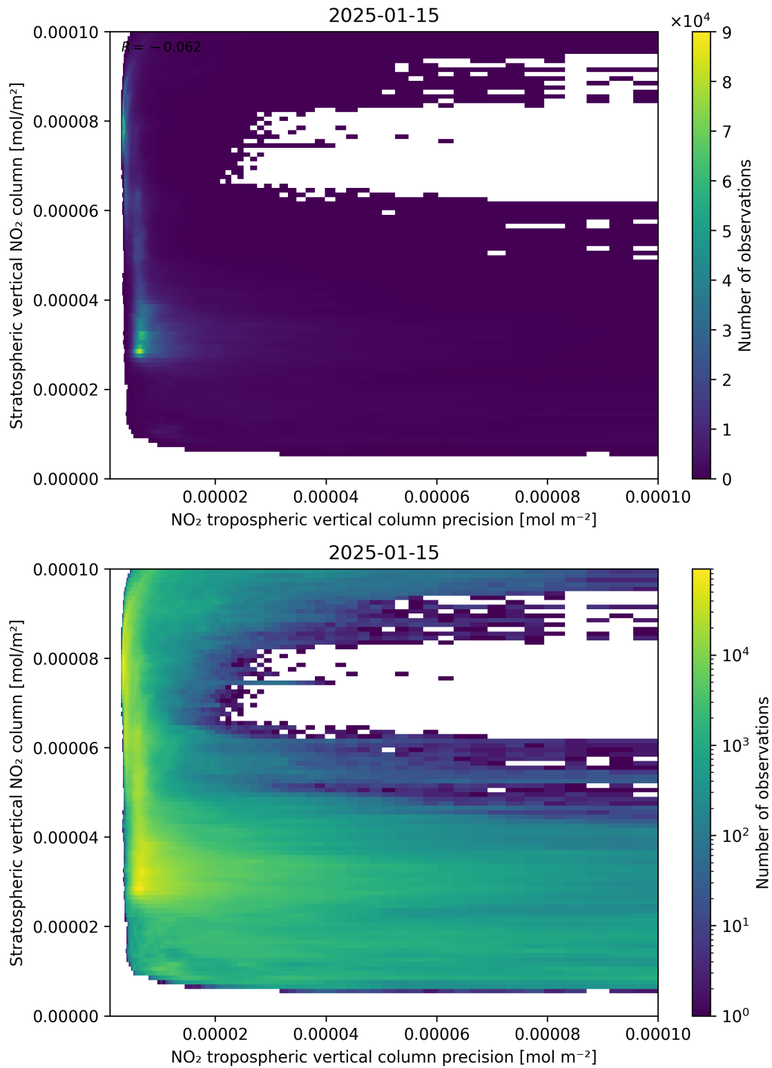
Figure 135: Scatter density plot of “NO 2 tropospheric vertical column precision” against “Stratospheric vertical NO 2 column” for 2025-01-14 to 2025-01-16.
