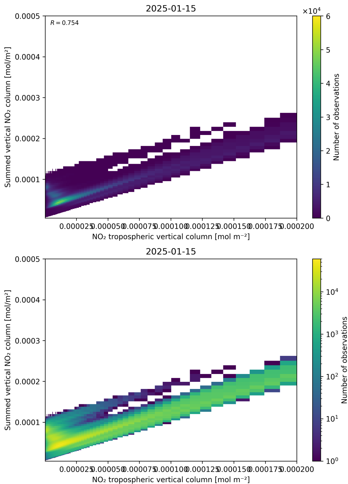
Figure 126: Scatter density plot of “NO 2 tropospheric vertical column” against “Summed vertical NO 2 column” for 2025-01-14 to 2025-01-16.
