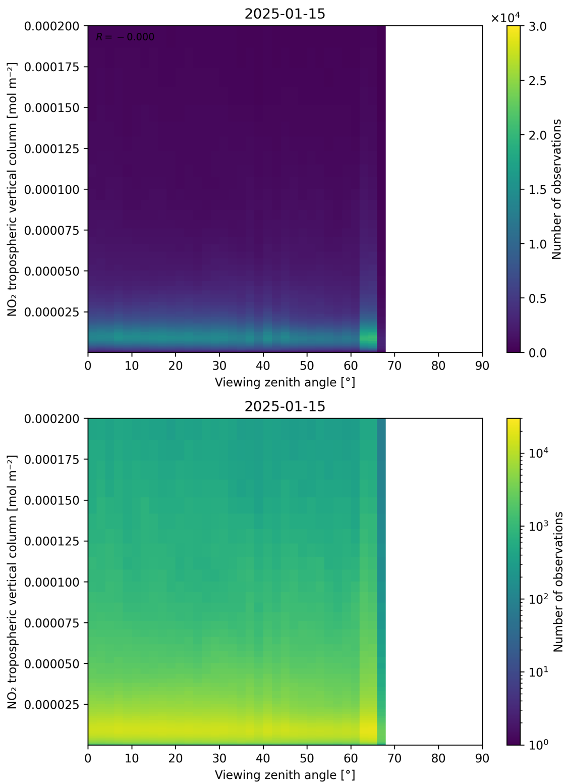
Figure 169: Scatter density plot of “Viewing zenith angle” against “NO 2 tropospheric vertical column” for 2025-01-14 to 2025-01-16.
