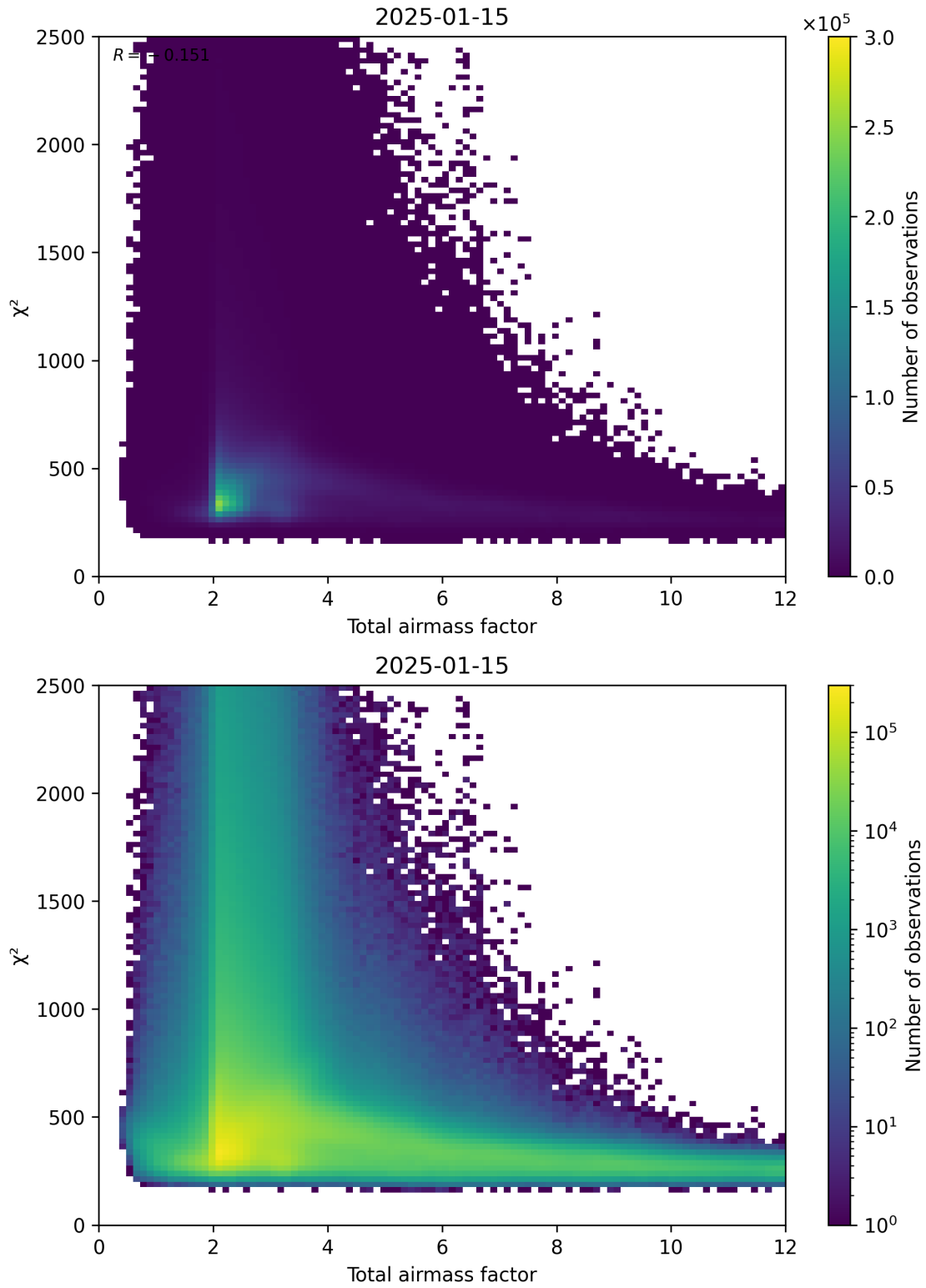
Figure 63: Scatter density plot of “Total airmass factor” against “ \chi^2 ” for 2025-01-14 to 2025-01-16.
