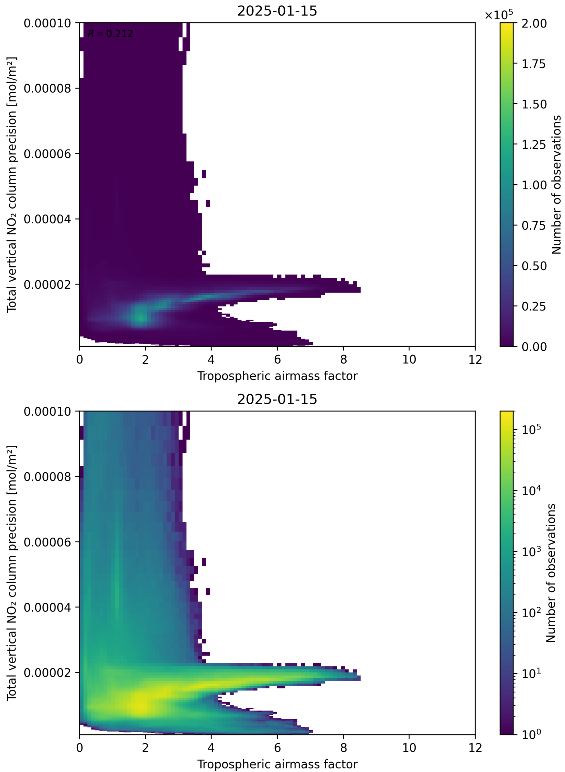
Figure 78: Scatter density plot of “Tropospheric air mass factor” against “Total vertical NO 2 column precision” for 2025-01-14 to 2025-01-16.
