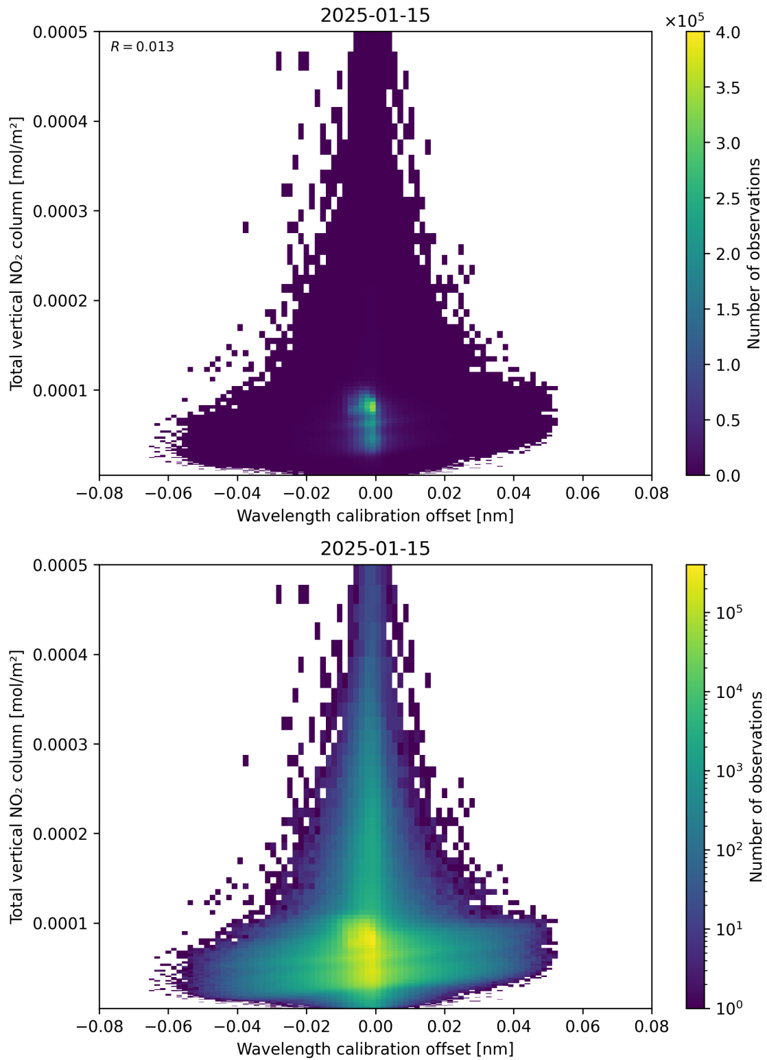
Figure 179: Scatter density plot of “Wavelength calibration offset” against “Total vertical NO 2 column” for 2025-01-14 to 2025-01-16.
