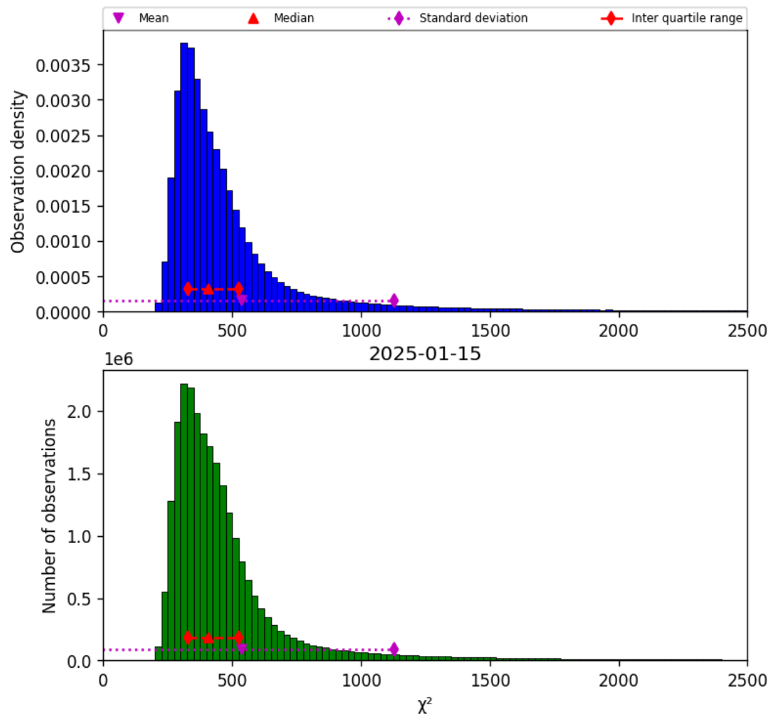
Figure 42: Histogram of “ \chi^2 ” for 2025-01-14 to 2025-01-16
