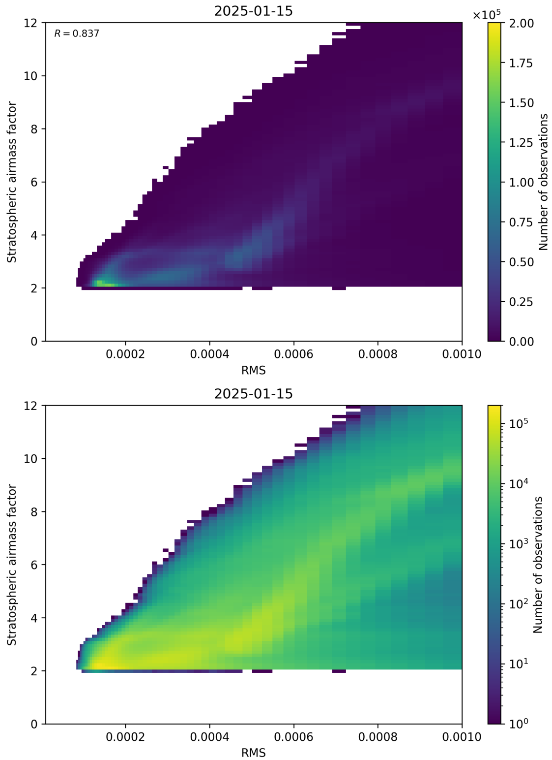
Figure 144: Scatter density plot of “RMS” against “Stratospheric airmass factor” for 2025-01-14 to 2025-01-16.
