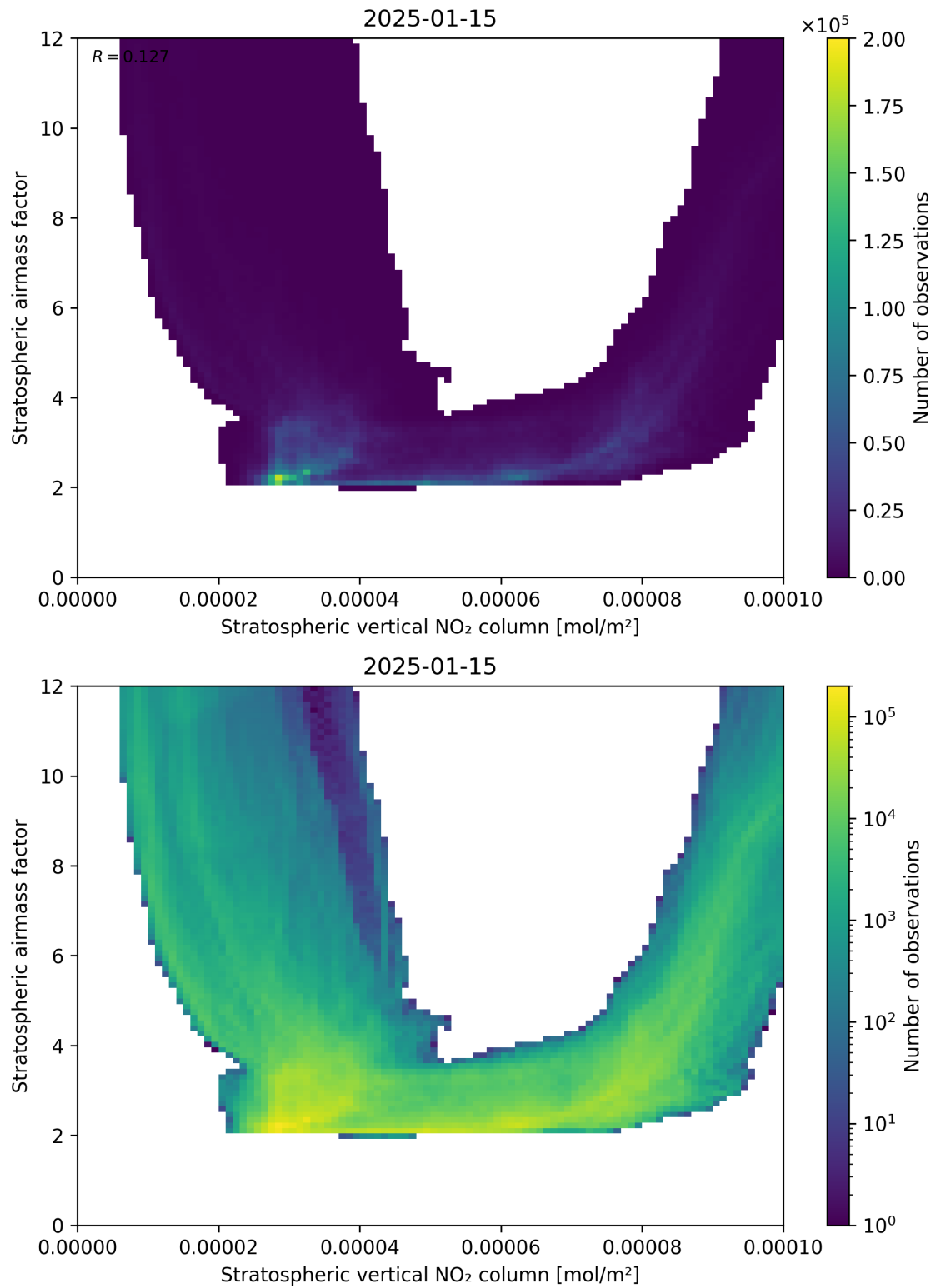
Figure 96: Scatter density plot of “Stratospheric vertical NO 2 column” against “Stratospheric airmass factor” for 2025-01-14 to 2025-01-16.
