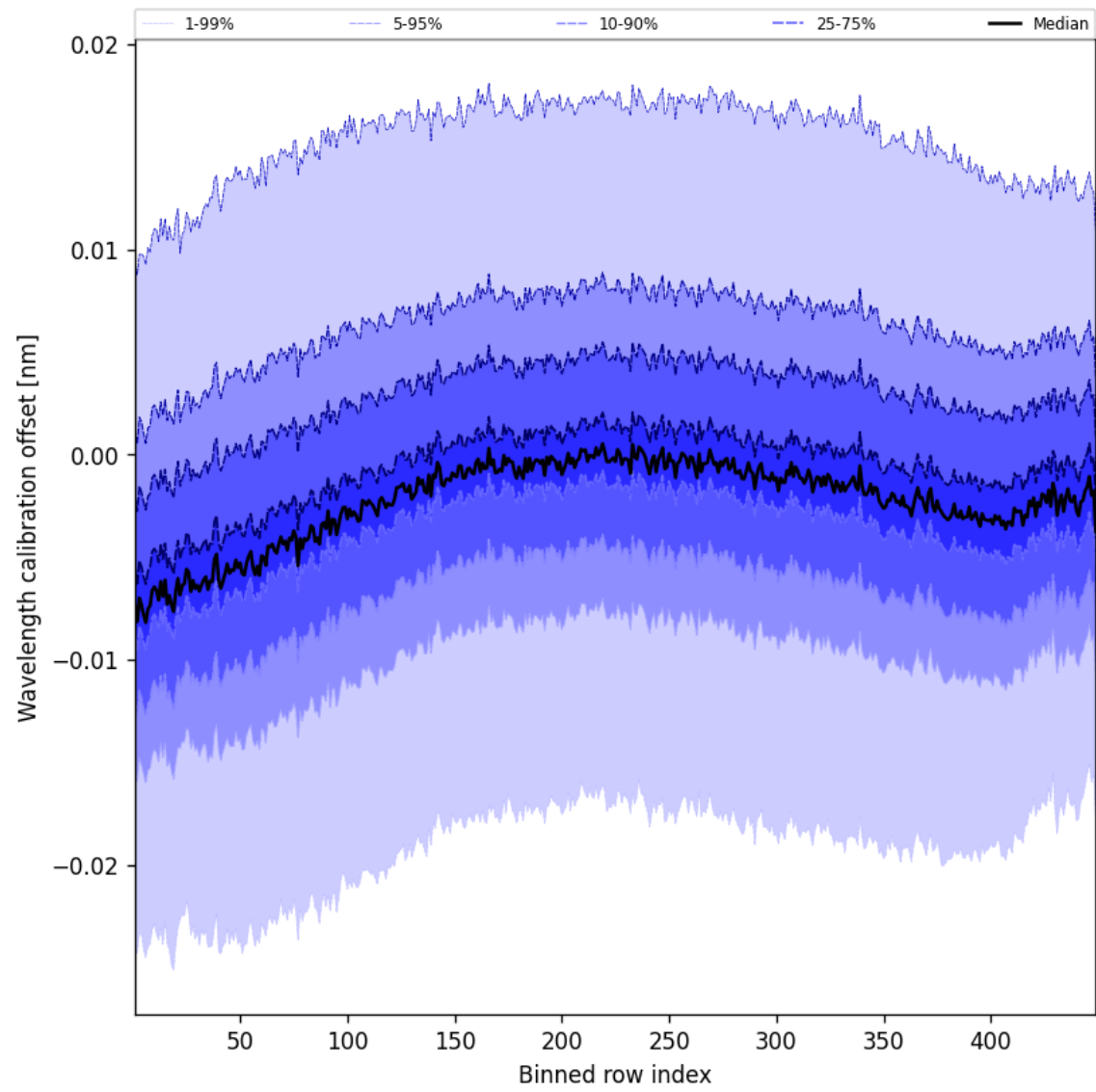
Figure 52: Along track statistics of “Wavelength calibration offset” for 2025-01-15 to 2025-01-17
