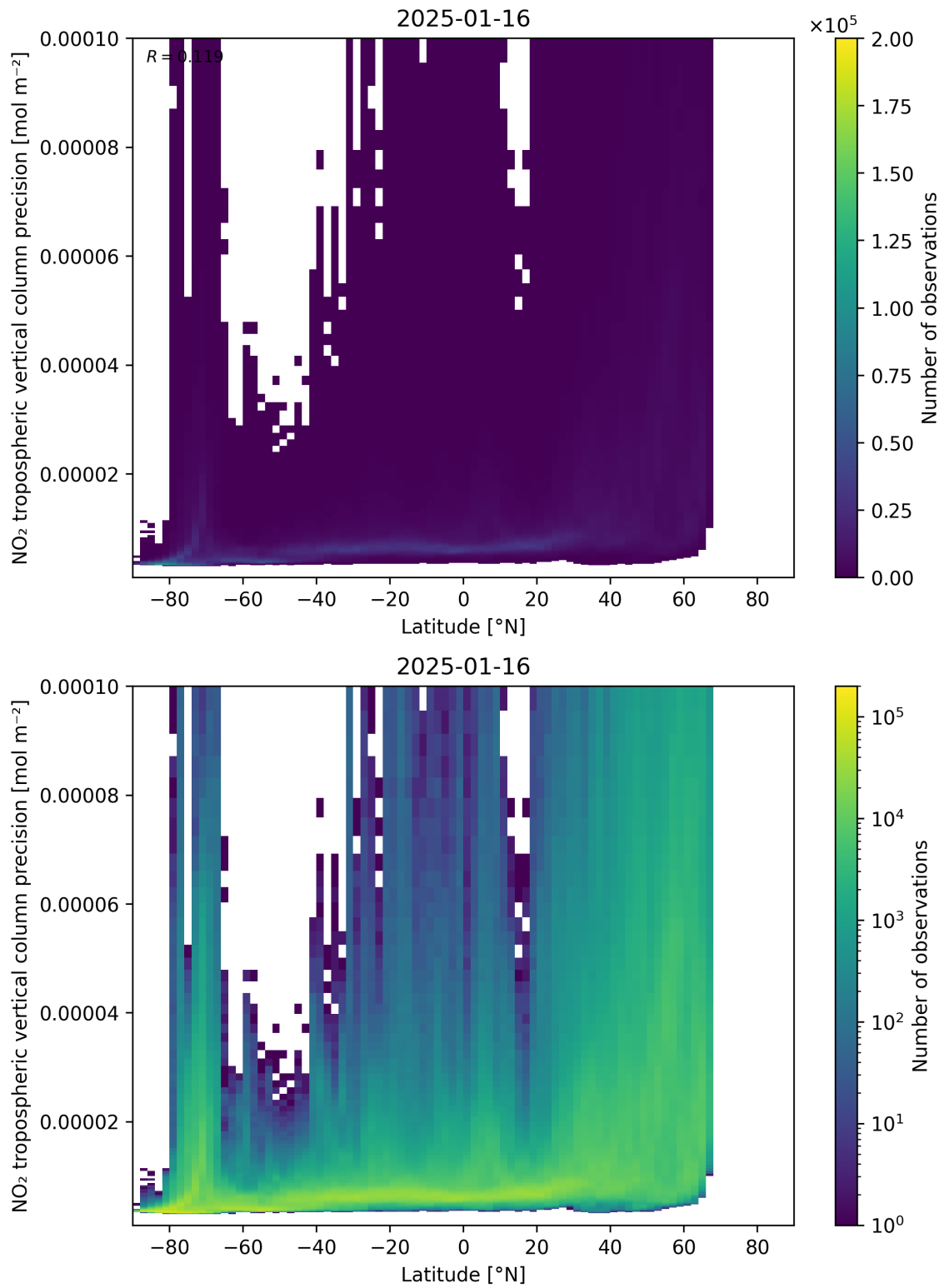
Figure 93: Scatter density plot of “Latitude” against “NO 2 tropospheric vertical column precision” for 2025-01-15 to 2025-01-17.
