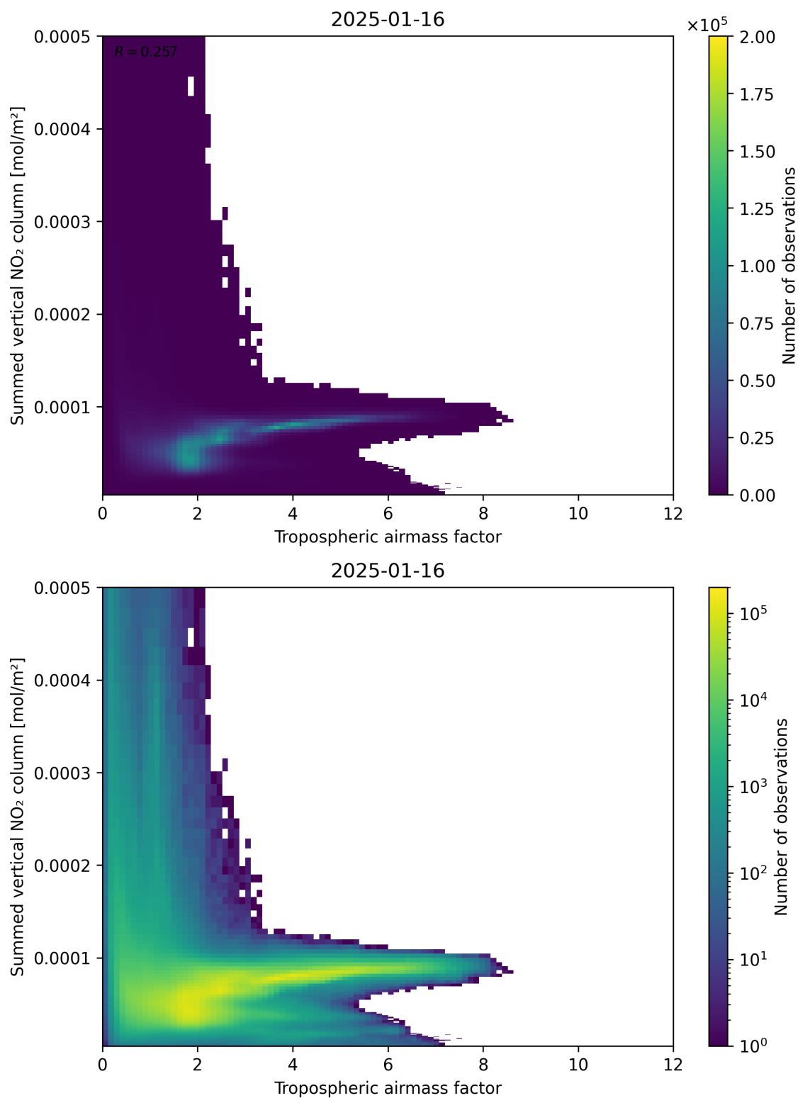
Figure 75: Scatter density plot of “Tropospheric air mass factor” against “Summed vertical NO 2 column” for 2025-01-15 to 2025-01-17.
