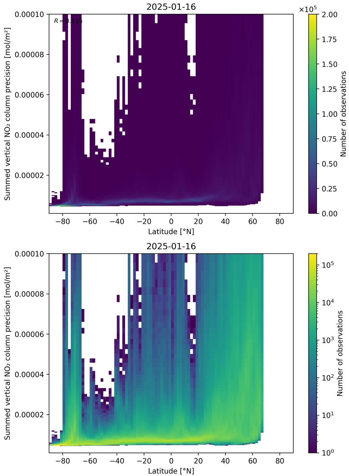
Figure 89: Scatter density plot of “Latitude” against “Summed vertical NO 2 column precision” for 2025-01-15 to 2025-01-17.
