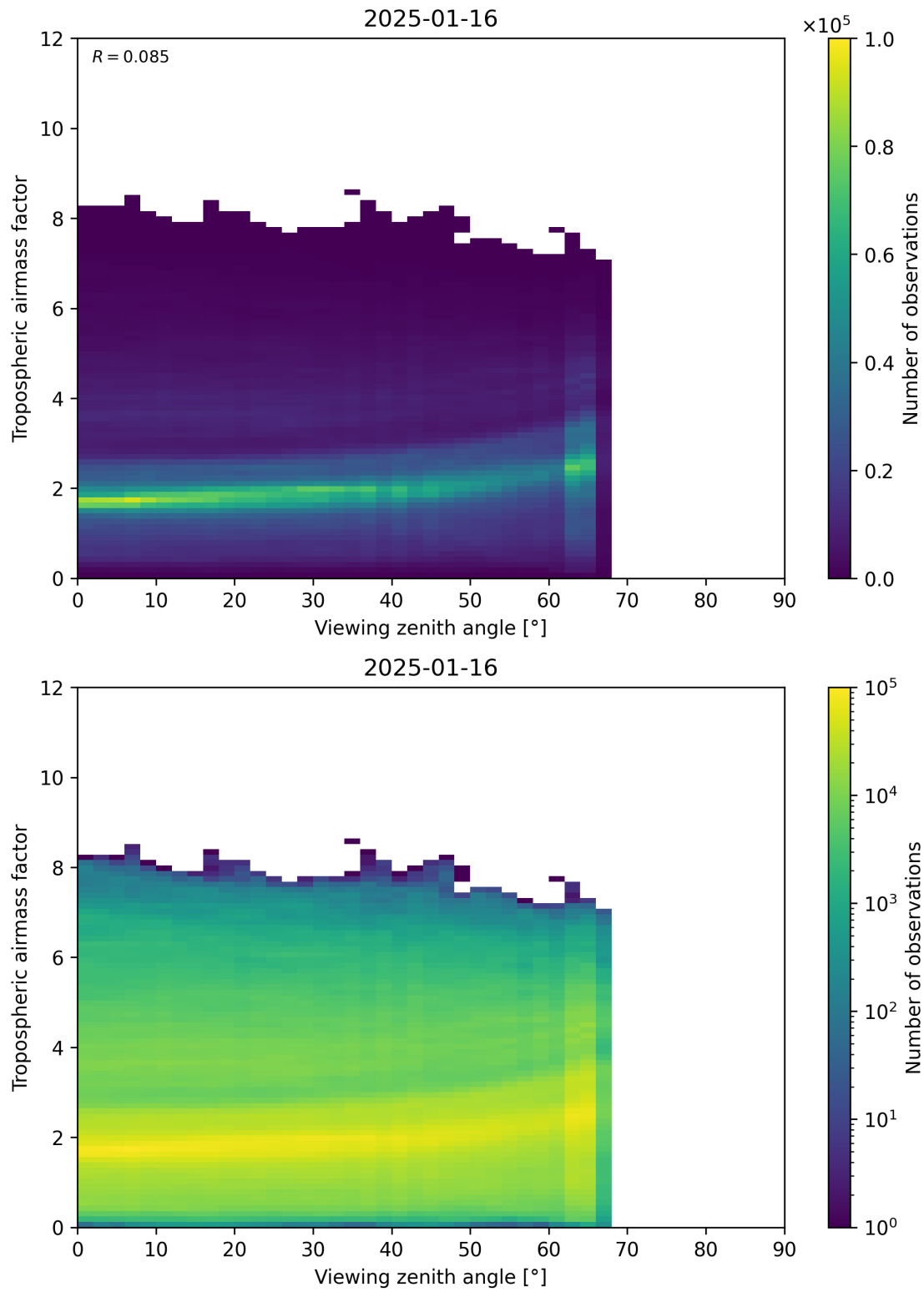
Figure 161: Scatter density plot of “Viewing zenith angle” against “Tropospheric airmass factor” for 2025-01-15 to 2025-01-17.
