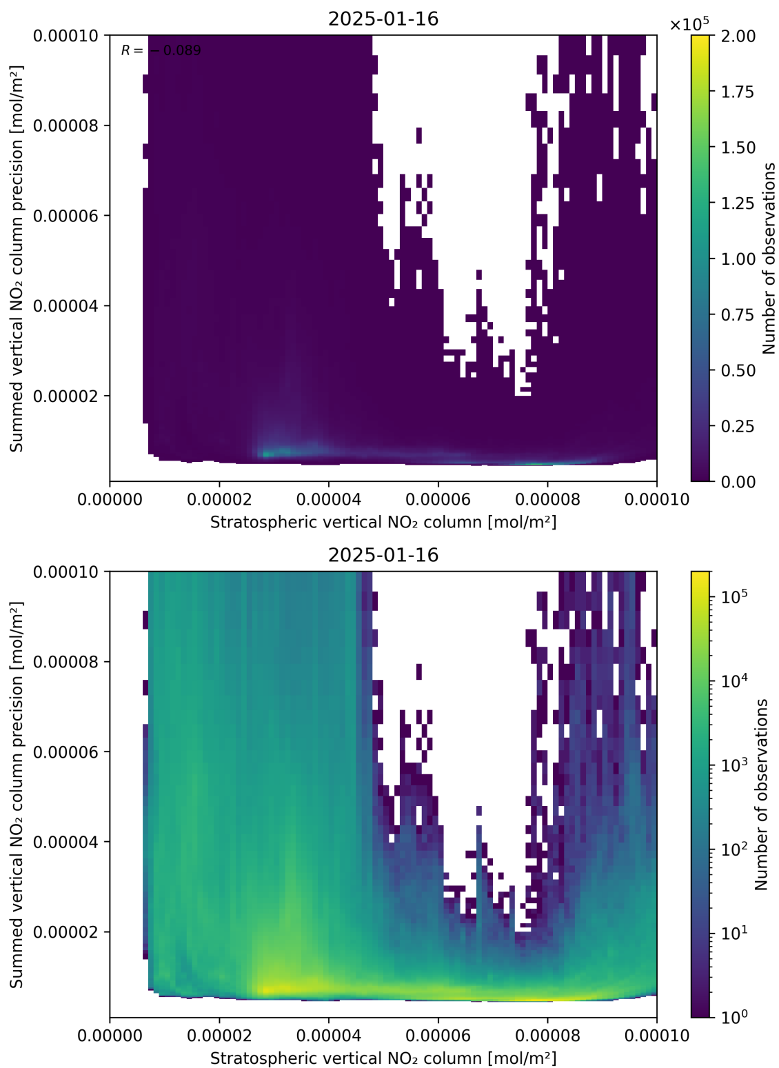
Figure 99: Scatter density plot of “Stratospheric vertical NO 2 column” against “Summed vertical NO 2 column precision” for 2025-01-15 to 2025-01-17.
