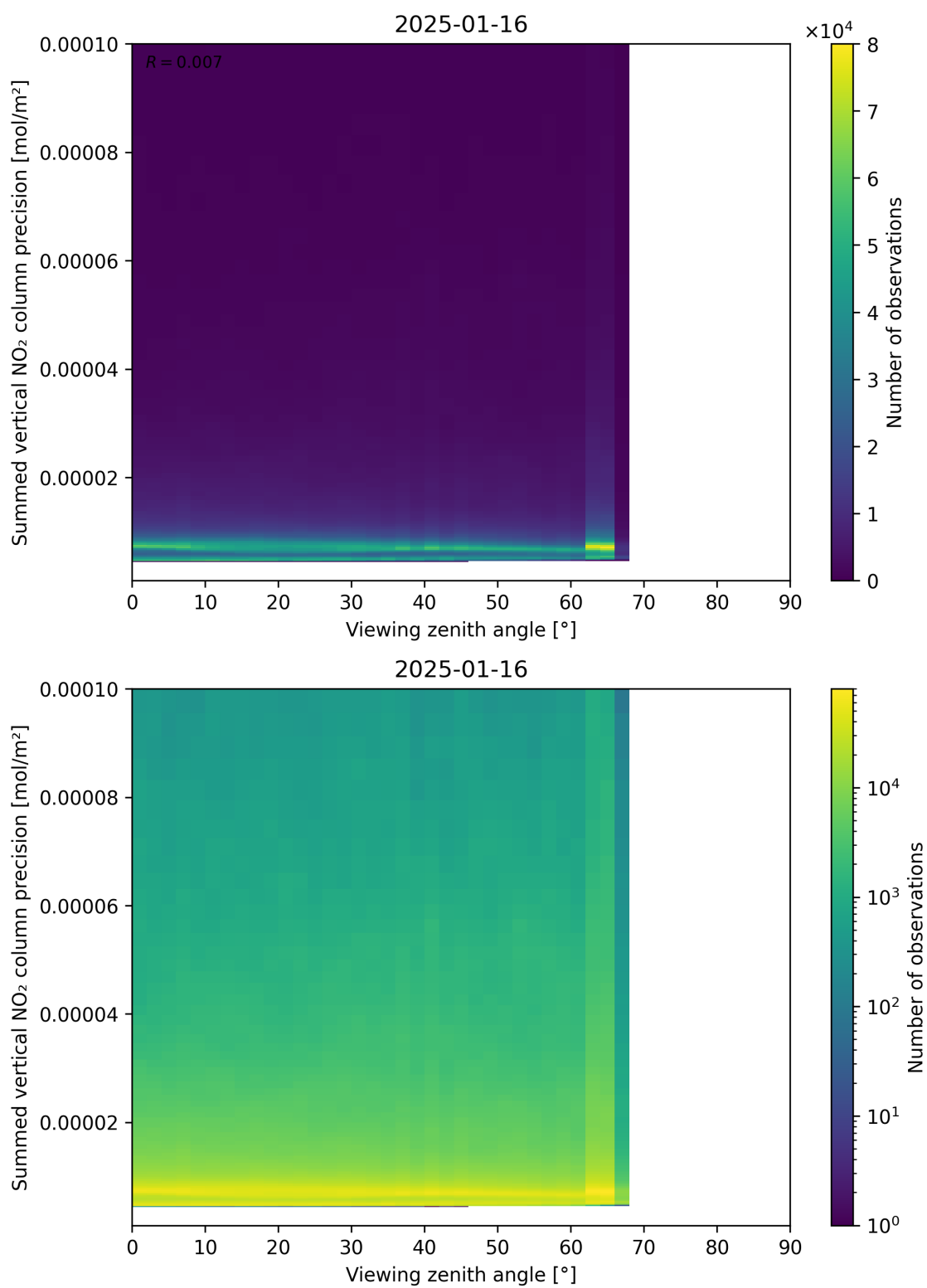
Figure 166: Scatter density plot of “Viewing zenith angle” against “Summed vertical NO 2 column precision” for 2025-01-15 to 2025-01-17.
