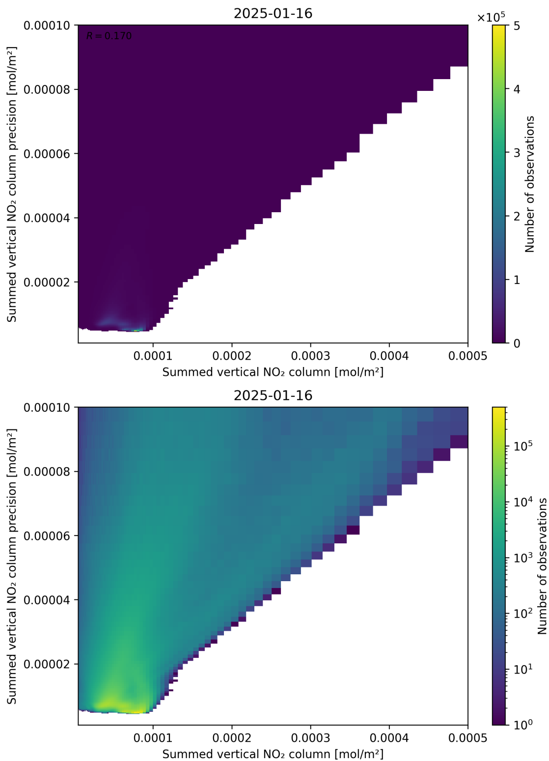
Figure 105: Scatter density plot of “Summed vertical NO 2 column” against “Summed vertical NO 2 column precision” for 2025-01-15 to 2025-01-17.
