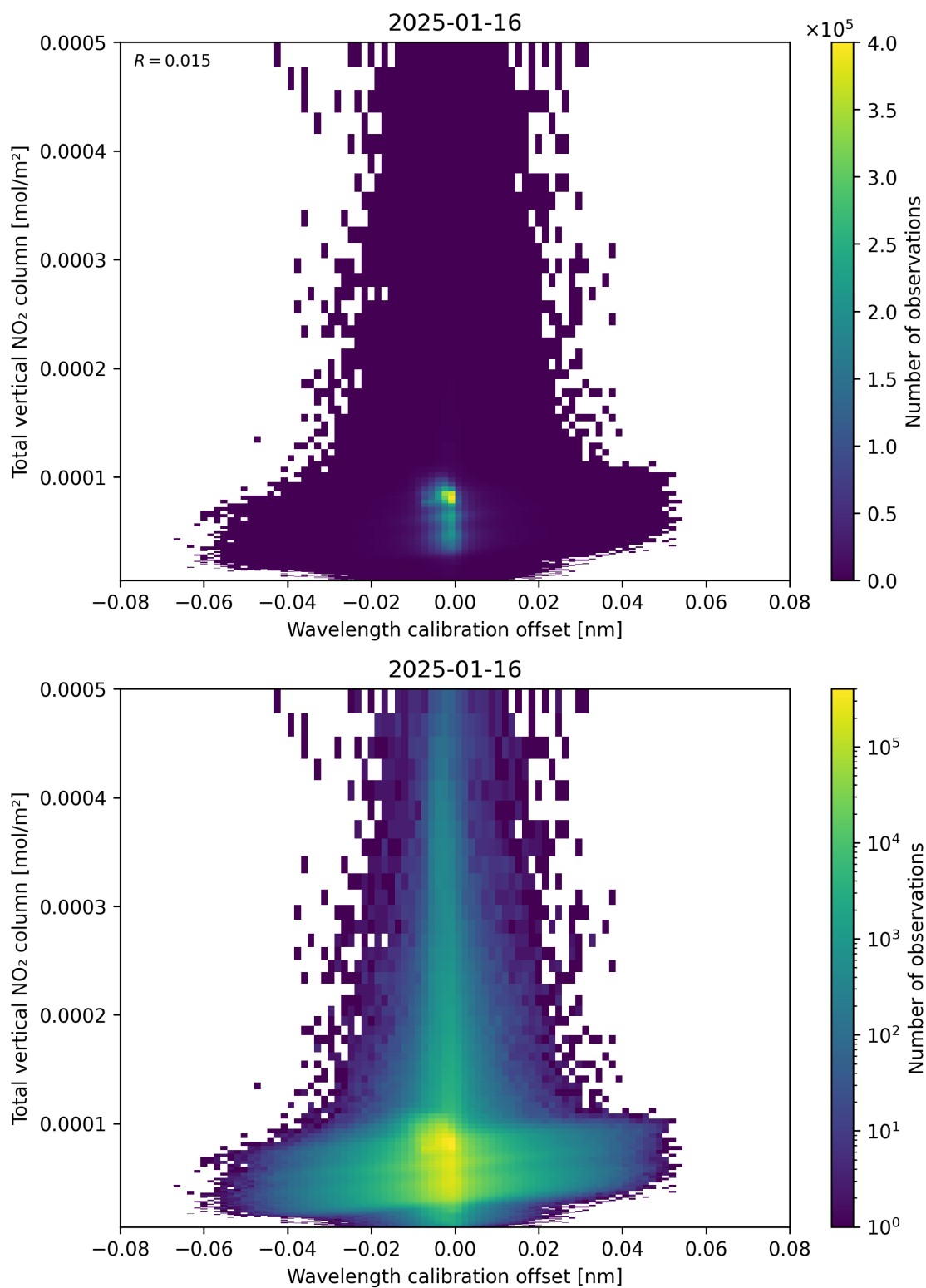
Figure 179: Scatter density plot of “Wavelength calibration offset” against “Total vertical NO 2 column” for 2025-01-15 to 2025-01-17.
