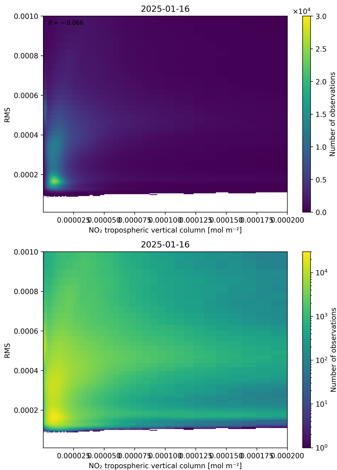
Figure 142: Scatter density plot of “NO 2 tropospheric vertical column” against “RMS” for 2025-01-15 to 2025-01-17.
