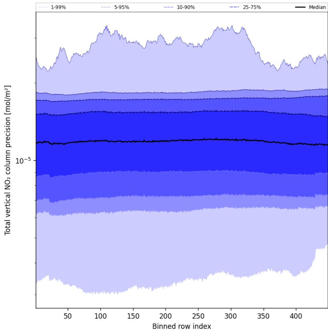
Figure 56: Along track statistics of “Total vertical NO 2 column precision” for 2025-01-15 to 2025-01-17
