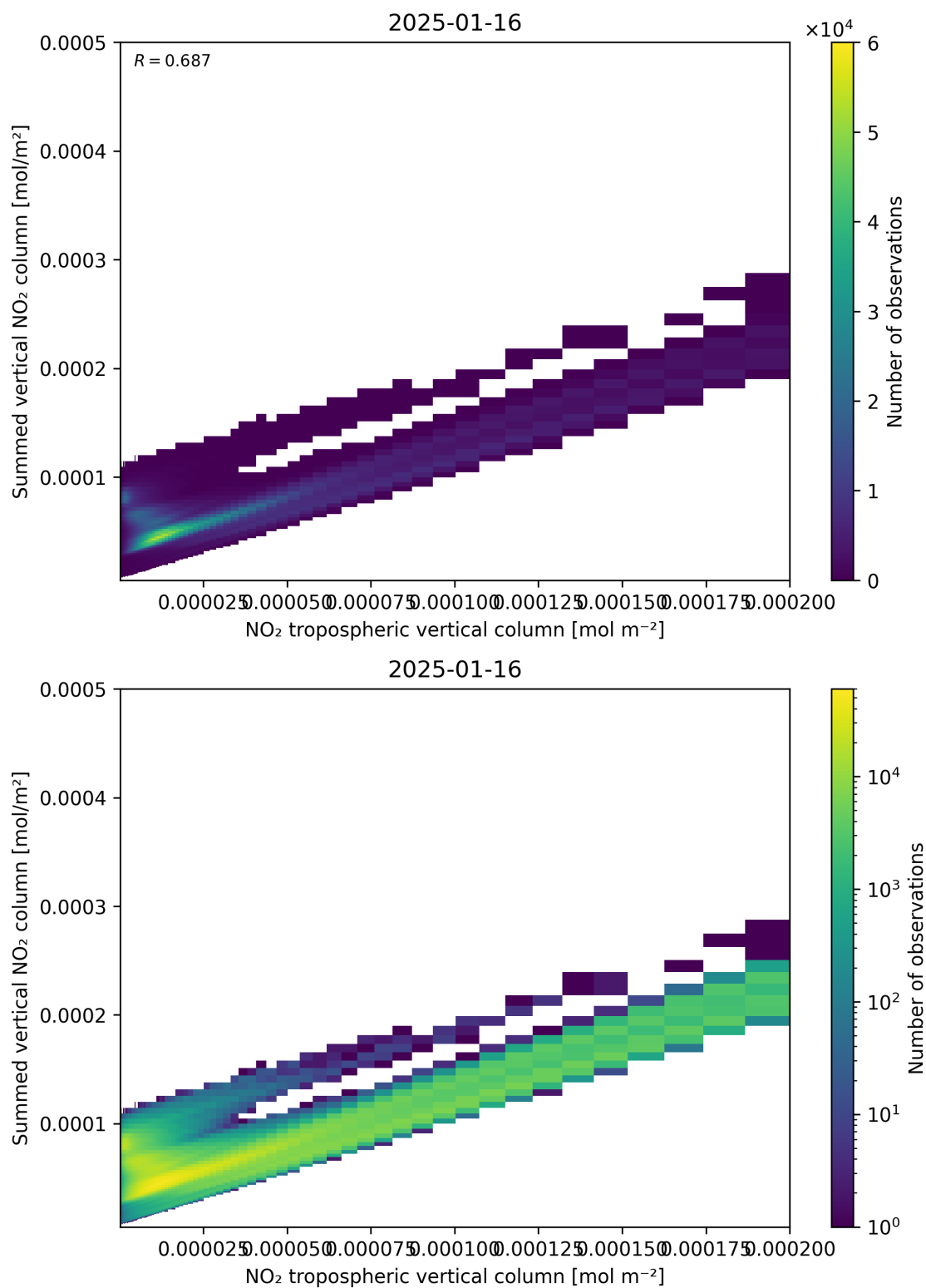
Figure 126: Scatter density plot of “NO 2 tropospheric vertical column” against “Summed vertical NO 2 column” for 2025-01-15 to 2025-01-17.
