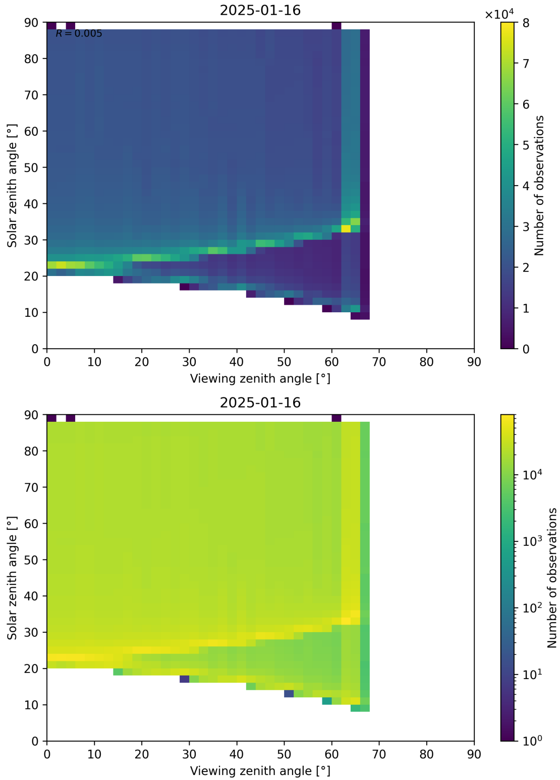
Figure 172: Scatter density plot of “Viewing zenith angle” against “Solar zenith angle” for 2025-01-15 to 2025-01-17.
