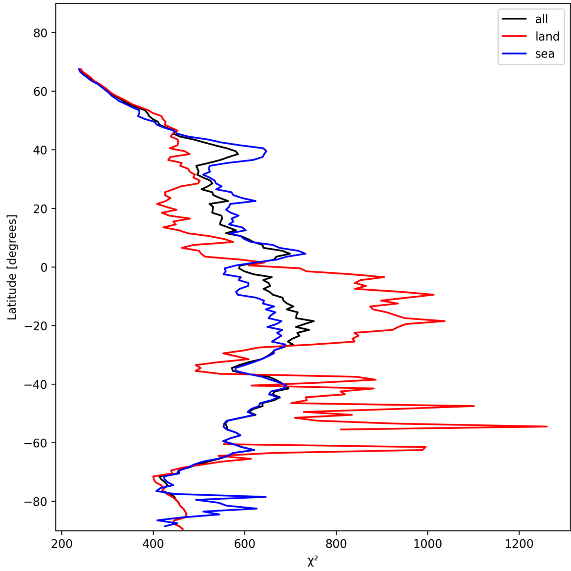
Figure 25: Zonal average of “ \chi^2 ” for 2025-01-15 to 2025-01-17.
