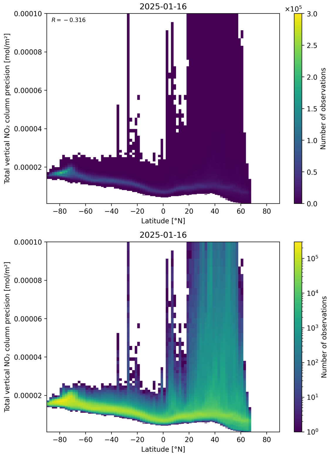
Figure 91: Scatter density plot of “Latitude” against “Total vertical NO 2 column precision” for 2025-01-15 to 2025-01-17.
