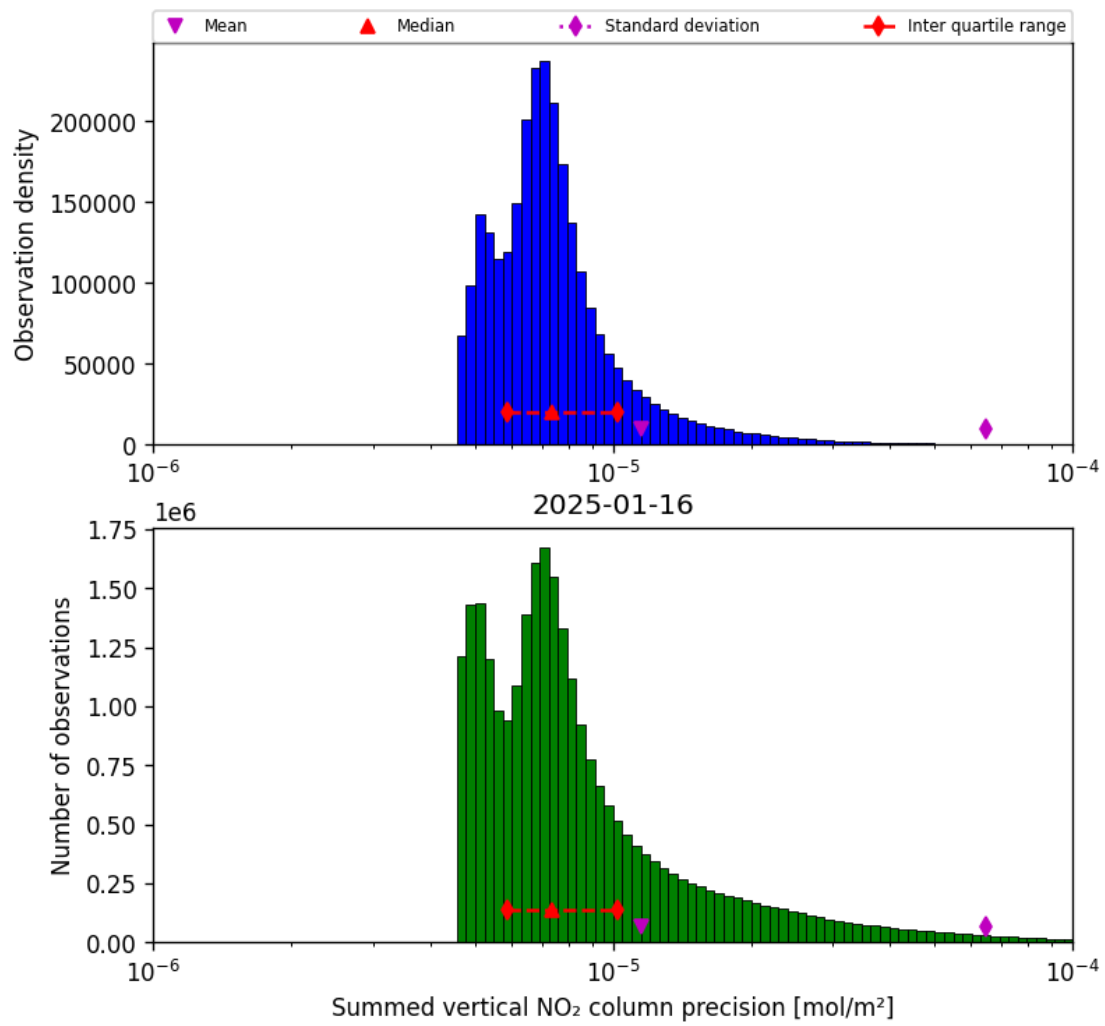
Figure 41: Histogram of “Summed vertical NO 2 column precision” for 2025-01-15 to 2025-01-17
