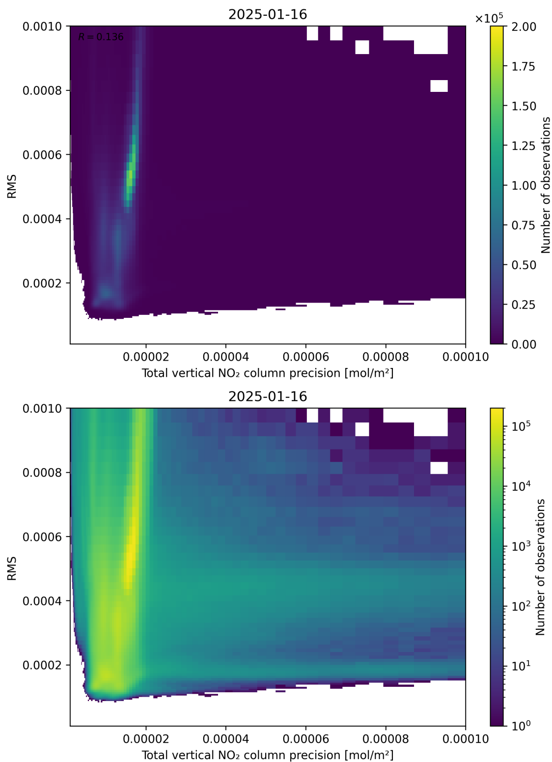
Figure 119: Scatter density plot of “Total vertical NO 2 column precision” against “RMS” for 2025-01-15 to 2025-01-17.
