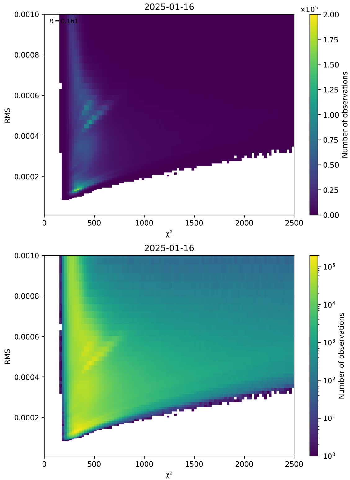
Figure 82: Scatter density plot of “ \chi^2 ” against “RMS” for 2025-01-15 to 2025-01-17.
