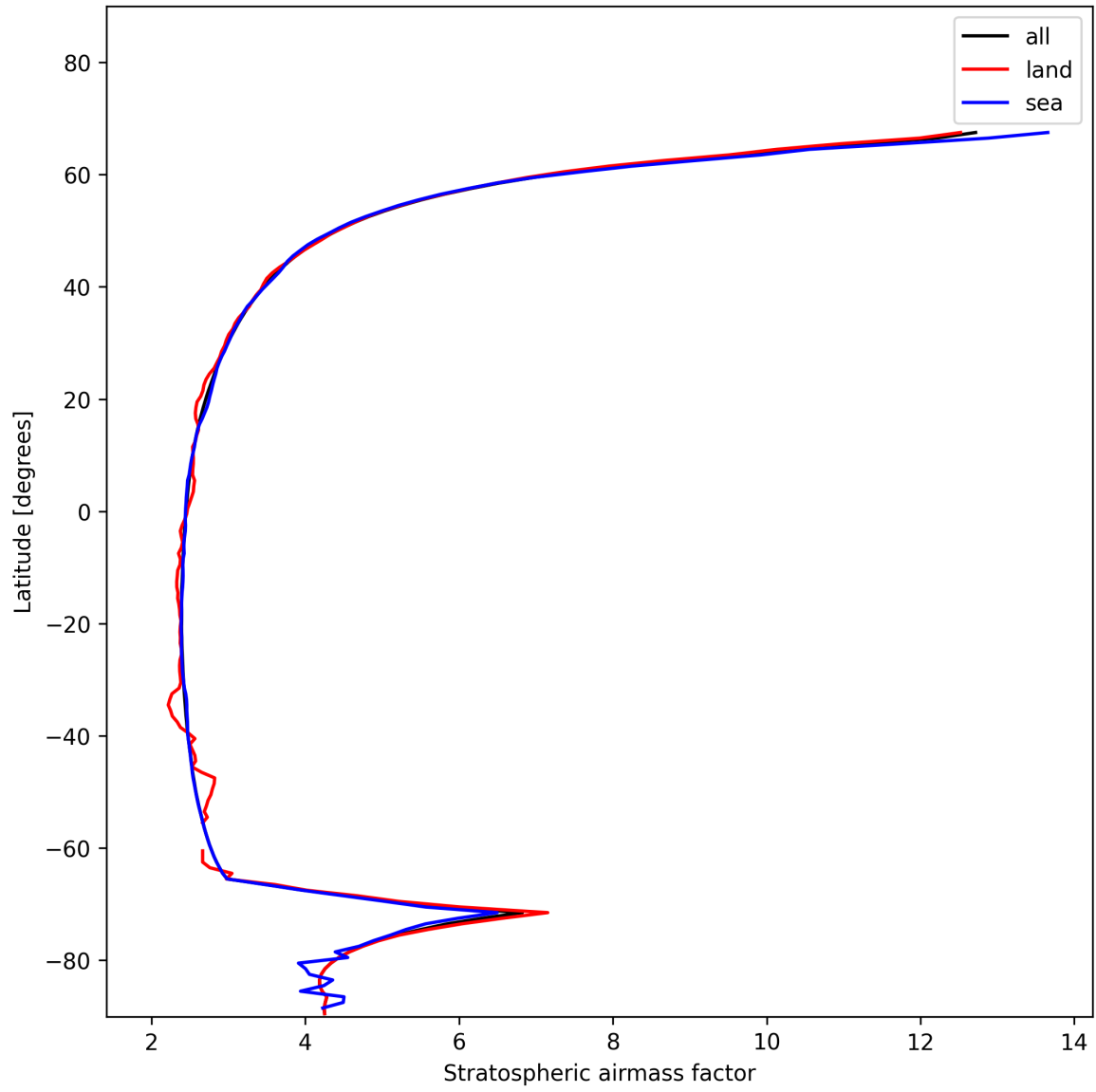
Figure 27: Zonal average of “Stratospheric air mass factor” for 2025-01-15 to 2025-01-17.
