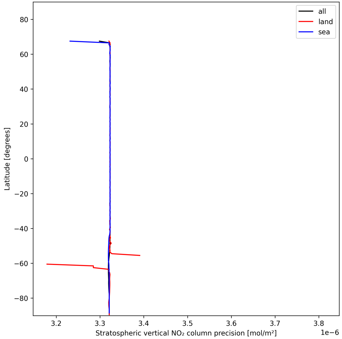
Figure 20: Zonal average of "Stratospheric vertical NO 2 column precision" for 2025-01-15 to 2025-01-17.
