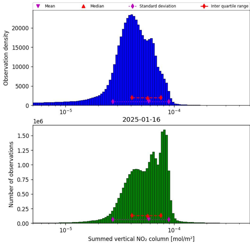
Figure 40: Histogram of “Summed vertical NO 2 column” for 2025-01-15 to 2025-01-17
