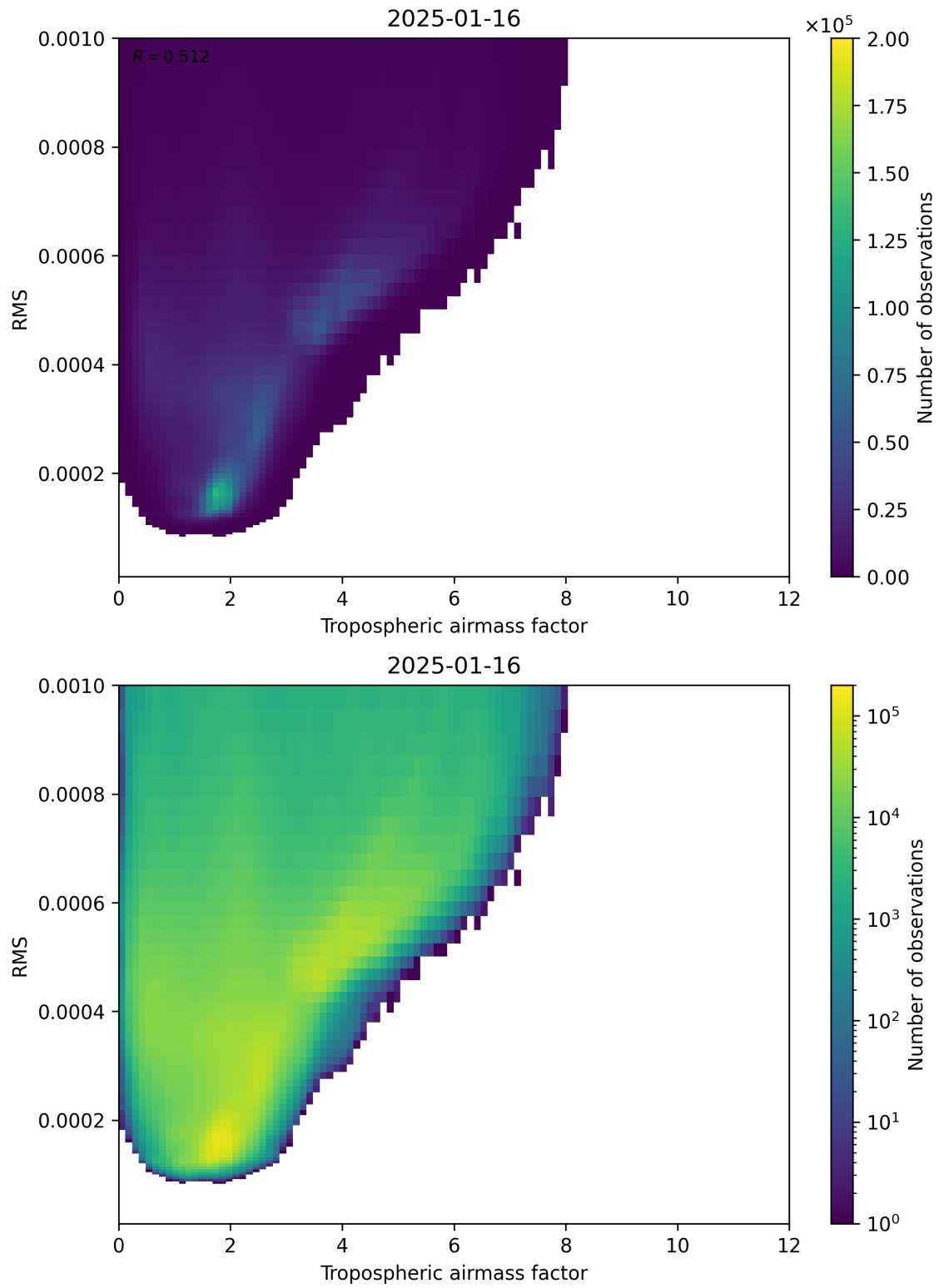
Figure 79: Scatter density plot of “Tropospheric airmass factor” against “RMS” for 2025-01-15 to 2025-01-17.
