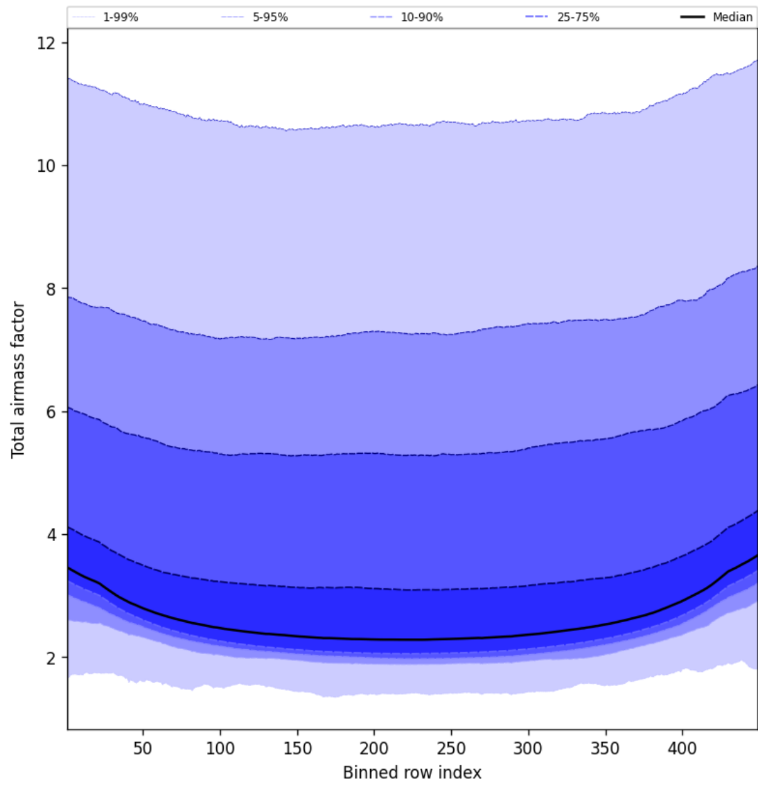
Figure 49: Along track statistics of “Total airmass factor” for 2025-01-15 to 2025-01-17
