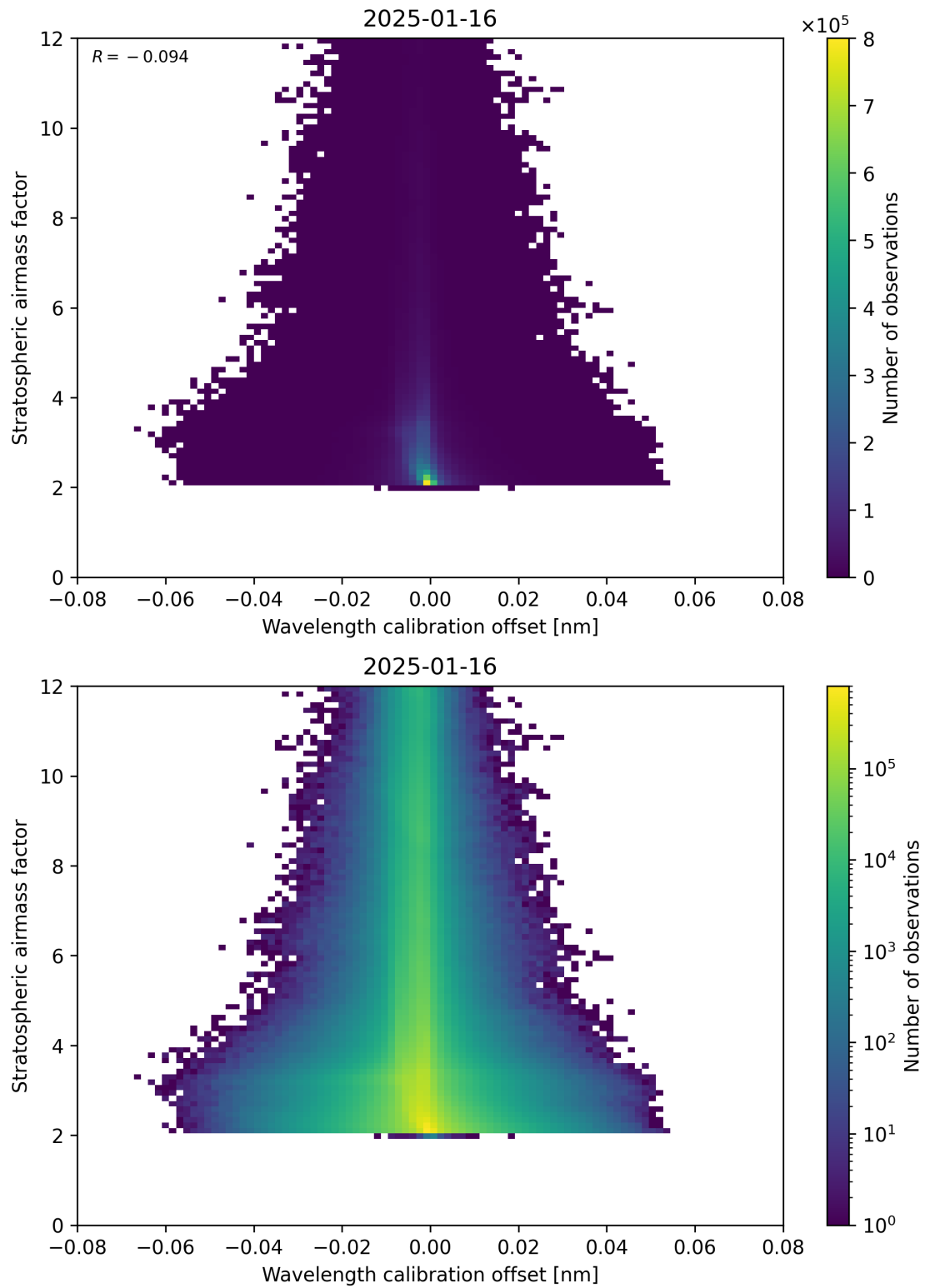
Figure 174: Scatter density plot of “Wavelength calibration offset” against “Stratospheric airmass factor” for 2025-01-15 to 2025-01-17.
