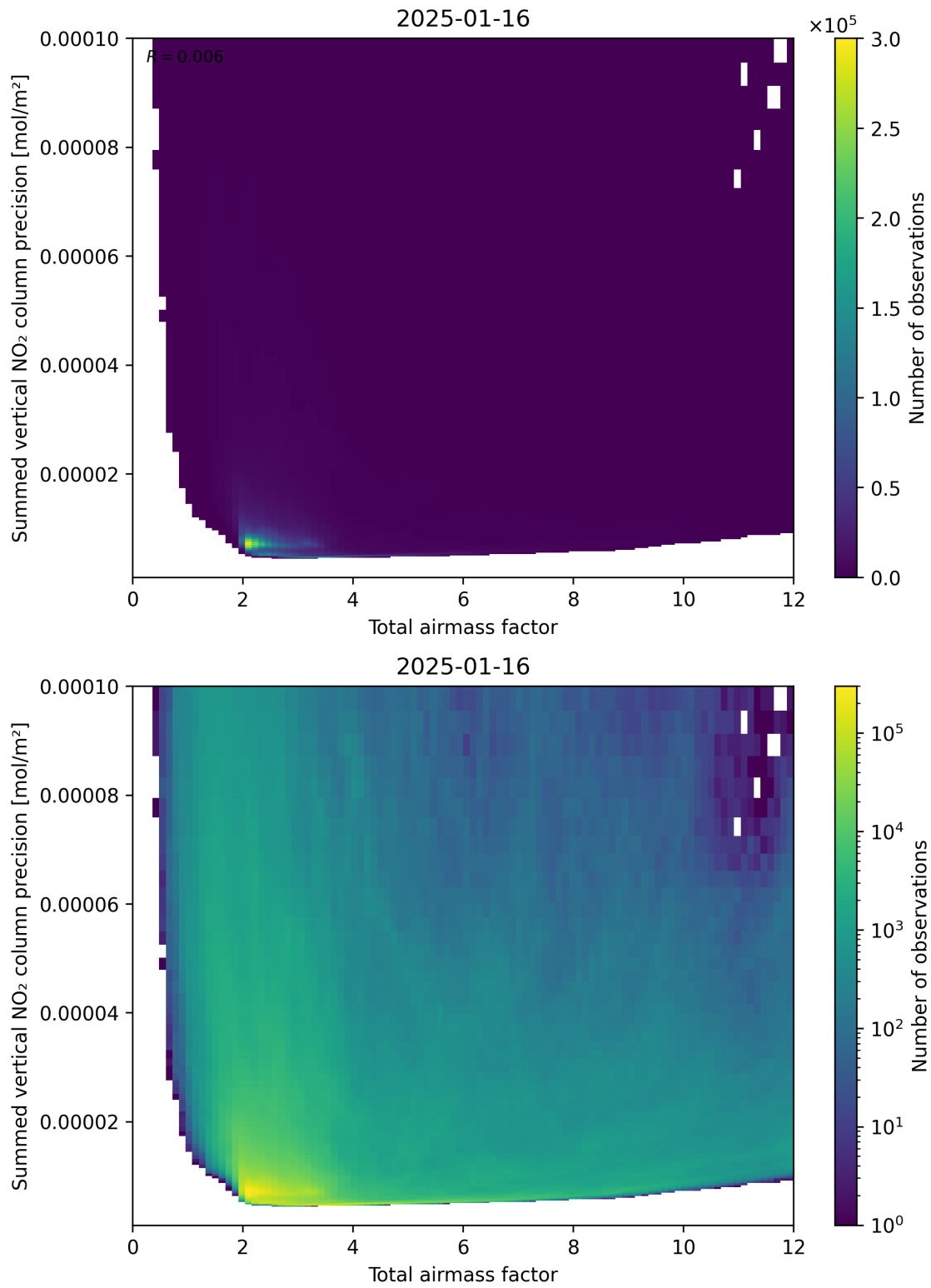
Figure 66: Scatter density plot of “Total airmass factor” against “Summed vertical NO 2 column precision” for 2025-01-15 to 2025-01-17.
