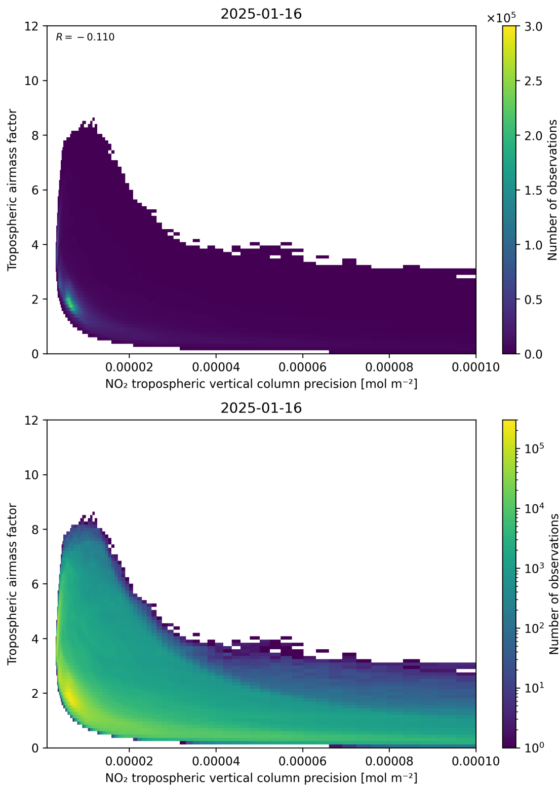
Figure 133: Scatter density plot of “NO 2 tropospheric vertical column precision” against “Tropospheric airmass factor” for 2025-01-15 to 2025-01-17.
