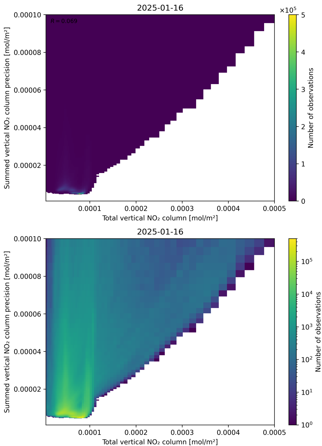
Figure 113: Scatter density plot of “Total vertical NO 2 column” against “Summed vertical NO 2 column precision” for 2025-01-15 to 2025-01-17.
