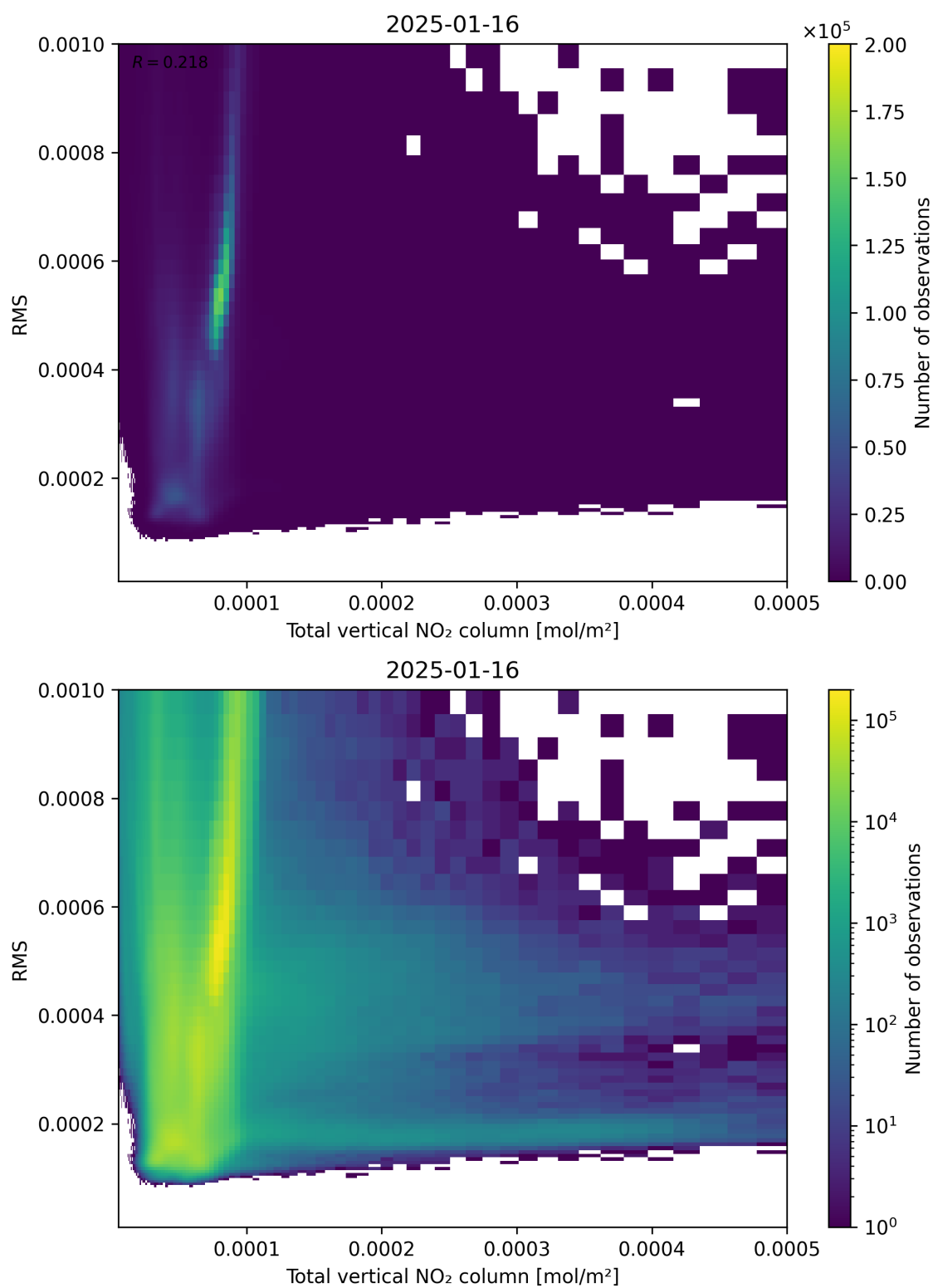
Figure 120: Scatter density plot of “Total vertical NO 2 column” against “RMS” for 2025-01-15 to 2025-01-17.
