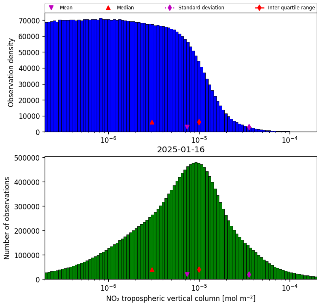
Figure 29: Histogram of “NO 2 tropospheric vertical column” for 2025-01-15 to 2025-01-17
