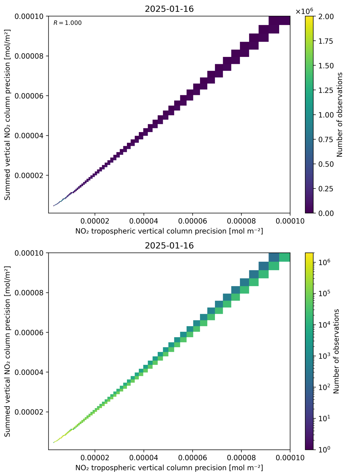
Figure 137: Scatter density plot of “NO 2 tropospheric vertical column precision” against “Summed vertical NO 2 column precision” for 2025-01-15 to 2025-01-17.
