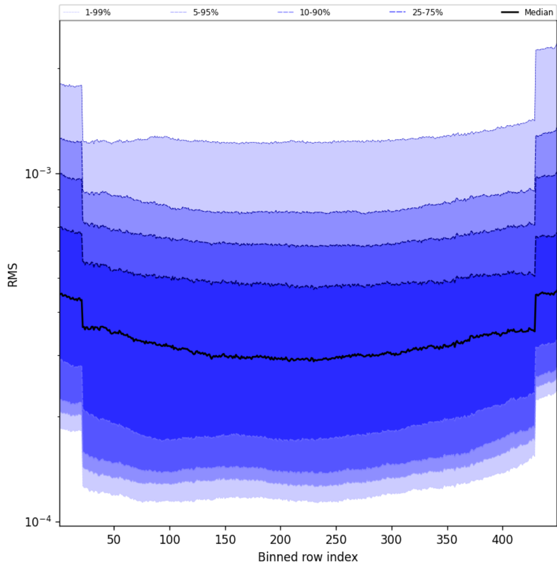
Figure 60: Along track statistics of “RMS” for 2025-01-15 to 2025-01-17
