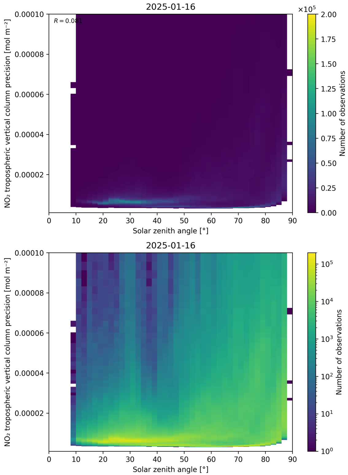
Figure 156: Scatter density plot of “Solar zenith angle” against “NO 2 tropospheric vertical column precision” for 2025-01-15 to 2025-01-17.
