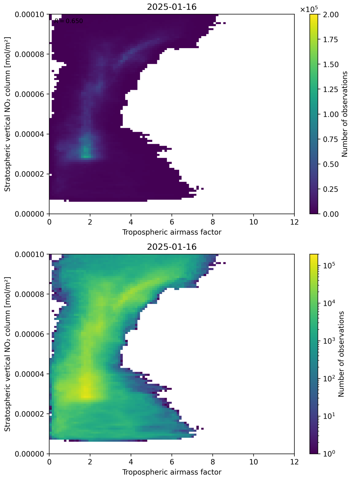
Figure 74: Scatter density plot of “Tropospheric airmass factor” against “Stratospheric vertical NO 2 column” for 2025-01-15 to 2025-01-17.
