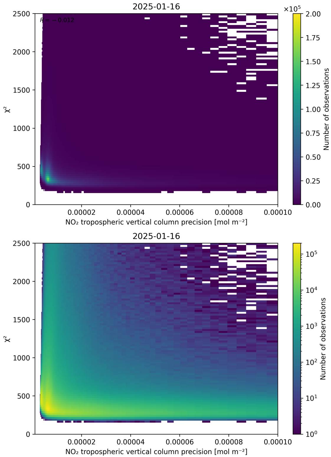
Figure 134: Scatter density plot of “NO 2 tropospheric vertical column precision” against “ \chi^2 ” for 2025-01-15 to 2025-01-17.
