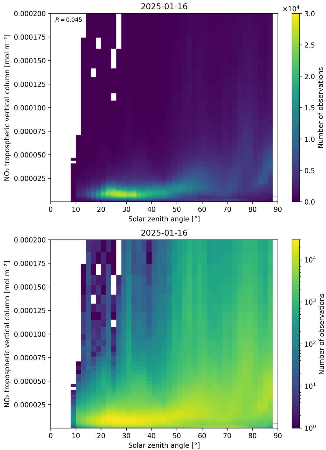
Figure 155: Scatter density plot of “Solar zenith angle” against “NO 2 tropospheric vertical column” for 2025-01-15 to 2025-01-17.
