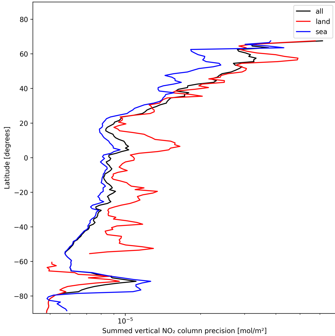
Figure 24: Zonal average of “Summed vertical NO 2 column precision” for 2025-01-15 to 2025-01-17.
