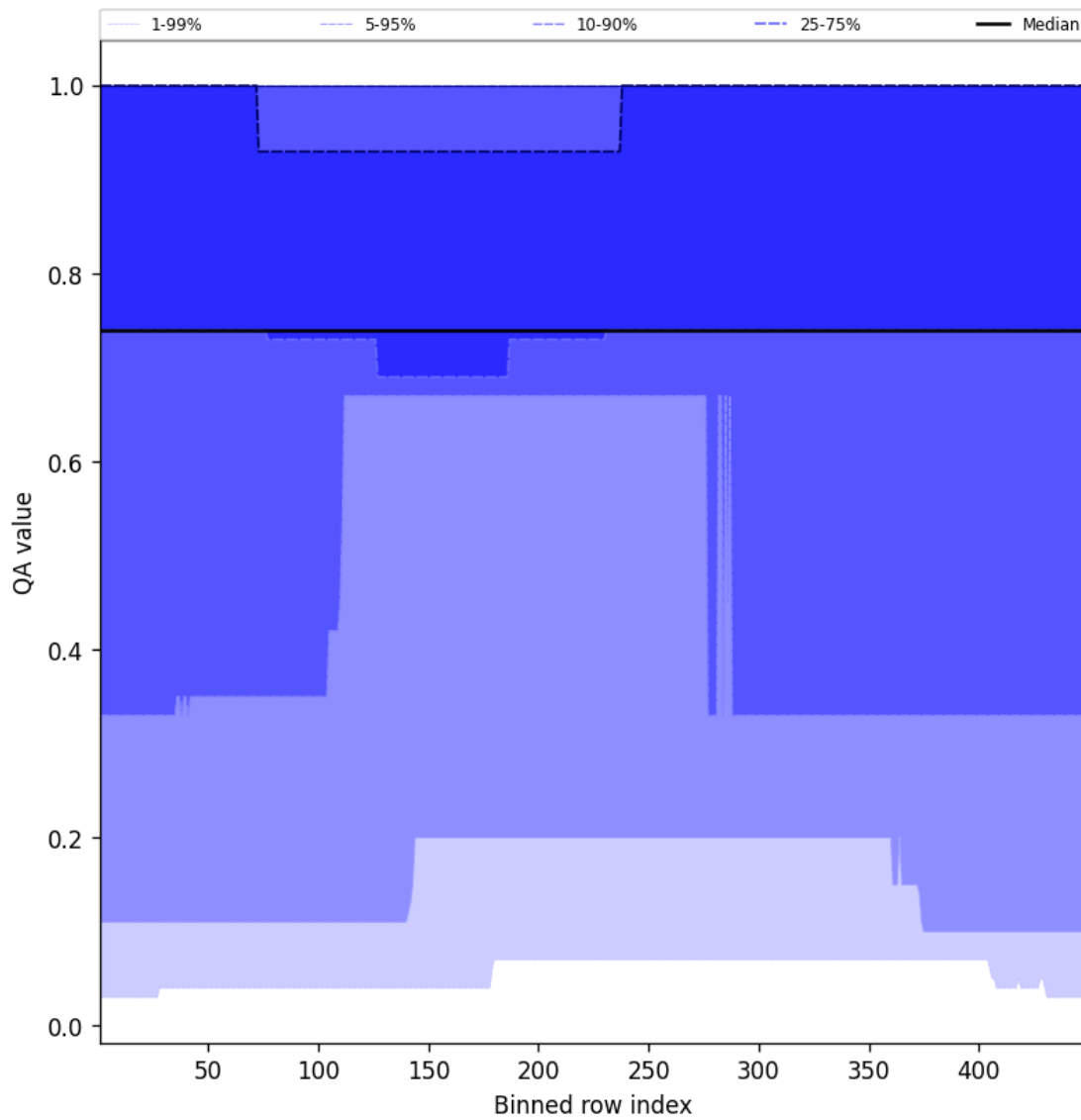
Figure 45: Along track statistics of “QA value” for 2025-01-15 to 2025-01-17
