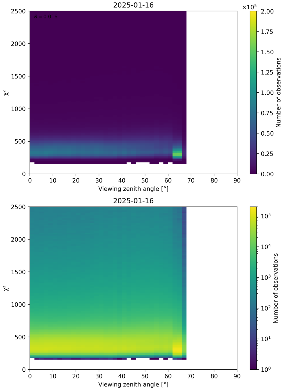
Figure 162: Scatter density plot of “Viewing zenith angle” against “ \chi^2 ” for 2025-01-15 to 2025-01-17.
