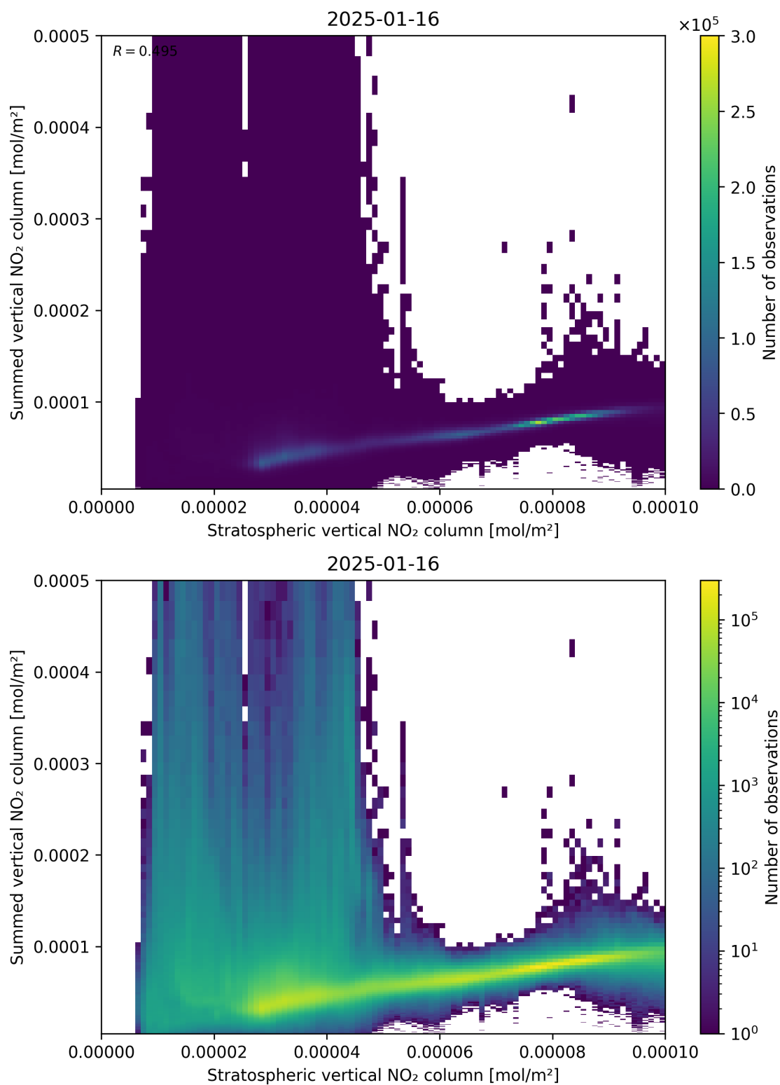
Figure 98: Scatter density plot of “Stratospheric vertical NO 2 column” against “Summed vertical NO 2 column” for 2025-01-15 to 2025-01-17.
