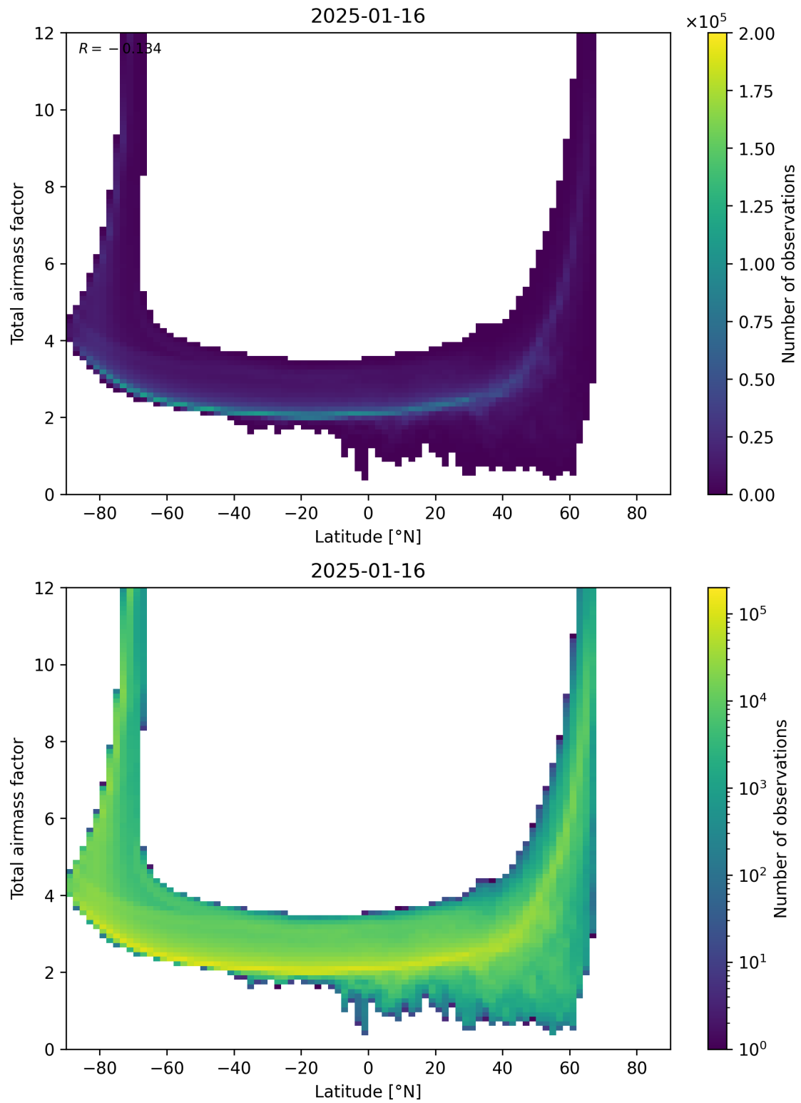
Figure 84: Scatter density plot of “Latitude” against “Total airmass factor” for 2025-01-15 to 2025-01-17.
