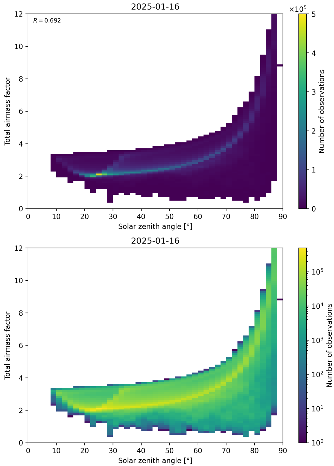
Figure 146: Scatter density plot of “Solar zenith angle” against “Total airmass factor” for 2025-01-15 to 2025-01-17.
