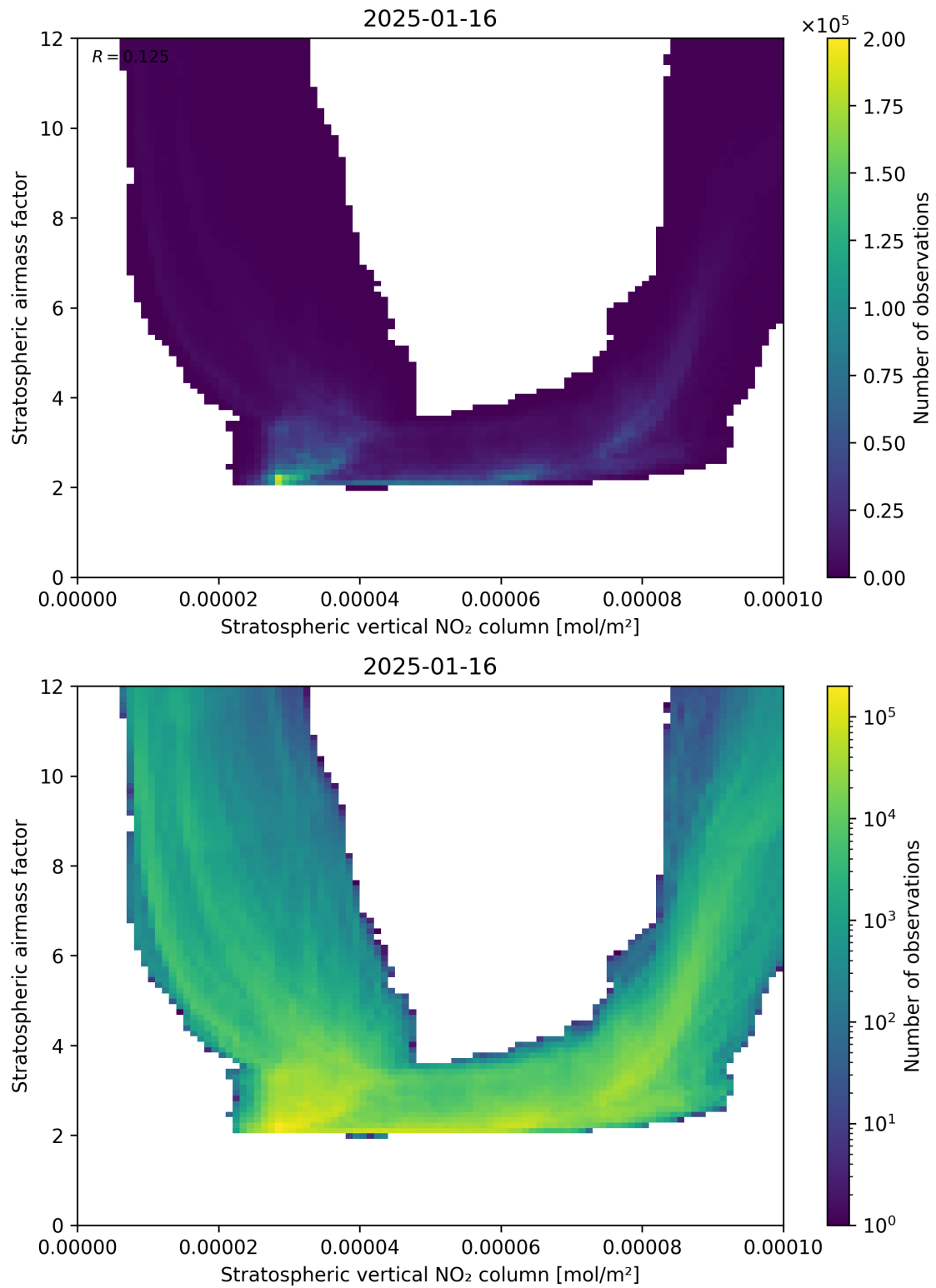
Figure 96: Scatter density plot of “Stratospheric vertical NO 2 column” against “Stratospheric airmass factor” for 2025-01-15 to 2025-01-17.
