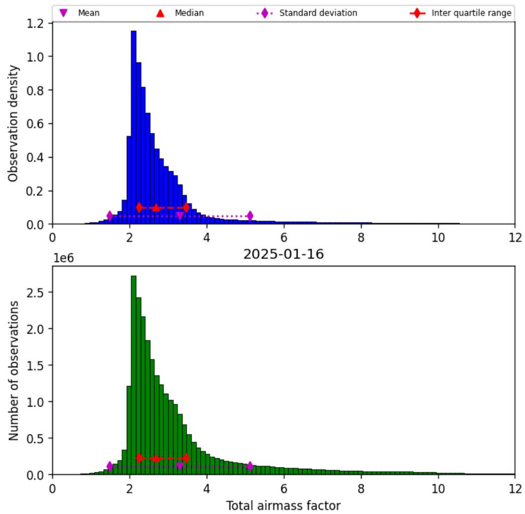
Figure 32: Histogram of “Total airmass factor” for 2025-01-15 to 2025-01-17
