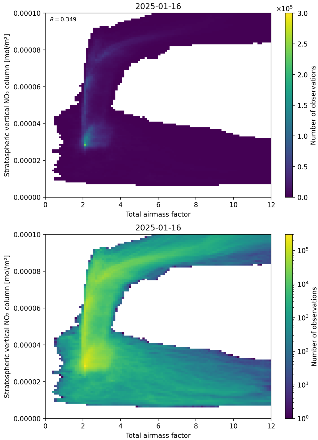
Figure 64: Scatter density plot of “Total airmass factor” against “Stratospheric vertical \text{NO}_2 column” for 2025-01-15 to 2025-01-17.
