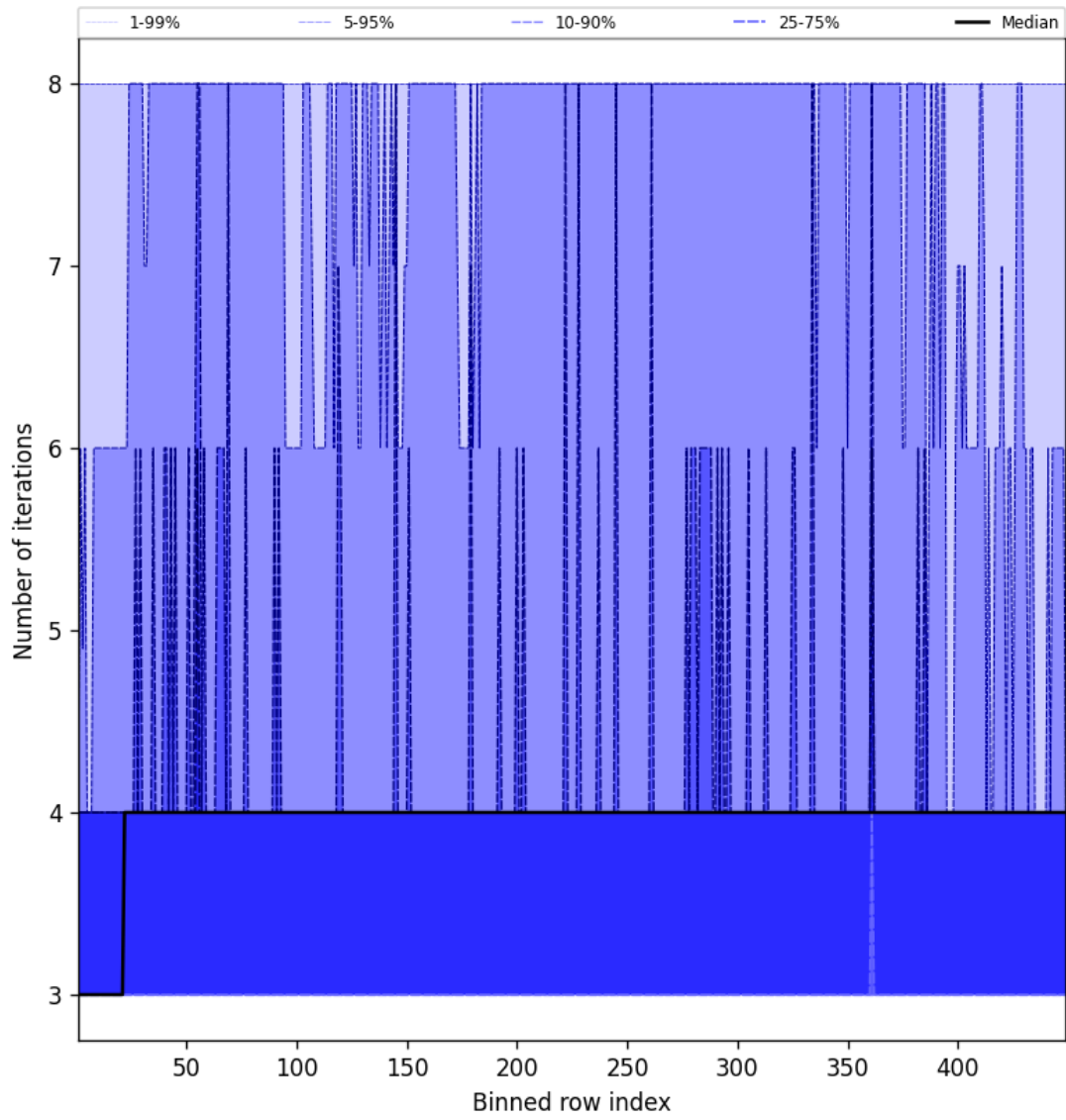
Figure 51: Along track statistics of “Number of iterations” for 2025-01-15 to 2025-01-17
