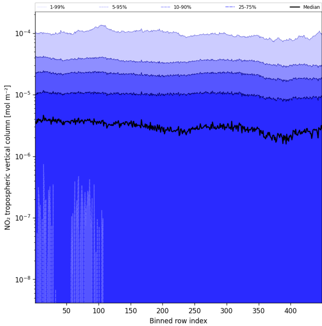
Figure 46: Along track statistics of “NO 2 tropospheric vertical column” for 2025-01-15 to 2025-01-17
