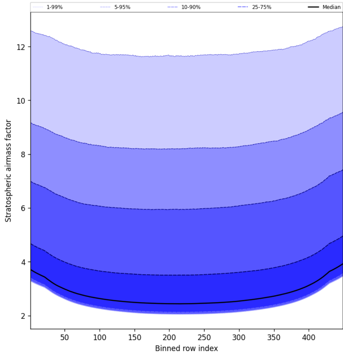
Figure 61: Along track statistics of “Stratospheric air mass factor” for 2025-01-15 to 2025-01-17
