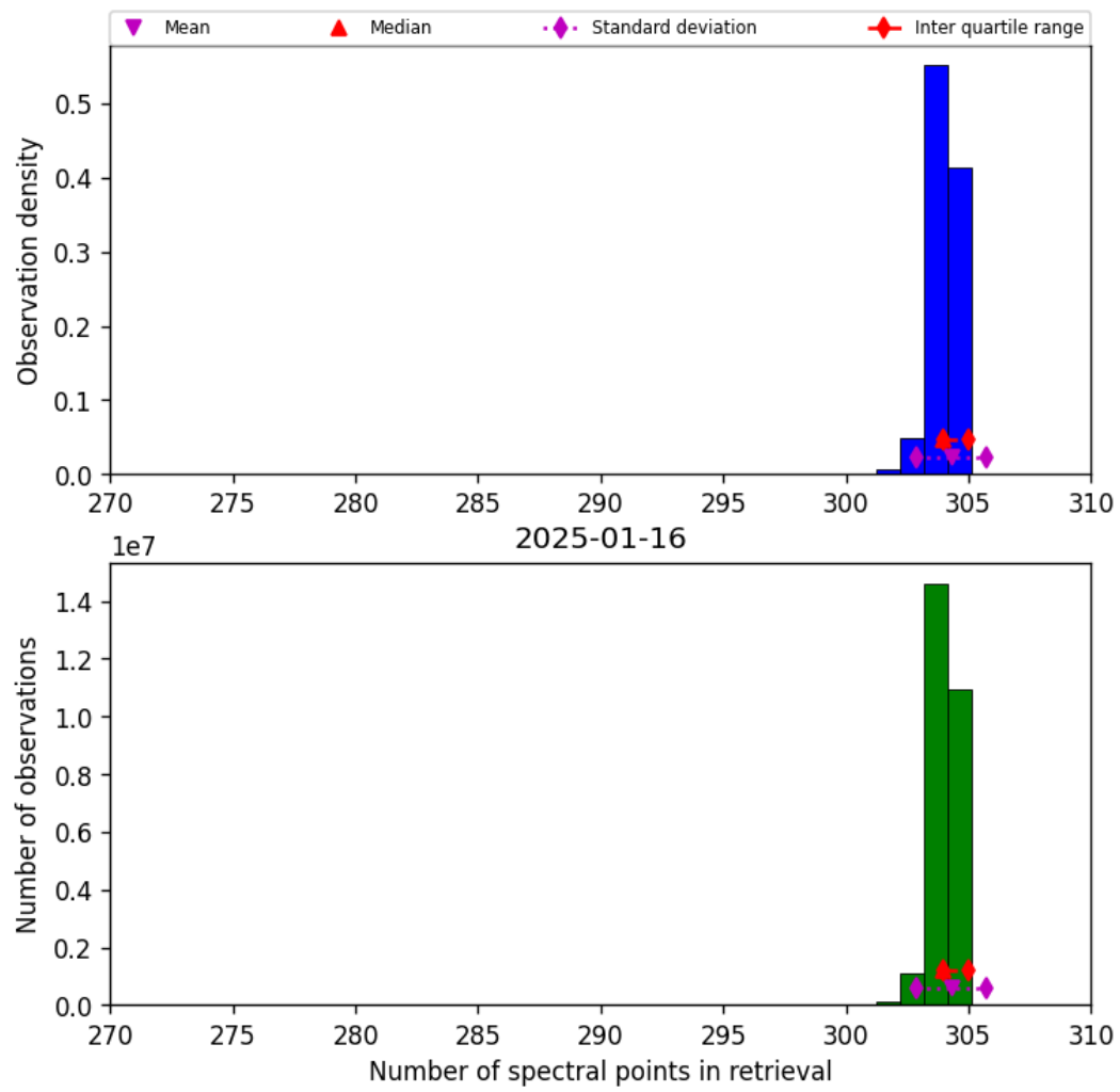
Figure 33: Histogram of “Number of spectral points in retrieval” for 2025-01-15 to 2025-01-17
