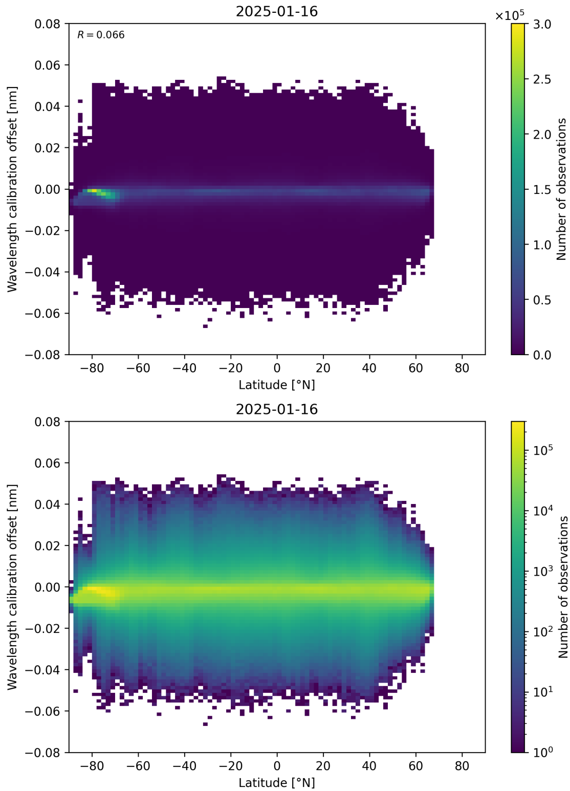
Figure 95: Scatter density plot of “Latitude” against “Wavelength calibration offset” for 2025-01-15 to 2025-01-17.
