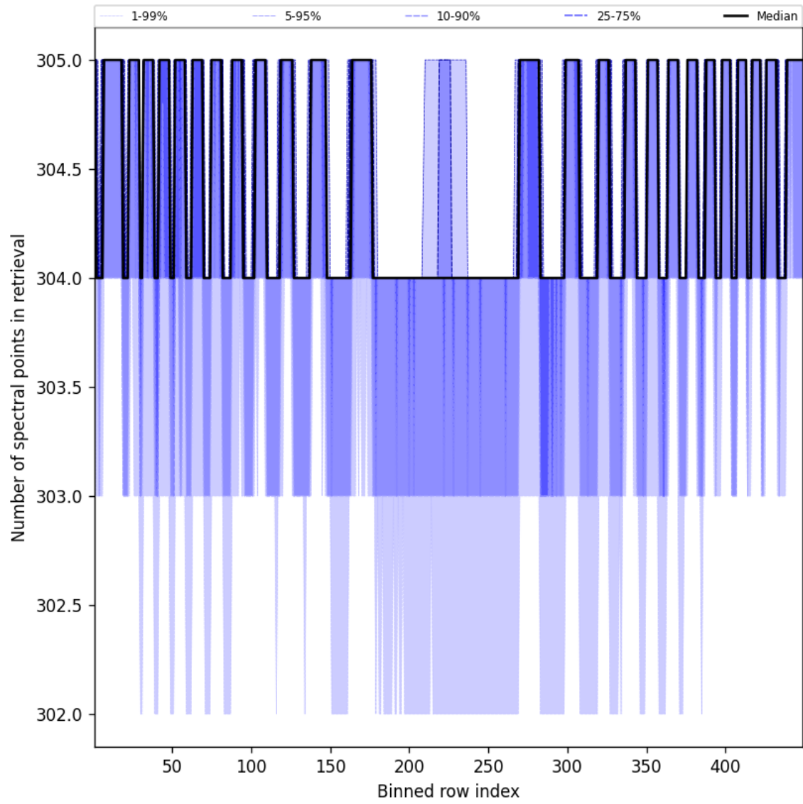
Figure 50: Along track statistics of “Number of spectral points in retrieval” for 2025-01-15 to 2025-01-17
