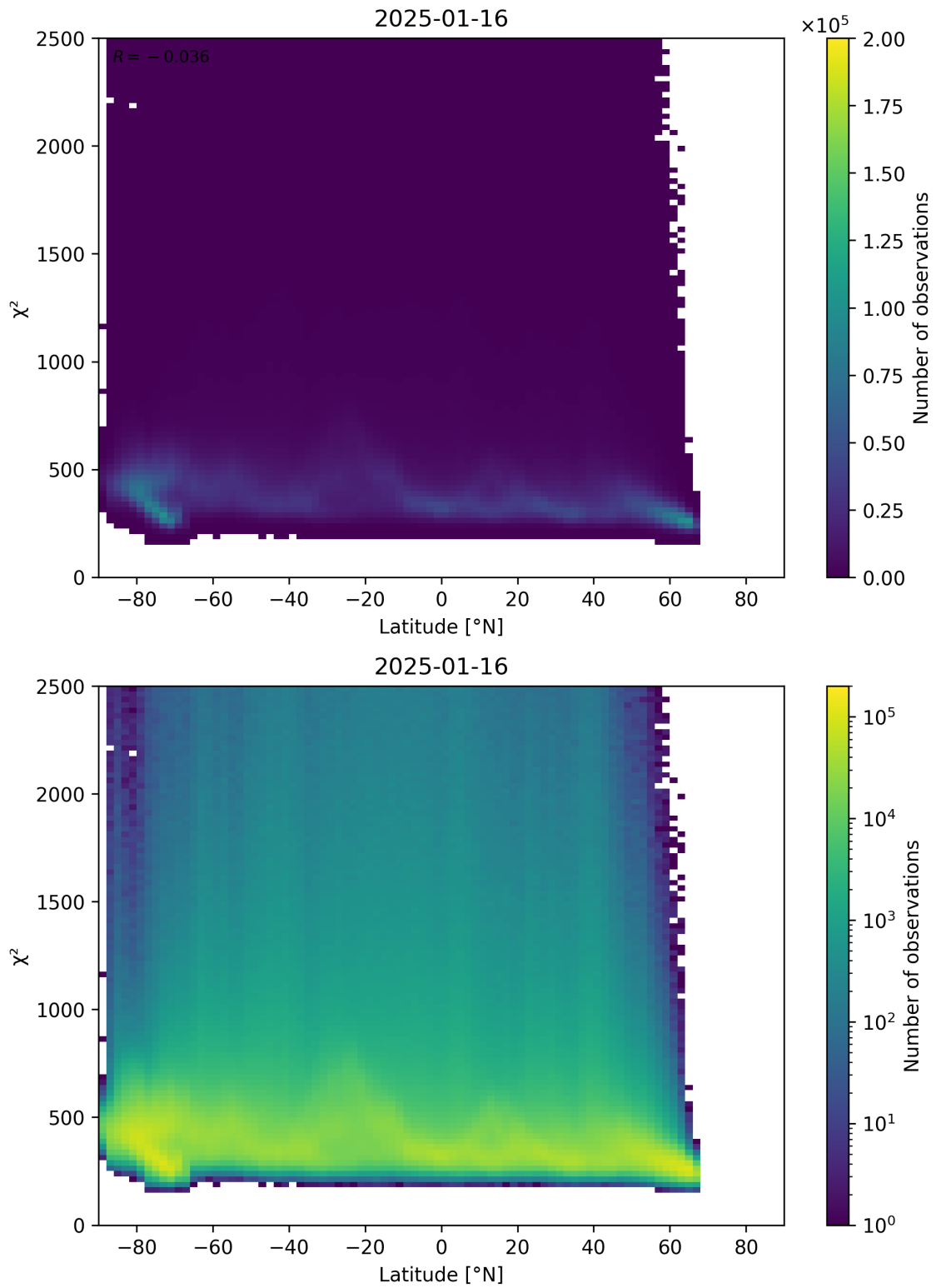
Figure 86: Scatter density plot of “Latitude” against “ \chi^2 ” for 2025-01-15 to 2025-01-17.
