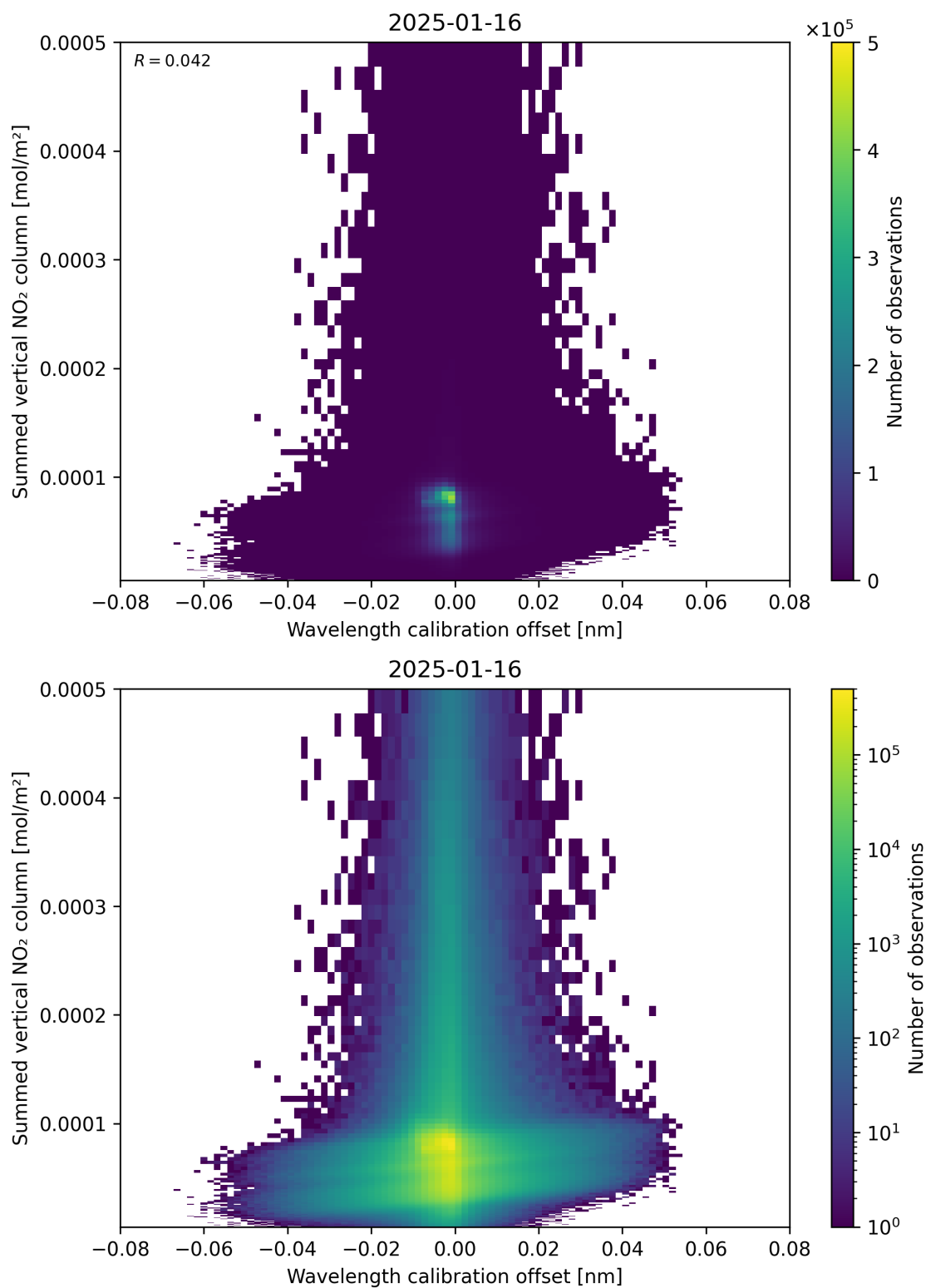
Figure 177: Scatter density plot of “Wavelength calibration offset” against “Summed vertical NO 2 column” for 2025-01-15 to 2025-01-17.
