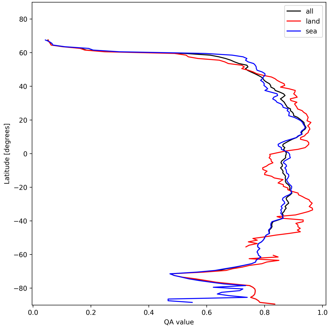
Figure 11: Zonal average of “QA value” for 2025-01-15 to 2025-01-17.
