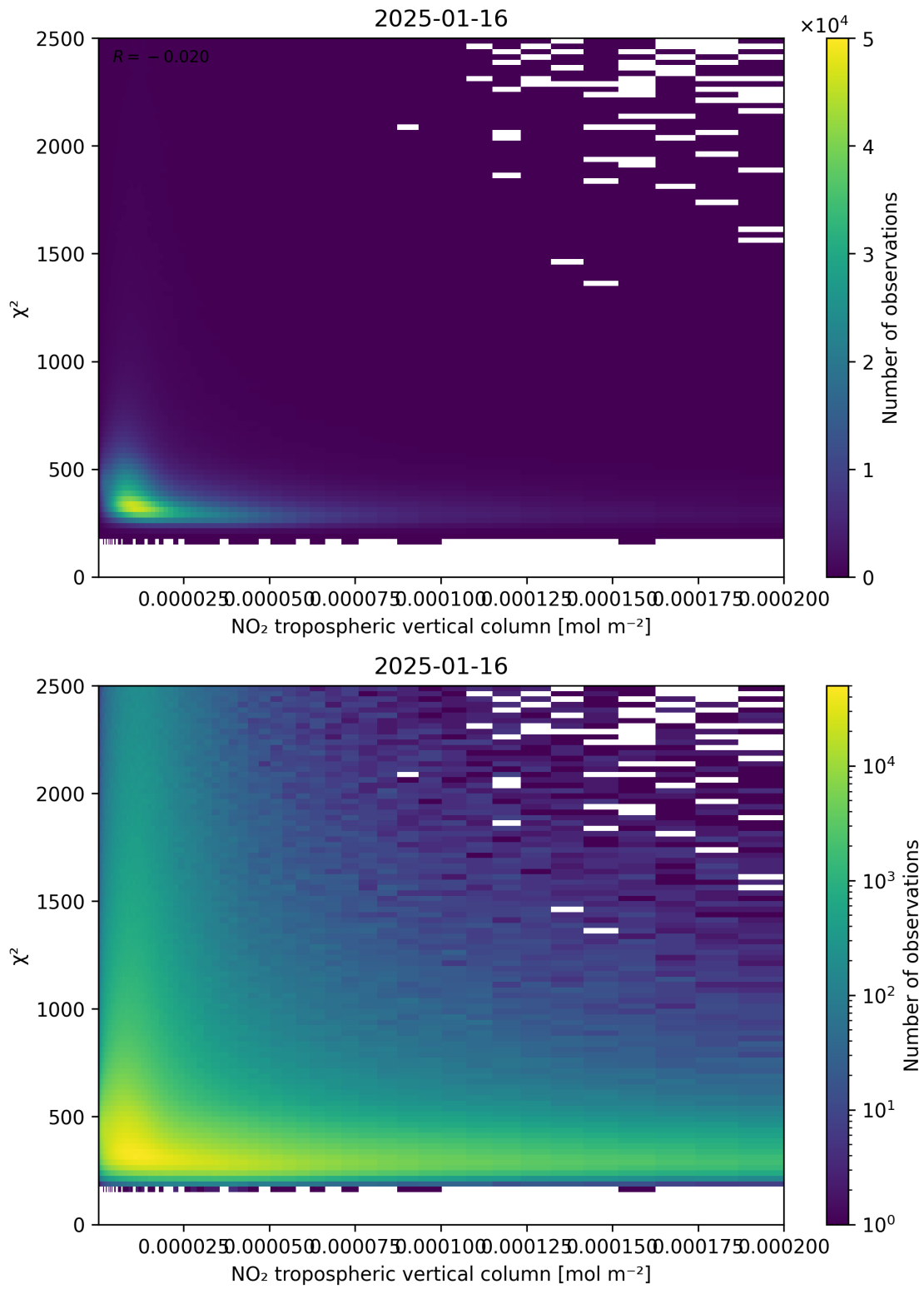
Figure 124: Scatter density plot of “NO 2 tropospheric vertical column” against “ \chi^2 ” for 2025-01-15 to 2025-01-17.
