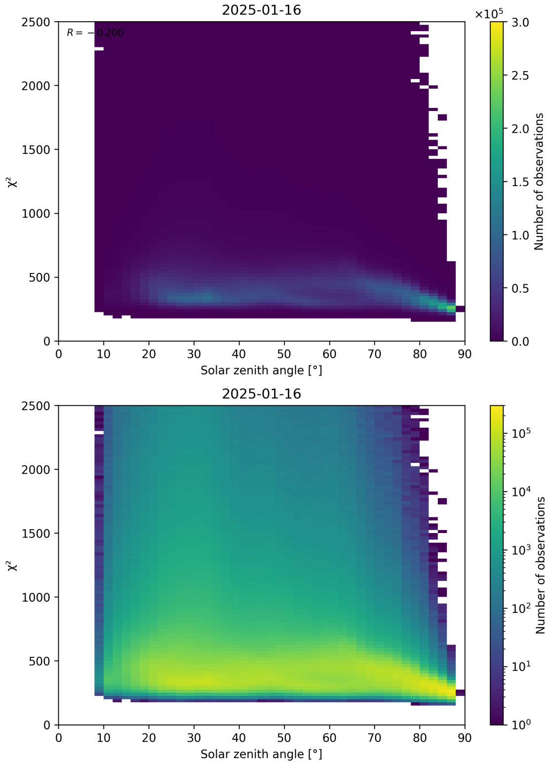
Figure 148: Scatter density plot of “Solar zenith angle” against “ \chi^2 ” for 2025-01-15 to 2025-01-17.
