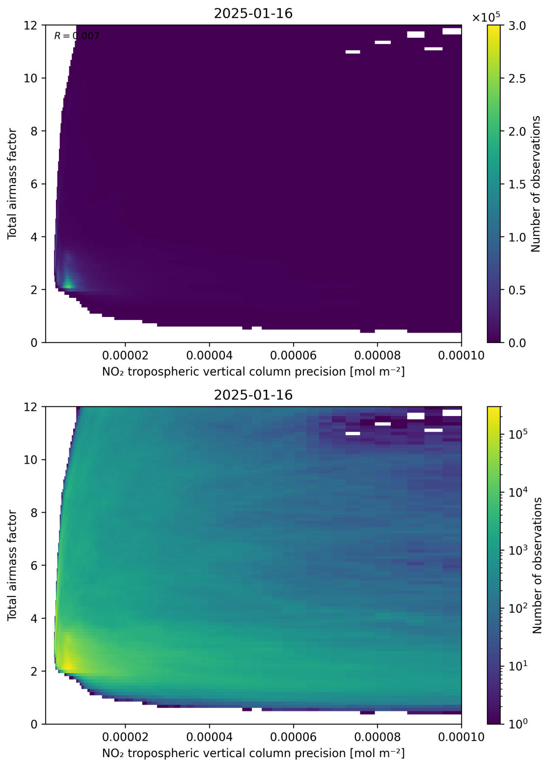
Figure 132: Scatter density plot of “NO 2 tropospheric vertical column precision” against “Total air mass factor” for 2025-01-15 to 2025-01-17.
