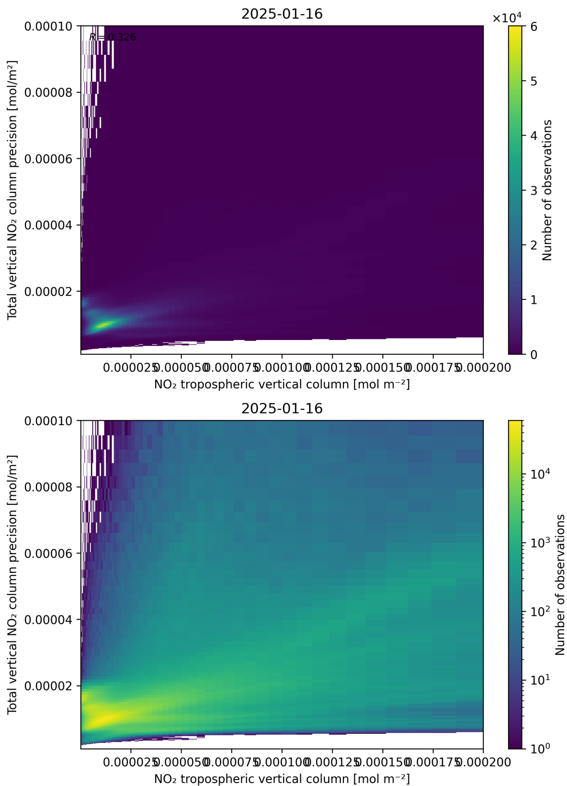
Figure 129: Scatter density plot of “NO 2 tropospheric vertical column” against “Total vertical NO 2 column precision” for 2025-01-15 to 2025-01-17.
