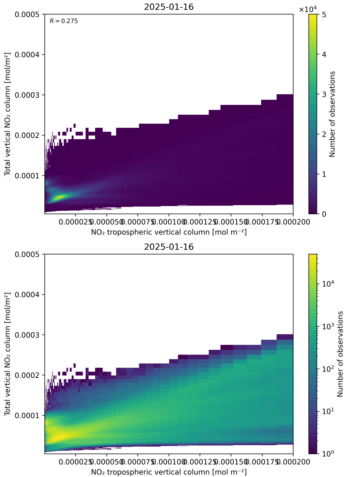
Figure 128: Scatter density plot of “NO 2 tropospheric vertical column” against “Total vertical NO 2 column” for 2025-01-15 to 2025-01-17.
