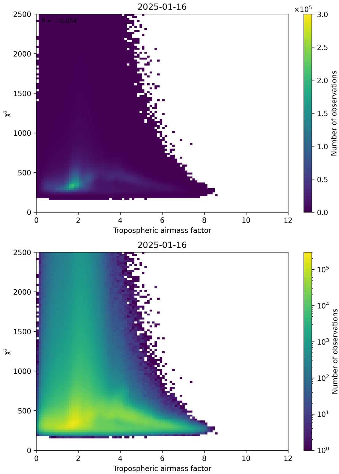
Figure 73: Scatter density plot of “Tropospheric airmass factor” against “ \chi^2 ” for 2025-01-15 to 2025-01-17.
