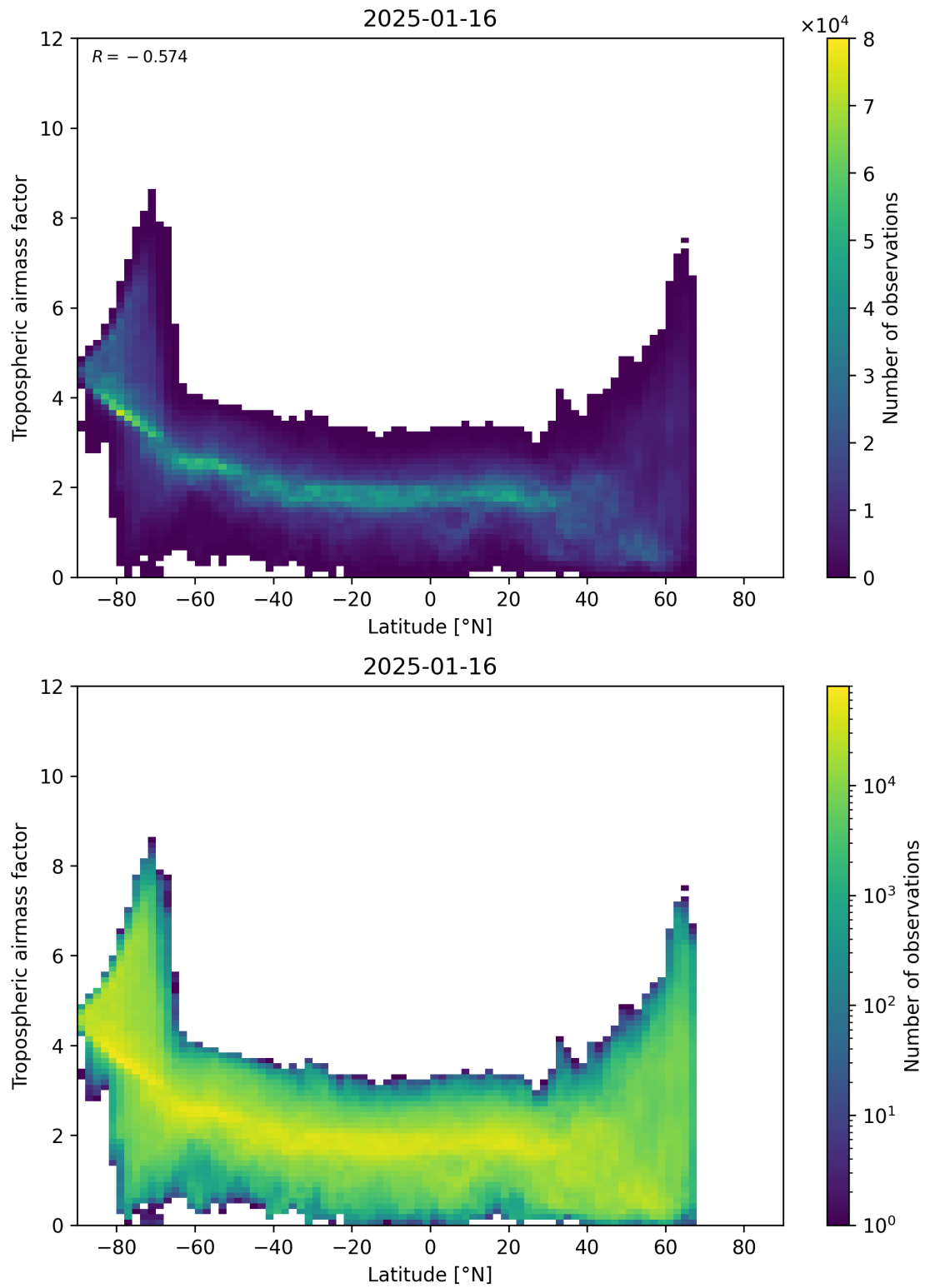
Figure 85: Scatter density plot of “Latitude” against “Tropospheric airmass factor” for 2025-01-15 to 2025-01-17.
