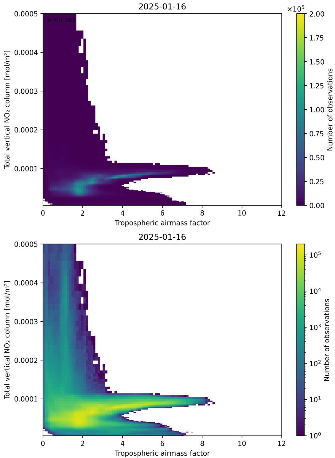
Figure 77: Scatter density plot of “Tropospheric airmass factor” against “Total vertical NO 2 column” for 2025-01-15 to 2025-01-17.
