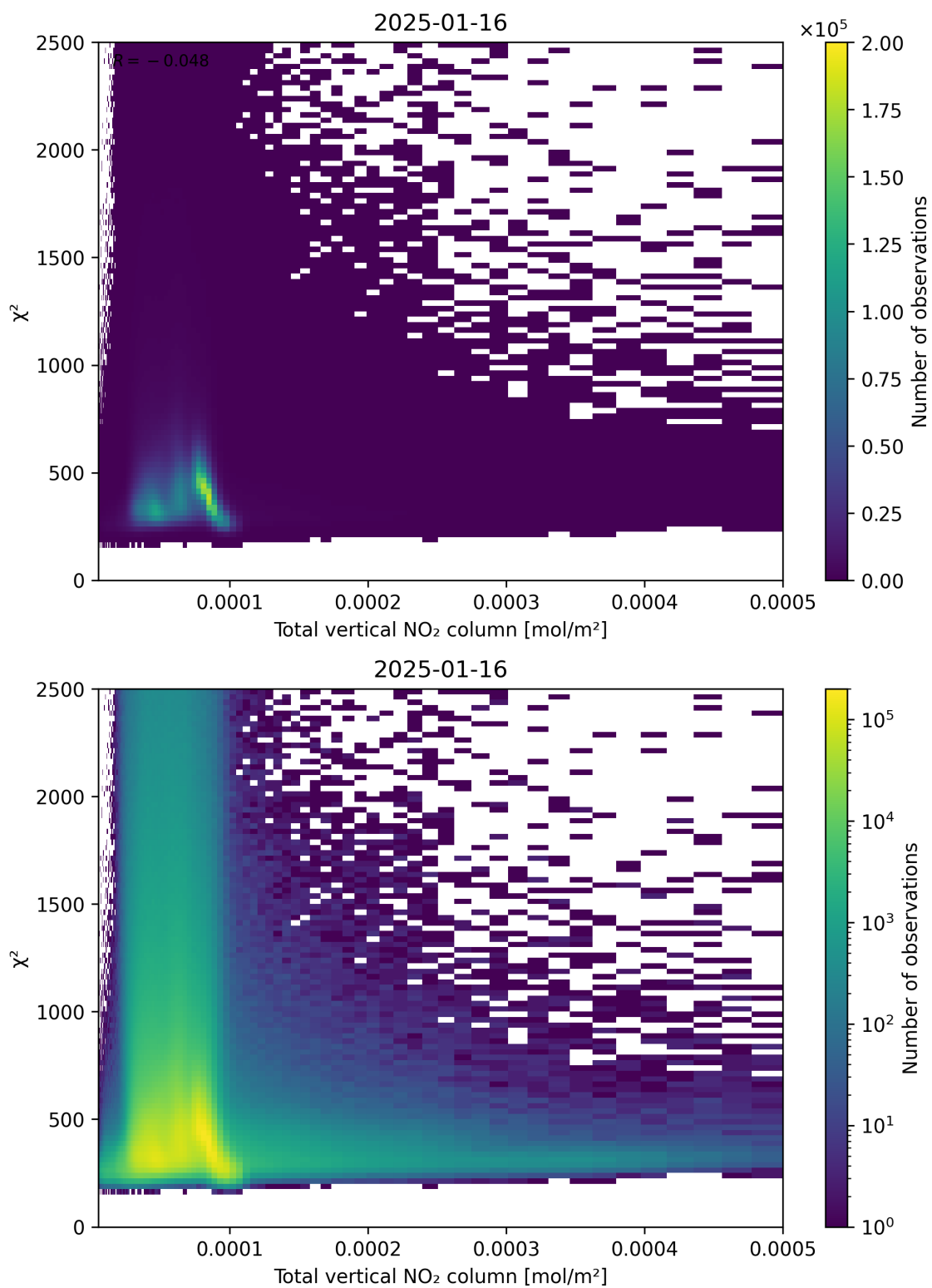
Figure 111: Scatter density plot of “Total vertical NO 2 column” against “ \chi^2 ” for 2025-01-15 to 2025-01-17.
