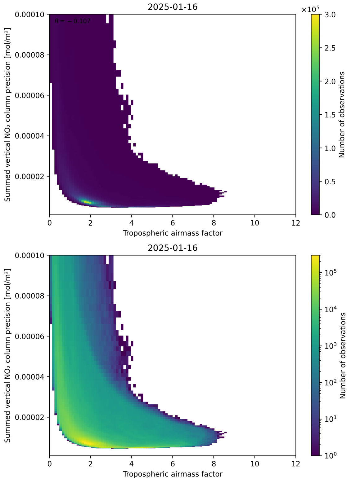
Figure 76: Scatter density plot of “Tropospheric air mass factor” against “Summed vertical NO 2 column precision” for 2025-01-15 to 2025-01-17.
