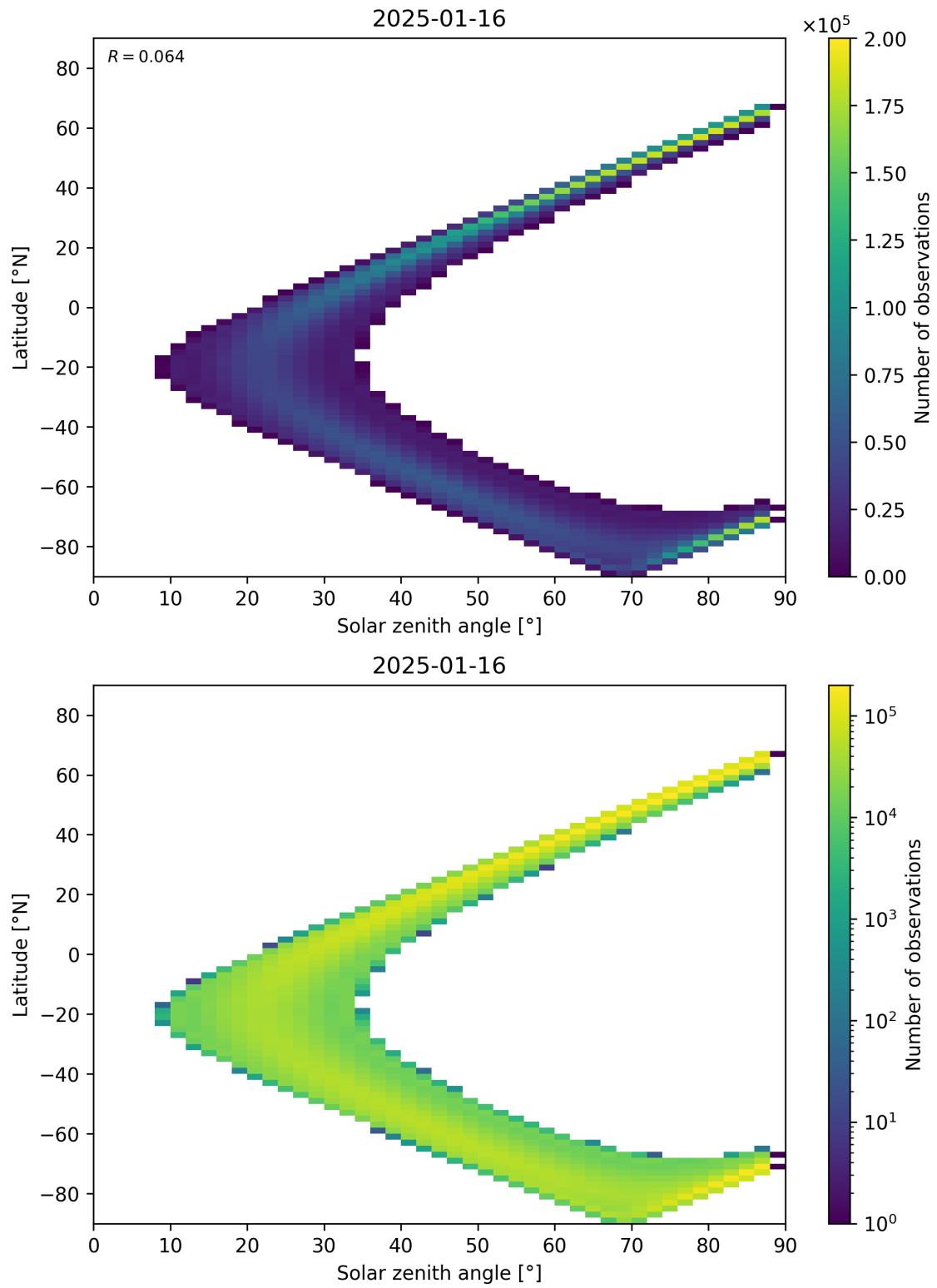
Figure 149: Scatter density plot of “Solar zenith angle” against “Latitude” for 2025-01-15 to 2025-01-17.
