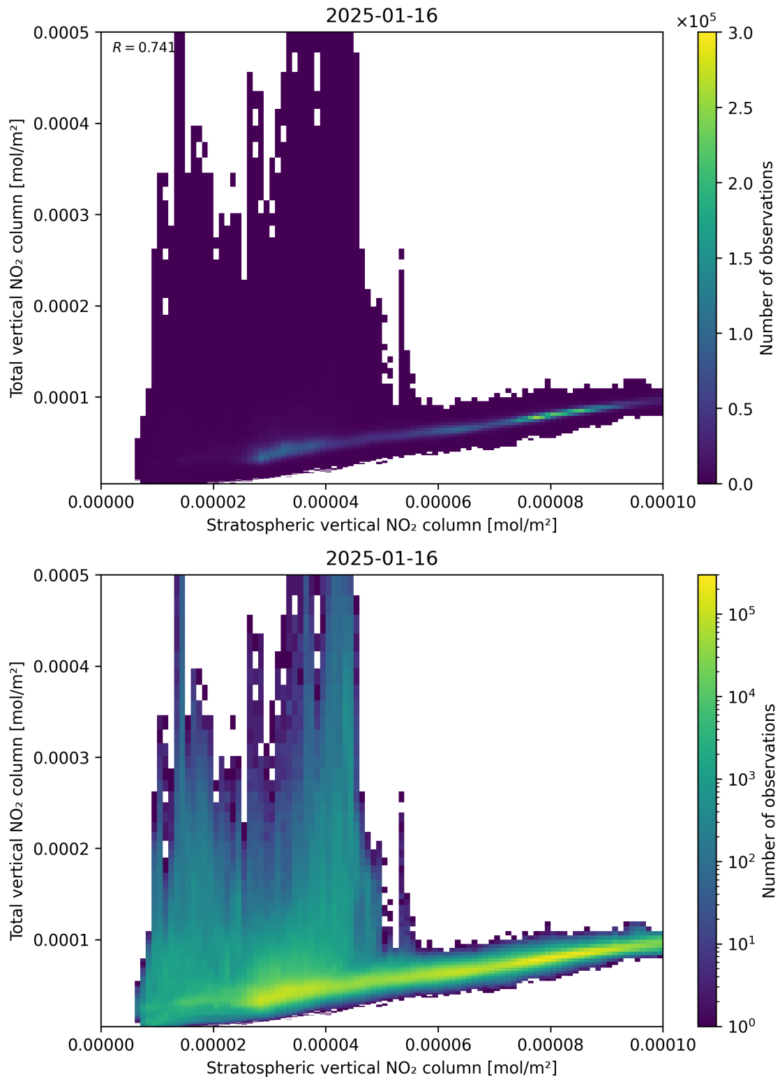
Figure 100: Scatter density plot of “Stratospheric vertical NO 2 column” against “Total vertical NO 2 column” for 2025-01-15 to 2025-01-17.
