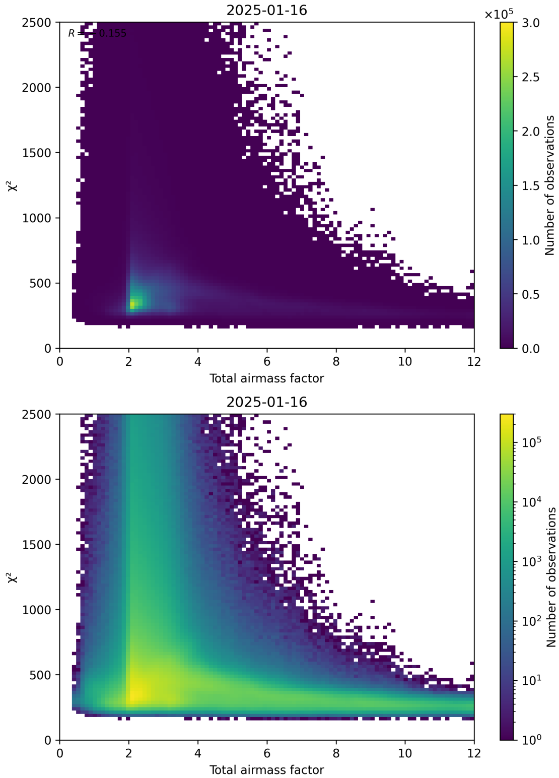
Figure 63: Scatter density plot of “Total airmass factor” against “ \chi^2 ” for 2025-01-15 to 2025-01-17.
