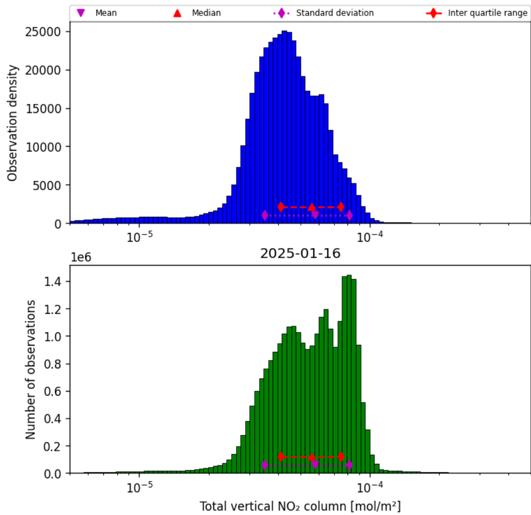
Figure 38: Histogram of "Total vertical NO 2 column" for 2025-01-15 to 2025-01-17
