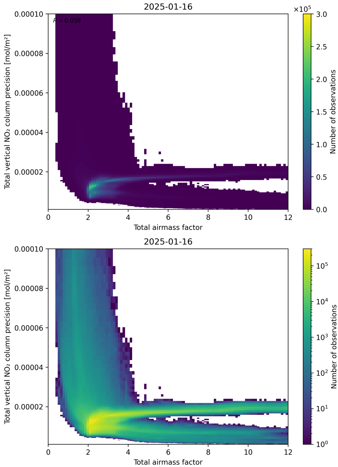
Figure 68: Scatter density plot of “Total airmass factor” against “Total vertical NO 2 column precision” for 2025-01-15 to 2025-01-17.
