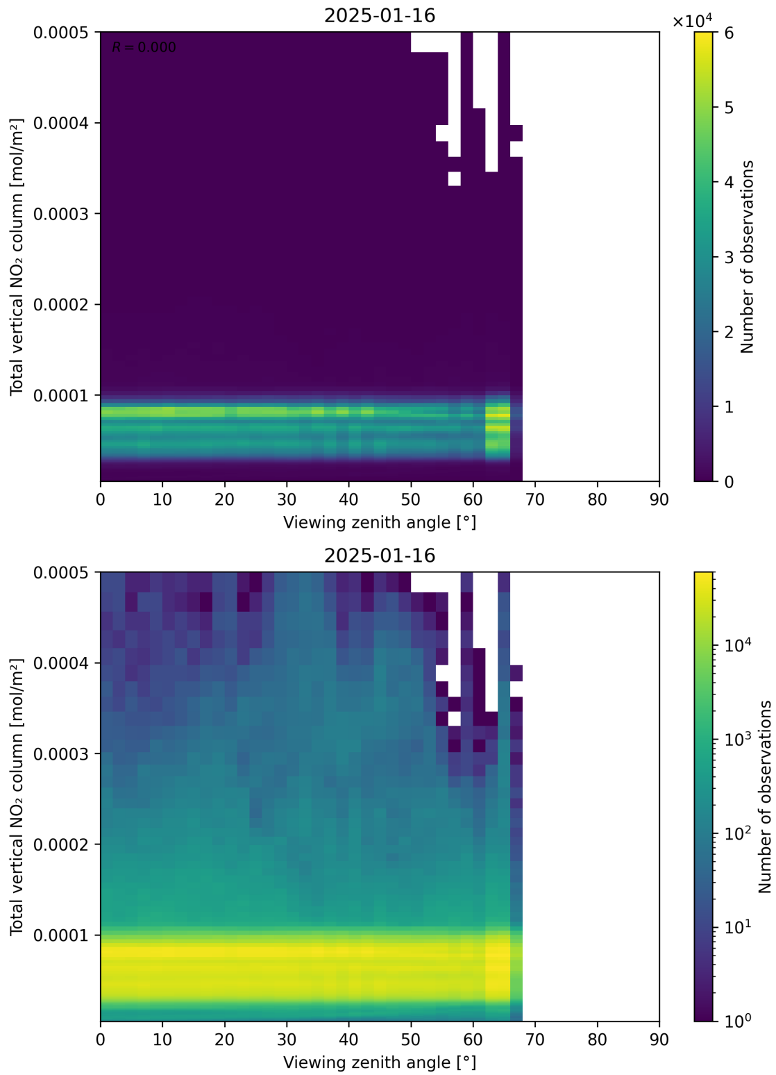
Figure 167: Scatter density plot of “Viewing zenith angle” against “Total vertical NO 2 column” for 2025-01-15 to 2025-01-17.
