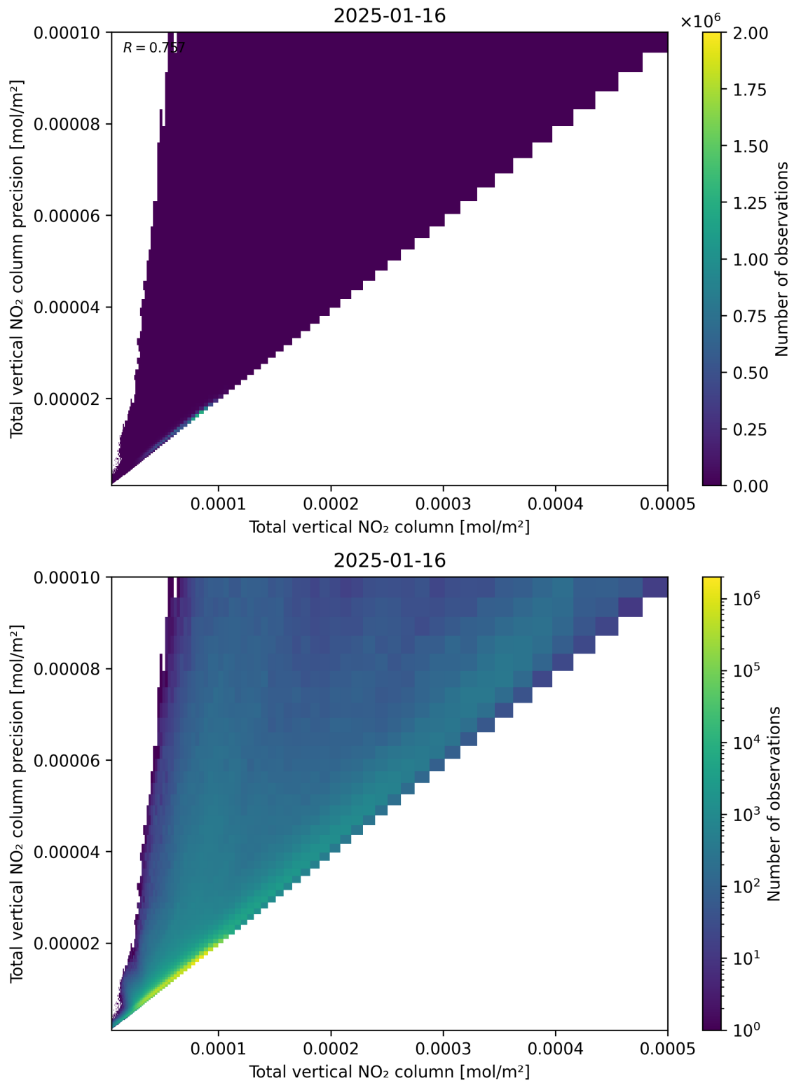
Figure 114: Scatter density plot of “Total vertical NO 2 column” against “Total vertical NO 2 column precision” for 2025-01-15 to 2025-01-17.
