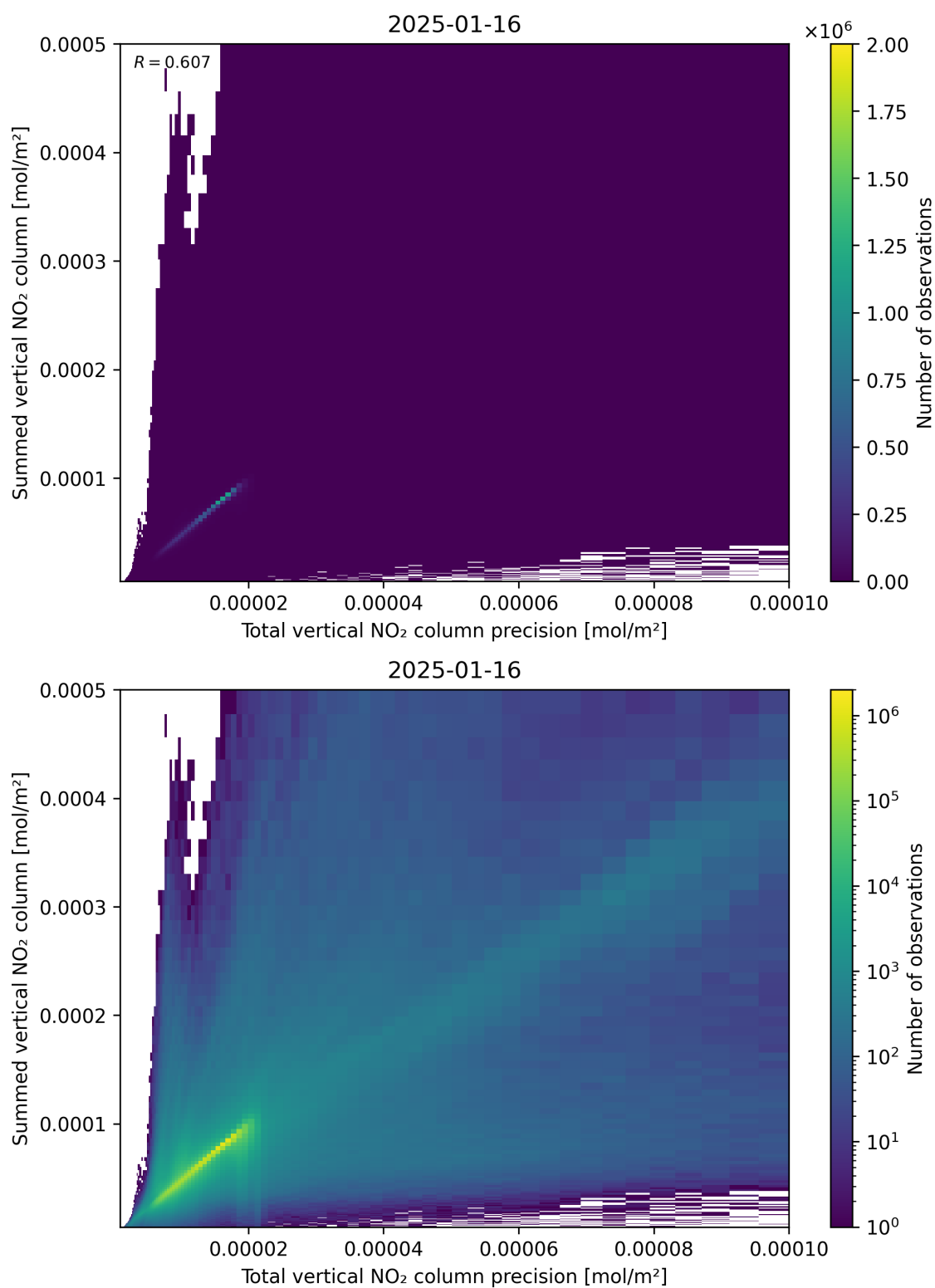
Figure 117: Scatter density plot of “Total vertical NO 2 column precision” against “Summed vertical NO 2 column” for 2025-01-15 to 2025-01-17.
