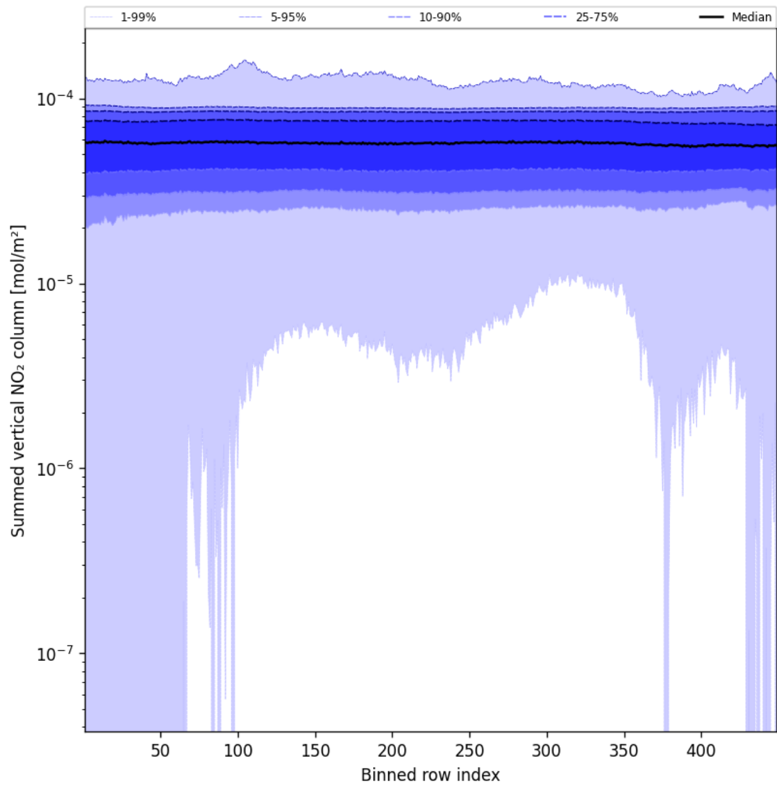
Figure 57: Along track statistics of “Summed vertical NO 2 column” for 2025-01-15 to 2025-01-17
