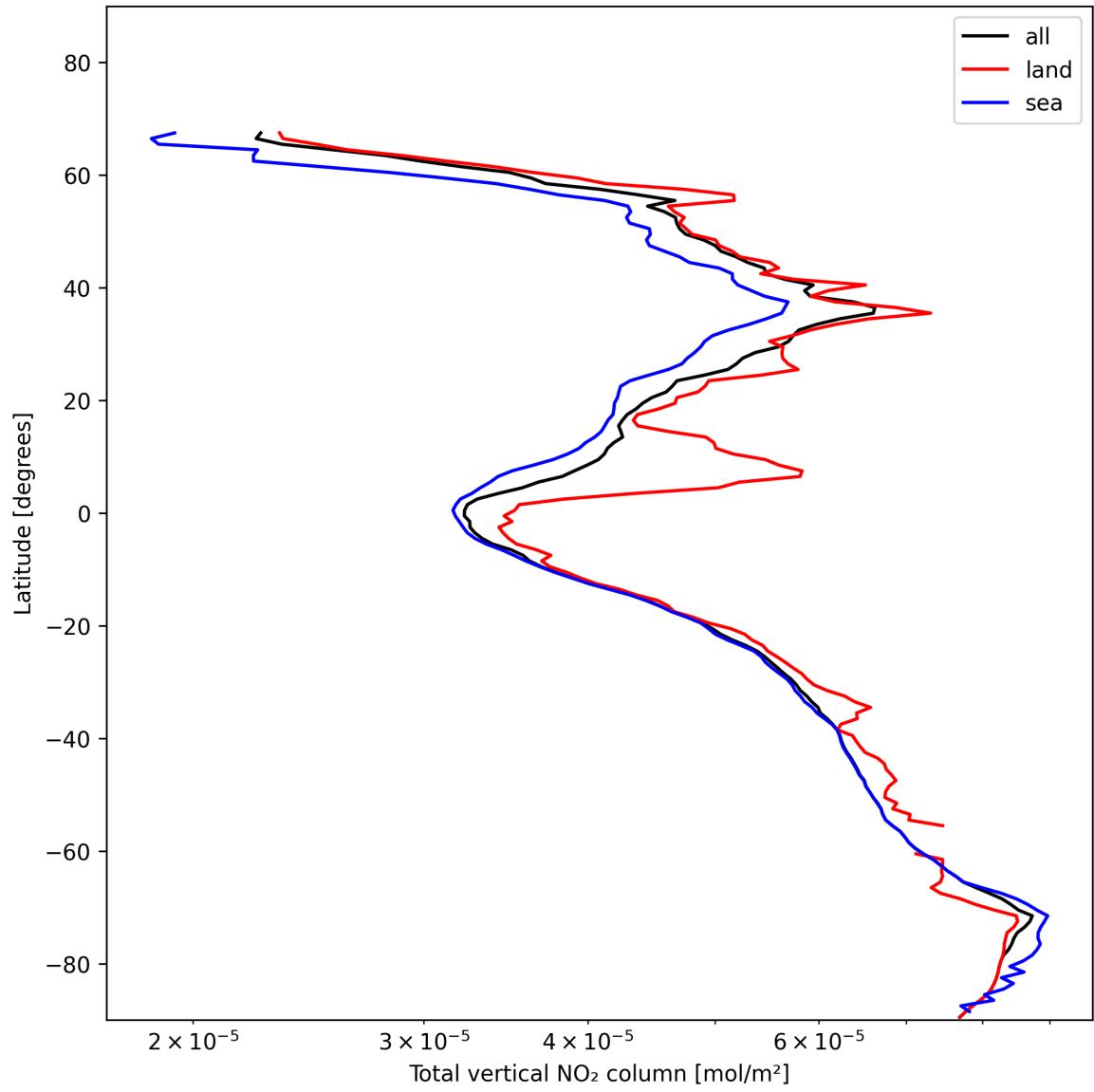
Figure 21: Zonal average of “Total vertical NO 2 column” for 2025-01-15 to 2025-01-17.
