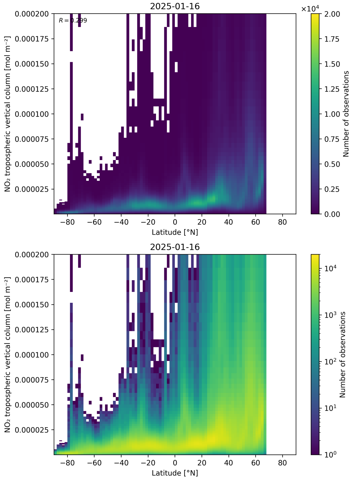
Figure 92: Scatter density plot of “Latitude” against “NO 2 tropospheric vertical column” for 2025-01-15 to 2025-01-17.
