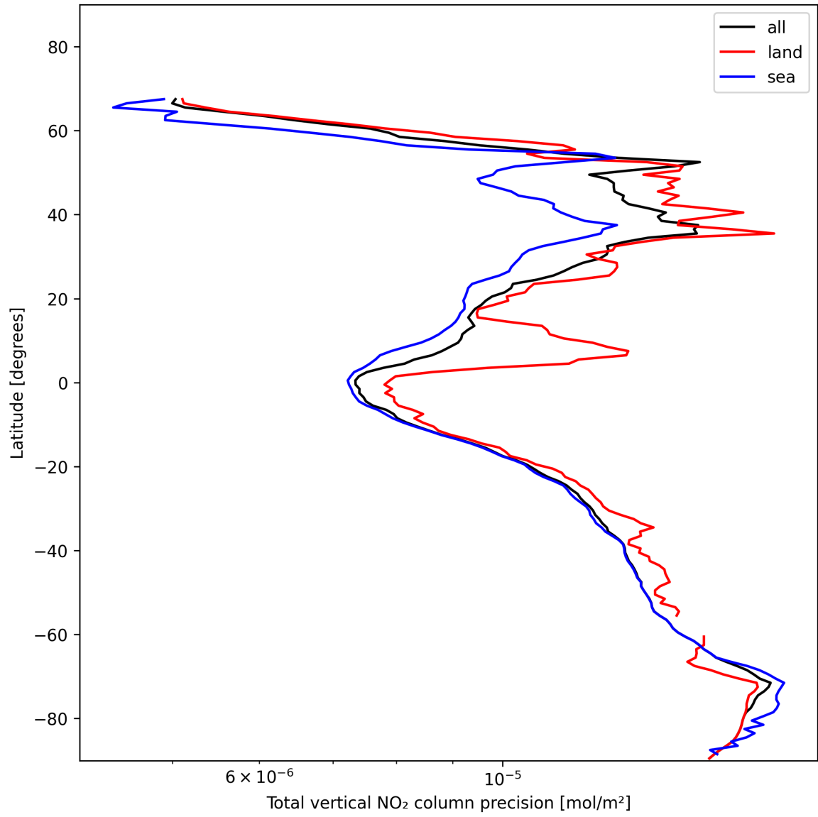
Figure 22: Zonal average of "Total vertical NO 2 column precision" for 2025-01-15 to 2025-01-17.
