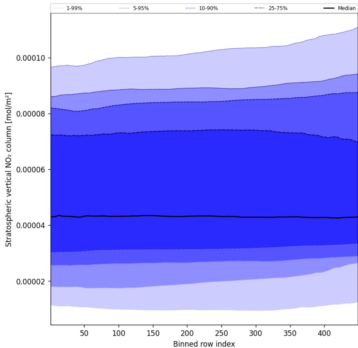
Figure 53: Along track statistics of “Stratospheric vertical NO 2 column” for 2025-01-15 to 2025-01-17
