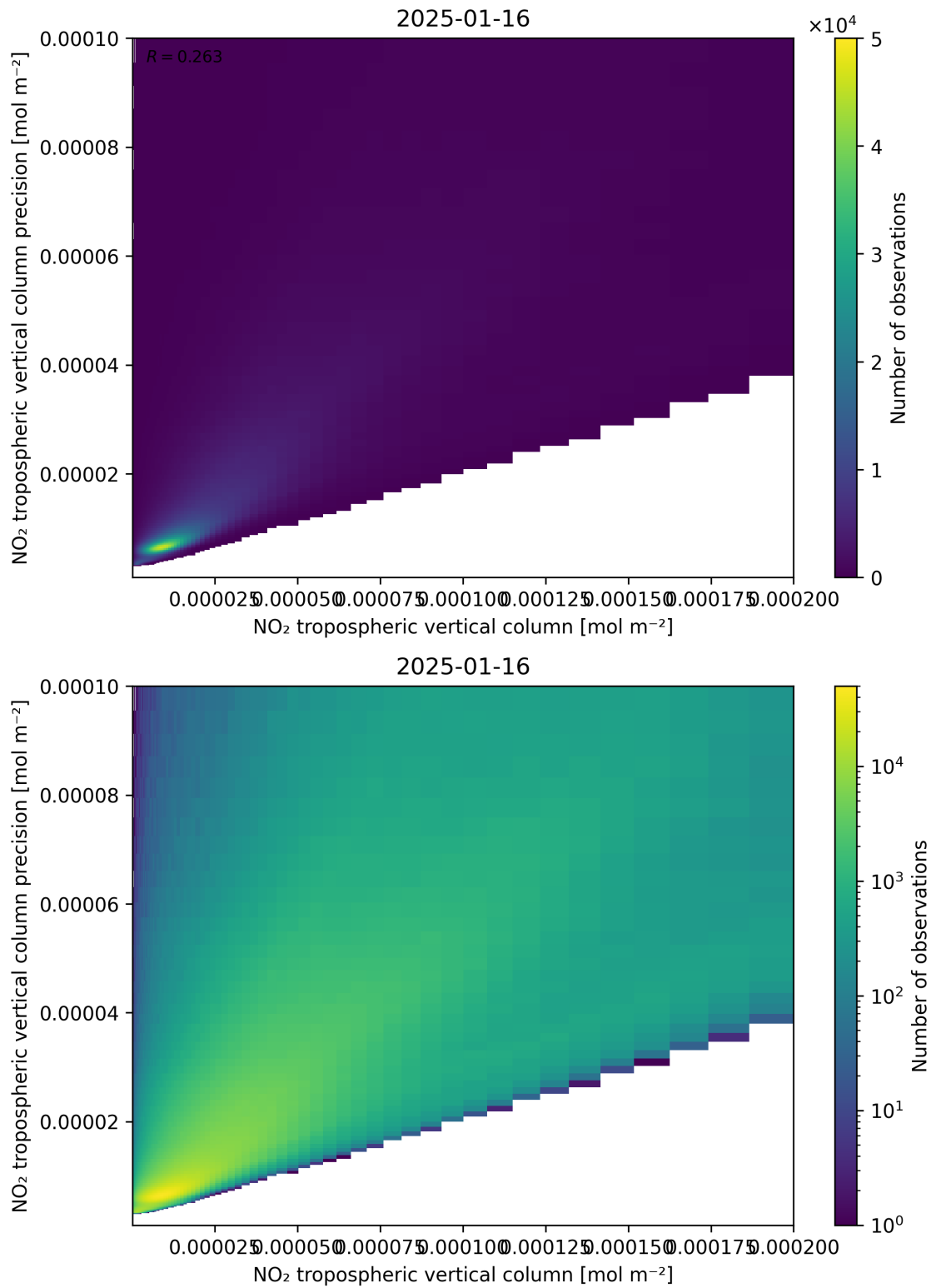
Figure 130: Scatter density plot of “NO 2 tropospheric vertical column” against “NO 2 tropospheric vertical column precision” for 2025-01-15 to 2025-01-17.
