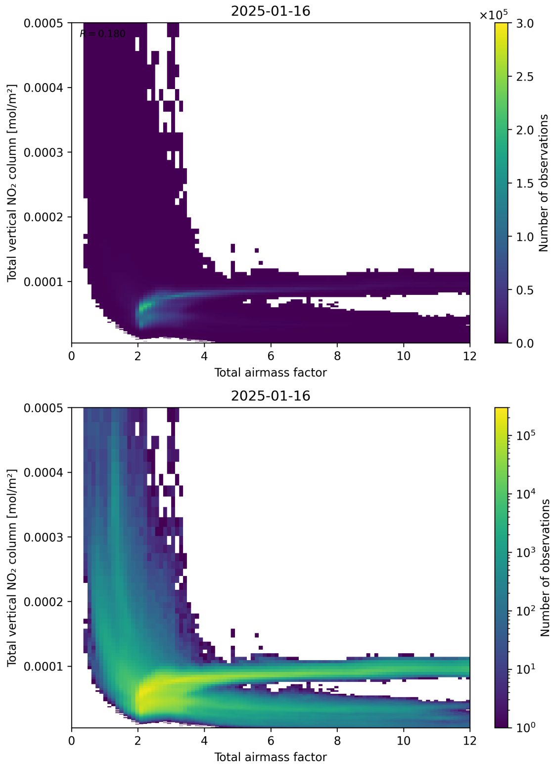
Figure 67: Scatter density plot of “Total air mass factor” against “Total vertical NO 2 column” for 2025-01-15 to 2025-01-17.
