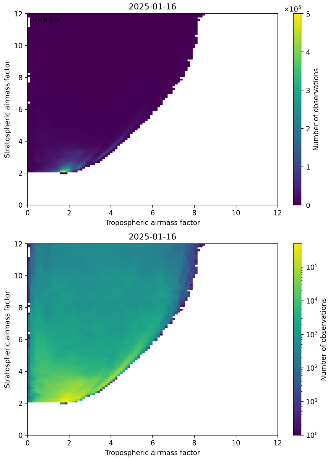
Figure 71: Scatter density plot of “Tropospheric airmass factor” against “Stratospheric airmass factor” for 2025-01-15 to 2025-01-17.
