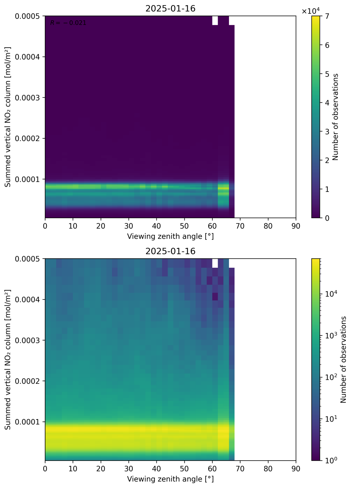
Figure 165: Scatter density plot of “Viewing zenith angle” against “Summed vertical NO 2 column” for 2025-01-15 to 2025-01-17.
