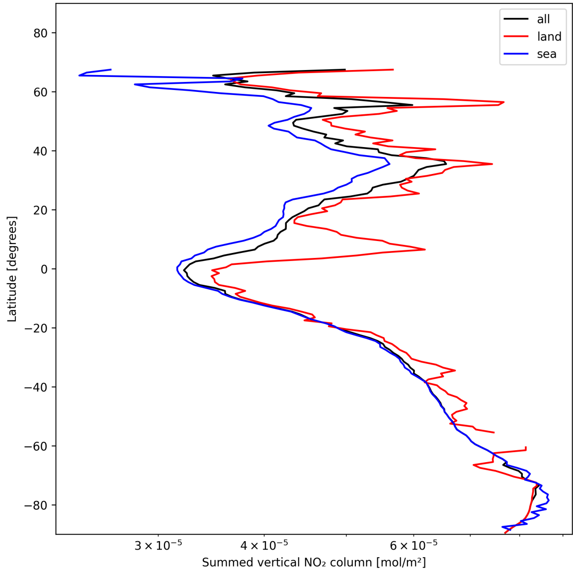
Figure 23: Zonal average of “Summed vertical NO 2 column” for 2025-01-15 to 2025-01-17.
