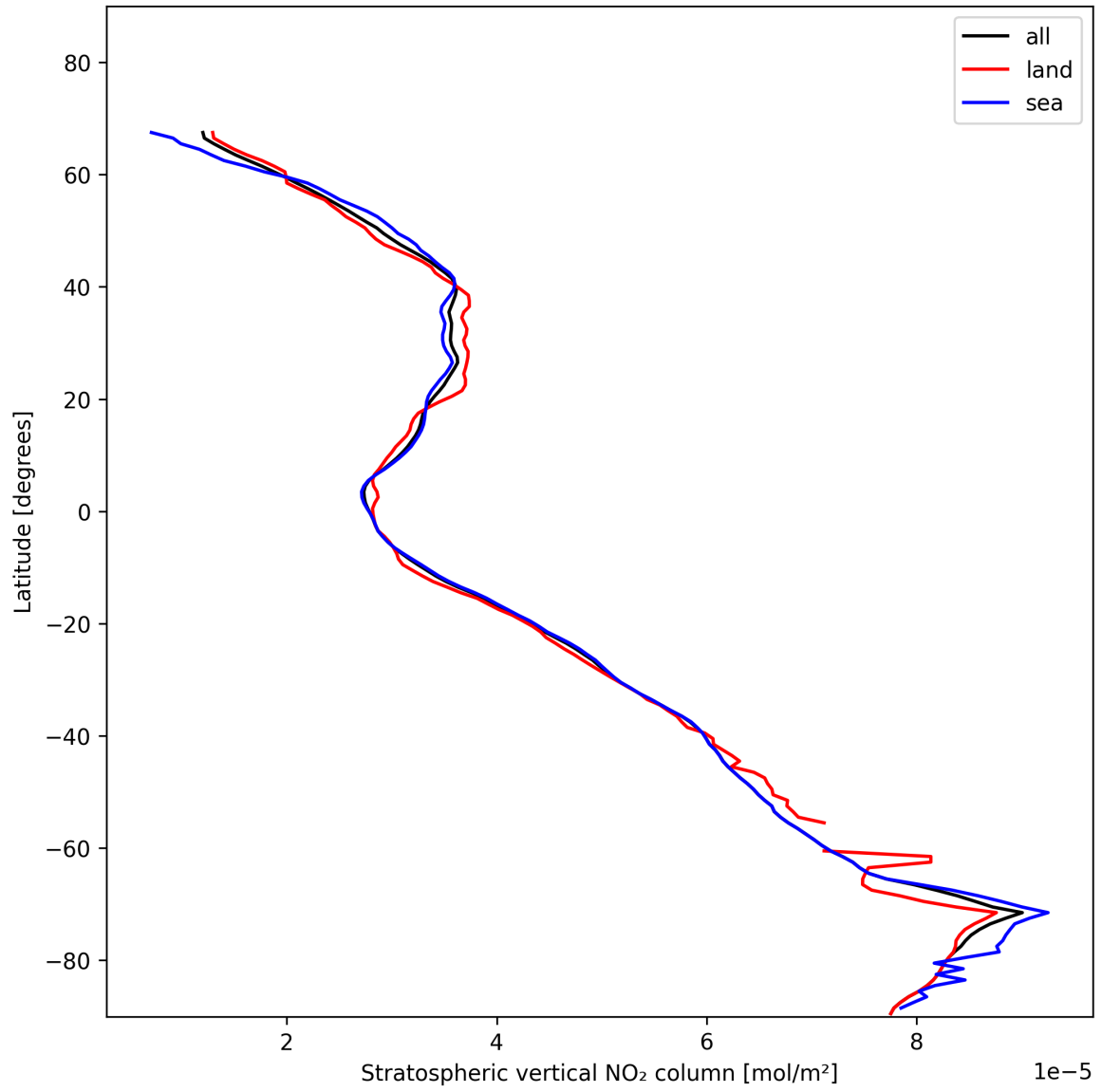
Figure 19: Zonal average of “Stratospheric vertical NO 2 column” for 2025-01-15 to 2025-01-17.
