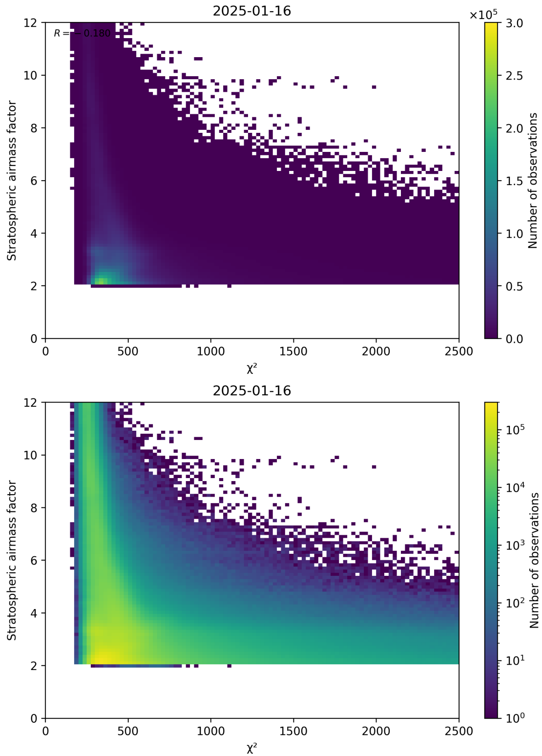
Figure 81: Scatter density plot of “ \chi^2 ” against “Stratospheric airmass factor” for 2025-01-15 to 2025-01-17.
