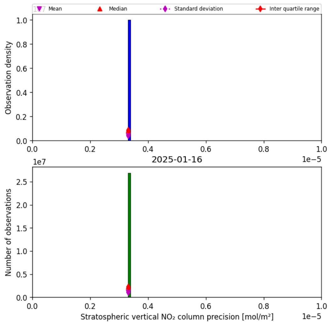
Figure 37: Histogram of “Stratospheric vertical NO 2 column precision” for 2025-01-15 to 2025-01-17
