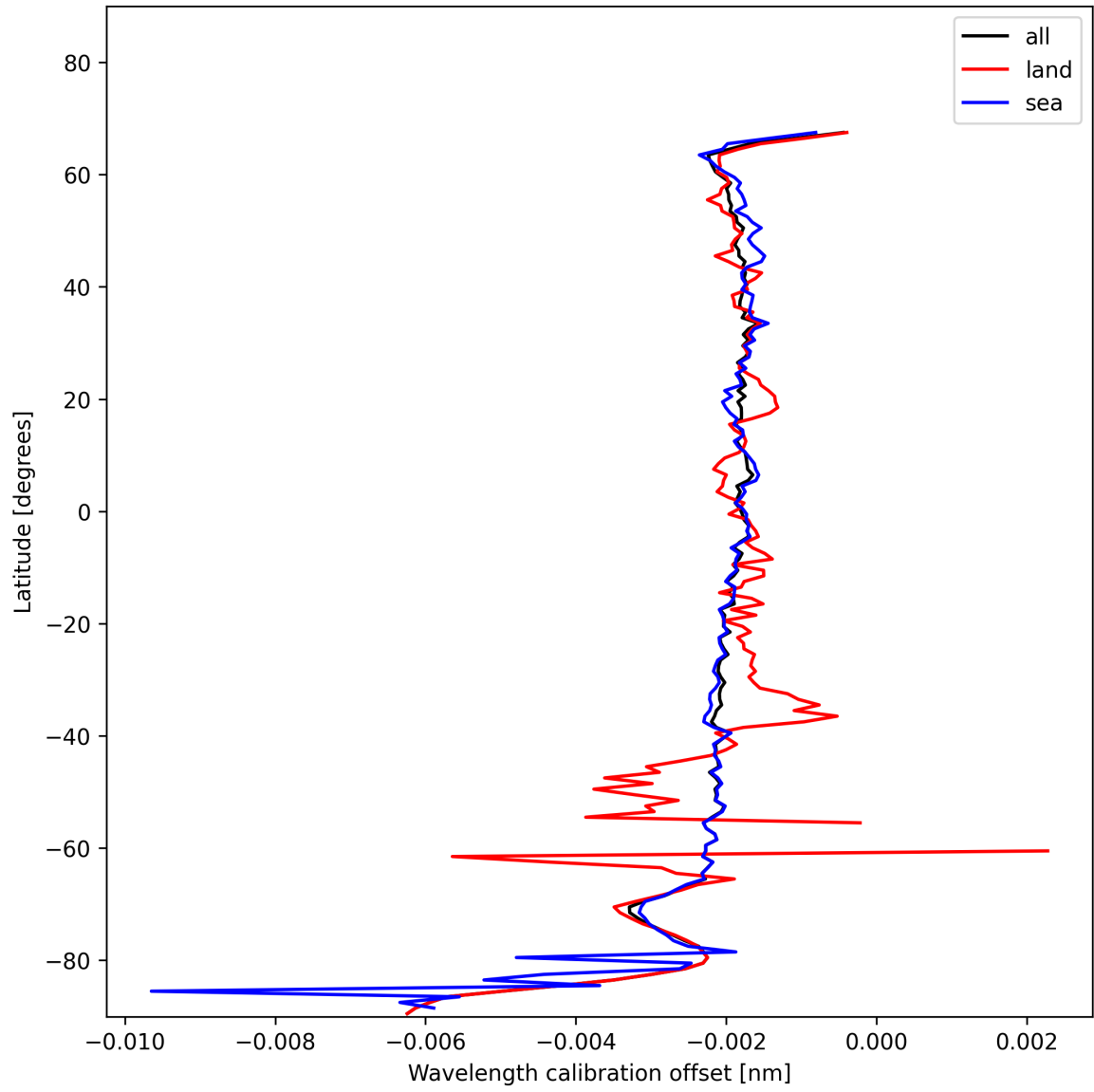
Figure 18: Zonal average of “Wavelength calibration offset” for 2025-01-15 to 2025-01-17.
