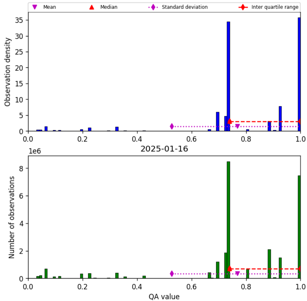
Figure 28: Histogram of “QA value” for 2025-01-15 to 2025-01-17
