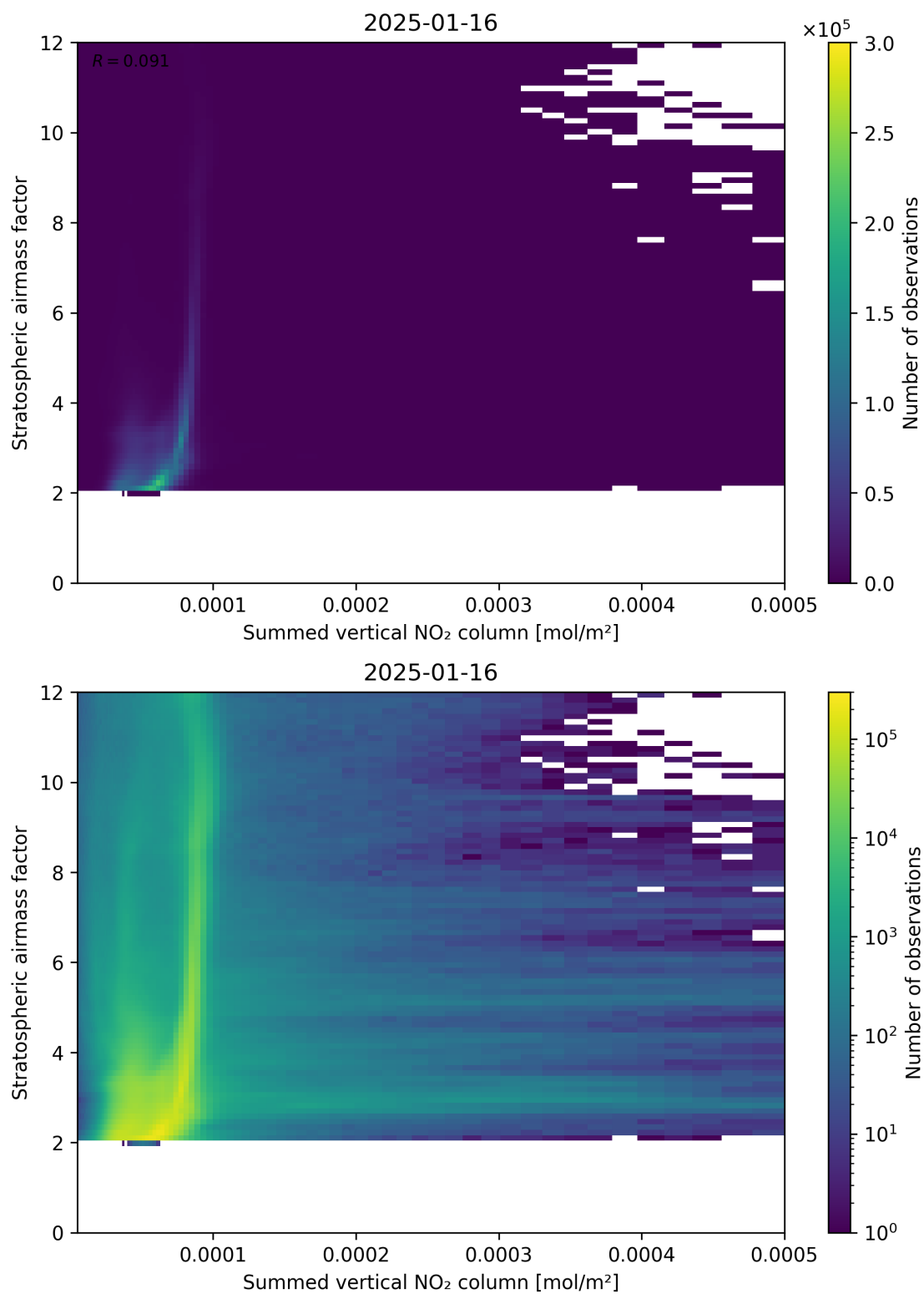
Figure 103: Scatter density plot of “Summed vertical NO 2 column” against “Stratospheric airmass factor” for 2025-01-15 to 2025-01-17.
