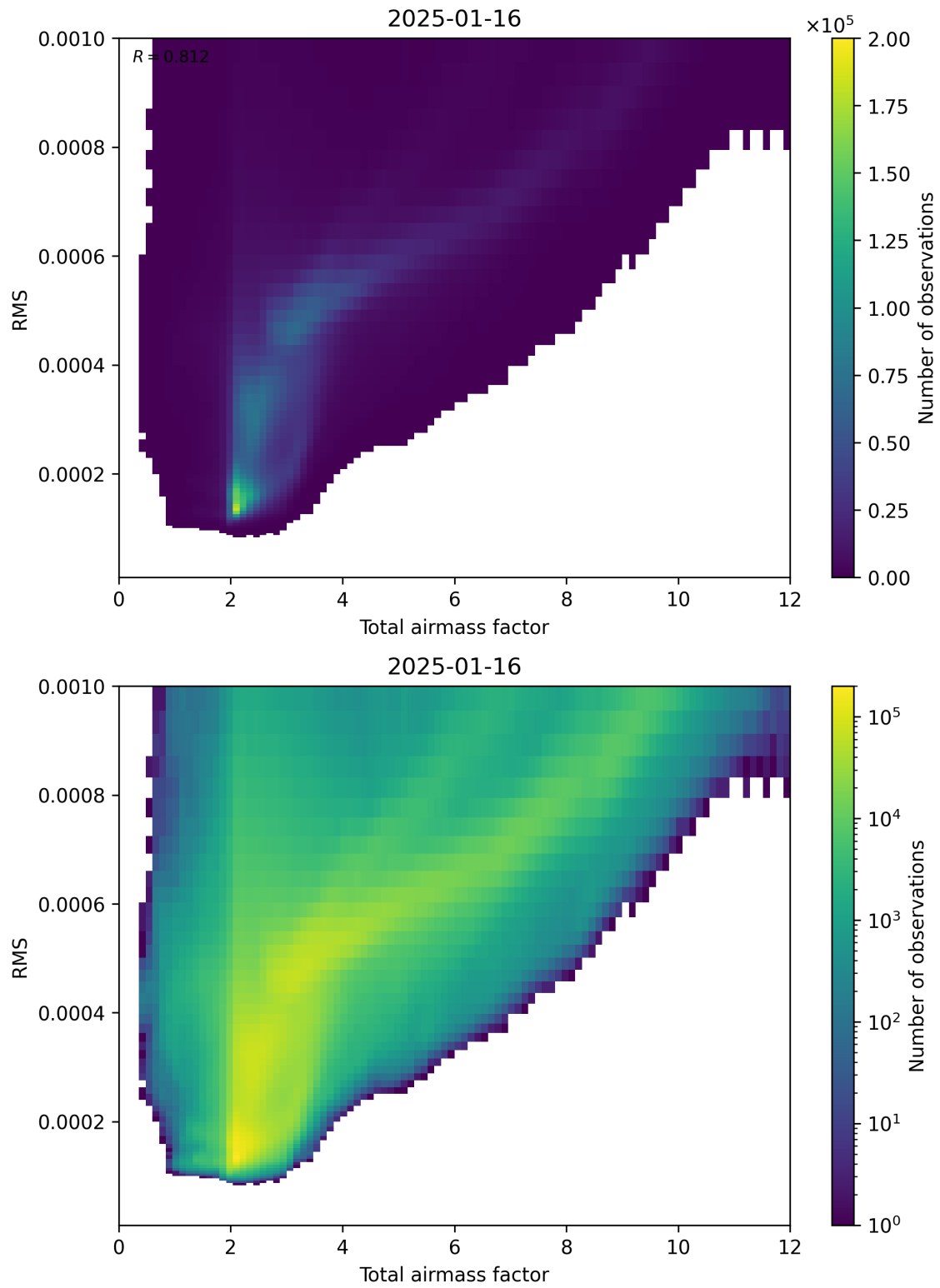
Figure 69: Scatter density plot of “Total airmass factor” against “RMS” for 2025-01-15 to 2025-01-17.
