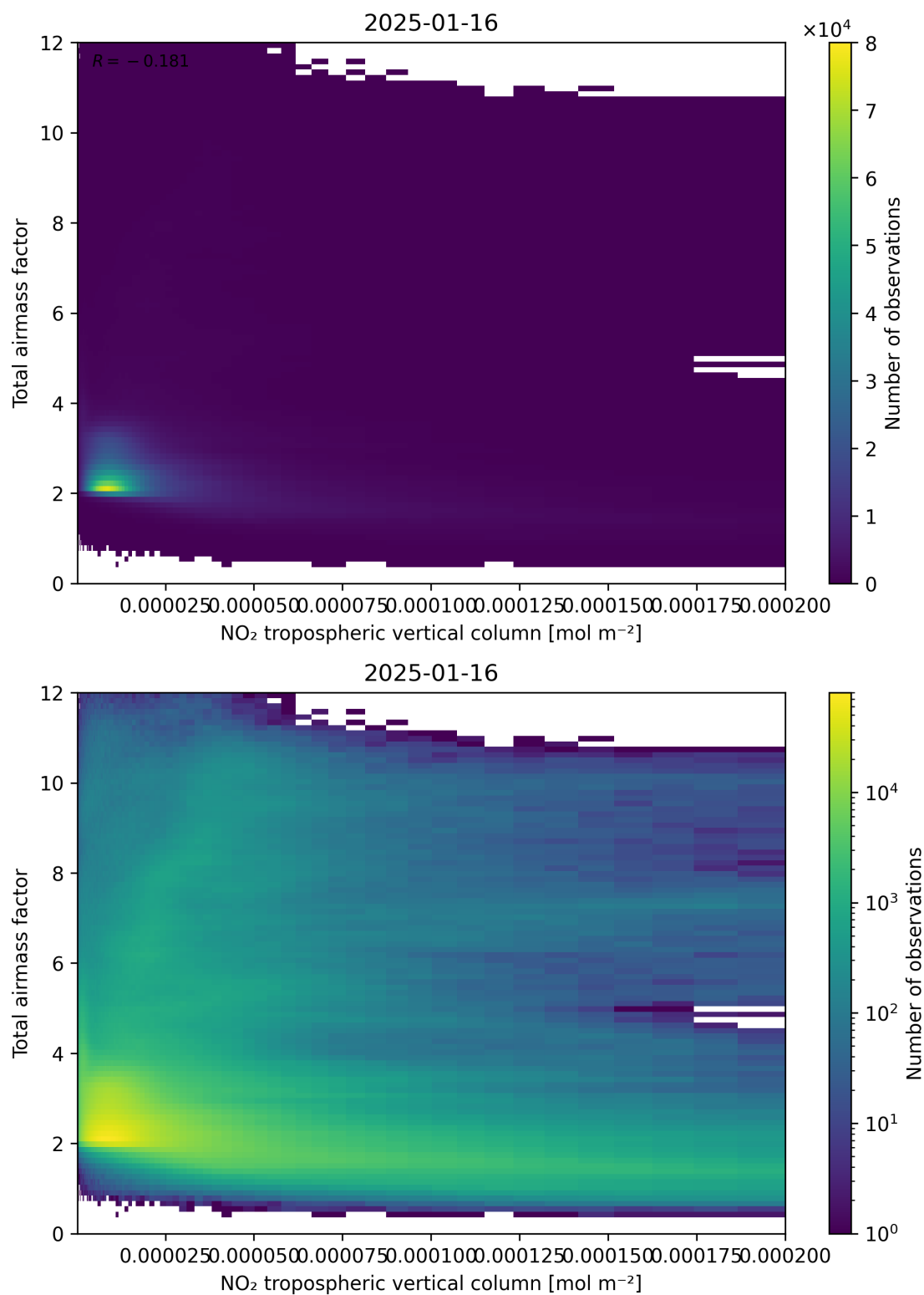
Figure 122: Scatter density plot of “NO 2 tropospheric vertical column” against “Total air mass factor” for 2025-01-15 to 2025-01-17.
