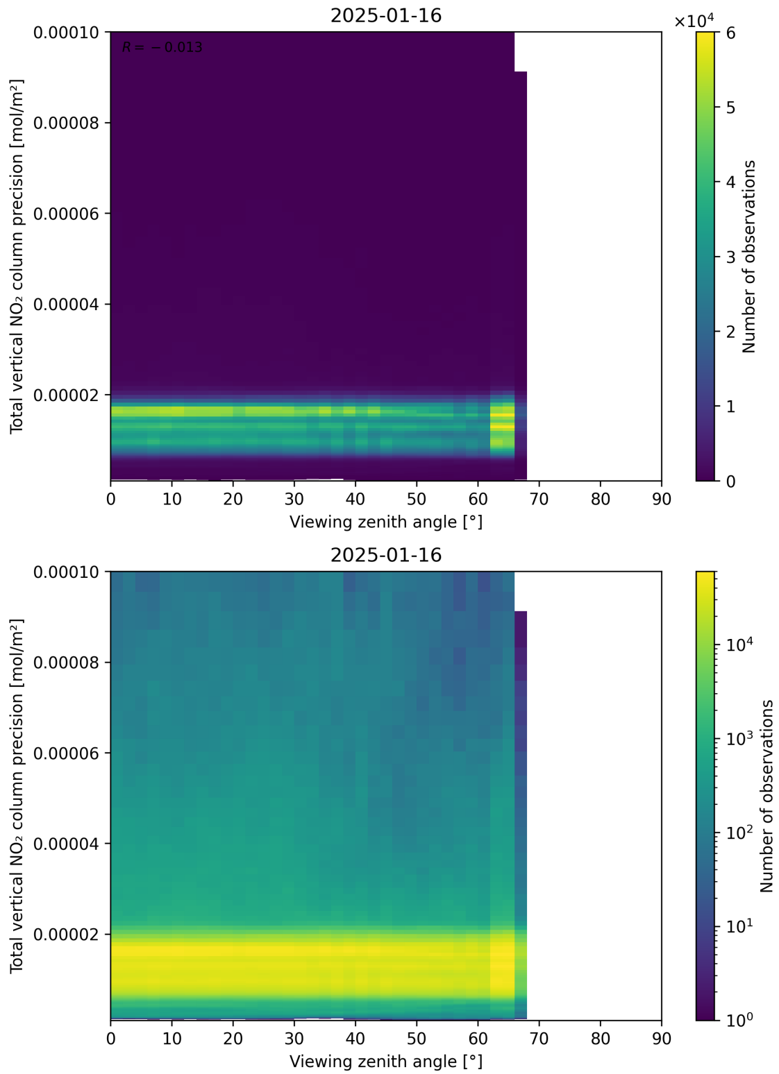
Figure 168: Scatter density plot of “Viewing zenith angle” against “Total vertical NO 2 column precision” for 2025-01-15 to 2025-01-17.
