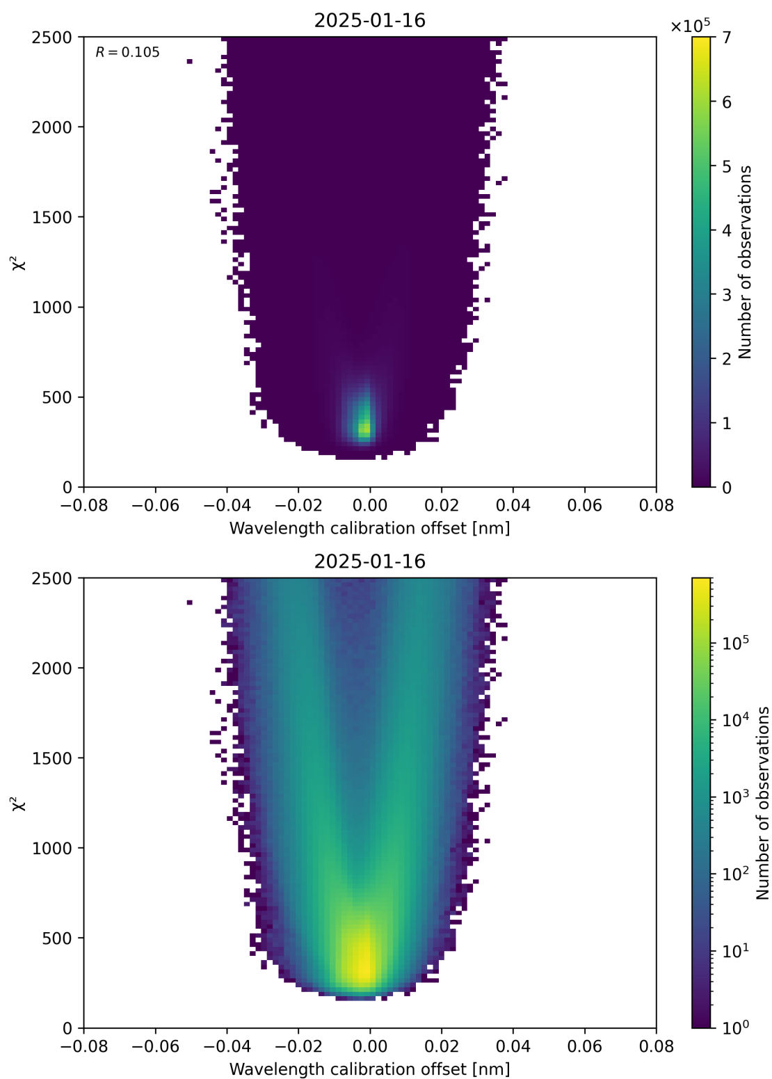
Figure 175: Scatter density plot of “Wavelength calibration offset” against “ \chi^2 ” for 2025-01-15 to 2025-01-17.
