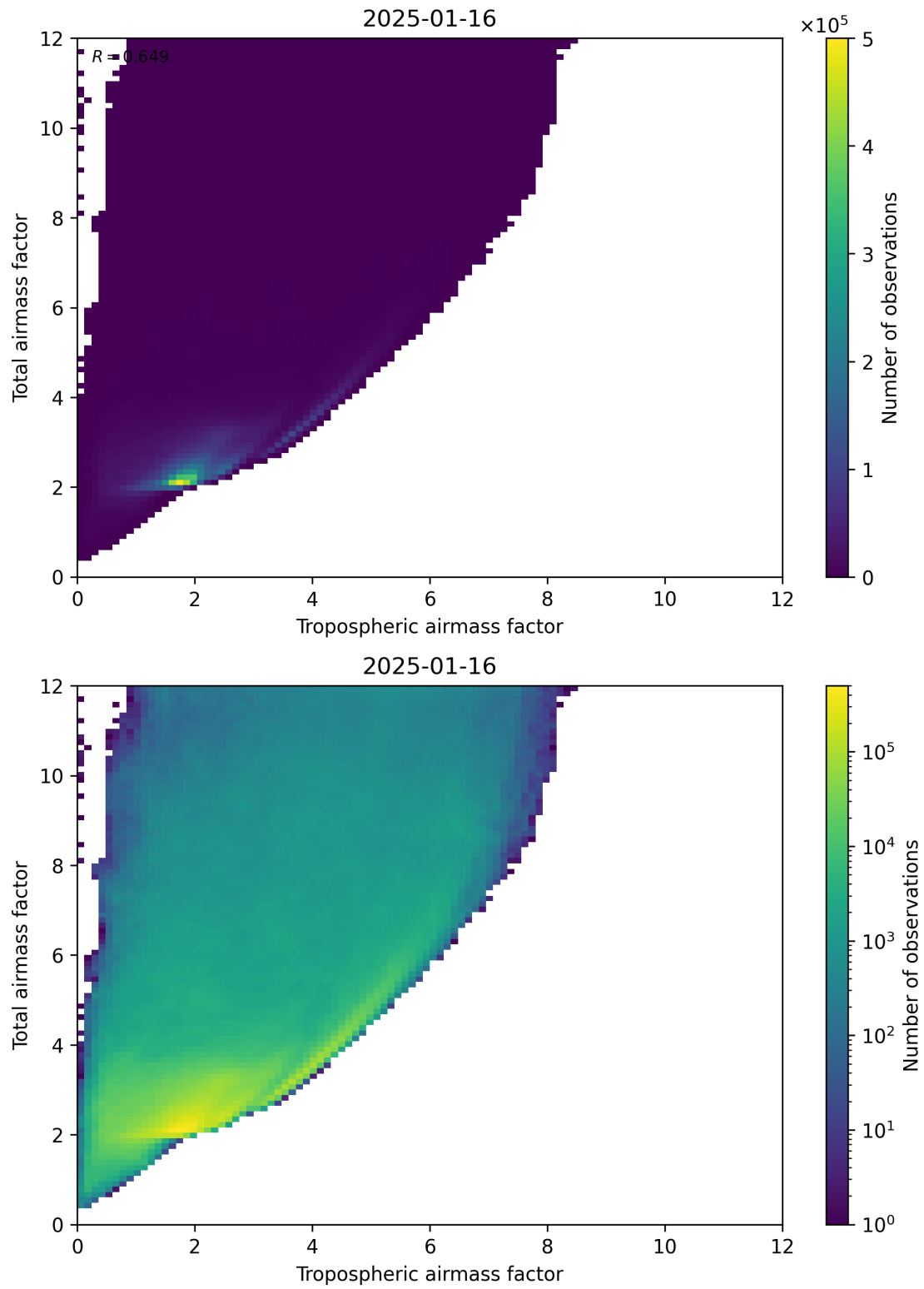
Figure 72: Scatter density plot of “Tropospheric airmass factor” against “Total airmass factor” for 2025-01-15 to 2025-01-17.
