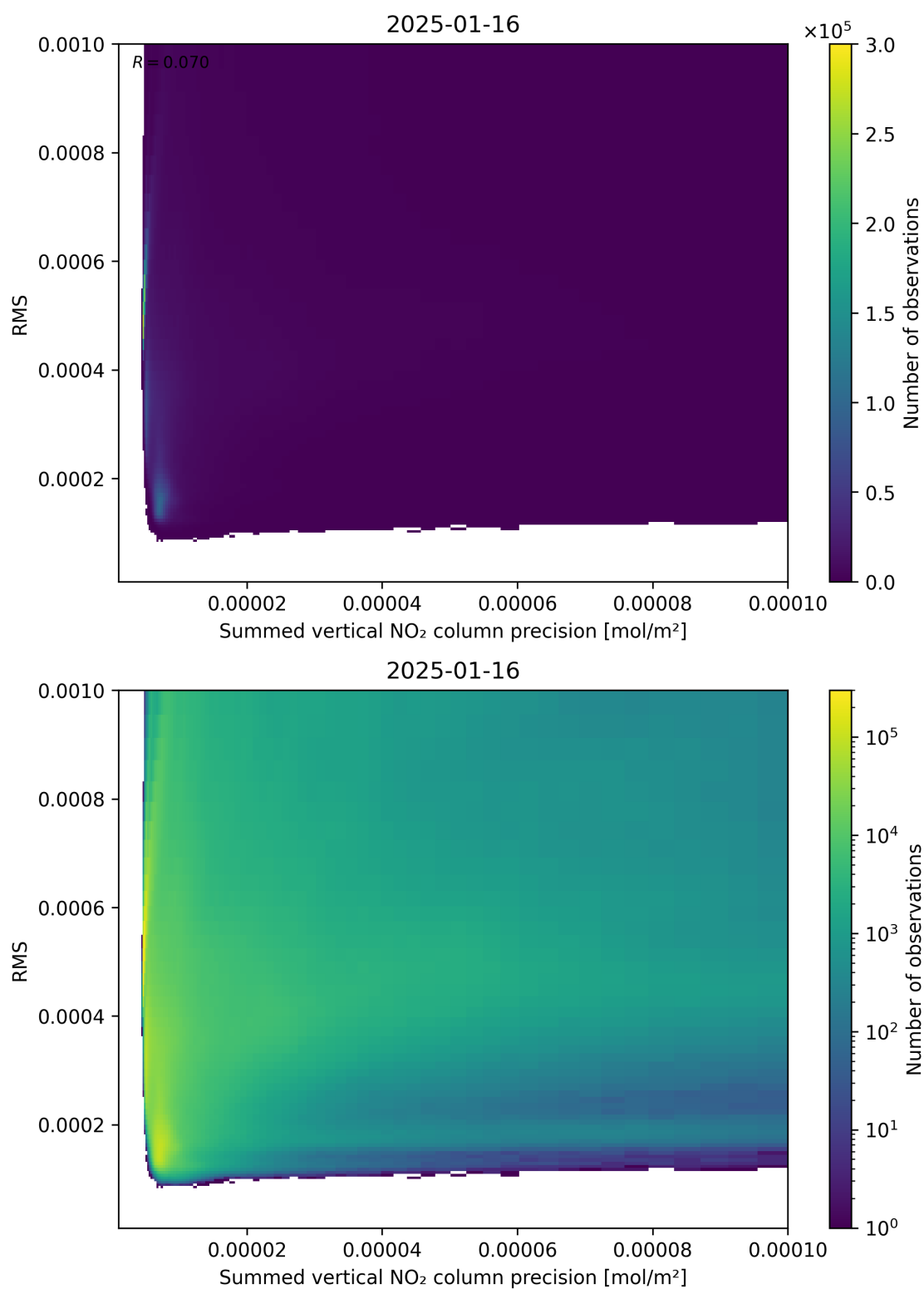
Figure 108: Scatter density plot of “Summed vertical NO 2 column precision” against “RMS” for 2025-01-15 to 2025-01-17.
