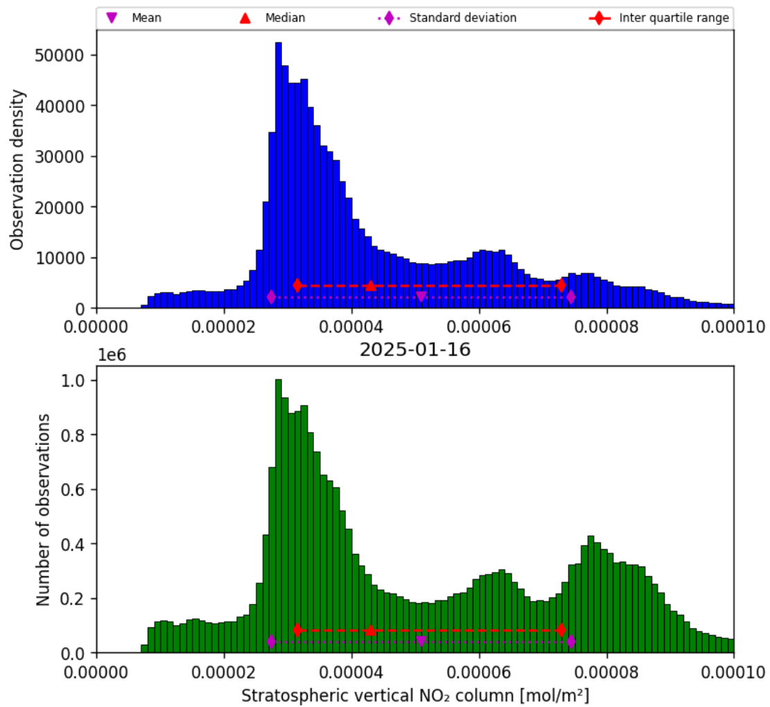
Figure 36: Histogram of “Stratospheric vertical NO 2 column” for 2025-01-15 to 2025-01-17
