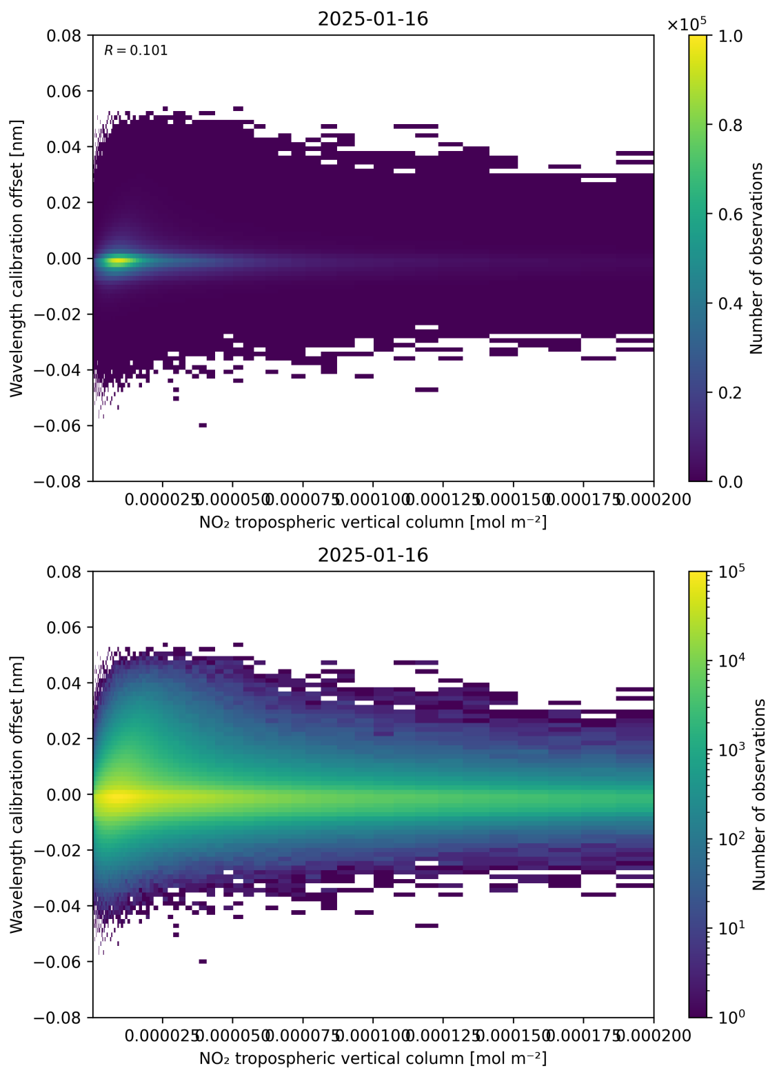
Figure 143: Scatter density plot of “NO 2 tropospheric vertical column” against “Wavelength calibration offset” for 2025-01-15 to 2025-01-17.
