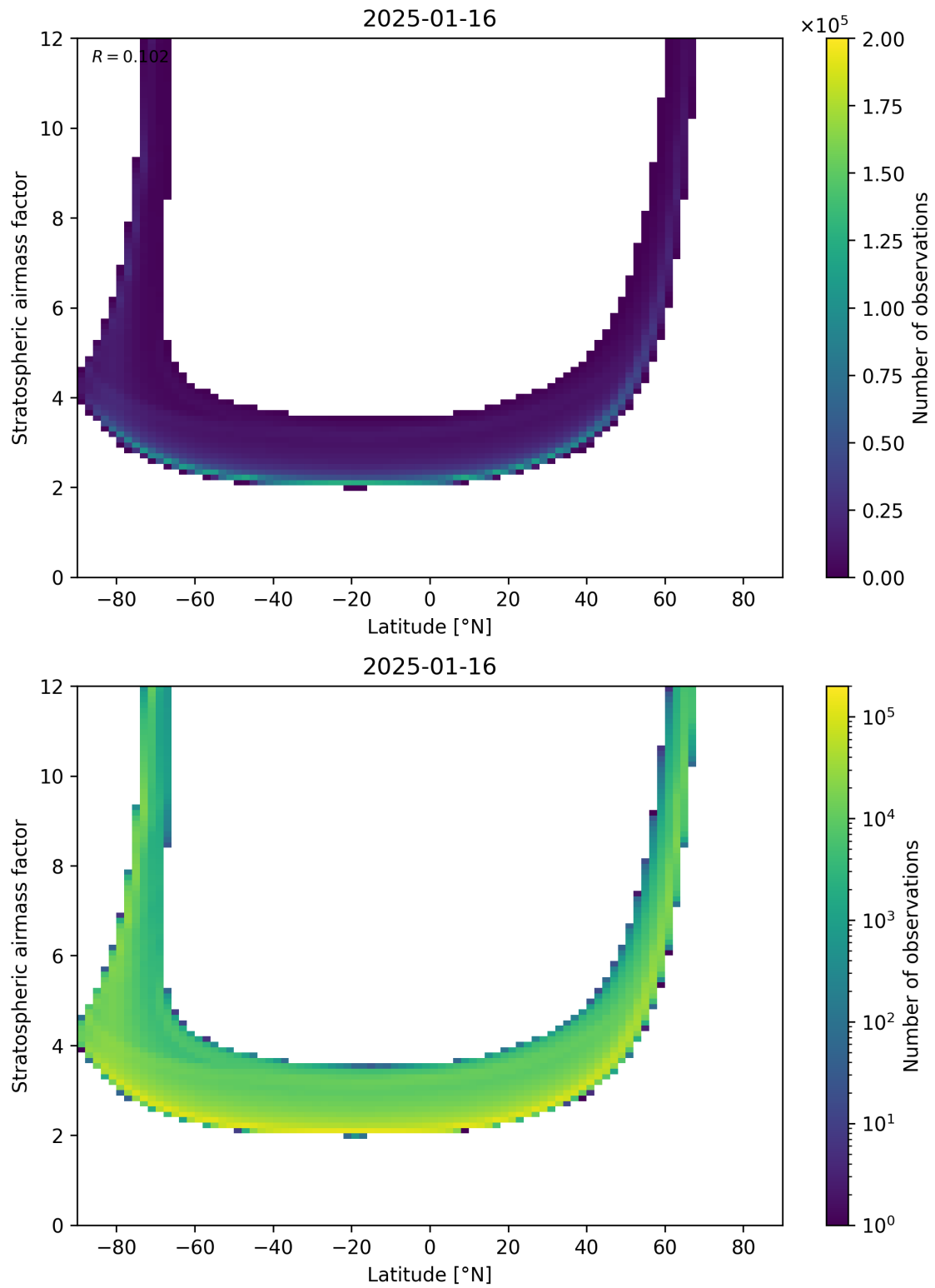
Figure 83: Scatter density plot of “Latitude” against “Stratospheric air mass factor” for 2025-01-15 to 2025-01-17.
