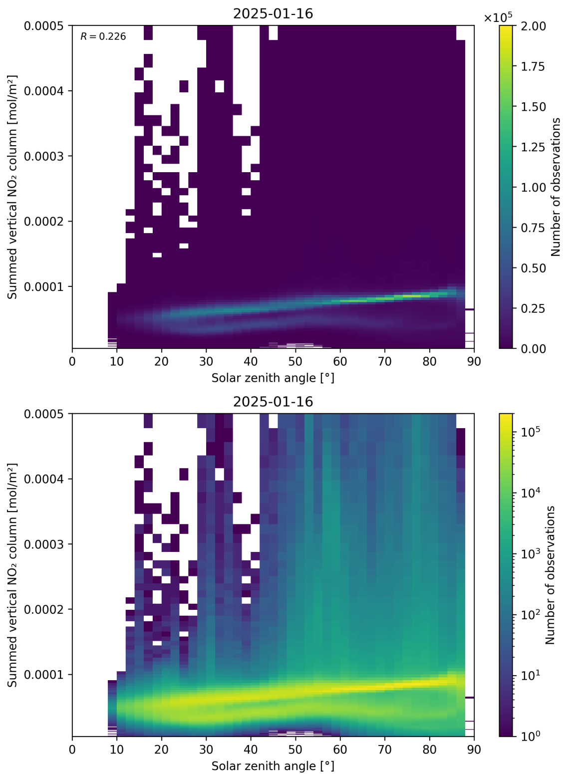
Figure 151: Scatter density plot of “Solar zenith angle” against “Summed vertical NO 2 column” for 2025-01-15 to 2025-01-17.
