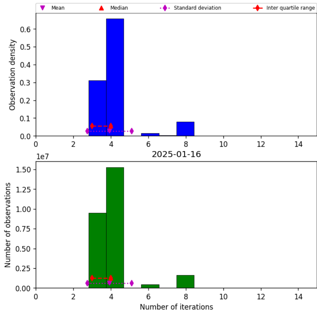
Figure 34: Histogram of “Number of iterations” for 2025-01-15 to 2025-01-17
