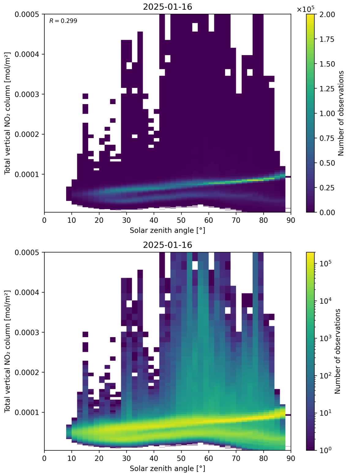
Figure 153: Scatter density plot of “Solar zenith angle” against “Total vertical NO 2 column” for 2025-01-15 to 2025-01-17.
