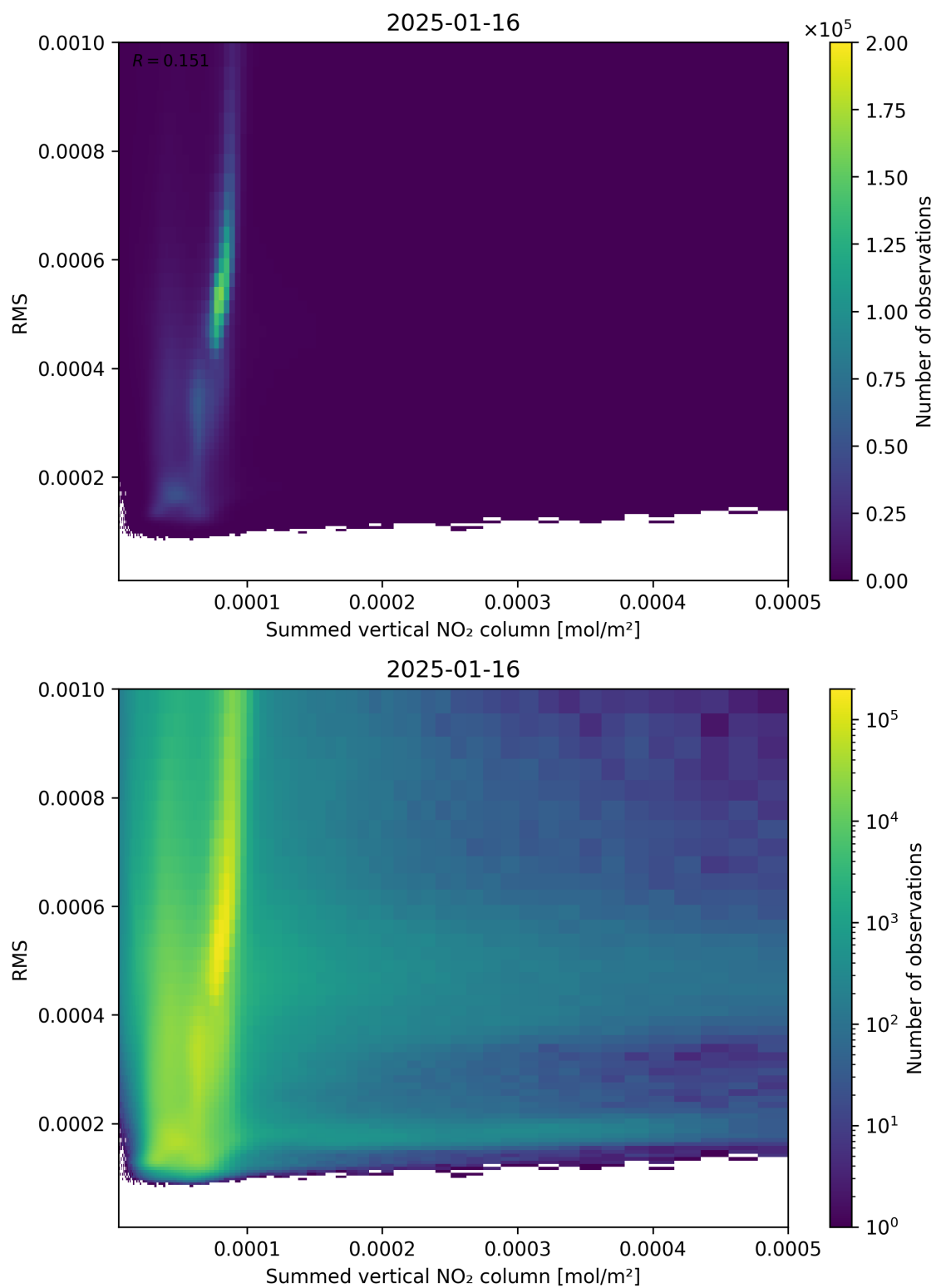
Figure 109: Scatter density plot of “Summed vertical NO 2 column” against “RMS” for 2025-01-15 to 2025-01-17.
