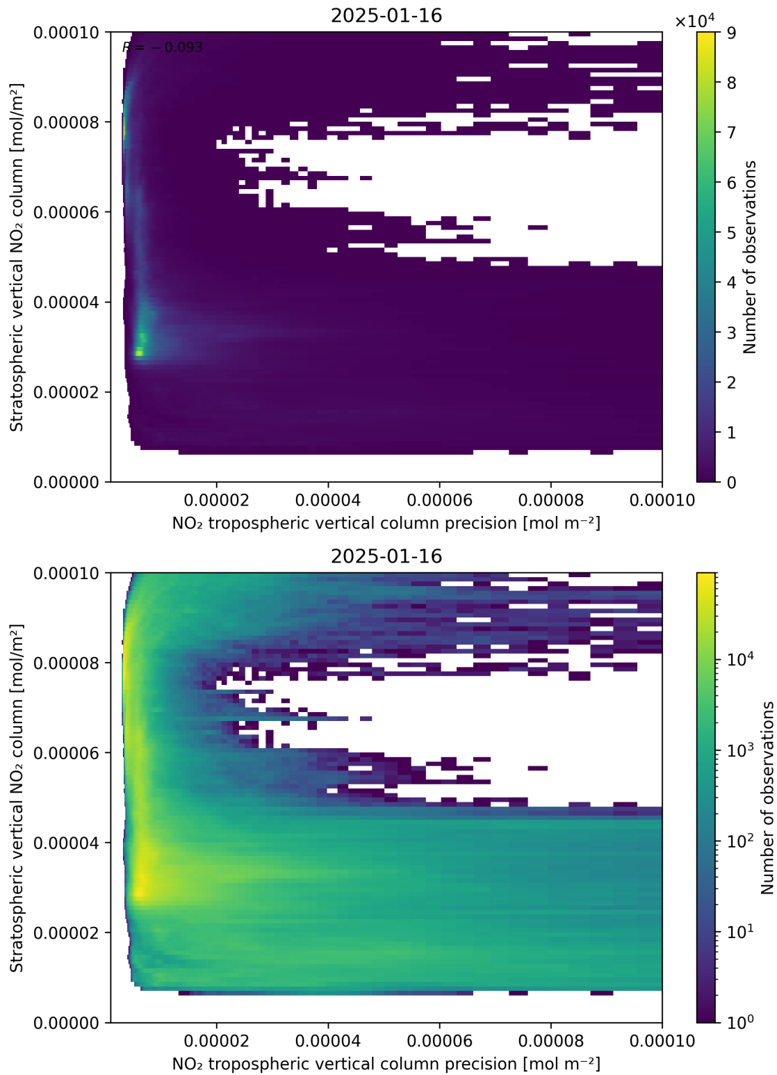
Figure 135: Scatter density plot of “NO 2 tropospheric vertical column precision” against “Stratospheric vertical NO 2 column” for 2025-01-15 to 2025-01-17.
