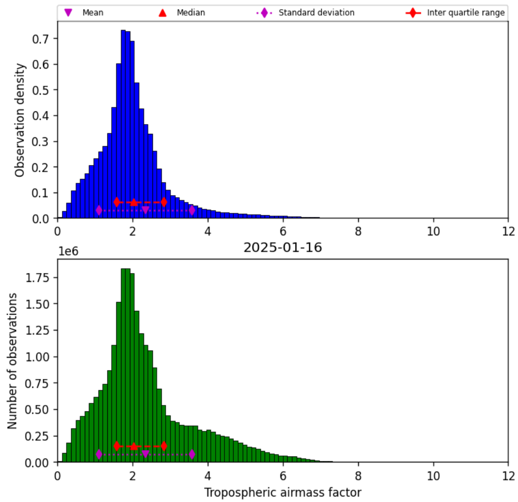
Figure 31: Histogram of “Tropospheric airmass factor” for 2025-01-15 to 2025-01-17
