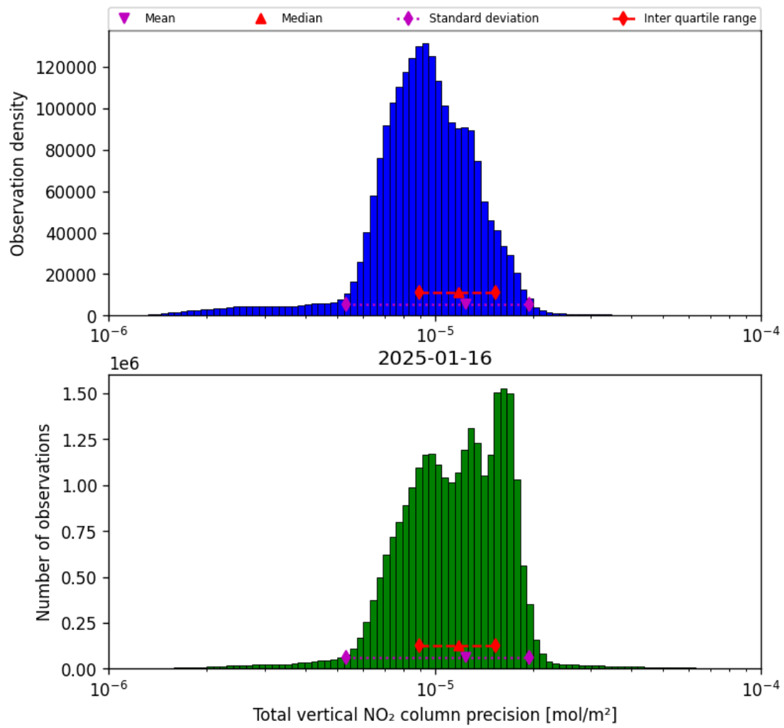
Figure 39: Histogram of “Total vertical NO 2 column precision” for 2025-01-15 to 2025-01-17
