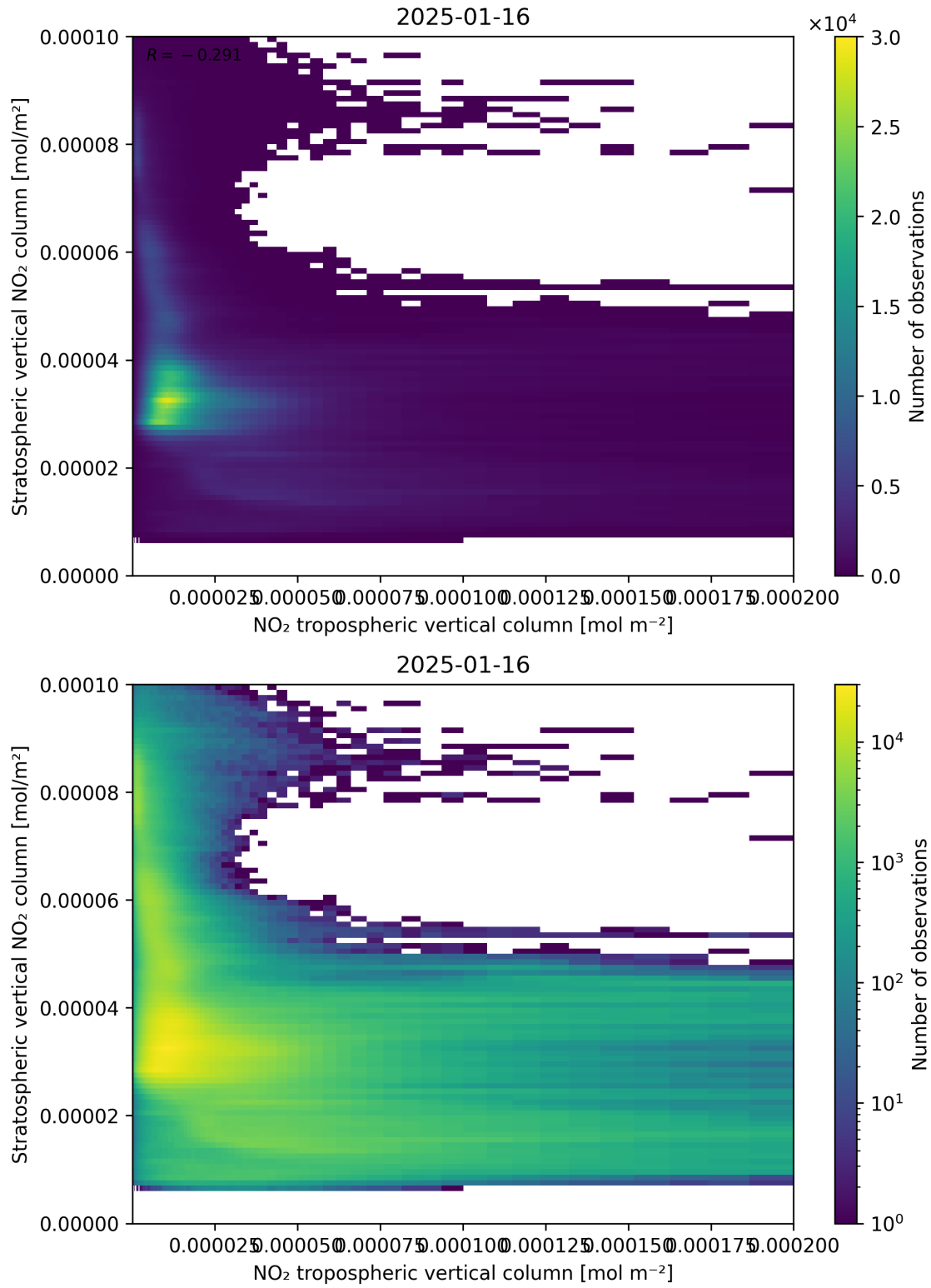
Figure 125: Scatter density plot of “NO 2 tropospheric vertical column” against “Stratospheric vertical NO 2 column” for 2025-01-15 to 2025-01-17.
