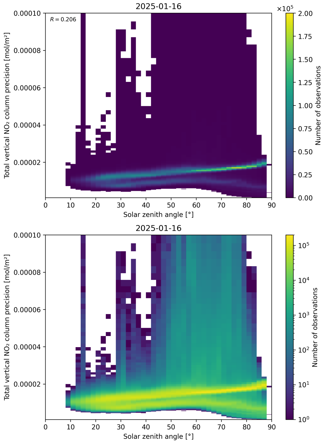
Figure 154: Scatter density plot of “Solar zenith angle” against “Total vertical NO 2 column precision” for 2025-01-15 to 2025-01-17.
