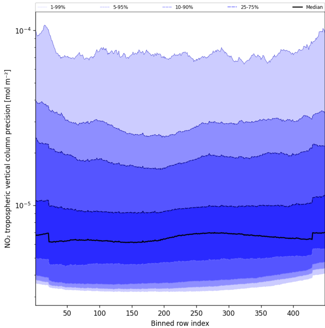
Figure 47: Along track statistics of “NO 2 tropospheric vertical column precision” for 2025-01-15 to 2025-01-17
