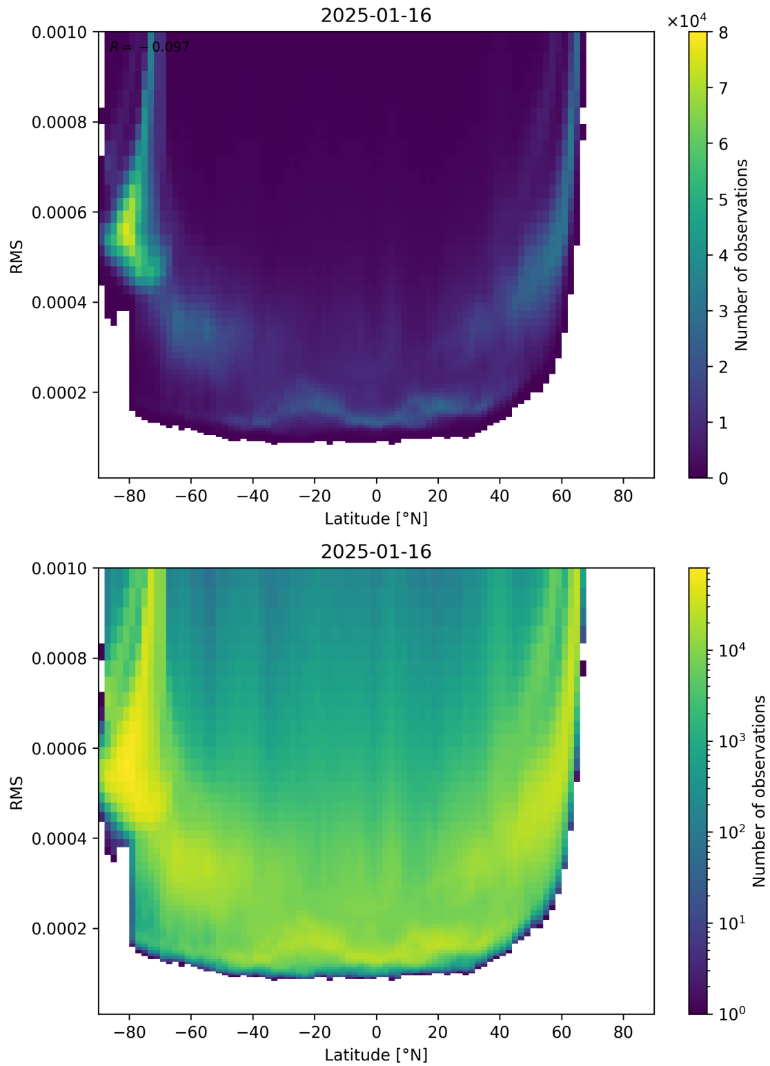
Figure 94: Scatter density plot of “Latitude” against “RMS” for 2025-01-15 to 2025-01-17.
