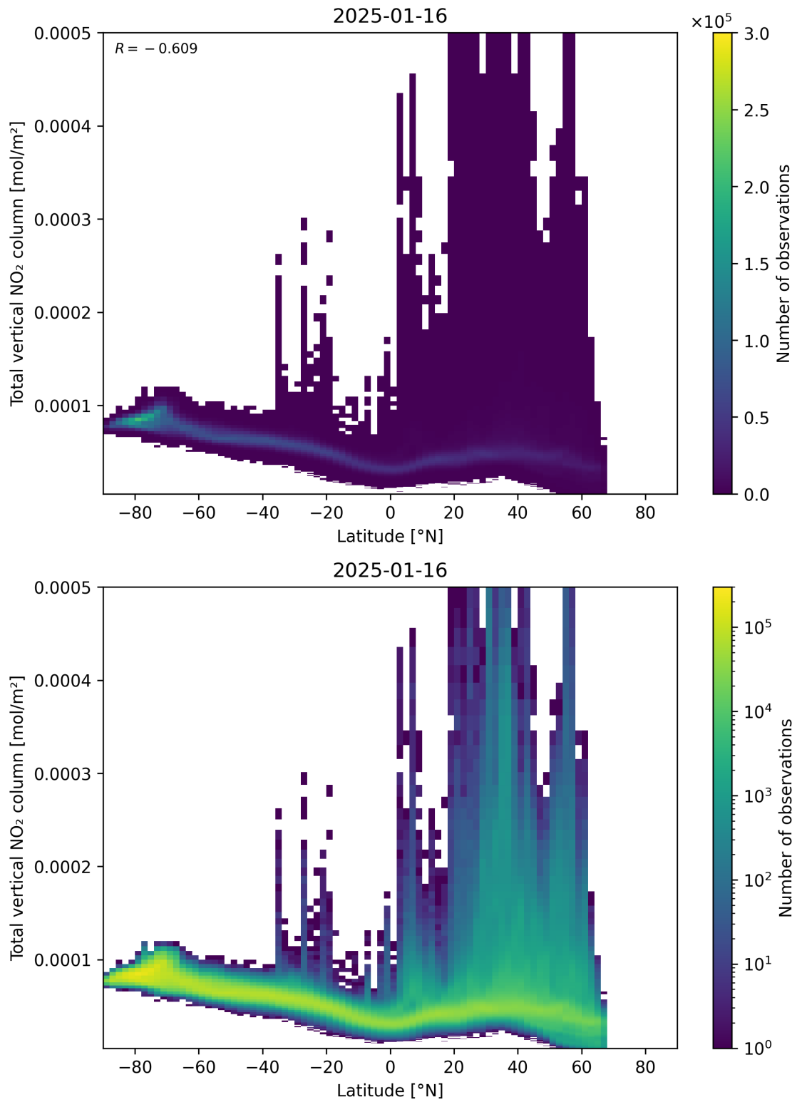
Figure 90: Scatter density plot of “Latitude” against “Total vertical NO 2 column” for 2025-01-15 to 2025-01-17.
