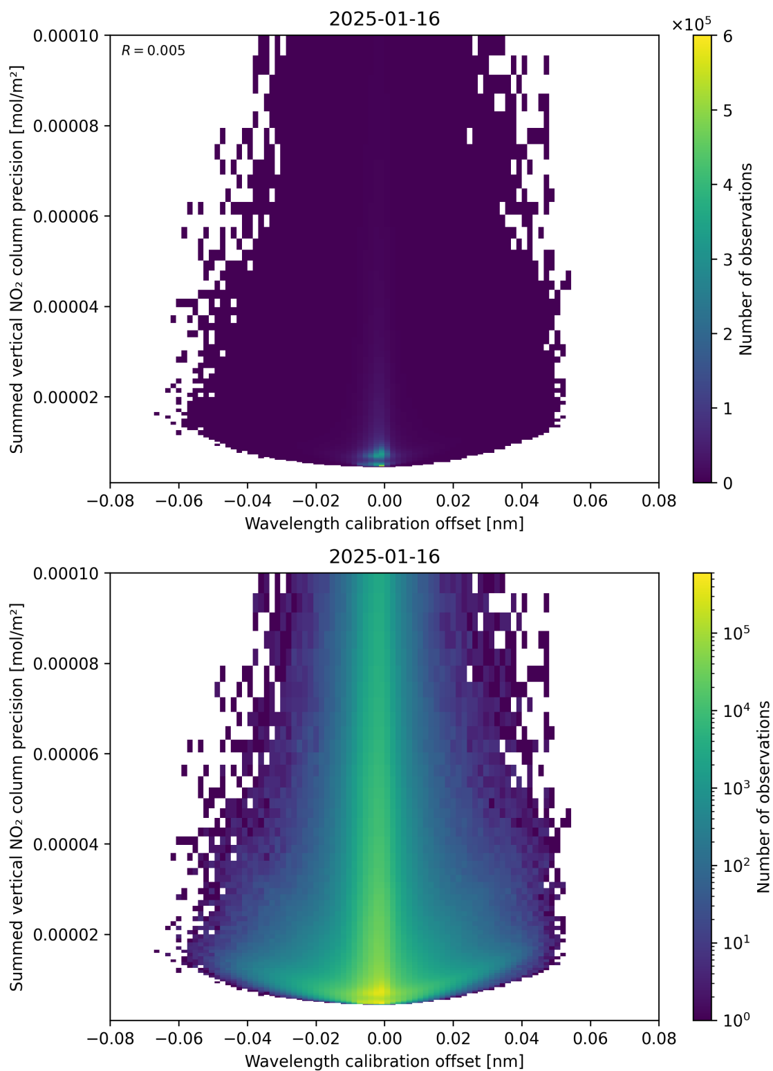
Figure 178: Scatter density plot of “Wavelength calibration offset” against “Summed vertical NO 2 column precision” for 2025-01-15 to 2025-01-17.
