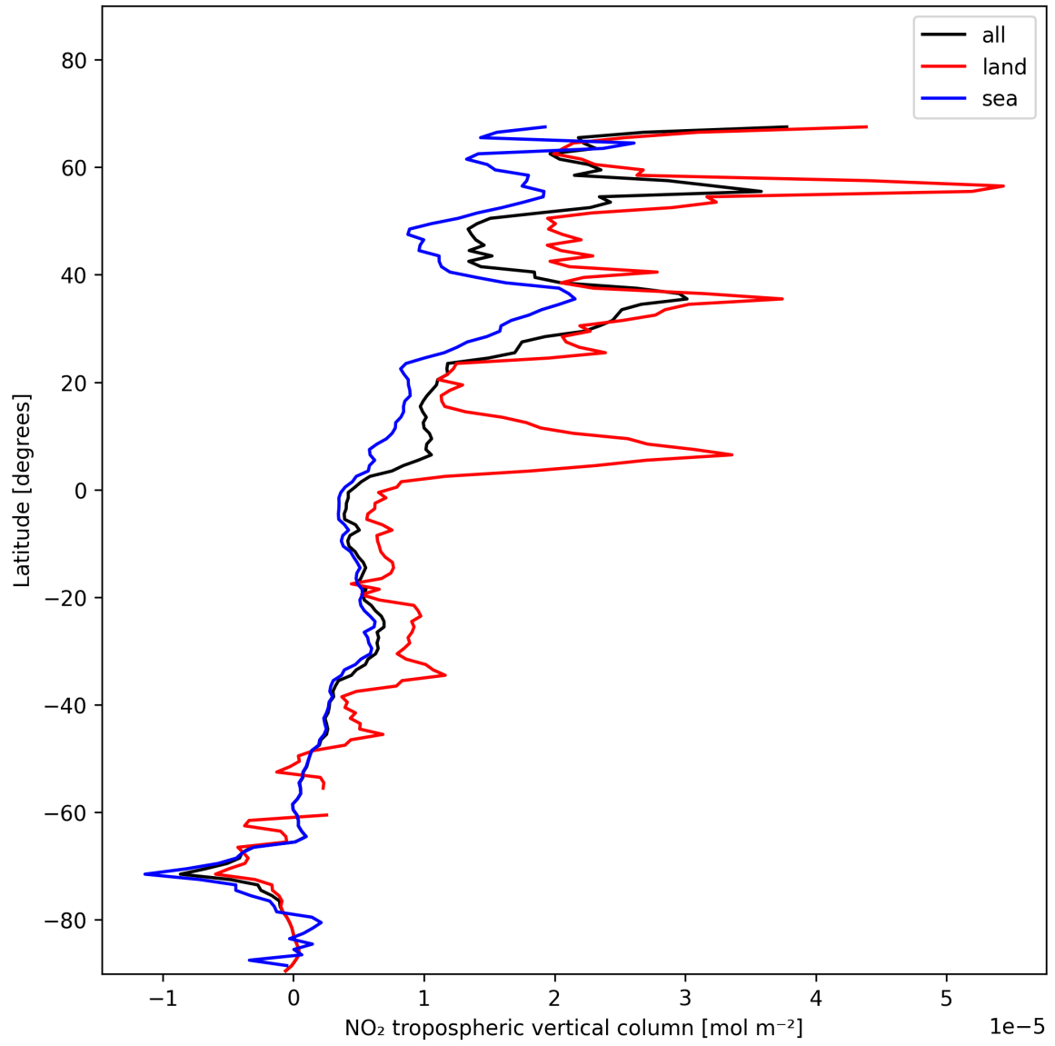
Figure 12: Zonal average of “NO 2 tropospheric vertical column” for 2025-01-15 to 2025-01-17.
