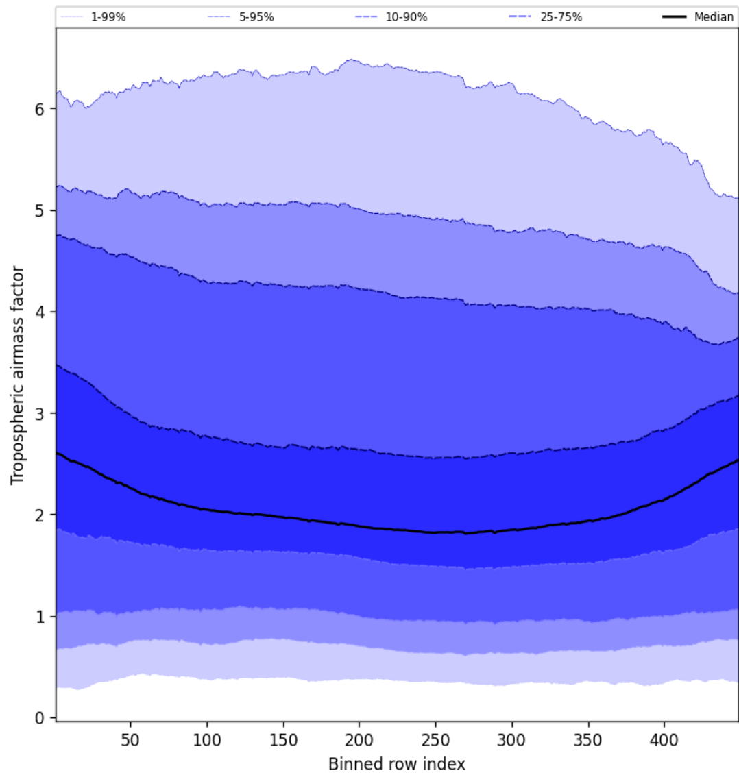
Figure 48: Along track statistics of “Tropospheric air mass factor” for 2025-01-15 to 2025-01-17
