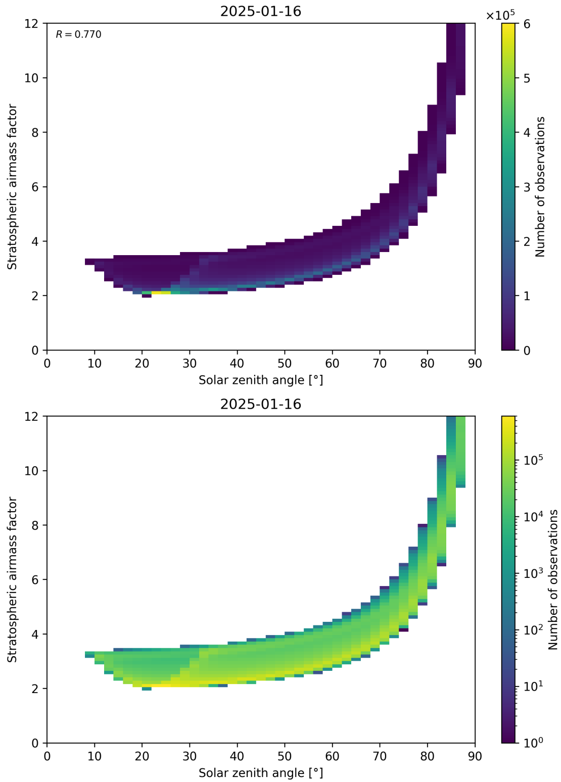
Figure 145: Scatter density plot of “Solar zenith angle” against “Stratospheric airmass factor” for 2025-01-15 to 2025-01-17.
