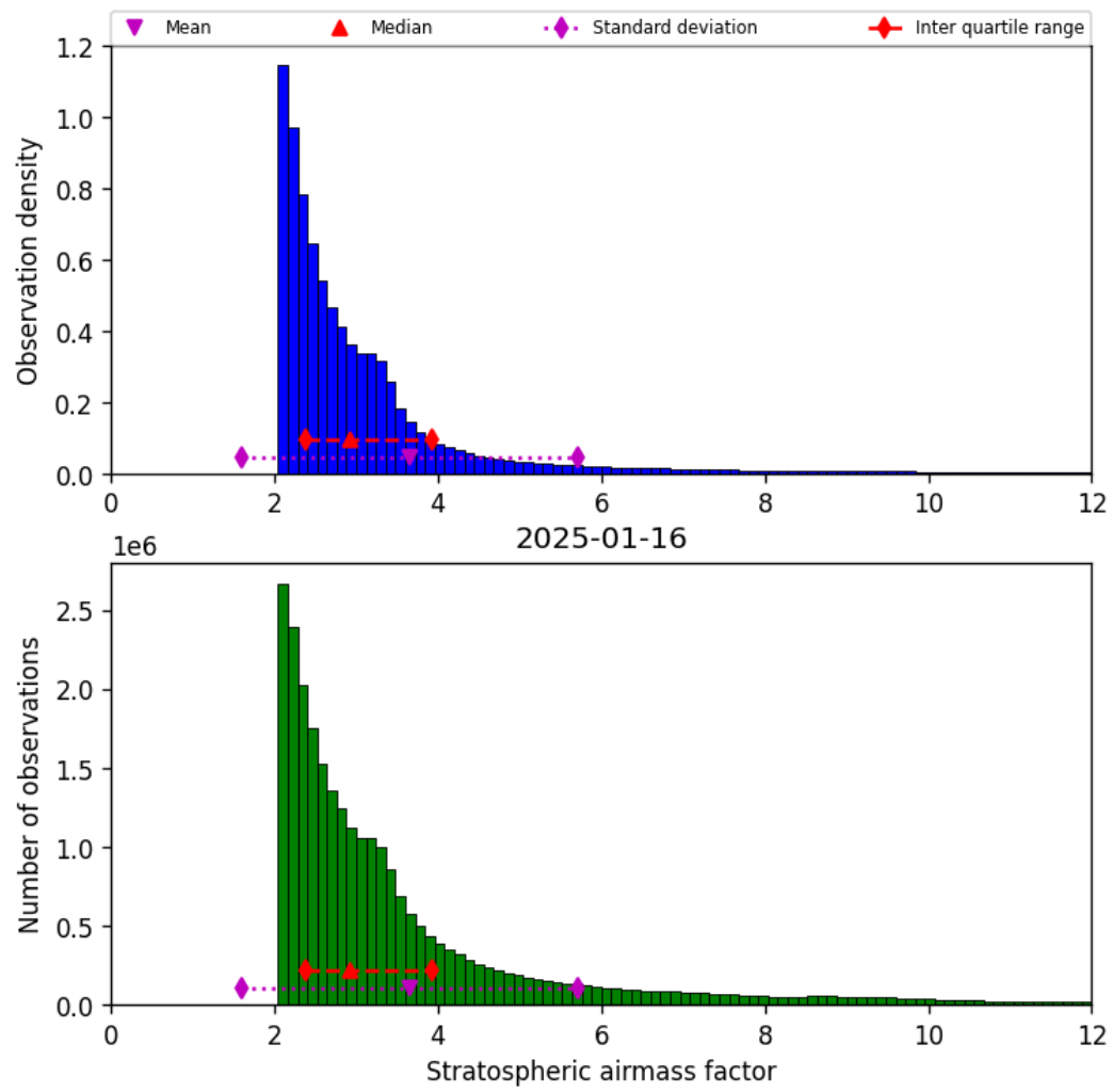
Figure 44: Histogram of “Stratospheric airmass factor” for 2025-01-15 to 2025-01-17
