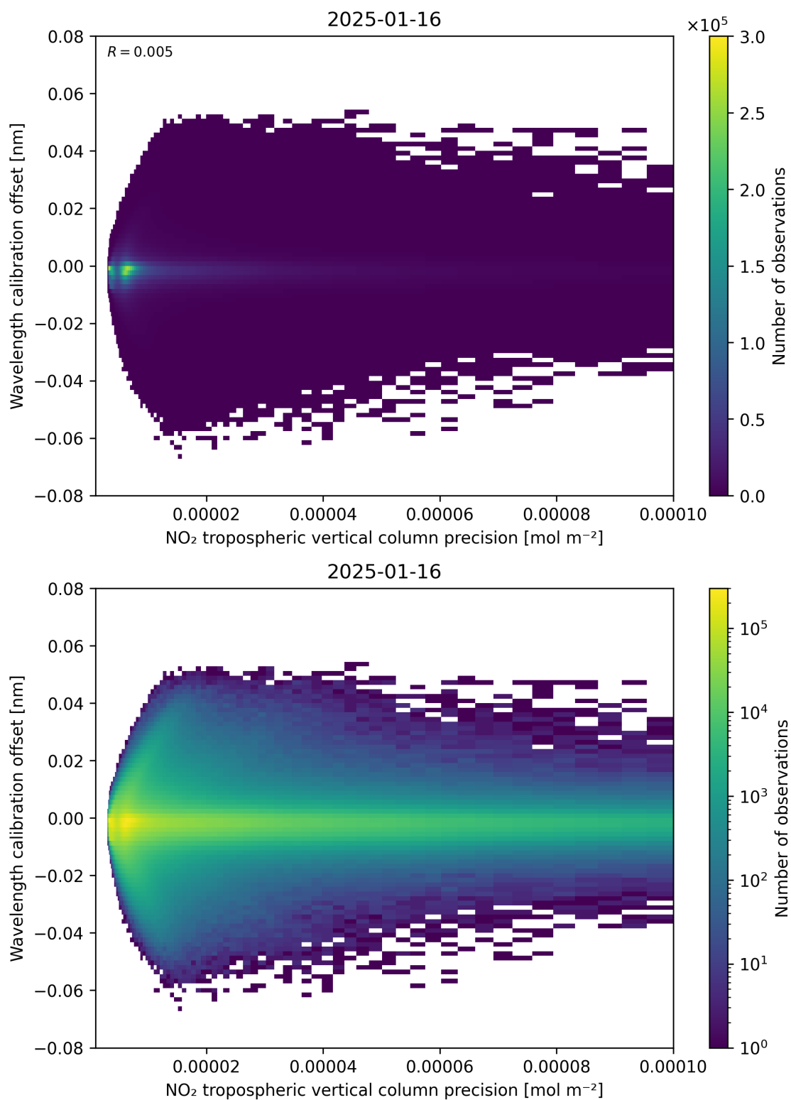
Figure 141: Scatter density plot of “NO 2 tropospheric vertical column precision” against “Wavelength calibration offset” for 2025-01-15 to 2025-01-17.
