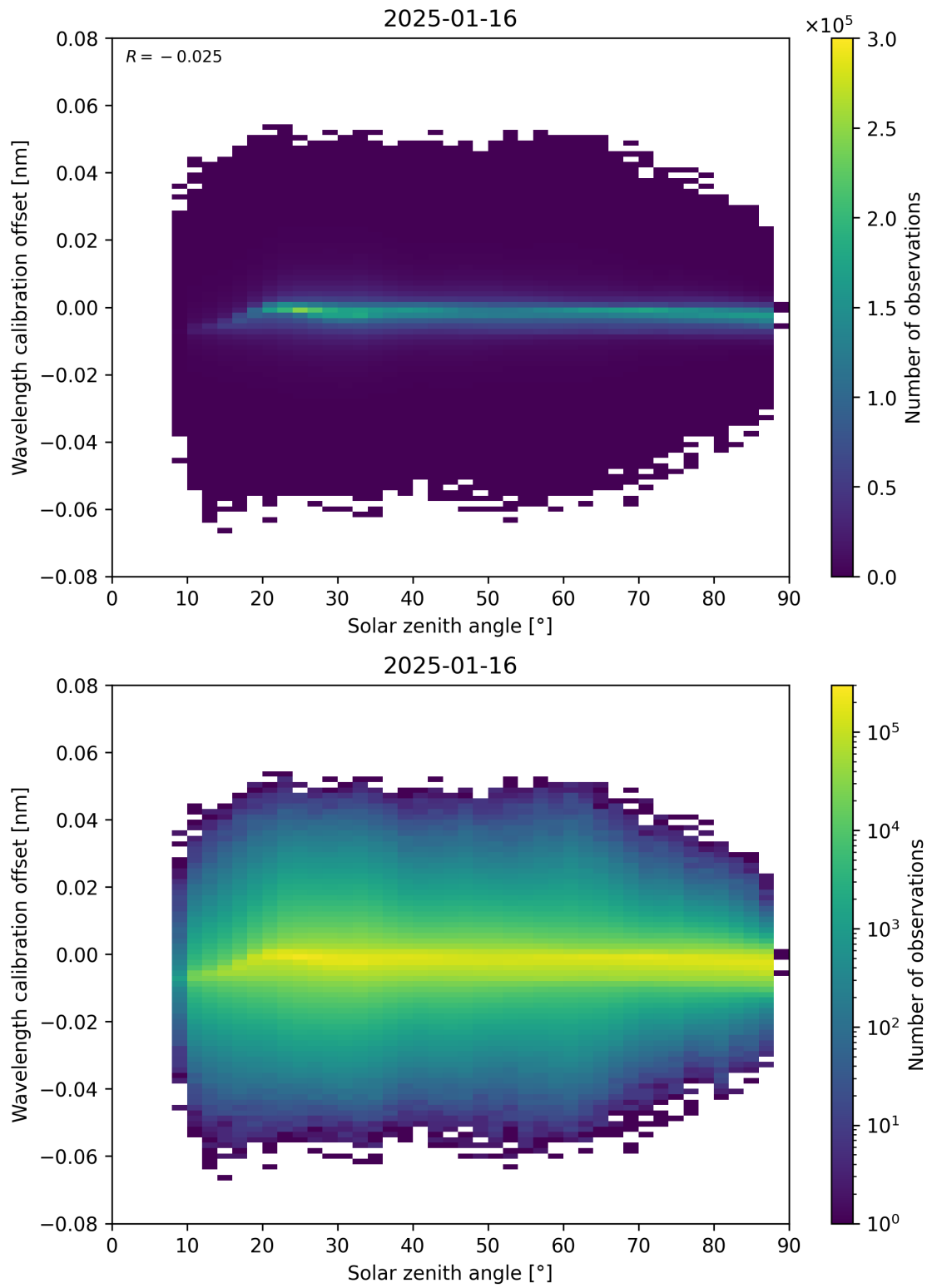
Figure 158: Scatter density plot of “Solar zenith angle” against “Wavelength calibration offset” for 2025-01-15 to 2025-01-17.
