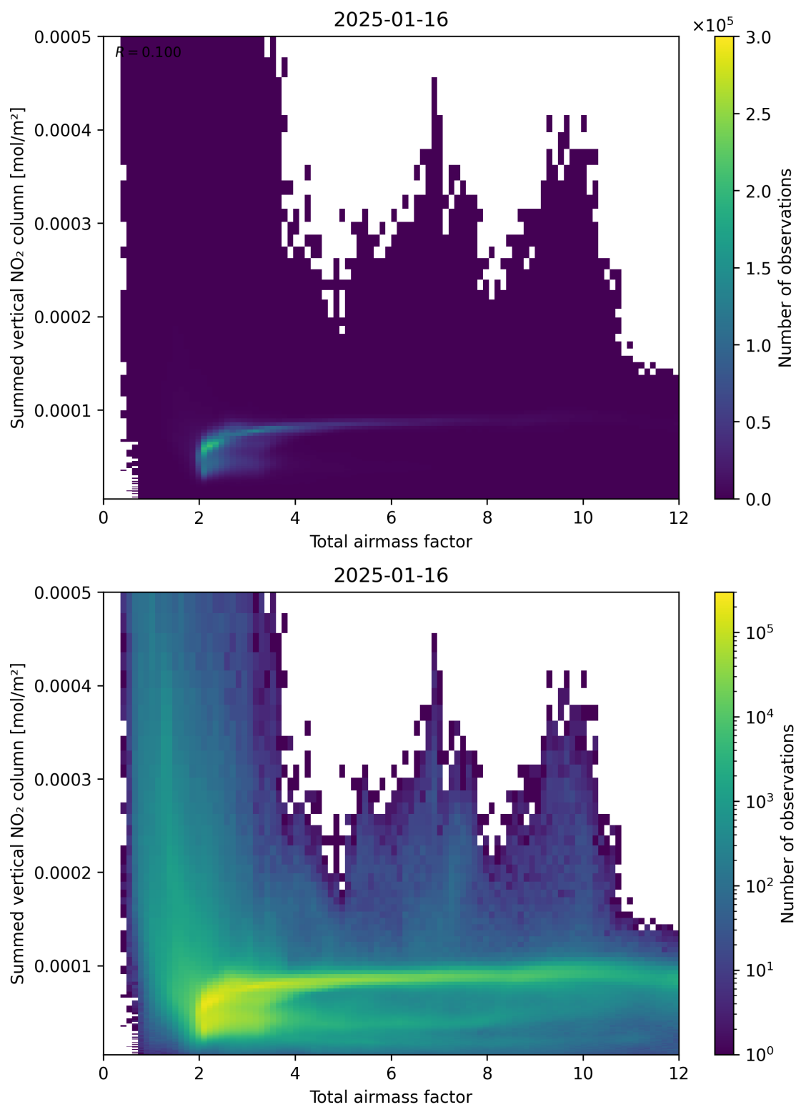
Figure 65: Scatter density plot of “Total airmass factor” against “Summed vertical NO 2 column” for 2025-01-15 to 2025-01-17.
