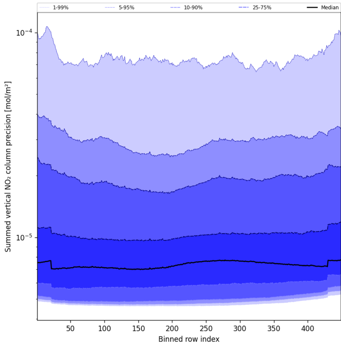
Figure 58: Along track statistics of “Summed vertical NO 2 column precision” for 2025-01-15 to 2025-01-17
