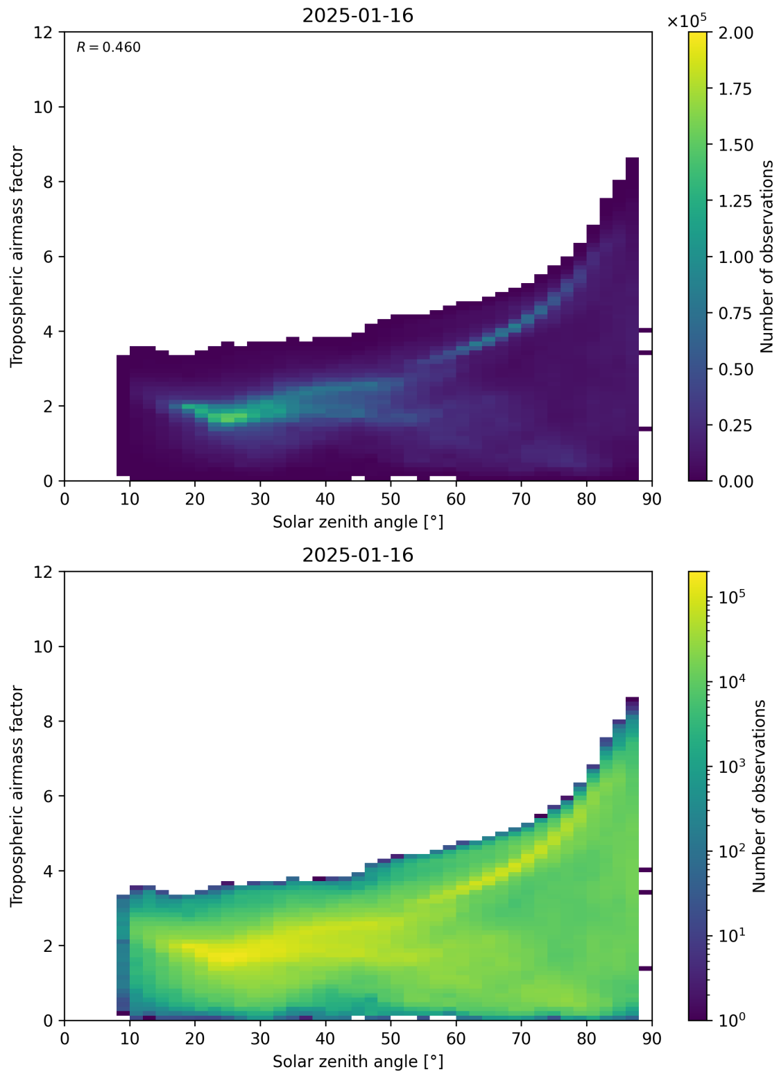
Figure 147: Scatter density plot of “Solar zenith angle” against “Tropospheric airmass factor” for 2025-01-15 to 2025-01-17.
