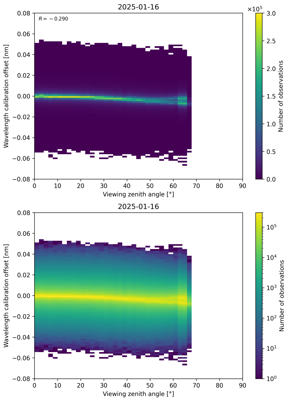
Figure 173: Scatter density plot of “Viewing zenith angle” against “Wavelength calibration offset” for 2025-01-15 to 2025-01-17.
