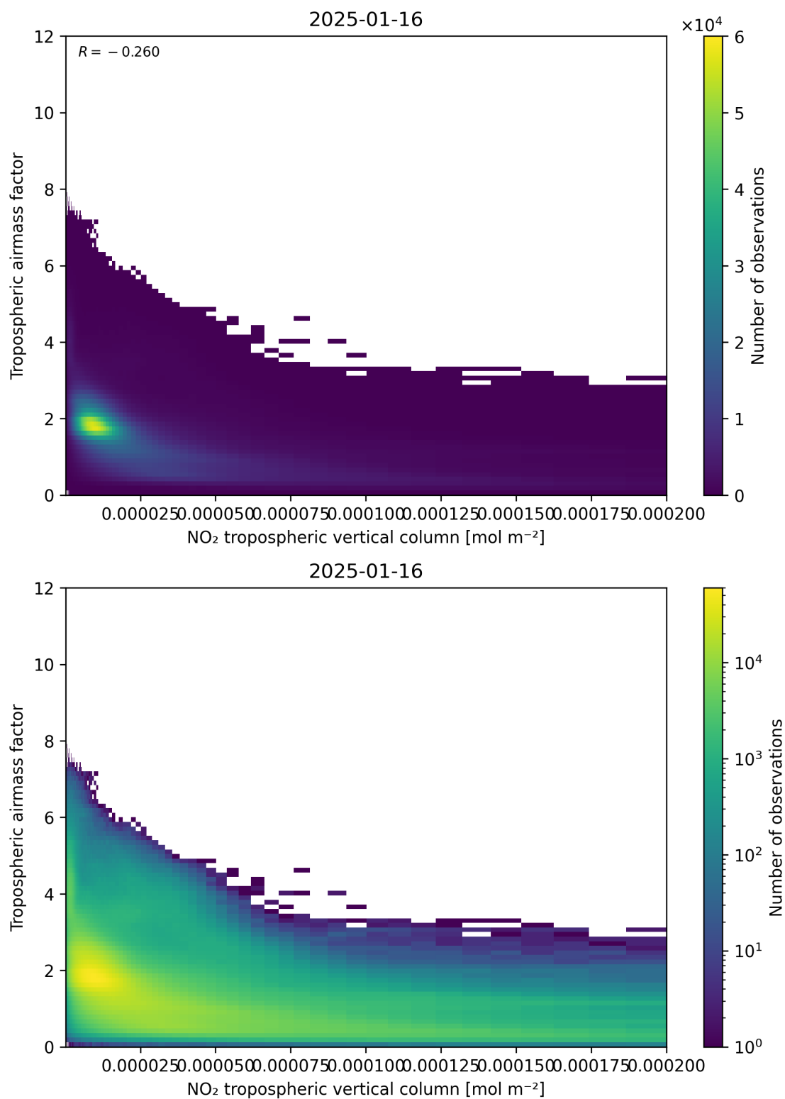
Figure 123: Scatter density plot of “NO 2 tropospheric vertical column” against “Tropospheric air mass factor” for 2025-01-15 to 2025-01-17.
