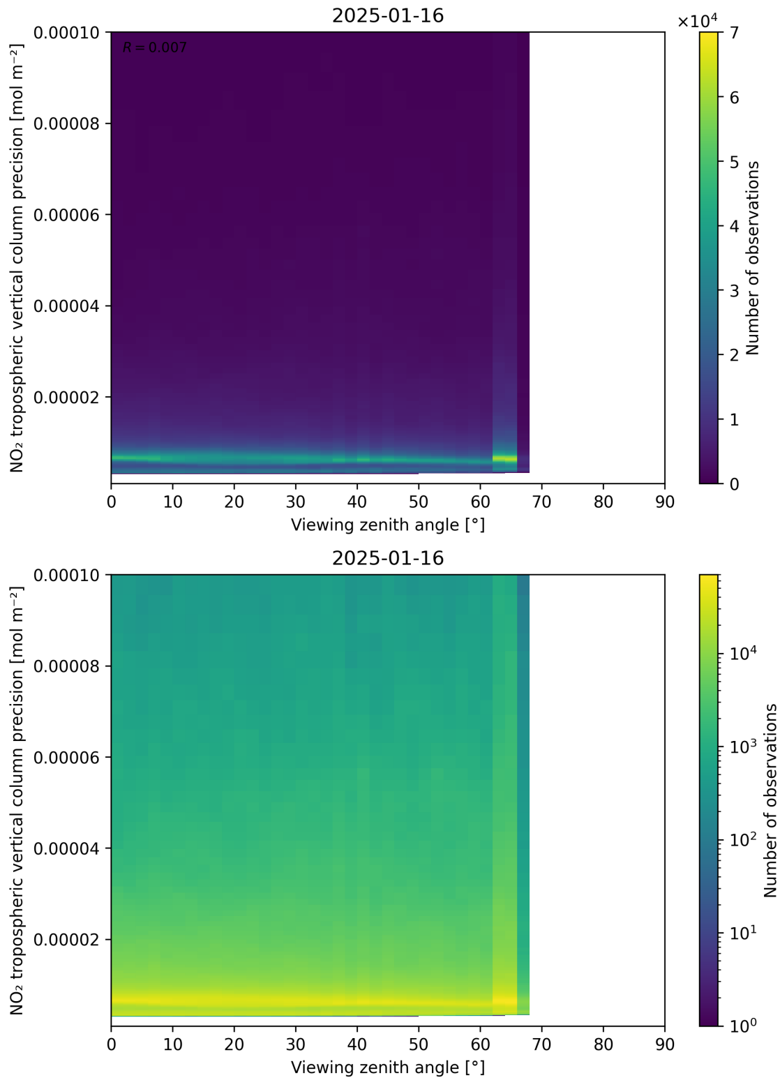
Figure 170: Scatter density plot of “Viewing zenith angle” against “NO 2 tropospheric vertical column precision” for 2025-01-15 to 2025-01-17.
