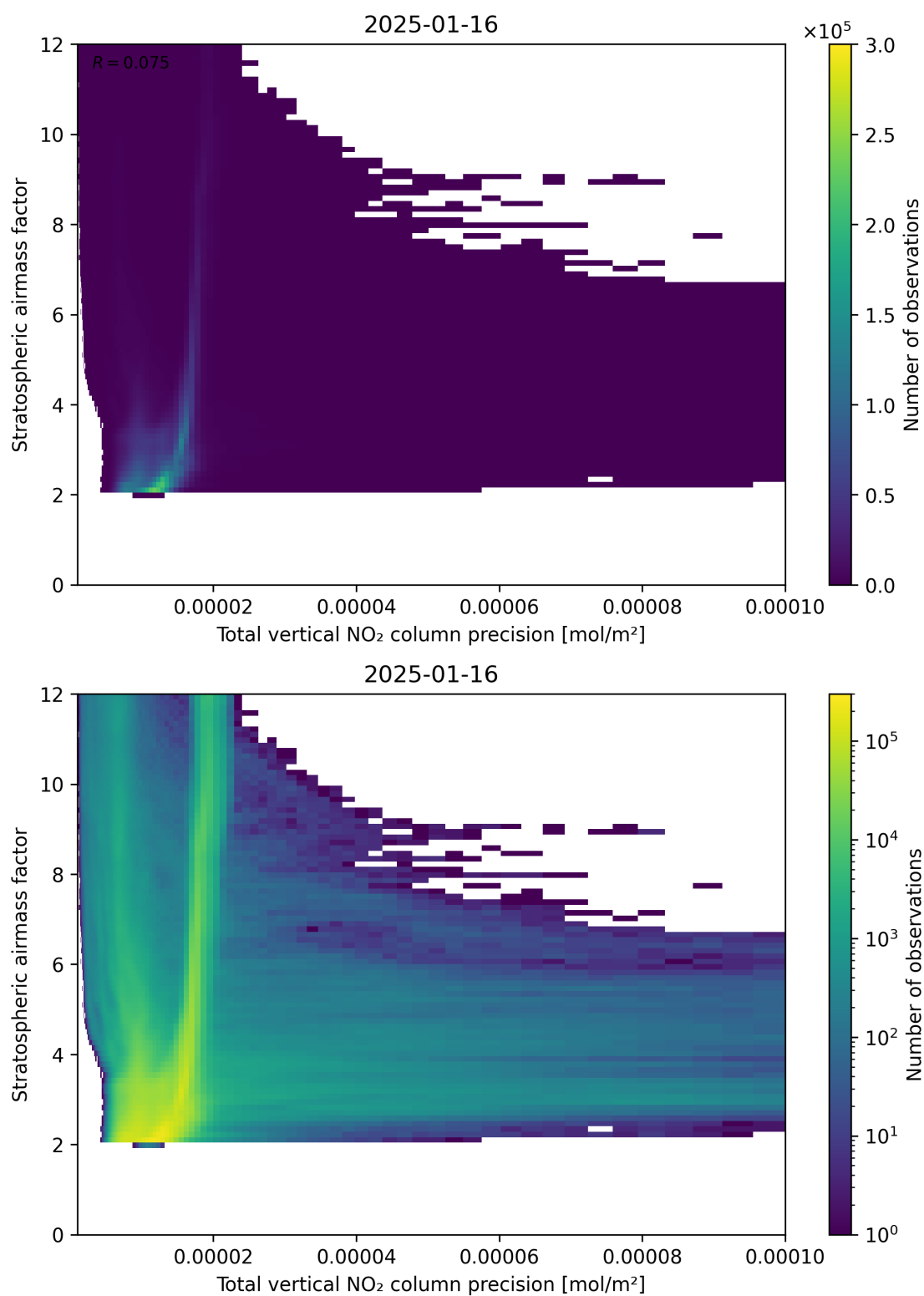
Figure 115: Scatter density plot of “Total vertical NO 2 column precision” against “Stratospheric air mass factor” for 2025-01-15 to 2025-01-17.
