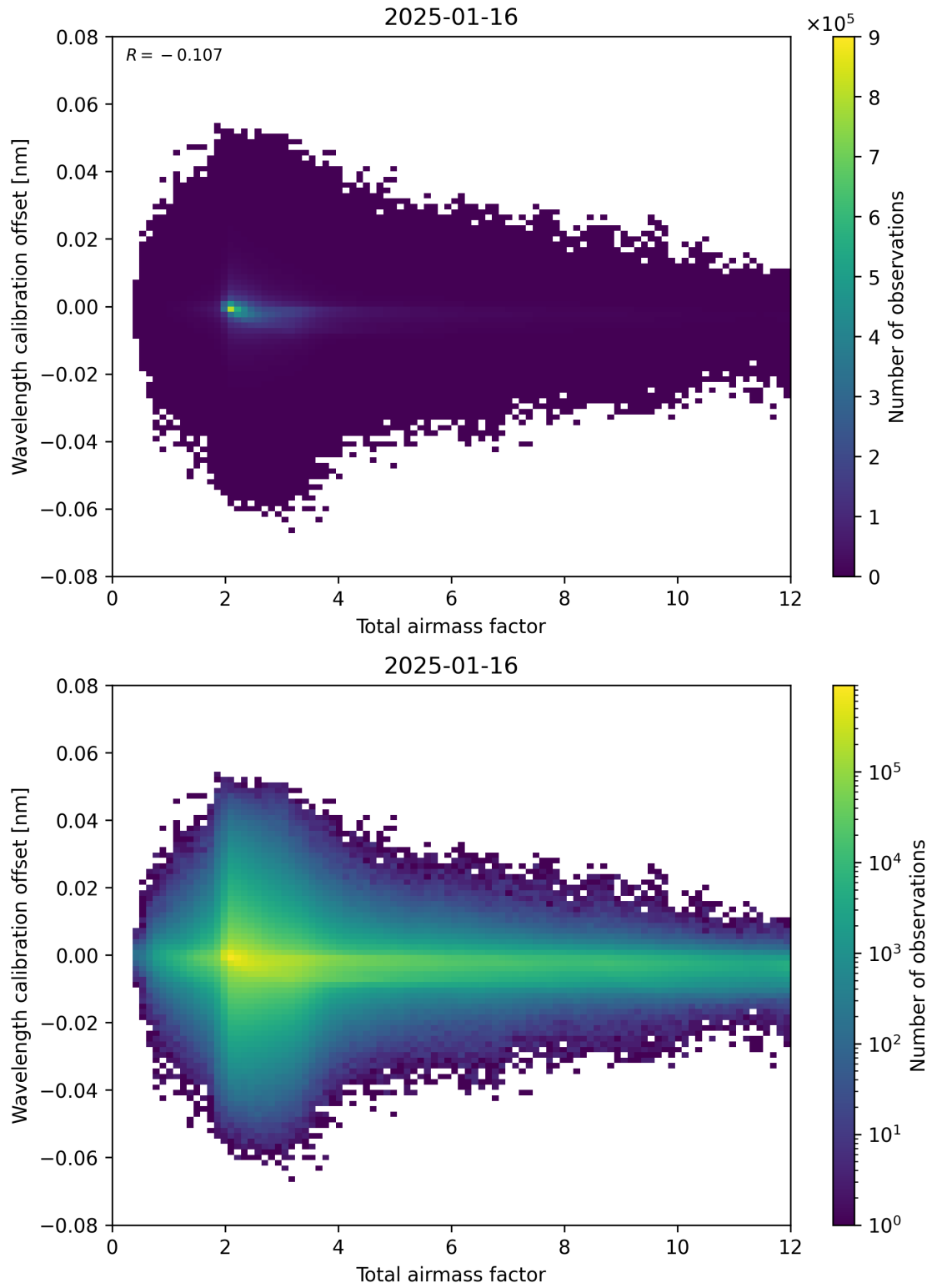
Figure 70: Scatter density plot of “Total airmass factor” against “Wavelength calibration offset” for 2025-01-15 to 2025-01-17.
