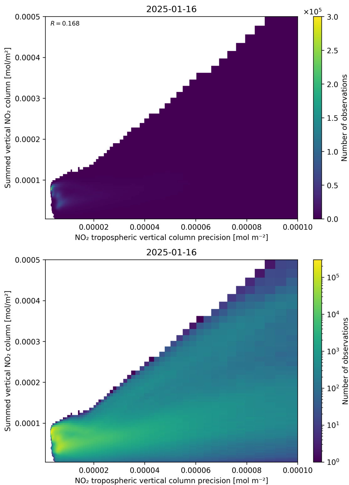
Figure 136: Scatter density plot of “NO 2 tropospheric vertical column precision” against “Summed vertical NO 2 column” for 2025-01-15 to 2025-01-17.
