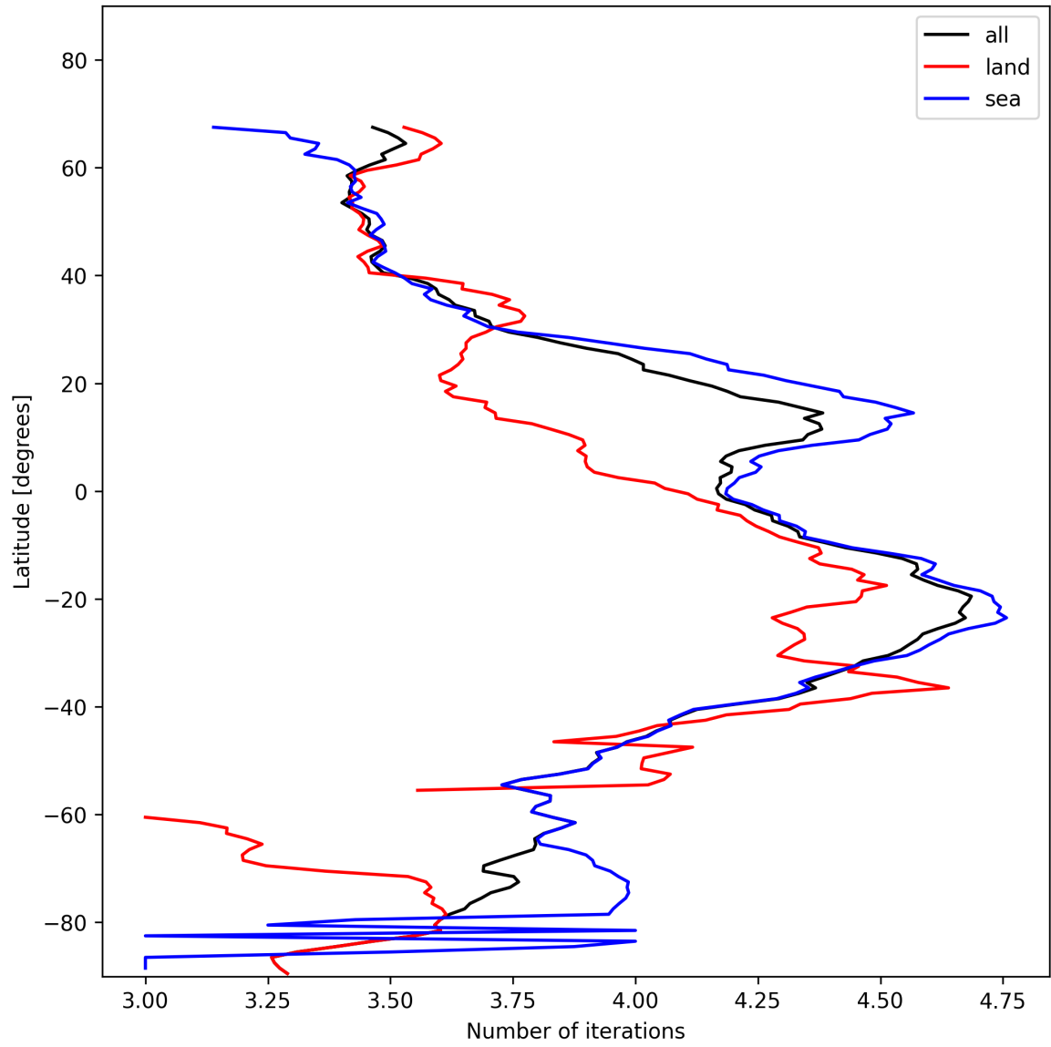
Figure 17: Zonal average of “Number of iterations” for 2025-01-15 to 2025-01-17.
