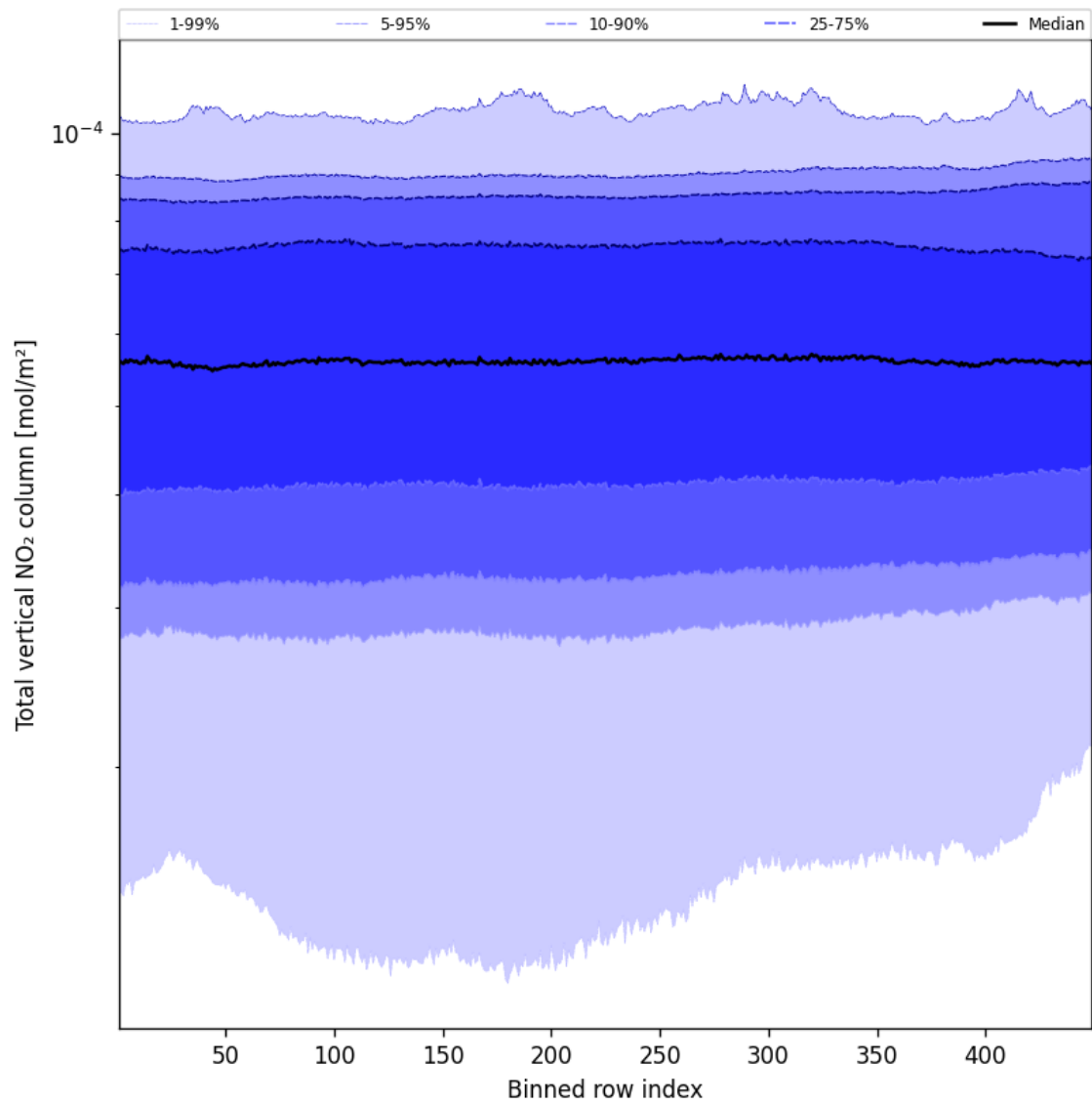
Figure 55: Along track statistics of “Total vertical NO 2 column” for 2025-01-15 to 2025-01-17
