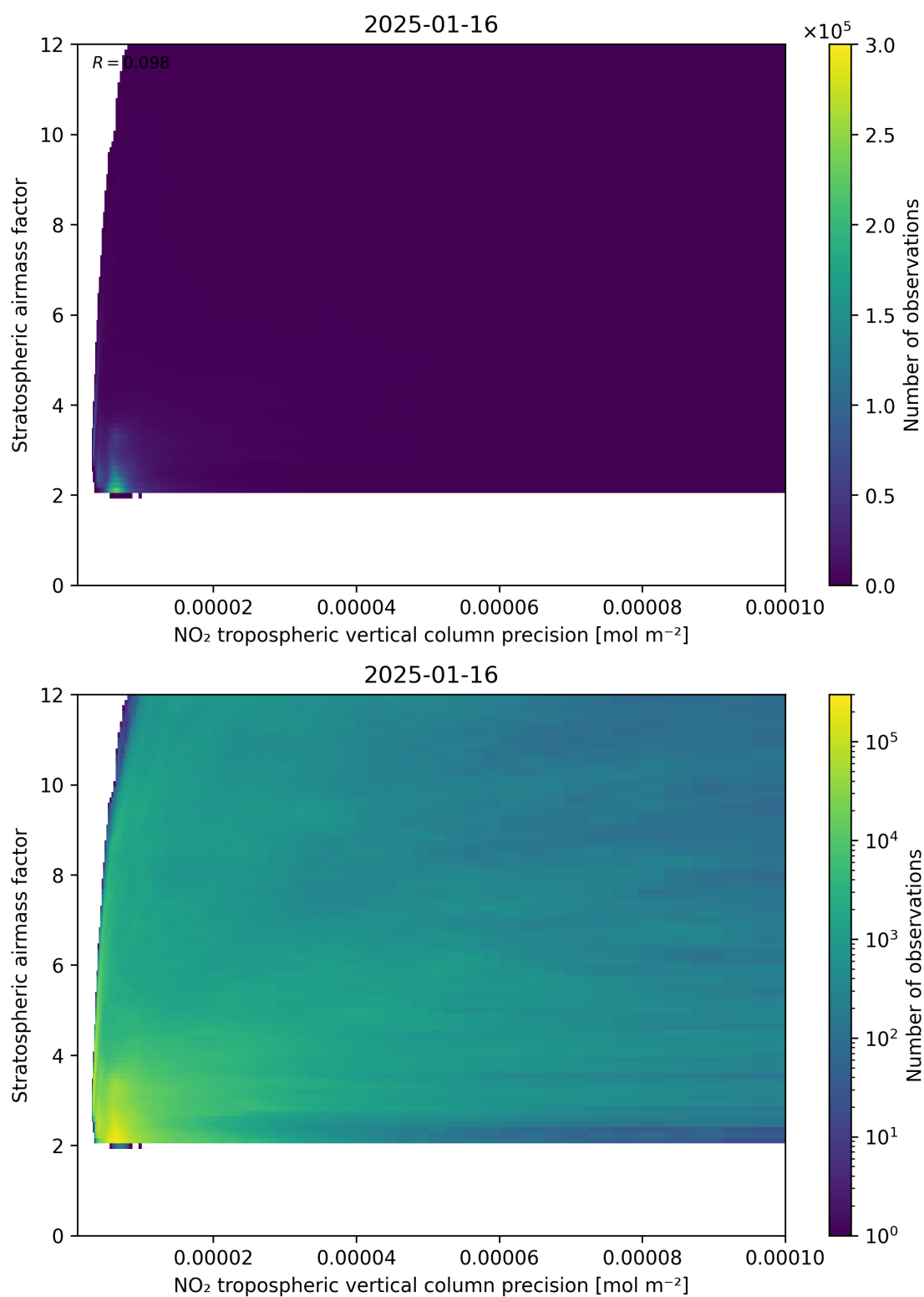
Figure 131: Scatter density plot of “NO 2 tropospheric vertical column precision” against “Stratospheric airmass factor” for 2025-01-15 to 2025-01-17.
