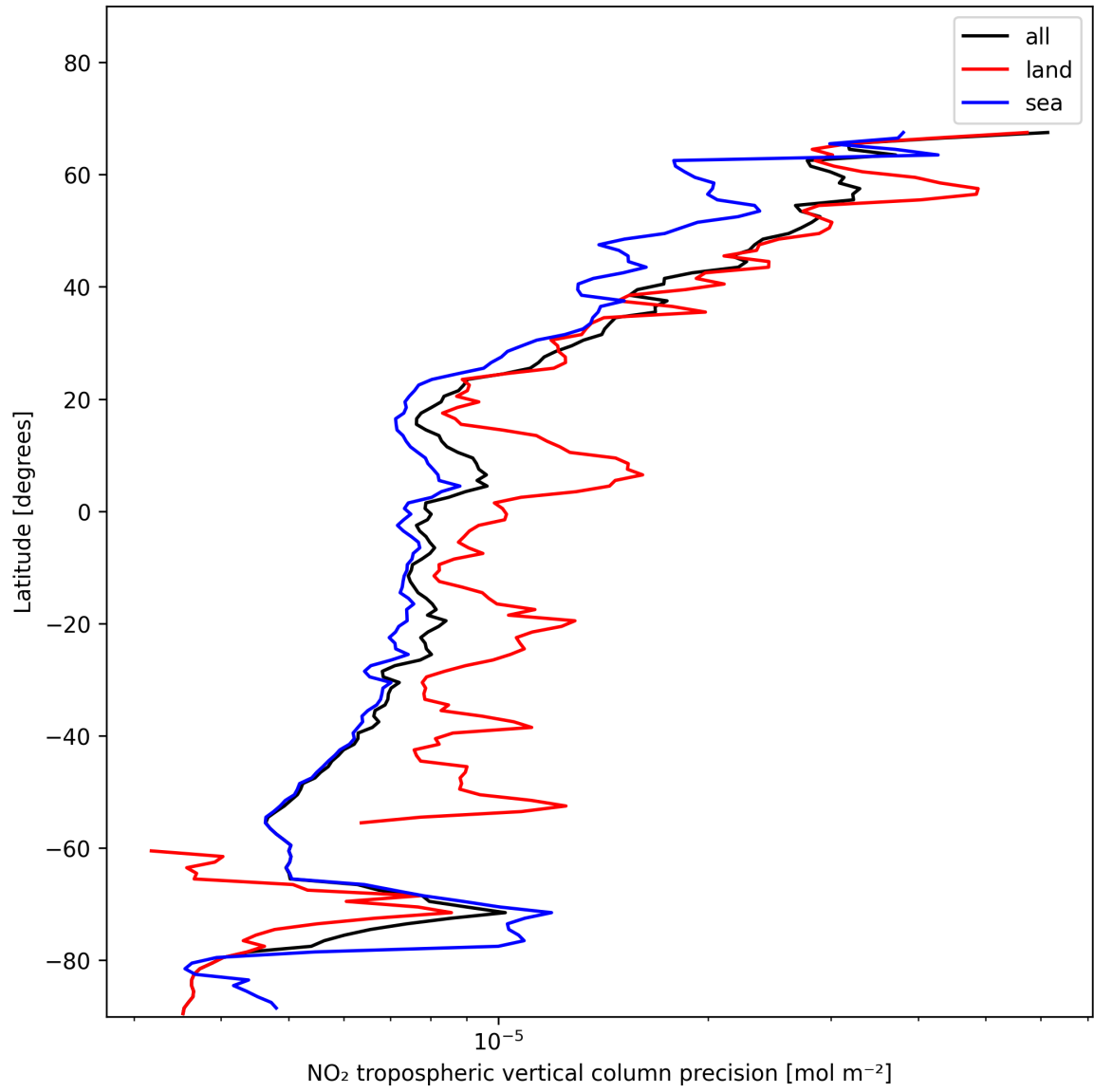
Figure 13: Zonal average of “NO 2 tropospheric vertical column precision” for 2025-01-15 to 2025-01-17.
