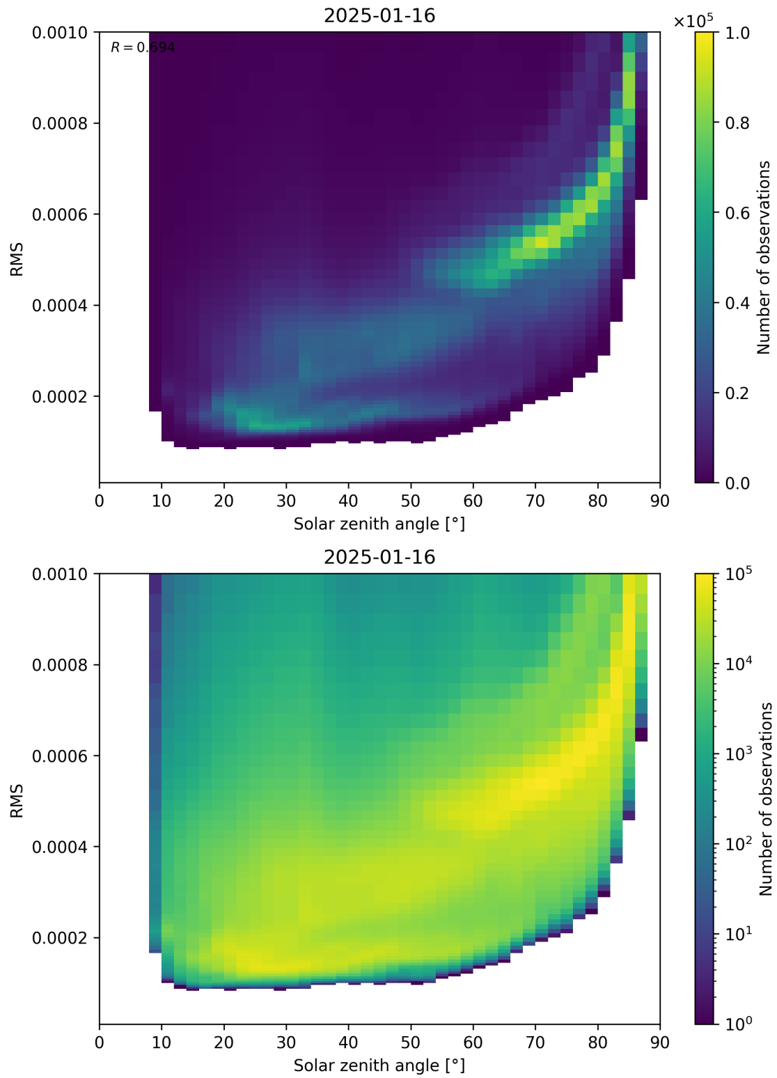
Figure 157: Scatter density plot of “Solar zenith angle” against “RMS” for 2025-01-15 to 2025-01-17.
