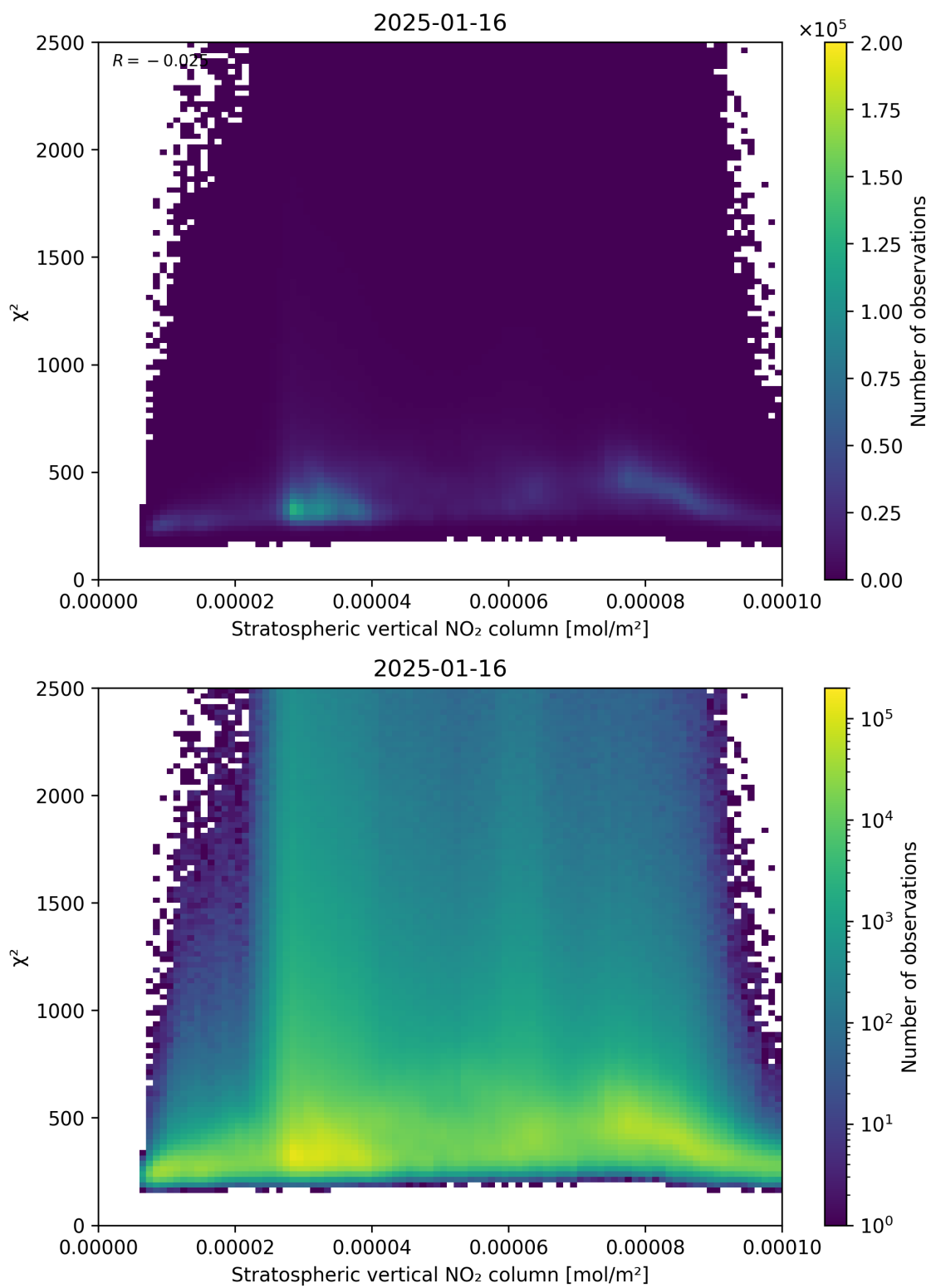
Figure 97: Scatter density plot of “Stratospheric vertical NO 2 column” against “ \chi^2 ” for 2025-01-15 to 2025-01-17.
