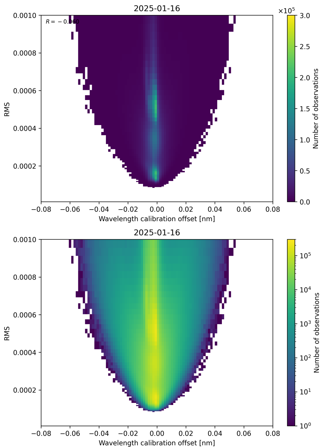
Figure 181: Scatter density plot of “Wavelength calibration offset” against “RMS” for 2025-01-15 to 2025-01-17.
