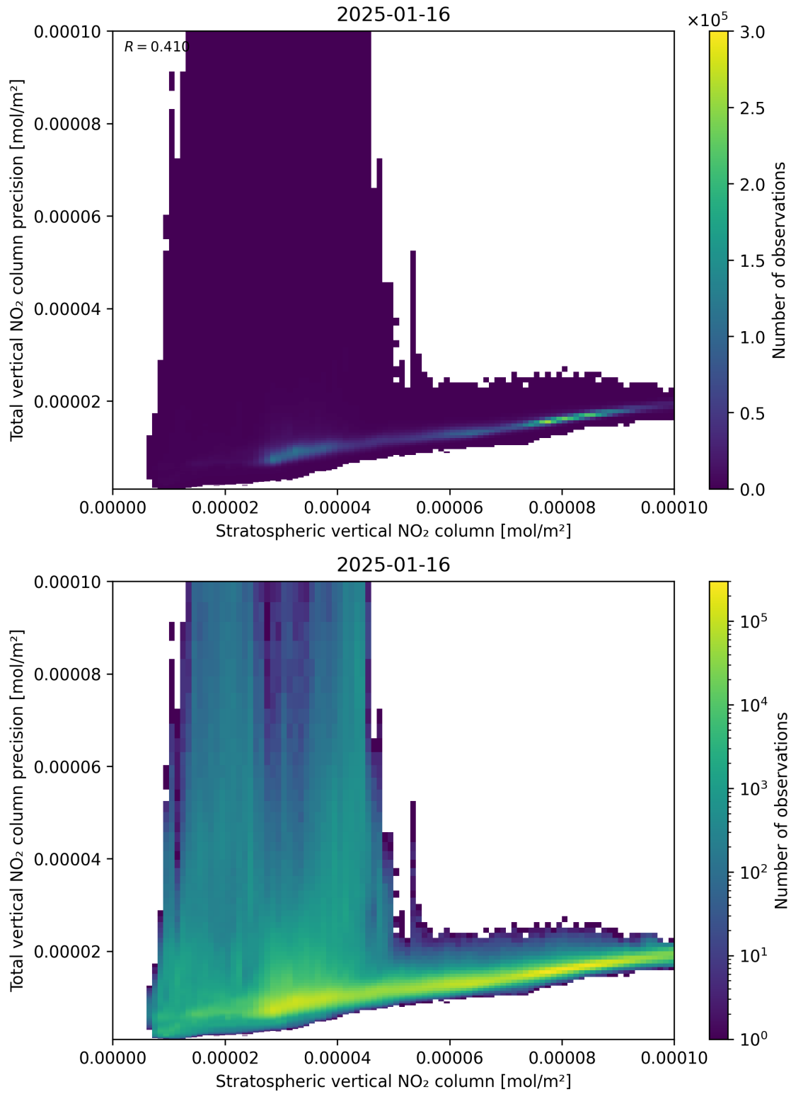
Figure 101: Scatter density plot of “Stratospheric vertical NO 2 column” against “Total vertical NO 2 column precision” for 2025-01-15 to 2025-01-17.
