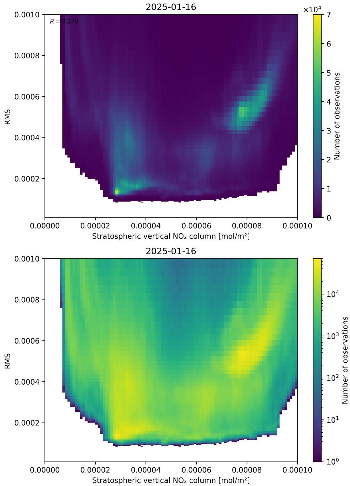
Figure 102: Scatter density plot of “Stratospheric vertical NO 2 column” against “RMS” for 2025-01-15 to 2025-01-17.
