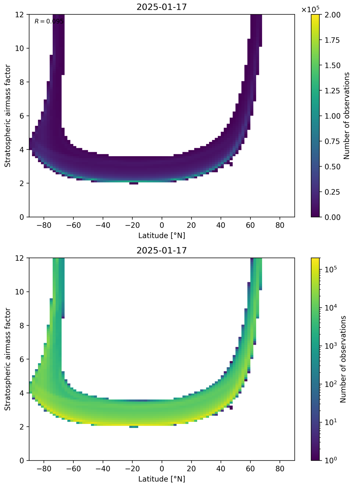
Figure 83: Scatter density plot of “Latitude” against “Stratospheric air mass factor” for 2025-01-17 to 2025-01-18.
