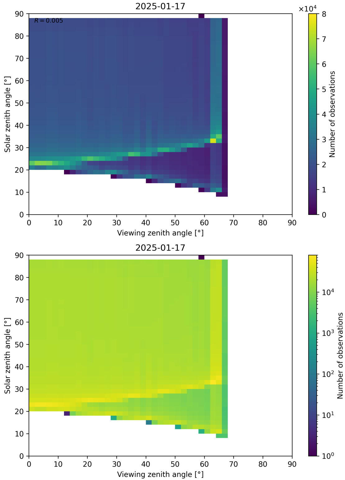
Figure 172: Scatter density plot of “Viewing zenith angle” against “Solar zenith angle” for 2025-01-17 to 2025-01-18.
