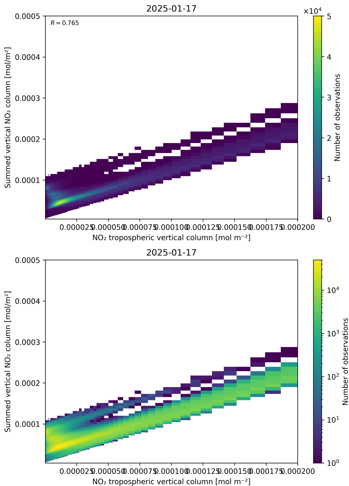
Figure 126: Scatter density plot of “NO 2 tropospheric vertical column” against “Summed vertical NO 2 column” for 2025-01-17 to 2025-01-18.
