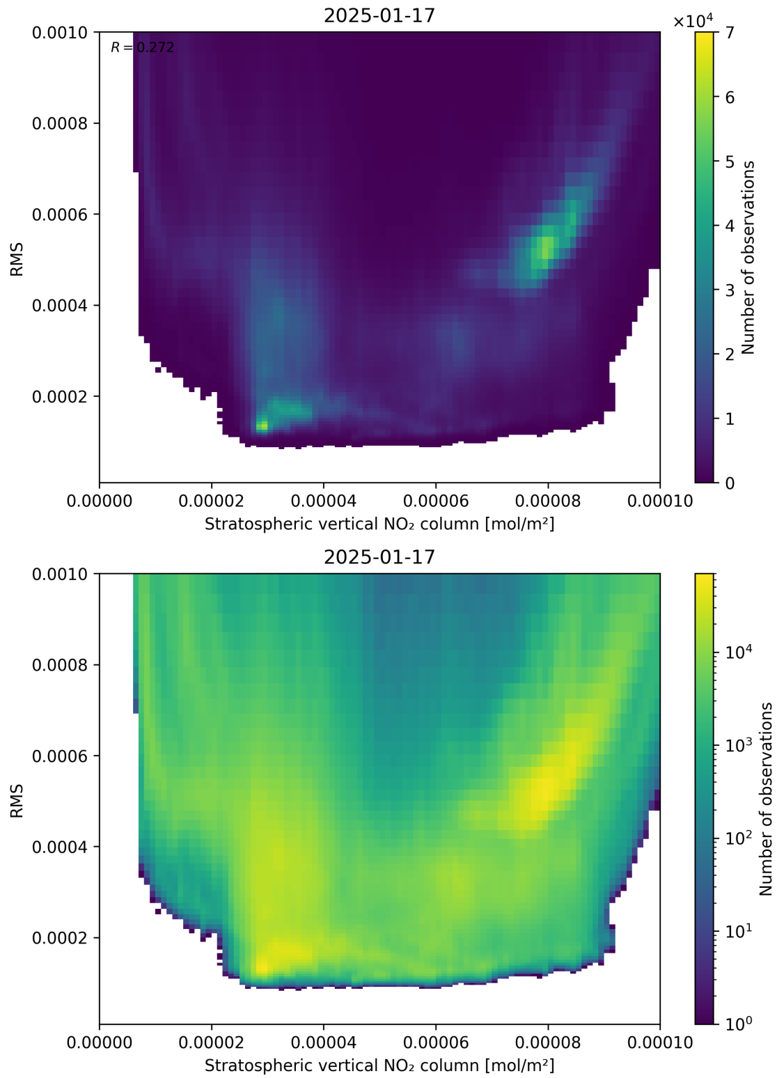
Figure 102: Scatter density plot of “Stratospheric vertical NO 2 column” against “RMS” for 2025-01-17 to 2025-01-18.
