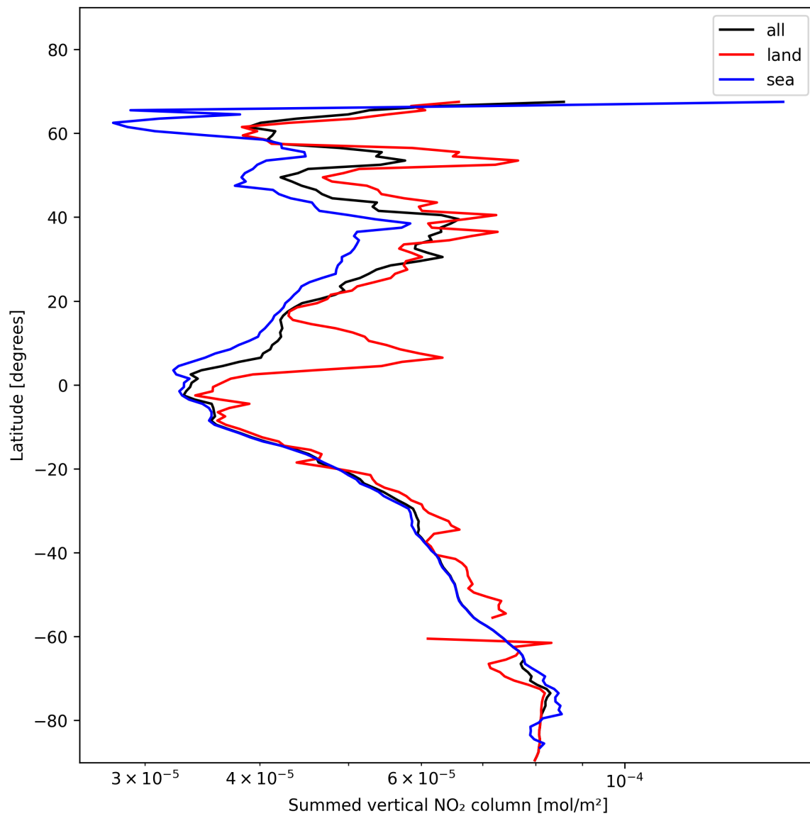
Figure 23: Zonal average of “Summed vertical NO 2 column” for 2025-01-17 to 2025-01-18.
