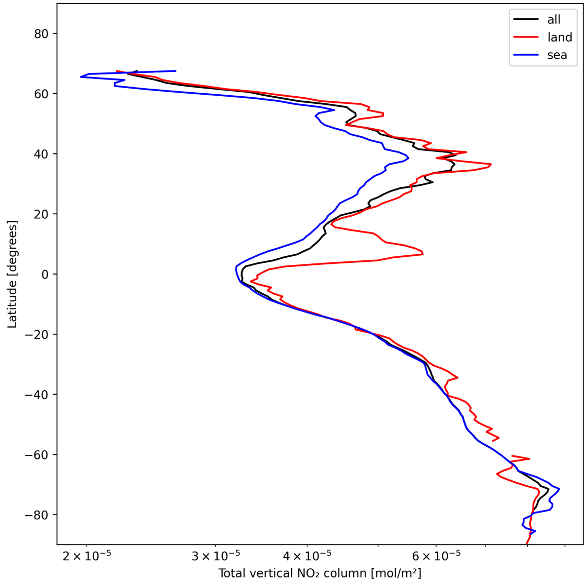
Figure 21: Zonal average of “Total vertical NO 2 column” for 2025-01-17 to 2025-01-18.
