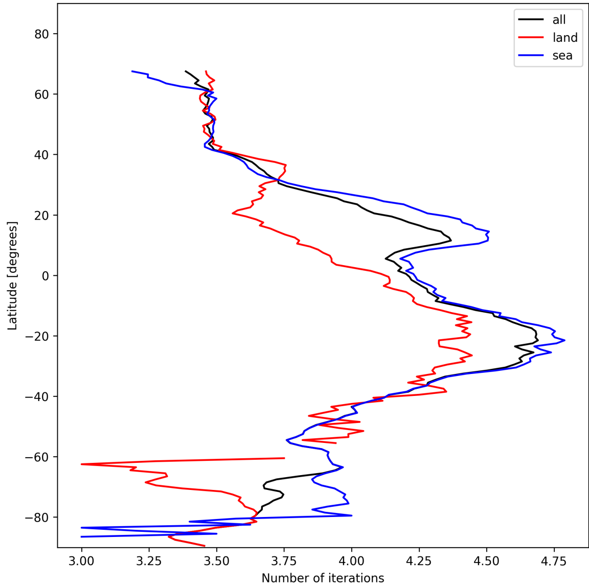
Figure 17: Zonal average of “Number of iterations” for 2025-01-17 to 2025-01-18.
