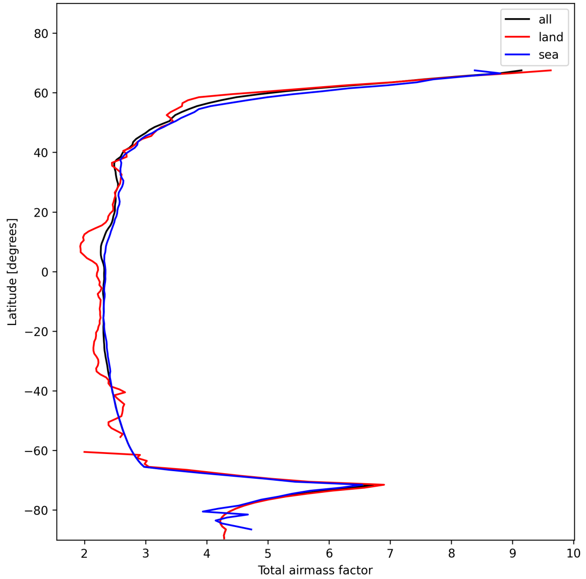
Figure 15: Zonal average of “Total airmass factor” for 2025-01-17 to 2025-01-18.
