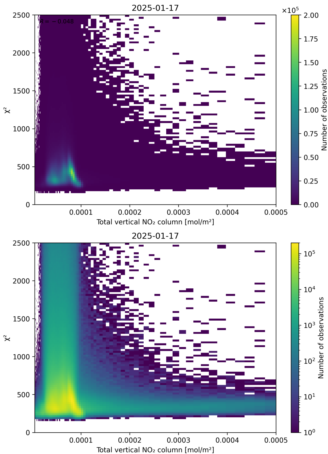
Figure 111: Scatter density plot of “Total vertical NO 2 column” against “ \chi^2 ” for 2025-01-17 to 2025-01-18.
