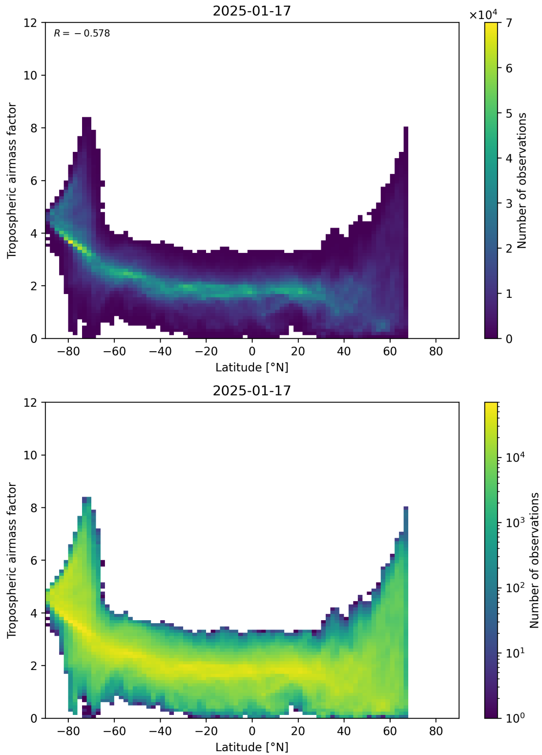
Figure 85: Scatter density plot of “Latitude” against “Tropospheric air mass factor” for 2025-01-17 to 2025-01-18.
