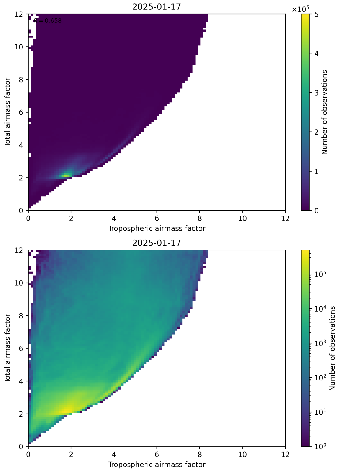
Figure 72: Scatter density plot of “Tropospheric airmass factor” against “Total airmass factor” for 2025-01-17 to 2025-01-18.
