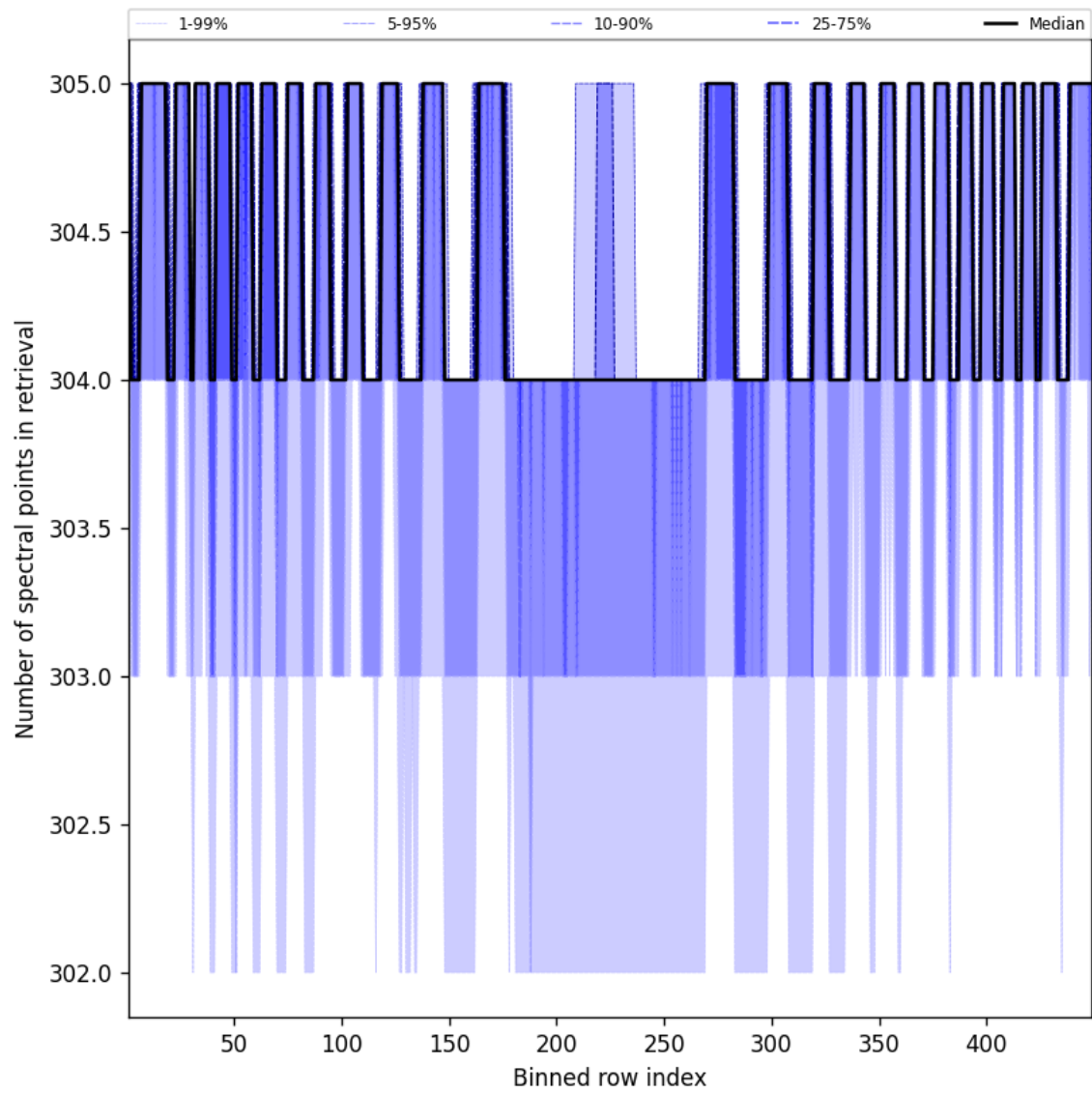
Figure 50: Along track statistics of “Number of spectral points in retrieval” for 2025-01-17 to 2025-01-18
