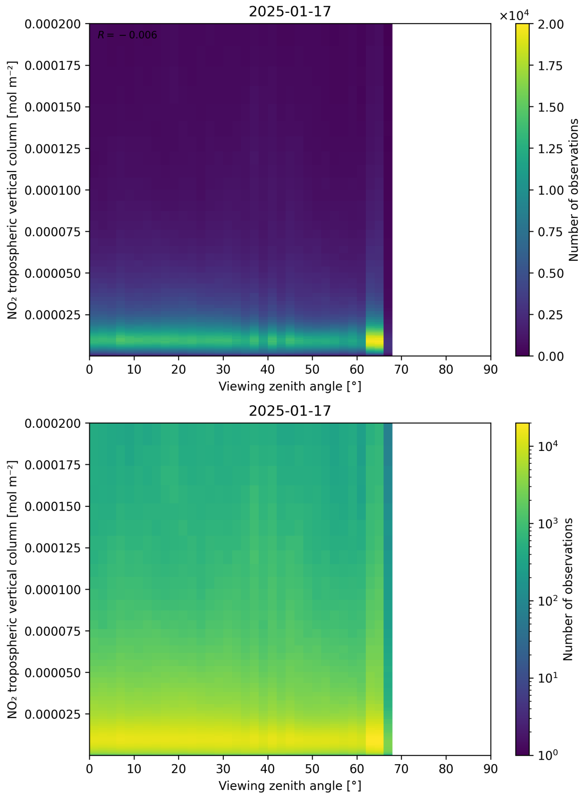
Figure 169: Scatter density plot of “Viewing zenith angle” against “NO 2 tropospheric vertical column” for 2025-01-17 to 2025-01-18.
