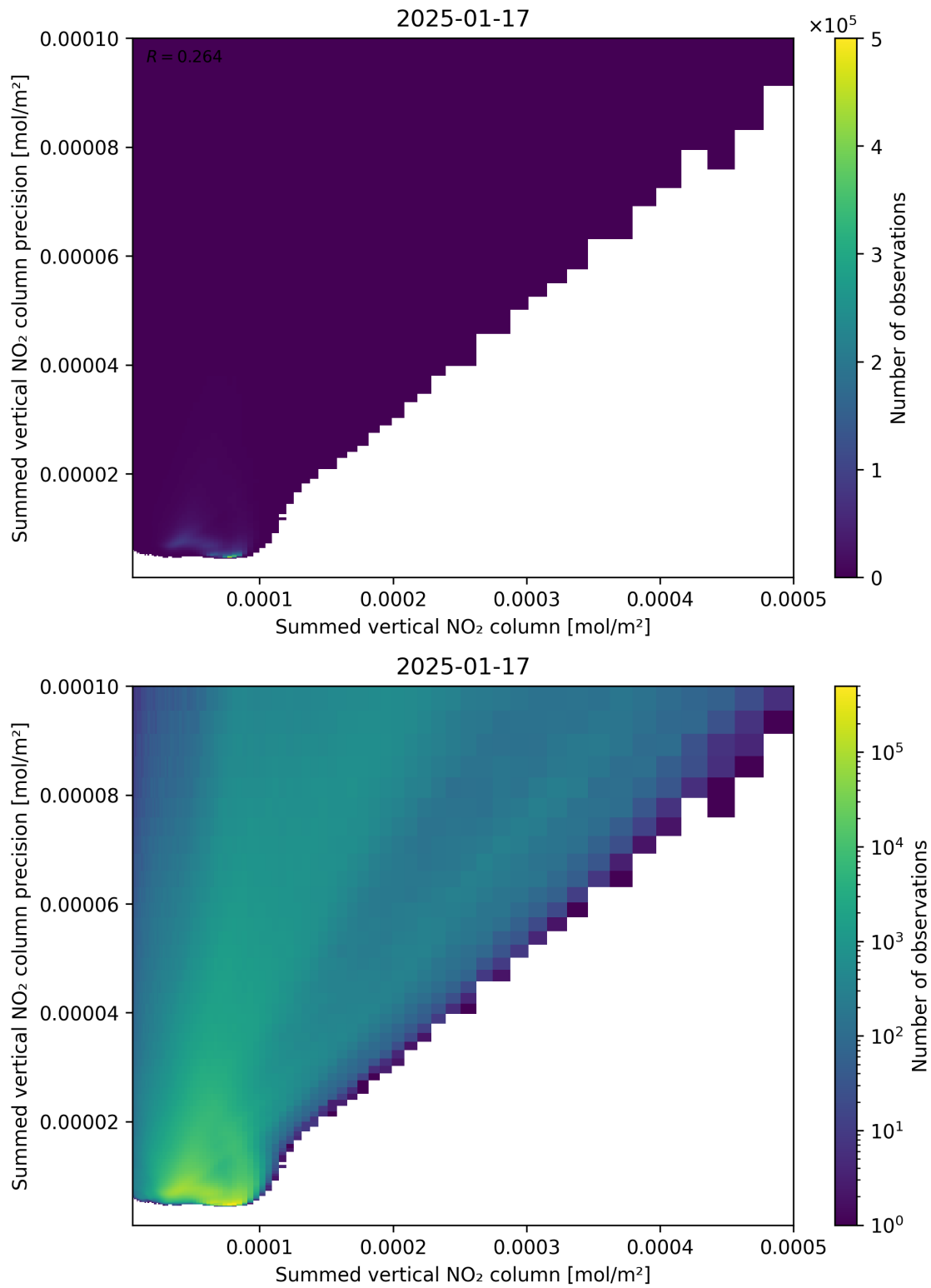
Figure 105: Scatter density plot of “Summed vertical NO 2 column” against “Summed vertical NO 2 column precision” for 2025-01-17 to 2025-01-18.
