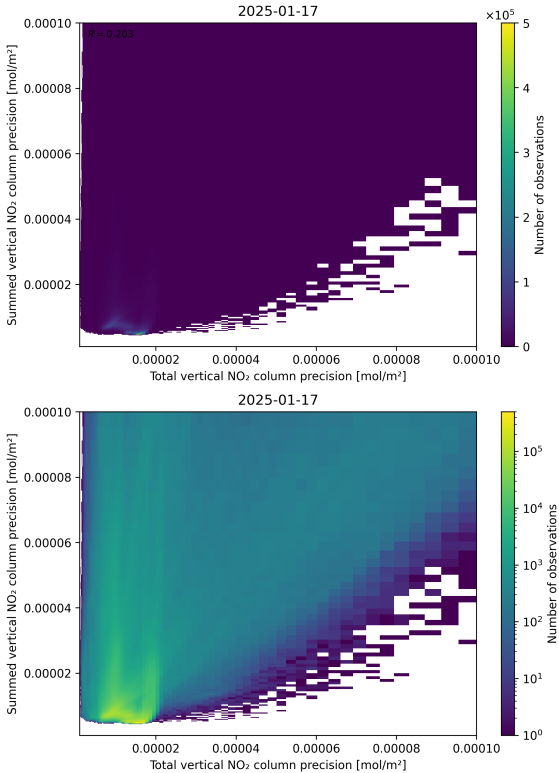
Figure 118: Scatter density plot of “Total vertical NO 2 column precision” against “Summed vertical NO 2 column precision” for 2025-01-17 to 2025-01-18.
