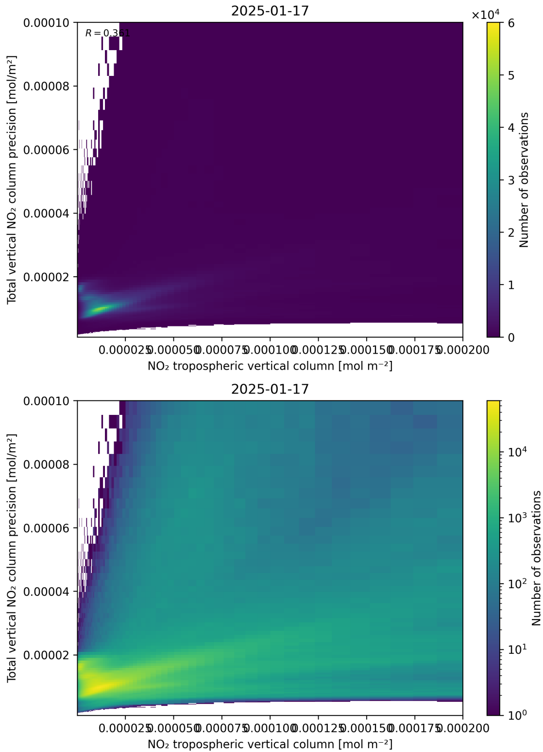
Figure 129: Scatter density plot of “NO 2 tropospheric vertical column” against “Total vertical NO 2 column precision” for 2025-01-17 to 2025-01-18.
