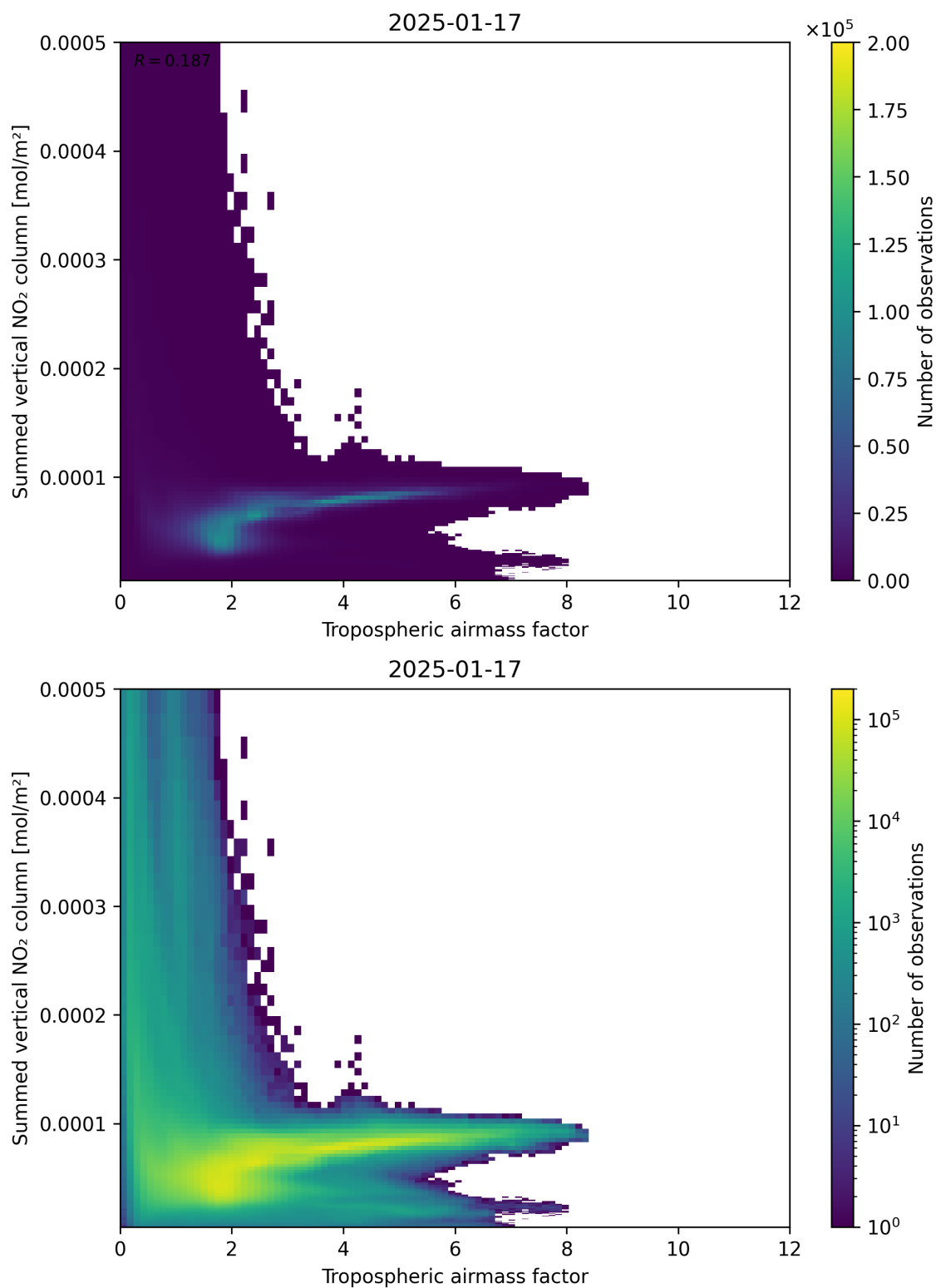
Figure 75: Scatter density plot of “Tropospheric air mass factor” against “Summed vertical NO 2 column” for 2025-01-17 to 2025-01-18.
