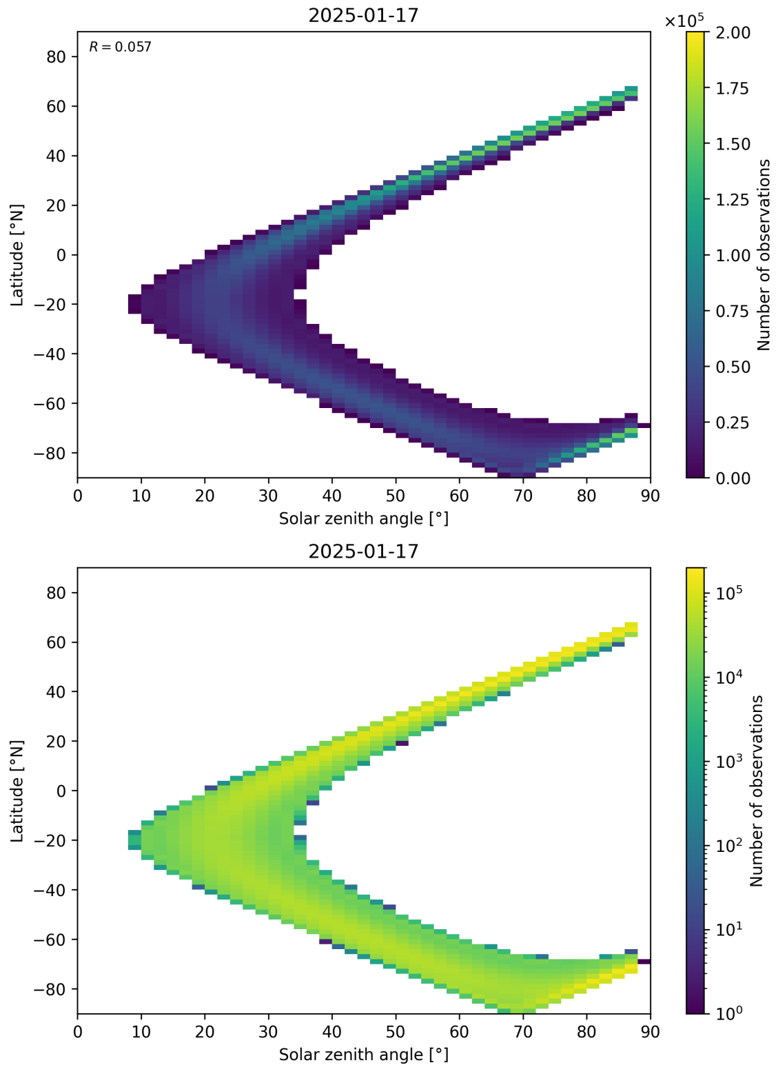
Figure 149: Scatter density plot of “Solar zenith angle” against “Latitude” for 2025-01-17 to 2025-01-18.
