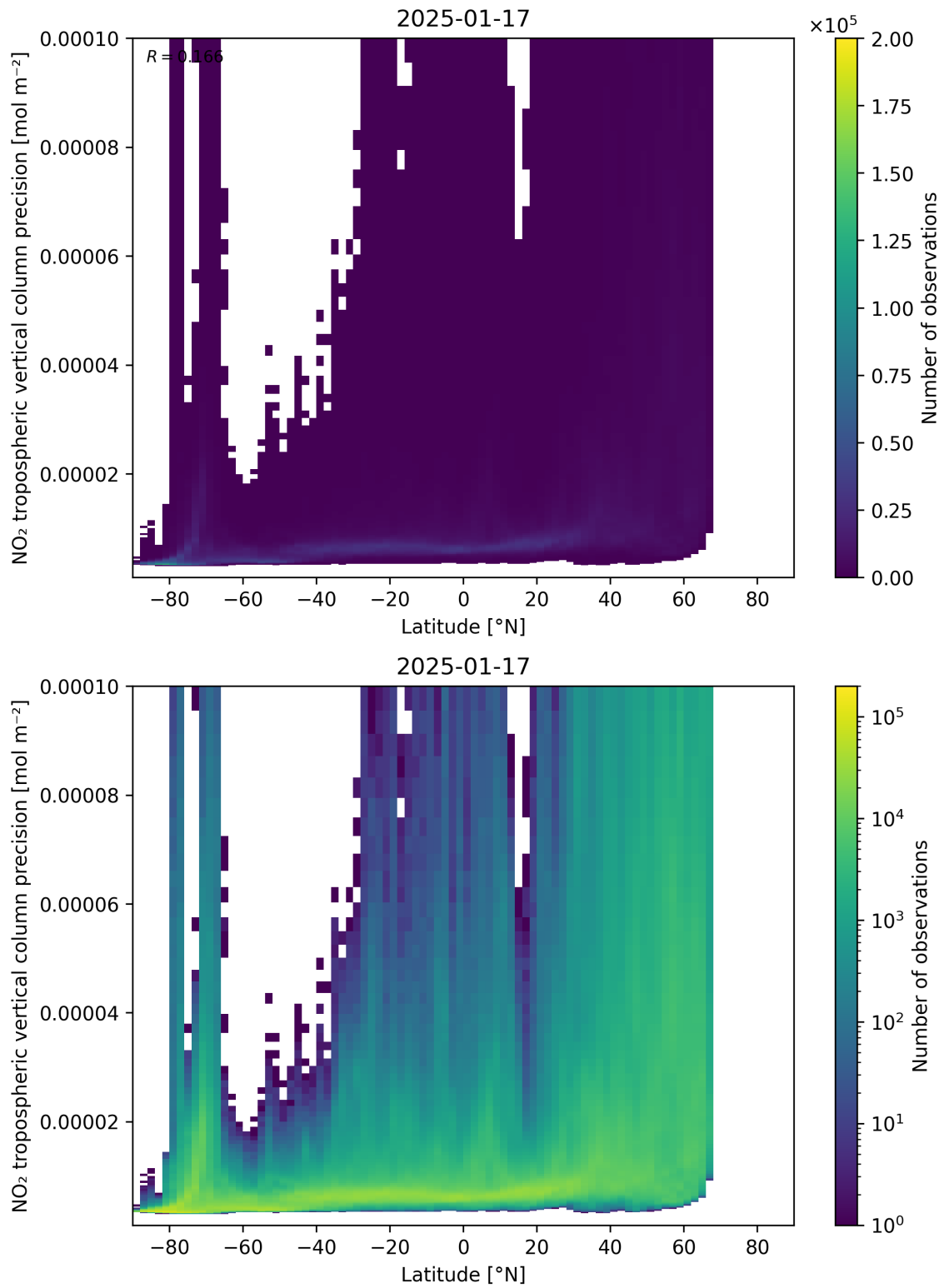
Figure 93: Scatter density plot of “Latitude” against “NO 2 tropospheric vertical column precision” for 2025-01-17 to 2025-01-18.
