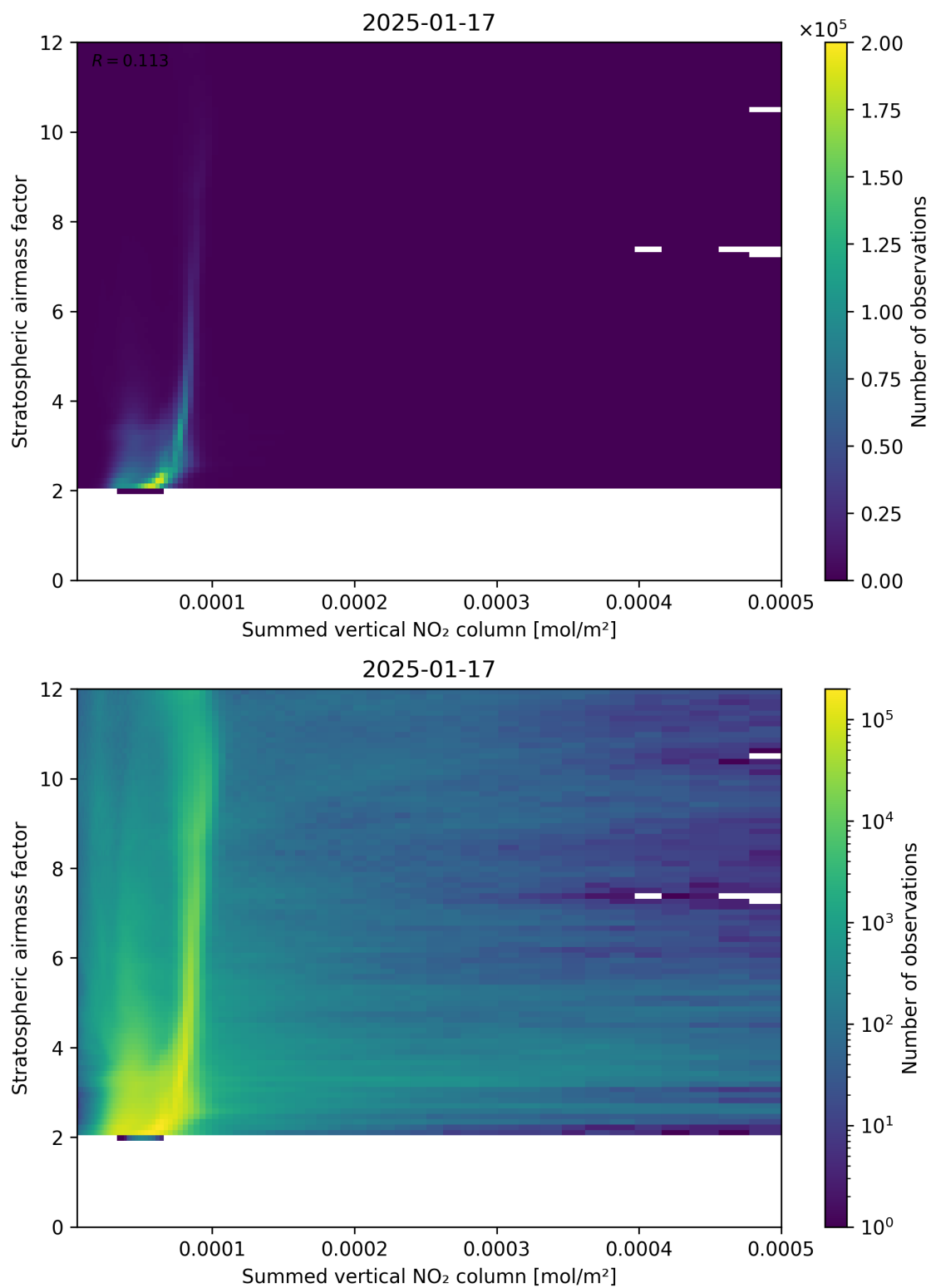
Figure 103: Scatter density plot of “Summed vertical NO 2 column” against “Stratospheric air mass factor” for 2025-01-17 to 2025-01-18.
