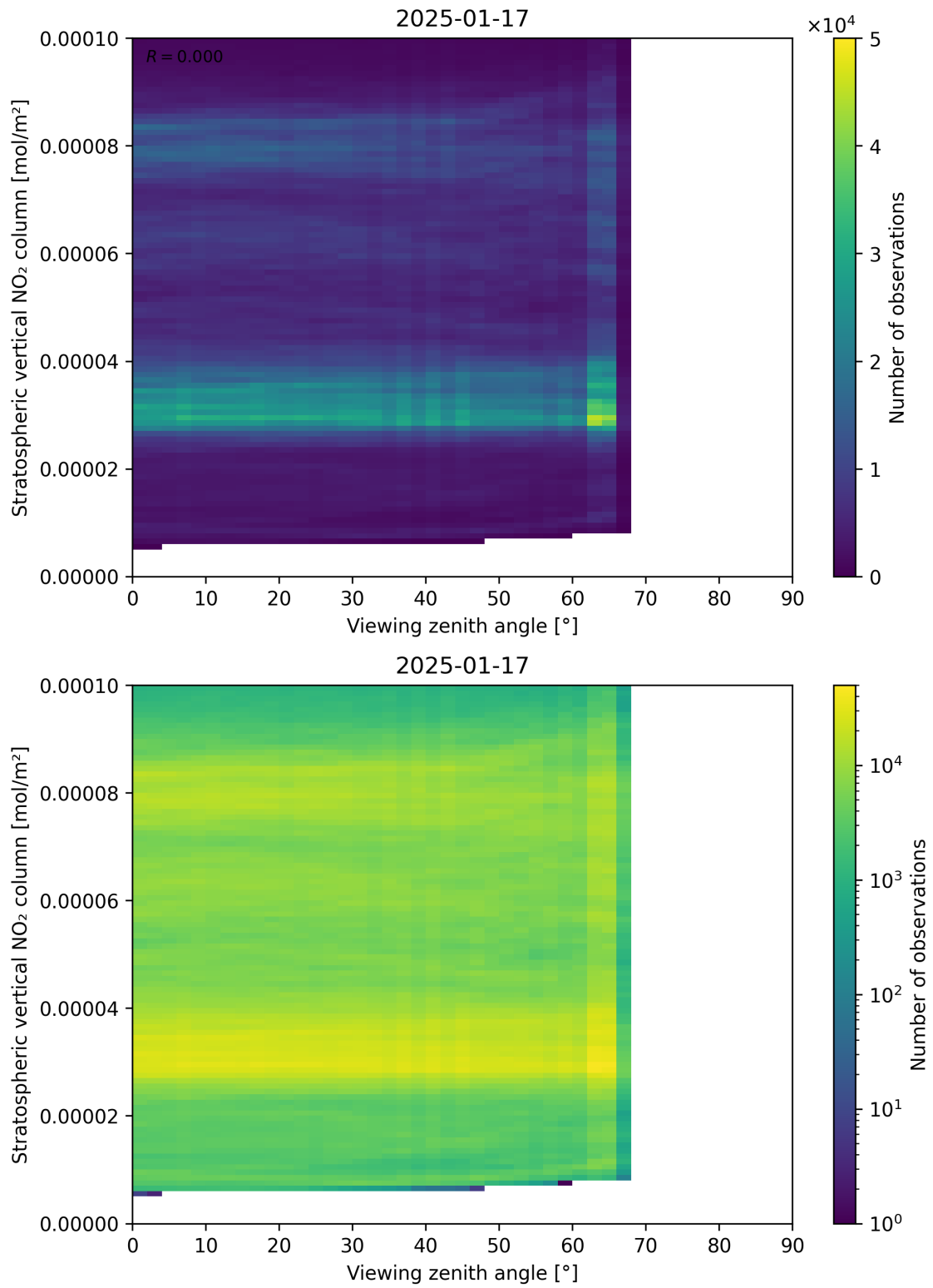
Figure 164: Scatter density plot of “Viewing zenith angle” against “Stratospheric vertical NO 2 column” for 2025-01-17 to 2025-01-18.
