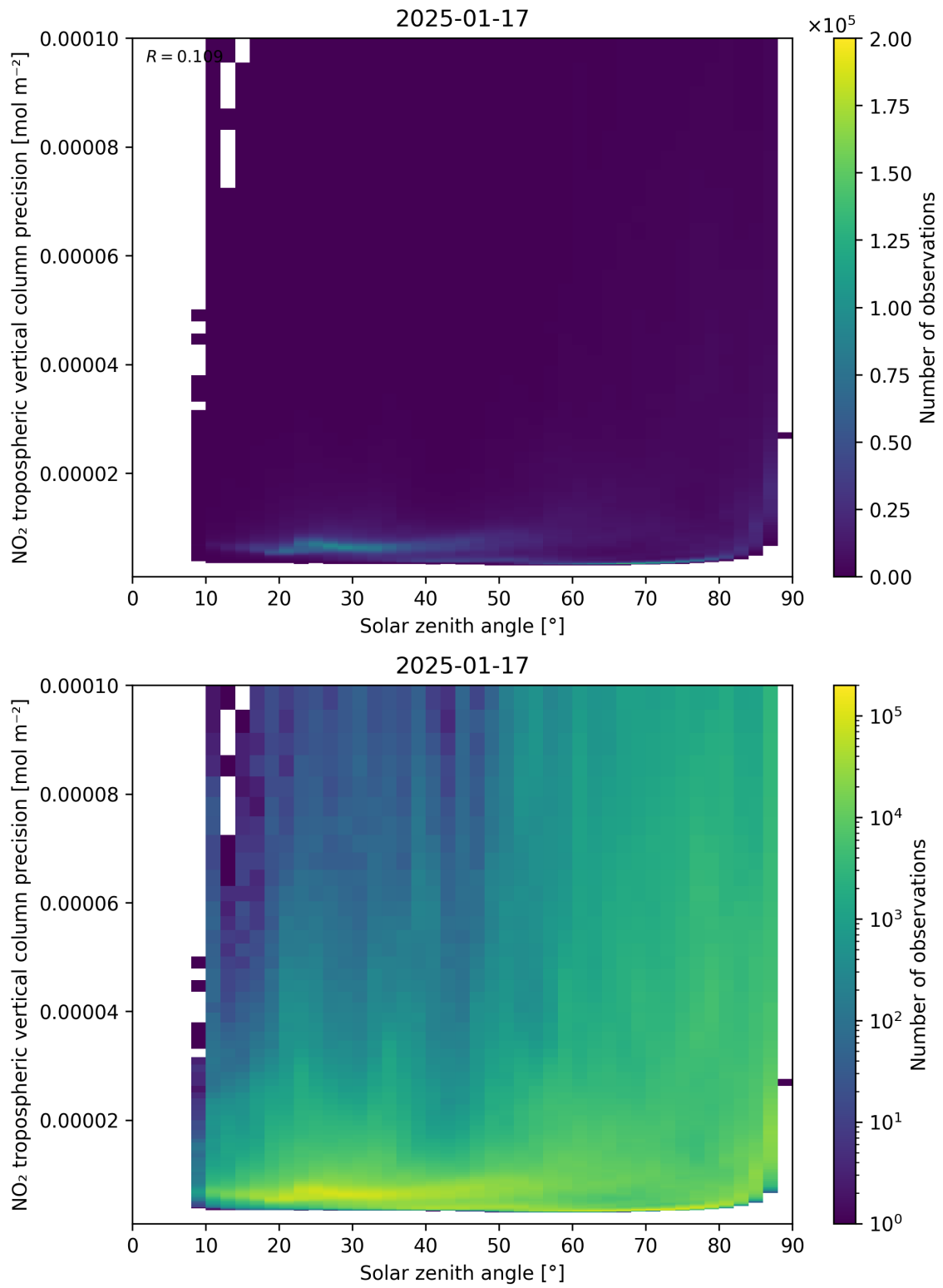
Figure 156: Scatter density plot of “Solar zenith angle” against “NO 2 tropospheric vertical column precision” for 2025-01-17 to 2025-01-18.
