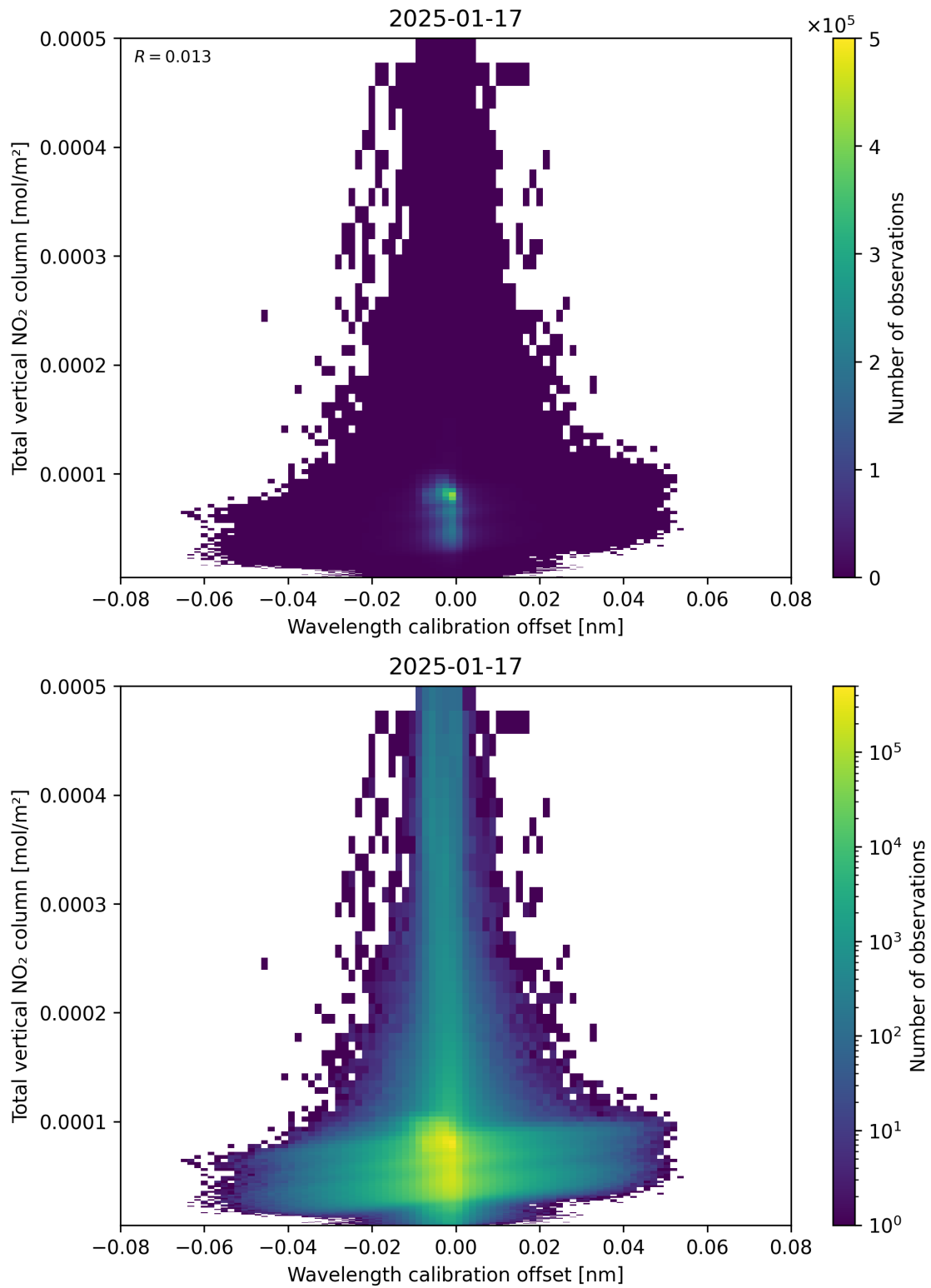
Figure 179: Scatter density plot of “Wavelength calibration offset” against “Total vertical NO 2 column” for 2025-01-17 to 2025-01-18.
