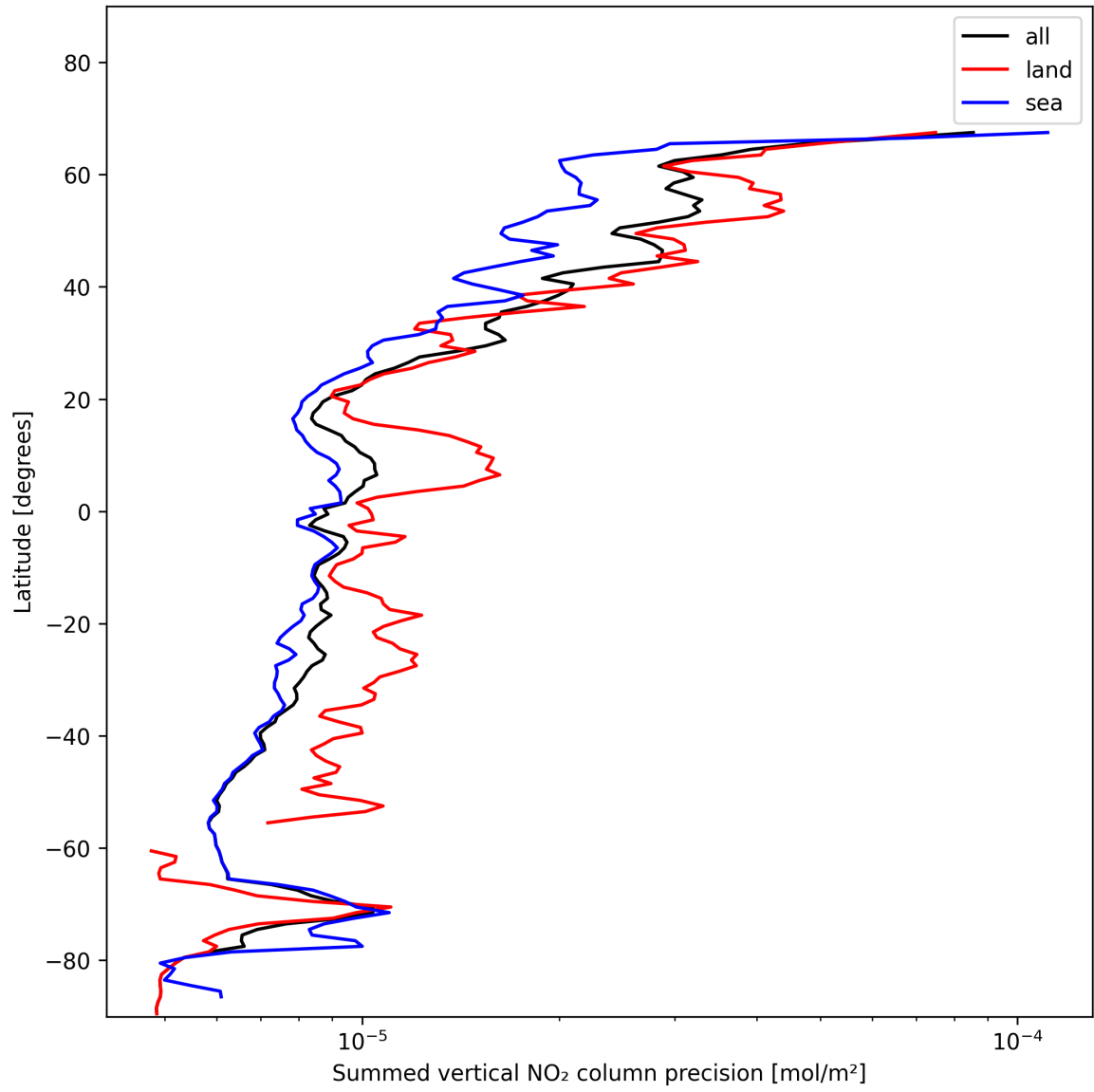
Figure 24: Zonal average of “Summed vertical NO 2 column precision” for 2025-01-17 to 2025-01-18.
