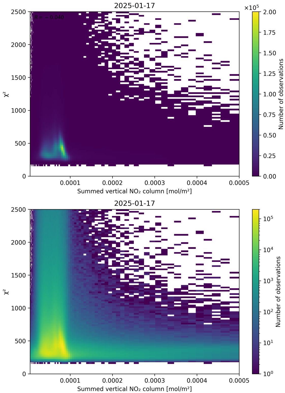
Figure 104: Scatter density plot of “Summed vertical NO 2 column” against “ \chi^2 ” for 2025-01-17 to 2025-01-18.
