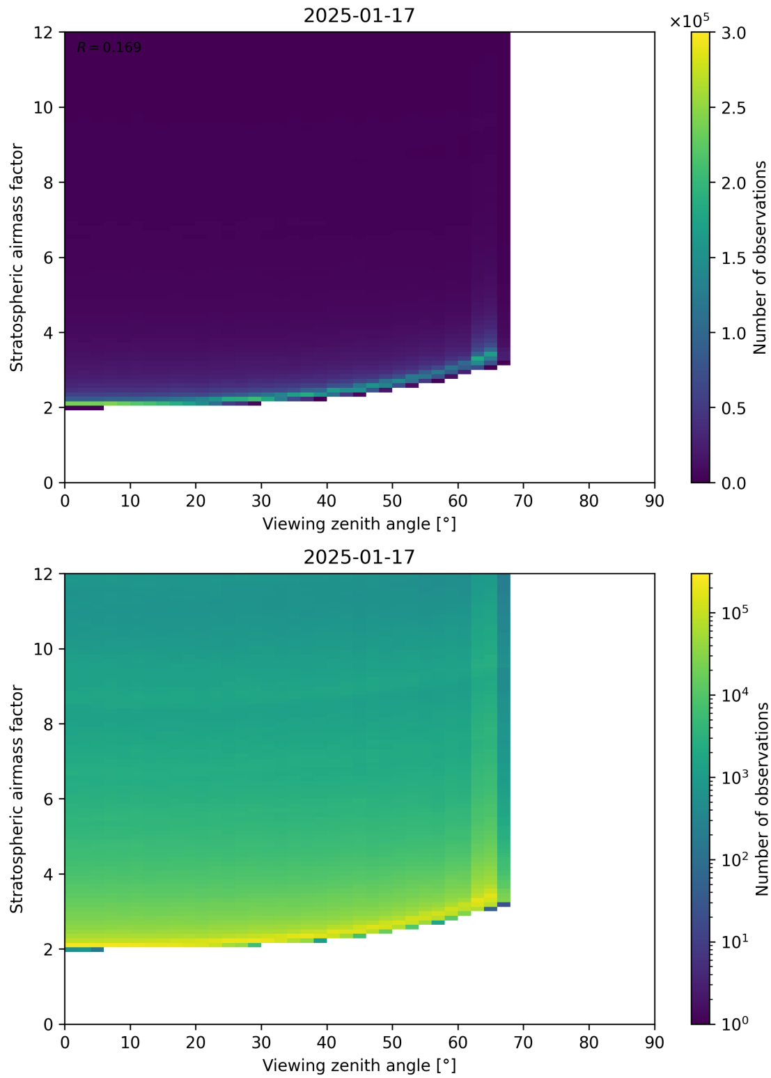
Figure 159: Scatter density plot of “Viewing zenith angle” against “Stratospheric airmass factor” for 2025-01-17 to 2025-01-18.
