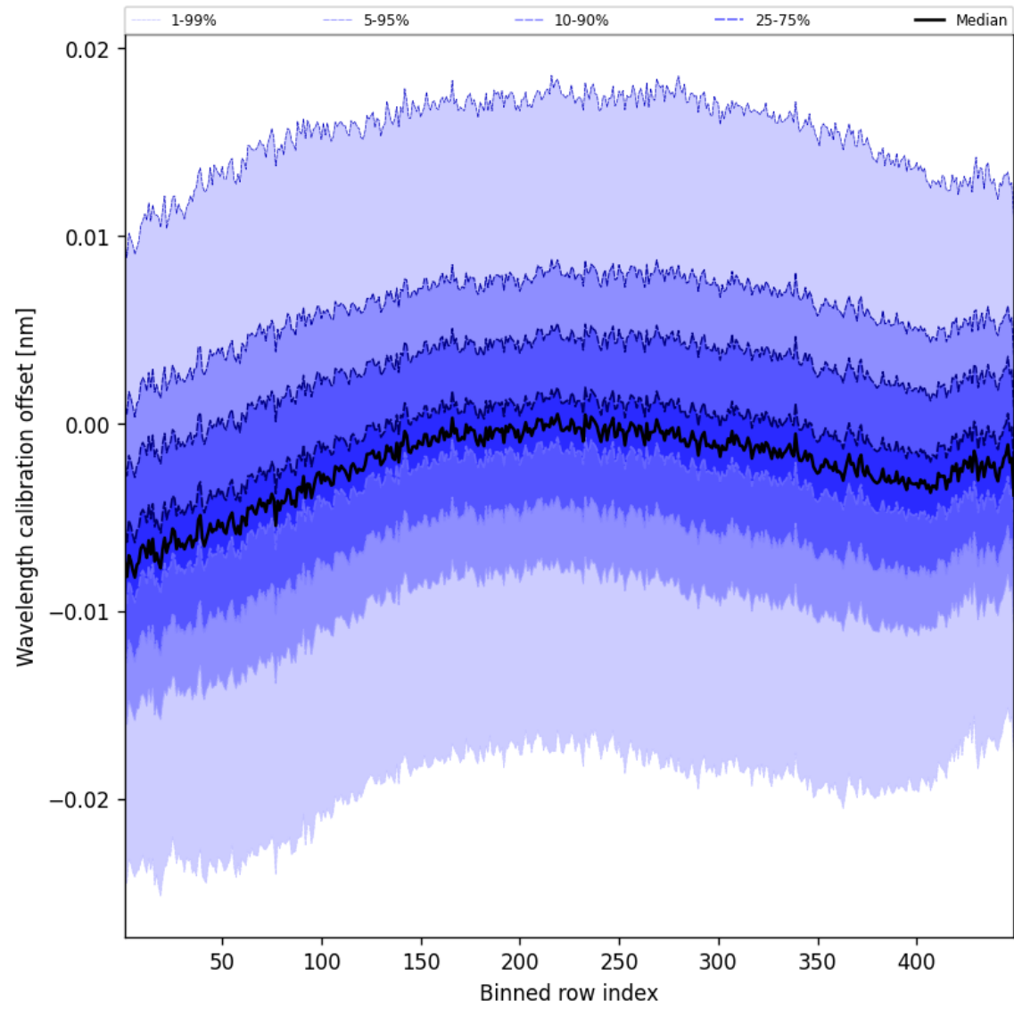
Figure 52: Along track statistics of “Wavelength calibration offset” for 2025-01-17 to 2025-01-18
