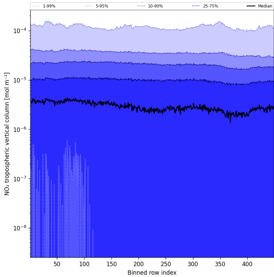
Figure 46: Along track statistics of “NO 2 tropospheric vertical column” for 2025-01-17 to 2025-01-18
