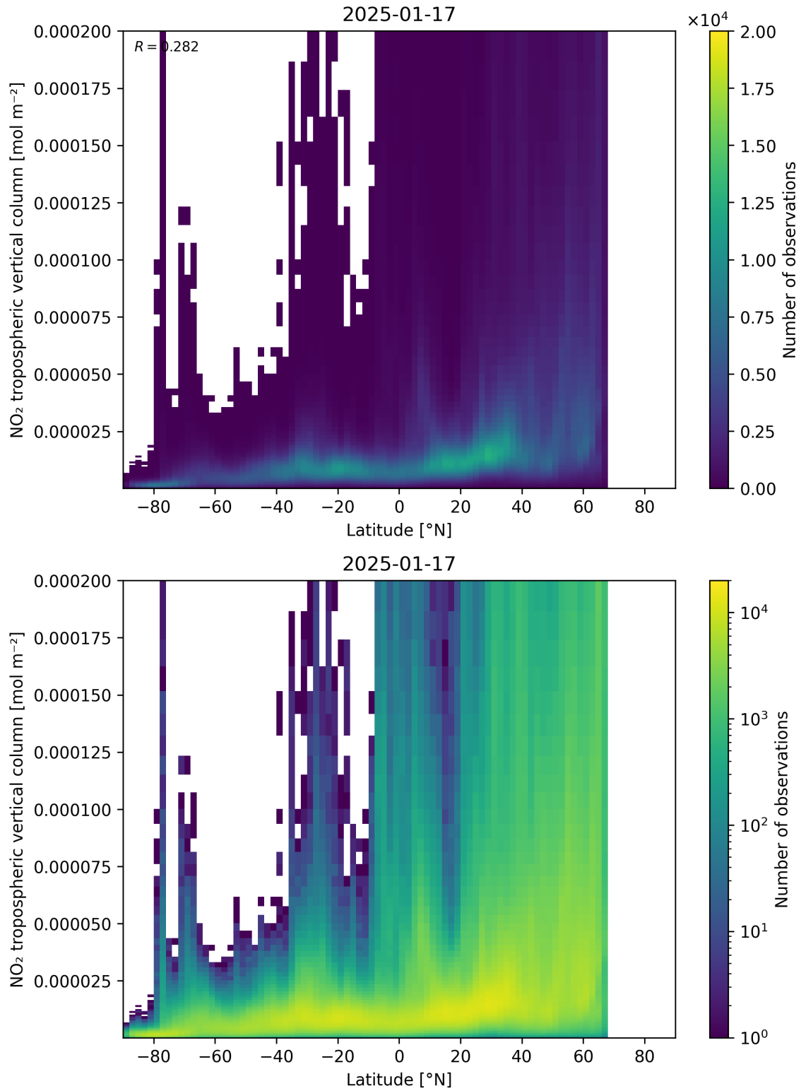
Figure 92: Scatter density plot of “Latitude” against “NO 2 tropospheric vertical column” for 2025-01-17 to 2025-01-18.
