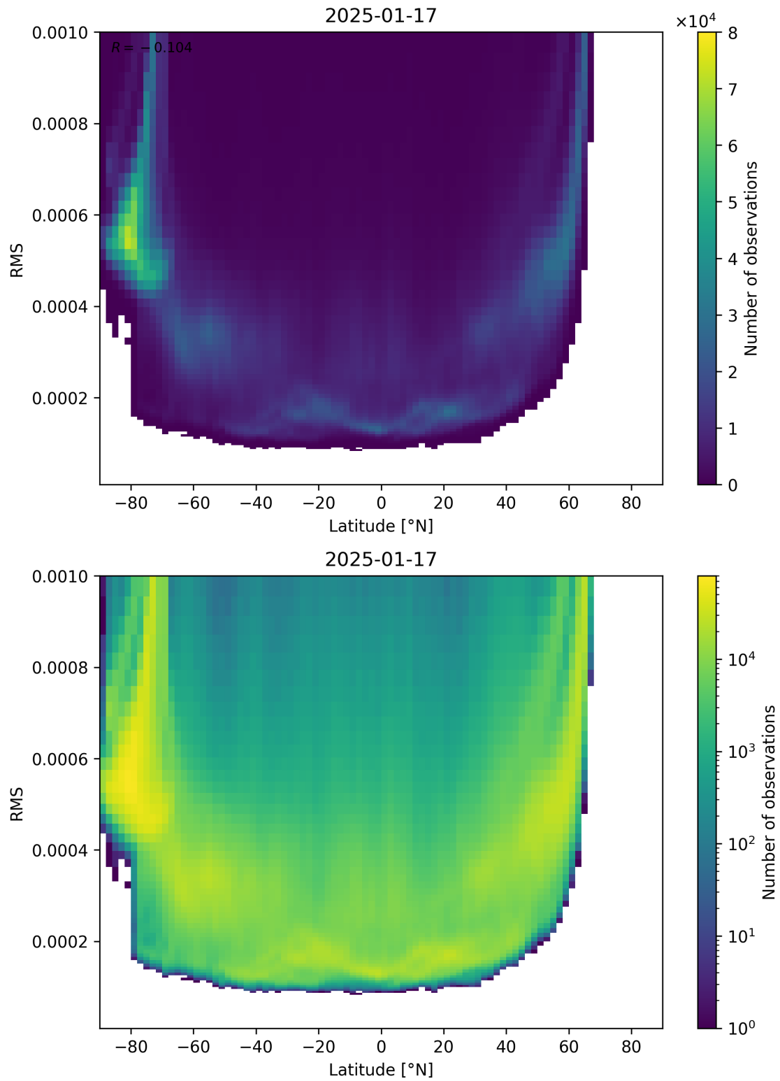
Figure 94: Scatter density plot of “Latitude” against “RMS” for 2025-01-17 to 2025-01-18.
