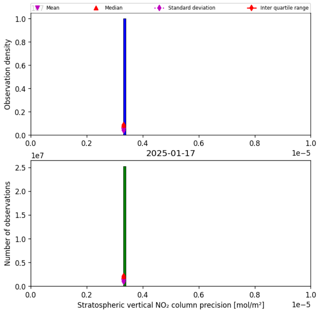
Figure 37: Histogram of “Stratospheric vertical NO 2 column precision” for 2025-01-17 to 2025-01-18
