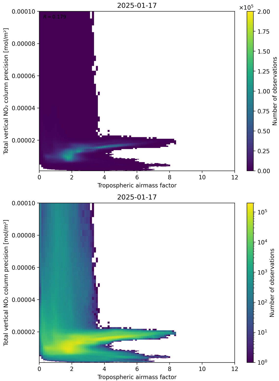
Figure 78: Scatter density plot of “Tropospheric air mass factor” against “Total vertical NO 2 column precision” for 2025-01-17 to 2025-01-18.
