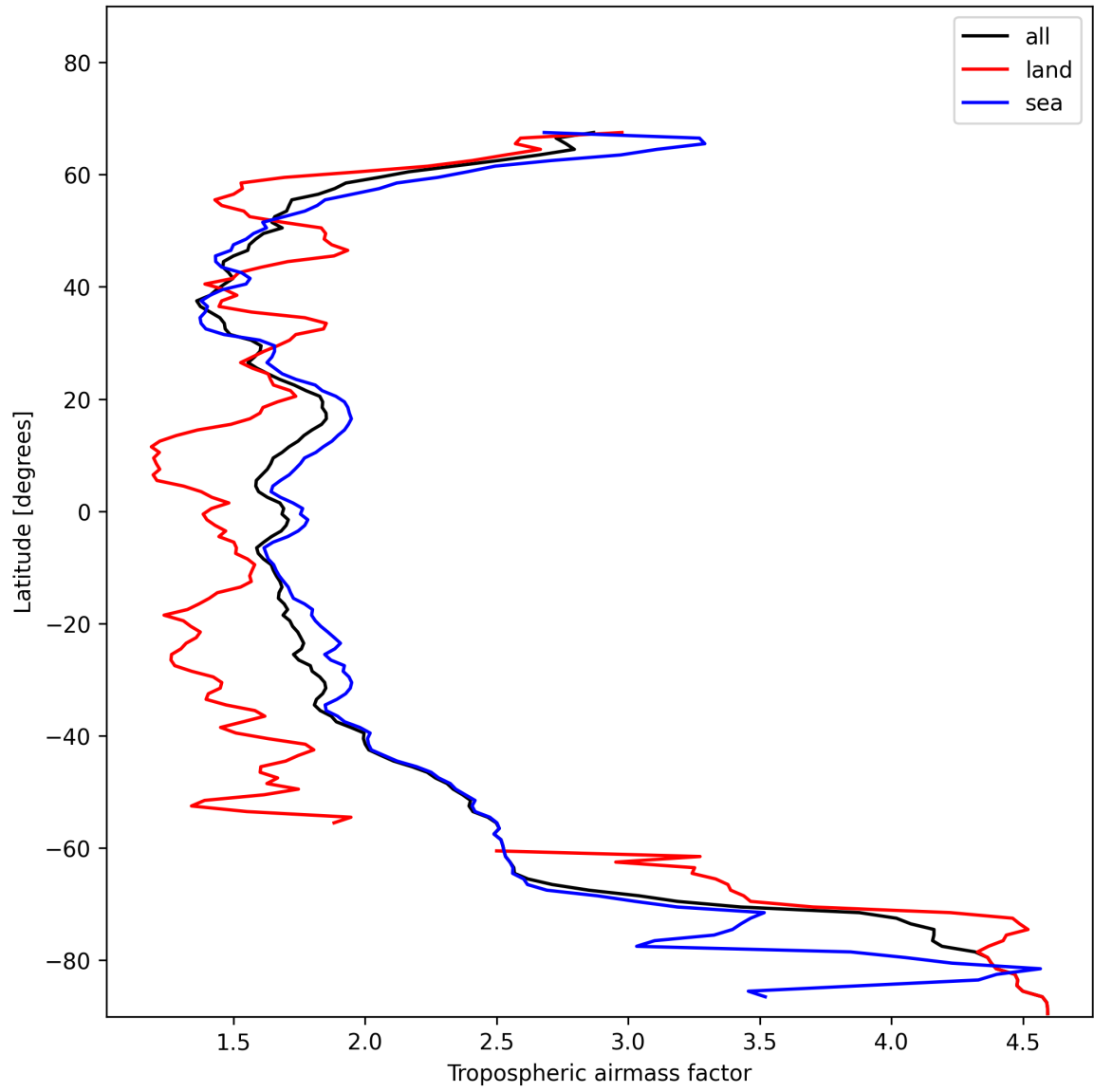
Figure 14: Zonal average of “Tropospheric airmass factor” for 2025-01-17 to 2025-01-18.
