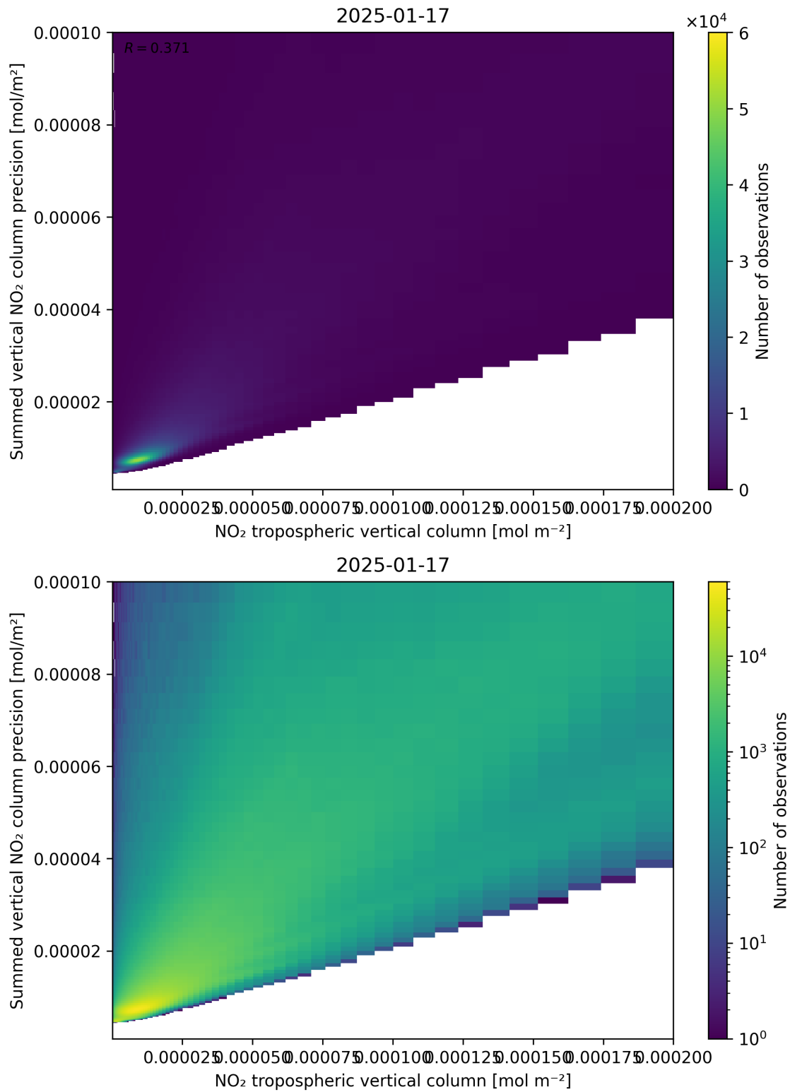
Figure 127: Scatter density plot of “NO 2 tropospheric vertical column” against “Summed vertical NO 2 column precision” for 2025-01-17 to 2025-01-18.
