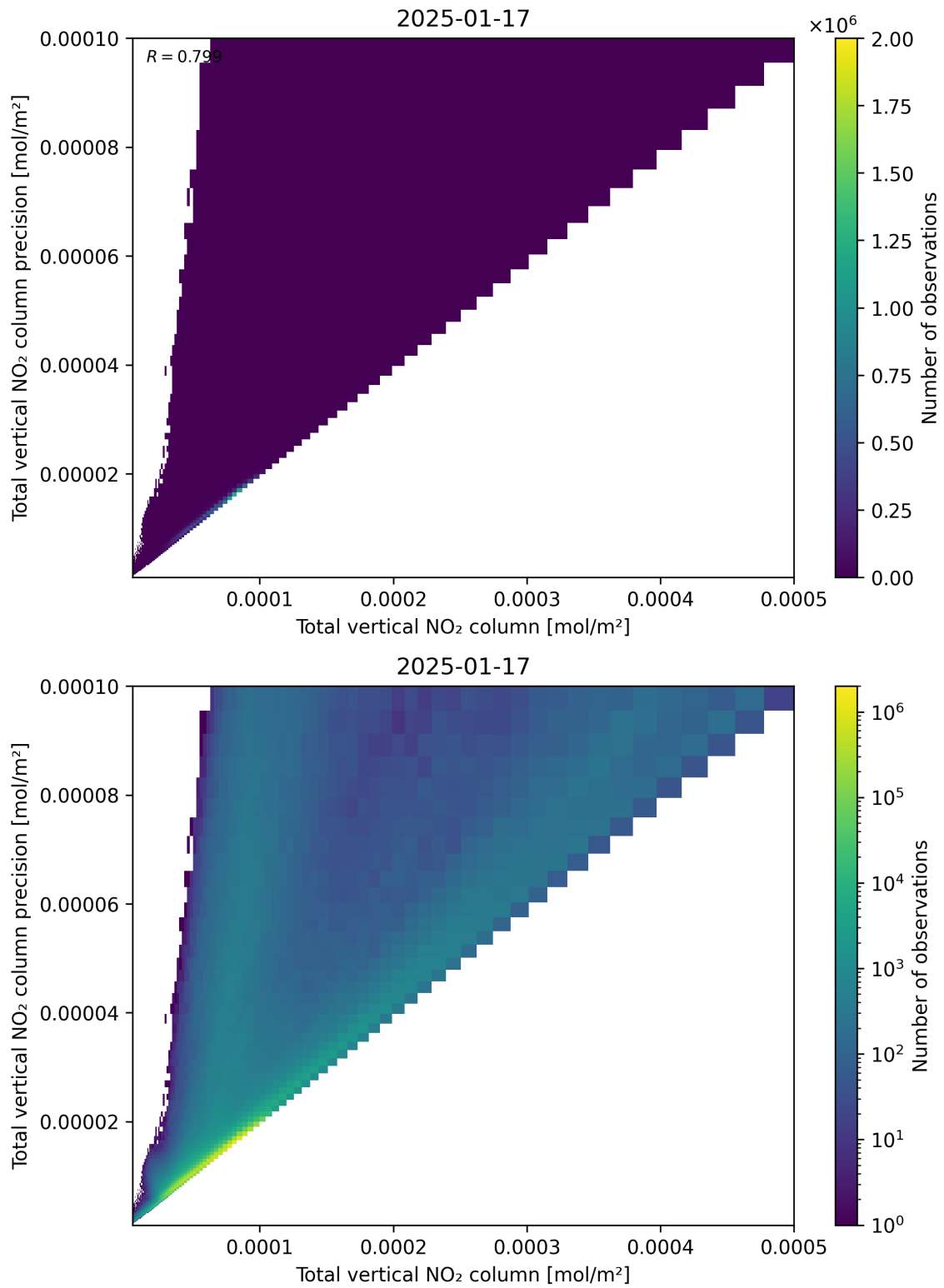
Figure 114: Scatter density plot of “Total vertical NO 2 column” against “Total vertical NO 2 column precision” for 2025-01-17 to 2025-01-18.
