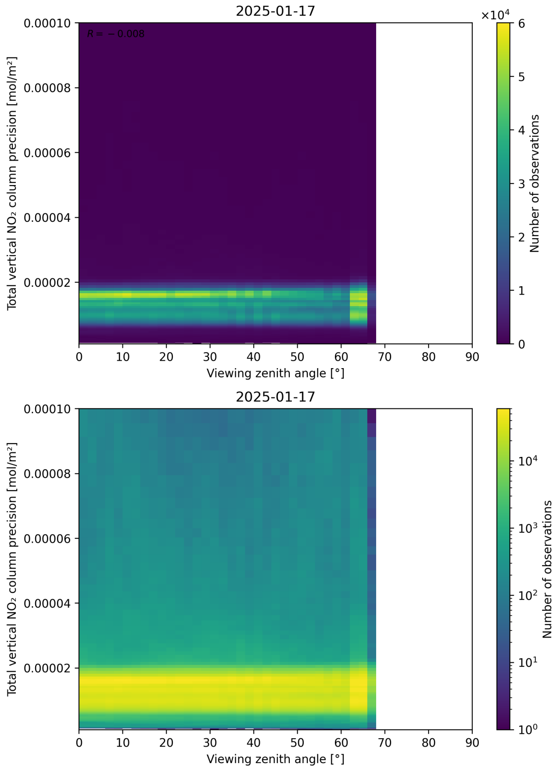
Figure 168: Scatter density plot of “Viewing zenith angle” against “Total vertical NO 2 column precision” for 2025-01-17 to 2025-01-18.
