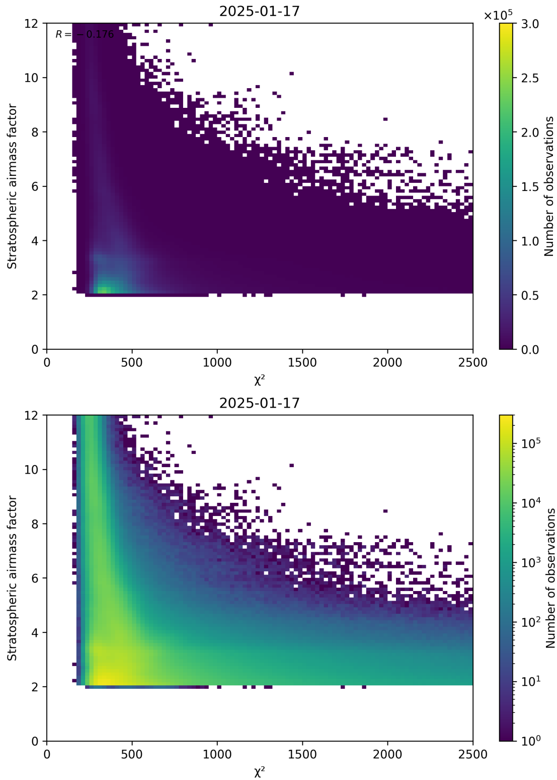
Figure 81: Scatter density plot of “ \chi^2 ” against “Stratospheric airmass factor” for 2025-01-17 to 2025-01-18.
