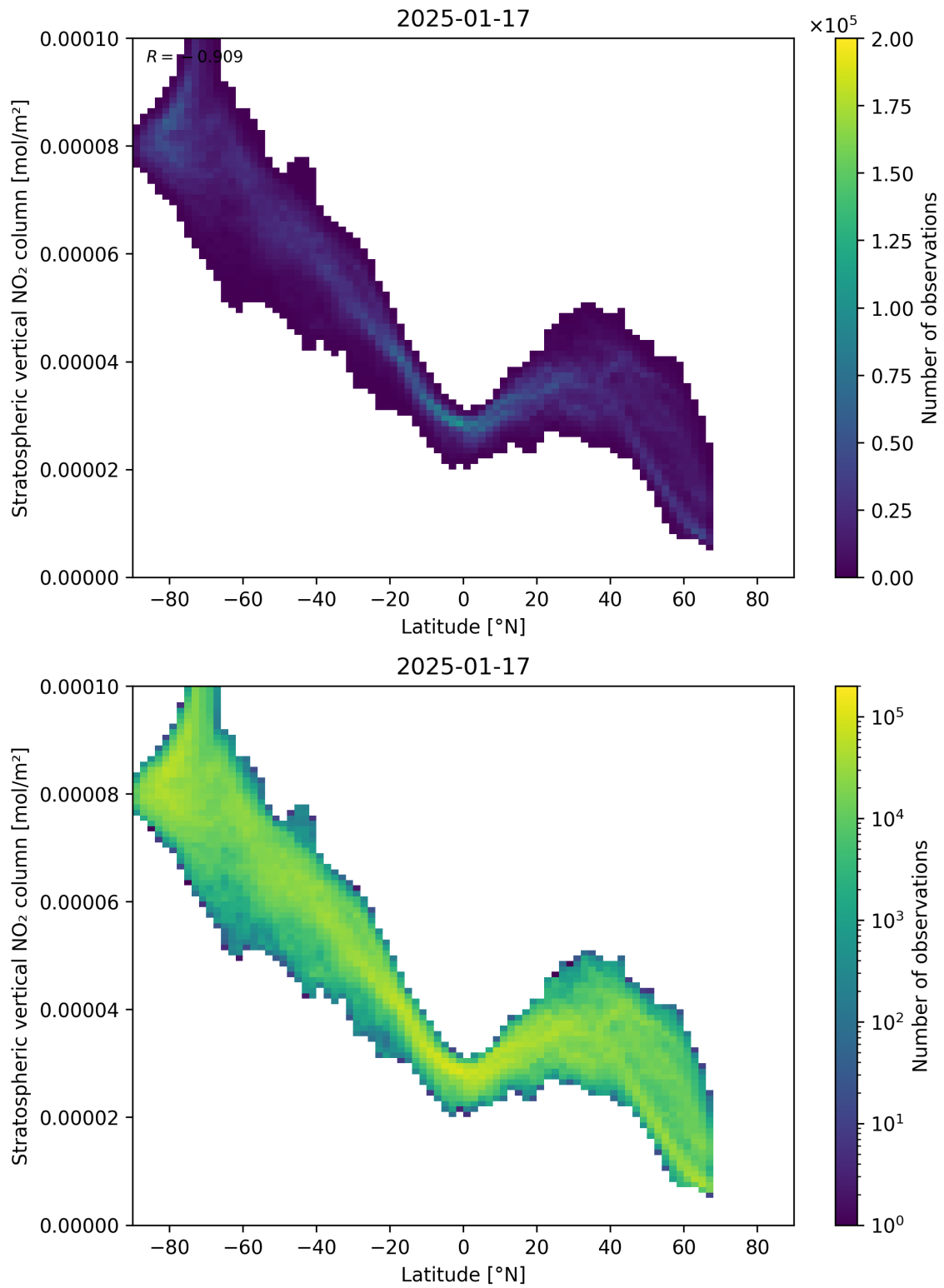
Figure 87: Scatter density plot of “Latitude” against “Stratospheric vertical NO 2 column” for 2025-01-17 to 2025-01-18.
