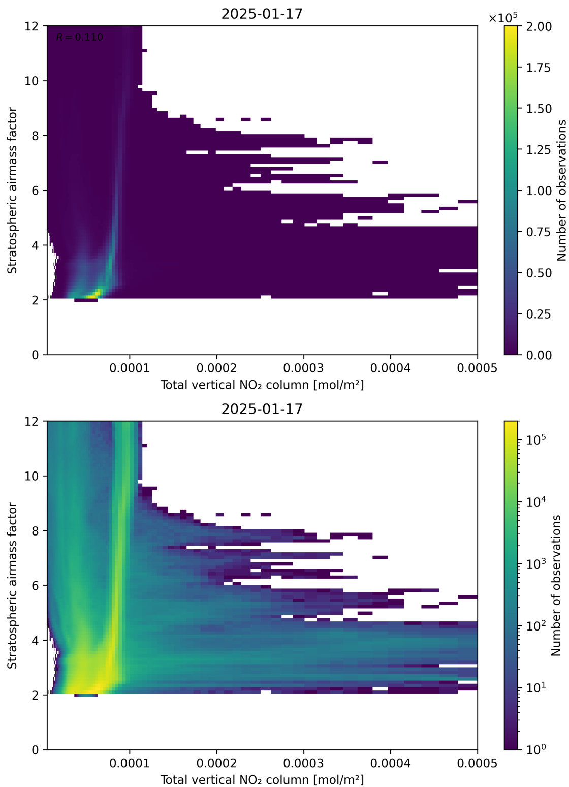
Figure 110: Scatter density plot of “Total vertical NO 2 column” against “Stratospheric airmass factor” for 2025-01-17 to 2025-01-18.
