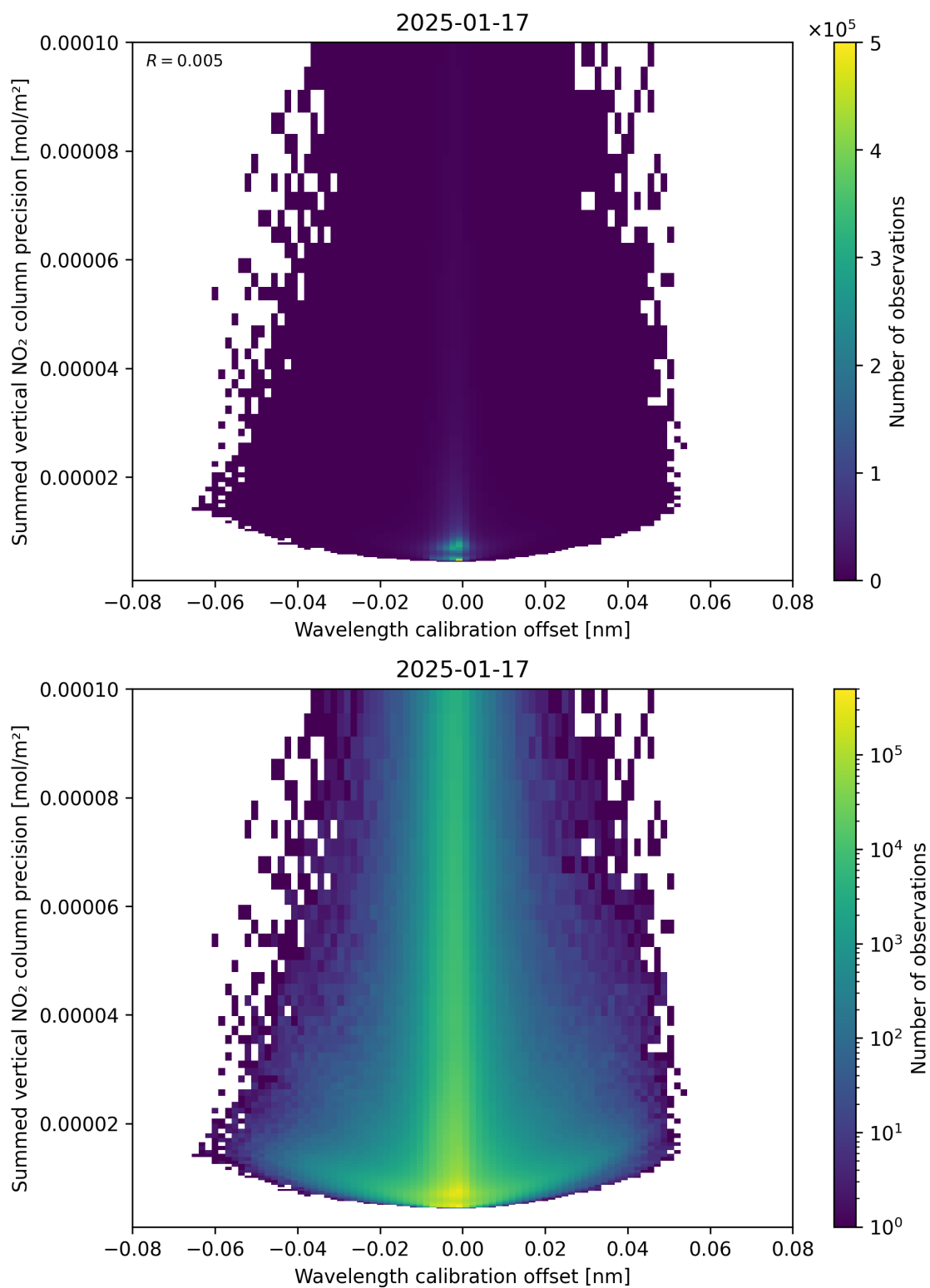
Figure 178: Scatter density plot of “Wavelength calibration offset” against “Summed vertical NO 2 column precision” for 2025-01-17 to 2025-01-18.
