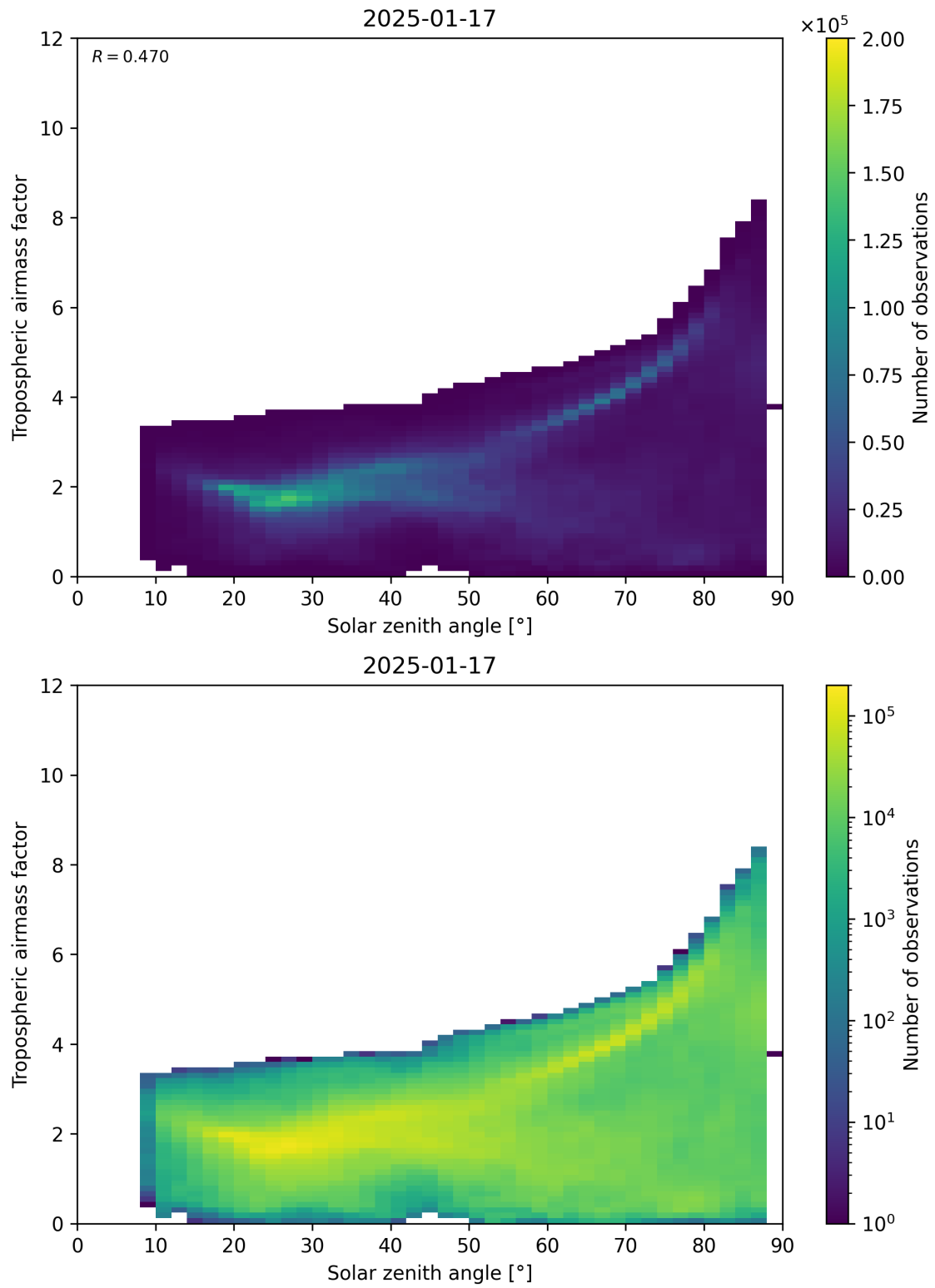
Figure 147: Scatter density plot of “Solar zenith angle” against “Tropospheric airmass factor” for 2025-01-17 to 2025-01-18.
