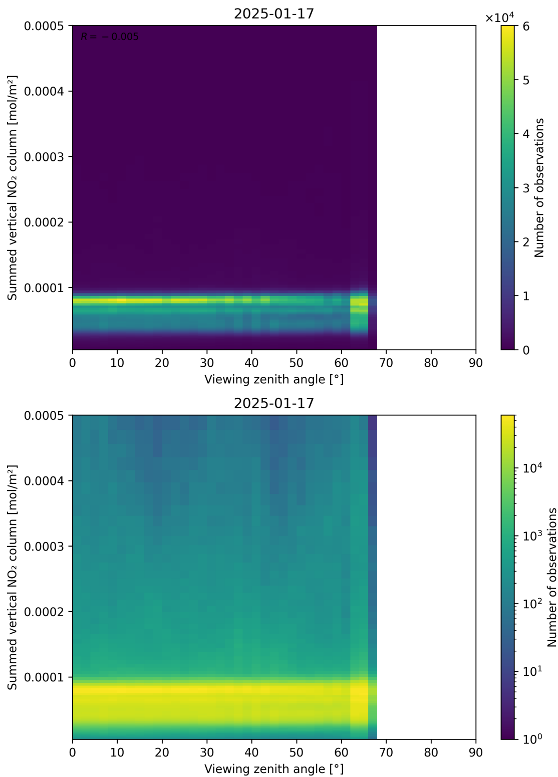
Figure 165: Scatter density plot of “Viewing zenith angle” against “Summed vertical NO 2 column” for 2025-01-17 to 2025-01-18.
