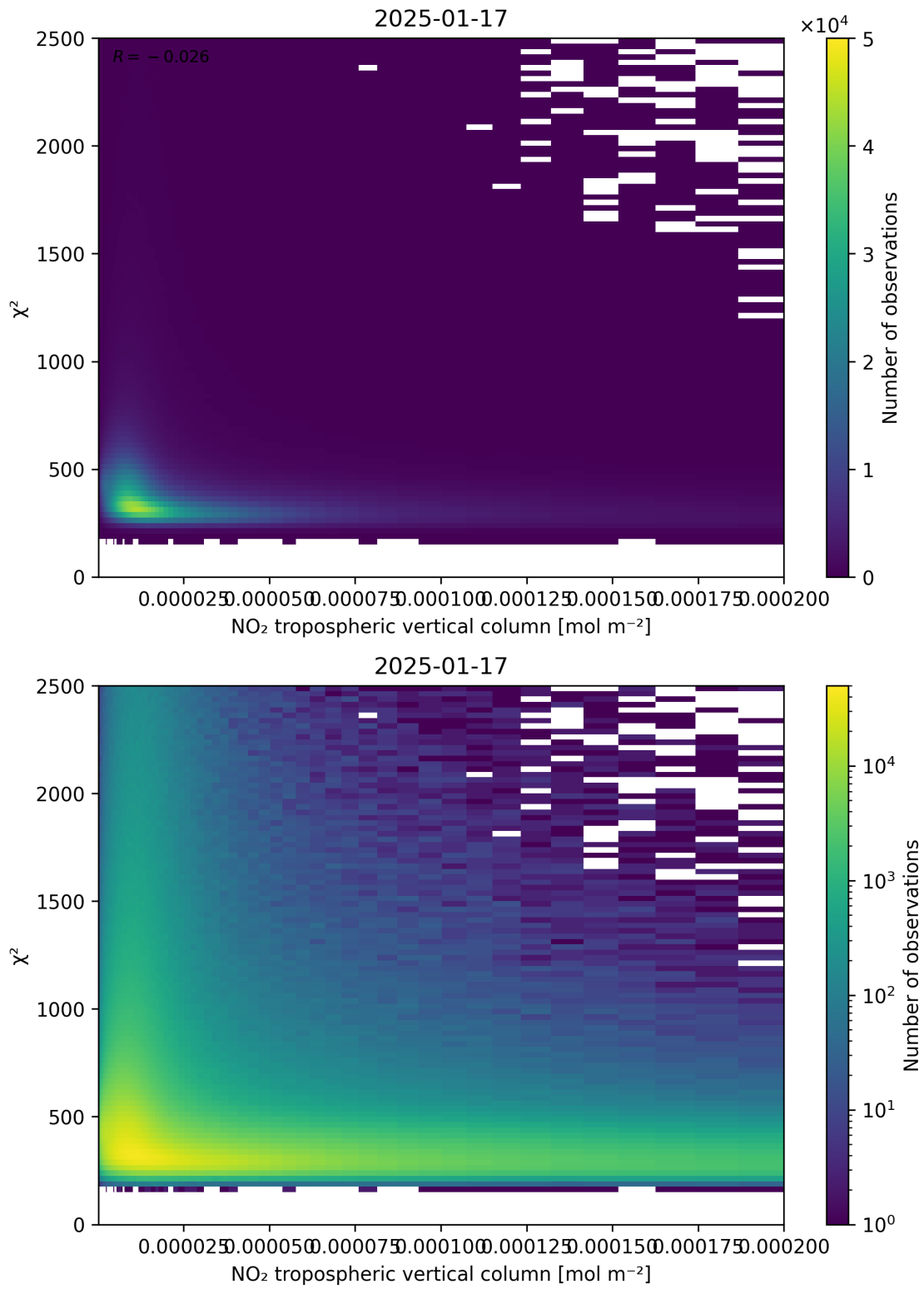
Figure 124: Scatter density plot of “NO 2 tropospheric vertical column” against “ \chi^2 ” for 2025-01-17 to 2025-01-18.
