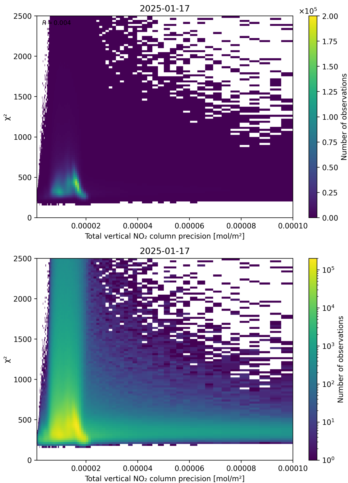
Figure 116: Scatter density plot of “Total vertical NO 2 column precision” against “ \chi^2 ” for 2025-01-17 to 2025-01-18.
