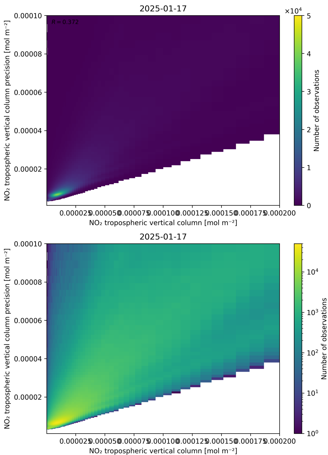
Figure 130: Scatter density plot of “NO 2 tropospheric vertical column” against “NO 2 tropospheric vertical column precision” for 2025-01-17 to 2025-01-18.
