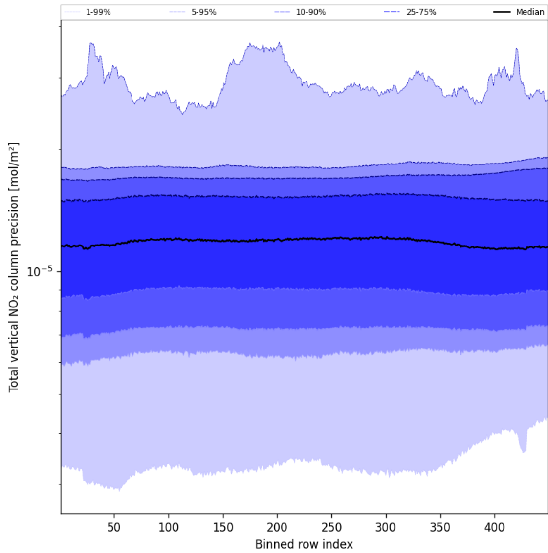
Figure 56: Along track statistics of “Total vertical NO 2 column precision” for 2025-01-17 to 2025-01-18
