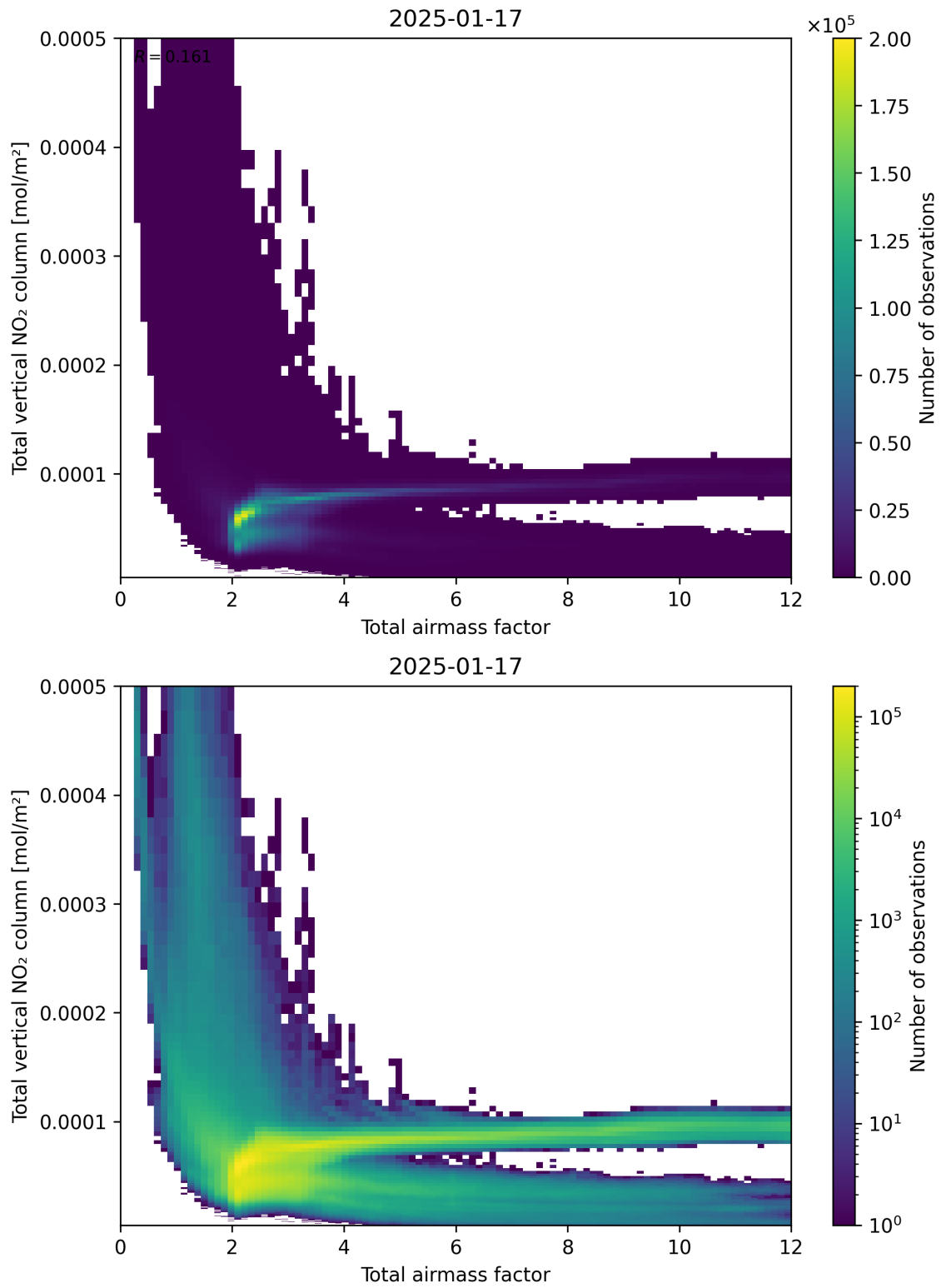
Figure 67: Scatter density plot of “Total airmass factor” against “Total vertical NO 2 column” for 2025-01-17 to 2025-01-18.
