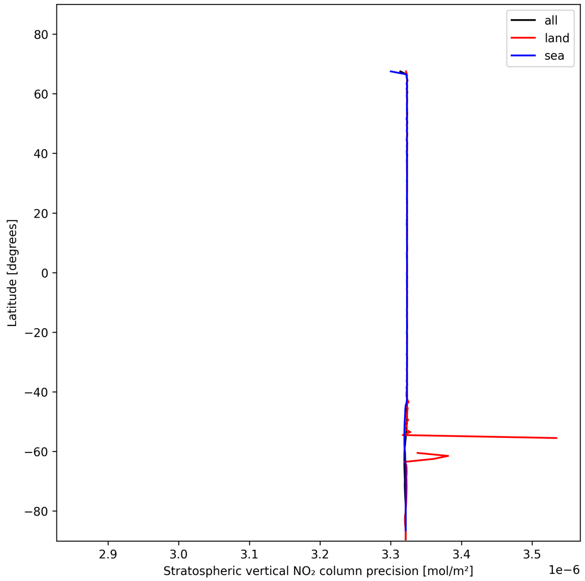
Figure 20: Zonal average of “Stratospheric vertical NO 2 column precision” for 2025-01-17 to 2025-01-18.
