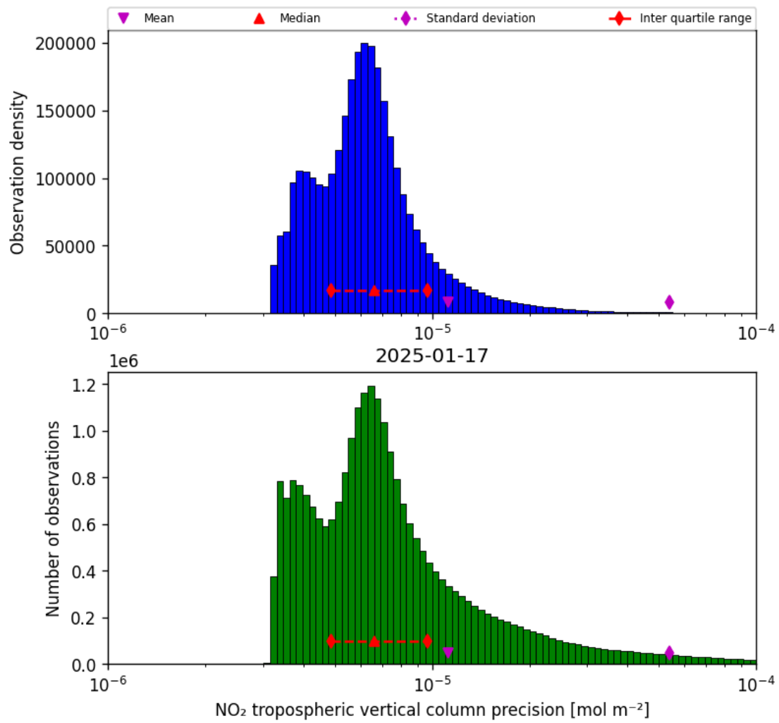
Figure 30: Histogram of “NO 2 tropospheric vertical column precision” for 2025-01-17 to 2025-01-18
