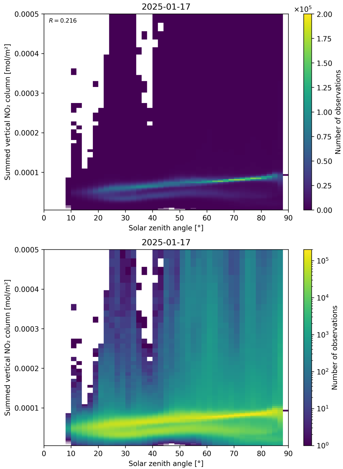
Figure 151: Scatter density plot of “Solar zenith angle” against “Summed vertical NO 2 column” for 2025-01-17 to 2025-01-18.
