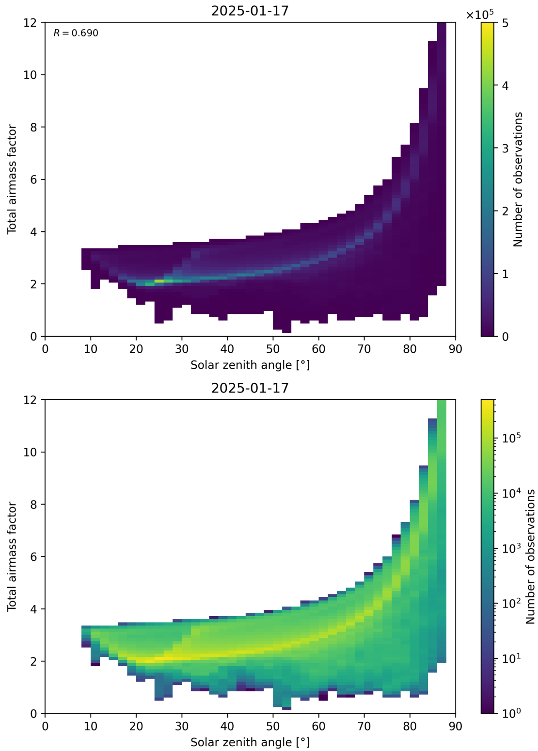
Figure 146: Scatter density plot of “Solar zenith angle” against “Total air mass factor” for 2025-01-17 to 2025-01-18.
