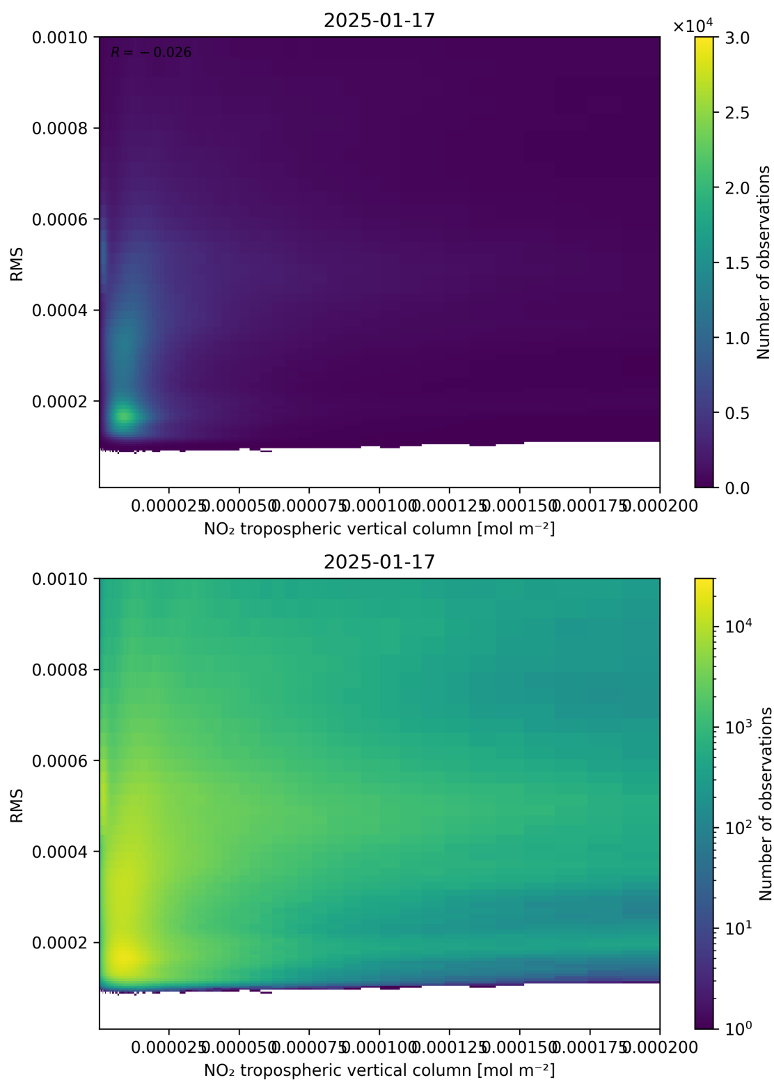
Figure 142: Scatter density plot of “NO 2 tropospheric vertical column” against “RMS” for 2025-01-17 to 2025-01-18.
