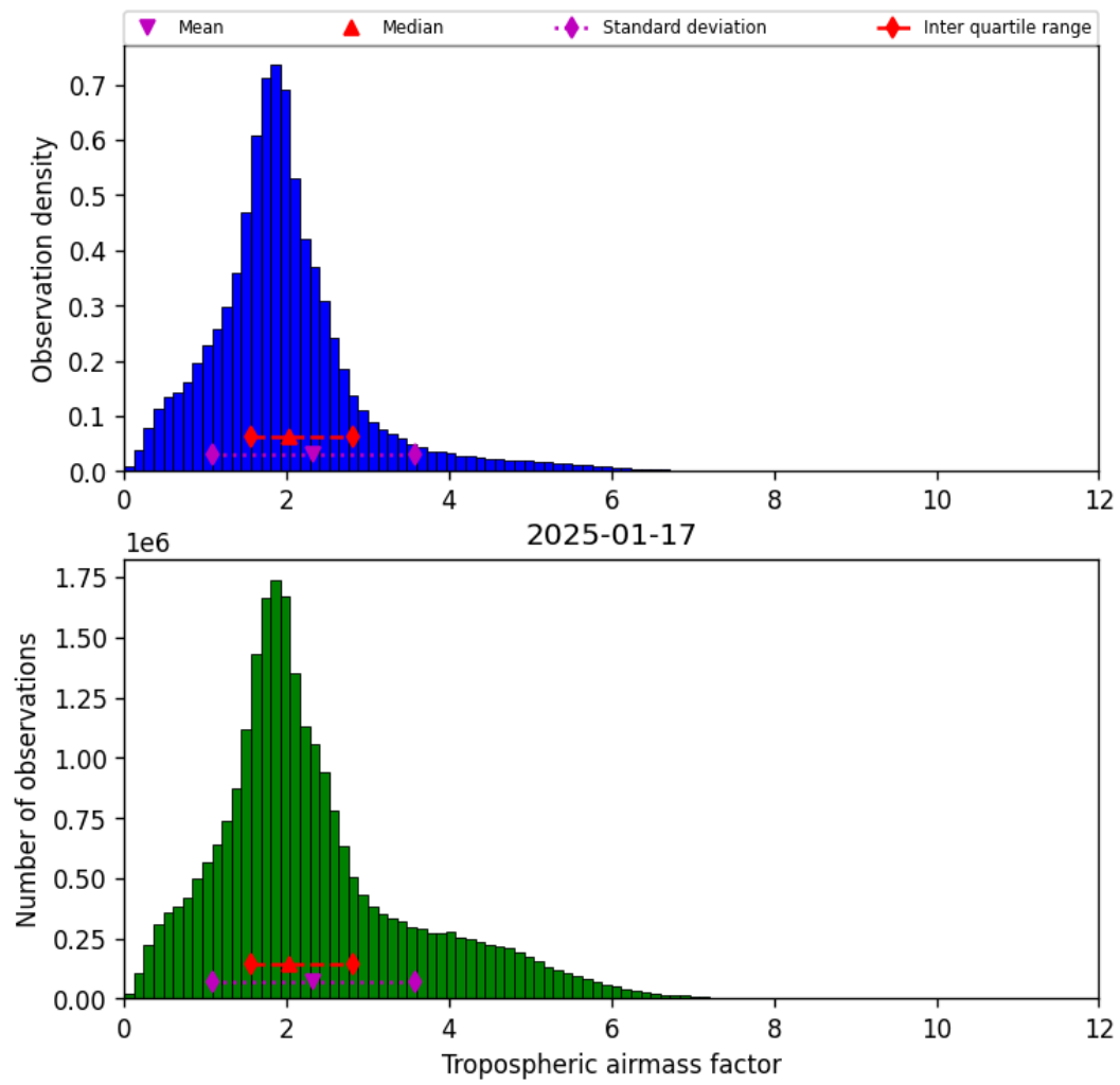
Figure 31: Histogram of “Tropospheric airmass factor” for 2025-01-17 to 2025-01-18
