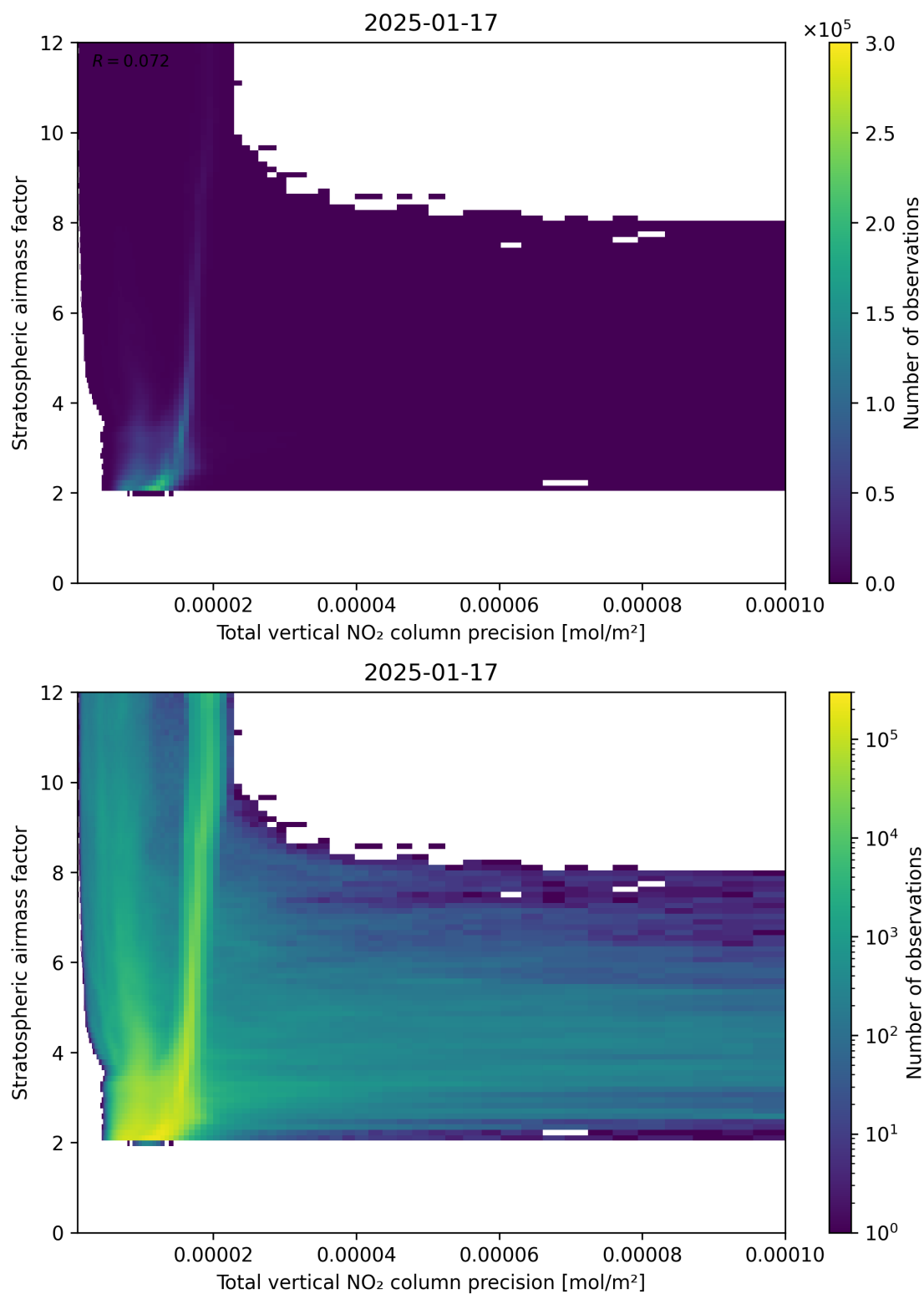
Figure 115: Scatter density plot of “Total vertical NO 2 column precision” against “Stratospheric air mass factor” for 2025-01-17 to 2025-01-18.
