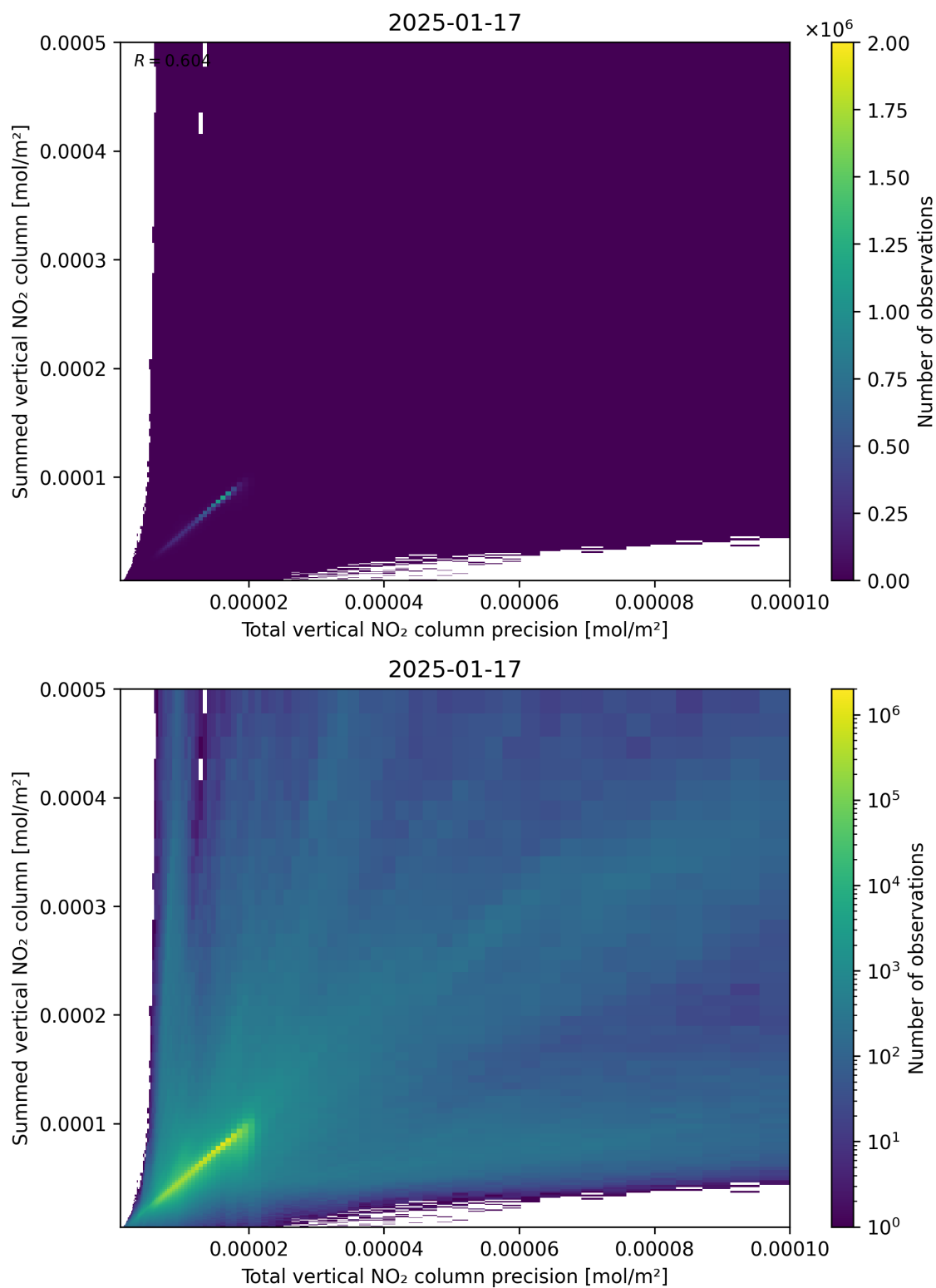
Figure 117: Scatter density plot of “Total vertical NO 2 column precision” against “Summed vertical NO 2 column” for 2025-01-17 to 2025-01-18.
