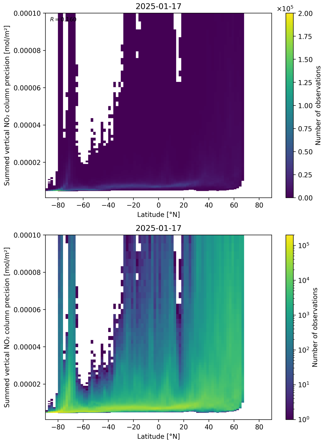
Figure 89: Scatter density plot of “Latitude” against “Summed vertical NO 2 column precision” for 2025-01-17 to 2025-01-18.
