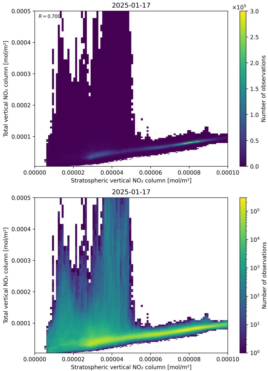
Figure 100: Scatter density plot of “Stratospheric vertical NO 2 column” against “Total vertical NO 2 column” for 2025-01-17 to 2025-01-18.
