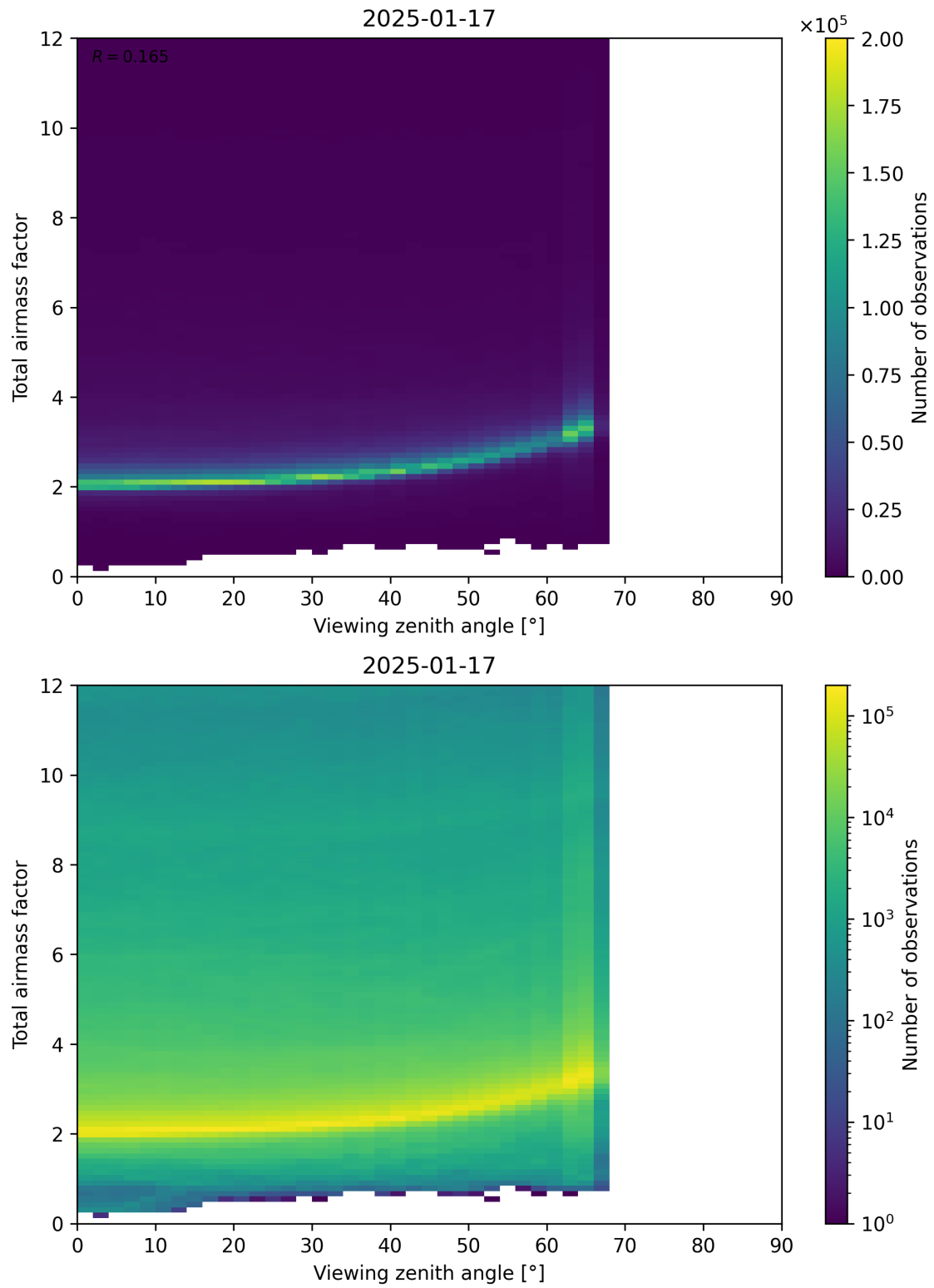
Figure 160: Scatter density plot of “Viewing zenith angle” against “Total airmass factor” for 2025-01-17 to 2025-01-18.
