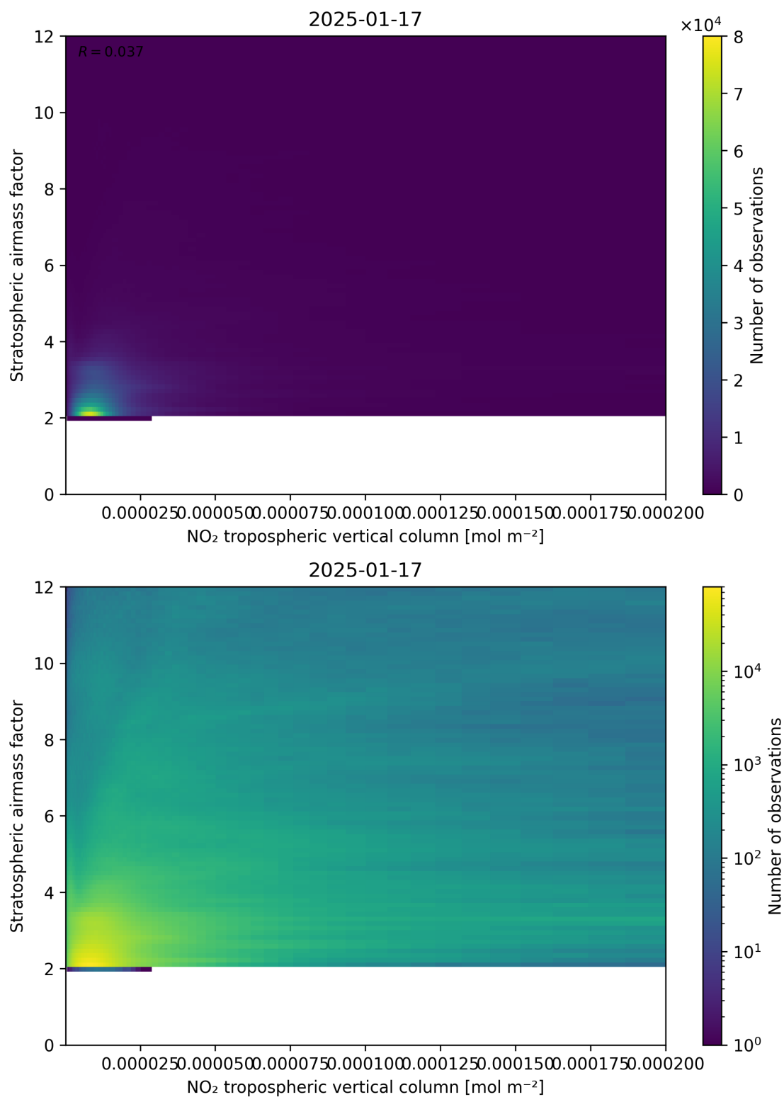
Figure 121: Scatter density plot of “NO 2 tropospheric vertical column” against “Stratospheric airmass factor” for 2025-01-17 to 2025-01-18.
