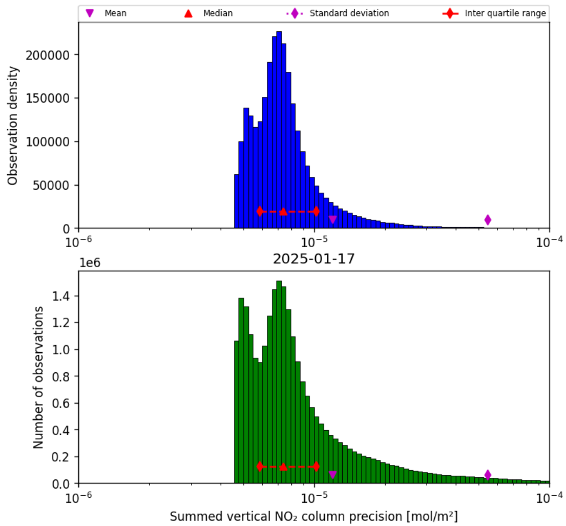
Figure 41: Histogram of “Summed vertical NO 2 column precision” for 2025-01-17 to 2025-01-18
