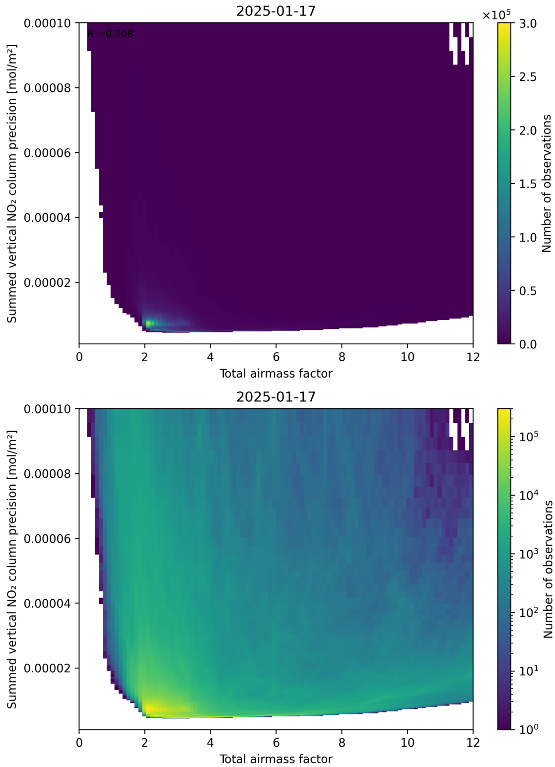
Figure 66: Scatter density plot of “Total airmass factor” against “Summed vertical NO 2 column precision” for 2025-01-17 to 2025-01-18.
