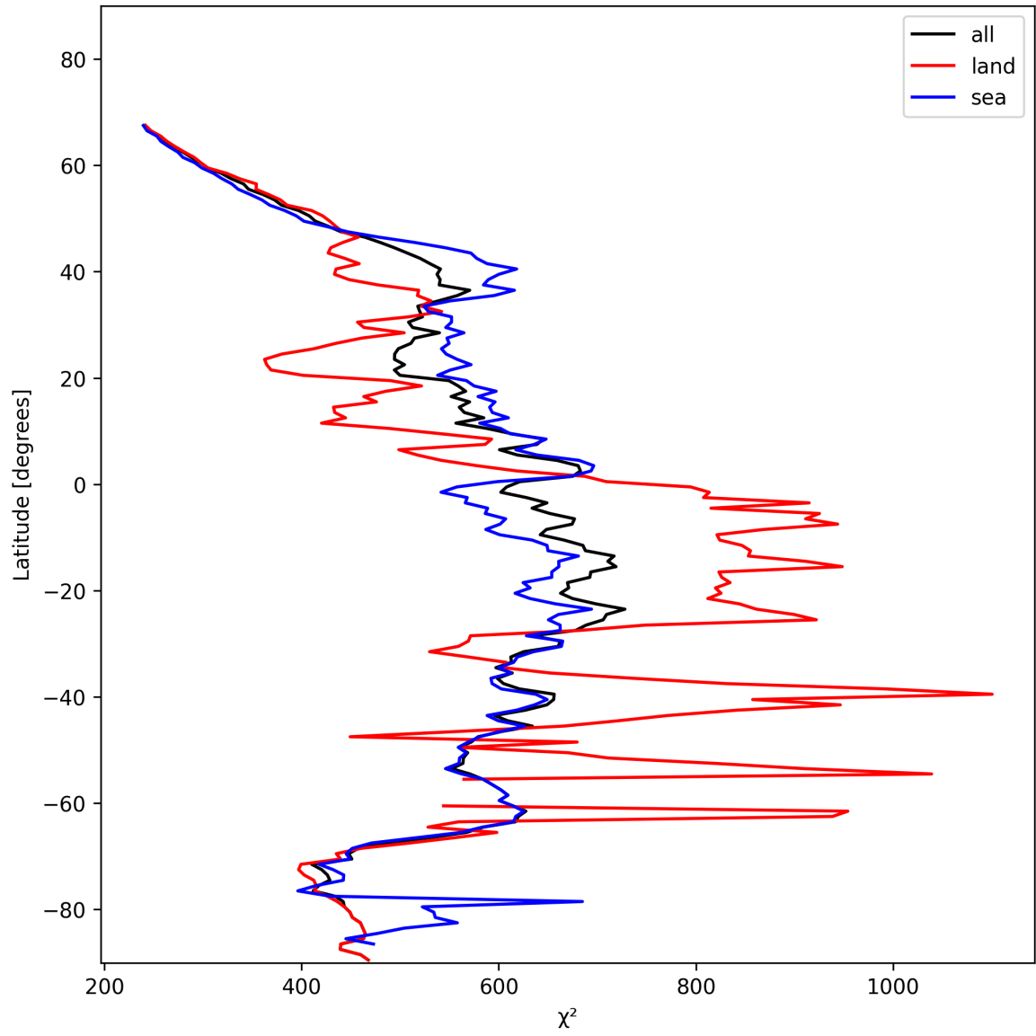
Figure 25: Zonal average of “ \chi^2 ” for 2025-01-17 to 2025-01-18.
