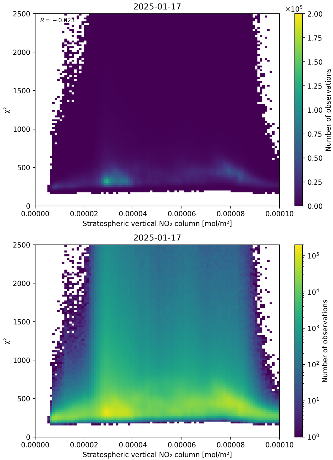
Figure 97: Scatter density plot of “Stratospheric vertical NO 2 column” against “ \chi^2 ” for 2025-01-17 to 2025-01-18.
