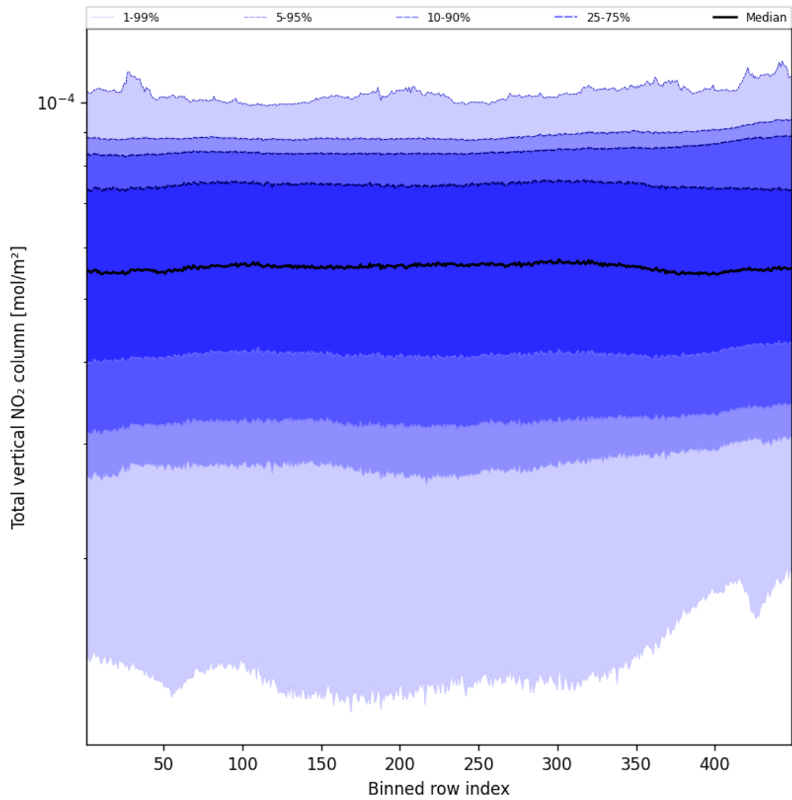
Figure 55: Along track statistics of “Total vertical NO 2 column” for 2025-01-17 to 2025-01-18
