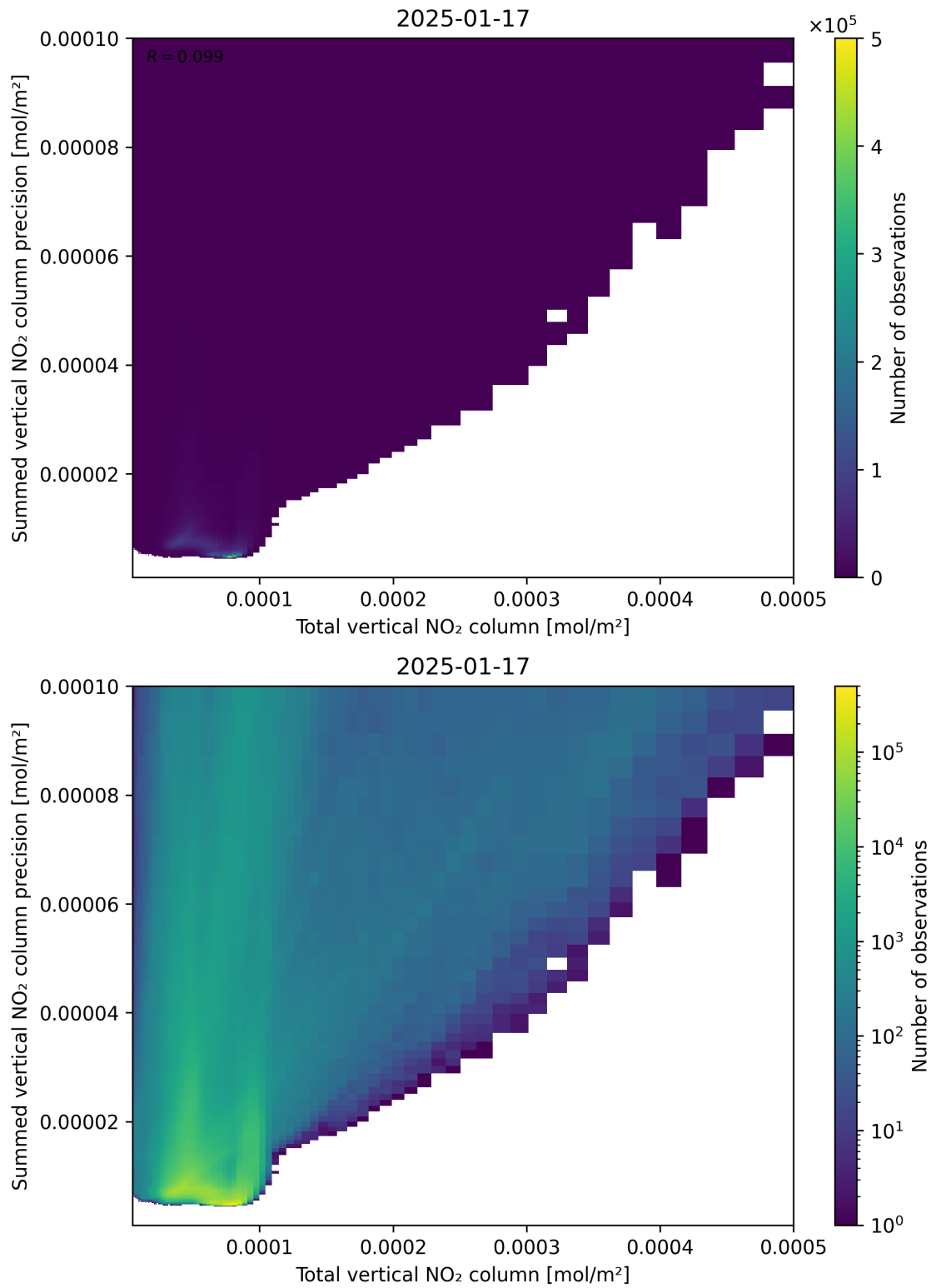
Figure 113: Scatter density plot of “Total vertical NO 2 column” against “Summed vertical NO 2 column precision” for 2025-01-17 to 2025-01-18.
