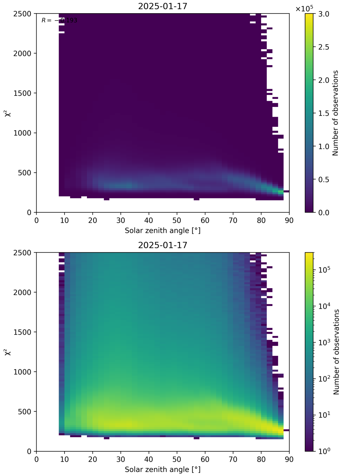
Figure 148: Scatter density plot of “Solar zenith angle” against “ \chi^2 ” for 2025-01-17 to 2025-01-18.
