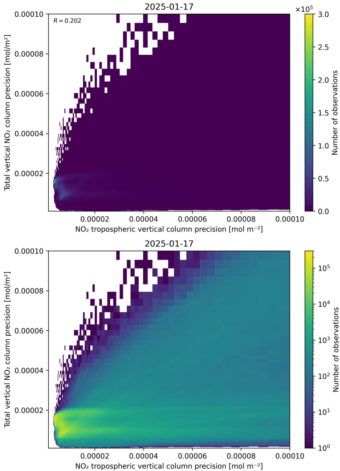
Figure 139: Scatter density plot of “NO 2 tropospheric vertical column precision” against “Total vertical NO 2 column precision” for 2025-01-17 to 2025-01-18.
