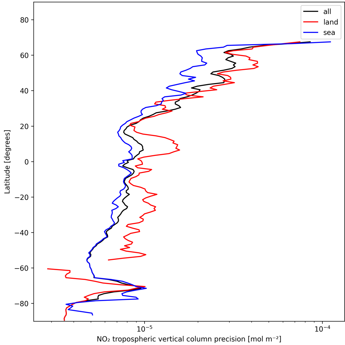
Figure 13: Zonal average of “NO 2 tropospheric vertical column precision” for 2025-01-17 to 2025-01-18.
