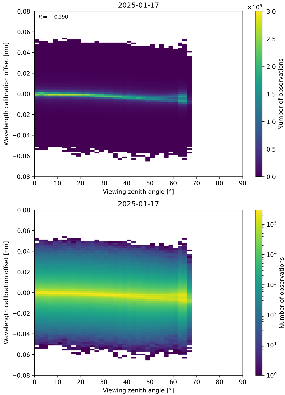
Figure 173: Scatter density plot of “Viewing zenith angle” against “Wavelength calibration offset” for 2025-01-17 to 2025-01-18.
