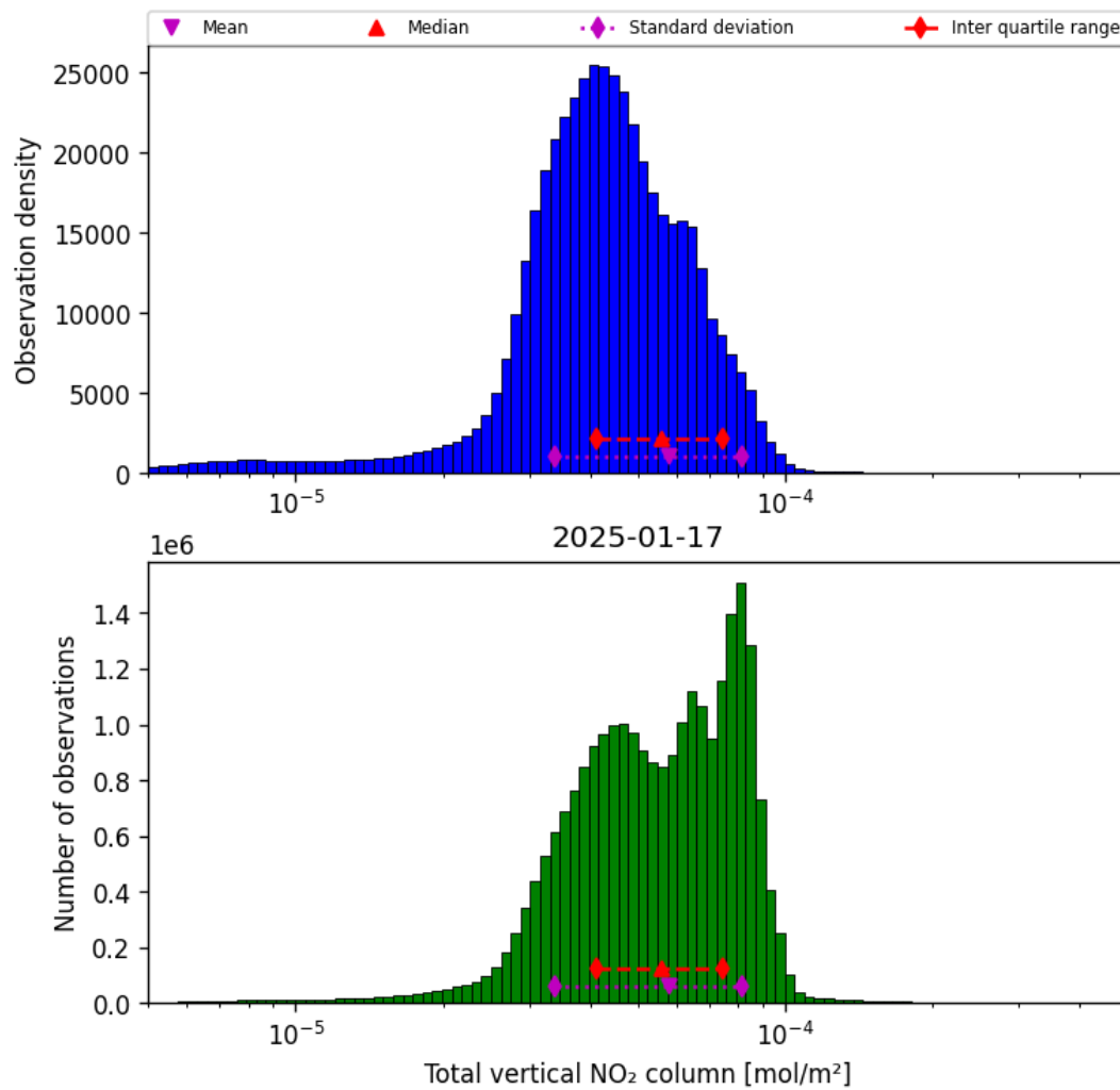
Figure 38: Histogram of "Total vertical NO 2 column" for 2025-01-17 to 2025-01-18
