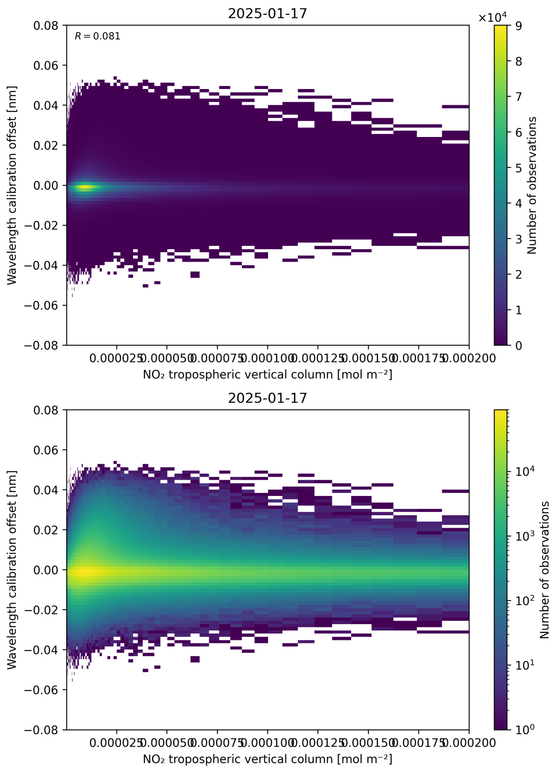
Figure 143: Scatter density plot of “NO 2 tropospheric vertical column” against “Wavelength calibration offset” for 2025-01-17 to 2025-01-18.
