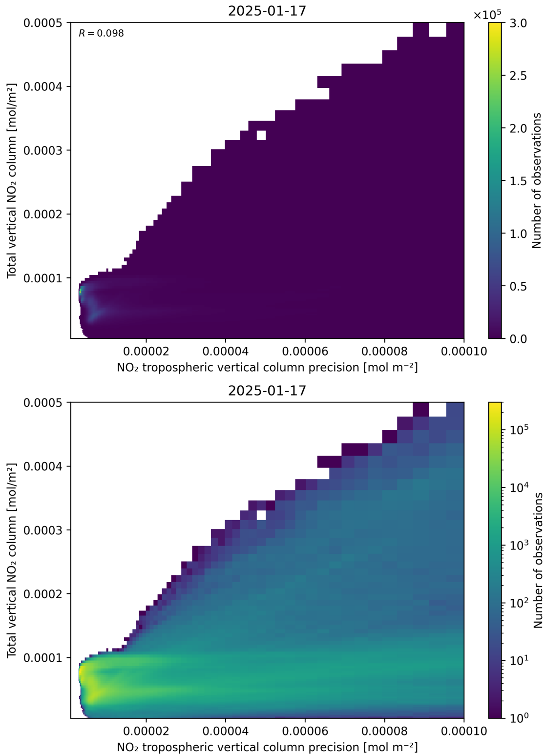
Figure 138: Scatter density plot of “NO 2 tropospheric vertical column precision” against “Total vertical NO 2 column” for 2025-01-17 to 2025-01-18.
