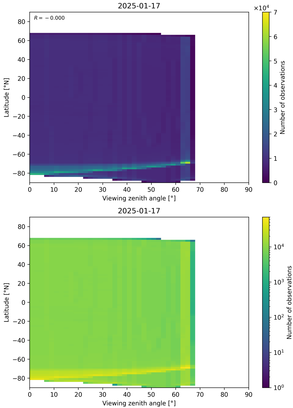
Figure 163: Scatter density plot of “Viewing zenith angle” against “Latitude” for 2025-01-17 to 2025-01-18.
