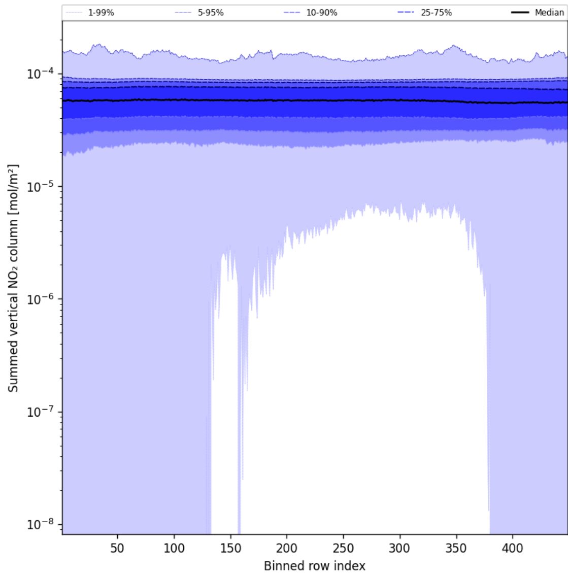
Figure 57: Along track statistics of "Summed vertical NO 2 column" for 2025-01-17 to 2025-01-18
