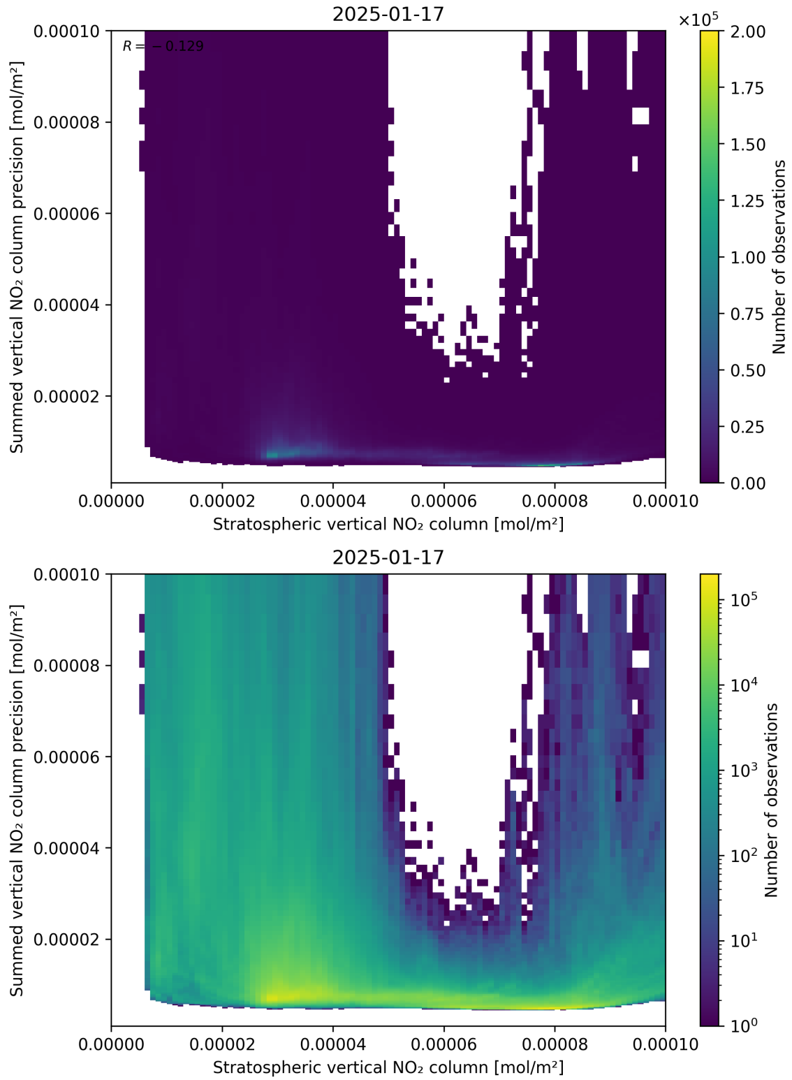
Figure 99: Scatter density plot of “Stratospheric vertical NO 2 column” against “Summed vertical NO 2 column precision” for 2025-01-17 to 2025-01-18.
