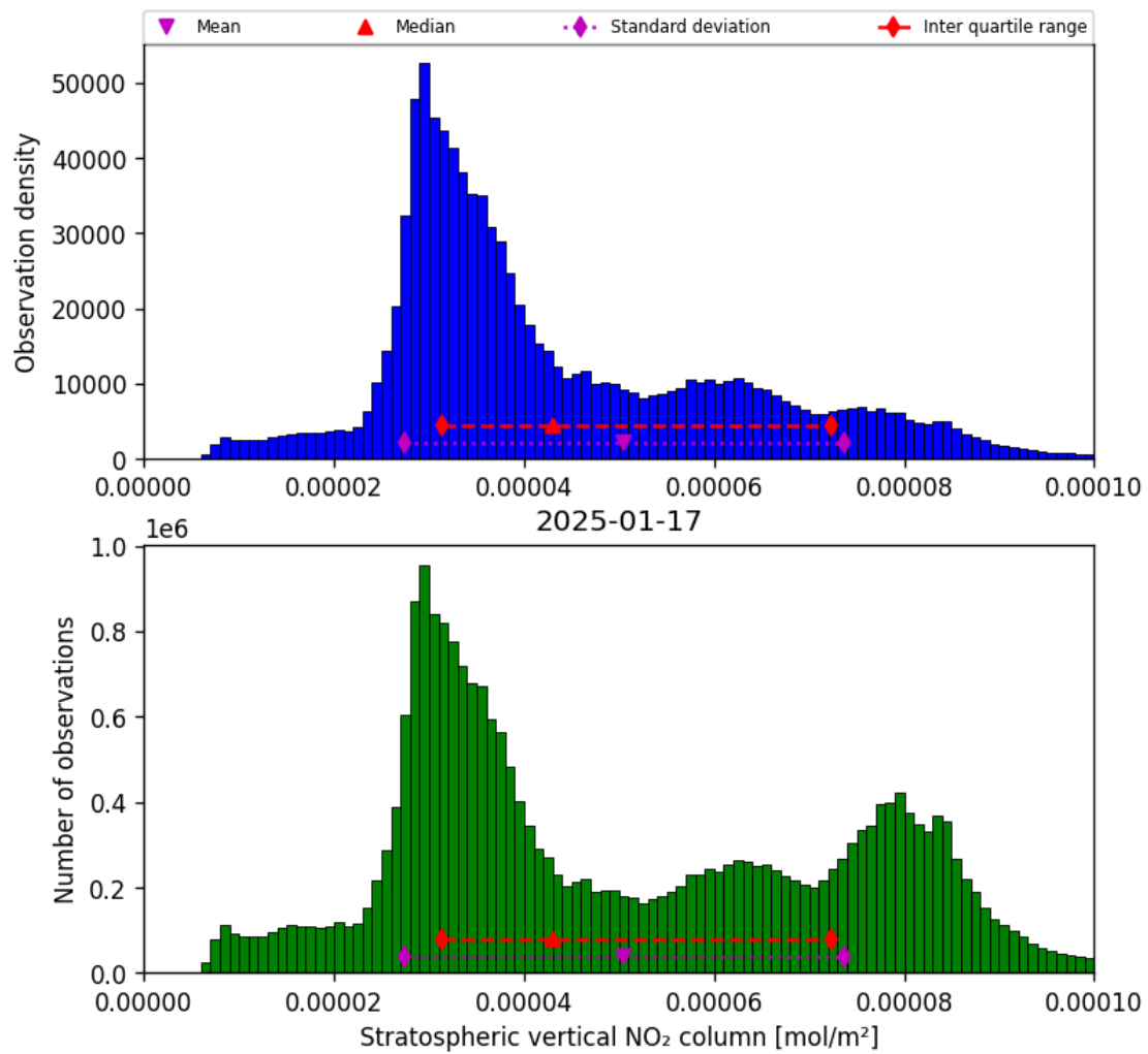
Figure 36: Histogram of “Stratospheric vertical NO 2 column” for 2025-01-17 to 2025-01-18
