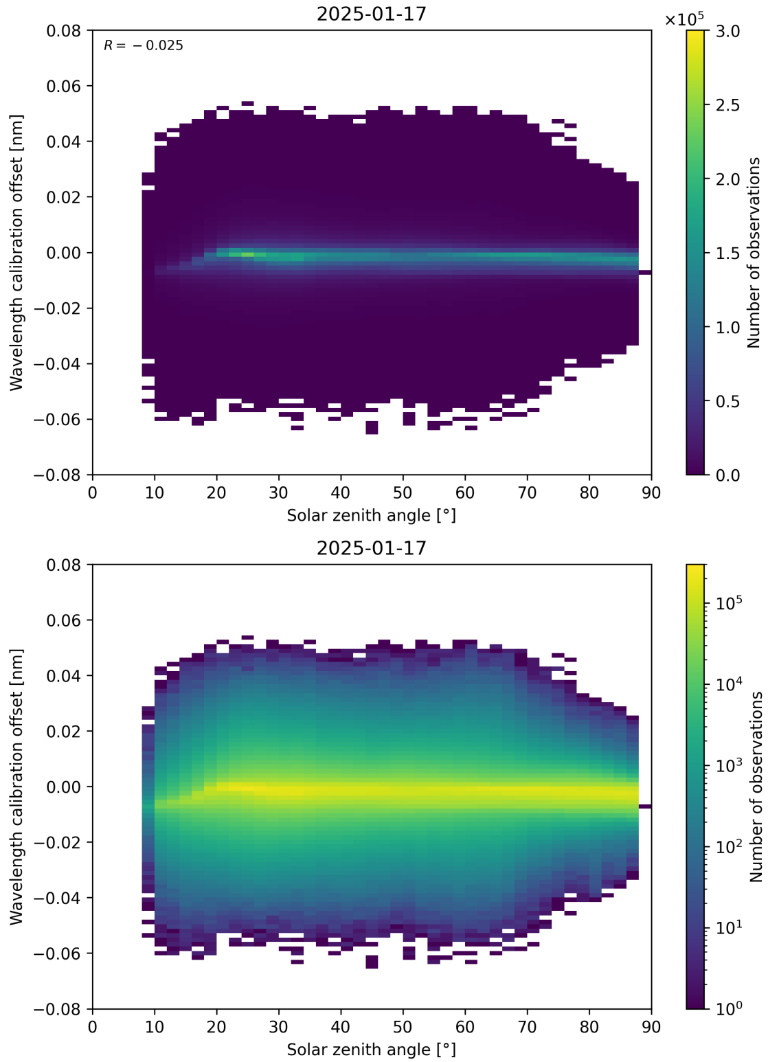
Figure 158: Scatter density plot of “Solar zenith angle” against “Wavelength calibration offset” for 2025-01-17 to 2025-01-18.
