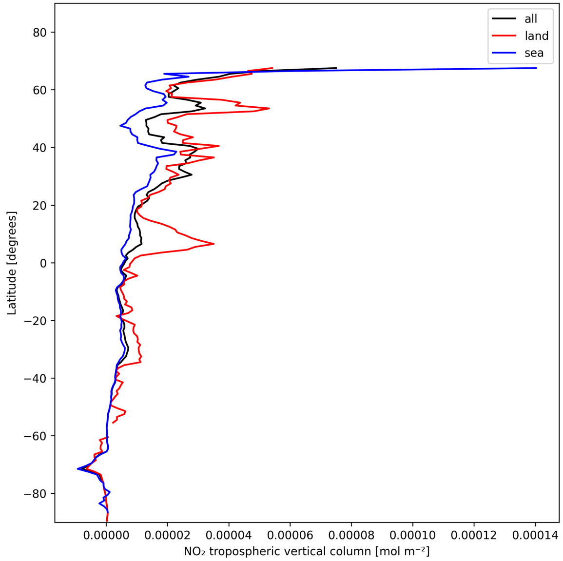
Figure 12: Zonal average of “NO 2 tropospheric vertical column” for 2025-01-17 to 2025-01-18.
