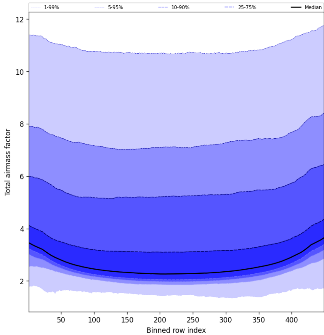
Figure 49: Along track statistics of “Total airmass factor” for 2025-01-17 to 2025-01-18
