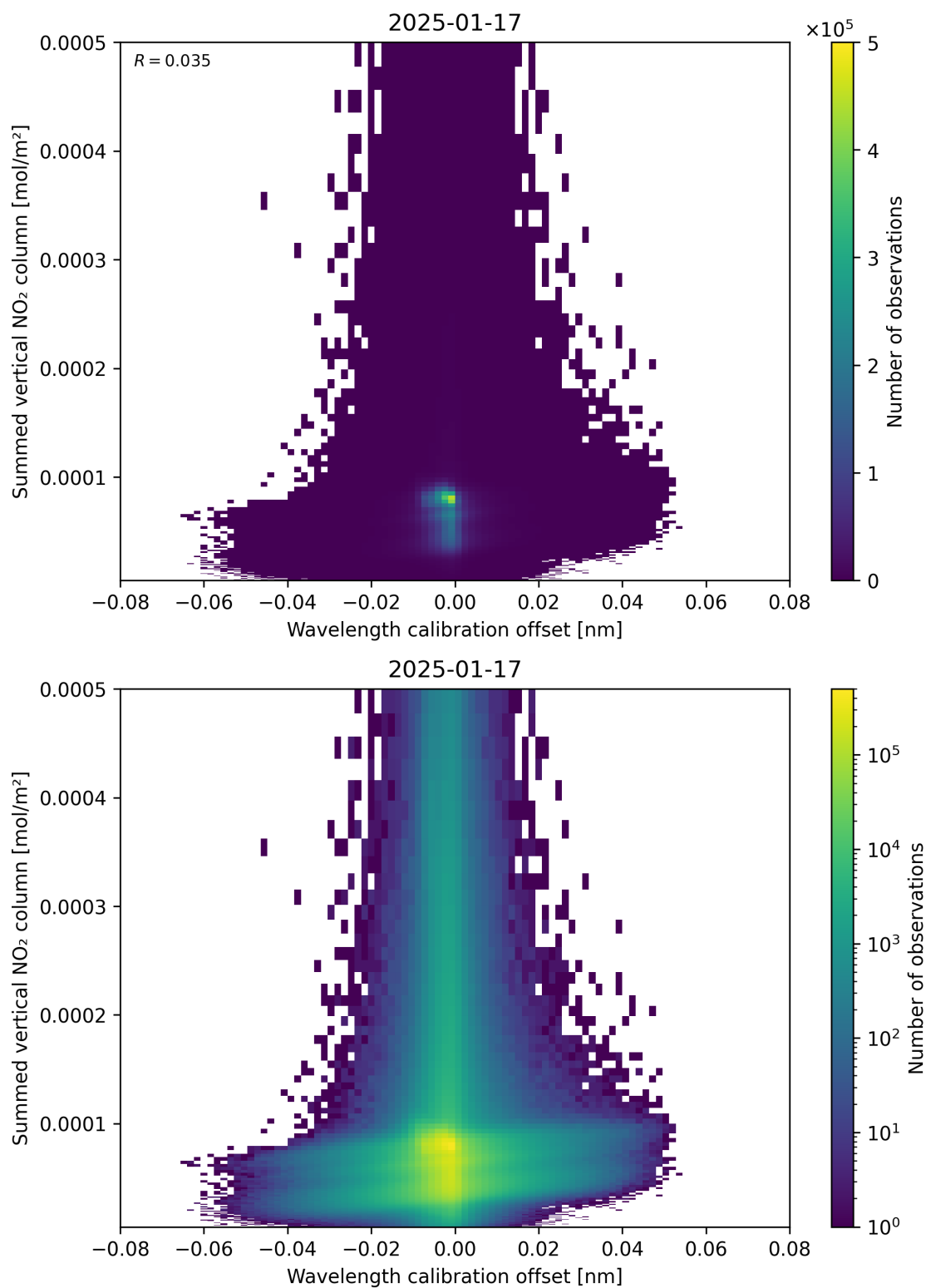
Figure 177: Scatter density plot of “Wavelength calibration offset” against “Summed vertical NO 2 column” for 2025-01-17 to 2025-01-18.
