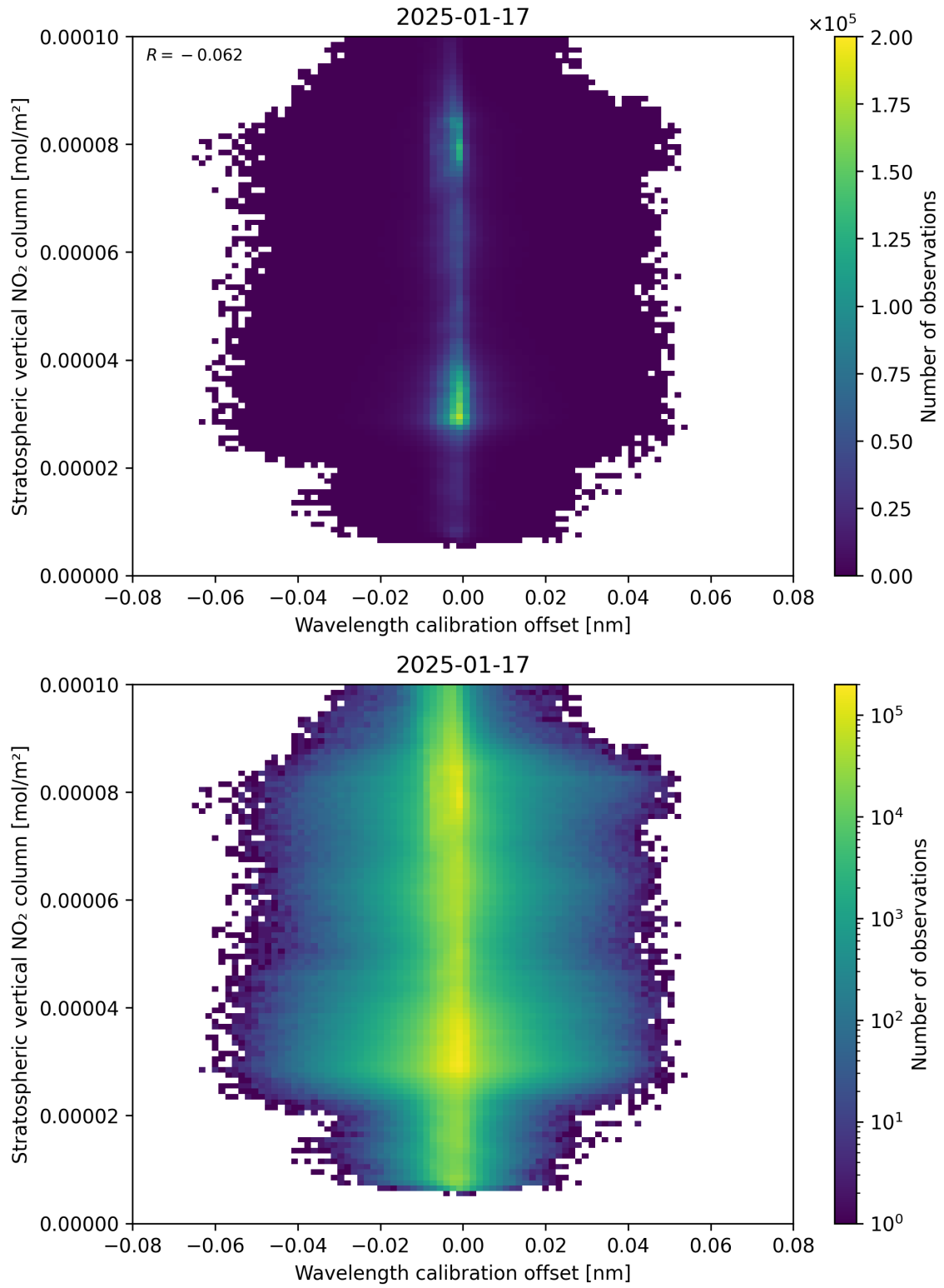
Figure 176: Scatter density plot of “Wavelength calibration offset” against “Stratospheric vertical NO 2 column” for 2025-01-17 to 2025-01-18.
