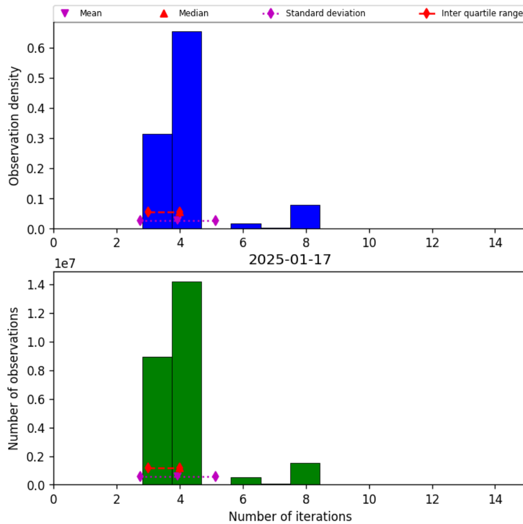
Figure 34: Histogram of “Number of iterations” for 2025-01-17 to 2025-01-18
