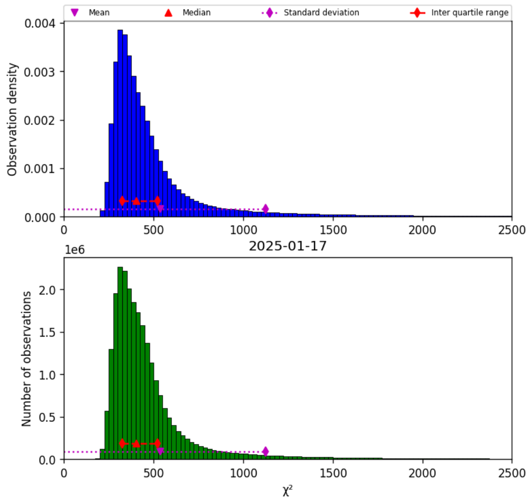
Figure 42: Histogram of “ \chi^2 ” for 2025-01-17 to 2025-01-18
