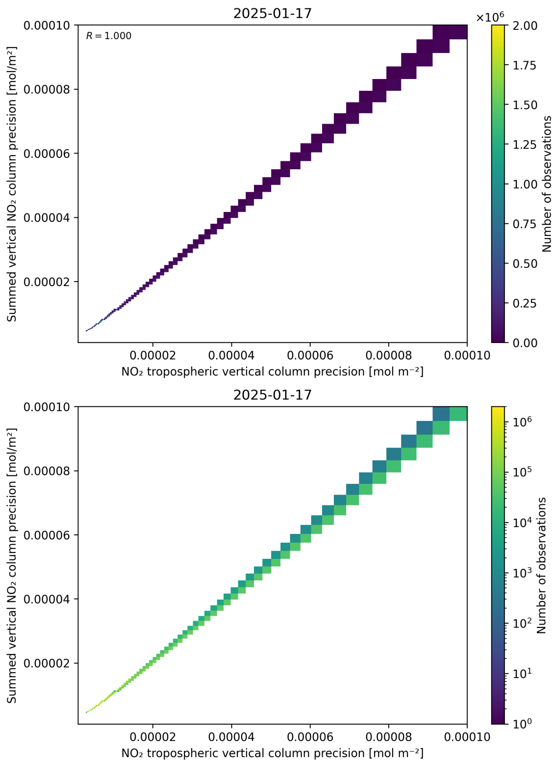
Figure 137: Scatter density plot of “NO 2 tropospheric vertical column precision” against “Summed vertical NO 2 column precision” for 2025-01-17 to 2025-01-18.
