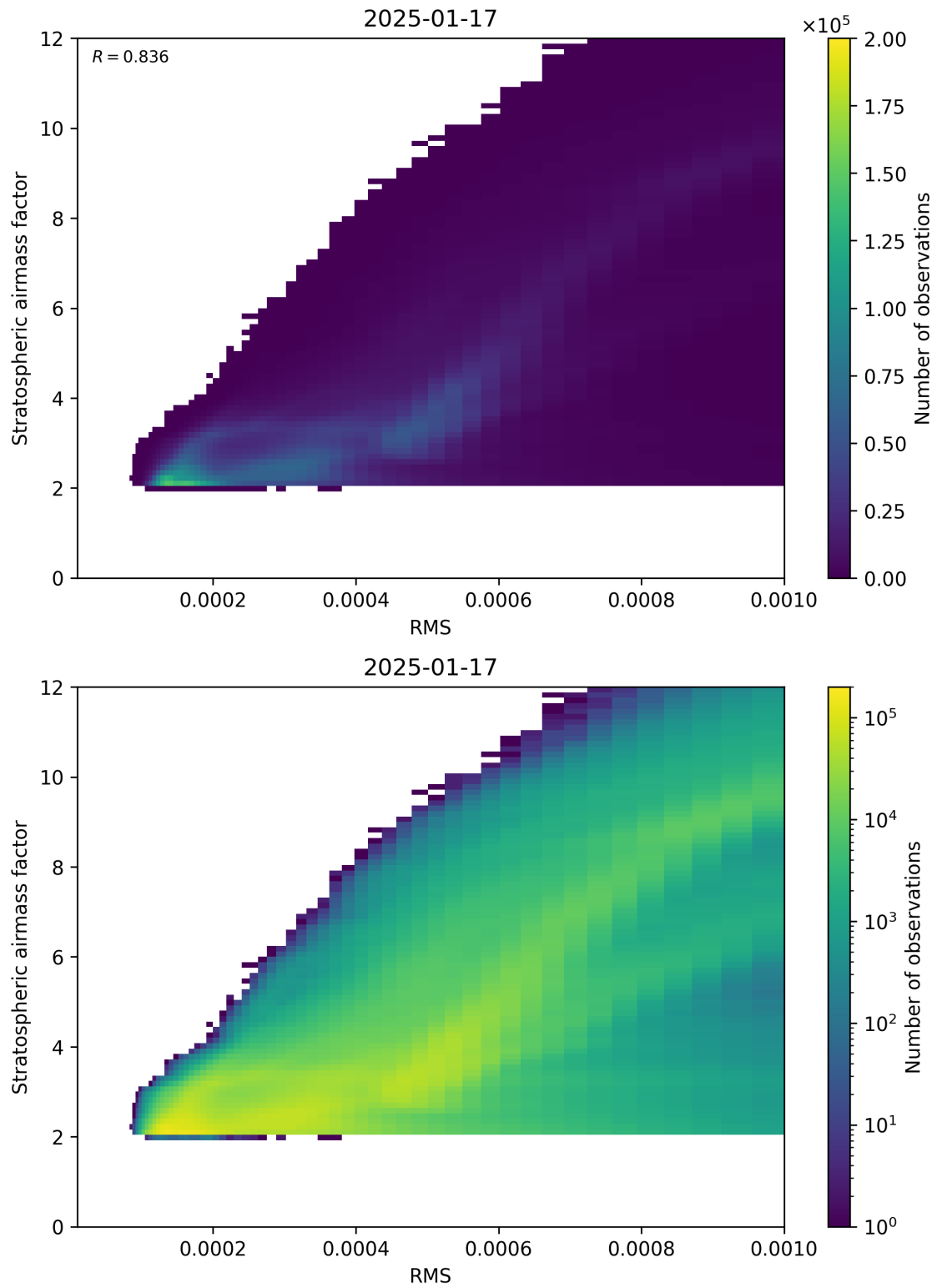
Figure 144: Scatter density plot of “RMS” against “Stratospheric airmass factor” for 2025-01-17 to 2025-01-18.
