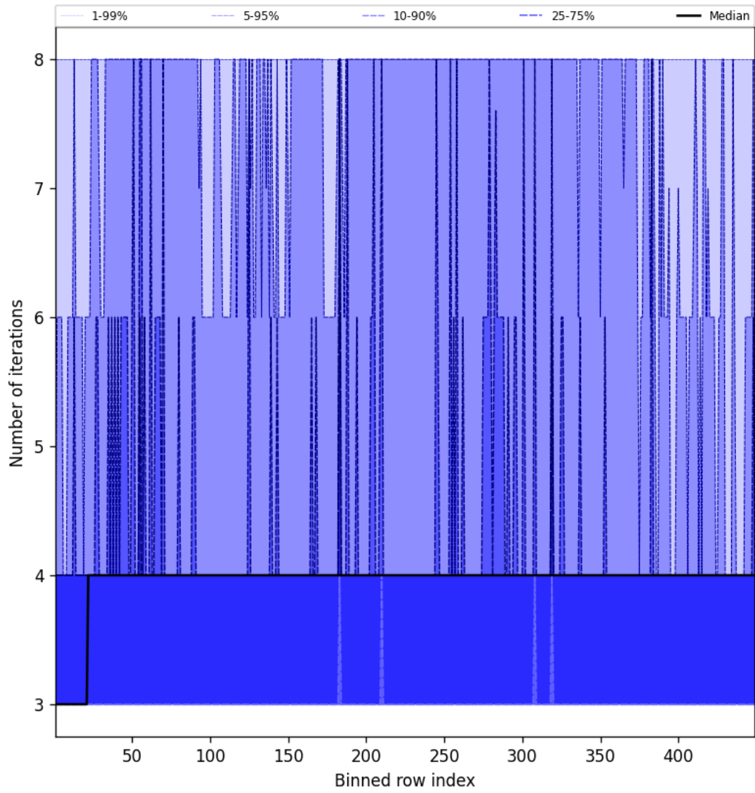
Figure 51: Along track statistics of “Number of iterations” for 2025-01-17 to 2025-01-18
