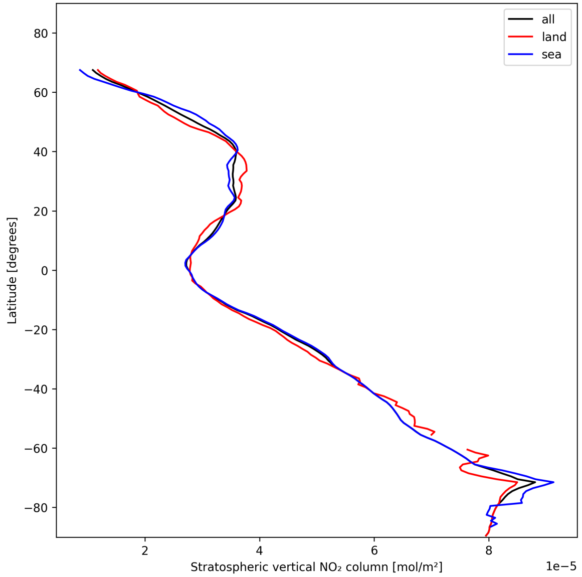
Figure 19: Zonal average of “Stratospheric vertical NO 2 column” for 2025-01-17 to 2025-01-18.
