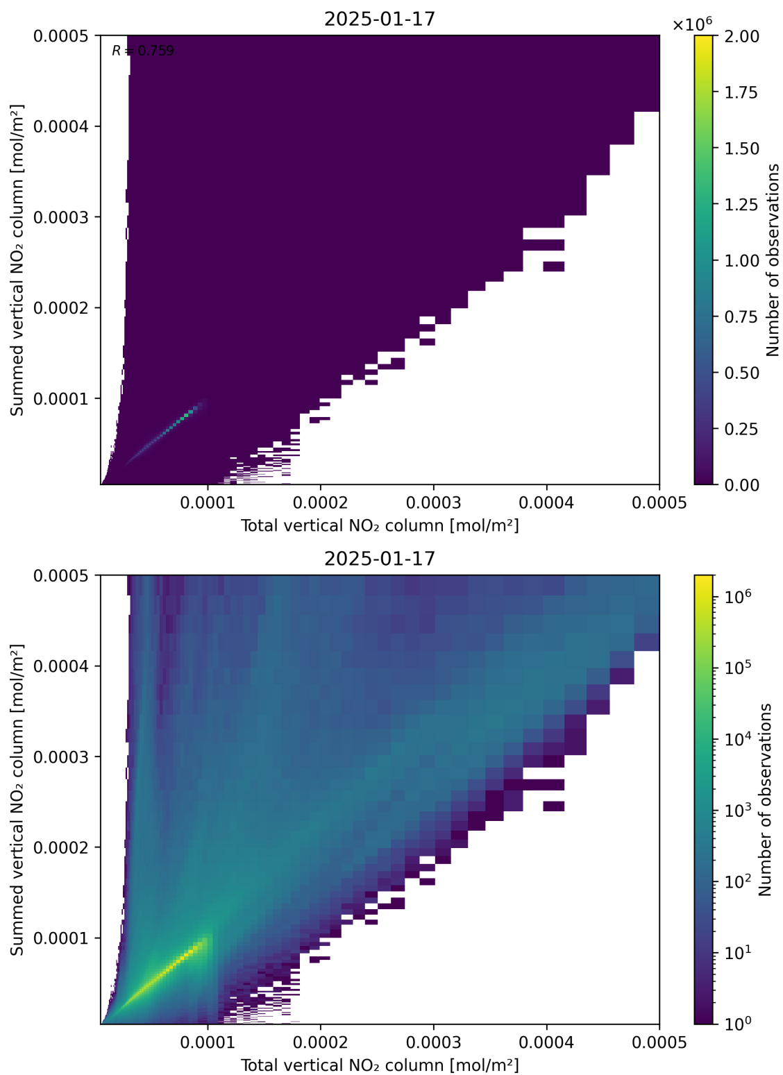
Figure 112: Scatter density plot of “Total vertical NO 2 column” against “Summed vertical NO 2 column” for 2025-01-17 to 2025-01-18.
