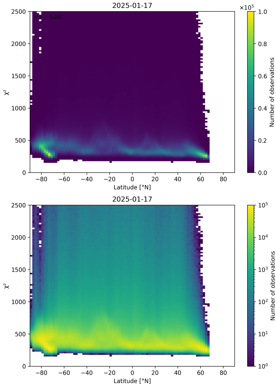
Figure 86: Scatter density plot of “Latitude” against “ \chi^2 ” for 2025-01-17 to 2025-01-18.
