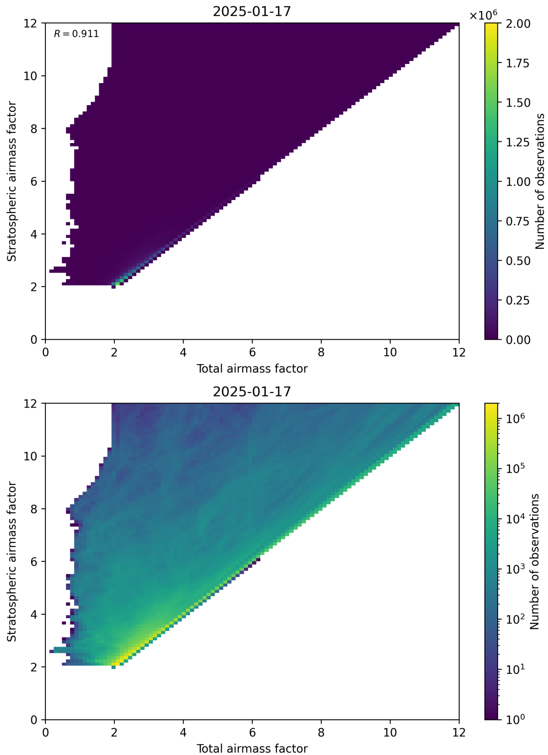
Figure 62: Scatter density plot of “Total airmass factor” against “Stratospheric airmass factor” for 2025-01-17 to 2025-01-18.
