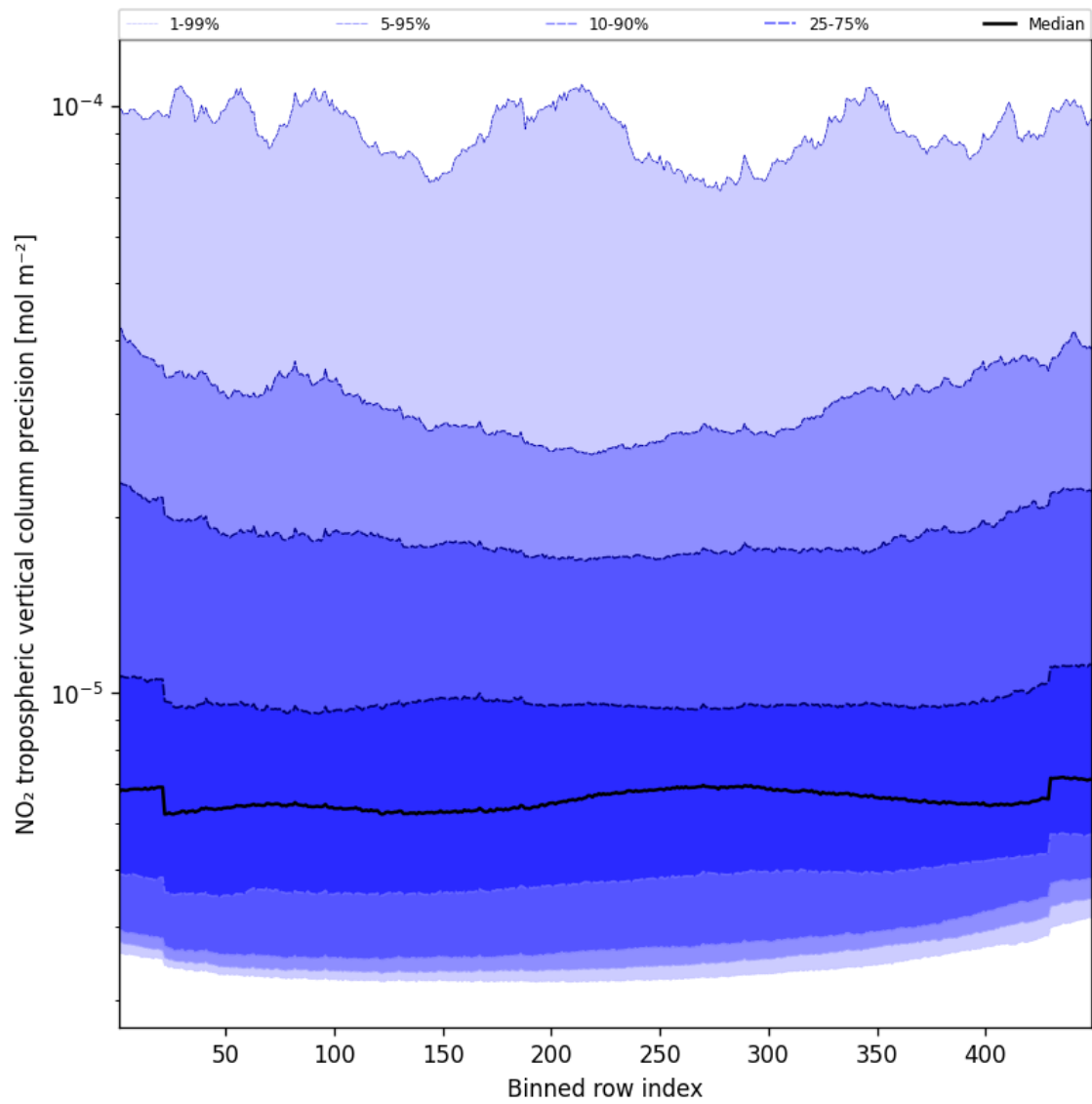
Figure 47: Along track statistics of “NO 2 tropospheric vertical column precision” for 2025-01-17 to 2025-01-18
