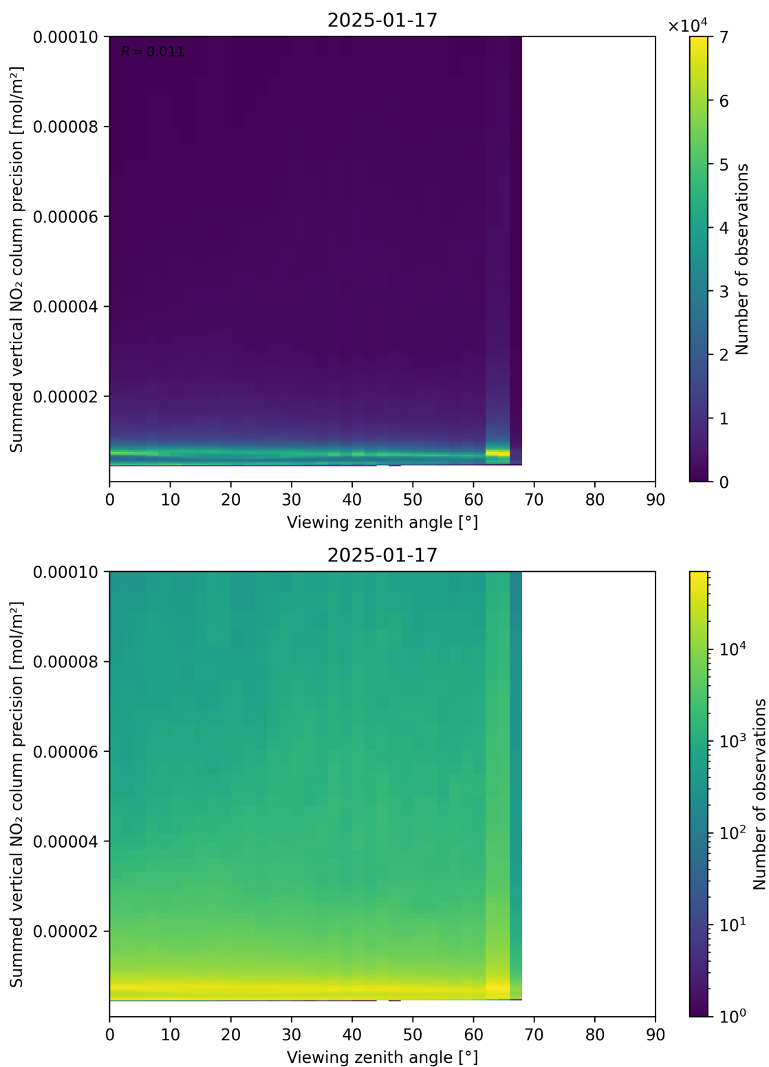
Figure 166: Scatter density plot of “Viewing zenith angle” against “Summed vertical NO 2 column precision” for 2025-01-17 to 2025-01-18.
