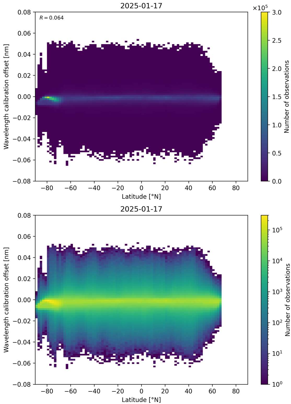
Figure 95: Scatter density plot of “Latitude” against “Wavelength calibration offset” for 2025-01-17 to 2025-01-18.
