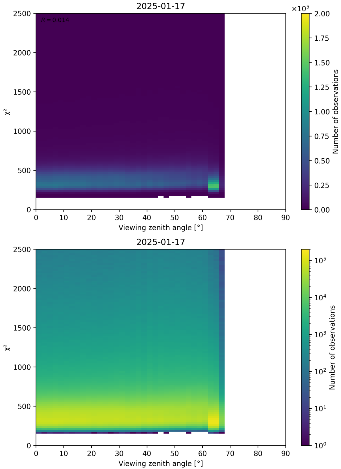
Figure 162: Scatter density plot of “Viewing zenith angle” against “ \chi^2 ” for 2025-01-17 to 2025-01-18.
