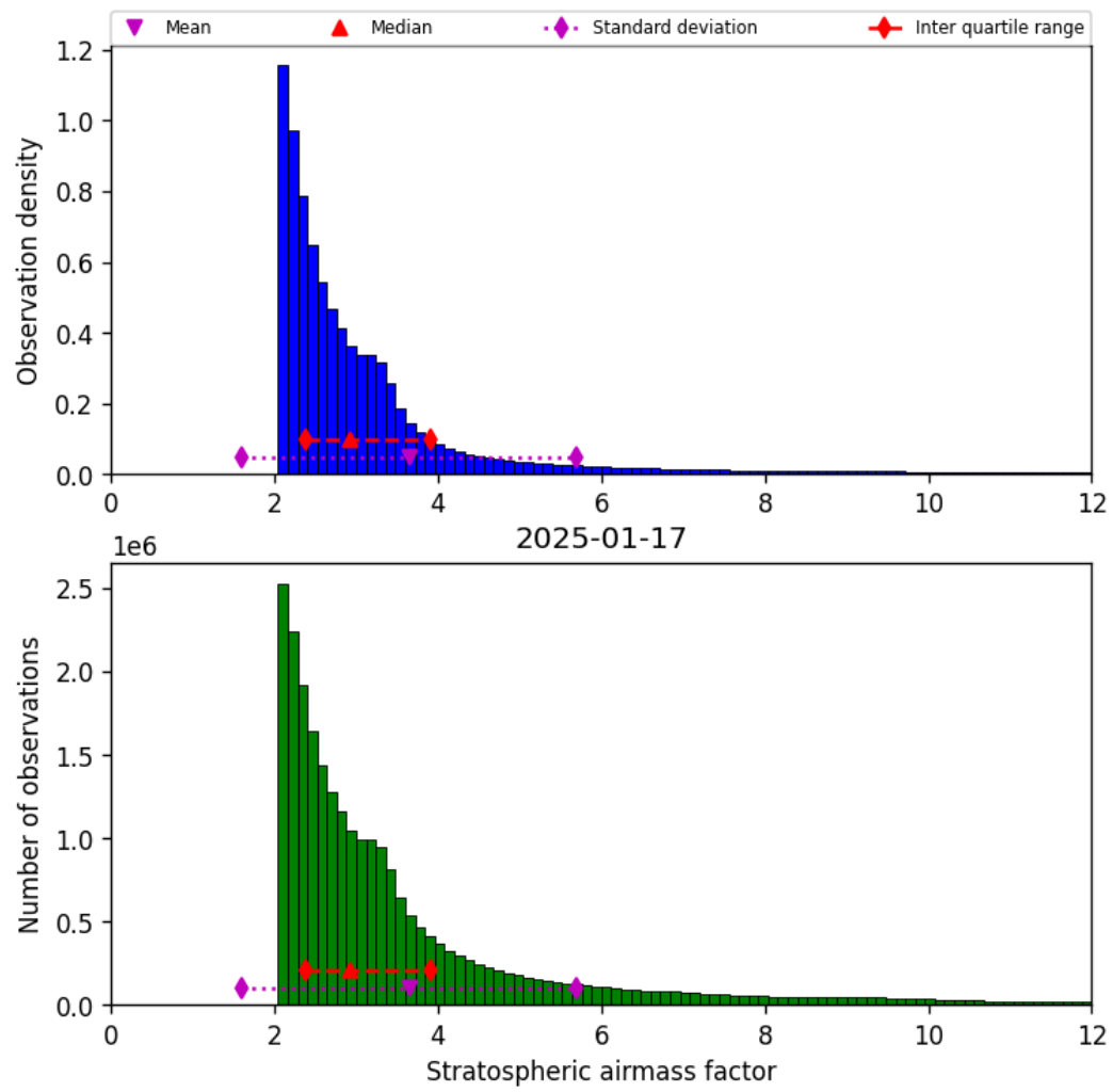
Figure 44: Histogram of “Stratospheric airmass factor” for 2025-01-17 to 2025-01-18
