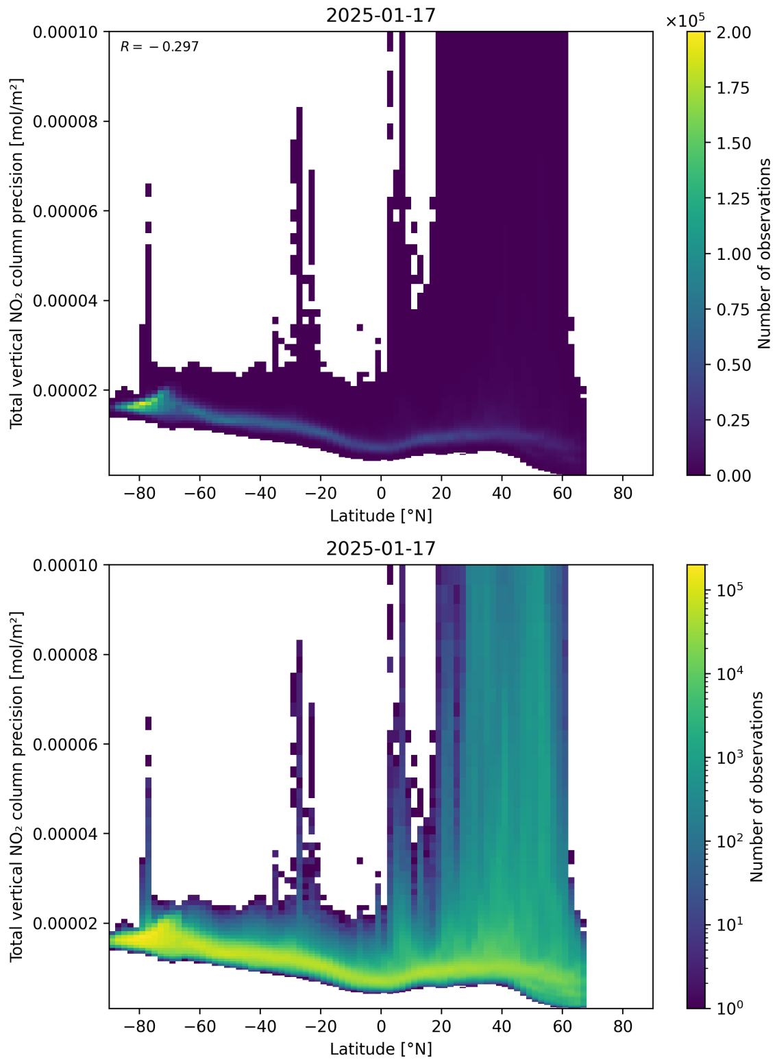
Figure 91: Scatter density plot of “Latitude” against “Total vertical NO 2 column precision” for 2025-01-17 to 2025-01-18.
