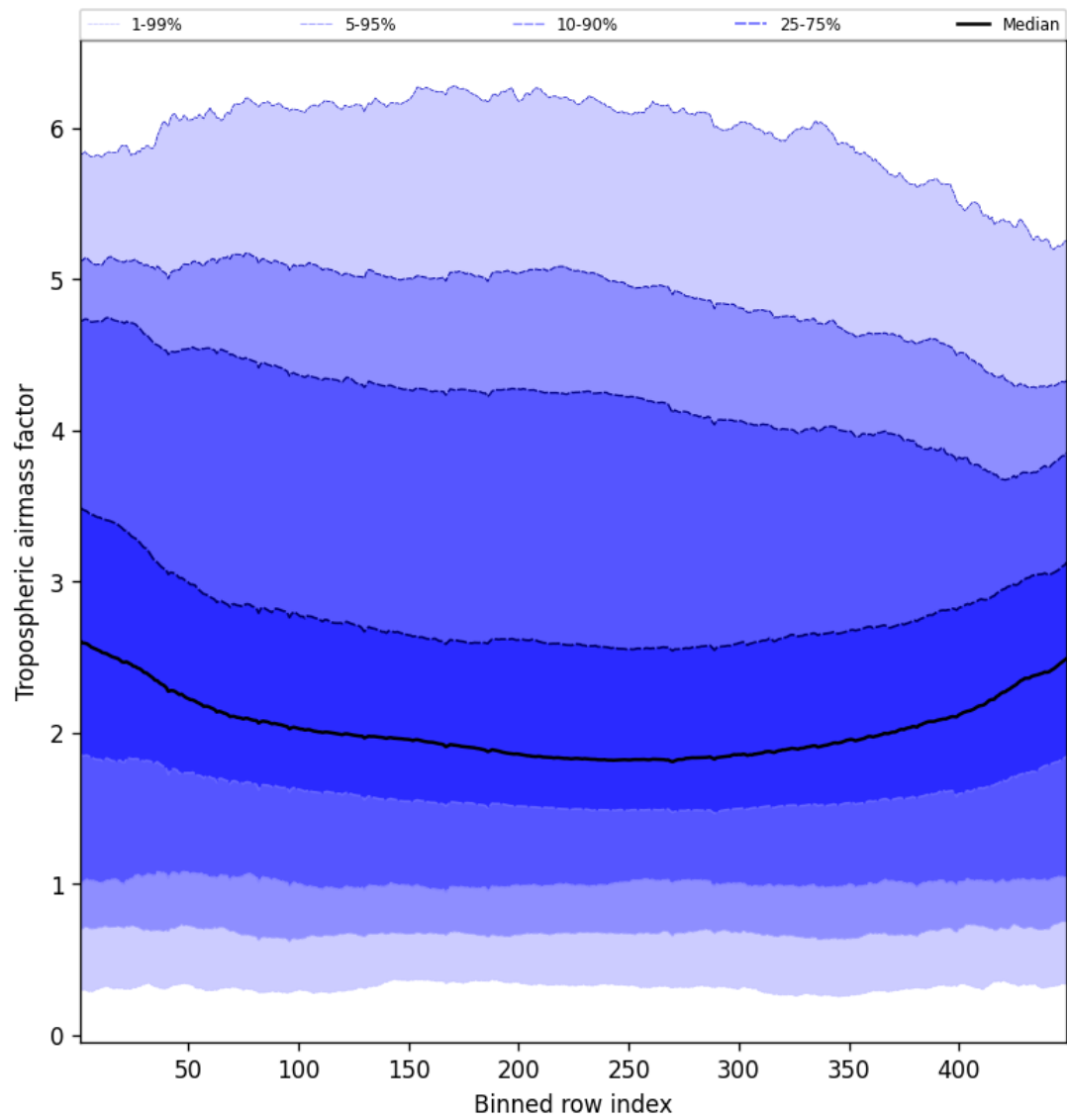
Figure 48: Along track statistics of “Tropospheric airmass factor” for 2025-01-17 to 2025-01-18
