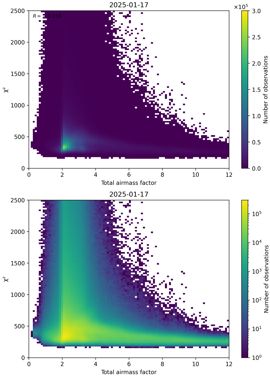
Figure 63: Scatter density plot of “Total airmass factor” against “ \chi^2 ” for 2025-01-17 to 2025-01-18.
