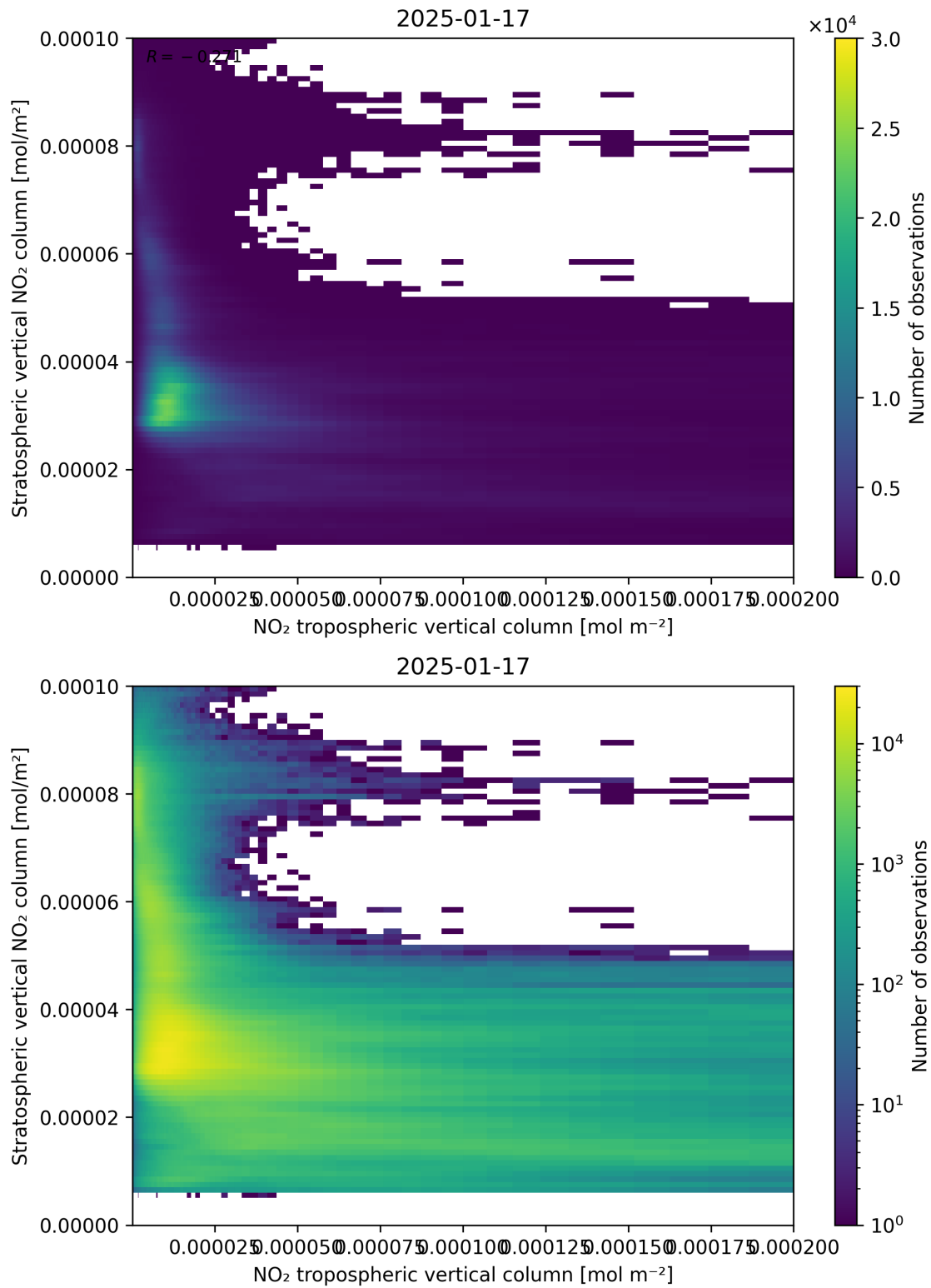
Figure 125: Scatter density plot of “NO 2 tropospheric vertical column” against “Stratospheric vertical NO 2 column” for 2025-01-17 to 2025-01-18.
