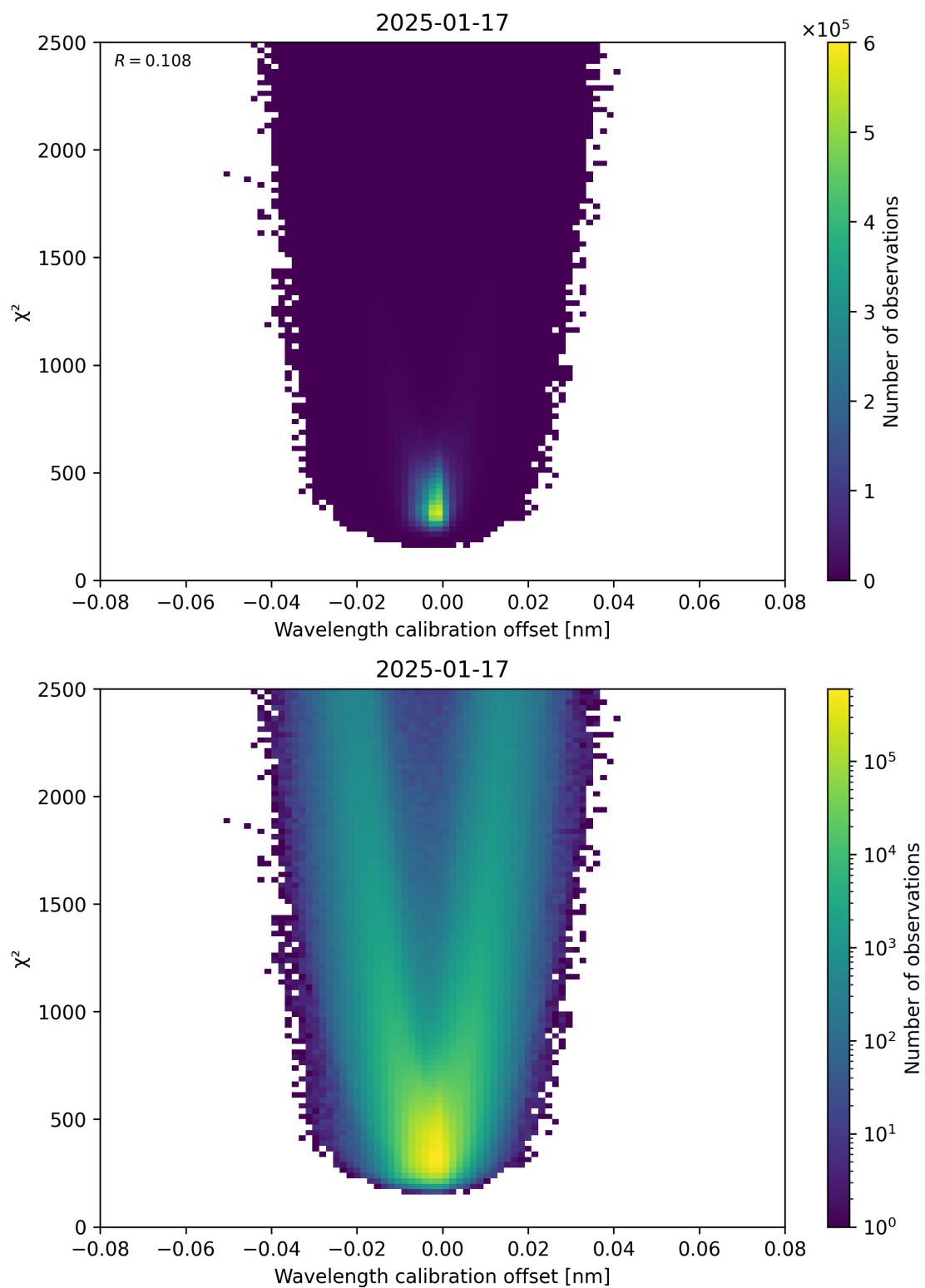
Figure 175: Scatter density plot of “Wavelength calibration offset” against “ \chi^2 ” for 2025-01-17 to 2025-01-18.
