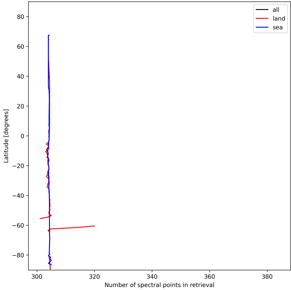
Figure 16: Zonal average of “Number of spectral points in retrieval” for 2025-01-17 to 2025-01-18.
