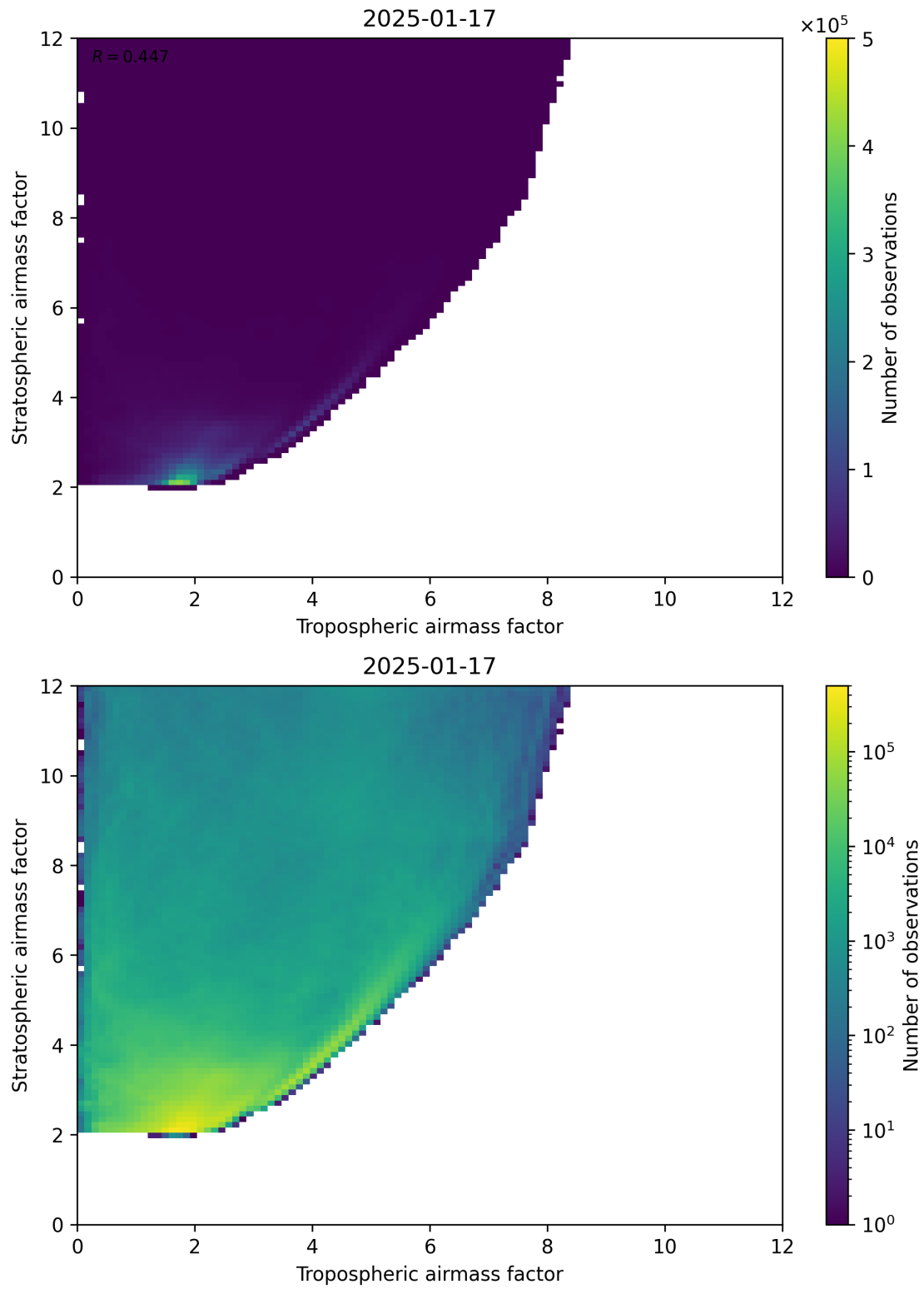
Figure 71: Scatter density plot of “Tropospheric airmass factor” against “Stratospheric airmass factor” for 2025-01-17 to 2025-01-18.
