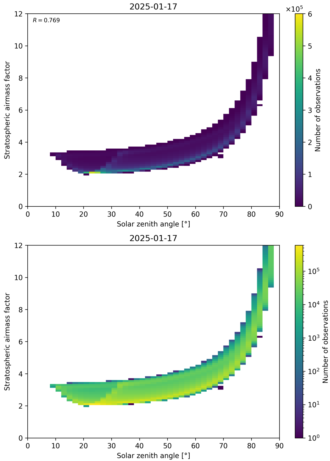
Figure 145: Scatter density plot of “Solar zenith angle” against “Stratospheric airmass factor” for 2025-01-17 to 2025-01-18.
