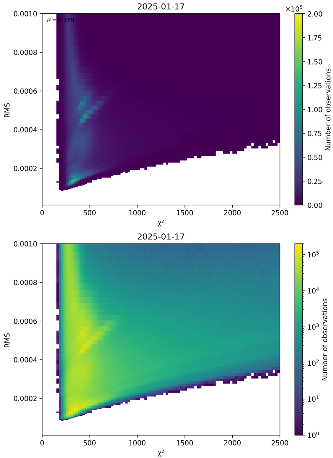
Figure 82: Scatter density plot of “ \chi^2 ” against “RMS” for 2025-01-17 to 2025-01-18.
