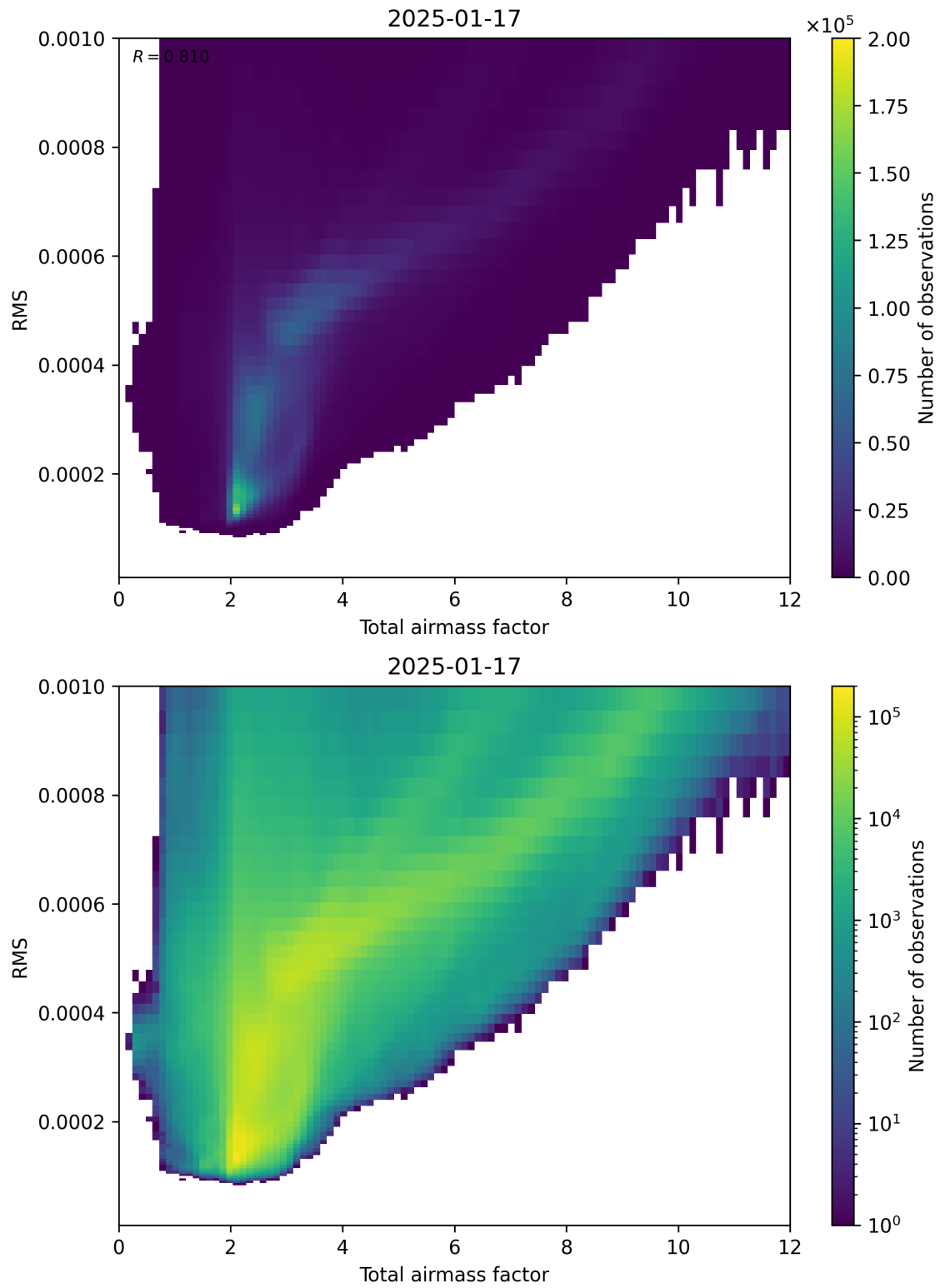
Figure 69: Scatter density plot of “Total airmass factor” against “RMS” for 2025-01-17 to 2025-01-18.
