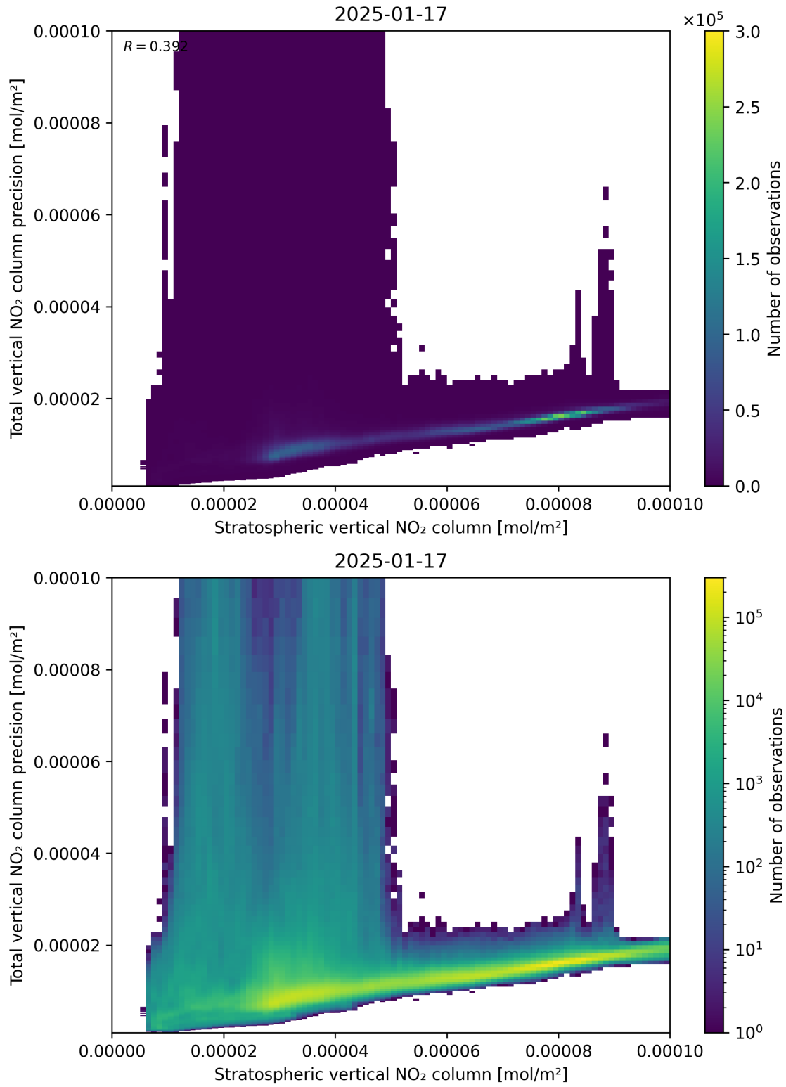
Figure 101: Scatter density plot of “Stratospheric vertical NO 2 column” against “Total vertical NO 2 column precision” for 2025-01-17 to 2025-01-18.
