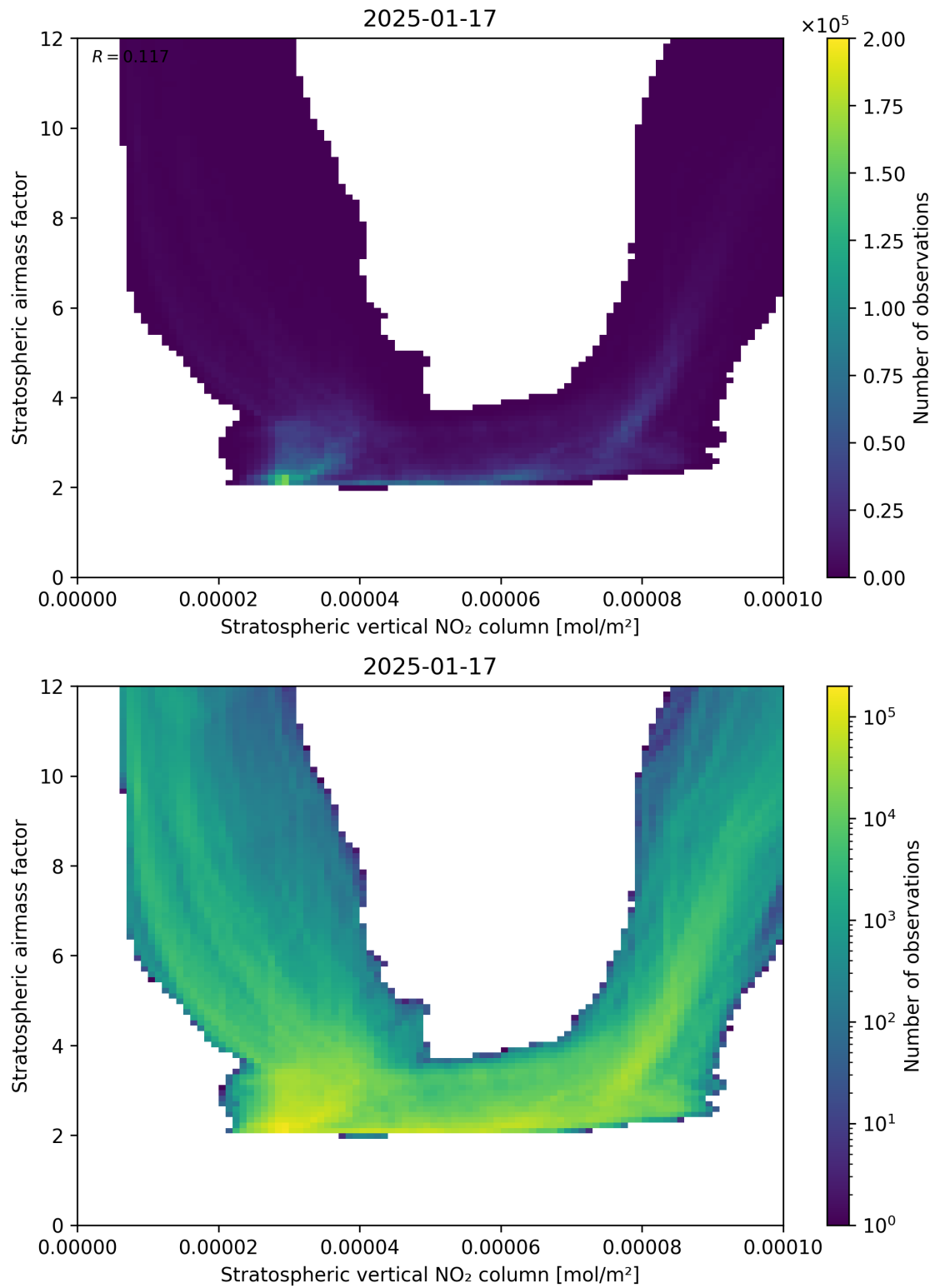
Figure 96: Scatter density plot of “Stratospheric vertical NO 2 column” against “Stratospheric airmass factor” for 2025-01-17 to 2025-01-18.
