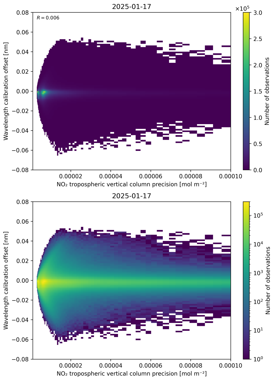
Figure 141: Scatter density plot of “NO 2 tropospheric vertical column precision” against “Wavelength calibration offset” for 2025-01-17 to 2025-01-18.
