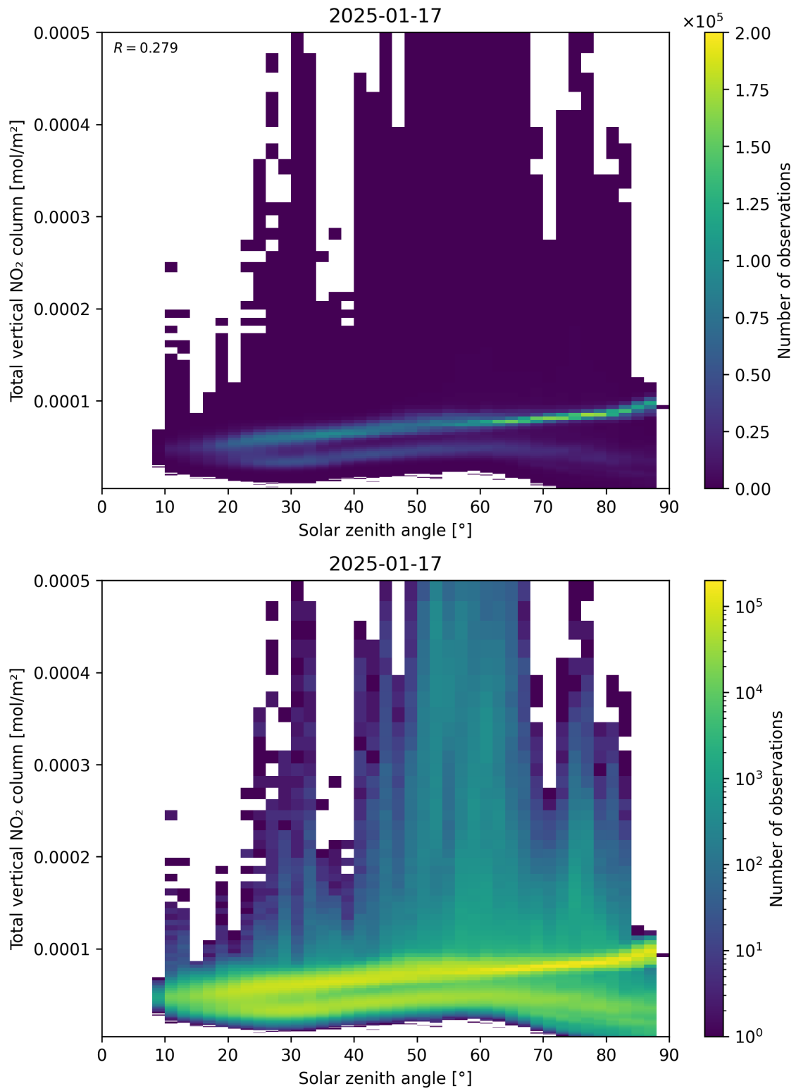
Figure 153: Scatter density plot of “Solar zenith angle” against “Total vertical NO 2 column” for 2025-01-17 to 2025-01-18.
