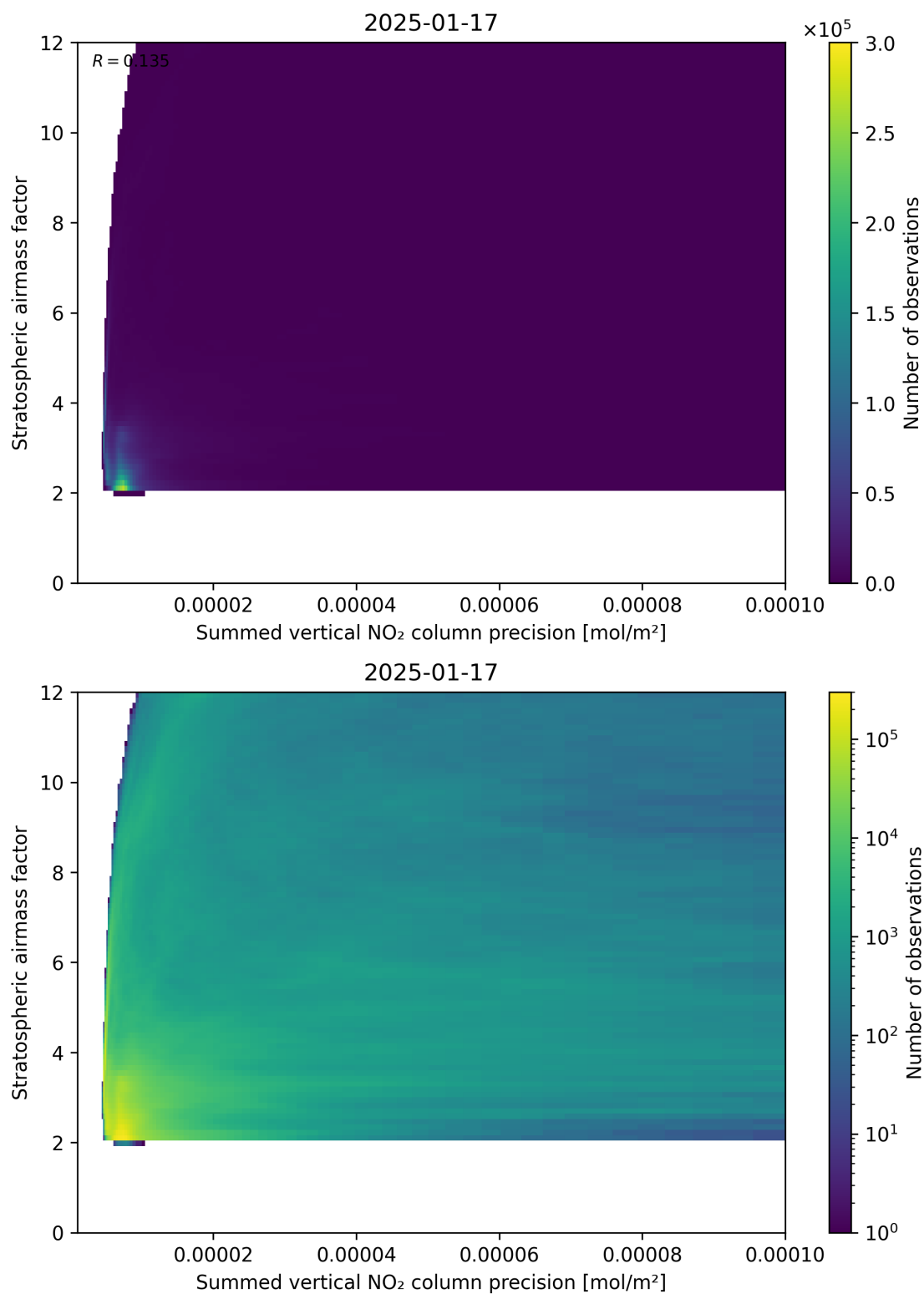
Figure 106: Scatter density plot of “Summed vertical NO 2 column precision” against “Stratospheric airmass factor” for 2025-01-17 to 2025-01-18.
