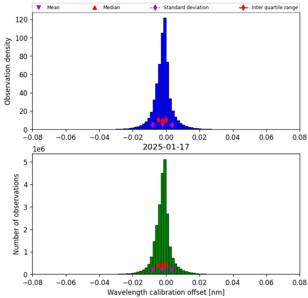
Figure 35: Histogram of “Wavelength calibration offset” for 2025-01-17 to 2025-01-18
