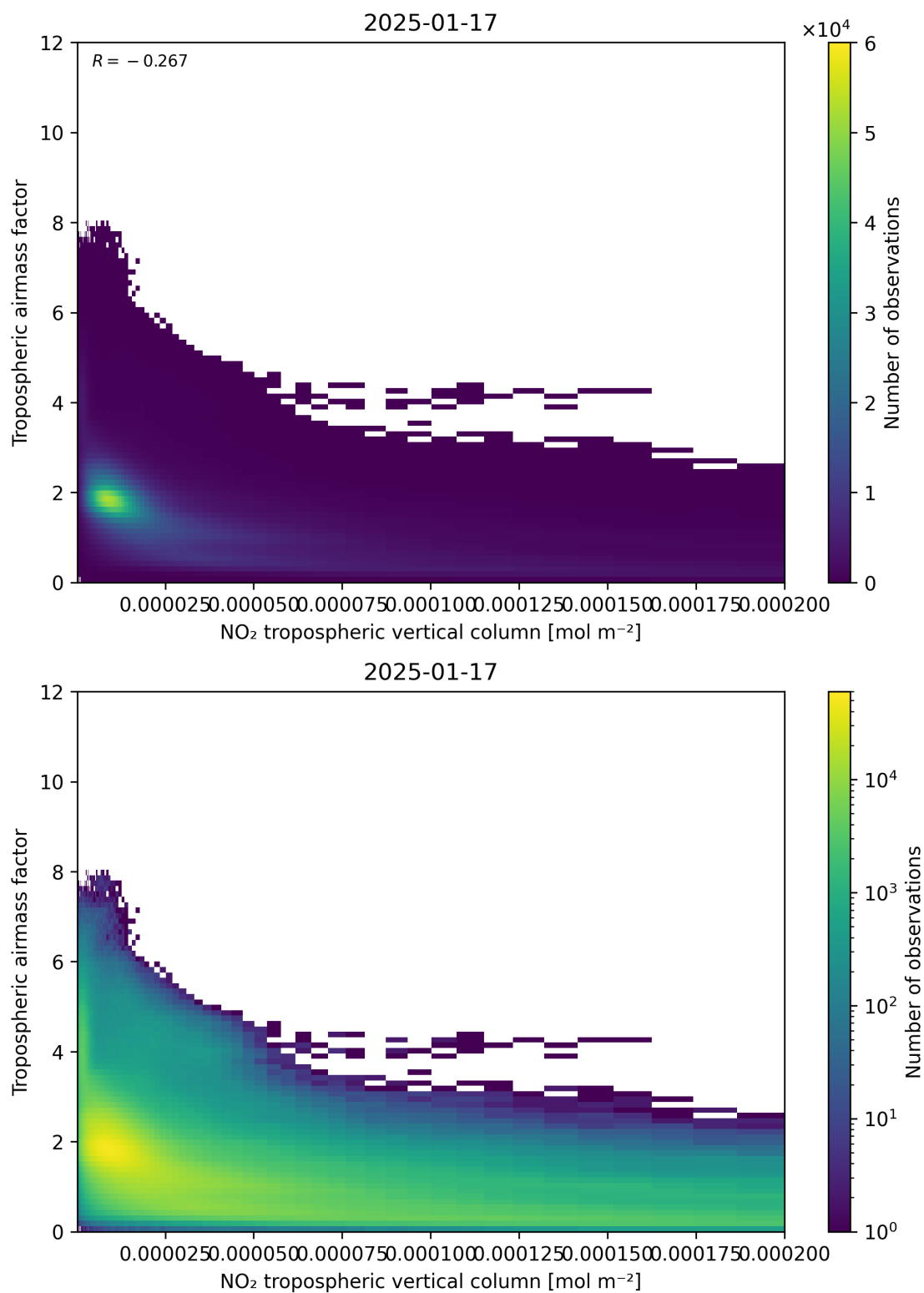
Figure 123: Scatter density plot of “NO 2 tropospheric vertical column” against “Tropospheric air mass factor” for 2025-01-17 to 2025-01-18.
