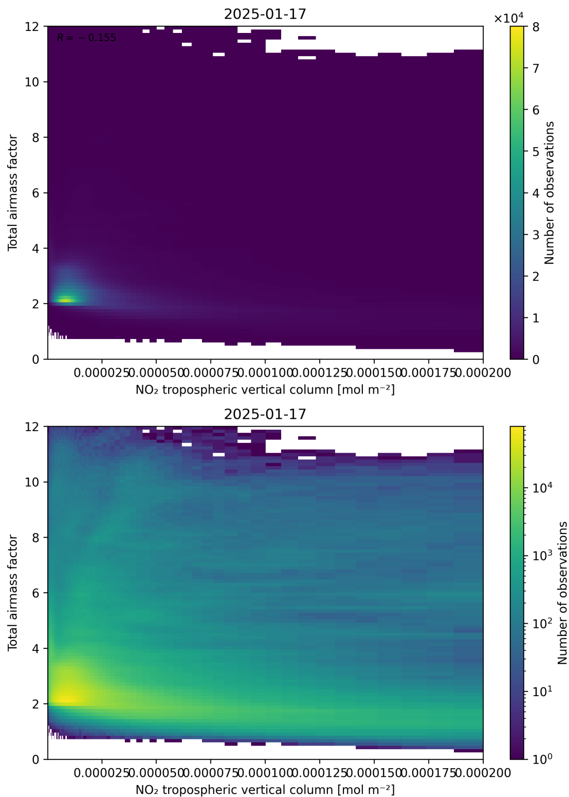
Figure 122: Scatter density plot of “NO 2 tropospheric vertical column” against “Total air mass factor” for 2025-01-17 to 2025-01-18.
