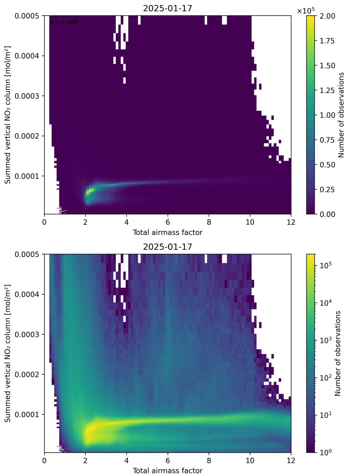
Figure 65: Scatter density plot of “Total airmass factor” against “Summed vertical NO 2 column” for 2025-01-17 to 2025-01-18.
