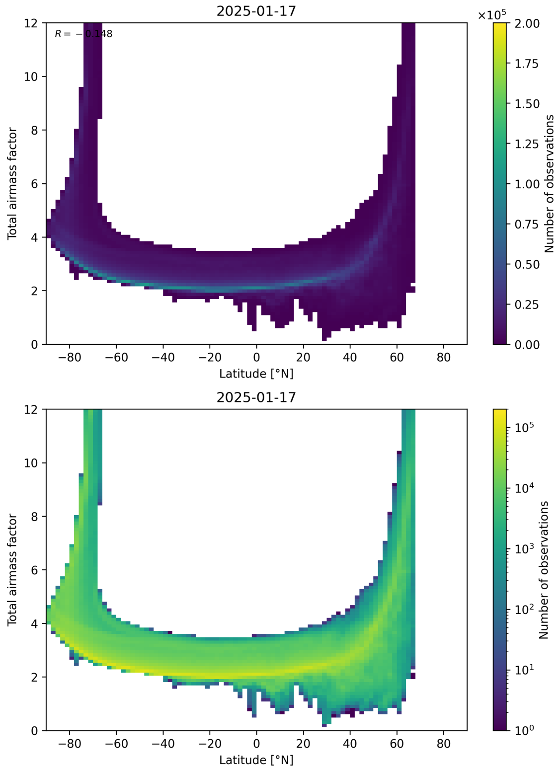
Figure 84: Scatter density plot of “Latitude” against “Total airmass factor” for 2025-01-17 to 2025-01-18.
