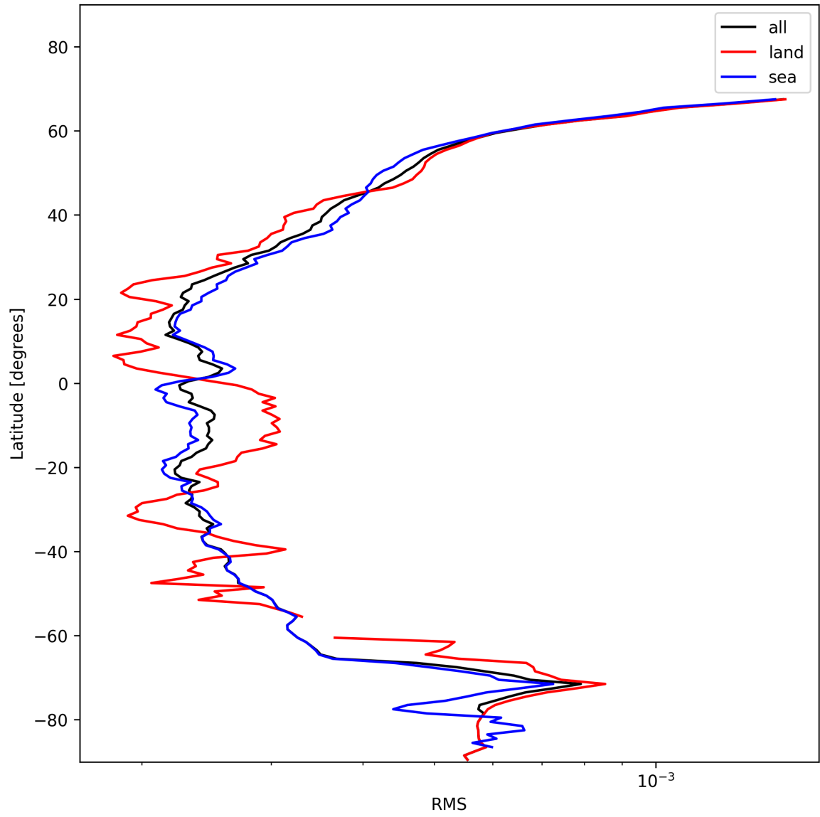
Figure 26: Zonal average of “RMS” for 2025-01-17 to 2025-01-18.
