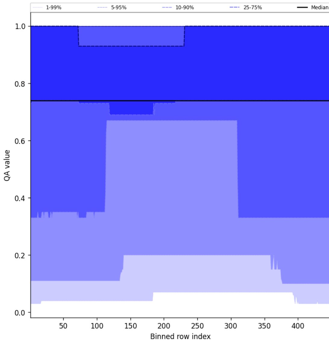
Figure 45: Along track statistics of “QA value” for 2025-01-17 to 2025-01-18
