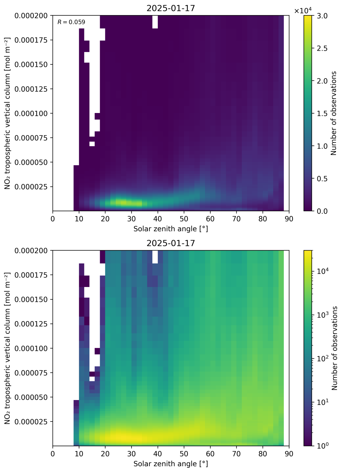
Figure 155: Scatter density plot of “Solar zenith angle” against “NO 2 tropospheric vertical column” for 2025-01-17 to 2025-01-18.
