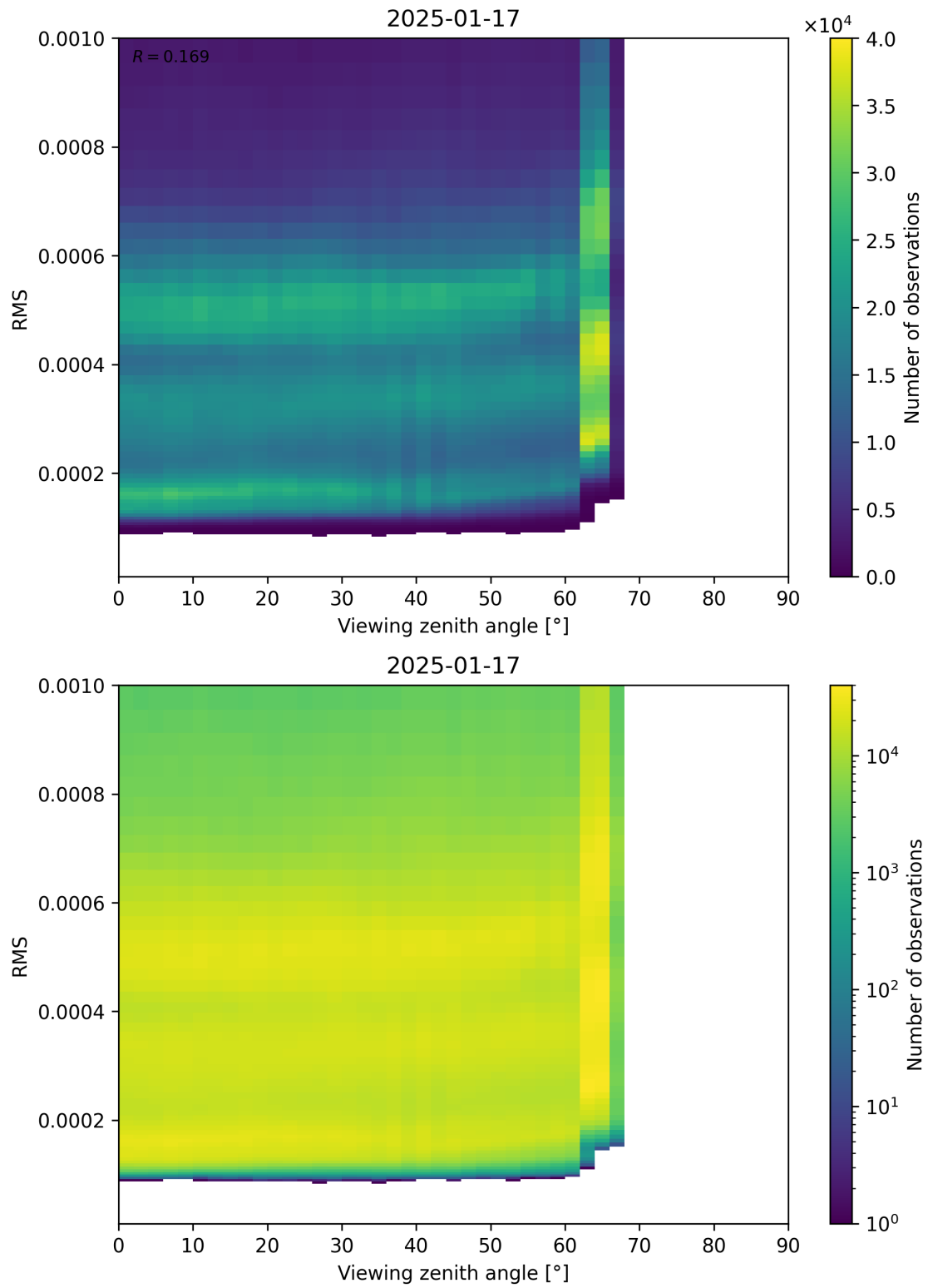
Figure 171: Scatter density plot of “Viewing zenith angle” against “RMS” for 2025-01-17 to 2025-01-18.
