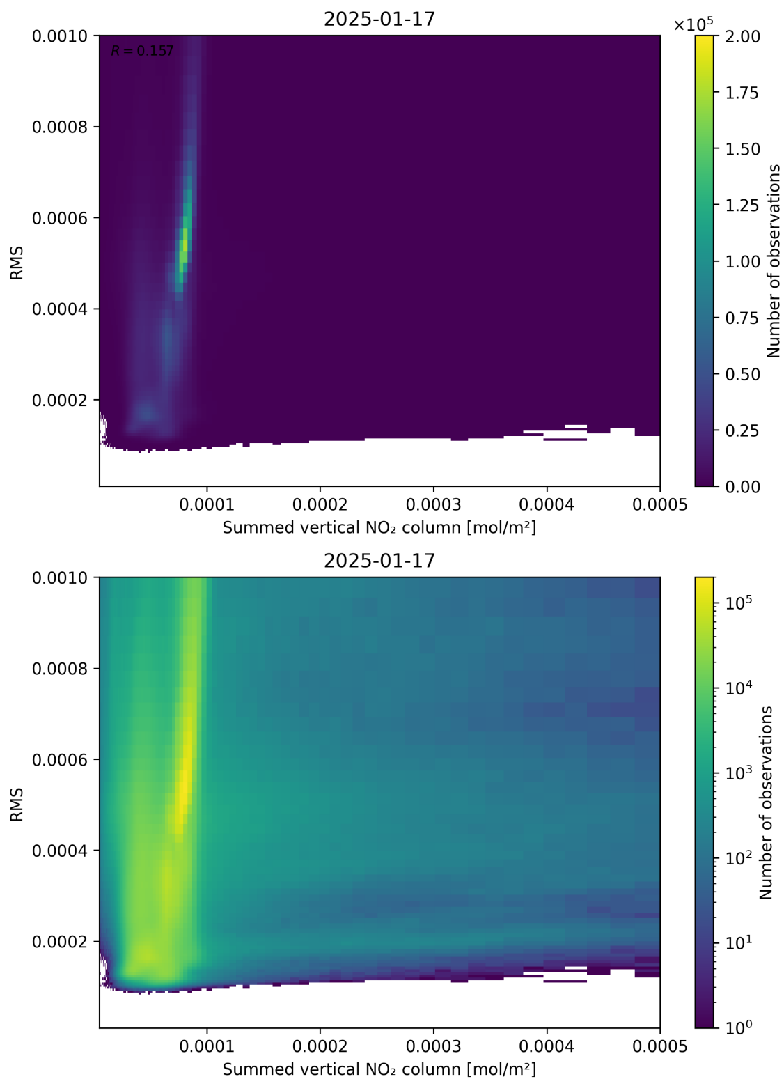
Figure 109: Scatter density plot of “Summed vertical NO 2 column” against “RMS” for 2025-01-17 to 2025-01-18.
