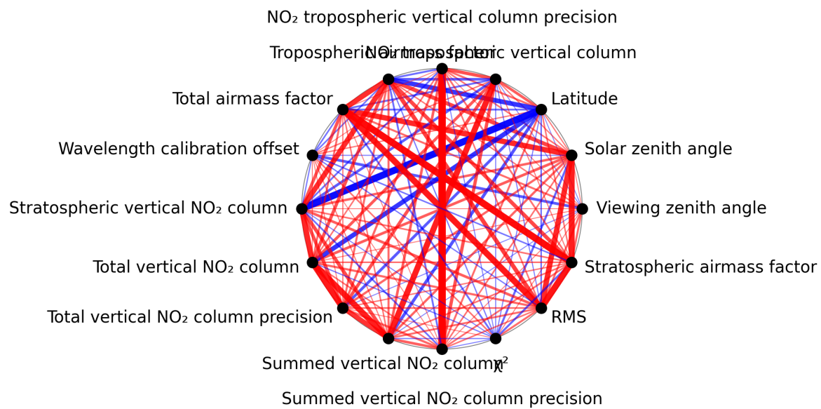
Figure 1: Map of correlation graph for 2025-01-17 to 2025-01-18.
