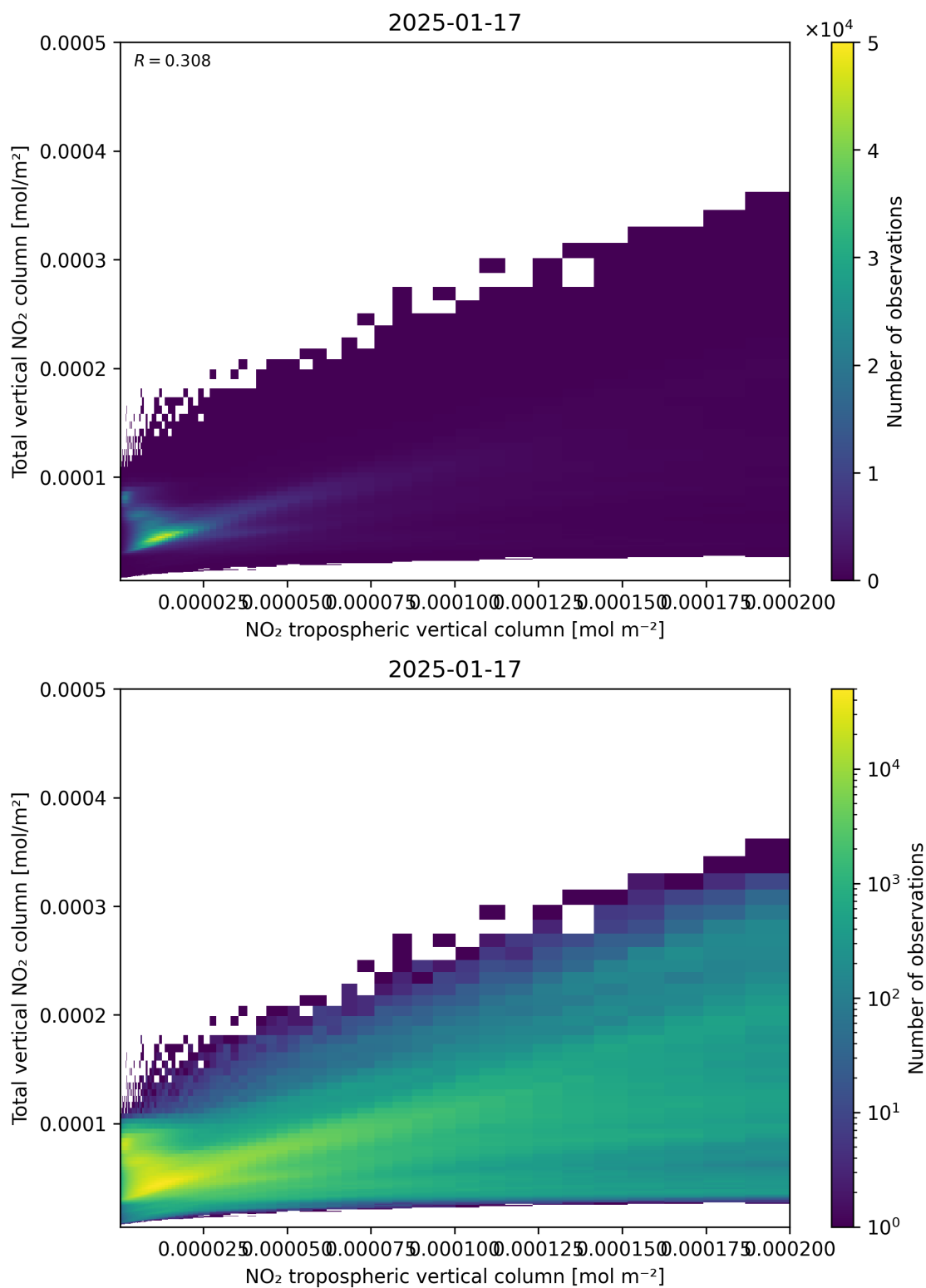
Figure 128: Scatter density plot of “NO 2 tropospheric vertical column” against “Total vertical NO 2 column” for 2025-01-17 to 2025-01-18.
