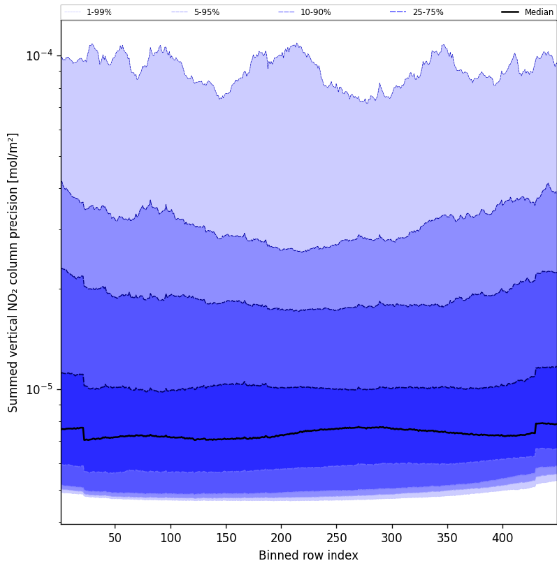
Figure 58: Along track statistics of “Summed vertical NO 2 column precision” for 2025-01-17 to 2025-01-18
