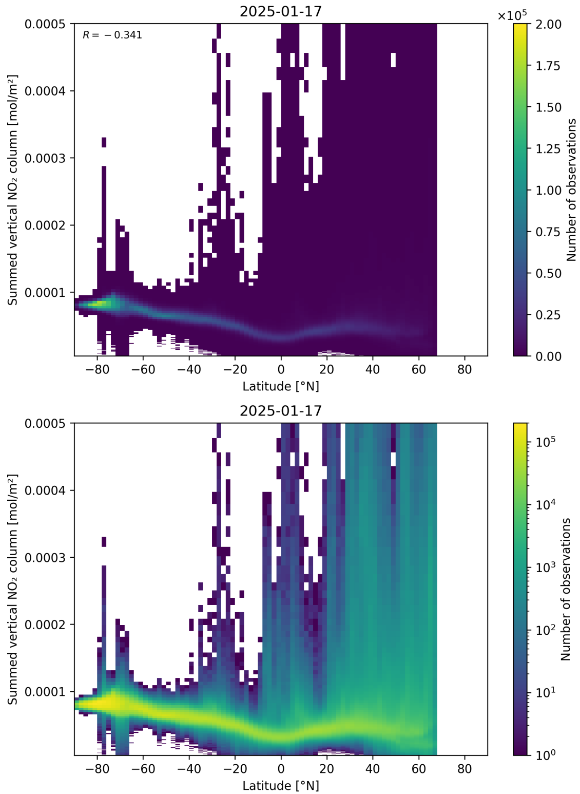
Figure 88: Scatter density plot of “Latitude” against “Summed vertical NO 2 column” for 2025-01-17 to 2025-01-18.
