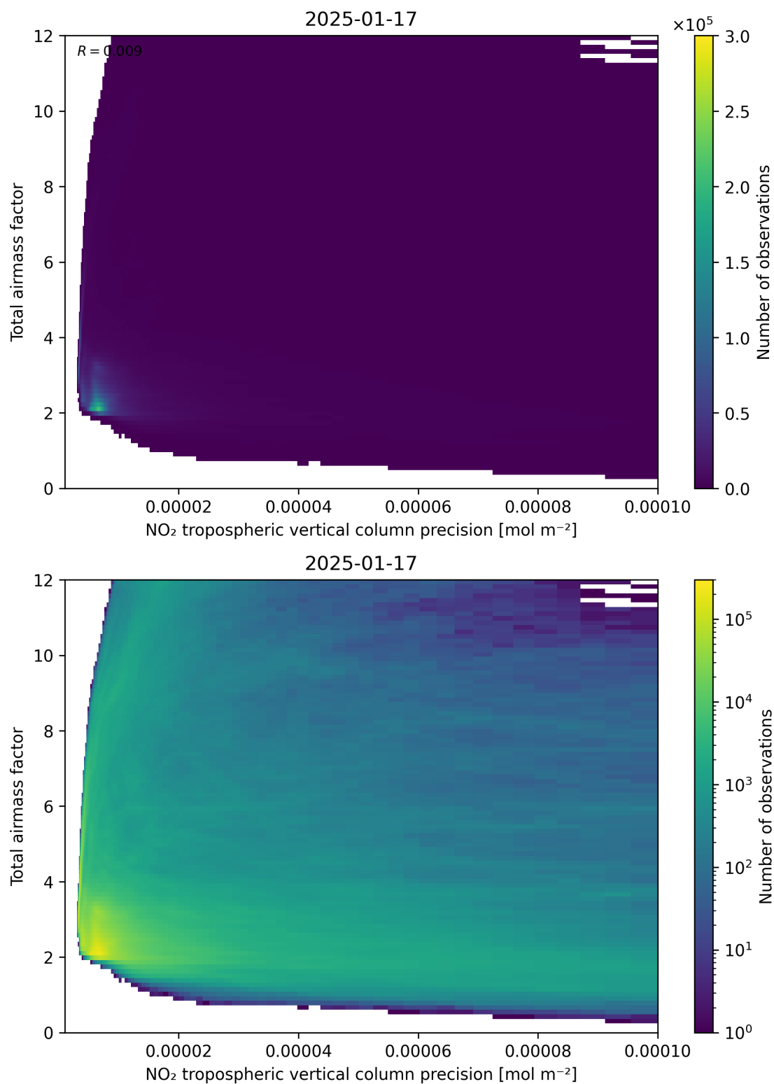
Figure 132: Scatter density plot of “NO 2 tropospheric vertical column precision” against “Total air mass factor” for 2025-01-17 to 2025-01-18.
