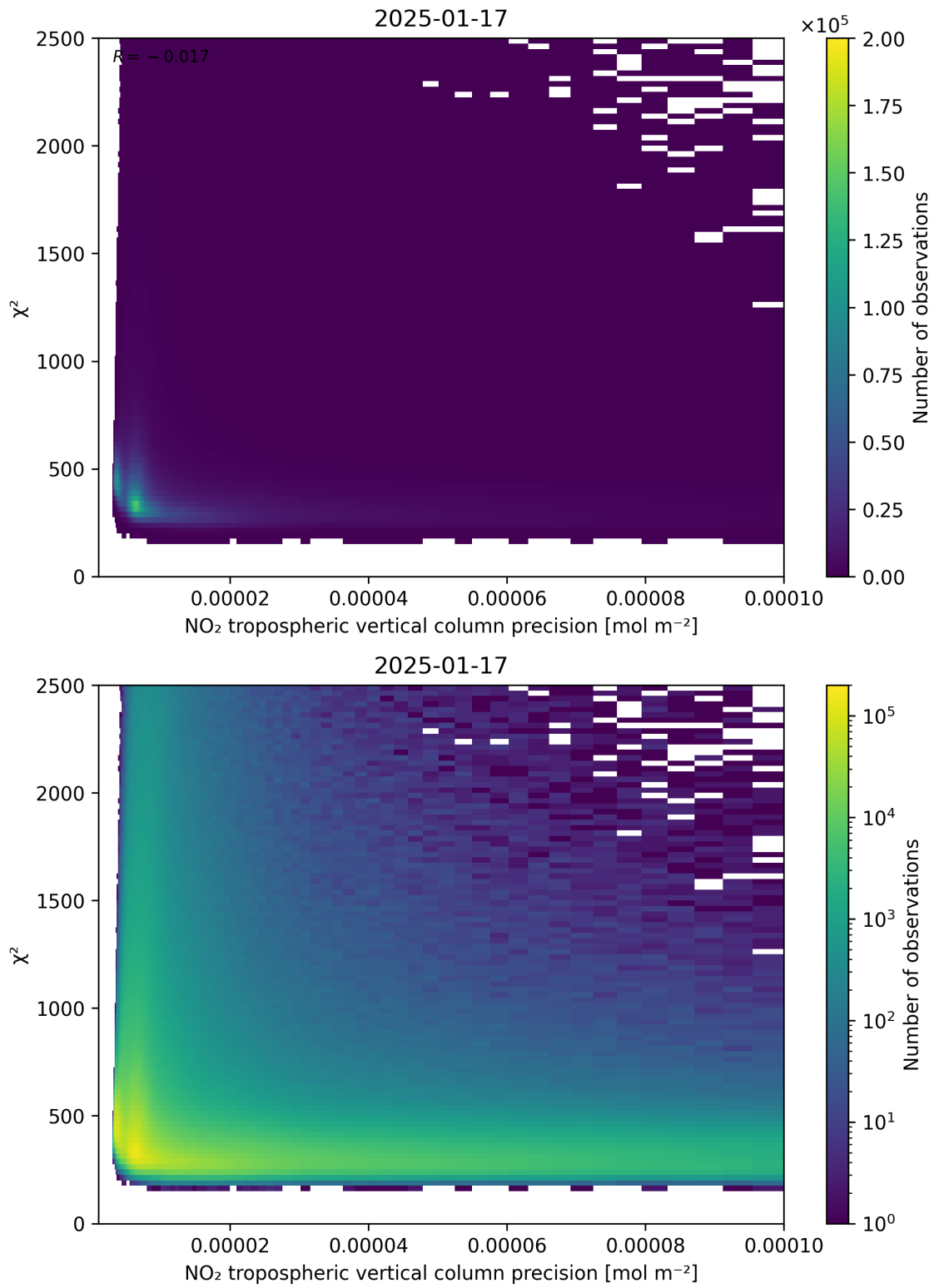
Figure 134: Scatter density plot of “NO 2 tropospheric vertical column precision” against “ \chi^2 ” for 2025-01-17 to 2025-01-18.
