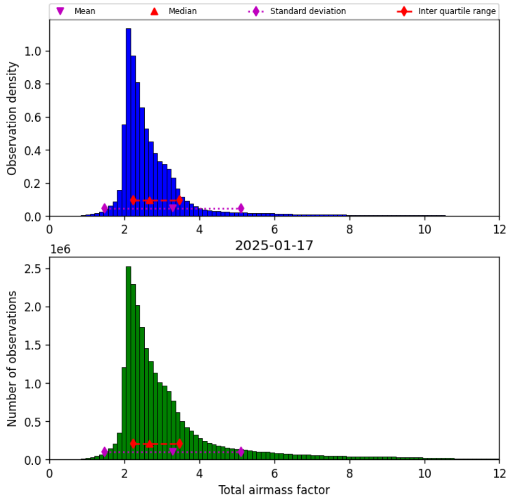
Figure 32: Histogram of “Total airmass factor” for 2025-01-17 to 2025-01-18
