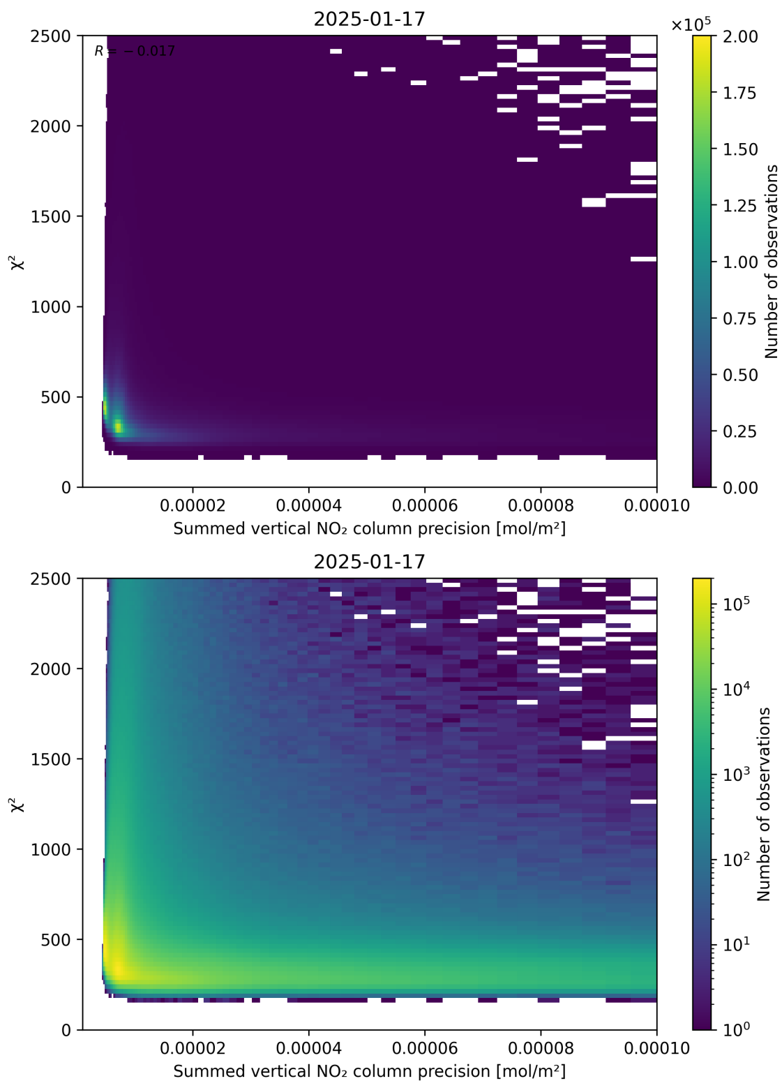
Figure 107: Scatter density plot of “Summed vertical NO 2 column precision” against “ \chi^2 ” for 2025-01-17 to 2025-01-18.
