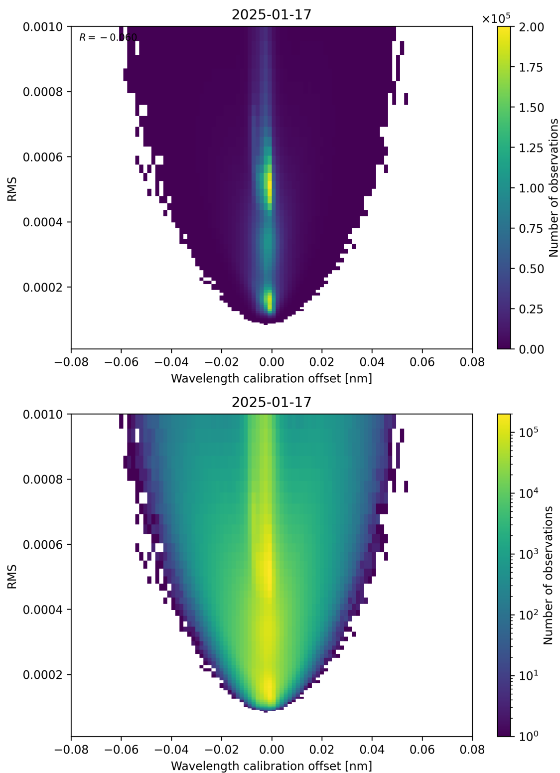
Figure 181: Scatter density plot of “Wavelength calibration offset” against “RMS” for 2025-01-17 to 2025-01-18.
