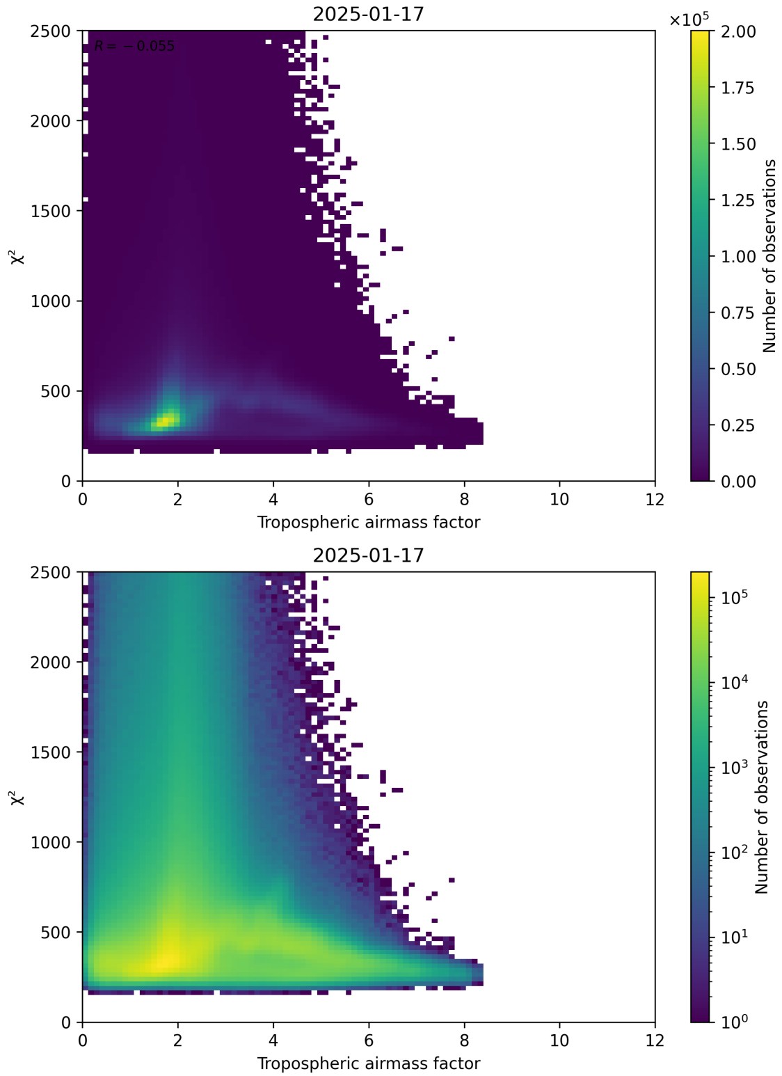
Figure 73: Scatter density plot of “Tropospheric airmass factor” against “ \chi^2 ” for 2025-01-17 to 2025-01-18.
