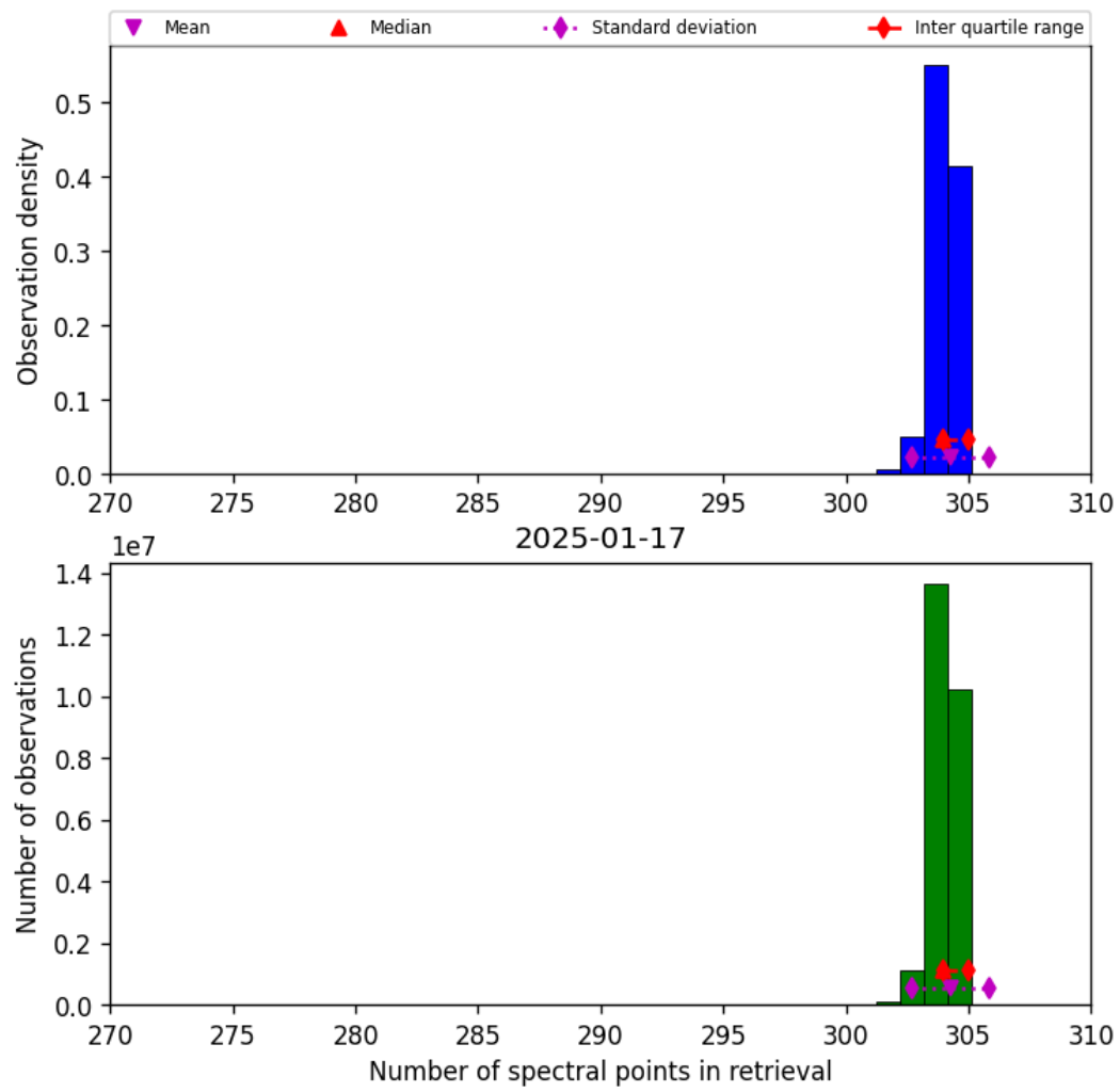
Figure 33: Histogram of “Number of spectral points in retrieval” for 2025-01-17 to 2025-01-18
