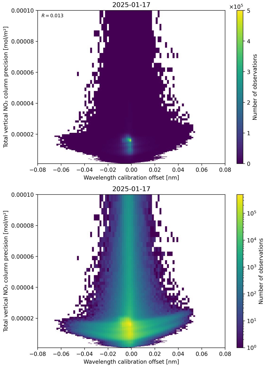
Figure 180: Scatter density plot of “Wavelength calibration offset” against “Total vertical NO 2 column precision” for 2025-01-17 to 2025-01-18.
