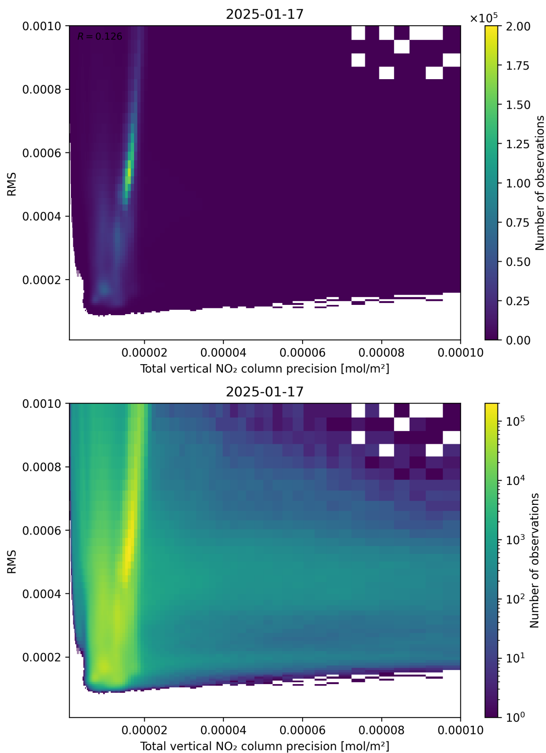
Figure 119: Scatter density plot of “Total vertical NO 2 column precision” against “RMS” for 2025-01-17 to 2025-01-18.
