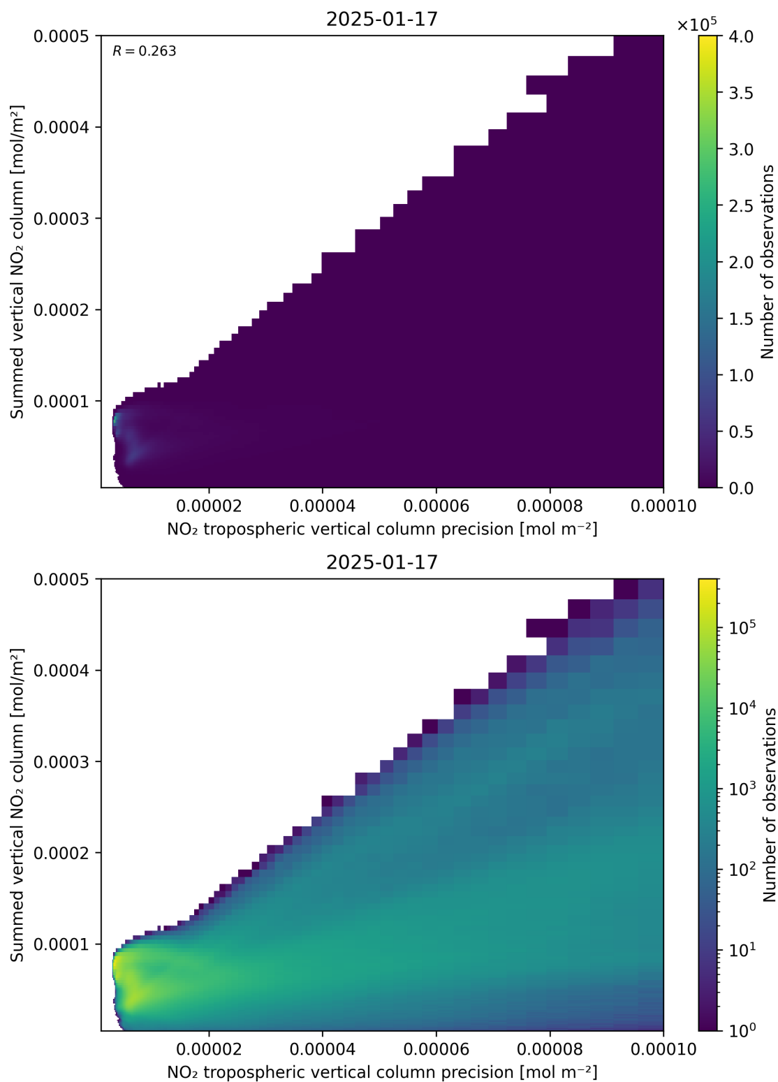
Figure 136: Scatter density plot of “NO 2 tropospheric vertical column precision” against “Summed vertical NO 2 column” for 2025-01-17 to 2025-01-18.
