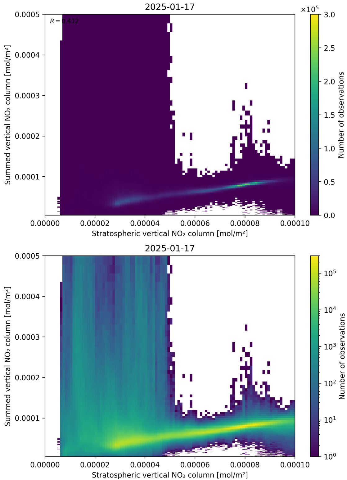
Figure 98: Scatter density plot of “Stratospheric vertical NO 2 column” against “Summed vertical NO 2 column” for 2025-01-17 to 2025-01-18.
