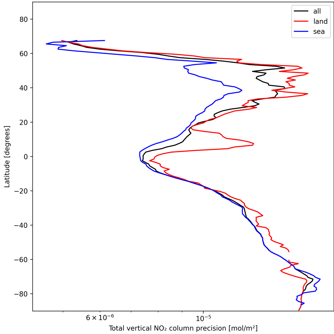
Figure 22: Zonal average of “Total vertical NO 2 column precision” for 2025-01-17 to 2025-01-18.
