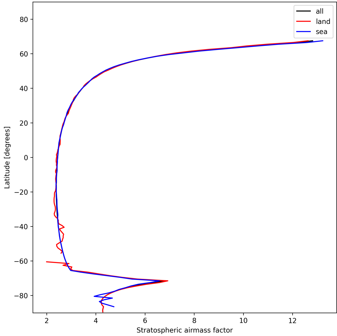
Figure 27: Zonal average of “Stratospheric airmass factor” for 2025-01-17 to 2025-01-18.
