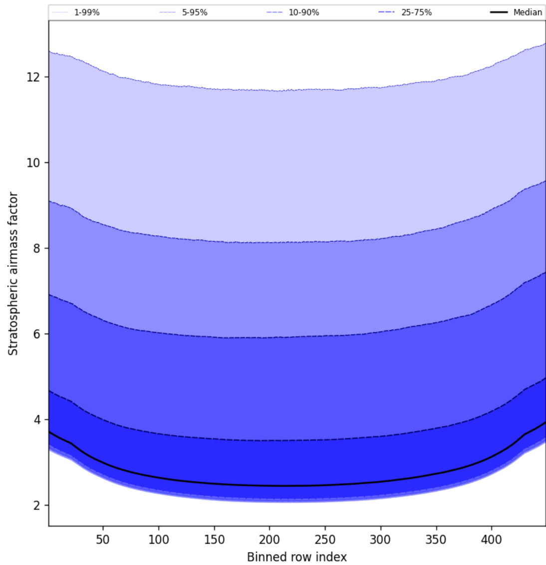
Figure 61: Along track statistics of “Stratospheric air mass factor” for 2025-01-17 to 2025-01-18
