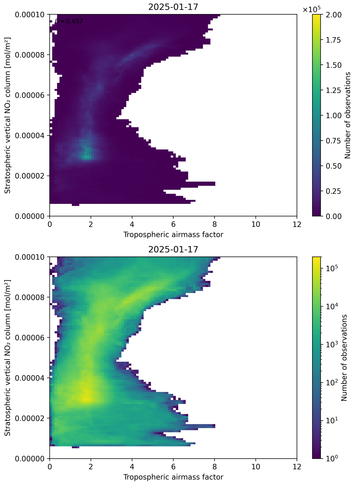
Figure 74: Scatter density plot of “Tropospheric air mass factor” against “Stratospheric vertical NO 2 column” for 2025-01-17 to 2025-01-18.
