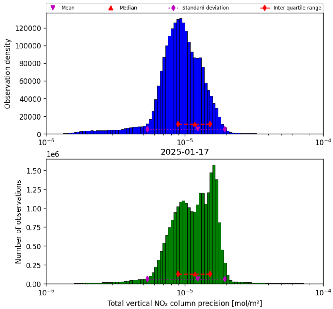
Figure 39: Histogram of “Total vertical NO 2 column precision” for 2025-01-17 to 2025-01-18
