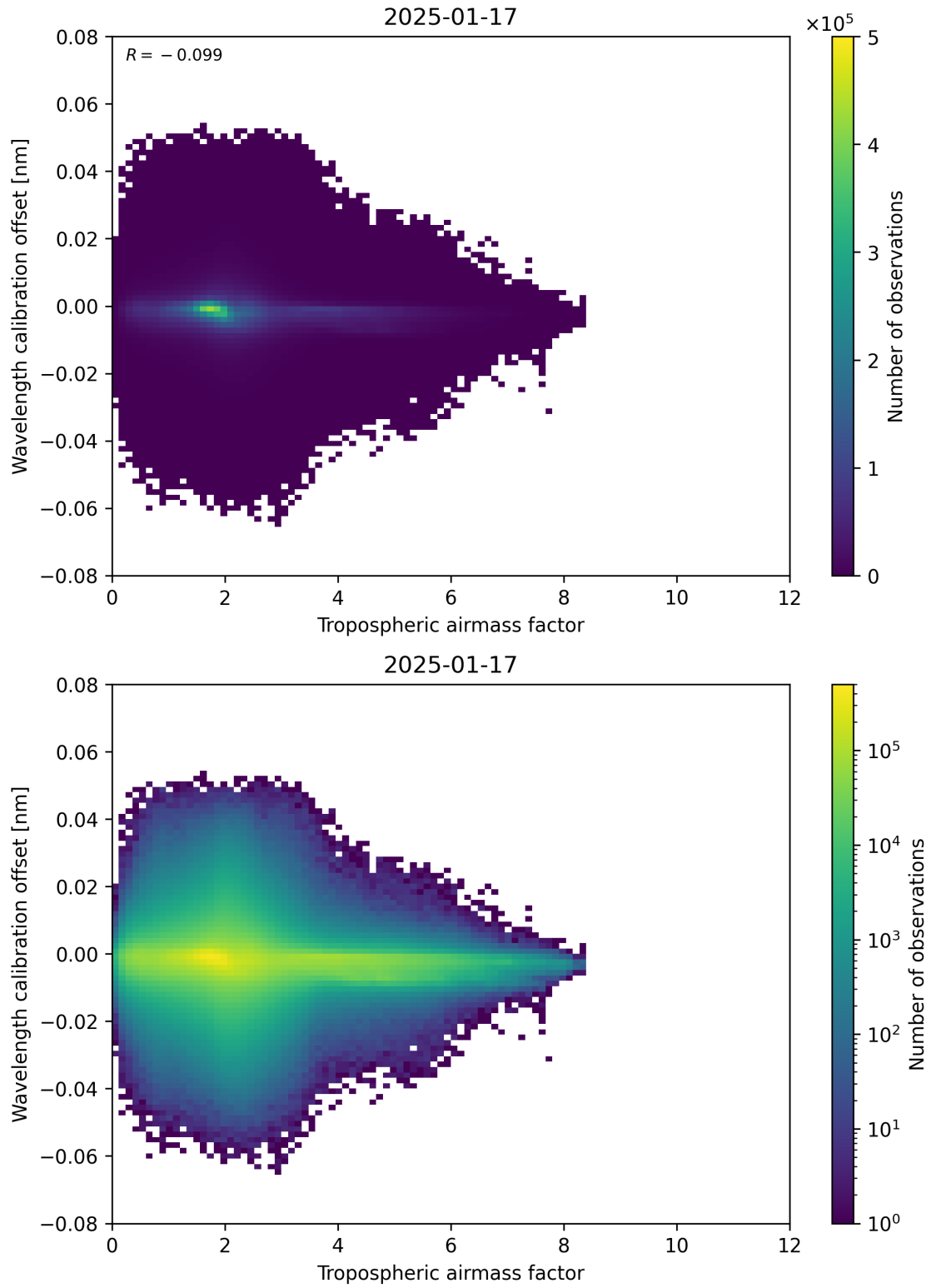
Figure 80: Scatter density plot of “Tropospheric airmass factor” against “Wavelength calibration offset” for 2025-01-17 to 2025-01-18.
