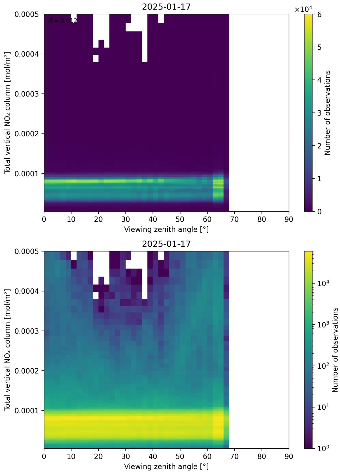
Figure 167: Scatter density plot of “Viewing zenith angle” against “Total vertical NO 2 column” for 2025-01-17 to 2025-01-18.
