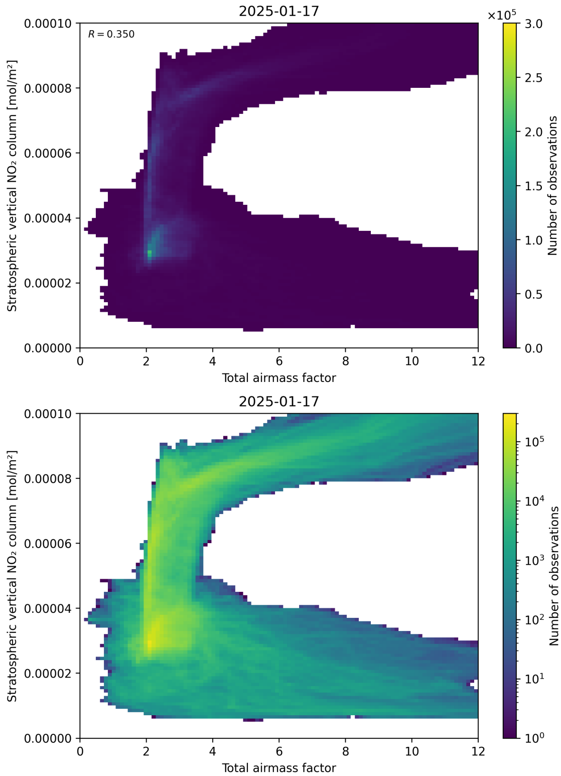
Figure 64: Scatter density plot of “Total airmass factor” against “Stratospheric vertical \text{NO}_2 column” for 2025-01-17 to 2025-01-18.
