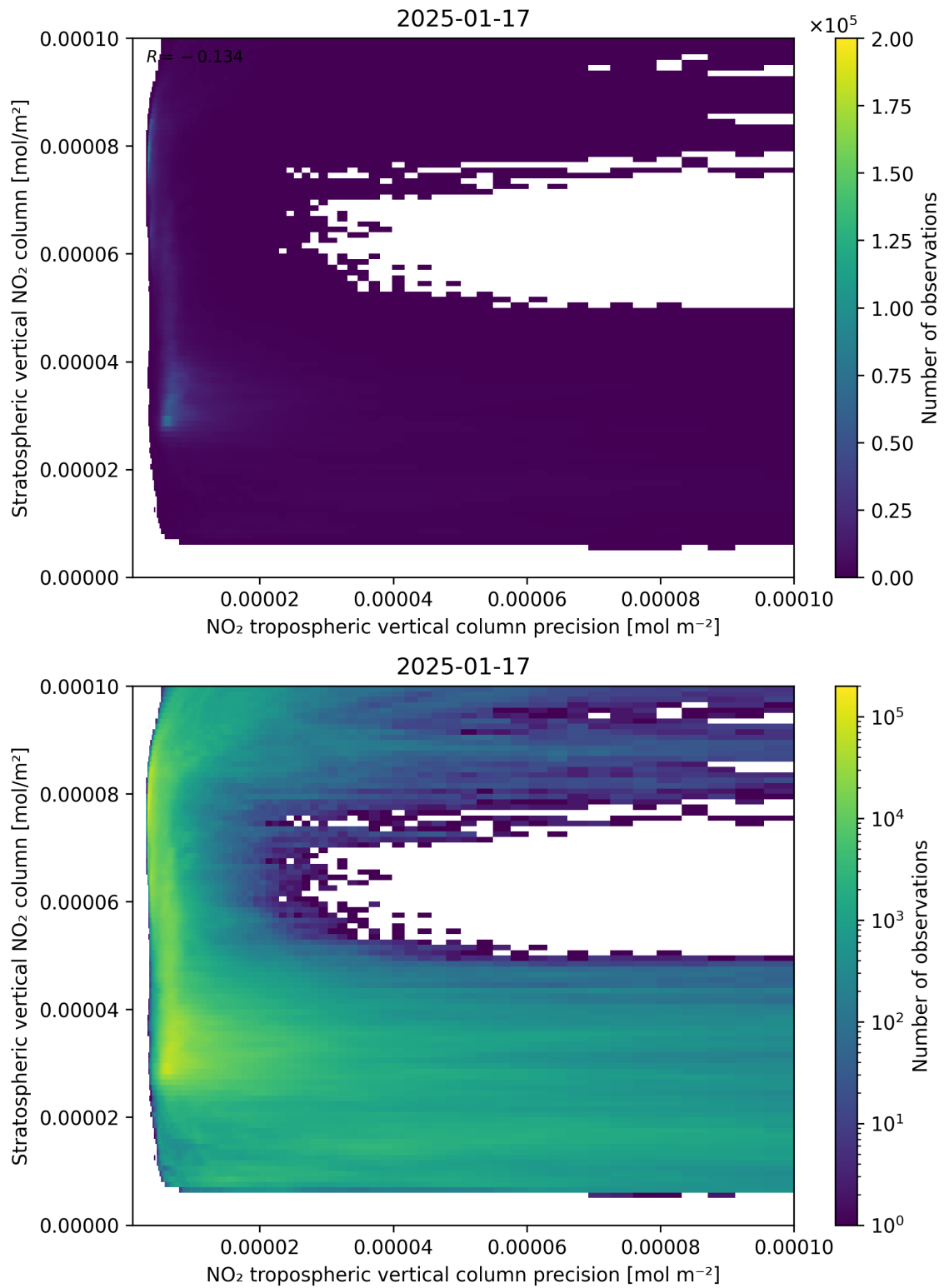
Figure 135: Scatter density plot of “NO 2 tropospheric vertical column precision” against “Stratospheric vertical NO 2 column” for 2025-01-17 to 2025-01-18.
