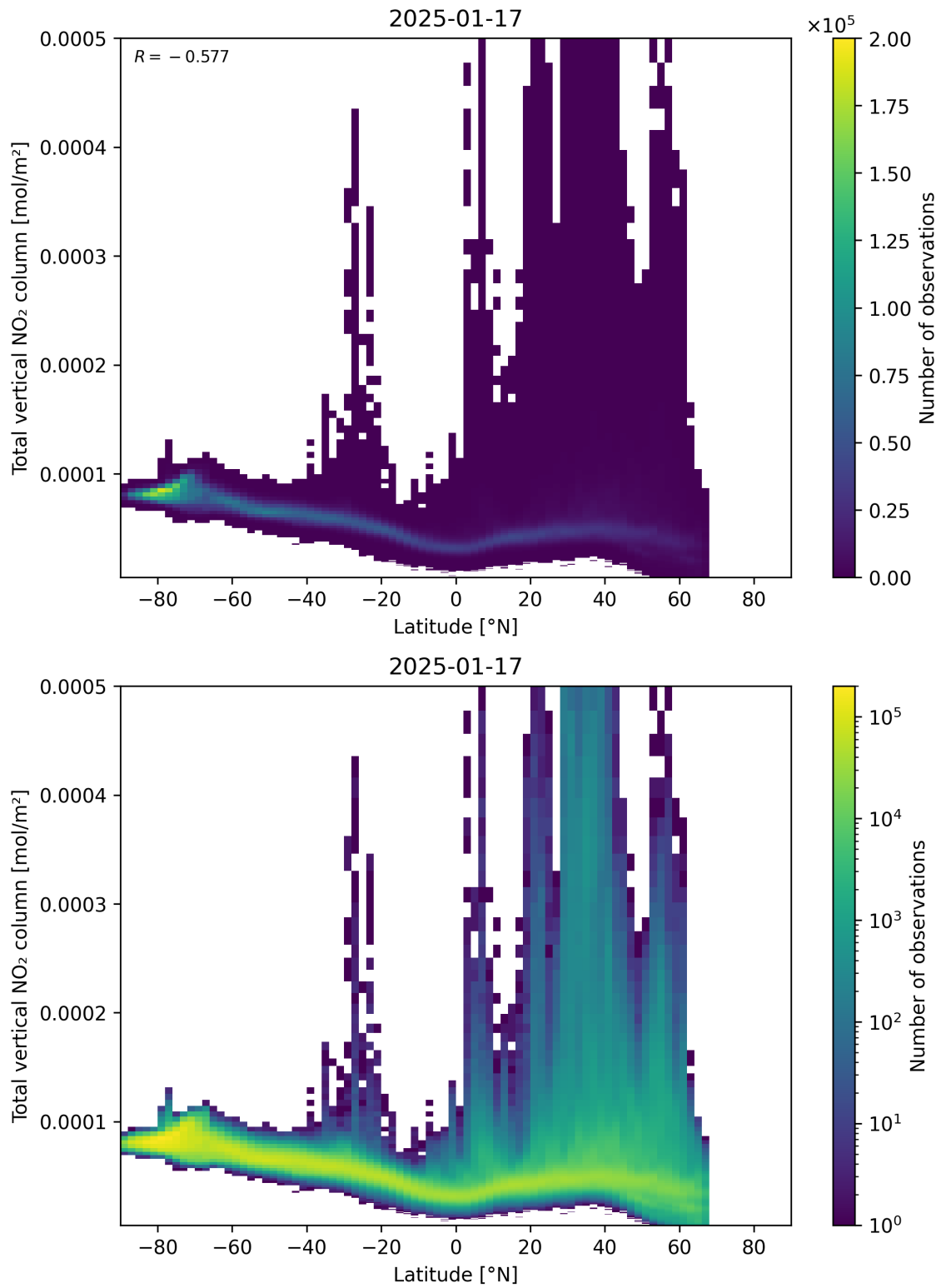
Figure 90: Scatter density plot of “Latitude” against “Total vertical NO 2 column” for 2025-01-17 to 2025-01-18.
