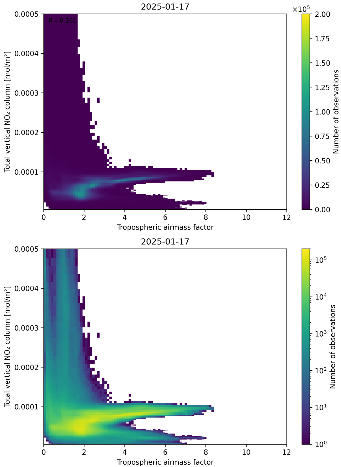
Figure 77: Scatter density plot of “Tropospheric airmass factor” against “Total vertical \text{NO}_2 column” for 2025-01-17 to 2025-01-18.
