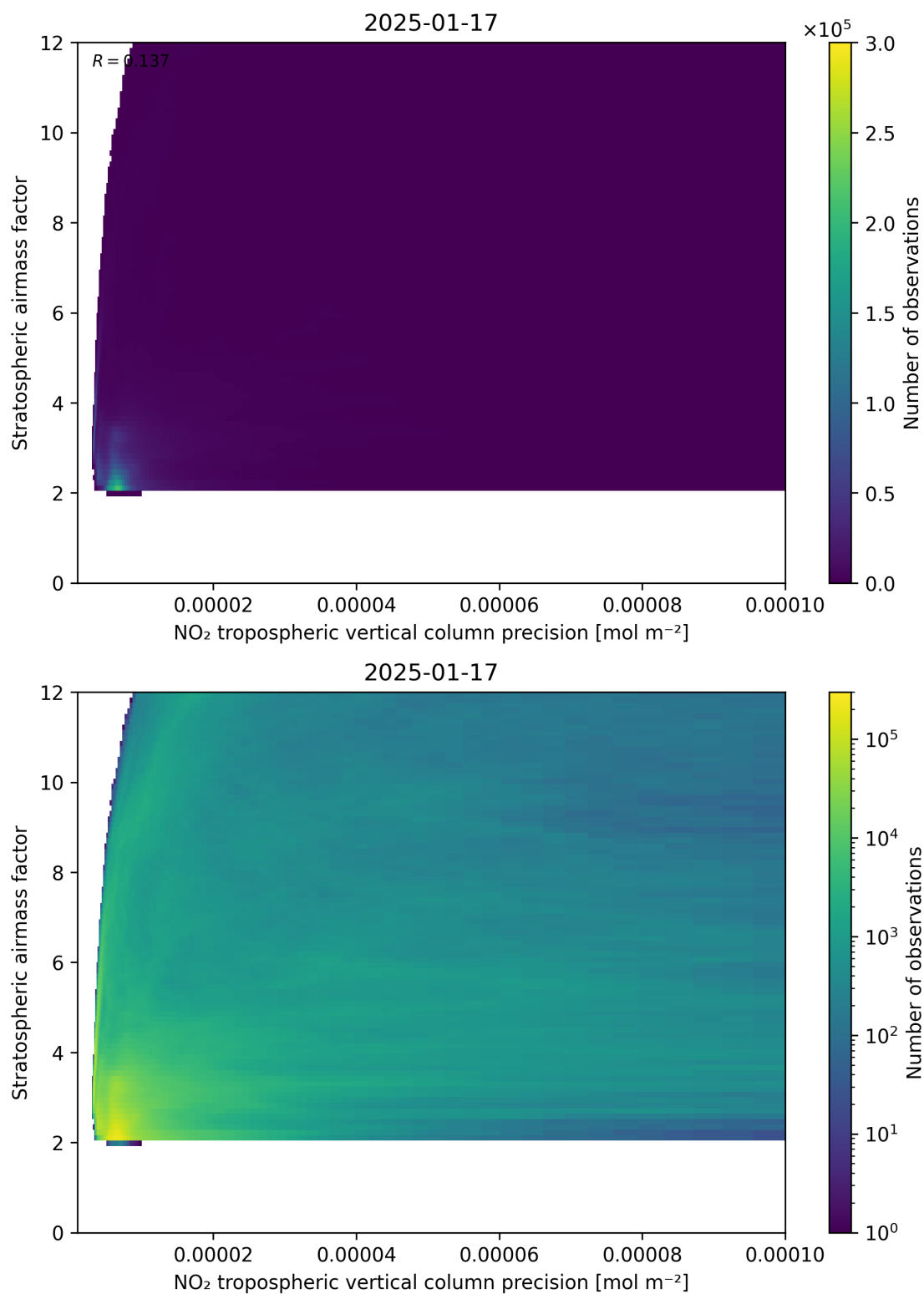
Figure 131: Scatter density plot of “NO 2 tropospheric vertical column precision” against “Stratospheric airmass factor” for 2025-01-17 to 2025-01-18.
