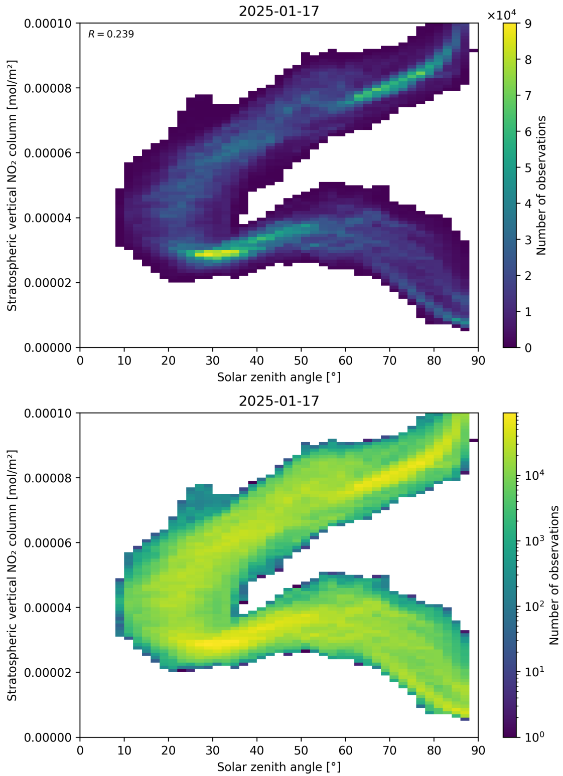
Figure 150: Scatter density plot of “Solar zenith angle” against “Stratospheric vertical NO 2 column” for 2025-01-17 to 2025-01-18.
