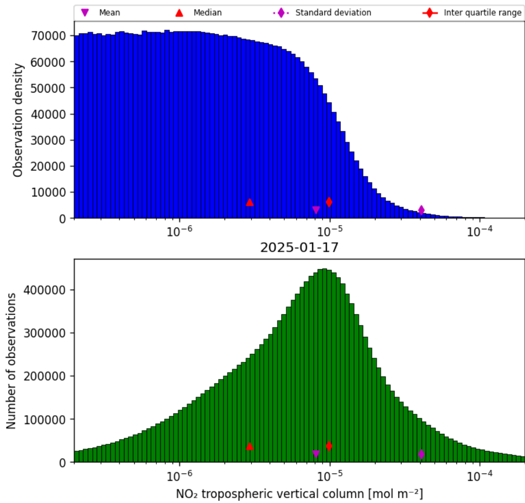
Figure 29: Histogram of “NO 2 tropospheric vertical column” for 2025-01-17 to 2025-01-18
