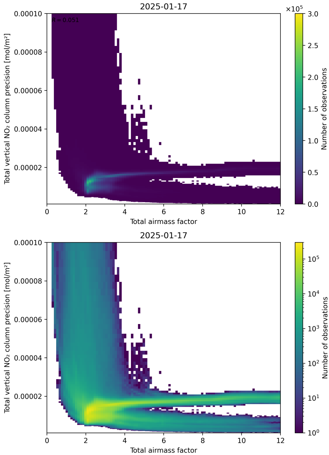
Figure 68: Scatter density plot of “Total airmass factor” against “Total vertical NO 2 column precision” for 2025-01-17 to 2025-01-18.
