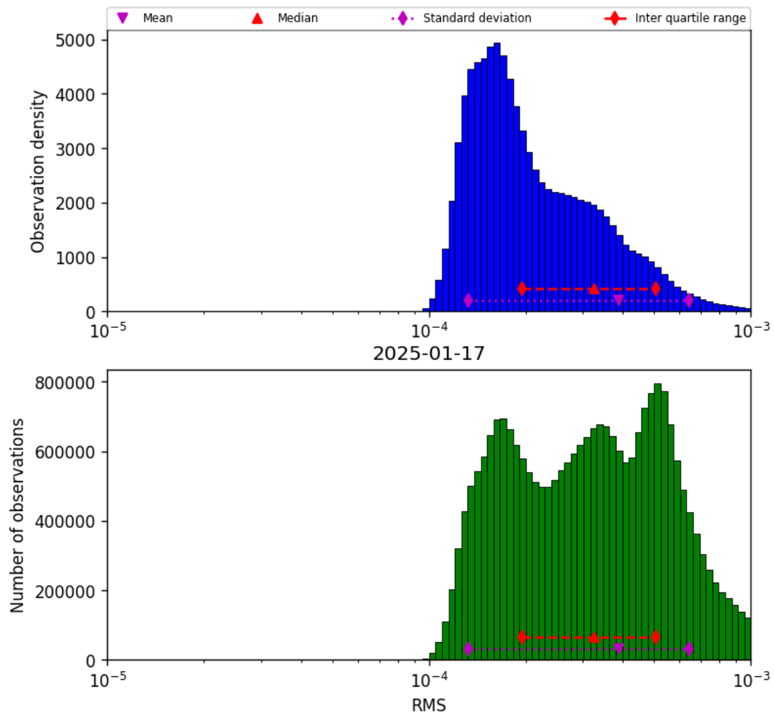
Figure 43: Histogram of “RMS” for 2025-01-17 to 2025-01-18
