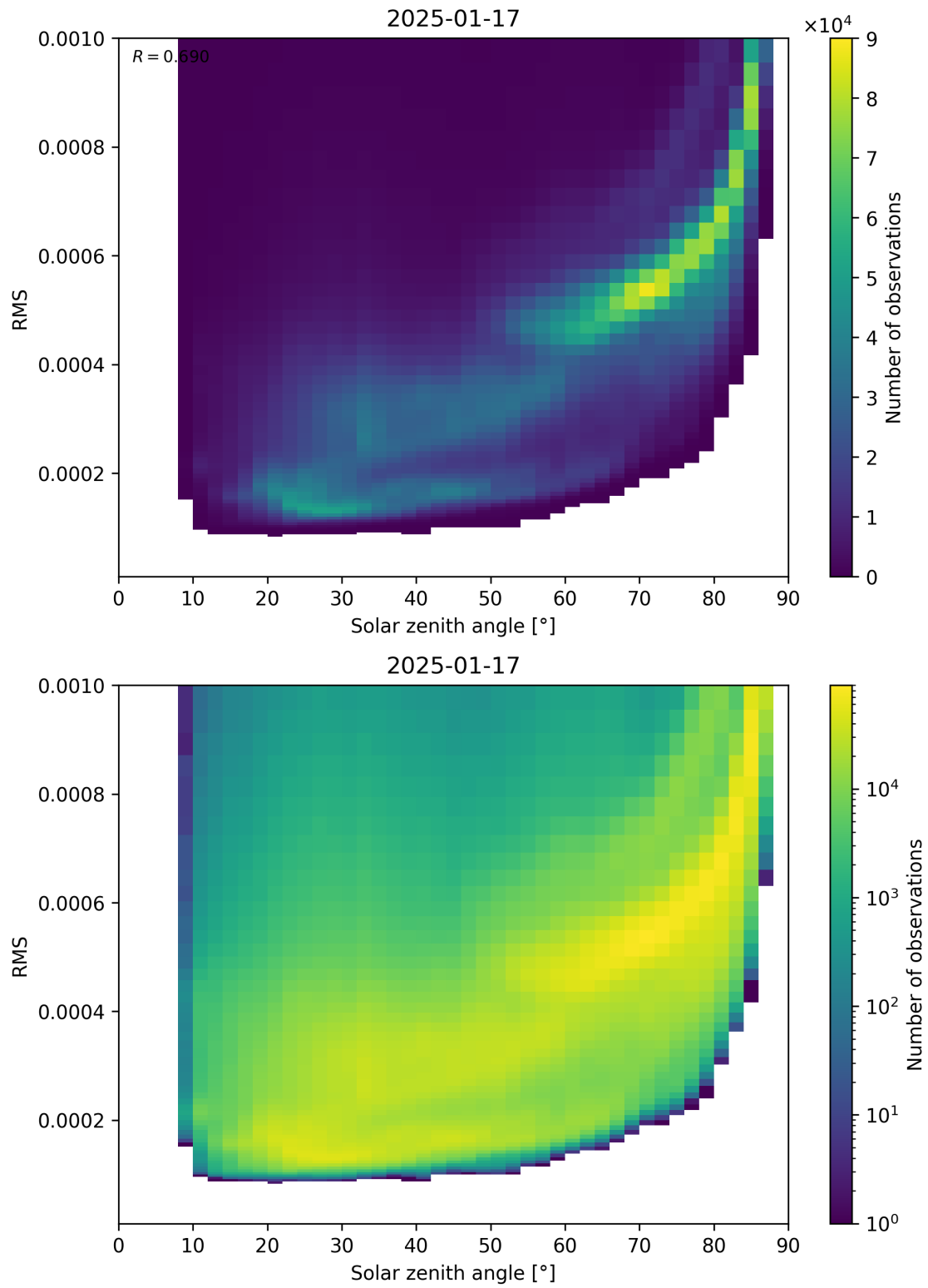
Figure 157: Scatter density plot of “Solar zenith angle” against “RMS” for 2025-01-17 to 2025-01-18.
