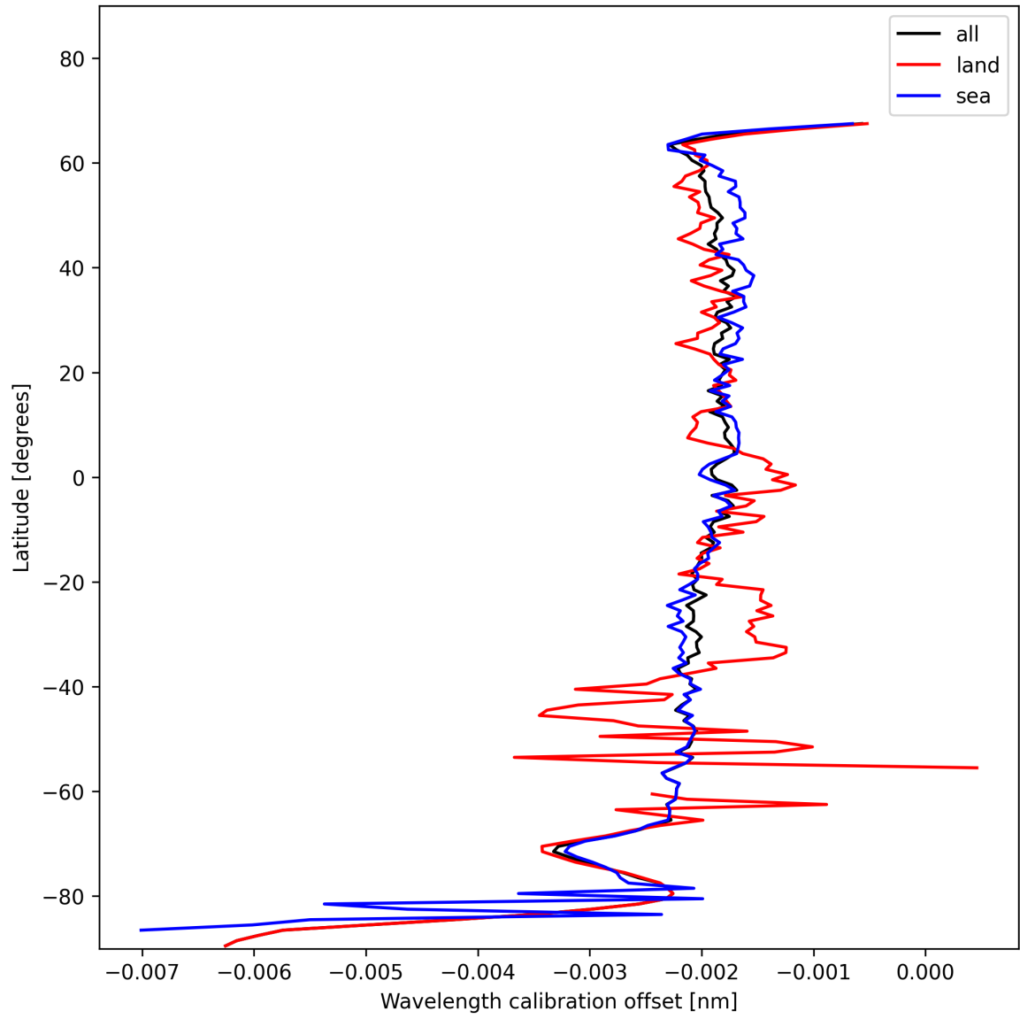
Figure 18: Zonal average of “Wavelength calibration offset” for 2025-01-17 to 2025-01-18.
