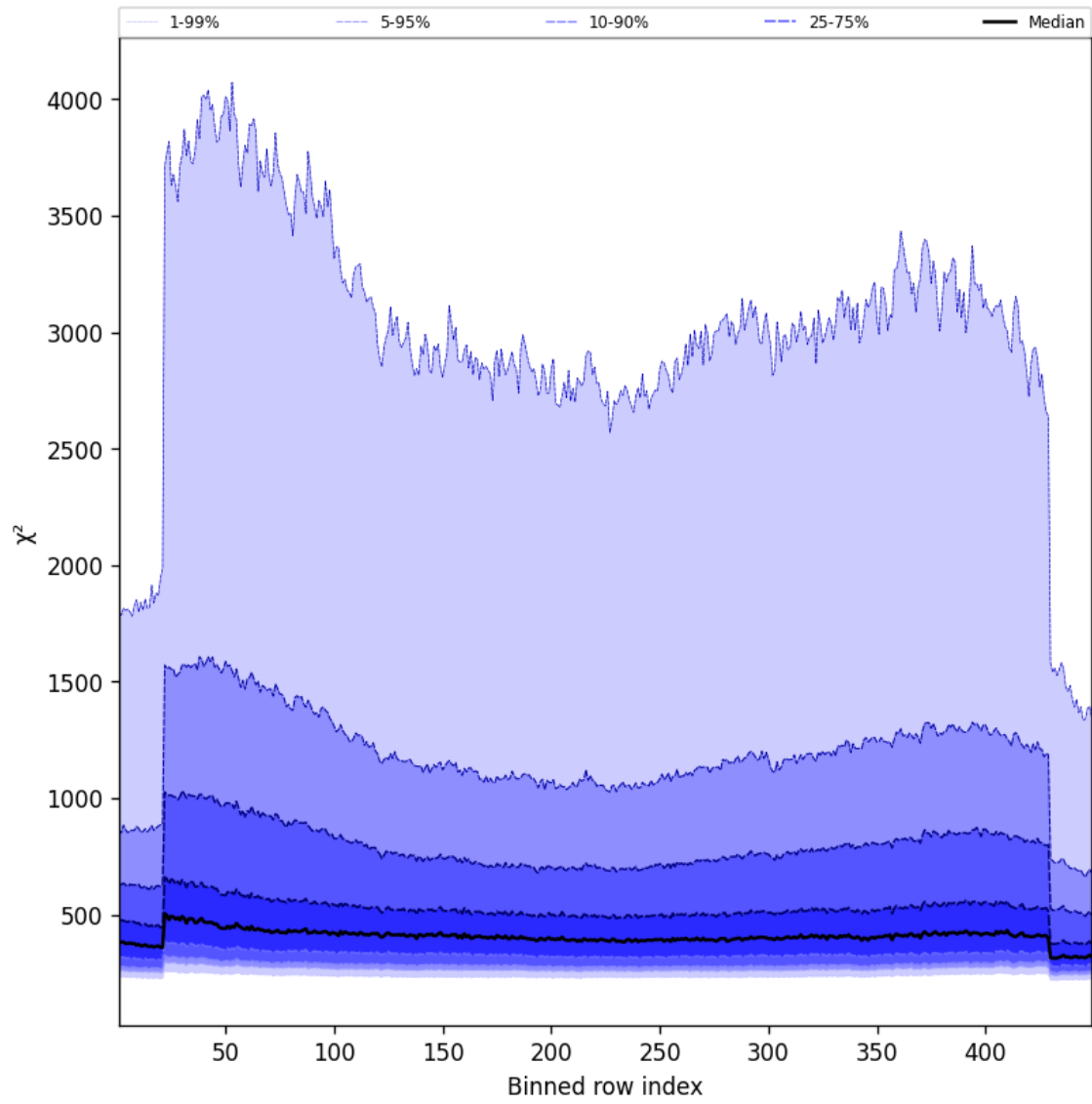
Figure 59: Along track statistics of “ \chi^2 ” for 2025-01-17 to 2025-01-18
