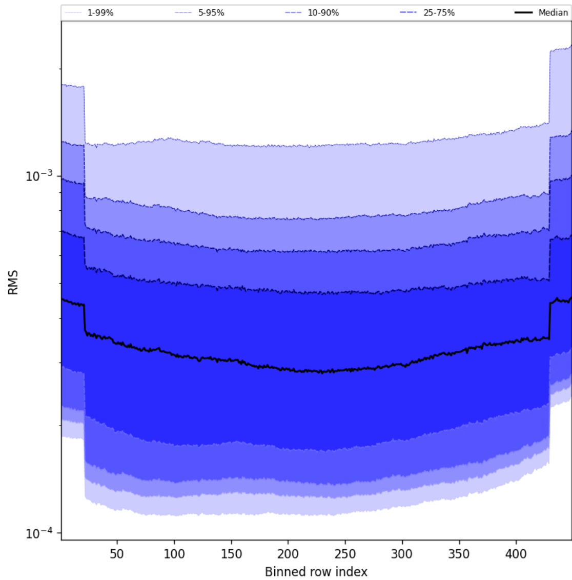
Figure 60: Along track statistics of “RMS” for 2025-01-17 to 2025-01-18
