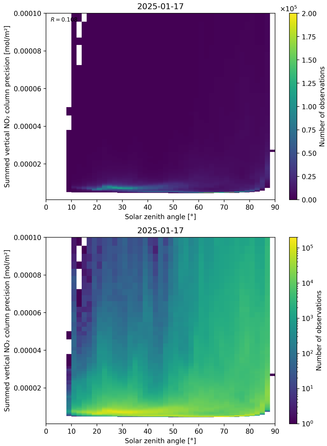
Figure 152: Scatter density plot of “Solar zenith angle” against “Summed vertical NO 2 column precision” for 2025-01-17 to 2025-01-18.
