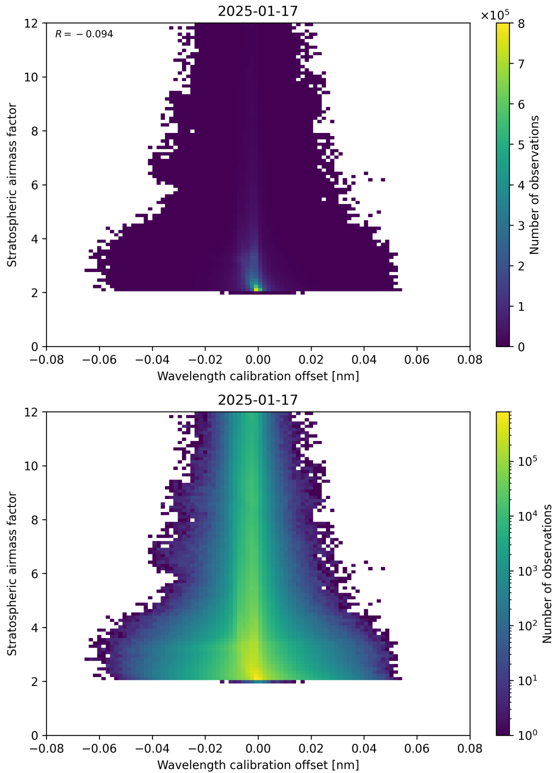
Figure 174: Scatter density plot of “Wavelength calibration offset” against “Stratospheric airmass factor” for 2025-01-17 to 2025-01-18.
