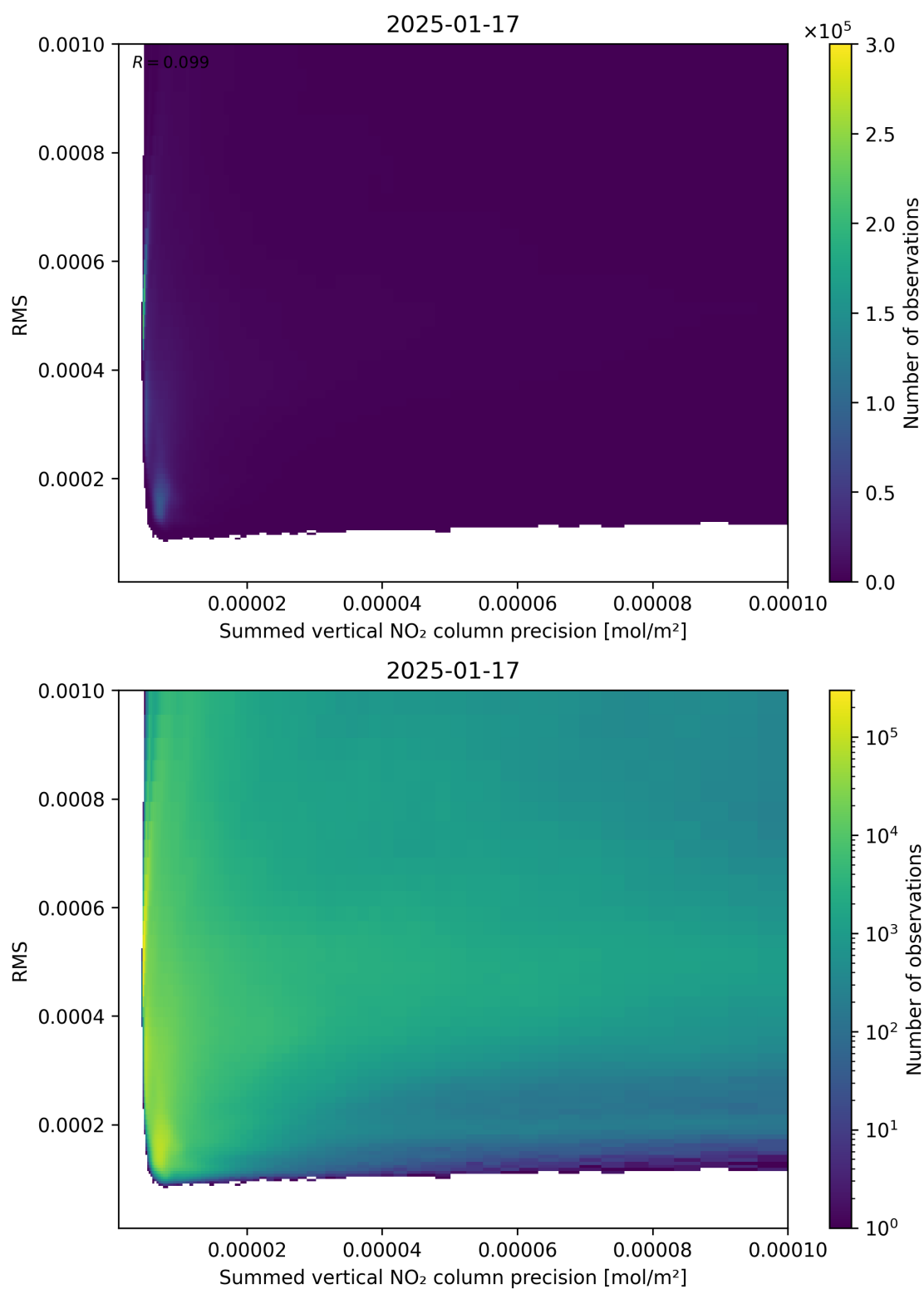
Figure 108: Scatter density plot of “Summed vertical NO 2 column precision” against “RMS” for 2025-01-17 to 2025-01-18.
