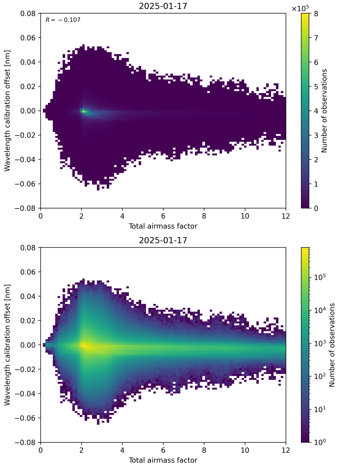
Figure 70: Scatter density plot of “Total airmass factor” against “Wavelength calibration offset” for 2025-01-17 to 2025-01-18.
