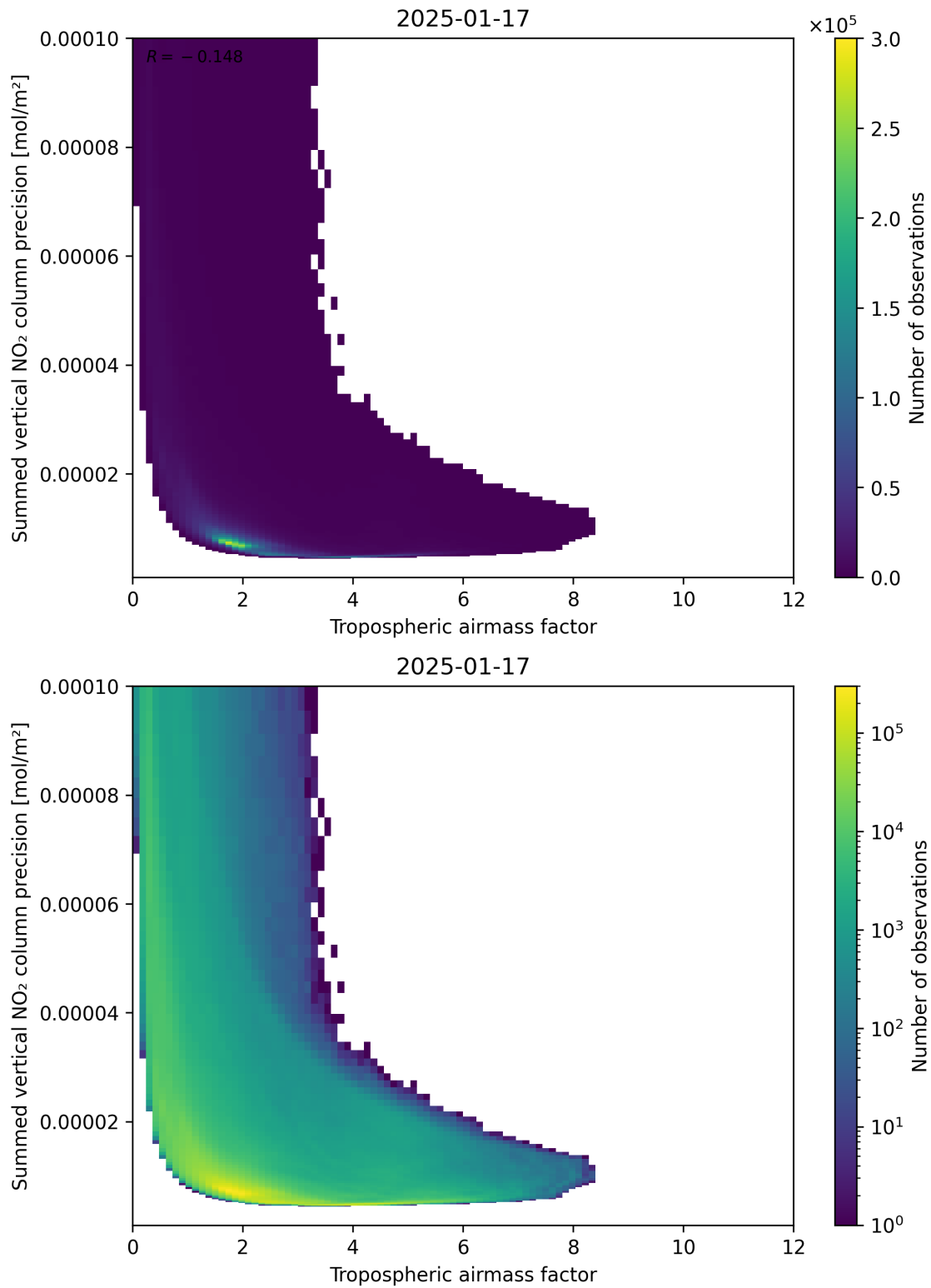
Figure 76: Scatter density plot of “Tropospheric air mass factor” against “Summed vertical NO 2 column precision” for 2025-01-17 to 2025-01-18.
