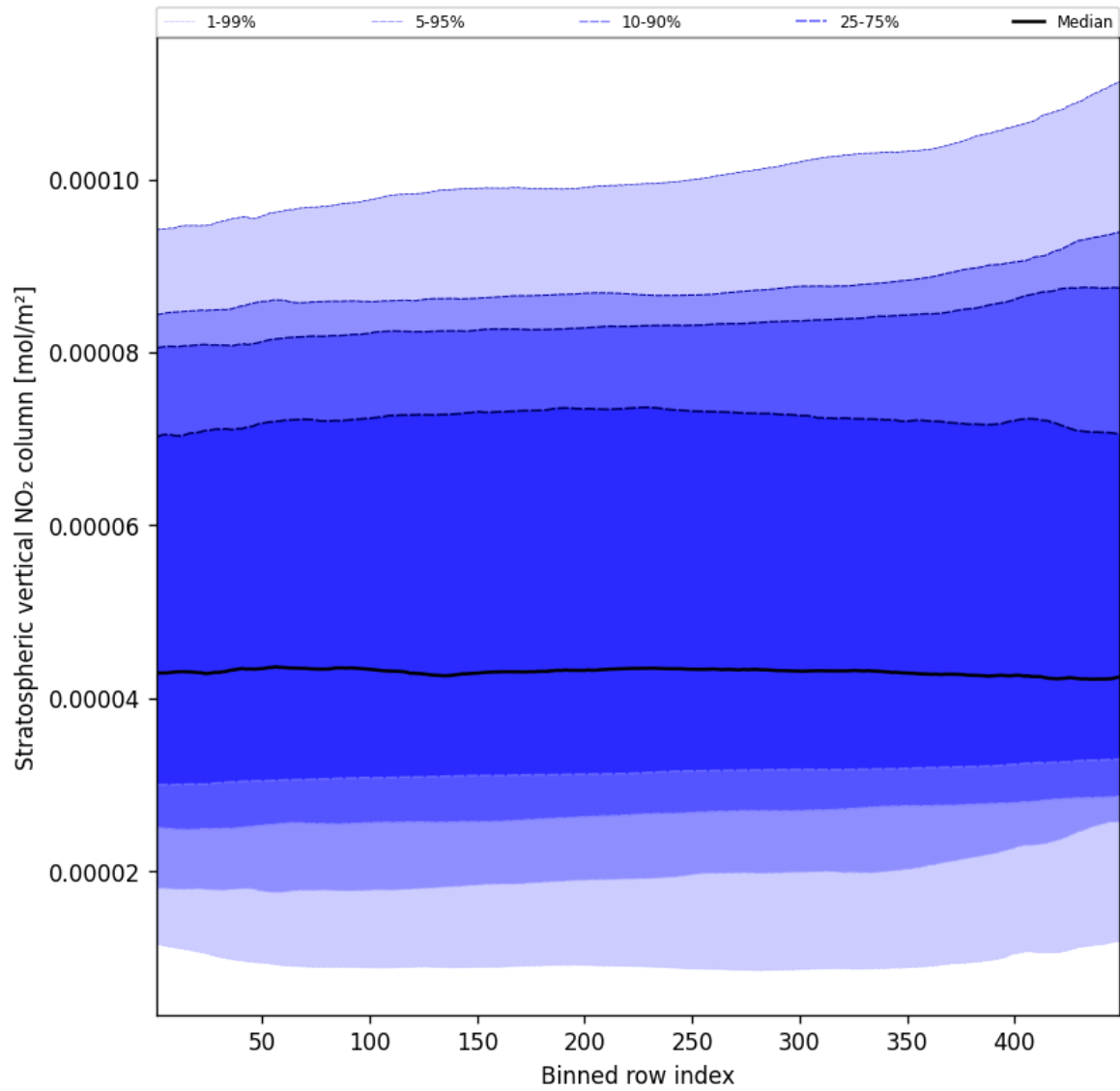
Figure 53: Along track statistics of “Stratospheric vertical NO 2 column” for 2025-01-17 to 2025-01-18
