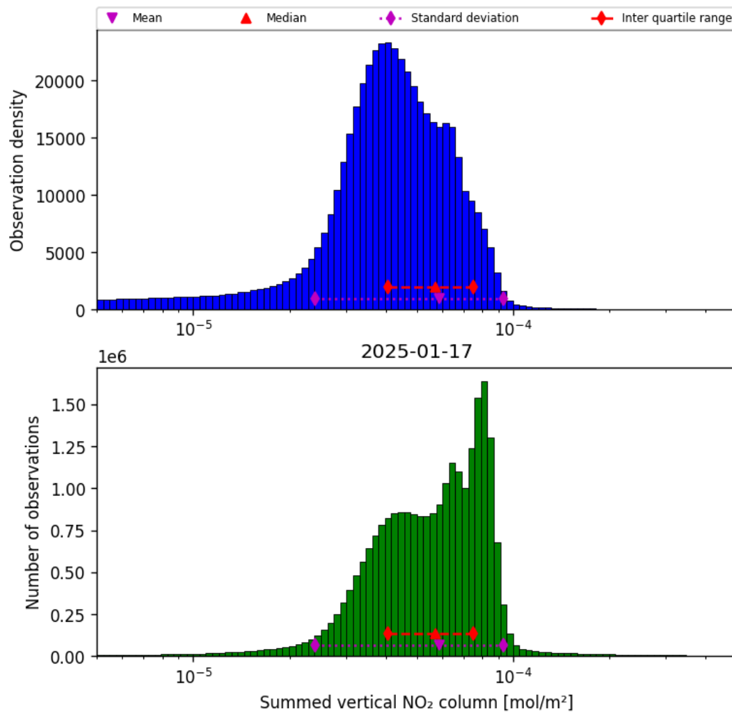
Figure 40: Histogram of “Summed vertical NO 2 column” for 2025-01-17 to 2025-01-18
