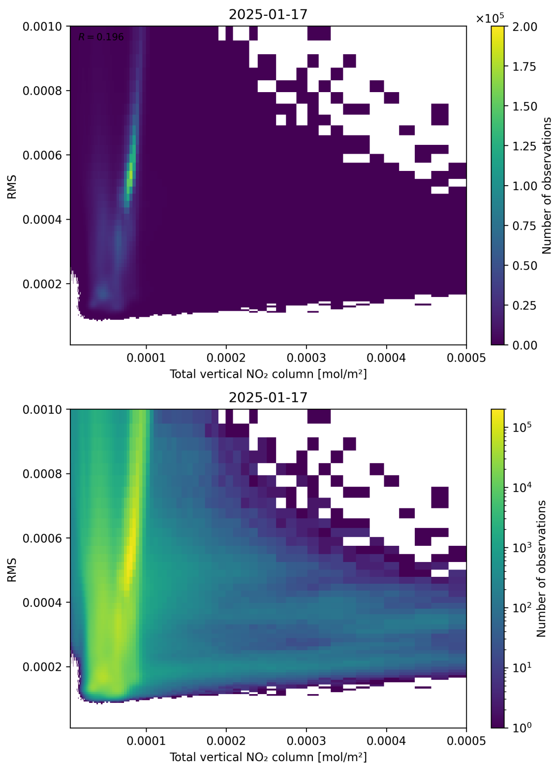
Figure 120: Scatter density plot of “Total vertical NO 2 column” against “RMS” for 2025-01-17 to 2025-01-18.
