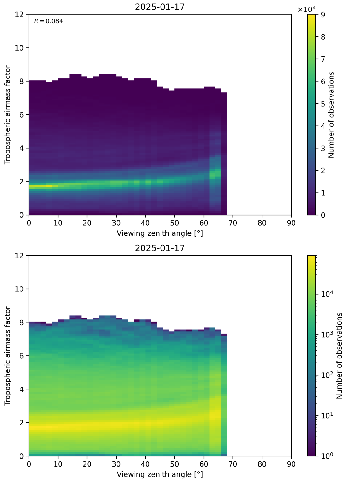
Figure 161: Scatter density plot of “Viewing zenith angle” against “Tropospheric airmass factor” for 2025-01-17 to 2025-01-18.
