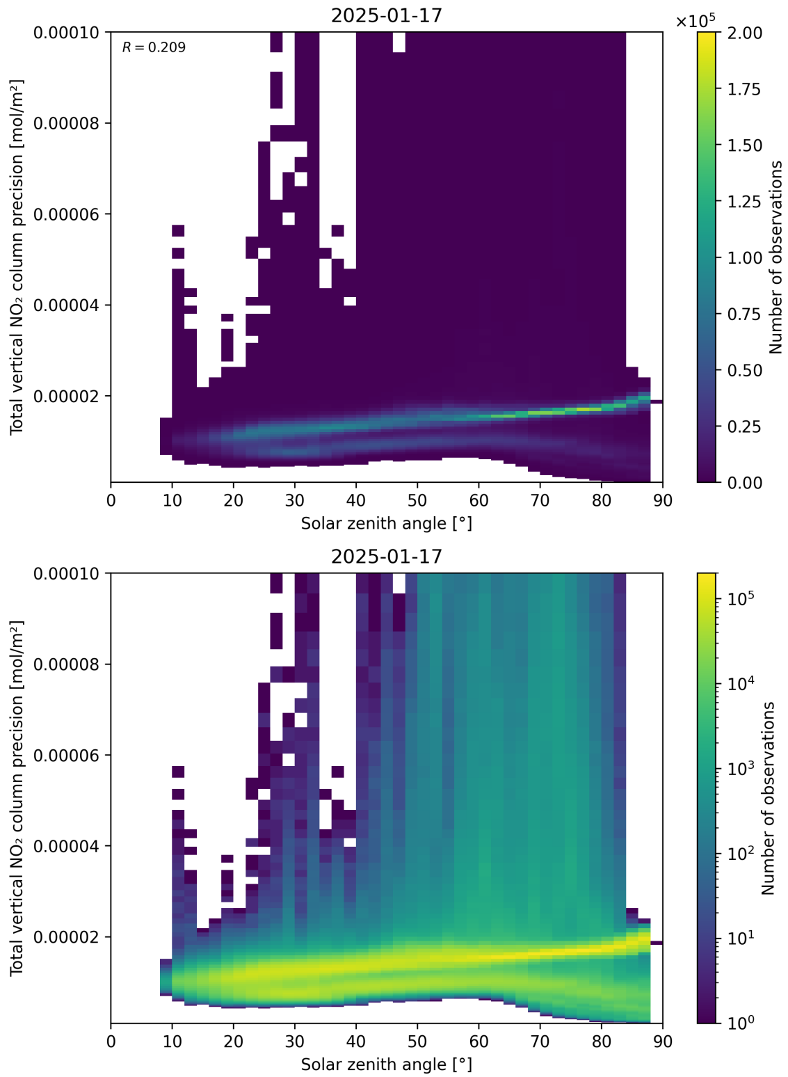
Figure 154: Scatter density plot of “Solar zenith angle” against “Total vertical NO 2 column precision” for 2025-01-17 to 2025-01-18.
