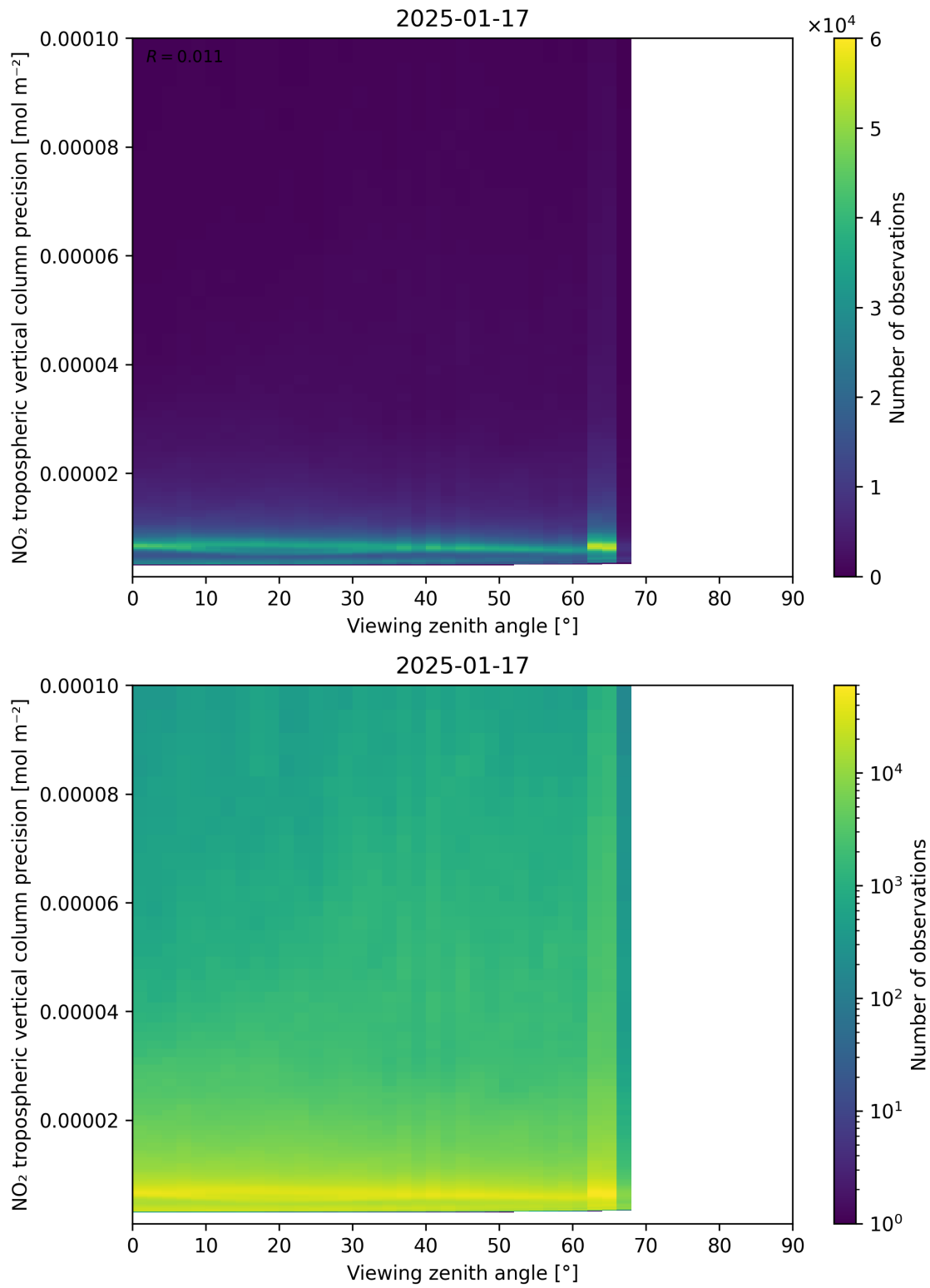
Figure 170: Scatter density plot of “Viewing zenith angle” against “NO 2 tropospheric vertical column precision” for 2025-01-17 to 2025-01-18.
