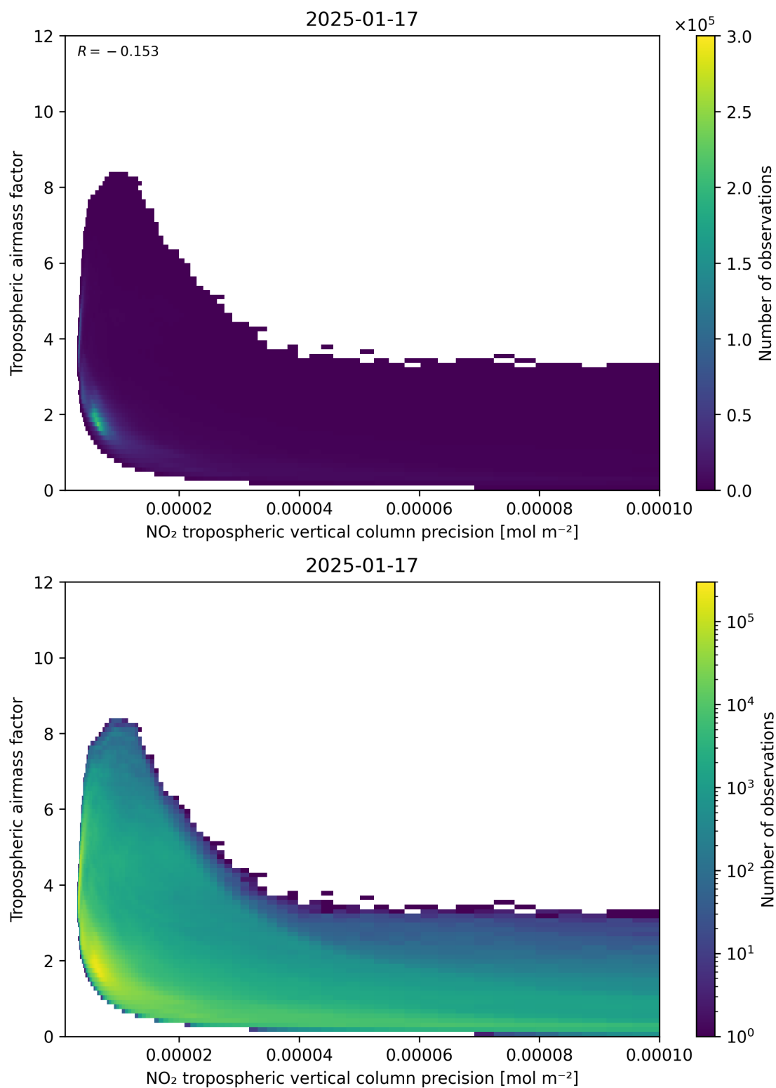
Figure 133: Scatter density plot of “NO 2 tropospheric vertical column precision” against “Tropospheric air mass factor” for 2025-01-17 to 2025-01-18.
