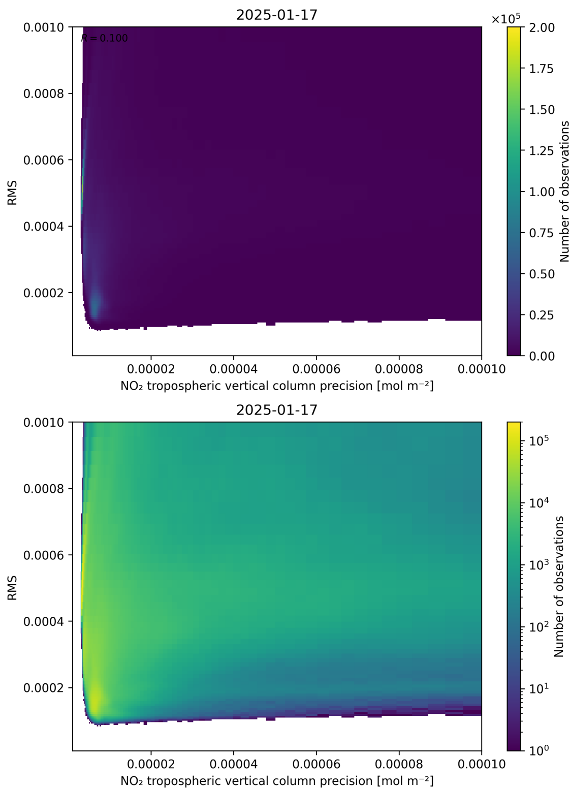
Figure 140: Scatter density plot of “NO 2 tropospheric vertical column precision” against “RMS” for 2025-01-17 to 2025-01-18.
