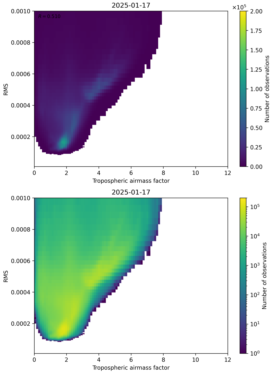
Figure 79: Scatter density plot of “Tropospheric airmass factor” against “RMS” for 2025-01-17 to 2025-01-18.
