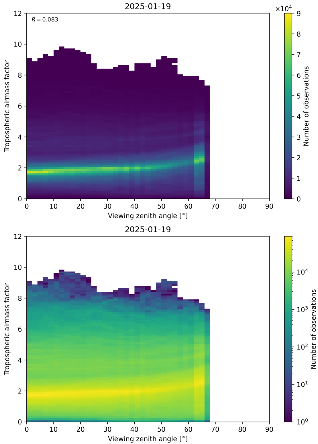
Figure 161: Scatter density plot of “Viewing zenith angle” against “Tropospheric airmass factor” for 2025-01-18 to 2025-01-20.
