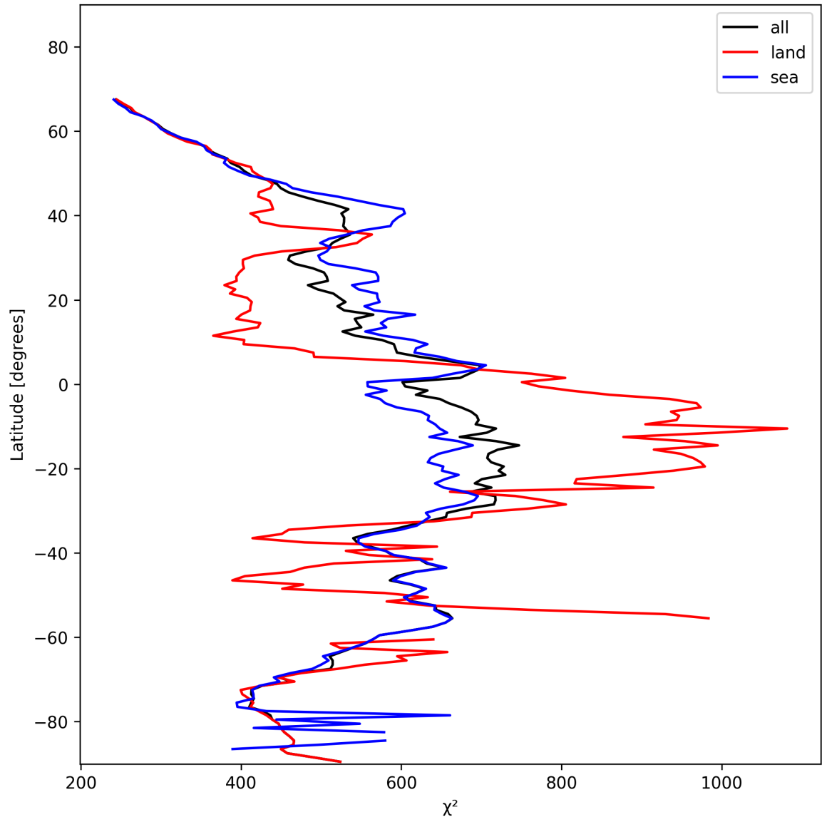
Figure 25: Zonal average of “ \chi^2 ” for 2025-01-18 to 2025-01-20.
