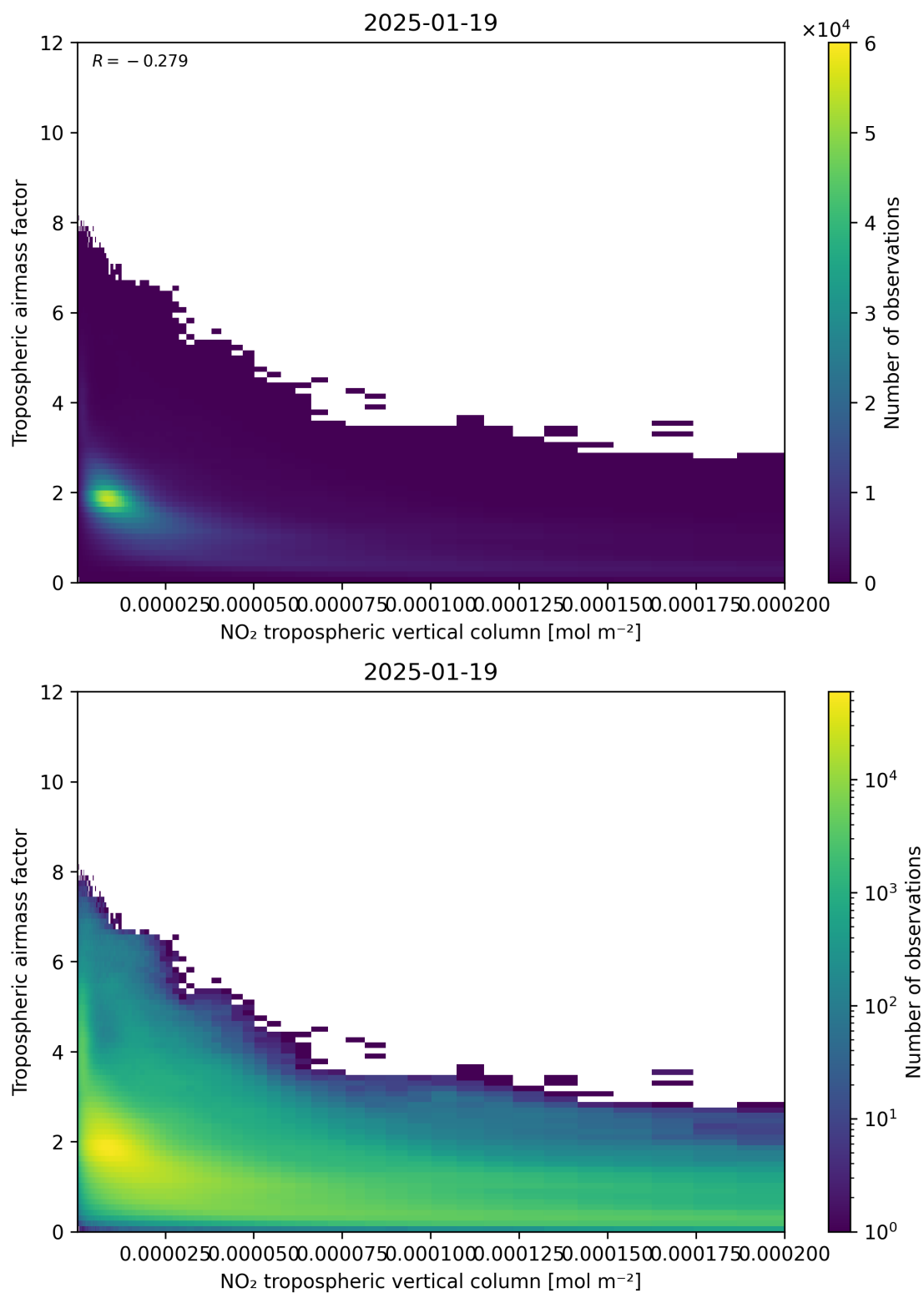
Figure 123: Scatter density plot of “NO 2 tropospheric vertical column” against “Tropospheric air mass factor” for 2025-01-18 to 2025-01-20.
