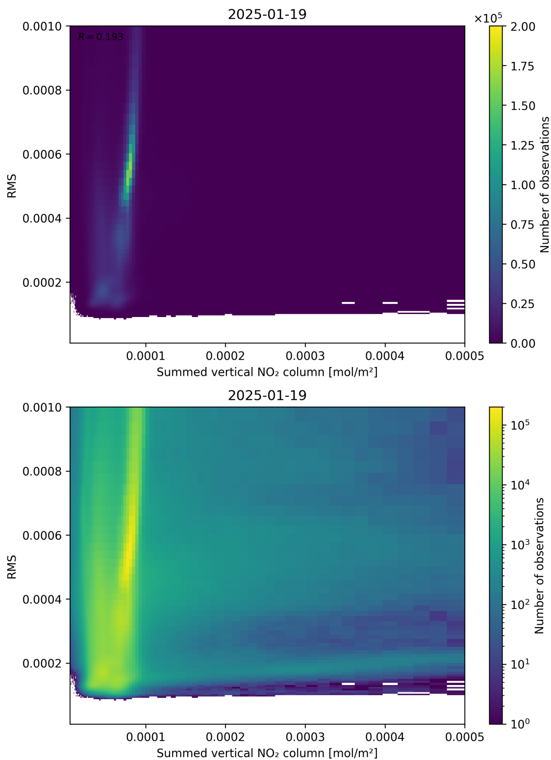
Figure 109: Scatter density plot of “Summed vertical NO 2 column” against “RMS” for 2025-01-18 to 2025-01-20.
