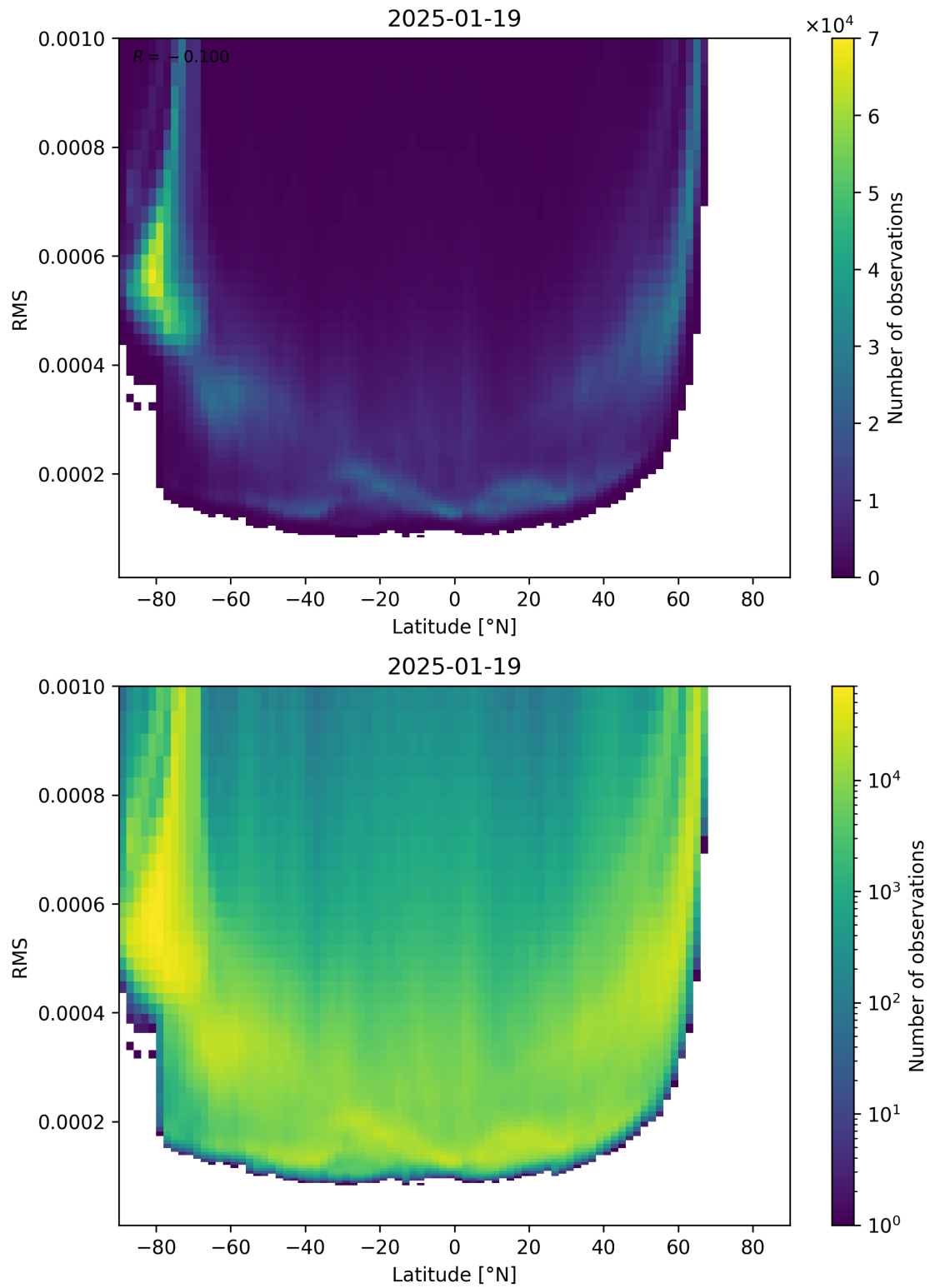
Figure 94: Scatter density plot of “Latitude” against “RMS” for 2025-01-18 to 2025-01-20.
