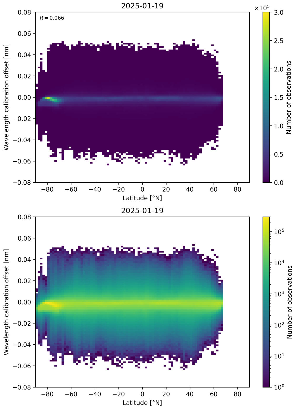
Figure 95: Scatter density plot of “Latitude” against “Wavelength calibration offset” for 2025-01-18 to 2025-01-20.
