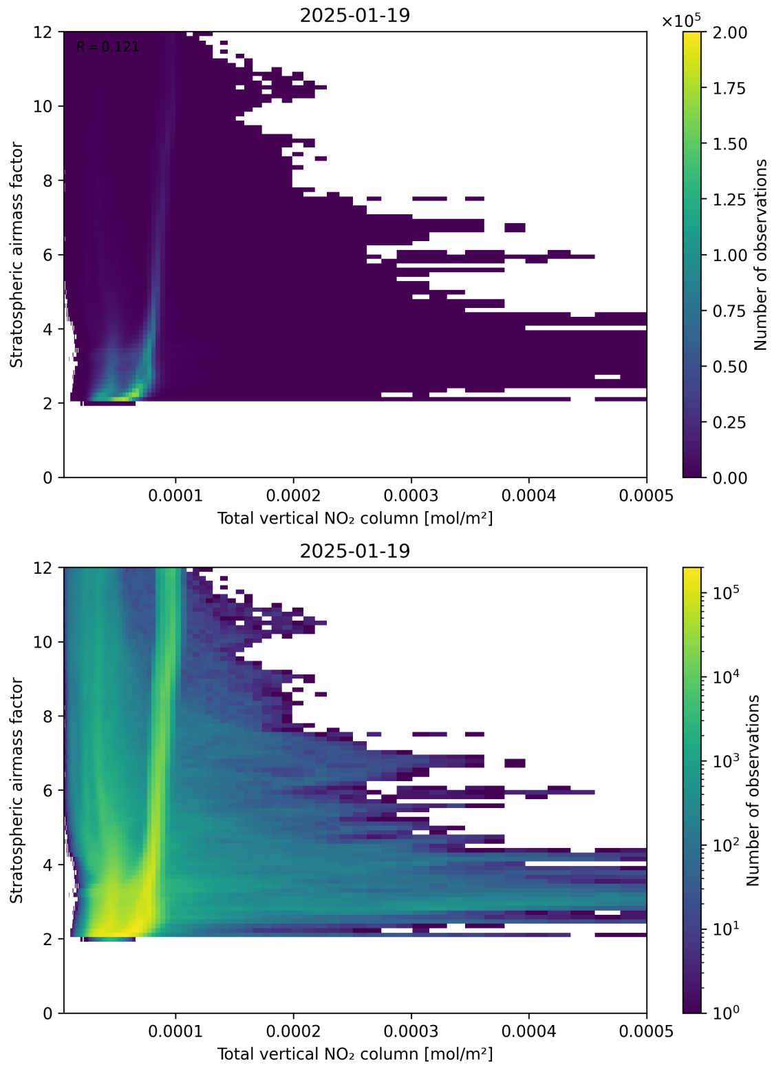
Figure 110: Scatter density plot of “Total vertical NO 2 column” against “Stratospheric airmass factor” for 2025-01-18 to 2025-01-20.
