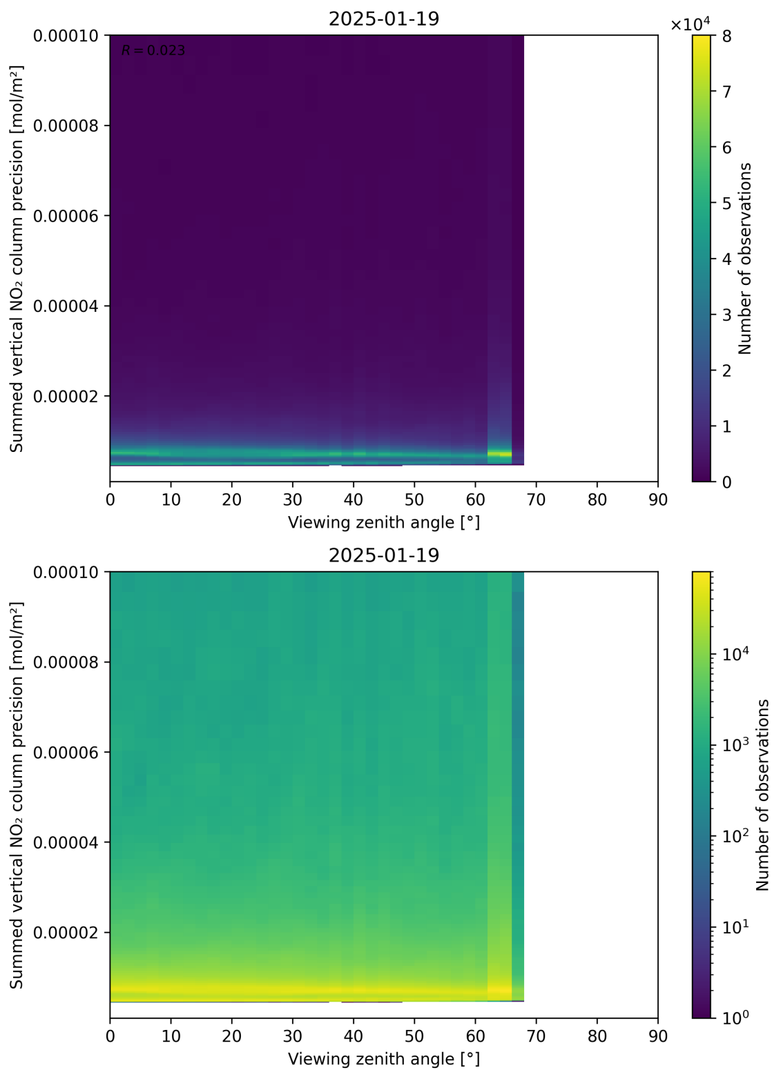
Figure 166: Scatter density plot of “Viewing zenith angle” against “Summed vertical NO 2 column precision” for 2025-01-18 to 2025-01-20.
