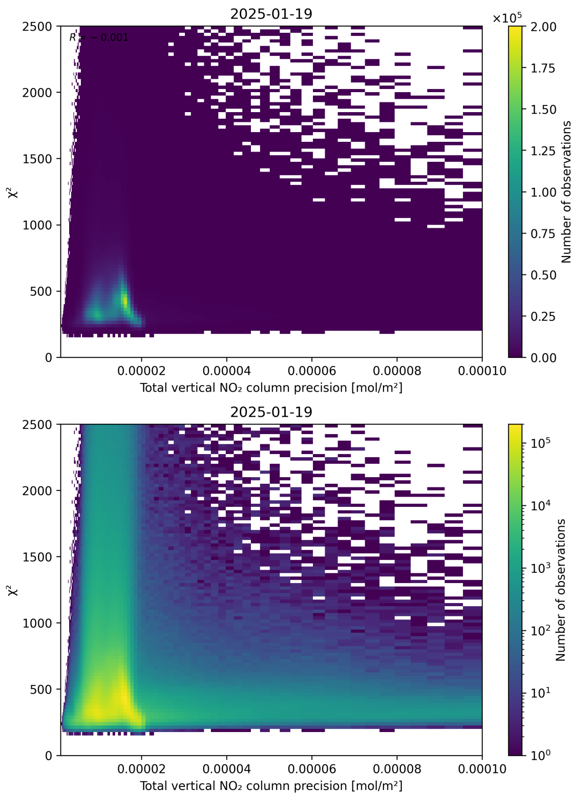
Figure 116: Scatter density plot of “Total vertical NO 2 column precision” against “ \chi^2 ” for 2025-01-18 to 2025-01-20.
