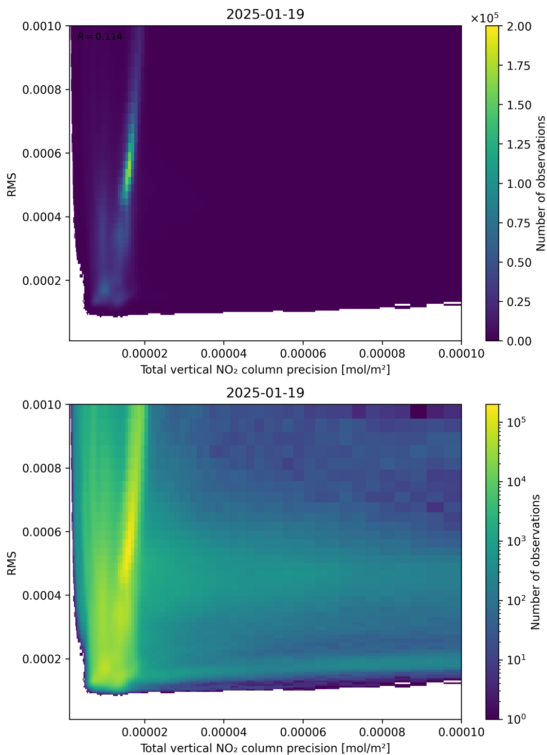
Figure 119: Scatter density plot of “Total vertical NO 2 column precision” against “RMS” for 2025-01-18 to 2025-01-20.
