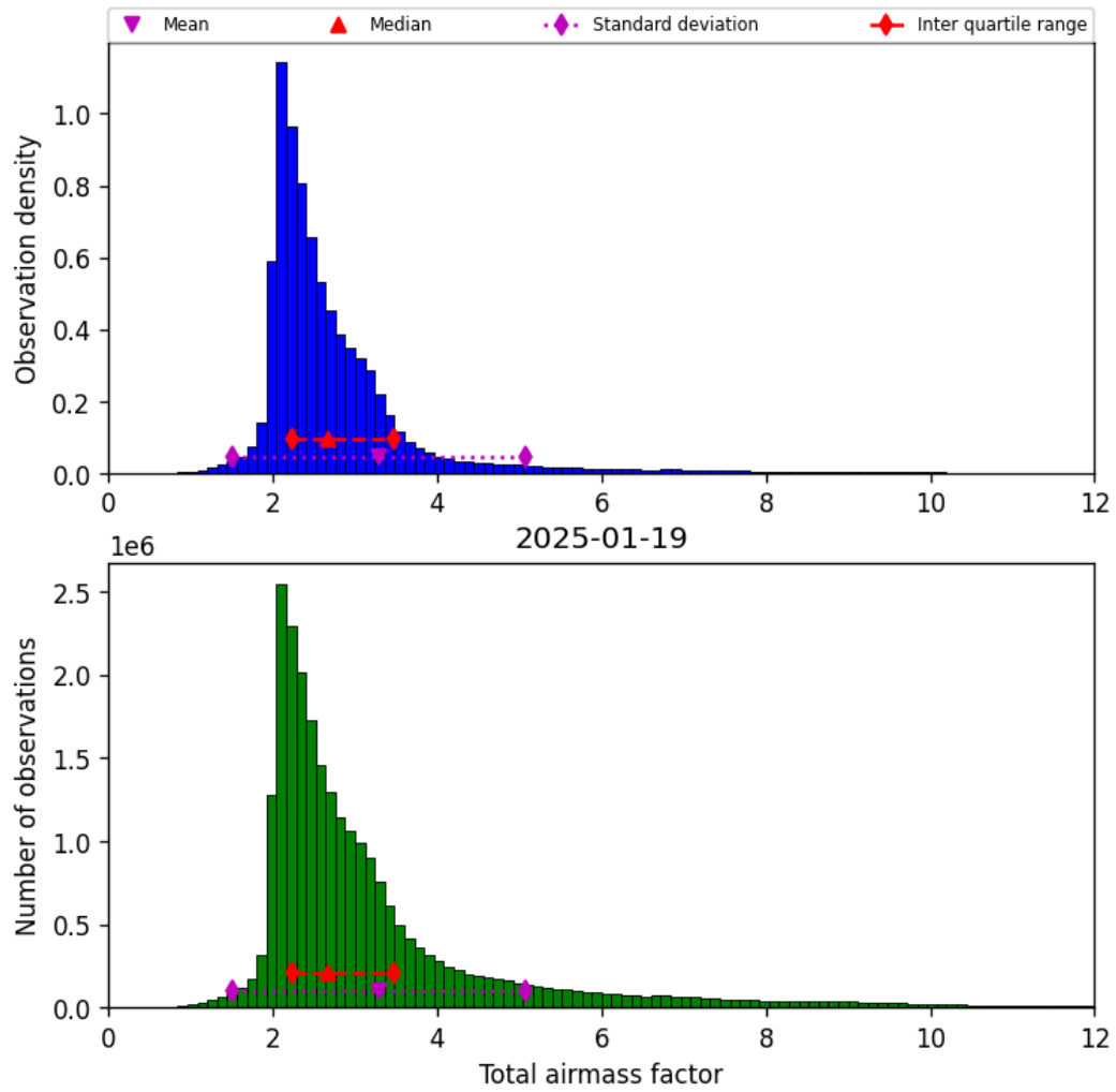
Figure 32: Histogram of “Total airmass factor” for 2025-01-18 to 2025-01-20
