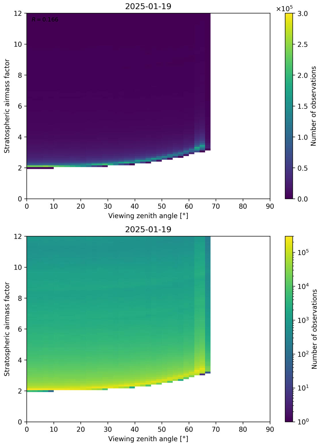
Figure 159: Scatter density plot of “Viewing zenith angle” against “Stratospheric airmass factor” for 2025-01-18 to 2025-01-20.
