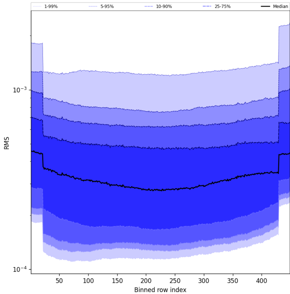
Figure 60: Along track statistics of “RMS” for 2025-01-18 to 2025-01-20
