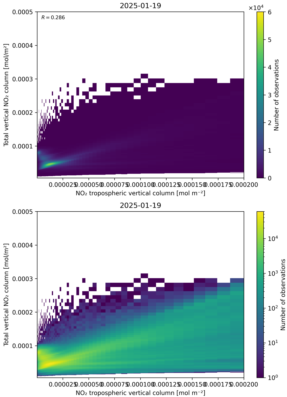
Figure 128: Scatter density plot of “NO 2 tropospheric vertical column” against “Total vertical NO 2 column” for 2025-01-18 to 2025-01-20.
