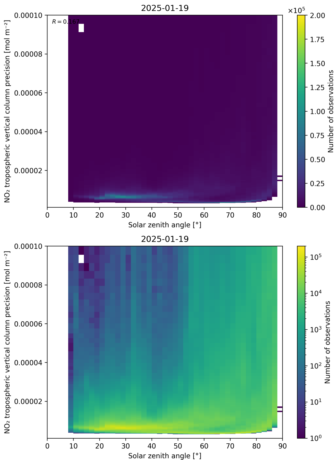
Figure 156: Scatter density plot of “Solar zenith angle” against “NO 2 tropospheric vertical column precision” for 2025-01-18 to 2025-01-20.
