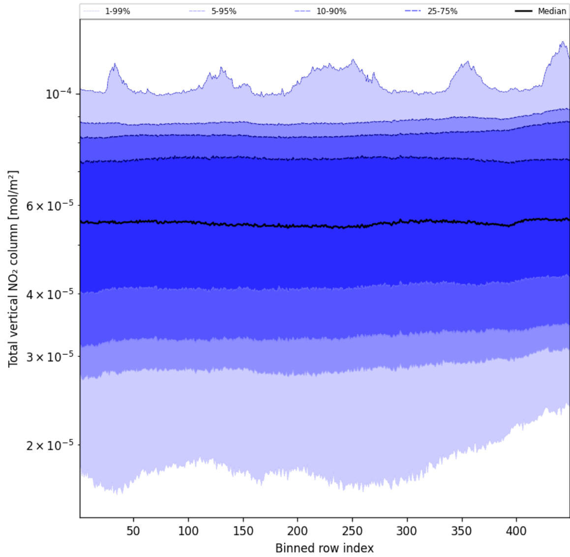
Figure 55: Along track statistics of “Total vertical NO 2 column” for 2025-01-18 to 2025-01-20
