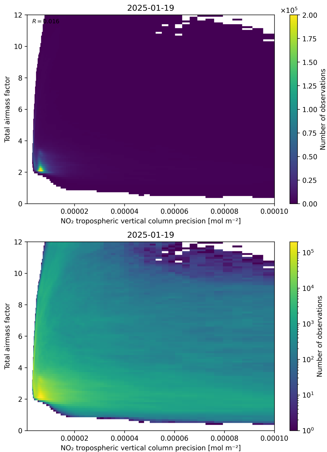
Figure 132: Scatter density plot of “NO 2 tropospheric vertical column precision” against “Total air mass factor” for 2025-01-18 to 2025-01-20.
