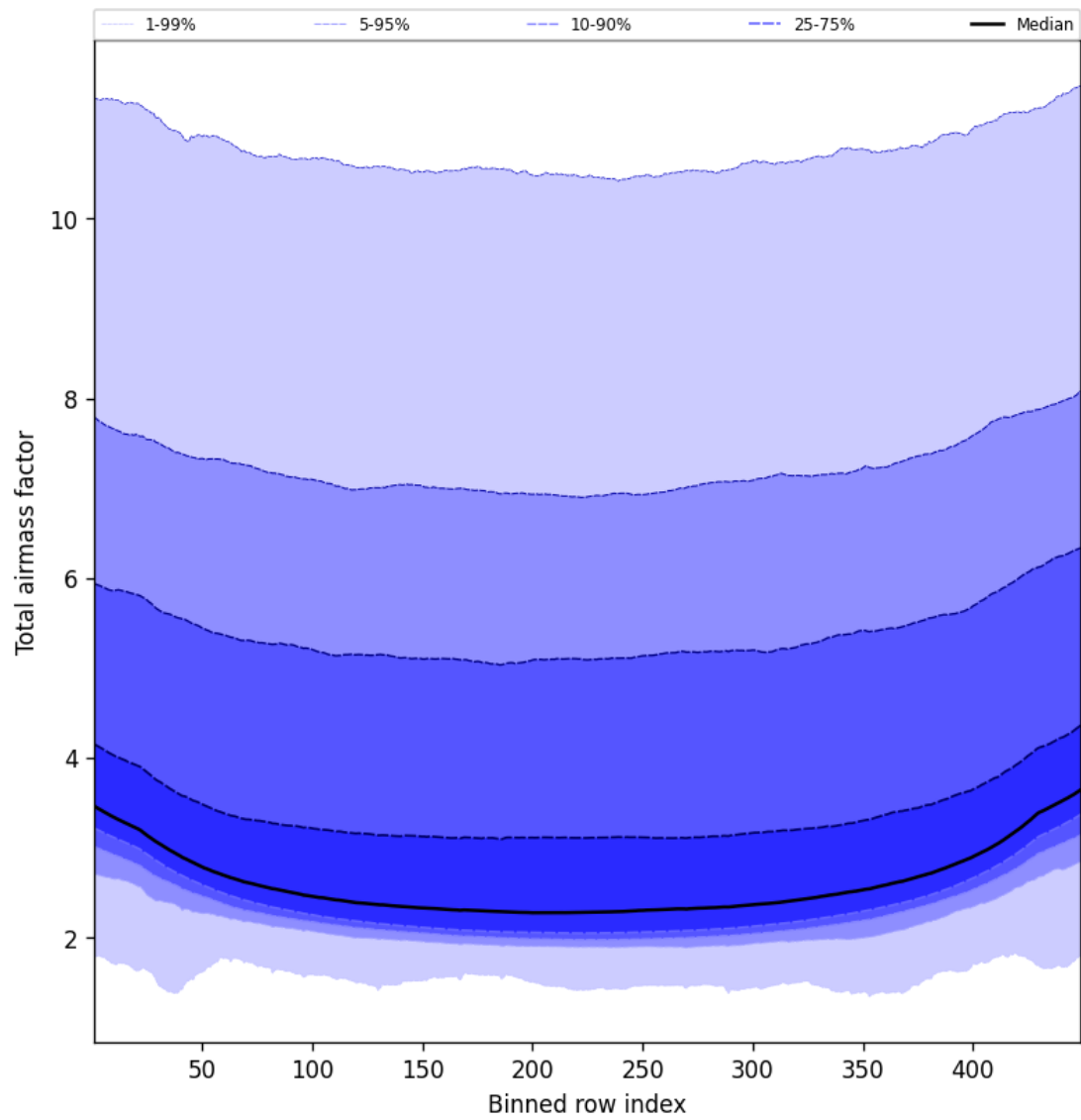
Figure 49: Along track statistics of “Total airmass factor” for 2025-01-18 to 2025-01-20
