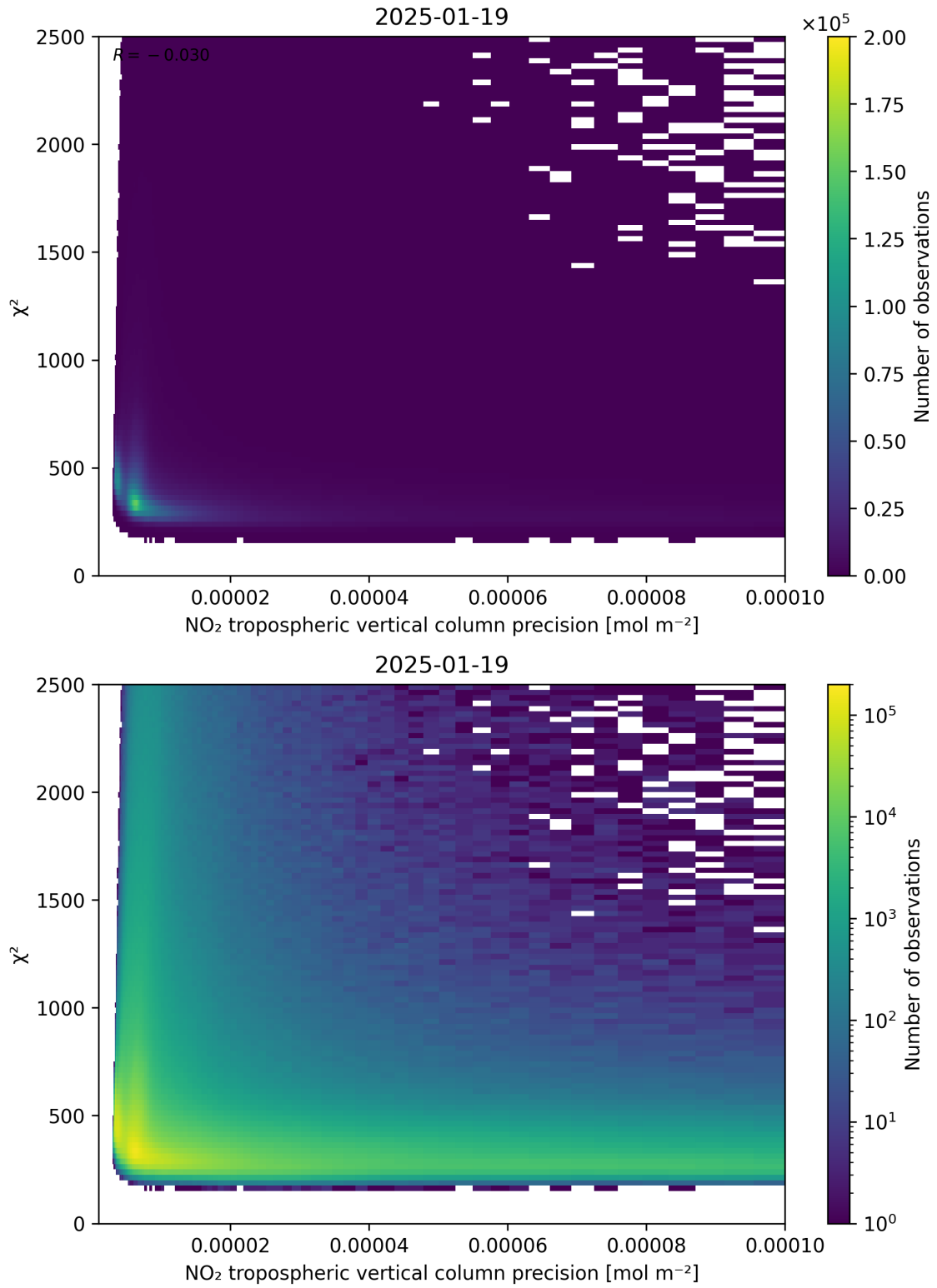
Figure 134: Scatter density plot of “NO 2 tropospheric vertical column precision” against “ \chi^2 ” for 2025-01-18 to 2025-01-20.
