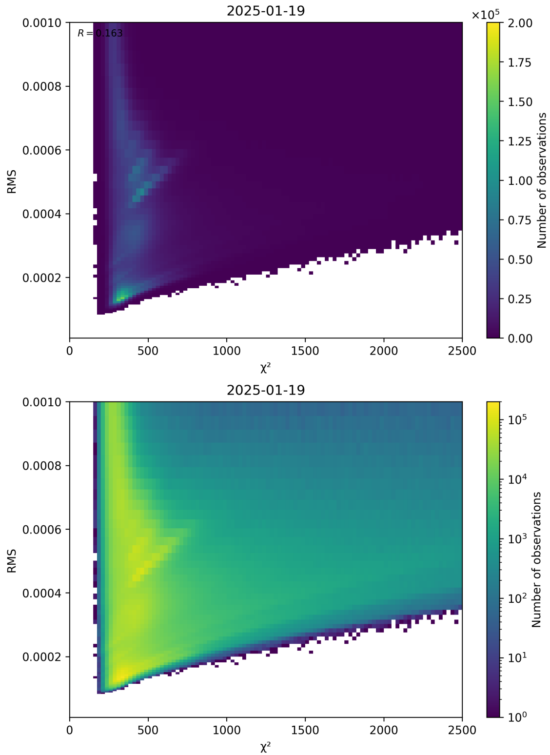
Figure 82: Scatter density plot of “ \chi^2 ” against “RMS” for 2025-01-18 to 2025-01-20.
