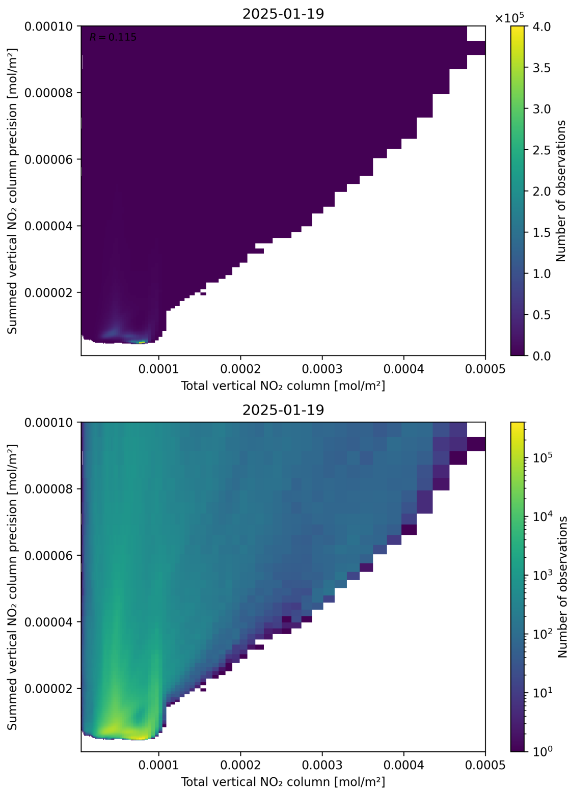
Figure 113: Scatter density plot of “Total vertical NO 2 column” against “Summed vertical NO 2 column precision” for 2025-01-18 to 2025-01-20.
