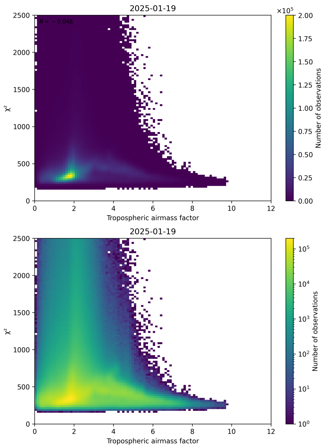
Figure 73: Scatter density plot of “Tropospheric airmass factor” against “ \chi^2 ” for 2025-01-18 to 2025-01-20.
