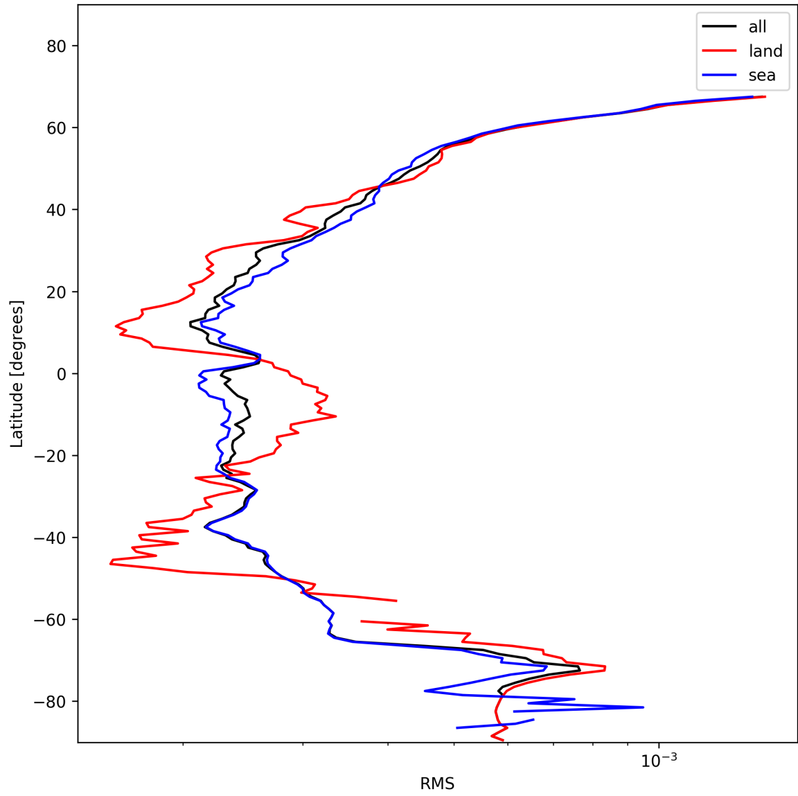
Figure 26: Zonal average of “RMS” for 2025-01-18 to 2025-01-20.
