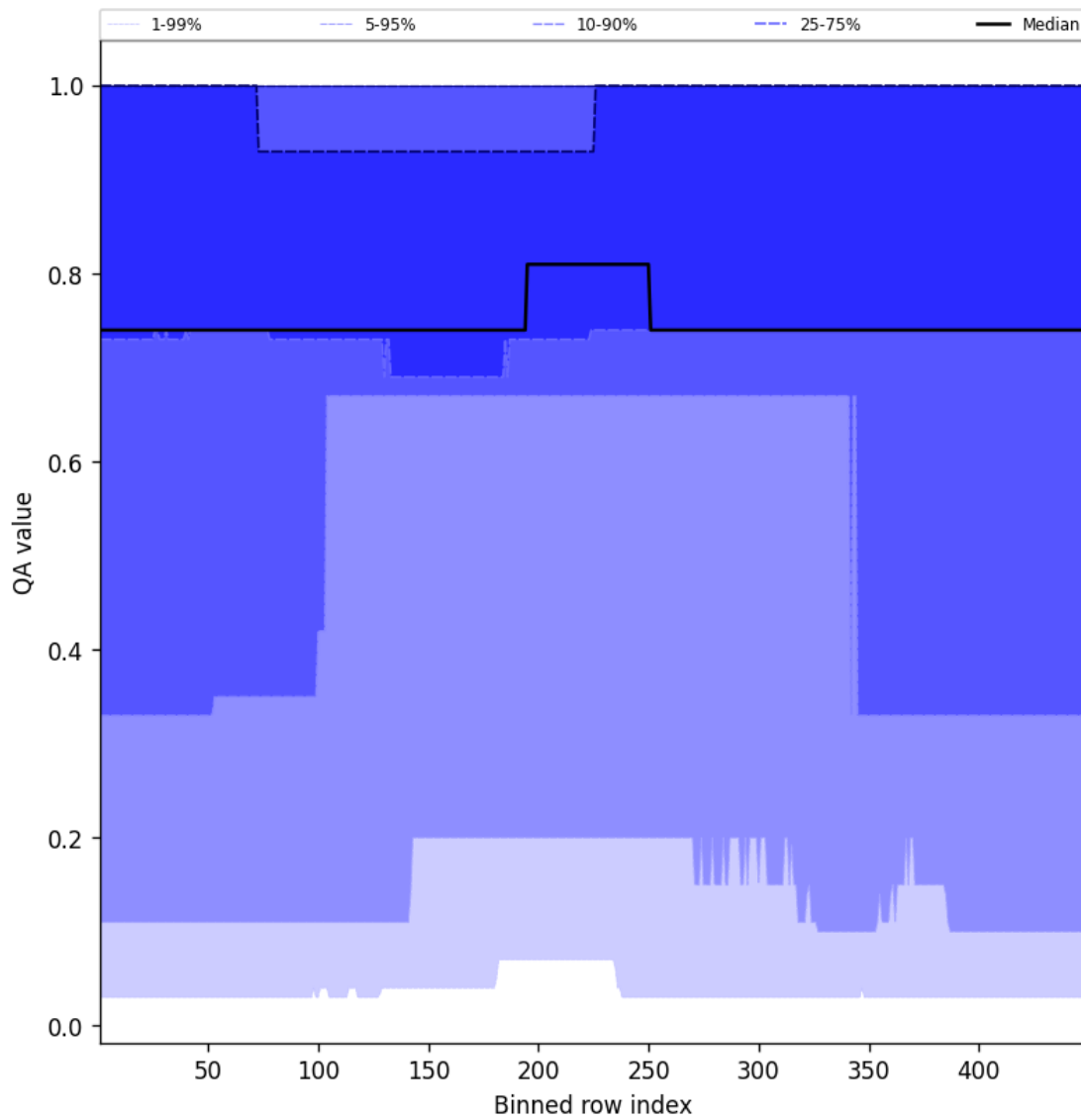
Figure 45: Along track statistics of “QA value” for 2025-01-18 to 2025-01-20
