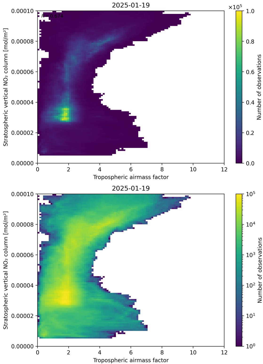
Figure 74: Scatter density plot of “Tropospheric air mass factor” against “Stratospheric vertical NO 2 column” for 2025-01-18 to 2025-01-20.
