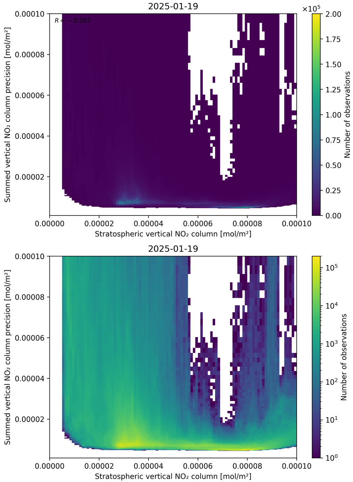
Figure 99: Scatter density plot of “Stratospheric vertical NO 2 column” against “Summed vertical NO 2 column precision” for 2025-01-18 to 2025-01-20.
