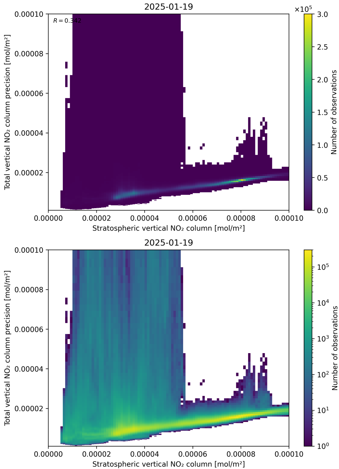
Figure 101: Scatter density plot of “Stratospheric vertical NO 2 column” against “Total vertical NO 2 column precision” for 2025-01-18 to 2025-01-20.
