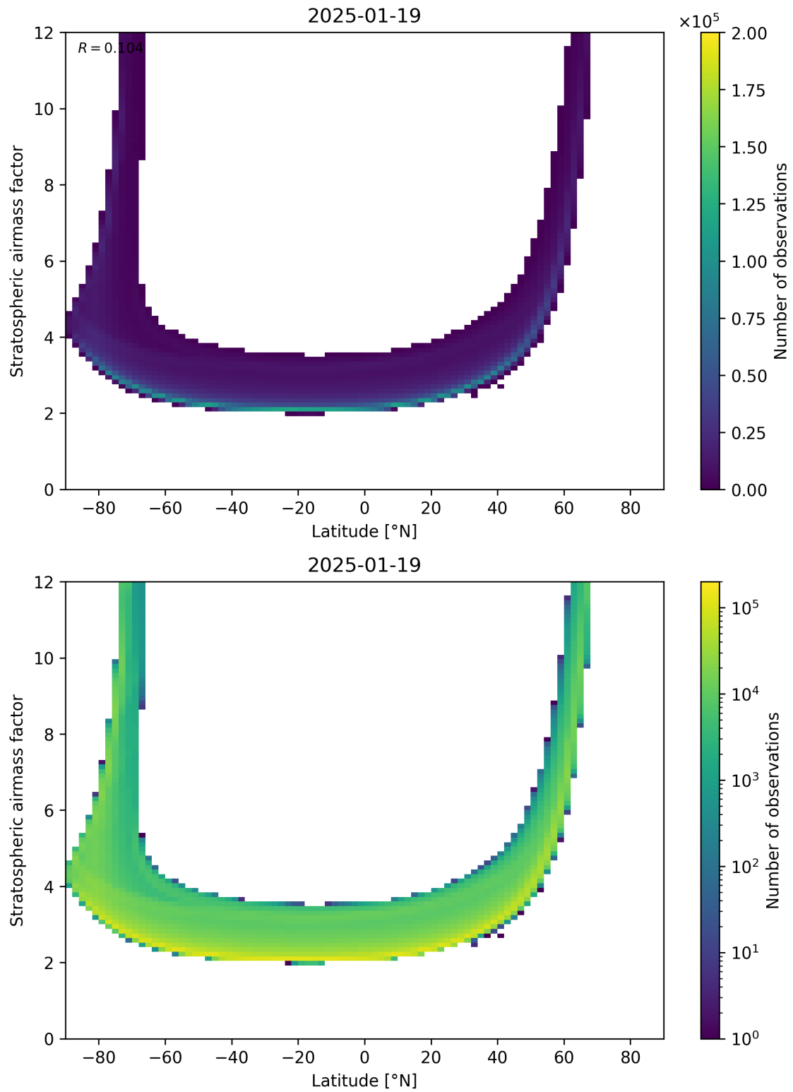
Figure 83: Scatter density plot of “Latitude” against “Stratospheric air mass factor” for 2025-01-18 to 2025-01-20.
