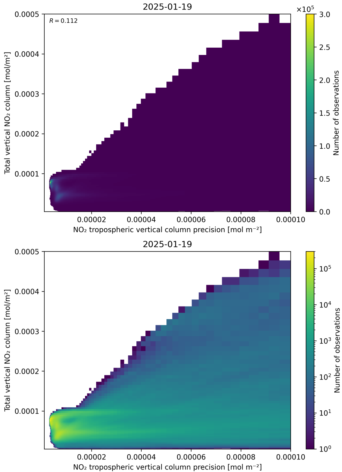
Figure 138: Scatter density plot of “NO 2 tropospheric vertical column precision” against “Total vertical NO 2 column” for 2025-01-18 to 2025-01-20.
