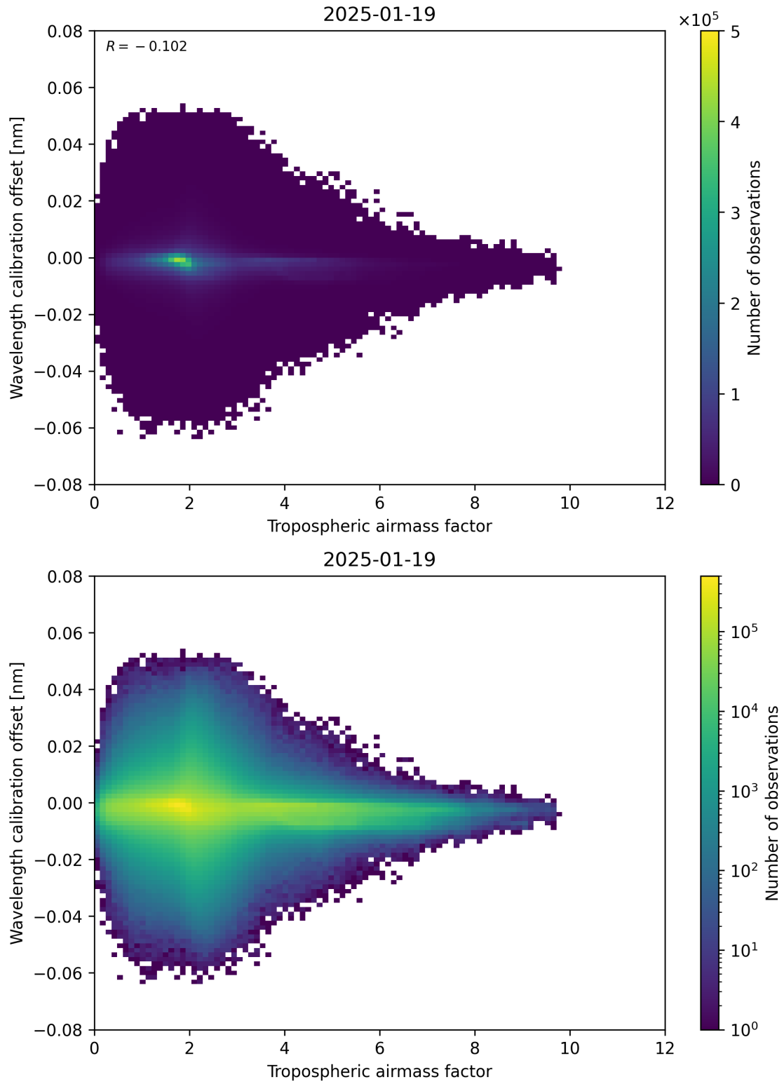
Figure 80: Scatter density plot of “Tropospheric airmass factor” against “Wavelength calibration offset” for 2025-01-18 to 2025-01-20.
