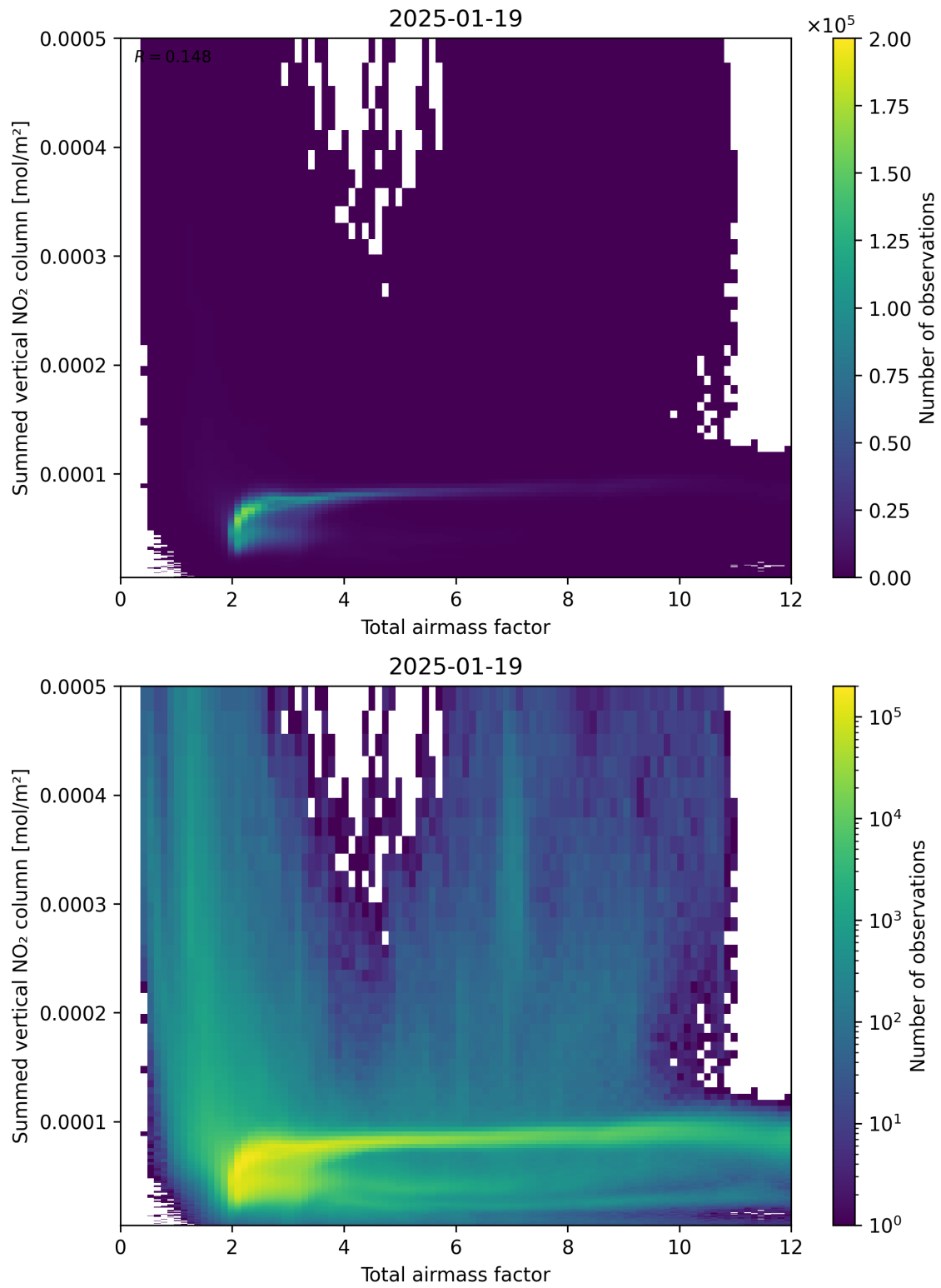
Figure 65: Scatter density plot of “Total airmass factor” against “Summed vertical NO 2 column” for 2025-01-18 to 2025-01-20.
