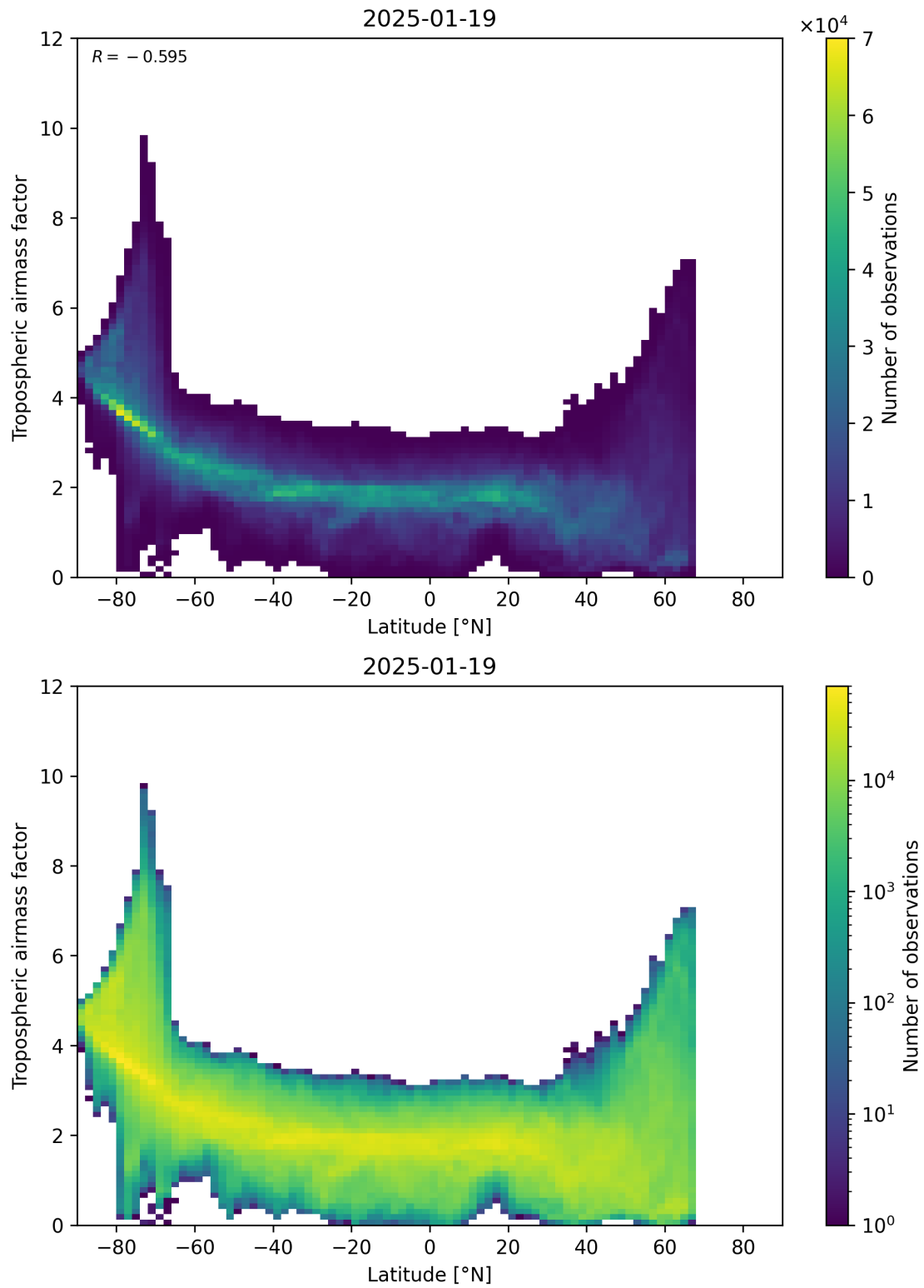
Figure 85: Scatter density plot of “Latitude” against “Tropospheric airmass factor” for 2025-01-18 to 2025-01-20.
