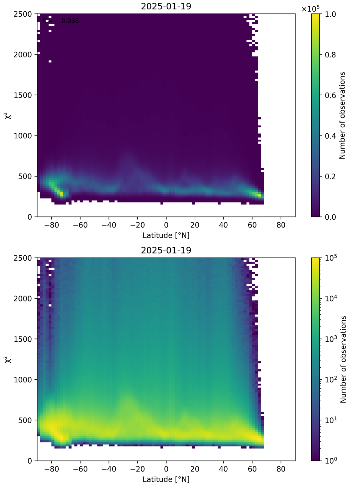
Figure 86: Scatter density plot of “Latitude” against “ \chi^2 ” for 2025-01-18 to 2025-01-20.
