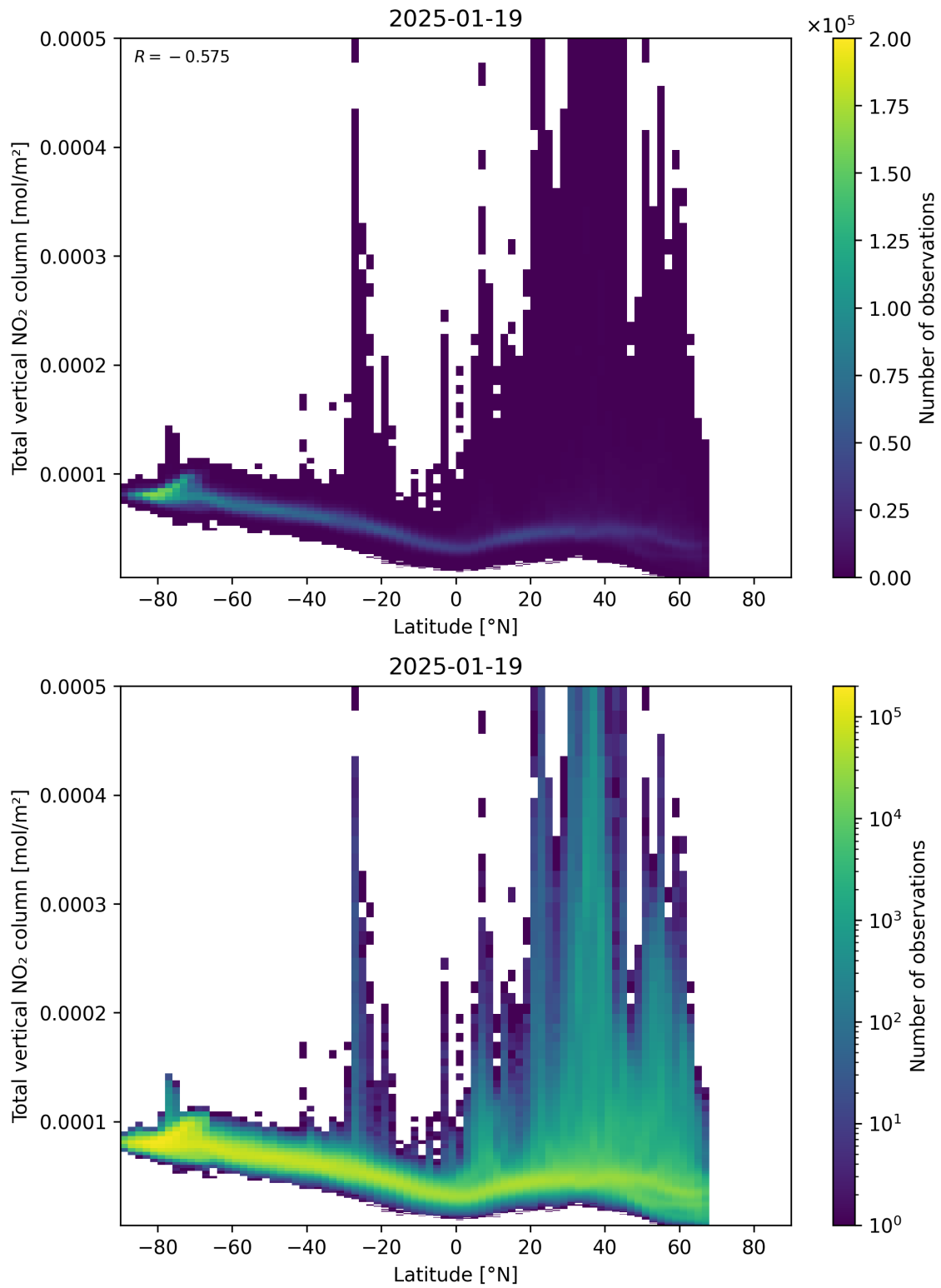
Figure 90: Scatter density plot of “Latitude” against “Total vertical NO 2 column” for 2025-01-18 to 2025-01-20.
