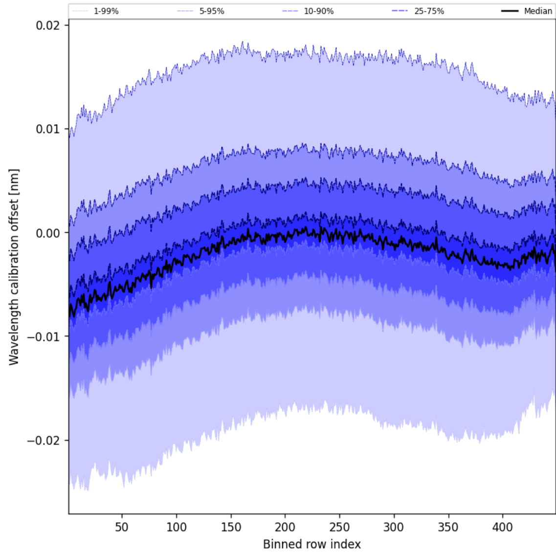
Figure 52: Along track statistics of “Wavelength calibration offset” for 2025-01-18 to 2025-01-20
