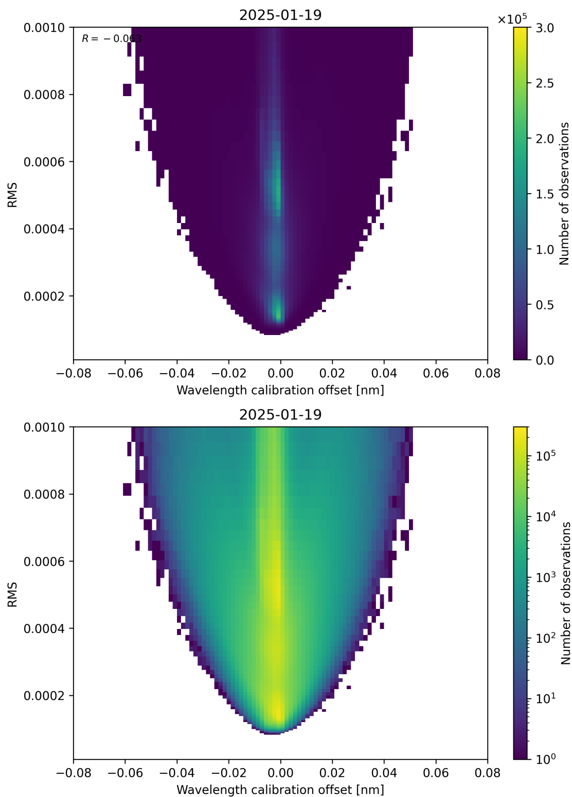
Figure 181: Scatter density plot of “Wavelength calibration offset” against “RMS” for 2025-01-18 to 2025-01-20.
