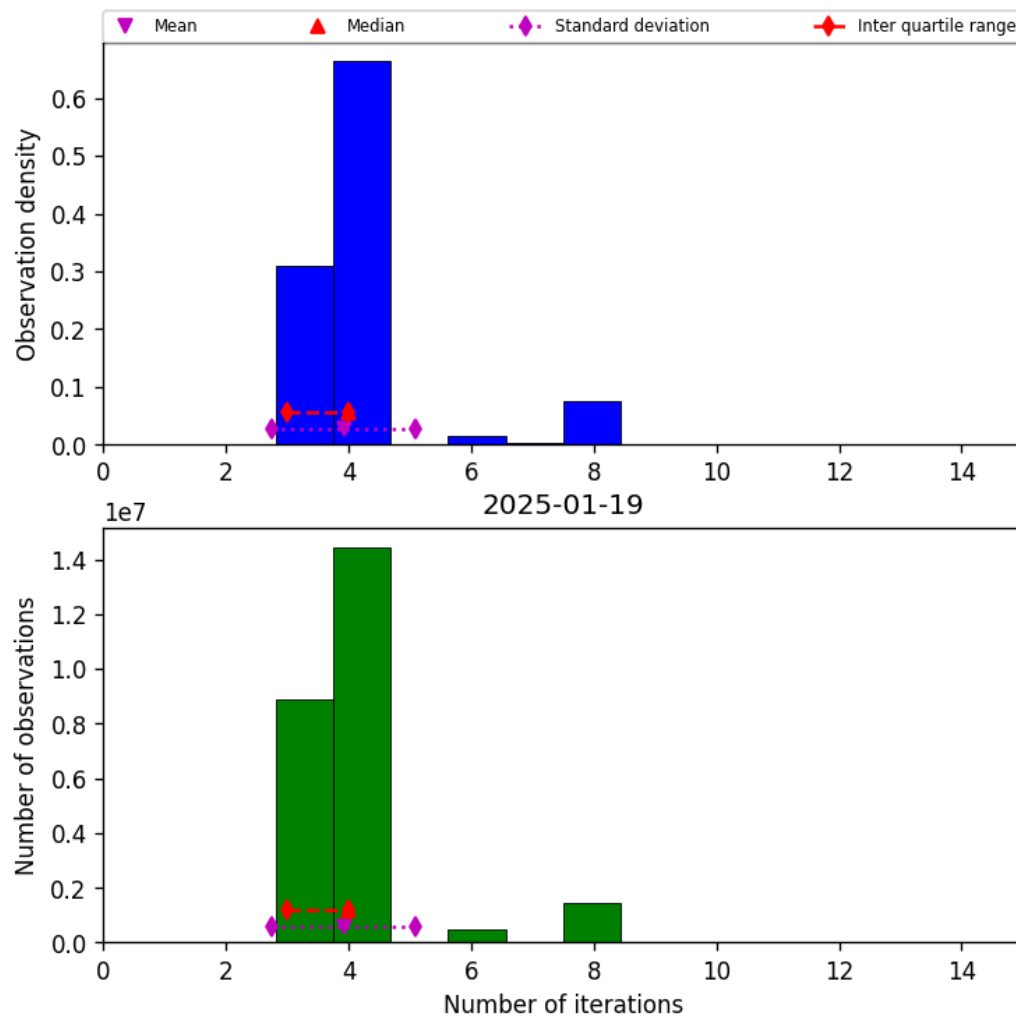
Figure 34: Histogram of “Number of iterations” for 2025-01-18 to 2025-01-20
