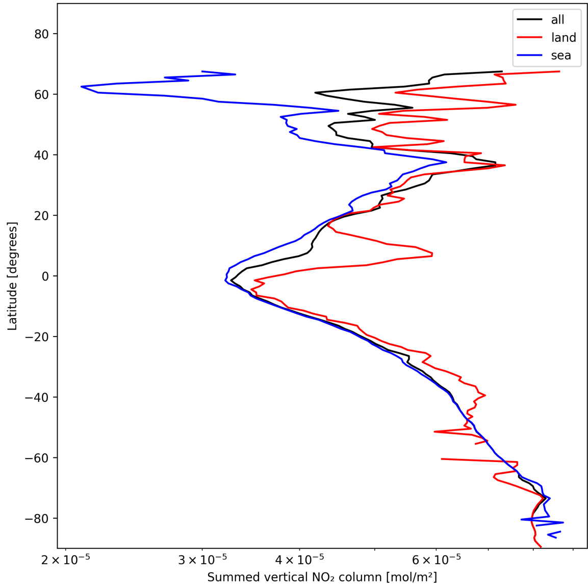
Figure 23: Zonal average of “Summed vertical NO 2 column” for 2025-01-18 to 2025-01-20.
