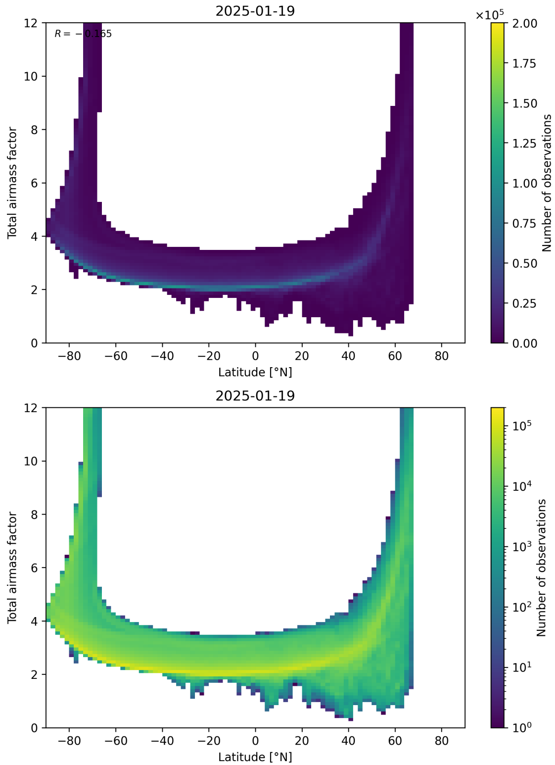
Figure 84: Scatter density plot of “Latitude” against “Total airmass factor” for 2025-01-18 to 2025-01-20.
