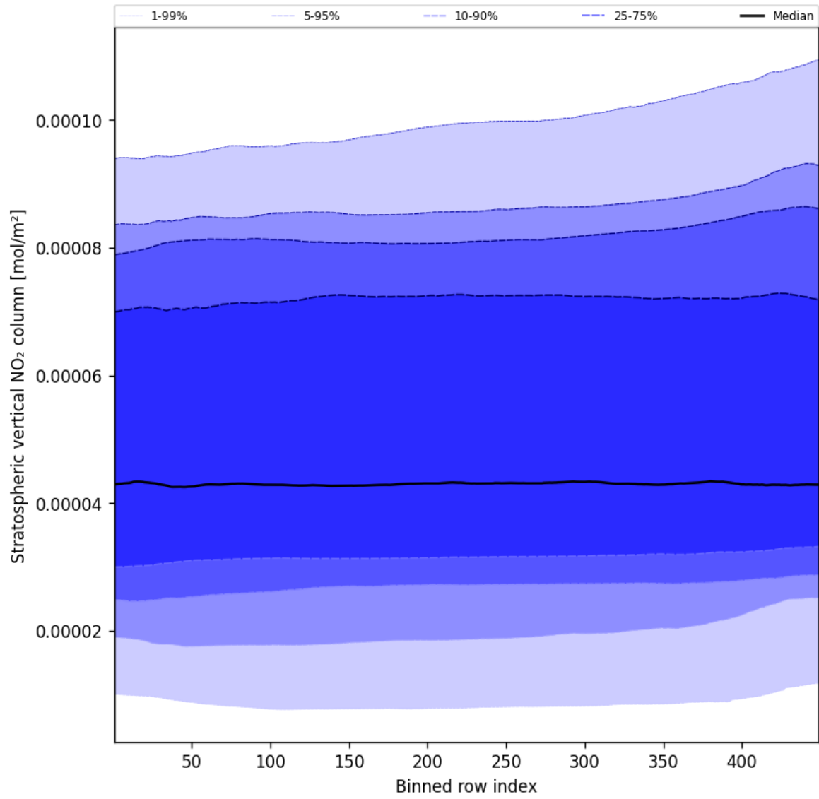
Figure 53: Along track statistics of “Stratospheric vertical NO 2 column” for 2025-01-18 to 2025-01-20
