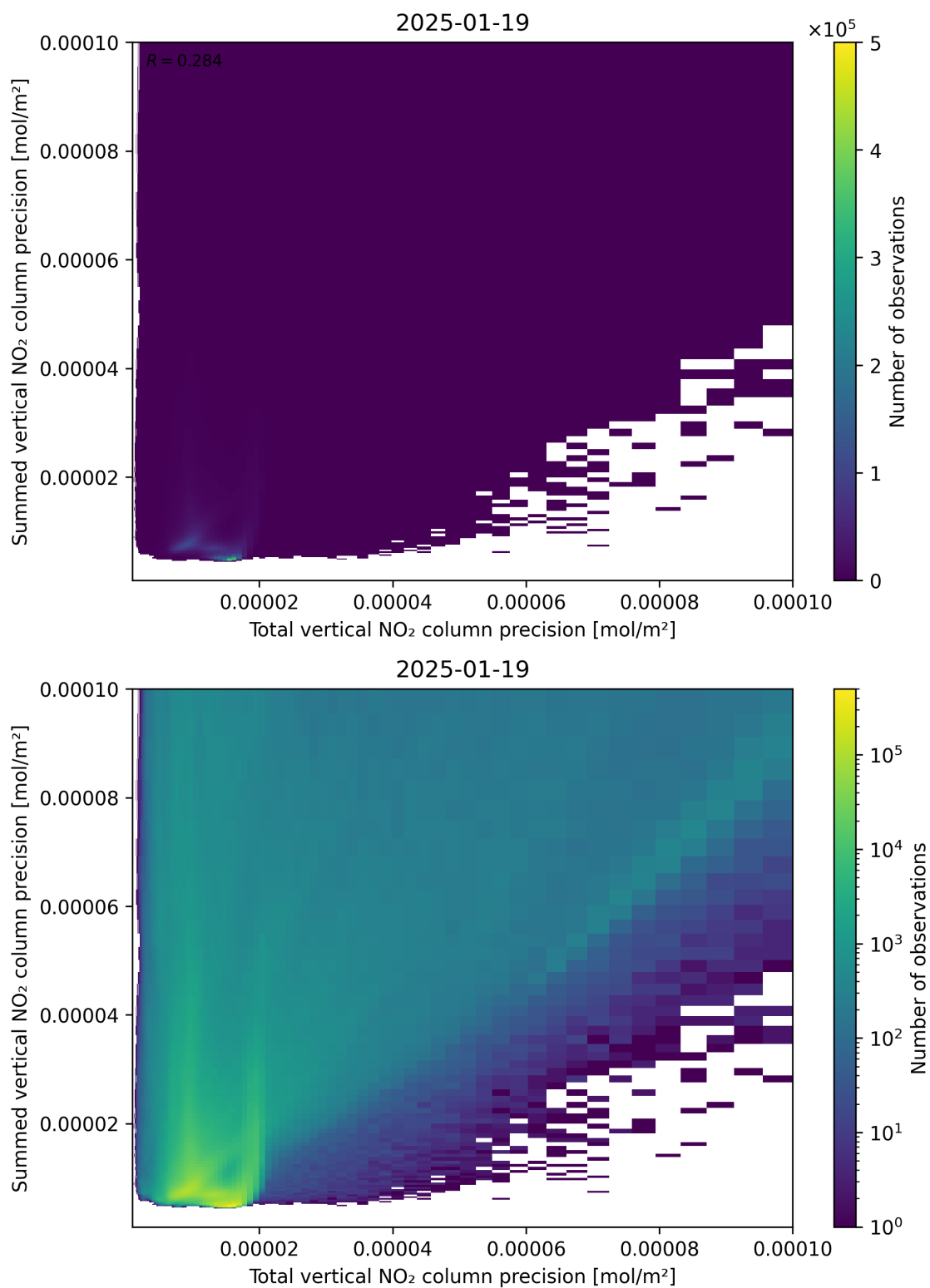
Figure 118: Scatter density plot of “Total vertical NO 2 column precision” against “Summed vertical NO 2 column precision” for 2025-01-18 to 2025-01-20.
