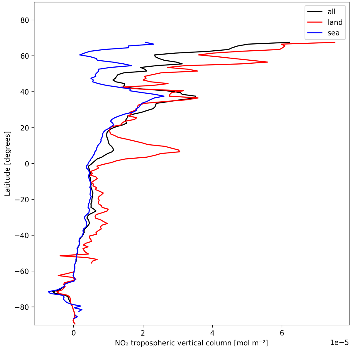
Figure 12: Zonal average of “NO 2 tropospheric vertical column” for 2025-01-18 to 2025-01-20.
