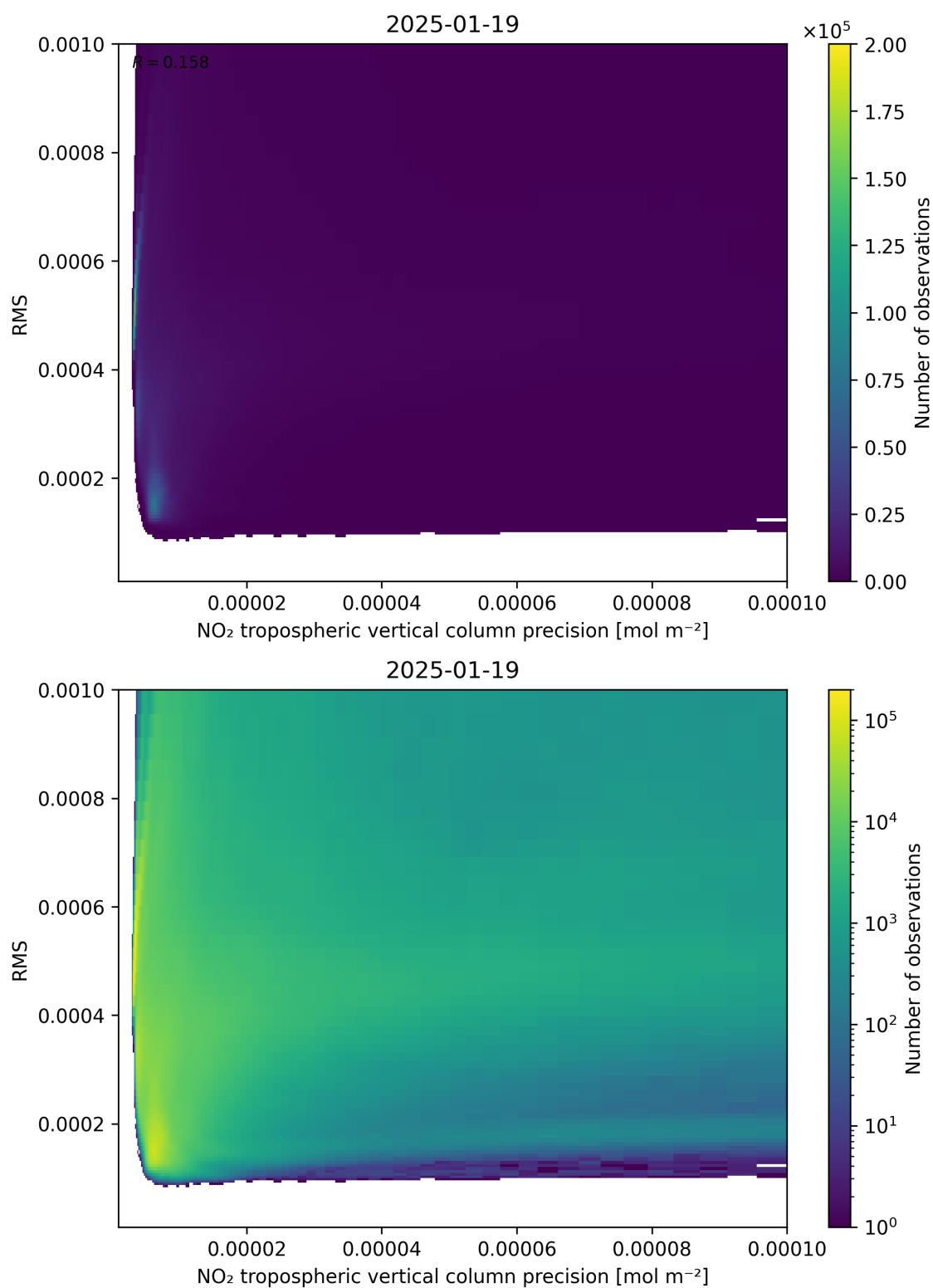
Figure 140: Scatter density plot of “NO 2 tropospheric vertical column precision” against “RMS” for 2025-01-18 to 2025-01-20.
