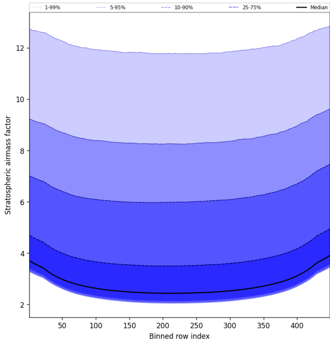
Figure 61: Along track statistics of “Stratospheric airmass factor” for 2025-01-18 to 2025-01-20
