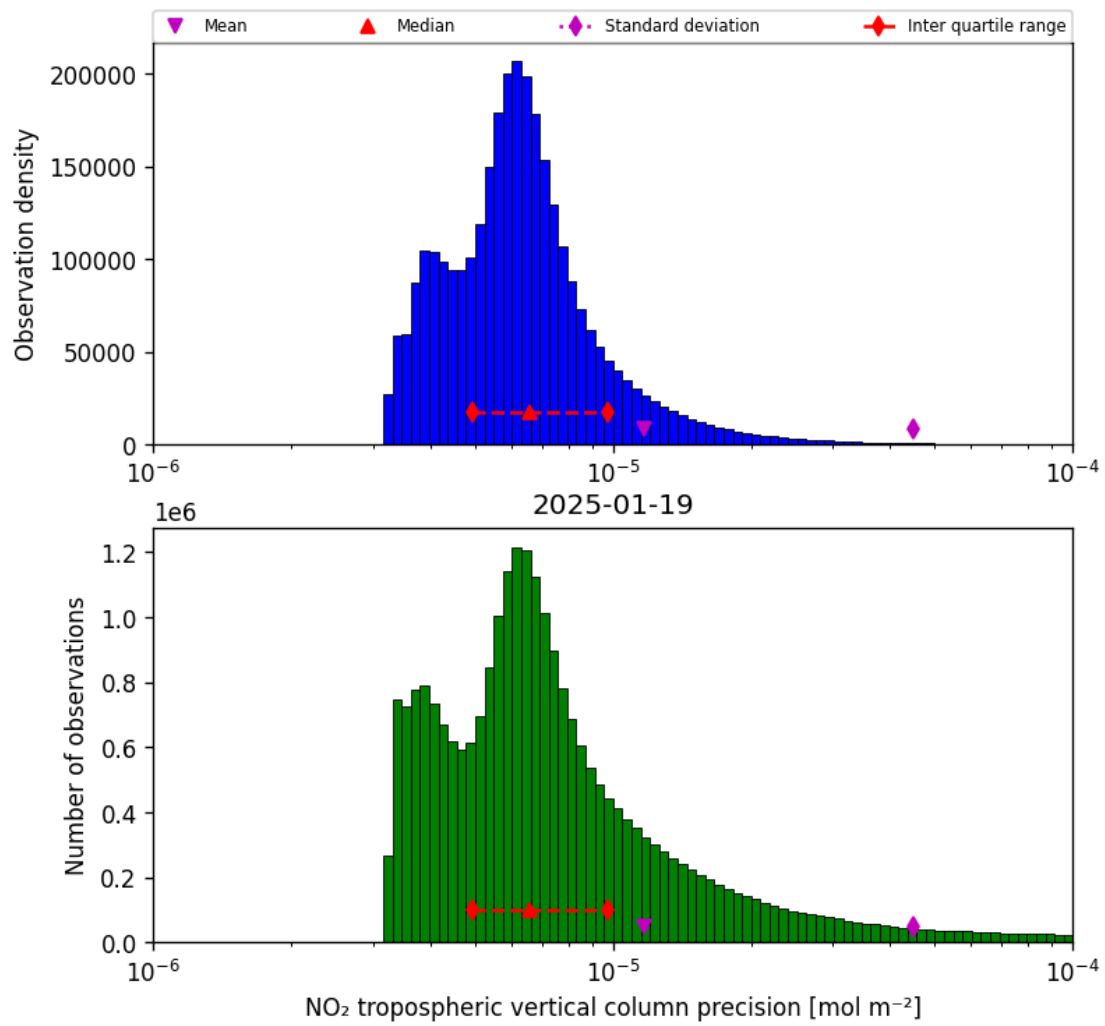
Figure 30: Histogram of “NO 2 tropospheric vertical column precision” for 2025-01-18 to 2025-01-20
