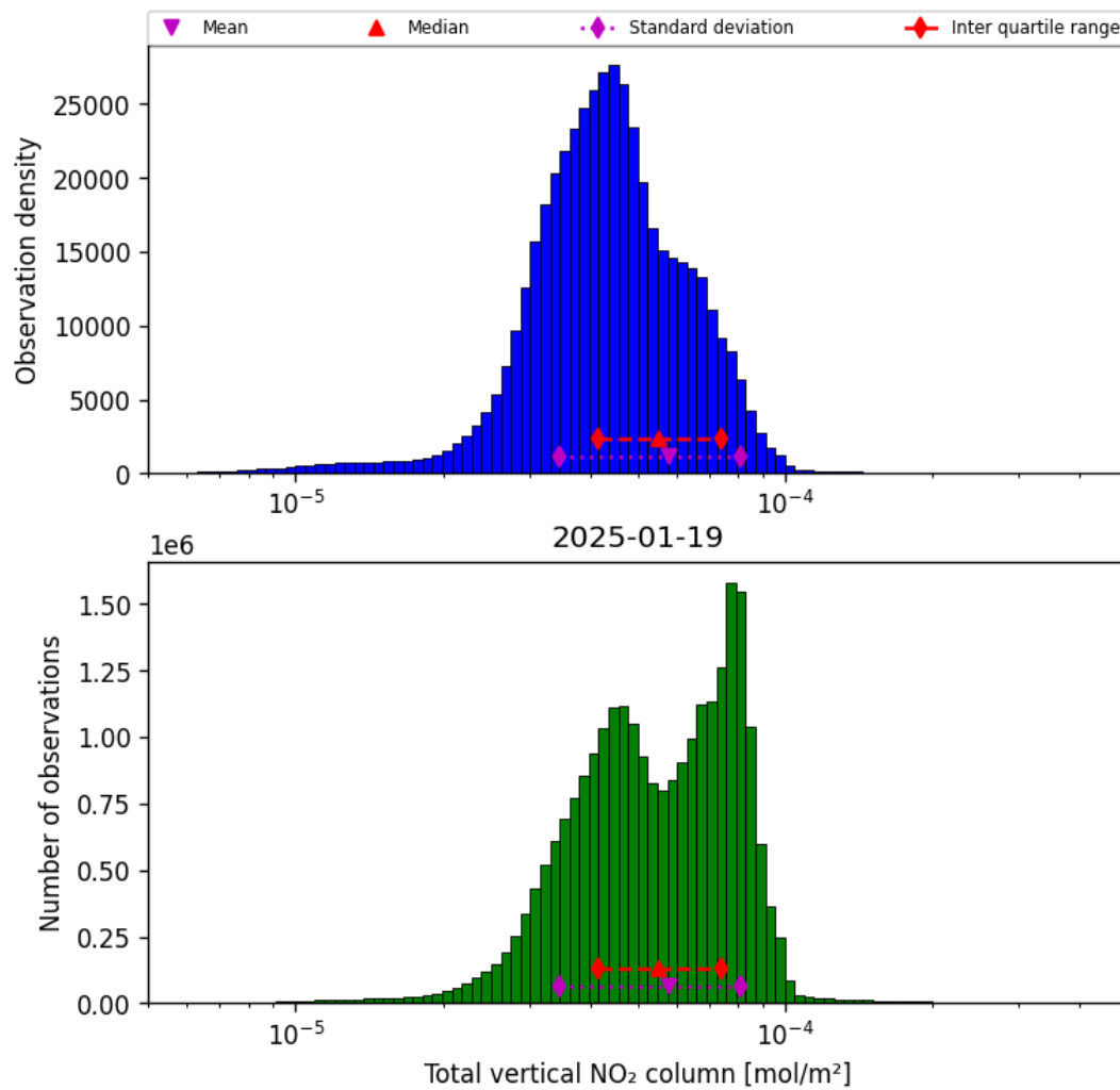
Figure 38: Histogram of “Total vertical NO 2 column” for 2025-01-18 to 2025-01-20
