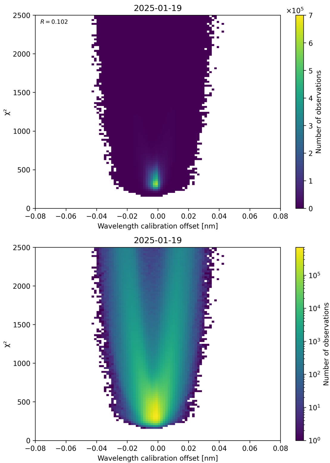
Figure 175: Scatter density plot of “Wavelength calibration offset” against “ \chi^2 ” for 2025-01-18 to 2025-01-20.
