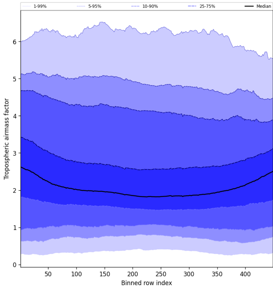
Figure 48: Along track statistics of “Tropospheric airmass factor” for 2025-01-18 to 2025-01-20
