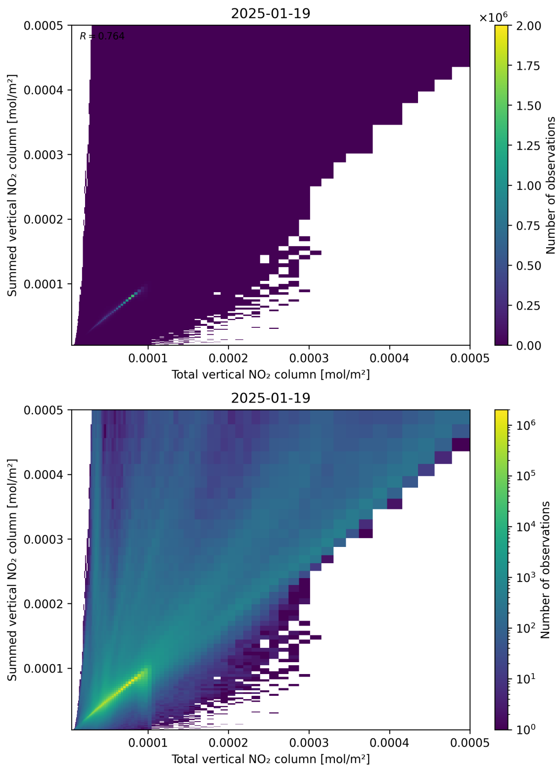
Figure 112: Scatter density plot of “Total vertical NO 2 column” against “Summed vertical NO 2 column” for 2025-01-18 to 2025-01-20.
