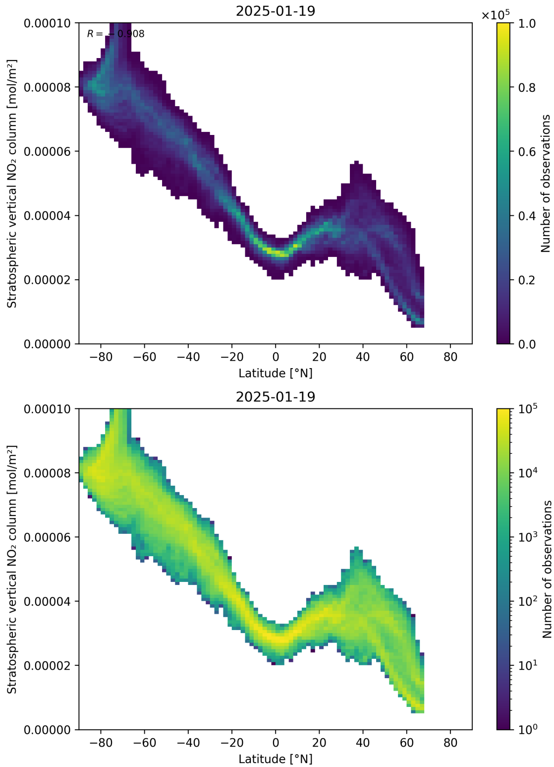
Figure 87: Scatter density plot of “Latitude” against “Stratospheric vertical NO 2 column” for 2025-01-18 to 2025-01-20.
