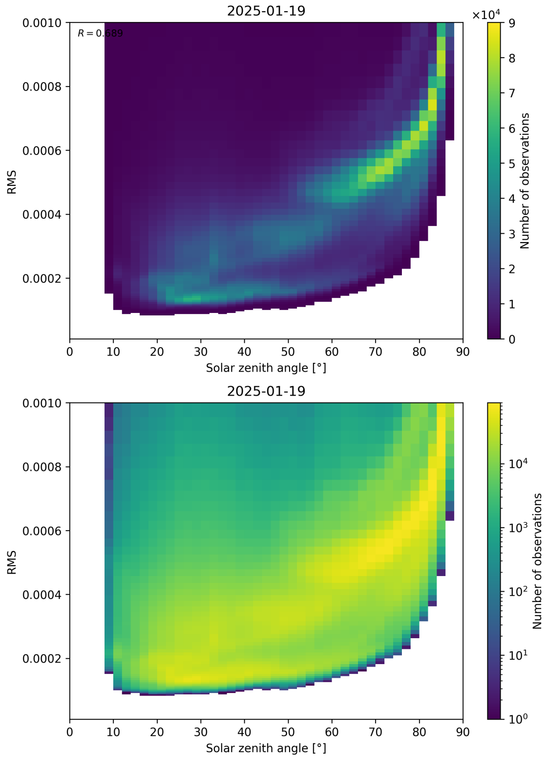
Figure 157: Scatter density plot of “Solar zenith angle” against “RMS” for 2025-01-18 to 2025-01-20.
