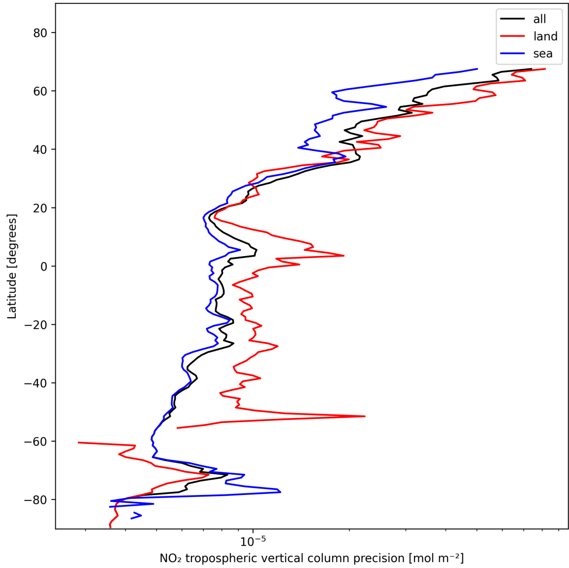
Figure 13: Zonal average of “NO 2 tropospheric vertical column precision” for 2025-01-18 to 2025-01-20.
