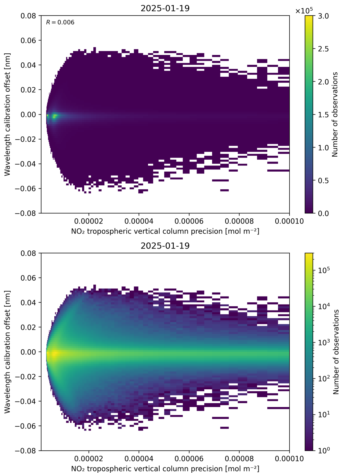
Figure 141: Scatter density plot of “NO 2 tropospheric vertical column precision” against “Wavelength calibration offset” for 2025-01-18 to 2025-01-20.
