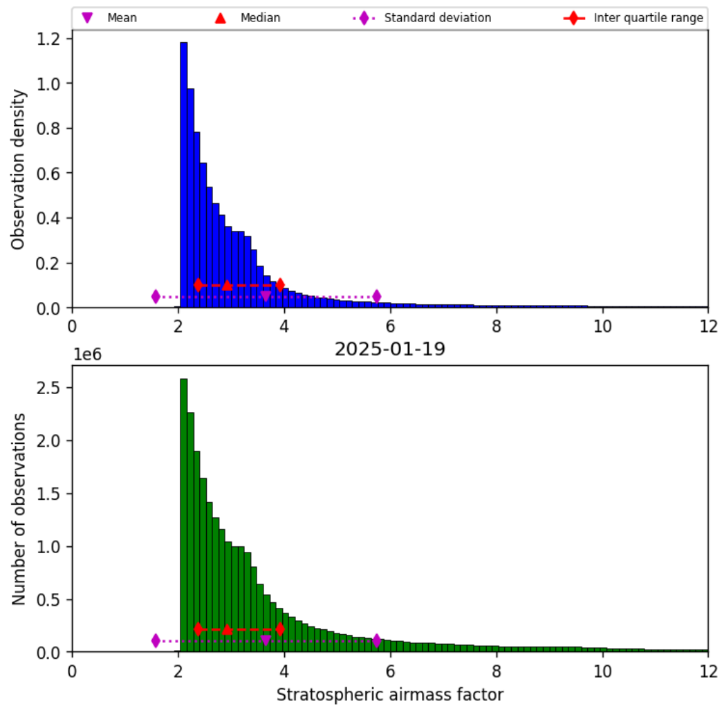
Figure 44: Histogram of “Stratospheric airmass factor” for 2025-01-18 to 2025-01-20
