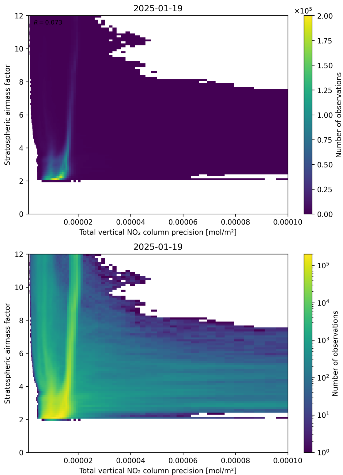
Figure 115: Scatter density plot of “Total vertical NO 2 column precision” against “Stratospheric airmass factor” for 2025-01-18 to 2025-01-20.
