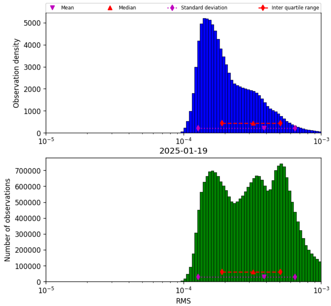
Figure 43: Histogram of “RMS” for 2025-01-18 to 2025-01-20
