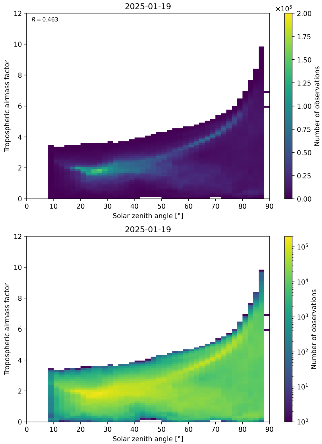
Figure 147: Scatter density plot of “Solar zenith angle” against “Tropospheric airmass factor” for 2025-01-18 to 2025-01-20.
