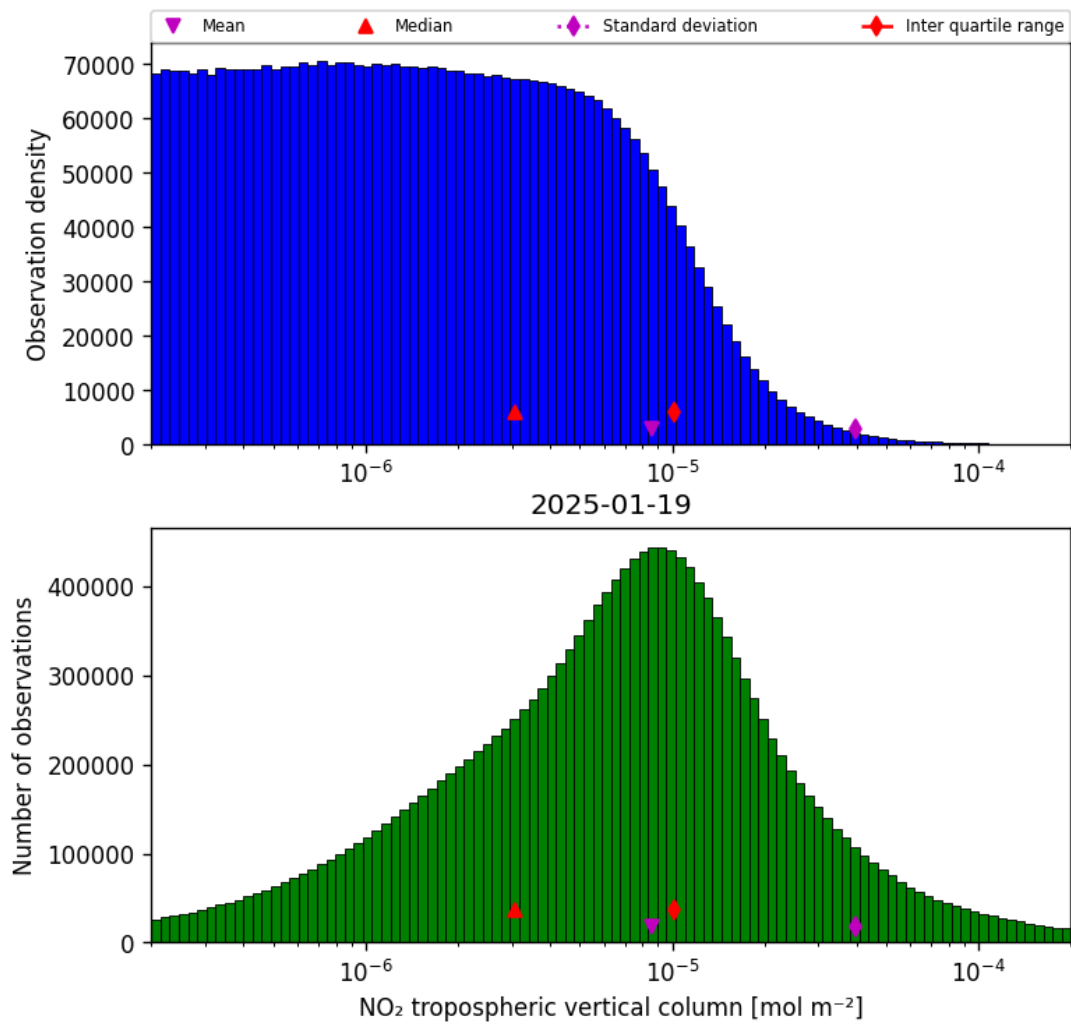
Figure 29: Histogram of “NO 2 tropospheric vertical column” for 2025-01-18 to 2025-01-20
