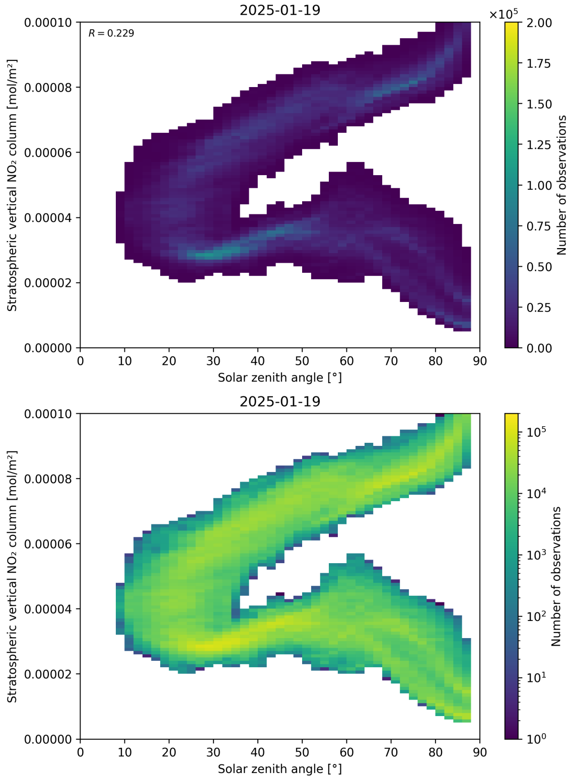
Figure 150: Scatter density plot of “Solar zenith angle” against “Stratospheric vertical NO 2 column” for 2025-01-18 to 2025-01-20.
