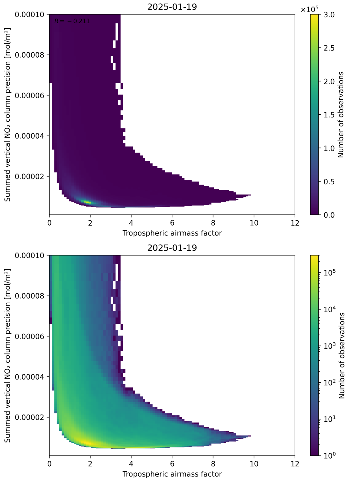
Figure 76: Scatter density plot of “Tropospheric airmass factor” against “Summed vertical NO 2 column precision” for 2025-01-18 to 2025-01-20.
