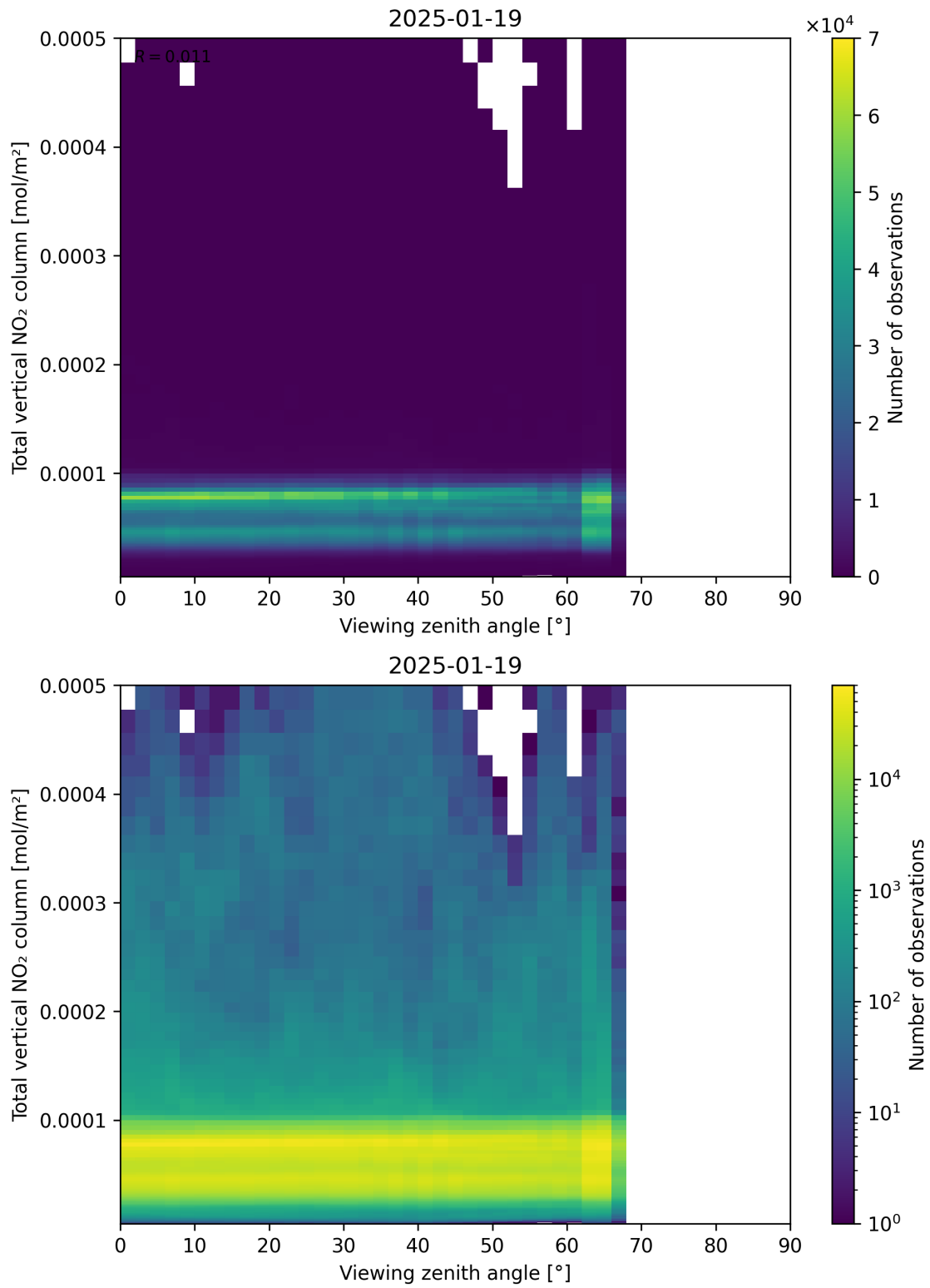
Figure 167: Scatter density plot of “Viewing zenith angle” against “Total vertical NO 2 column” for 2025-01-18 to 2025-01-20.
