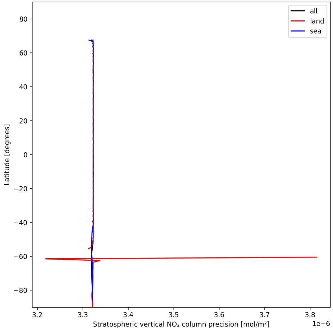
Figure 20: Zonal average of “Stratospheric vertical NO 2 column precision” for 2025-01-18 to 2025-01-20.
