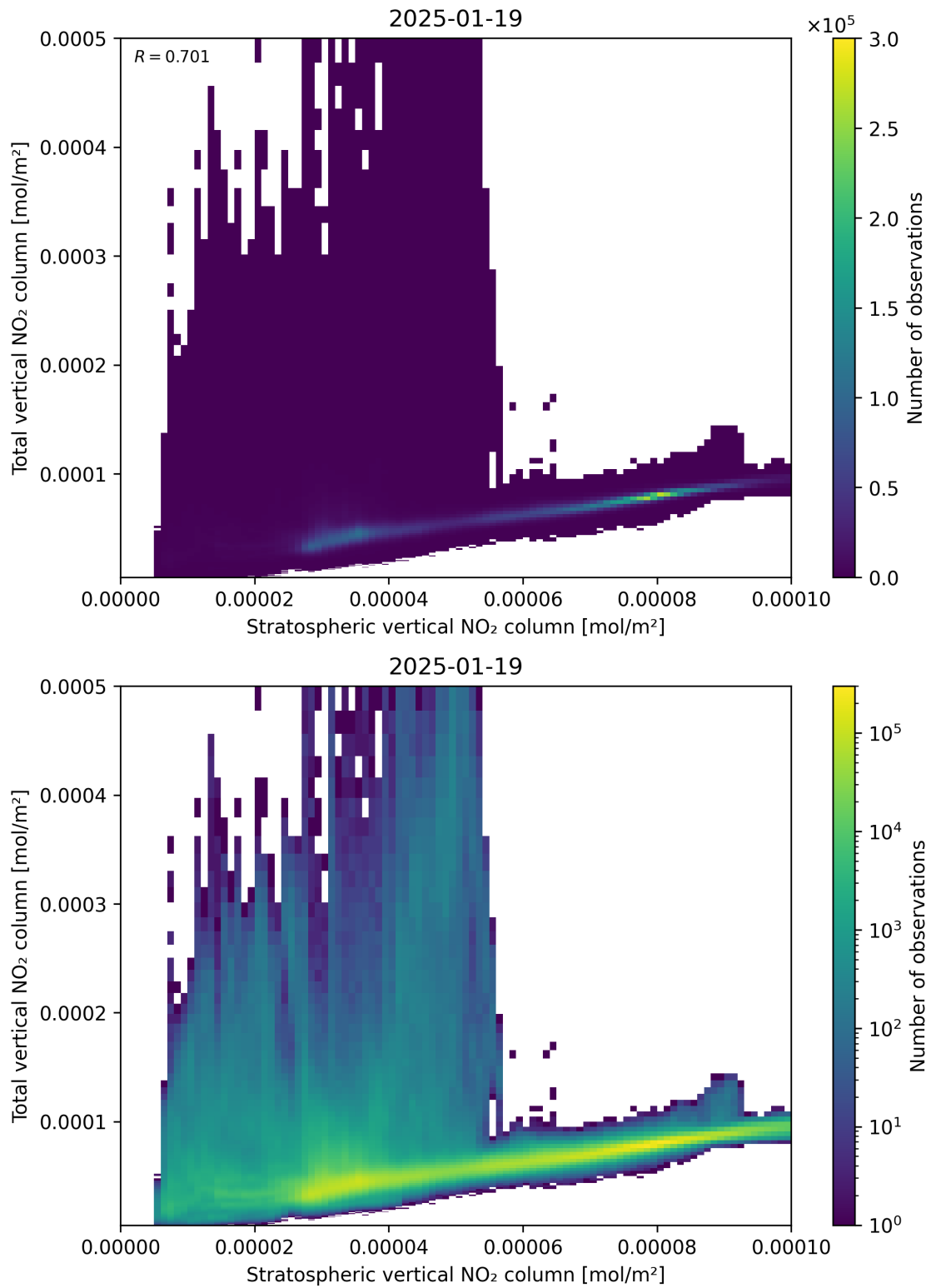
Figure 100: Scatter density plot of “Stratospheric vertical NO 2 column” against “Total vertical NO 2 column” for 2025-01-18 to 2025-01-20.
