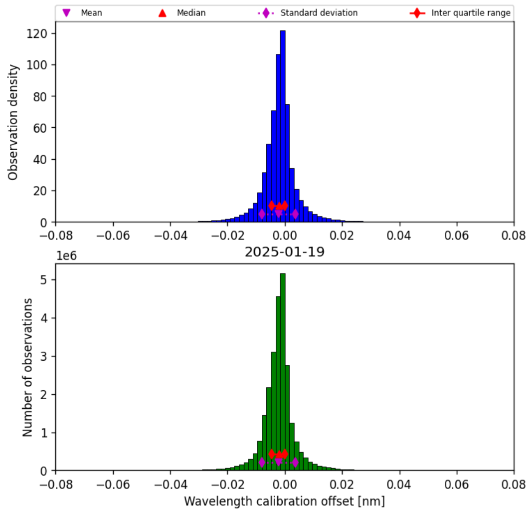
Figure 35: Histogram of “Wavelength calibration offset” for 2025-01-18 to 2025-01-20
