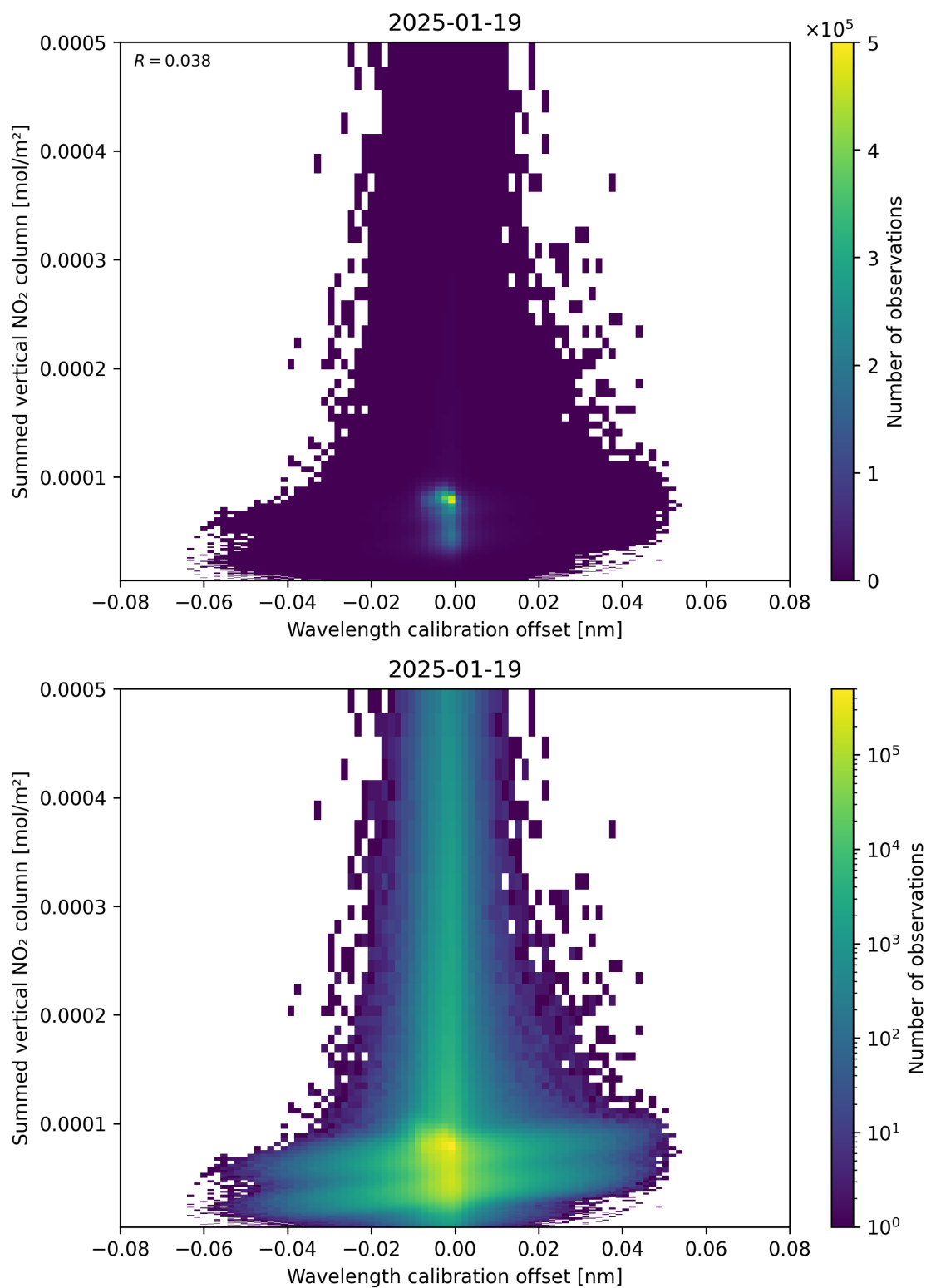
Figure 177: Scatter density plot of “Wavelength calibration offset” against “Summed vertical NO 2 column” for 2025-01-18 to 2025-01-20.
