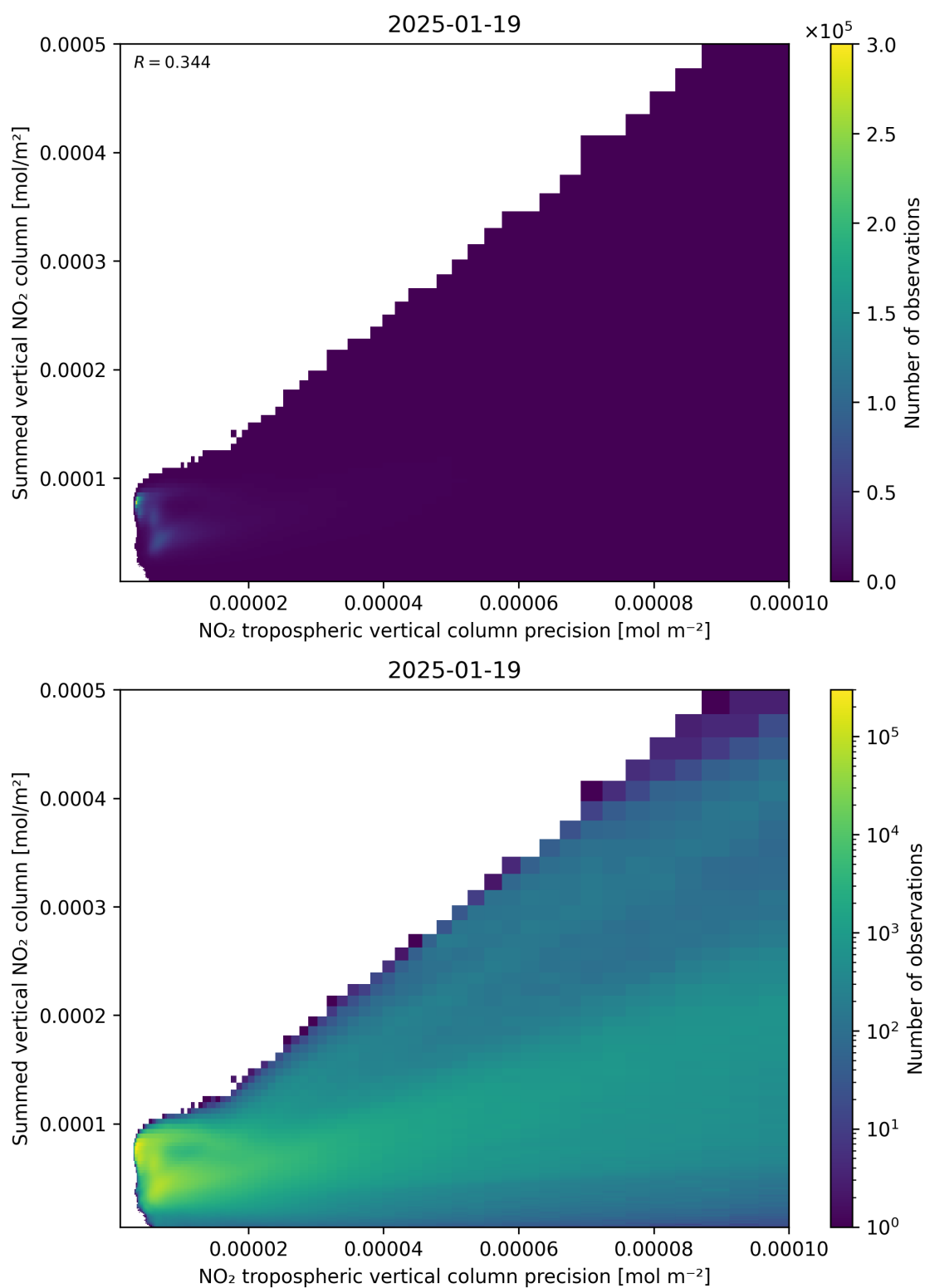
Figure 136: Scatter density plot of “NO 2 tropospheric vertical column precision” against “Summed vertical NO 2 column” for 2025-01-18 to 2025-01-20.
