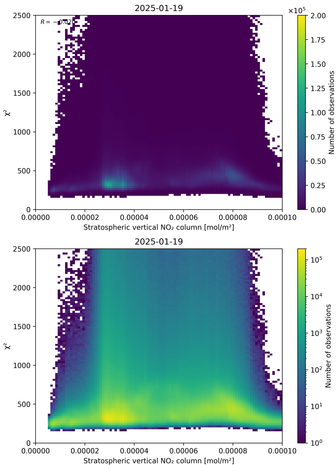
Figure 97: Scatter density plot of “Stratospheric vertical NO 2 column” against “ \chi^2 ” for 2025-01-18 to 2025-01-20.
