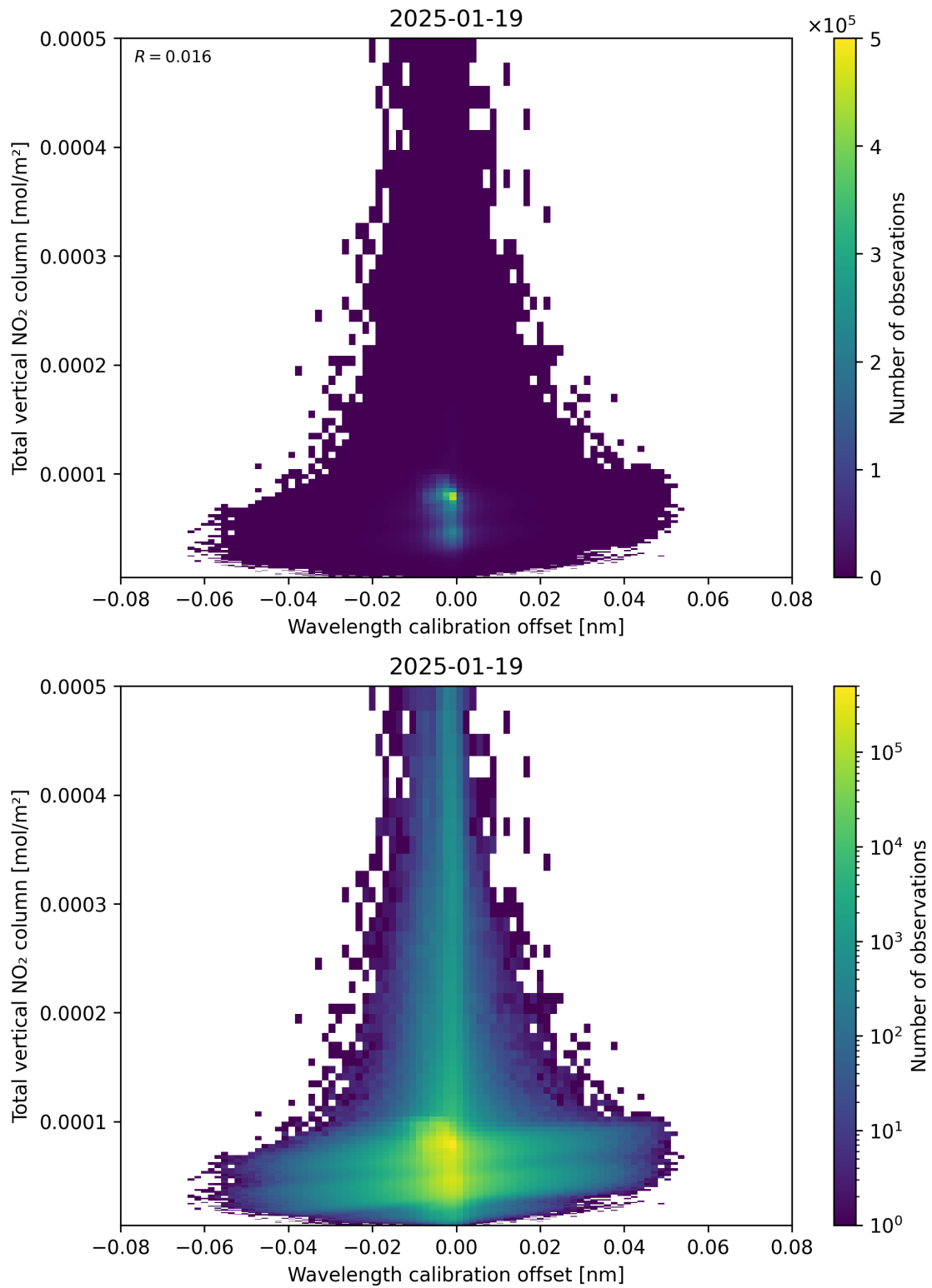
Figure 179: Scatter density plot of “Wavelength calibration offset” against “Total vertical NO 2 column” for 2025-01-18 to 2025-01-20.
