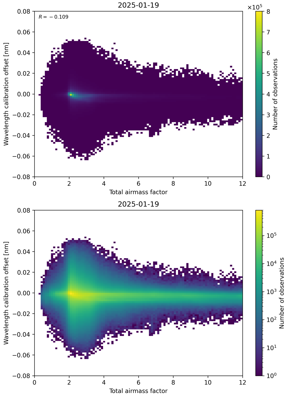
Figure 70: Scatter density plot of “Total airmass factor” against “Wavelength calibration offset” for 2025-01-18 to 2025-01-20.
