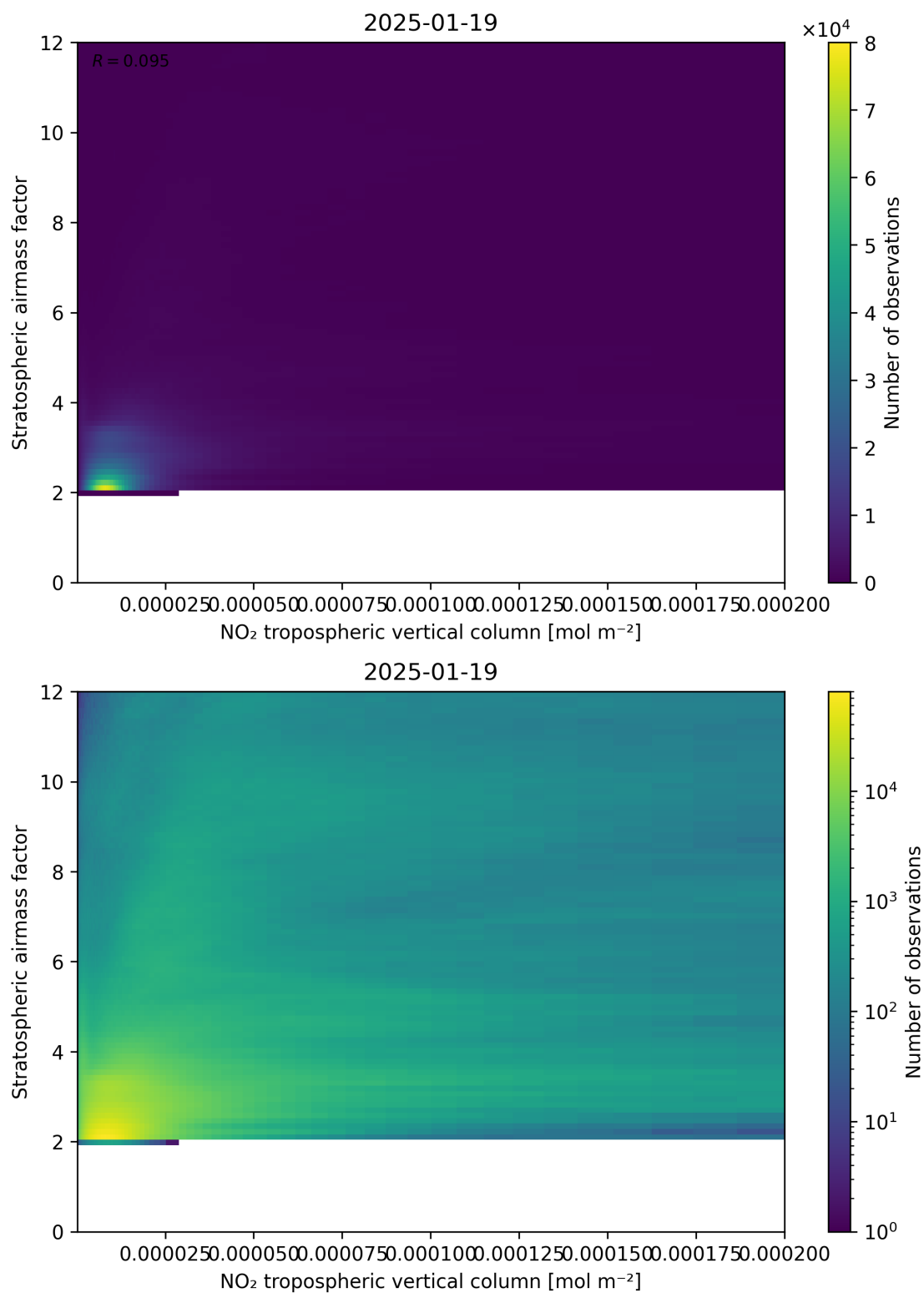
Figure 121: Scatter density plot of “NO 2 tropospheric vertical column” against “Stratospheric airmass factor” for 2025-01-18 to 2025-01-20.
