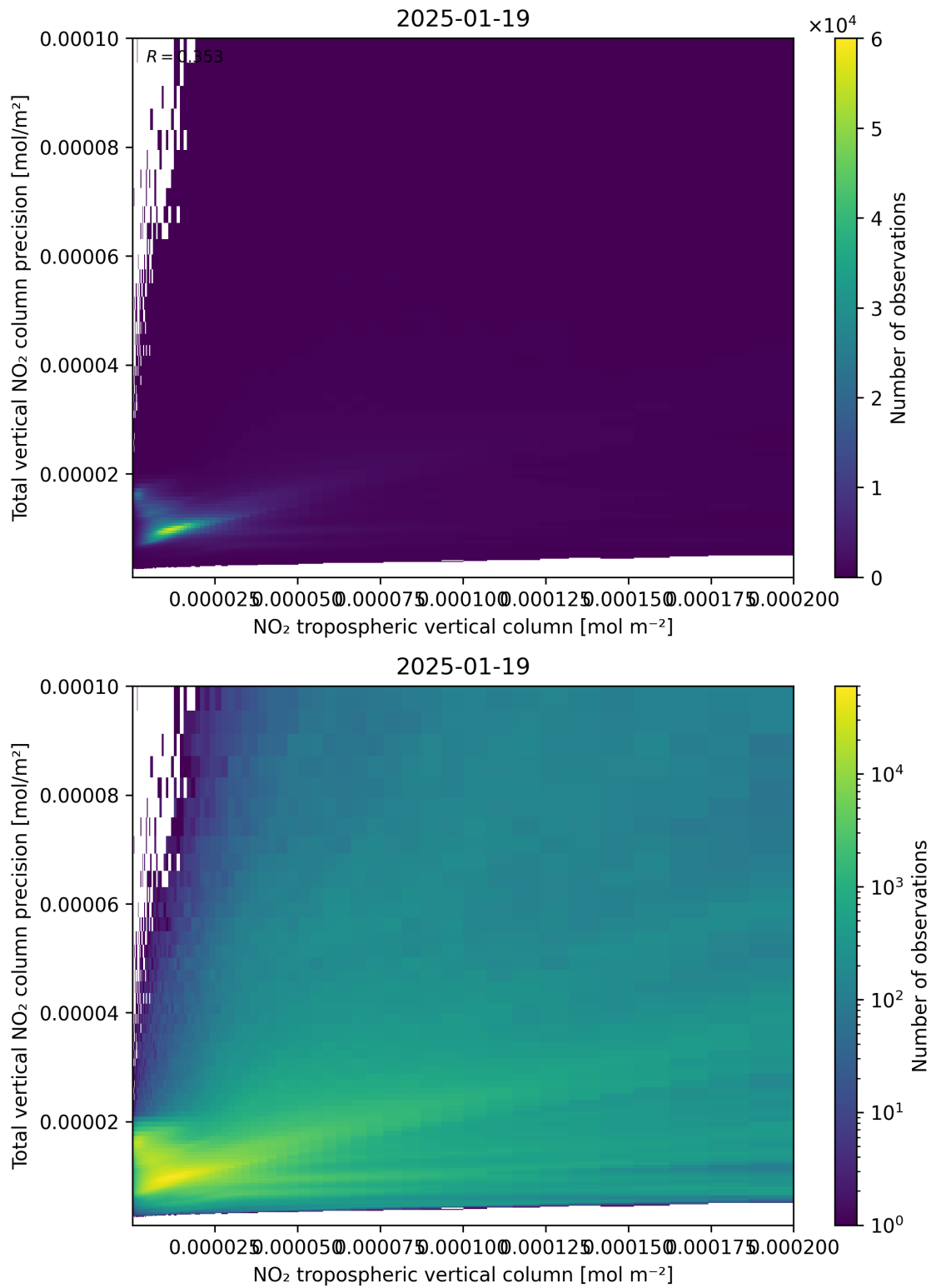
Figure 129: Scatter density plot of “NO 2 tropospheric vertical column” against “Total vertical NO 2 column precision” for 2025-01-18 to 2025-01-20.
