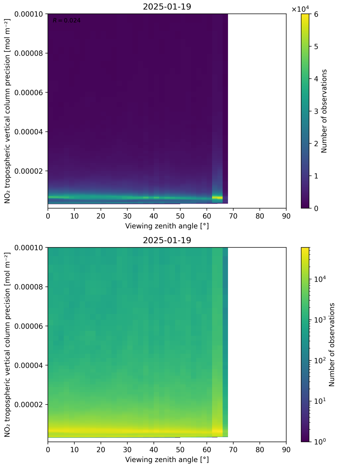
Figure 170: Scatter density plot of “Viewing zenith angle” against “NO 2 tropospheric vertical column precision” for 2025-01-18 to 2025-01-20.
