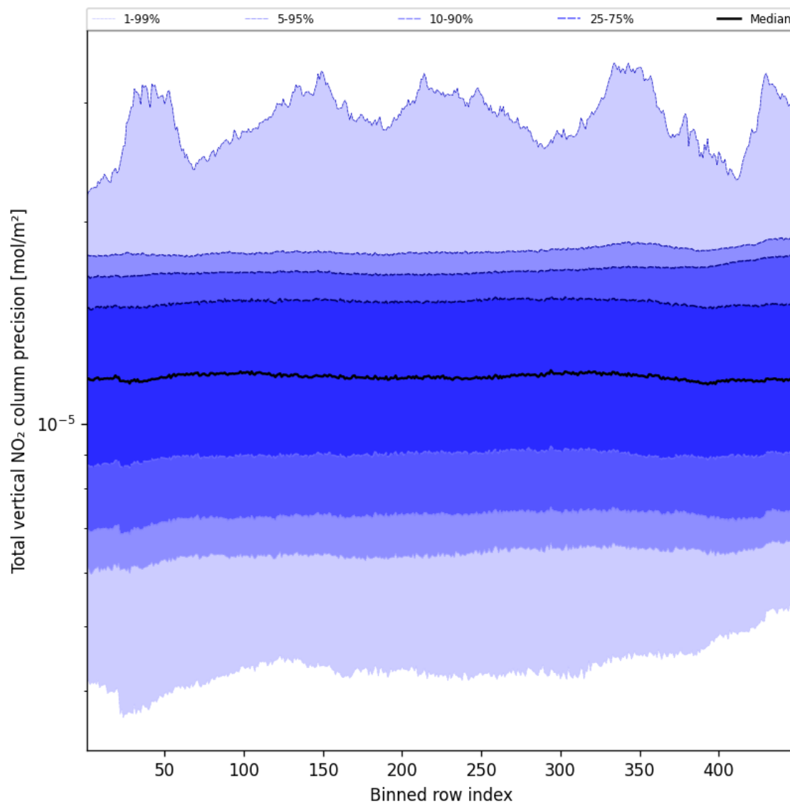
Figure 56: Along track statistics of “Total vertical NO 2 column precision” for 2025-01-18 to 2025-01-20
