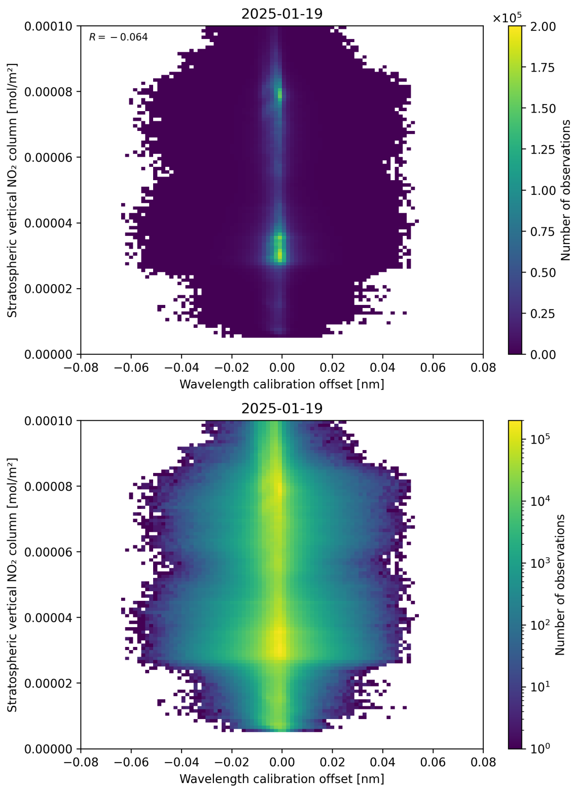
Figure 176: Scatter density plot of “Wavelength calibration offset” against “Stratospheric vertical NO 2 column” for 2025-01-18 to 2025-01-20.
