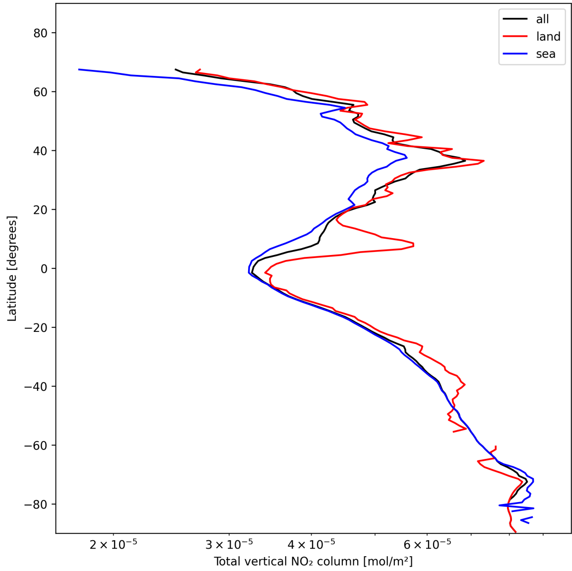
Figure 21: Zonal average of “Total vertical NO 2 column” for 2025-01-18 to 2025-01-20.
