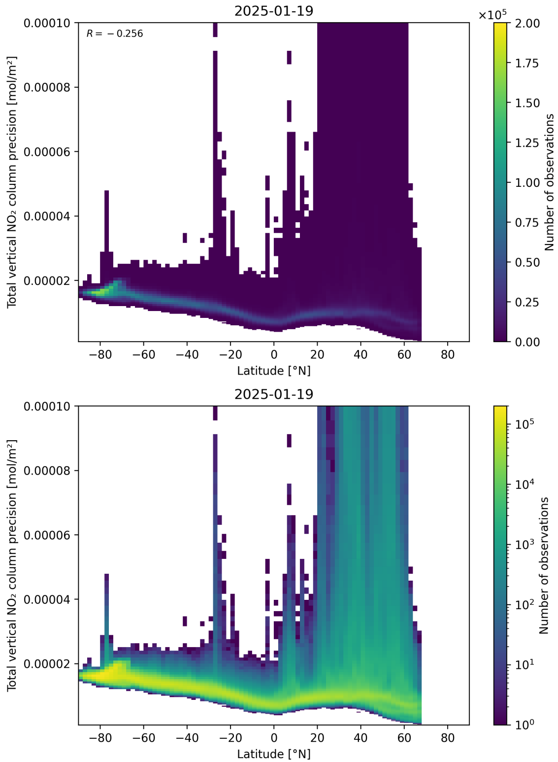
Figure 91: Scatter density plot of “Latitude” against “Total vertical NO 2 column precision” for 2025-01-18 to 2025-01-20.
