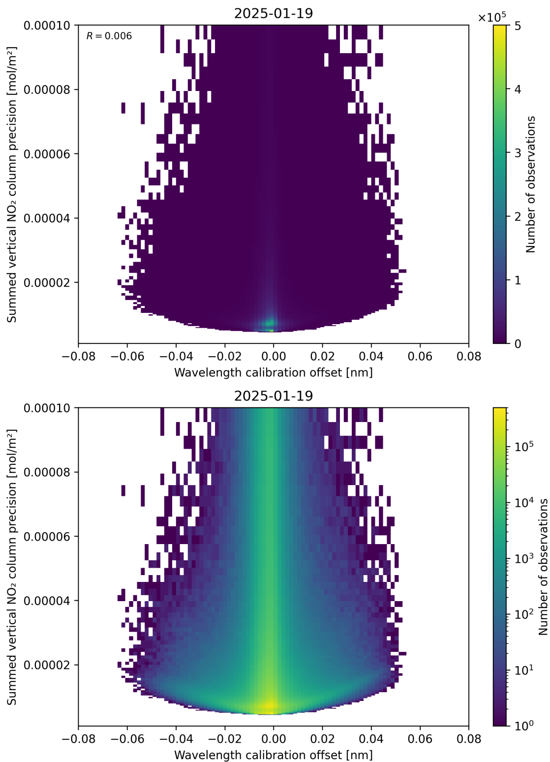
Figure 178: Scatter density plot of “Wavelength calibration offset” against “Summed vertical NO 2 column precision” for 2025-01-18 to 2025-01-20.
