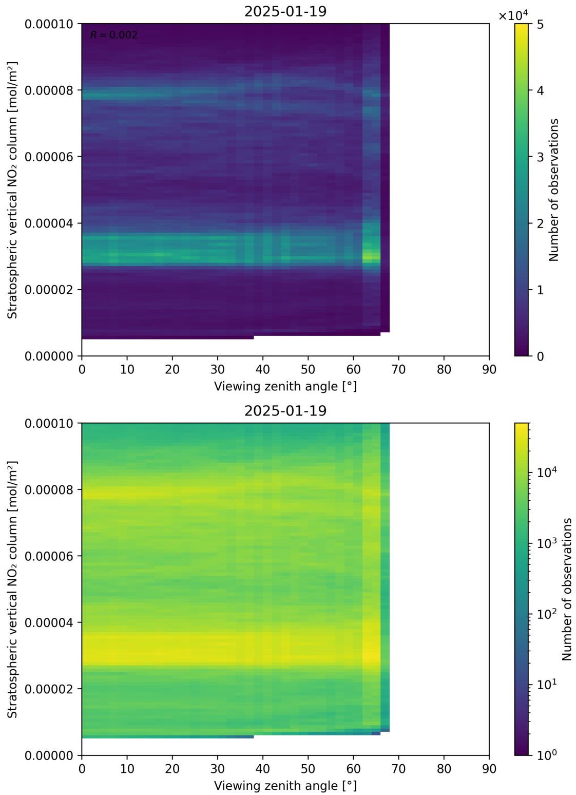
Figure 164: Scatter density plot of “Viewing zenith angle” against “Stratospheric vertical NO 2 column” for 2025-01-18 to 2025-01-20.
