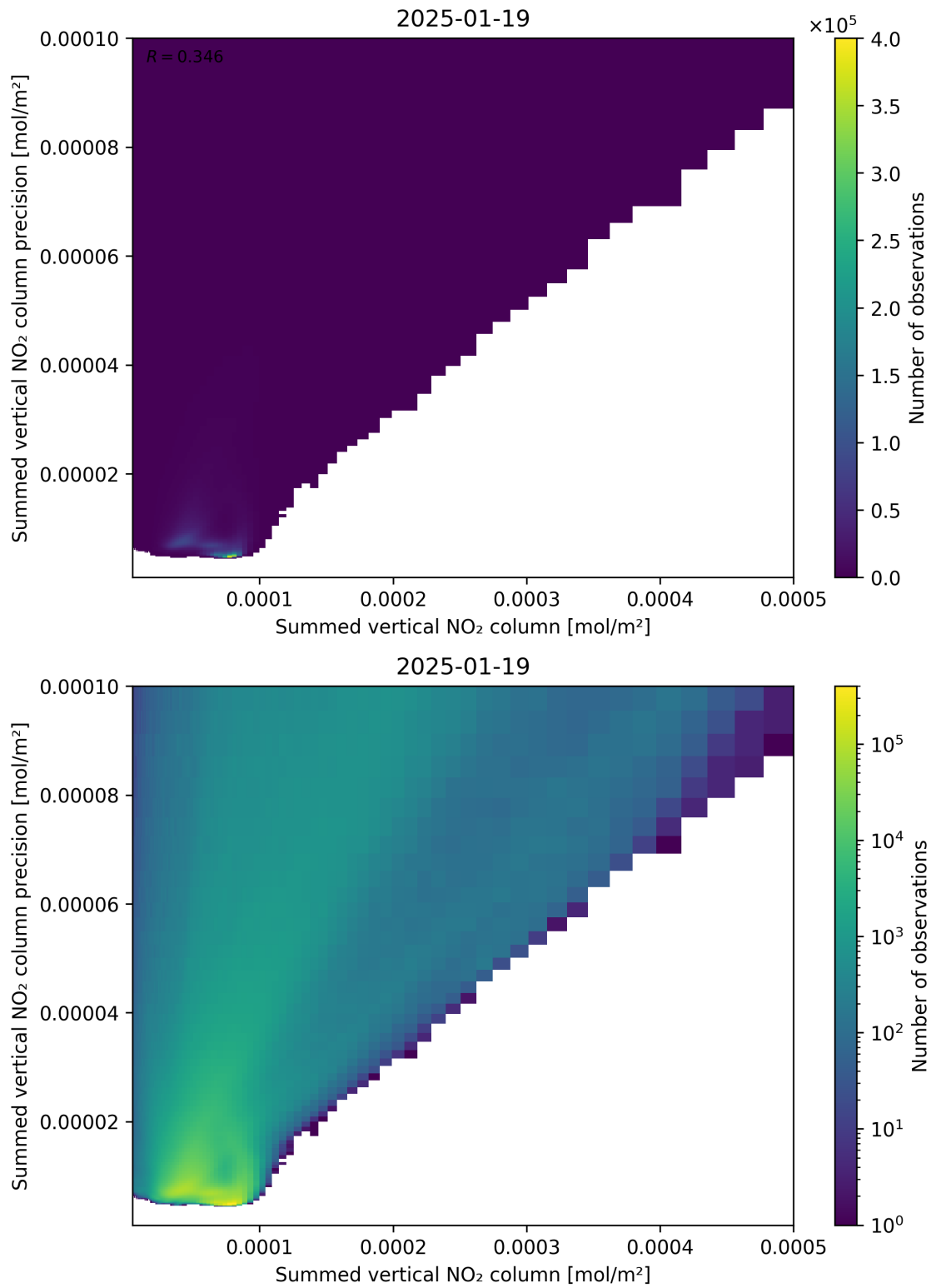
Figure 105: Scatter density plot of “Summed vertical NO 2 column” against “Summed vertical NO 2 column precision” for 2025-01-18 to 2025-01-20.
