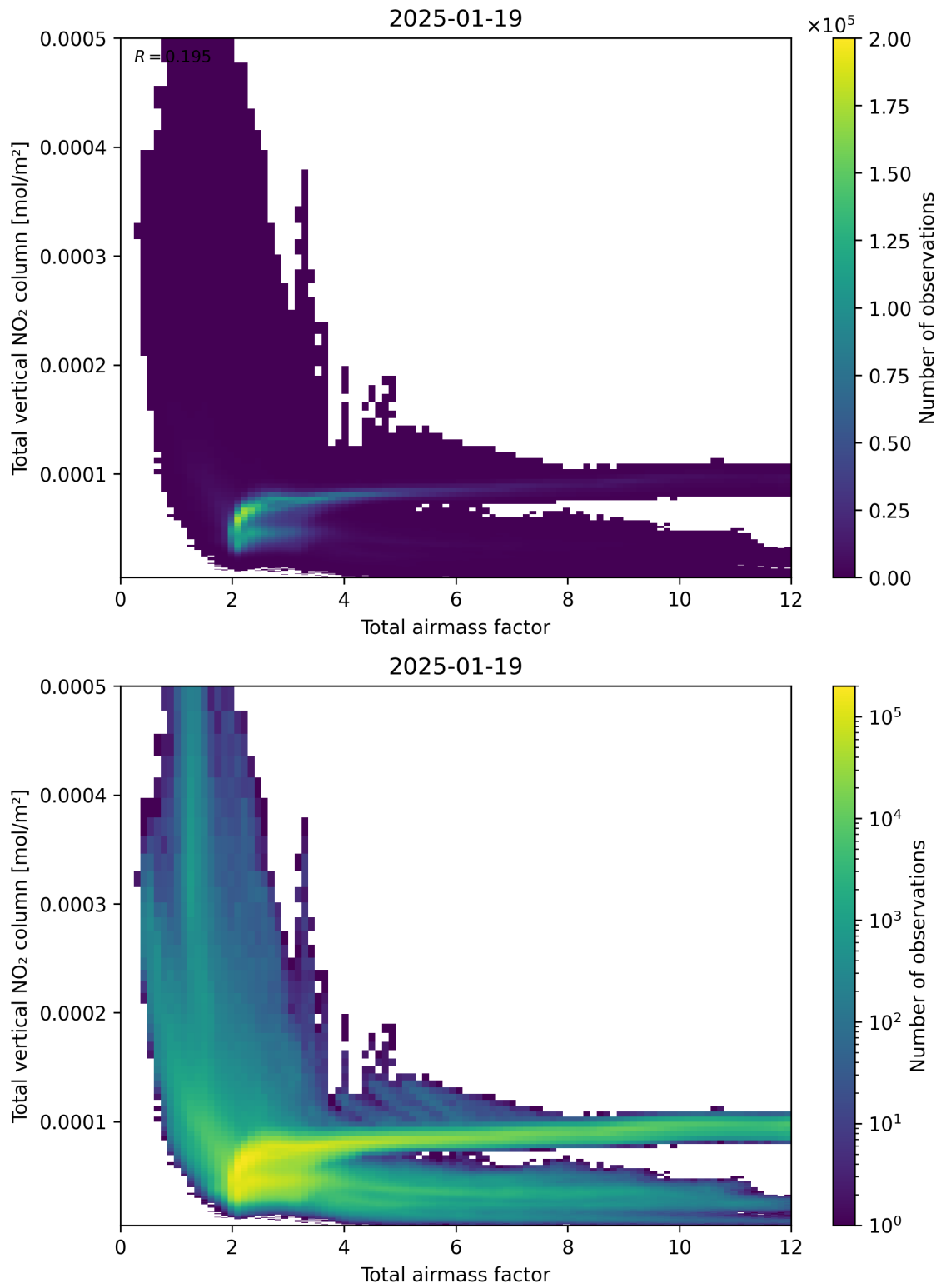
Figure 67: Scatter density plot of “Total air mass factor” against “Total vertical NO 2 column” for 2025-01-18 to 2025-01-20.
