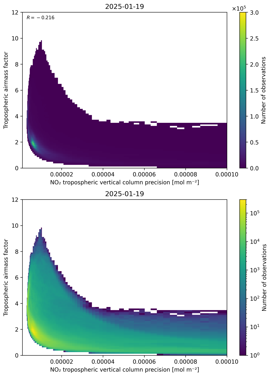
Figure 133: Scatter density plot of “NO 2 tropospheric vertical column precision” against “Tropospheric air mass factor” for 2025-01-18 to 2025-01-20.
