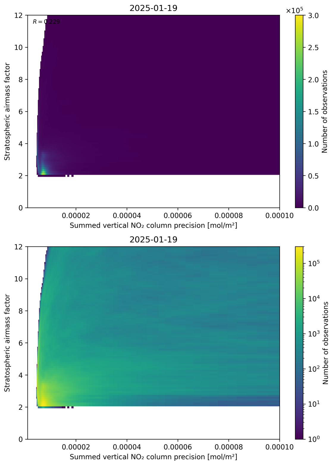
Figure 106: Scatter density plot of “Summed vertical NO 2 column precision” against “Stratospheric airmass factor” for 2025-01-18 to 2025-01-20.
