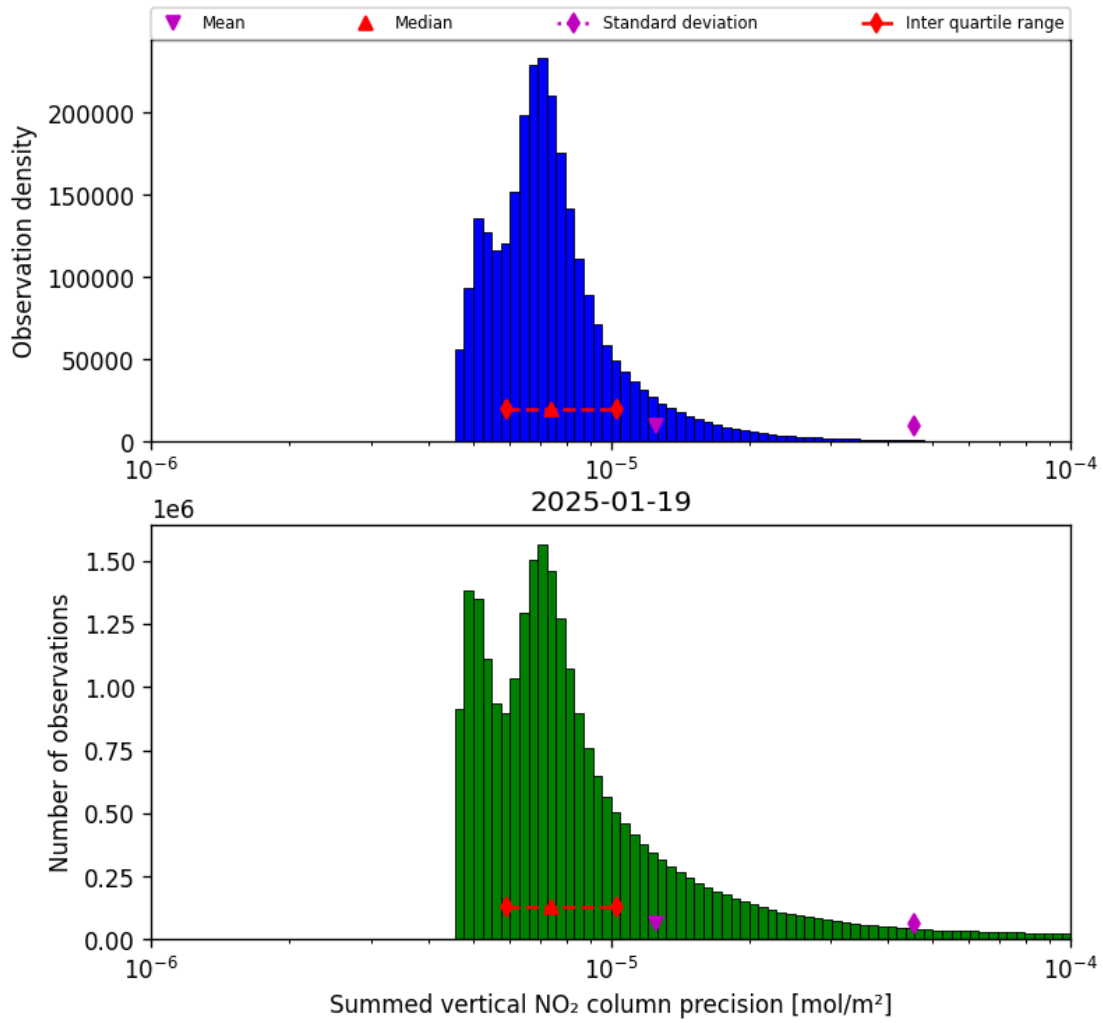
Figure 41: Histogram of “Summed vertical NO 2 column precision” for 2025-01-18 to 2025-01-20
