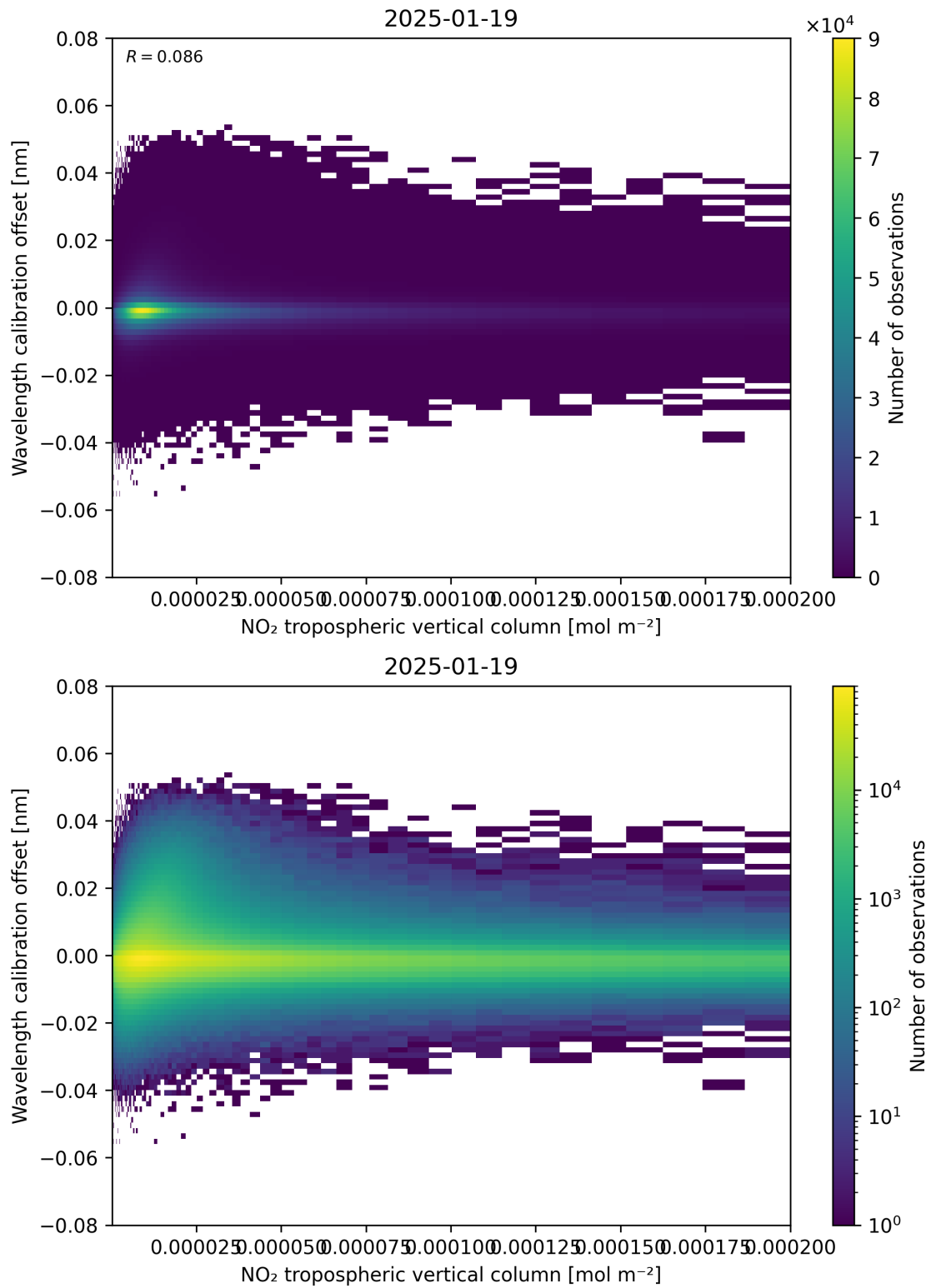
Figure 143: Scatter density plot of “NO 2 tropospheric vertical column” against “Wavelength calibration offset” for 2025-01-18 to 2025-01-20.
