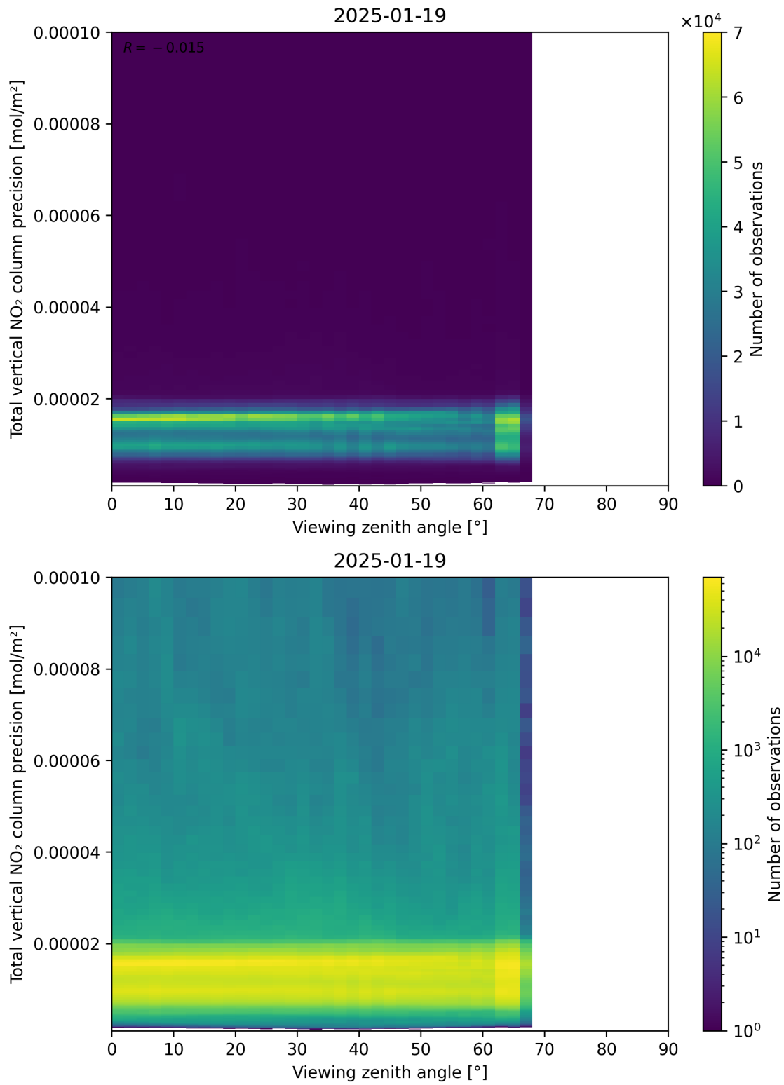
Figure 168: Scatter density plot of “Viewing zenith angle” against “Total vertical NO 2 column precision” for 2025-01-18 to 2025-01-20.
