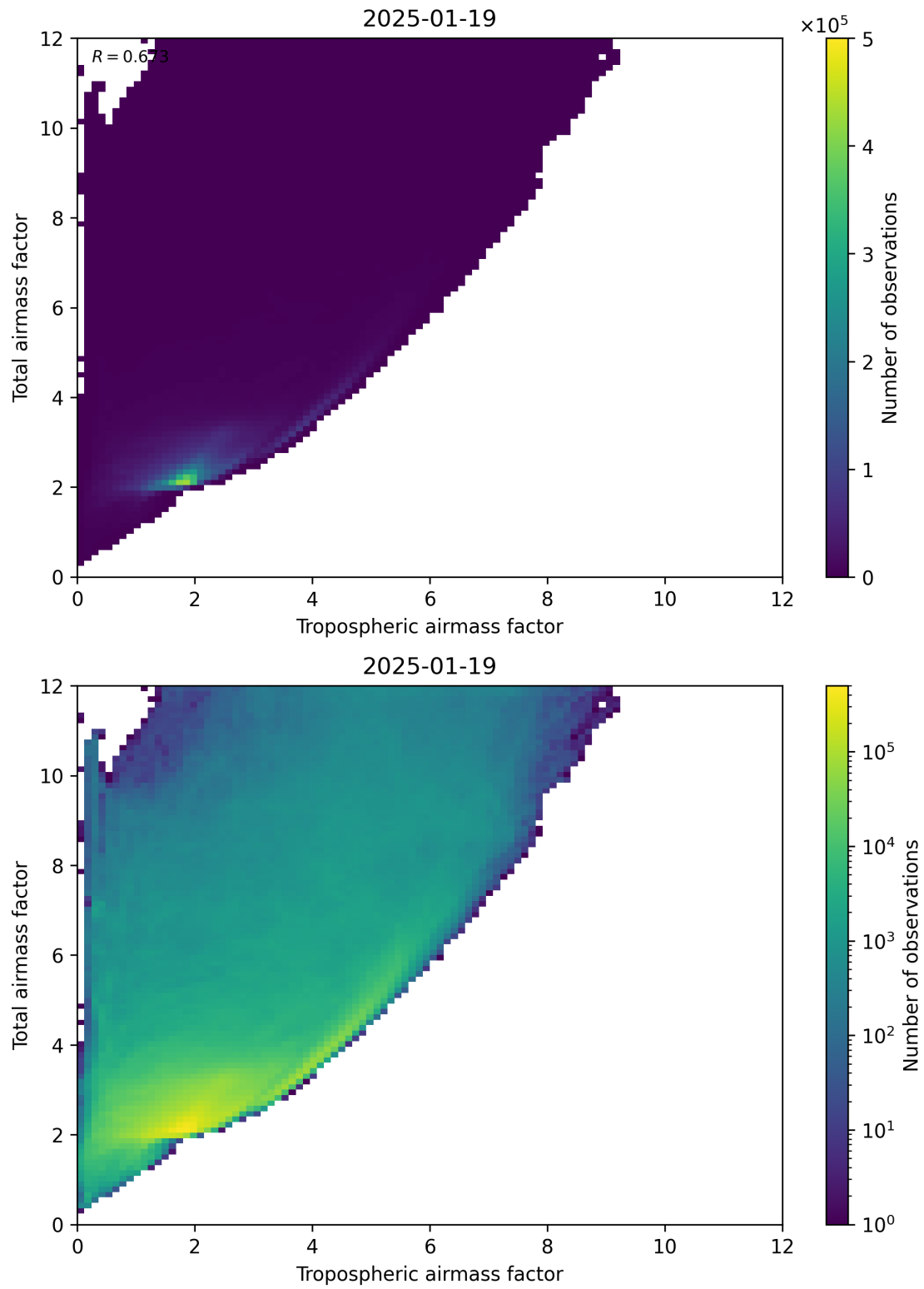
Figure 72: Scatter density plot of “Tropospheric airmass factor” against “Total airmass factor” for 2025-01-18 to 2025-01-20.
