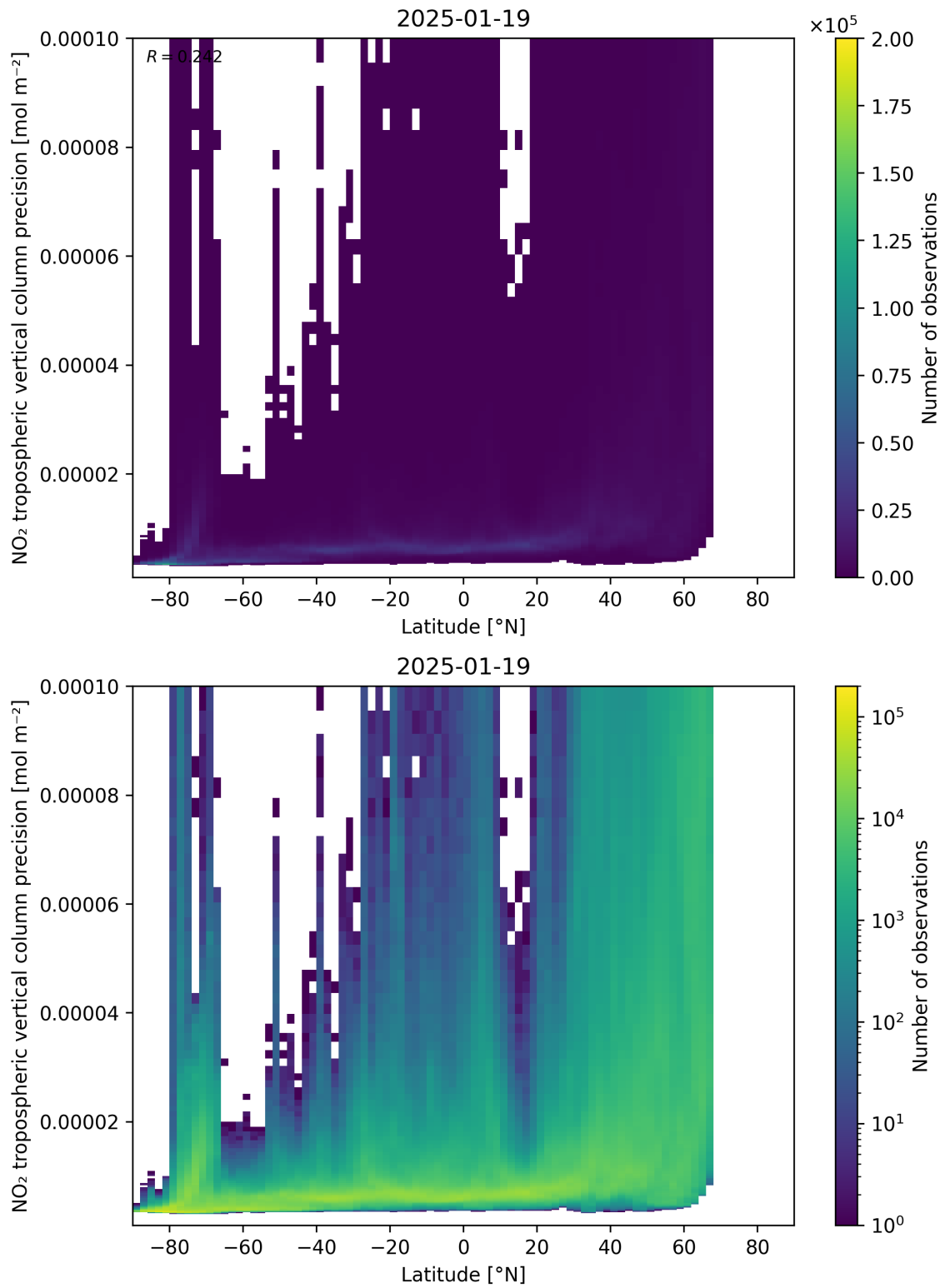
Figure 93: Scatter density plot of “Latitude” against “NO 2 tropospheric vertical column precision” for 2025-01-18 to 2025-01-20.
