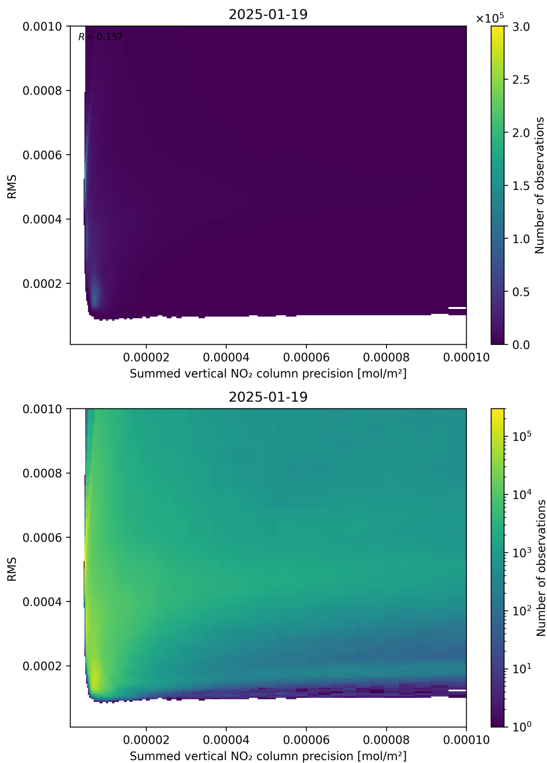
Figure 108: Scatter density plot of “Summed vertical NO 2 column precision” against “RMS” for 2025-01-18 to 2025-01-20.
