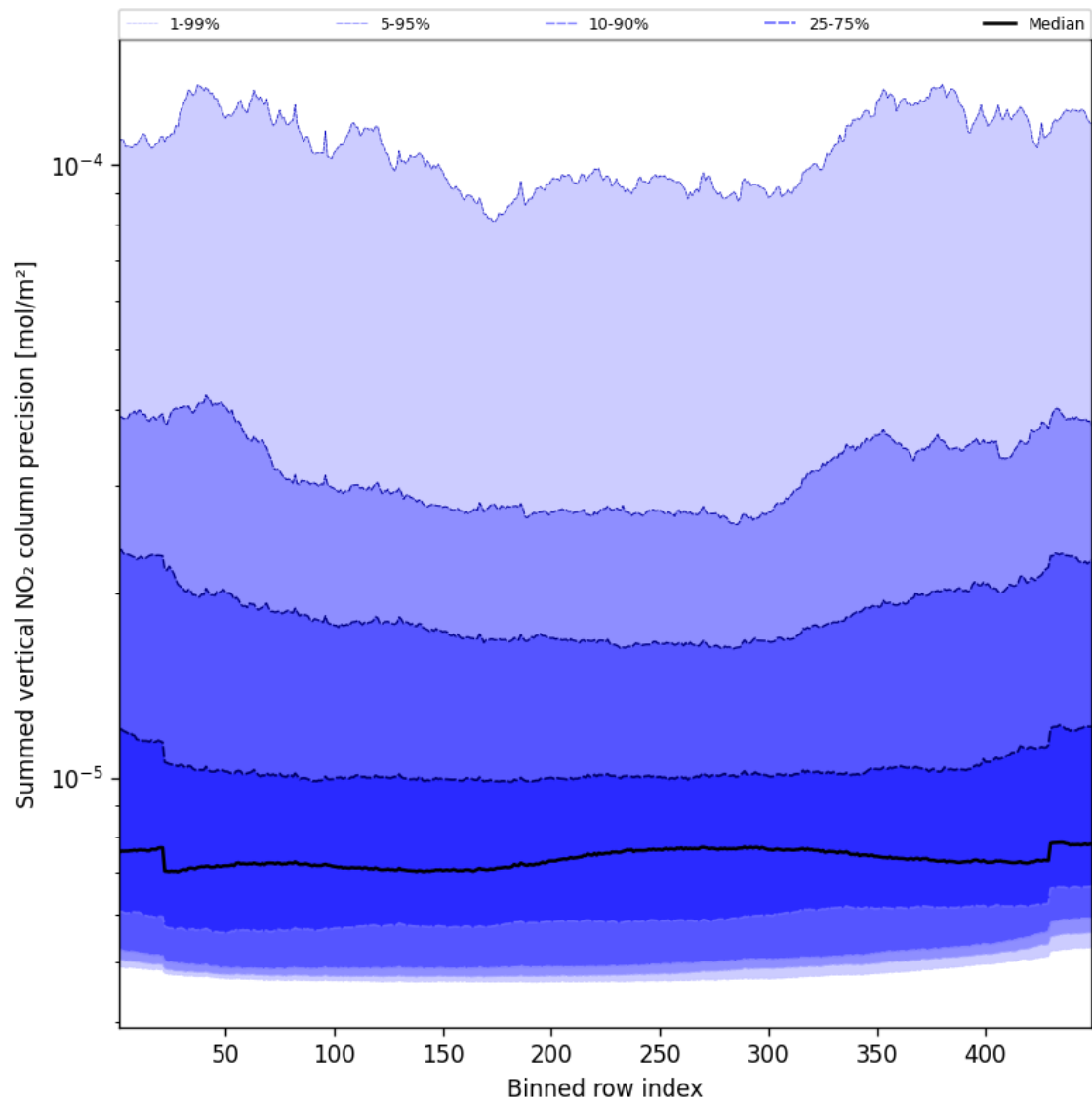
Figure 58: Along track statistics of “Summed vertical NO 2 column precision” for 2025-01-18 to 2025-01-20
