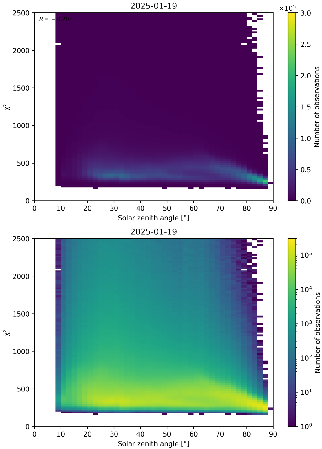
Figure 148: Scatter density plot of “Solar zenith angle” against “ \chi^2 ” for 2025-01-18 to 2025-01-20.
