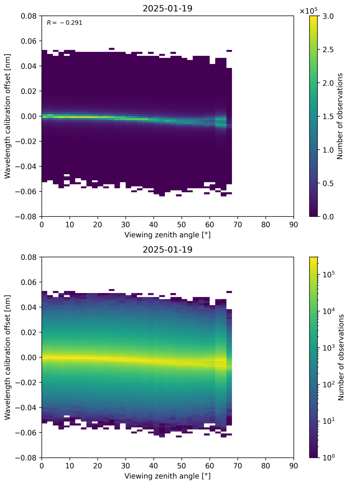
Figure 173: Scatter density plot of “Viewing zenith angle” against “Wavelength calibration offset” for 2025-01-18 to 2025-01-20.
