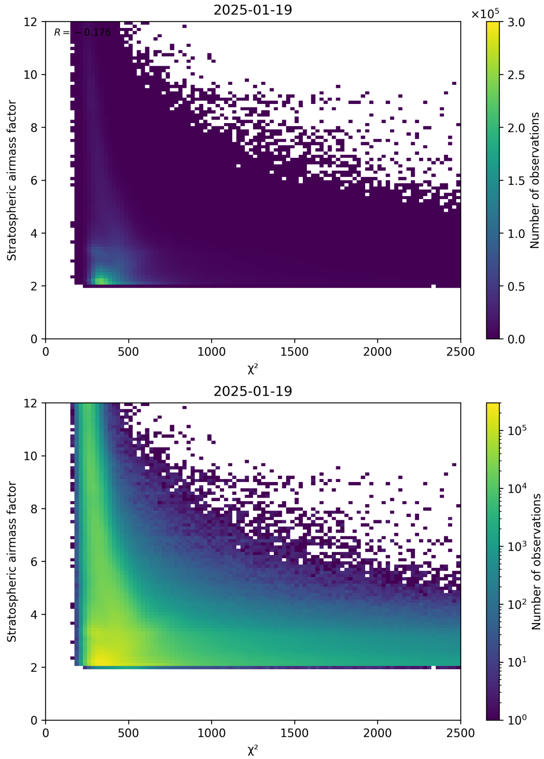
Figure 81: Scatter density plot of “ \chi^2 ” against “Stratospheric airmass factor” for 2025-01-18 to 2025-01-20.
