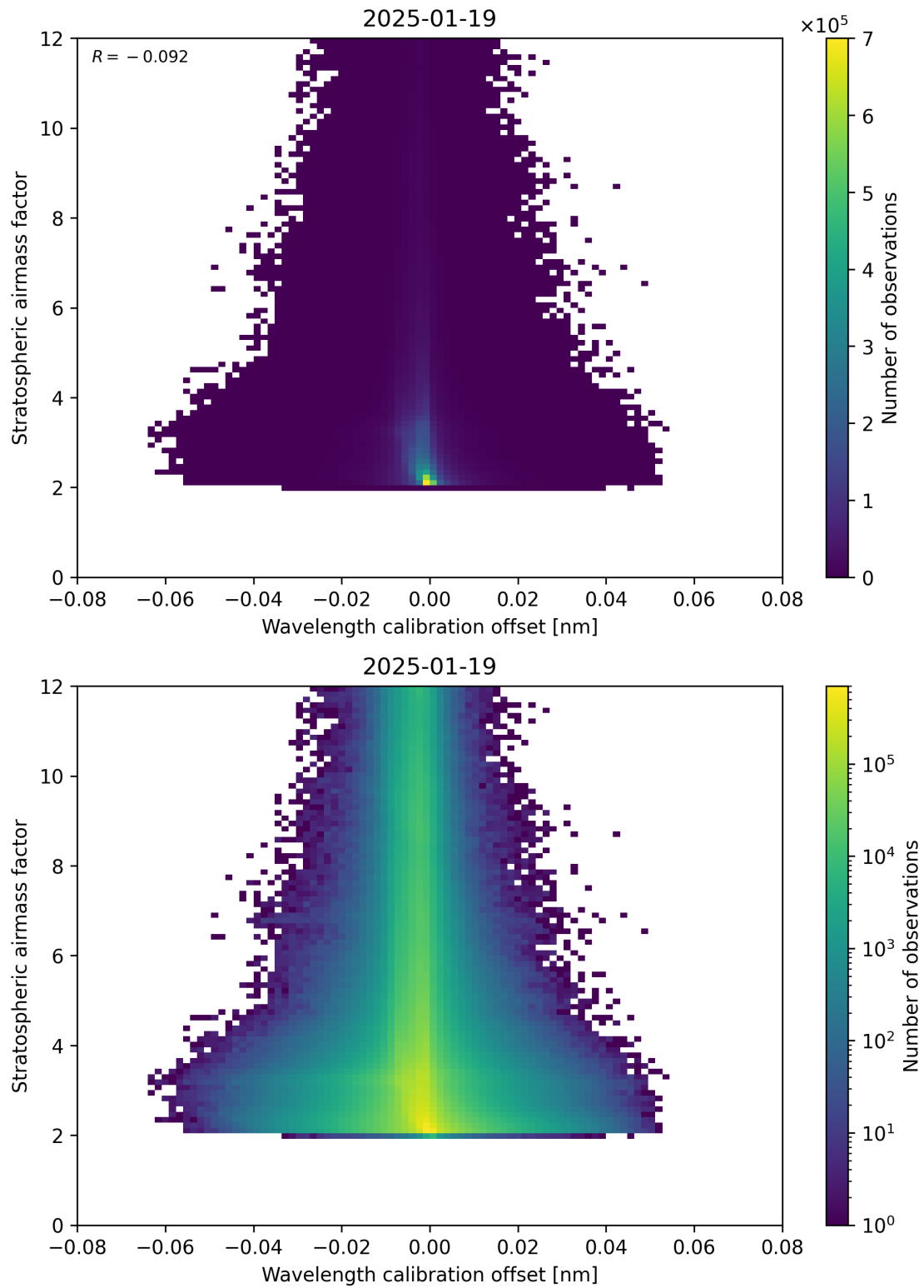
Figure 174: Scatter density plot of “Wavelength calibration offset” against “Stratospheric airmass factor” for 2025-01-18 to 2025-01-20.
