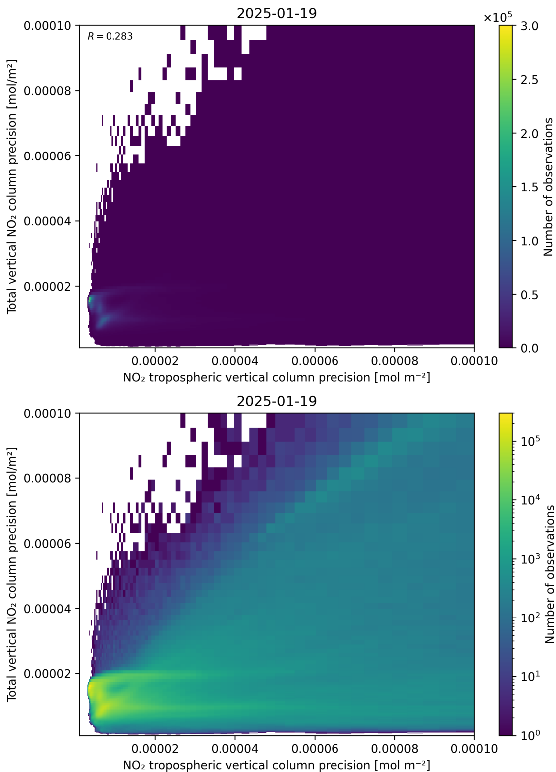
Figure 139: Scatter density plot of “NO 2 tropospheric vertical column precision” against “Total vertical NO 2 column precision” for 2025-01-18 to 2025-01-20.
