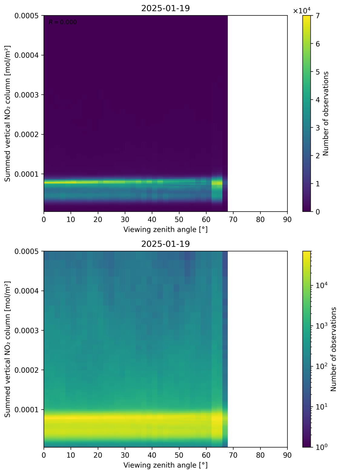
Figure 165: Scatter density plot of “Viewing zenith angle” against “Summed vertical NO 2 column” for 2025-01-18 to 2025-01-20.
