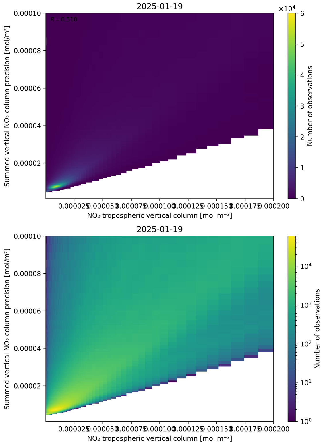
Figure 127: Scatter density plot of “NO 2 tropospheric vertical column” against “Summed vertical NO 2 column precision” for 2025-01-18 to 2025-01-20.
