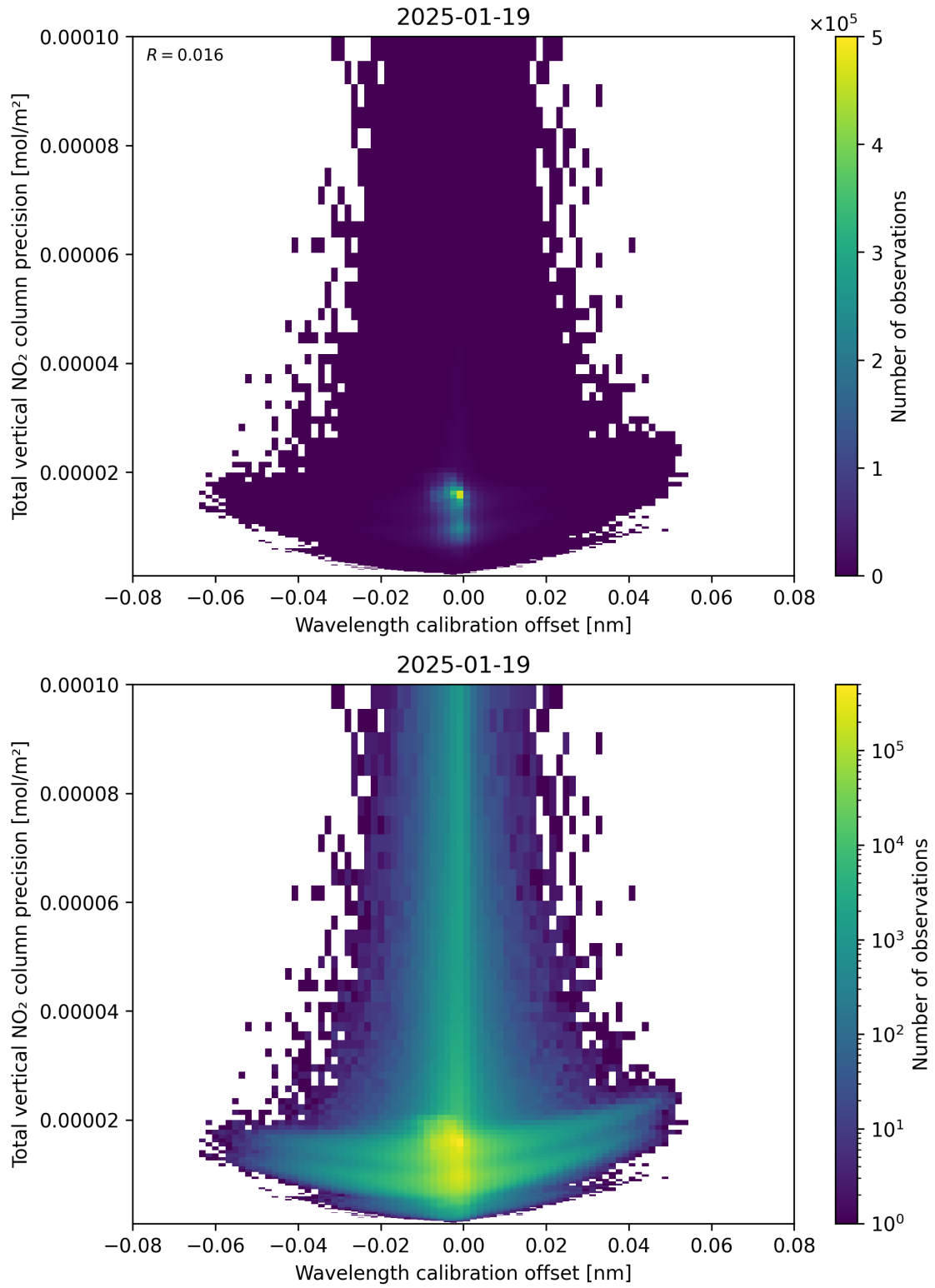
Figure 180: Scatter density plot of “Wavelength calibration offset” against “Total vertical NO 2 column precision” for 2025-01-18 to 2025-01-20.
