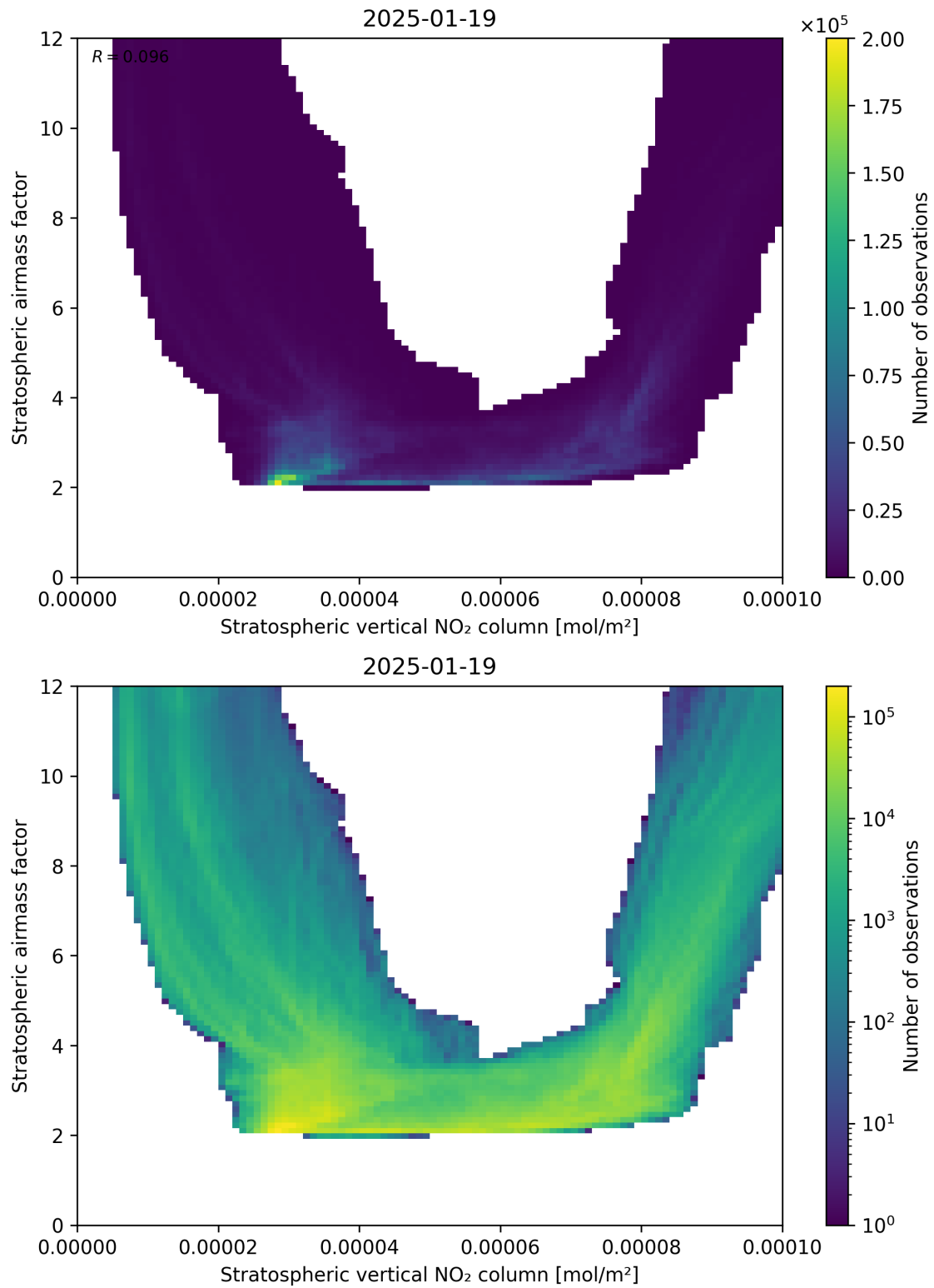
Figure 96: Scatter density plot of “Stratospheric vertical NO 2 column” against “Stratospheric airmass factor” for 2025-01-18 to 2025-01-20.
