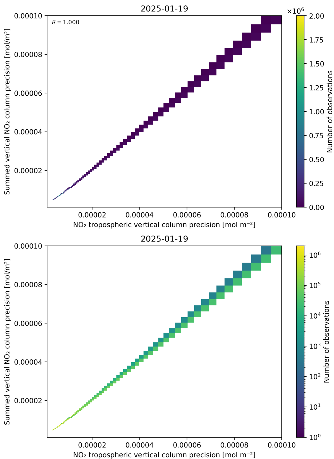
Figure 137: Scatter density plot of “NO 2 tropospheric vertical column precision” against “Summed vertical NO 2 column precision” for 2025-01-18 to 2025-01-20.
