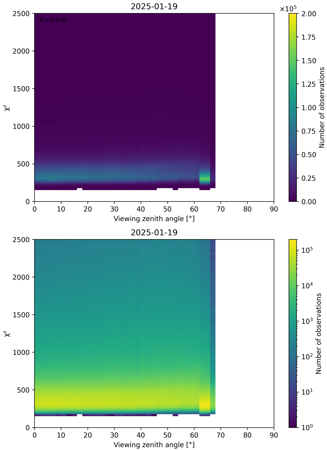
Figure 162: Scatter density plot of “Viewing zenith angle” against “ \chi^2 ” for 2025-01-18 to 2025-01-20.
