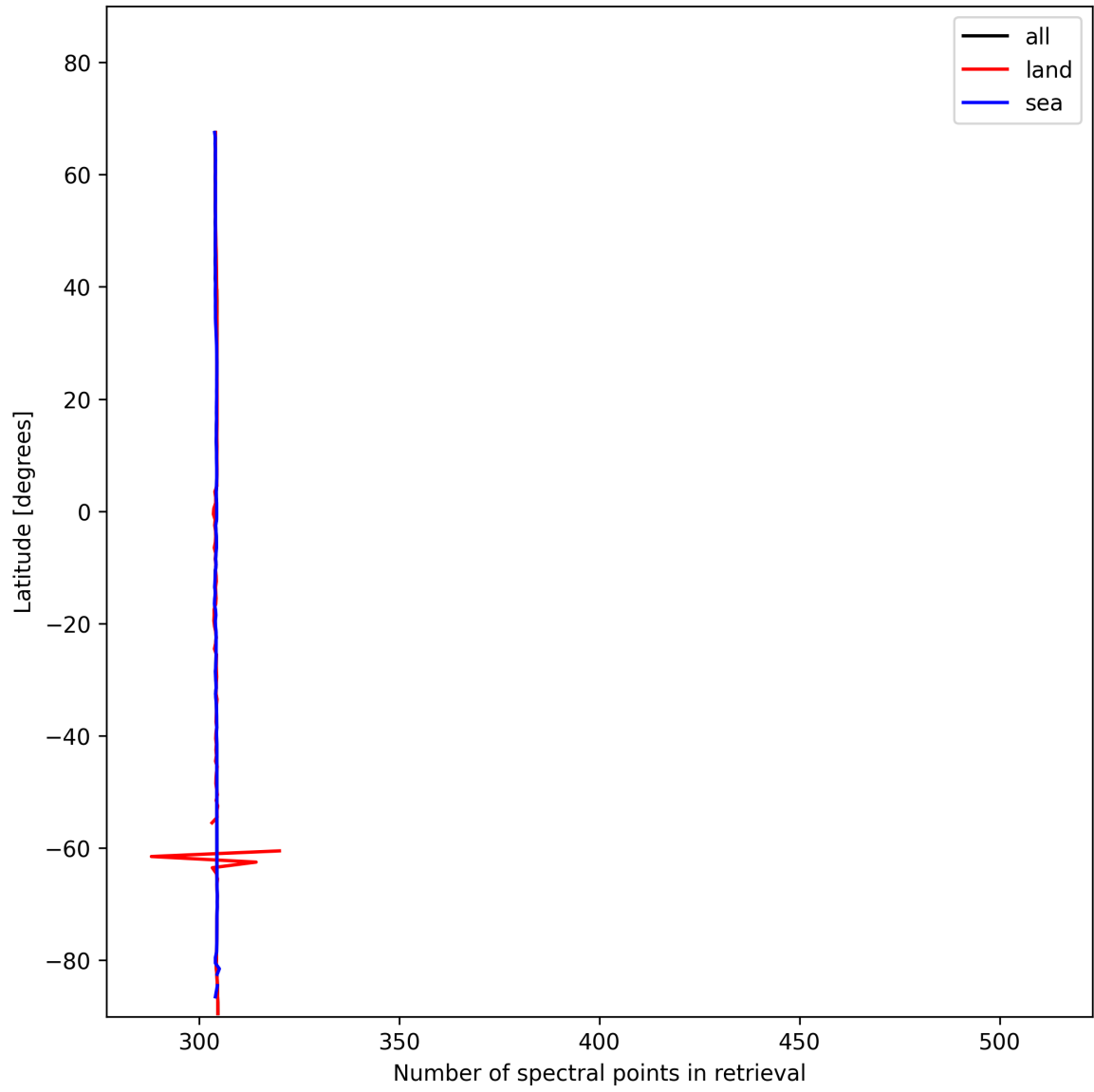
Figure 16: Zonal average of “Number of spectral points in retrieval” for 2025-01-18 to 2025-01-20.
