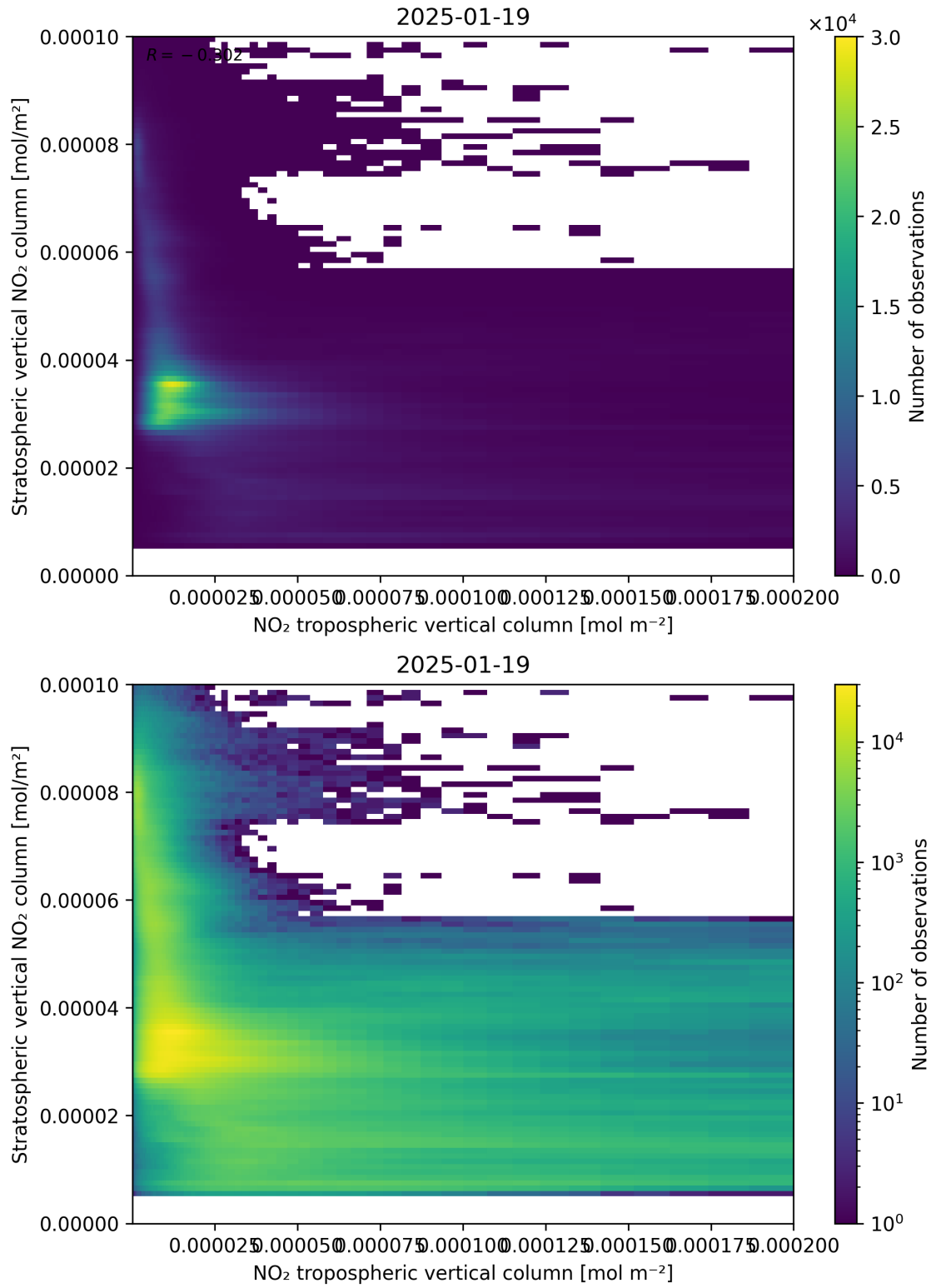
Figure 125: Scatter density plot of “NO 2 tropospheric vertical column” against “Stratospheric vertical NO 2 column” for 2025-01-18 to 2025-01-20.
