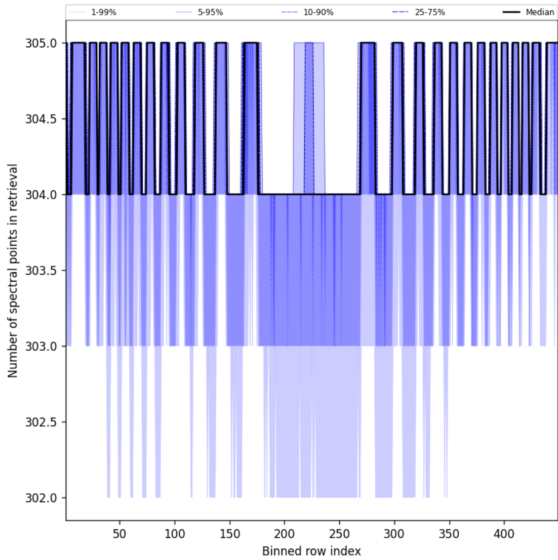
Figure 50: Along track statistics of “Number of spectral points in retrieval” for 2025-01-18 to 2025-01-20
