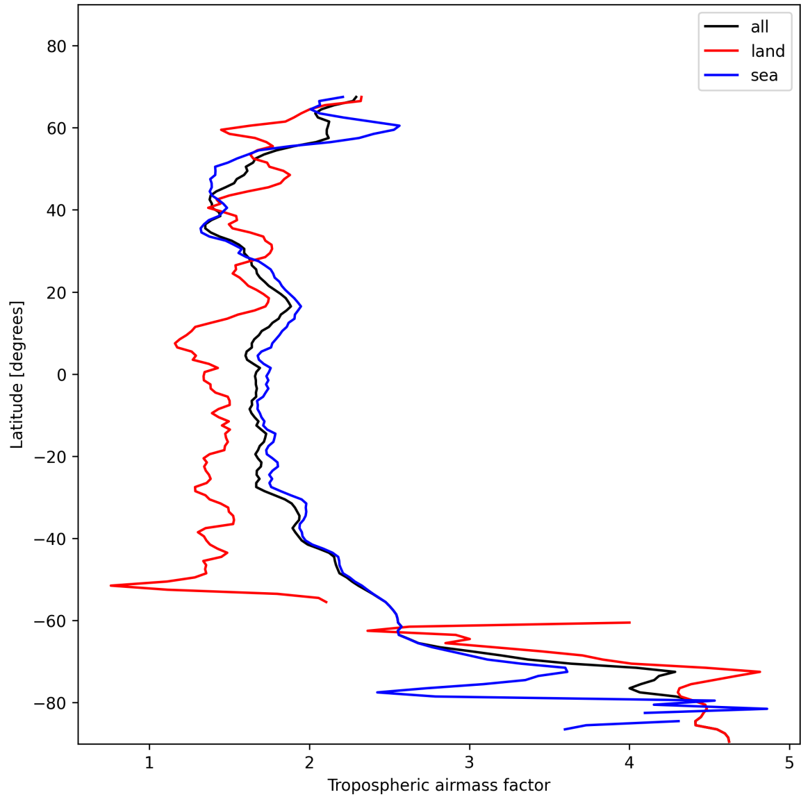
Figure 14: Zonal average of “Tropospheric airmass factor” for 2025-01-18 to 2025-01-20.
