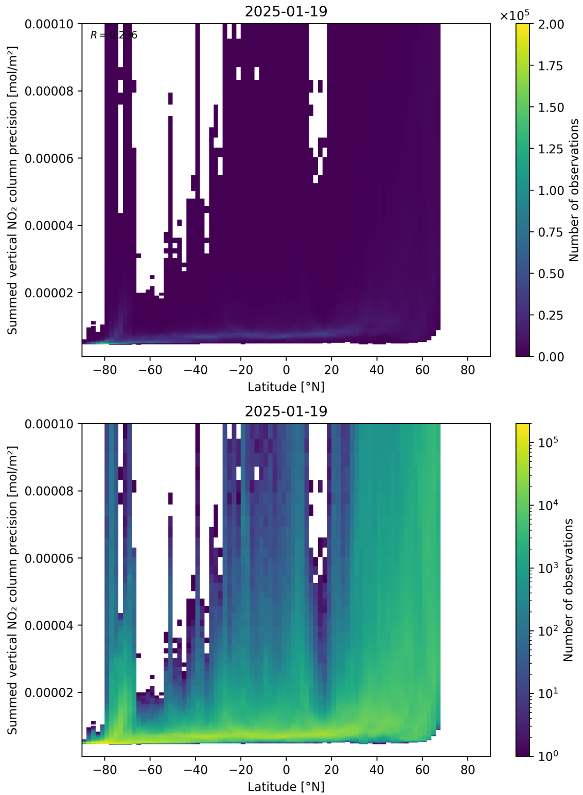
Figure 89: Scatter density plot of “Latitude” against “Summed vertical NO 2 column precision” for 2025-01-18 to 2025-01-20.
