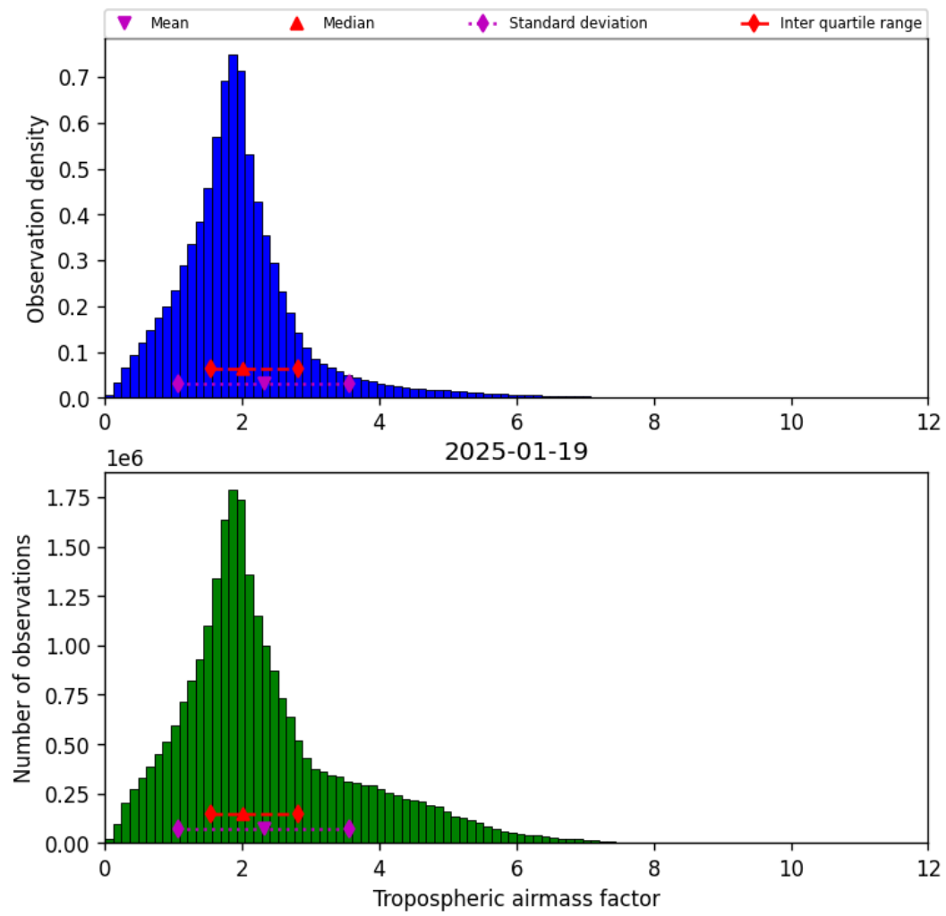
Figure 31: Histogram of “Tropospheric airmass factor” for 2025-01-18 to 2025-01-20
