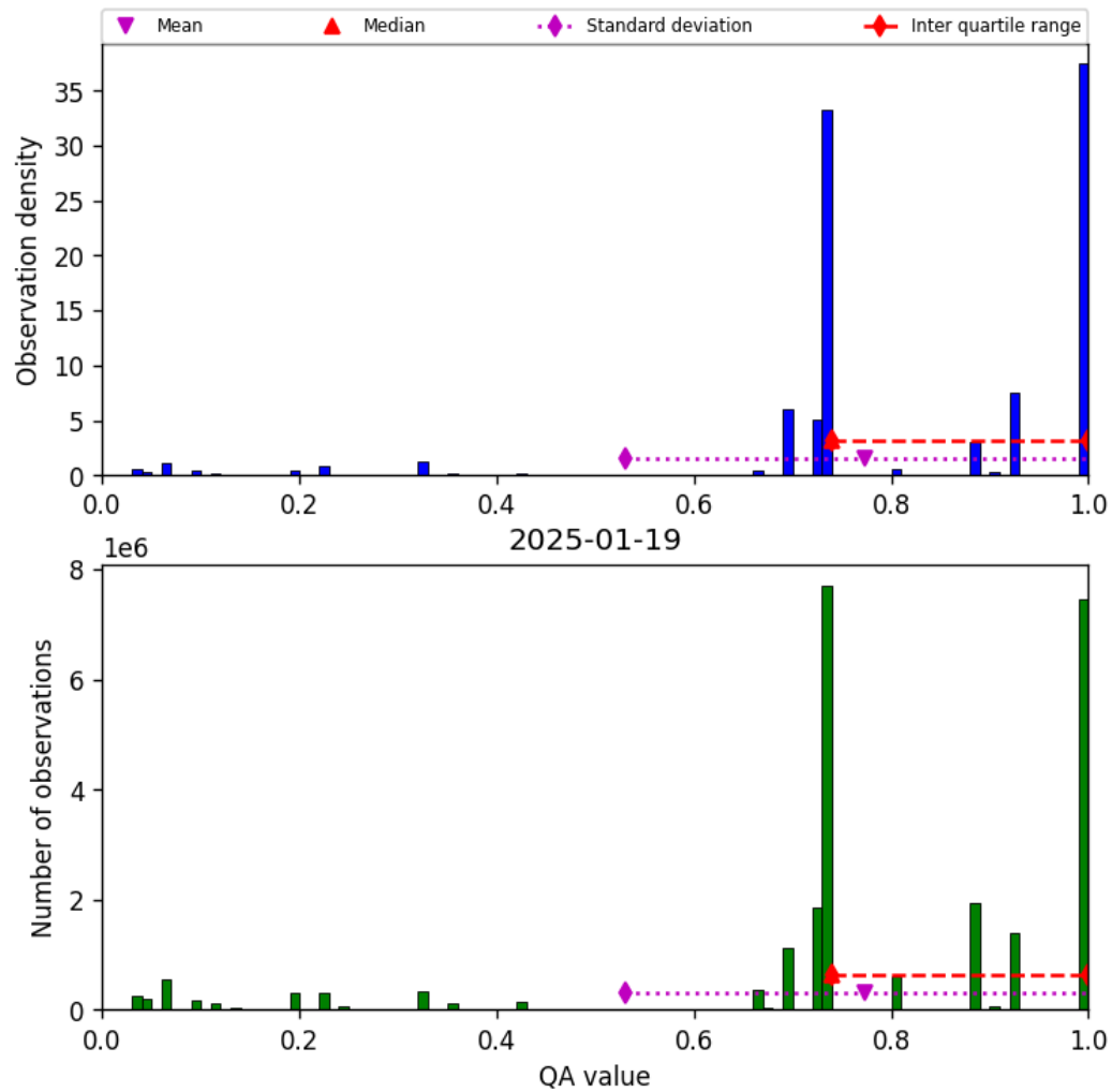
Figure 28: Histogram of “QA value” for 2025-01-18 to 2025-01-20
