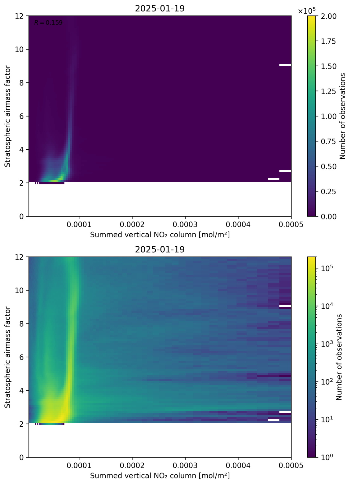
Figure 103: Scatter density plot of “Summed vertical NO 2 column” against “Stratospheric airmass factor” for 2025-01-18 to 2025-01-20.
