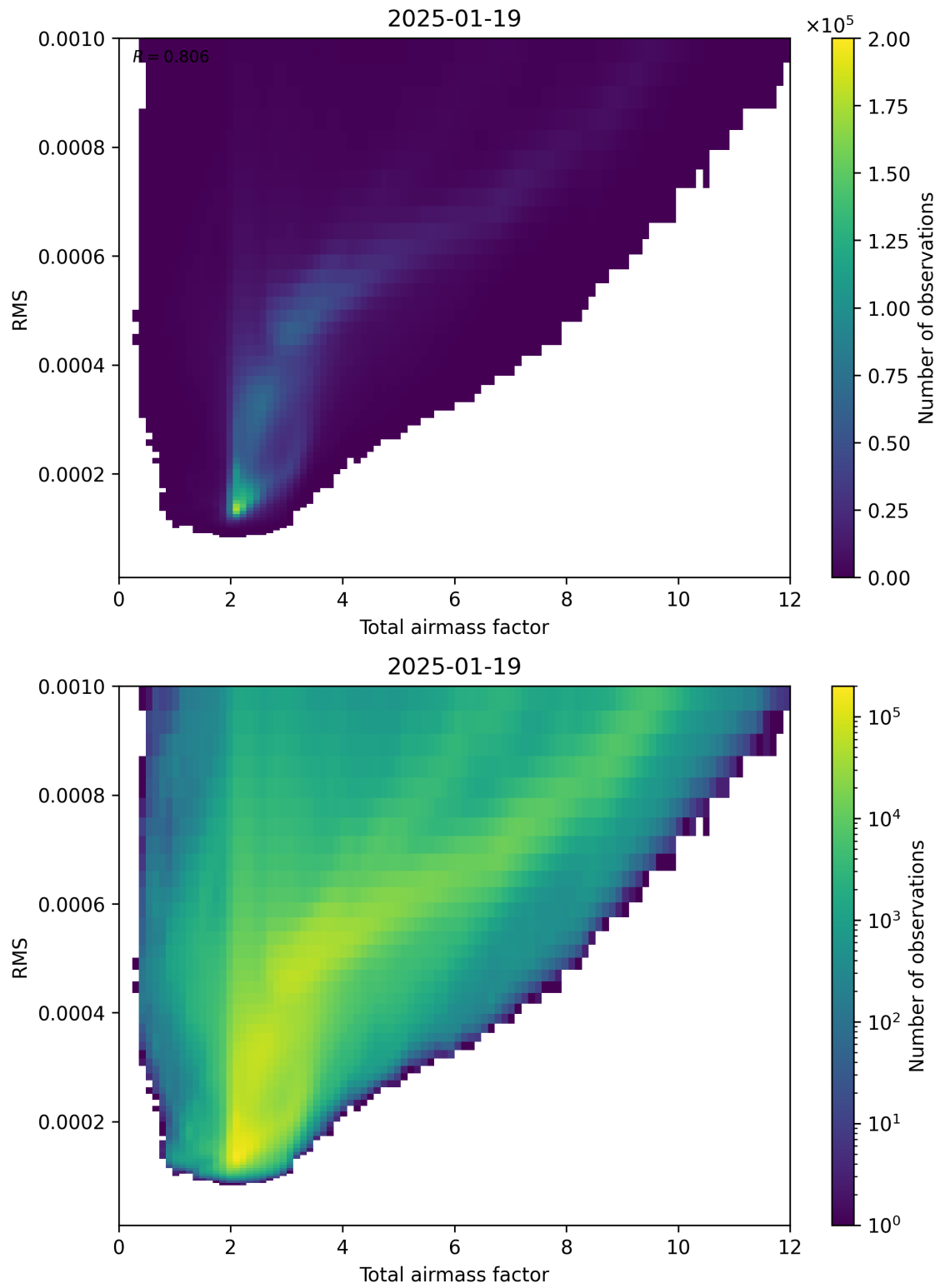
Figure 69: Scatter density plot of “Total airmass factor” against “RMS” for 2025-01-18 to 2025-01-20.
