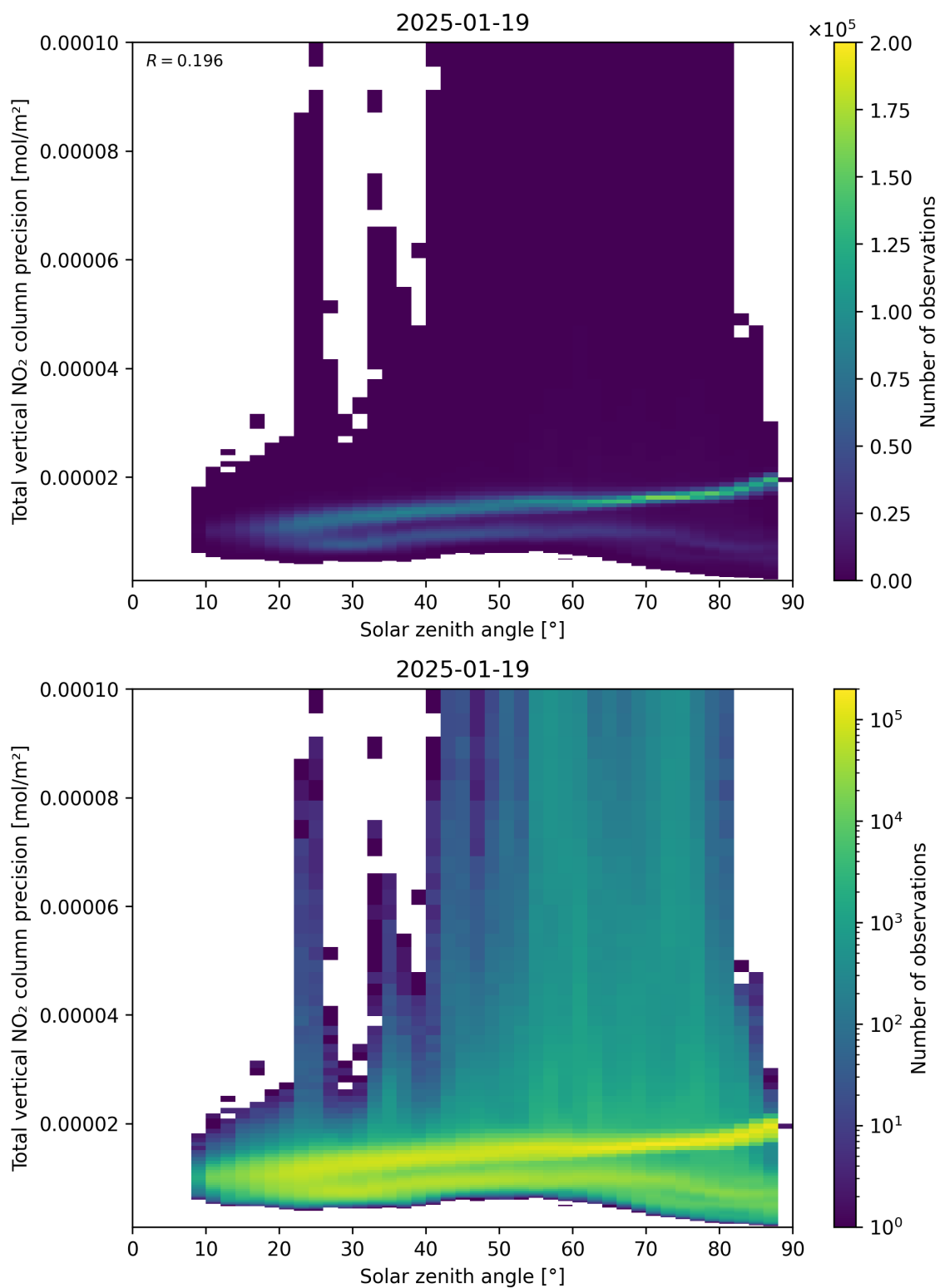
Figure 154: Scatter density plot of “Solar zenith angle” against “Total vertical NO 2 column precision” for 2025-01-18 to 2025-01-20.
