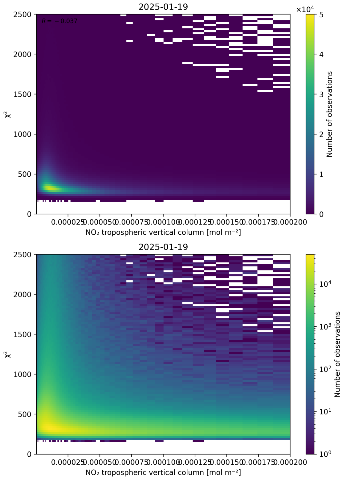
Figure 124: Scatter density plot of “NO 2 tropospheric vertical column” against “ \chi^2 ” for 2025-01-18 to 2025-01-20.
