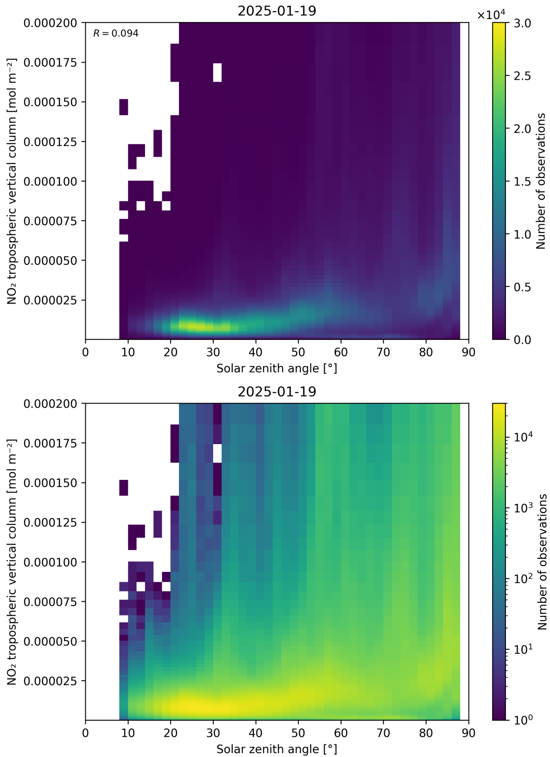
Figure 155: Scatter density plot of “Solar zenith angle” against “NO 2 tropospheric vertical column” for 2025-01-18 to 2025-01-20.
