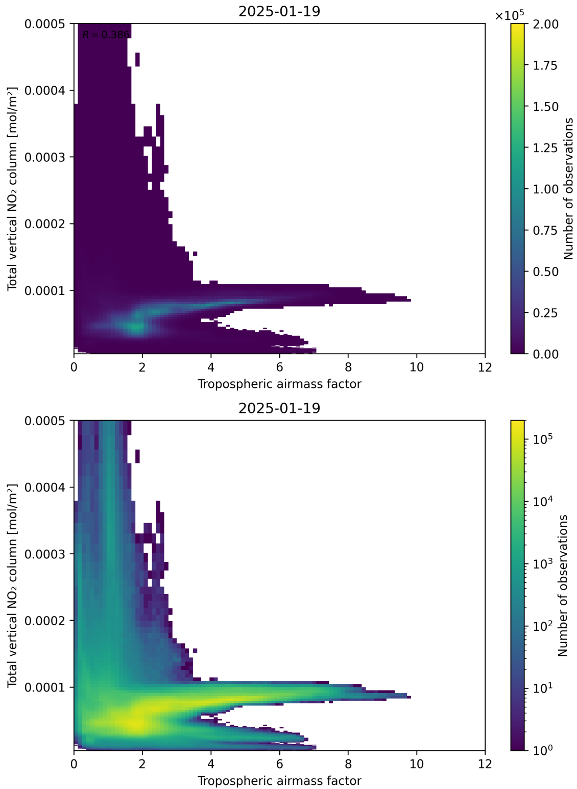
Figure 77: Scatter density plot of “Tropospheric airmass factor” against “Total vertical NO 2 column” for 2025-01-18 to 2025-01-20.
