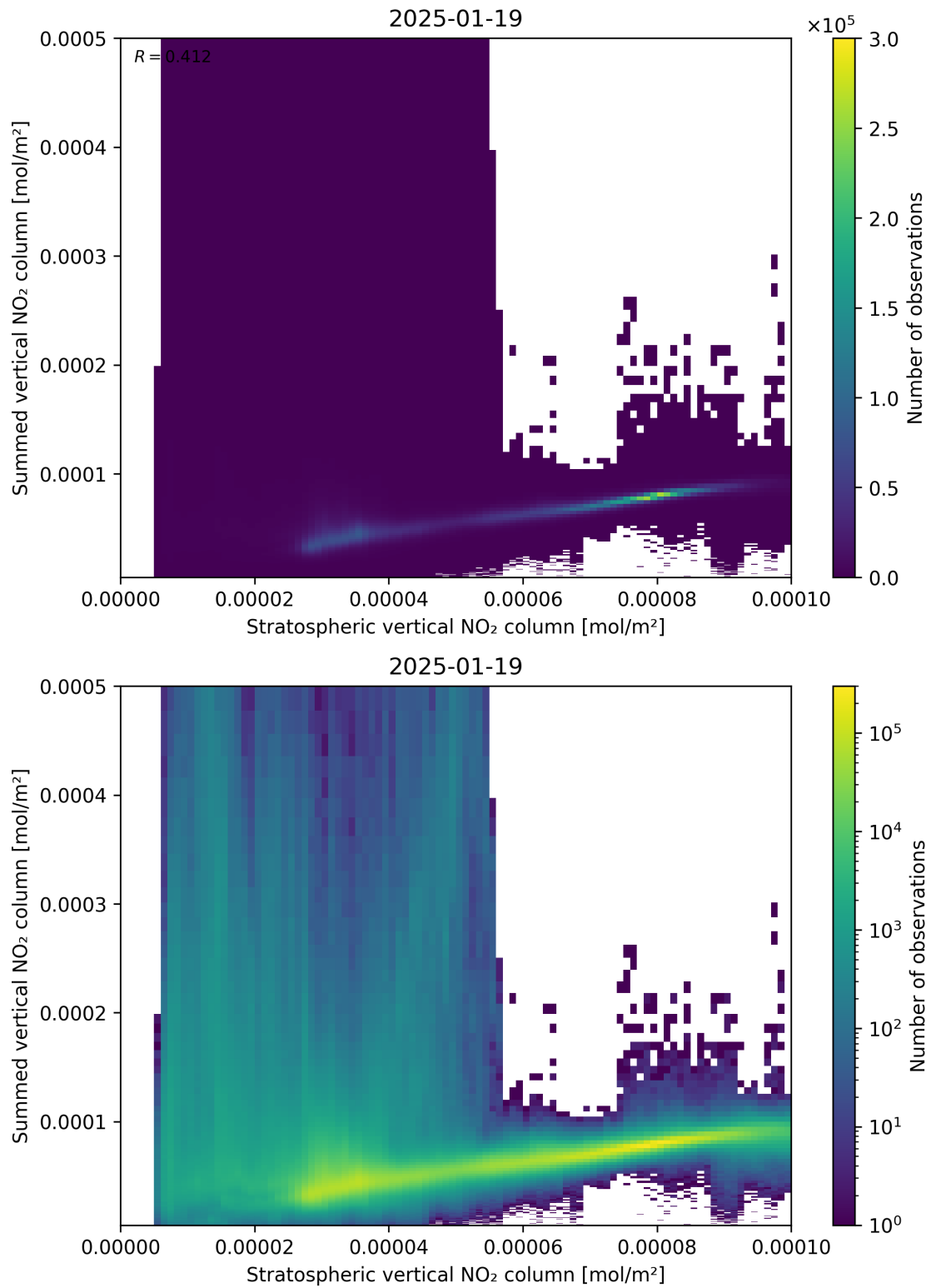
Figure 98: Scatter density plot of “Stratospheric vertical NO 2 column” against “Summed vertical NO 2 column” for 2025-01-18 to 2025-01-20.
