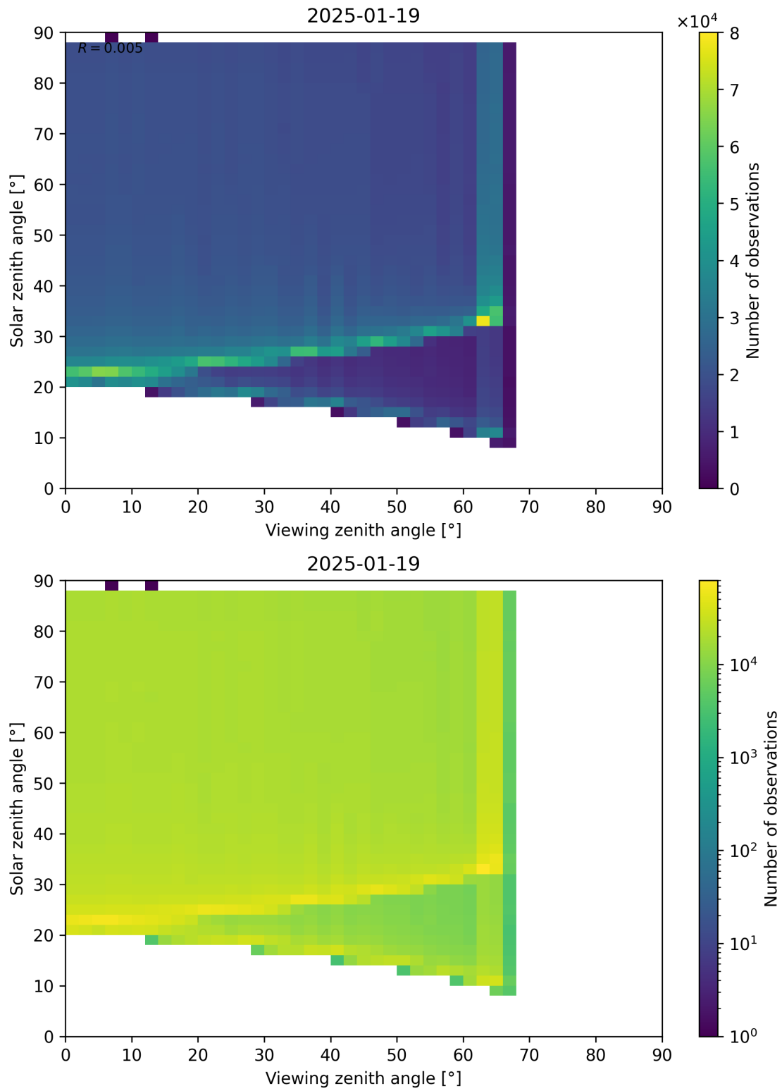
Figure 172: Scatter density plot of “Viewing zenith angle” against “Solar zenith angle” for 2025-01-18 to 2025-01-20.
