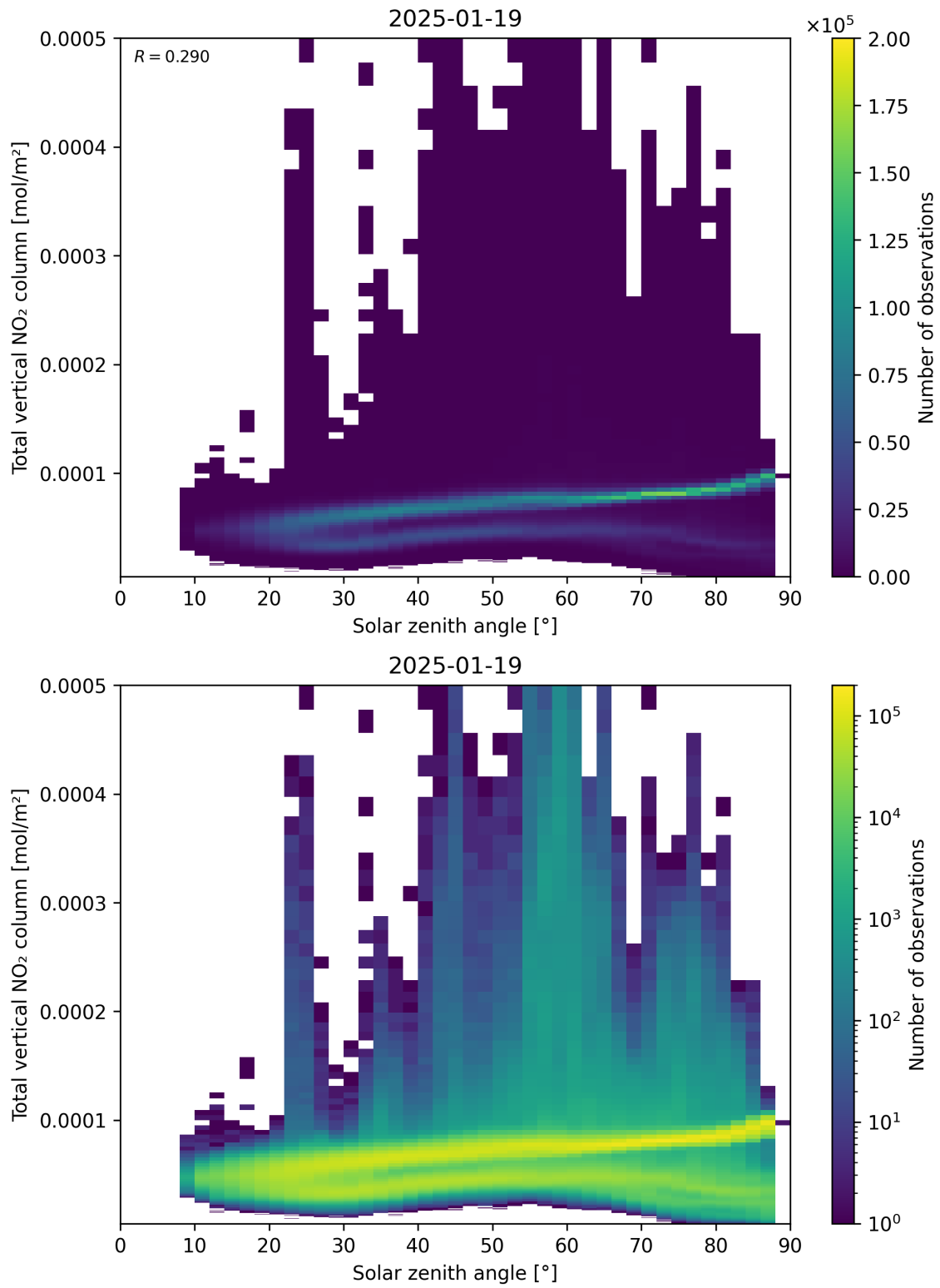
Figure 153: Scatter density plot of “Solar zenith angle” against “Total vertical NO 2 column” for 2025-01-18 to 2025-01-20.
