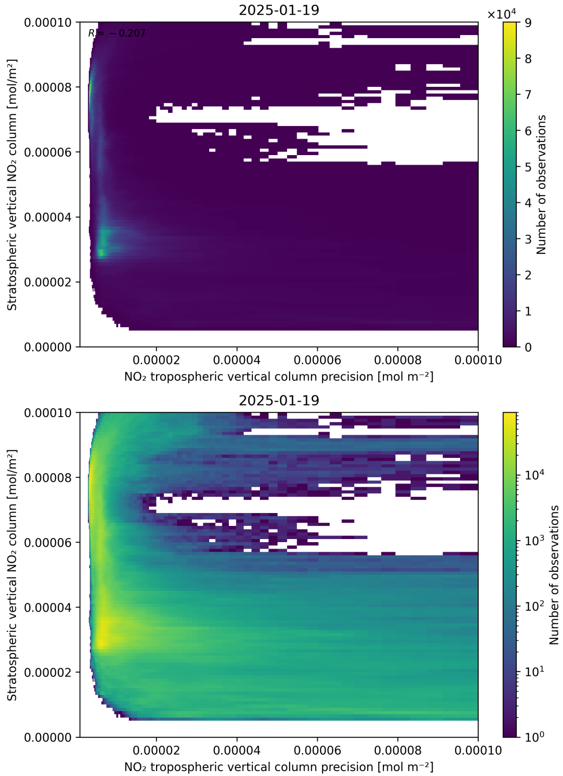
Figure 135: Scatter density plot of “NO 2 tropospheric vertical column precision” against “Stratospheric vertical NO 2 column” for 2025-01-18 to 2025-01-20.
