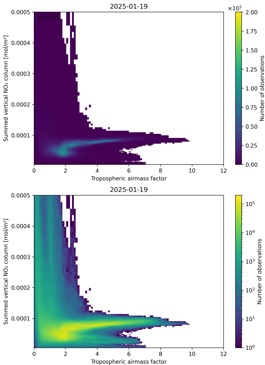
Figure 75: Scatter density plot of “Tropospheric airmass factor” against “Summed vertical NO 2 column” for 2025-01-18 to 2025-01-20.
