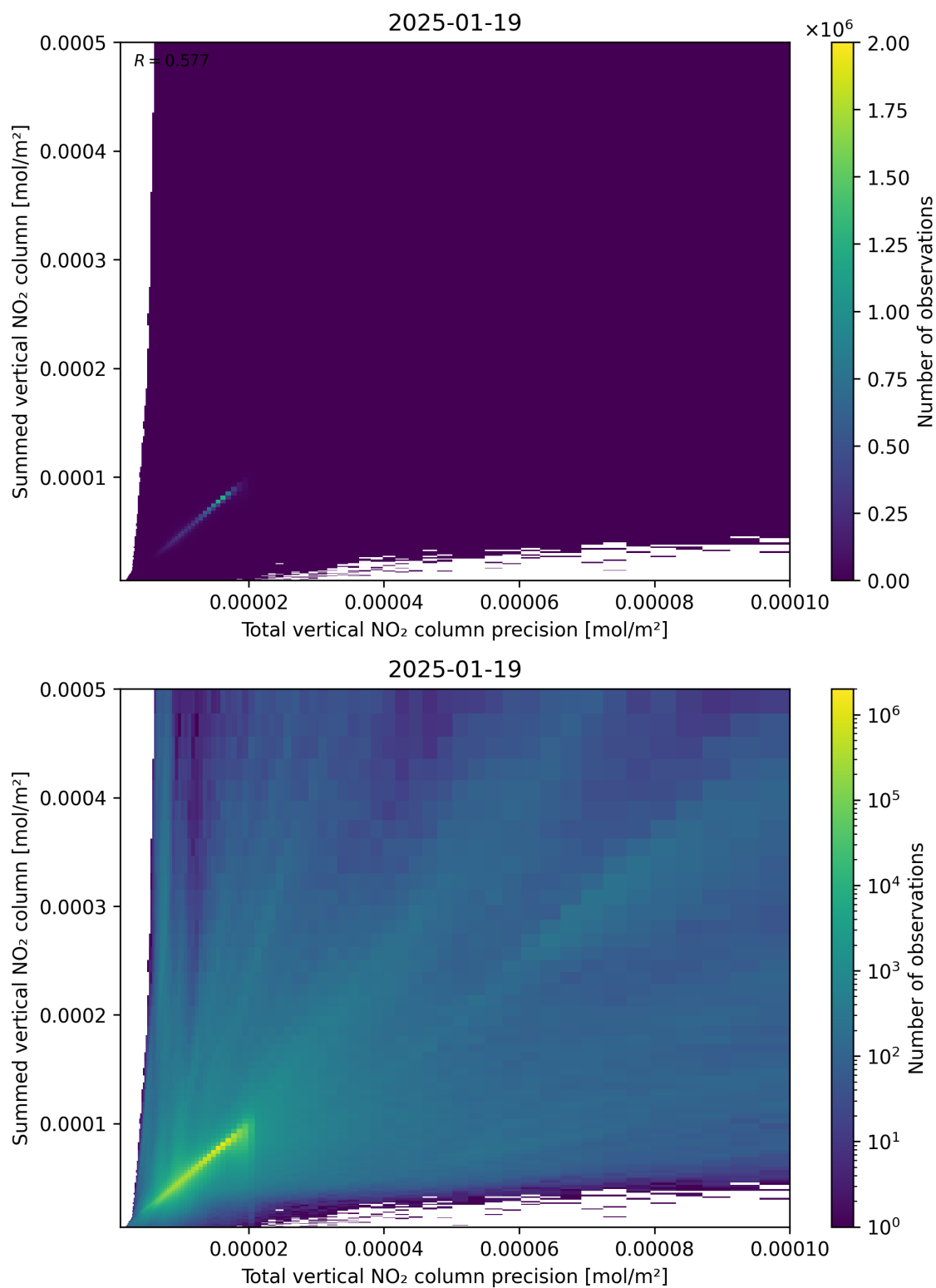
Figure 117: Scatter density plot of “Total vertical NO 2 column precision” against “Summed vertical NO 2 column” for 2025-01-18 to 2025-01-20.
