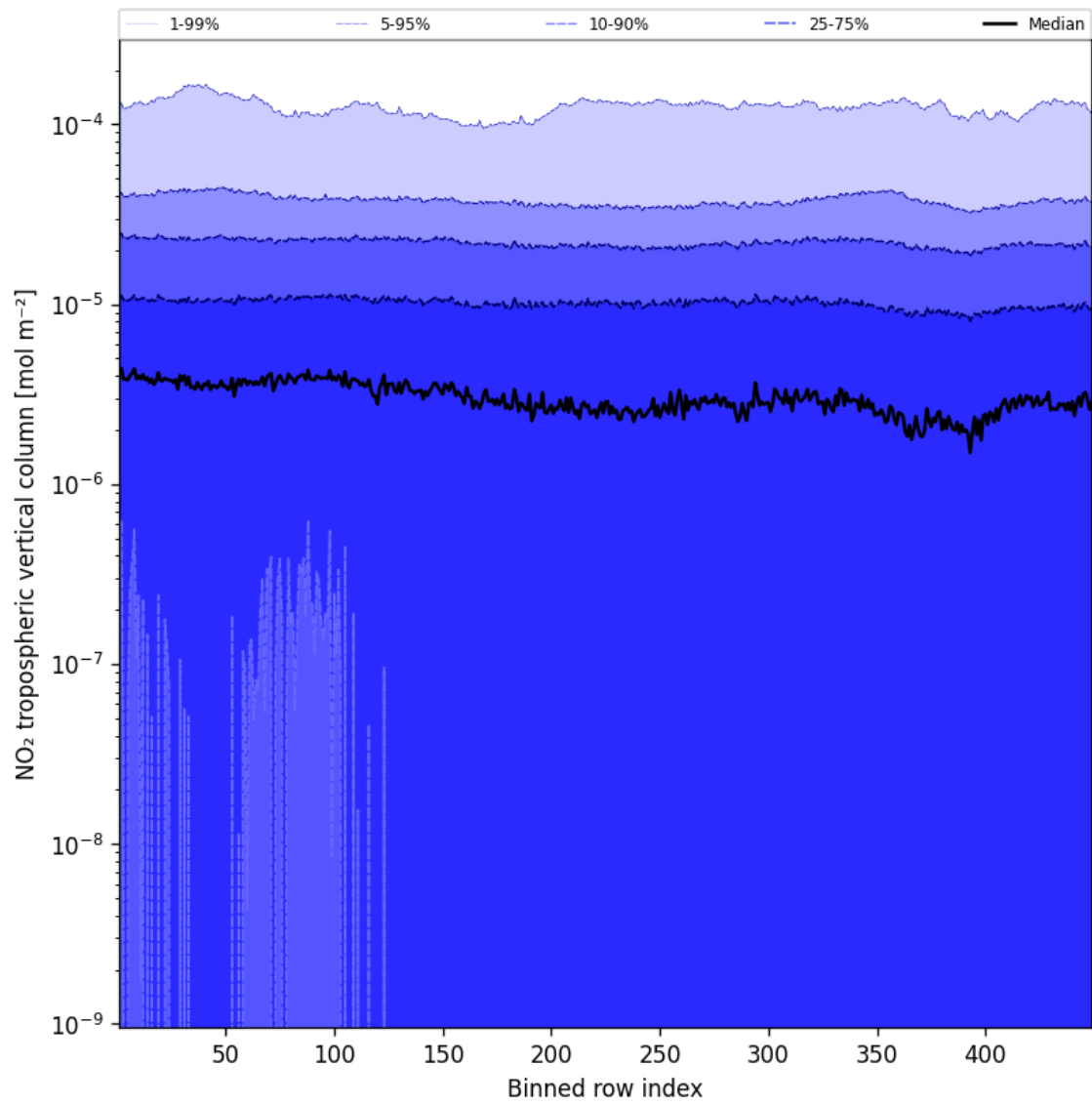
Figure 46: Along track statistics of “NO 2 tropospheric vertical column” for 2025-01-18 to 2025-01-20
