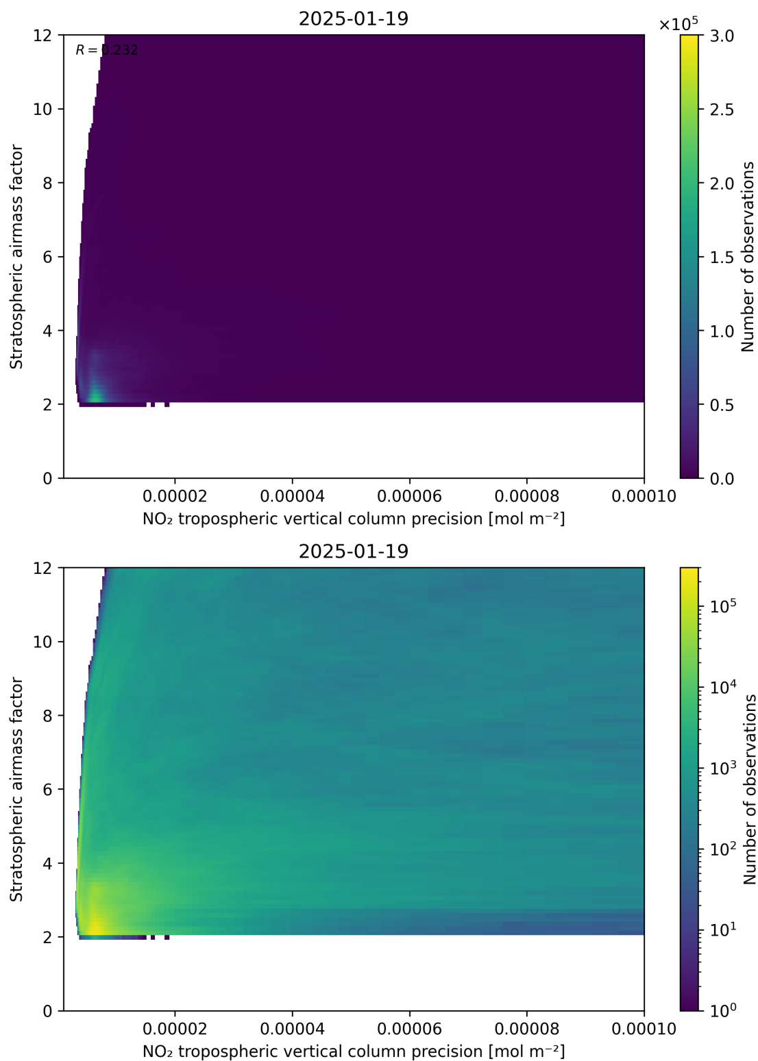
Figure 131: Scatter density plot of “NO 2 tropospheric vertical column precision” against “Stratospheric airmass factor” for 2025-01-18 to 2025-01-20.
