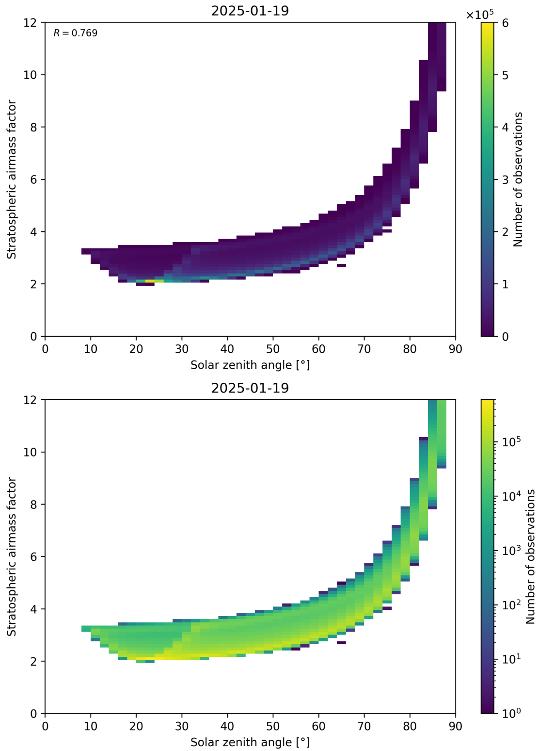
Figure 145: Scatter density plot of “Solar zenith angle” against “Stratospheric airmass factor” for 2025-01-18 to 2025-01-20.
