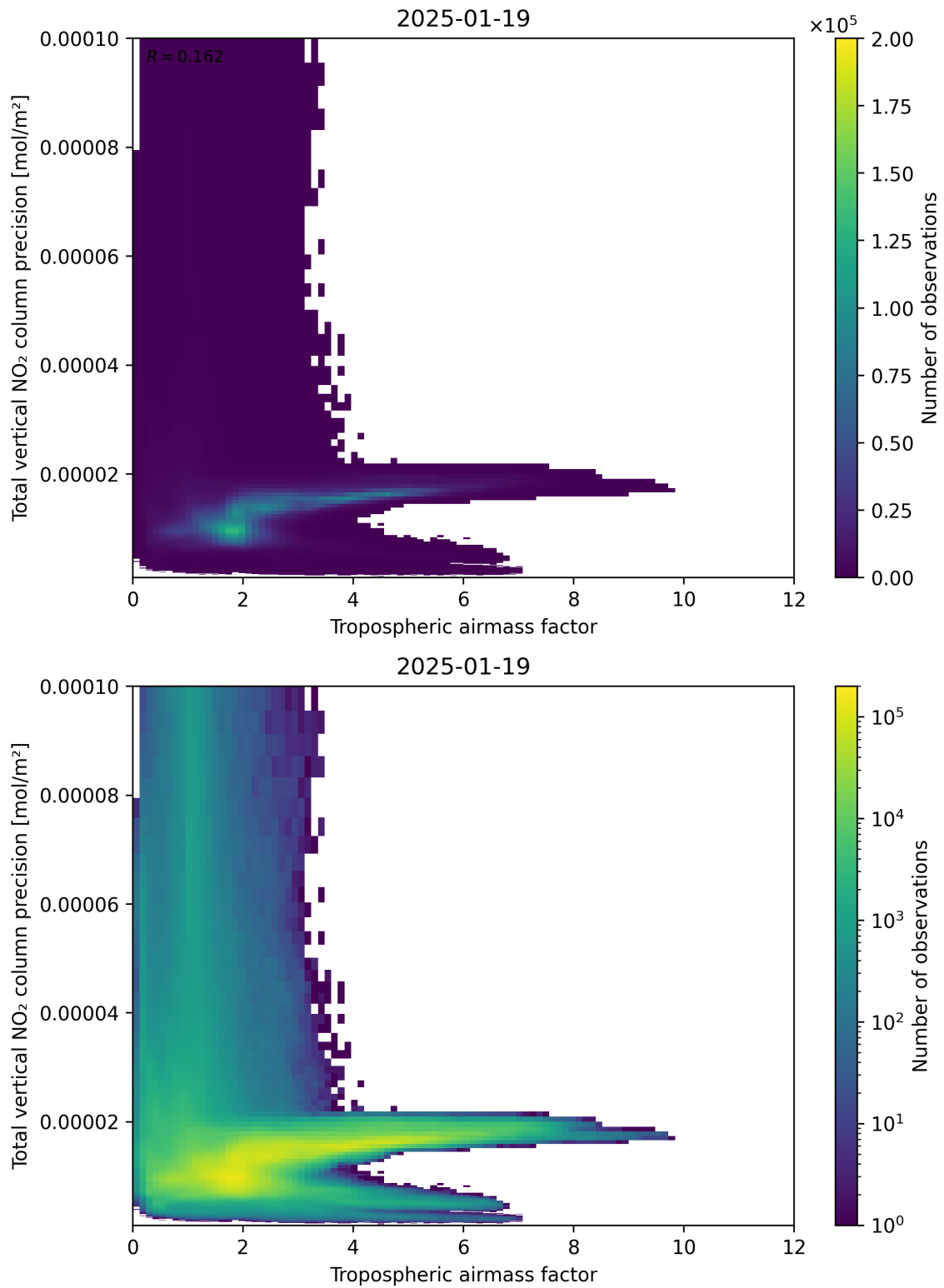
Figure 78: Scatter density plot of “Tropospheric air mass factor” against “Total vertical NO 2 column precision” for 2025-01-18 to 2025-01-20.
