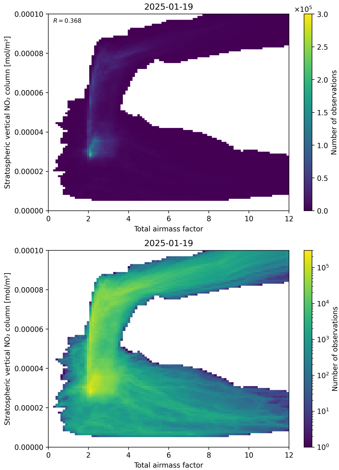
Figure 64: Scatter density plot of “Total airmass factor” against “Stratospheric vertical NO 2 column” for 2025-01-18 to 2025-01-20.
