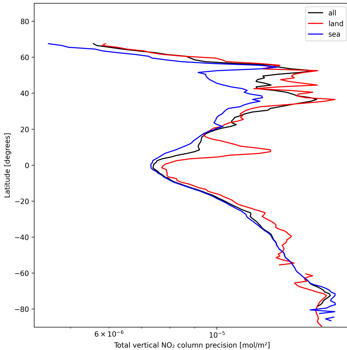
Figure 22: Zonal average of “Total vertical NO 2 column precision” for 2025-01-18 to 2025-01-20.
