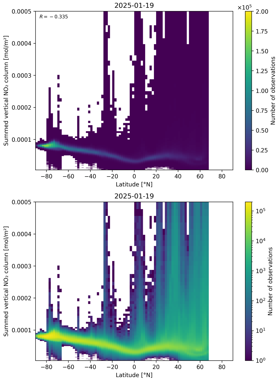
Figure 88: Scatter density plot of “Latitude” against “Summed vertical NO 2 column” for 2025-01-18 to 2025-01-20.
