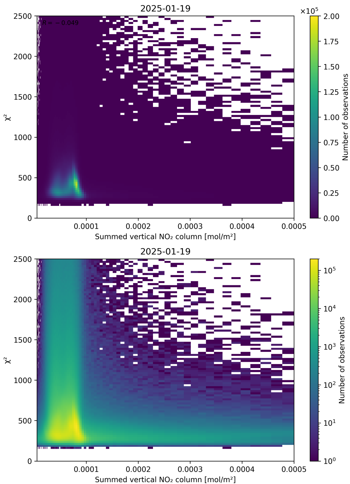
Figure 104: Scatter density plot of “Summed vertical NO 2 column” against “ \chi^2 ” for 2025-01-18 to 2025-01-20.
