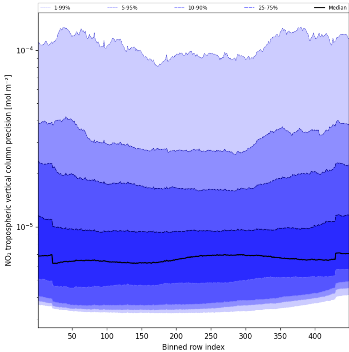
Figure 47: Along track statistics of “NO 2 tropospheric vertical column precision” for 2025-01-18 to 2025-01-20
