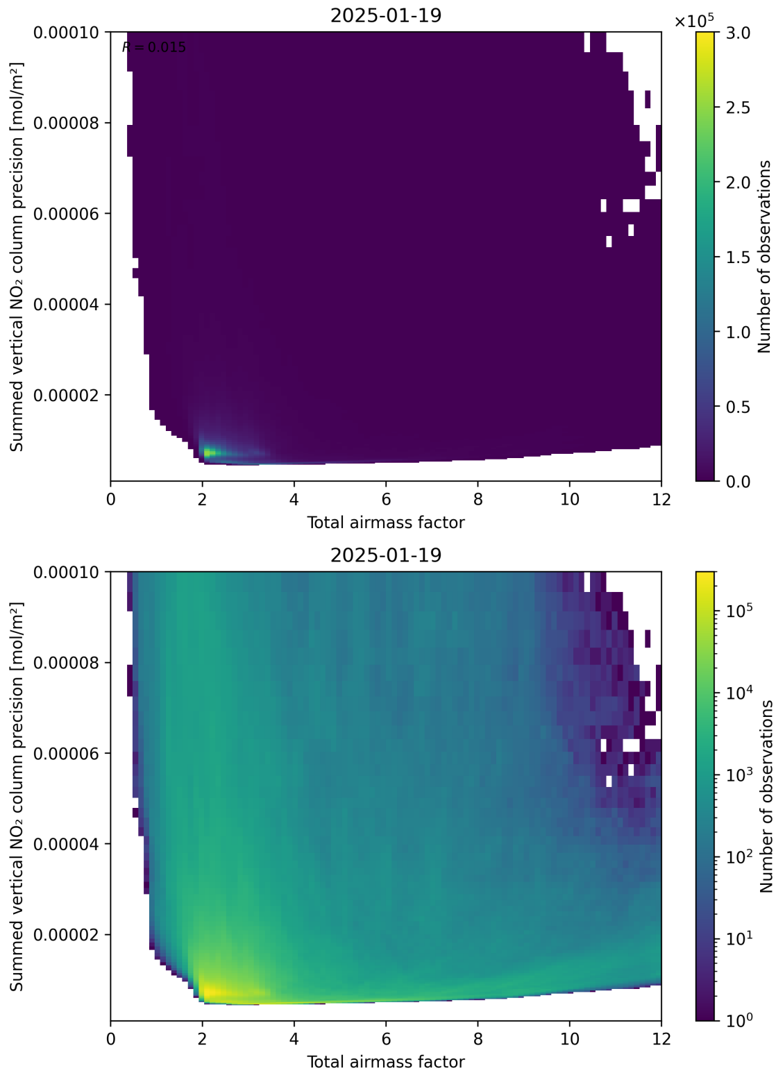
Figure 66: Scatter density plot of “Total airmass factor” against “Summed vertical NO 2 column precision” for 2025-01-18 to 2025-01-20.
