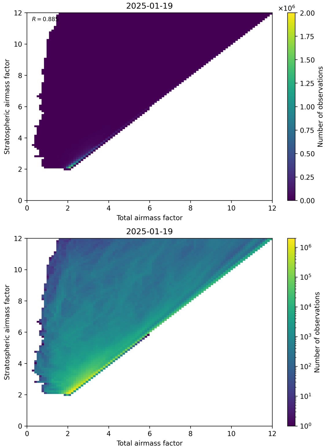
Figure 62: Scatter density plot of “Total airmass factor” against “Stratospheric airmass factor” for 2025-01-18 to 2025-01-20.
