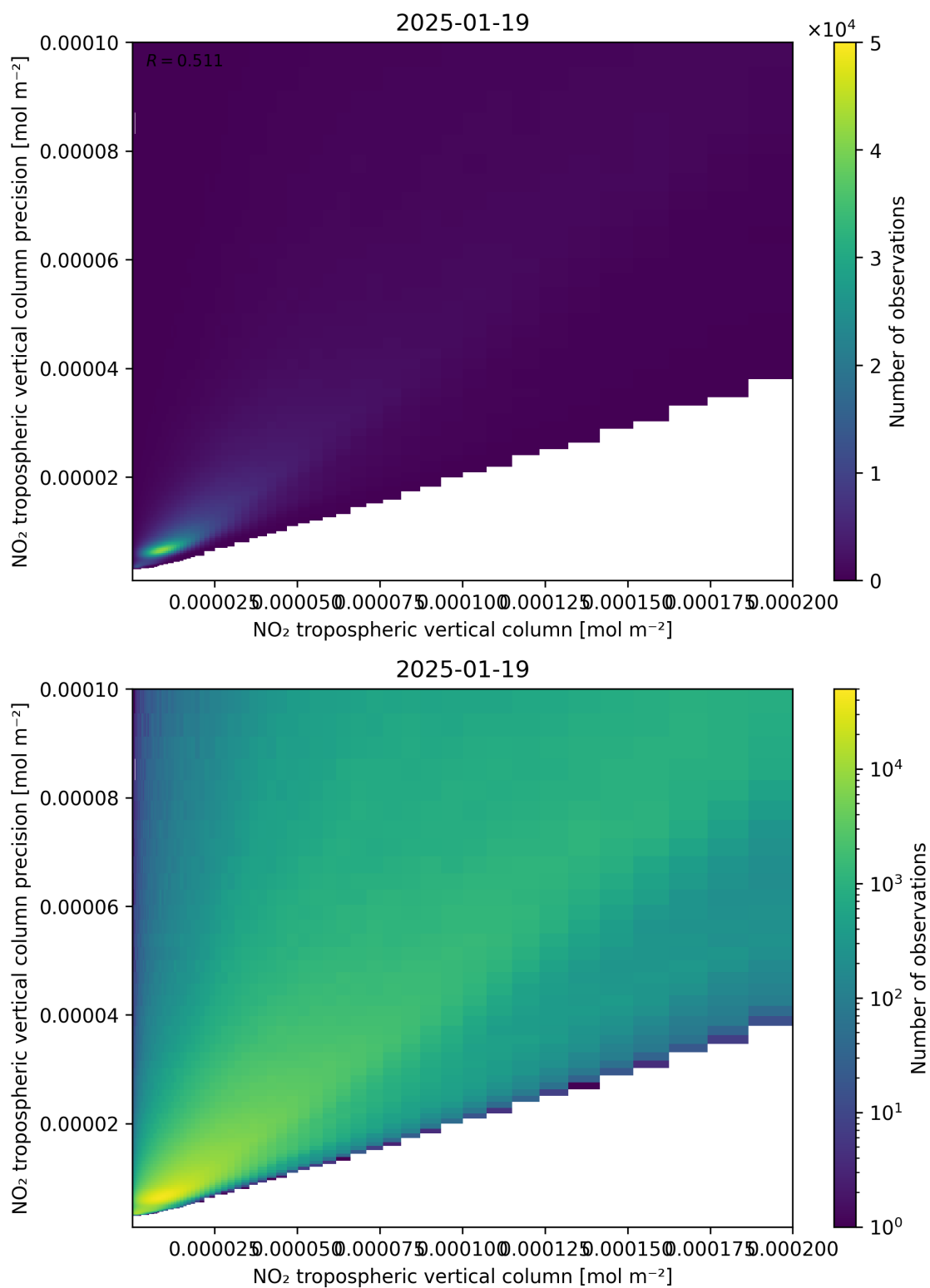
Figure 130: Scatter density plot of “NO 2 tropospheric vertical column” against “NO 2 tropospheric vertical column precision” for 2025-01-18 to 2025-01-20.
