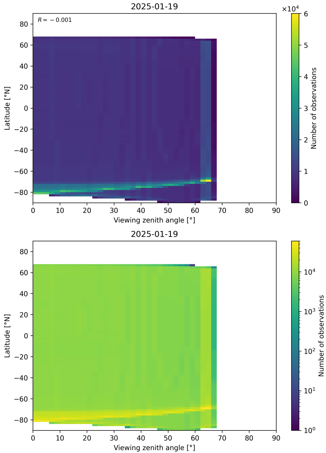
Figure 163: Scatter density plot of “Viewing zenith angle” against “Latitude” for 2025-01-18 to 2025-01-20.
