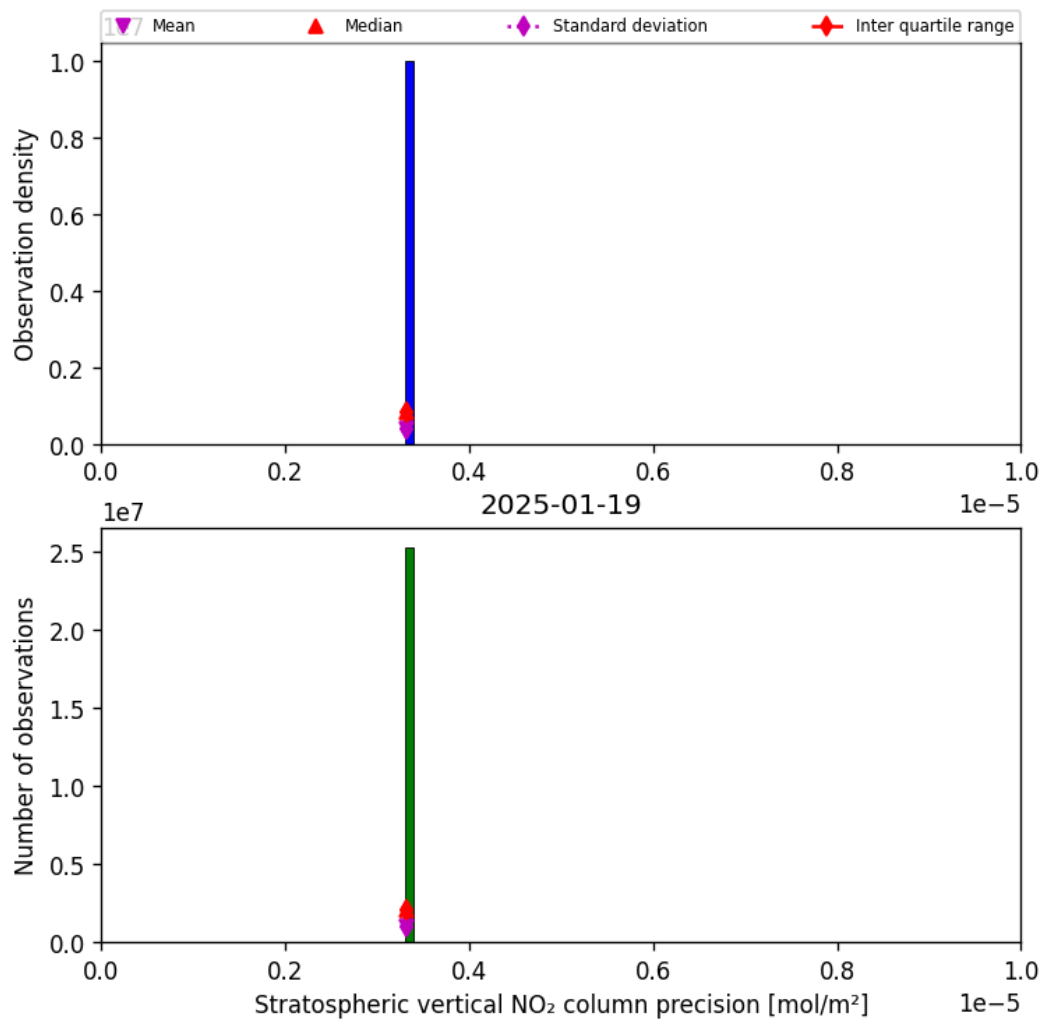
Figure 37: Histogram of “Stratospheric vertical NO 2 column precision” for 2025-01-18 to 2025-01-20
