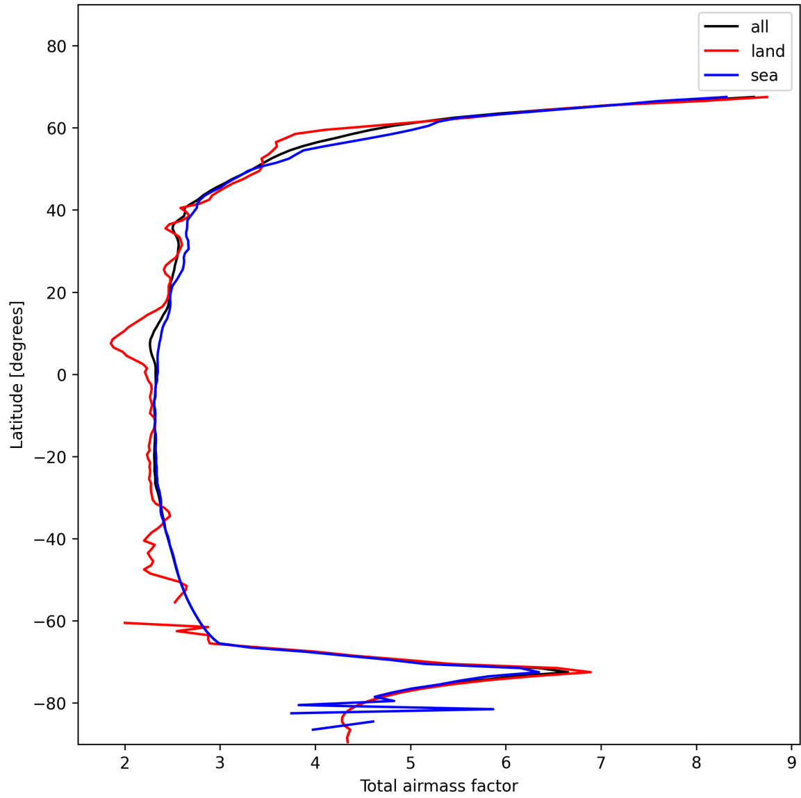
Figure 15: Zonal average of “Total airmass factor” for 2025-01-18 to 2025-01-20.
