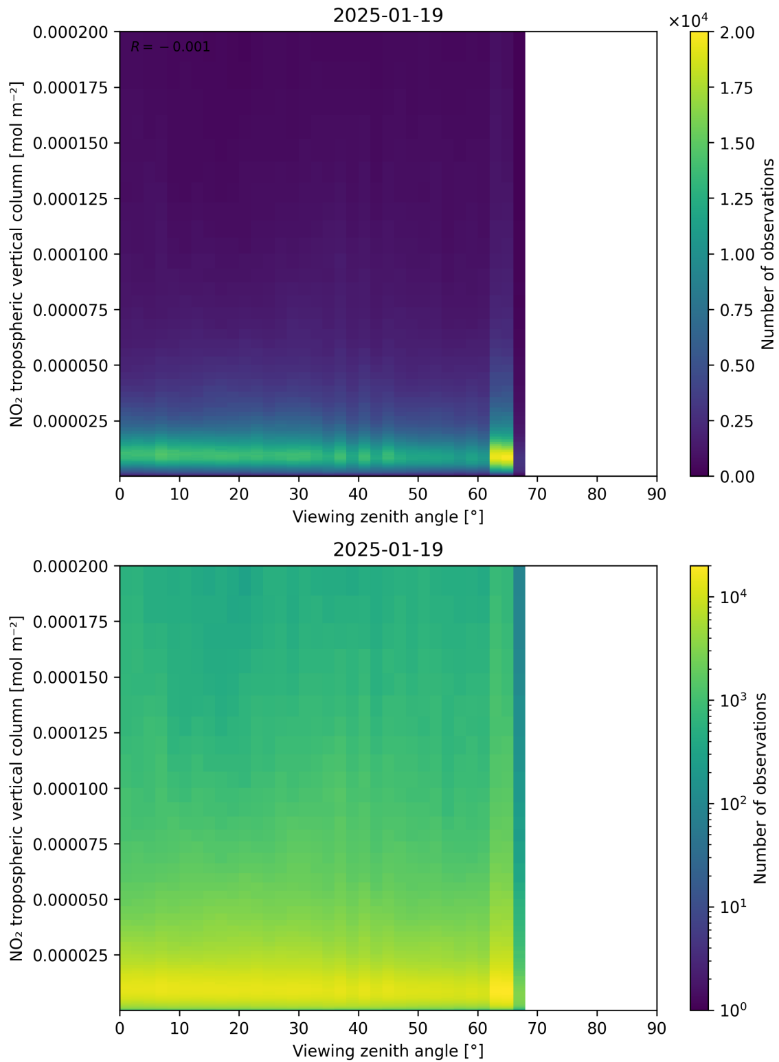
Figure 169: Scatter density plot of “Viewing zenith angle” against “NO 2 tropospheric vertical column” for 2025-01-18 to 2025-01-20.
