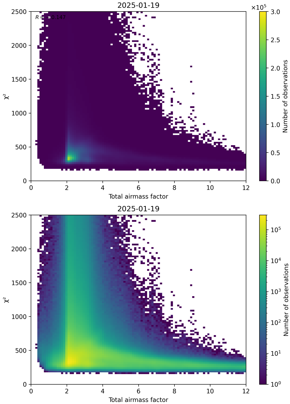
Figure 63: Scatter density plot of “Total airmass factor” against “ \chi^2 ” for 2025-01-18 to 2025-01-20.
