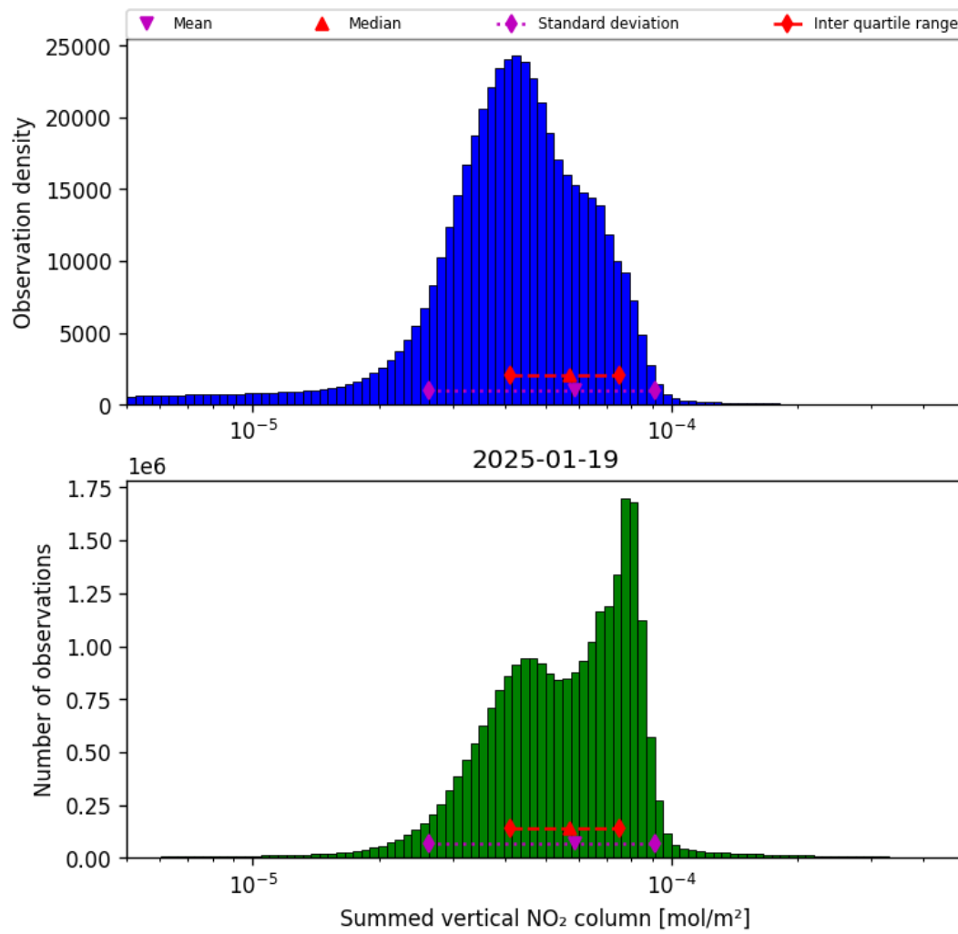
Figure 40: Histogram of “Summed vertical NO 2 column” for 2025-01-18 to 2025-01-20
