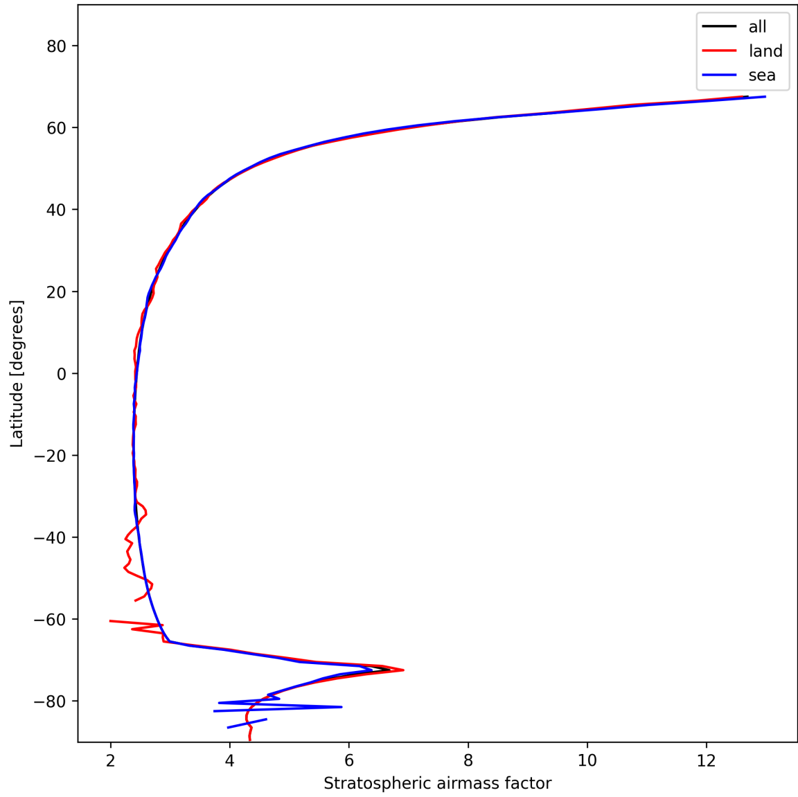
Figure 27: Zonal average of “Stratospheric air mass factor” for 2025-01-18 to 2025-01-20.
