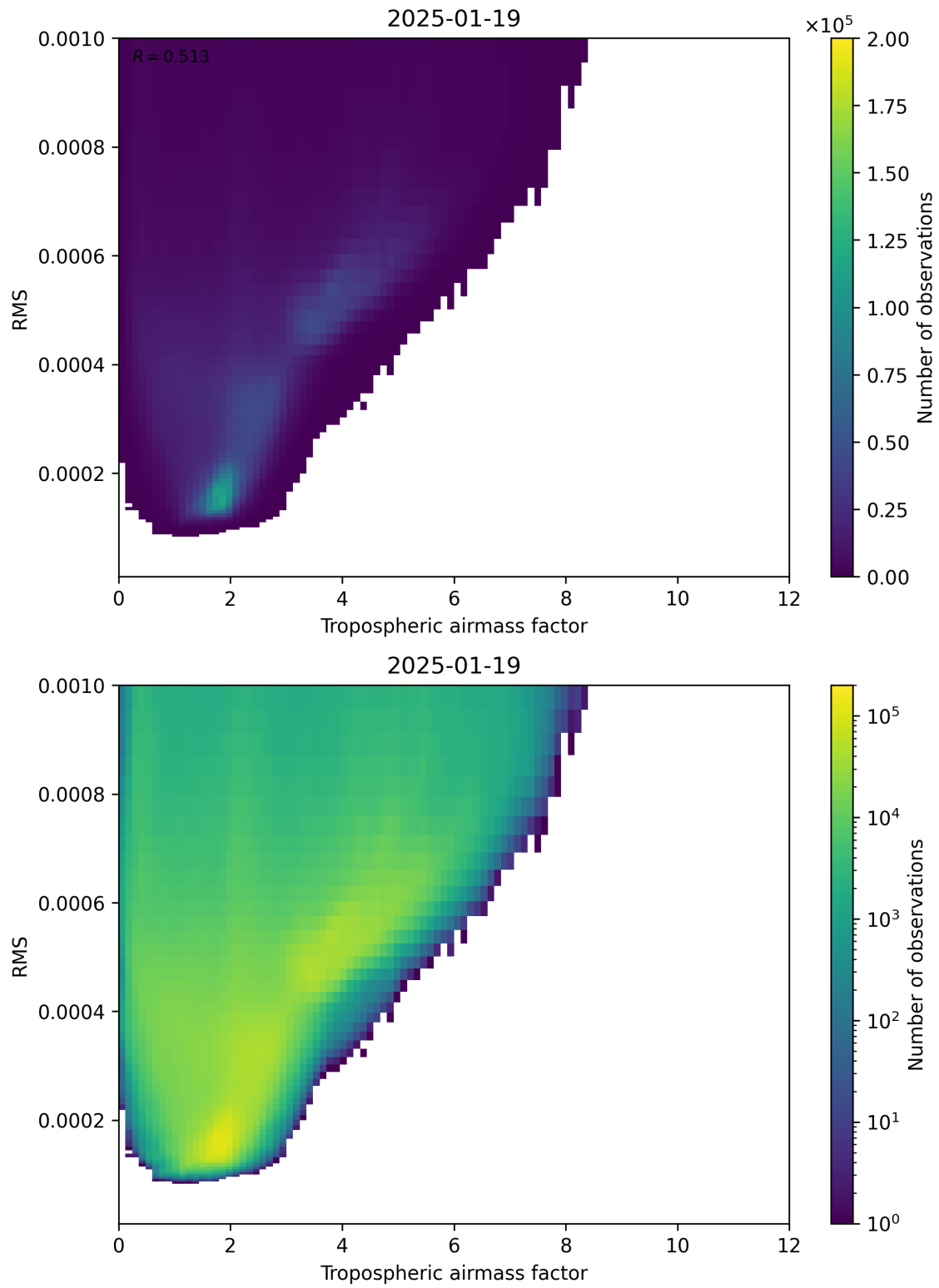
Figure 79: Scatter density plot of “Tropospheric airmass factor” against “RMS” for 2025-01-18 to 2025-01-20.
