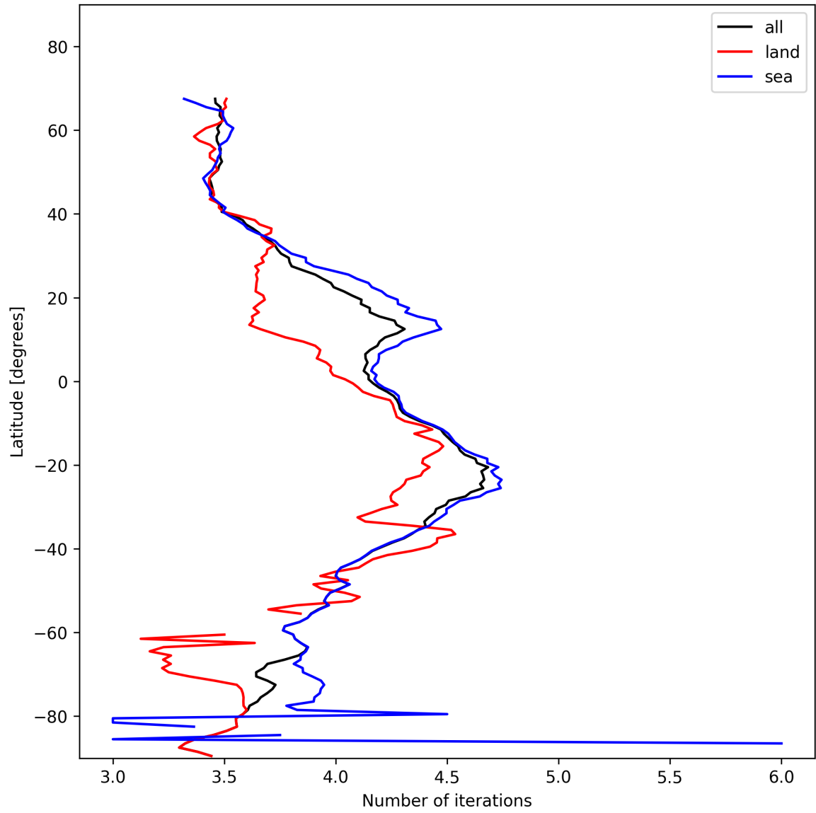
Figure 17: Zonal average of “Number of iterations” for 2025-01-18 to 2025-01-20.
