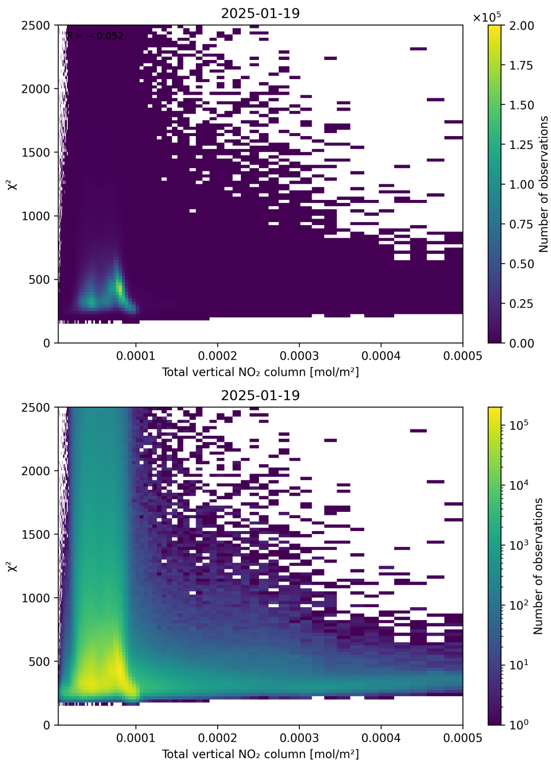
Figure 111: Scatter density plot of “Total vertical NO 2 column” against “ \chi^2 ” for 2025-01-18 to 2025-01-20.
