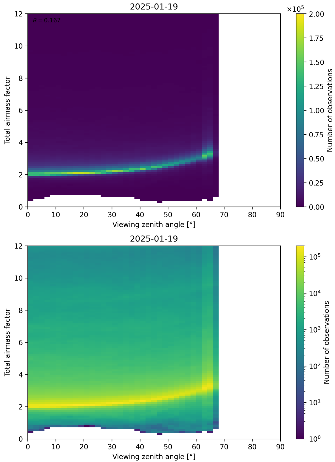
Figure 160: Scatter density plot of “Viewing zenith angle” against “Total airmass factor” for 2025-01-18 to 2025-01-20.
