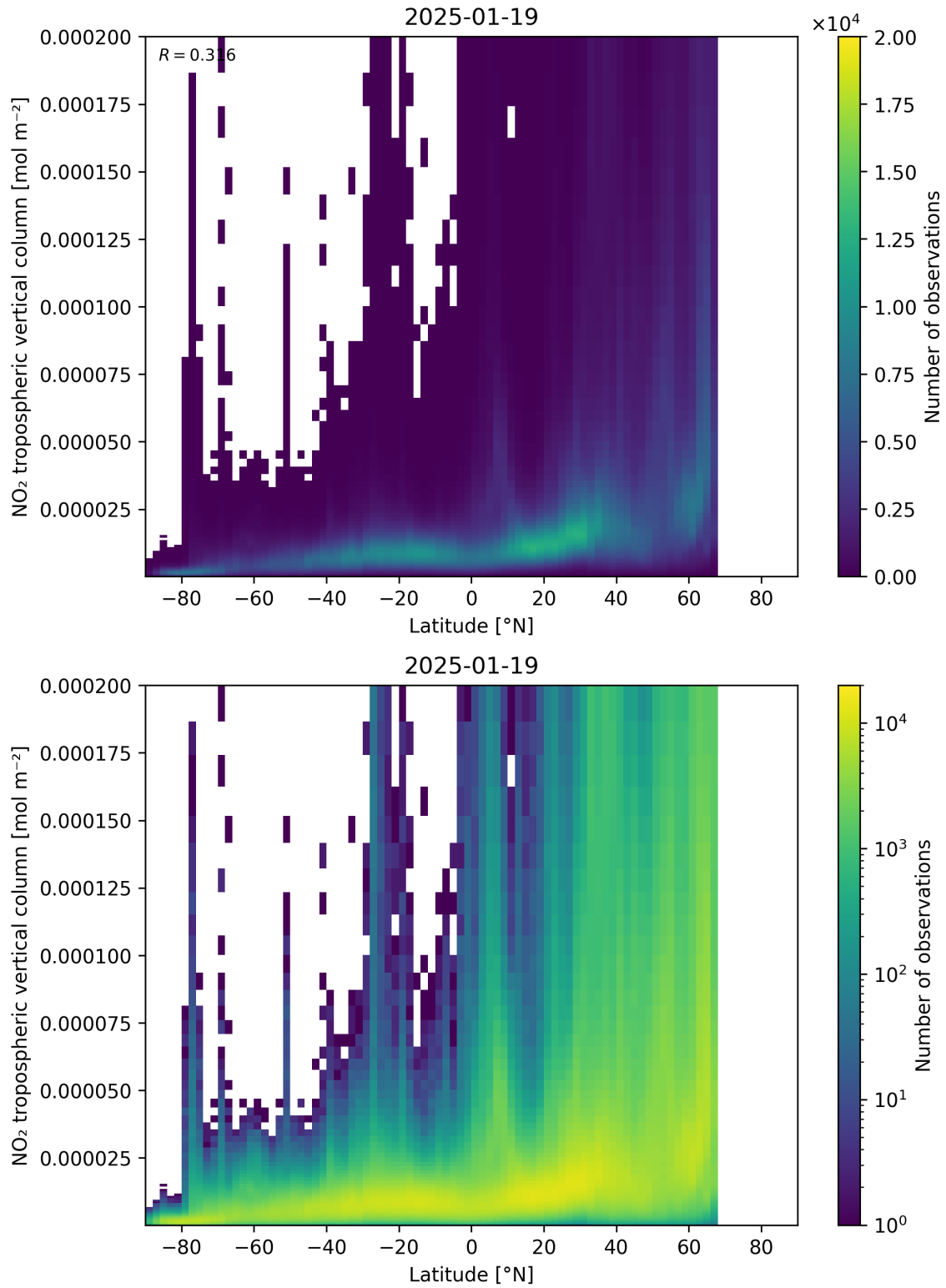
Figure 92: Scatter density plot of “Latitude” against “NO 2 tropospheric vertical column” for 2025-01-18 to 2025-01-20.
