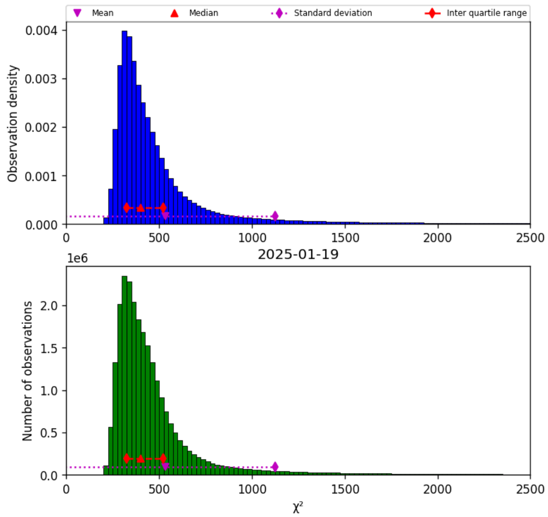
Figure 42: Histogram of “ \chi^2 ” for 2025-01-18 to 2025-01-20
