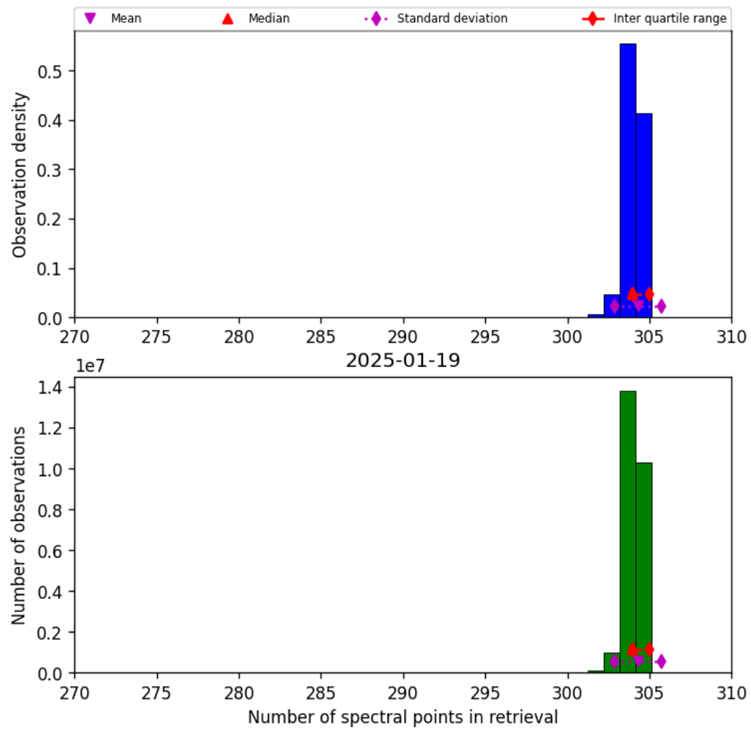
Figure 33: Histogram of “Number of spectral points in retrieval” for 2025-01-18 to 2025-01-20
