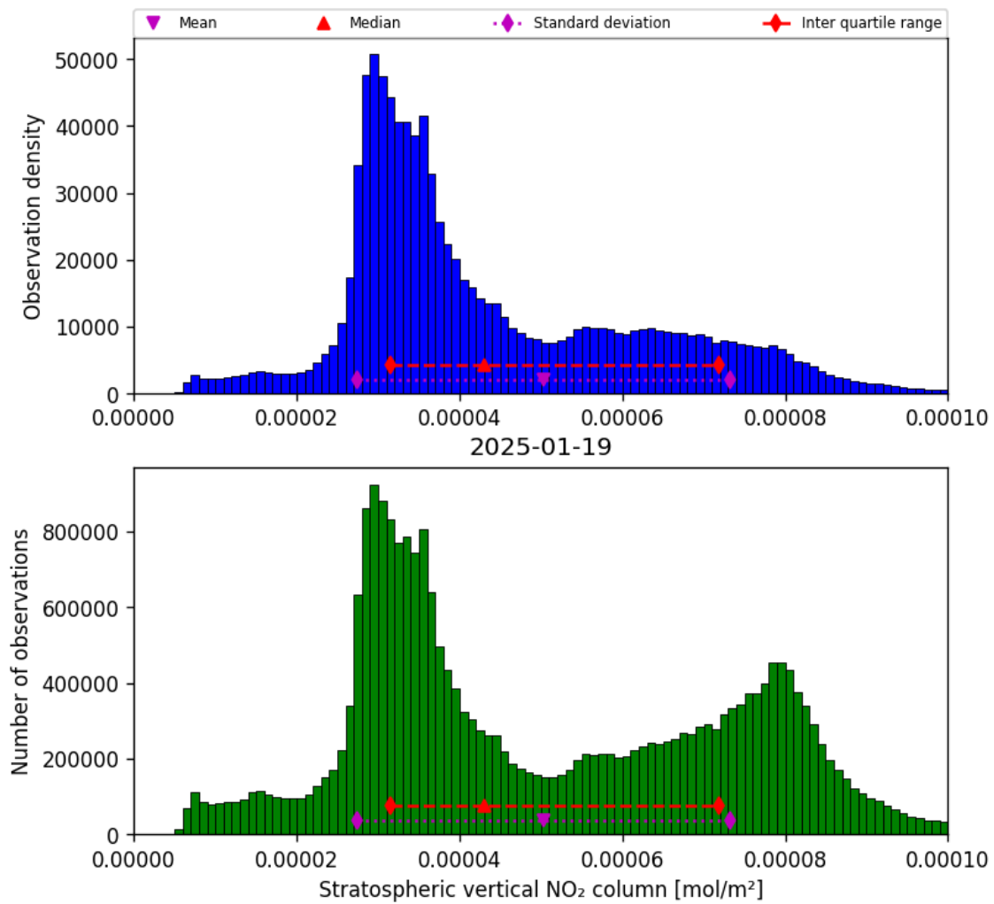
Figure 36: Histogram of “Stratospheric vertical NO 2 column” for 2025-01-18 to 2025-01-20
