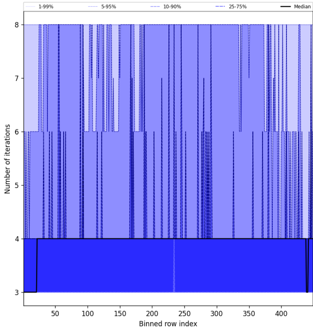
Figure 51: Along track statistics of “Number of iterations” for 2025-01-18 to 2025-01-20
