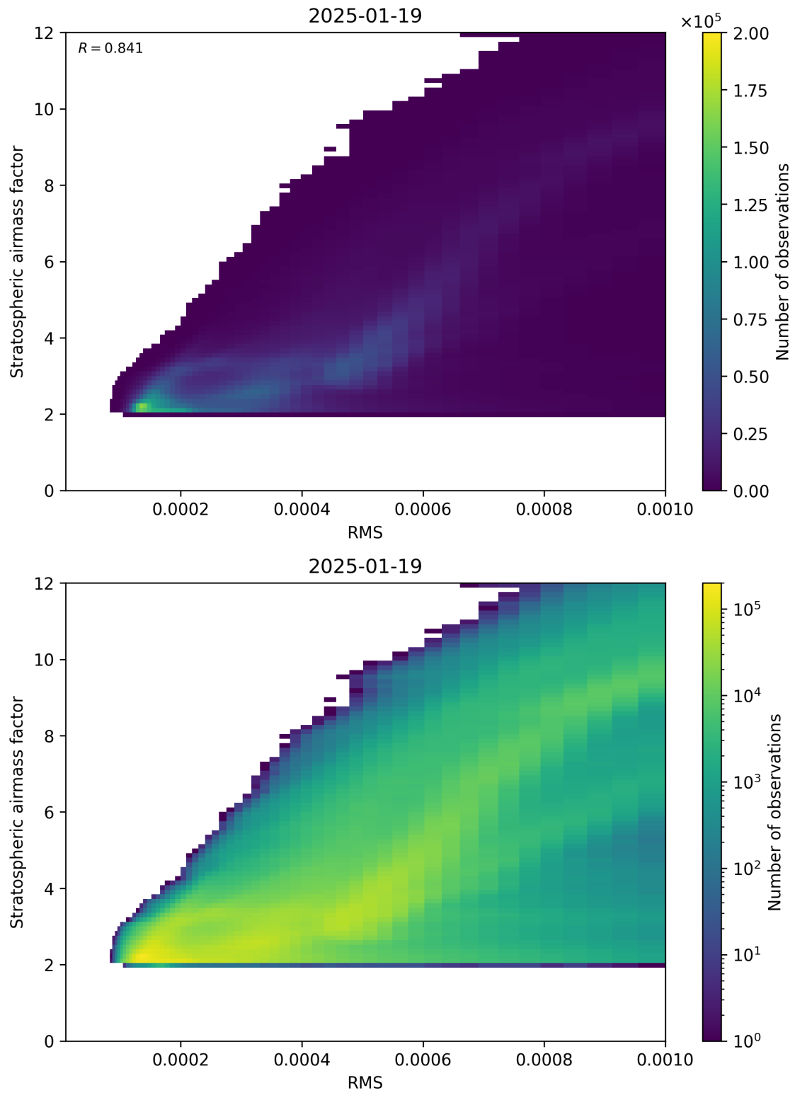
Figure 144: Scatter density plot of “RMS” against “Stratospheric airmass factor” for 2025-01-18 to 2025-01-20.
