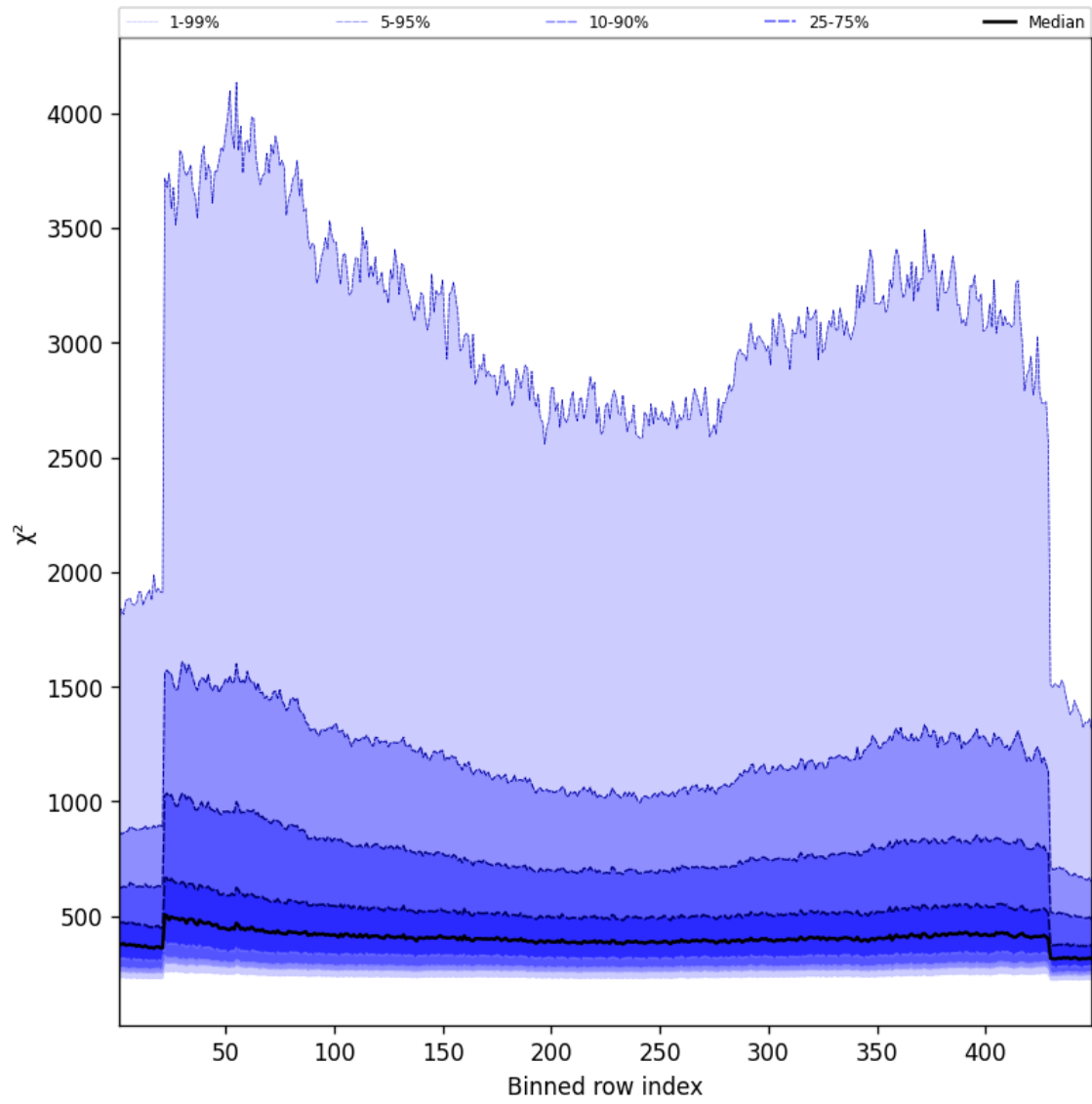
Figure 59: Along track statistics of “ \chi^2 ” for 2025-01-18 to 2025-01-20
