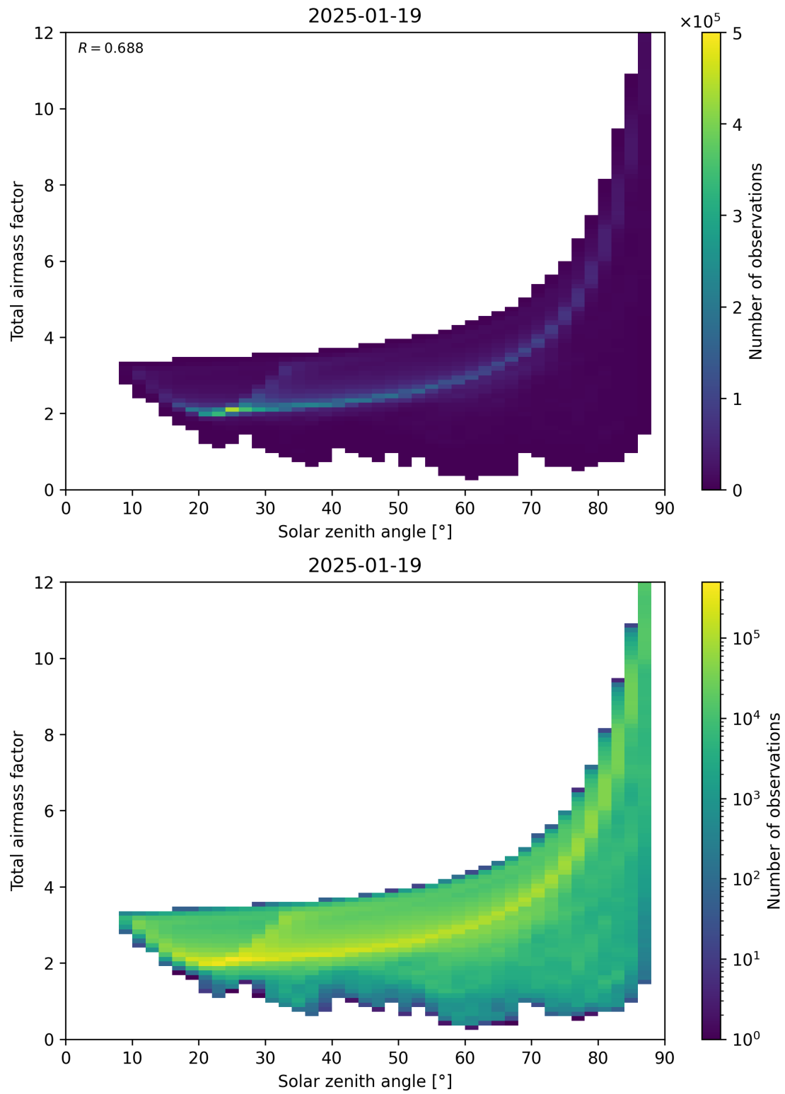
Figure 146: Scatter density plot of “Solar zenith angle” against “Total air mass factor” for 2025-01-18 to 2025-01-20.
