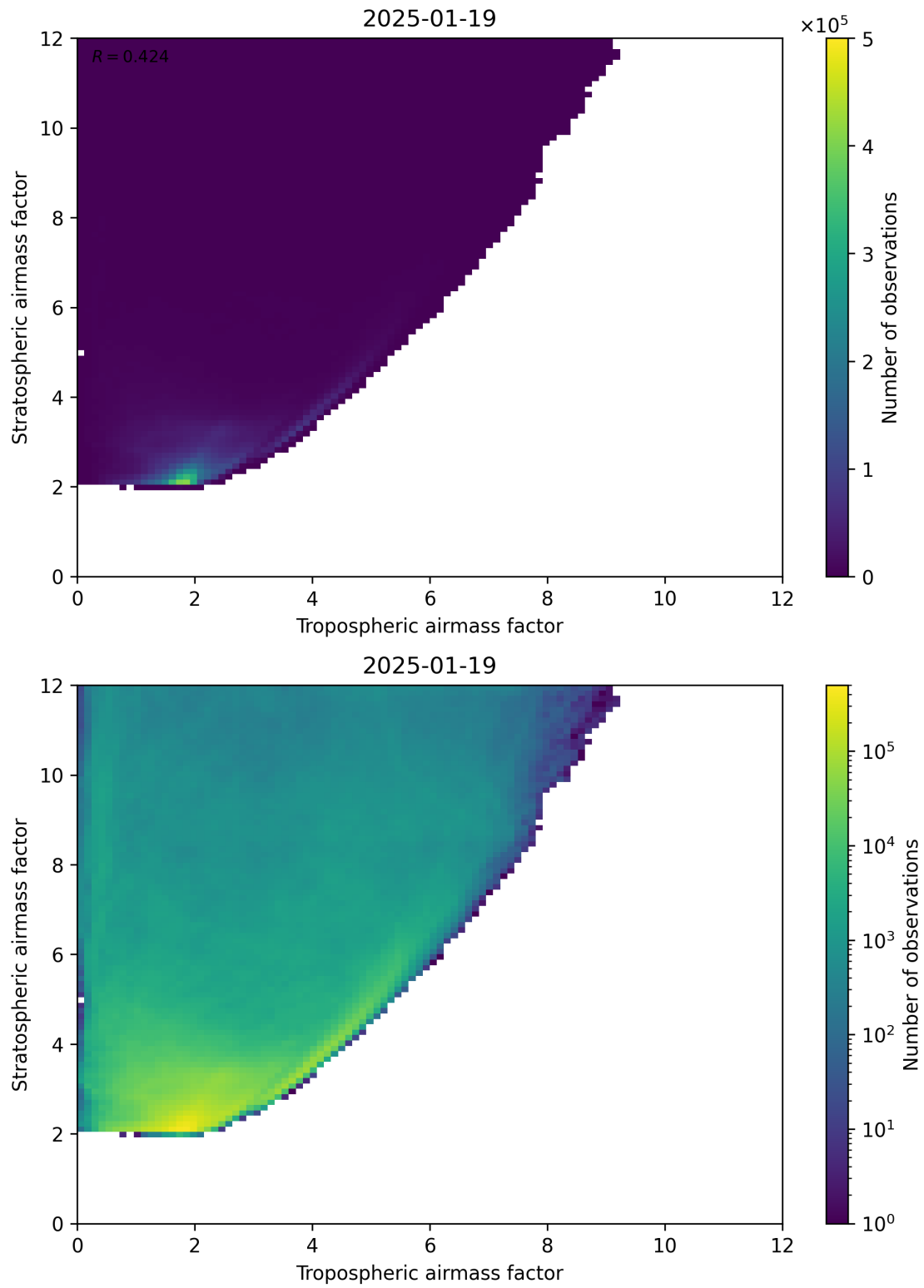
Figure 71: Scatter density plot of “Tropospheric airmass factor” against “Stratospheric airmass factor” for 2025-01-18 to 2025-01-20.
