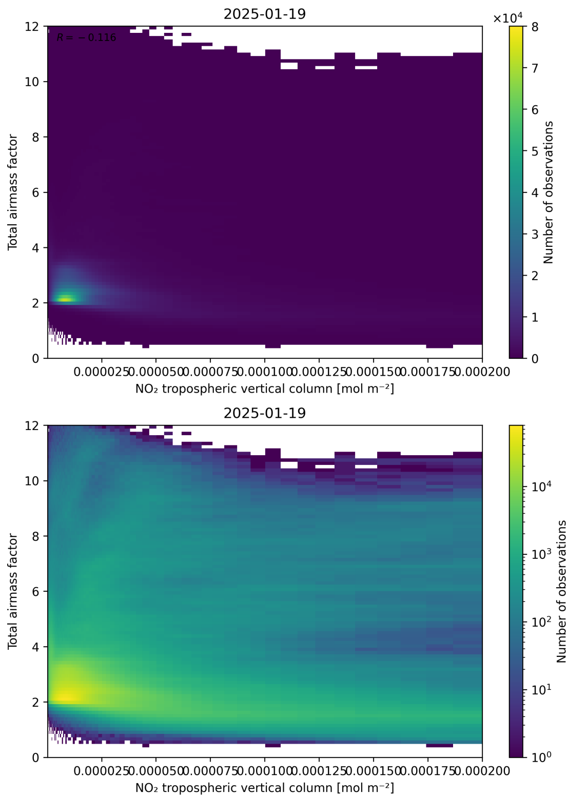
Figure 122: Scatter density plot of “NO 2 tropospheric vertical column” against “Total air mass factor” for 2025-01-18 to 2025-01-20.
