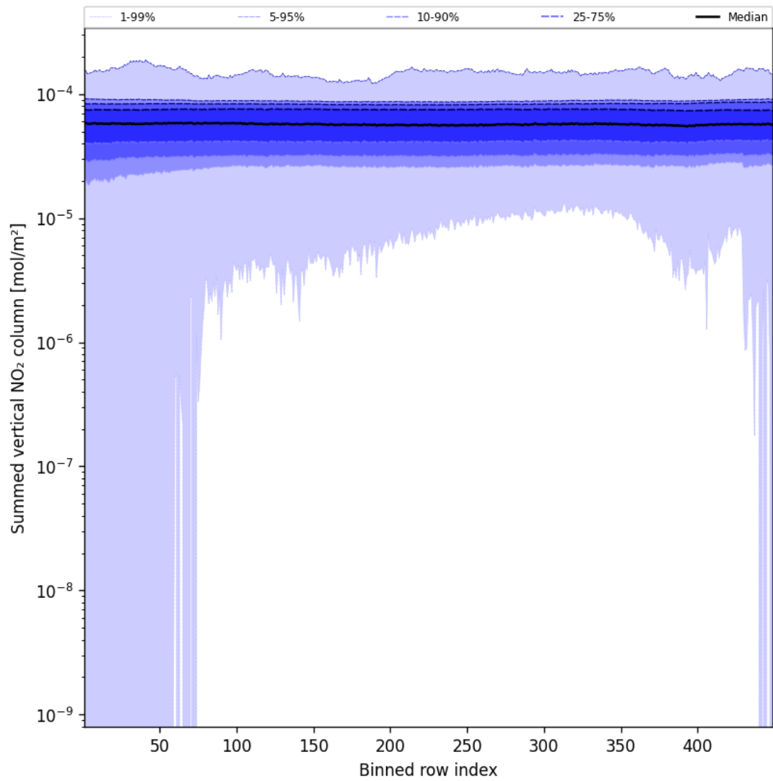
Figure 57: Along track statistics of “Summed vertical NO 2 column” for 2025-01-18 to 2025-01-20
