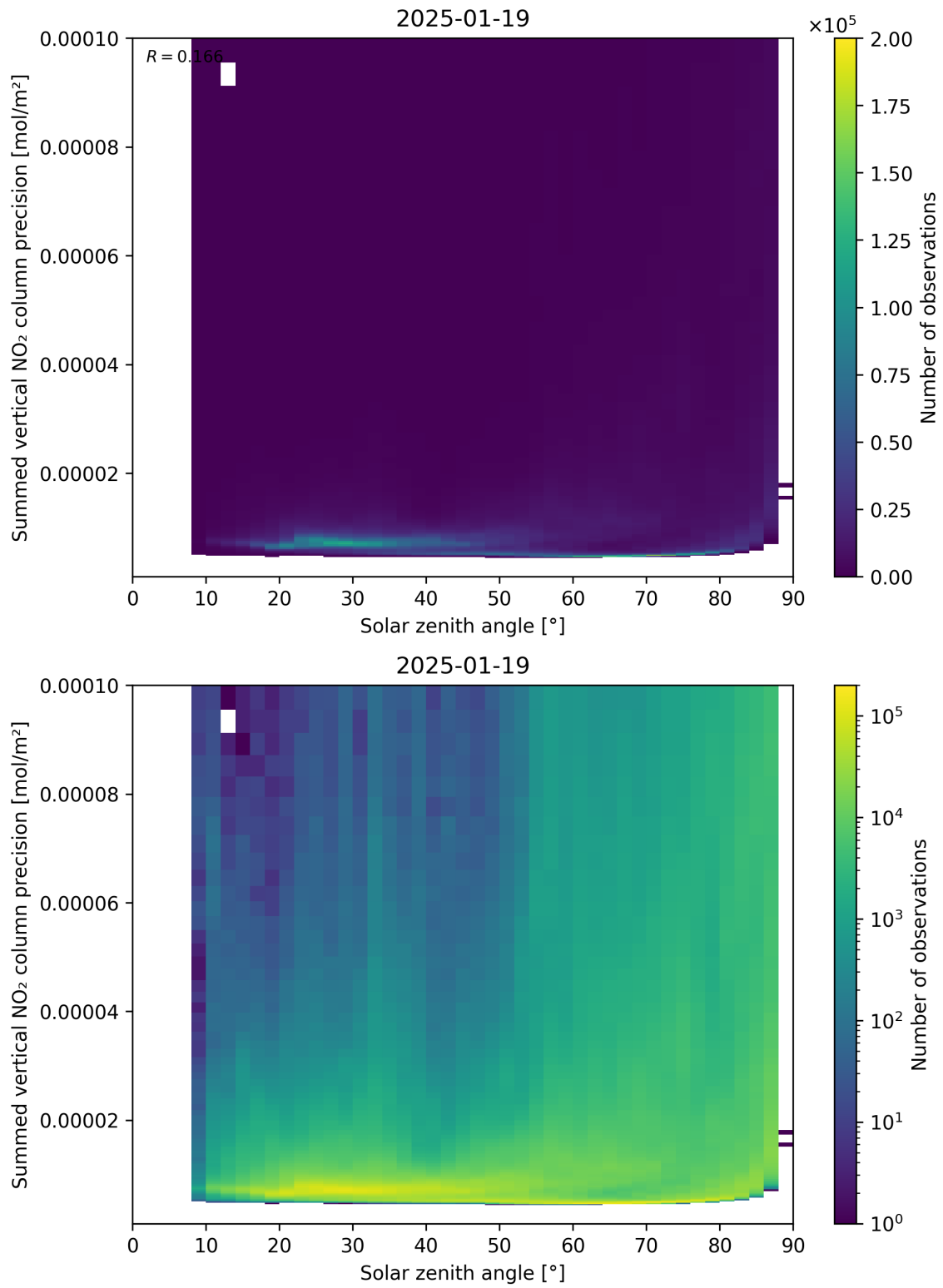
Figure 152: Scatter density plot of “Solar zenith angle” against “Summed vertical NO 2 column precision” for 2025-01-18 to 2025-01-20.
