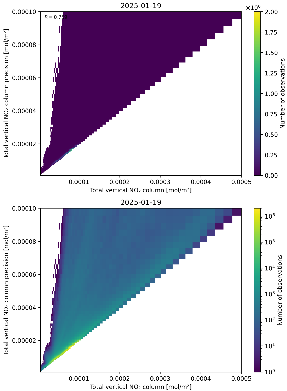
Figure 114: Scatter density plot of “Total vertical NO 2 column” against “Total vertical NO 2 column precision” for 2025-01-18 to 2025-01-20.
