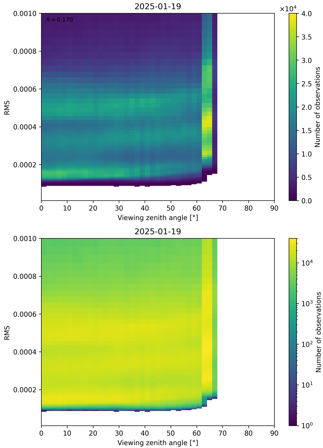
Figure 171: Scatter density plot of “Viewing zenith angle” against “RMS” for 2025-01-18 to 2025-01-20.
