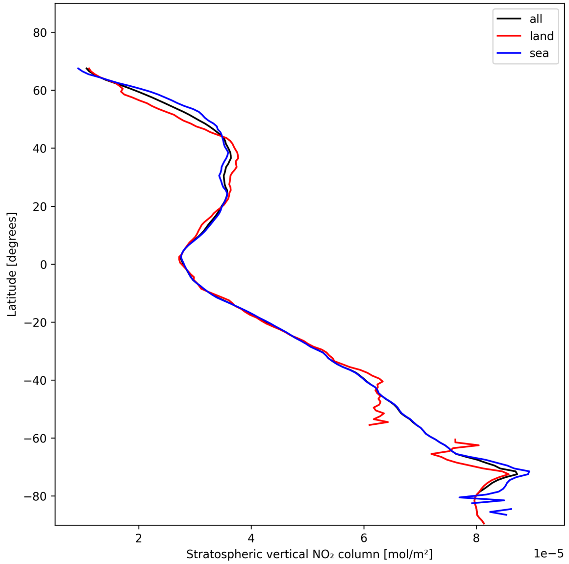
Figure 19: Zonal average of “Stratospheric vertical NO 2 column” for 2025-01-18 to 2025-01-20.
