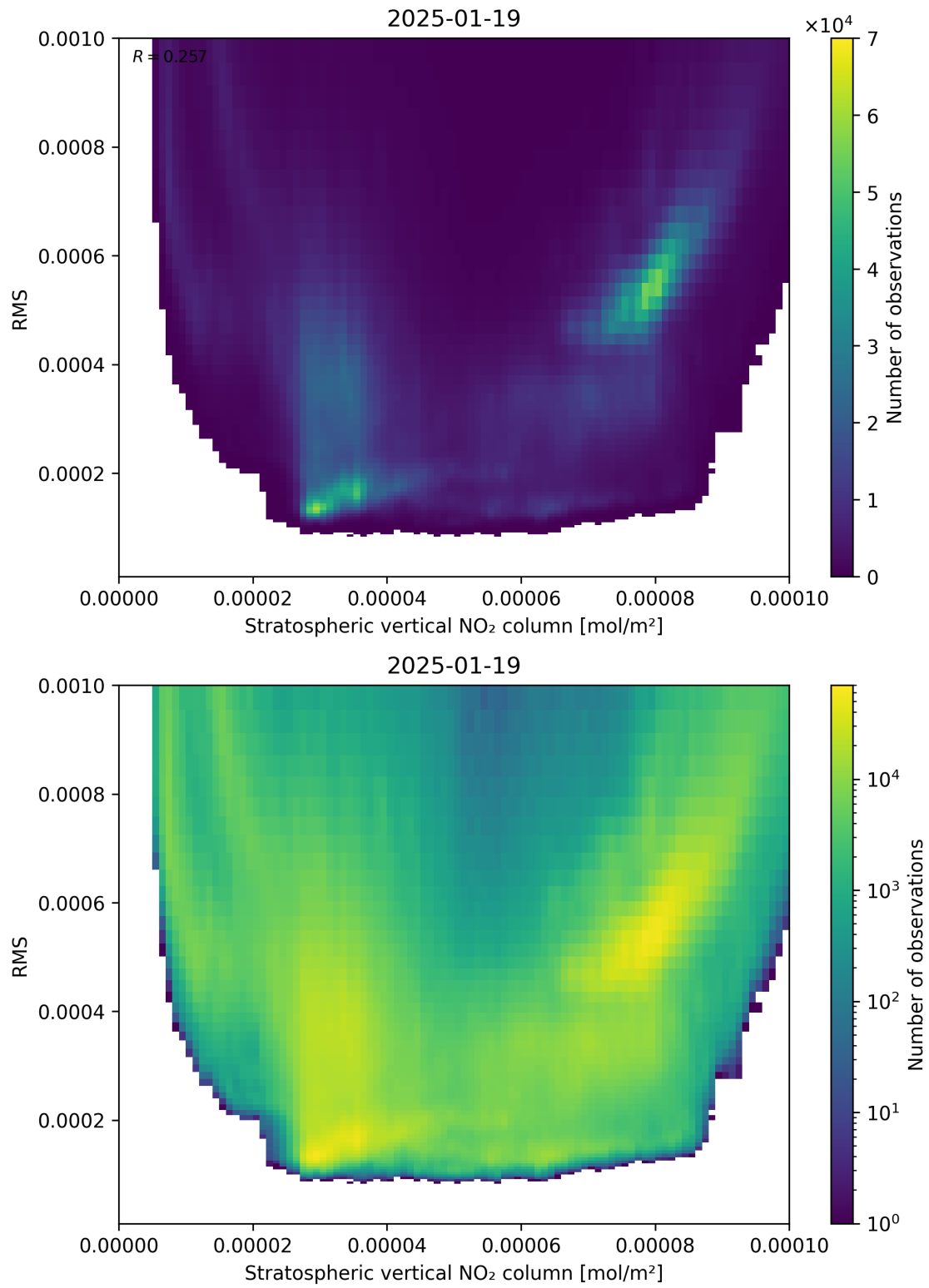
Figure 102: Scatter density plot of “Stratospheric vertical NO 2 column” against “RMS” for 2025-01-18 to 2025-01-20.
