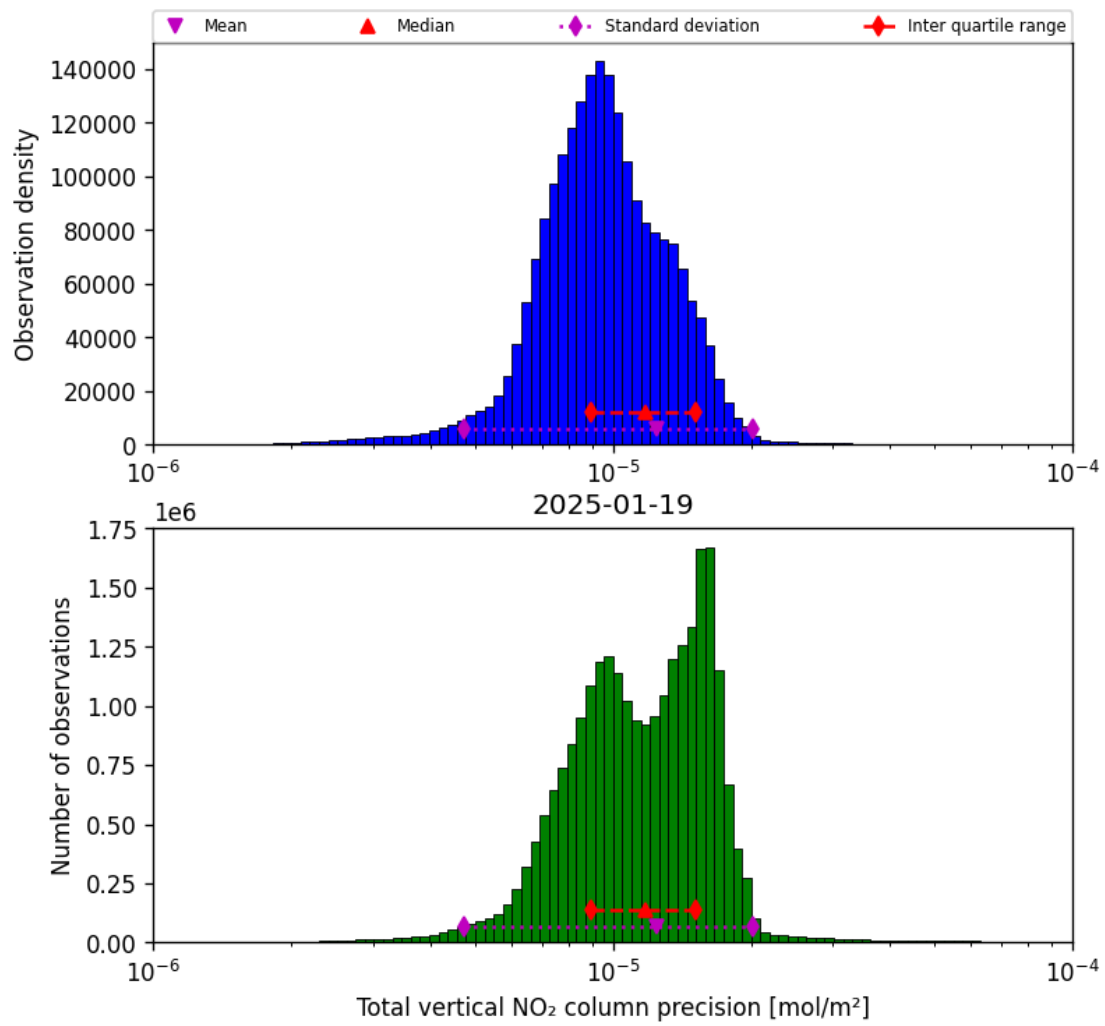
Figure 39: Histogram of “Total vertical NO 2 column precision” for 2025-01-18 to 2025-01-20
