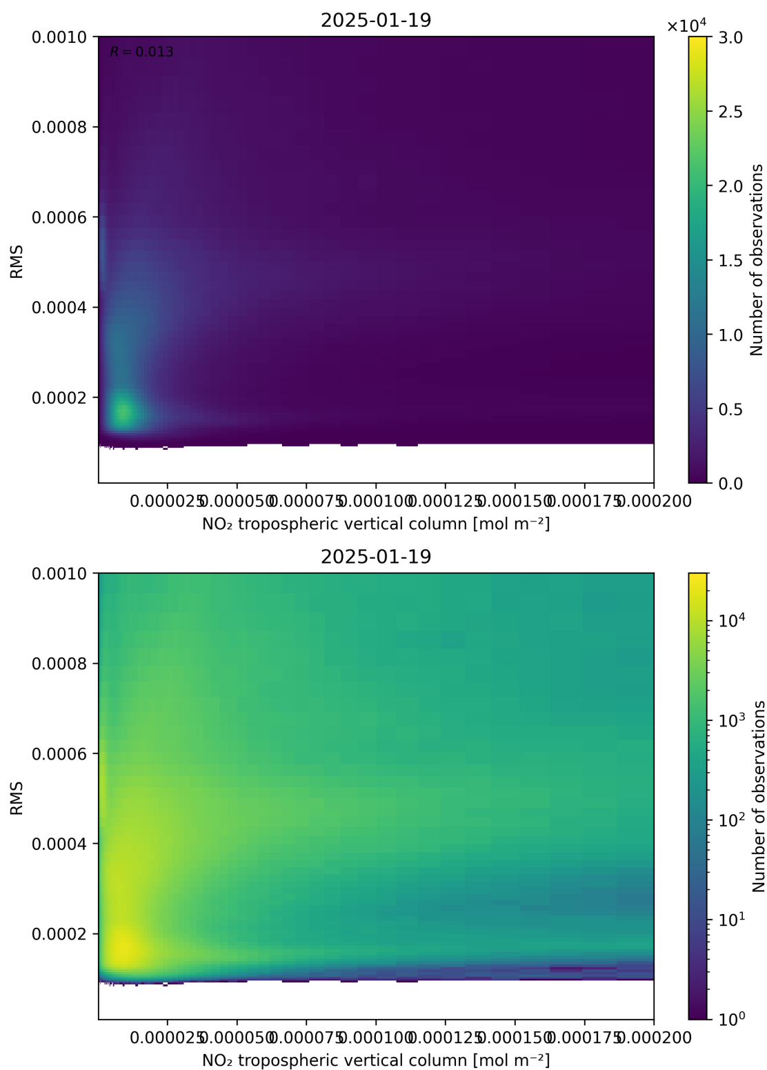
Figure 142: Scatter density plot of “NO 2 tropospheric vertical column” against “RMS” for 2025-01-18 to 2025-01-20.
