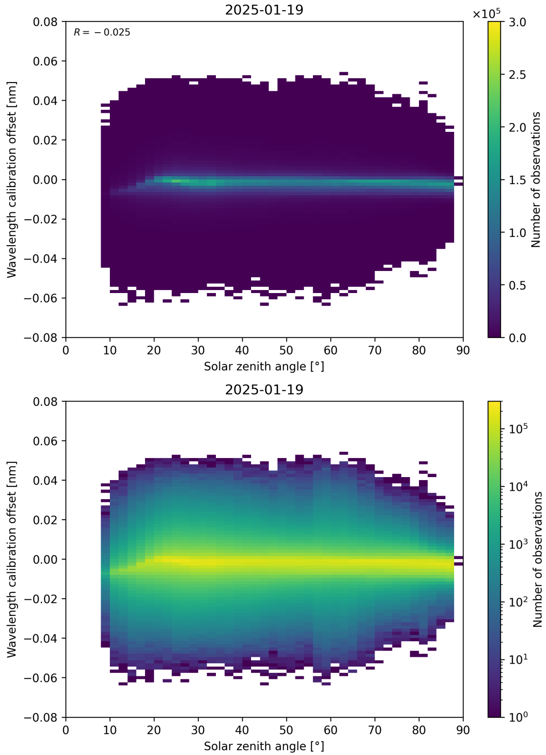
Figure 158: Scatter density plot of “Solar zenith angle” against “Wavelength calibration offset” for 2025-01-18 to 2025-01-20.
