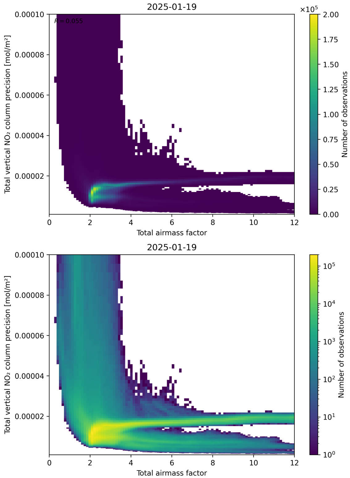
Figure 68: Scatter density plot of “Total airmass factor” against “Total vertical NO 2 column precision” for 2025-01-18 to 2025-01-20.
