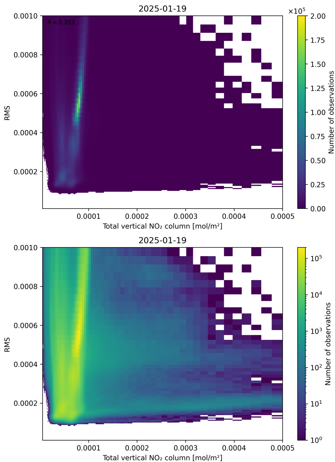
Figure 120: Scatter density plot of “Total vertical NO 2 column” against “RMS” for 2025-01-18 to 2025-01-20.
