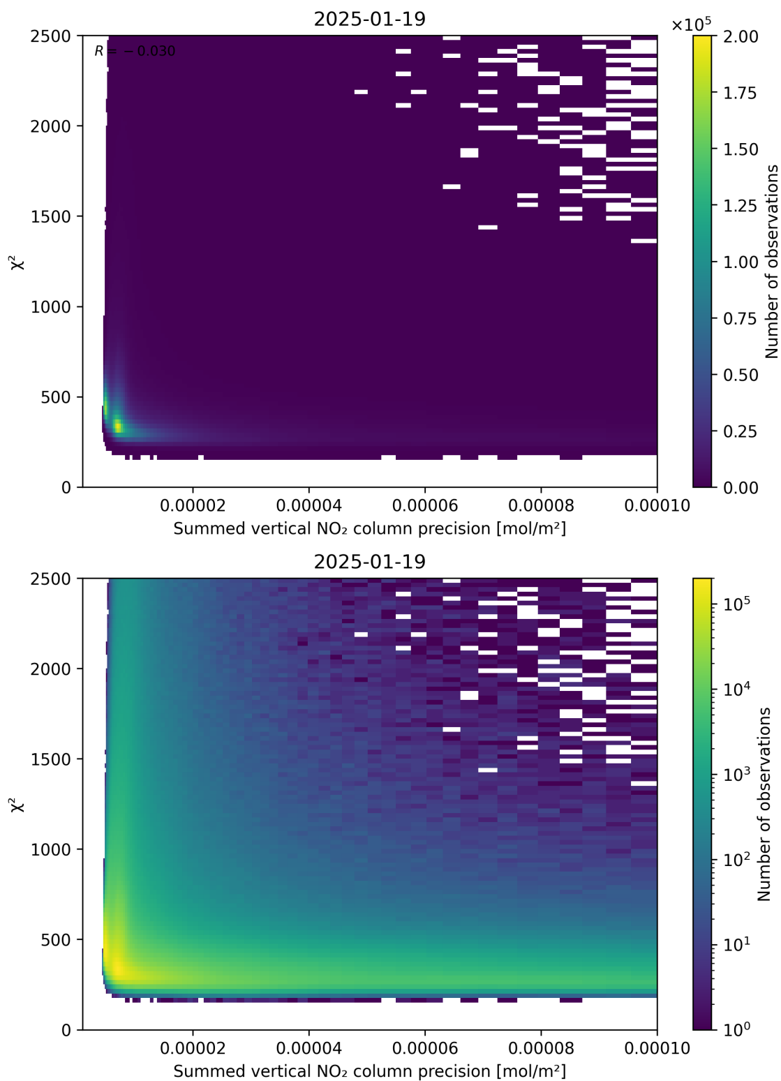
Figure 107: Scatter density plot of “Summed vertical NO 2 column precision” against “ \chi^2 ” for 2025-01-18 to 2025-01-20.
