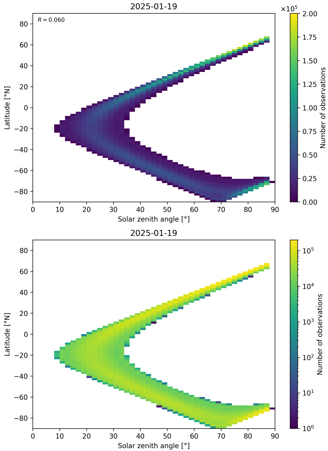
Figure 149: Scatter density plot of “Solar zenith angle” against “Latitude” for 2025-01-18 to 2025-01-20.
