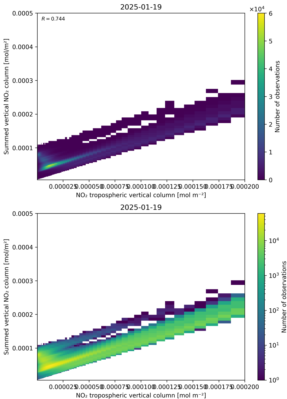
Figure 126: Scatter density plot of “NO 2 tropospheric vertical column” against “Summed vertical NO 2 column” for 2025-01-18 to 2025-01-20.
