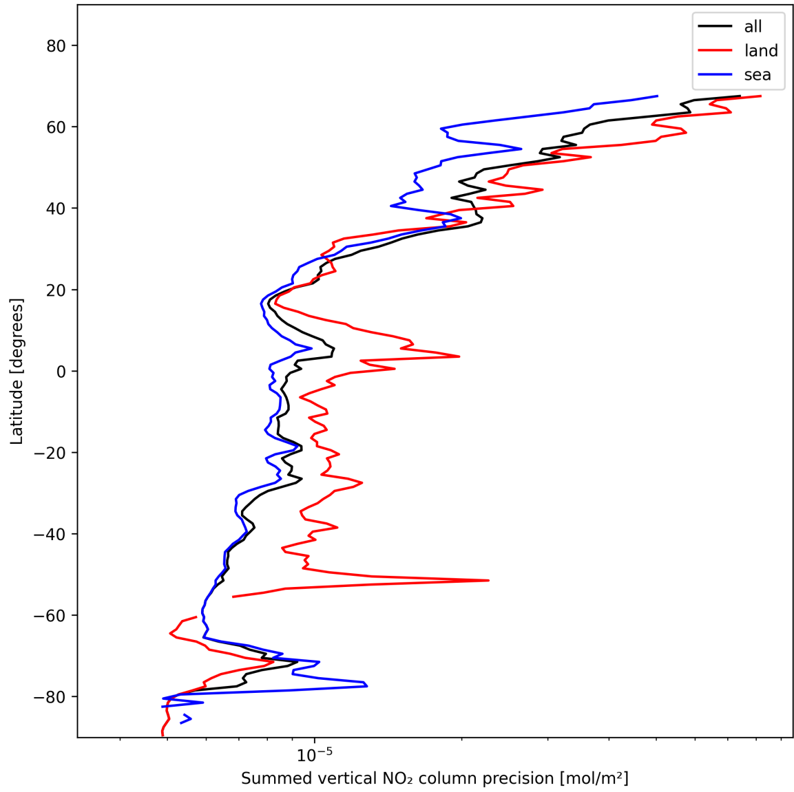
Figure 24: Zonal average of “Summed vertical NO 2 column precision” for 2025-01-18 to 2025-01-20.
