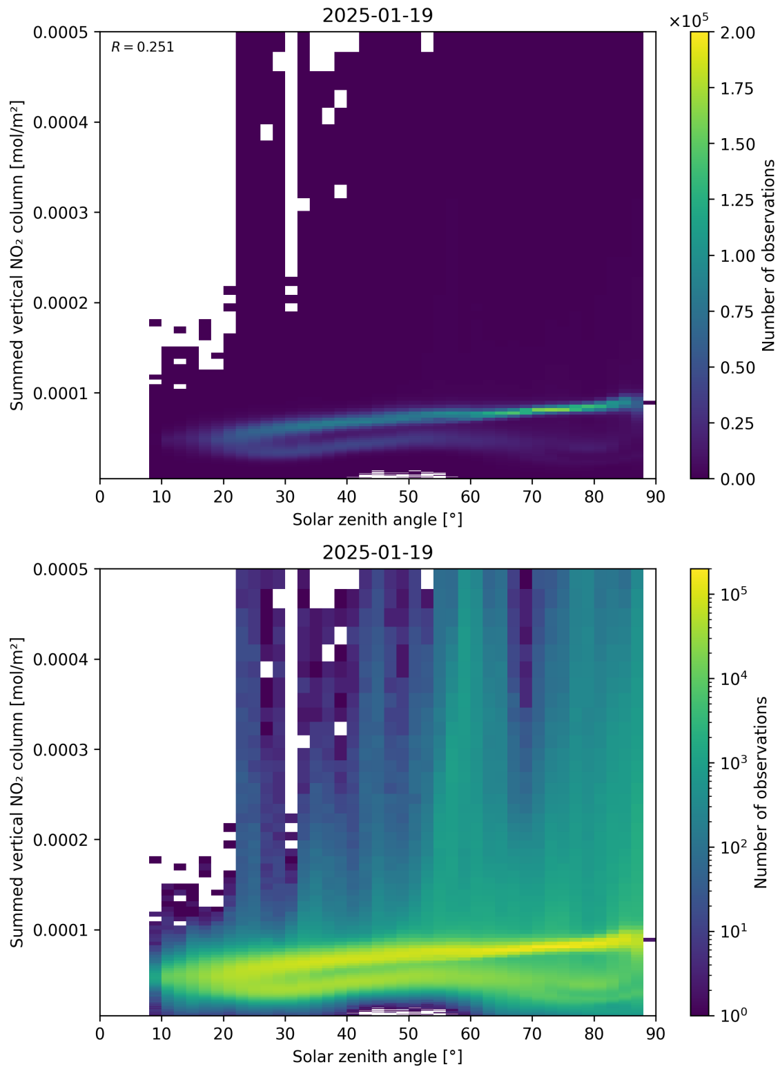
Figure 151: Scatter density plot of “Solar zenith angle” against “Summed vertical NO 2 column” for 2025-01-18 to 2025-01-20.
