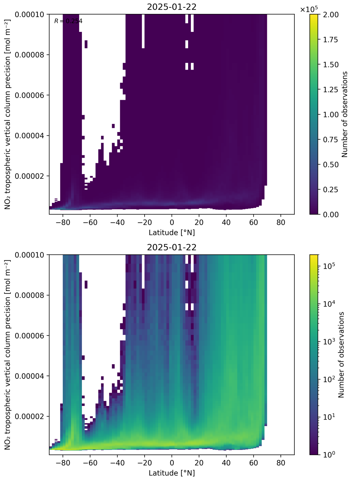
Figure 93: Scatter density plot of “Latitude” against “NO 2 tropospheric vertical column precision” for 2025-01-21 to 2025-01-23.
