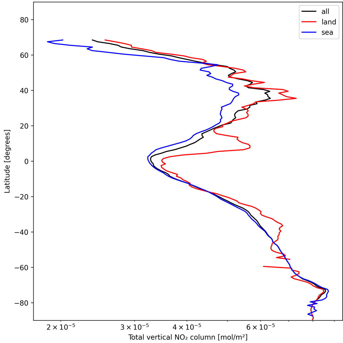
Figure 21: Zonal average of “Total vertical NO 2 column” for 2025-01-21 to 2025-01-23.
