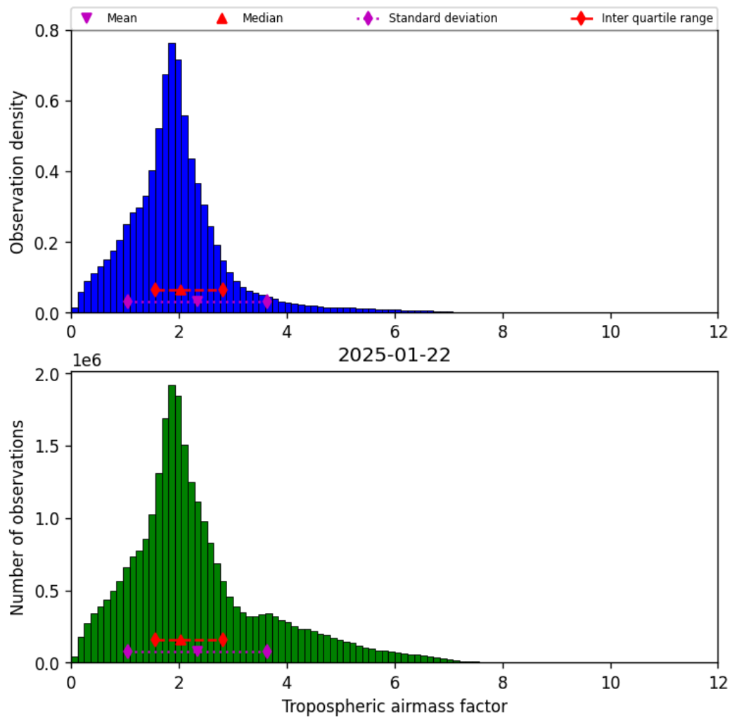
Figure 31: Histogram of “Tropospheric airmass factor” for 2025-01-21 to 2025-01-23
