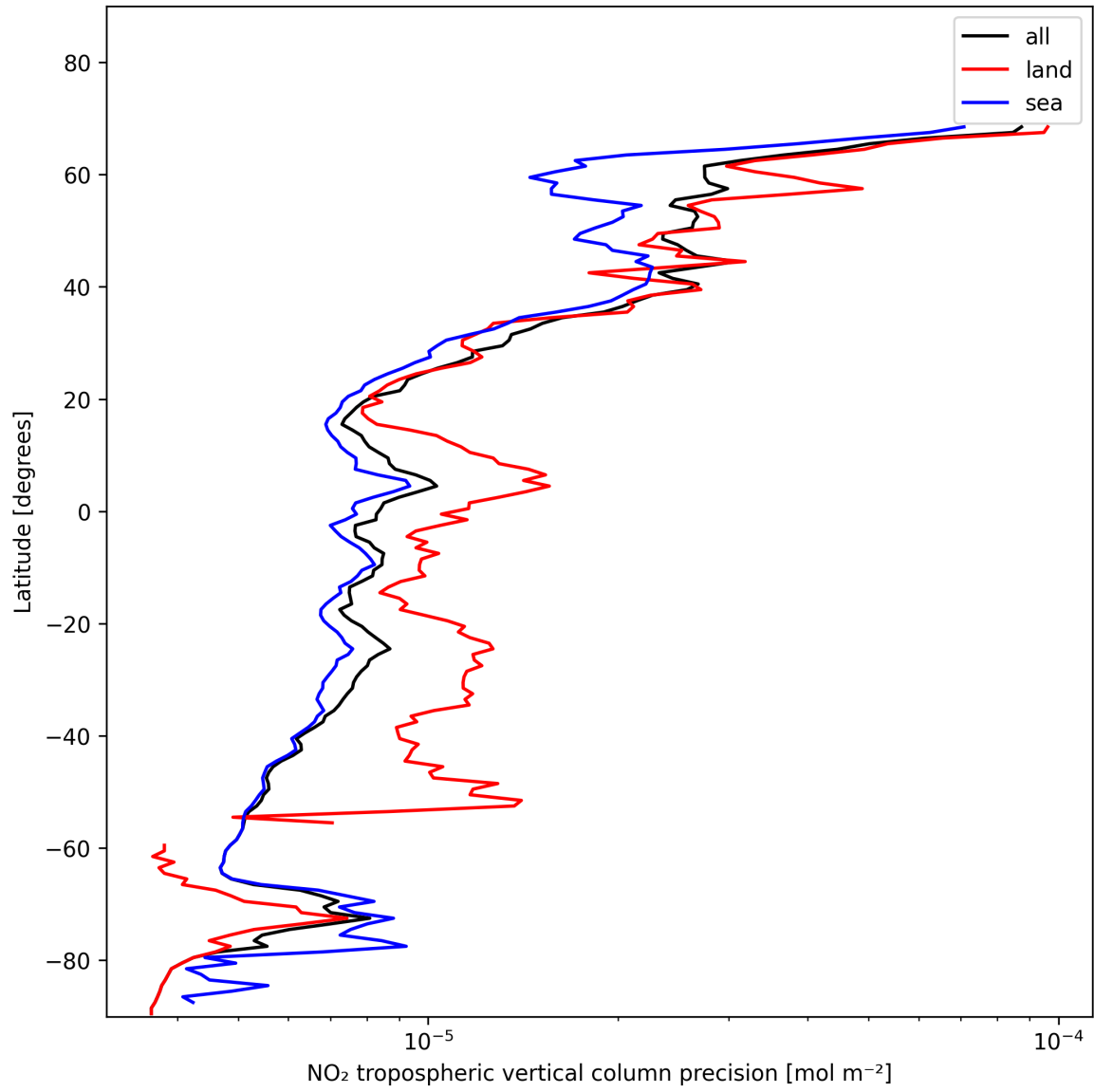
Figure 13: Zonal average of “NO 2 tropospheric vertical column precision” for 2025-01-21 to 2025-01-23.
