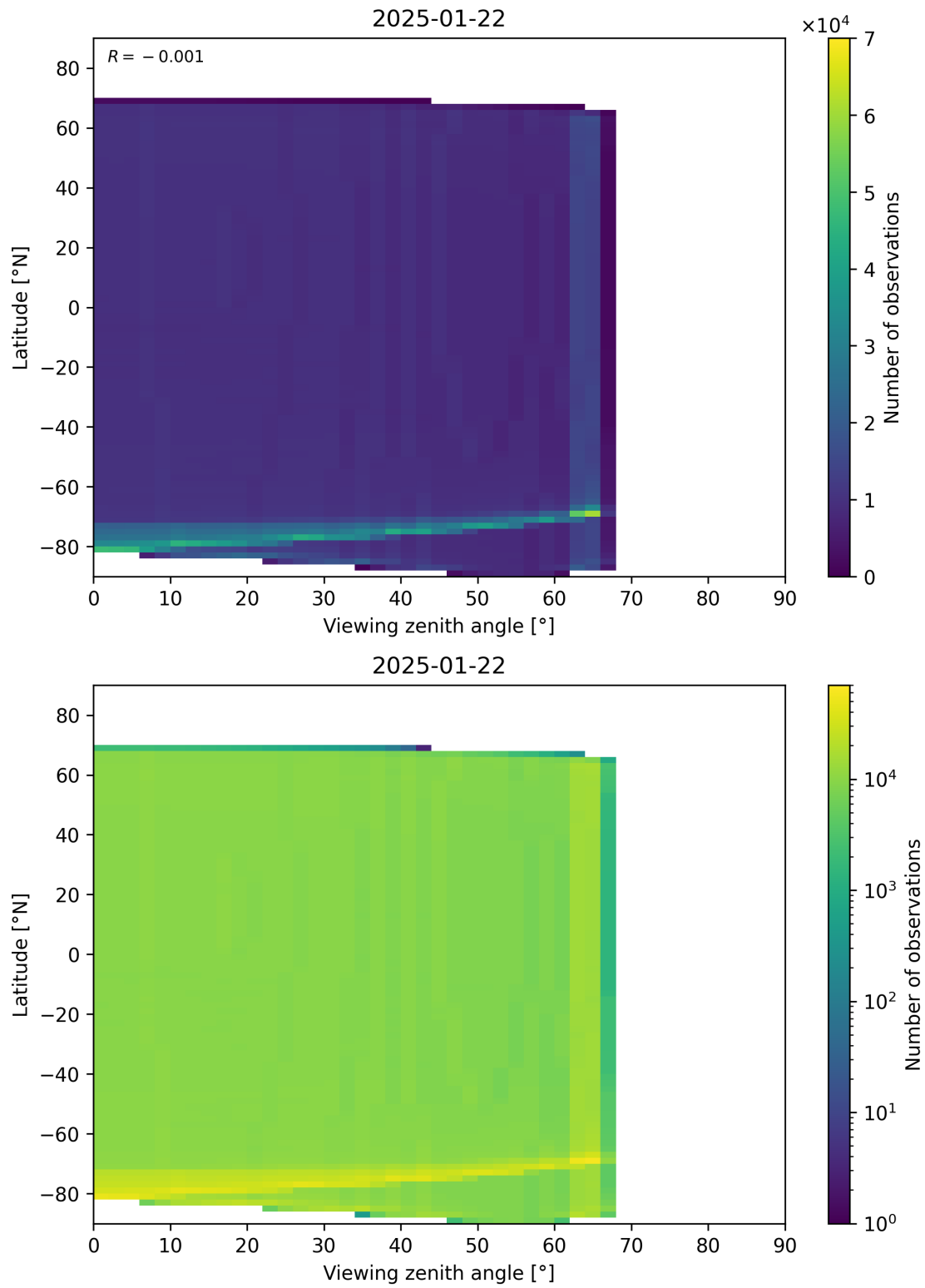
Figure 163: Scatter density plot of “Viewing zenith angle” against “Latitude” for 2025-01-21 to 2025-01-23.
