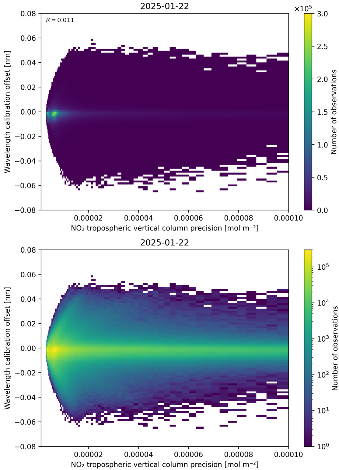
Figure 141: Scatter density plot of “NO 2 tropospheric vertical column precision” against “Wavelength calibration offset” for 2025-01-21 to 2025-01-23.
