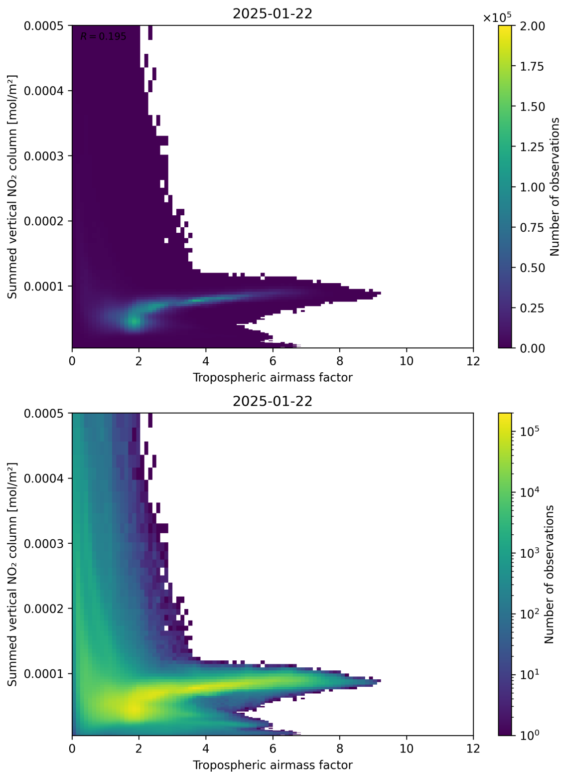
Figure 75: Scatter density plot of “Tropospheric airmass factor” against “Summed vertical NO 2 column” for 2025-01-21 to 2025-01-23.
