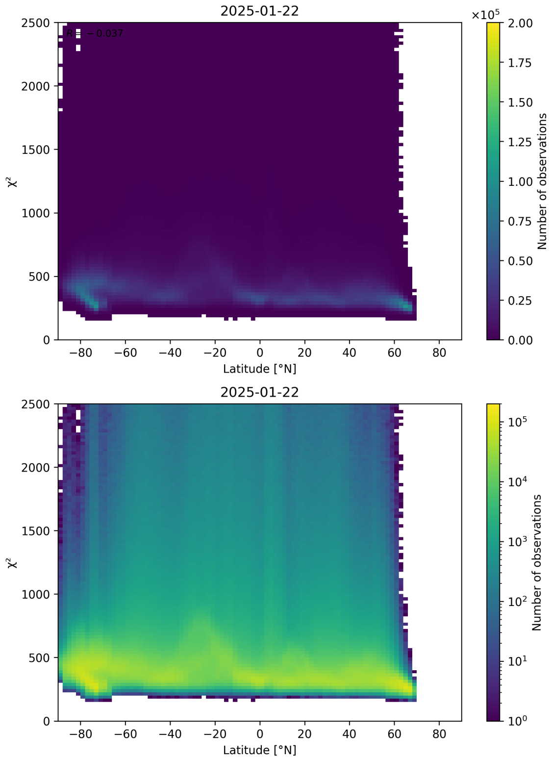
Figure 86: Scatter density plot of “Latitude” against “ \chi^2 ” for 2025-01-21 to 2025-01-23.
