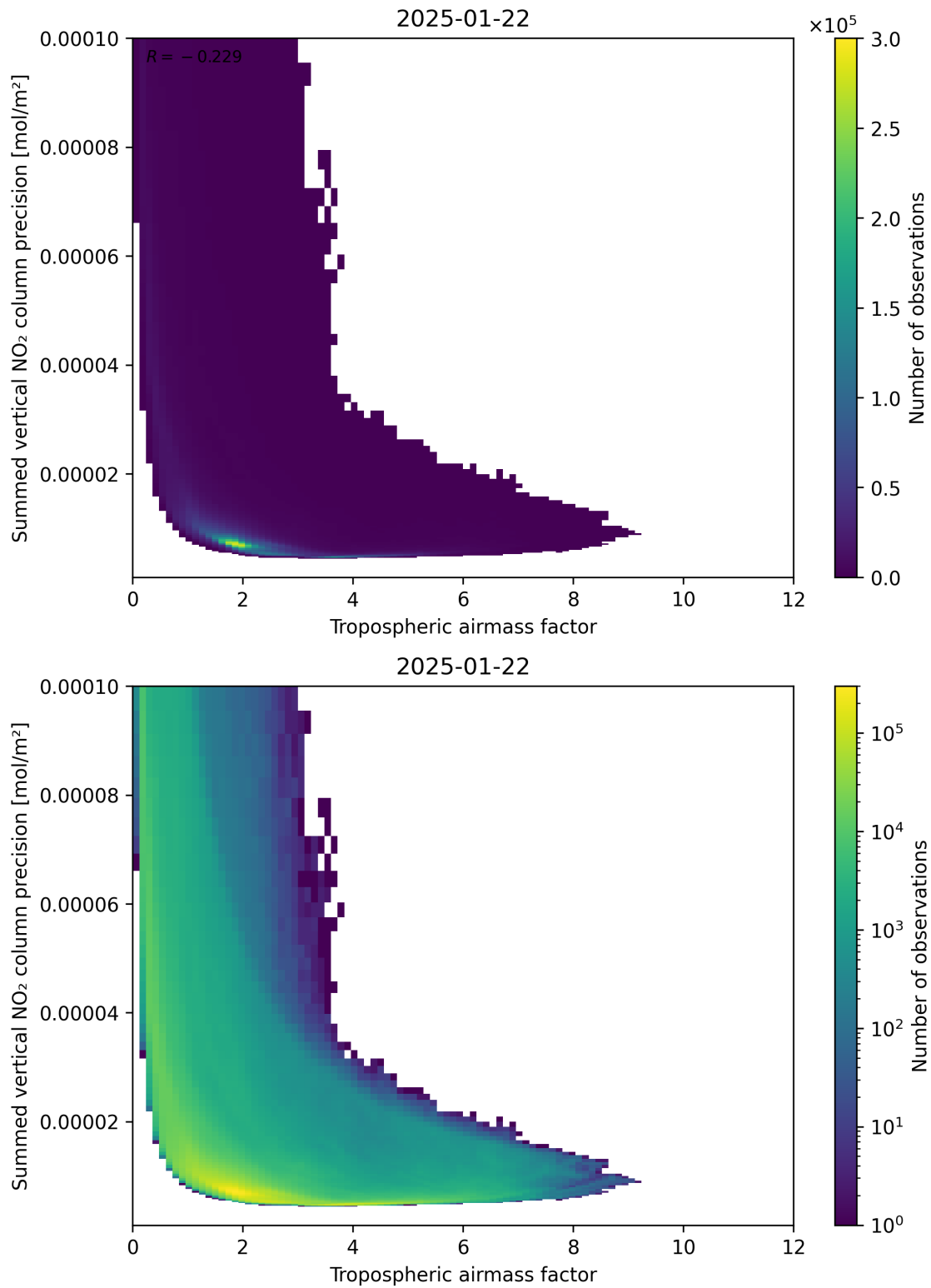
Figure 76: Scatter density plot of “Tropospheric air mass factor” against “Summed vertical NO 2 column precision” for 2025-01-21 to 2025-01-23.
