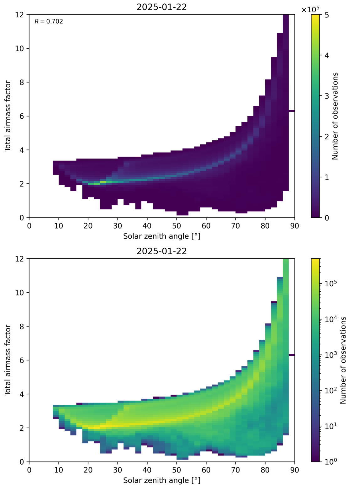
Figure 146: Scatter density plot of “Solar zenith angle” against “Total air mass factor” for 2025-01-21 to 2025-01-23.
