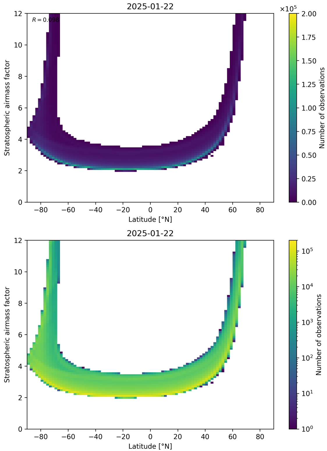
Figure 83: Scatter density plot of “Latitude” against “Stratospheric air mass factor” for 2025-01-21 to 2025-01-23.
