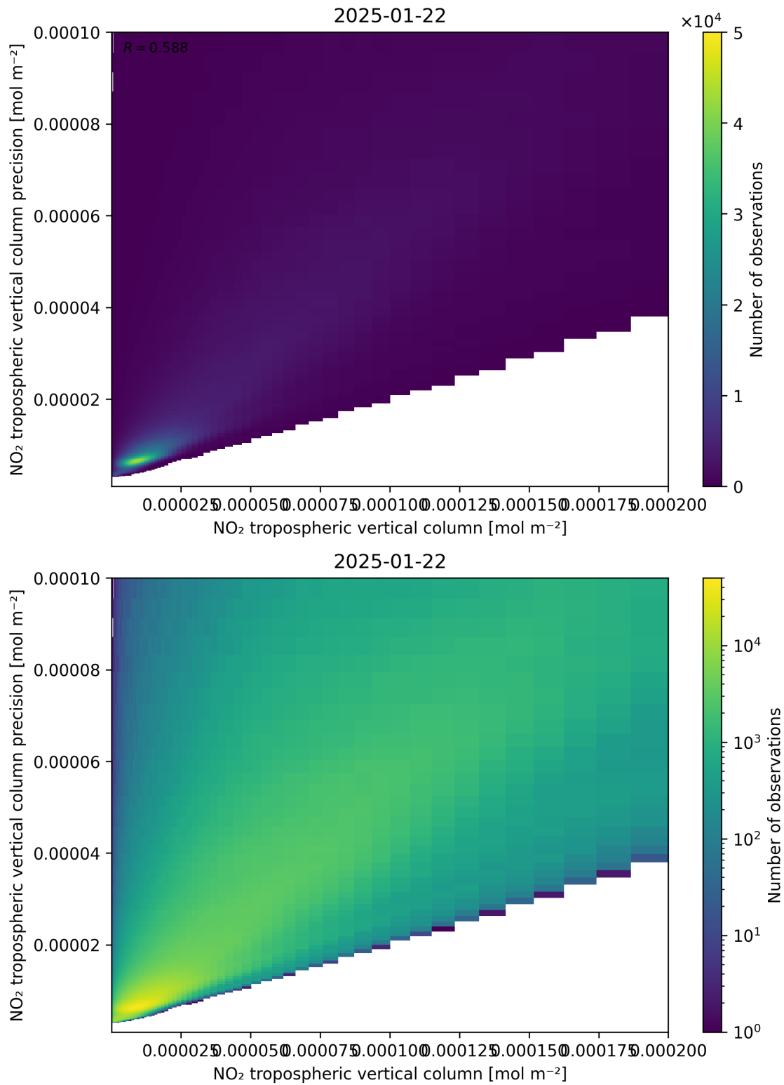
Figure 130: Scatter density plot of “NO 2 tropospheric vertical column” against “NO 2 tropospheric vertical column precision” for 2025-01-21 to 2025-01-23.
