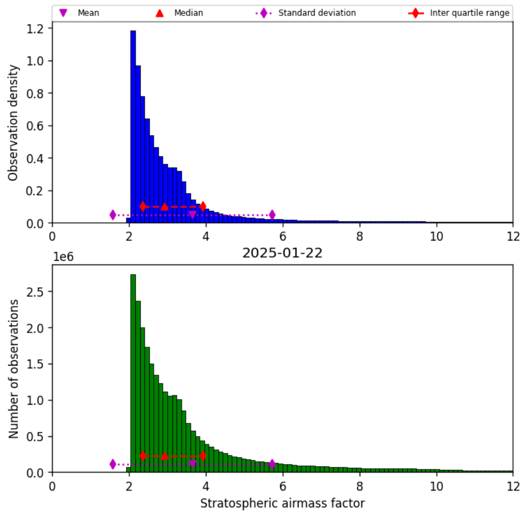
Figure 44: Histogram of “Stratospheric airmass factor” for 2025-01-21 to 2025-01-23
