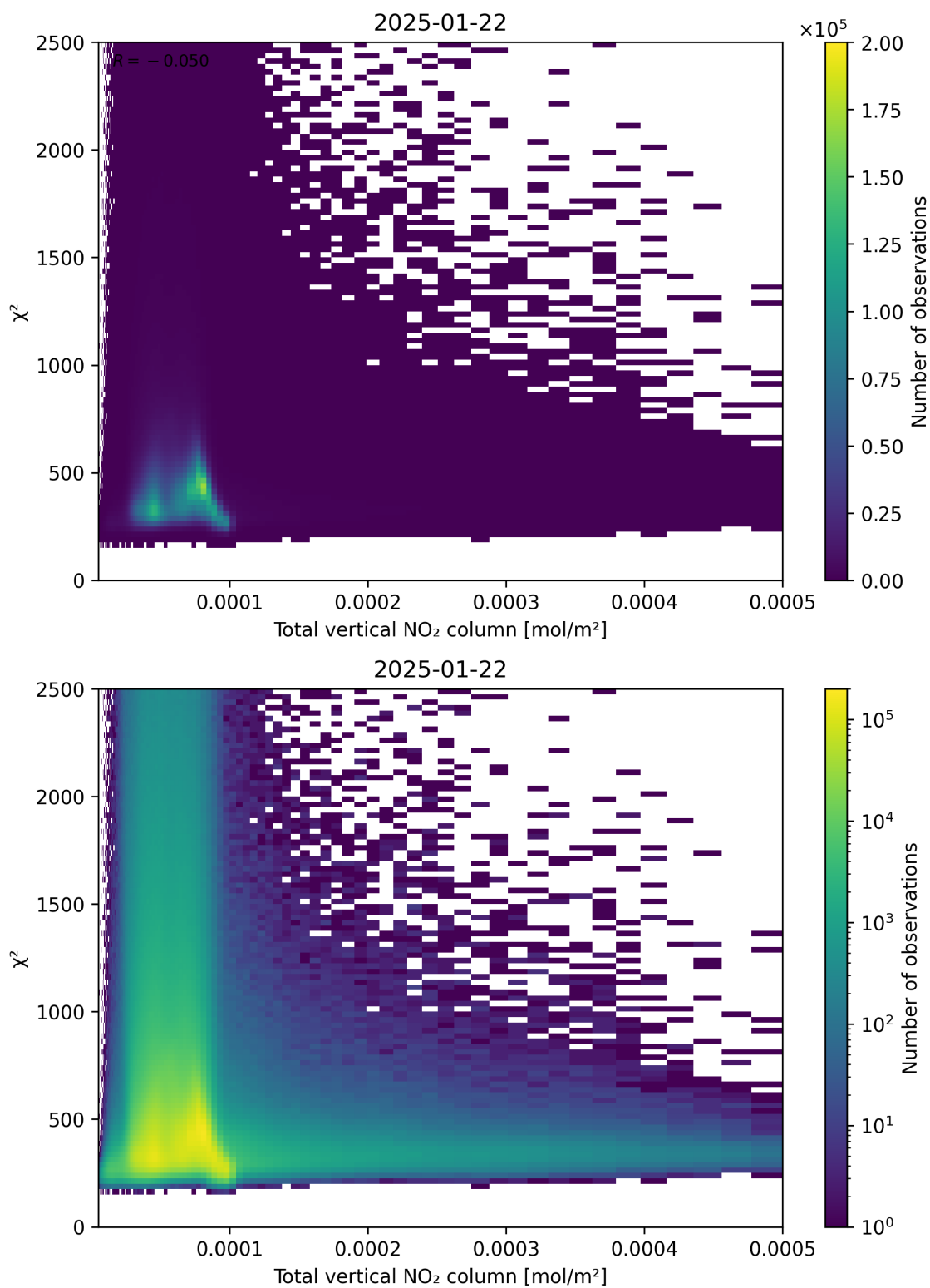
Figure 111: Scatter density plot of “Total vertical NO 2 column” against “ \chi^2 ” for 2025-01-21 to 2025-01-23.
