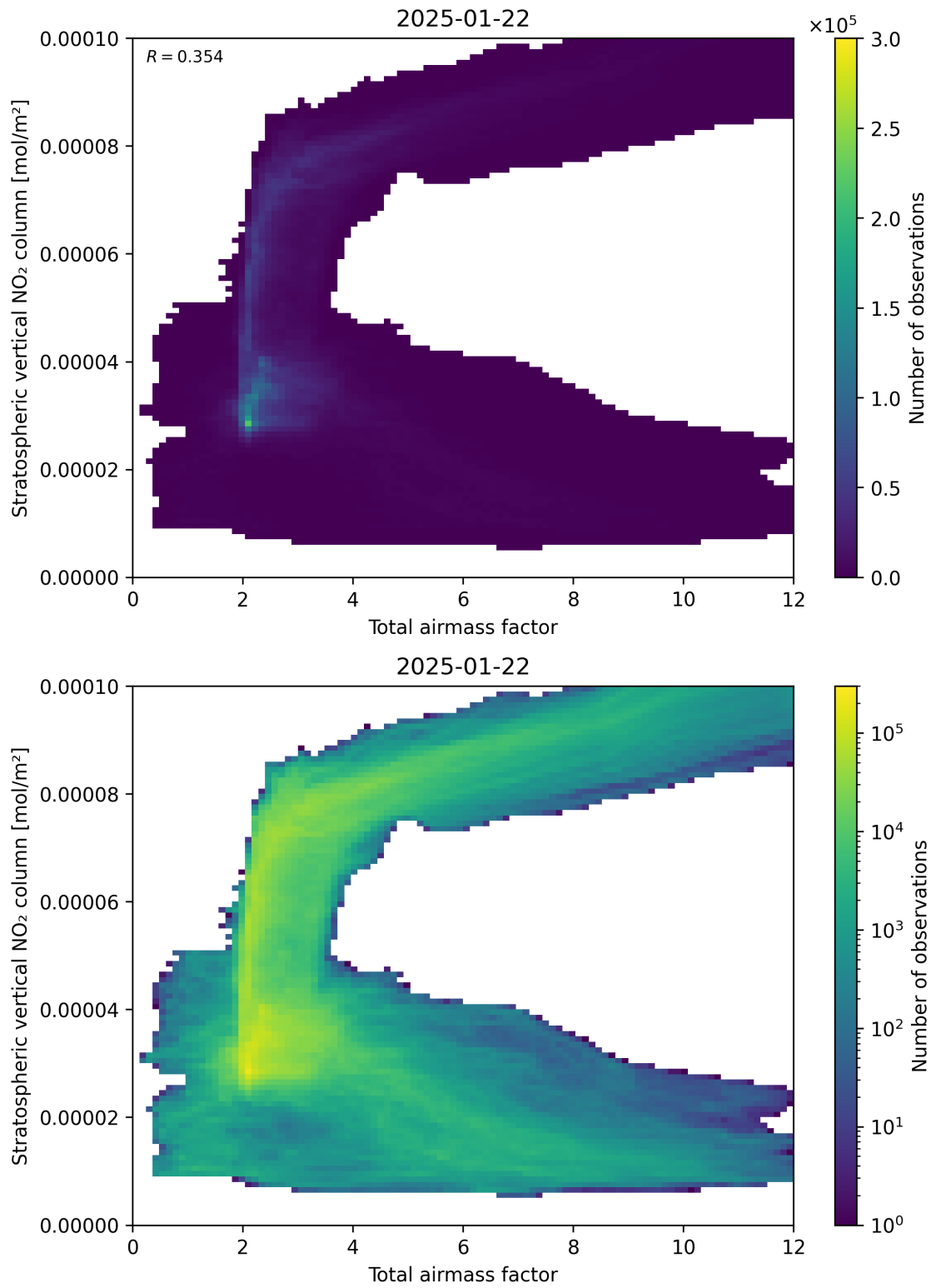
Figure 64: Scatter density plot of “Total airmass factor” against “Stratospheric vertical \text{NO}_2 column” for 2025-01-21 to 2025-01-23.
