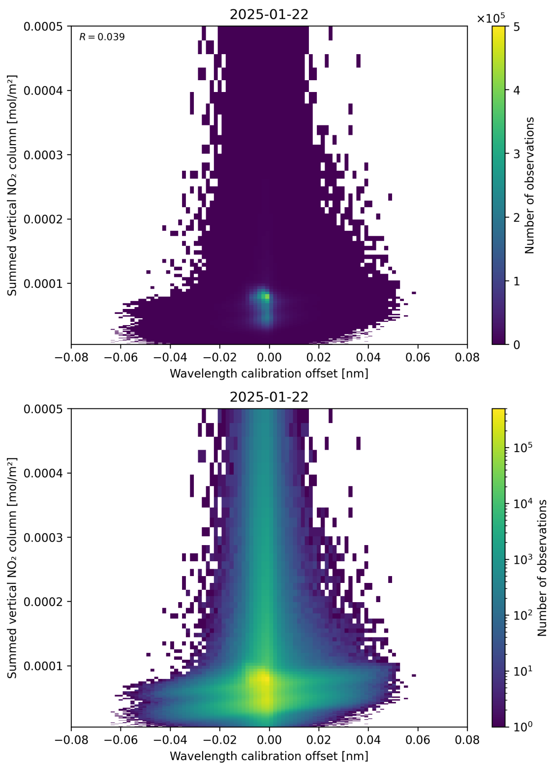
Figure 177: Scatter density plot of “Wavelength calibration offset” against “Summed vertical NO 2 column” for 2025-01-21 to 2025-01-23.
