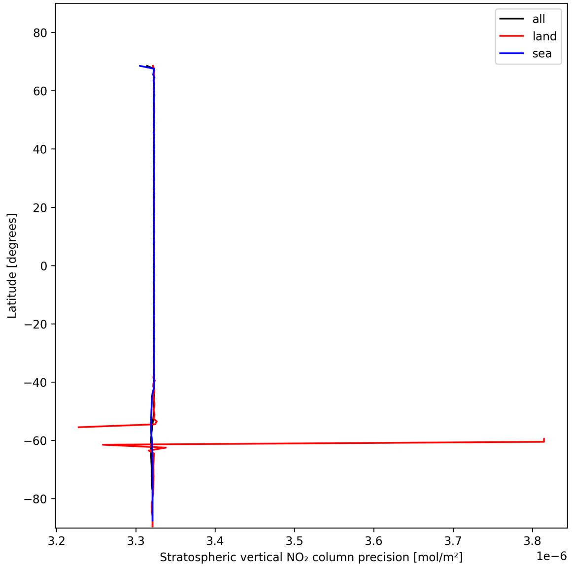
Figure 20: Zonal average of “Stratospheric vertical NO 2 column precision” for 2025-01-21 to 2025-01-23.
