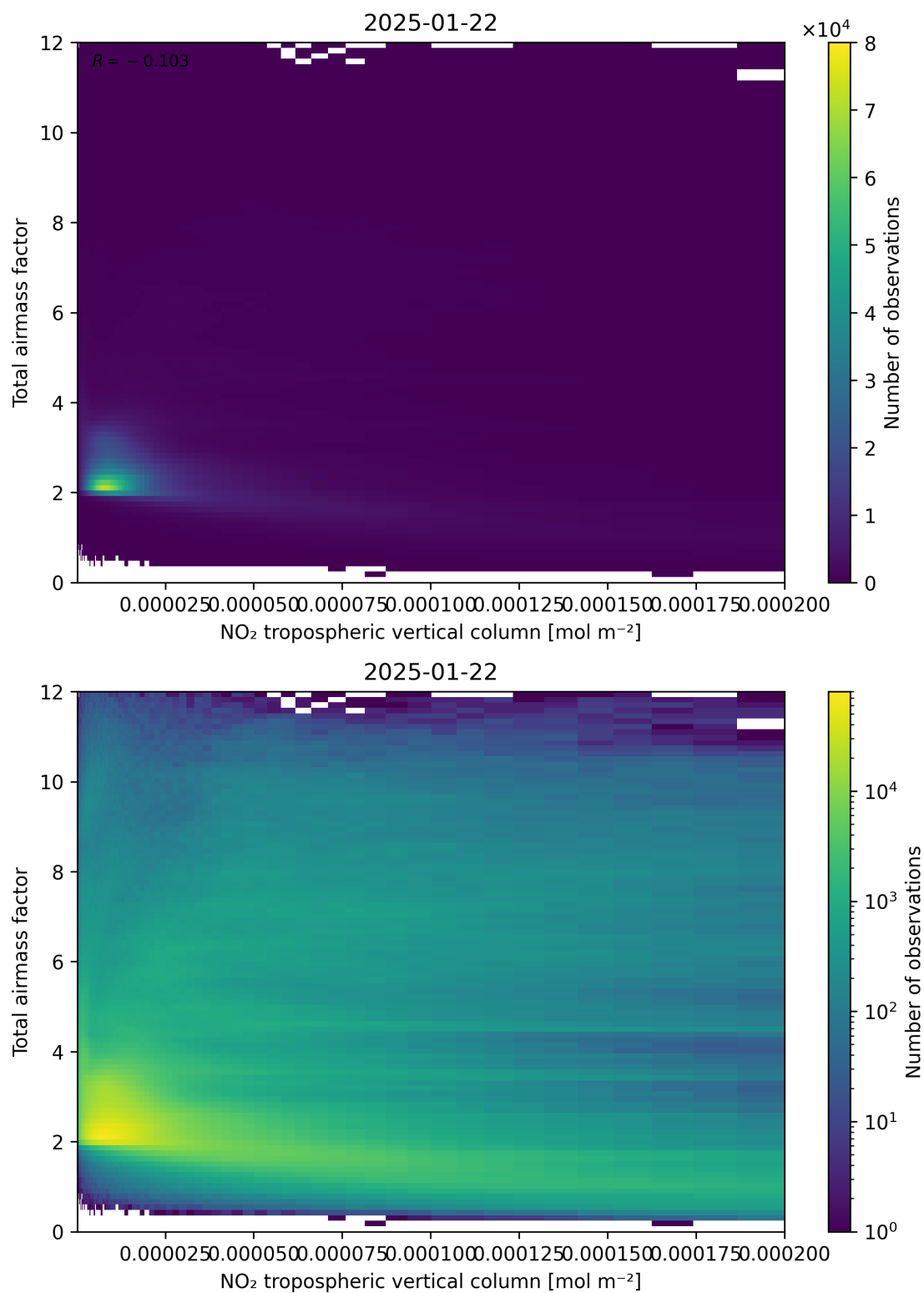
Figure 122: Scatter density plot of “NO 2 tropospheric vertical column” against “Total air mass factor” for 2025-01-21 to 2025-01-23.
