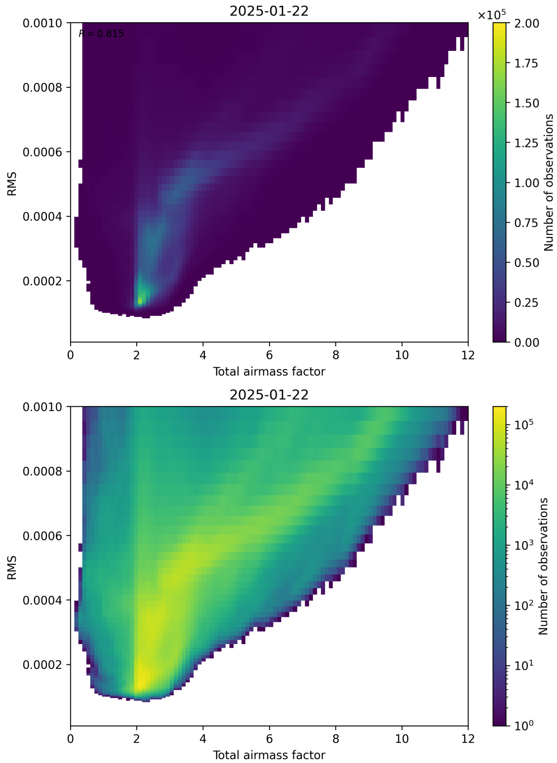
Figure 69: Scatter density plot of “Total airmass factor” against “RMS” for 2025-01-21 to 2025-01-23.
