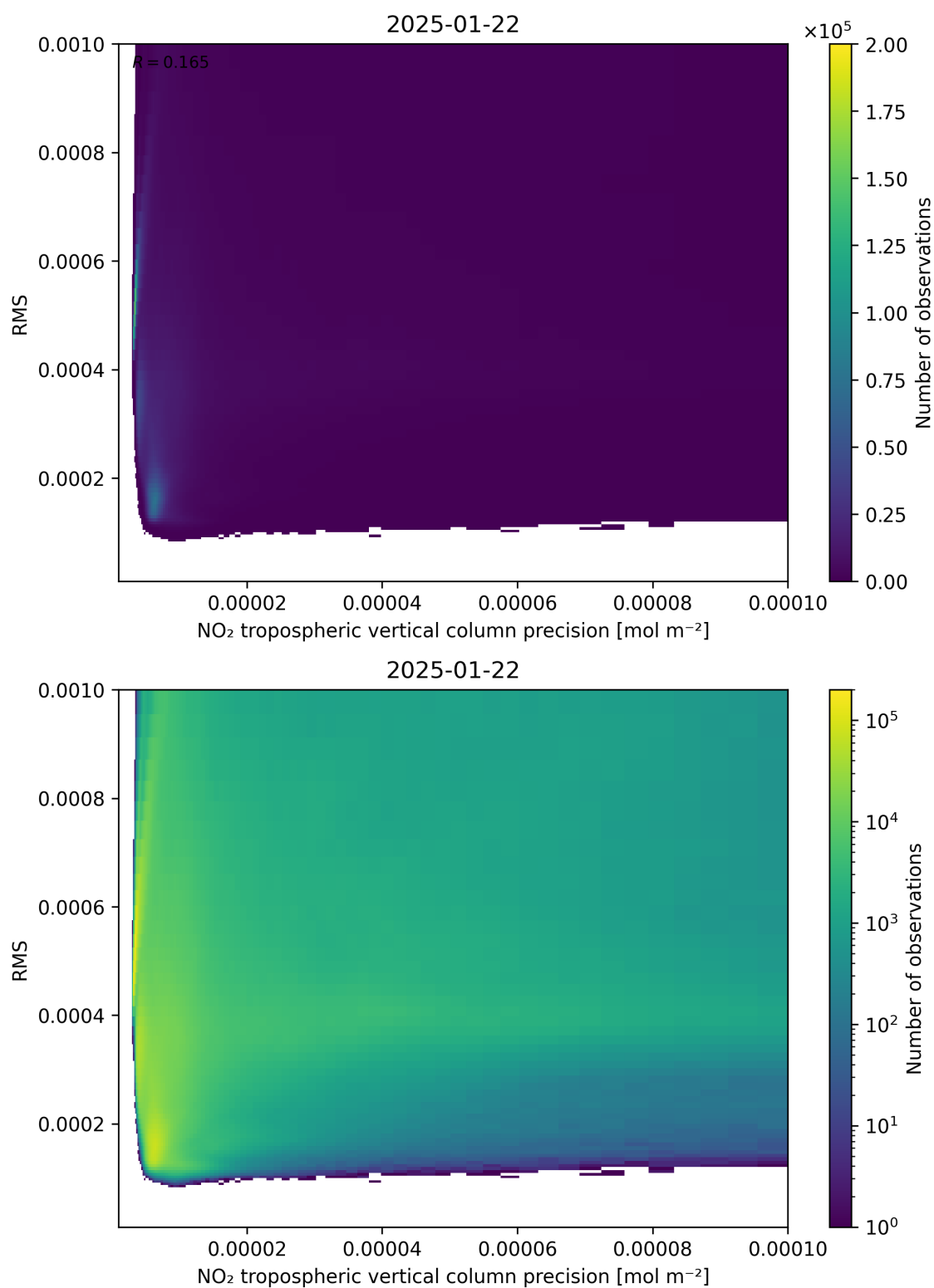
Figure 140: Scatter density plot of “NO 2 tropospheric vertical column precision” against “RMS” for 2025-01-21 to 2025-01-23.
