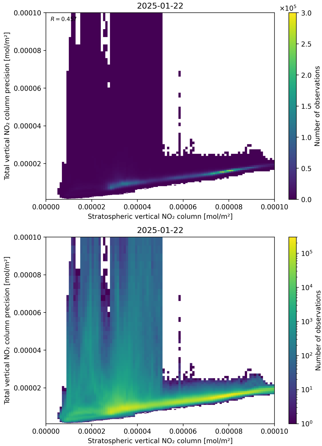
Figure 101: Scatter density plot of “Stratospheric vertical NO 2 column” against “Total vertical NO 2 column precision” for 2025-01-21 to 2025-01-23.
