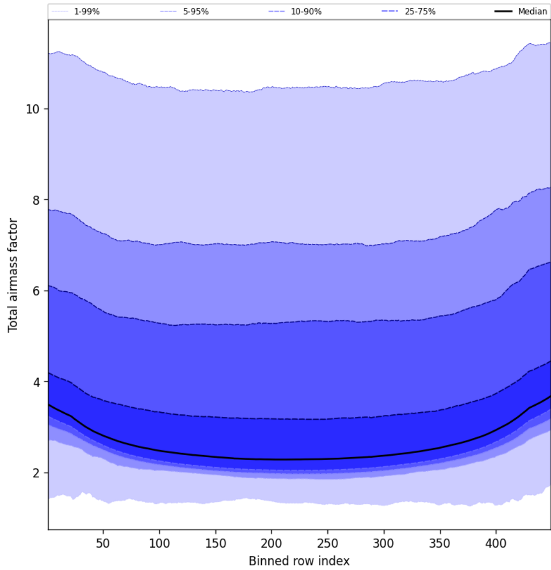
Figure 49: Along track statistics of “Total airmass factor” for 2025-01-21 to 2025-01-23
