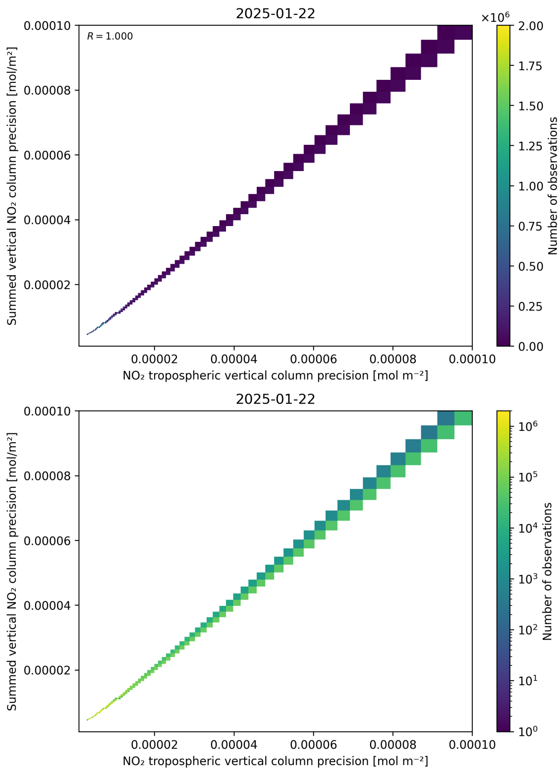
Figure 137: Scatter density plot of “NO 2 tropospheric vertical column precision” against “Summed vertical NO 2 column precision” for 2025-01-21 to 2025-01-23.
