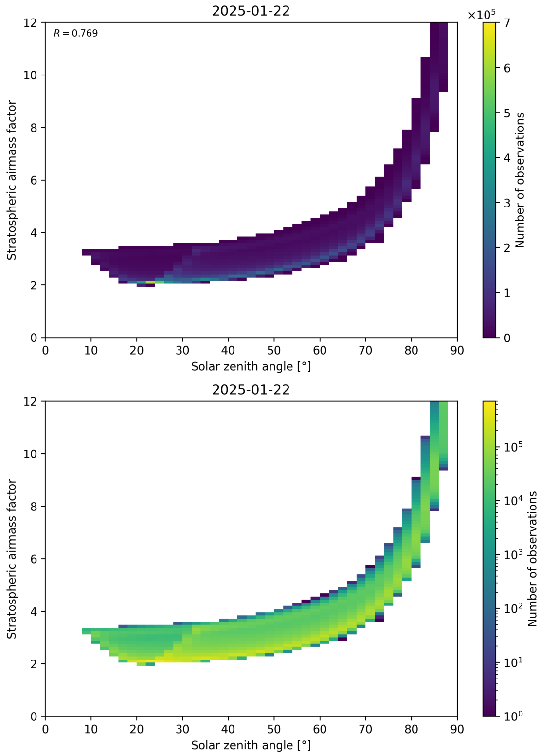
Figure 145: Scatter density plot of “Solar zenith angle” against “Stratospheric airmass factor” for 2025-01-21 to 2025-01-23.
