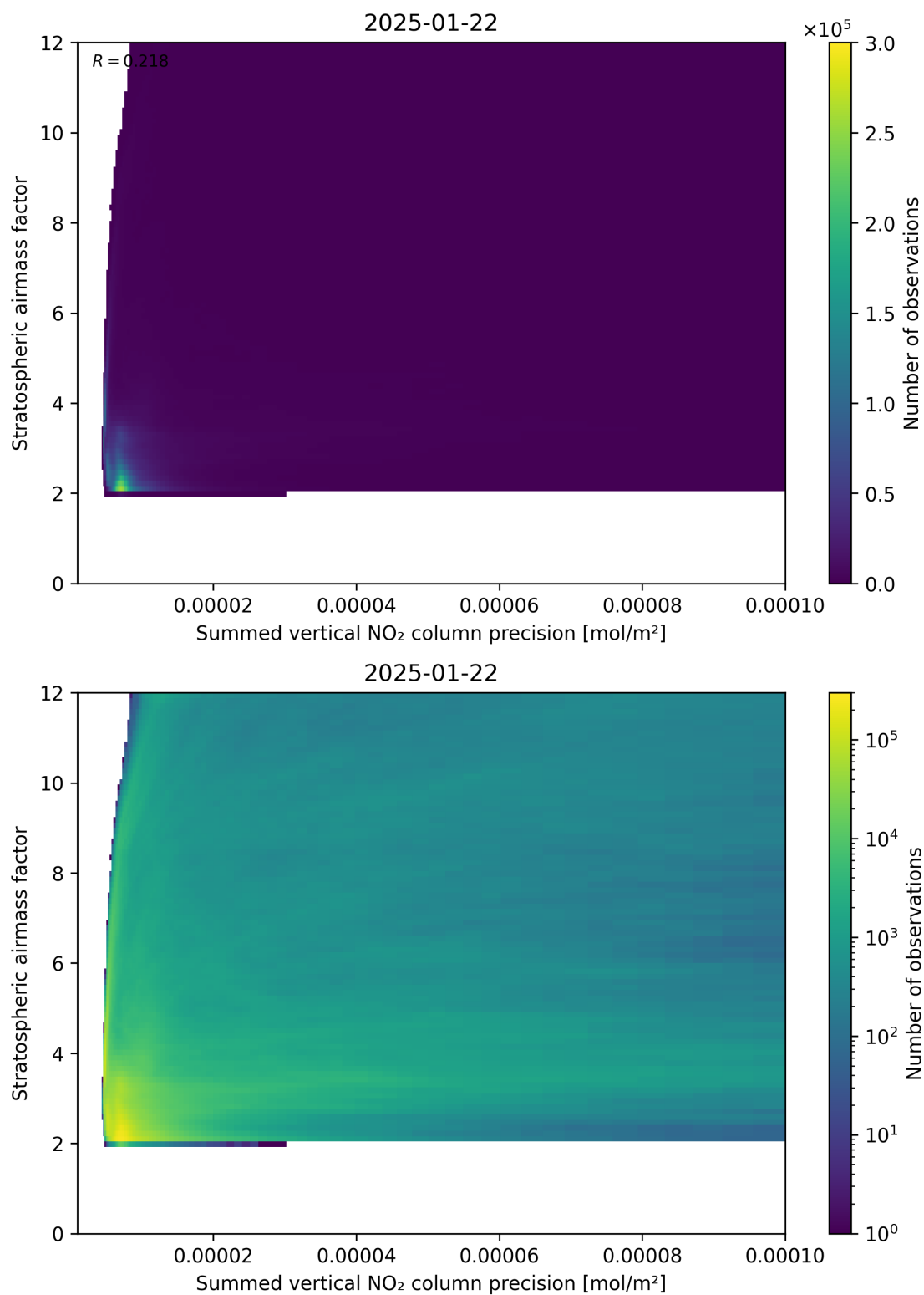
Figure 106: Scatter density plot of “Summed vertical NO 2 column precision” against “Stratospheric airmass factor” for 2025-01-21 to 2025-01-23.
