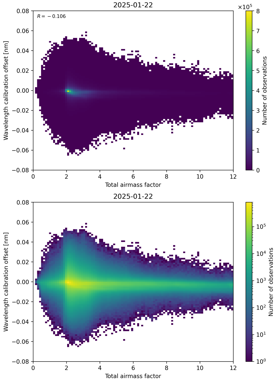
Figure 70: Scatter density plot of “Total airmass factor” against “Wavelength calibration offset” for 2025-01-21 to 2025-01-23.
