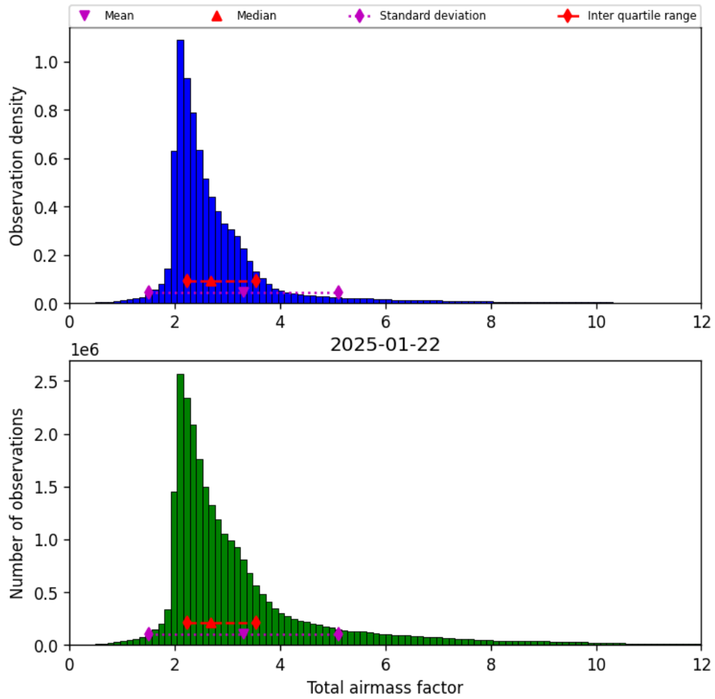
Figure 32: Histogram of “Total airmass factor” for 2025-01-21 to 2025-01-23
