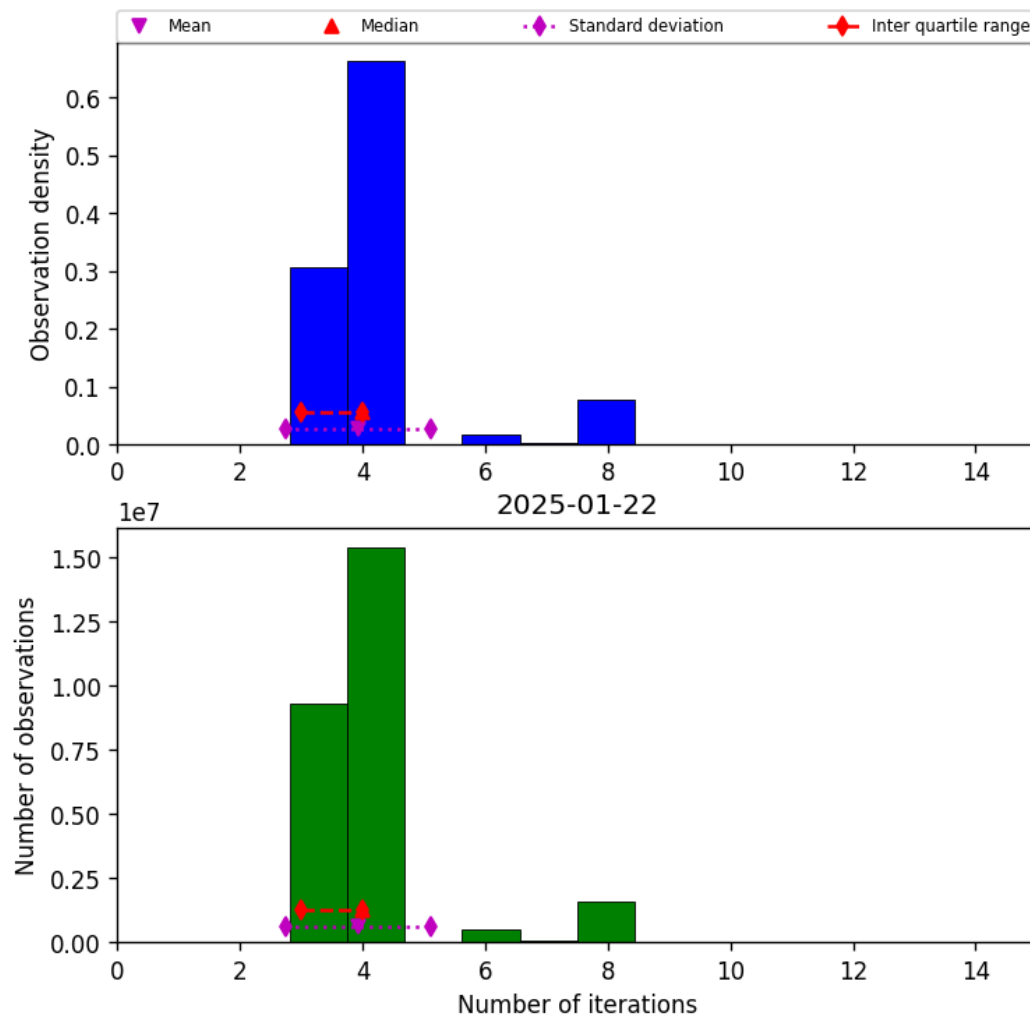
Figure 34: Histogram of “Number of iterations” for 2025-01-21 to 2025-01-23
