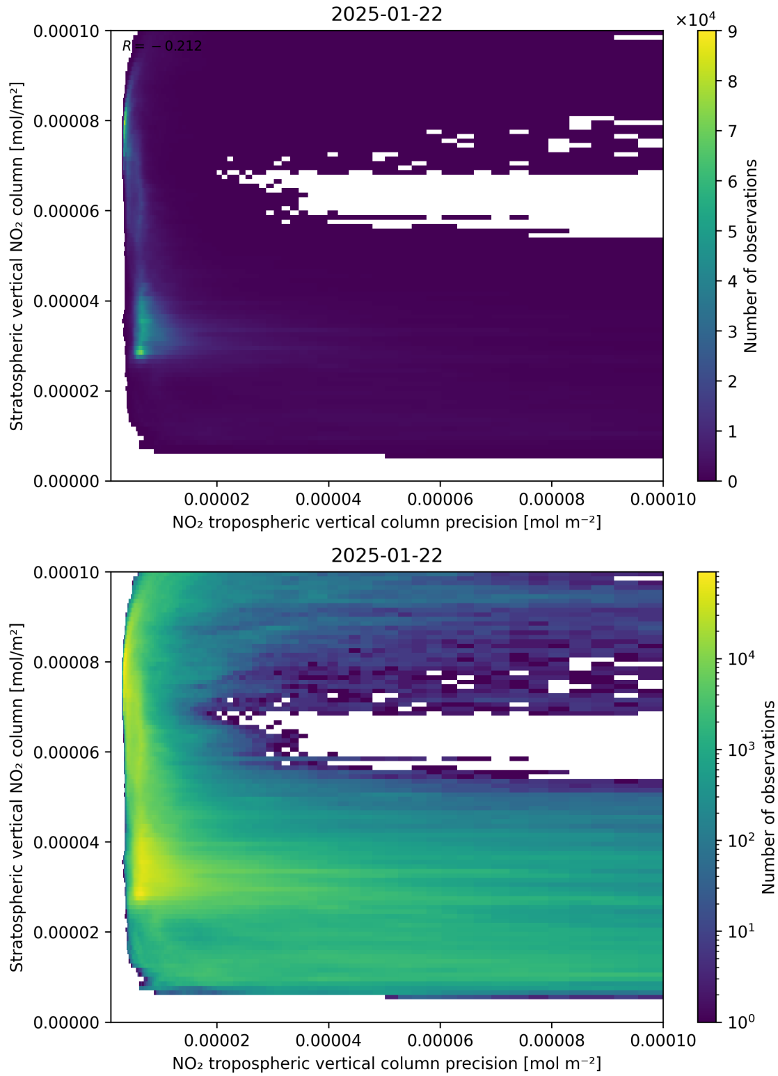
Figure 135: Scatter density plot of “NO 2 tropospheric vertical column precision” against “Stratospheric vertical NO 2 column” for 2025-01-21 to 2025-01-23.
