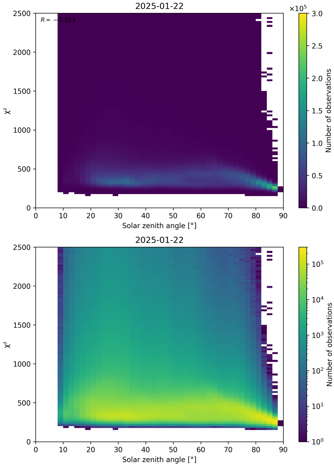
Figure 148: Scatter density plot of “Solar zenith angle” against “ \chi^2 ” for 2025-01-21 to 2025-01-23.
