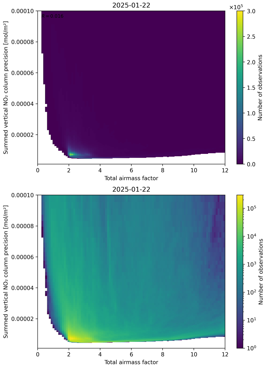
Figure 66: Scatter density plot of “Total airmass factor” against “Summed vertical NO 2 column precision” for 2025-01-21 to 2025-01-23.
