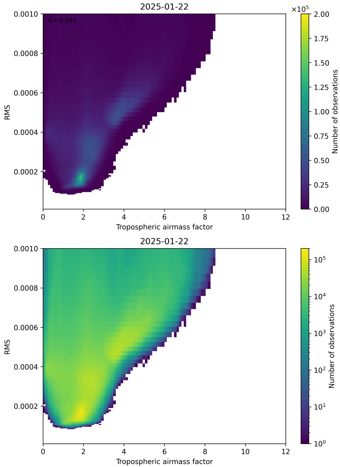
Figure 79: Scatter density plot of “Tropospheric airmass factor” against “RMS” for 2025-01-21 to 2025-01-23.
