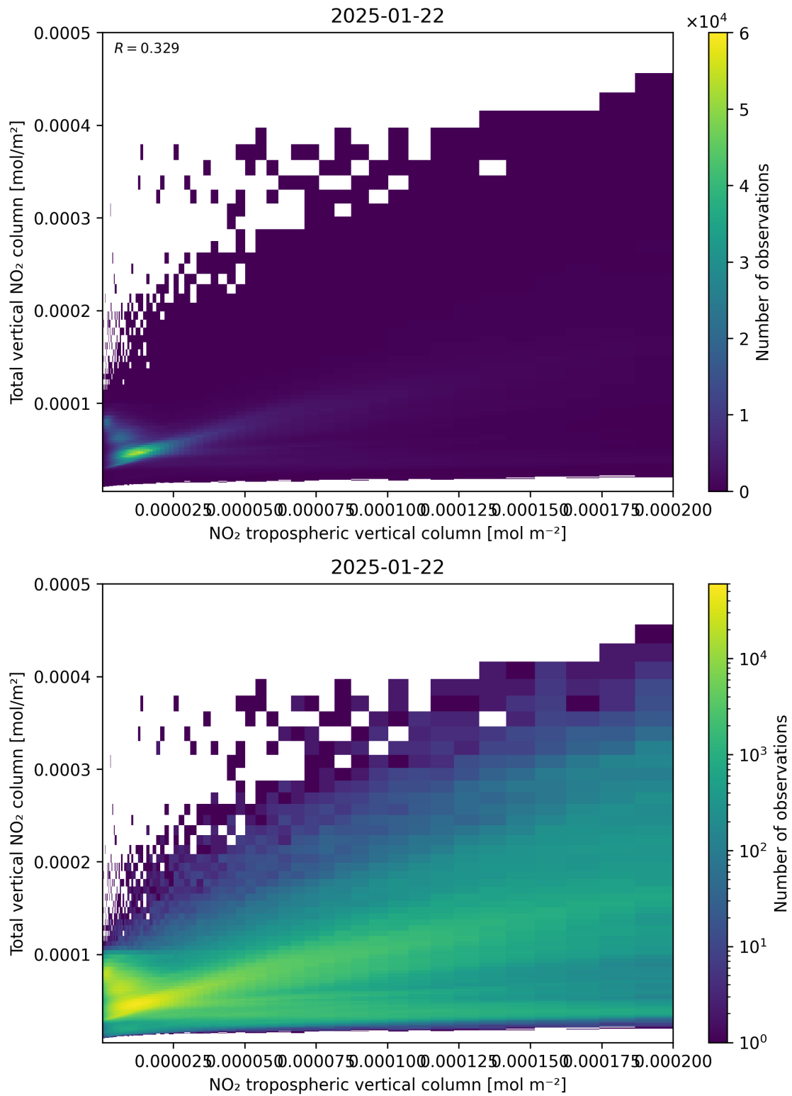
Figure 128: Scatter density plot of “NO 2 tropospheric vertical column” against “Total vertical NO 2 column” for 2025-01-21 to 2025-01-23.
