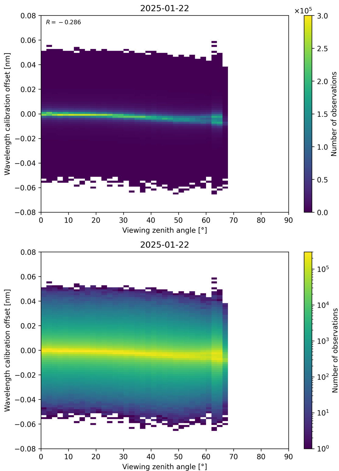
Figure 173: Scatter density plot of “Viewing zenith angle” against “Wavelength calibration offset” for 2025-01-21 to 2025-01-23.
