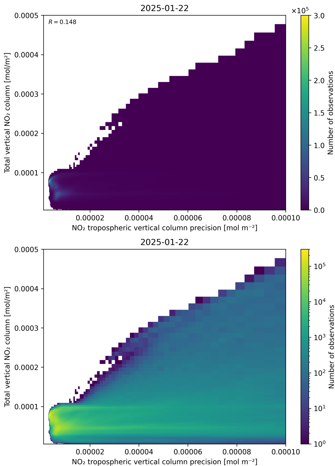
Figure 138: Scatter density plot of “NO 2 tropospheric vertical column precision” against “Total vertical NO 2 column” for 2025-01-21 to 2025-01-23.
