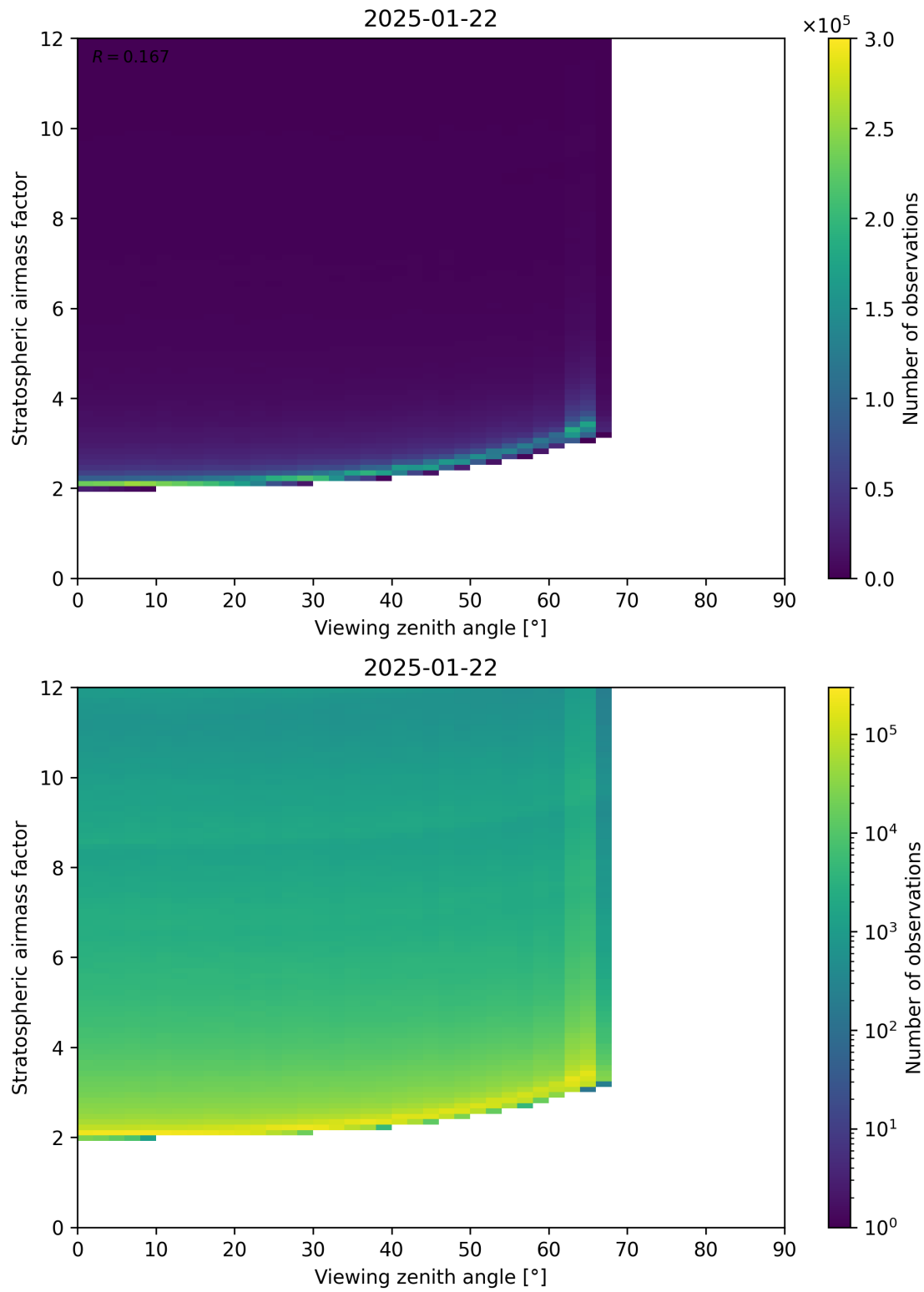
Figure 159: Scatter density plot of “Viewing zenith angle” against “Stratospheric airmass factor” for 2025-01-21 to 2025-01-23.
