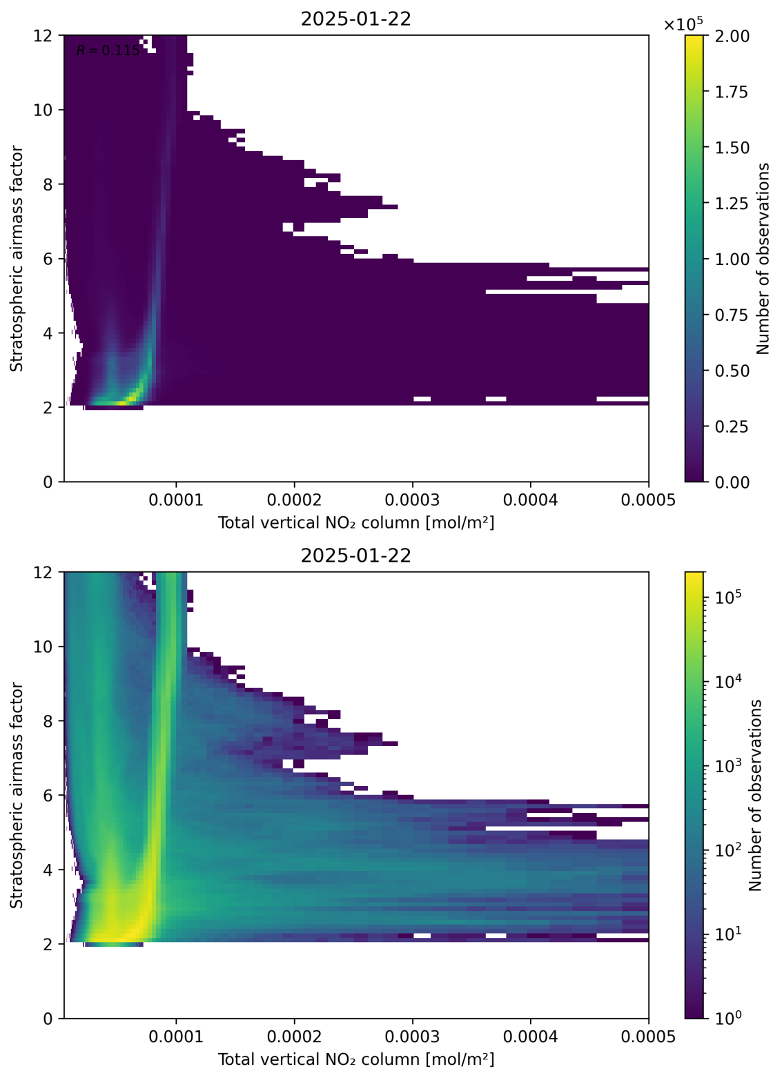
Figure 110: Scatter density plot of “Total vertical NO 2 column” against “Stratospheric airmass factor” for 2025-01-21 to 2025-01-23.
