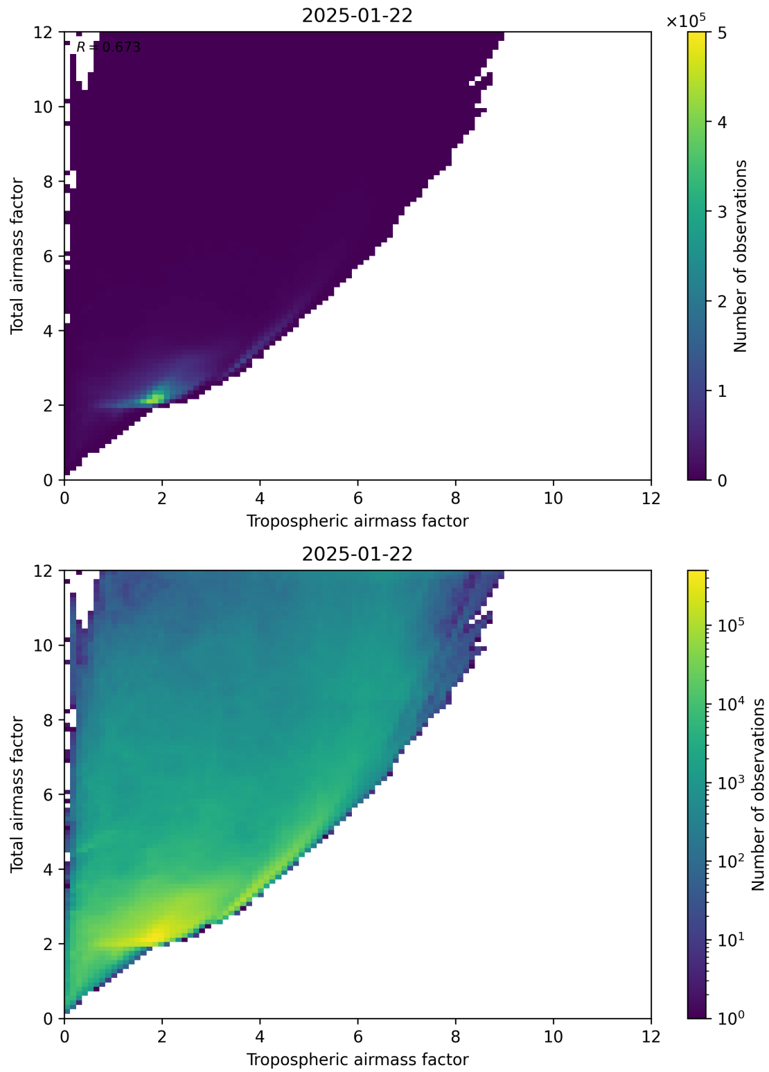
Figure 72: Scatter density plot of “Tropospheric airmass factor” against “Total airmass factor” for 2025-01-21 to 2025-01-23.
