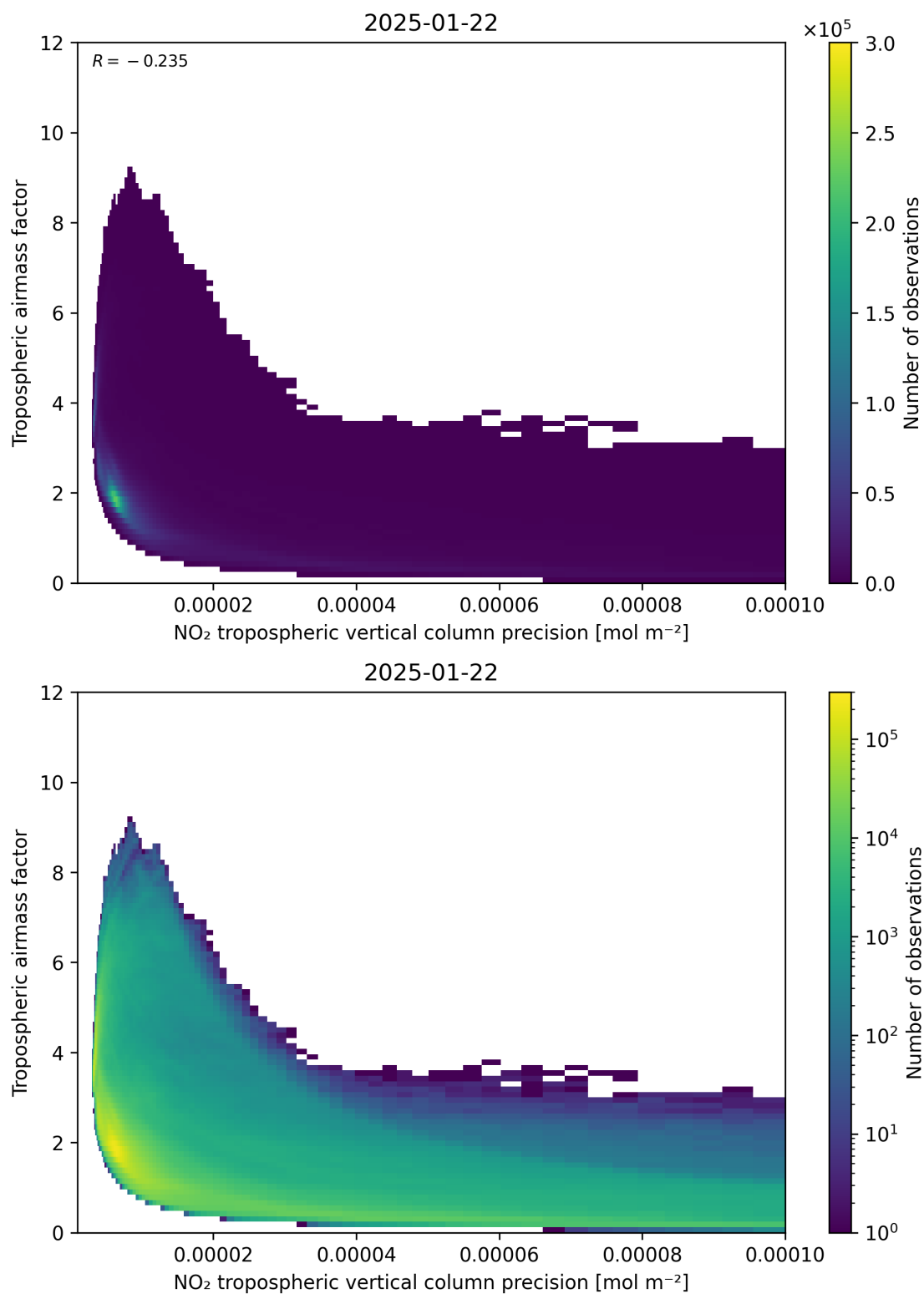
Figure 133: Scatter density plot of “NO 2 tropospheric vertical column precision” against “Tropospheric air mass factor” for 2025-01-21 to 2025-01-23.
