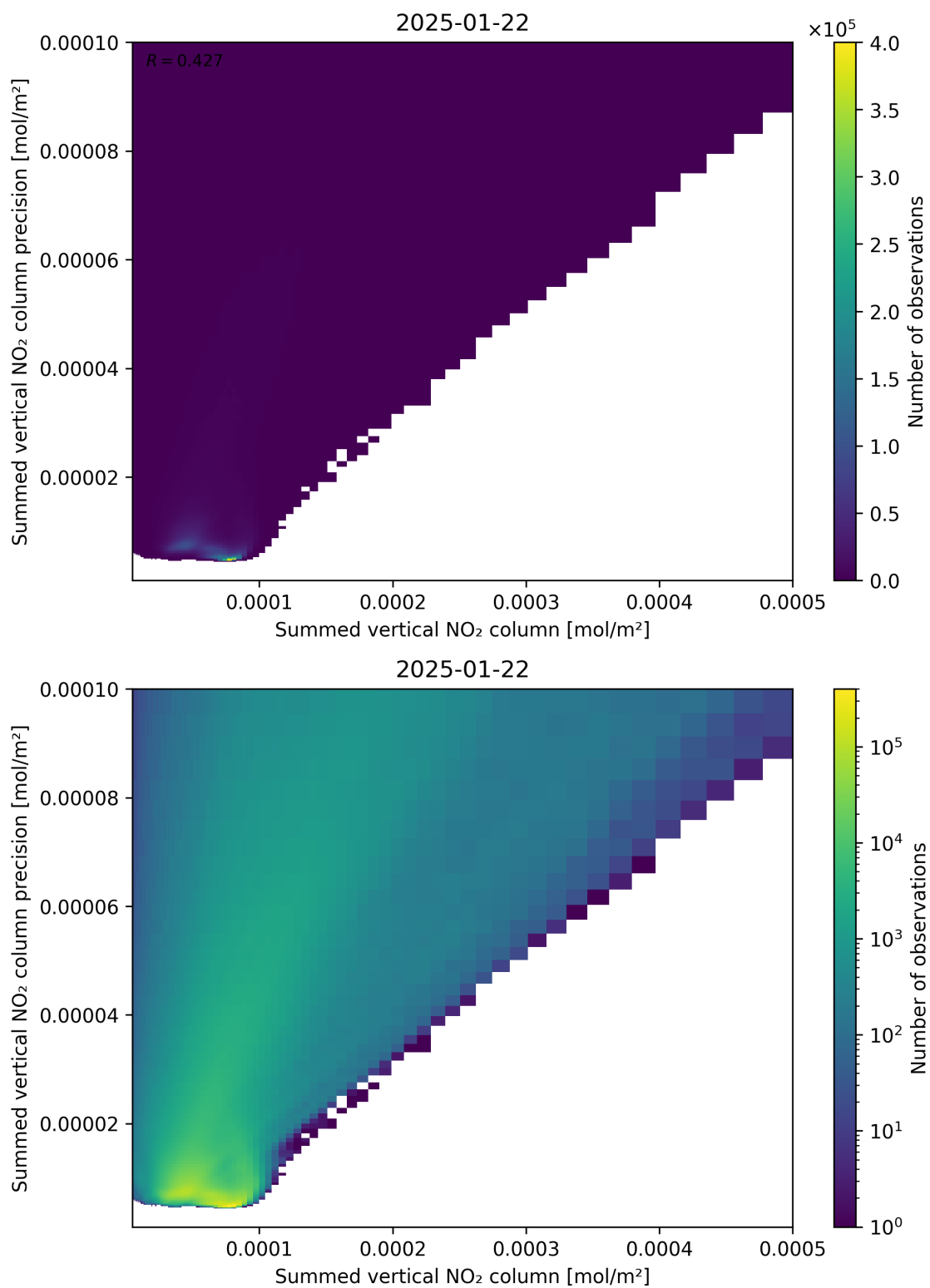
Figure 105: Scatter density plot of “Summed vertical NO 2 column” against “Summed vertical NO 2 column precision” for 2025-01-21 to 2025-01-23.
