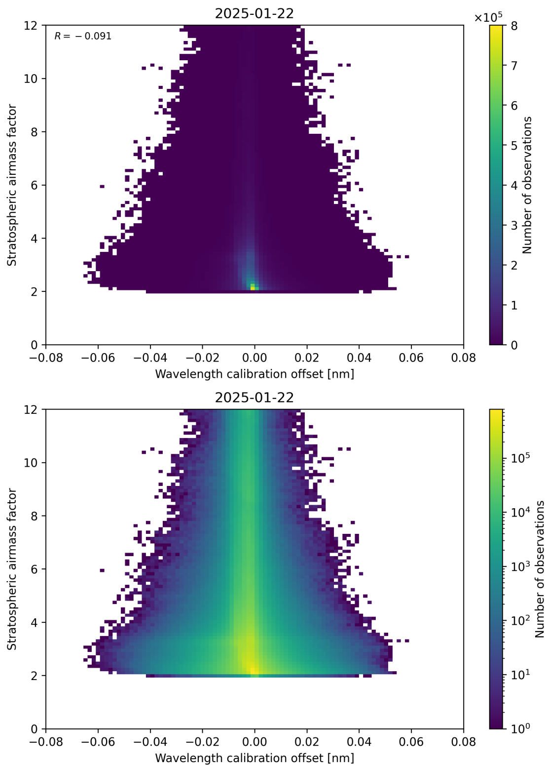
Figure 174: Scatter density plot of “Wavelength calibration offset” against “Stratospheric airmass factor” for 2025-01-21 to 2025-01-23.
