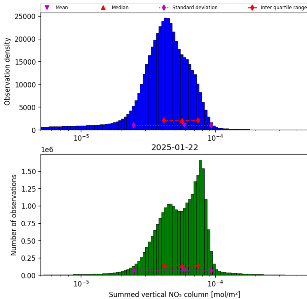
Figure 40: Histogram of “Summed vertical NO 2 column” for 2025-01-21 to 2025-01-23
