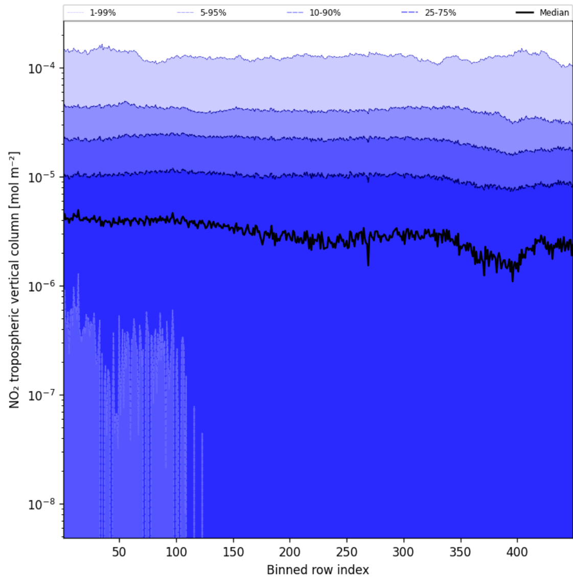
Figure 46: Along track statistics of “NO 2 tropospheric vertical column” for 2025-01-21 to 2025-01-23
