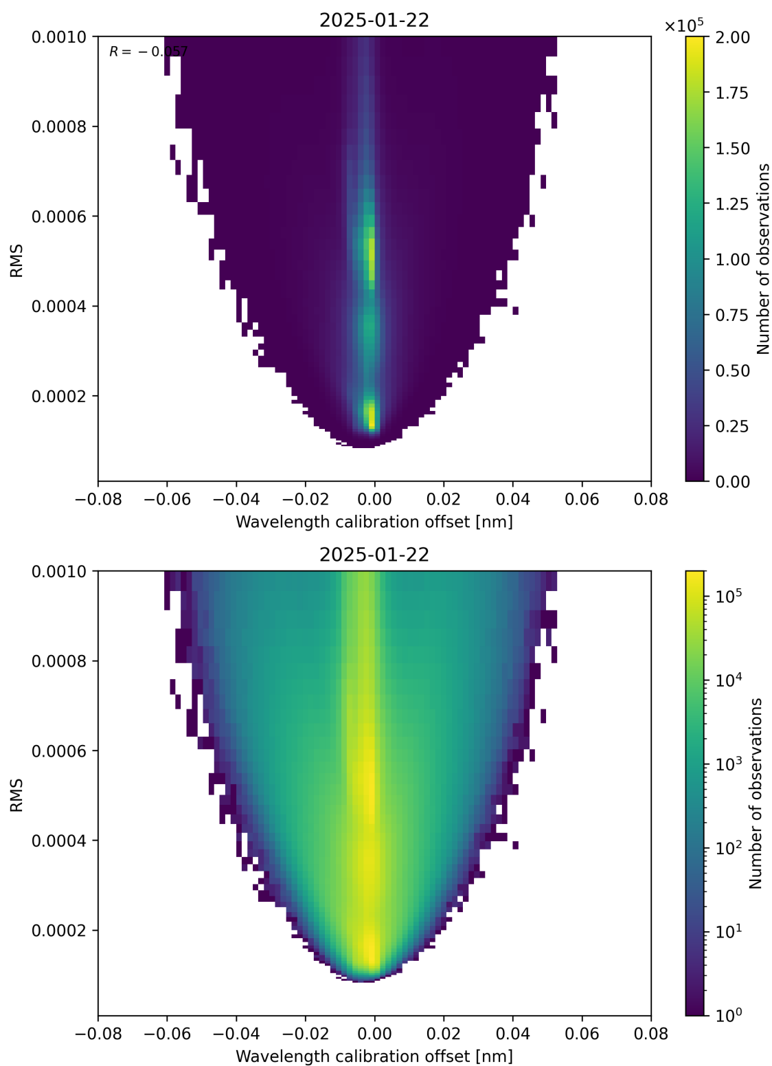
Figure 181: Scatter density plot of “Wavelength calibration offset” against “RMS” for 2025-01-21 to 2025-01-23.
