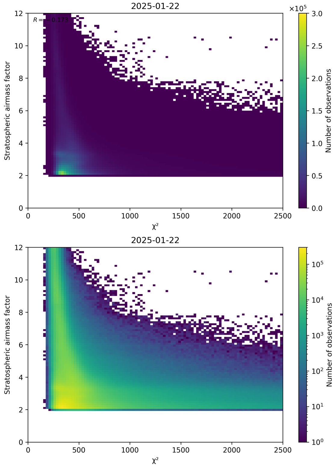
Figure 81: Scatter density plot of “ \chi^2 ” against “Stratospheric airmass factor” for 2025-01-21 to 2025-01-23.
