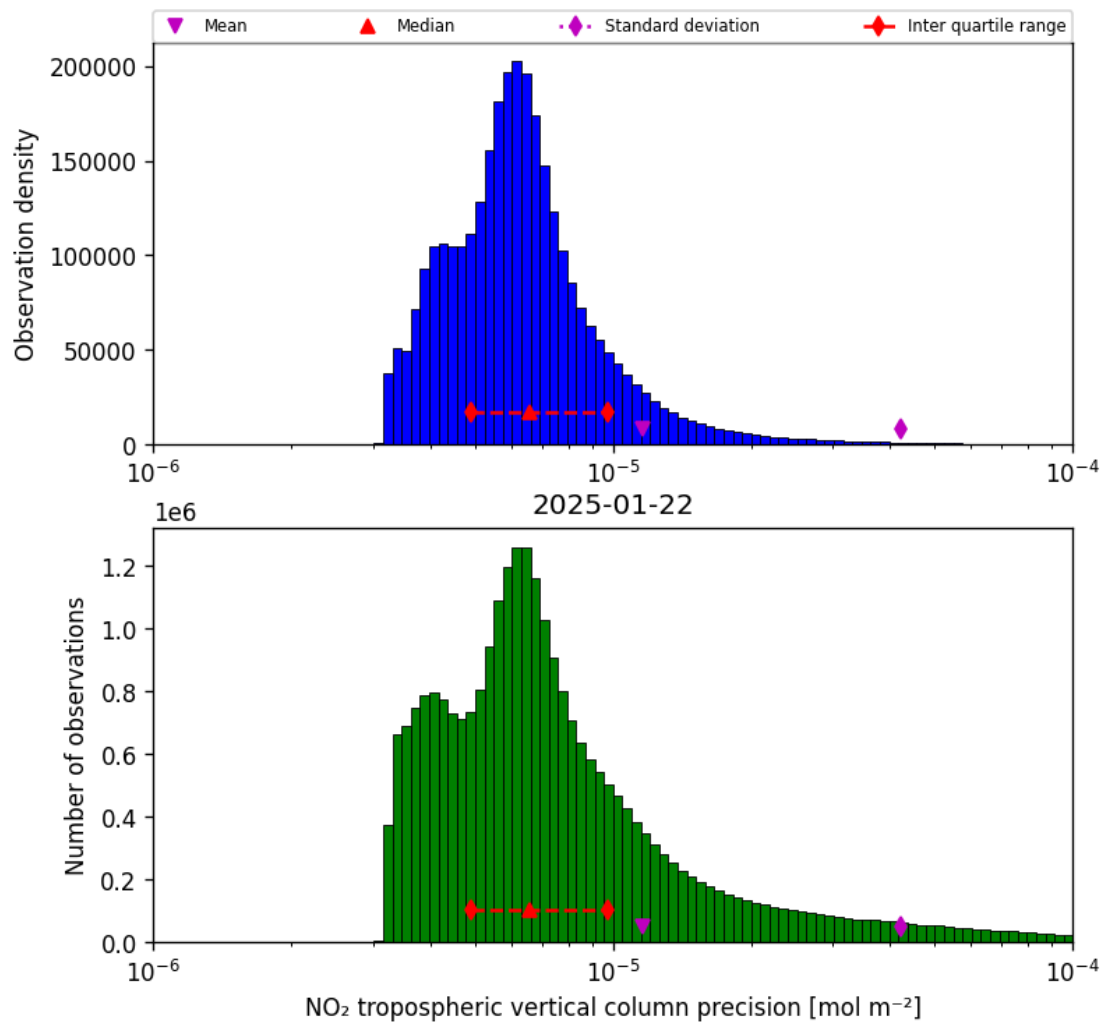
Figure 30: Histogram of “NO 2 tropospheric vertical column precision” for 2025-01-21 to 2025-01-23
