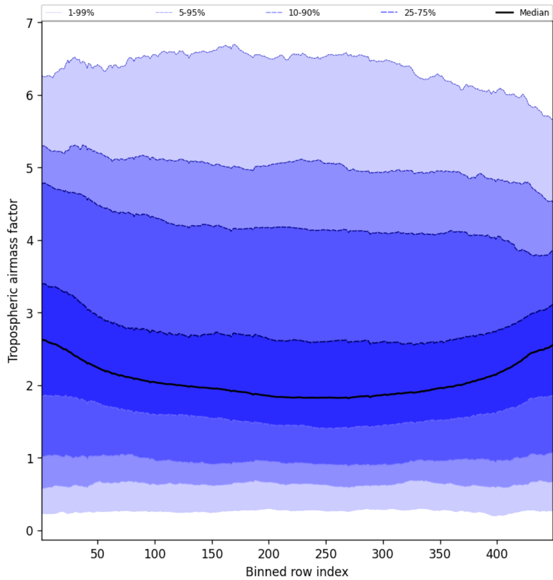
Figure 48: Along track statistics of “Tropospheric airmass factor” for 2025-01-21 to 2025-01-23
