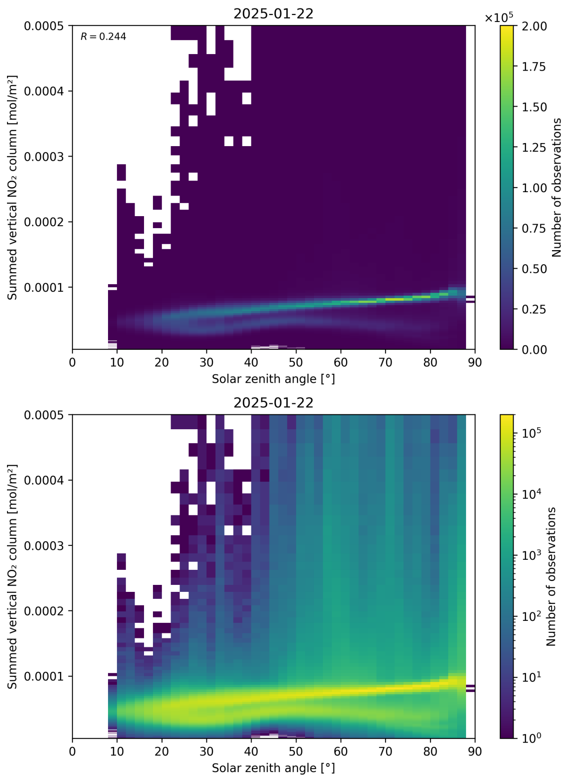
Figure 151: Scatter density plot of “Solar zenith angle” against “Summed vertical NO 2 column” for 2025-01-21 to 2025-01-23.
