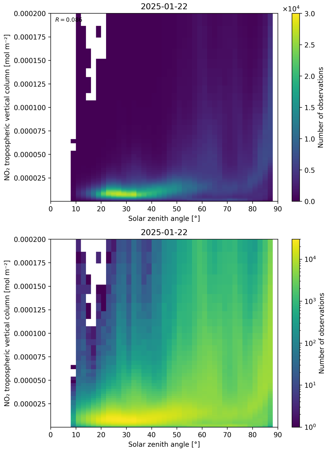
Figure 155: Scatter density plot of “Solar zenith angle” against “NO 2 tropospheric vertical column” for 2025-01-21 to 2025-01-23.
