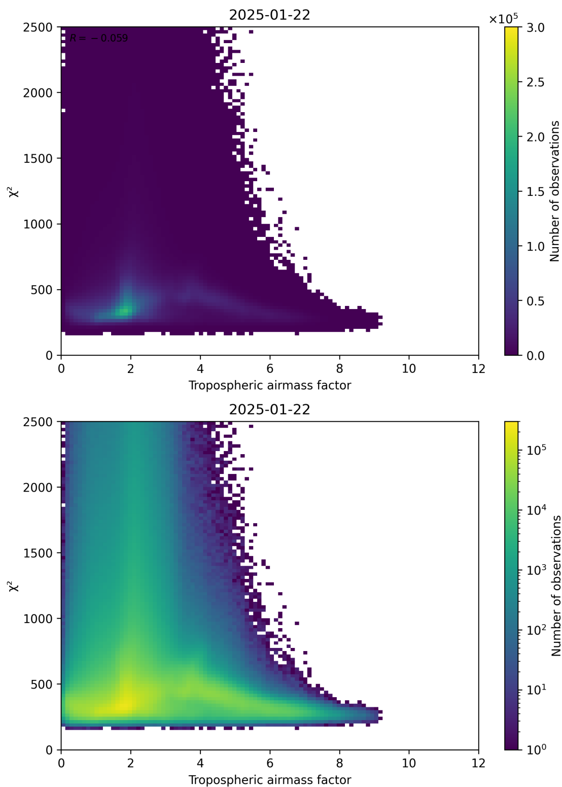
Figure 73: Scatter density plot of “Tropospheric airmass factor” against “ \chi^2 ” for 2025-01-21 to 2025-01-23.
