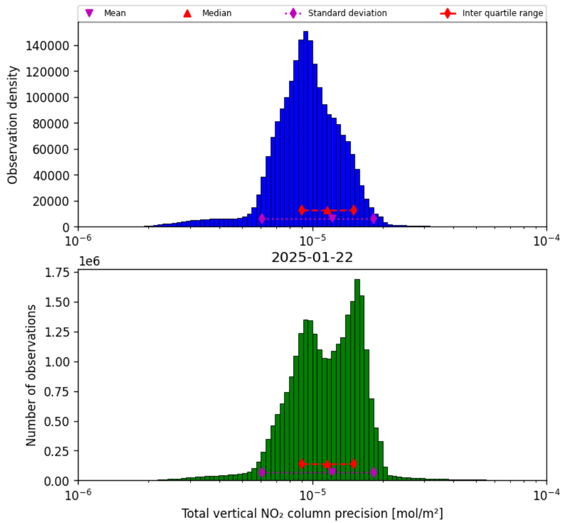
Figure 39: Histogram of “Total vertical NO 2 column precision” for 2025-01-21 to 2025-01-23
