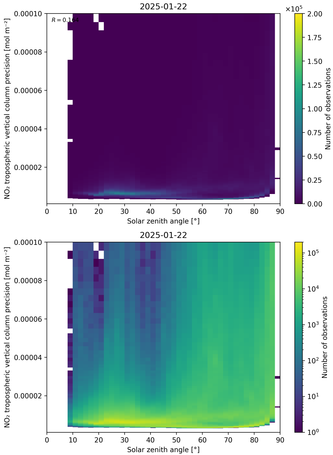
Figure 156: Scatter density plot of “Solar zenith angle” against “NO 2 tropospheric vertical column precision” for 2025-01-21 to 2025-01-23.
