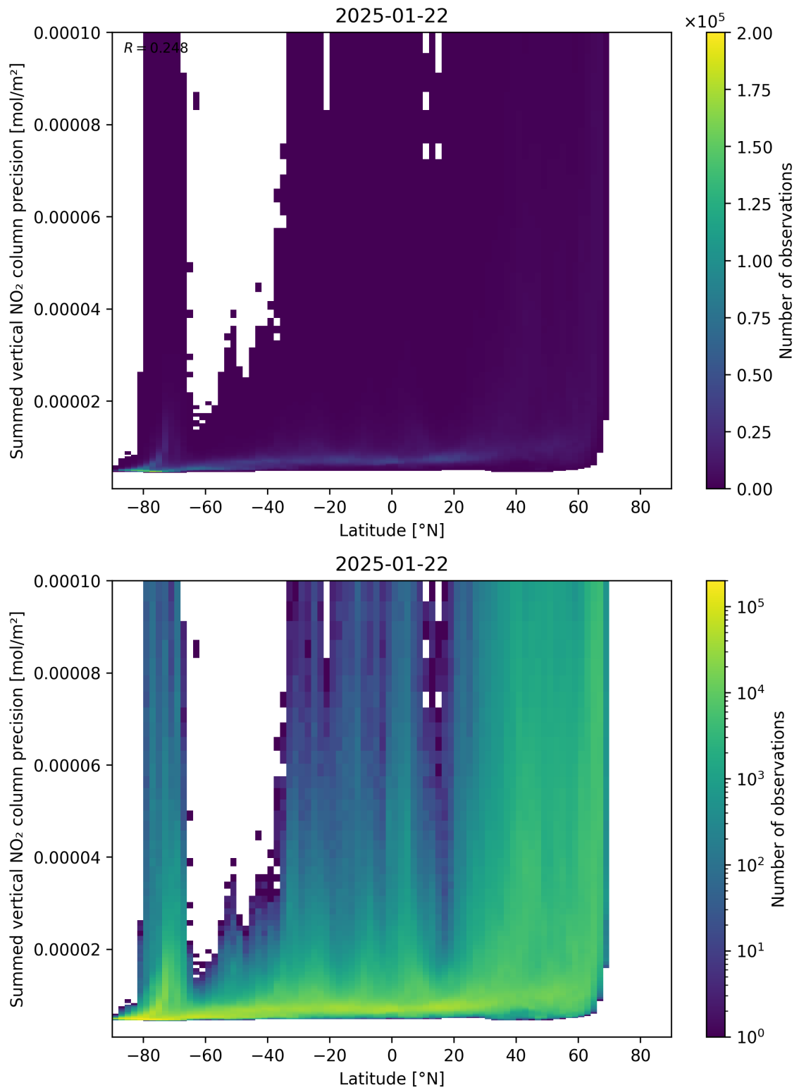
Figure 89: Scatter density plot of “Latitude” against “Summed vertical NO 2 column precision” for 2025-01-21 to 2025-01-23.
