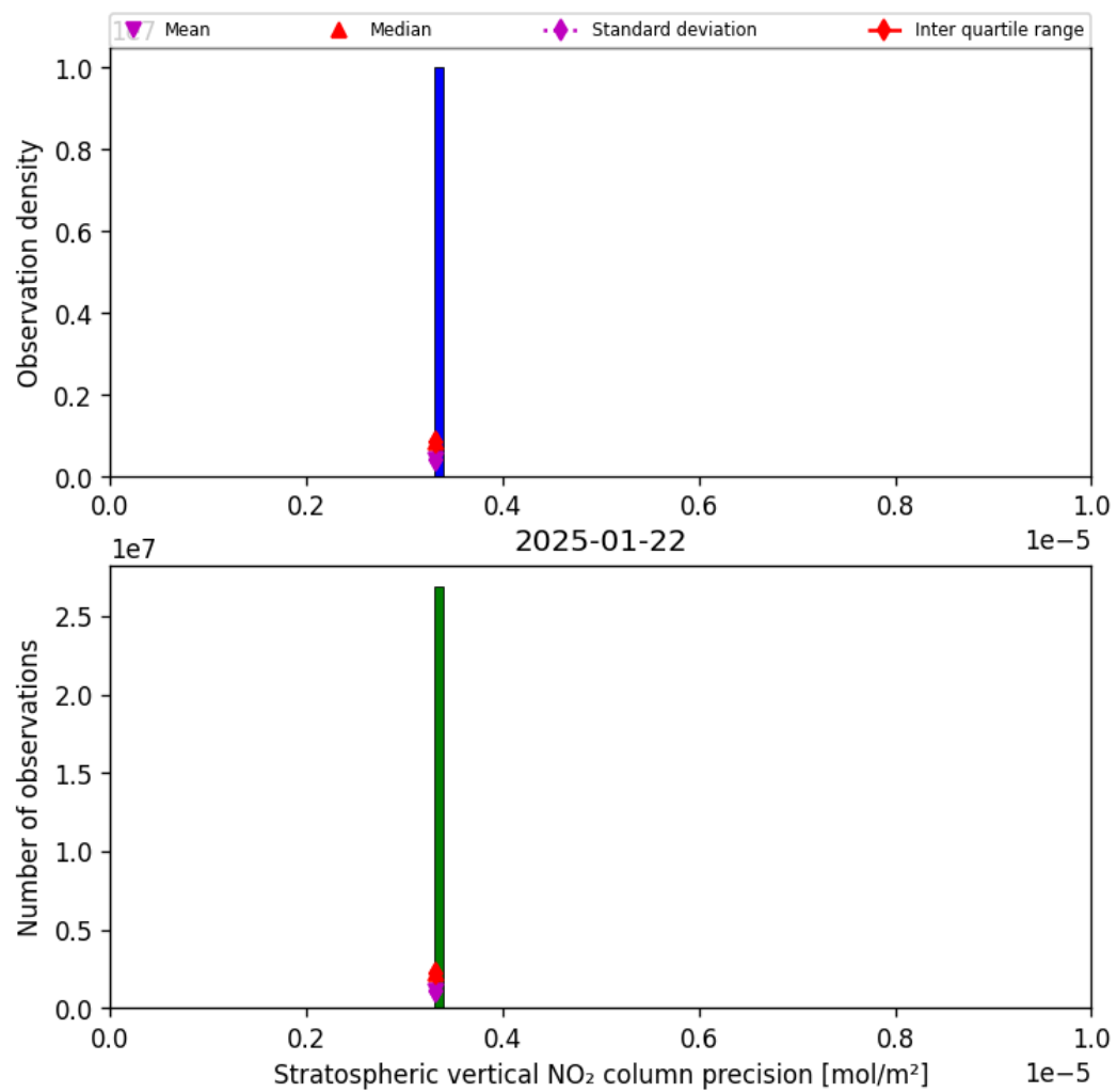
Figure 37: Histogram of “Stratospheric vertical NO 2 column precision” for 2025-01-21 to 2025-01-23
