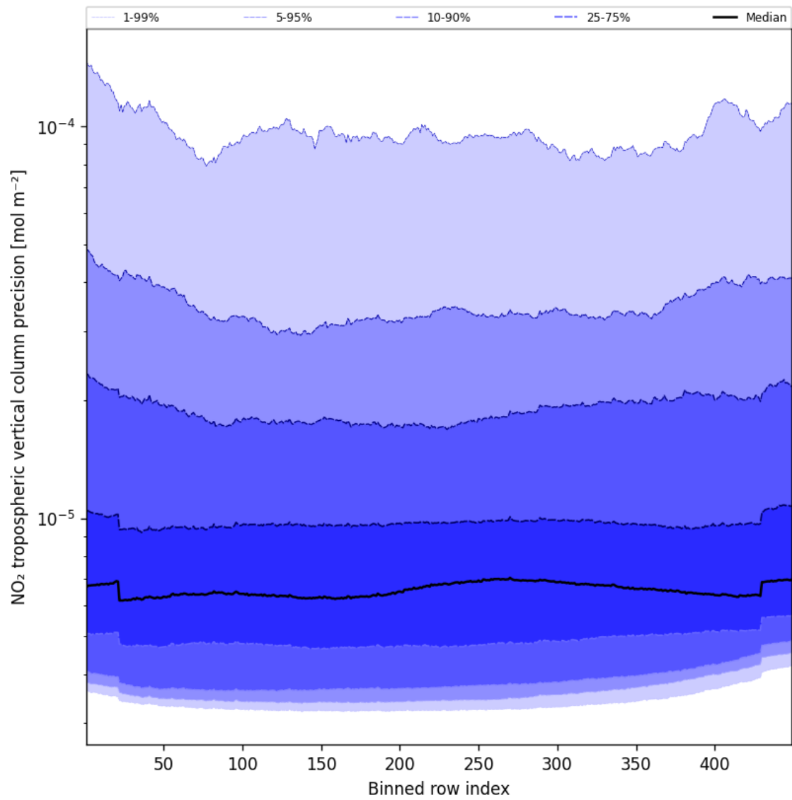
Figure 47: Along track statistics of “NO 2 tropospheric vertical column precision” for 2025-01-21 to 2025-01-23
