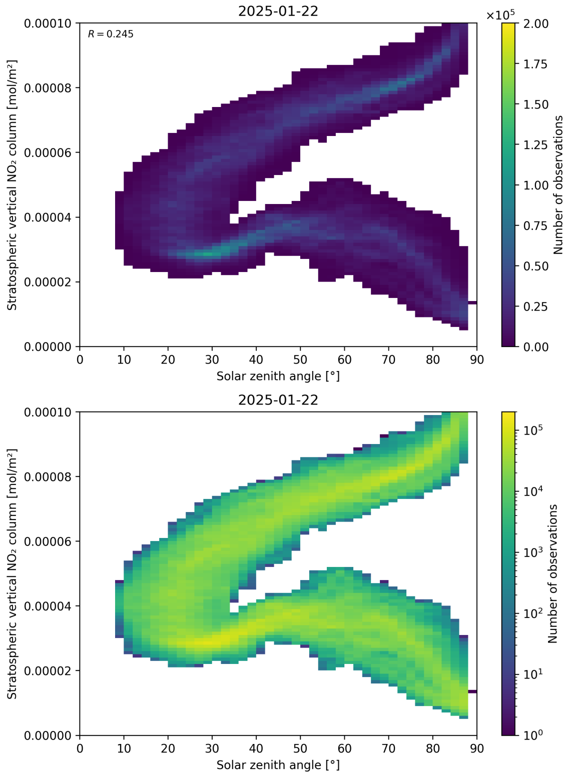
Figure 150: Scatter density plot of “Solar zenith angle” against “Stratospheric vertical NO 2 column” for 2025-01-21 to 2025-01-23.
