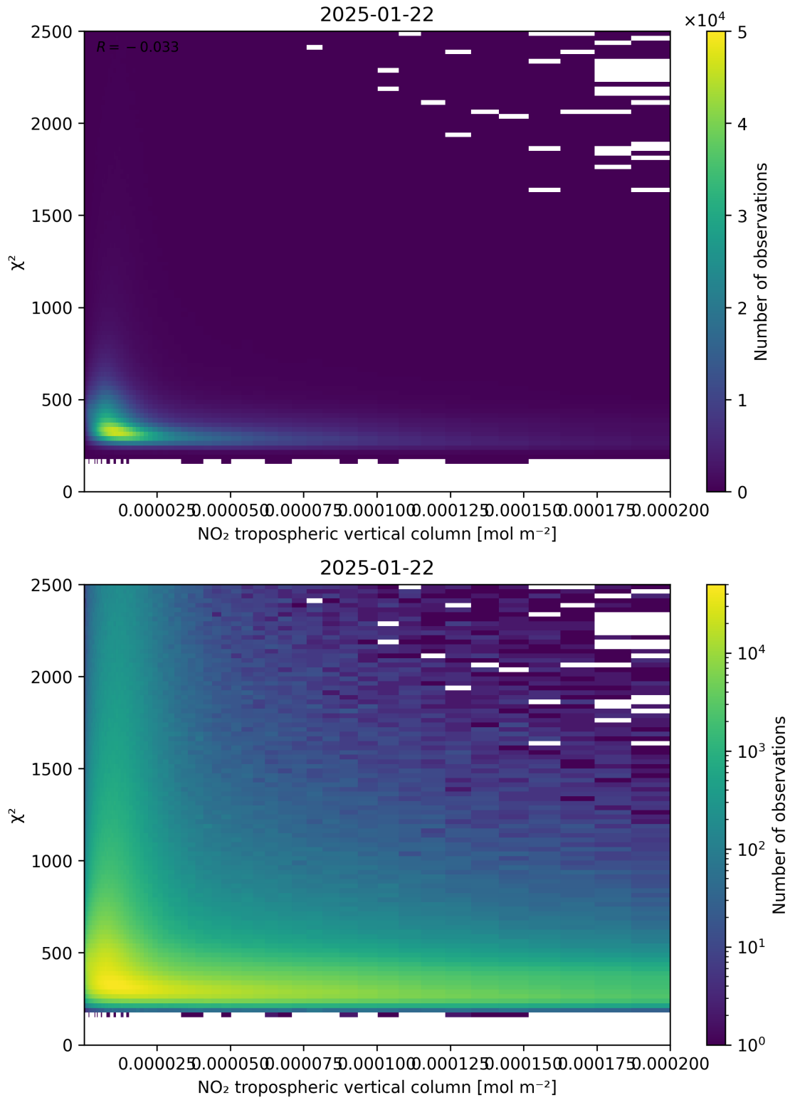
Figure 124: Scatter density plot of “NO 2 tropospheric vertical column” against “ \chi^2 ” for 2025-01-21 to 2025-01-23.
