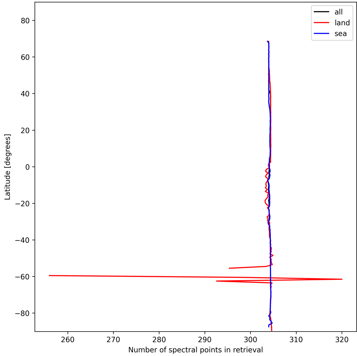
Figure 16: Zonal average of “Number of spectral points in retrieval” for 2025-01-21 to 2025-01-23.
