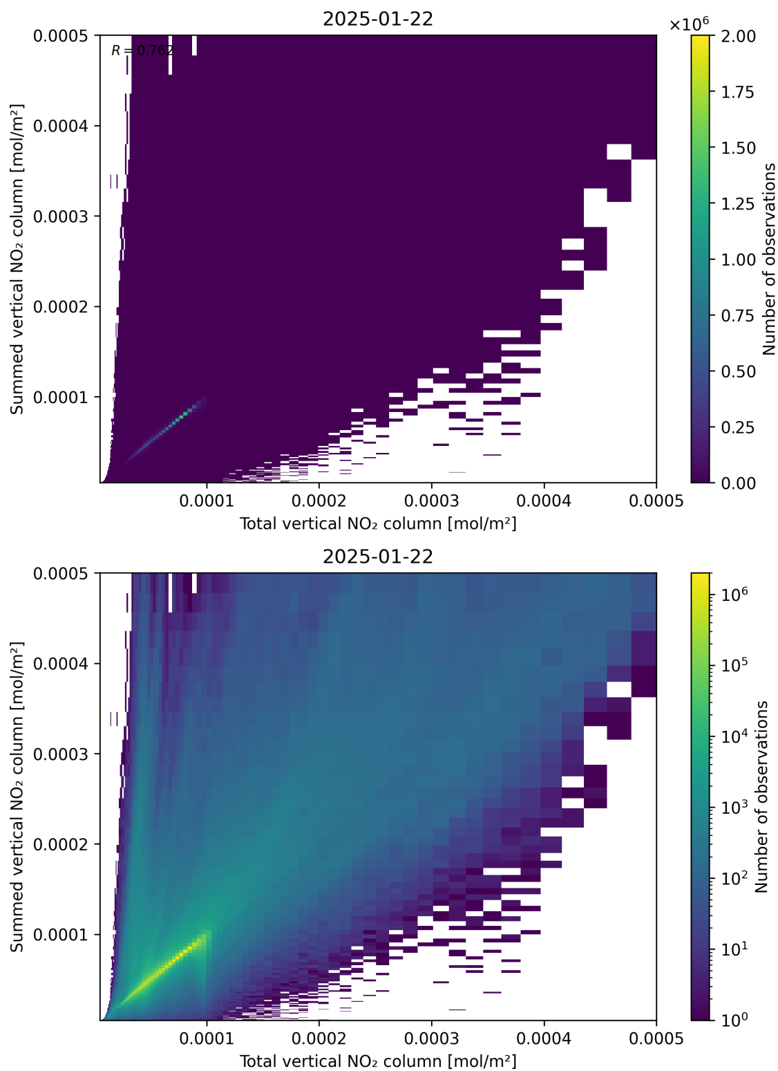
Figure 112: Scatter density plot of “Total vertical NO 2 column” against “Summed vertical NO 2 column” for 2025-01-21 to 2025-01-23.
