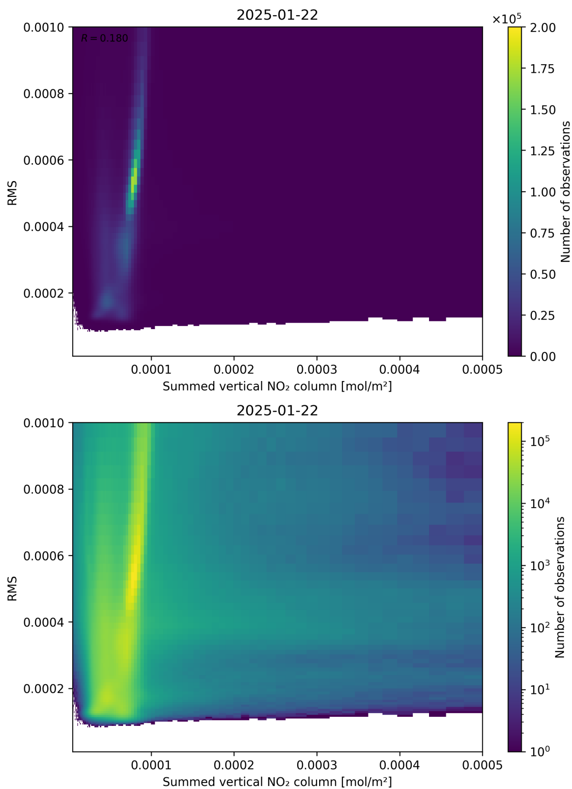
Figure 109: Scatter density plot of “Summed vertical NO 2 column” against “RMS” for 2025-01-21 to 2025-01-23.
