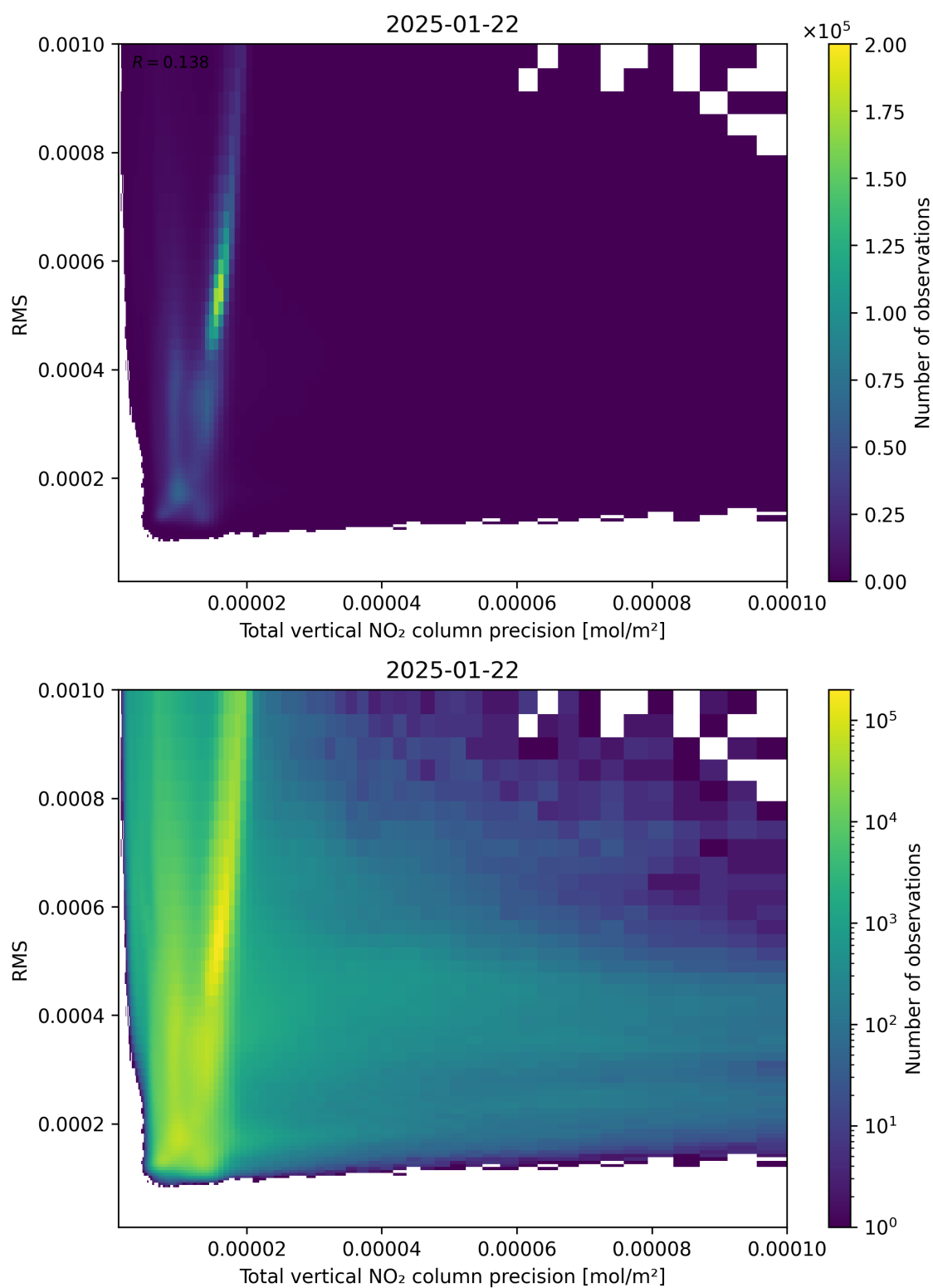
Figure 119: Scatter density plot of “Total vertical NO 2 column precision” against “RMS” for 2025-01-21 to 2025-01-23.
