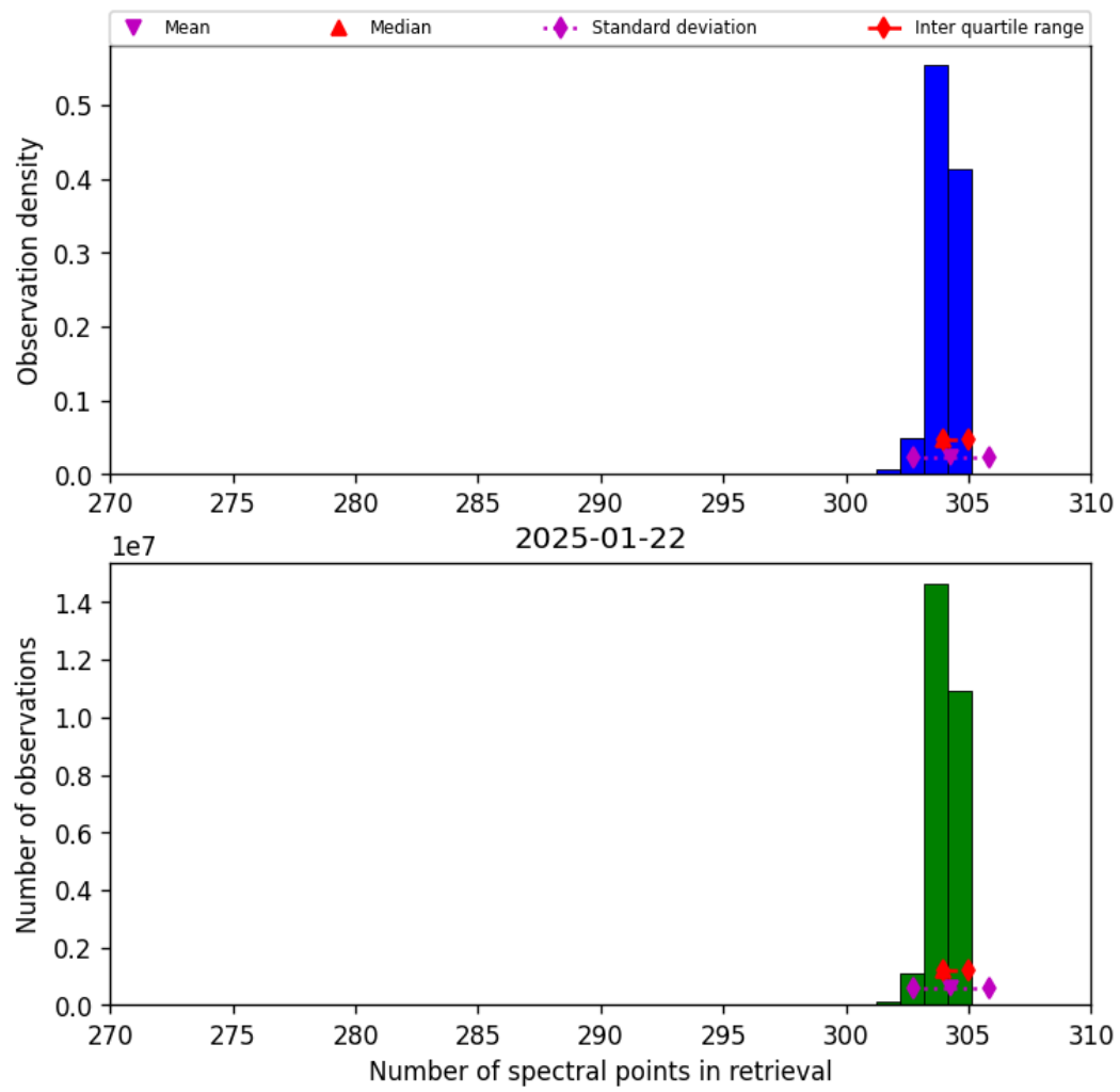
Figure 33: Histogram of “Number of spectral points in retrieval” for 2025-01-21 to 2025-01-23
