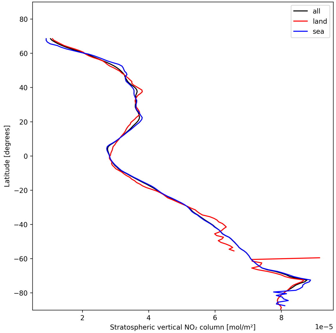
Figure 19: Zonal average of “Stratospheric vertical NO 2 column” for 2025-01-21 to 2025-01-23.
