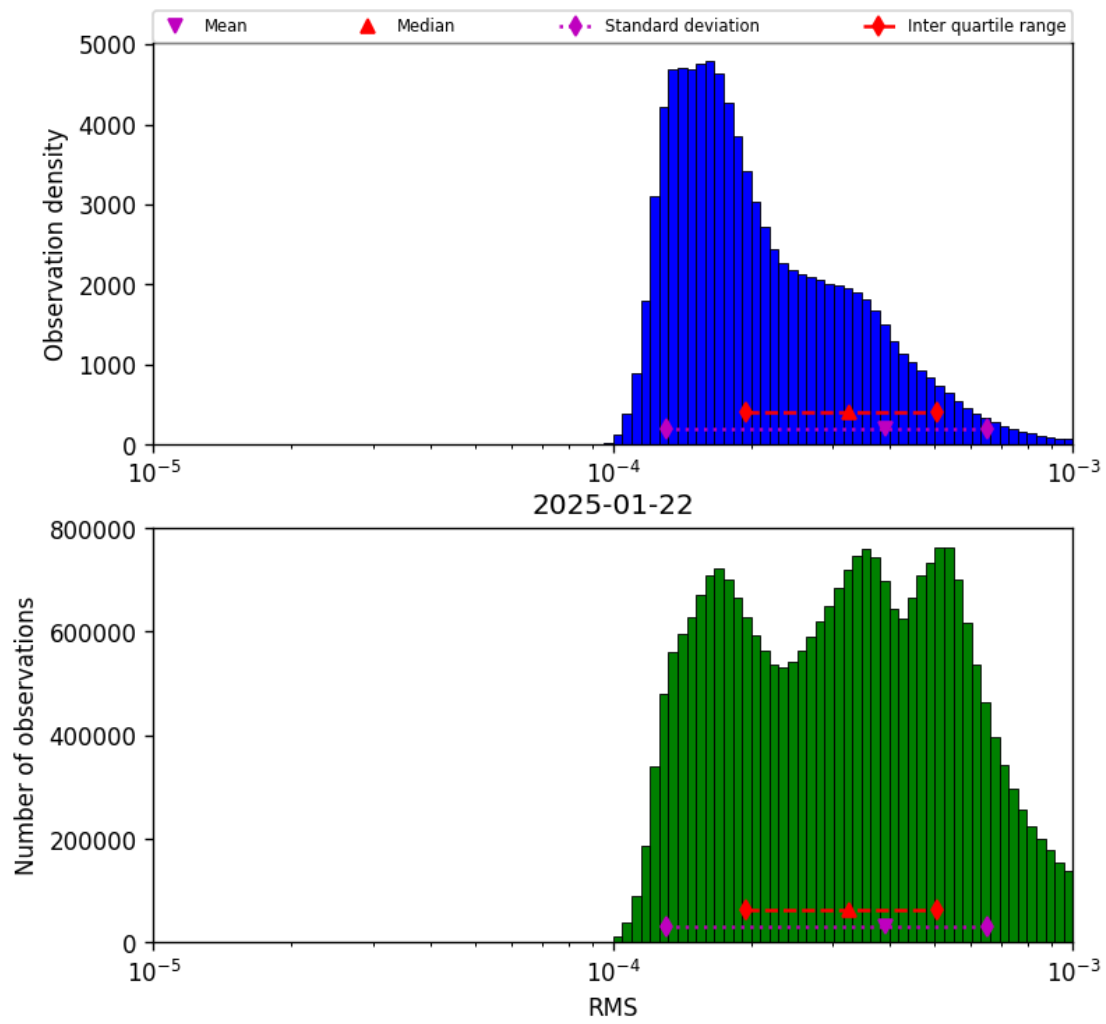
Figure 43: Histogram of “RMS” for 2025-01-21 to 2025-01-23
