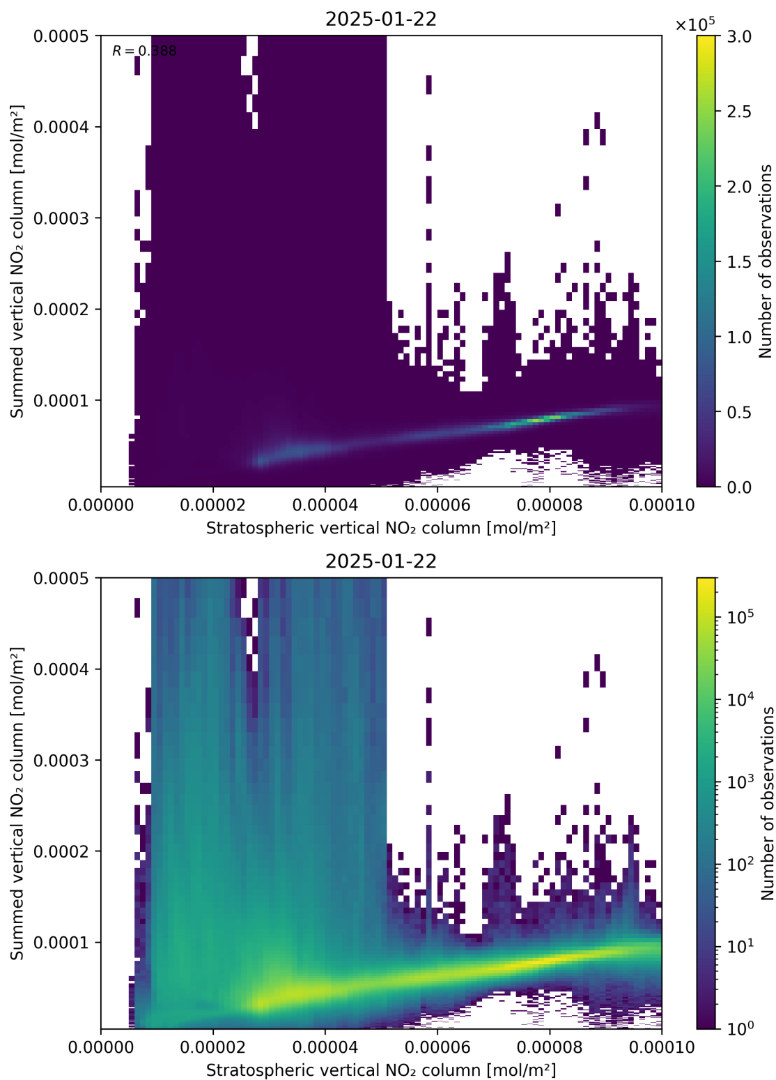
Figure 98: Scatter density plot of “Stratospheric vertical NO 2 column” against “Summed vertical NO 2 column” for 2025-01-21 to 2025-01-23.
