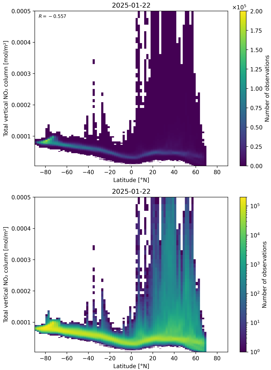
Figure 90: Scatter density plot of “Latitude” against “Total vertical NO 2 column” for 2025-01-21 to 2025-01-23.
