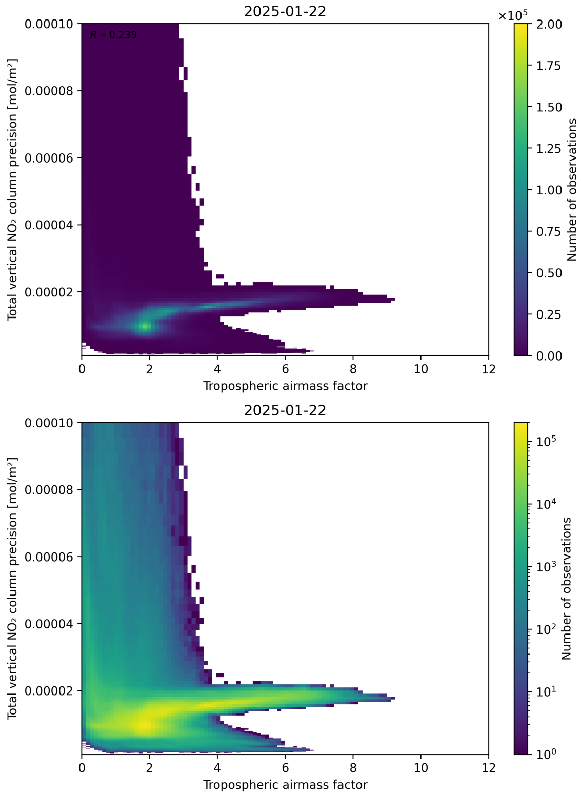
Figure 78: Scatter density plot of “Tropospheric air mass factor” against “Total vertical NO 2 column precision” for 2025-01-21 to 2025-01-23.
