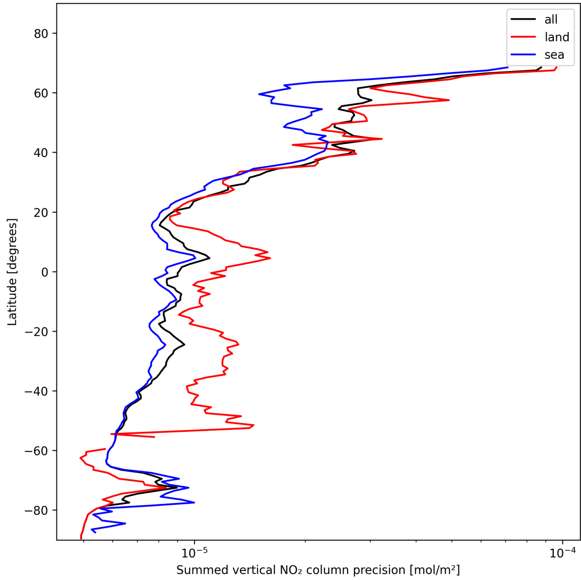
Figure 24: Zonal average of “Summed vertical NO 2 column precision” for 2025-01-21 to 2025-01-23.
