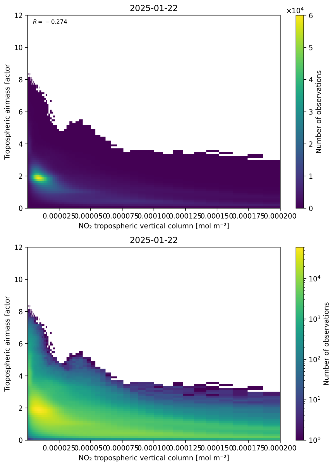
Figure 123: Scatter density plot of “NO 2 tropospheric vertical column” against “Tropospheric air mass factor” for 2025-01-21 to 2025-01-23.
