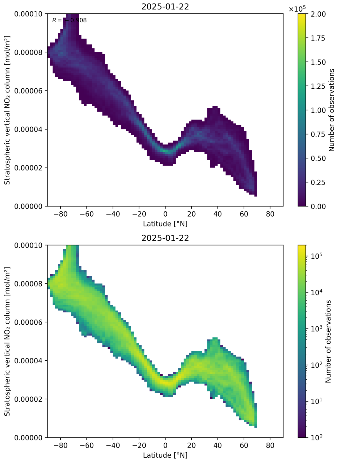
Figure 87: Scatter density plot of “Latitude” against “Stratospheric vertical NO 2 column” for 2025-01-21 to 2025-01-23.
