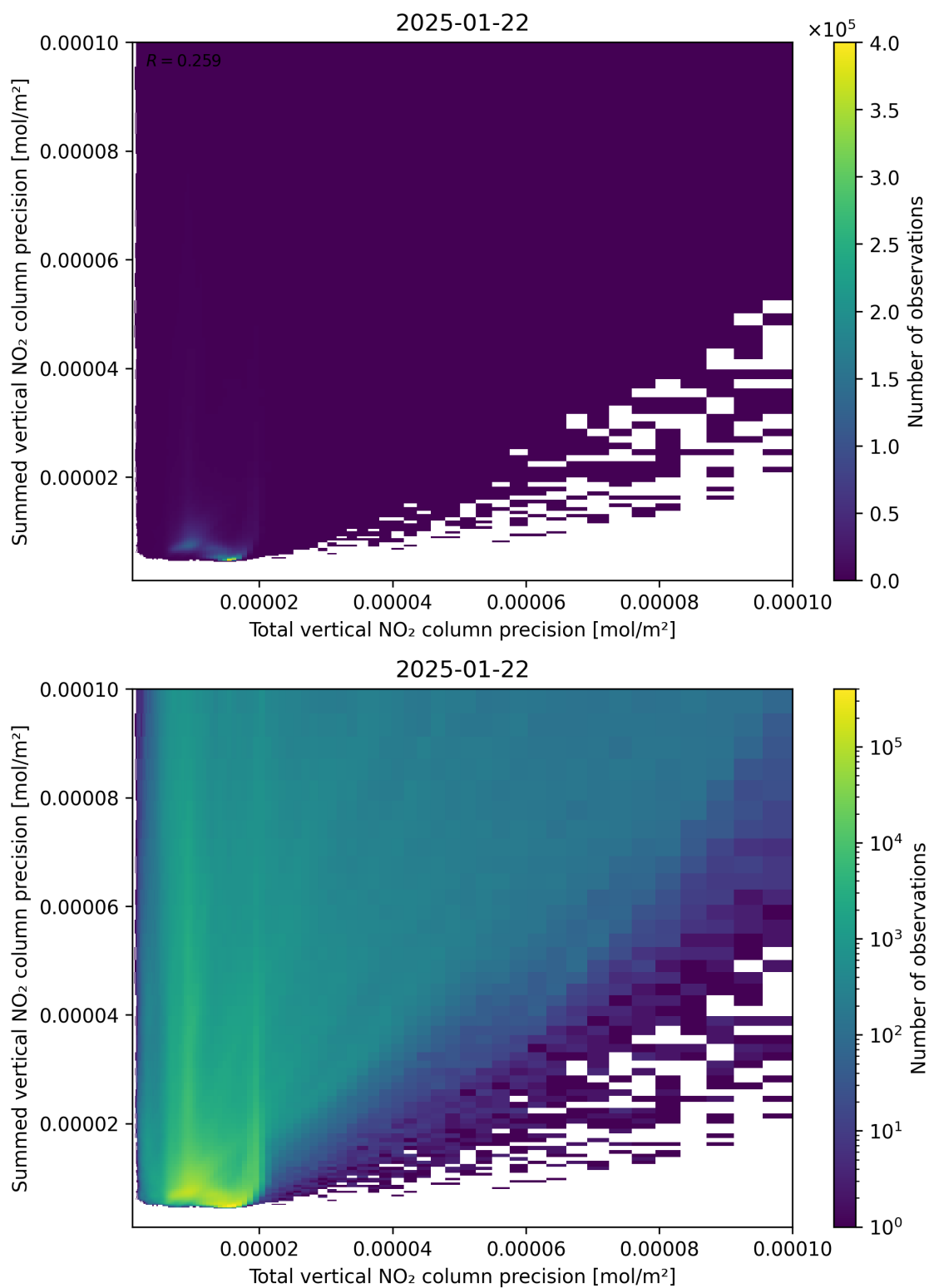
Figure 118: Scatter density plot of “Total vertical NO 2 column precision” against “Summed vertical NO 2 column precision” for 2025-01-21 to 2025-01-23.
