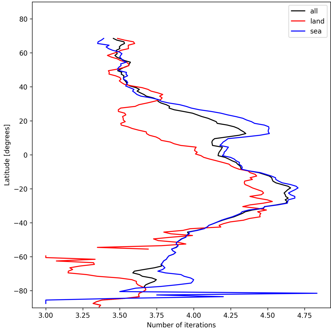
Figure 17: Zonal average of “Number of iterations” for 2025-01-21 to 2025-01-23.
