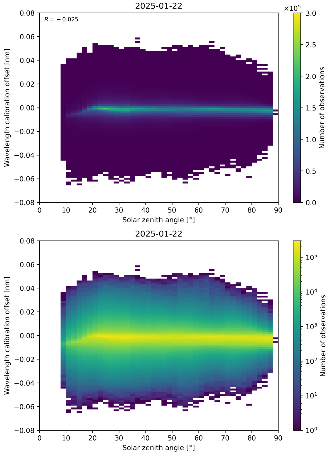
Figure 158: Scatter density plot of “Solar zenith angle” against “Wavelength calibration offset” for 2025-01-21 to 2025-01-23.
