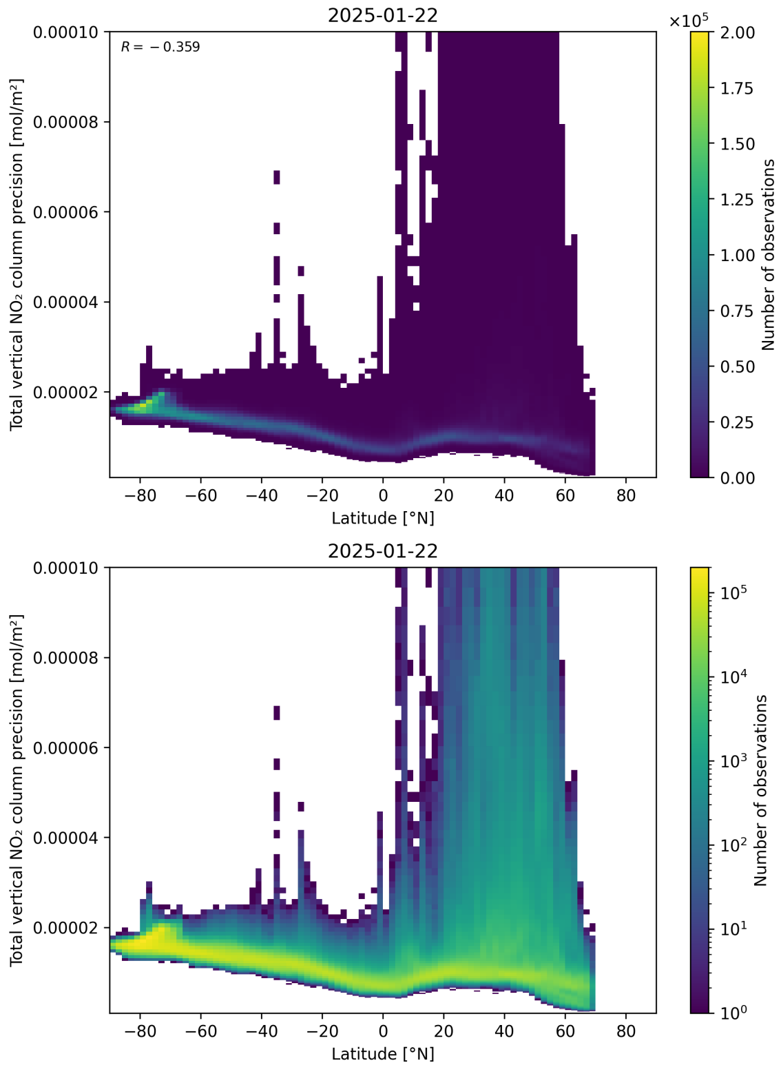
Figure 91: Scatter density plot of “Latitude” against “Total vertical NO 2 column precision” for 2025-01-21 to 2025-01-23.
