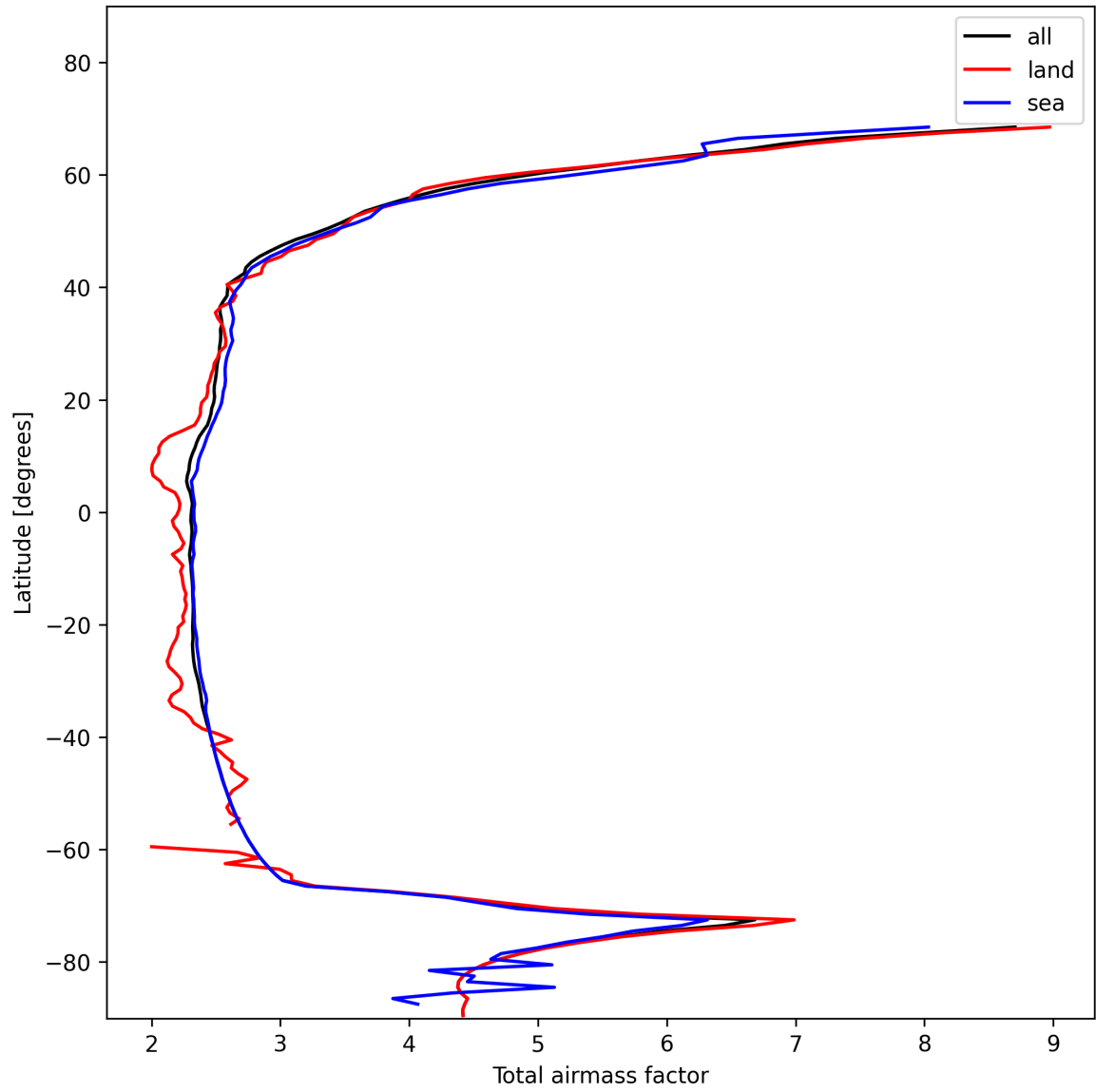
Figure 15: Zonal average of “Total airmass factor” for 2025-01-21 to 2025-01-23.
