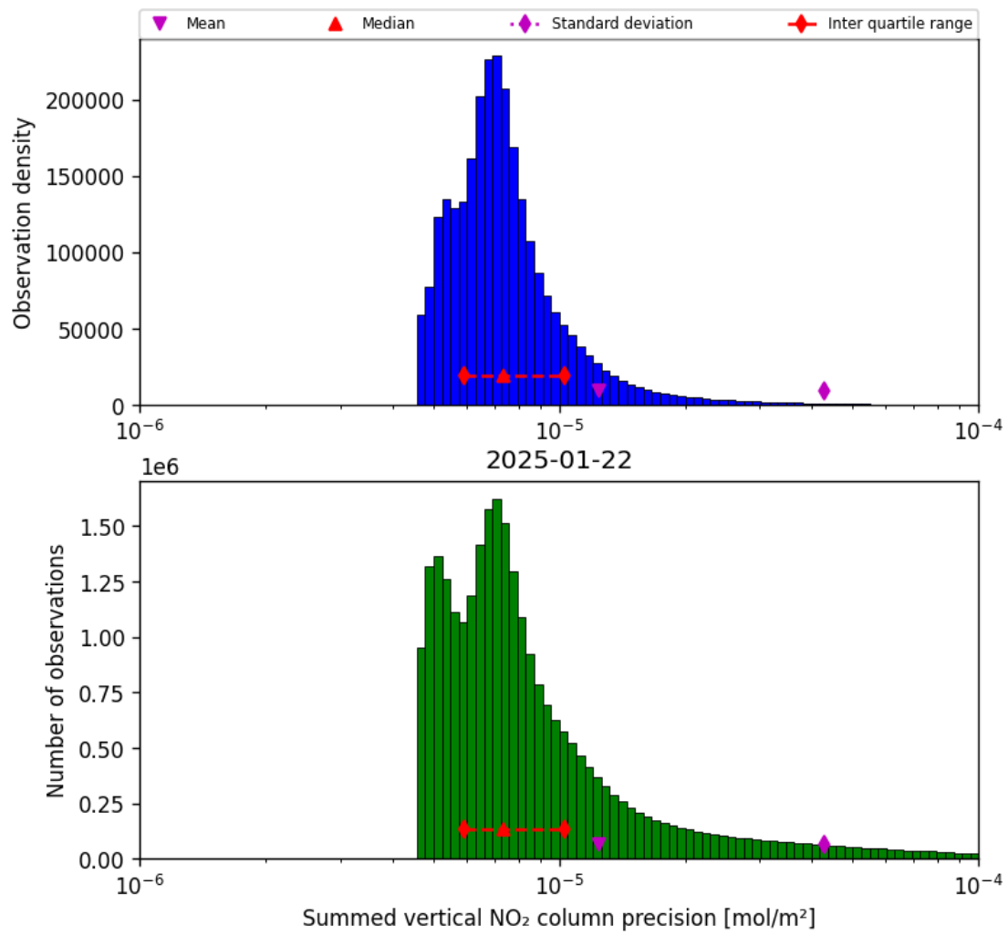
Figure 41: Histogram of “Summed vertical NO 2 column precision” for 2025-01-21 to 2025-01-23
