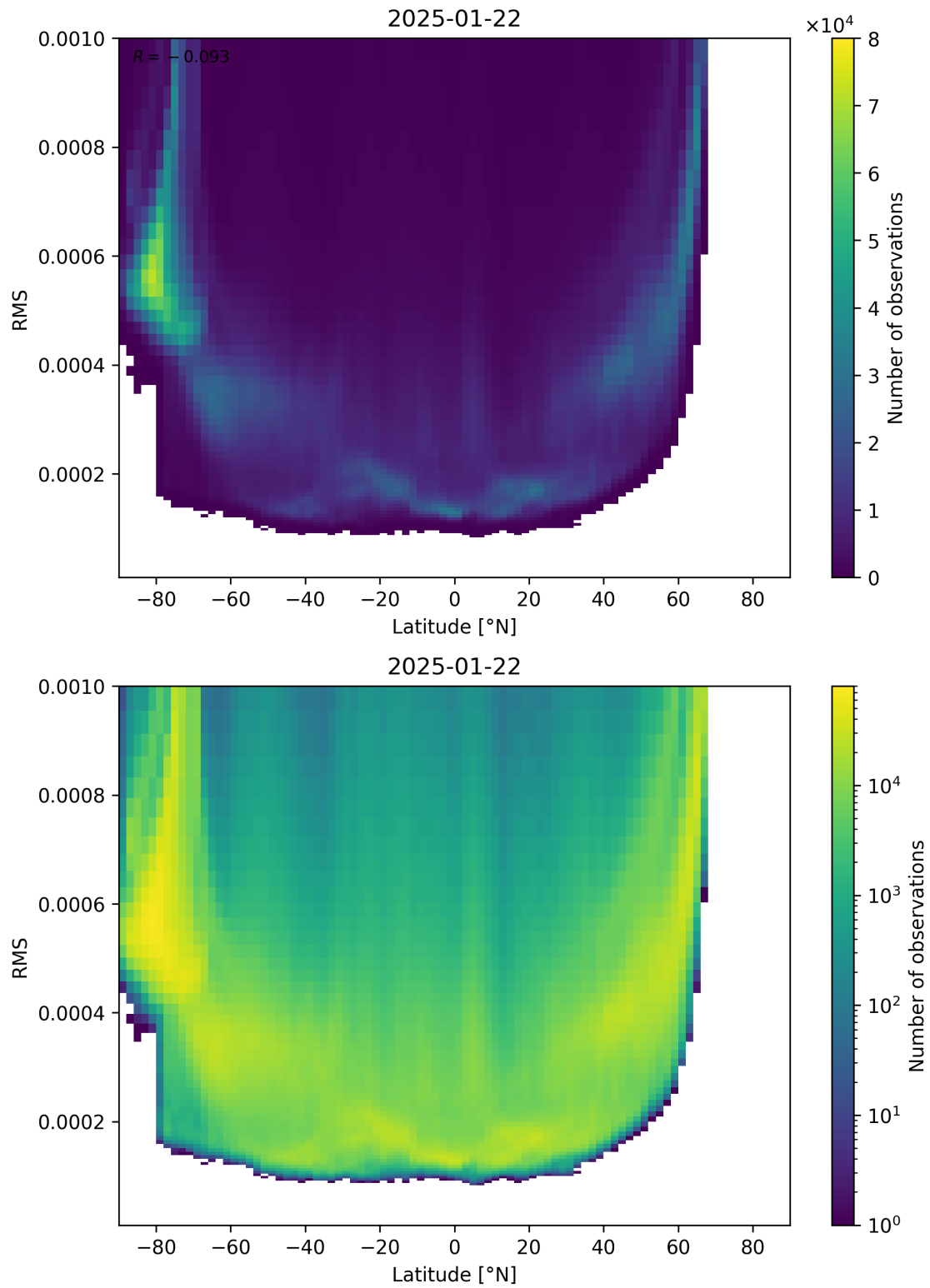
Figure 94: Scatter density plot of “Latitude” against “RMS” for 2025-01-21 to 2025-01-23.
