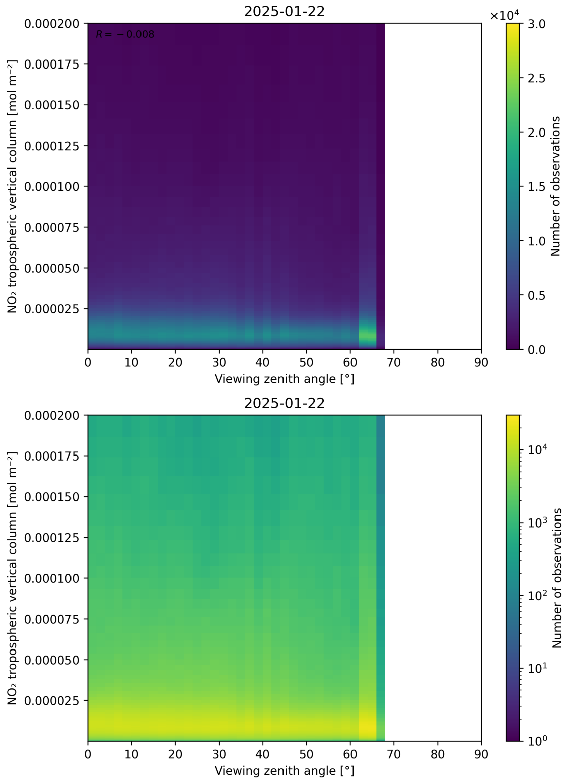
Figure 169: Scatter density plot of “Viewing zenith angle” against “NO 2 tropospheric vertical column” for 2025-01-21 to 2025-01-23.
