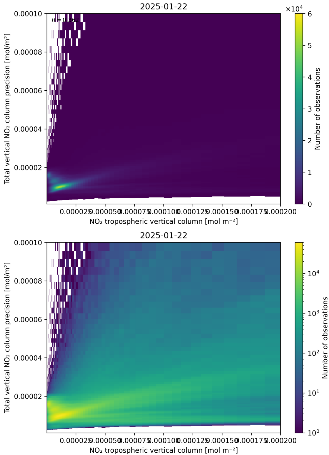
Figure 129: Scatter density plot of “NO 2 tropospheric vertical column” against “Total vertical NO 2 column precision” for 2025-01-21 to 2025-01-23.
