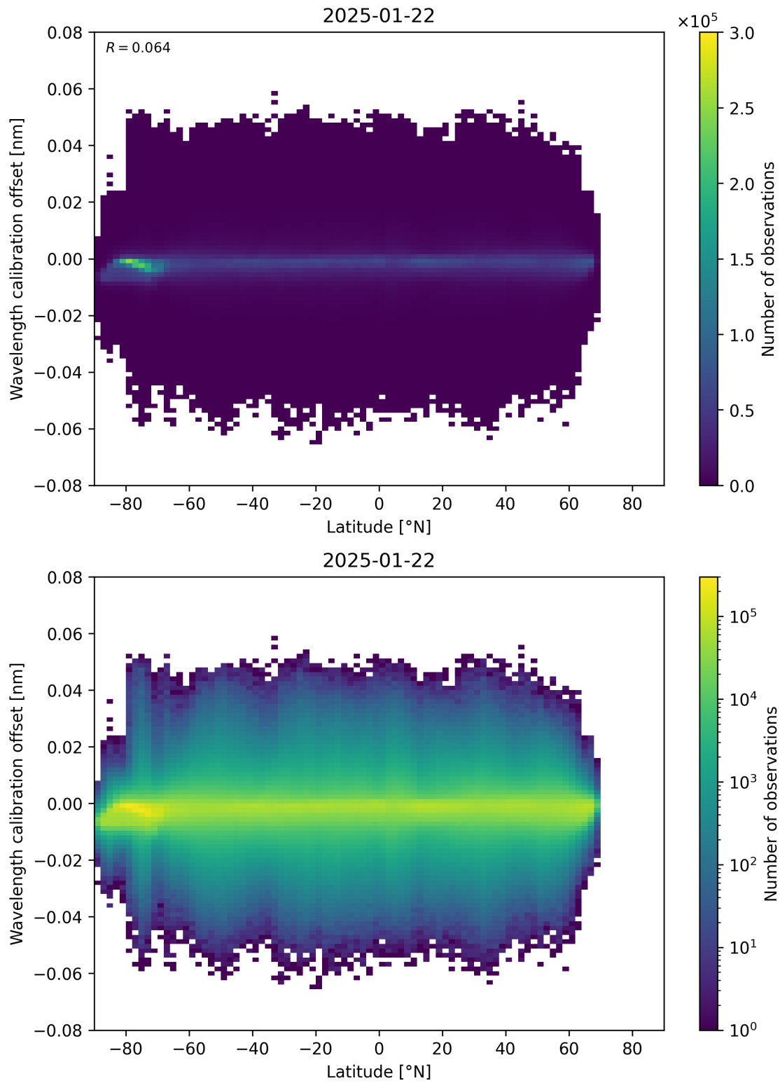
Figure 95: Scatter density plot of “Latitude” against “Wavelength calibration offset” for 2025-01-21 to 2025-01-23.
