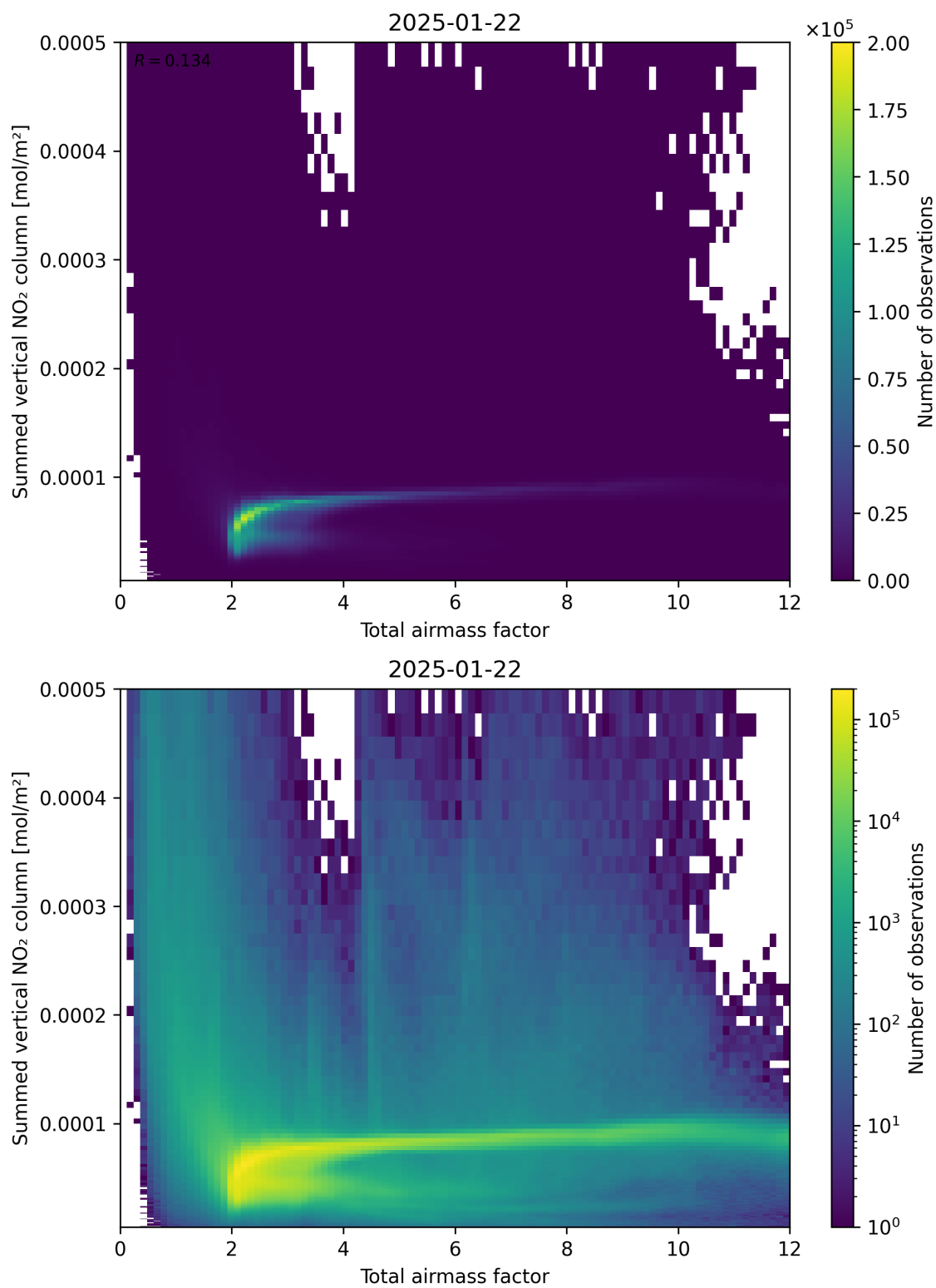
Figure 65: Scatter density plot of “Total airmass factor” against “Summed vertical NO 2 column” for 2025-01-21 to 2025-01-23.
