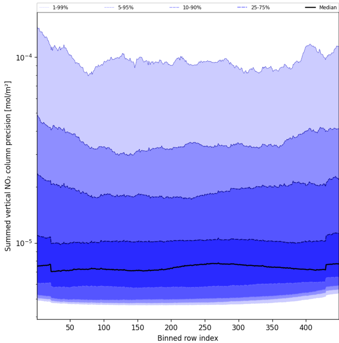
Figure 58: Along track statistics of “Summed vertical NO 2 column precision” for 2025-01-21 to 2025-01-23
