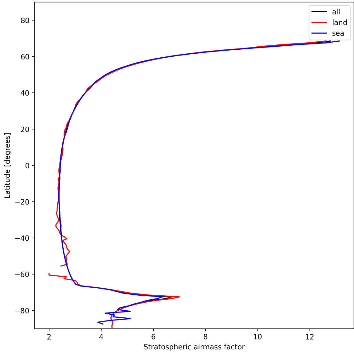
Figure 27: Zonal average of “Stratospheric airmass factor” for 2025-01-21 to 2025-01-23.
