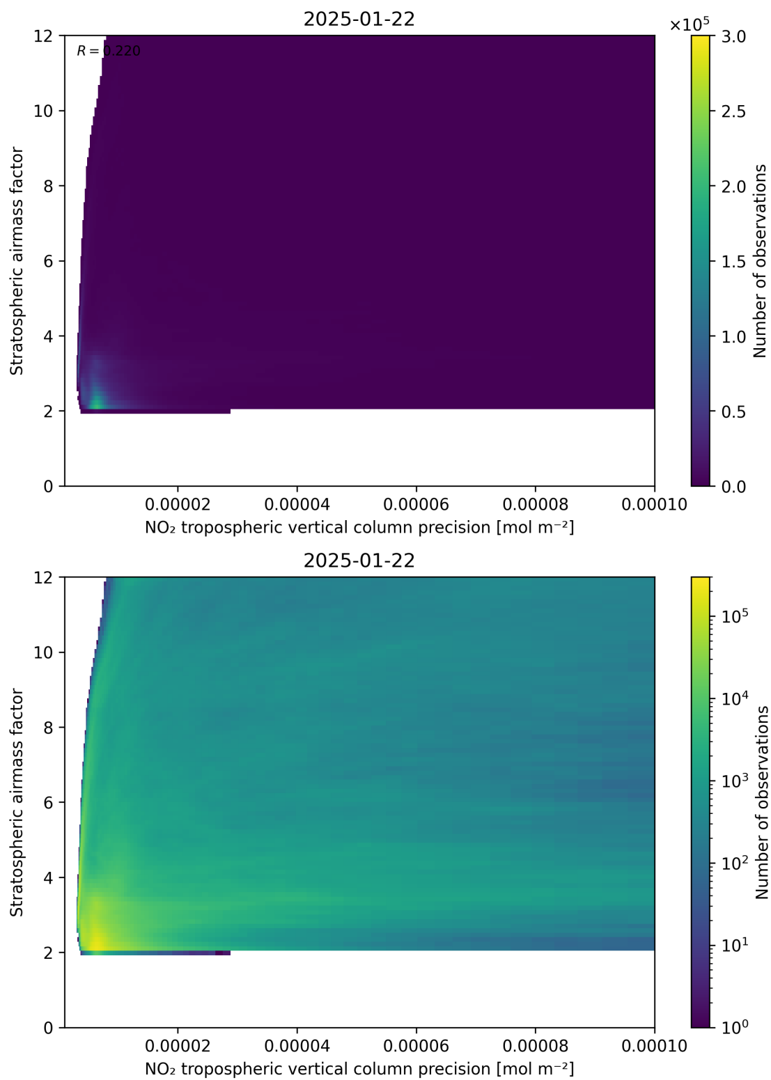
Figure 131: Scatter density plot of “NO 2 tropospheric vertical column precision” against “Stratospheric airmass factor” for 2025-01-21 to 2025-01-23.
