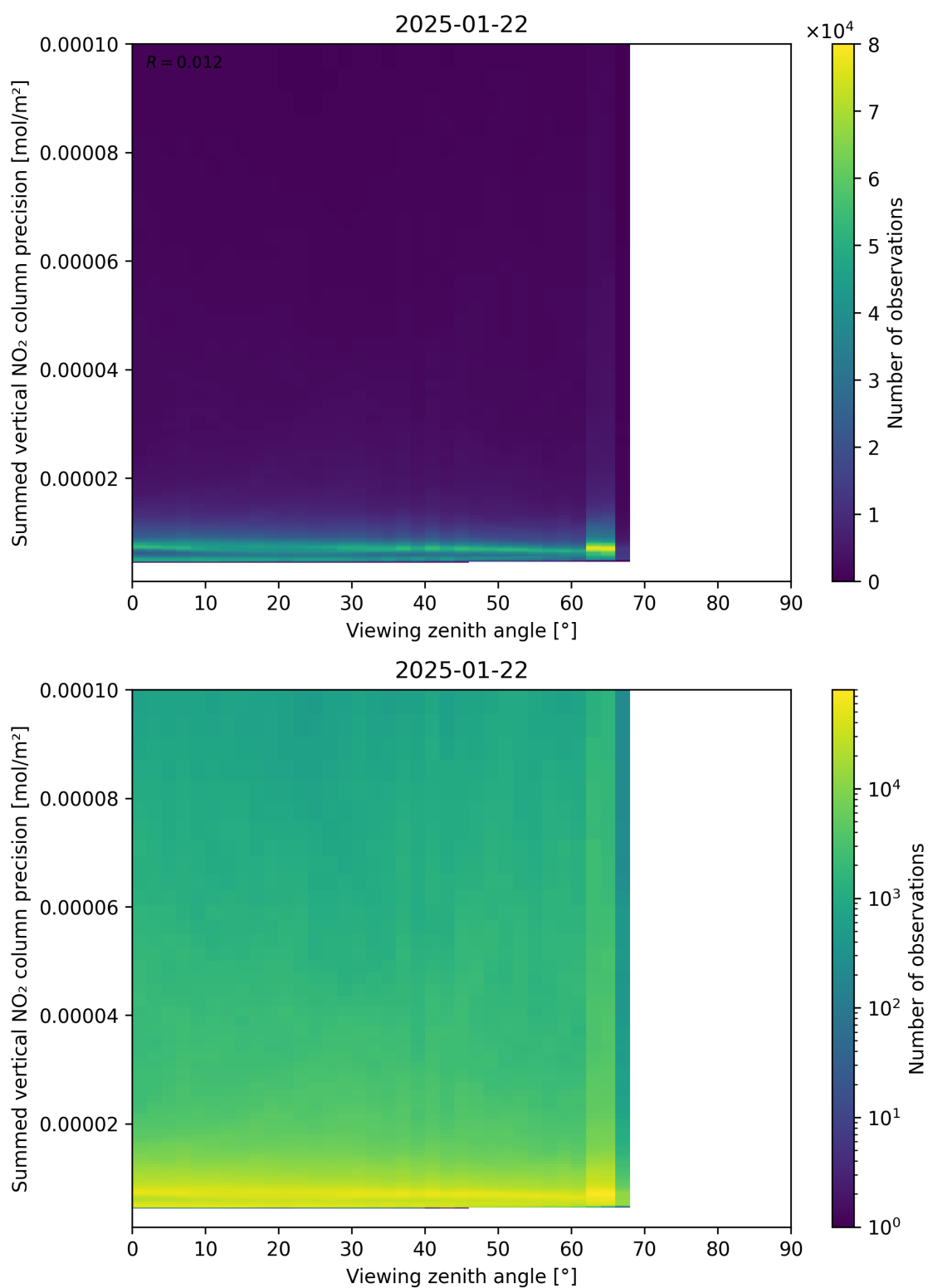
Figure 166: Scatter density plot of “Viewing zenith angle” against “Summed vertical NO 2 column precision” for 2025-01-21 to 2025-01-23.
