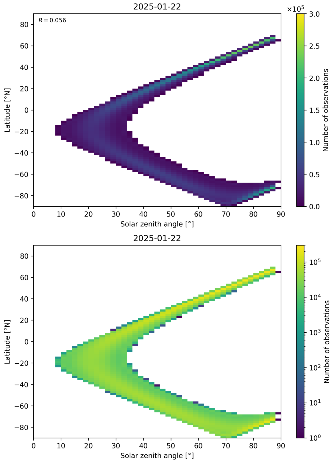
Figure 149: Scatter density plot of “Solar zenith angle” against “Latitude” for 2025-01-21 to 2025-01-23.
