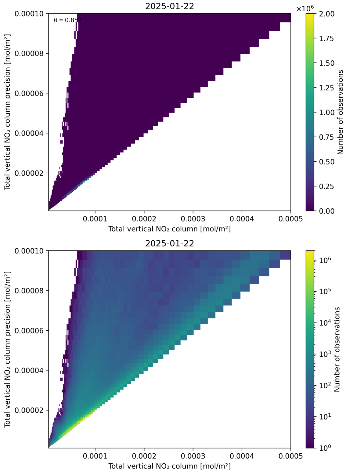
Figure 114: Scatter density plot of “Total vertical NO 2 column” against “Total vertical NO 2 column precision” for 2025-01-21 to 2025-01-23.
