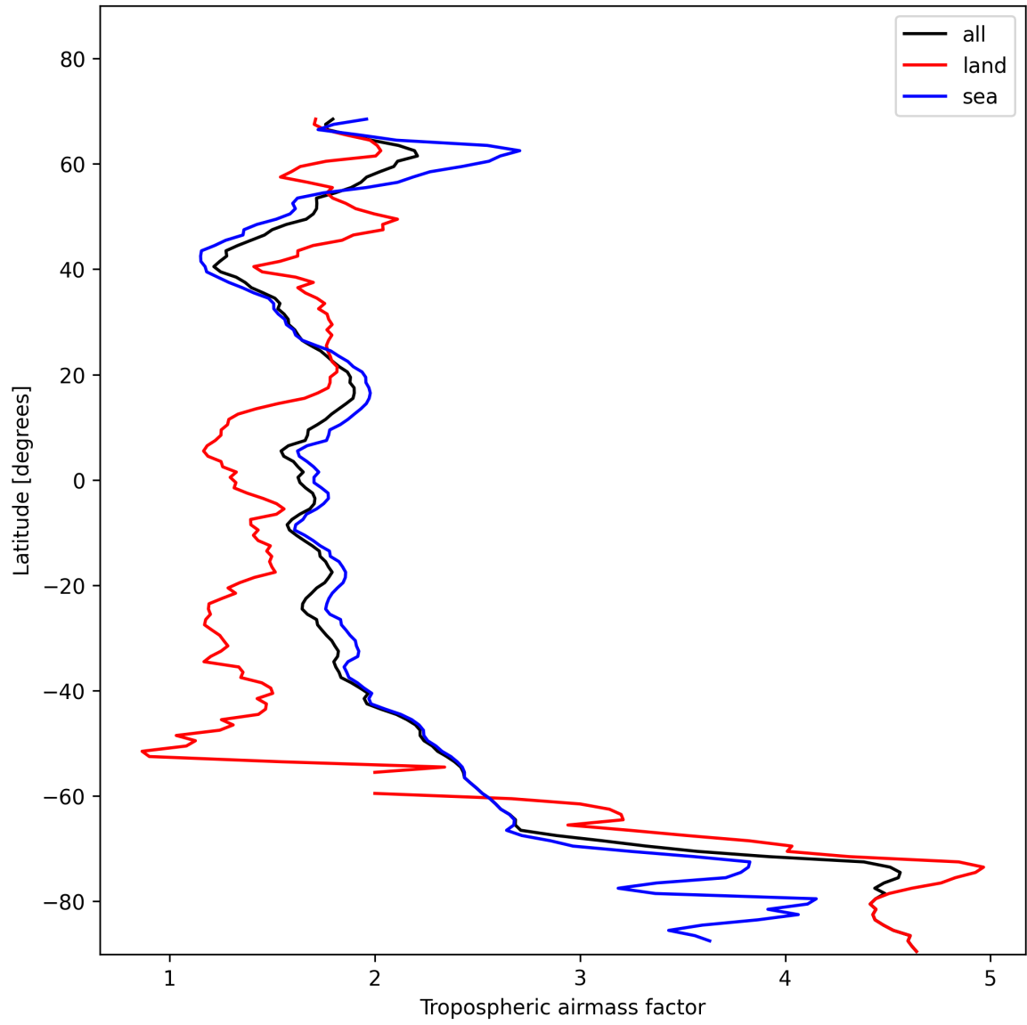
Figure 14: Zonal average of “Tropospheric air mass factor” for 2025-01-21 to 2025-01-23.
