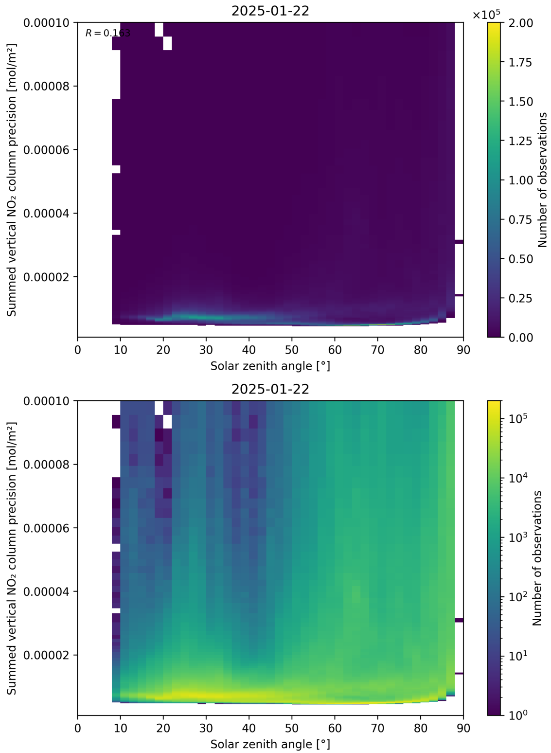
Figure 152: Scatter density plot of “Solar zenith angle” against “Summed vertical NO 2 column precision” for 2025-01-21 to 2025-01-23.
