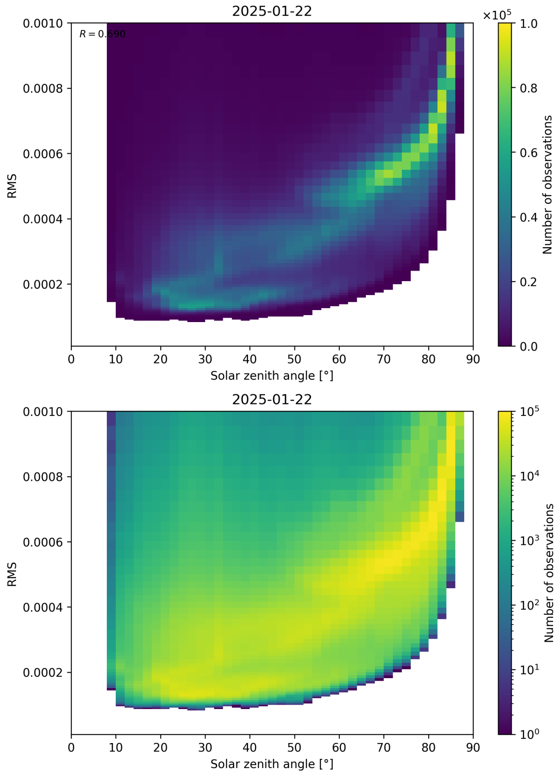
Figure 157: Scatter density plot of “Solar zenith angle” against “RMS” for 2025-01-21 to 2025-01-23.
