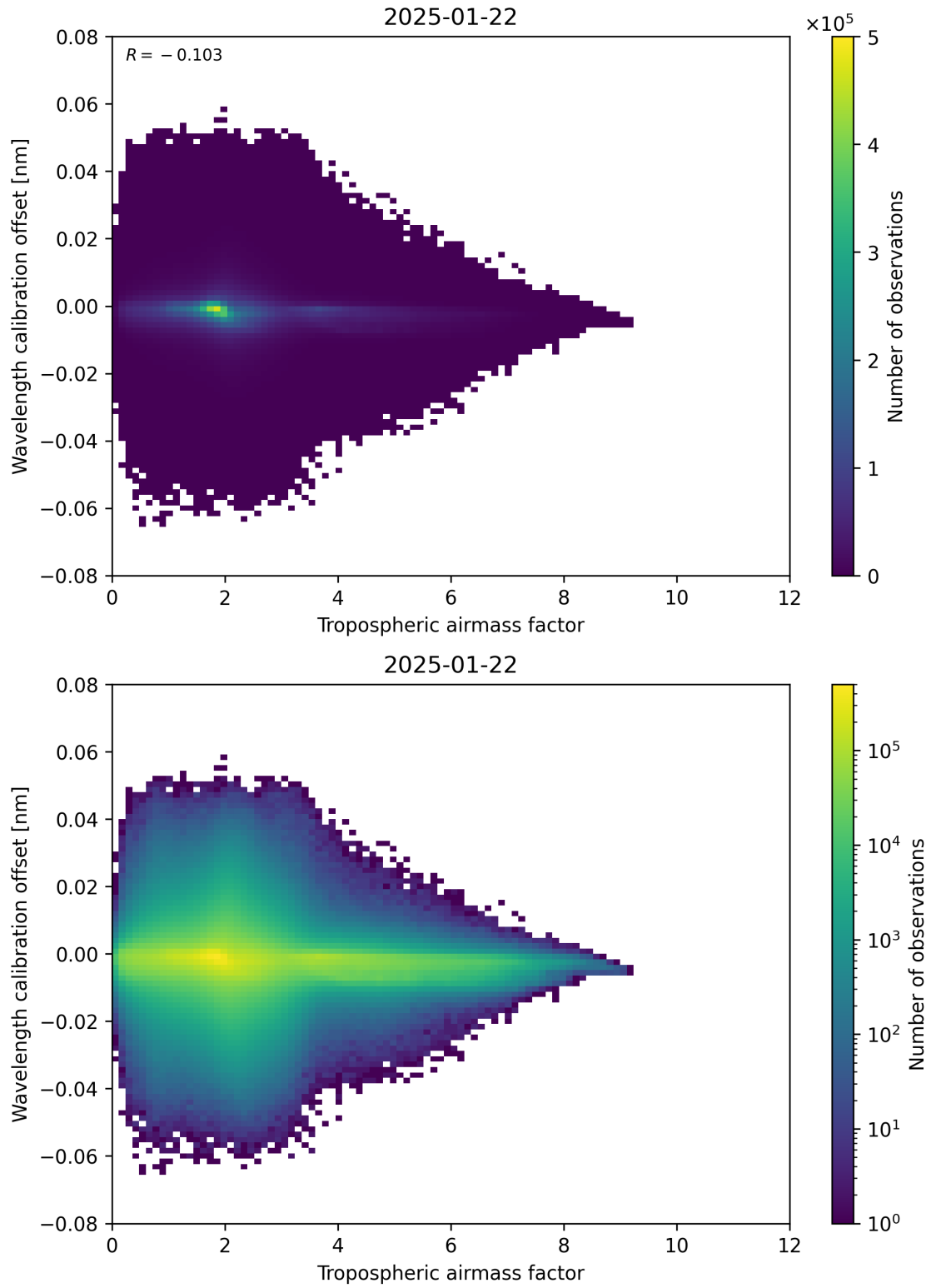
Figure 80: Scatter density plot of “Tropospheric airmass factor” against “Wavelength calibration offset” for 2025-01-21 to 2025-01-23.
