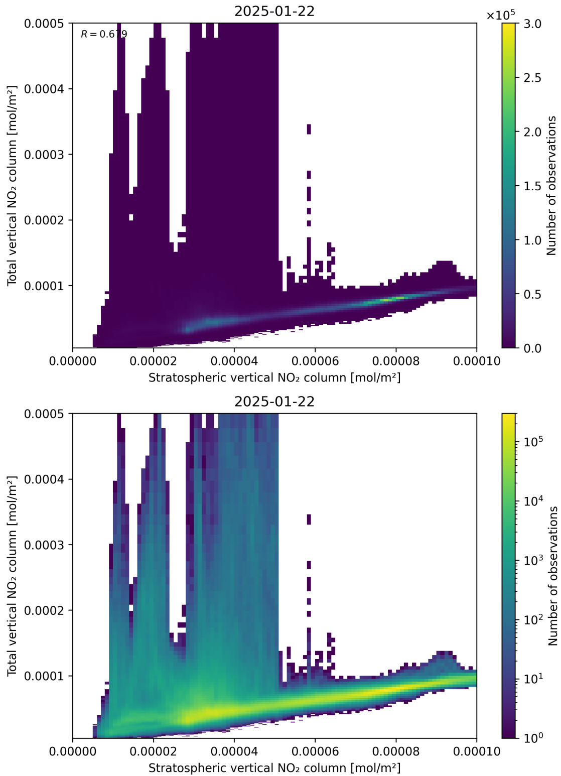
Figure 100: Scatter density plot of “Stratospheric vertical NO 2 column” against “Total vertical NO 2 column” for 2025-01-21 to 2025-01-23.
