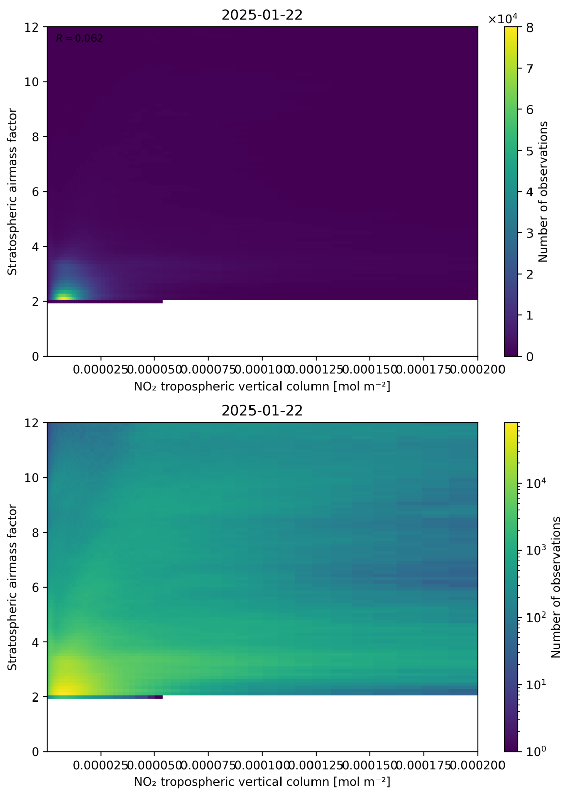
Figure 121: Scatter density plot of “NO 2 tropospheric vertical column” against “Stratospheric airmass factor” for 2025-01-21 to 2025-01-23.
