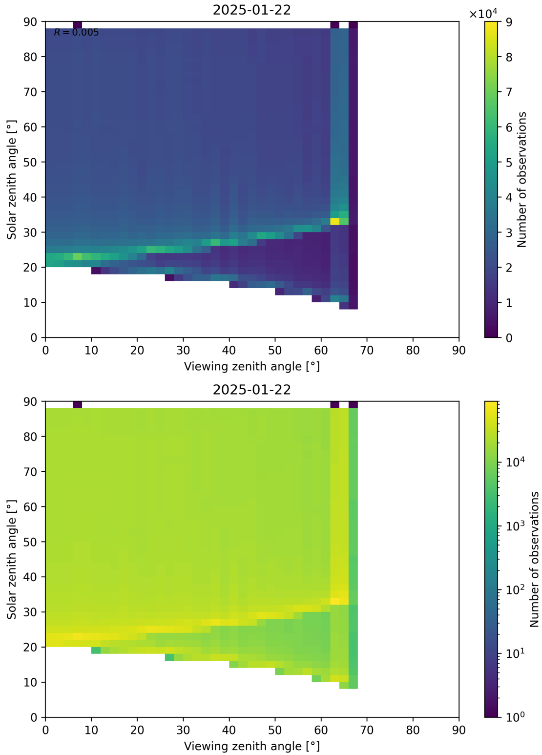
Figure 172: Scatter density plot of “Viewing zenith angle” against “Solar zenith angle” for 2025-01-21 to 2025-01-23.
