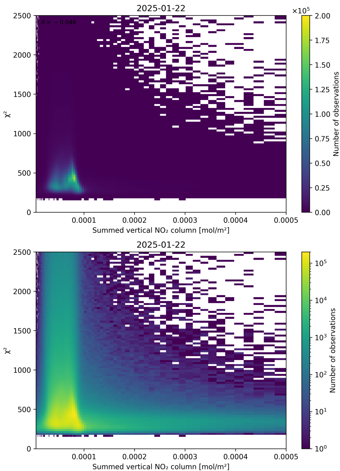
Figure 104: Scatter density plot of “Summed vertical NO 2 column” against “ \chi^2 ” for 2025-01-21 to 2025-01-23.
