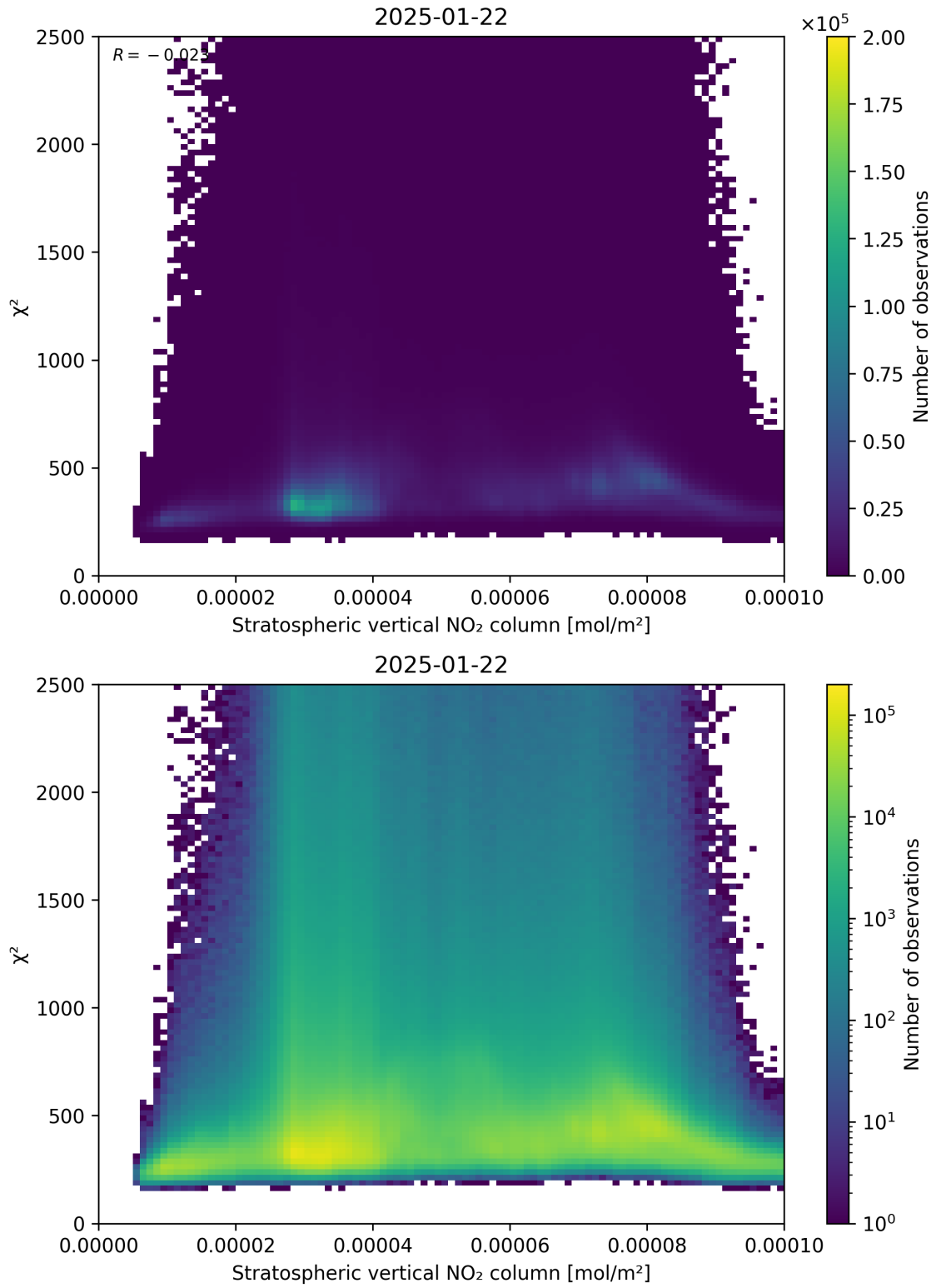
Figure 97: Scatter density plot of “Stratospheric vertical NO 2 column” against “ \chi^2 ” for 2025-01-21 to 2025-01-23.
