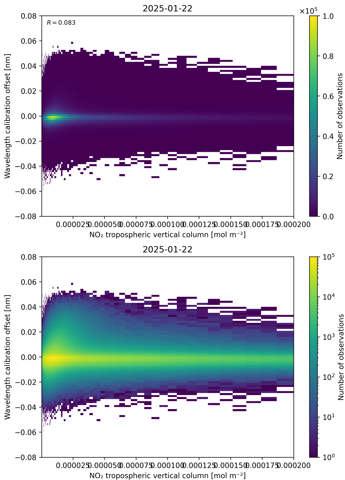
Figure 143: Scatter density plot of “NO 2 tropospheric vertical column” against “Wavelength calibration offset” for 2025-01-21 to 2025-01-23.
