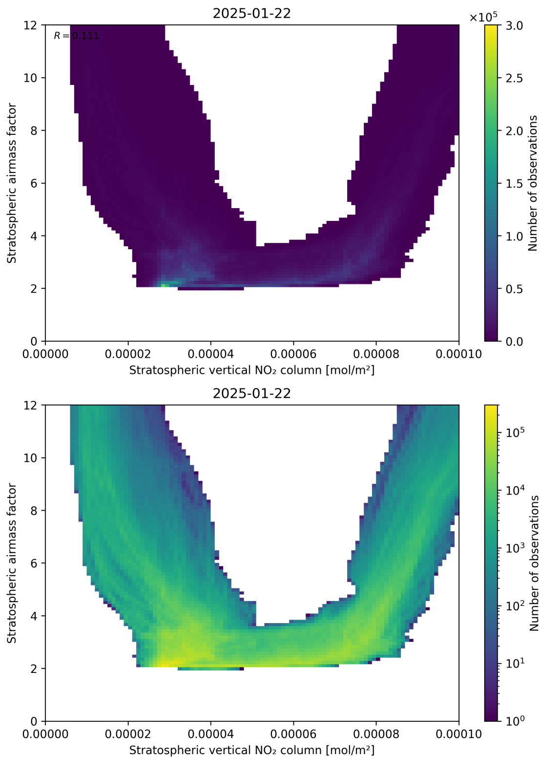
Figure 96: Scatter density plot of “Stratospheric vertical NO 2 column” against “Stratospheric airmass factor” for 2025-01-21 to 2025-01-23.
