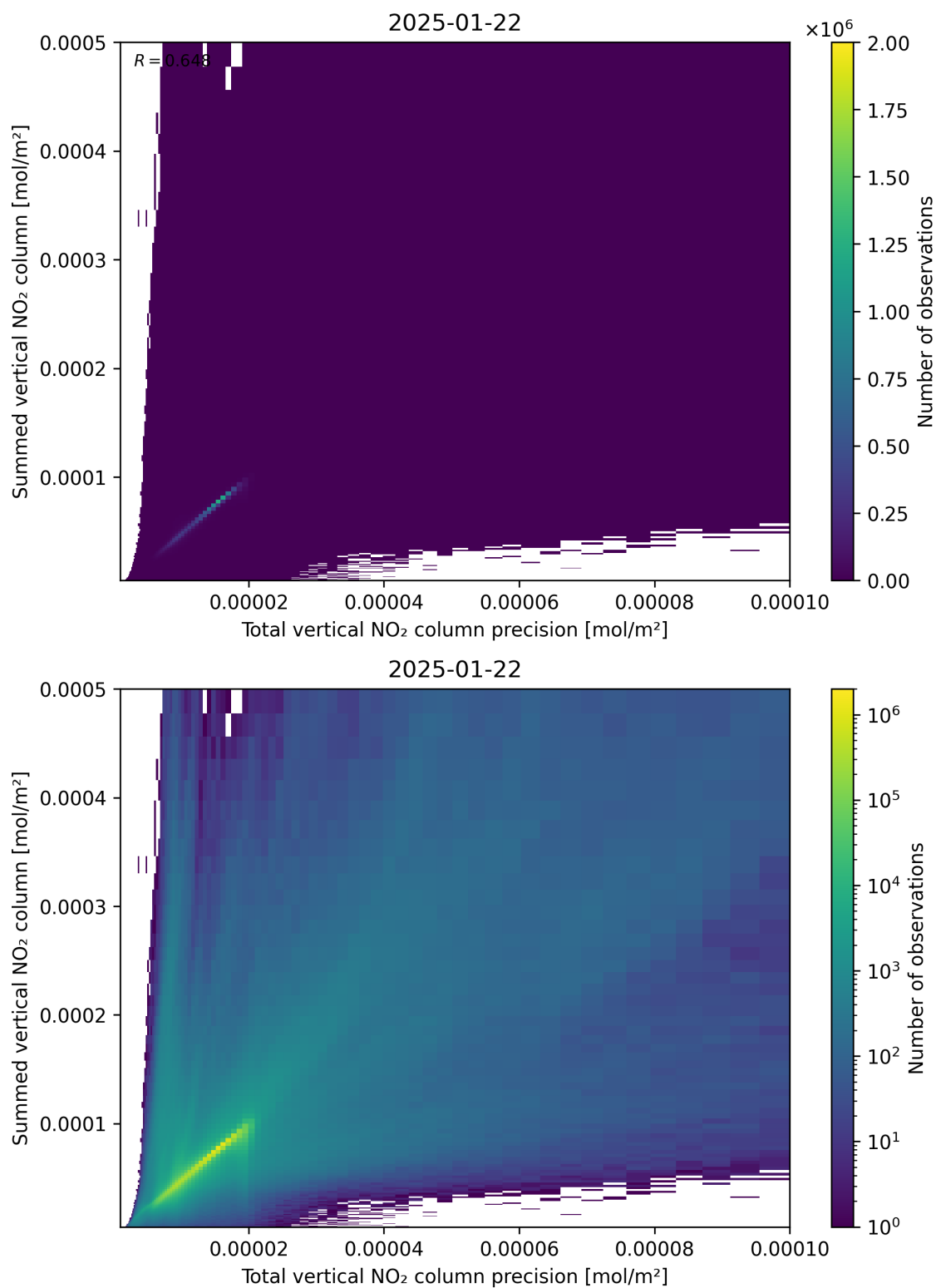
Figure 117: Scatter density plot of “Total vertical NO 2 column precision” against “Summed vertical NO 2 column” for 2025-01-21 to 2025-01-23.
