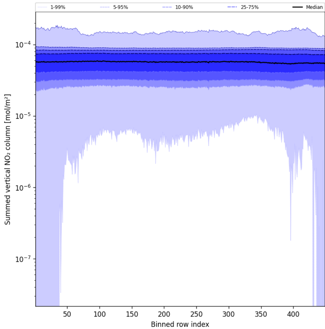
Figure 57: Along track statistics of “Summed vertical NO 2 column” for 2025-01-21 to 2025-01-23
