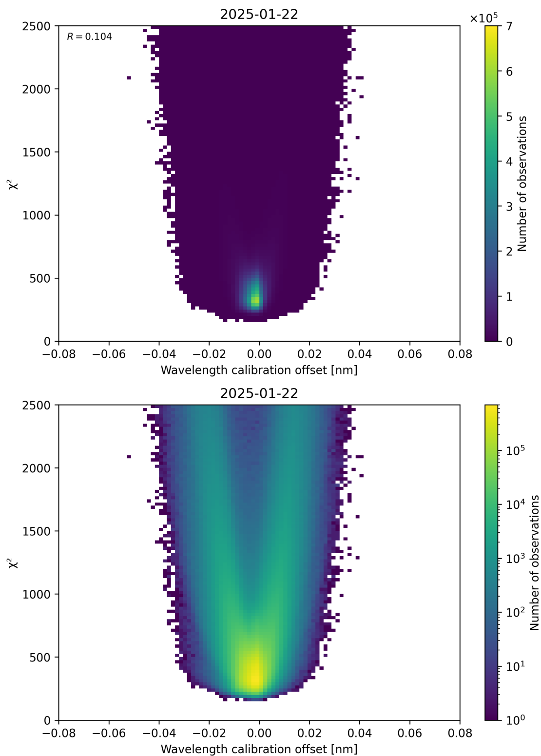
Figure 175: Scatter density plot of “Wavelength calibration offset” against “ \chi^2 ” for 2025-01-21 to 2025-01-23.
