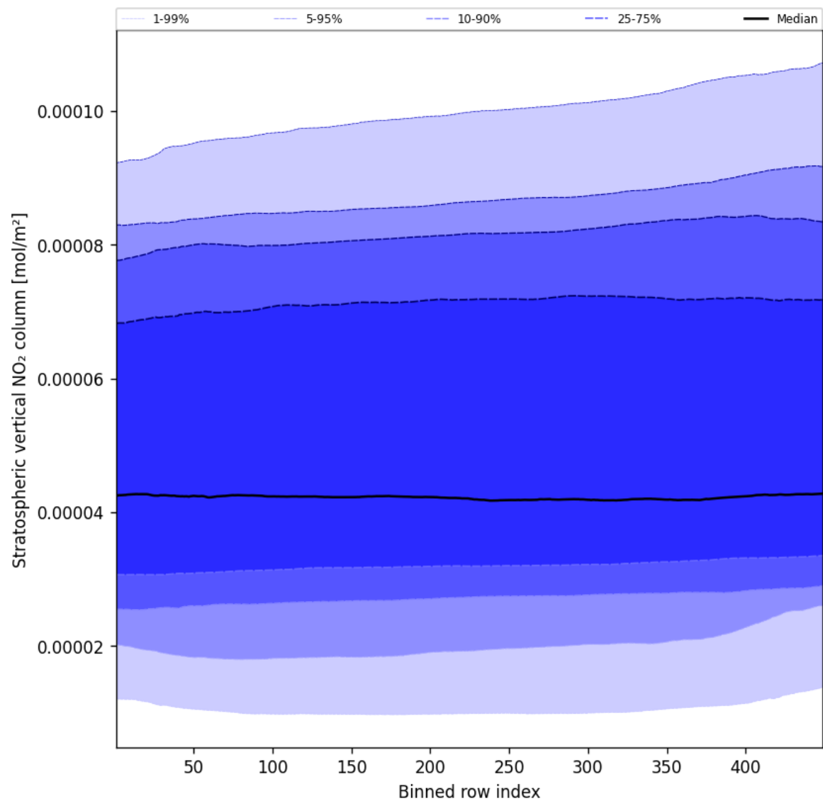
Figure 53: Along track statistics of “Stratospheric vertical NO 2 column” for 2025-01-21 to 2025-01-23
