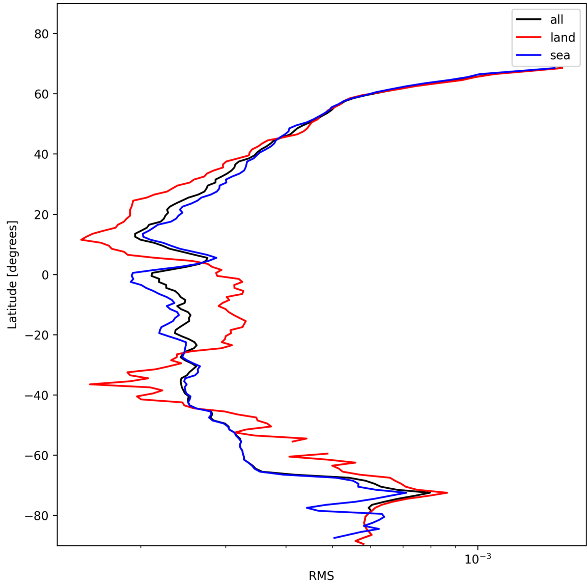
Figure 26: Zonal average of “RMS” for 2025-01-21 to 2025-01-23.
