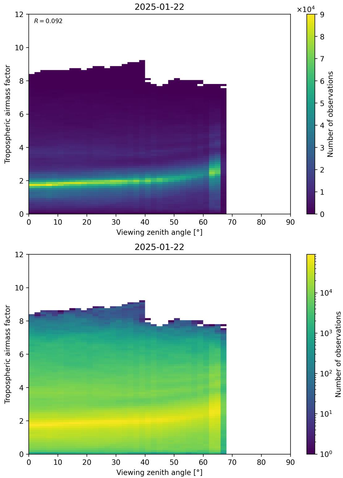
Figure 161: Scatter density plot of “Viewing zenith angle” against “Tropospheric airmass factor” for 2025-01-21 to 2025-01-23.
