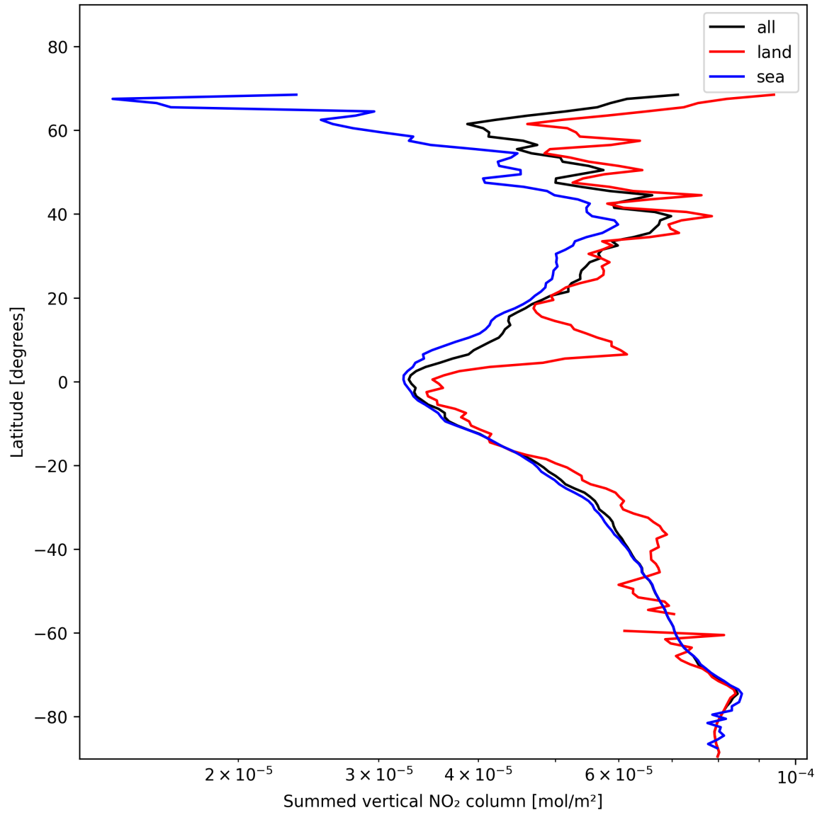
Figure 23: Zonal average of “Summed vertical NO 2 column” for 2025-01-21 to 2025-01-23.
