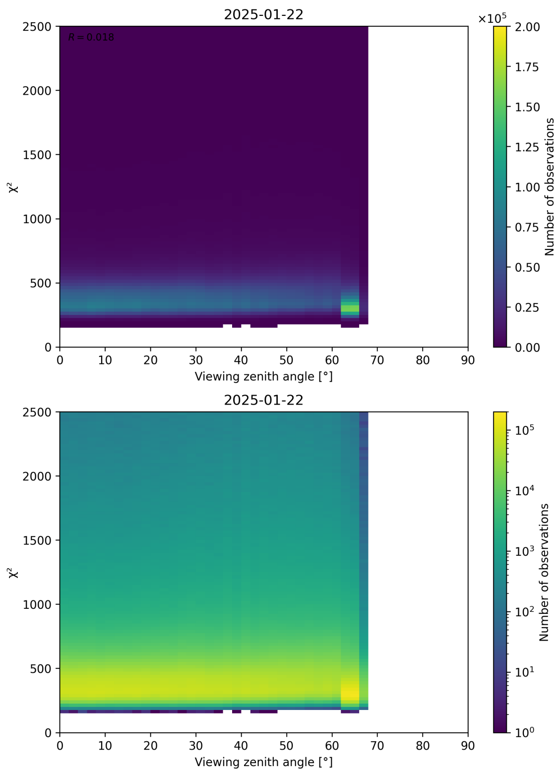
Figure 162: Scatter density plot of “Viewing zenith angle” against “ \chi^2 ” for 2025-01-21 to 2025-01-23.
