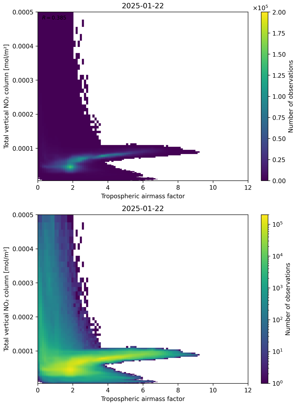
Figure 77: Scatter density plot of “Tropospheric airmass factor” against “Total vertical NO 2 column” for 2025-01-21 to 2025-01-23.
