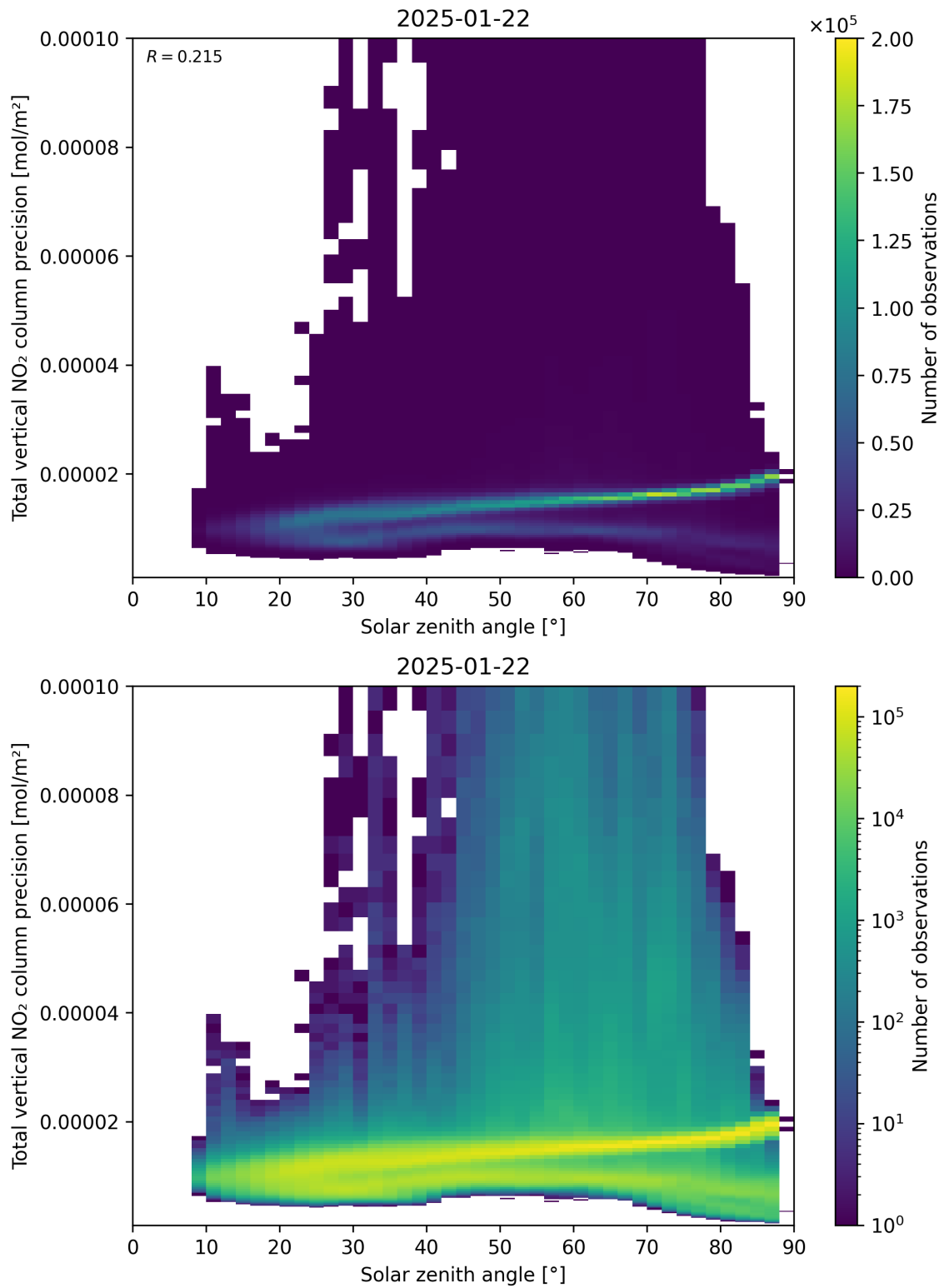
Figure 154: Scatter density plot of “Solar zenith angle” against “Total vertical NO 2 column precision” for 2025-01-21 to 2025-01-23.
