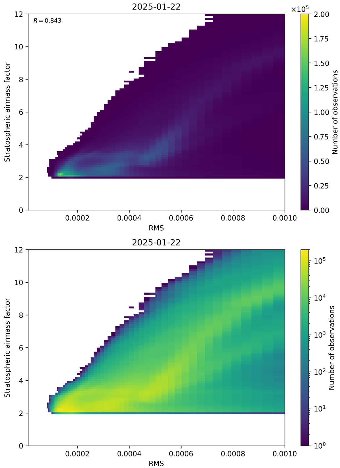
Figure 144: Scatter density plot of “RMS” against “Stratospheric airmass factor” for 2025-01-21 to 2025-01-23.
