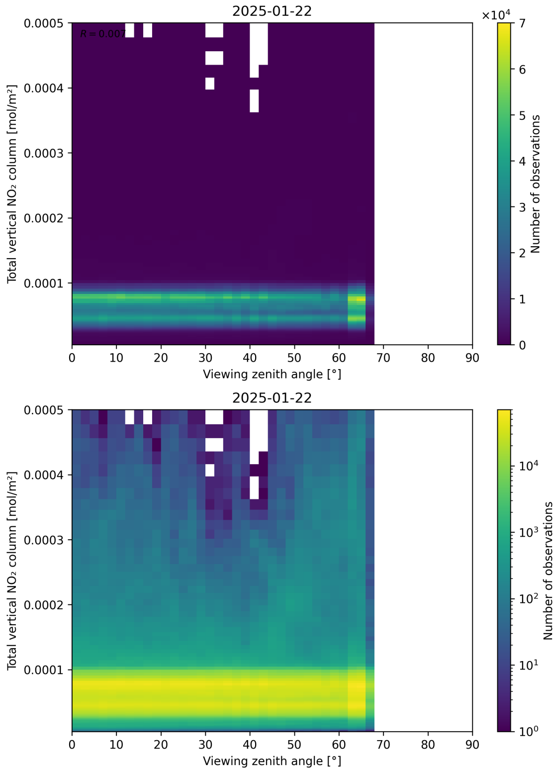
Figure 167: Scatter density plot of “Viewing zenith angle” against “Total vertical NO 2 column” for 2025-01-21 to 2025-01-23.
