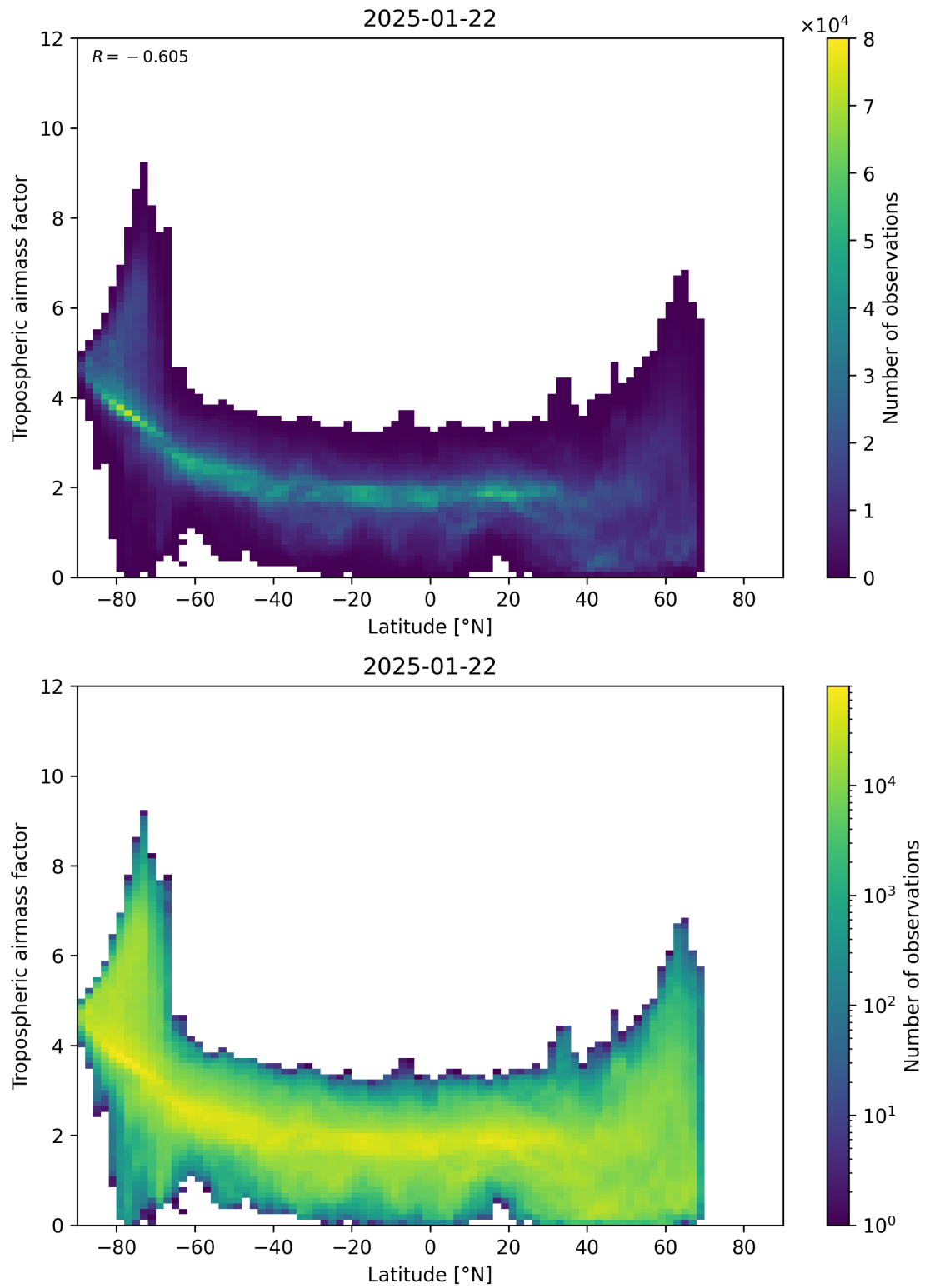
Figure 85: Scatter density plot of “Latitude” against “Tropospheric airmass factor” for 2025-01-21 to 2025-01-23.
