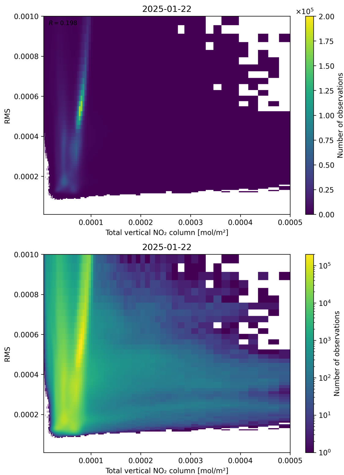
Figure 120: Scatter density plot of “Total vertical NO 2 column” against “RMS” for 2025-01-21 to 2025-01-23.
