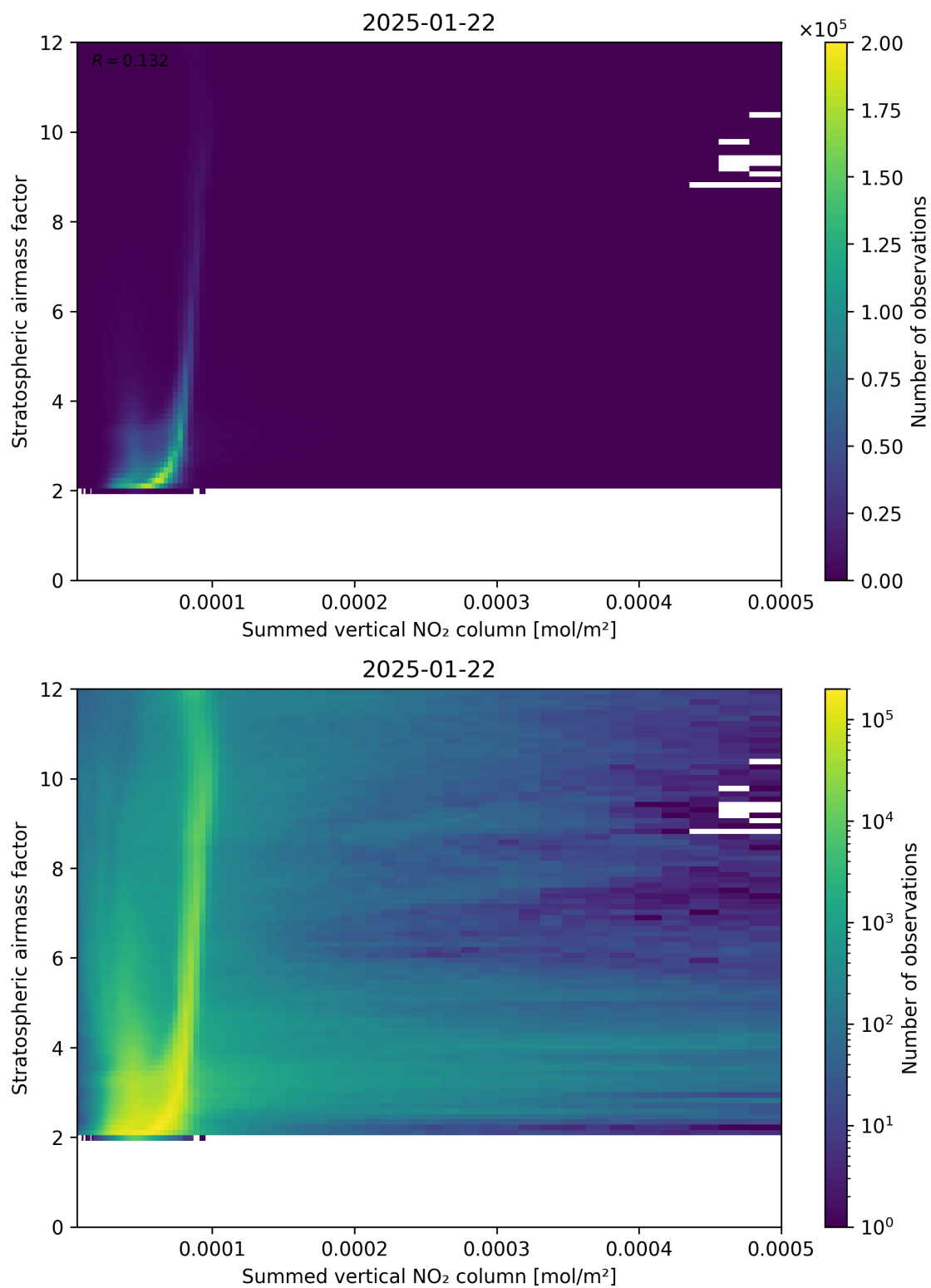
Figure 103: Scatter density plot of “Summed vertical NO 2 column” against “Stratospheric airmass factor” for 2025-01-21 to 2025-01-23.
