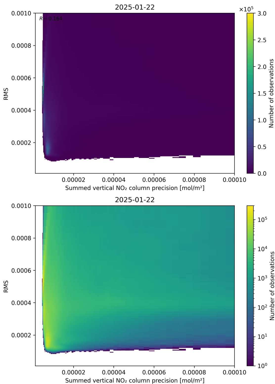
Figure 108: Scatter density plot of “Summed vertical NO 2 column precision” against “RMS” for 2025-01-21 to 2025-01-23.
