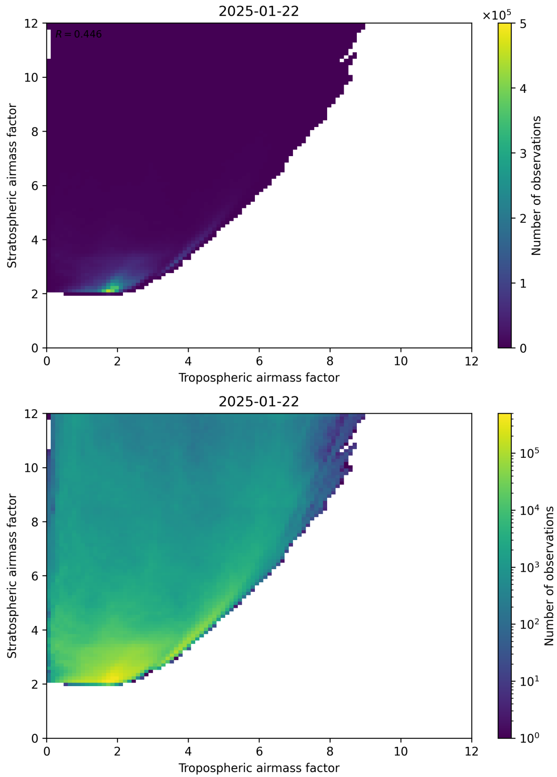
Figure 71: Scatter density plot of “Tropospheric airmass factor” against “Stratospheric airmass factor” for 2025-01-21 to 2025-01-23.
