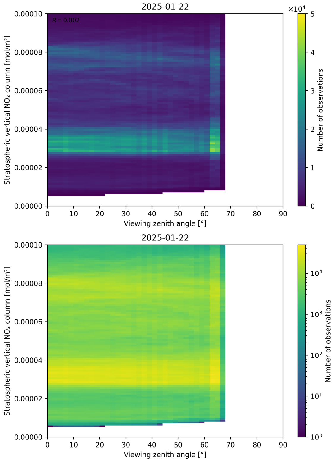
Figure 164: Scatter density plot of “Viewing zenith angle” against “Stratospheric vertical NO 2 column” for 2025-01-21 to 2025-01-23.
