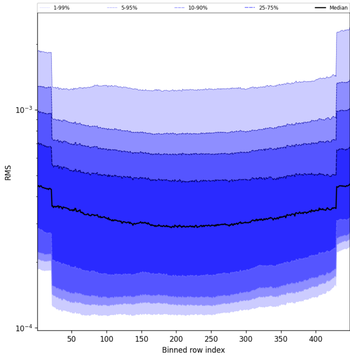
Figure 60: Along track statistics of “RMS” for 2025-01-21 to 2025-01-23
