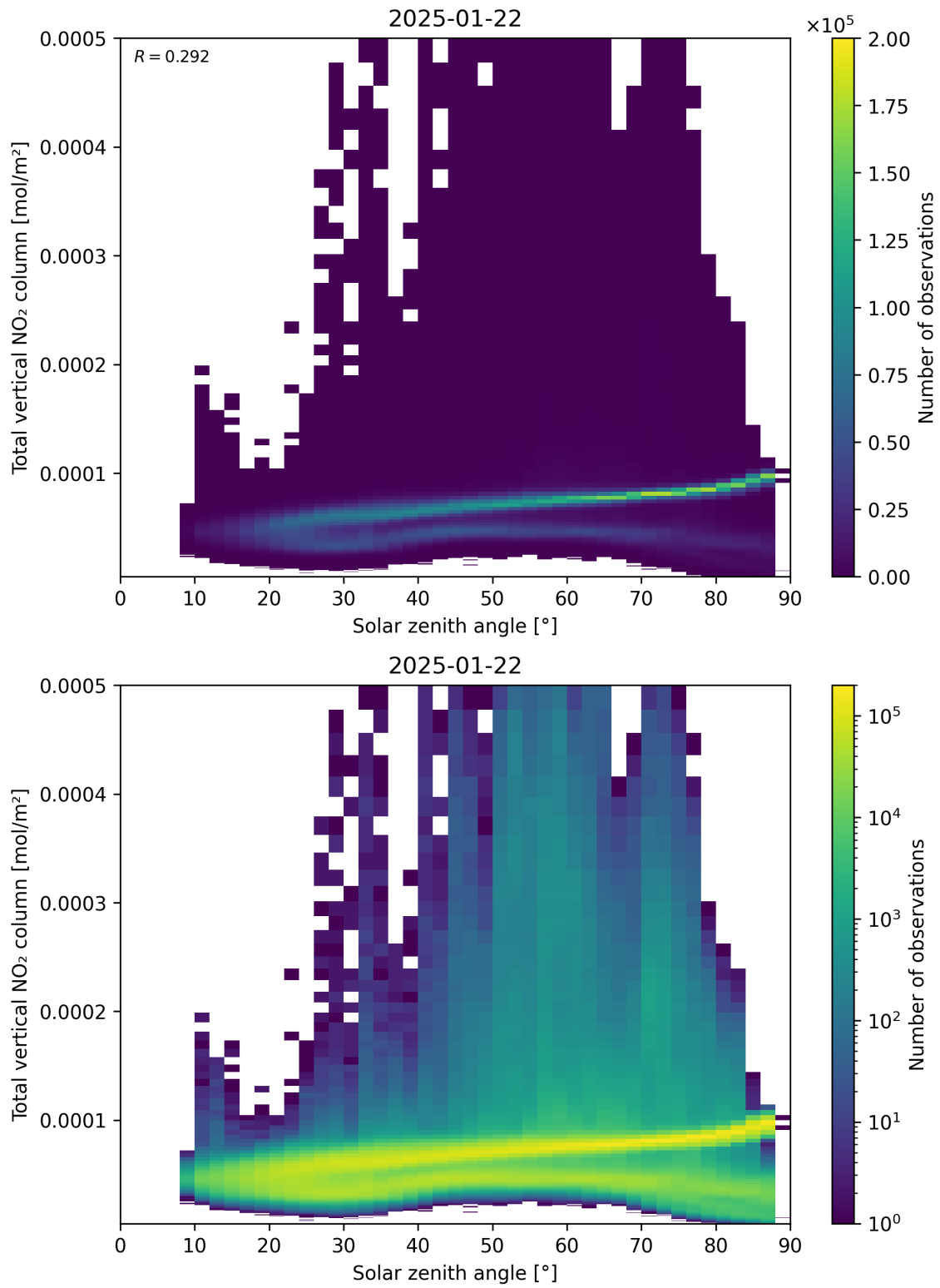
Figure 153: Scatter density plot of “Solar zenith angle” against “Total vertical NO 2 column” for 2025-01-21 to 2025-01-23.
