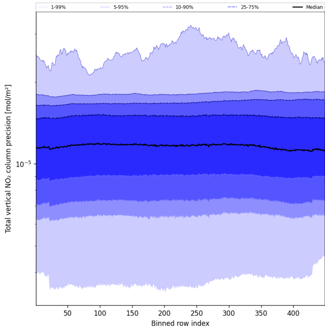
Figure 56: Along track statistics of “Total vertical NO 2 column precision” for 2025-01-21 to 2025-01-23
