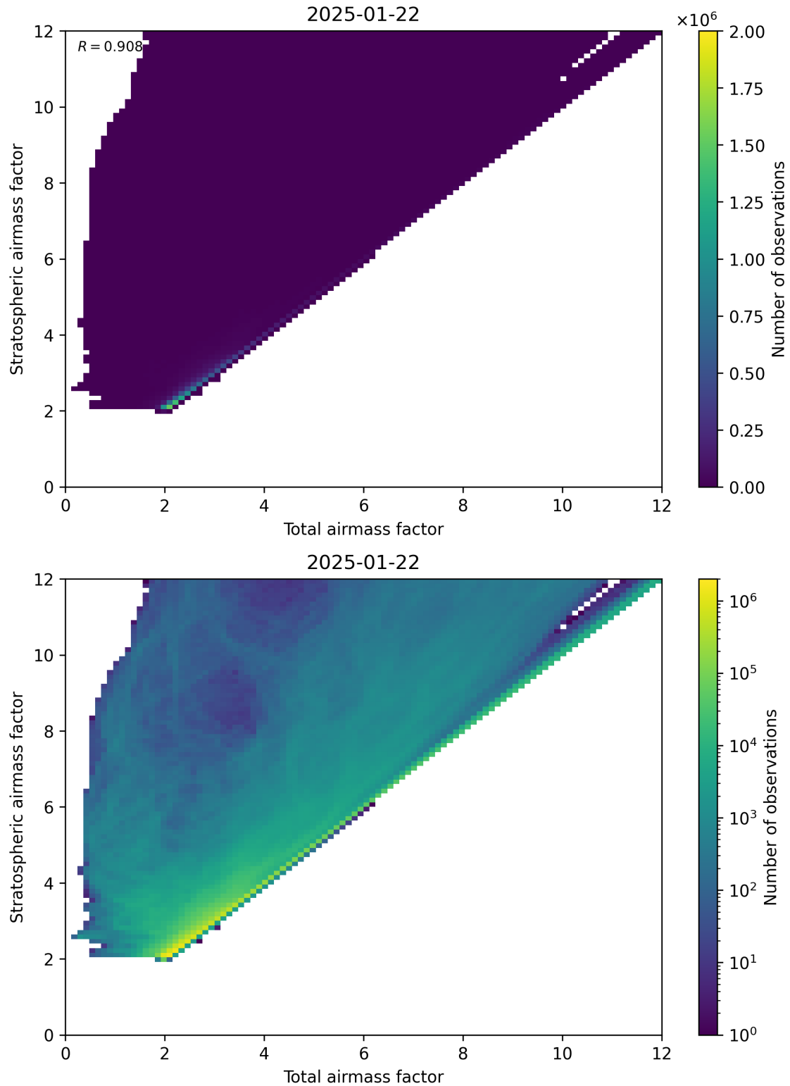
Figure 62: Scatter density plot of “Total airmass factor” against “Stratospheric airmass factor” for 2025-01-21 to 2025-01-23.
