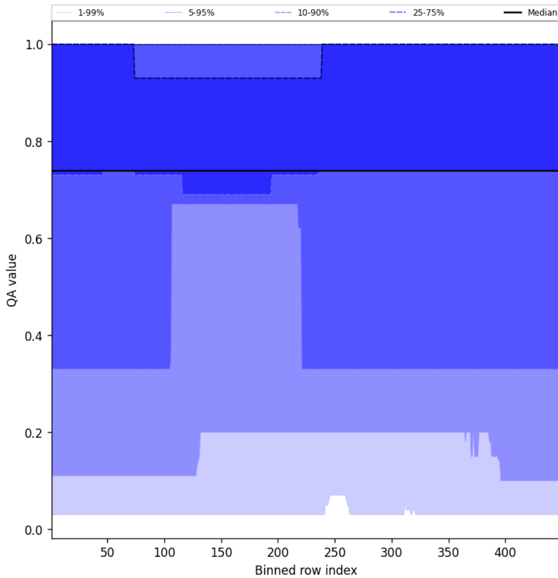
Figure 45: Along track statistics of “QA value” for 2025-01-21 to 2025-01-23
