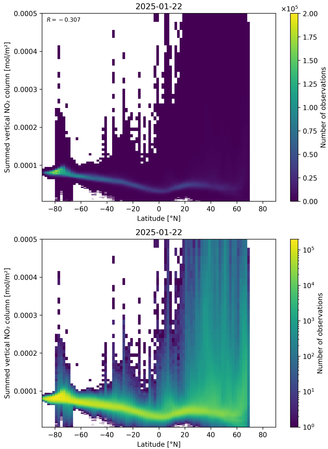
Figure 88: Scatter density plot of “Latitude” against “Summed vertical NO 2 column” for 2025-01-21 to 2025-01-23.
