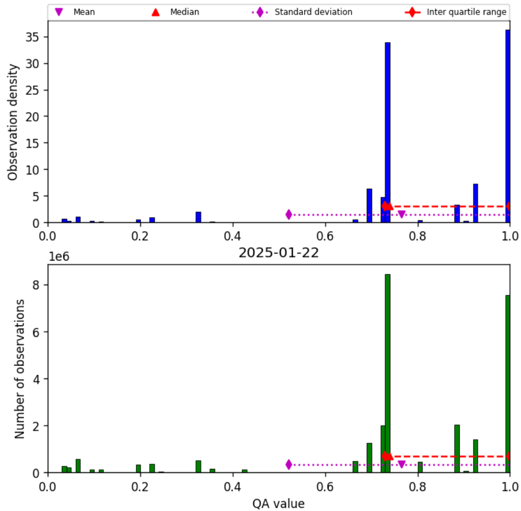
Figure 28: Histogram of “QA value” for 2025-01-21 to 2025-01-23
