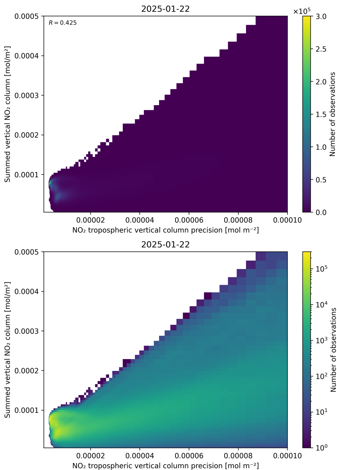
Figure 136: Scatter density plot of “NO 2 tropospheric vertical column precision” against “Summed vertical NO 2 column” for 2025-01-21 to 2025-01-23.
