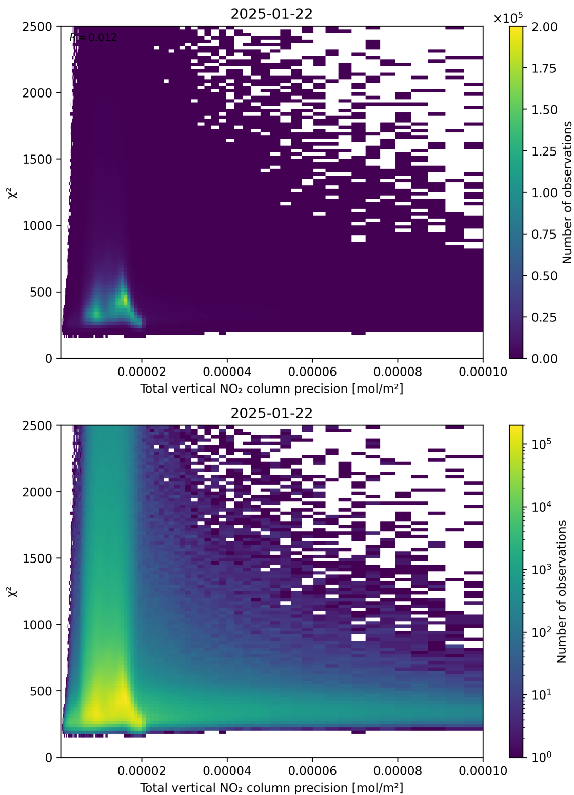
Figure 116: Scatter density plot of “Total vertical NO 2 column precision” against “ \chi^2 ” for 2025-01-21 to 2025-01-23.
