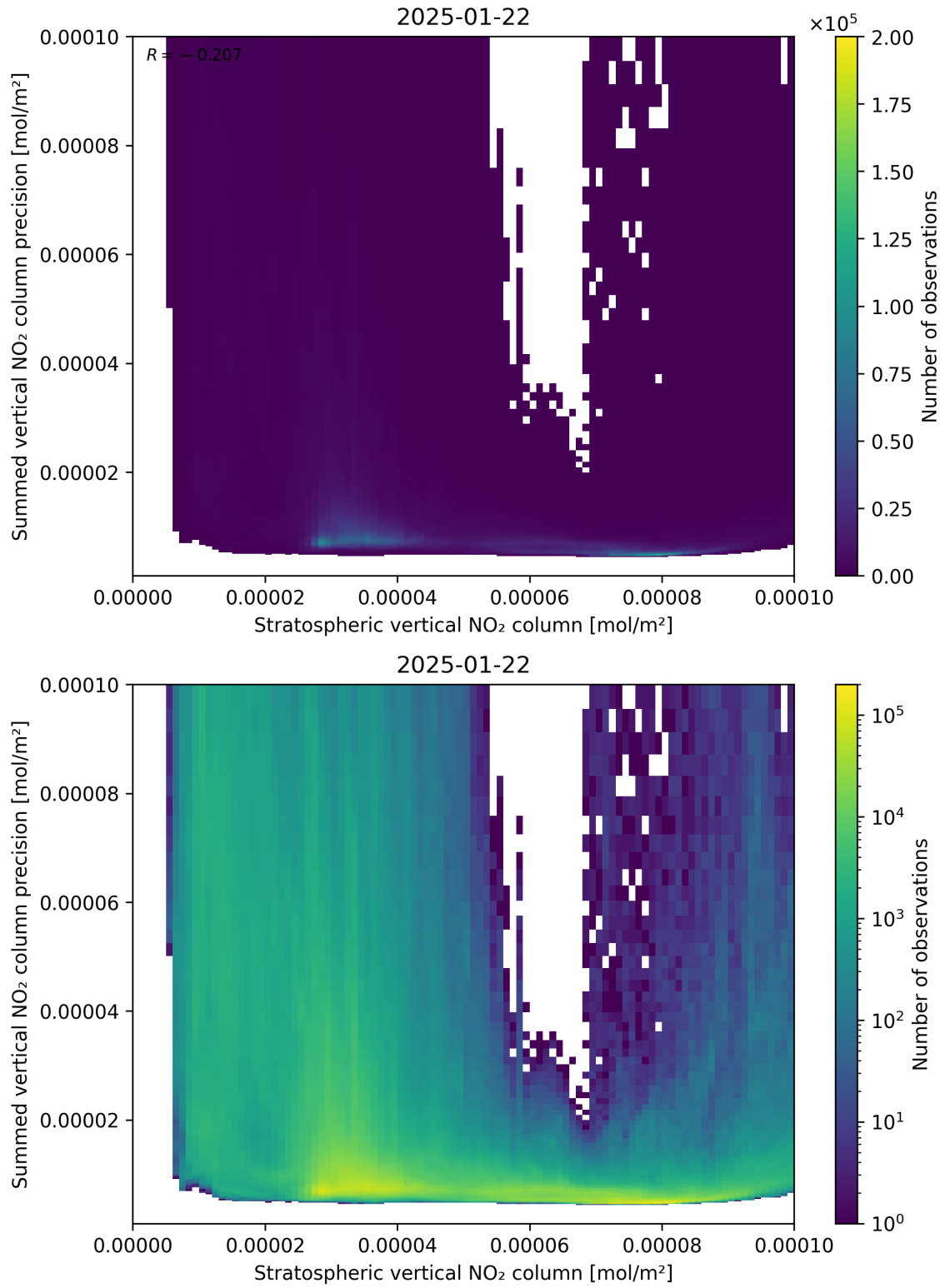
Figure 99: Scatter density plot of “Stratospheric vertical NO 2 column” against “Summed vertical NO 2 column precision” for 2025-01-21 to 2025-01-23.
