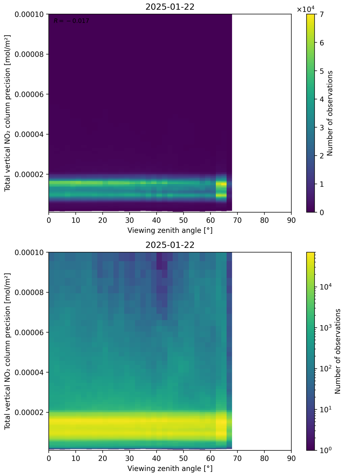
Figure 168: Scatter density plot of “Viewing zenith angle” against “Total vertical NO 2 column precision” for 2025-01-21 to 2025-01-23.
