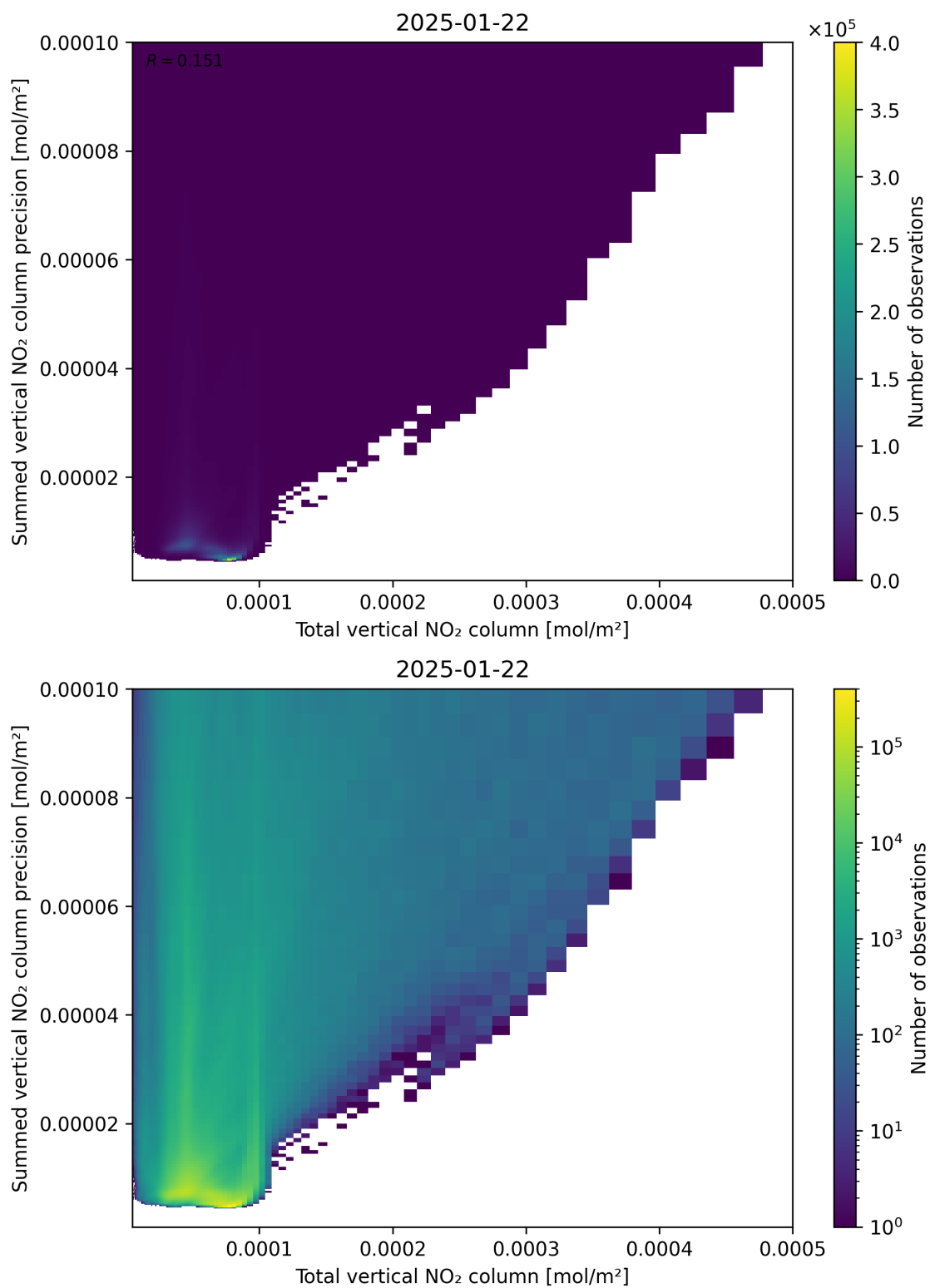
Figure 113: Scatter density plot of “Total vertical NO 2 column” against “Summed vertical NO 2 column precision” for 2025-01-21 to 2025-01-23.
