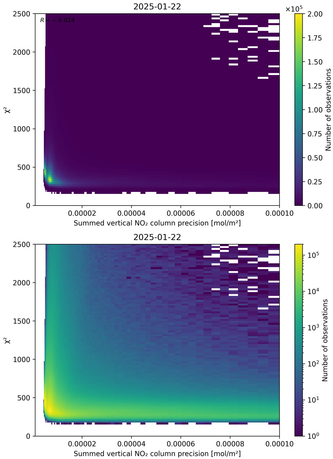
Figure 107: Scatter density plot of “Summed vertical NO 2 column precision” against “ \chi^2 ” for 2025-01-21 to 2025-01-23.
