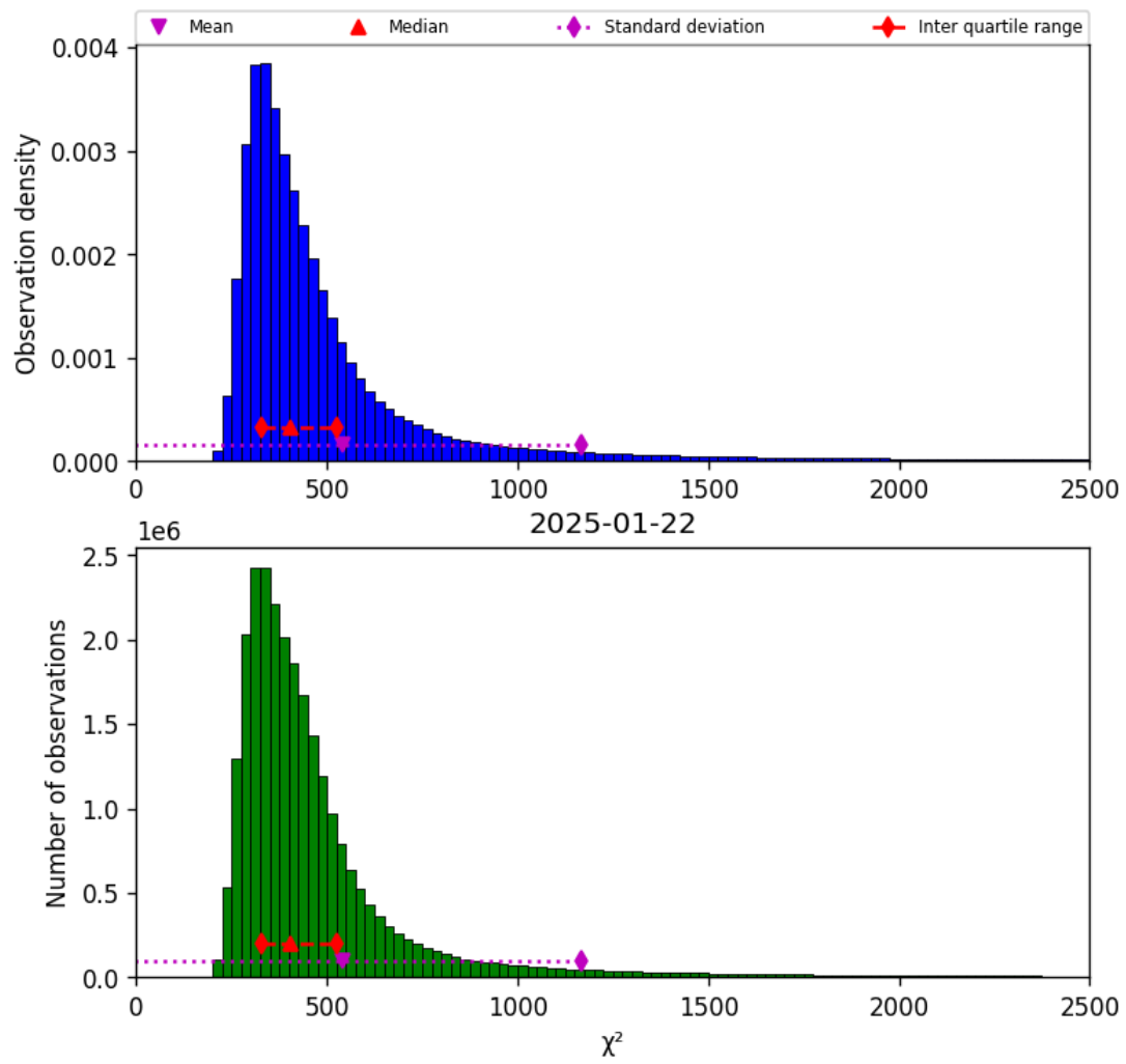
Figure 42: Histogram of " \chi^2 " for 2025-01-21 to 2025-01-23
