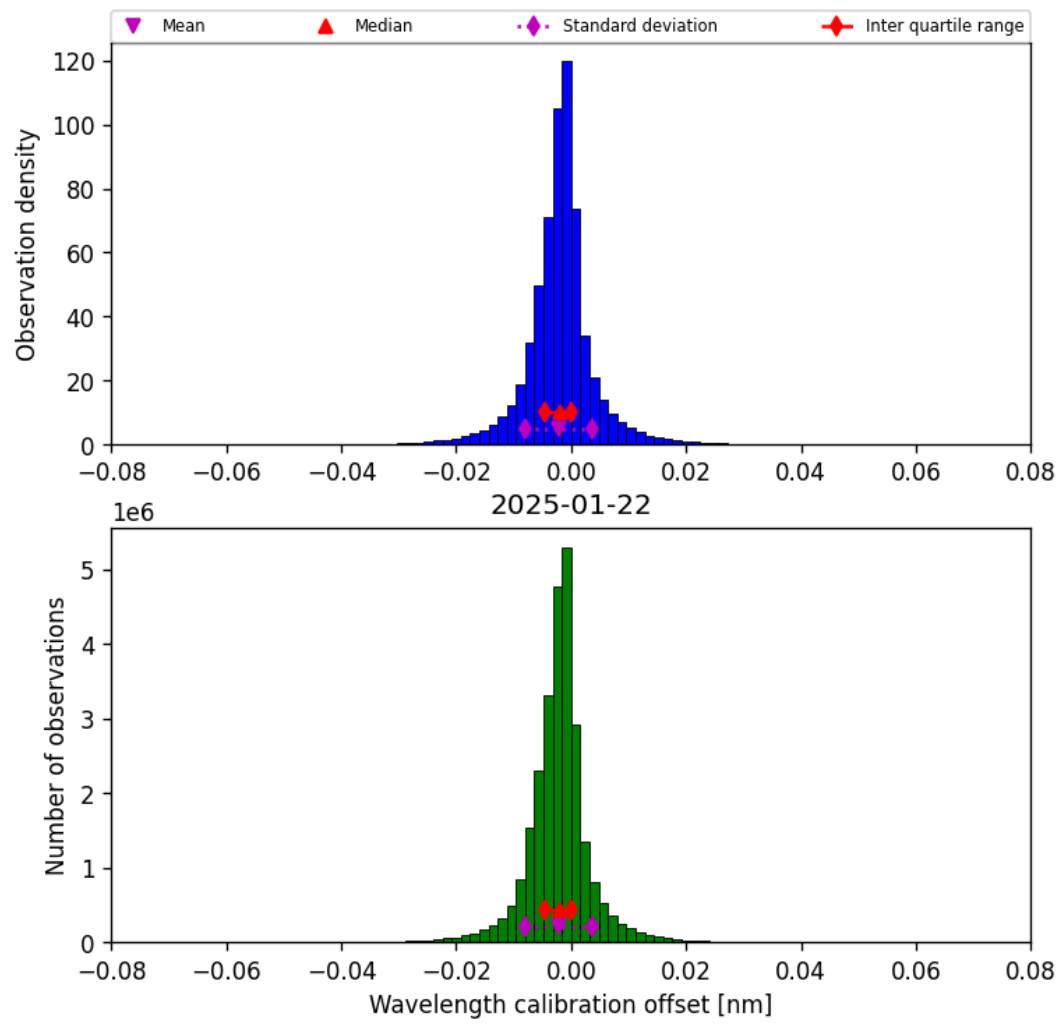
Figure 35: Histogram of “Wavelength calibration offset” for 2025-01-21 to 2025-01-23
