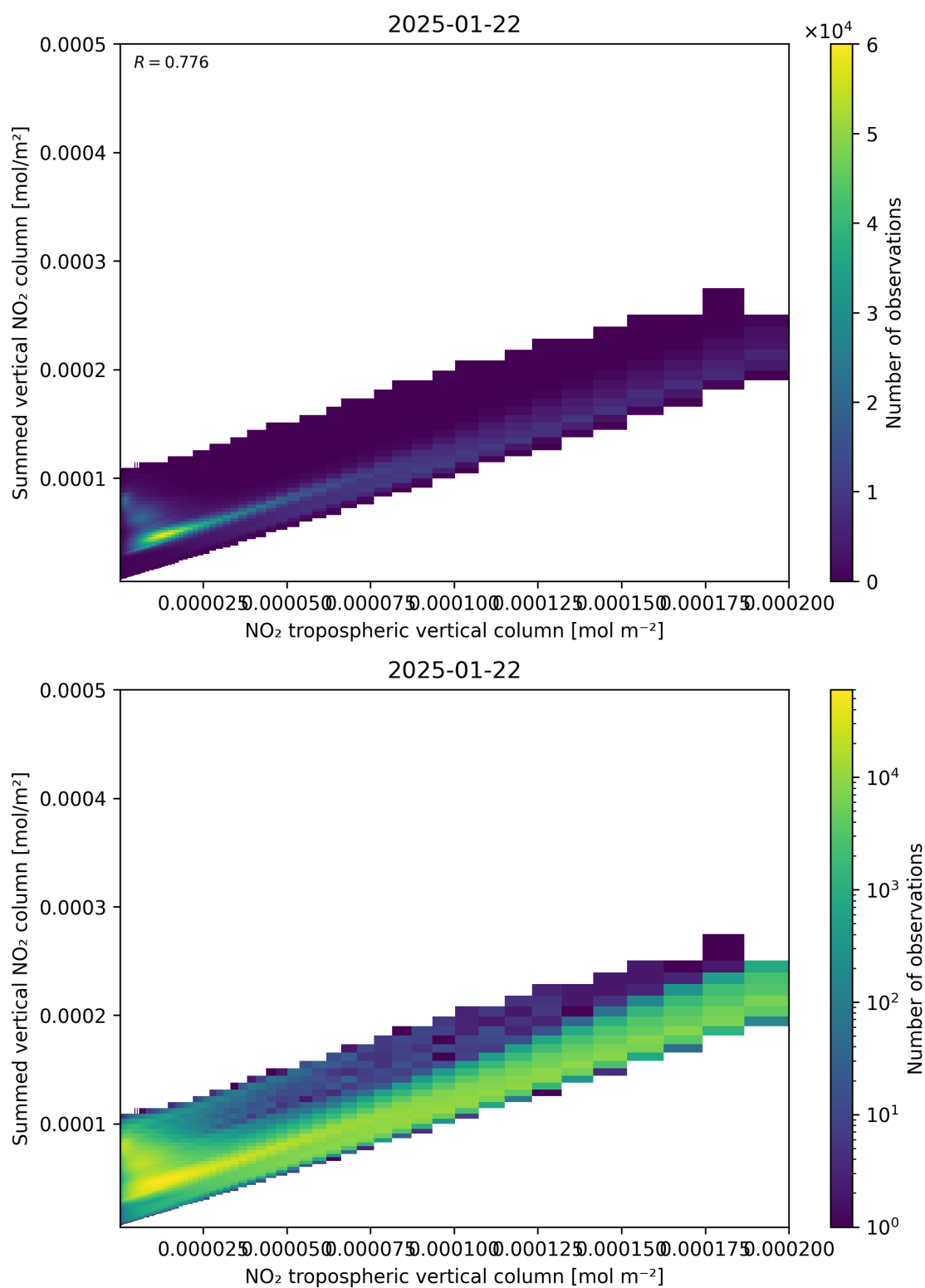
Figure 126: Scatter density plot of “NO 2 tropospheric vertical column” against “Summed vertical NO 2 column” for 2025-01-21 to 2025-01-23.
