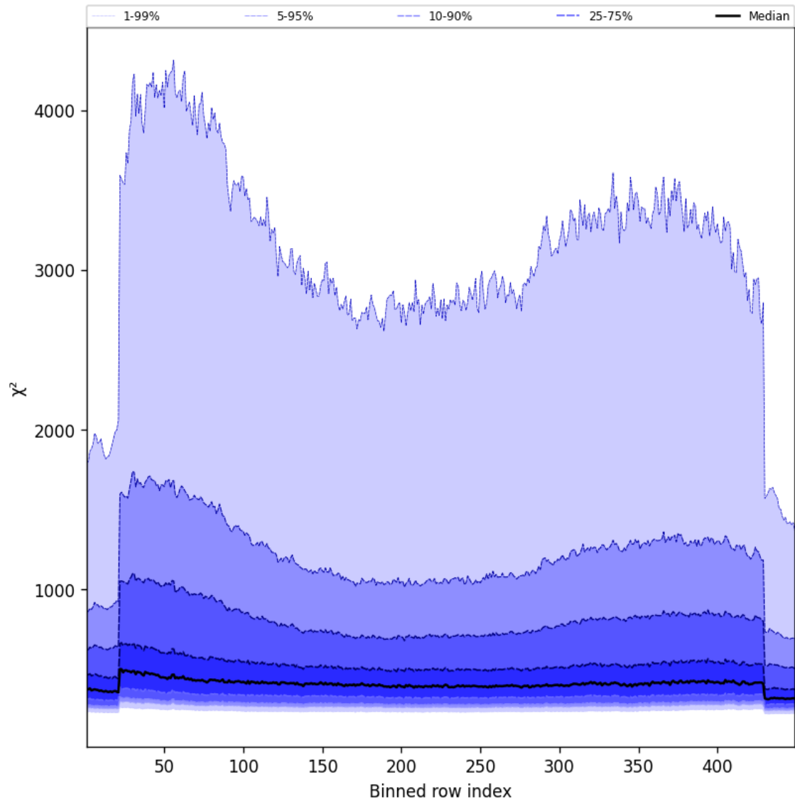
Figure 59: Along track statistics of “ \chi^2 ” for 2025-01-21 to 2025-01-23
