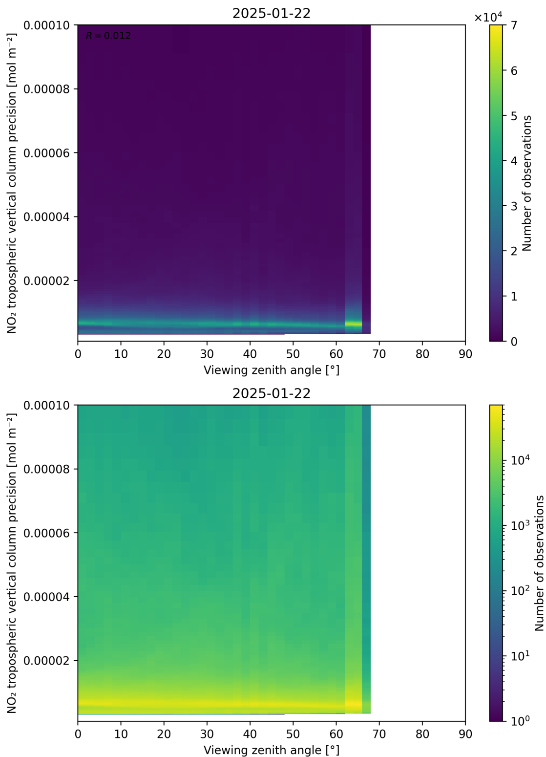
Figure 170: Scatter density plot of “Viewing zenith angle” against “NO 2 tropospheric vertical column precision” for 2025-01-21 to 2025-01-23.
