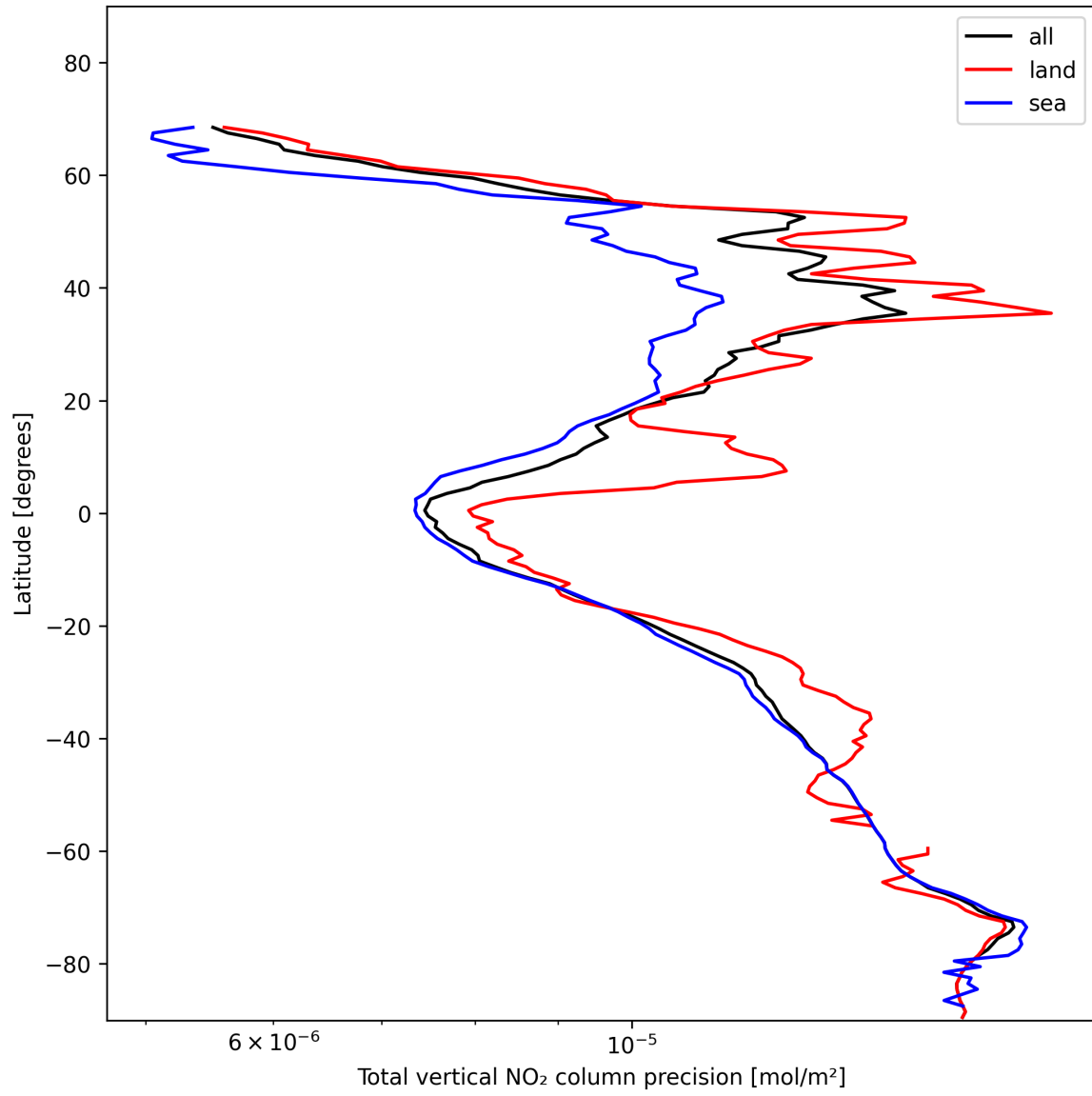
Figure 22: Zonal average of “Total vertical NO 2 column precision” for 2025-01-21 to 2025-01-23.
