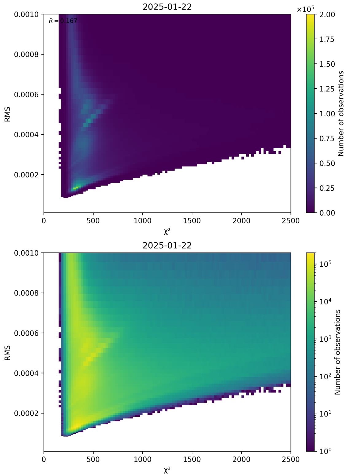
Figure 82: Scatter density plot of “ \chi^2 ” against “RMS” for 2025-01-21 to 2025-01-23.
