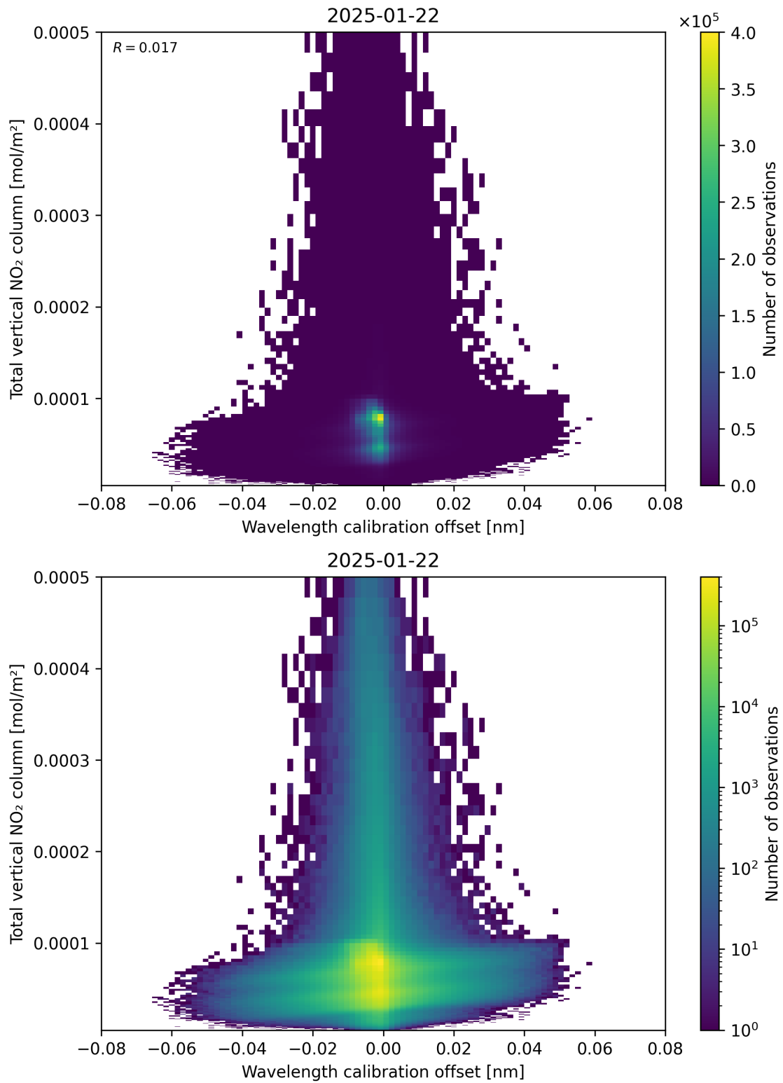
Figure 179: Scatter density plot of “Wavelength calibration offset” against “Total vertical NO 2 column” for 2025-01-21 to 2025-01-23.
