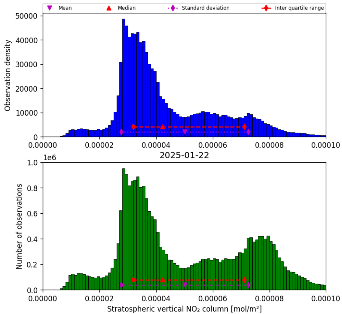
Figure 36: Histogram of “Stratospheric vertical NO 2 column” for 2025-01-21 to 2025-01-23
