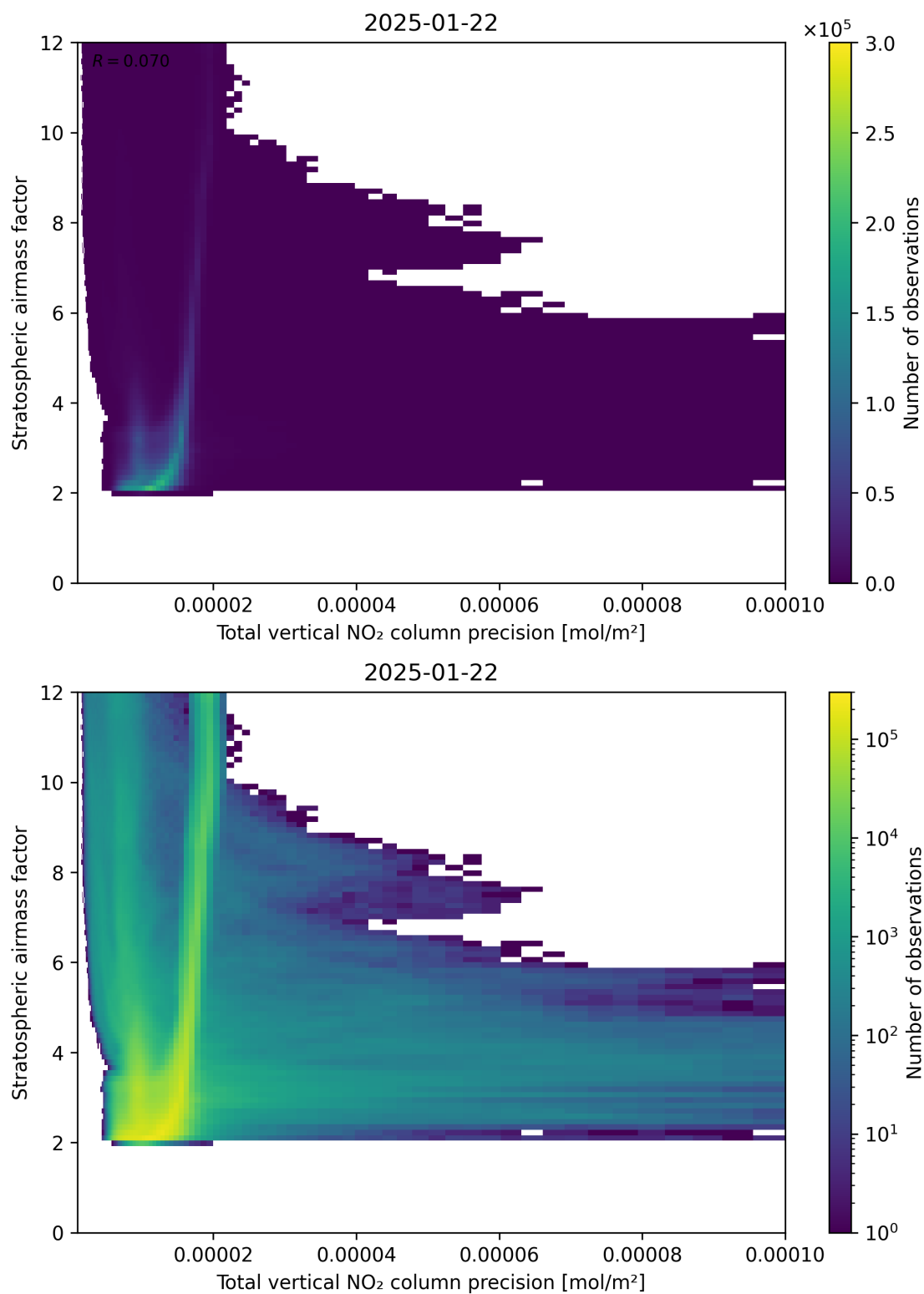
Figure 115: Scatter density plot of “Total vertical NO 2 column precision” against “Stratospheric air mass factor” for 2025-01-21 to 2025-01-23.
