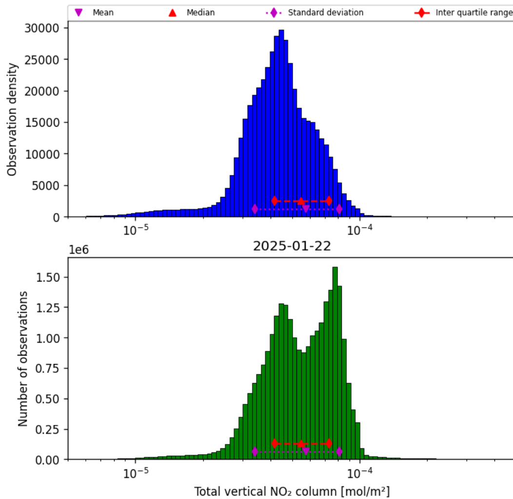
Figure 38: Histogram of “Total vertical NO 2 column” for 2025-01-21 to 2025-01-23
