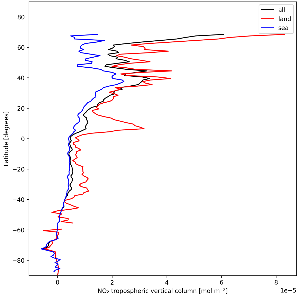
Figure 12: Zonal average of “NO 2 tropospheric vertical column” for 2025-01-21 to 2025-01-23.
