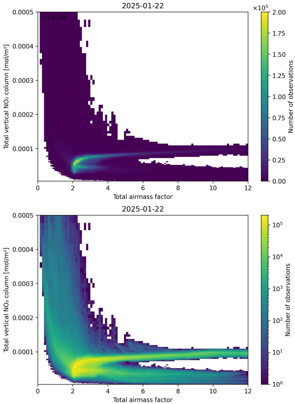
Figure 67: Scatter density plot of “Total airmass factor” against “Total vertical NO 2 column” for 2025-01-21 to 2025-01-23.
