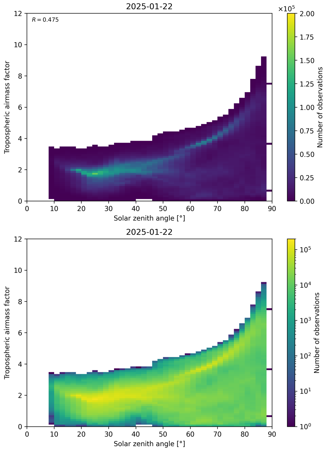
Figure 147: Scatter density plot of “Solar zenith angle” against “Tropospheric airmass factor” for 2025-01-21 to 2025-01-23.
