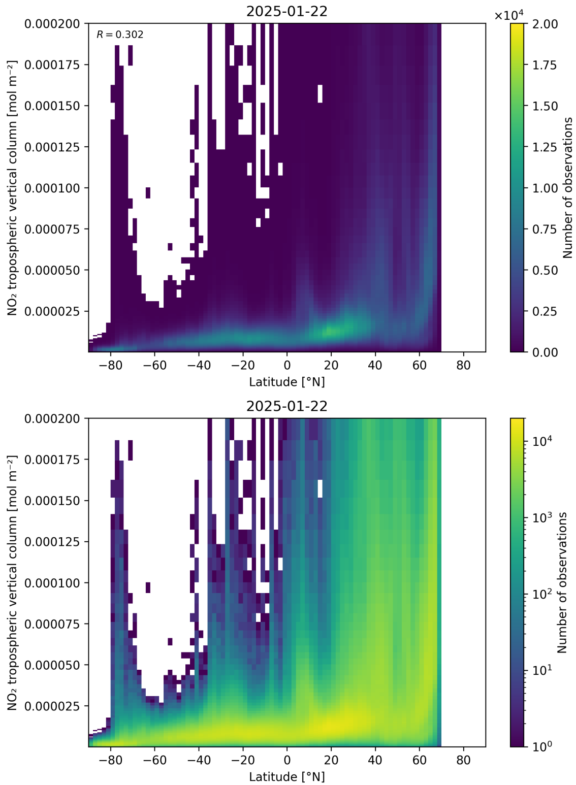
Figure 92: Scatter density plot of “Latitude” against “NO 2 tropospheric vertical column” for 2025-01-21 to 2025-01-23.
