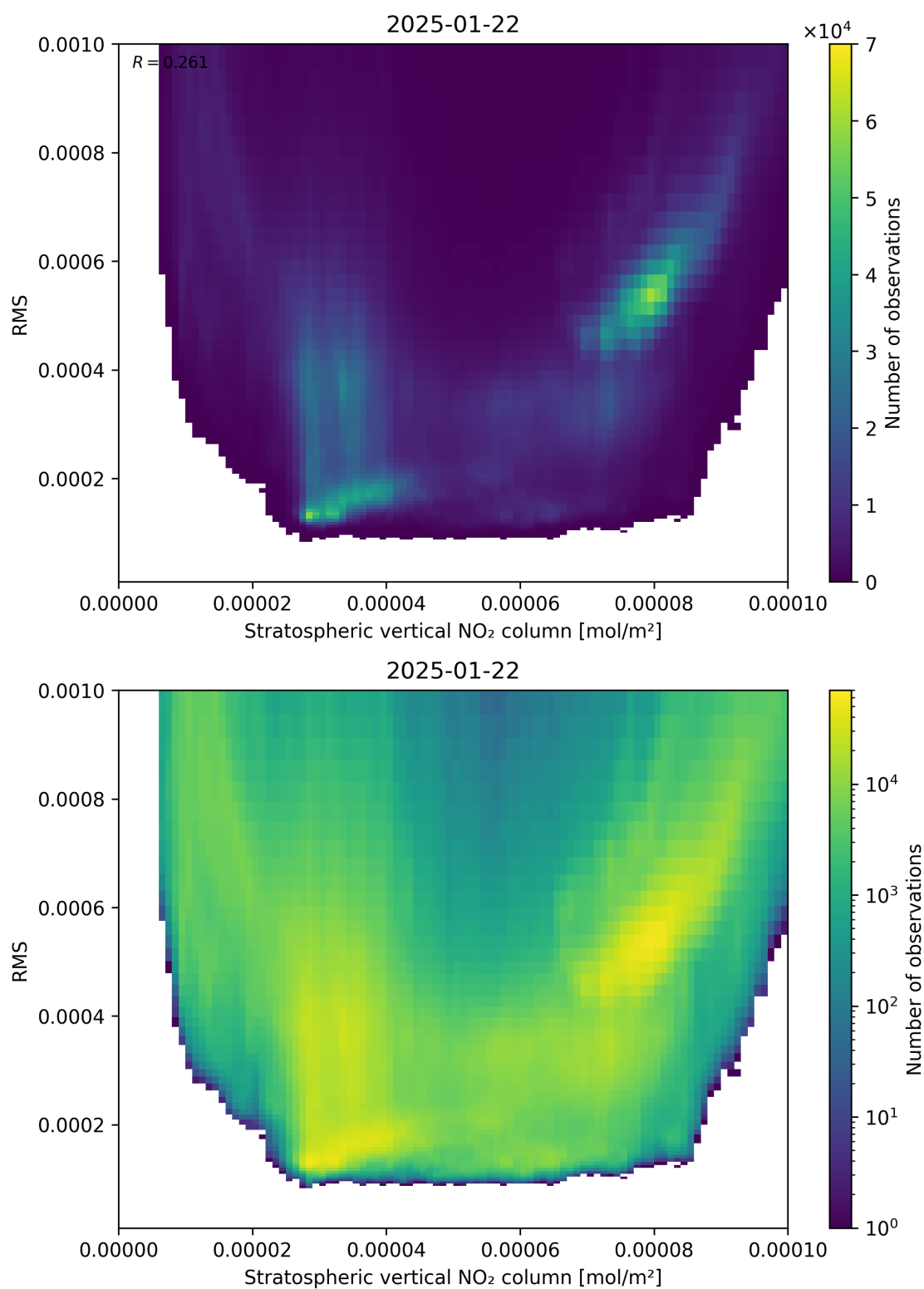
Figure 102: Scatter density plot of “Stratospheric vertical NO 2 column” against “RMS” for 2025-01-21 to 2025-01-23.
