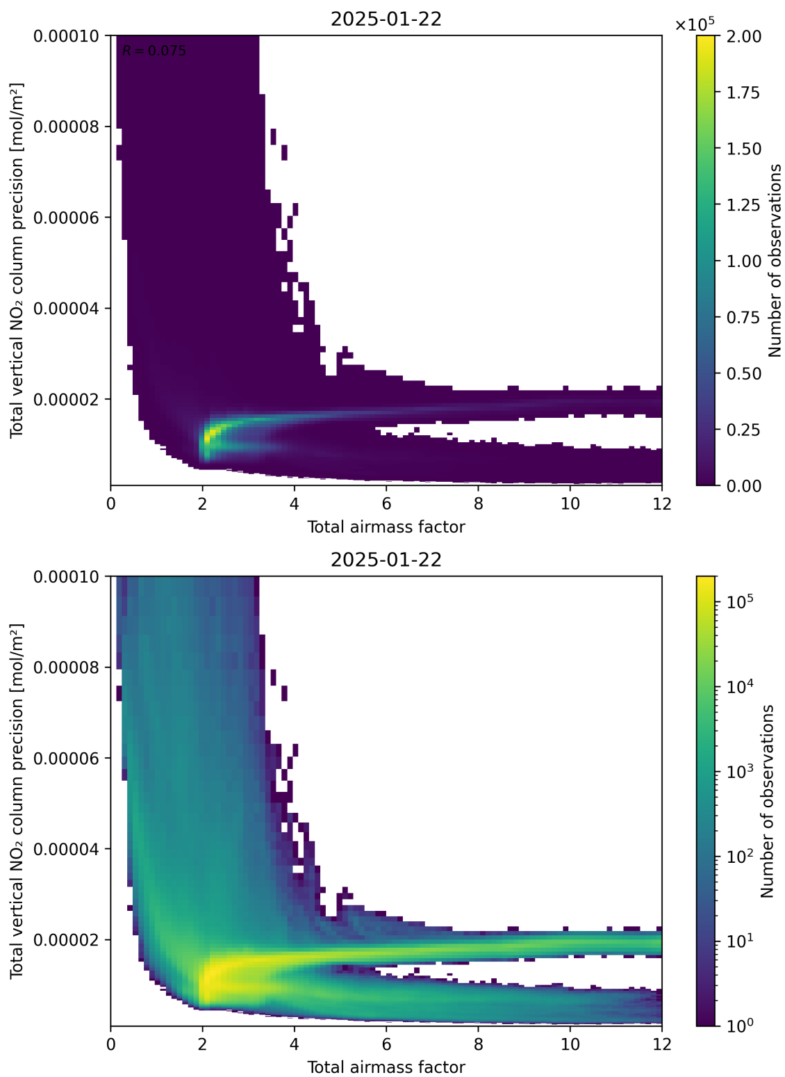
Figure 68: Scatter density plot of “Total airmass factor” against “Total vertical NO 2 column precision” for 2025-01-21 to 2025-01-23.
