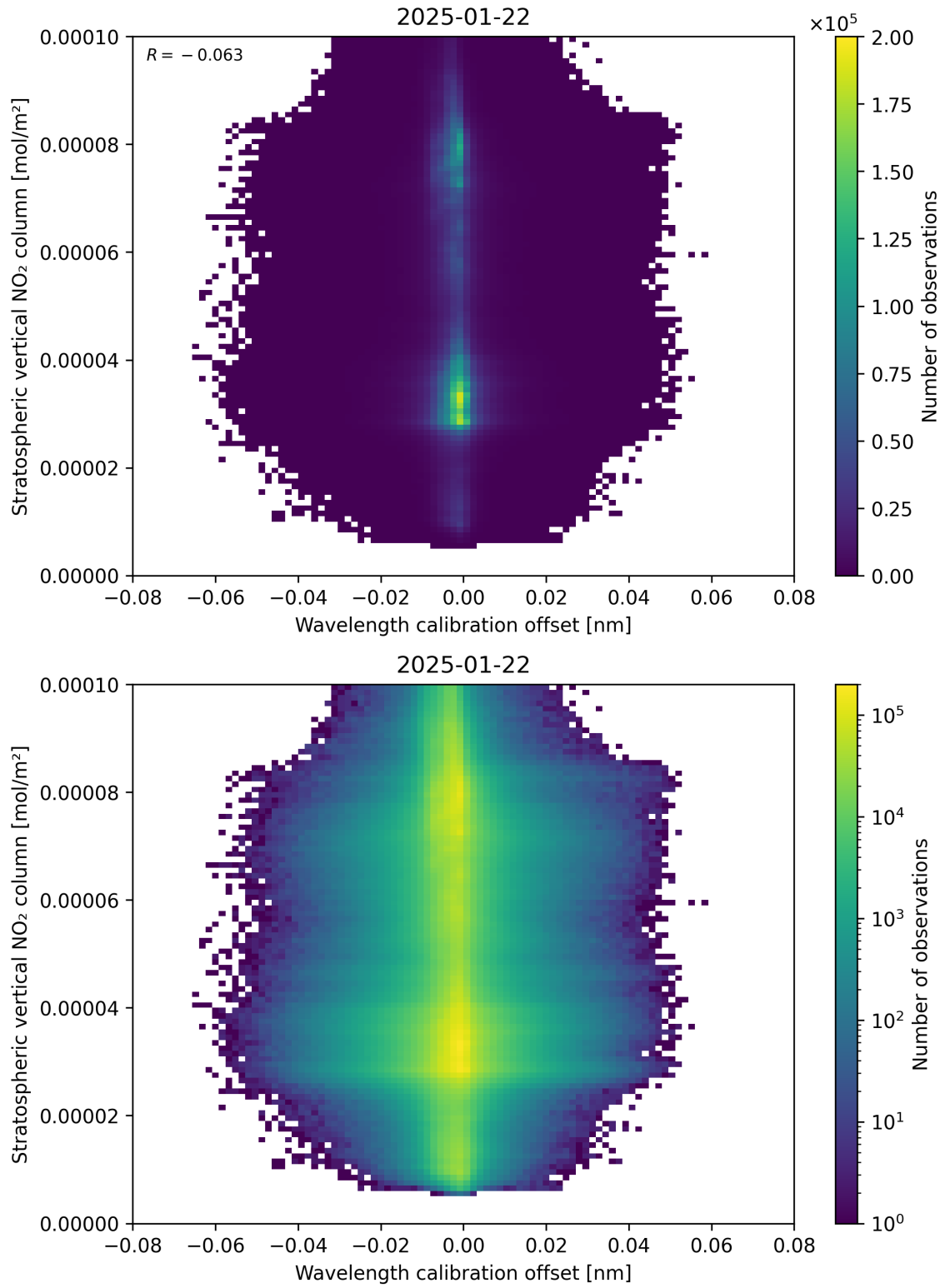
Figure 176: Scatter density plot of “Wavelength calibration offset” against “Stratospheric vertical NO 2 column” for 2025-01-21 to 2025-01-23.
