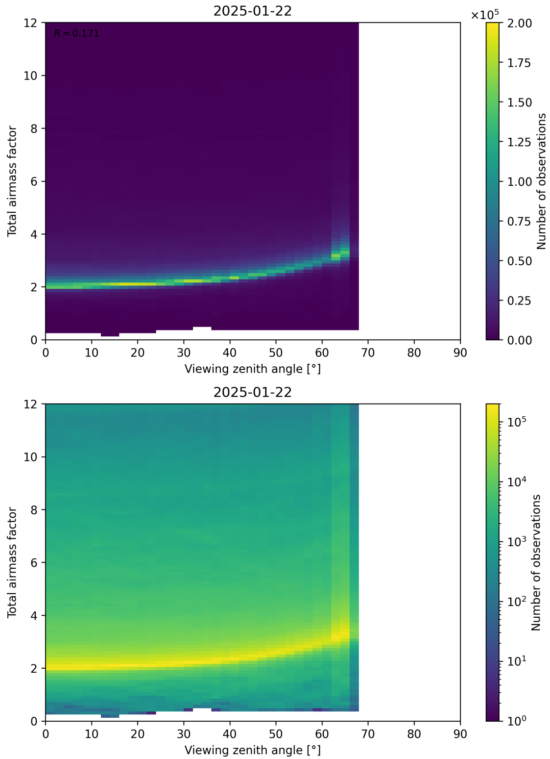
Figure 160: Scatter density plot of “Viewing zenith angle” against “Total airmass factor” for 2025-01-21 to 2025-01-23.
