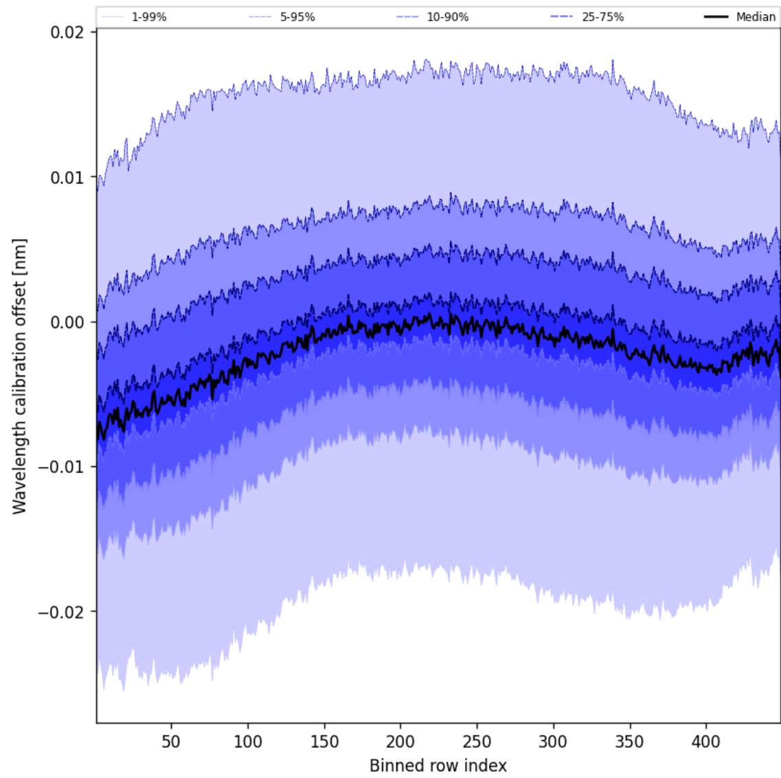
Figure 52: Along track statistics of “Wavelength calibration offset” for 2025-01-21 to 2025-01-23
