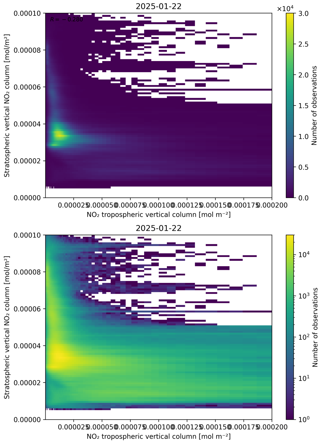
Figure 125: Scatter density plot of “NO 2 tropospheric vertical column” against “Stratospheric vertical NO 2 column” for 2025-01-21 to 2025-01-23.
