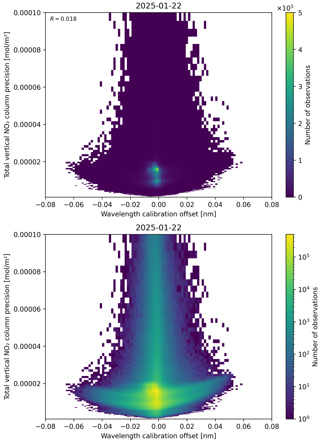
Figure 180: Scatter density plot of “Wavelength calibration offset” against “Total vertical NO 2 column precision” for 2025-01-21 to 2025-01-23.
