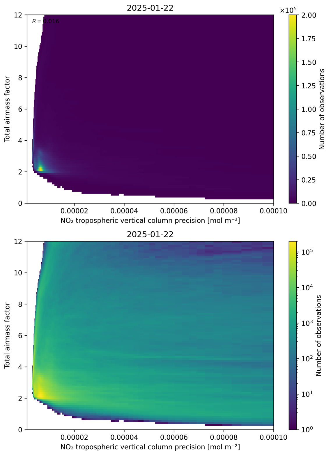
Figure 132: Scatter density plot of “NO 2 tropospheric vertical column precision” against “Total air mass factor” for 2025-01-21 to 2025-01-23.
