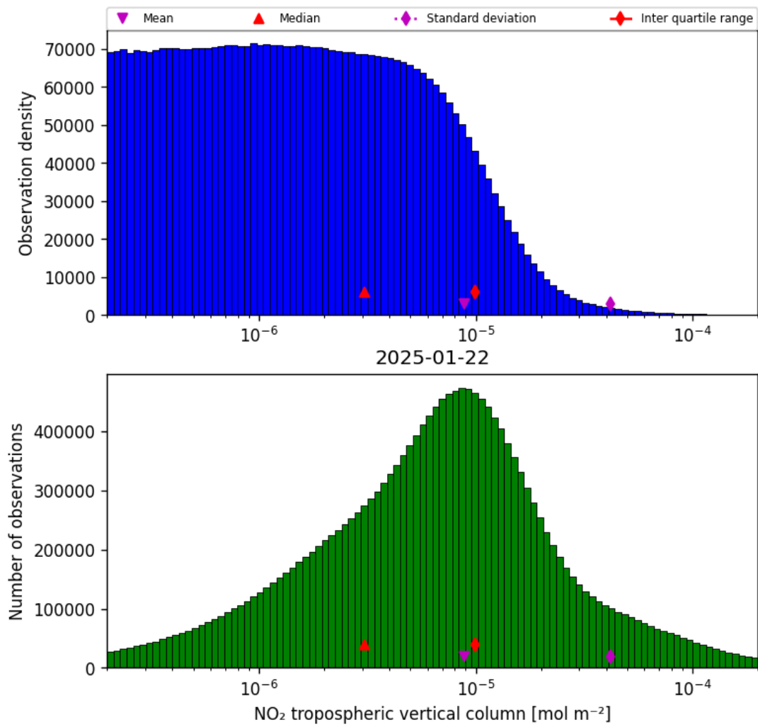
Figure 29: Histogram of “NO 2 tropospheric vertical column” for 2025-01-21 to 2025-01-23
