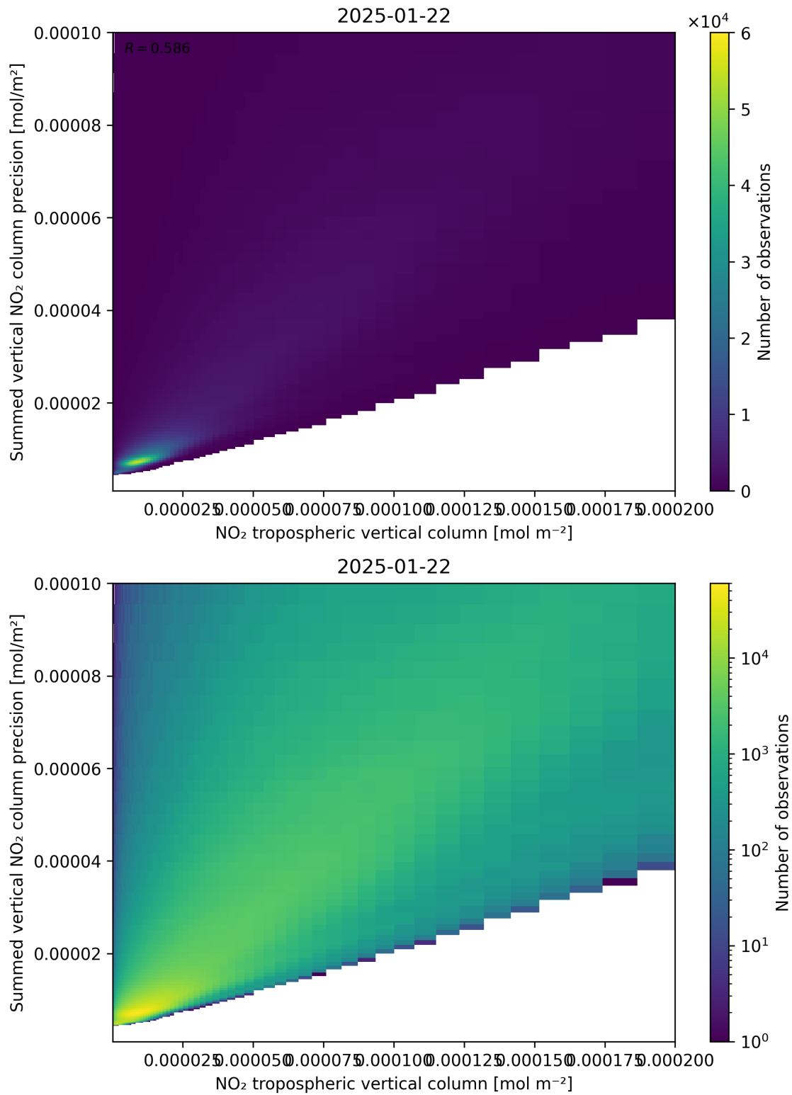
Figure 127: Scatter density plot of “NO 2 tropospheric vertical column” against “Summed vertical NO 2 column precision” for 2025-01-21 to 2025-01-23.
