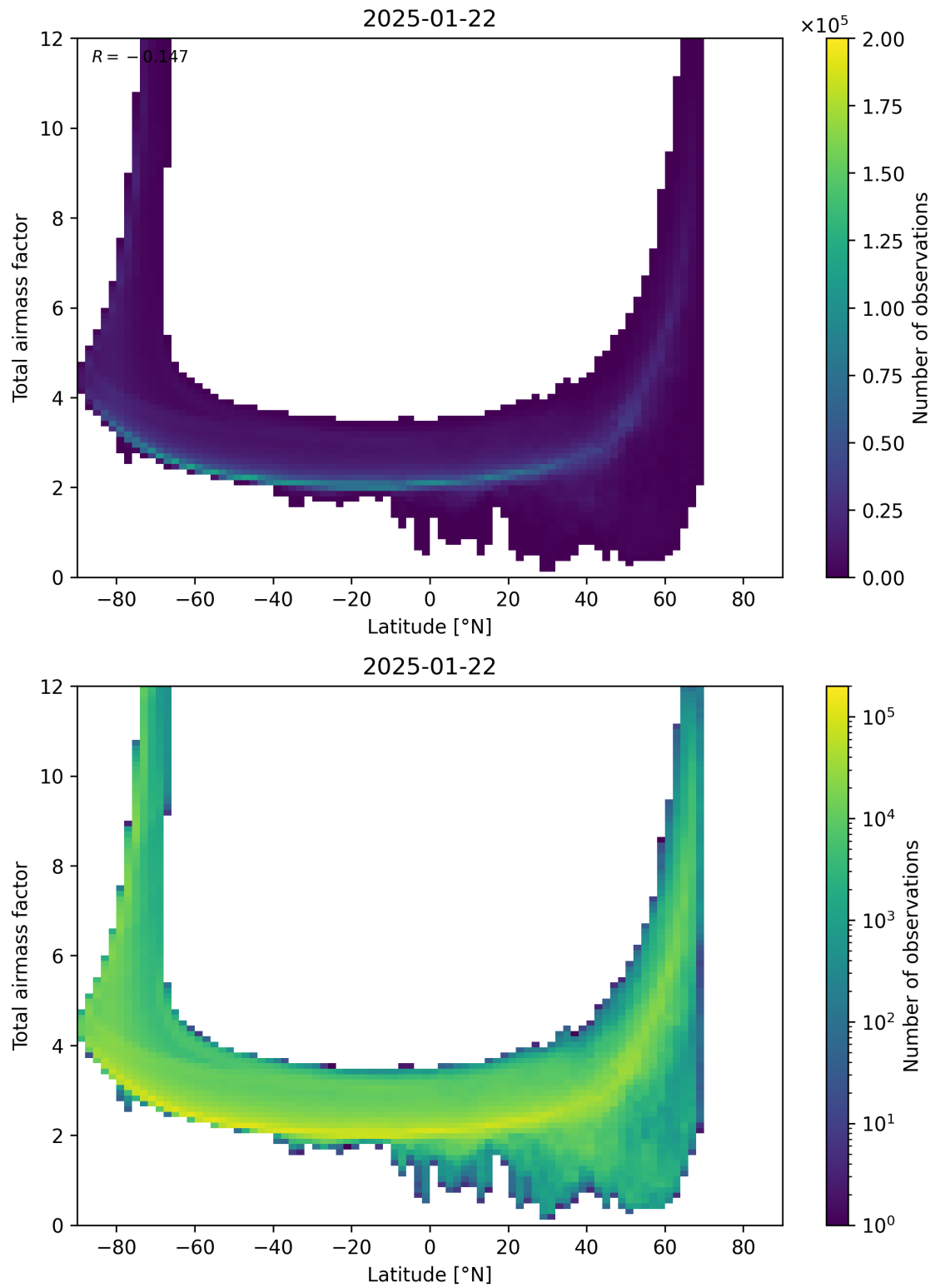
Figure 84: Scatter density plot of “Latitude” against “Total airmass factor” for 2025-01-21 to 2025-01-23.
