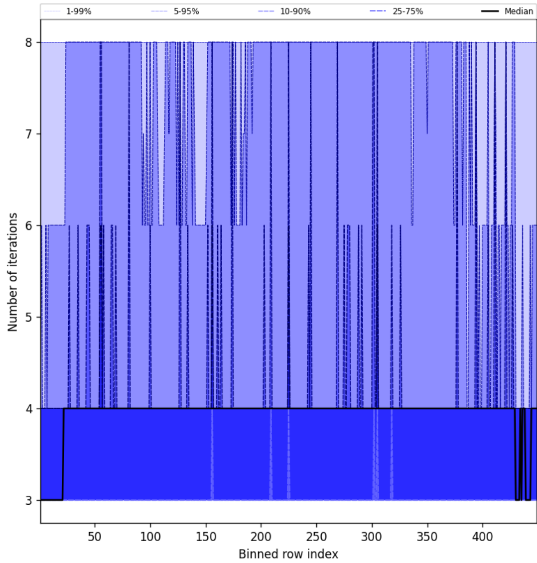
Figure 51: Along track statistics of “Number of iterations” for 2025-01-21 to 2025-01-23
