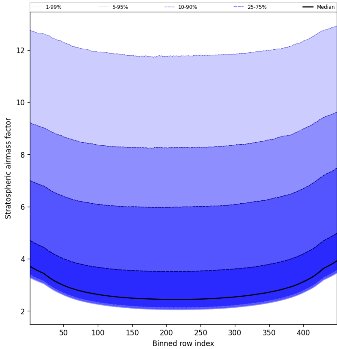
Figure 61: Along track statistics of “Stratospheric airmass factor” for 2025-01-21 to 2025-01-23
