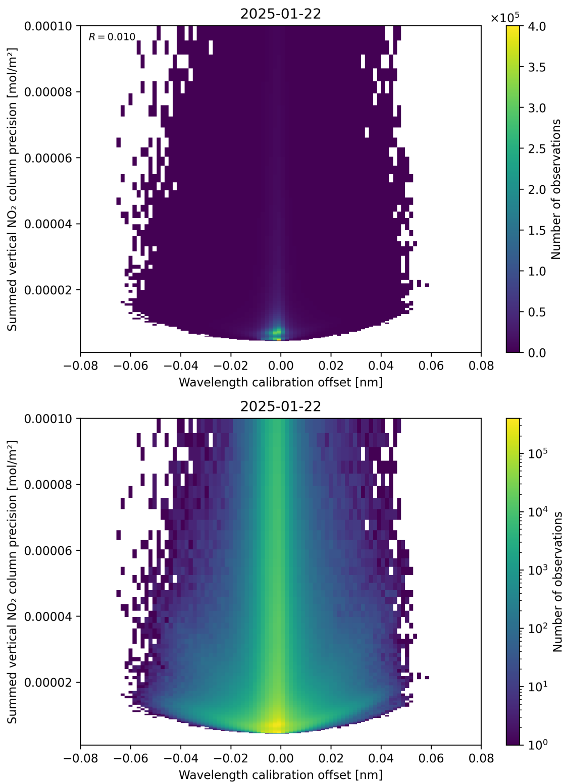
Figure 178: Scatter density plot of “Wavelength calibration offset” against “Summed vertical NO 2 column precision” for 2025-01-21 to 2025-01-23.
