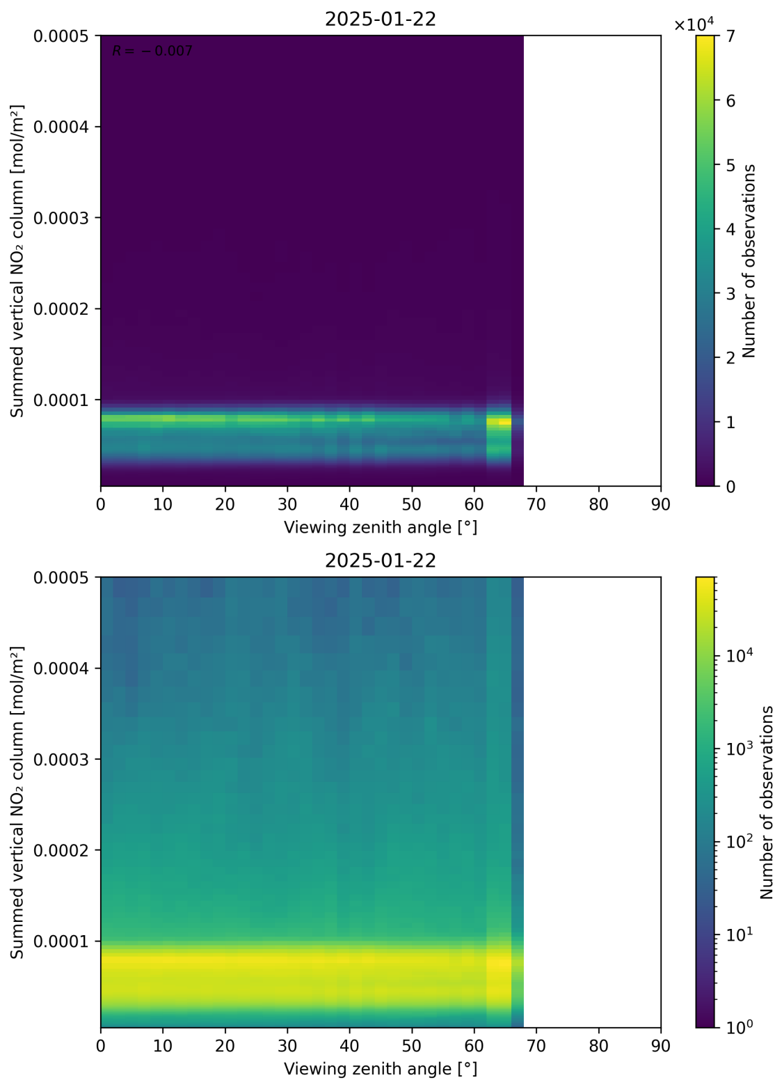
Figure 165: Scatter density plot of “Viewing zenith angle” against “Summed vertical NO 2 column” for 2025-01-21 to 2025-01-23.
