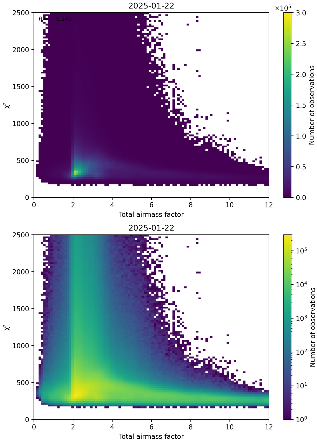
Figure 63: Scatter density plot of “Total airmass factor” against “ \chi^2 ” for 2025-01-21 to 2025-01-23.
