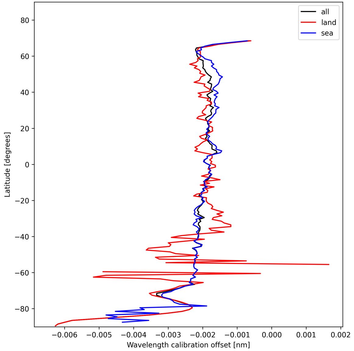
Figure 18: Zonal average of “Wavelength calibration offset” for 2025-01-21 to 2025-01-23.
