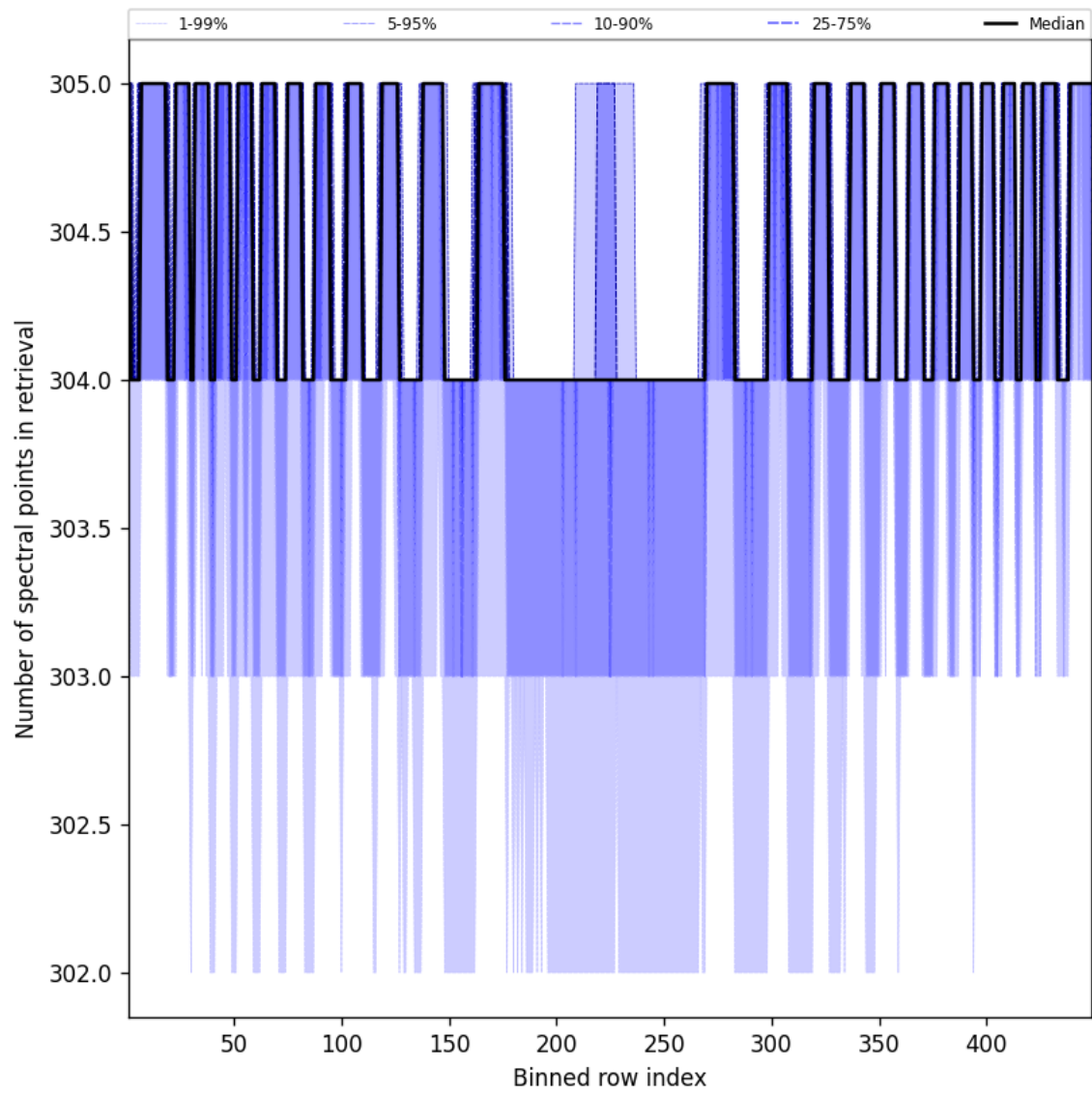
Figure 50: Along track statistics of “Number of spectral points in retrieval” for 2025-01-21 to 2025-01-23
