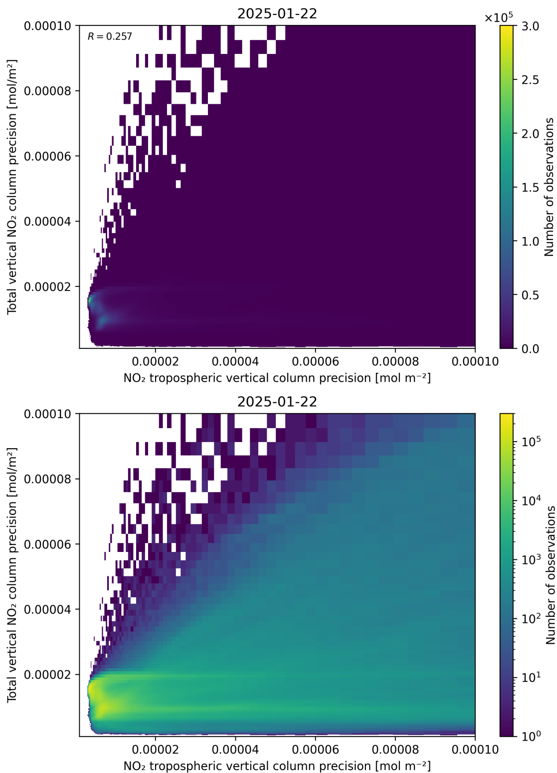
Figure 139: Scatter density plot of “NO 2 tropospheric vertical column precision” against “Total vertical NO 2 column precision” for 2025-01-21 to 2025-01-23.
