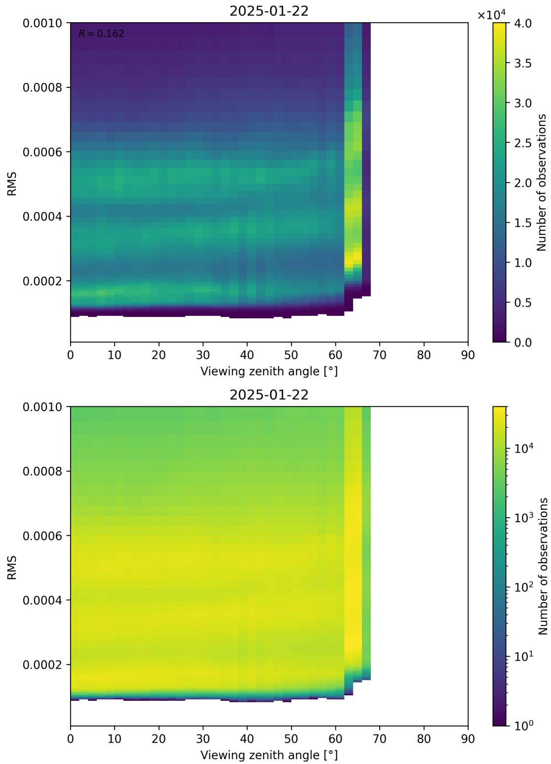
Figure 171: Scatter density plot of “Viewing zenith angle” against “RMS” for 2025-01-21 to 2025-01-23.
