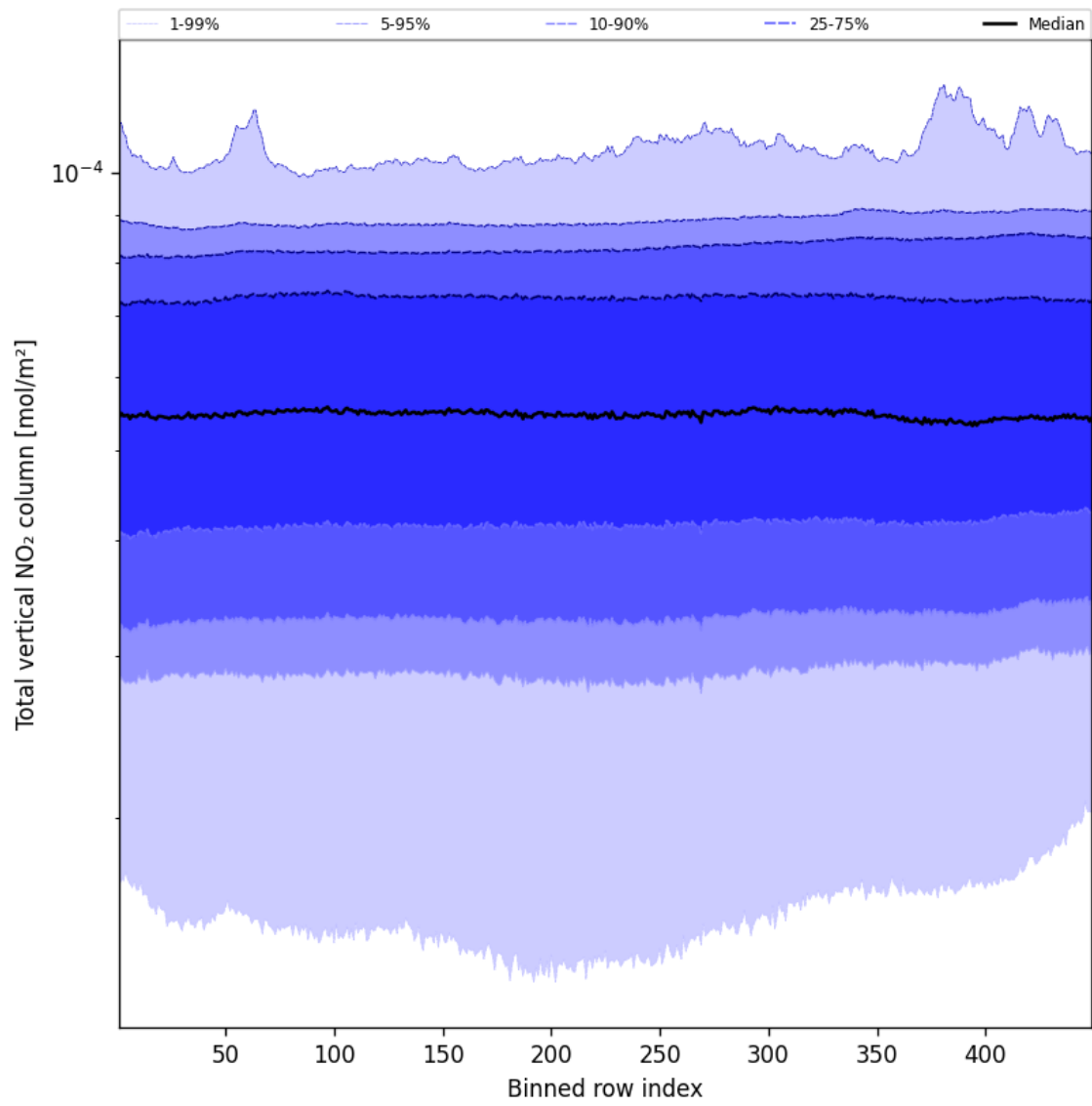
Figure 55: Along track statistics of “Total vertical NO 2 column” for 2025-01-21 to 2025-01-23
