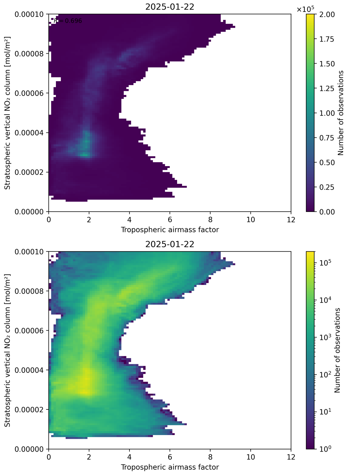
Figure 74: Scatter density plot of “Tropospheric air mass factor” against “Stratospheric vertical NO 2 column” for 2025-01-21 to 2025-01-23.
