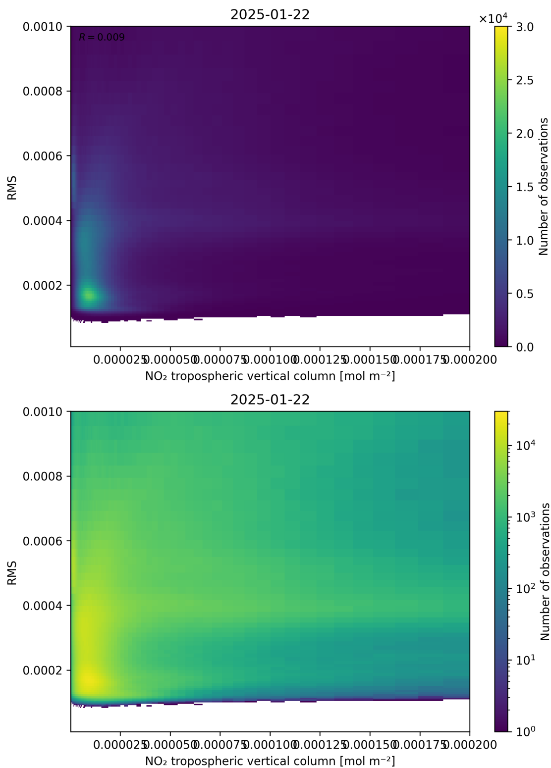
Figure 142: Scatter density plot of “NO 2 tropospheric vertical column” against “RMS” for 2025-01-21 to 2025-01-23.
