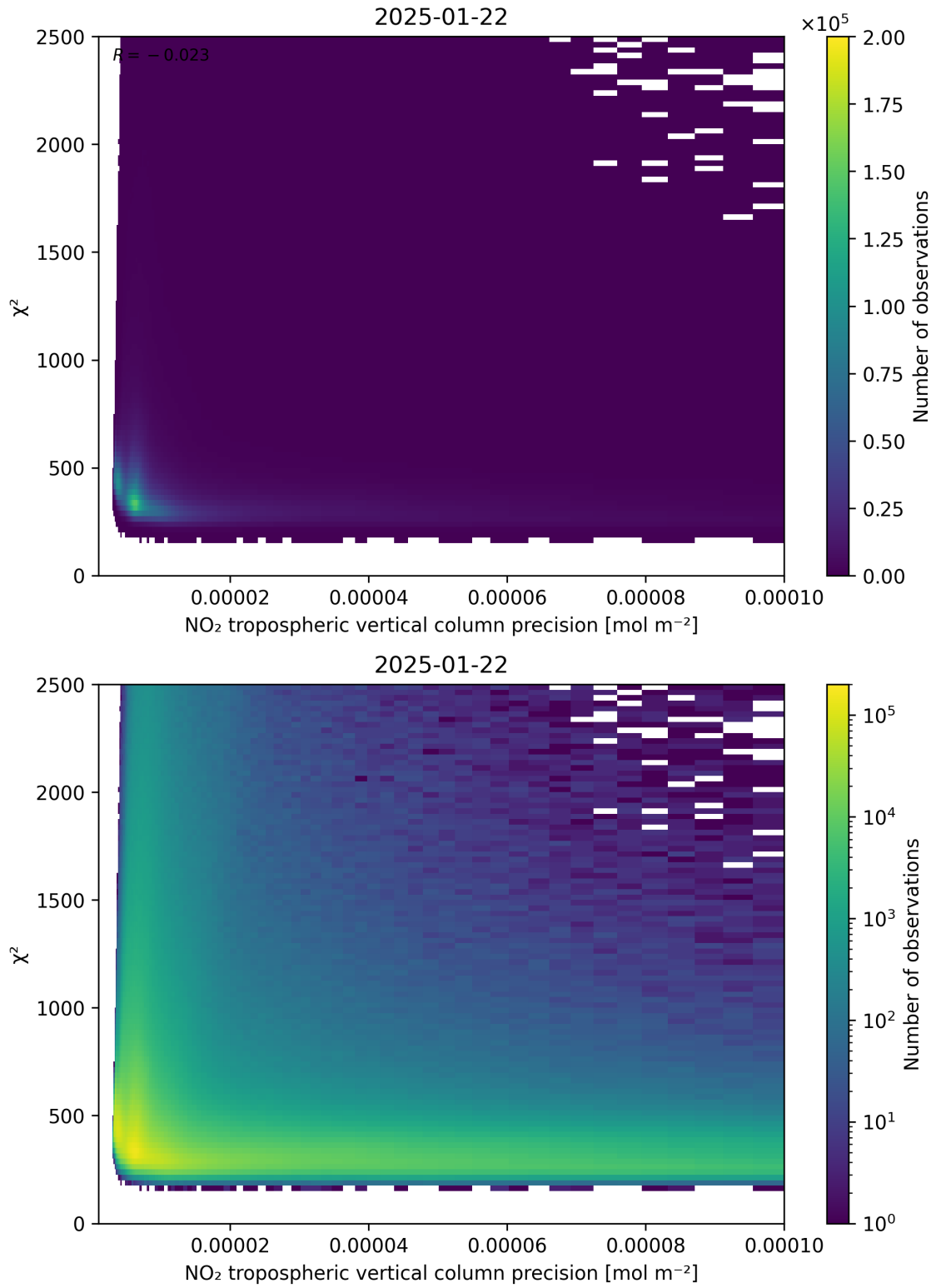
Figure 134: Scatter density plot of “NO 2 tropospheric vertical column precision” against “ \chi^2 ” for 2025-01-21 to 2025-01-23.
