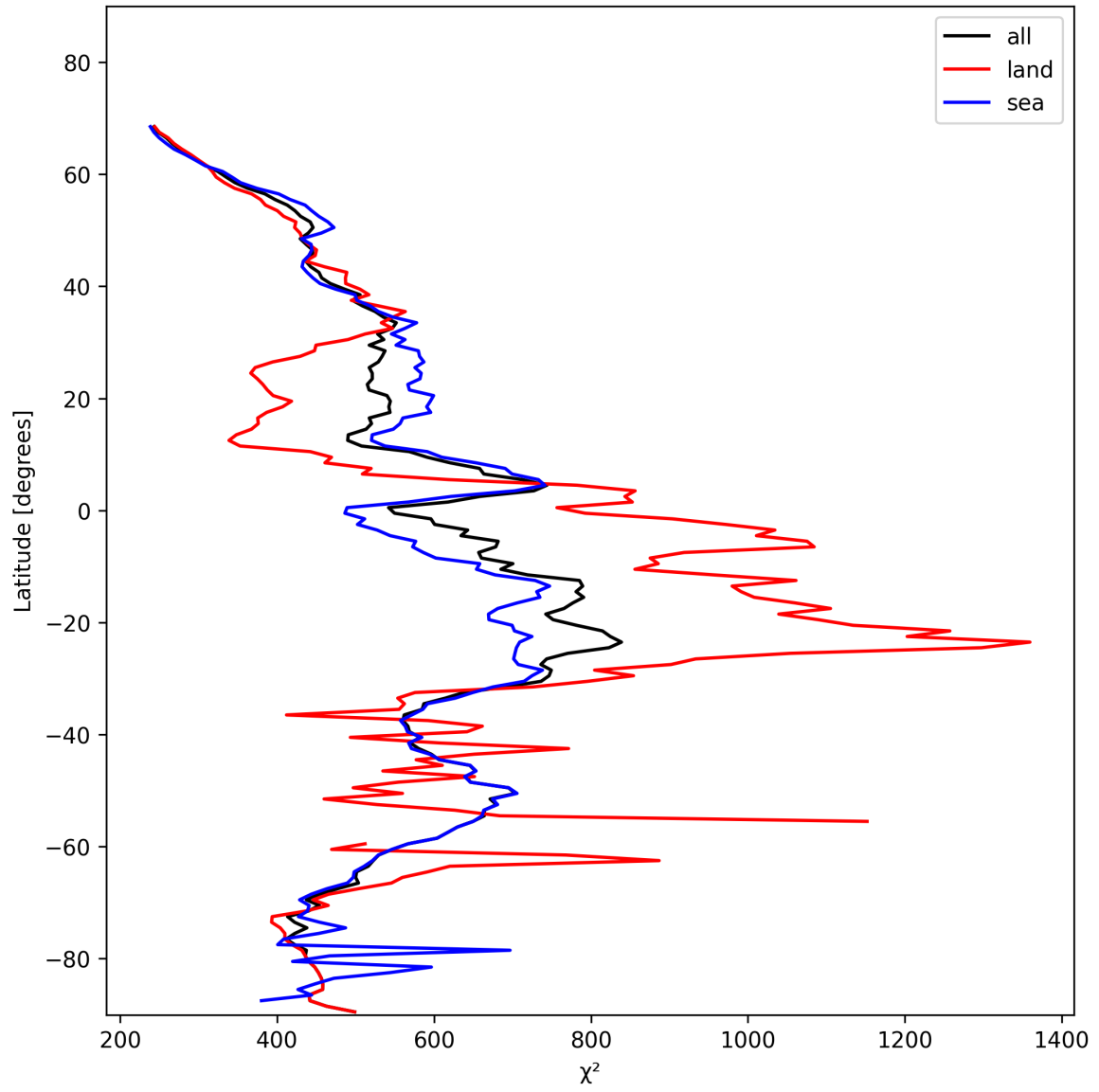
Figure 25: Zonal average of “ \chi^2 ” for 2025-01-21 to 2025-01-23.
