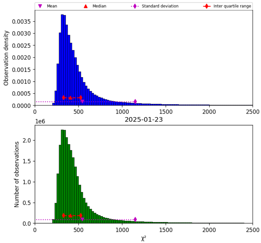
Figure 42: Histogram of “ \chi^2 ” for 2025-01-23 to 2025-01-24
