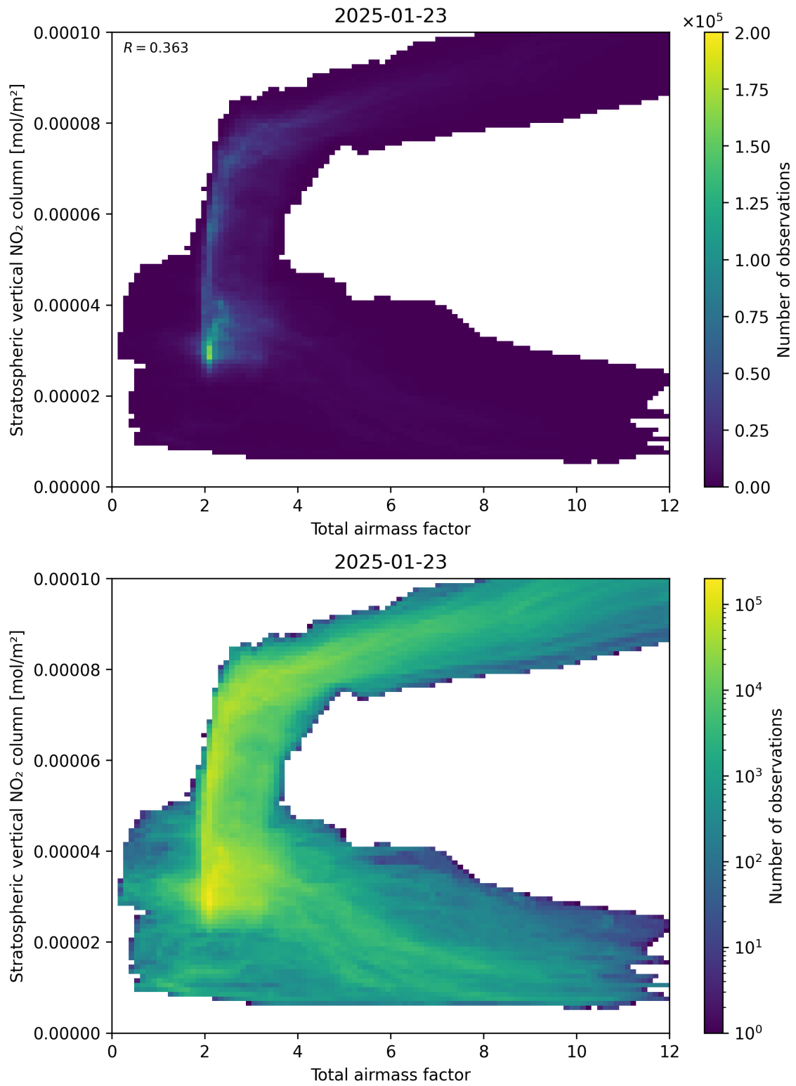
Figure 64: Scatter density plot of “Total airmass factor” against “Stratospheric vertical NO 2 column” for 2025-01-23 to 2025-01-24.
