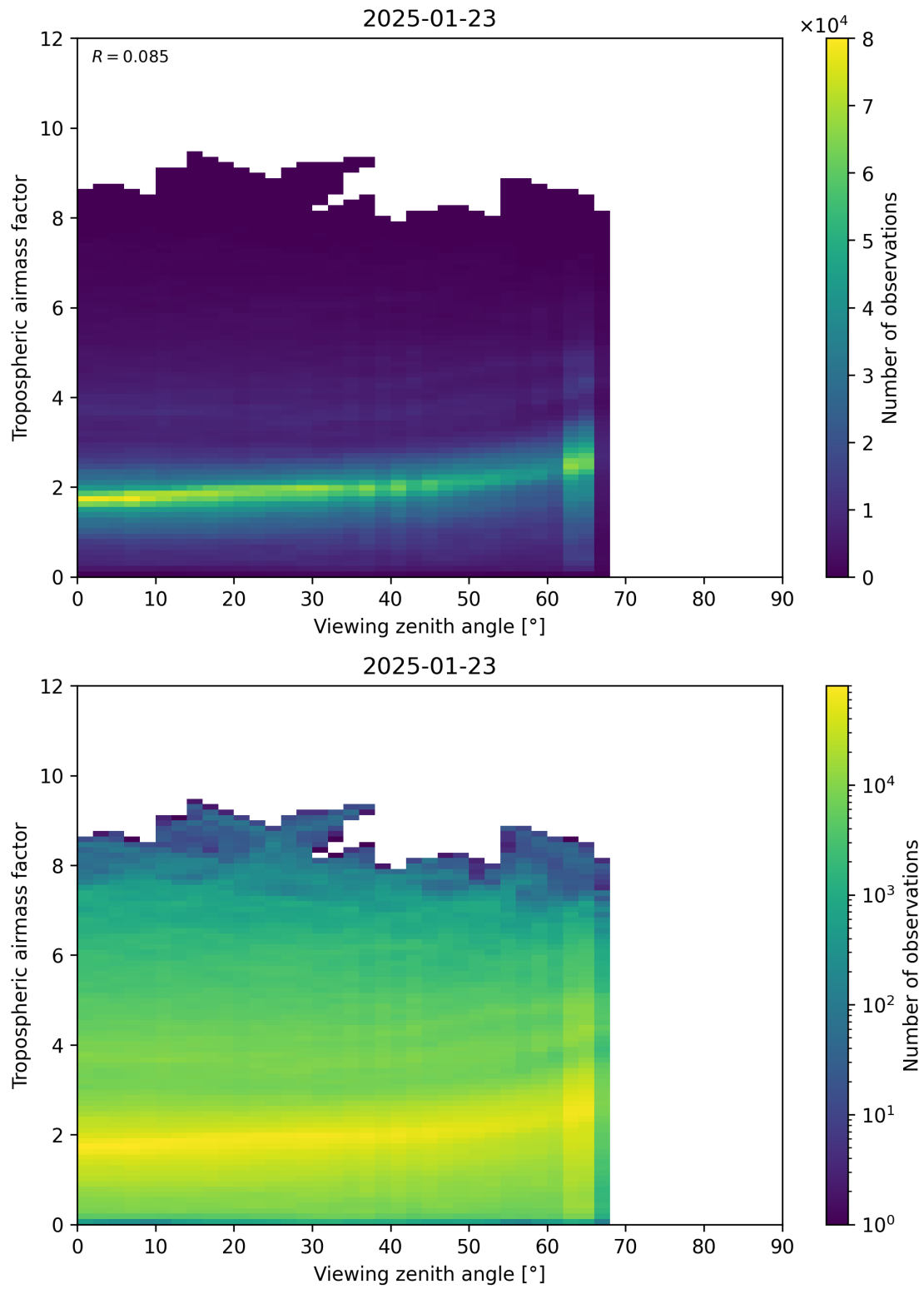
Figure 161: Scatter density plot of “Viewing zenith angle” against “Tropospheric airmass factor” for 2025-01-23 to 2025-01-24.
