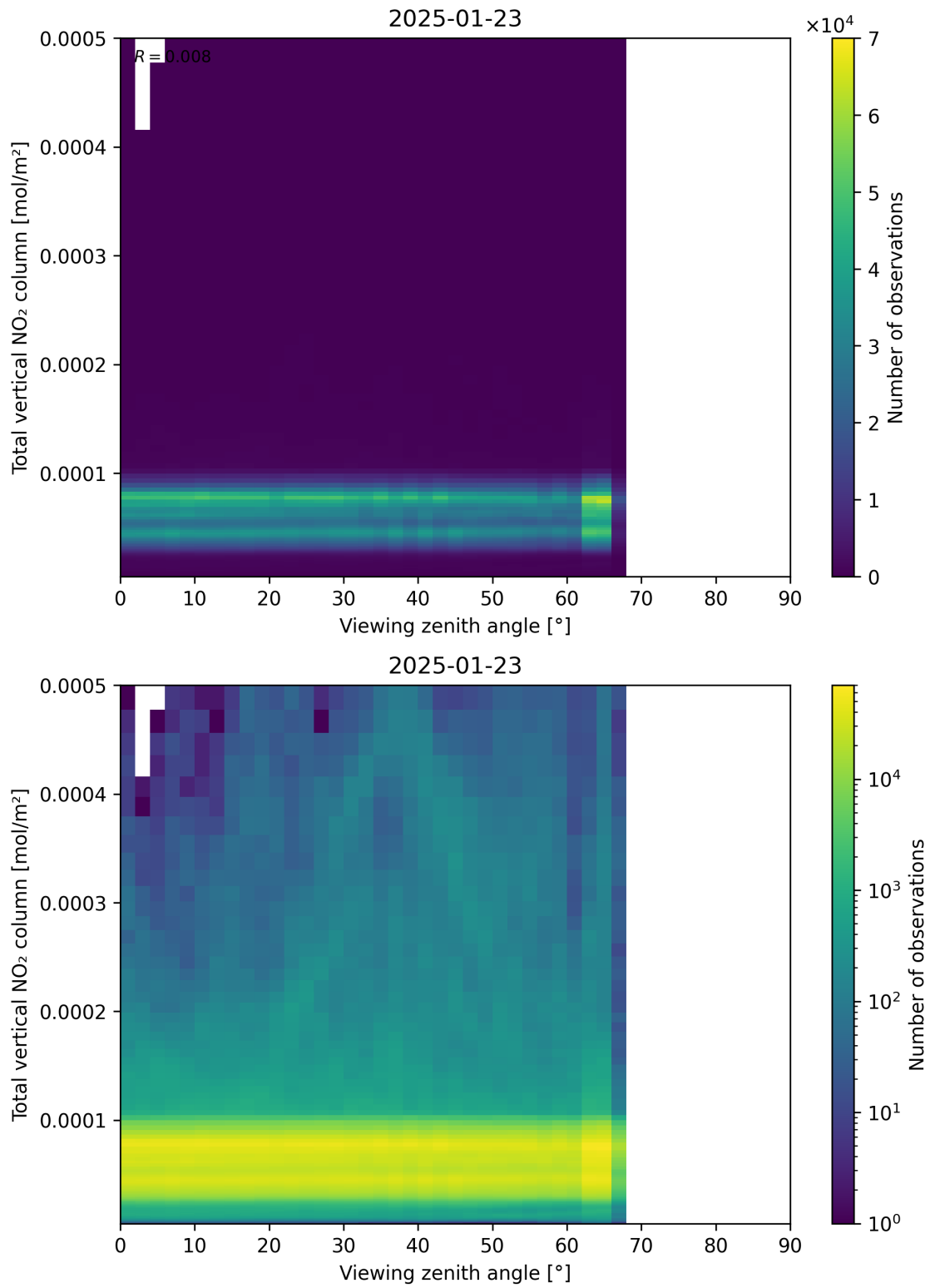
Figure 167: Scatter density plot of “Viewing zenith angle” against “Total vertical NO 2 column” for 2025-01-23 to 2025-01-24.
