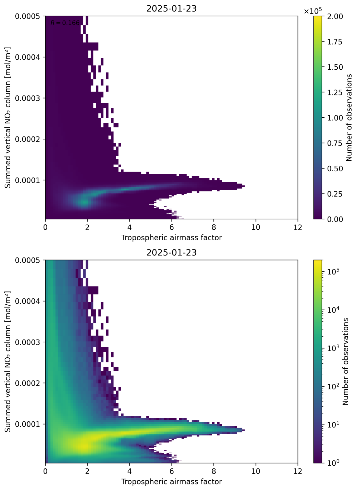
Figure 75: Scatter density plot of “Tropospheric air mass factor” against “Summed vertical NO 2 column” for 2025-01-23 to 2025-01-24.
