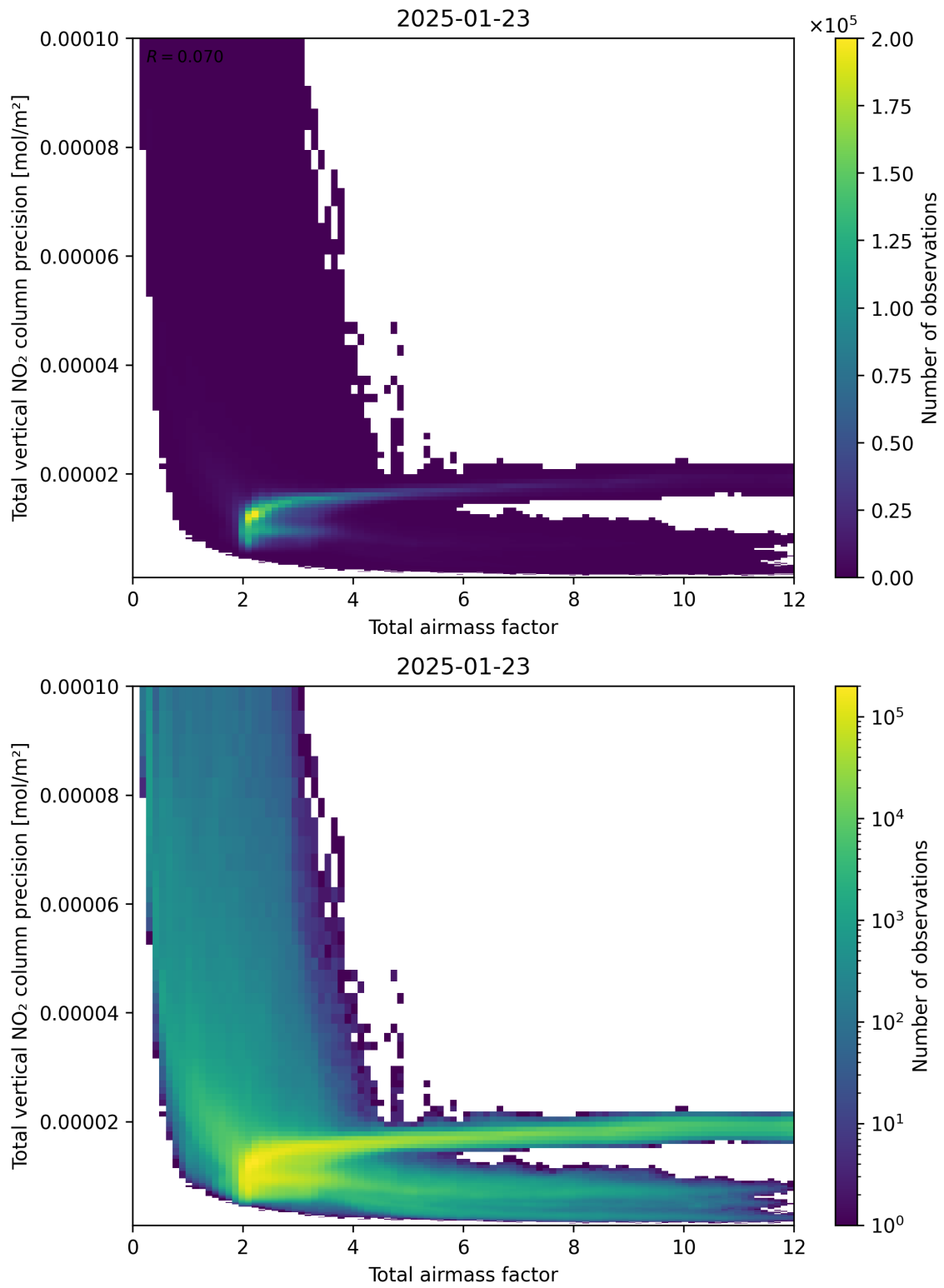
Figure 68: Scatter density plot of “Total airmass factor” against “Total vertical NO 2 column precision” for 2025-01-23 to 2025-01-24.
