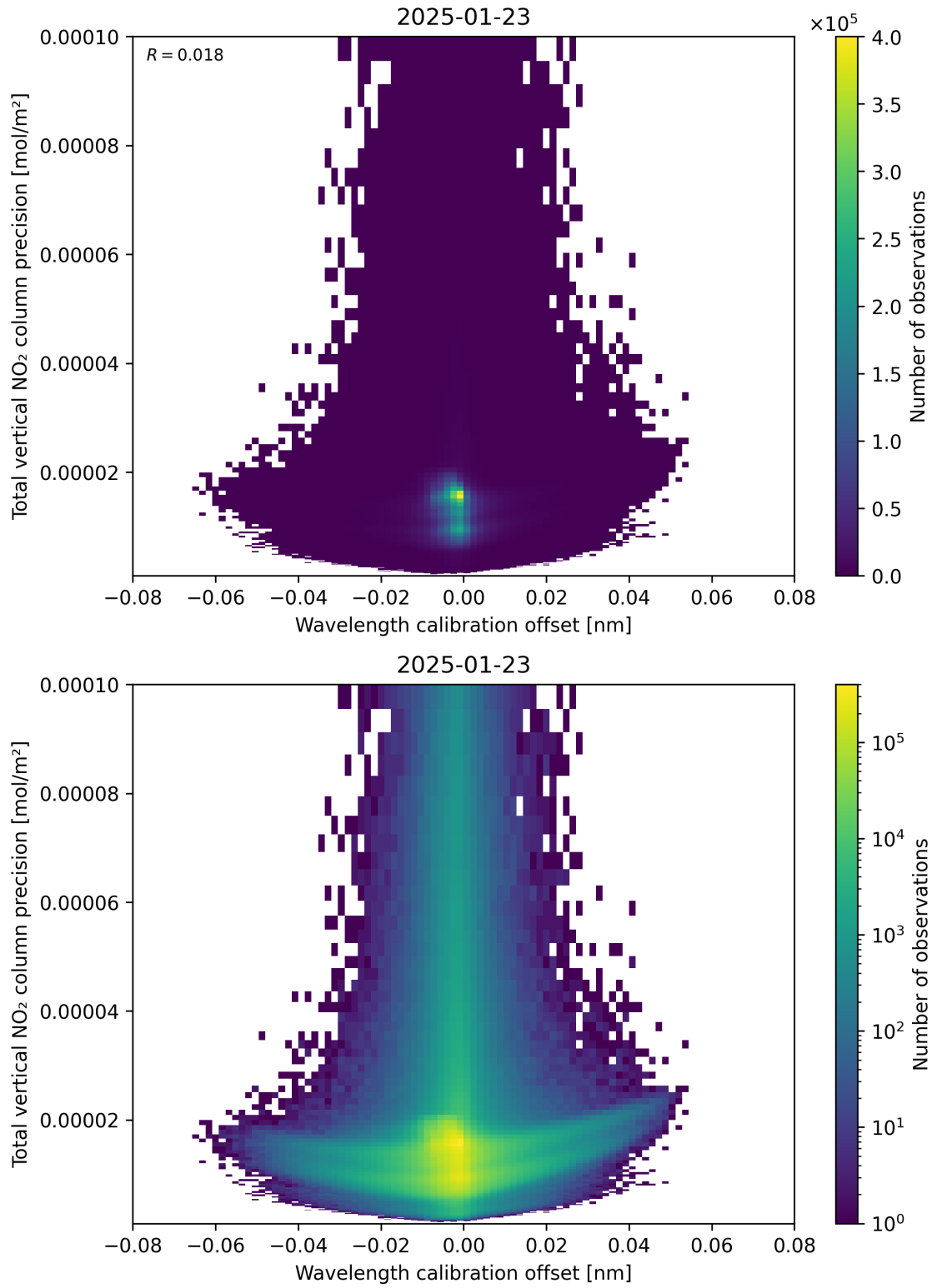
Figure 180: Scatter density plot of “Wavelength calibration offset” against “Total vertical NO 2 column precision” for 2025-01-23 to 2025-01-24.
