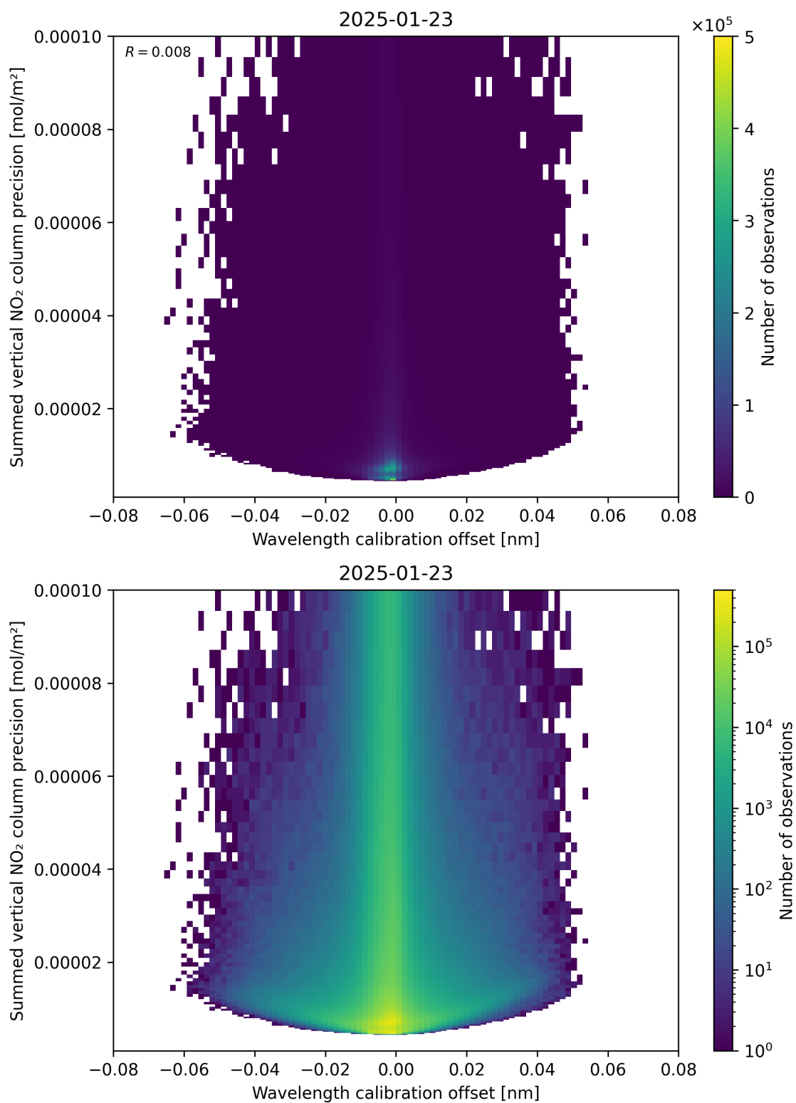
Figure 178: Scatter density plot of “Wavelength calibration offset” against “Summed vertical NO 2 column precision” for 2025-01-23 to 2025-01-24.
