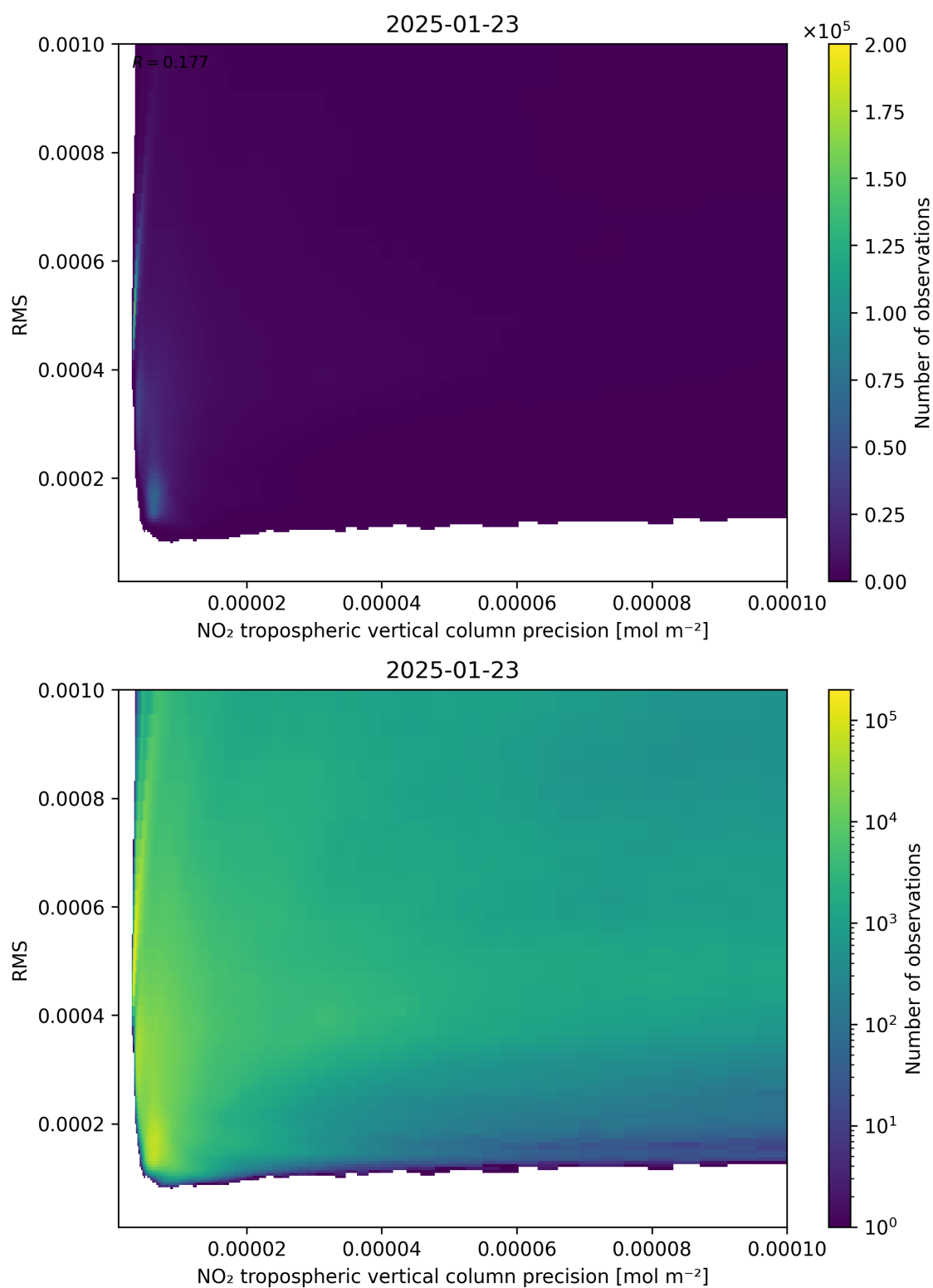
Figure 140: Scatter density plot of “NO 2 tropospheric vertical column precision” against “RMS” for 2025-01-23 to 2025-01-24.
