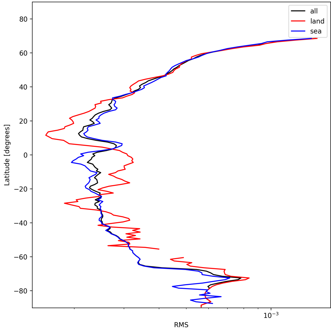
Figure 26: Zonal average of “RMS” for 2025-01-23 to 2025-01-24.
