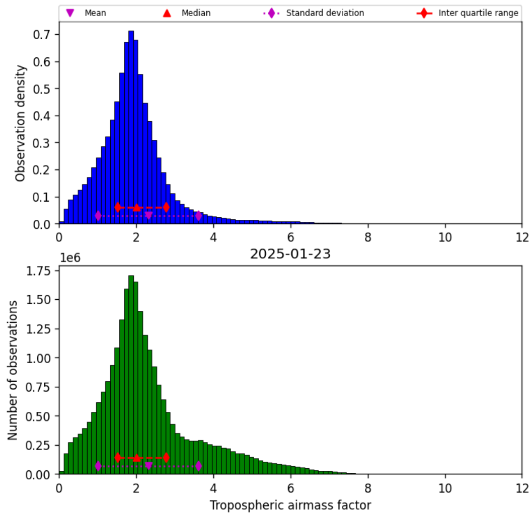
Figure 31: Histogram of “Tropospheric airmass factor” for 2025-01-23 to 2025-01-24
