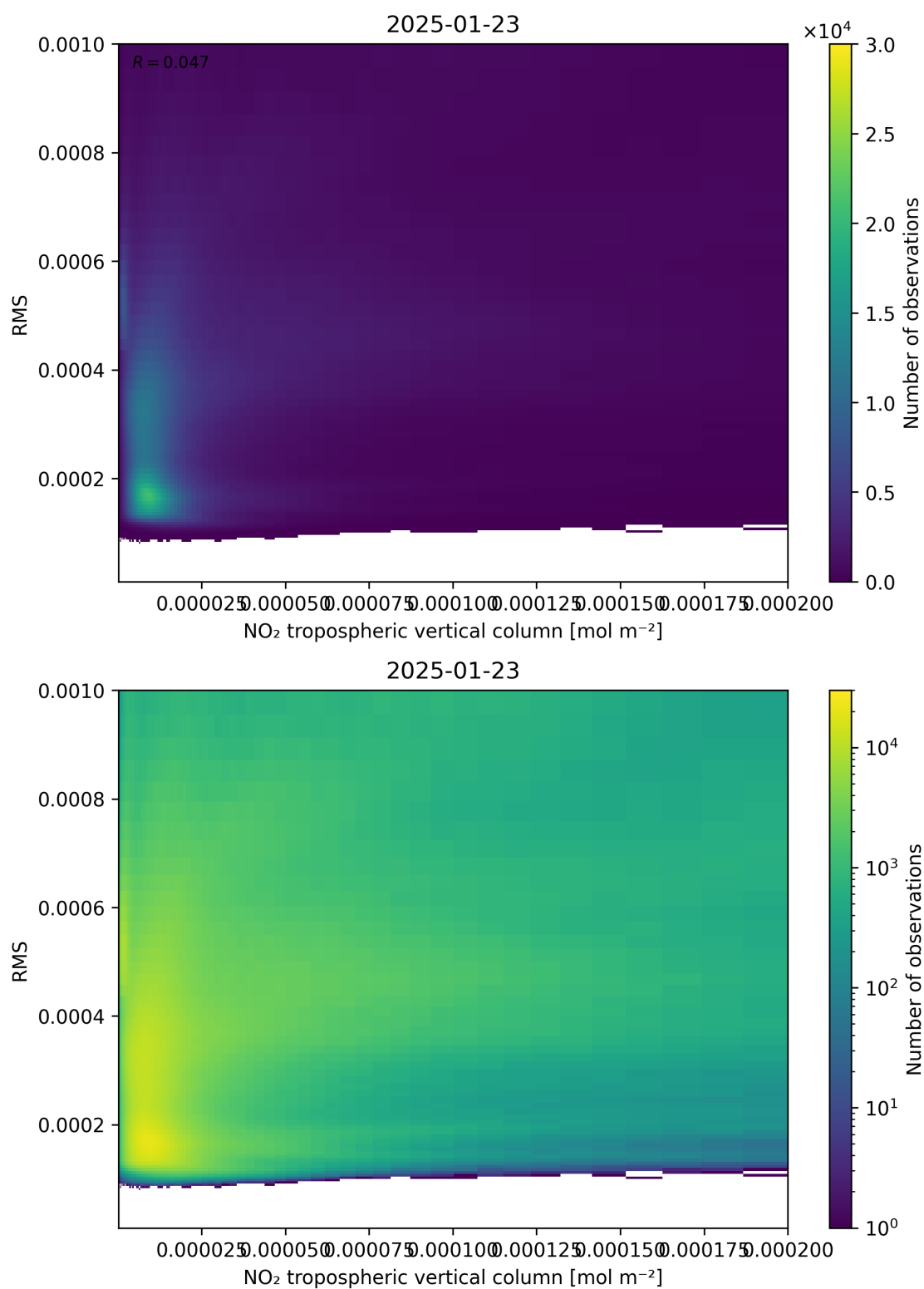
Figure 142: Scatter density plot of “NO 2 tropospheric vertical column” against “RMS” for 2025-01-23 to 2025-01-24.
