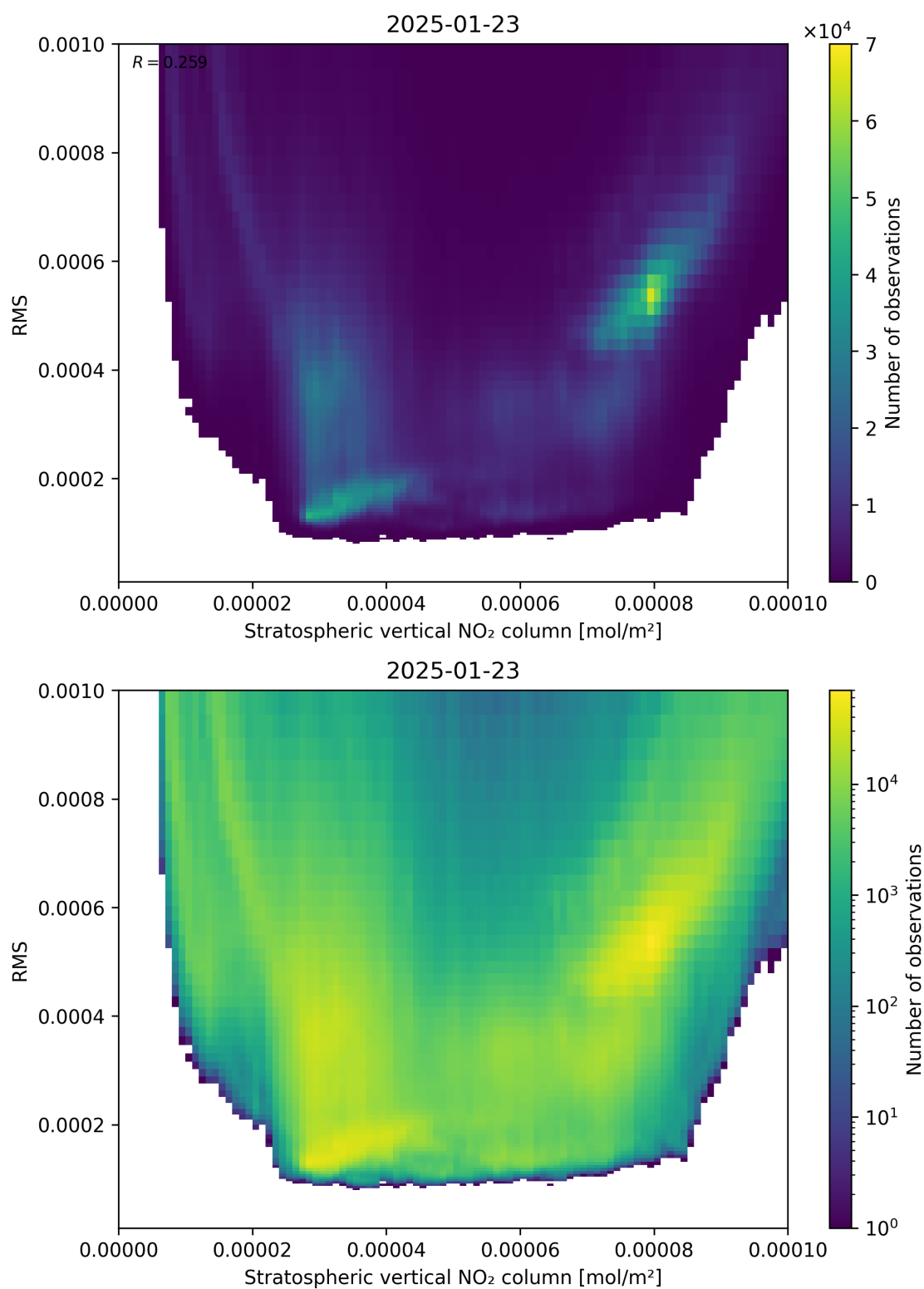
Figure 102: Scatter density plot of “Stratospheric vertical NO 2 column” against “RMS” for 2025-01-23 to 2025-01-24.
