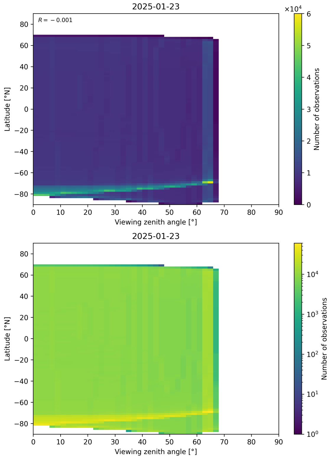
Figure 163: Scatter density plot of “Viewing zenith angle” against “Latitude” for 2025-01-23 to 2025-01-24.
