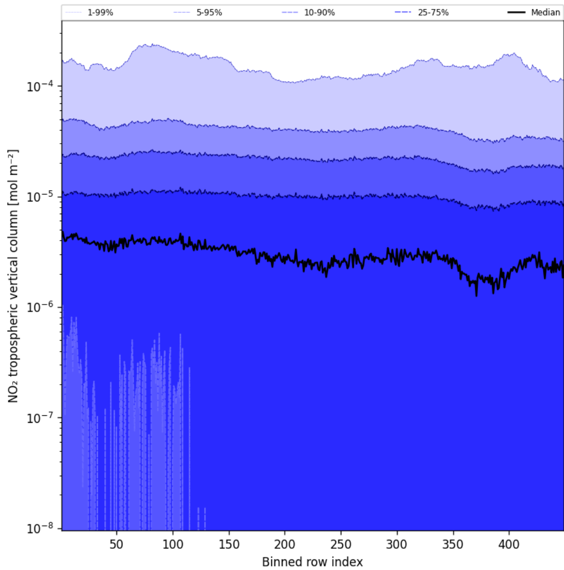
Figure 46: Along track statistics of “NO 2 tropospheric vertical column” for 2025-01-23 to 2025-01-24
