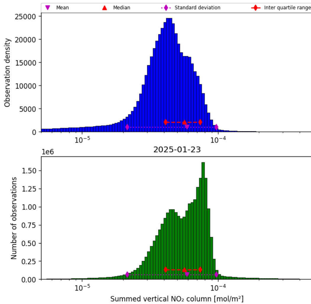
Figure 40: Histogram of “Summed vertical NO 2 column” for 2025-01-23 to 2025-01-24
