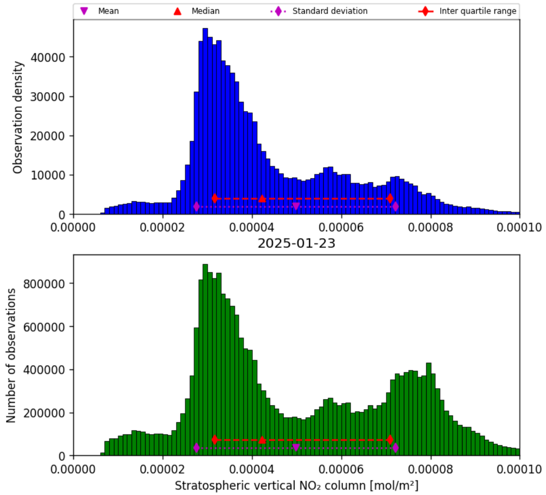
Figure 36: Histogram of “Stratospheric vertical NO 2 column” for 2025-01-23 to 2025-01-24
