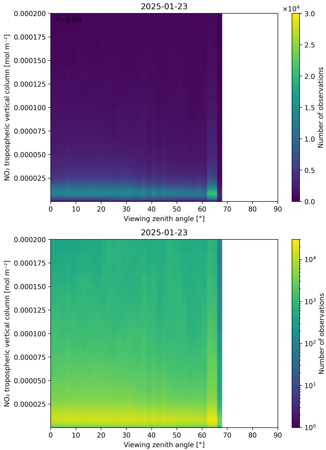
Figure 169: Scatter density plot of “Viewing zenith angle” against “NO 2 tropospheric vertical column” for 2025-01-23 to 2025-01-24.
