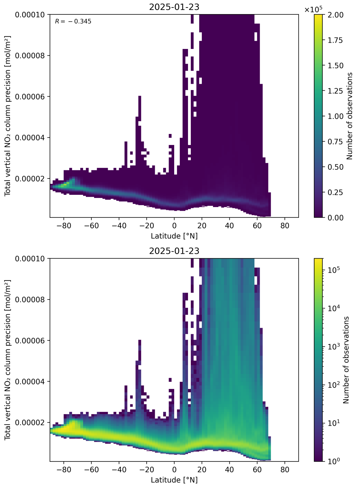
Figure 91: Scatter density plot of “Latitude” against “Total vertical NO 2 column precision” for 2025-01-23 to 2025-01-24.
