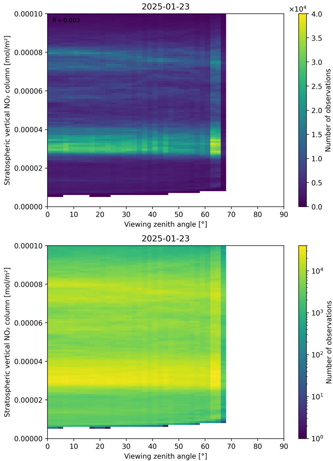
Figure 164: Scatter density plot of “Viewing zenith angle” against “Stratospheric vertical NO 2 column” for 2025-01-23 to 2025-01-24.
