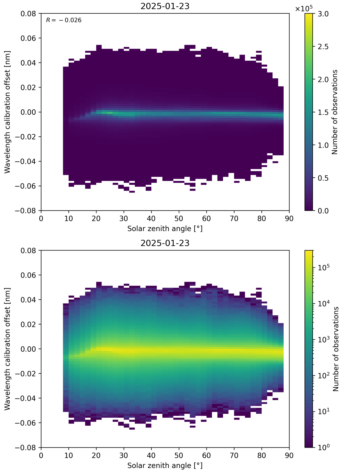
Figure 158: Scatter density plot of “Solar zenith angle” against “Wavelength calibration offset” for 2025-01-23 to 2025-01-24.
