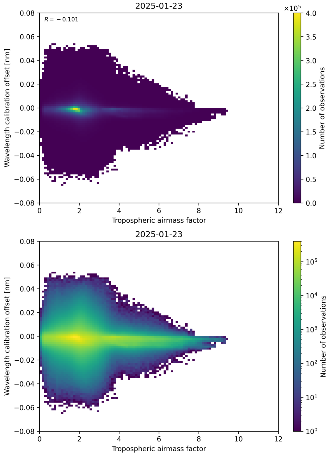
Figure 80: Scatter density plot of “Tropospheric airmass factor” against “Wavelength calibration offset” for 2025-01-23 to 2025-01-24.
