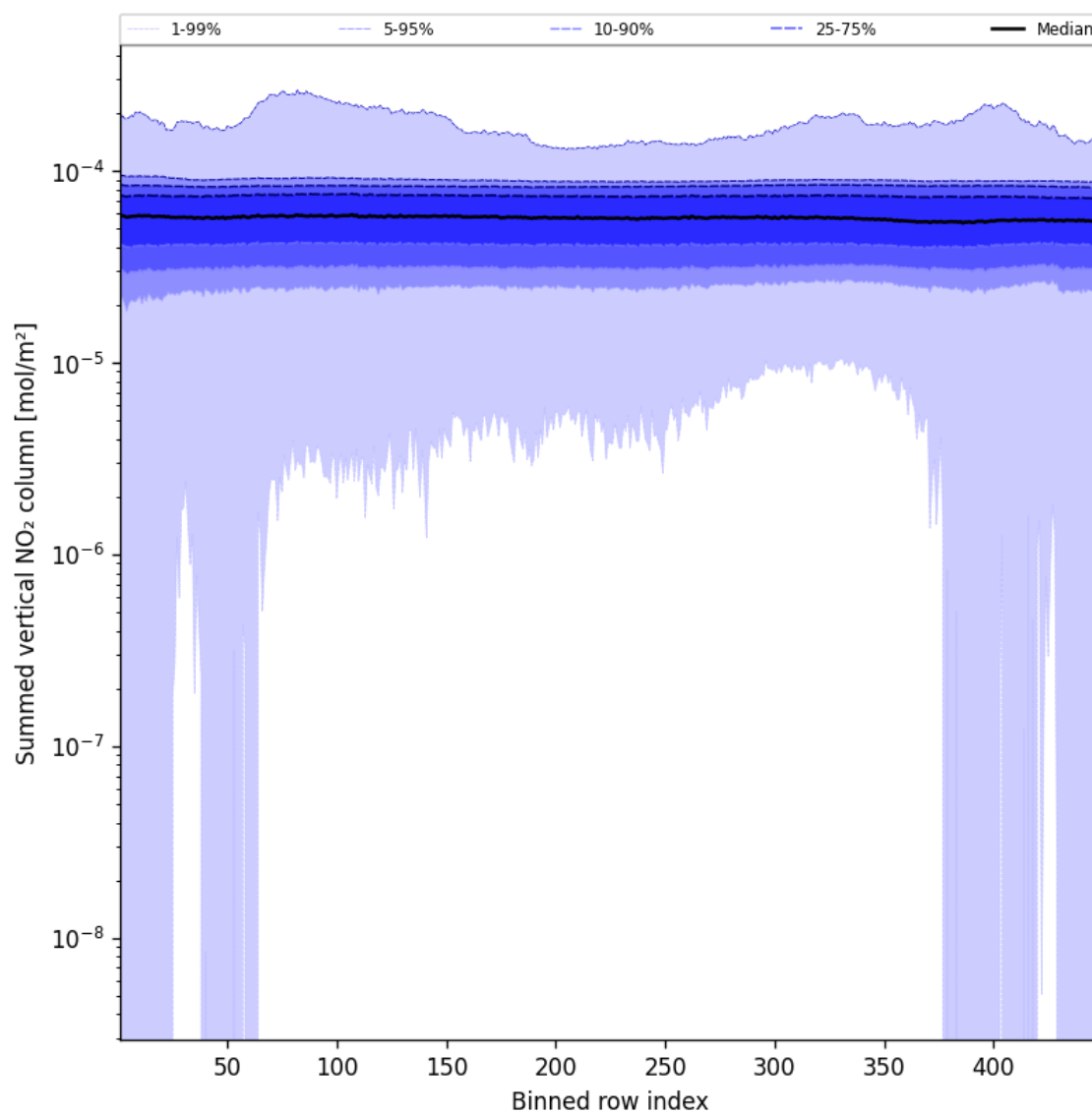
Figure 57: Along track statistics of “Summed vertical NO 2 column” for 2025-01-23 to 2025-01-24
