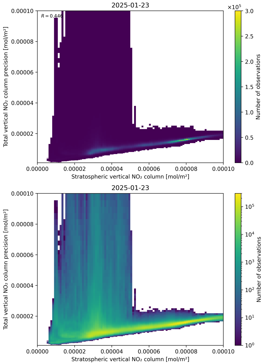
Figure 101: Scatter density plot of “Stratospheric vertical NO 2 column” against “Total vertical NO 2 column precision” for 2025-01-23 to 2025-01-24.
