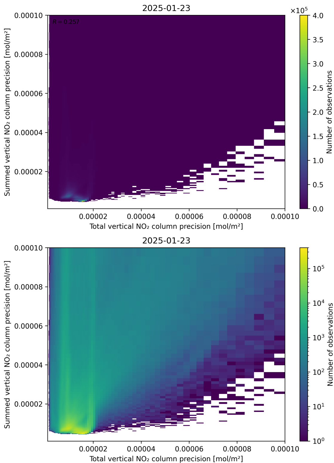
Figure 118: Scatter density plot of “Total vertical NO 2 column precision” against “Summed vertical NO 2 column precision” for 2025-01-23 to 2025-01-24.
