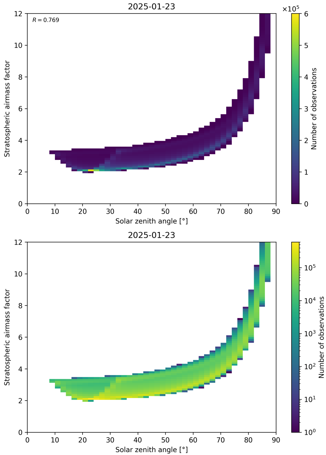
Figure 145: Scatter density plot of “Solar zenith angle” against “Stratospheric airmass factor” for 2025-01-23 to 2025-01-24.
