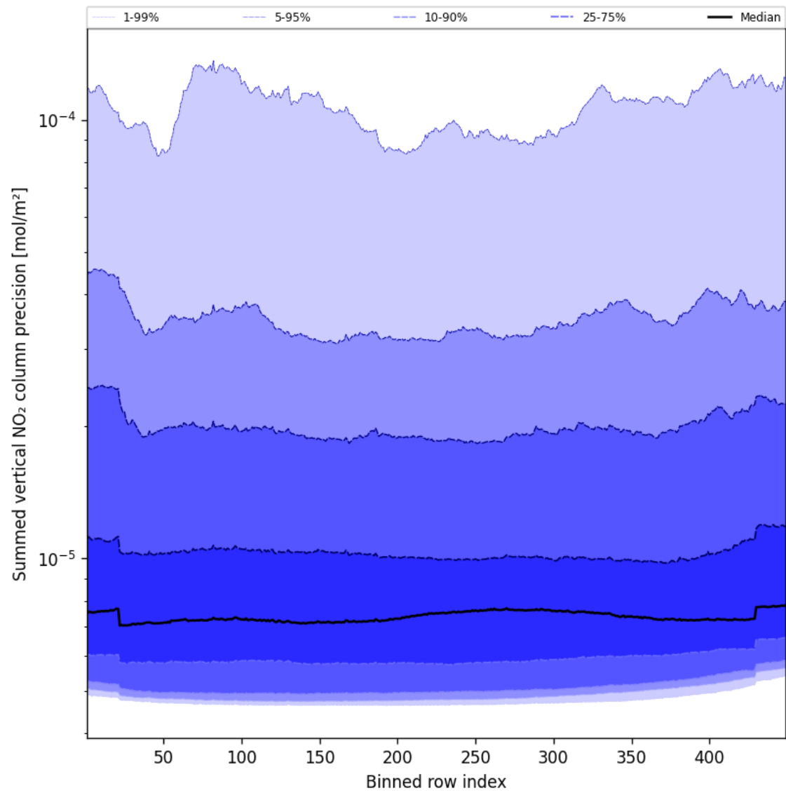
Figure 58: Along track statistics of “Summed vertical NO 2 column precision” for 2025-01-23 to 2025-01-24
