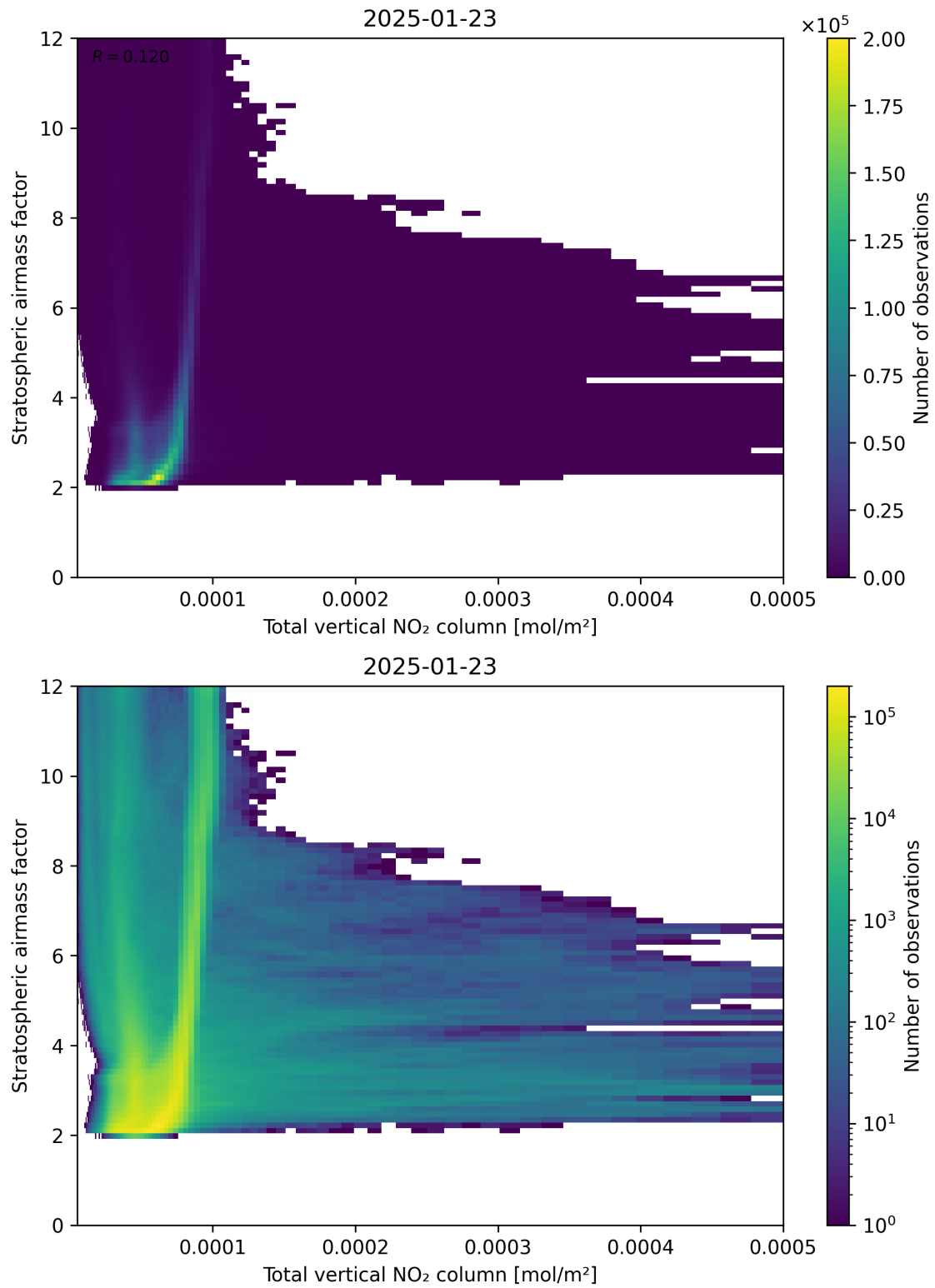
Figure 110: Scatter density plot of “Total vertical NO 2 column” against “Stratospheric airmass factor” for 2025-01-23 to 2025-01-24.
