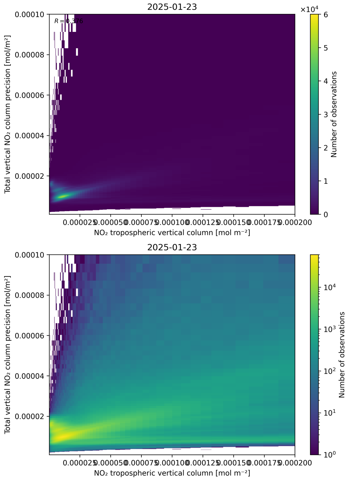
Figure 129: Scatter density plot of “NO 2 tropospheric vertical column” against “Total vertical NO 2 column precision” for 2025-01-23 to 2025-01-24.
