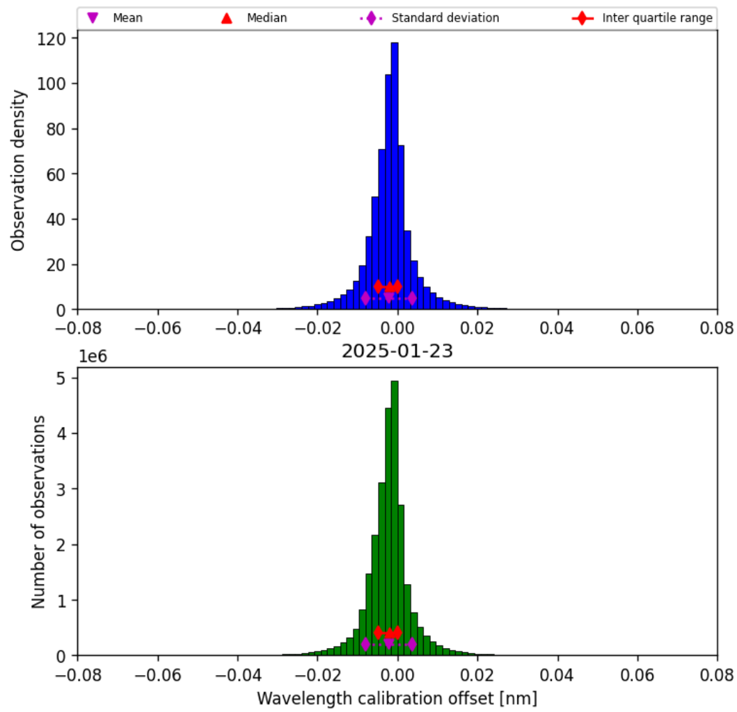
Figure 35: Histogram of “Wavelength calibration offset” for 2025-01-23 to 2025-01-24
