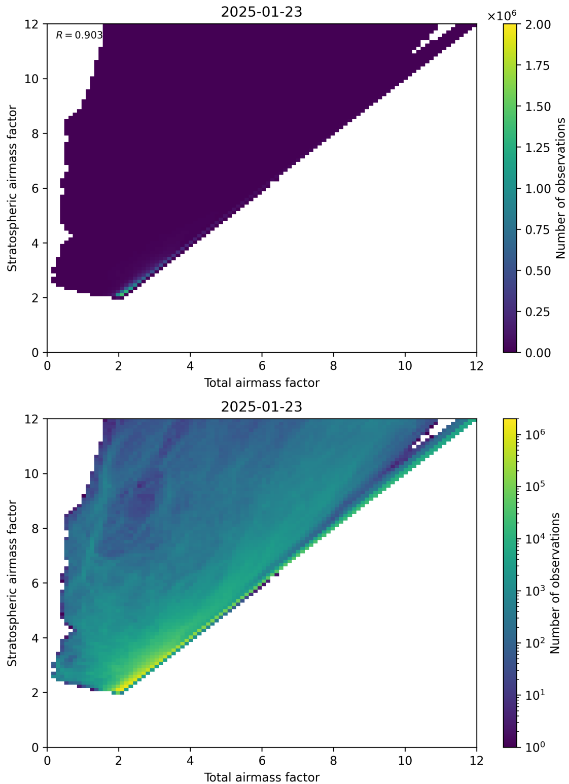
Figure 62: Scatter density plot of “Total air mass factor” against “Stratospheric air mass factor” for 2025-01-23 to 2025-01-24.
