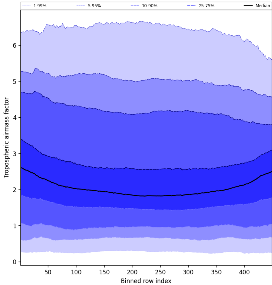
Figure 48: Along track statistics of “Tropospheric airmass factor” for 2025-01-23 to 2025-01-24
