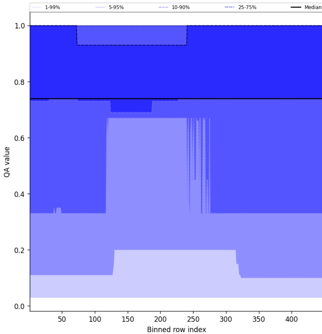
Figure 45: Along track statistics of “QA value” for 2025-01-23 to 2025-01-24
