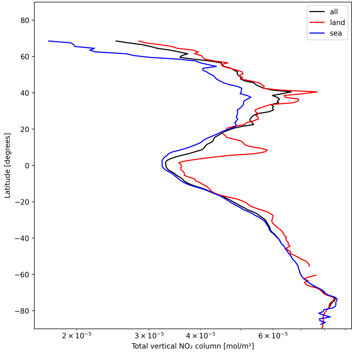
Figure 21: Zonal average of “Total vertical NO 2 column” for 2025-01-23 to 2025-01-24.
