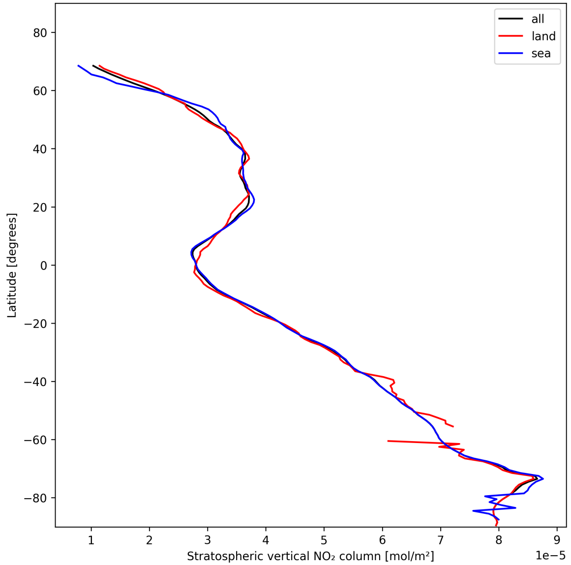
Figure 19: Zonal average of “Stratospheric vertical NO 2 column” for 2025-01-23 to 2025-01-24.
