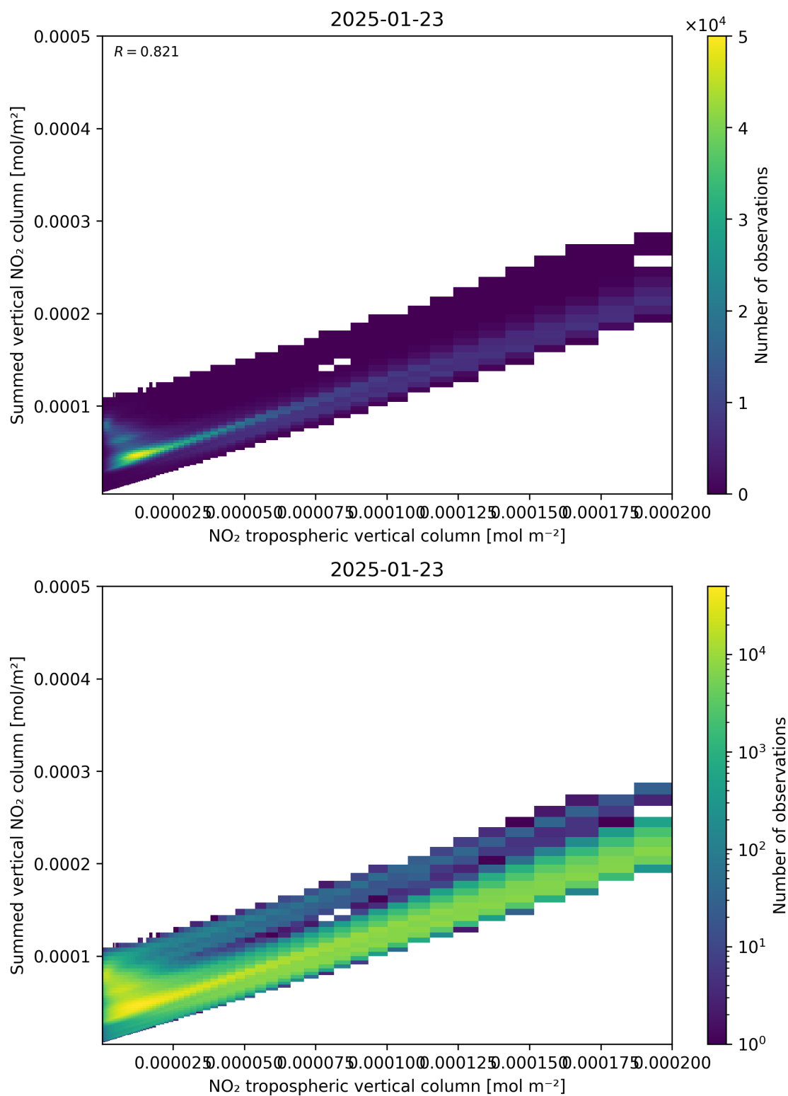
Figure 126: Scatter density plot of “NO 2 tropospheric vertical column” against “Summed vertical NO 2 column” for 2025-01-23 to 2025-01-24.
