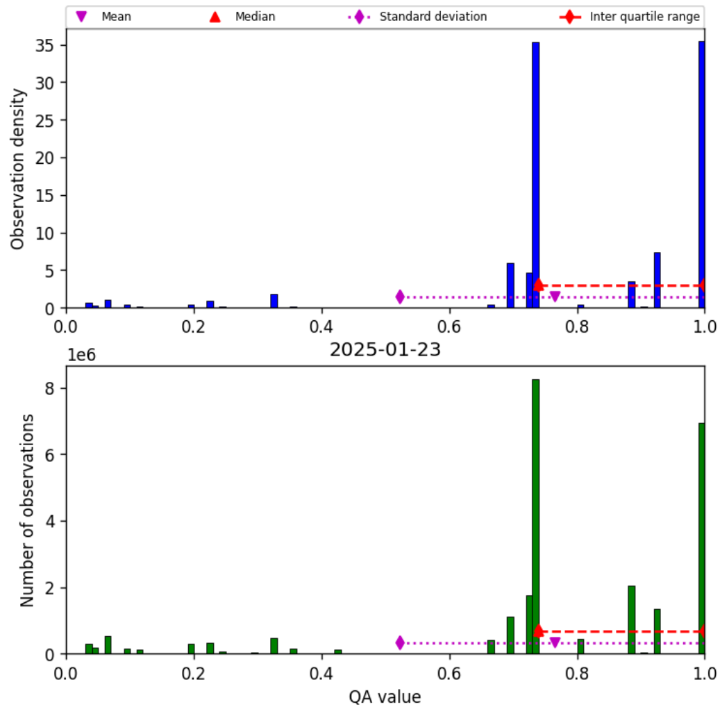
Figure 28: Histogram of “QA value” for 2025-01-23 to 2025-01-24
