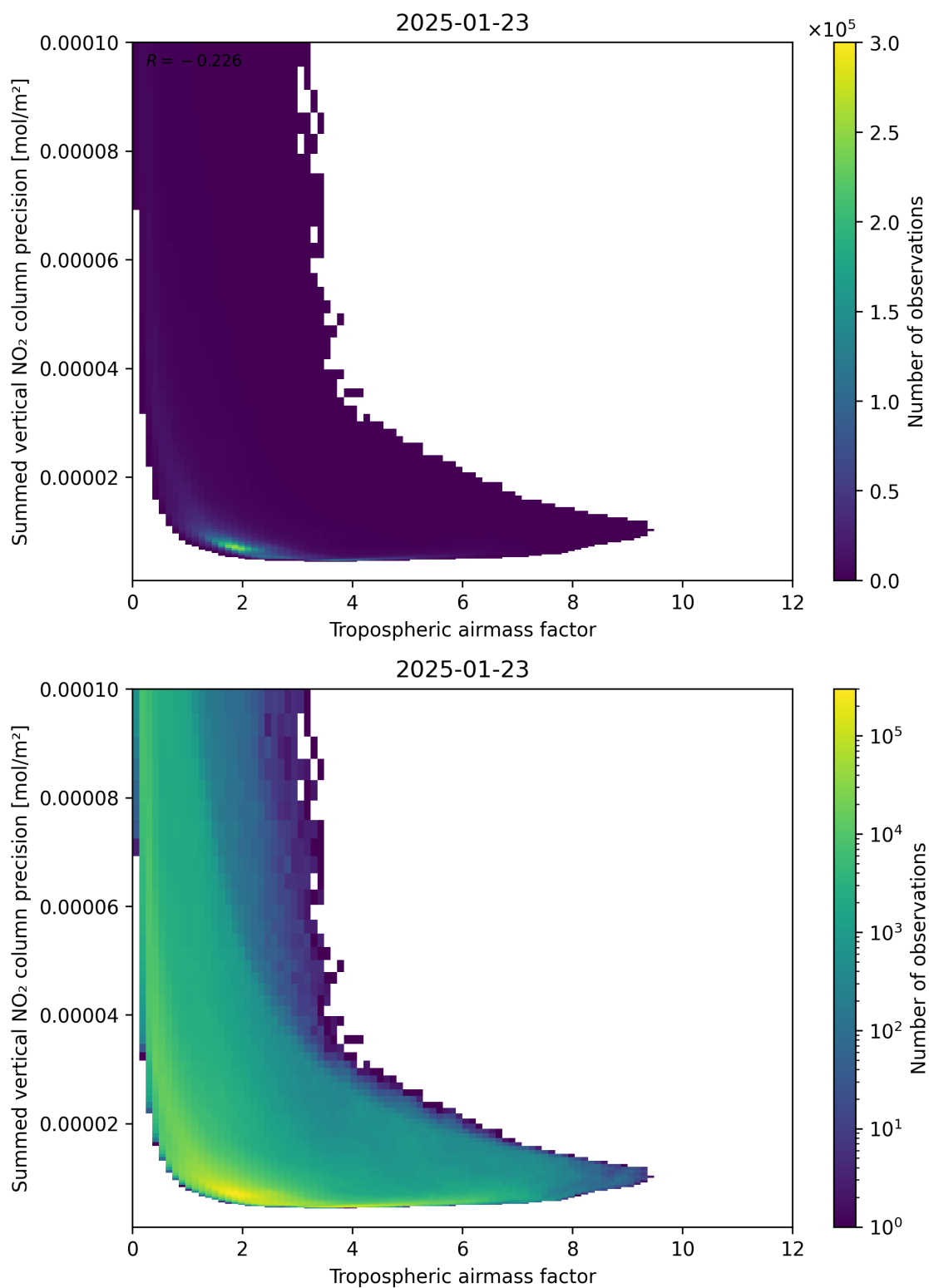
Figure 76: Scatter density plot of “Tropospheric air mass factor” against “Summed vertical NO 2 column precision” for 2025-01-23 to 2025-01-24.
