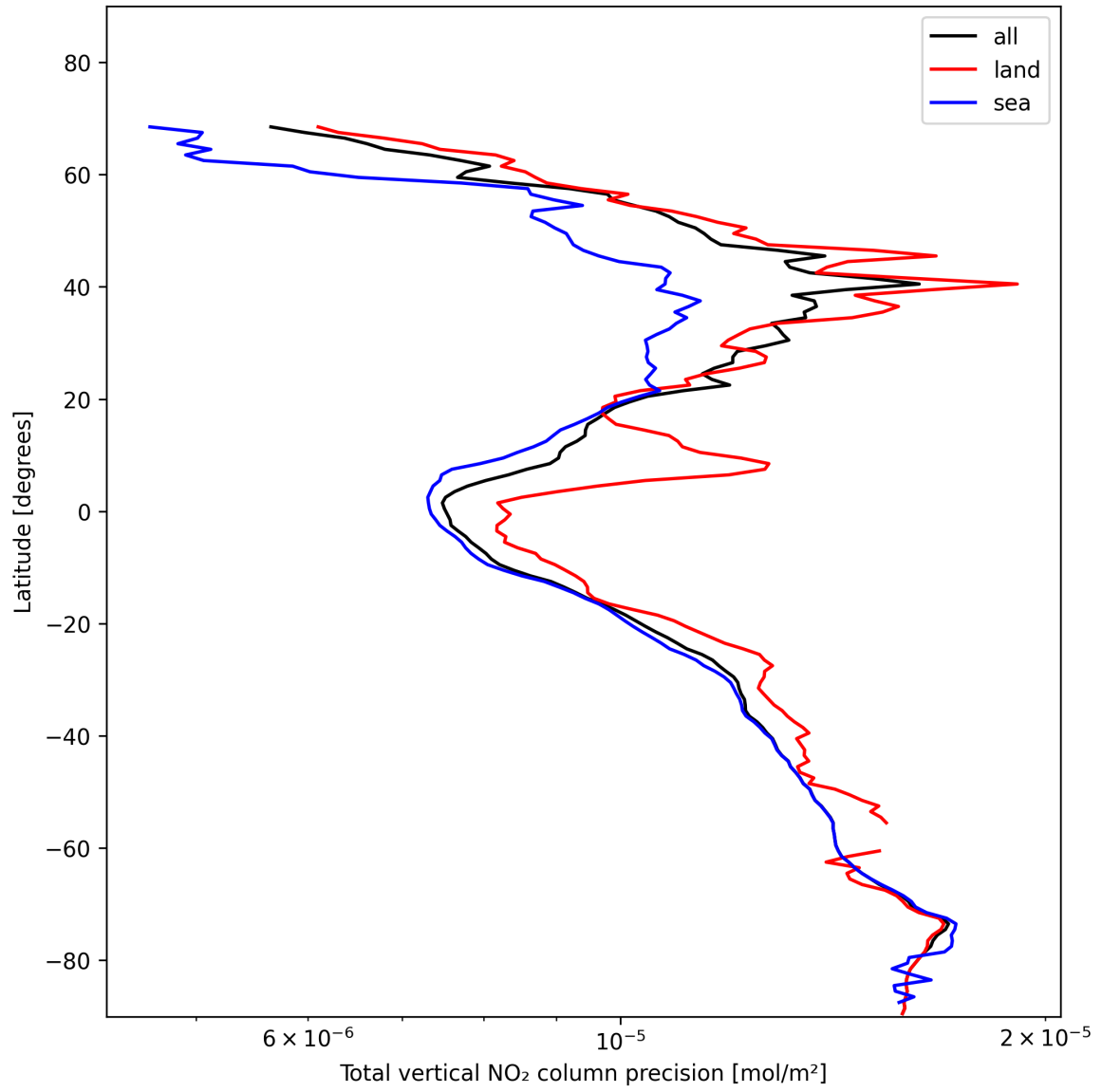
Figure 22: Zonal average of “Total vertical NO 2 column precision” for 2025-01-23 to 2025-01-24.
