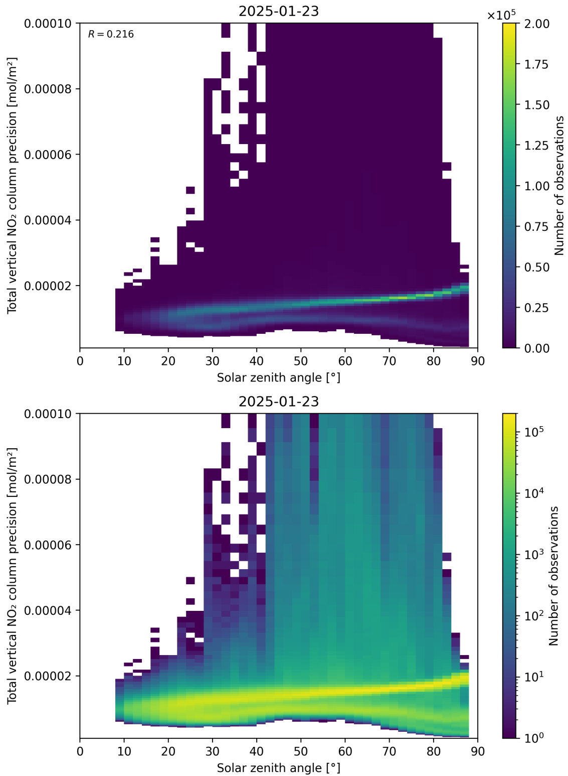
Figure 154: Scatter density plot of “Solar zenith angle” against “Total vertical NO 2 column precision” for 2025-01-23 to 2025-01-24.
