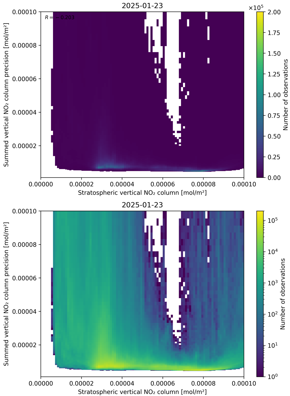
Figure 99: Scatter density plot of “Stratospheric vertical NO 2 column” against “Summed vertical NO 2 column precision” for 2025-01-23 to 2025-01-24.
