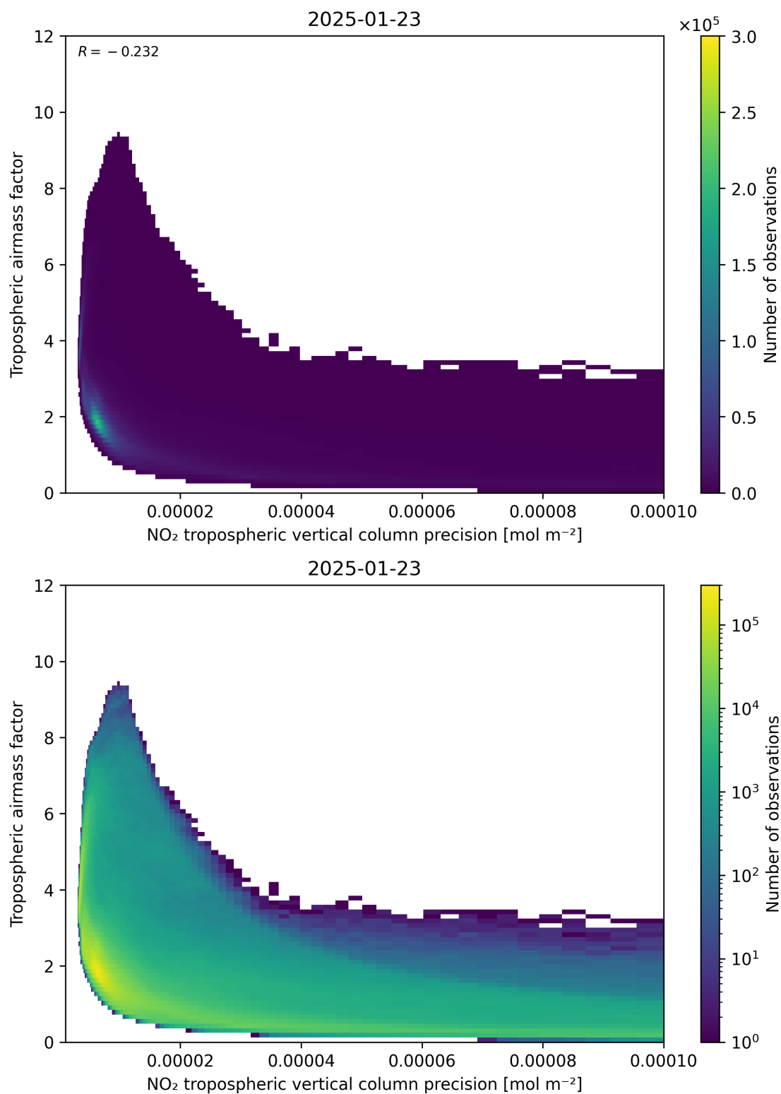
Figure 133: Scatter density plot of “NO 2 tropospheric vertical column precision” against “Tropospheric air mass factor” for 2025-01-23 to 2025-01-24.
