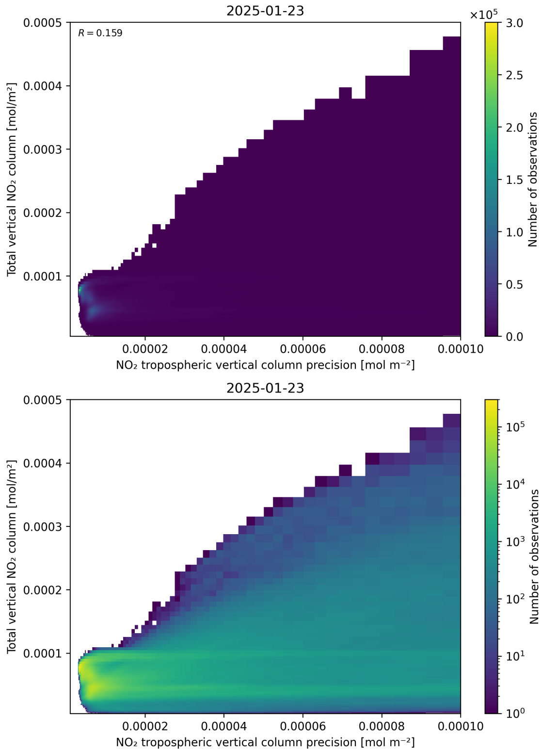
Figure 138: Scatter density plot of “NO 2 tropospheric vertical column precision” against “Total vertical NO 2 column” for 2025-01-23 to 2025-01-24.
