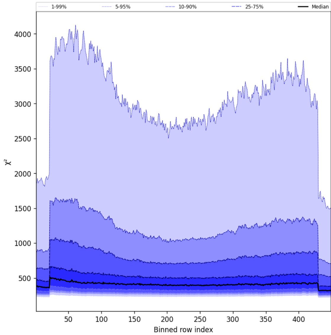
Figure 59: Along track statistics of “ \chi^2 ” for 2025-01-23 to 2025-01-24
