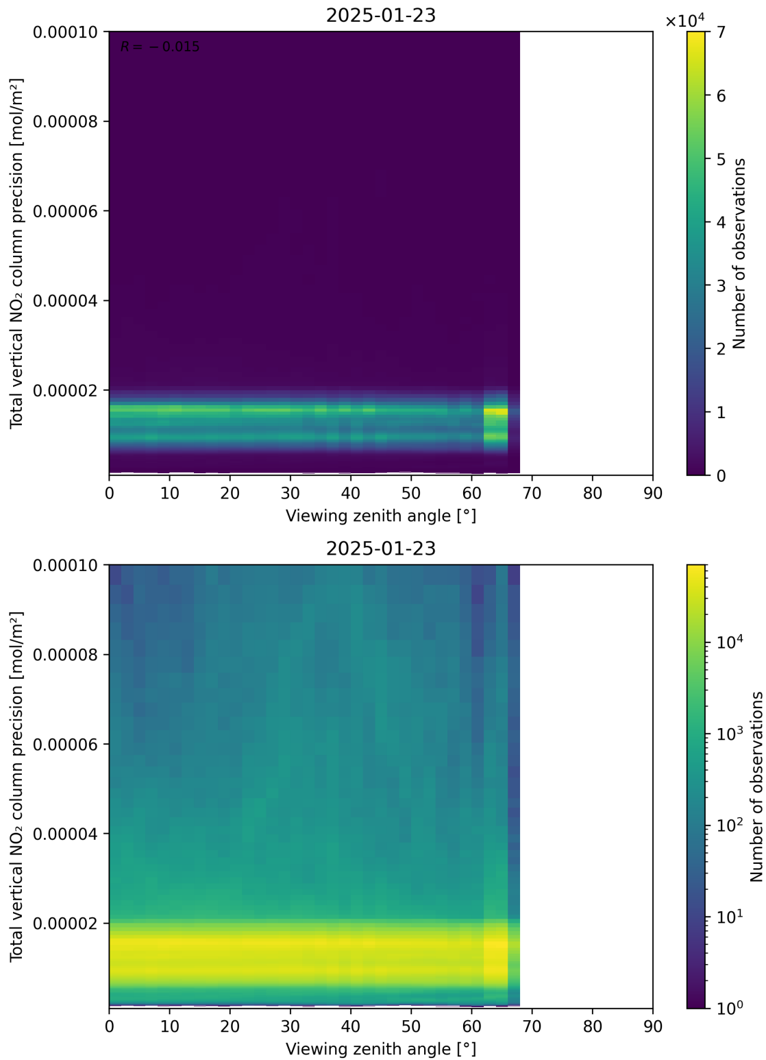
Figure 168: Scatter density plot of “Viewing zenith angle” against “Total vertical NO 2 column precision” for 2025-01-23 to 2025-01-24.
