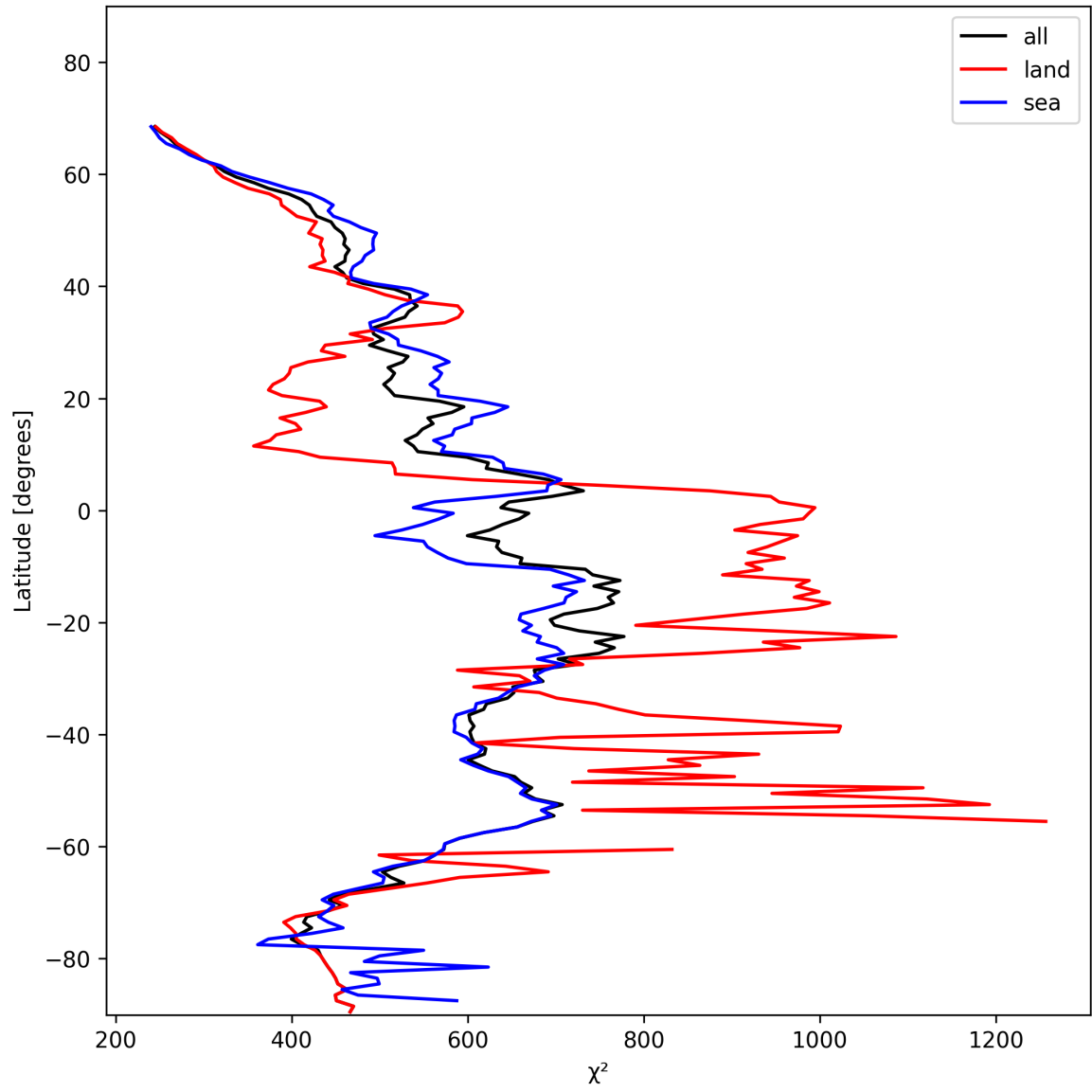
Figure 25: Zonal average of “ \chi^2 ” for 2025-01-23 to 2025-01-24.
