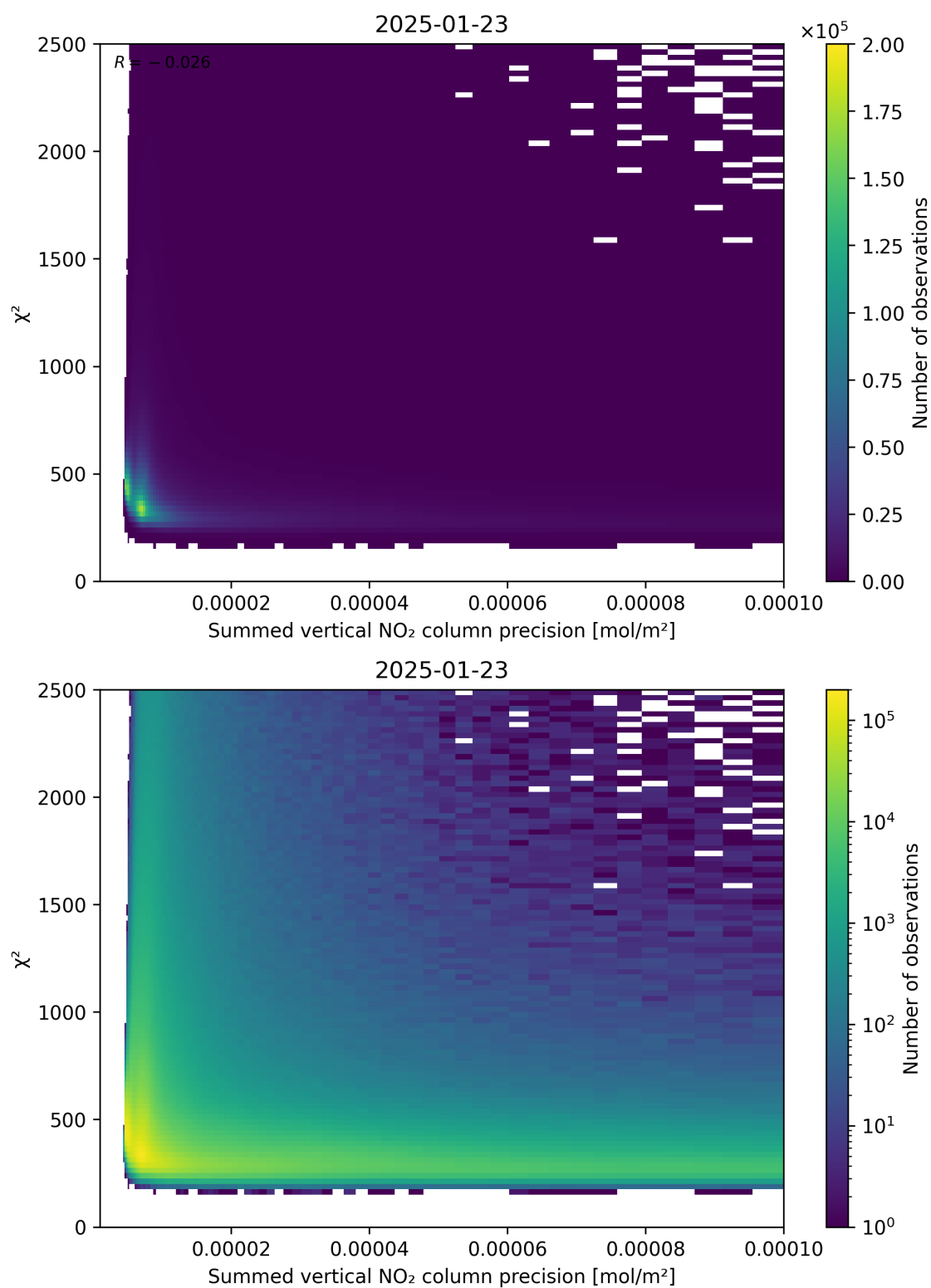
Figure 107: Scatter density plot of “Summed vertical NO 2 column precision” against “ \chi^2 ” for 2025-01-23 to 2025-01-24.
