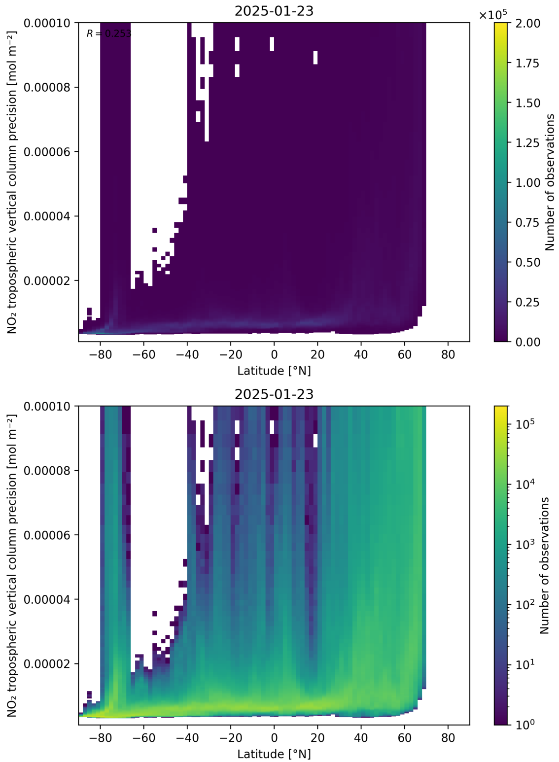
Figure 93: Scatter density plot of “Latitude” against “NO 2 tropospheric vertical column precision” for 2025-01-23 to 2025-01-24.
