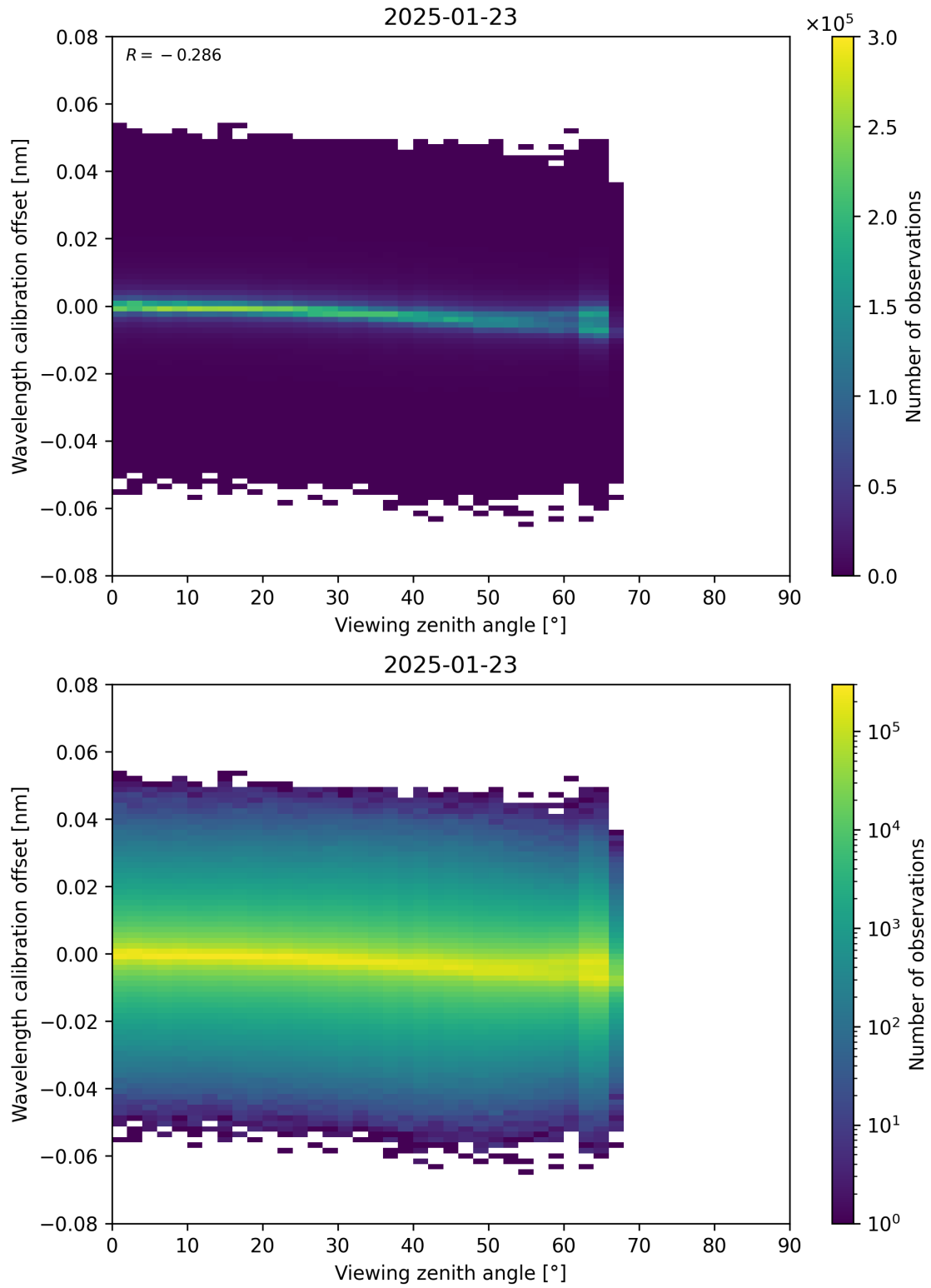
Figure 173: Scatter density plot of “Viewing zenith angle” against “Wavelength calibration offset” for 2025-01-23 to 2025-01-24.
