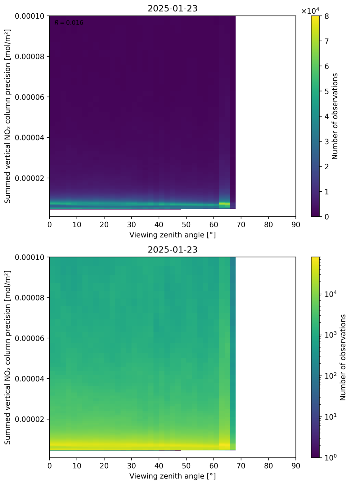
Figure 166: Scatter density plot of “Viewing zenith angle” against “Summed vertical NO 2 column precision” for 2025-01-23 to 2025-01-24.
