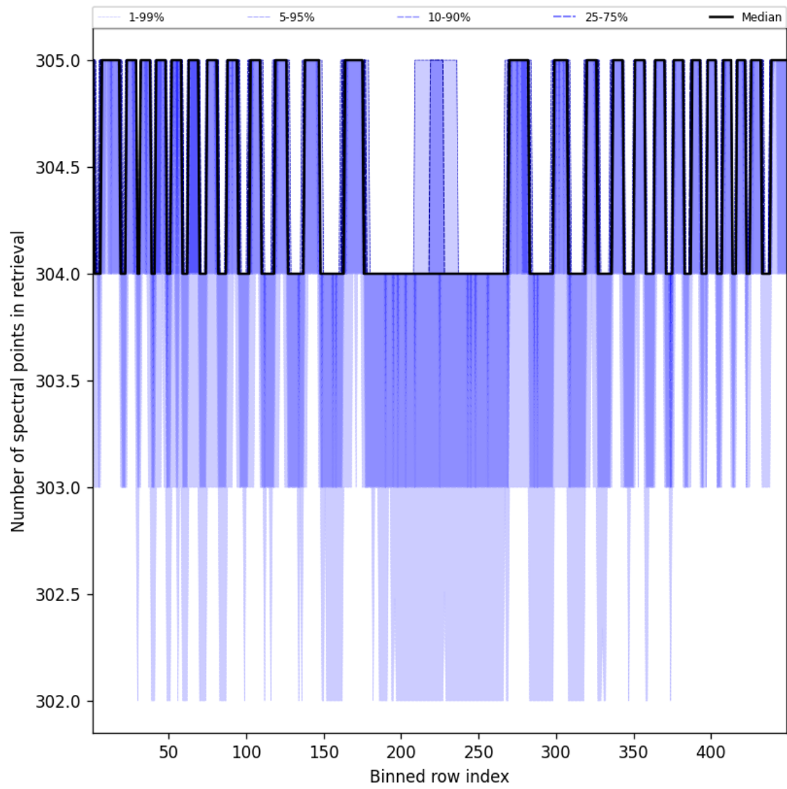
Figure 50: Along track statistics of “Number of spectral points in retrieval” for 2025-01-23 to 2025-01-24
