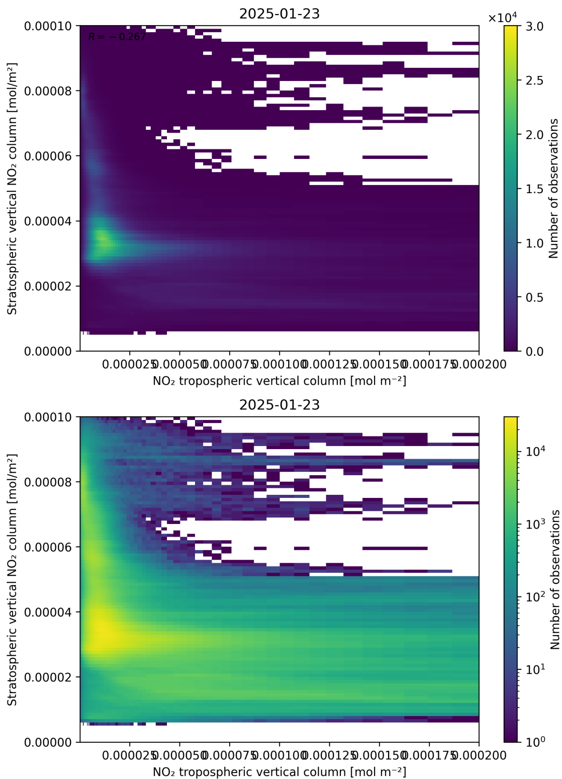
Figure 125: Scatter density plot of “NO 2 tropospheric vertical column” against “Stratospheric vertical NO 2 column” for 2025-01-23 to 2025-01-24.
