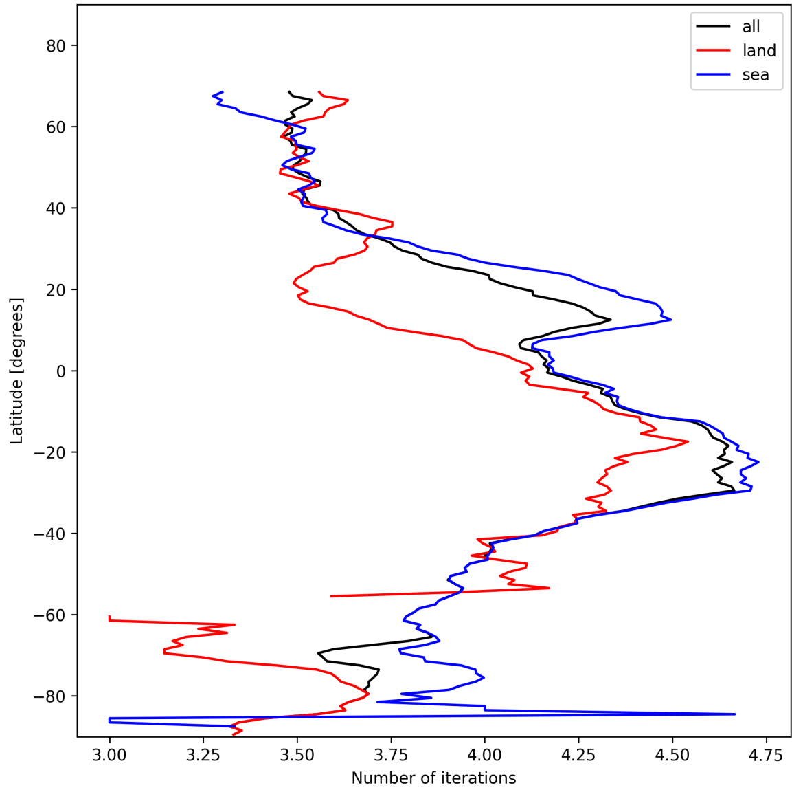
Figure 17: Zonal average of “Number of iterations” for 2025-01-23 to 2025-01-24.
