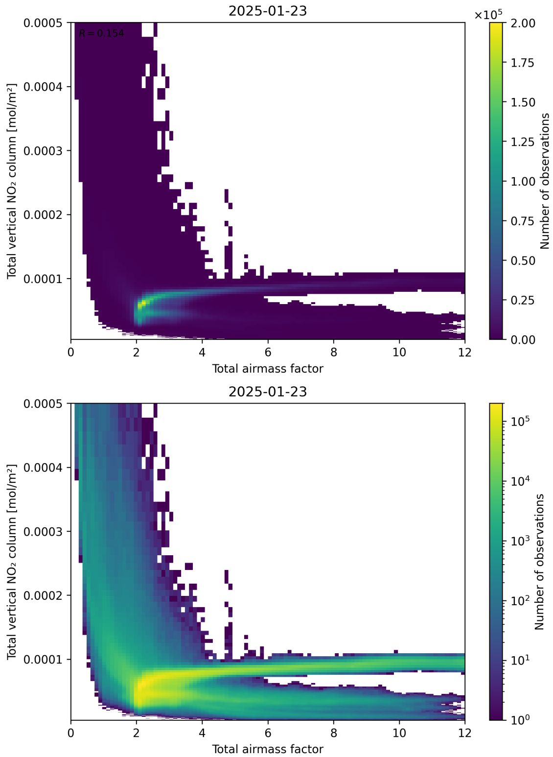
Figure 67: Scatter density plot of “Total airmass factor” against “Total vertical NO 2 column” for 2025-01-23 to 2025-01-24.
