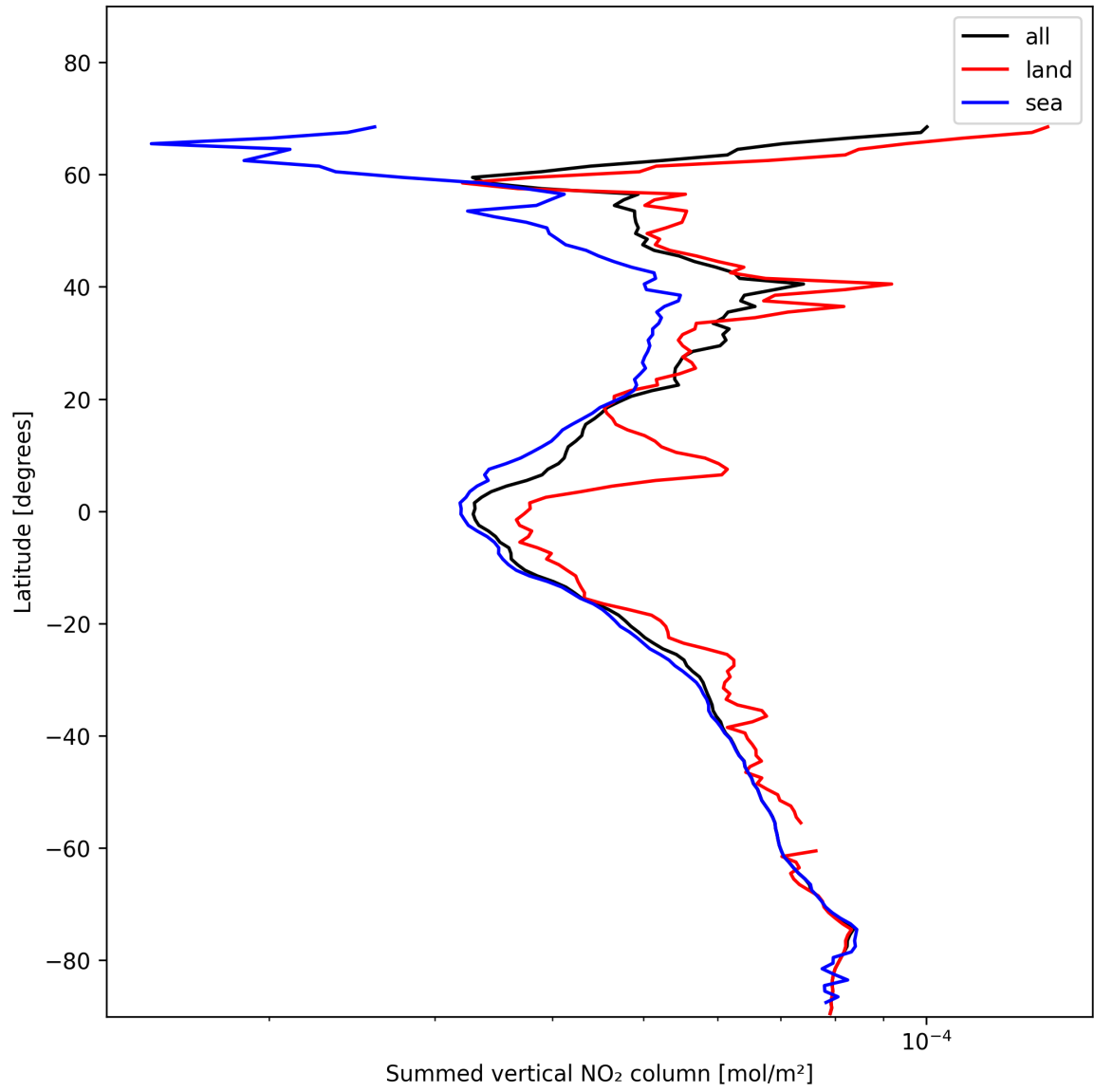
Figure 23: Zonal average of “Summed vertical NO 2 column” for 2025-01-23 to 2025-01-24.
