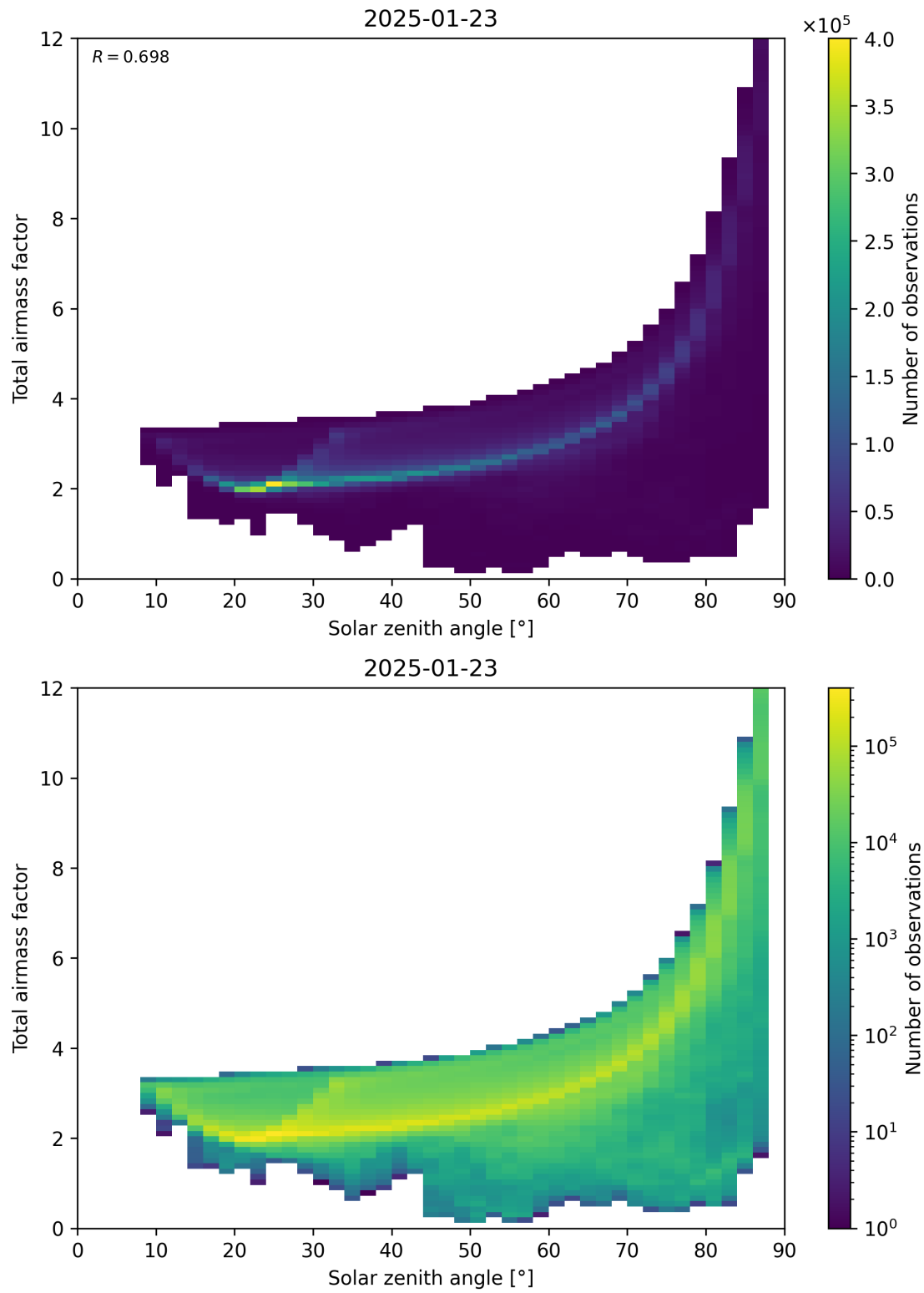
Figure 146: Scatter density plot of “Solar zenith angle” against “Total air mass factor” for 2025-01-23 to 2025-01-24.
