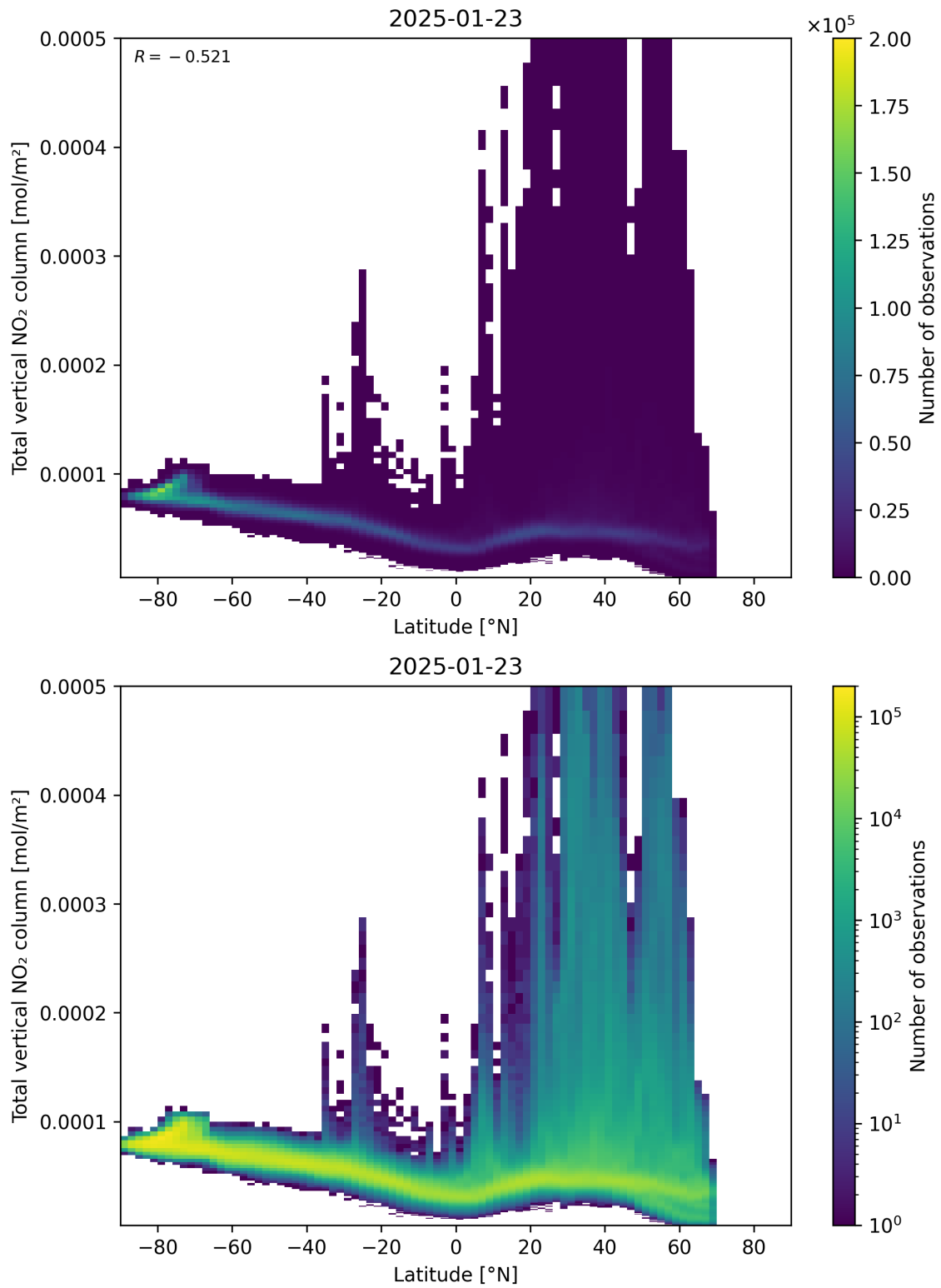
Figure 90: Scatter density plot of “Latitude” against “Total vertical NO 2 column” for 2025-01-23 to 2025-01-24.
