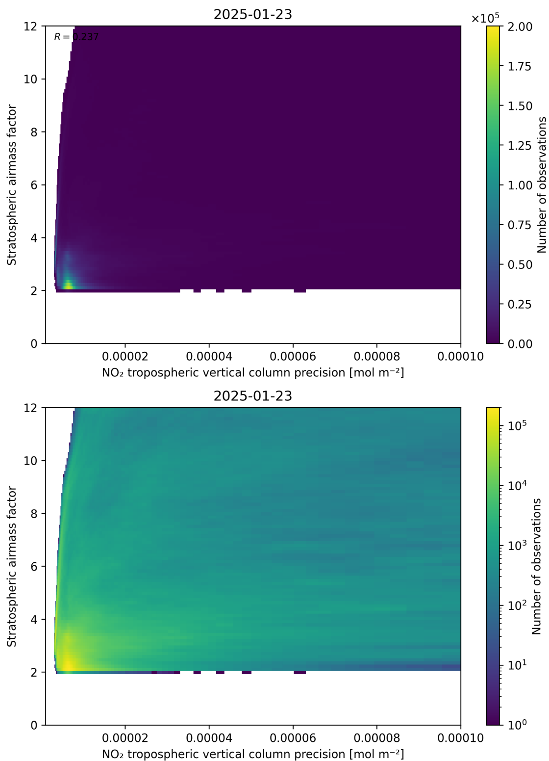
Figure 131: Scatter density plot of “NO 2 tropospheric vertical column precision” against “Stratospheric airmass factor” for 2025-01-23 to 2025-01-24.
