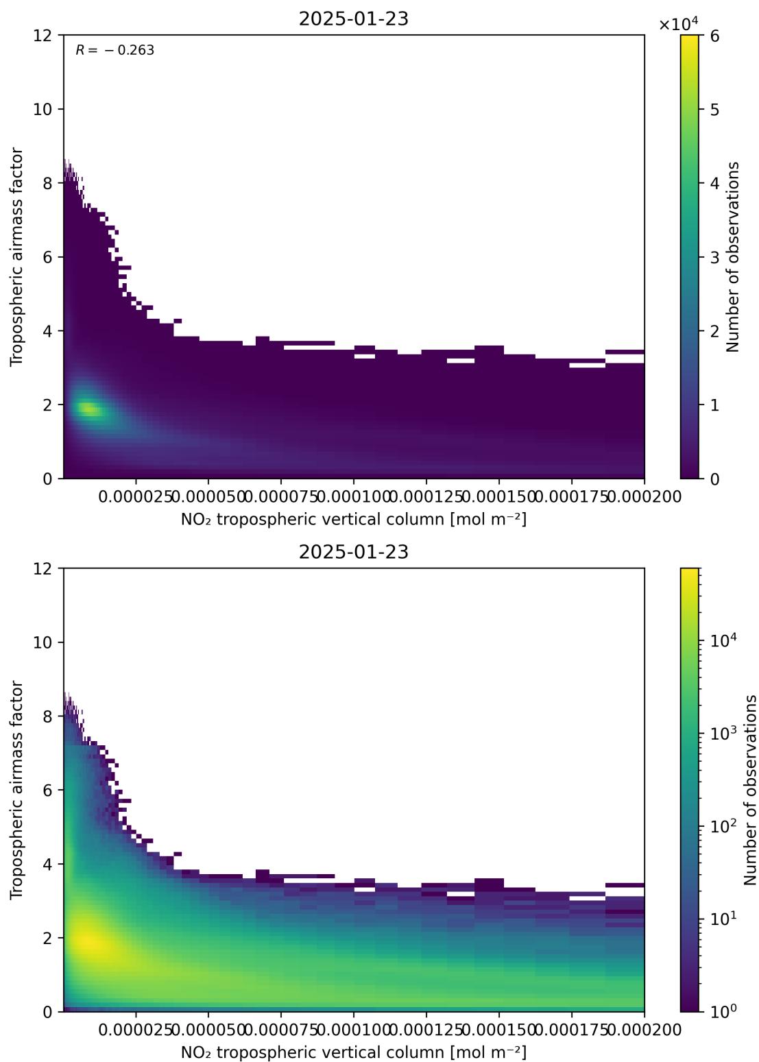
Figure 123: Scatter density plot of “NO 2 tropospheric vertical column” against “Tropospheric air mass factor” for 2025-01-23 to 2025-01-24.
