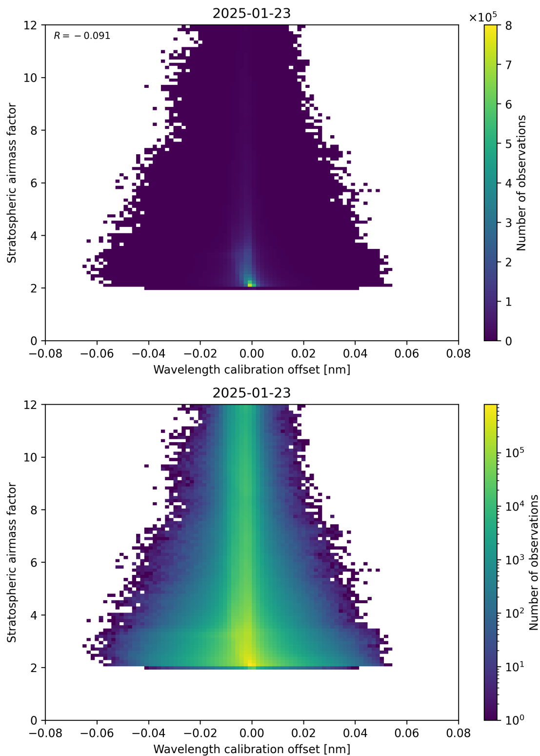
Figure 174: Scatter density plot of “Wavelength calibration offset” against “Stratospheric airmass factor” for 2025-01-23 to 2025-01-24.
