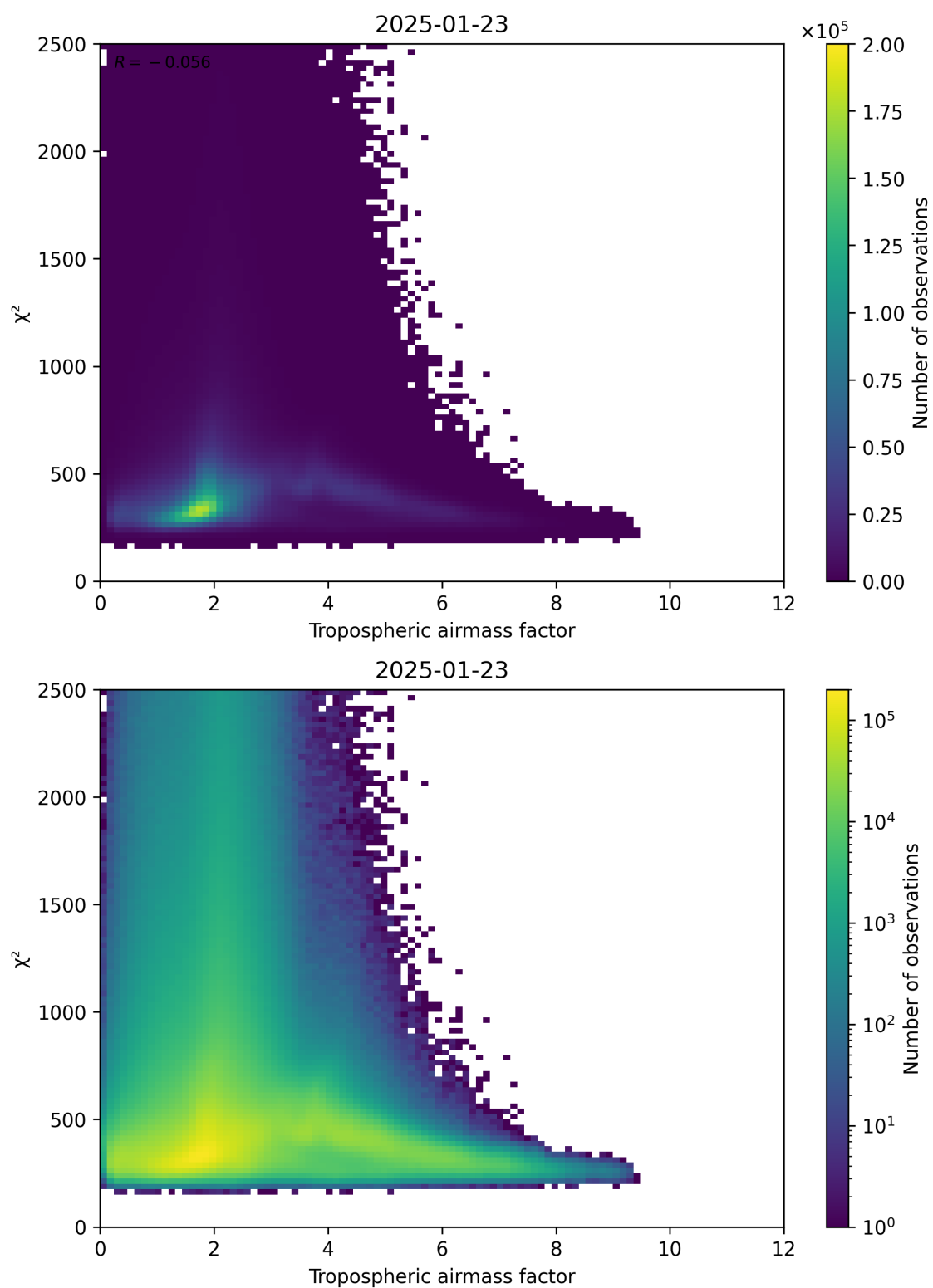
Figure 73: Scatter density plot of “Tropospheric airmass factor” against “ \chi^2 ” for 2025-01-23 to 2025-01-24.
