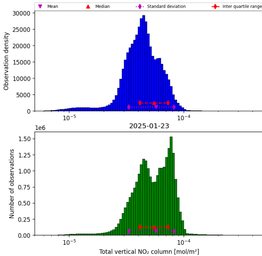
Figure 38: Histogram of “Total vertical NO 2 column” for 2025-01-23 to 2025-01-24
