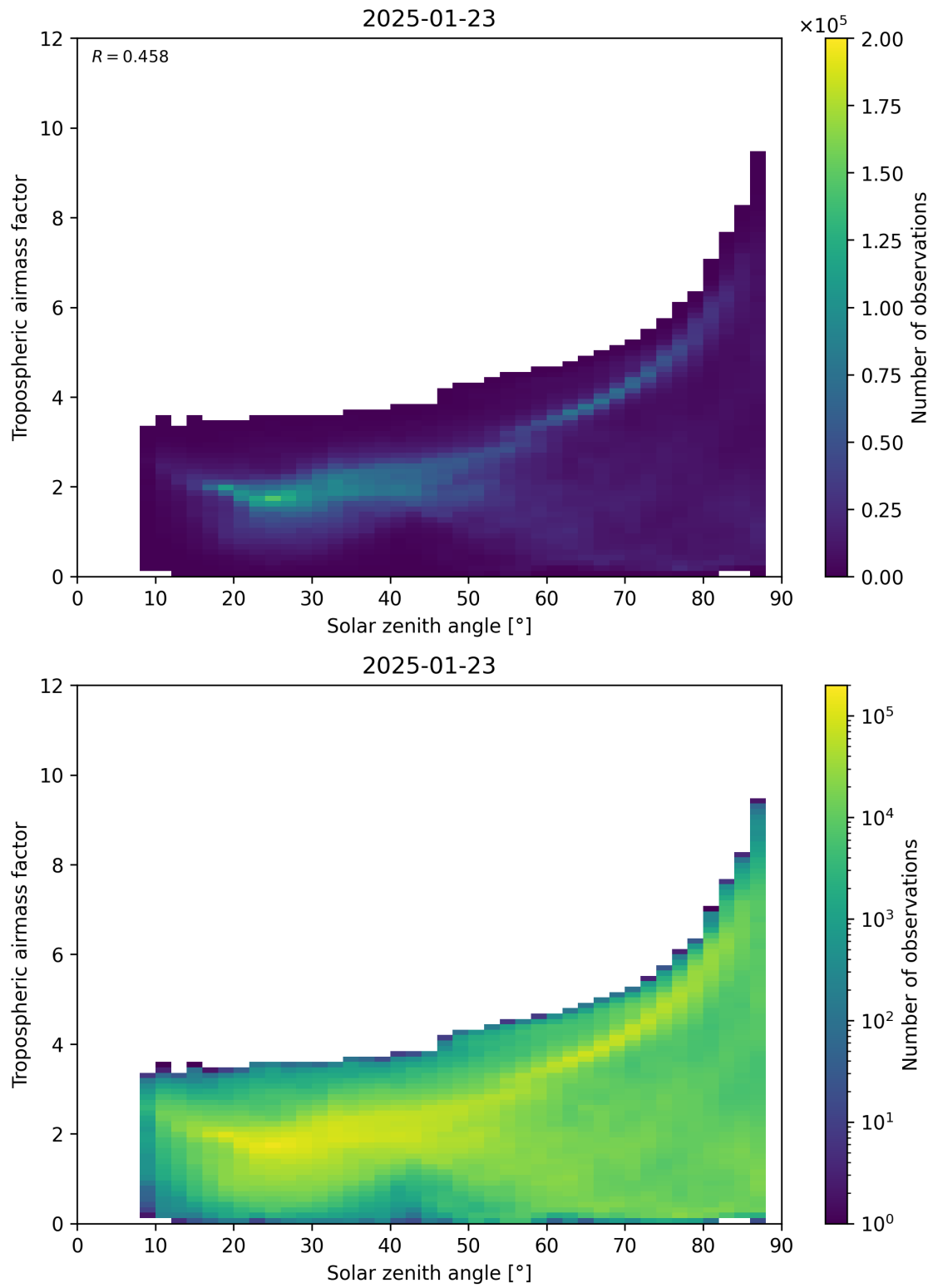
Figure 147: Scatter density plot of “Solar zenith angle” against “Tropospheric airmass factor” for 2025-01-23 to 2025-01-24.
