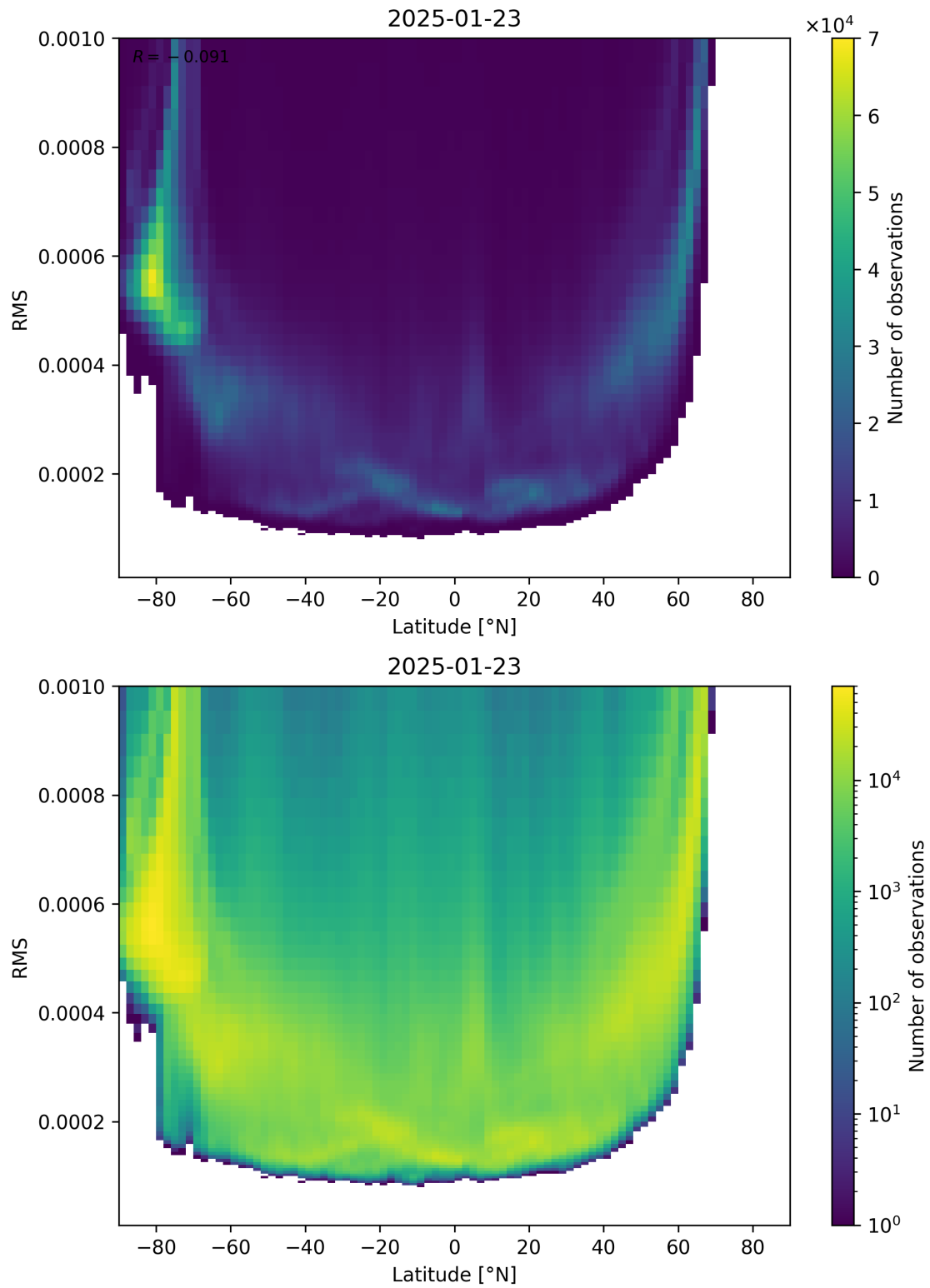
Figure 94: Scatter density plot of “Latitude” against “RMS” for 2025-01-23 to 2025-01-24.
