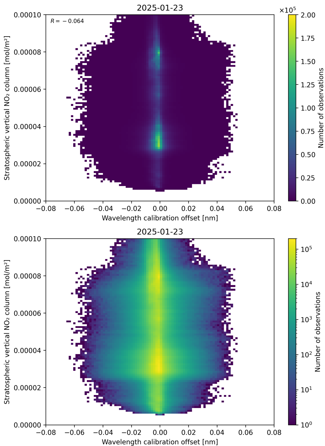
Figure 176: Scatter density plot of “Wavelength calibration offset” against “Stratospheric vertical NO 2 column” for 2025-01-23 to 2025-01-24.
