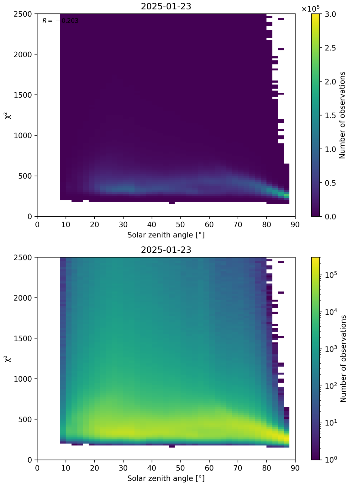
Figure 148: Scatter density plot of “Solar zenith angle” against “ \chi^2 ” for 2025-01-23 to 2025-01-24.
