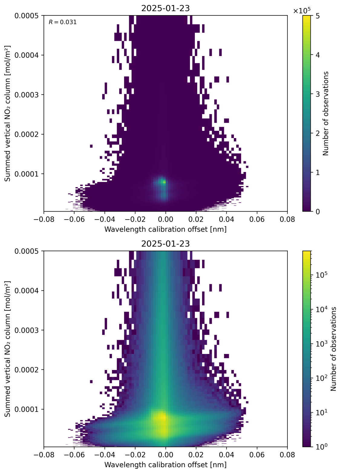
Figure 177: Scatter density plot of “Wavelength calibration offset” against “Summed vertical NO 2 column” for 2025-01-23 to 2025-01-24.
