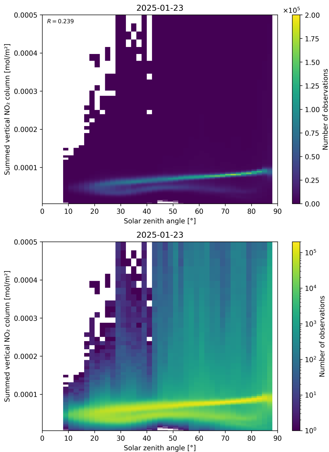
Figure 151: Scatter density plot of “Solar zenith angle” against “Summed vertical NO 2 column” for 2025-01-23 to 2025-01-24.
