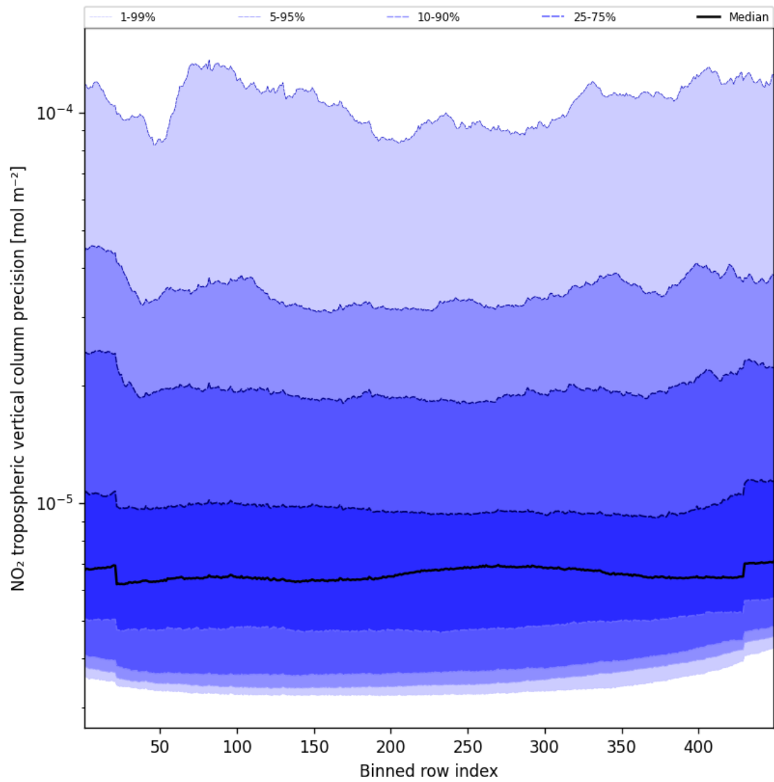
Figure 47: Along track statistics of “NO 2 tropospheric vertical column precision” for 2025-01-23 to 2025-01-24
