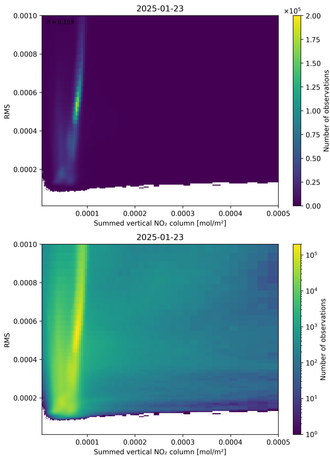
Figure 109: Scatter density plot of “Summed vertical NO 2 column” against “RMS” for 2025-01-23 to 2025-01-24.
