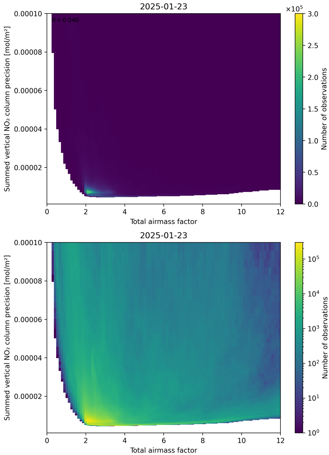
Figure 66: Scatter density plot of “Total airmass factor” against “Summed vertical NO 2 column precision” for 2025-01-23 to 2025-01-24.
