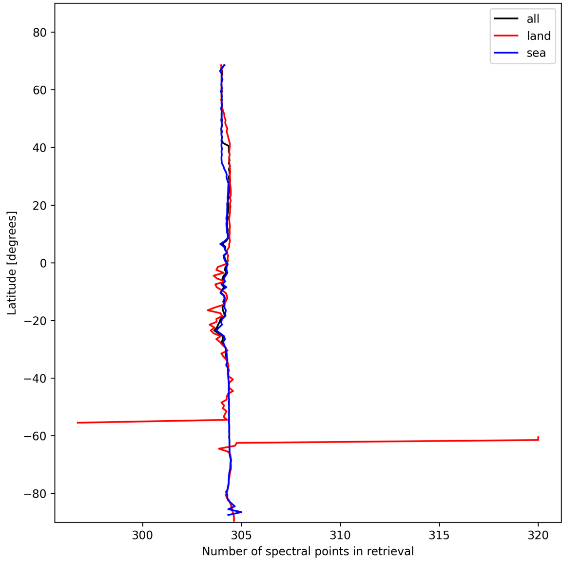
Figure 16: Zonal average of “Number of spectral points in retrieval” for 2025-01-23 to 2025-01-24.
