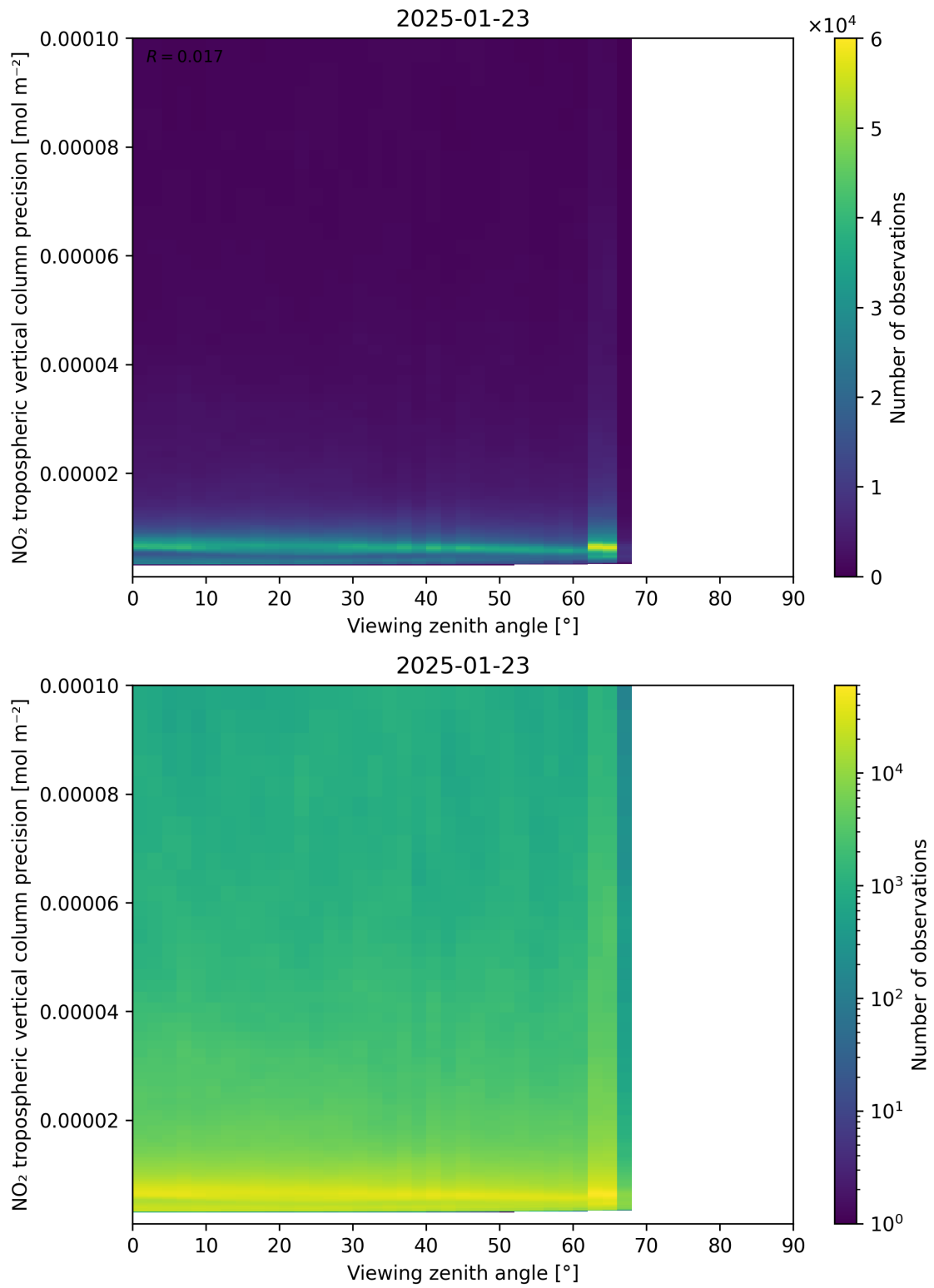
Figure 170: Scatter density plot of “Viewing zenith angle” against “NO 2 tropospheric vertical column precision” for 2025-01-23 to 2025-01-24.
