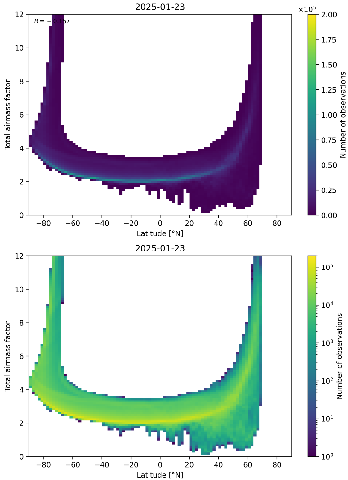
Figure 84: Scatter density plot of “Latitude” against “Total airmass factor” for 2025-01-23 to 2025-01-24.
