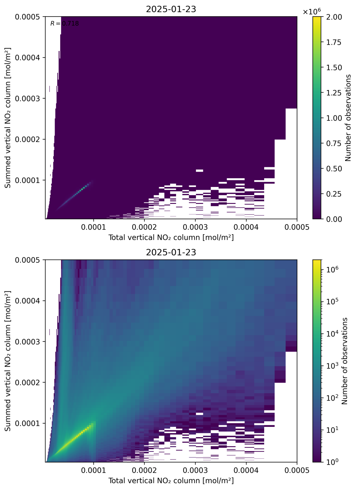
Figure 112: Scatter density plot of “Total vertical NO 2 column” against “Summed vertical NO 2 column” for 2025-01-23 to 2025-01-24.
