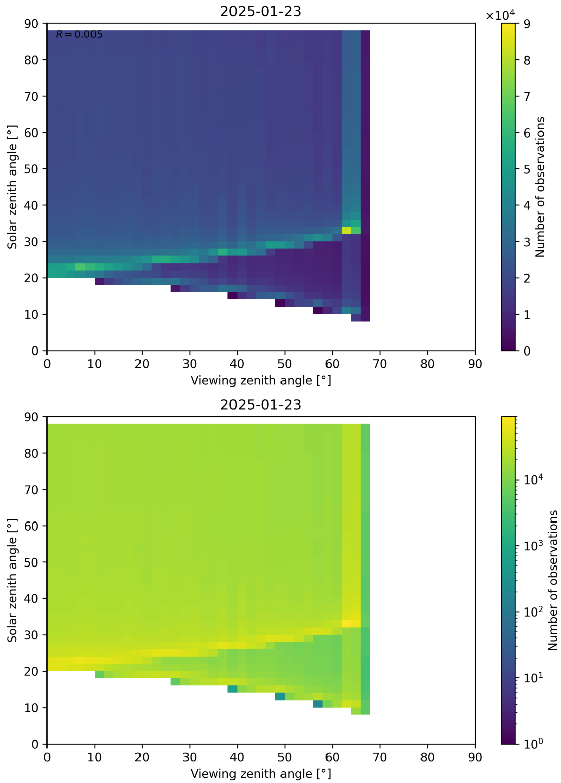
Figure 172: Scatter density plot of “Viewing zenith angle” against “Solar zenith angle” for 2025-01-23 to 2025-01-24.
