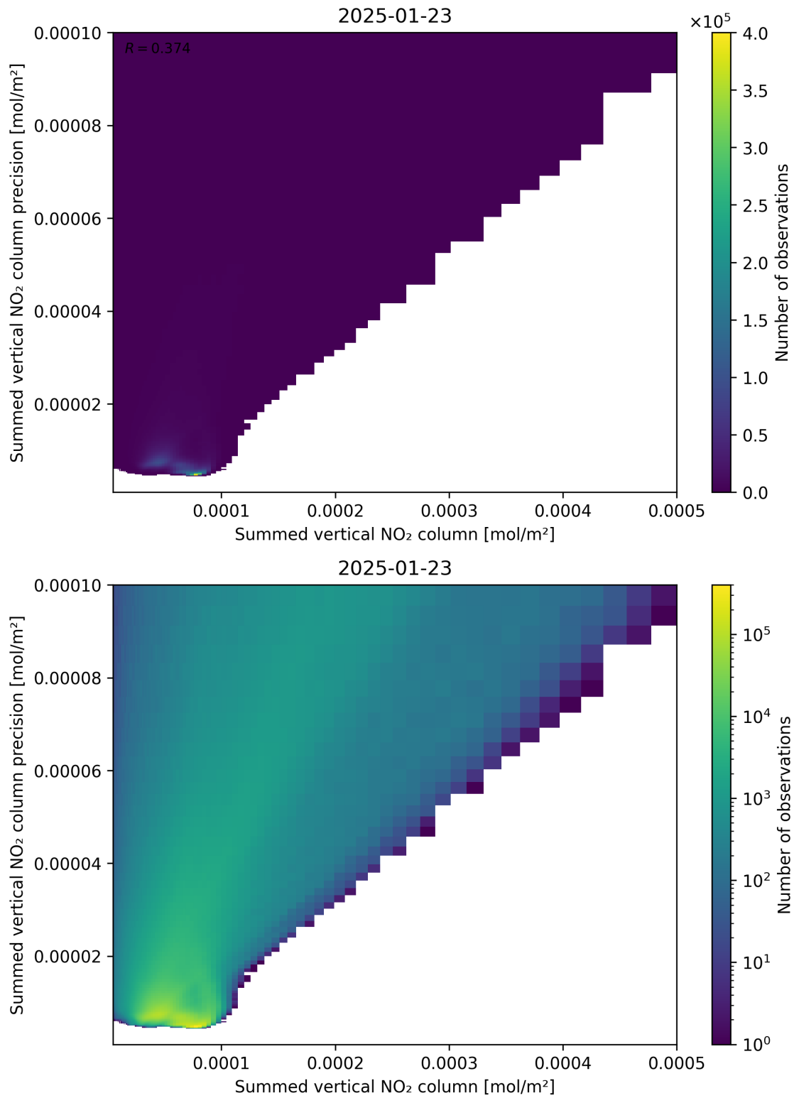
Figure 105: Scatter density plot of “Summed vertical NO 2 column” against “Summed vertical NO 2 column precision” for 2025-01-23 to 2025-01-24.
