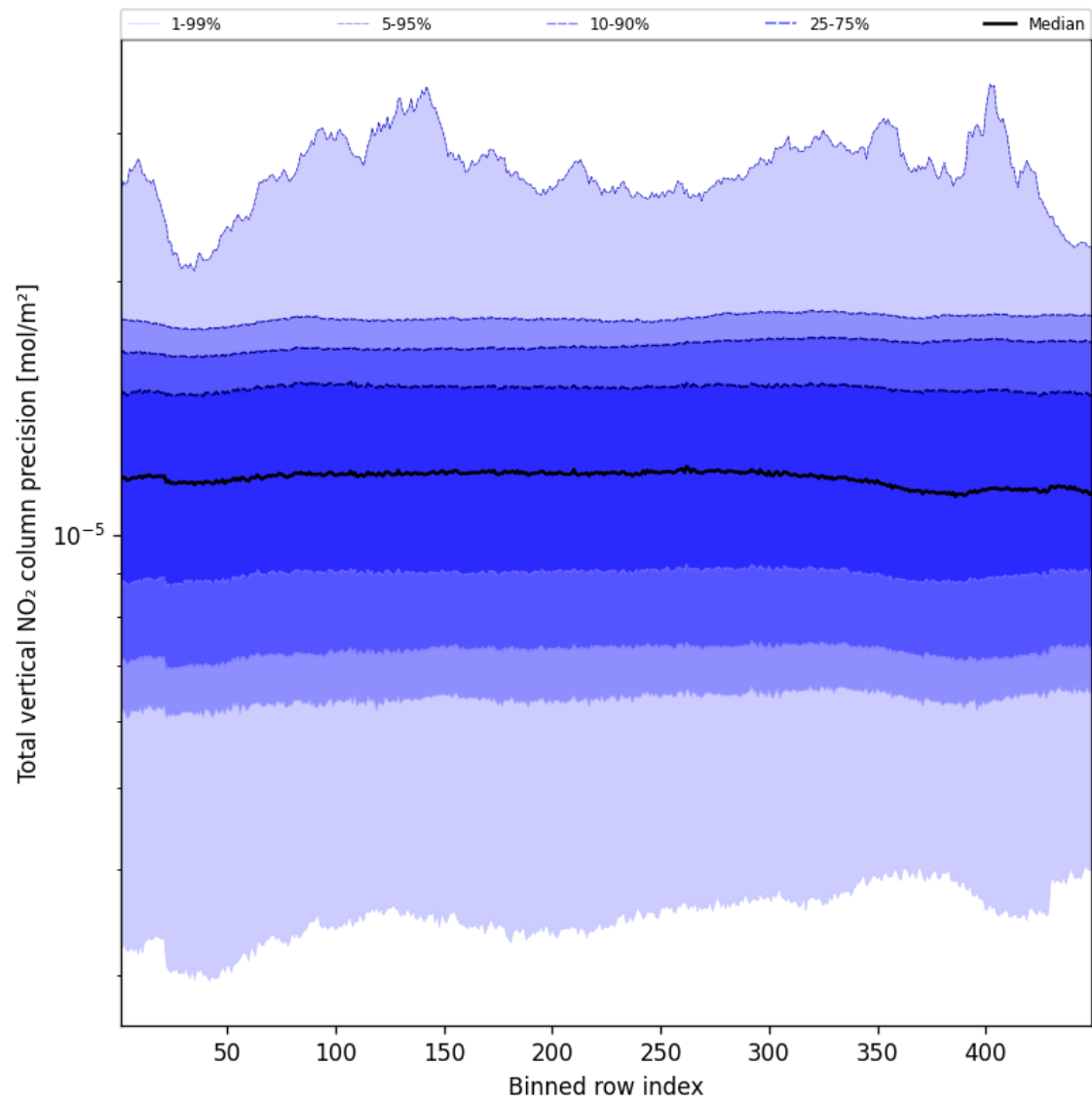
Figure 56: Along track statistics of “Total vertical NO 2 column precision” for 2025-01-23 to 2025-01-24
