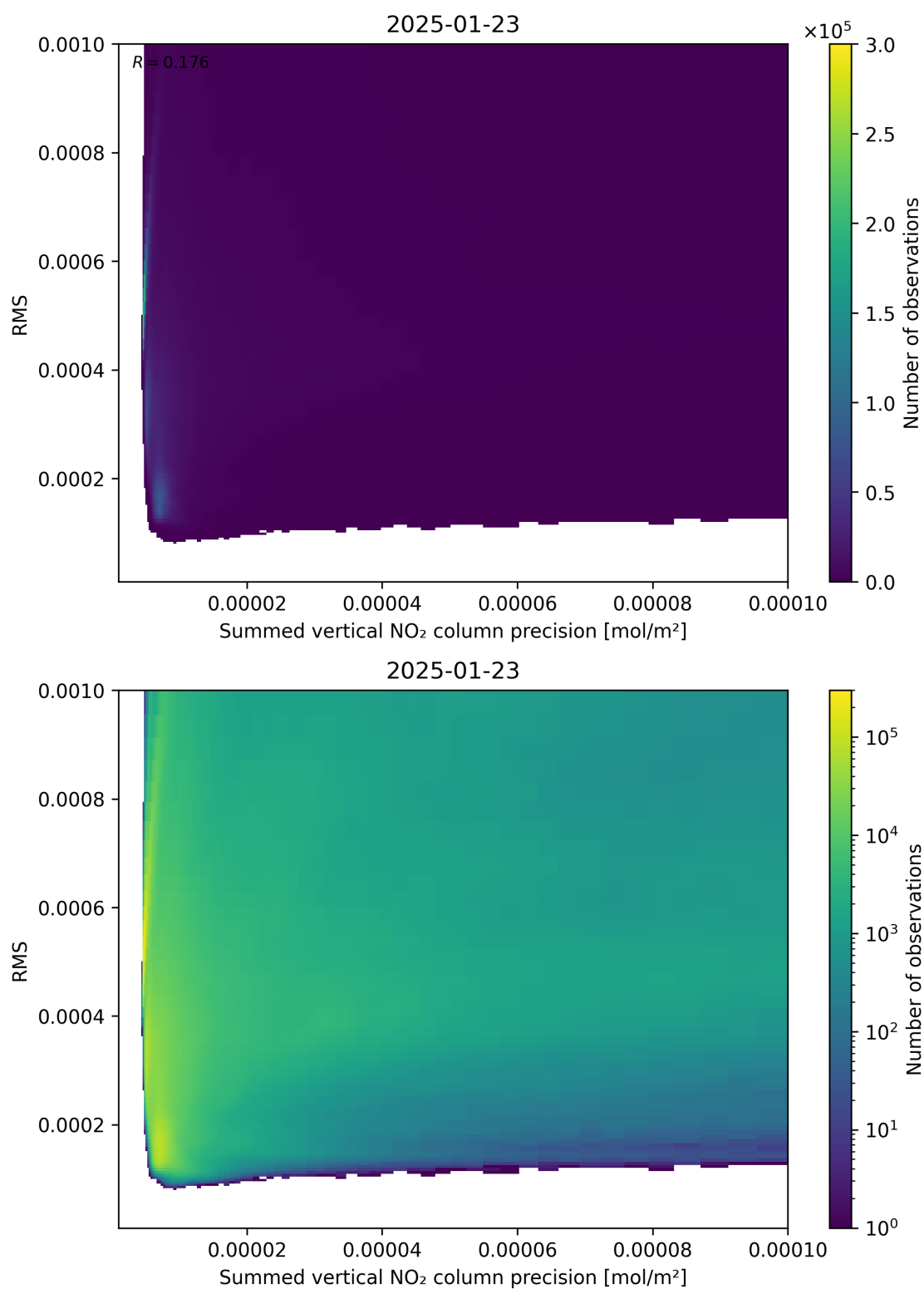
Figure 108: Scatter density plot of “Summed vertical NO 2 column precision” against “RMS” for 2025-01-23 to 2025-01-24.
