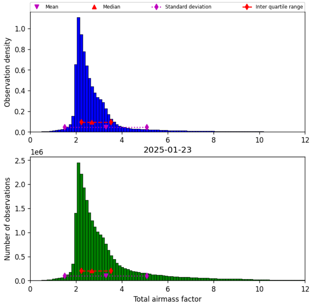
Figure 32: Histogram of “Total airmass factor” for 2025-01-23 to 2025-01-24
