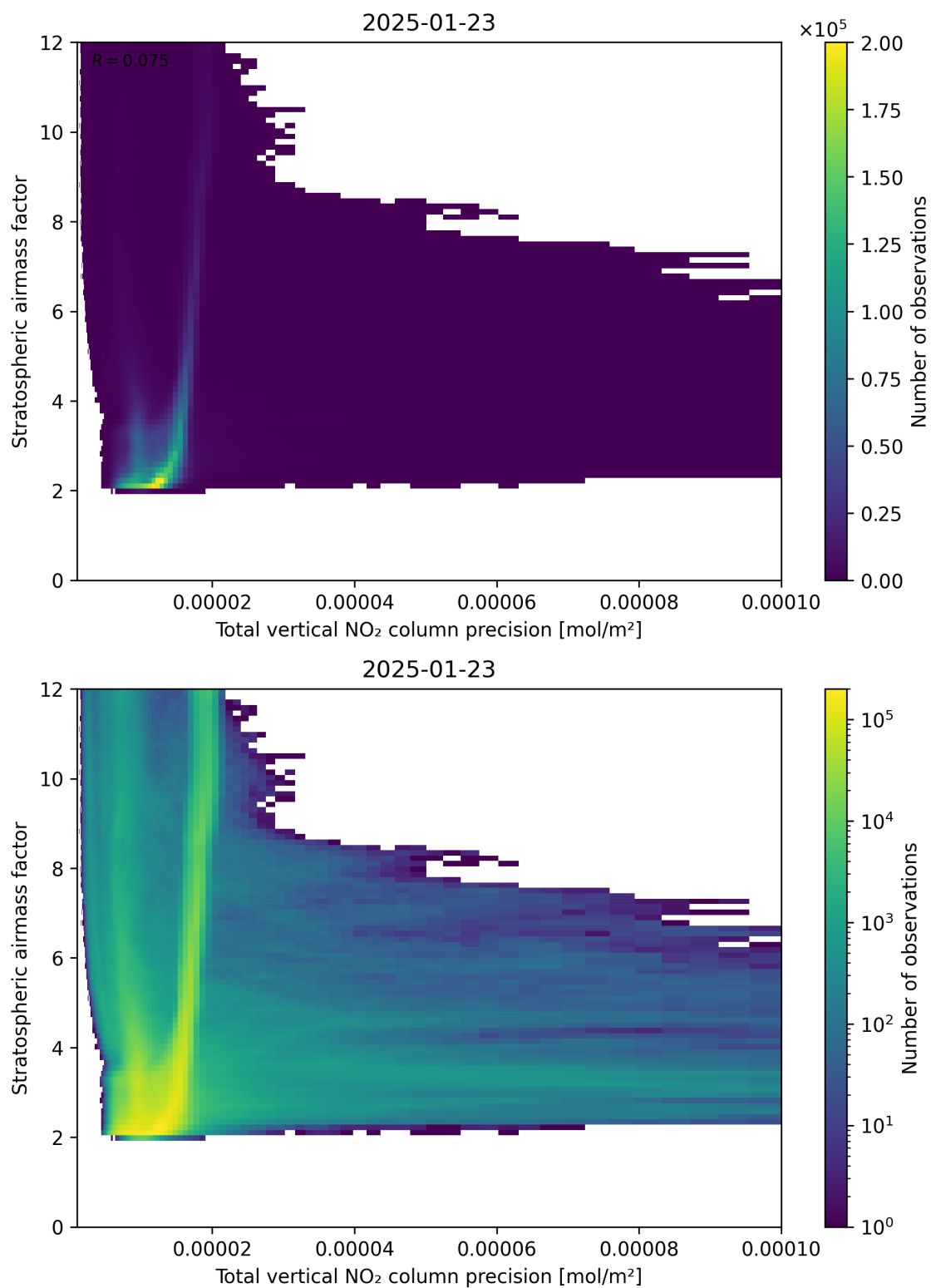
Figure 115: Scatter density plot of “Total vertical NO 2 column precision” against “Stratospheric air mass factor” for 2025-01-23 to 2025-01-24.
