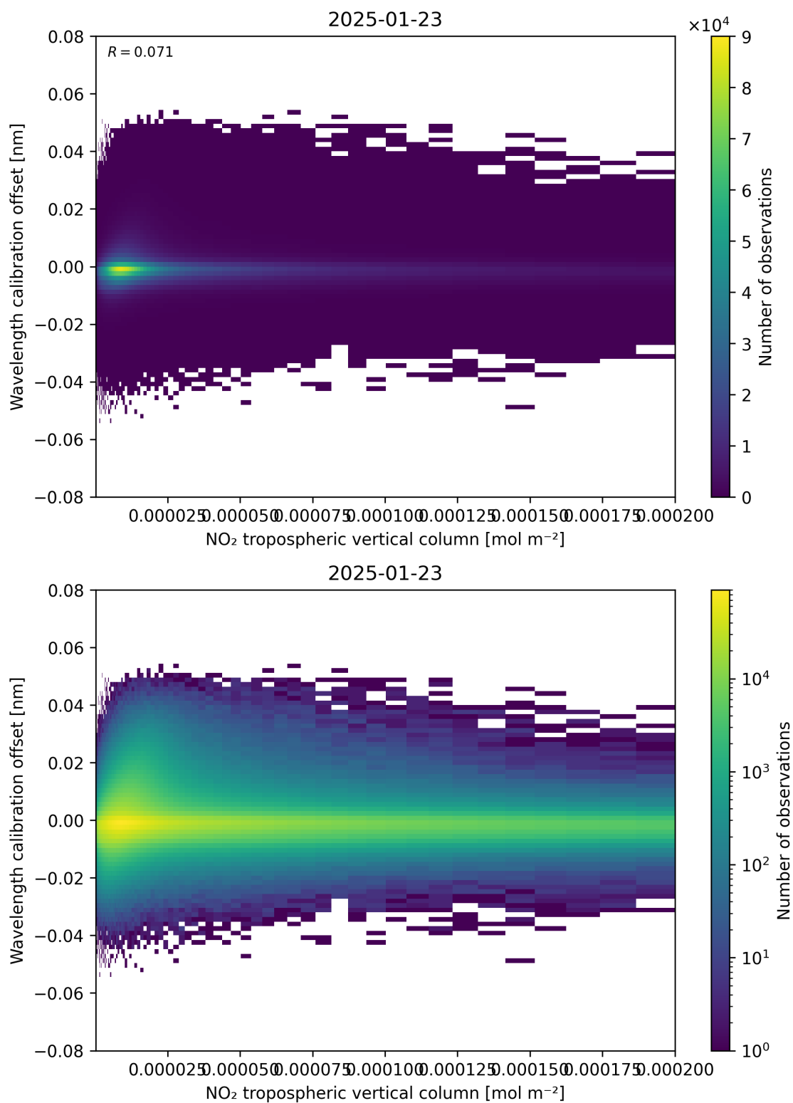
Figure 143: Scatter density plot of “NO 2 tropospheric vertical column” against “Wavelength calibration offset” for 2025-01-23 to 2025-01-24.
