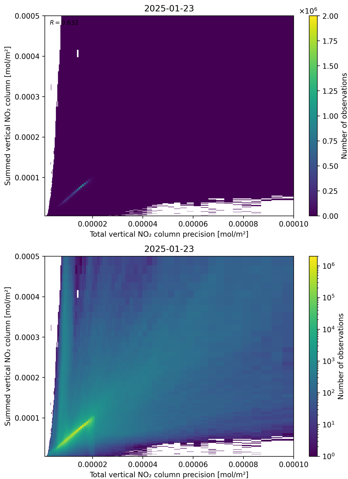
Figure 117: Scatter density plot of “Total vertical NO 2 column precision” against “Summed vertical NO 2 column” for 2025-01-23 to 2025-01-24.
