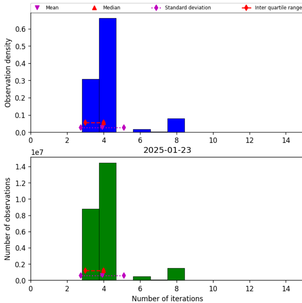
Figure 34: Histogram of “Number of iterations” for 2025-01-23 to 2025-01-24
