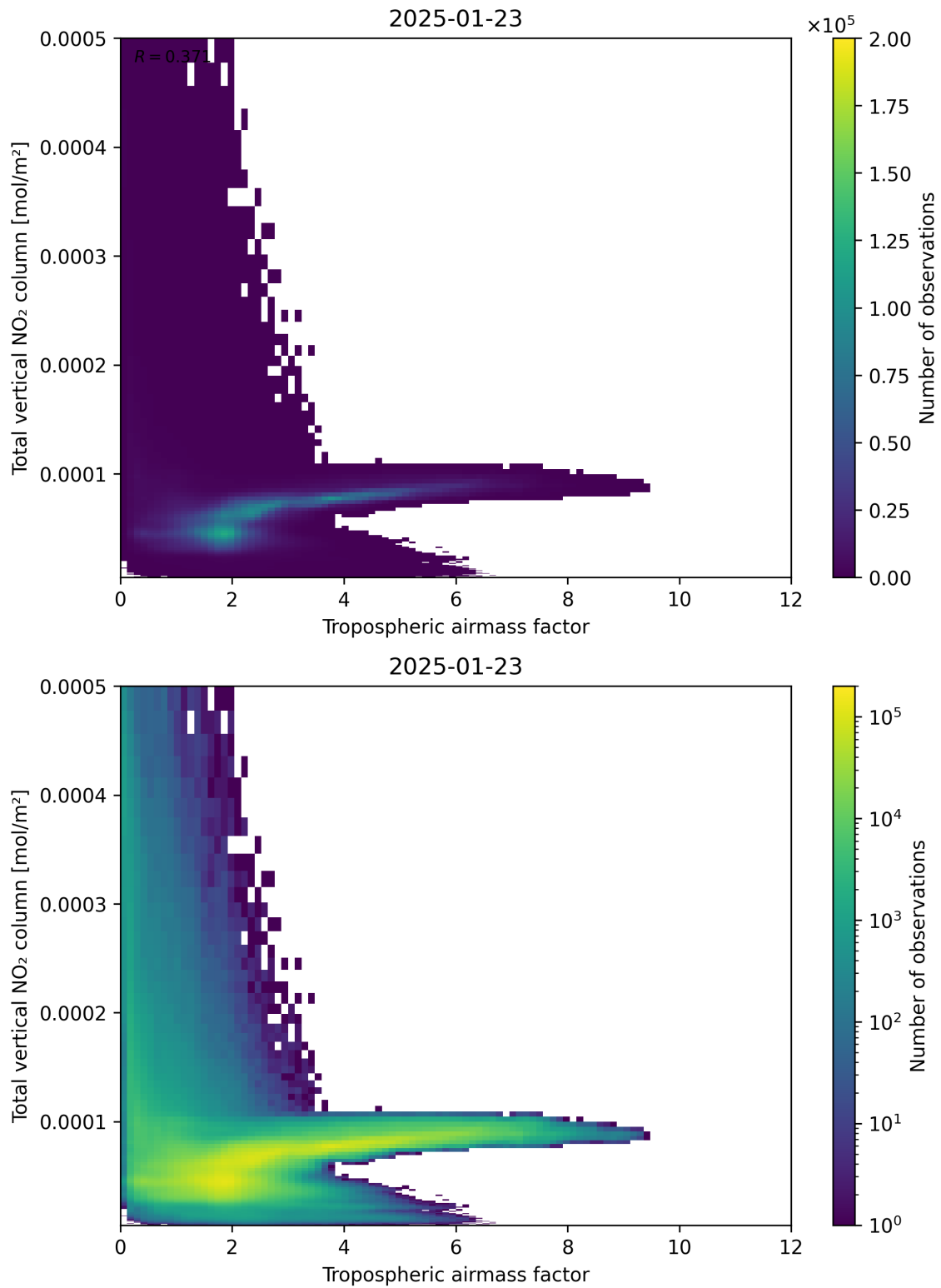
Figure 77: Scatter density plot of “Tropospheric airmass factor” against “Total vertical NO 2 column” for 2025-01-23 to 2025-01-24.
