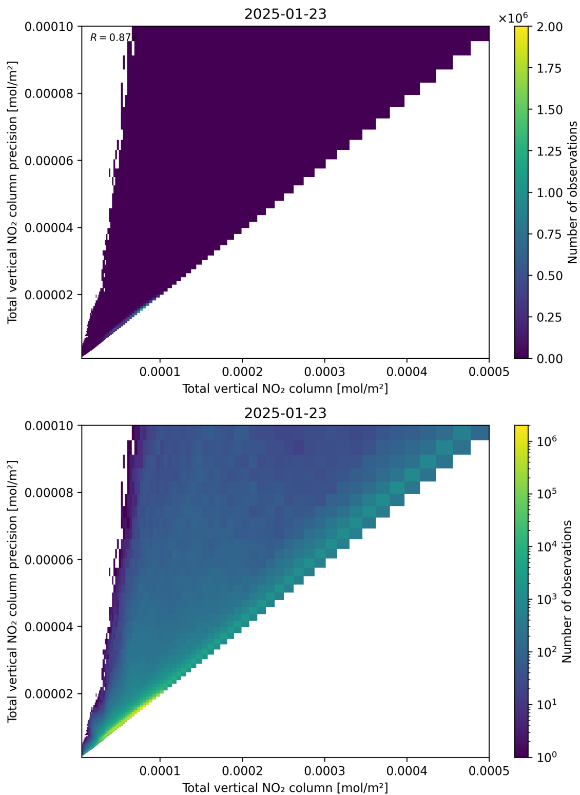
Figure 114: Scatter density plot of “Total vertical NO 2 column” against “Total vertical NO 2 column precision” for 2025-01-23 to 2025-01-24.
