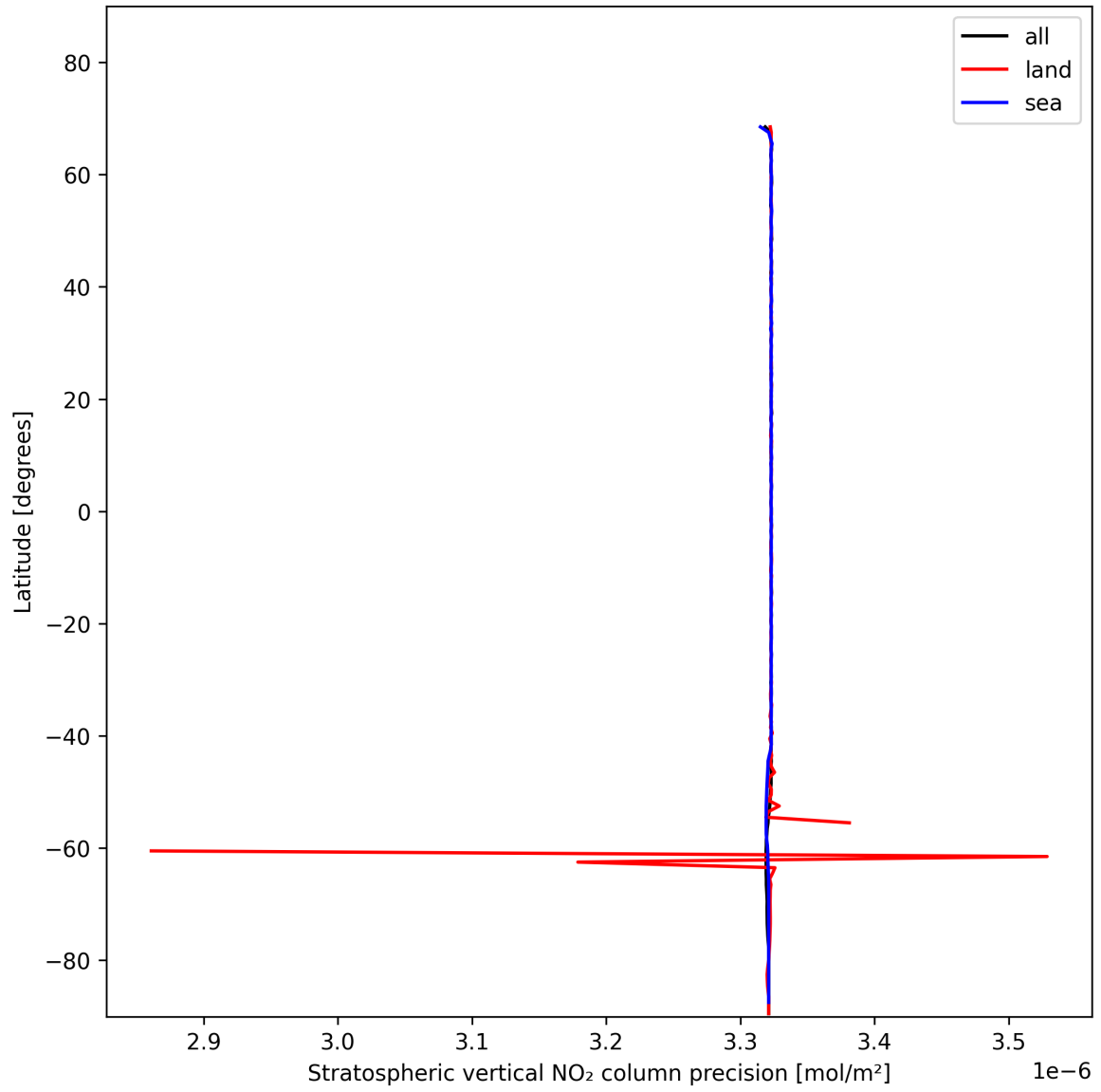
Figure 20: Zonal average of “Stratospheric vertical NO 2 column precision” for 2025-01-23 to 2025-01-24.
