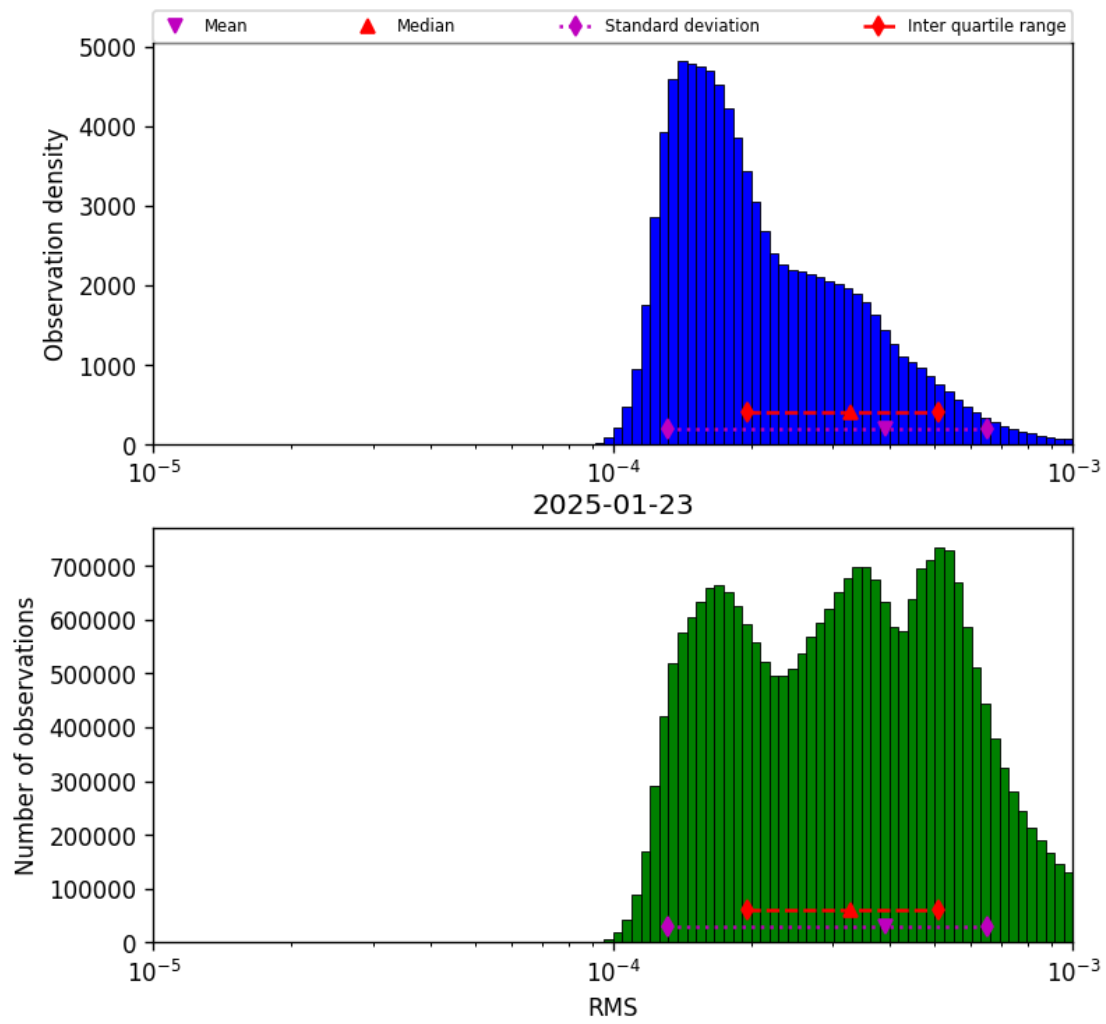
Figure 43: Histogram of “RMS” for 2025-01-23 to 2025-01-24
