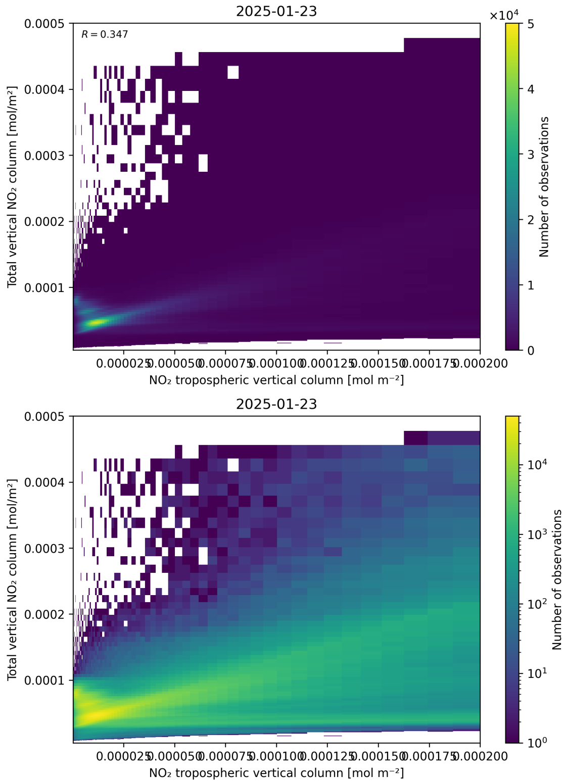
Figure 128: Scatter density plot of “NO 2 tropospheric vertical column” against “Total vertical NO 2 column” for 2025-01-23 to 2025-01-24.
