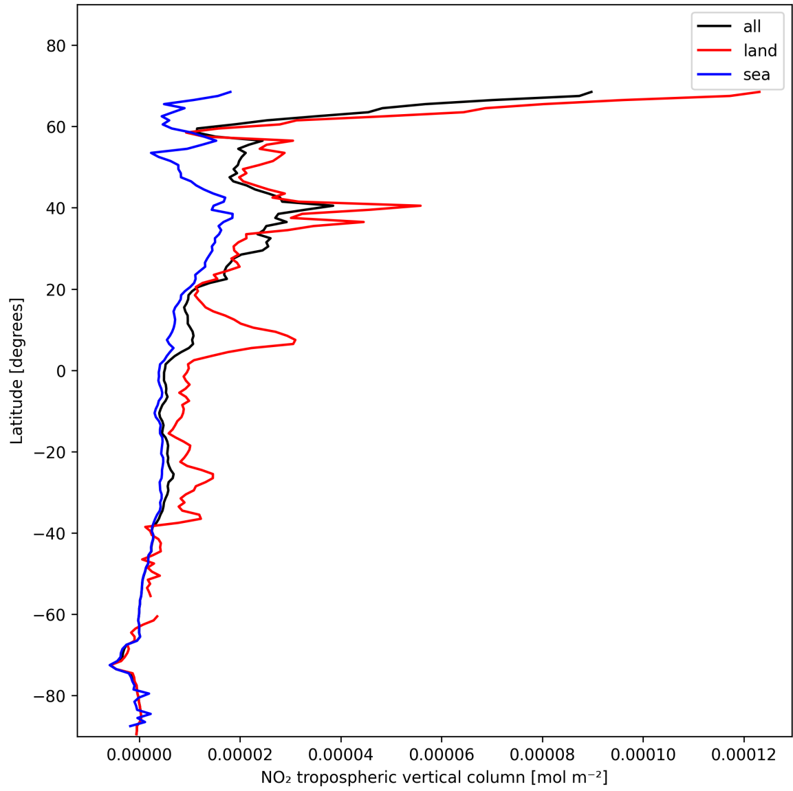
Figure 12: Zonal average of “NO 2 tropospheric vertical column” for 2025-01-23 to 2025-01-24.
