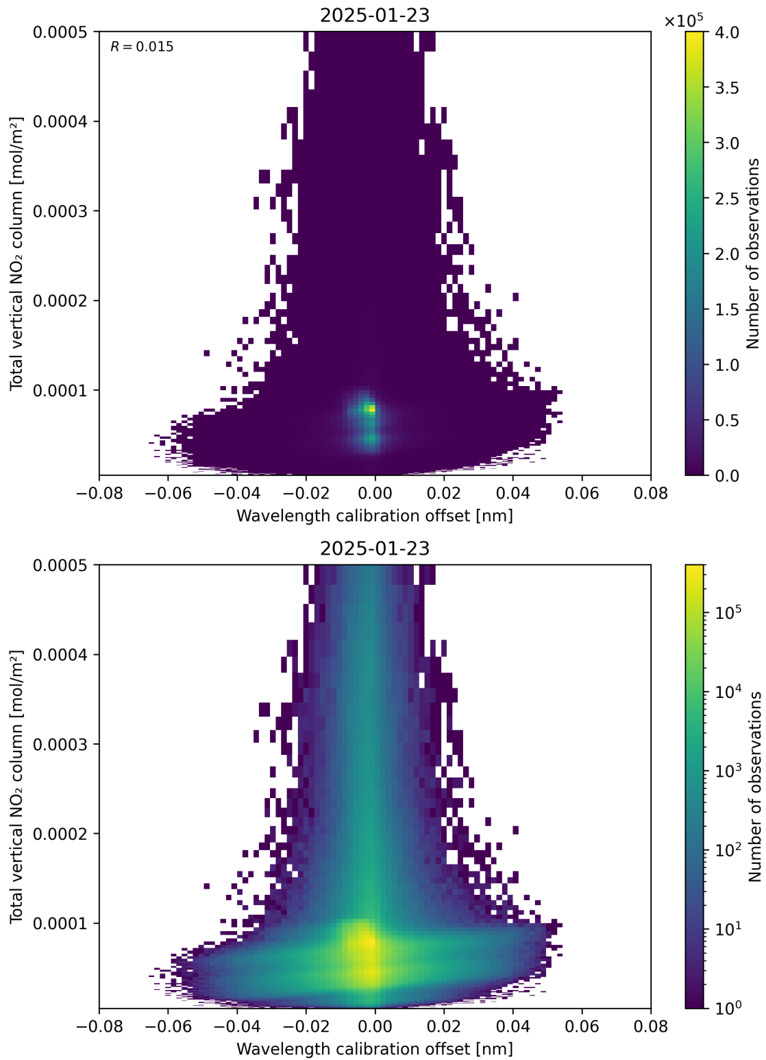
Figure 179: Scatter density plot of “Wavelength calibration offset” against “Total vertical NO 2 column” for 2025-01-23 to 2025-01-24.
