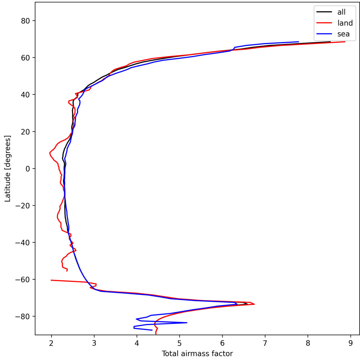
Figure 15: Zonal average of “Total airmass factor” for 2025-01-23 to 2025-01-24.
