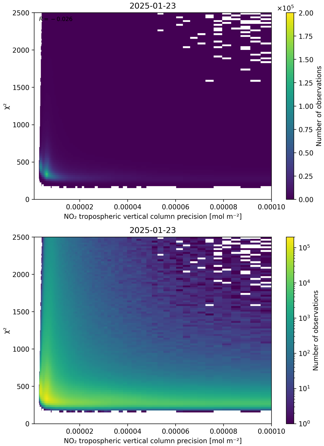
Figure 134: Scatter density plot of “NO 2 tropospheric vertical column precision” against “ \chi^2 ” for 2025-01-23 to 2025-01-24.
