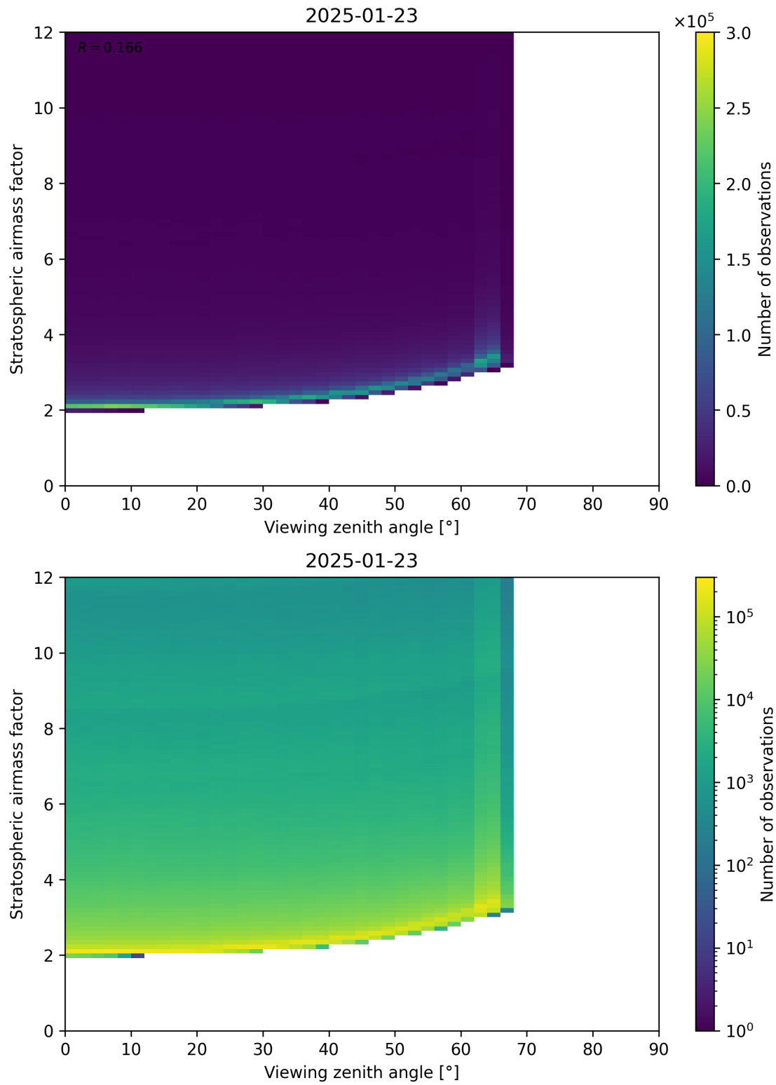
Figure 159: Scatter density plot of “Viewing zenith angle” against “Stratospheric airmass factor” for 2025-01-23 to 2025-01-24.
