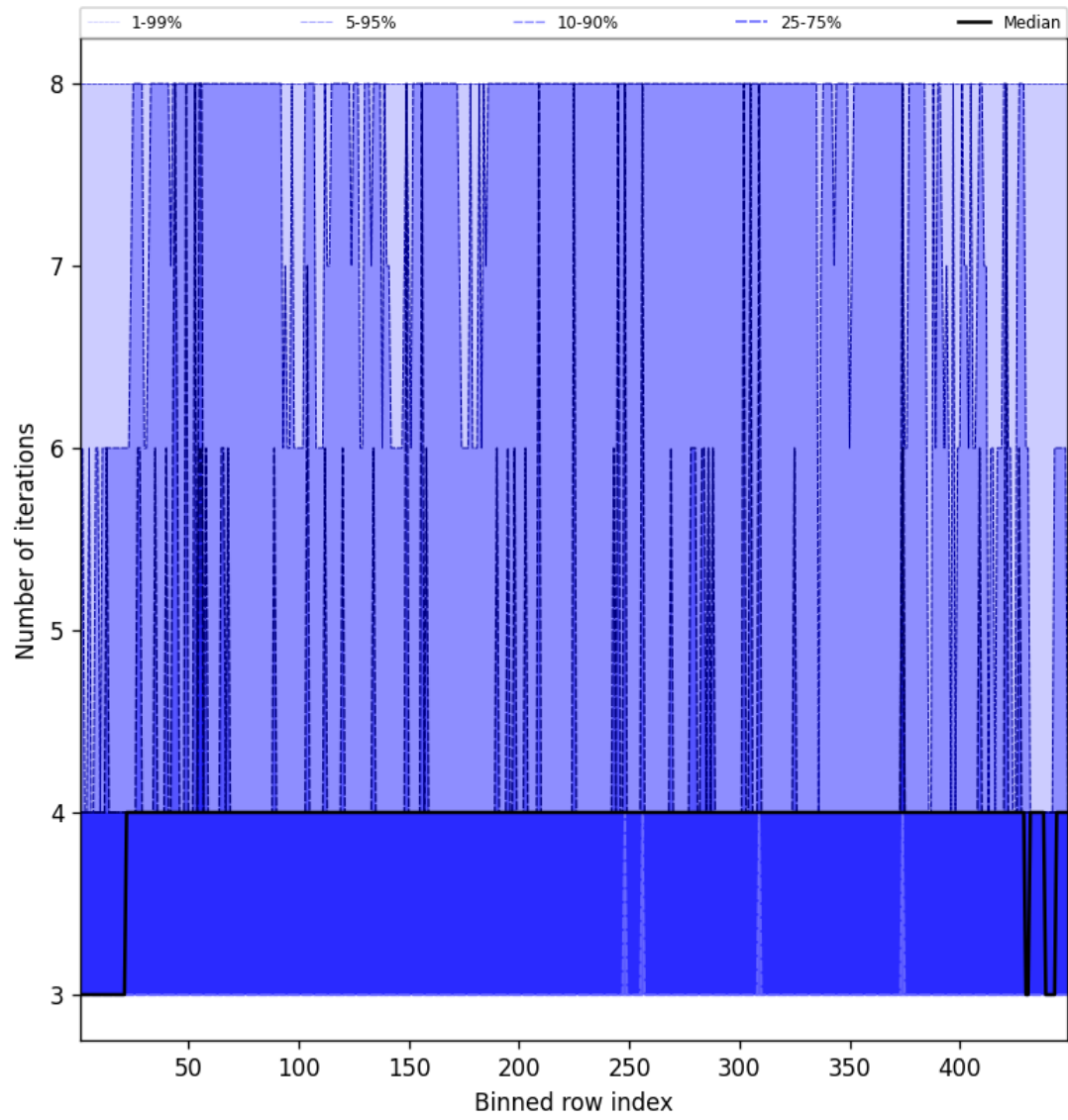
Figure 51: Along track statistics of “Number of iterations” for 2025-01-23 to 2025-01-24
