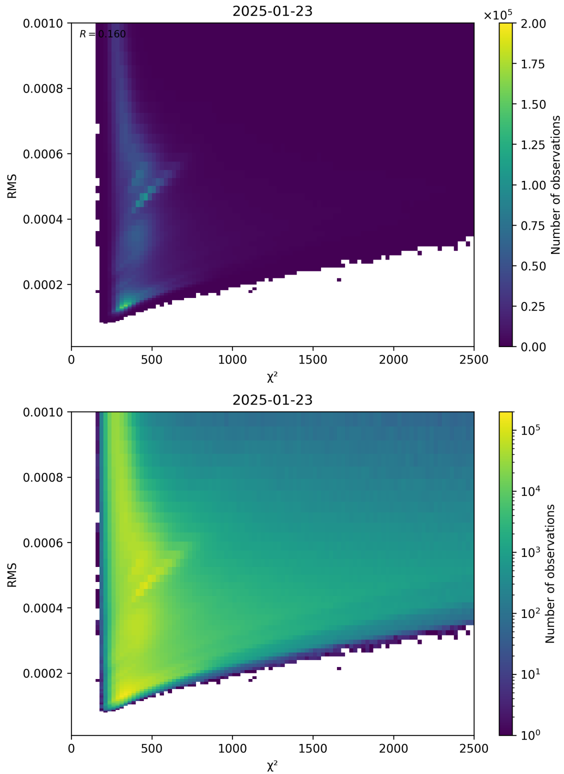
Figure 82: Scatter density plot of “ \chi^2 ” against “RMS” for 2025-01-23 to 2025-01-24.
