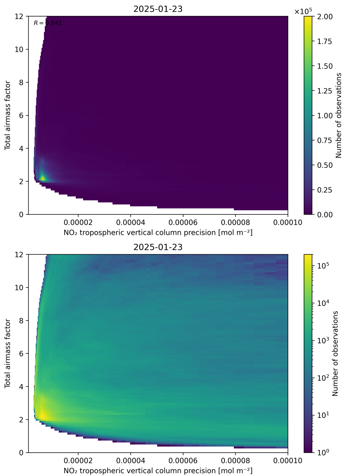
Figure 132: Scatter density plot of “NO 2 tropospheric vertical column precision” against “Total air mass factor” for 2025-01-23 to 2025-01-24.
