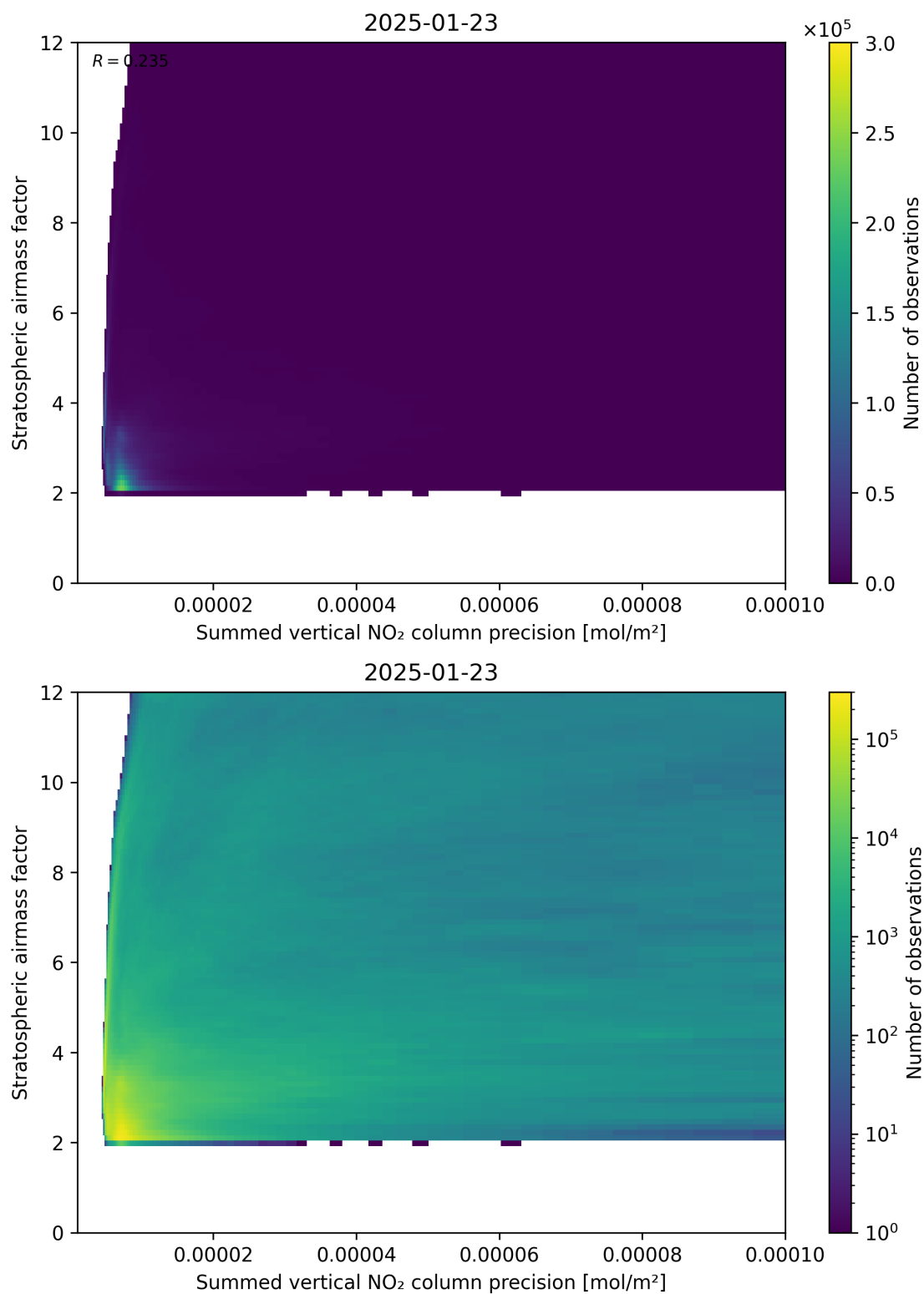
Figure 106: Scatter density plot of “Summed vertical NO 2 column precision” against “Stratospheric airmass factor” for 2025-01-23 to 2025-01-24.
