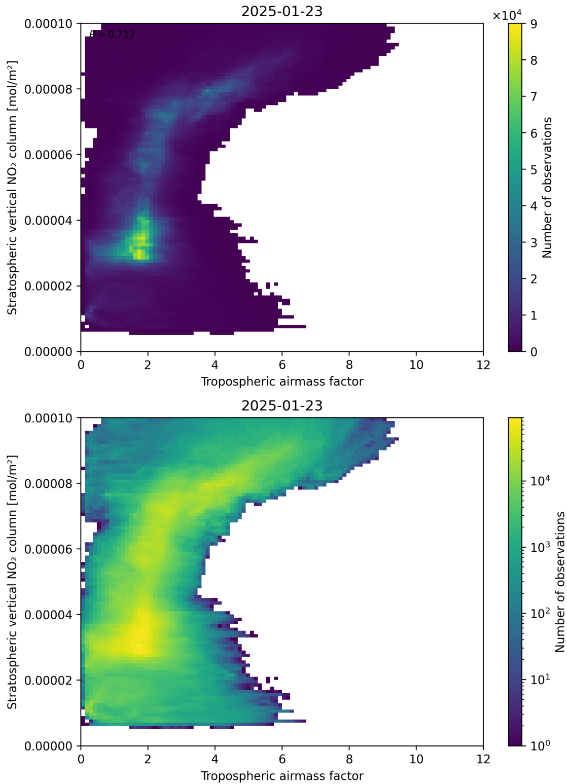
Figure 74: Scatter density plot of “Tropospheric air mass factor” against “Stratospheric vertical NO 2 column” for 2025-01-23 to 2025-01-24.
