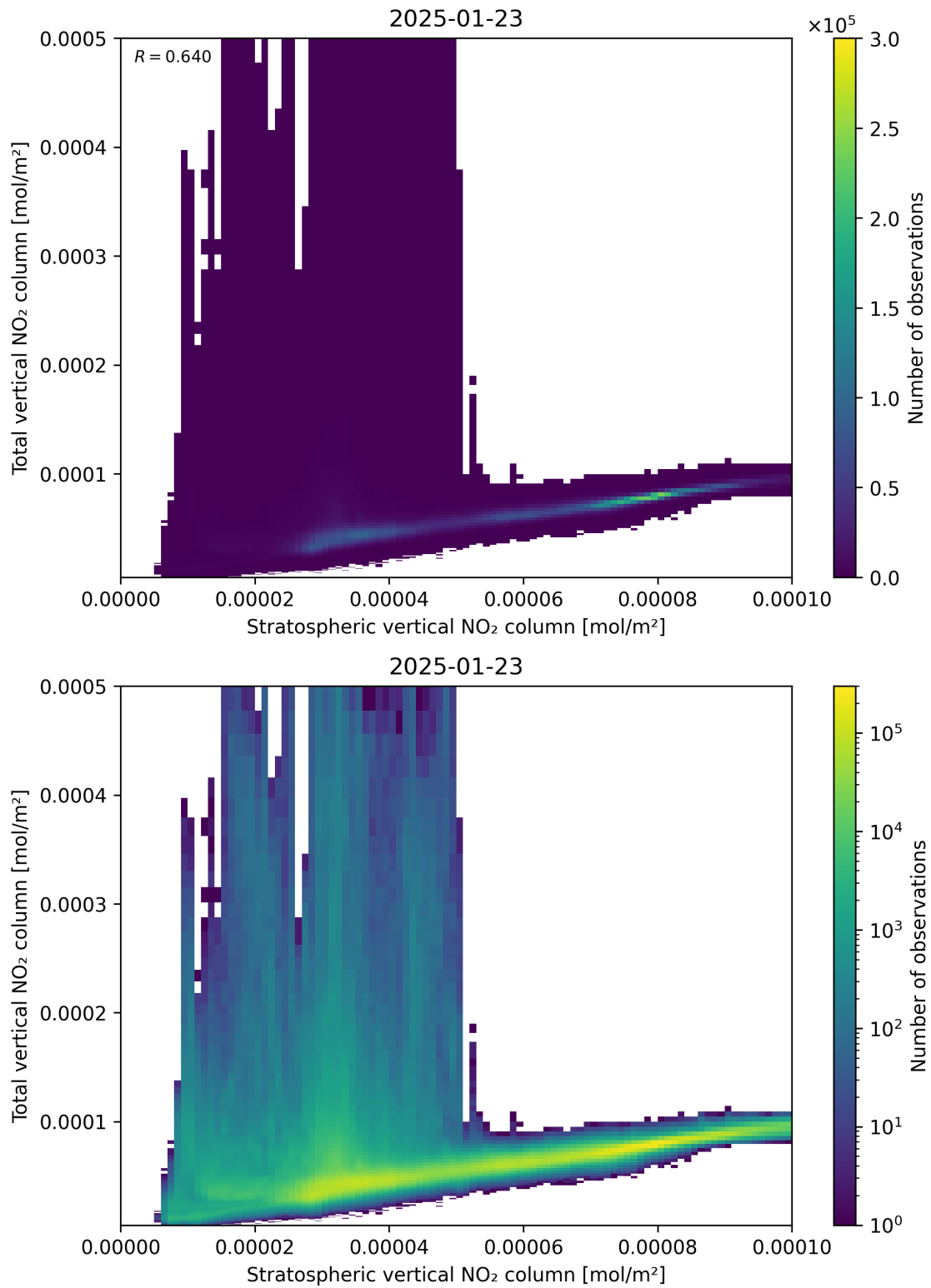
Figure 100: Scatter density plot of “Stratospheric vertical NO 2 column” against “Total vertical NO 2 column” for 2025-01-23 to 2025-01-24.
