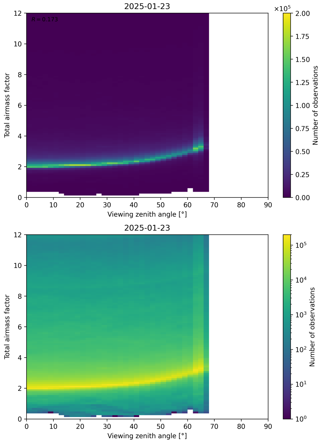
Figure 160: Scatter density plot of “Viewing zenith angle” against “Total airmass factor” for 2025-01-23 to 2025-01-24.
