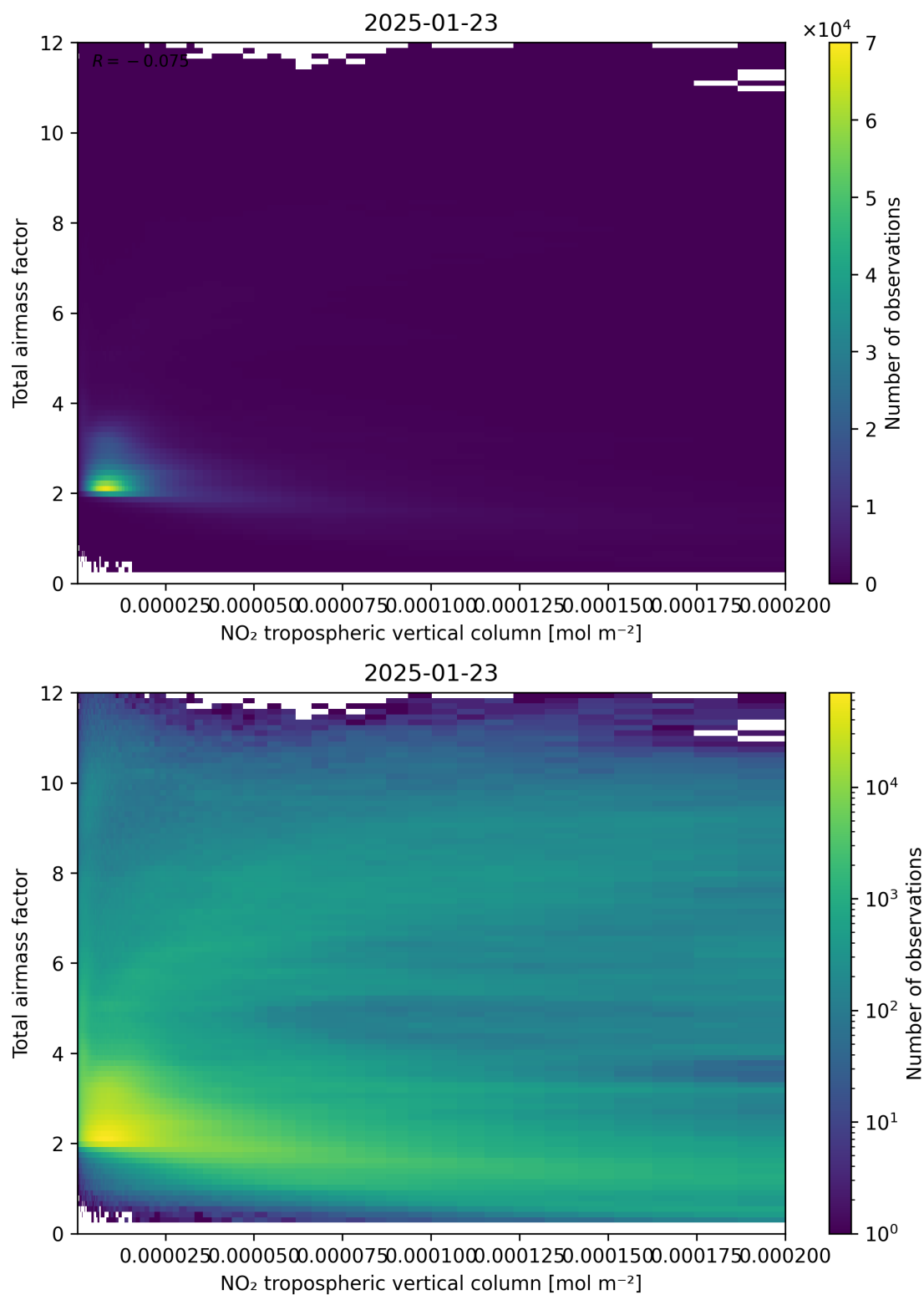
Figure 122: Scatter density plot of “NO 2 tropospheric vertical column” against “Total air mass factor” for 2025-01-23 to 2025-01-24.
