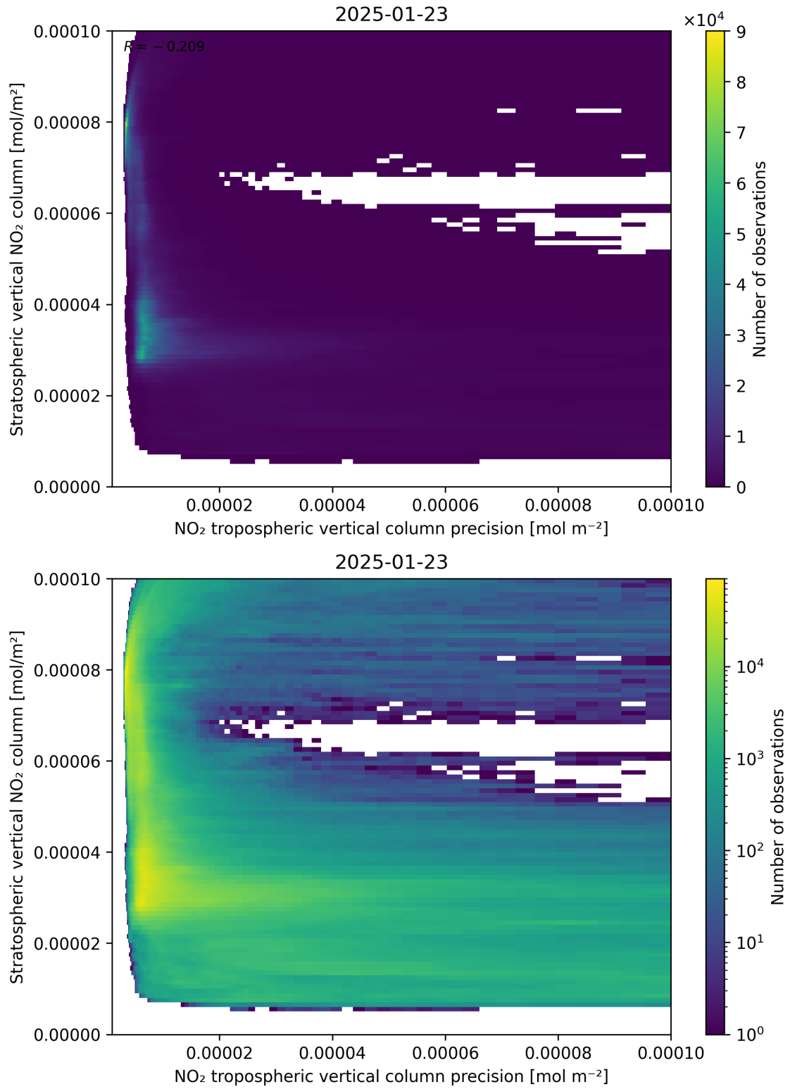
Figure 135: Scatter density plot of “NO 2 tropospheric vertical column precision” against “Stratospheric vertical NO 2 column” for 2025-01-23 to 2025-01-24.
