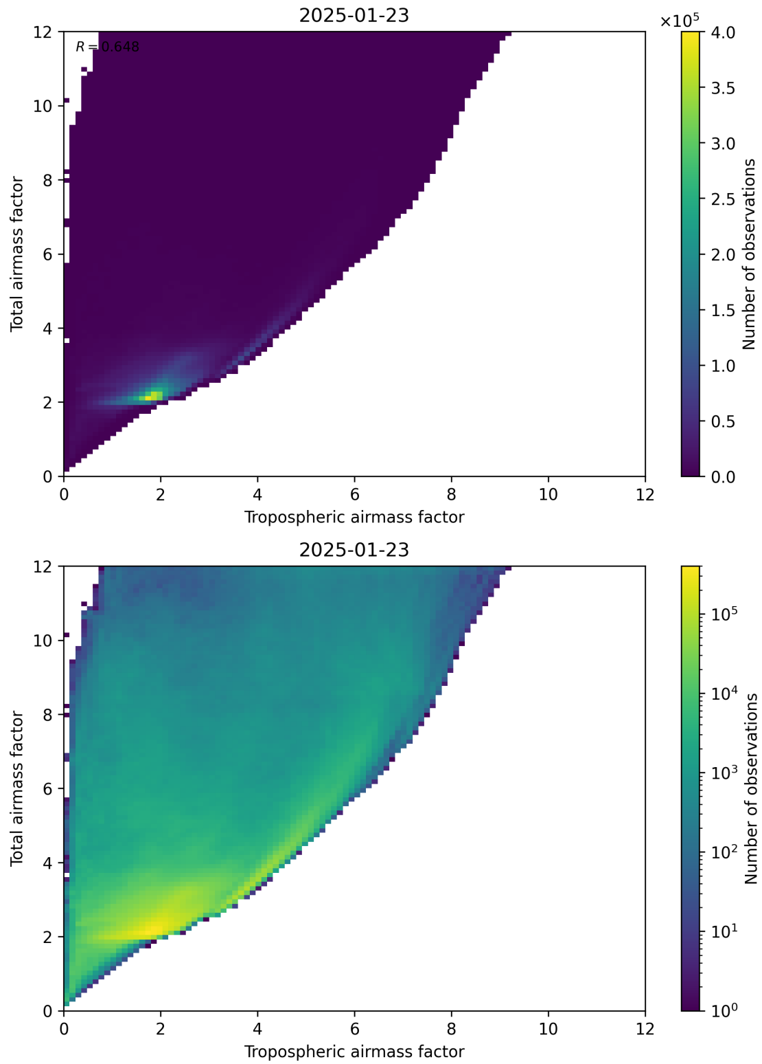
Figure 72: Scatter density plot of “Tropospheric airmass factor” against “Total airmass factor” for 2025-01-23 to 2025-01-24.
