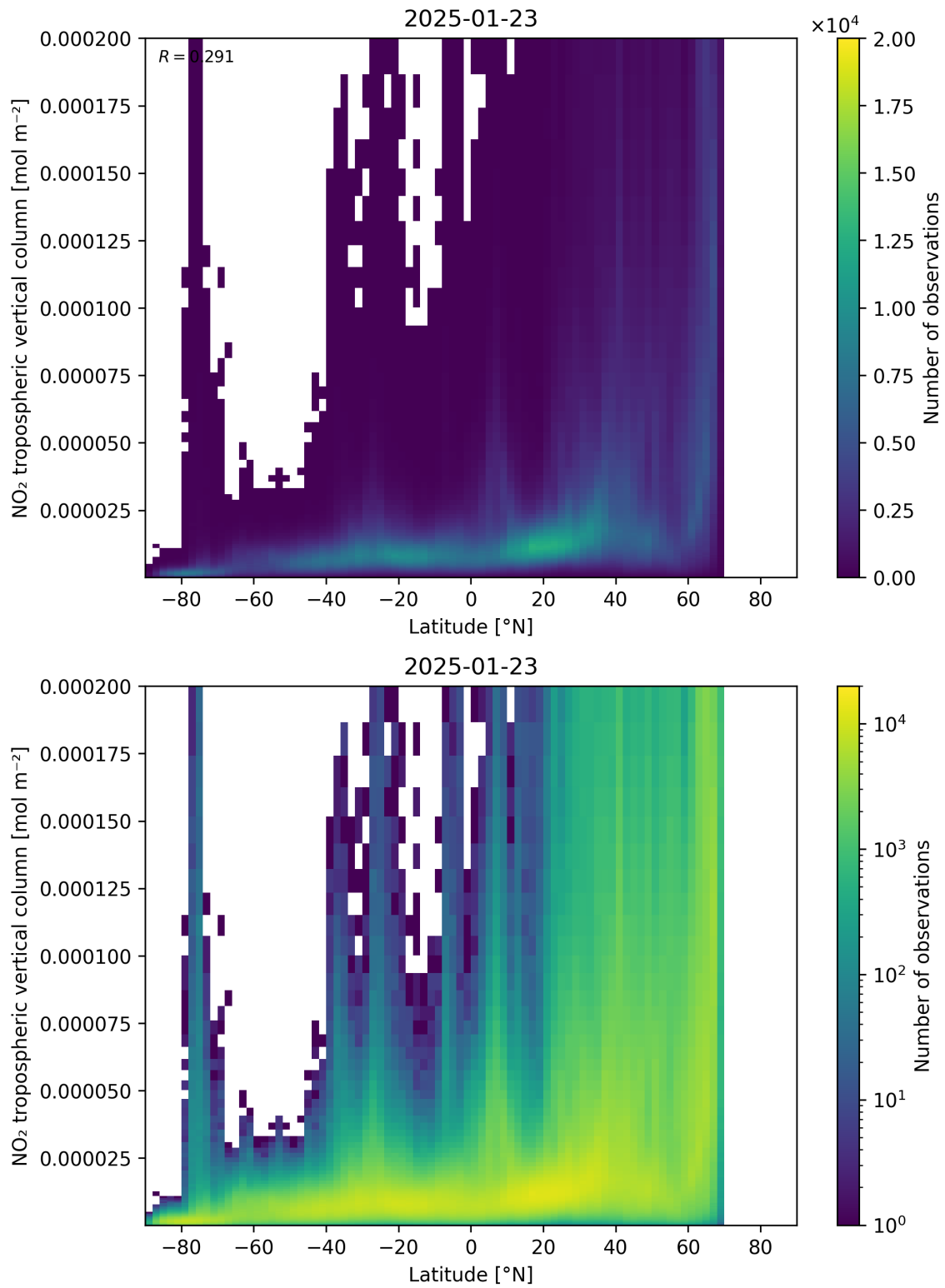
Figure 92: Scatter density plot of “Latitude” against “NO 2 tropospheric vertical column” for 2025-01-23 to 2025-01-24.
