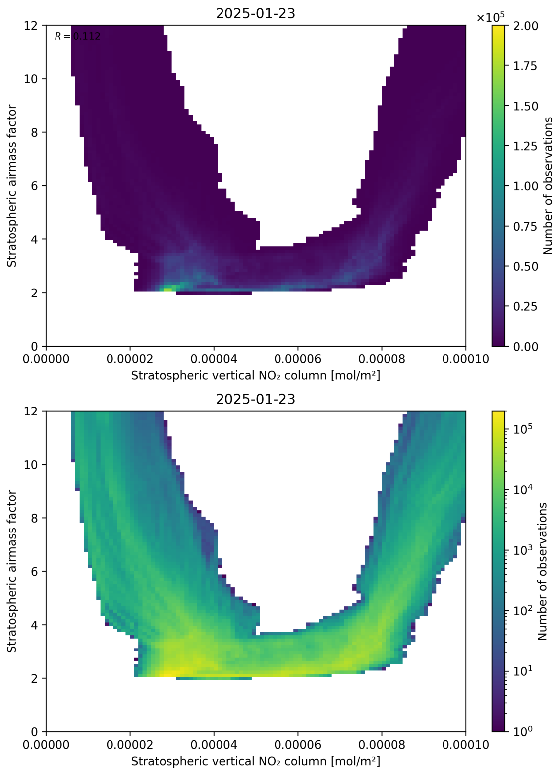
Figure 96: Scatter density plot of “Stratospheric vertical NO 2 column” against “Stratospheric airmass factor” for 2025-01-23 to 2025-01-24.
