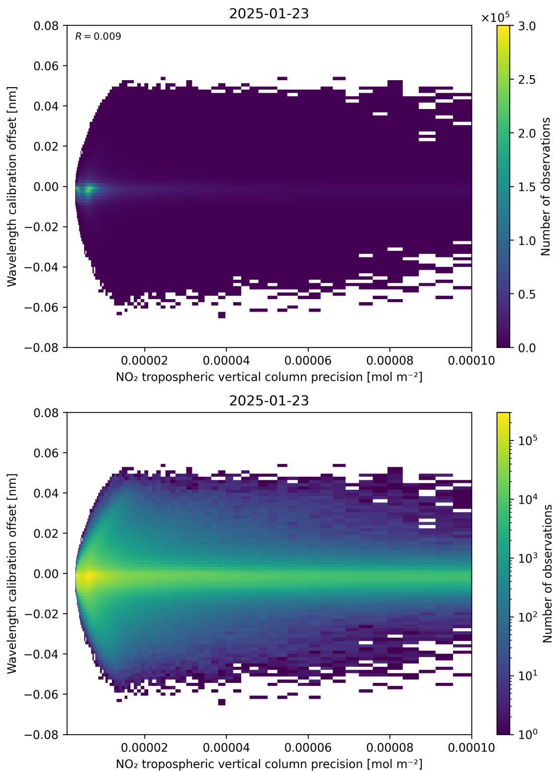
Figure 141: Scatter density plot of “NO 2 tropospheric vertical column precision” against “Wavelength calibration offset” for 2025-01-23 to 2025-01-24.
