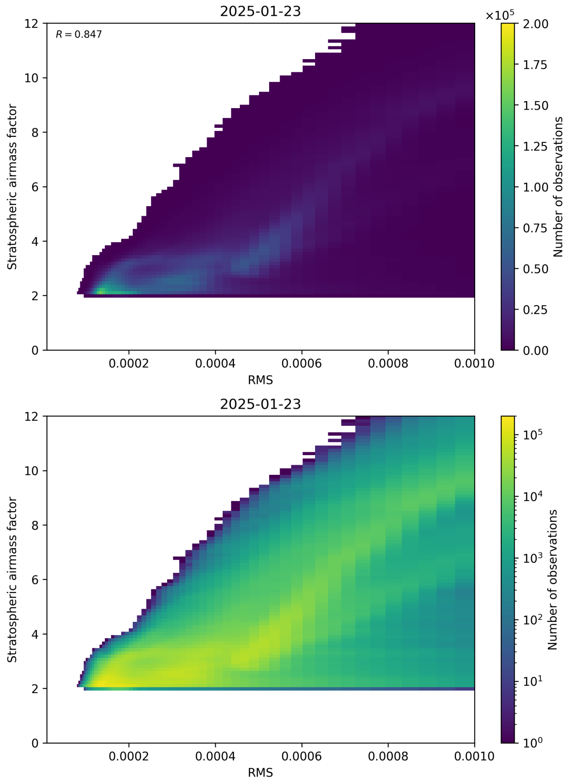
Figure 144: Scatter density plot of “RMS” against “Stratospheric airmass factor” for 2025-01-23 to 2025-01-24.
