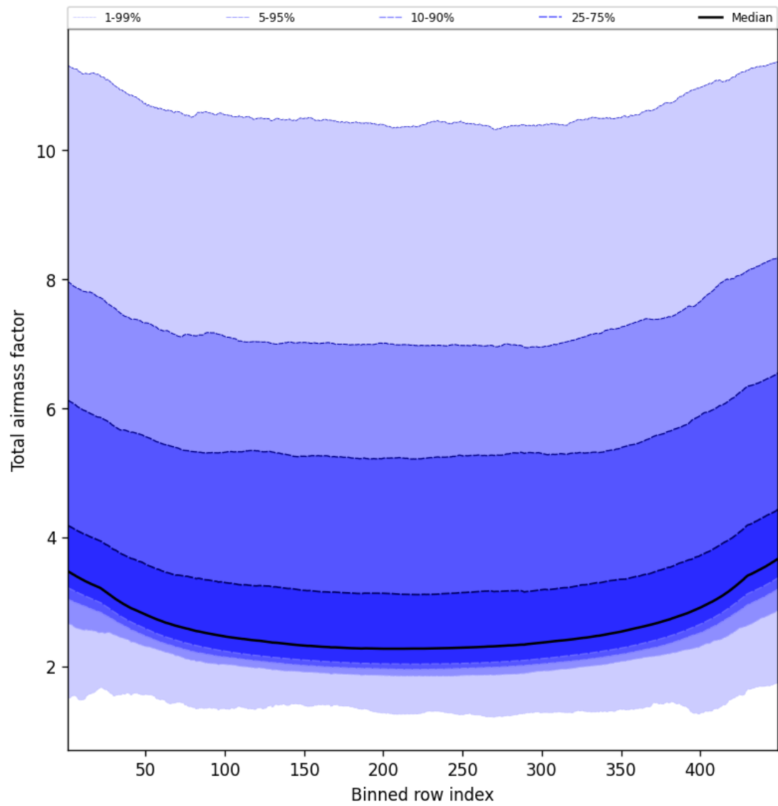
Figure 49: Along track statistics of “Total airmass factor” for 2025-01-23 to 2025-01-24
