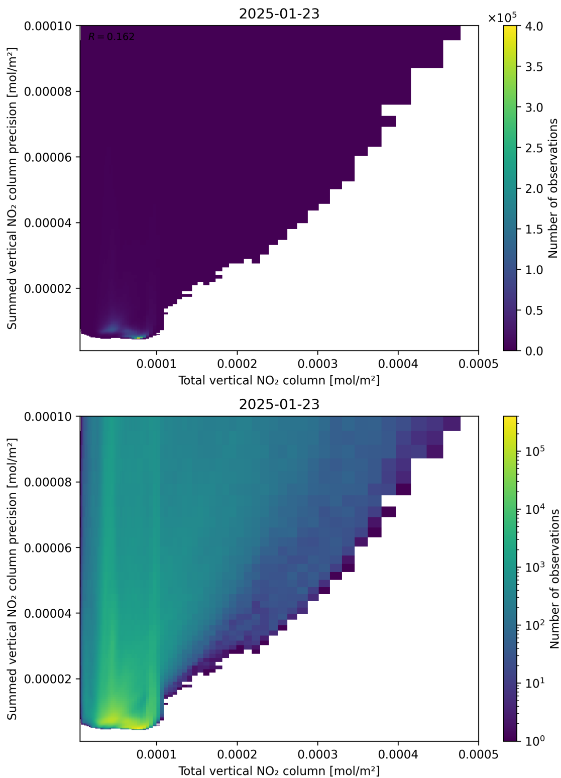
Figure 113: Scatter density plot of “Total vertical NO 2 column” against “Summed vertical NO 2 column precision” for 2025-01-23 to 2025-01-24.
