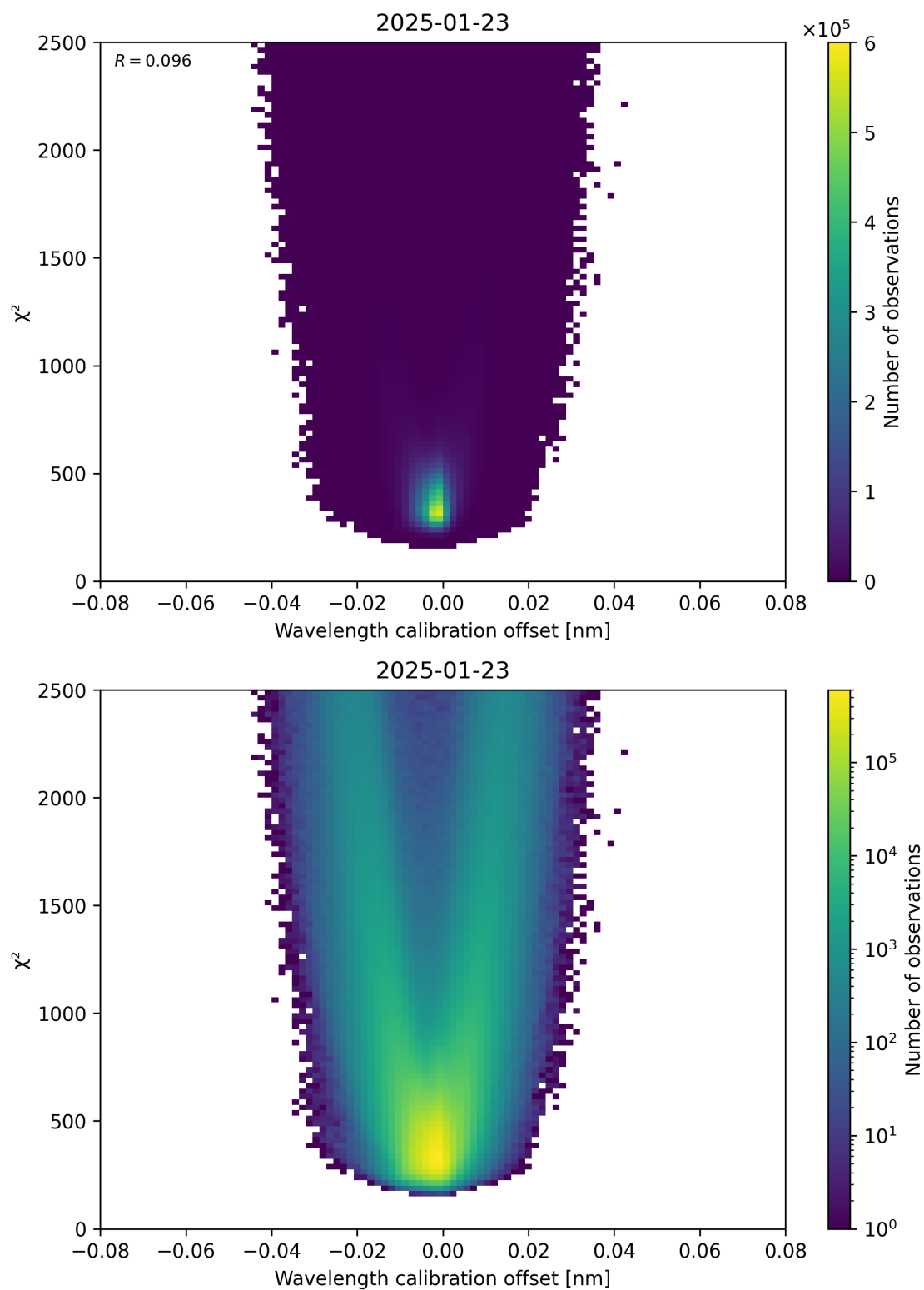
Figure 175: Scatter density plot of “Wavelength calibration offset” against “ \chi^2 ” for 2025-01-23 to 2025-01-24.
