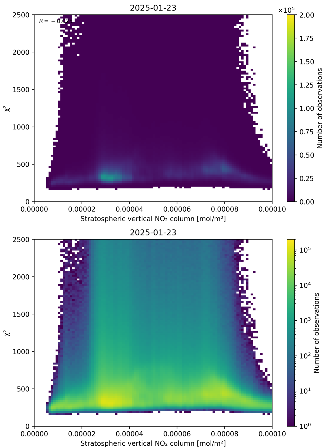
Figure 97: Scatter density plot of “Stratospheric vertical NO 2 column” against “ \chi^2 ” for 2025-01-23 to 2025-01-24.
