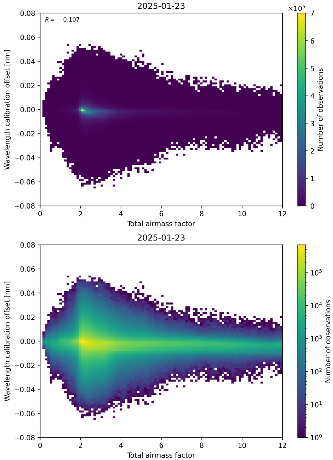
Figure 70: Scatter density plot of “Total airmass factor” against “Wavelength calibration offset” for 2025-01-23 to 2025-01-24.
