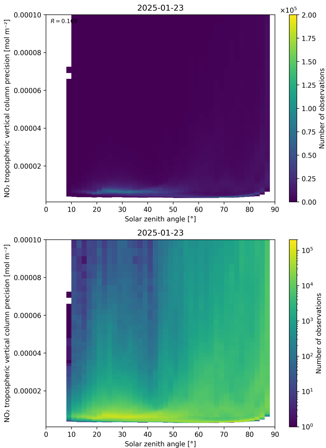
Figure 156: Scatter density plot of “Solar zenith angle” against “NO 2 tropospheric vertical column precision” for 2025-01-23 to 2025-01-24.
