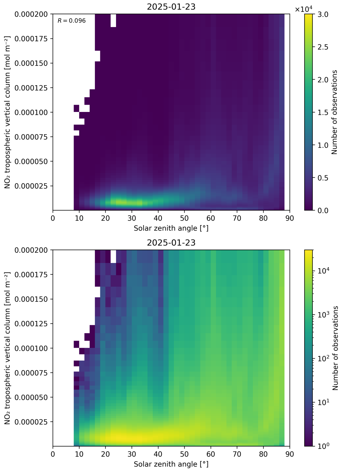
Figure 155: Scatter density plot of “Solar zenith angle” against “NO 2 tropospheric vertical column” for 2025-01-23 to 2025-01-24.
