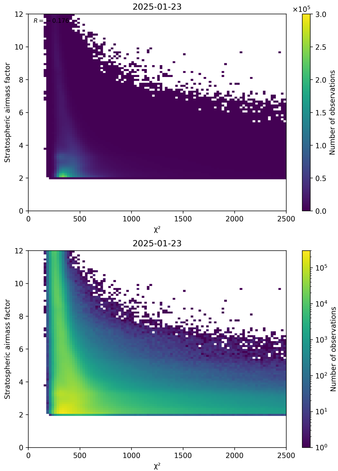
Figure 81: Scatter density plot of “ \chi^2 ” against “Stratospheric airmass factor” for 2025-01-23 to 2025-01-24.
