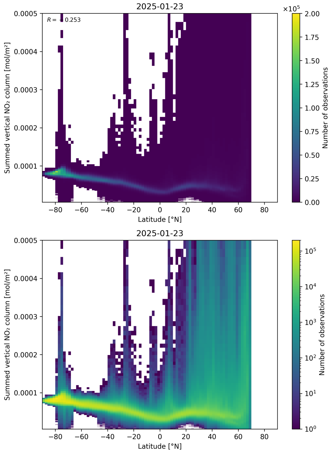
Figure 88: Scatter density plot of “Latitude” against “Summed vertical NO 2 column” for 2025-01-23 to 2025-01-24.
