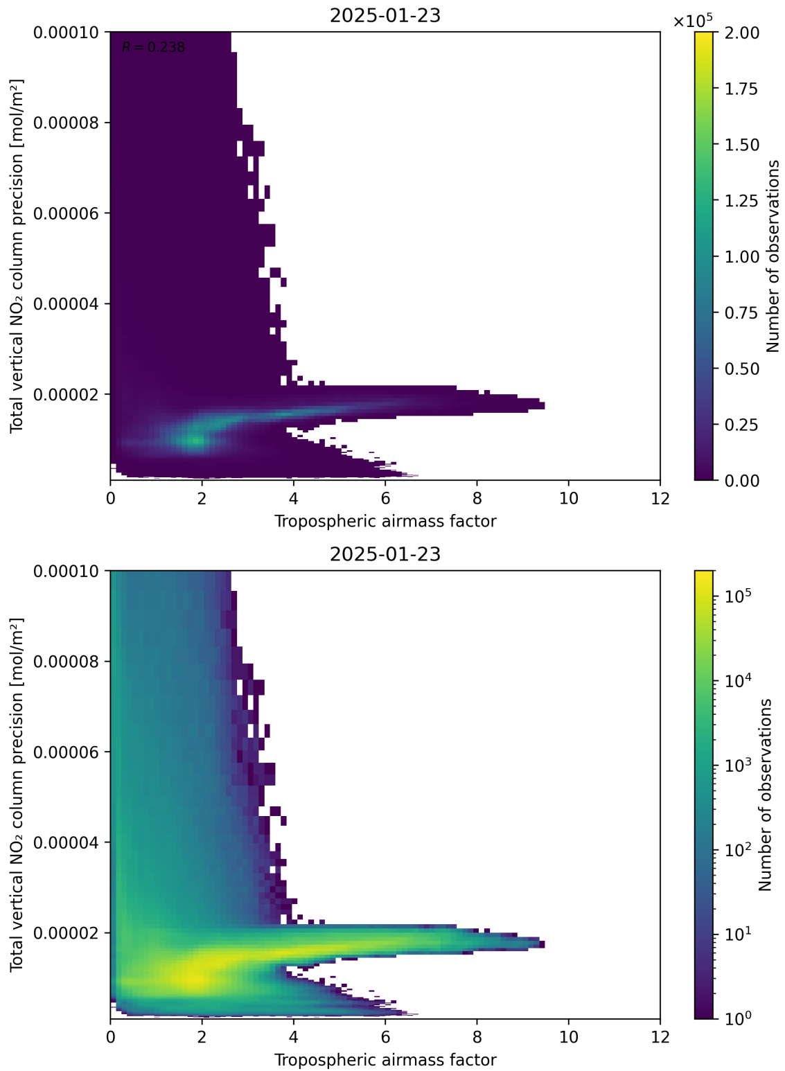
Figure 78: Scatter density plot of “Tropospheric air mass factor” against “Total vertical NO 2 column precision” for 2025-01-23 to 2025-01-24.
