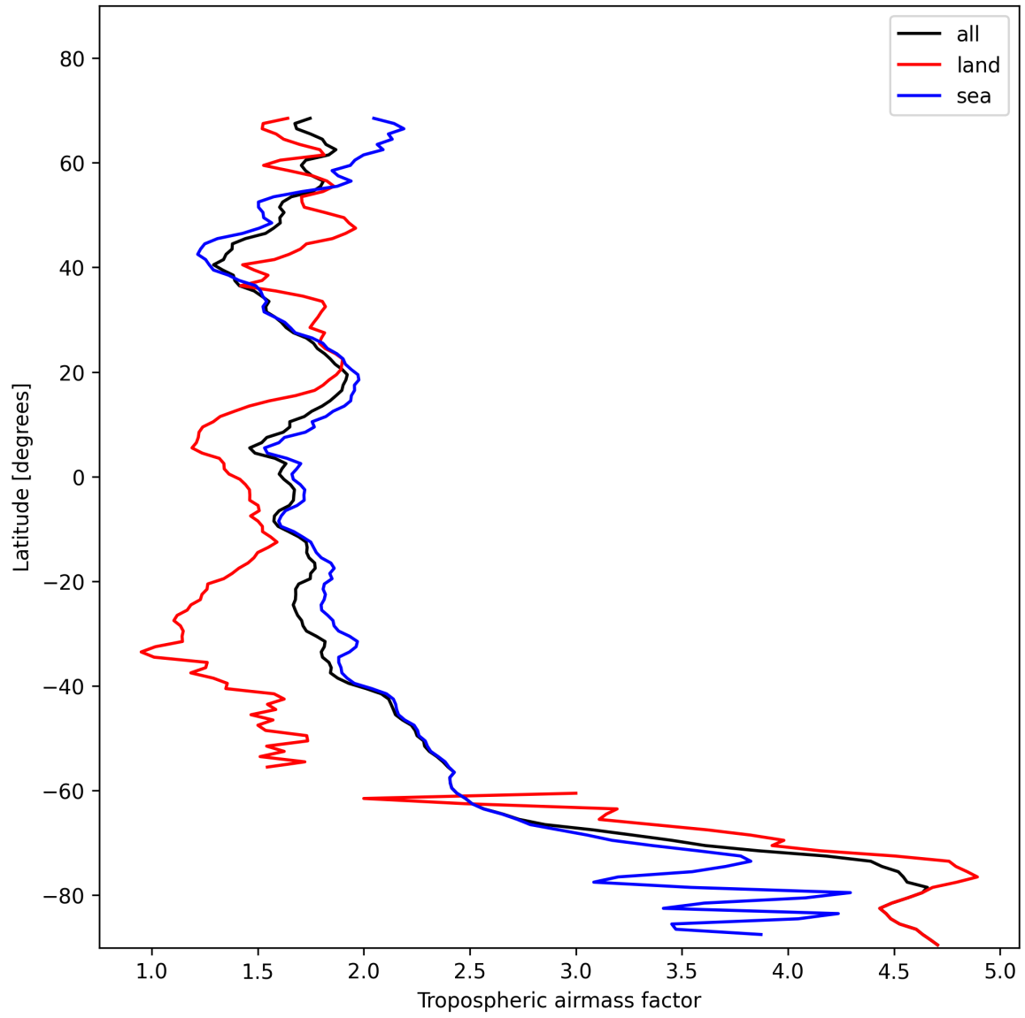
Figure 14: Zonal average of “Tropospheric airmass factor” for 2025-01-23 to 2025-01-24.
