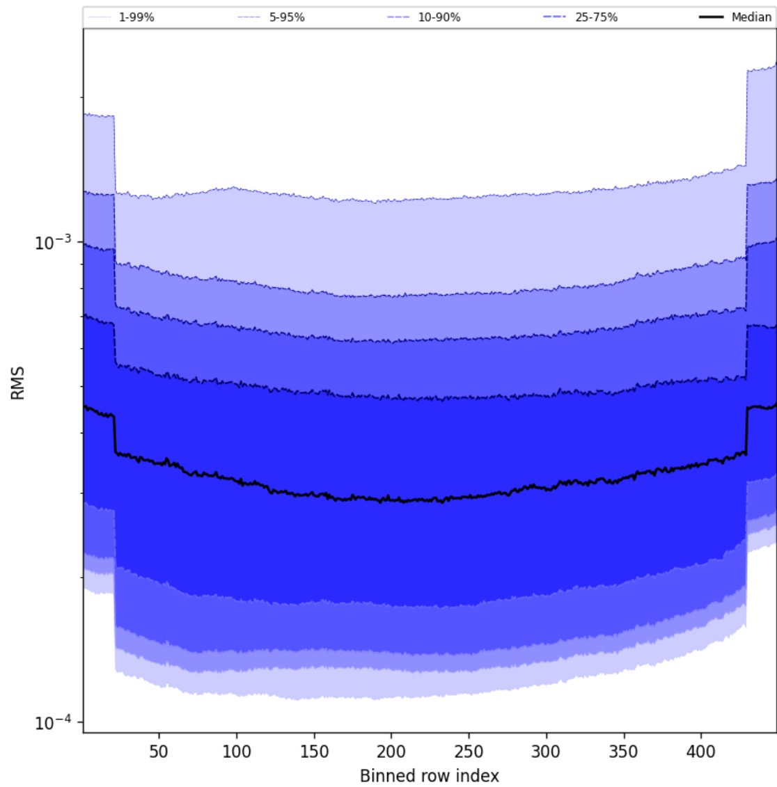
Figure 60: Along track statistics of “RMS” for 2025-01-23 to 2025-01-24
