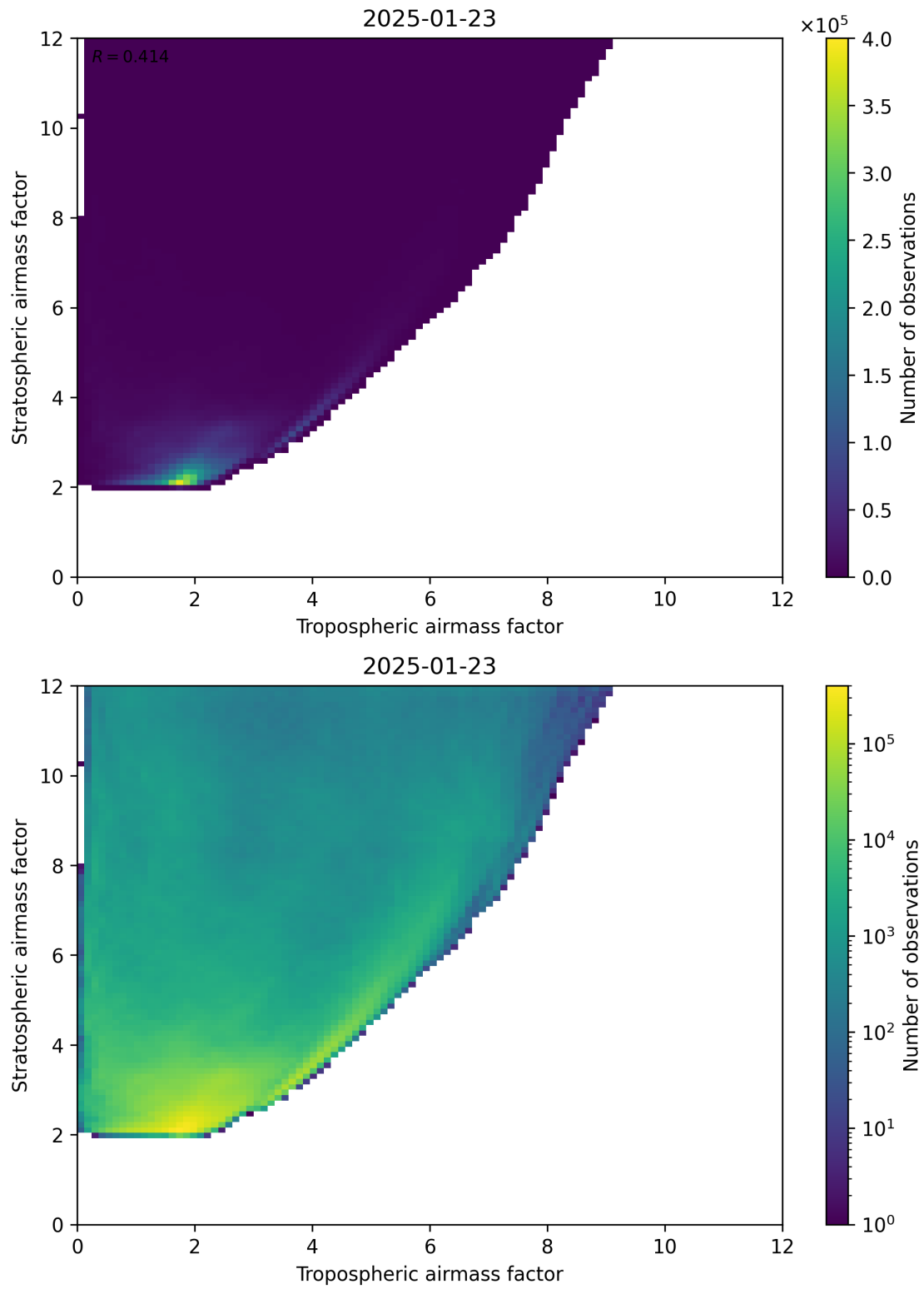
Figure 71: Scatter density plot of “Tropospheric airmass factor” against “Stratospheric airmass factor” for 2025-01-23 to 2025-01-24.
