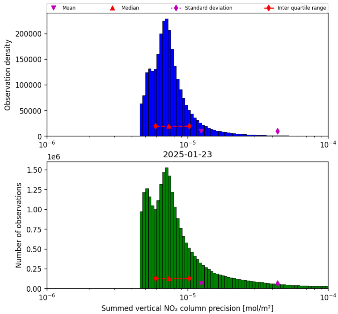
Figure 41: Histogram of “Summed vertical NO 2 column precision” for 2025-01-23 to 2025-01-24
