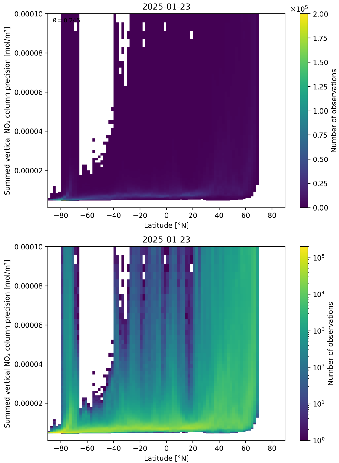
Figure 89: Scatter density plot of “Latitude” against “Summed vertical NO 2 column precision” for 2025-01-23 to 2025-01-24.
