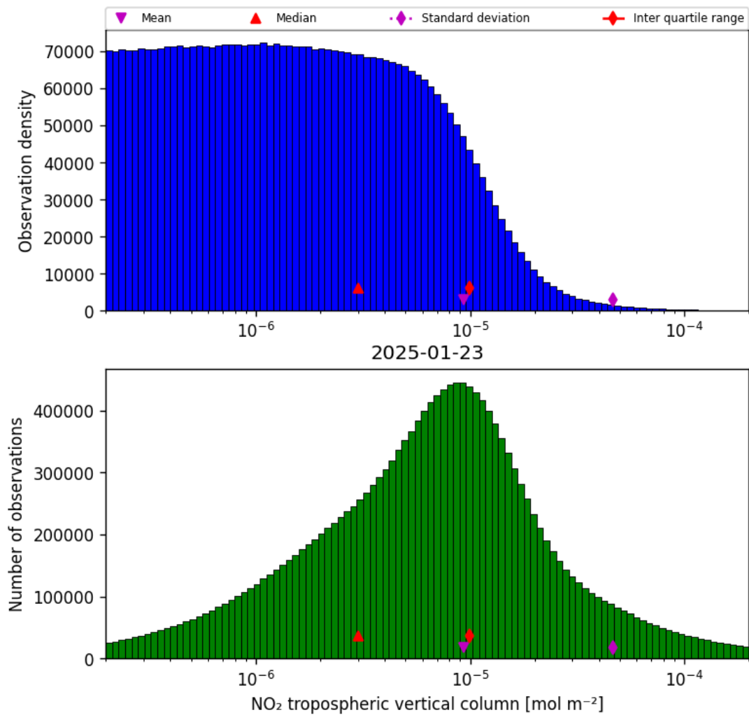
Figure 29: Histogram of “NO 2 tropospheric vertical column” for 2025-01-23 to 2025-01-24
