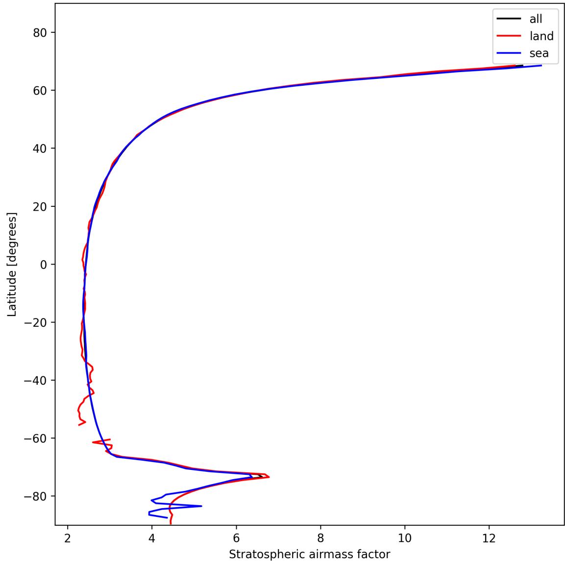
Figure 27: Zonal average of “Stratospheric airmass factor” for 2025-01-23 to 2025-01-24.
