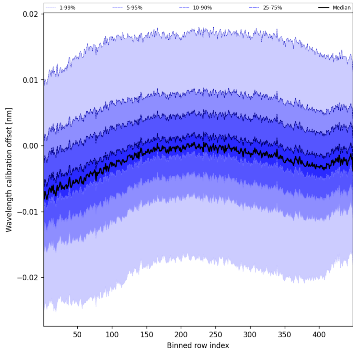
Figure 52: Along track statistics of “Wavelength calibration offset” for 2025-01-23 to 2025-01-24
