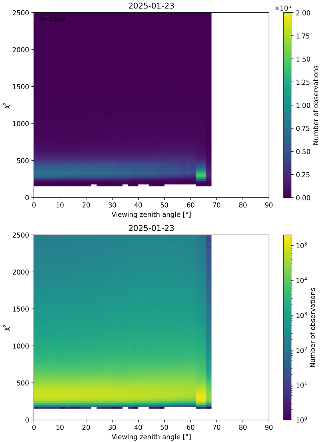
Figure 162: Scatter density plot of “Viewing zenith angle” against “ \chi^2 ” for 2025-01-23 to 2025-01-24.
