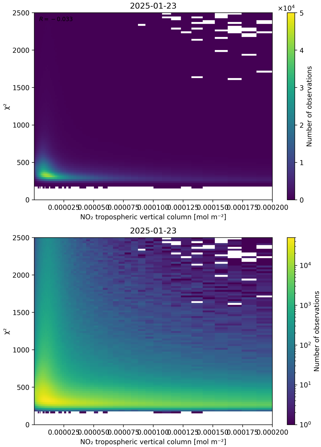
Figure 124: Scatter density plot of “NO 2 tropospheric vertical column” against “ \chi^2 ” for 2025-01-23 to 2025-01-24.
