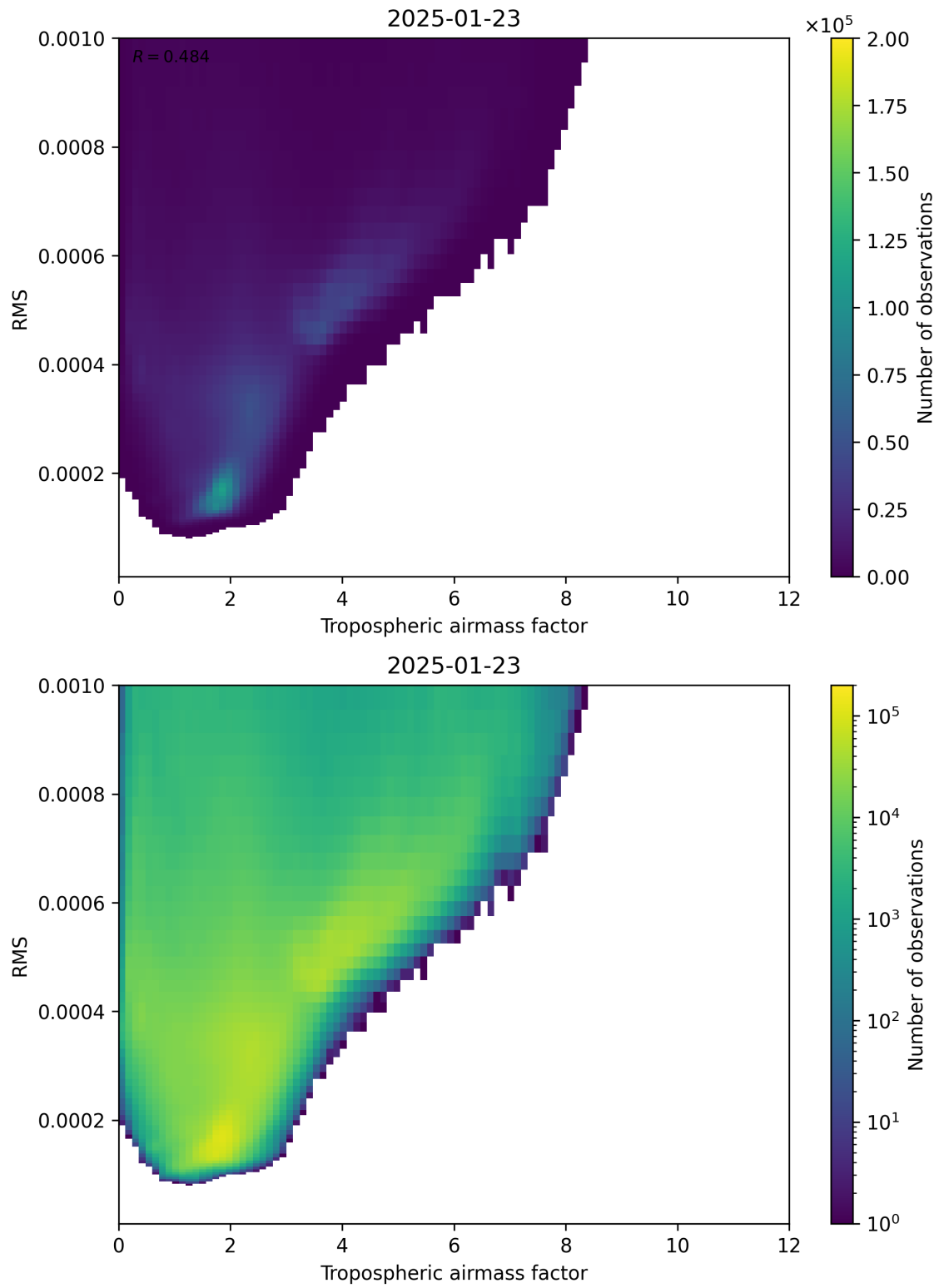
Figure 79: Scatter density plot of “Tropospheric airmass factor” against “RMS” for 2025-01-23 to 2025-01-24.
