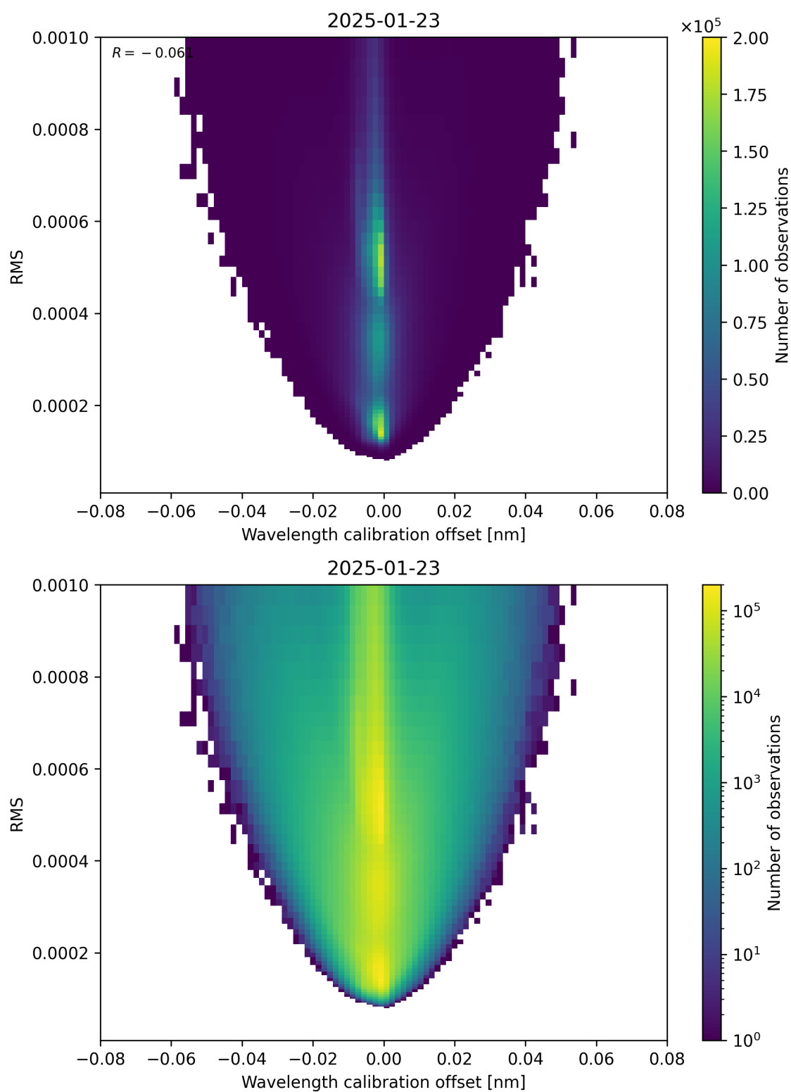
Figure 181: Scatter density plot of “Wavelength calibration offset” against “RMS” for 2025-01-23 to 2025-01-24.
