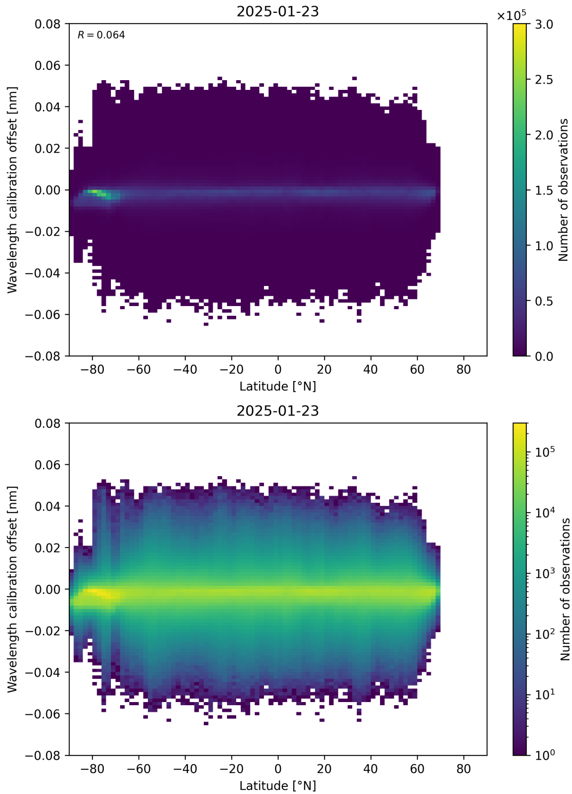
Figure 95: Scatter density plot of “Latitude” against “Wavelength calibration offset” for 2025-01-23 to 2025-01-24.
