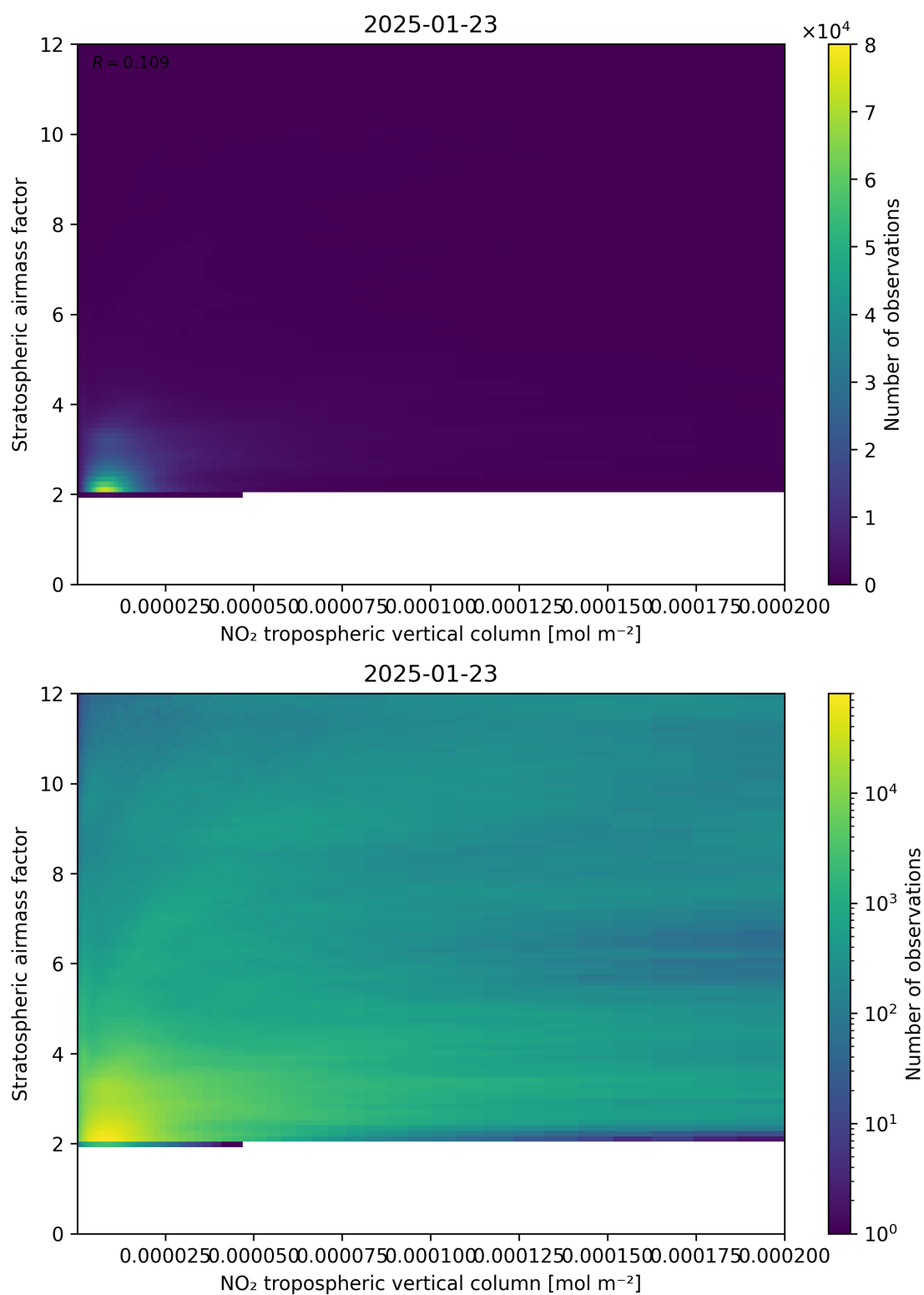
Figure 121: Scatter density plot of “NO 2 tropospheric vertical column” against “Stratospheric airmass factor” for 2025-01-23 to 2025-01-24.
