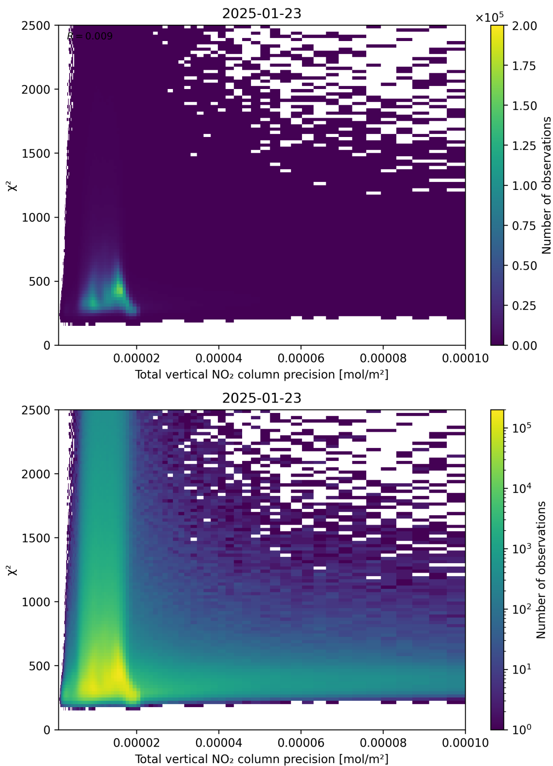
Figure 116: Scatter density plot of “Total vertical NO 2 column precision” against “ \chi^2 ” for 2025-01-23 to 2025-01-24.
