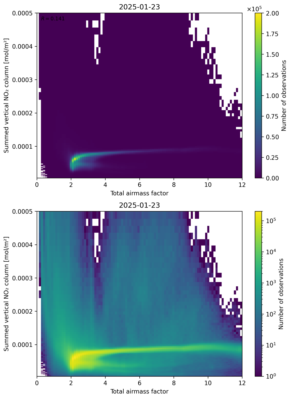
Figure 65: Scatter density plot of “Total airmass factor” against “Summed vertical NO 2 column” for 2025-01-23 to 2025-01-24.
