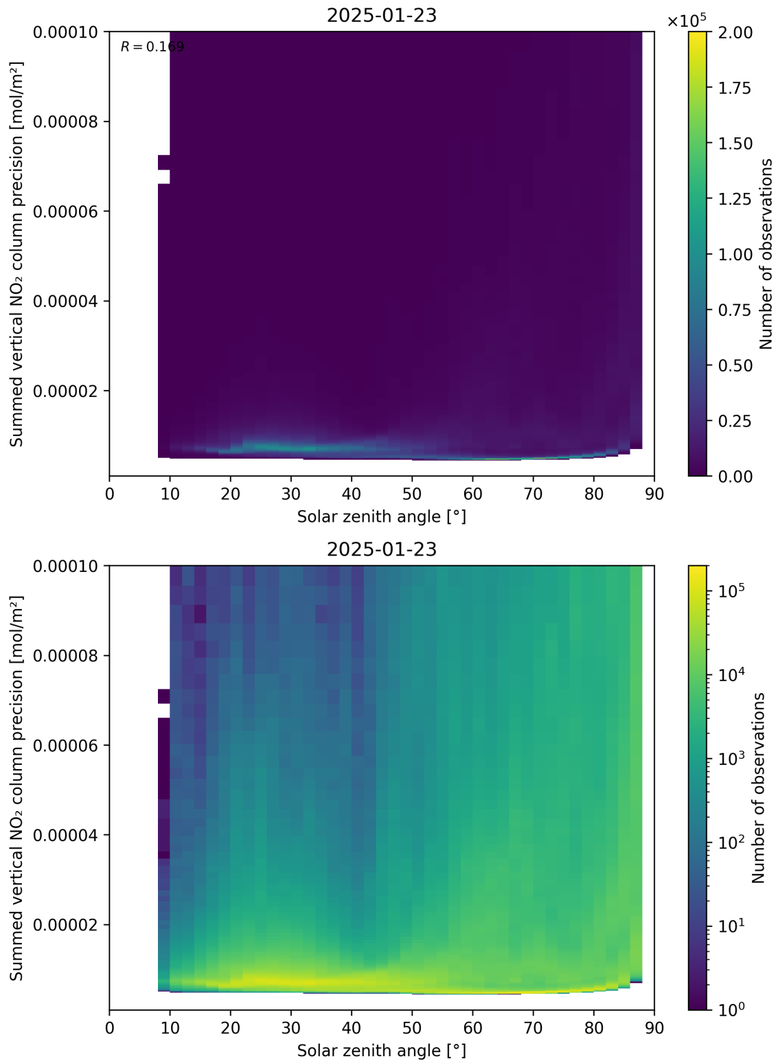
Figure 152: Scatter density plot of “Solar zenith angle” against “Summed vertical NO 2 column precision” for 2025-01-23 to 2025-01-24.
