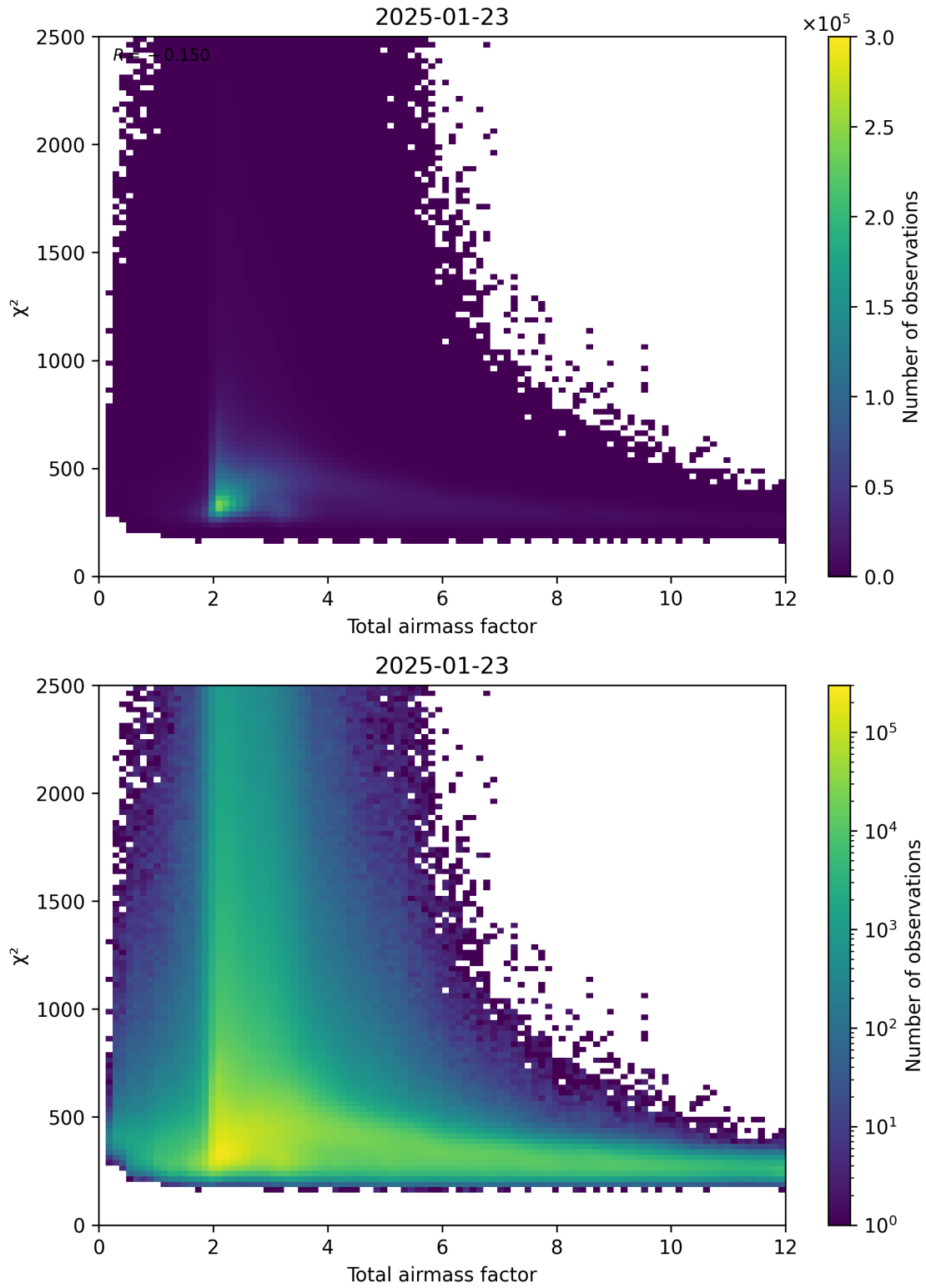
Figure 63: Scatter density plot of “Total airmass factor” against “ \chi^2 ” for 2025-01-23 to 2025-01-24.
