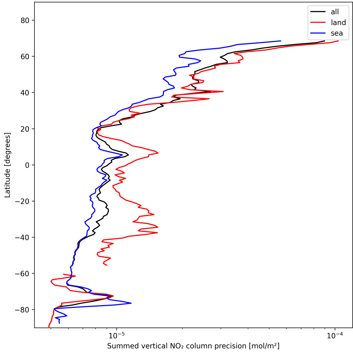
Figure 24: Zonal average of “Summed vertical NO 2 column precision” for 2025-01-23 to 2025-01-24.
