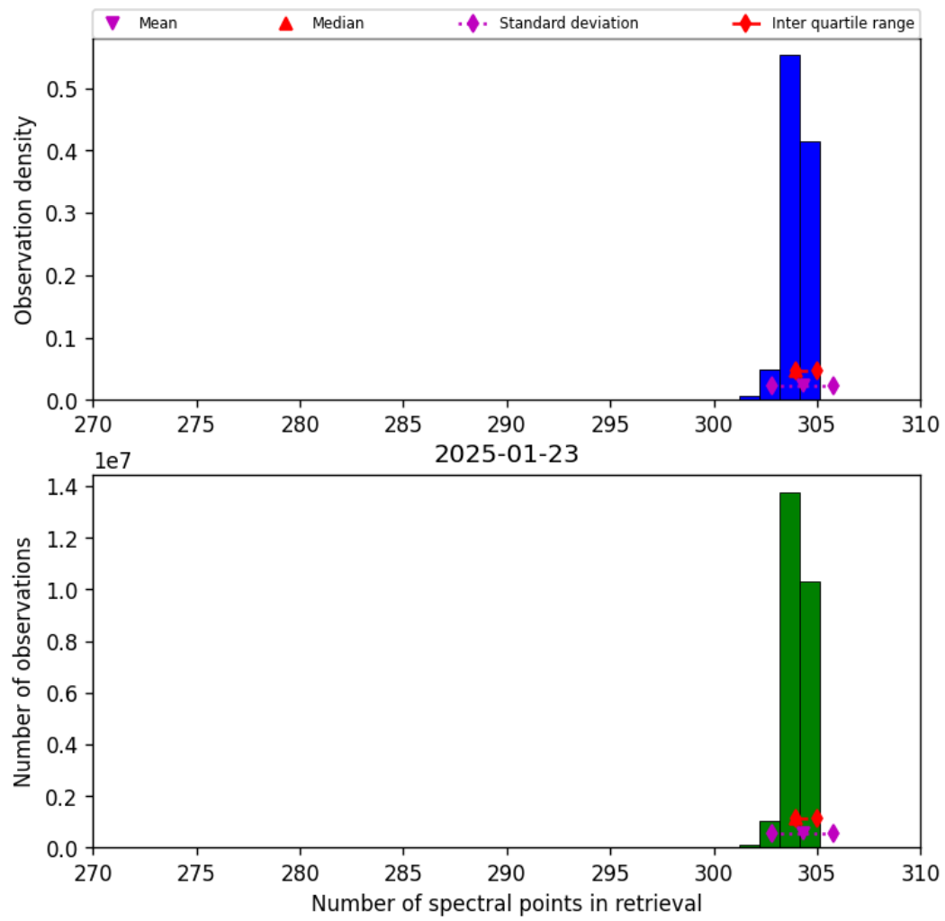
Figure 33: Histogram of “Number of spectral points in retrieval” for 2025-01-23 to 2025-01-24
