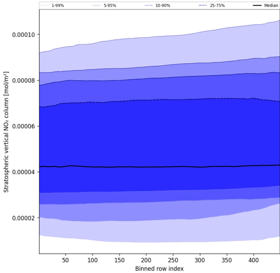
Figure 53: Along track statistics of “Stratospheric vertical NO 2 column” for 2025-01-23 to 2025-01-24
