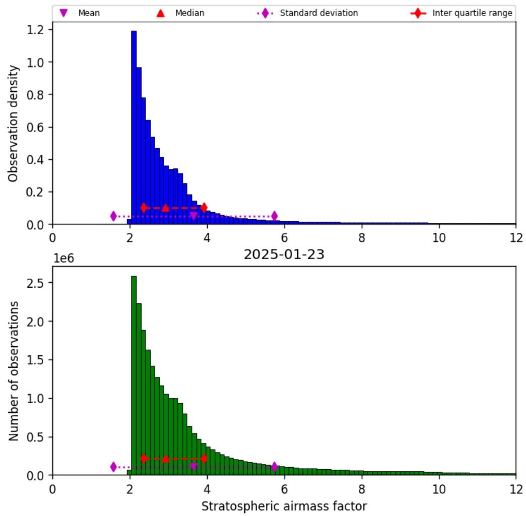
Figure 44: Histogram of “Stratospheric airmass factor” for 2025-01-23 to 2025-01-24
