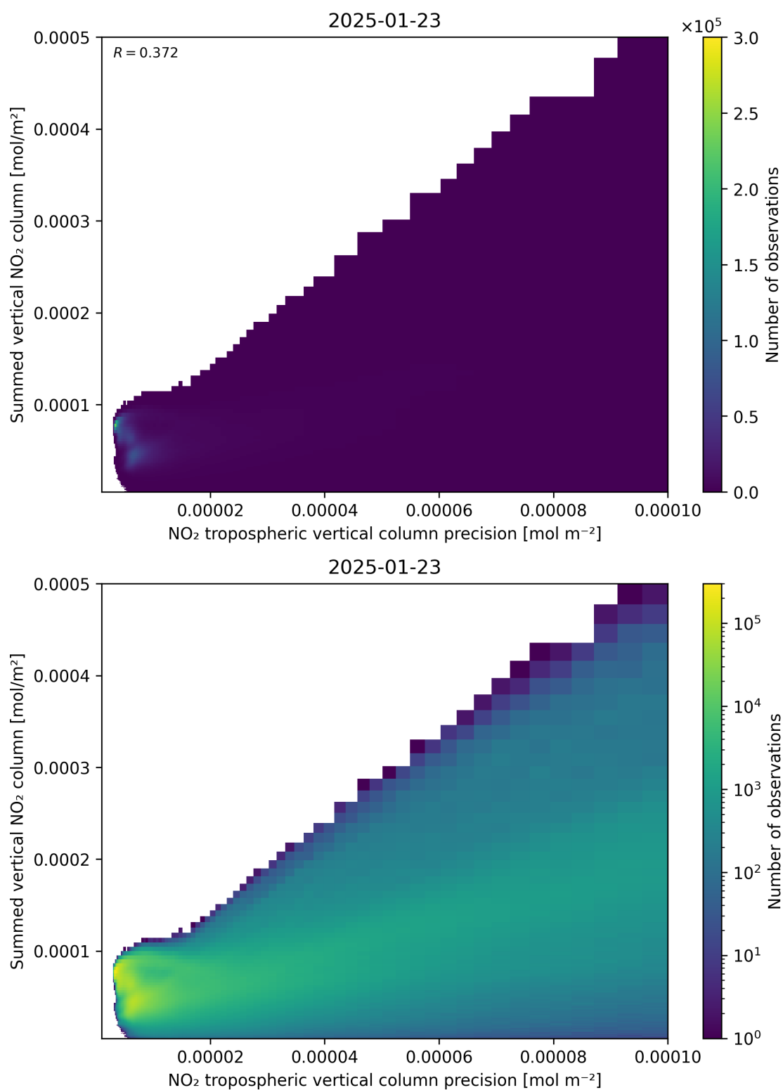
Figure 136: Scatter density plot of “NO 2 tropospheric vertical column precision” against “Summed vertical NO 2 column” for 2025-01-23 to 2025-01-24.
