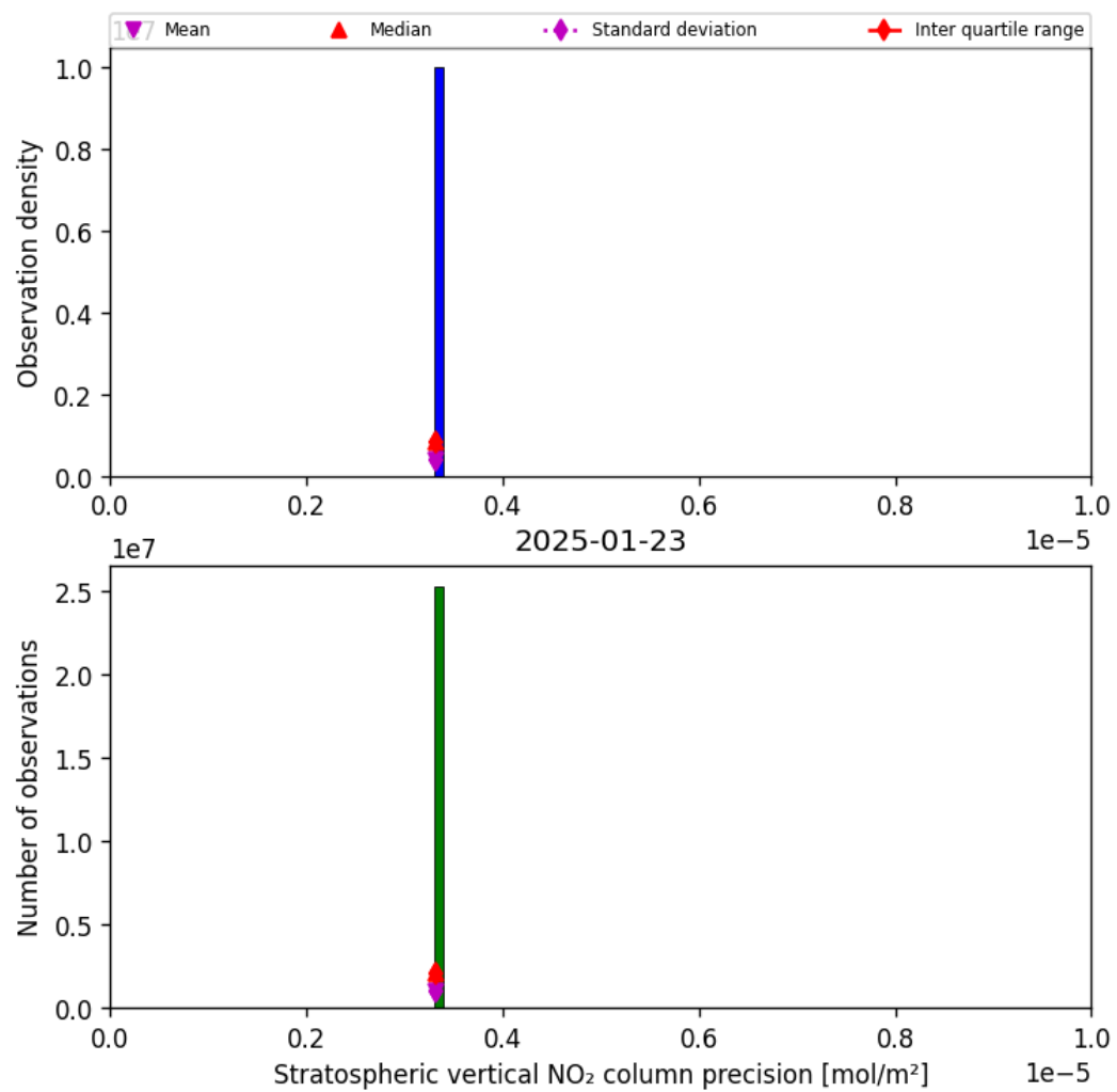
Figure 37: Histogram of “Stratospheric vertical NO 2 column precision” for 2025-01-23 to 2025-01-24
