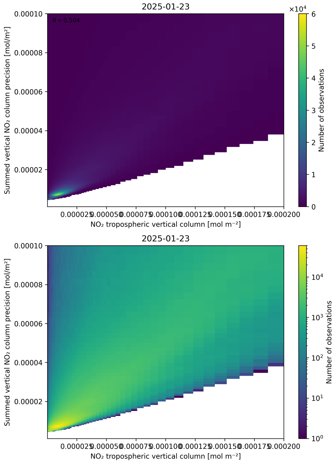
Figure 127: Scatter density plot of “NO 2 tropospheric vertical column” against “Summed vertical NO 2 column precision” for 2025-01-23 to 2025-01-24.
