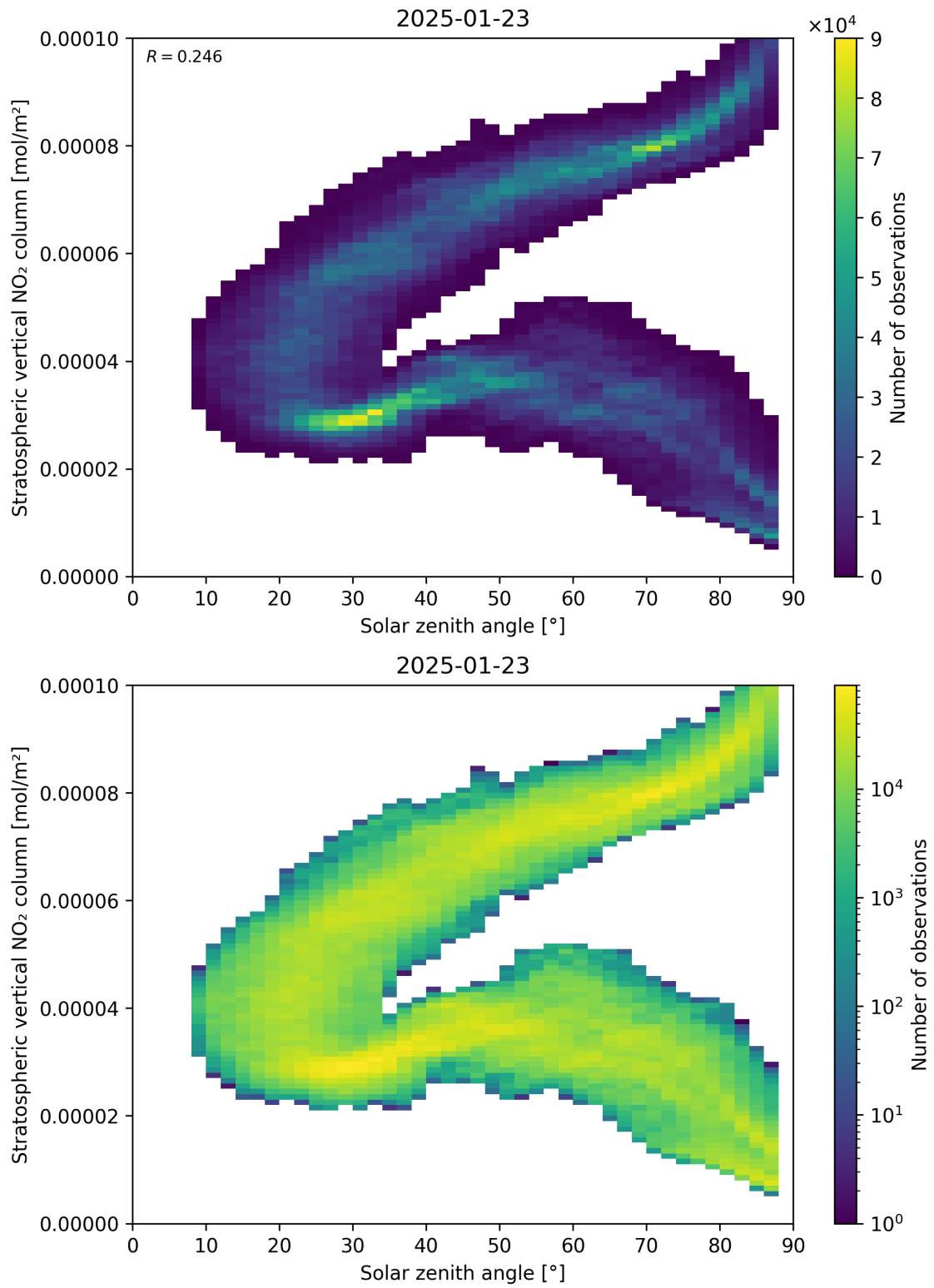
Figure 150: Scatter density plot of “Solar zenith angle” against “Stratospheric vertical NO 2 column” for 2025-01-23 to 2025-01-24.
