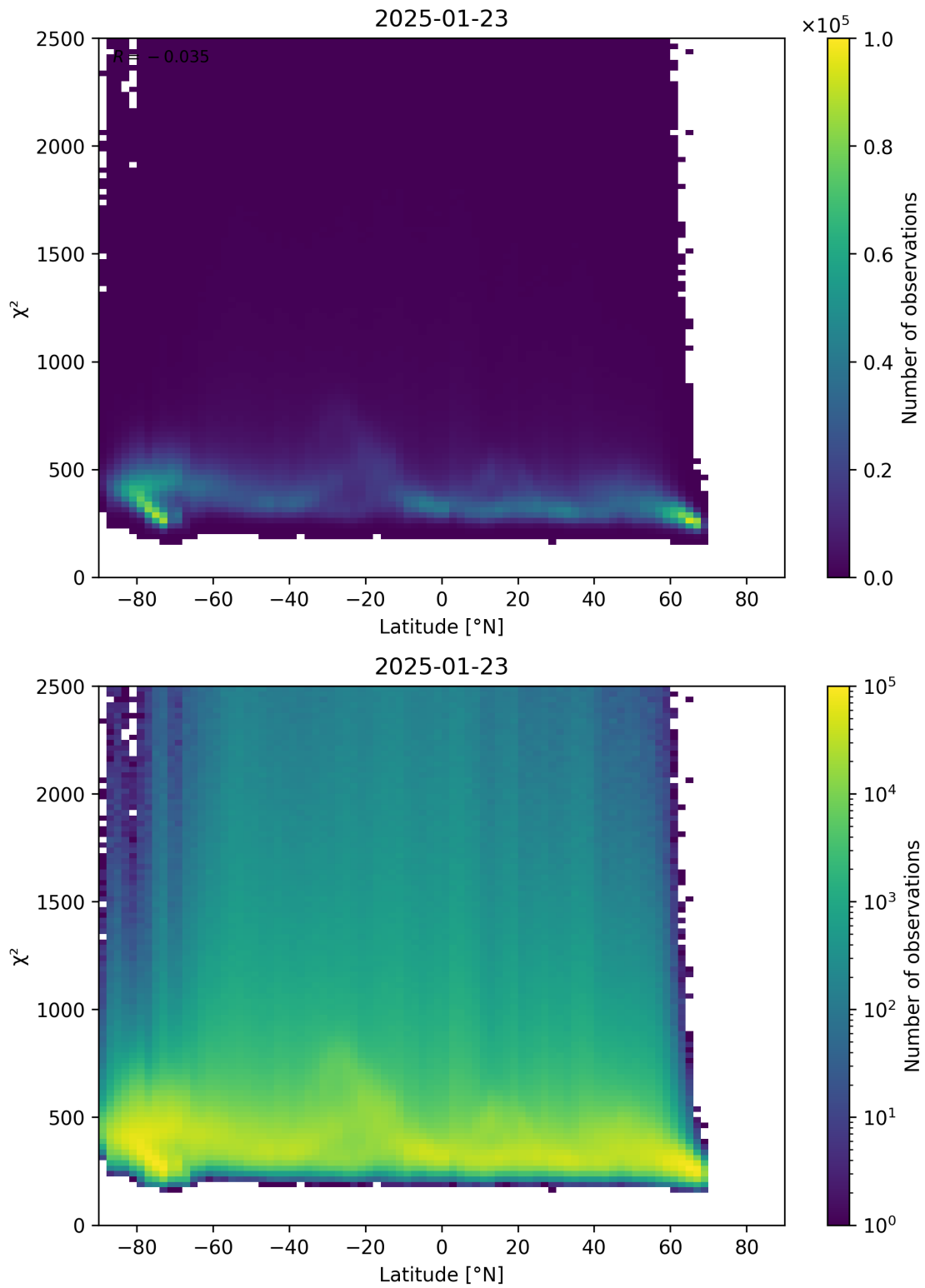
Figure 86: Scatter density plot of “Latitude” against “ \chi^2 ” for 2025-01-23 to 2025-01-24.
