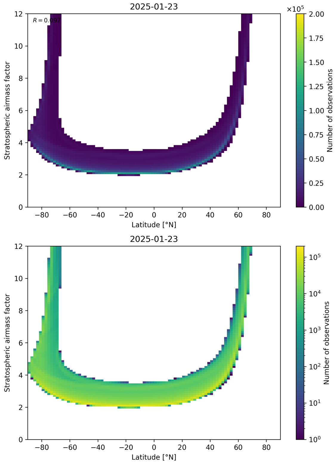
Figure 83: Scatter density plot of “Latitude” against “Stratospheric air mass factor” for 2025-01-23 to 2025-01-24.
