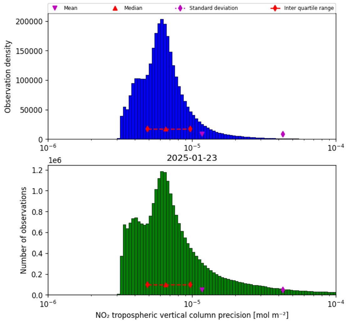
Figure 30: Histogram of “NO 2 tropospheric vertical column precision” for 2025-01-23 to 2025-01-24
