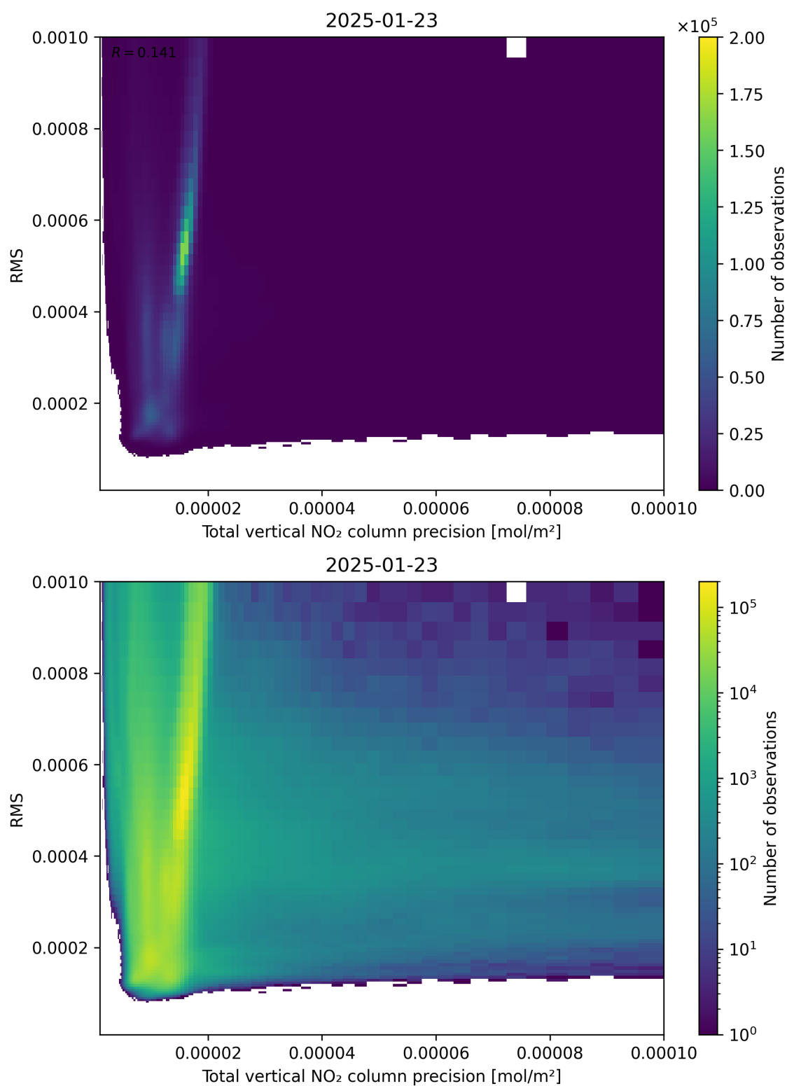
Figure 119: Scatter density plot of “Total vertical NO 2 column precision” against “RMS” for 2025-01-23 to 2025-01-24.
