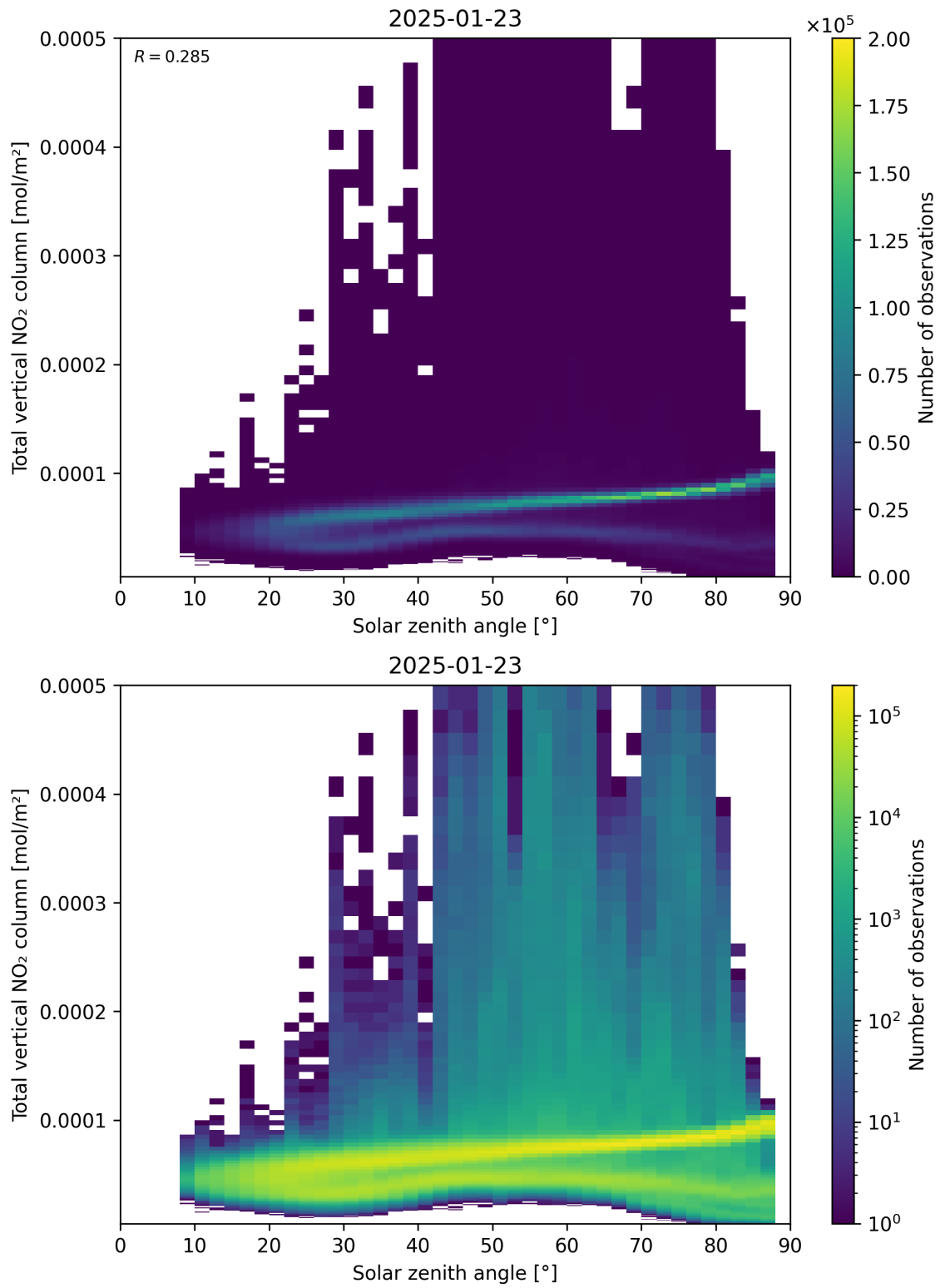
Figure 153: Scatter density plot of “Solar zenith angle” against “Total vertical NO 2 column” for 2025-01-23 to 2025-01-24.
