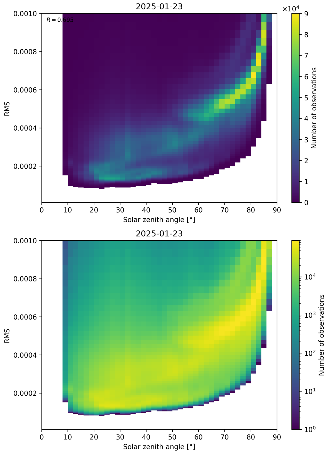
Figure 157: Scatter density plot of “Solar zenith angle” against “RMS” for 2025-01-23 to 2025-01-24.
