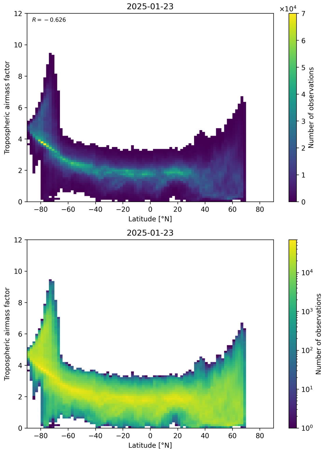
Figure 85: Scatter density plot of “Latitude” against “Tropospheric airmass factor” for 2025-01-23 to 2025-01-24.
