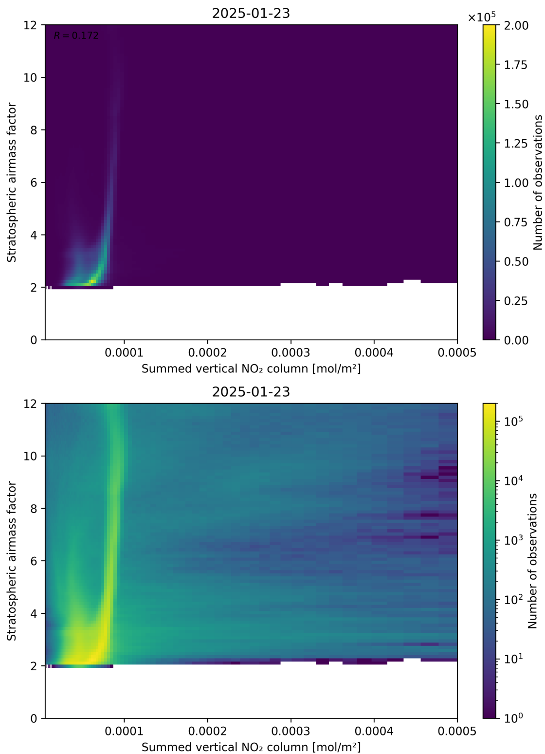
Figure 103: Scatter density plot of “Summed vertical NO 2 column” against “Stratospheric airmass factor” for 2025-01-23 to 2025-01-24.
