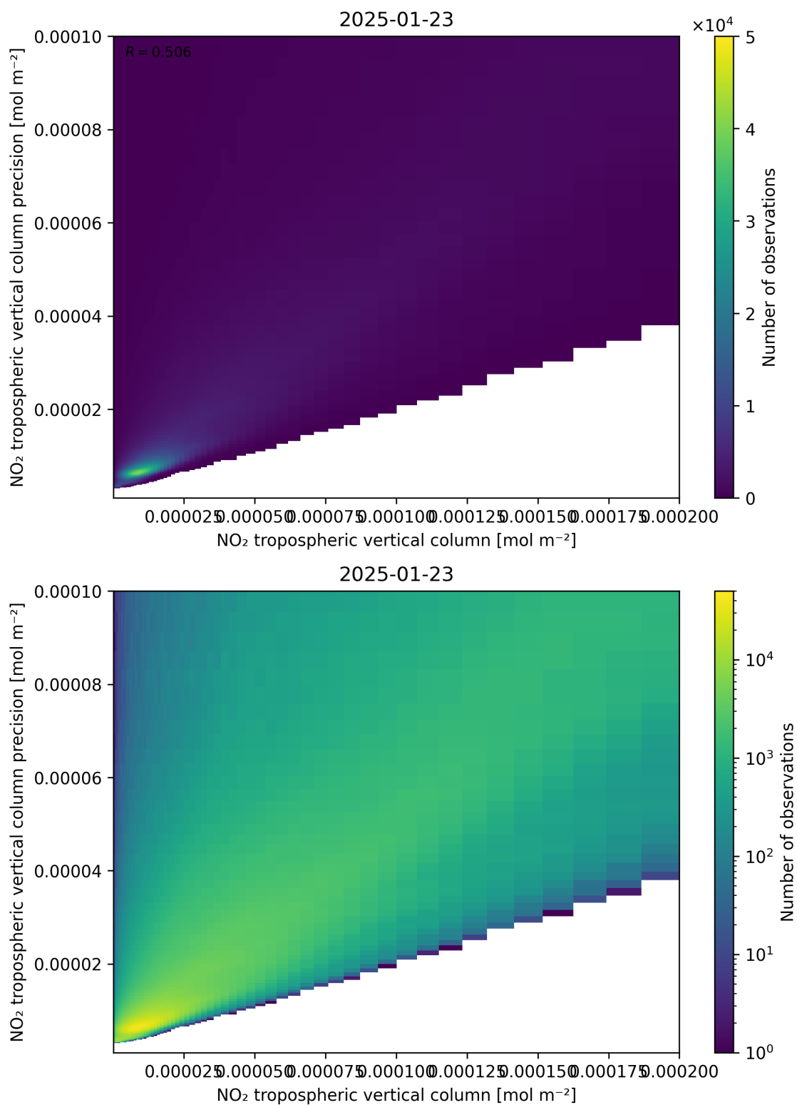
Figure 130: Scatter density plot of “NO 2 tropospheric vertical column” against “NO 2 tropospheric vertical column precision” for 2025-01-23 to 2025-01-24.
