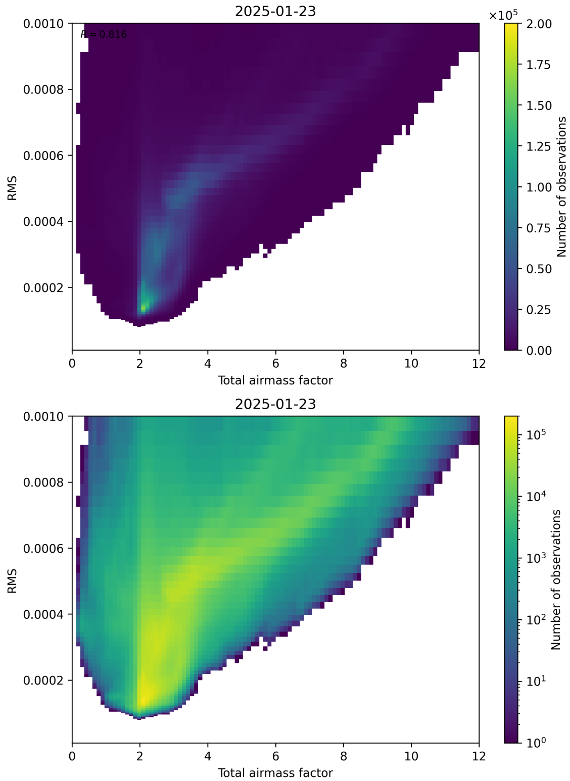
Figure 69: Scatter density plot of “Total airmass factor” against “RMS” for 2025-01-23 to 2025-01-24.
