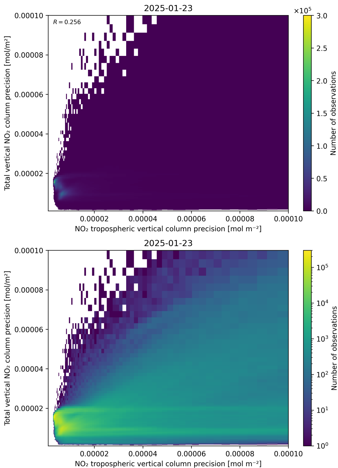
Figure 139: Scatter density plot of “NO 2 tropospheric vertical column precision” against “Total vertical NO 2 column precision” for 2025-01-23 to 2025-01-24.
