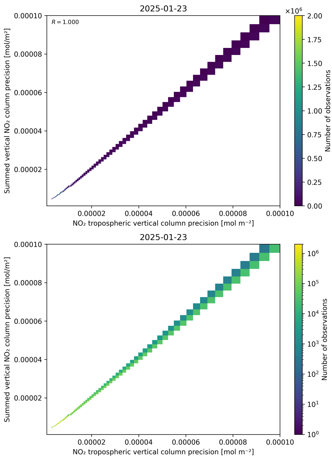
Figure 137: Scatter density plot of “NO 2 tropospheric vertical column precision” against “Summed vertical NO 2 column precision” for 2025-01-23 to 2025-01-24.
