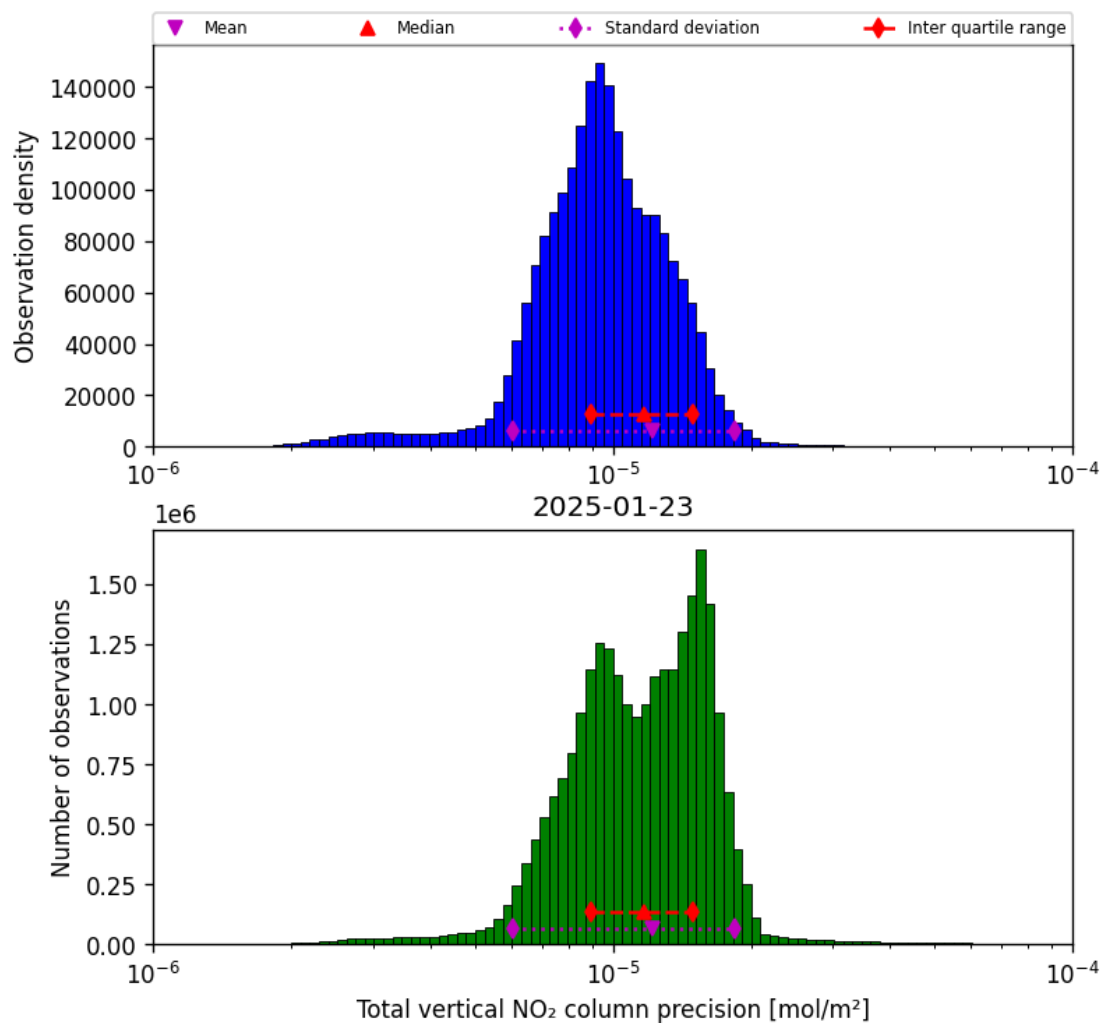
Figure 39: Histogram of “Total vertical NO 2 column precision” for 2025-01-23 to 2025-01-24
