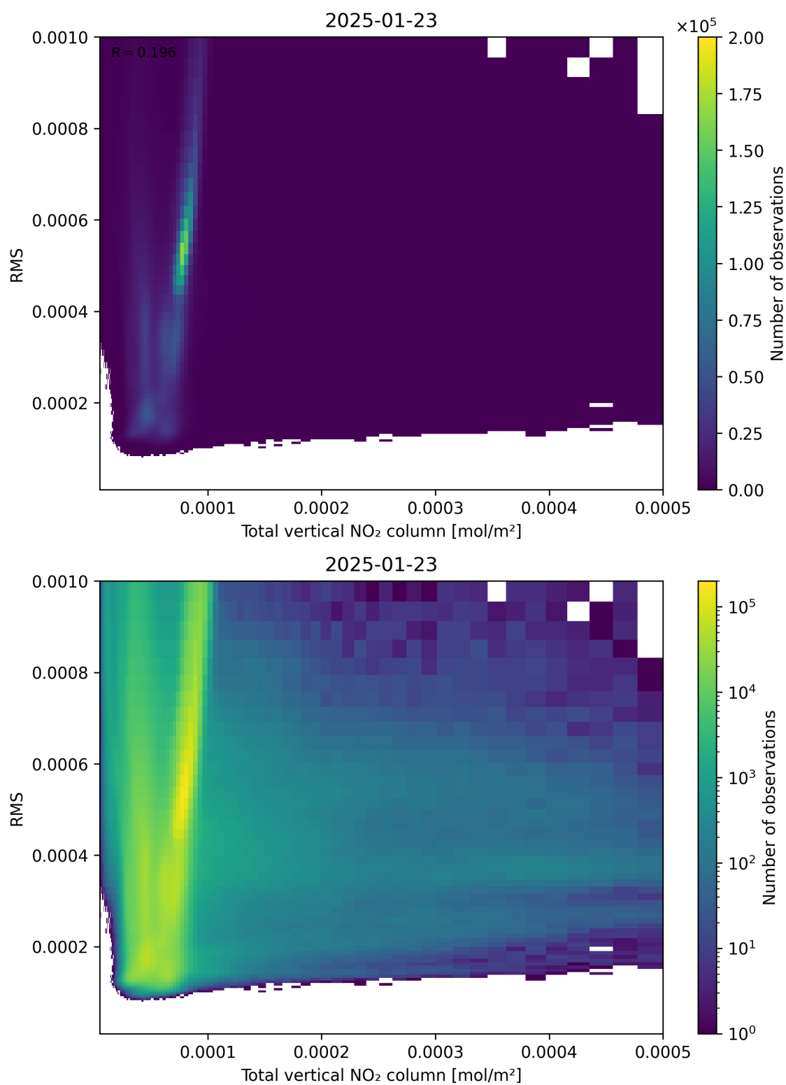
Figure 120: Scatter density plot of “Total vertical NO 2 column” against “RMS” for 2025-01-23 to 2025-01-24.
