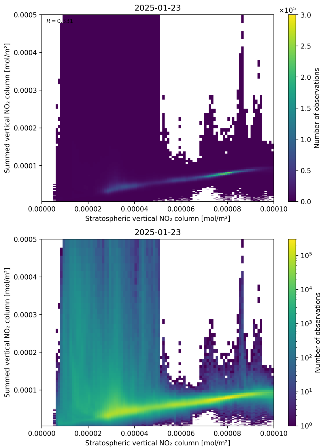
Figure 98: Scatter density plot of “Stratospheric vertical NO 2 column” against “Summed vertical NO 2 column” for 2025-01-23 to 2025-01-24.
