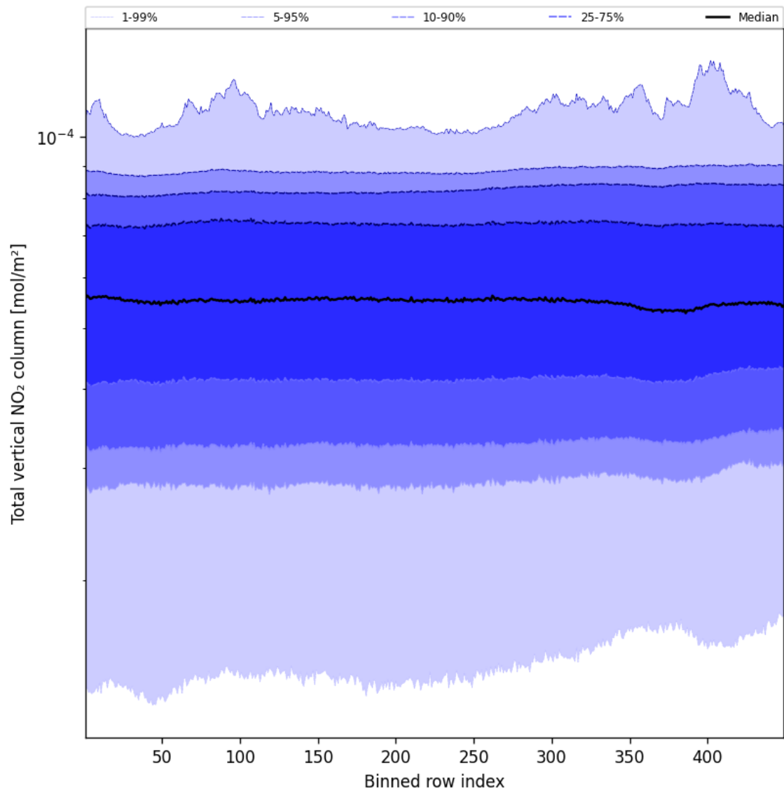
Figure 55: Along track statistics of “Total vertical NO 2 column” for 2025-01-23 to 2025-01-24
