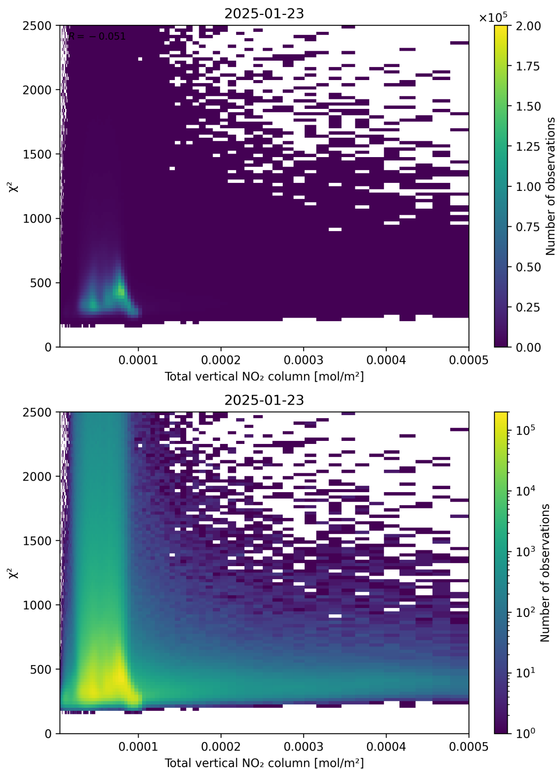
Figure 111: Scatter density plot of “Total vertical NO 2 column” against “ \chi^2 ” for 2025-01-23 to 2025-01-24.
