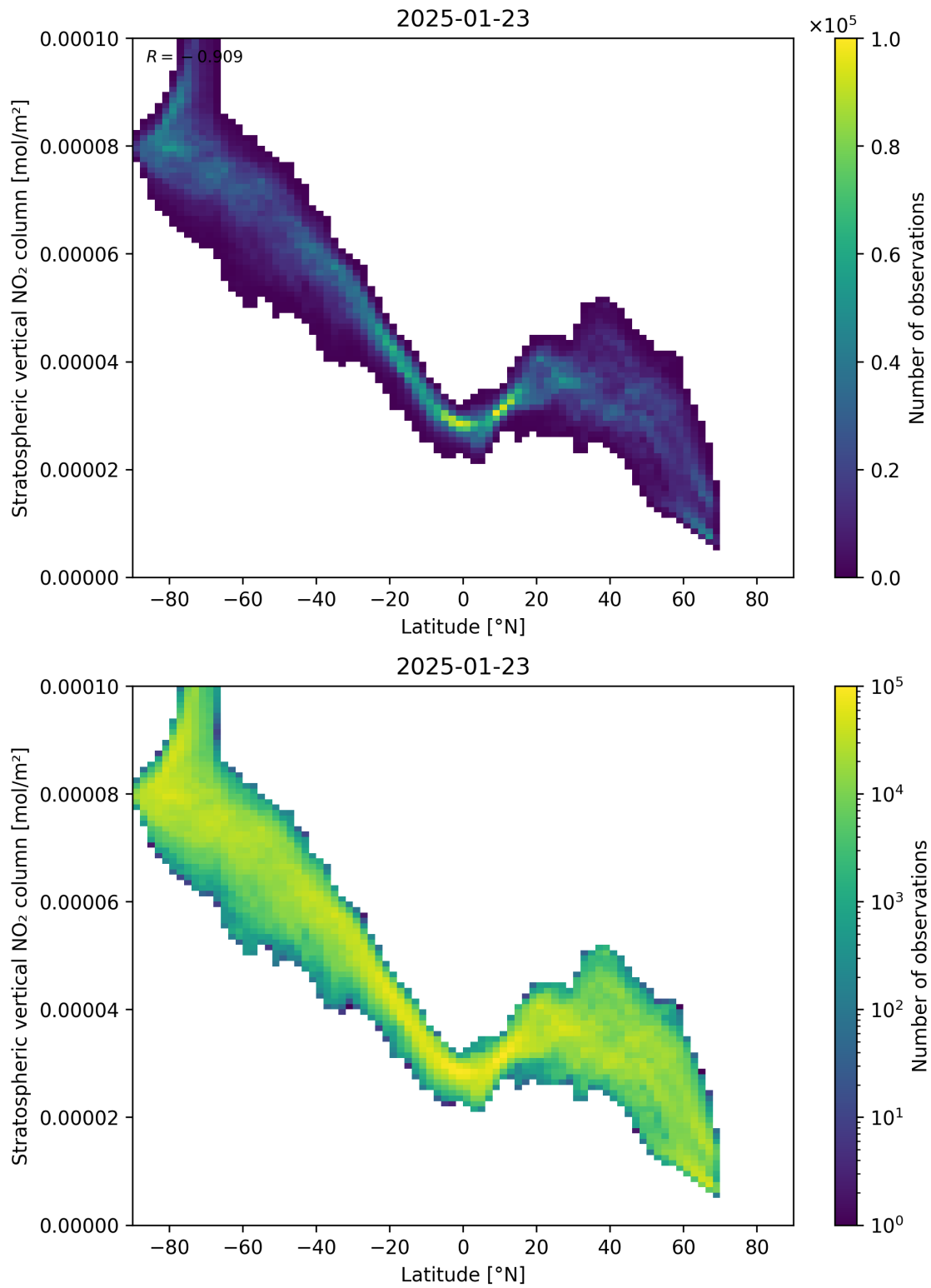
Figure 87: Scatter density plot of “Latitude” against “Stratospheric vertical NO 2 column” for 2025-01-23 to 2025-01-24.
