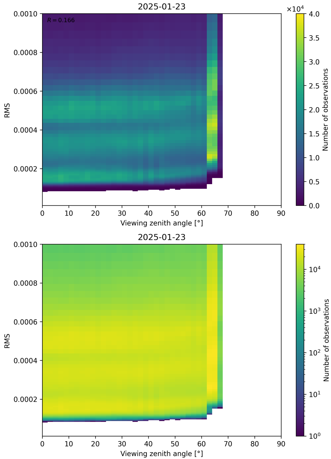
Figure 171: Scatter density plot of “Viewing zenith angle” against “RMS” for 2025-01-23 to 2025-01-24.
