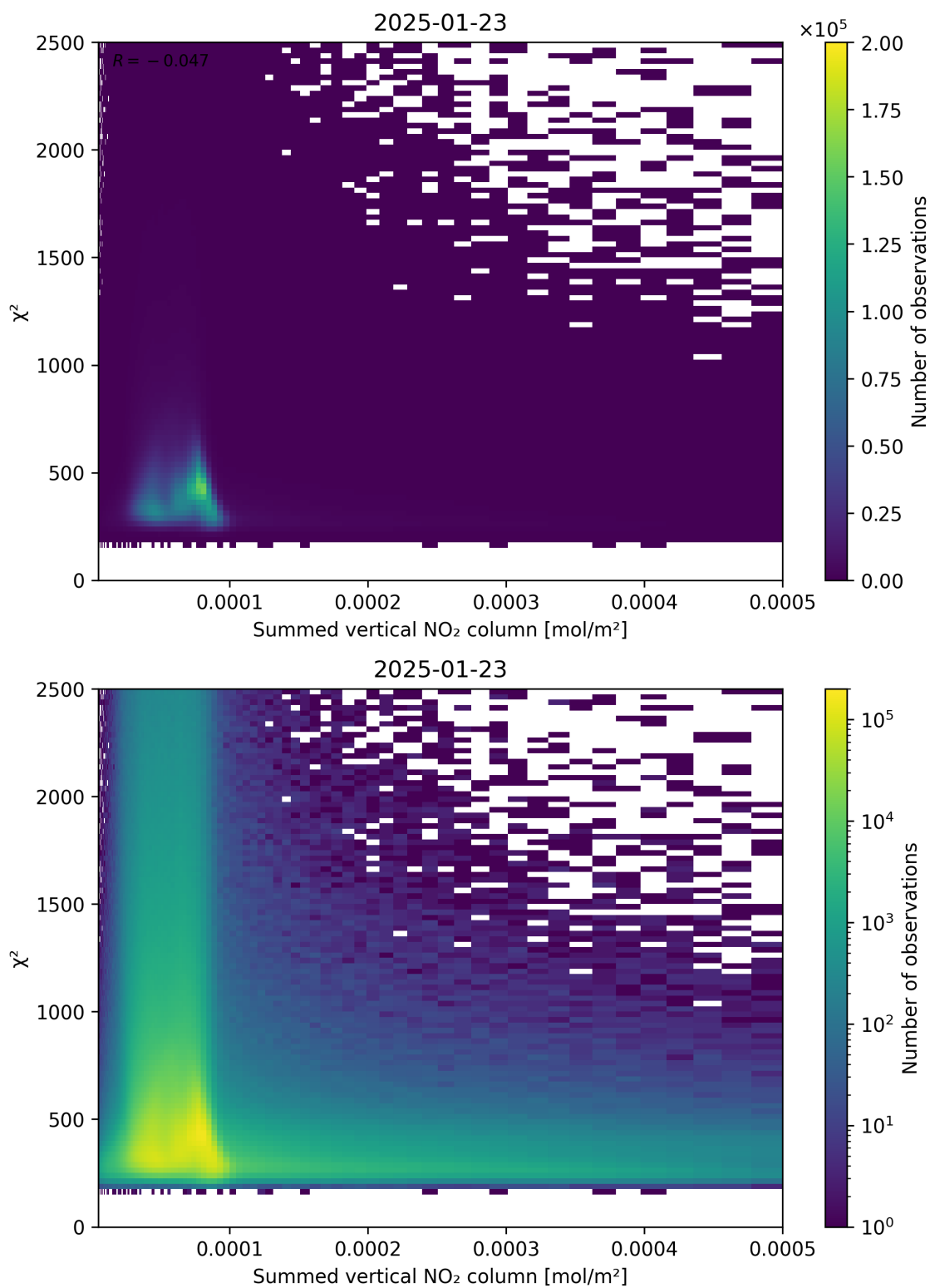
Figure 104: Scatter density plot of “Summed vertical NO 2 column” against “ \chi^2 ” for 2025-01-23 to 2025-01-24.
