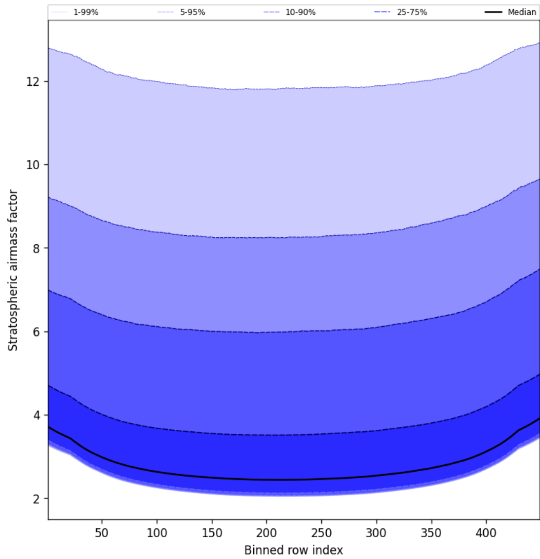
Figure 61: Along track statistics of “Stratospheric airmass factor” for 2025-01-23 to 2025-01-24
