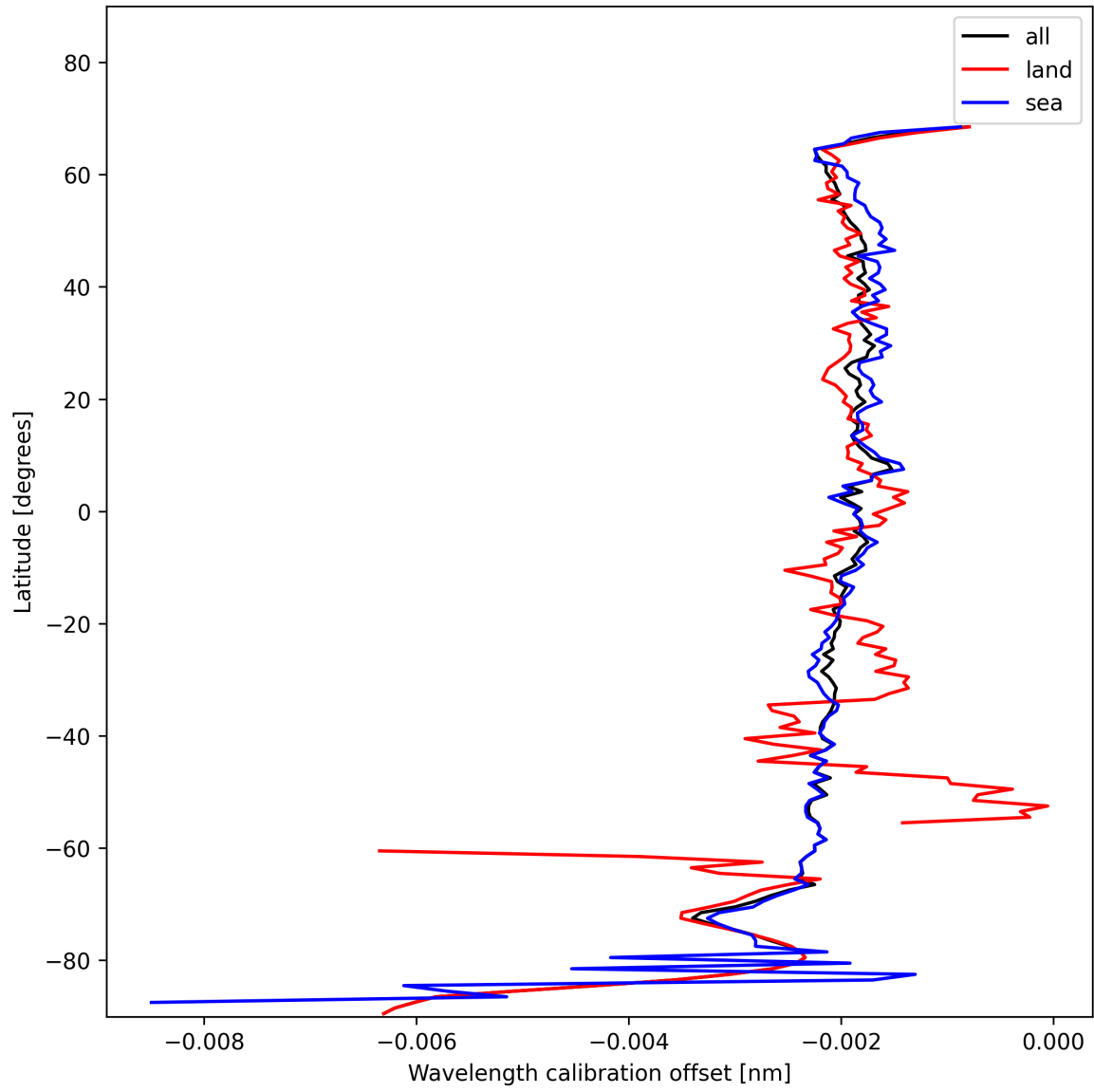
Figure 18: Zonal average of “Wavelength calibration offset” for 2025-01-23 to 2025-01-24.
