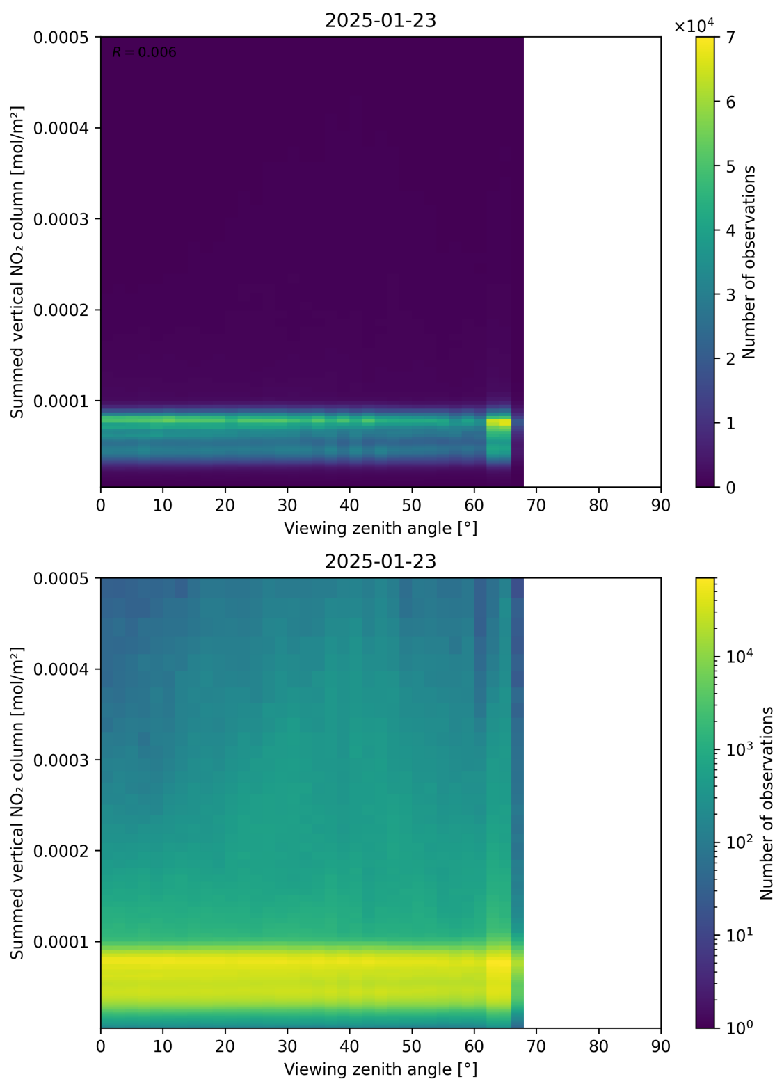
Figure 165: Scatter density plot of “Viewing zenith angle” against “Summed vertical NO 2 column” for 2025-01-23 to 2025-01-24.
