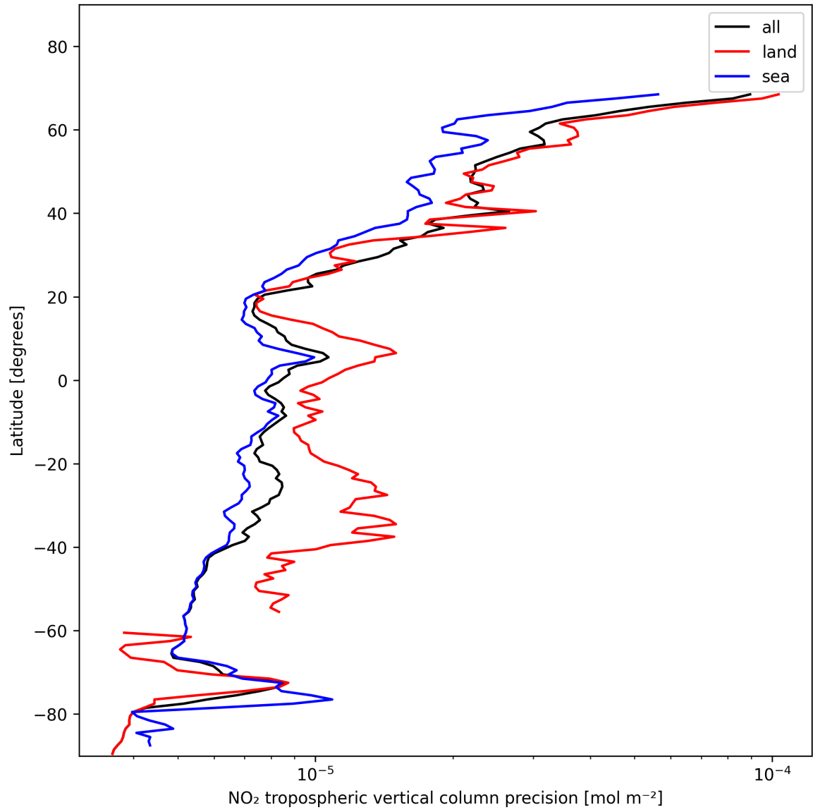
Figure 13: Zonal average of “NO 2 tropospheric vertical column precision” for 2025-01-23 to 2025-01-24.
