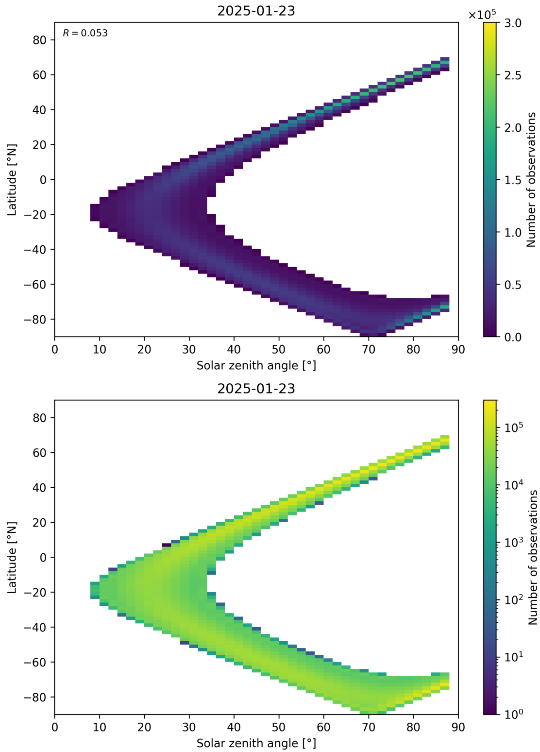
Figure 149: Scatter density plot of “Solar zenith angle” against “Latitude” for 2025-01-23 to 2025-01-24.
