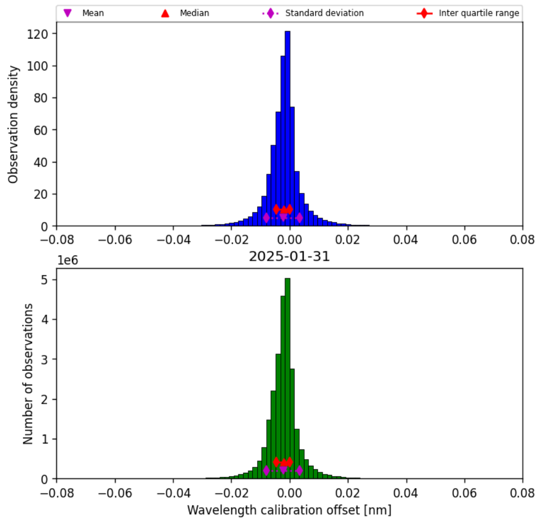
Figure 35: Histogram of “Wavelength calibration offset” for 2025-01-30 to 2025-02-01
