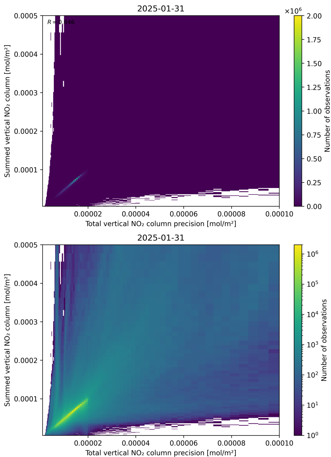
Figure 117: Scatter density plot of “Total vertical NO 2 column precision” against “Summed vertical NO 2 column” for 2025-01-30 to 2025-02-01.
