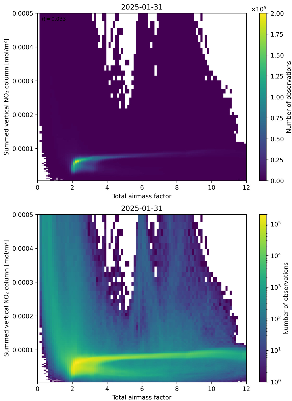
Figure 65: Scatter density plot of “Total airmass factor” against “Summed vertical NO 2 column” for 2025-01-30 to 2025-02-01.
