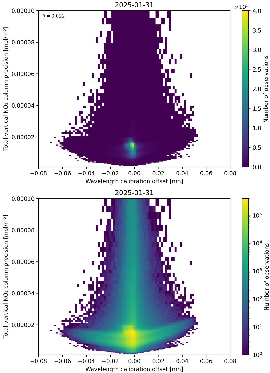
Figure 180: Scatter density plot of “Wavelength calibration offset” against “Total vertical NO 2 column precision” for 2025-01-30 to 2025-02-01.
