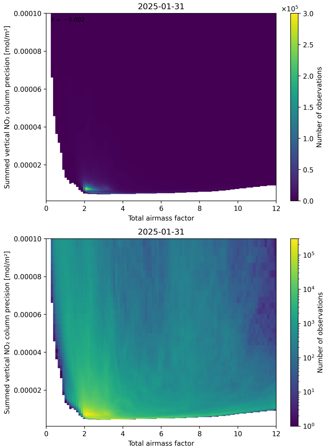
Figure 66: Scatter density plot of “Total airmass factor” against “Summed vertical NO 2 column precision” for 2025-01-30 to 2025-02-01.
