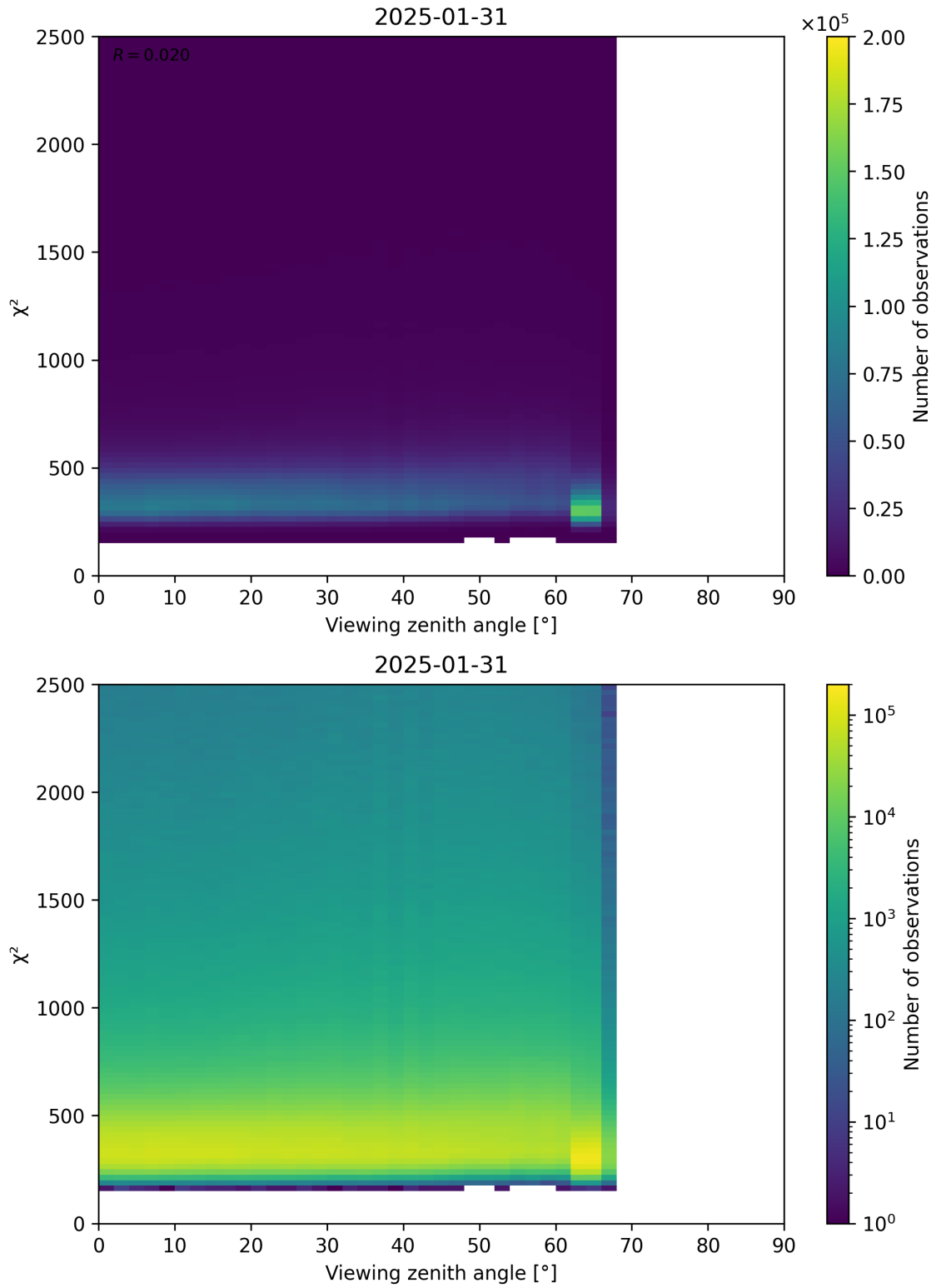
Figure 162: Scatter density plot of “Viewing zenith angle” against “ \chi^2 ” for 2025-01-30 to 2025-02-01.
