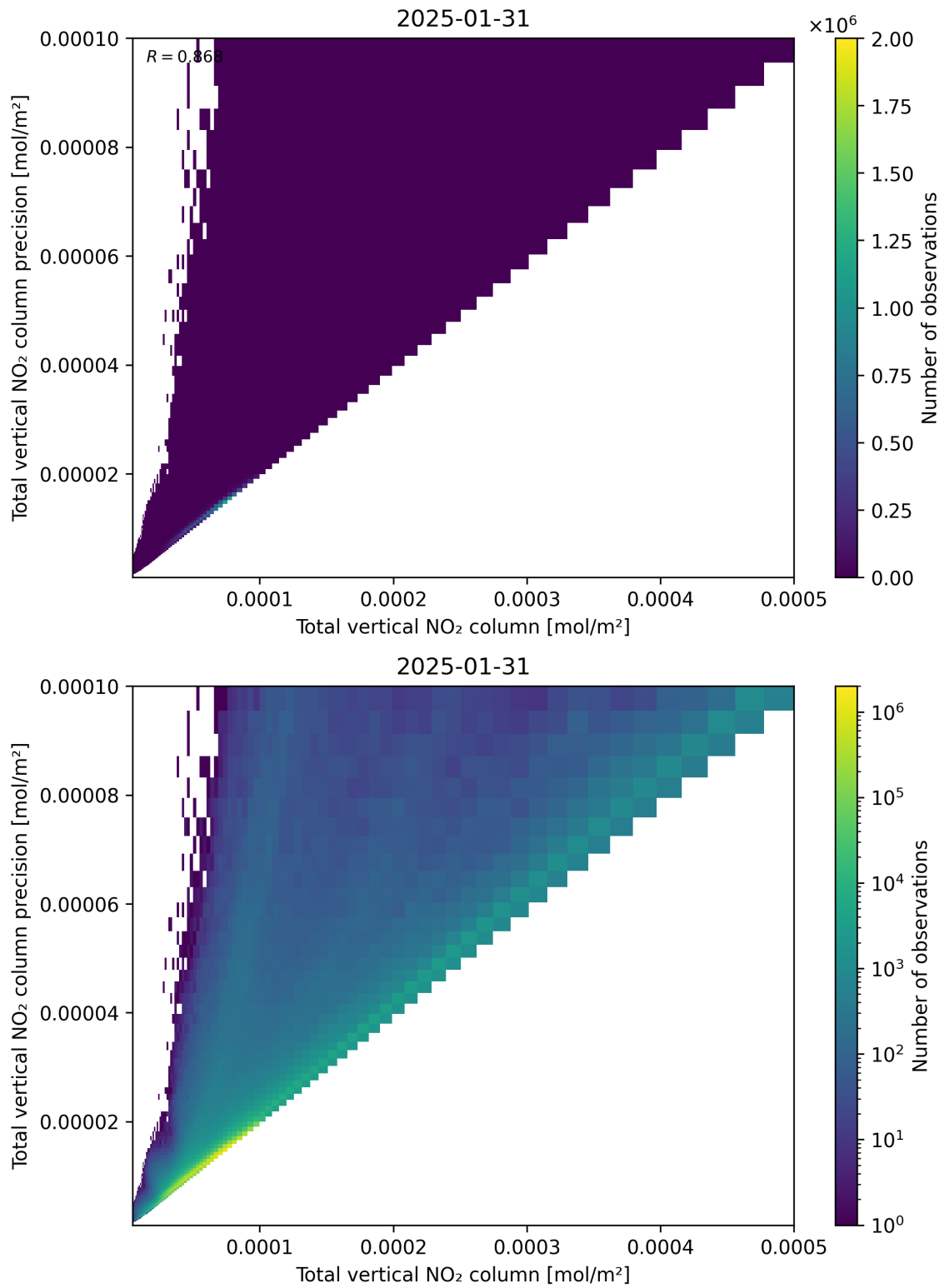
Figure 114: Scatter density plot of “Total vertical NO 2 column” against “Total vertical NO 2 column precision” for 2025-01-30 to 2025-02-01.
