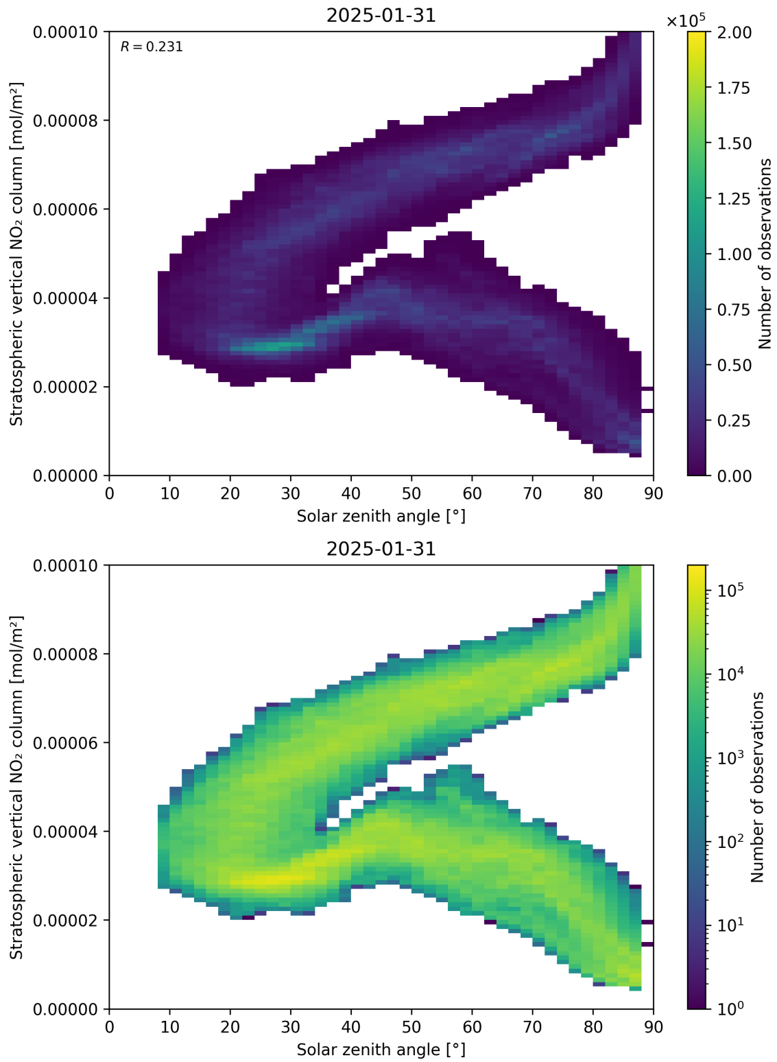
Figure 150: Scatter density plot of “Solar zenith angle” against “Stratospheric vertical NO 2 column” for 2025-01-30 to 2025-02-01.
