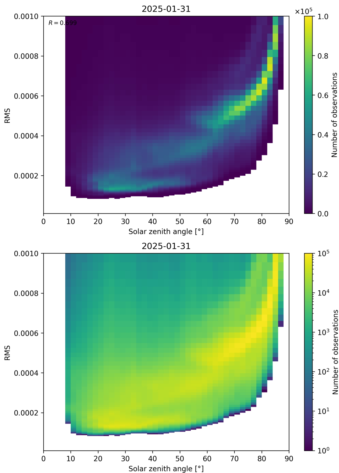
Figure 157: Scatter density plot of “Solar zenith angle” against “RMS” for 2025-01-30 to 2025-02-01.
