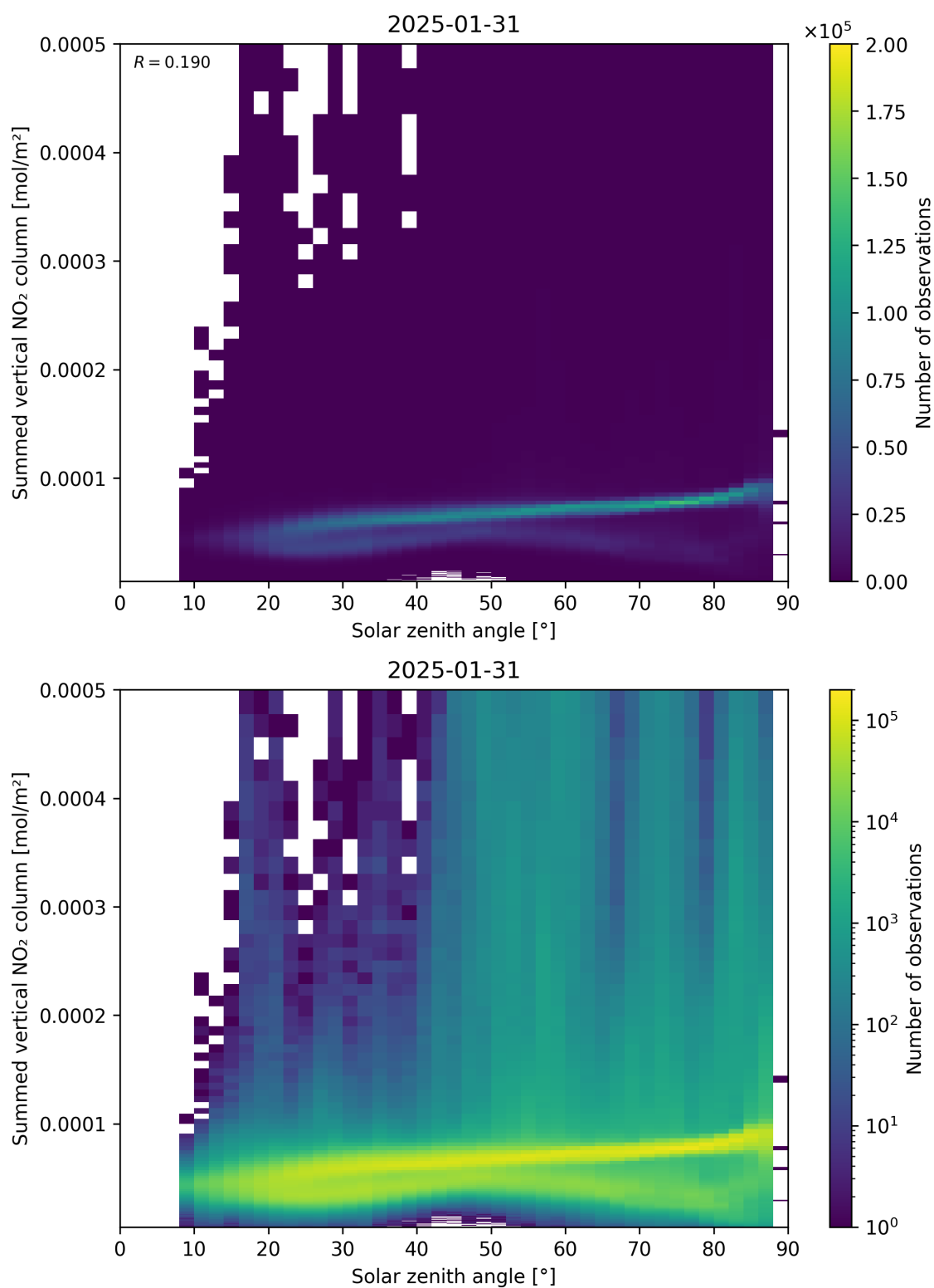
Figure 151: Scatter density plot of “Solar zenith angle” against “Summed vertical NO 2 column” for 2025-01-30 to 2025-02-01.
