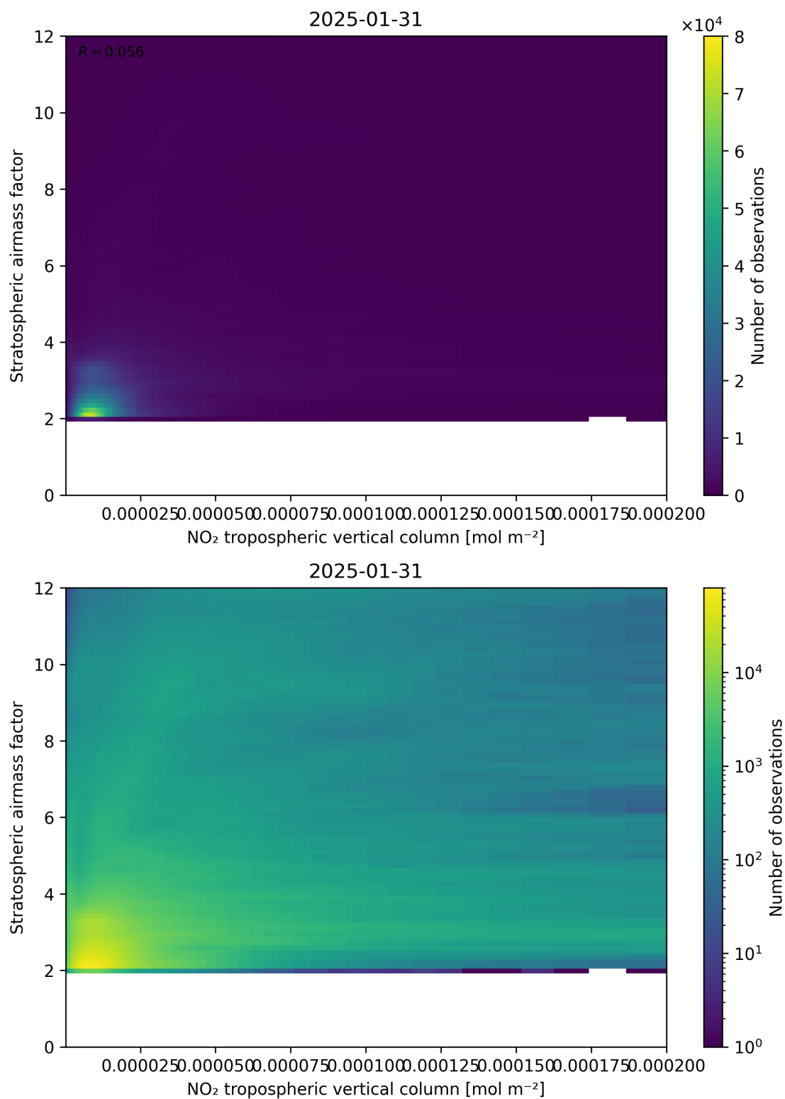
Figure 121: Scatter density plot of “NO 2 tropospheric vertical column” against “Stratospheric airmass factor” for 2025-01-30 to 2025-02-01.
