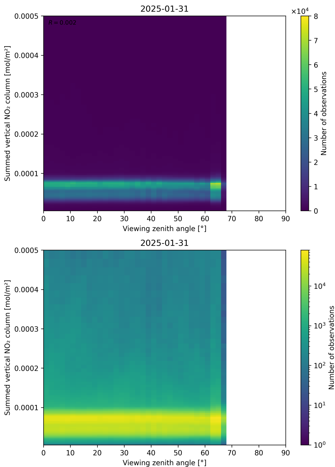
Figure 165: Scatter density plot of “Viewing zenith angle” against “Summed vertical NO 2 column” for 2025-01-30 to 2025-02-01.
