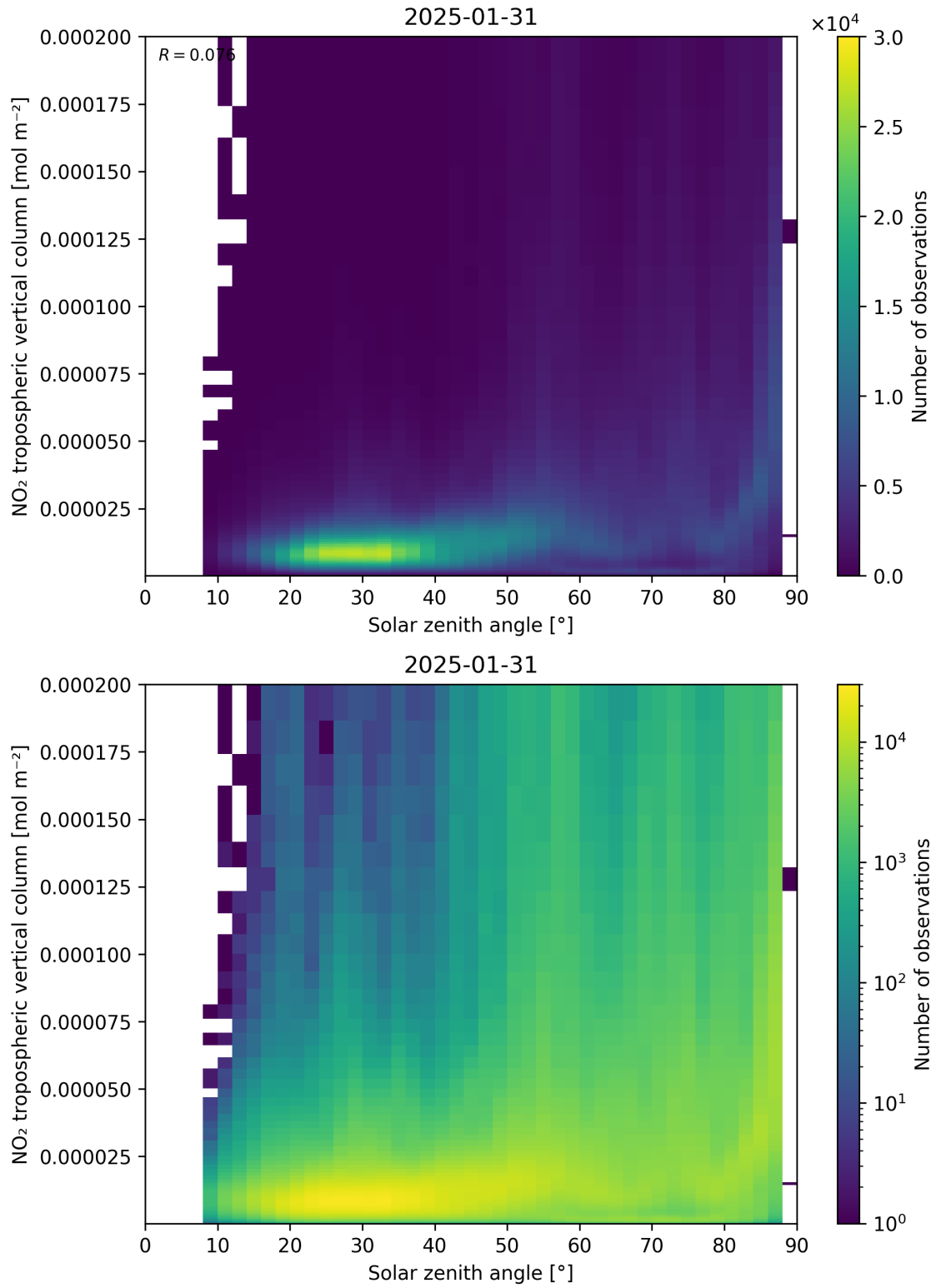
Figure 155: Scatter density plot of “Solar zenith angle” against “NO 2 tropospheric vertical column” for 2025-01-30 to 2025-02-01.
