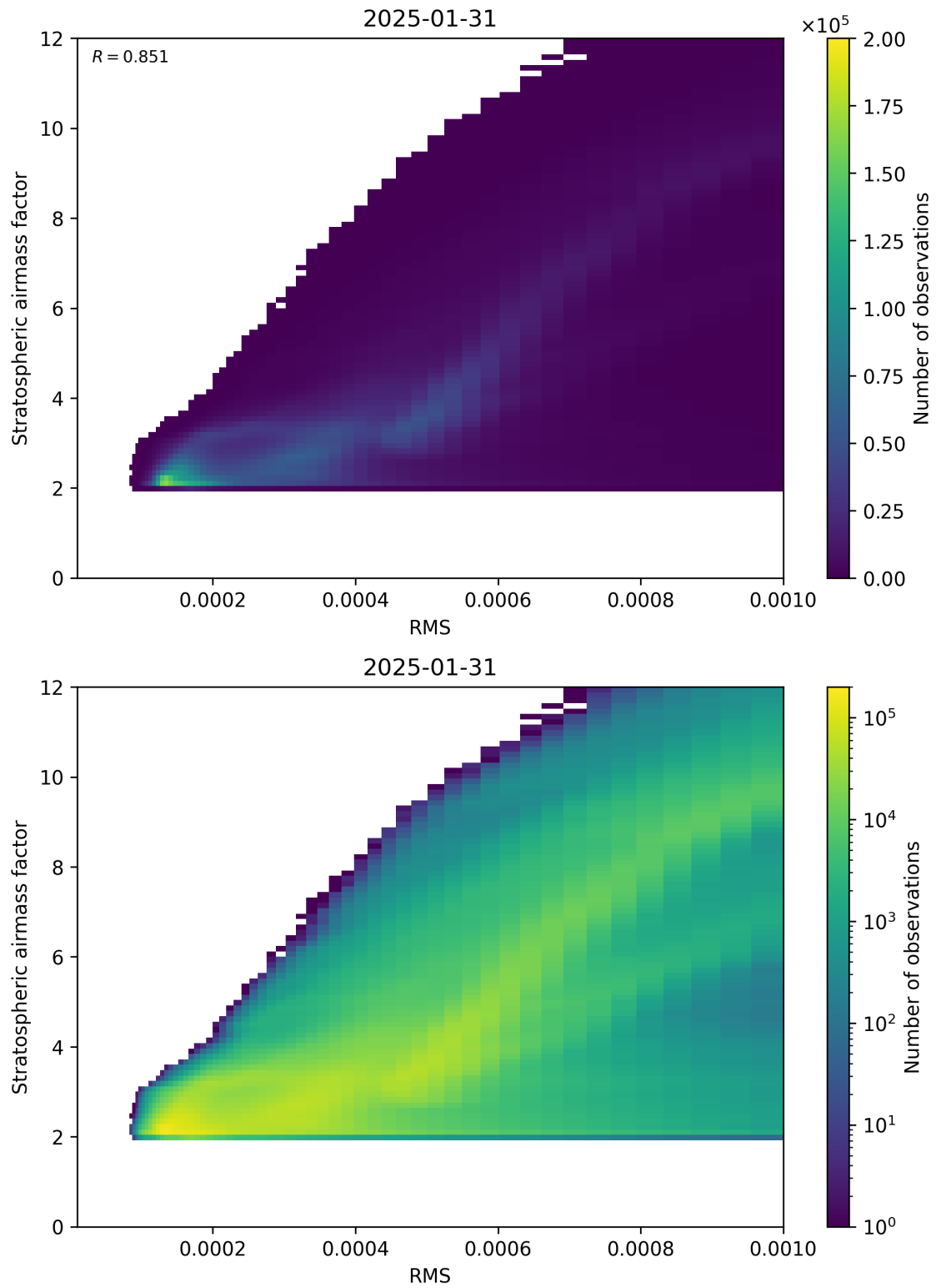
Figure 144: Scatter density plot of “RMS” against “Stratospheric airmass factor” for 2025-01-30 to 2025-02-01.
