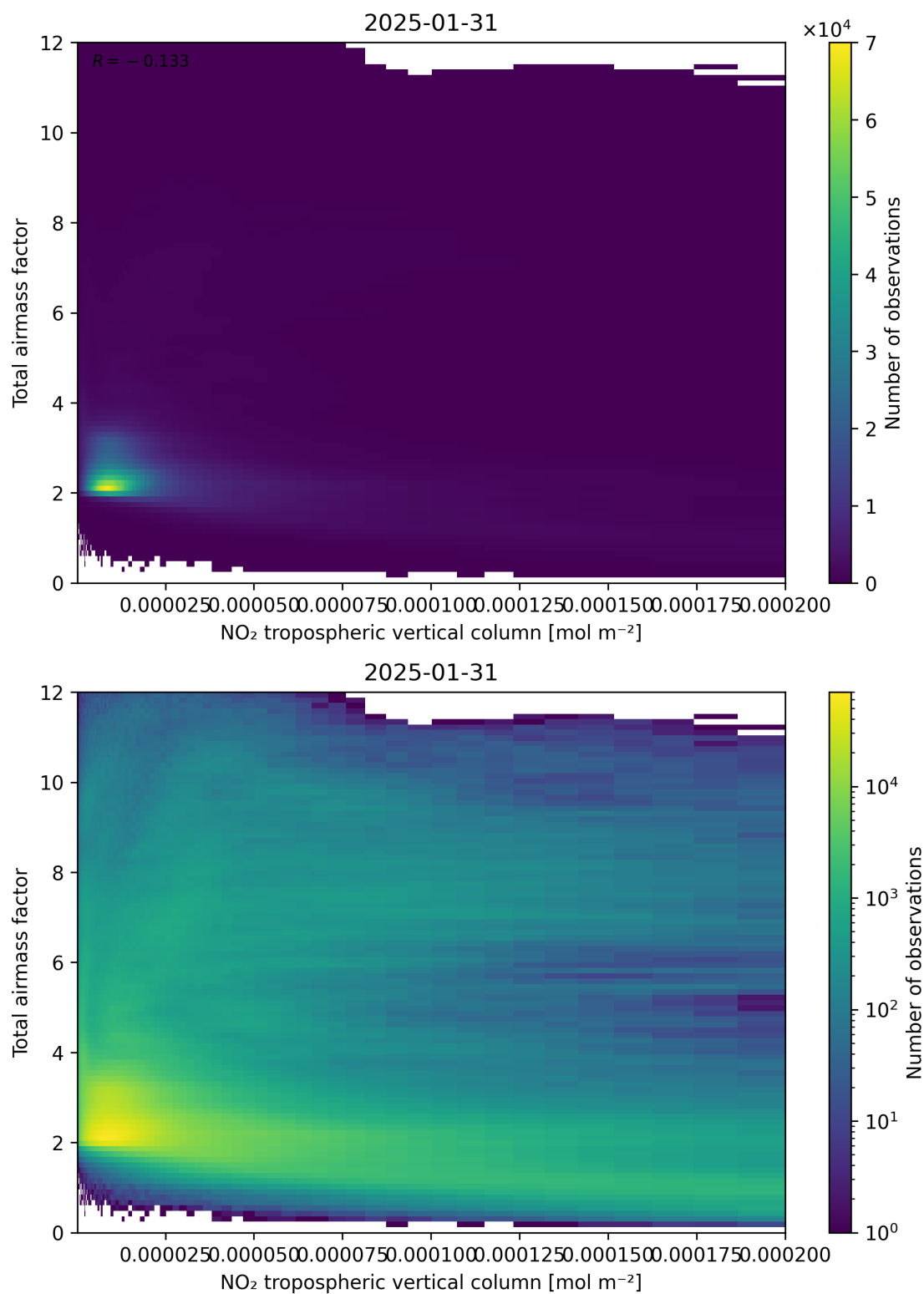
Figure 122: Scatter density plot of “NO 2 tropospheric vertical column” against “Total air mass factor” for 2025-01-30 to 2025-02-01.
