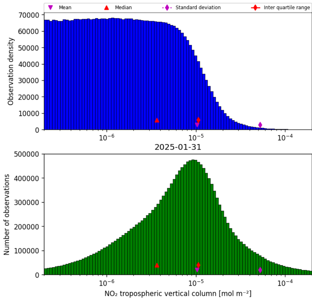
Figure 29: Histogram of “NO 2 tropospheric vertical column” for 2025-01-30 to 2025-02-01
