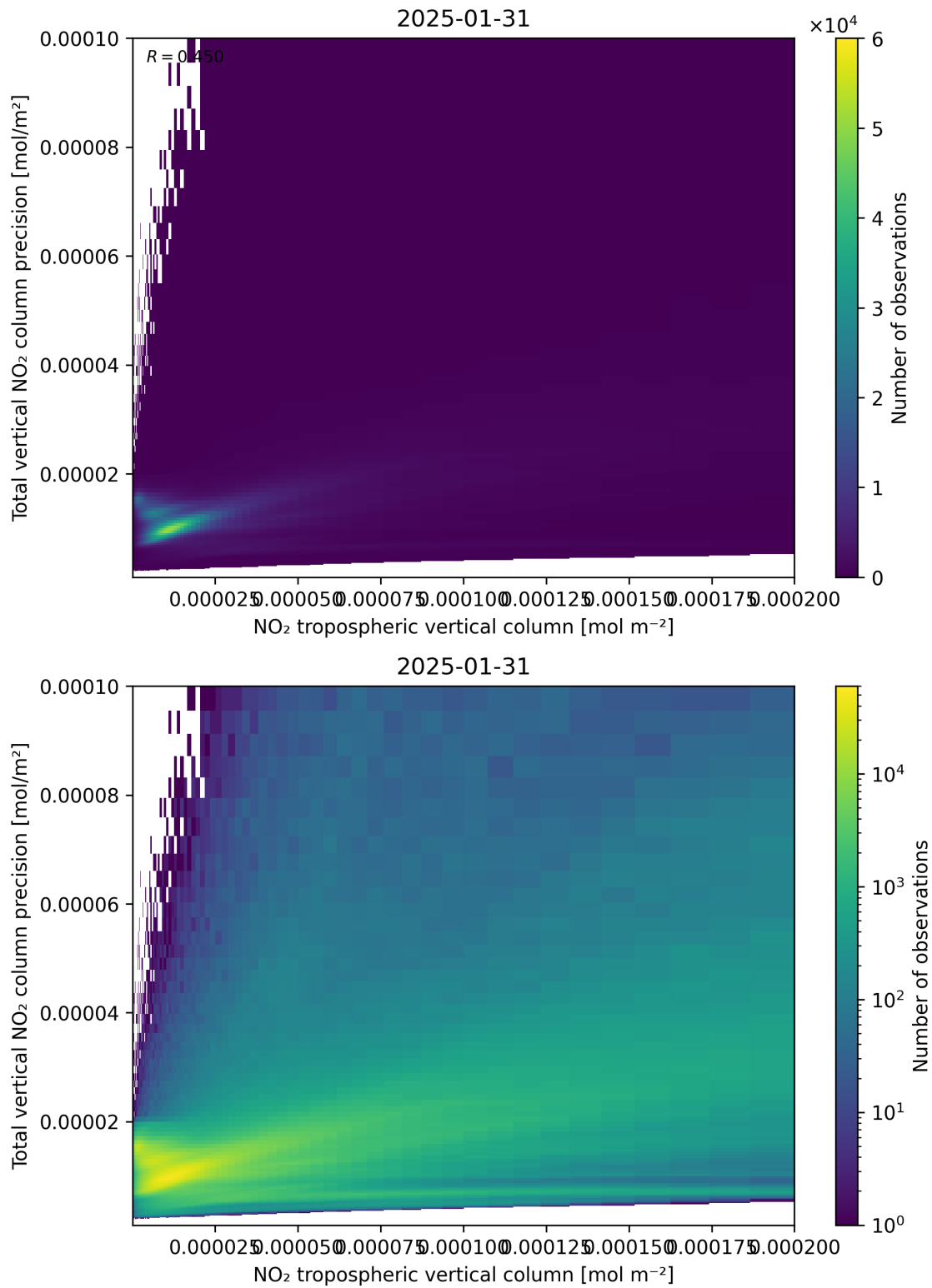
Figure 129: Scatter density plot of “NO 2 tropospheric vertical column” against “Total vertical NO 2 column precision” for 2025-01-30 to 2025-02-01.
