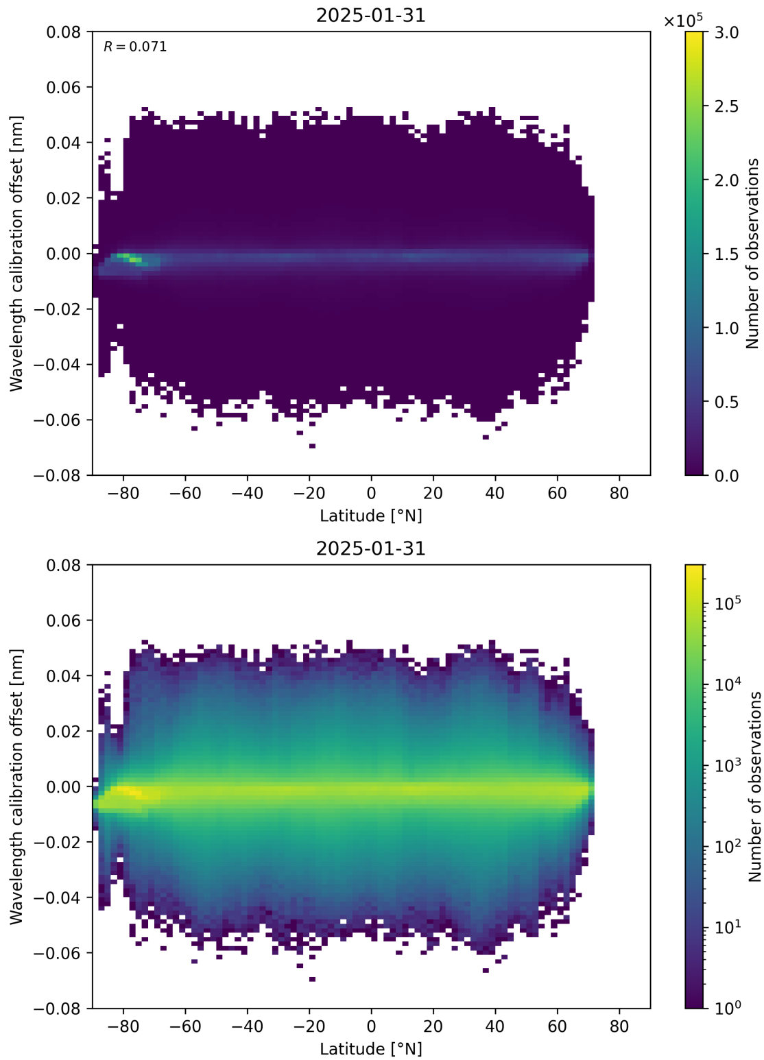
Figure 95: Scatter density plot of “Latitude” against “Wavelength calibration offset” for 2025-01-30 to 2025-02-01.
