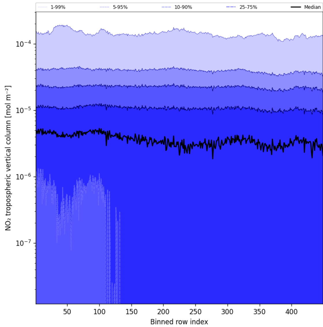
Figure 46: Along track statistics of “NO 2 tropospheric vertical column” for 2025-01-30 to 2025-02-01
