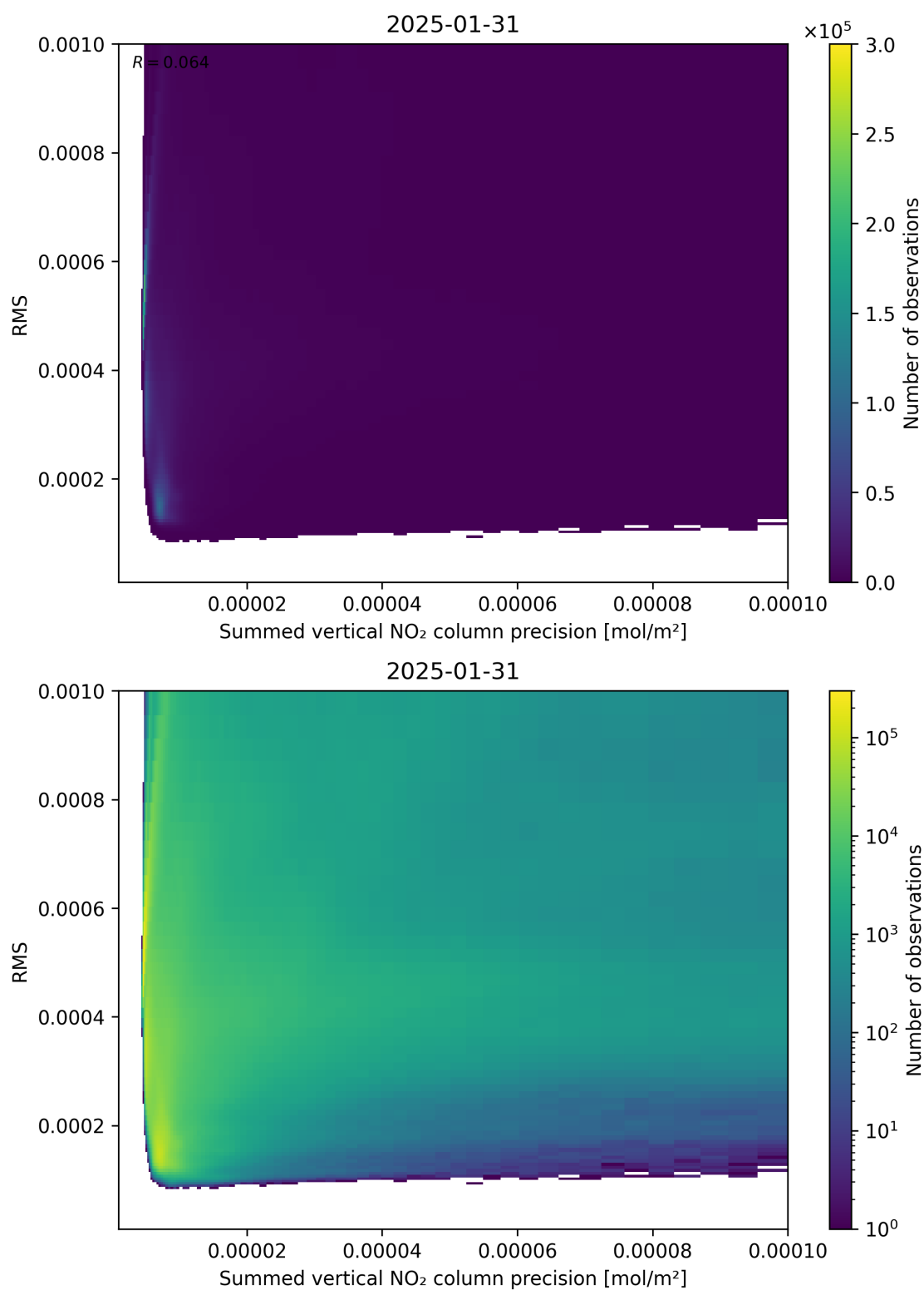
Figure 108: Scatter density plot of “Summed vertical NO 2 column precision” against “RMS” for 2025-01-30 to 2025-02-01.
