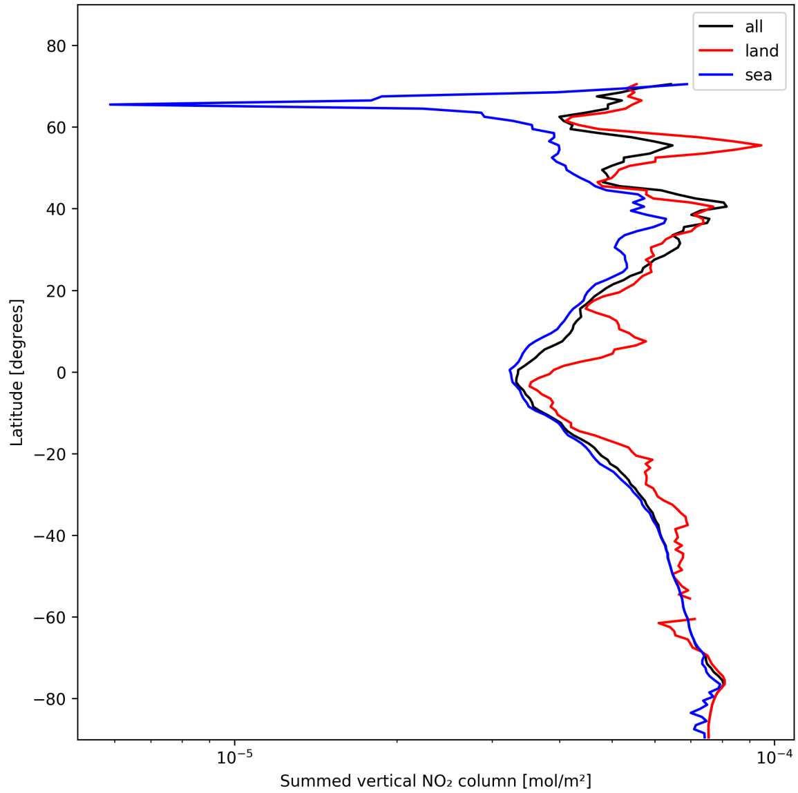
Figure 23: Zonal average of “Summed vertical NO 2 column” for 2025-01-30 to 2025-02-01.
