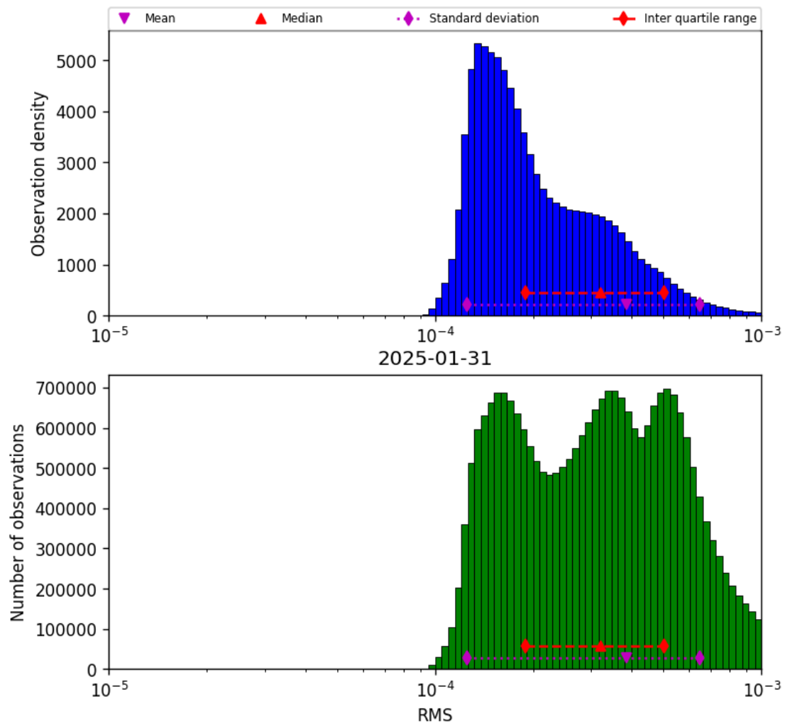
Figure 43: Histogram of “RMS” for 2025-01-30 to 2025-02-01
