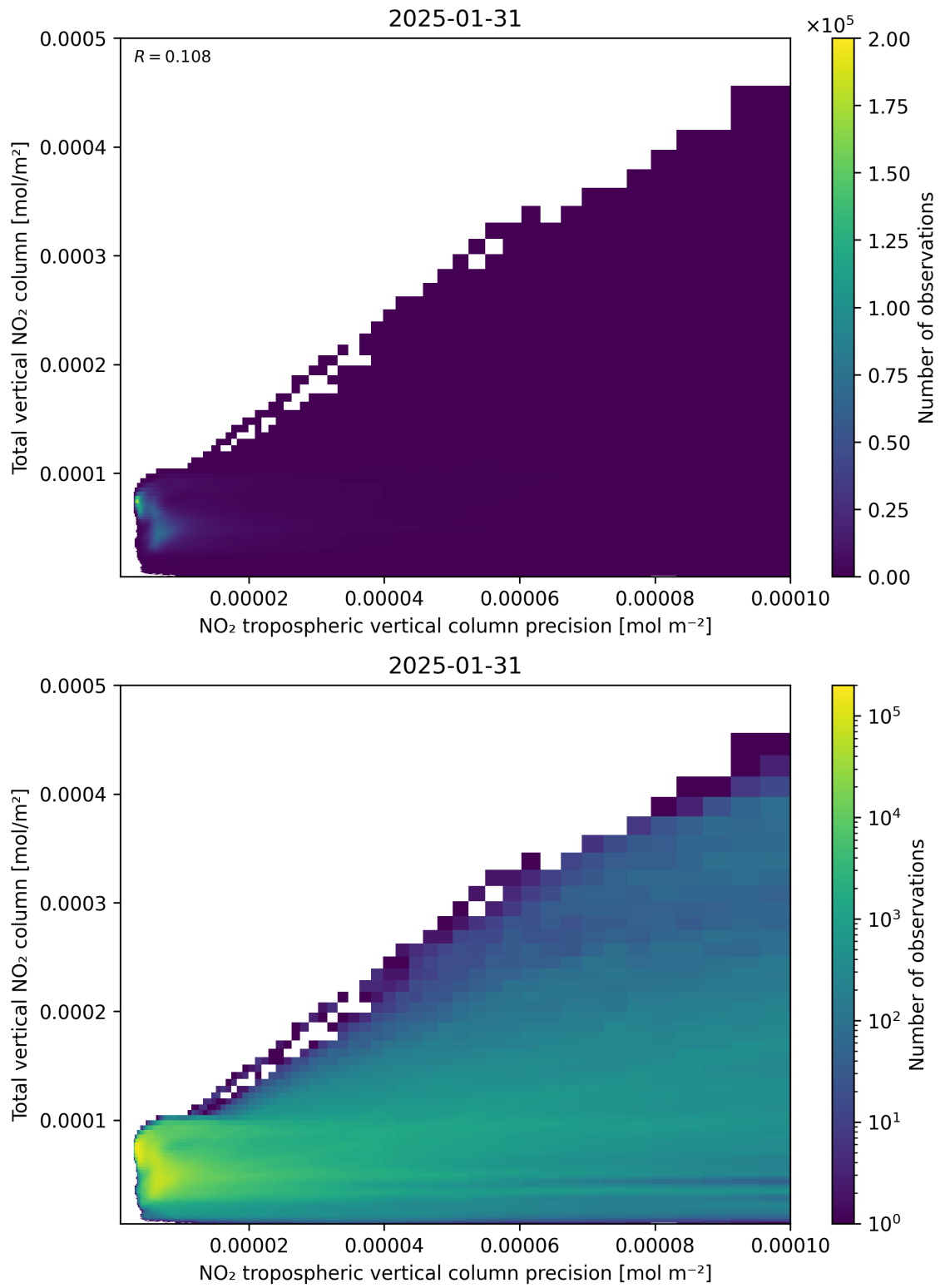
Figure 138: Scatter density plot of “NO 2 tropospheric vertical column precision” against “Total vertical NO 2 column” for 2025-01-30 to 2025-02-01.
