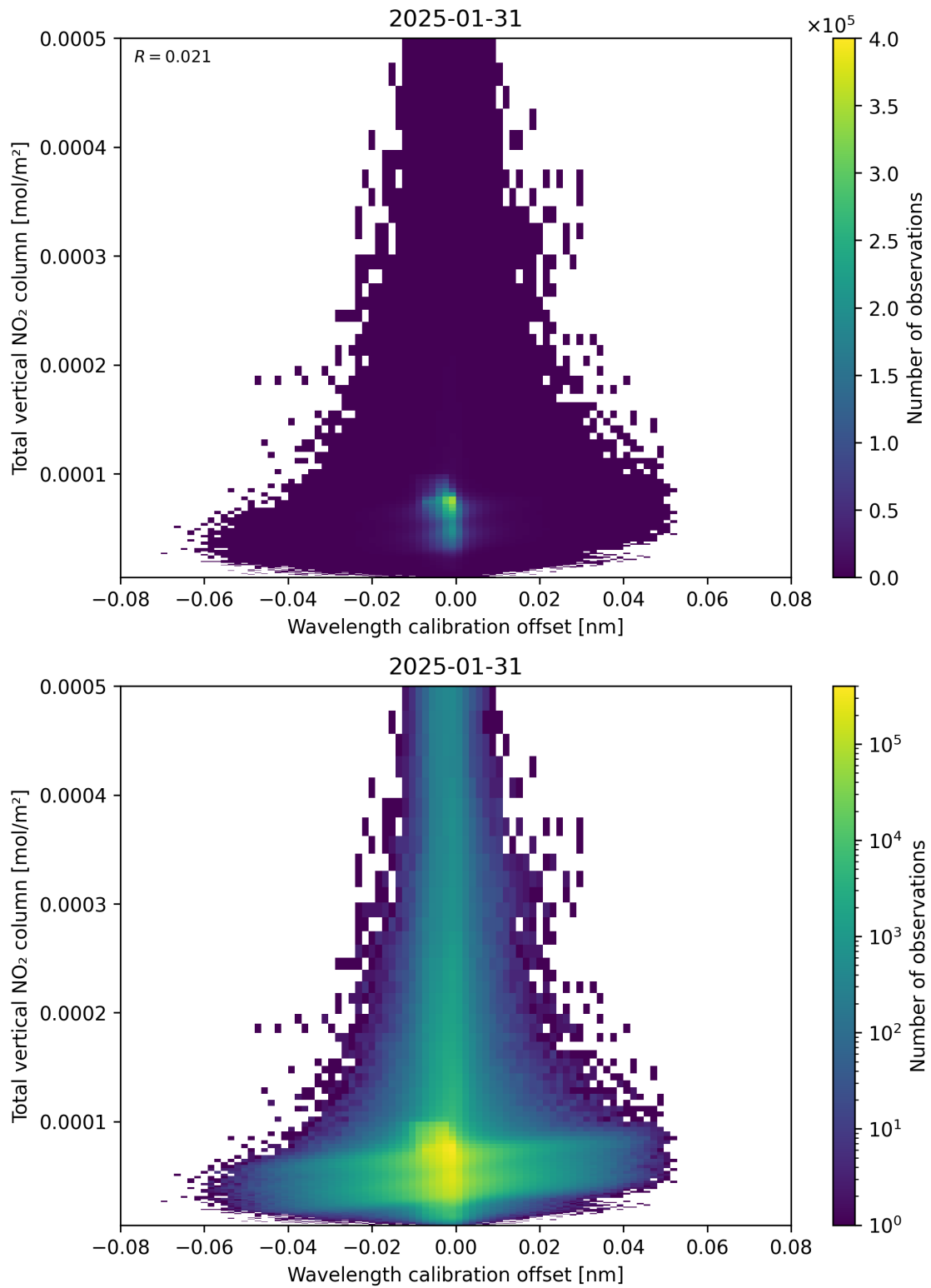
Figure 179: Scatter density plot of “Wavelength calibration offset” against “Total vertical NO 2 column” for 2025-01-30 to 2025-02-01.
