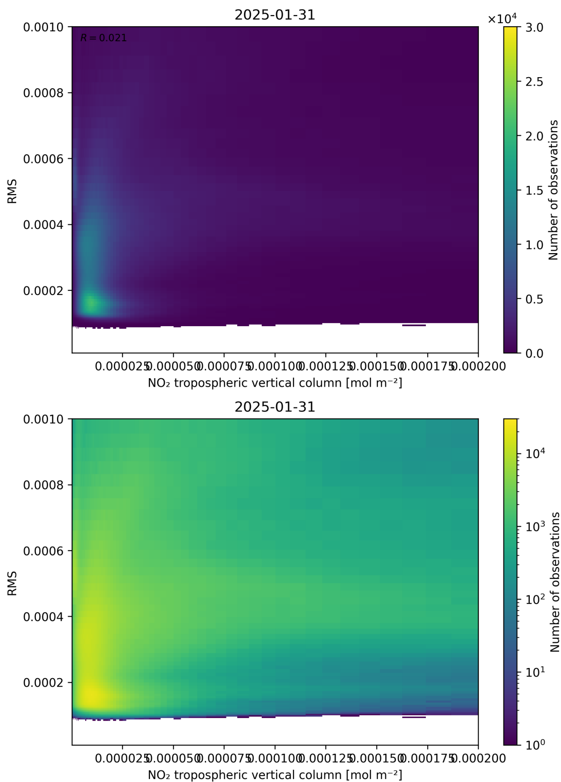
Figure 142: Scatter density plot of “NO 2 tropospheric vertical column” against “RMS” for 2025-01-30 to 2025-02-01.
