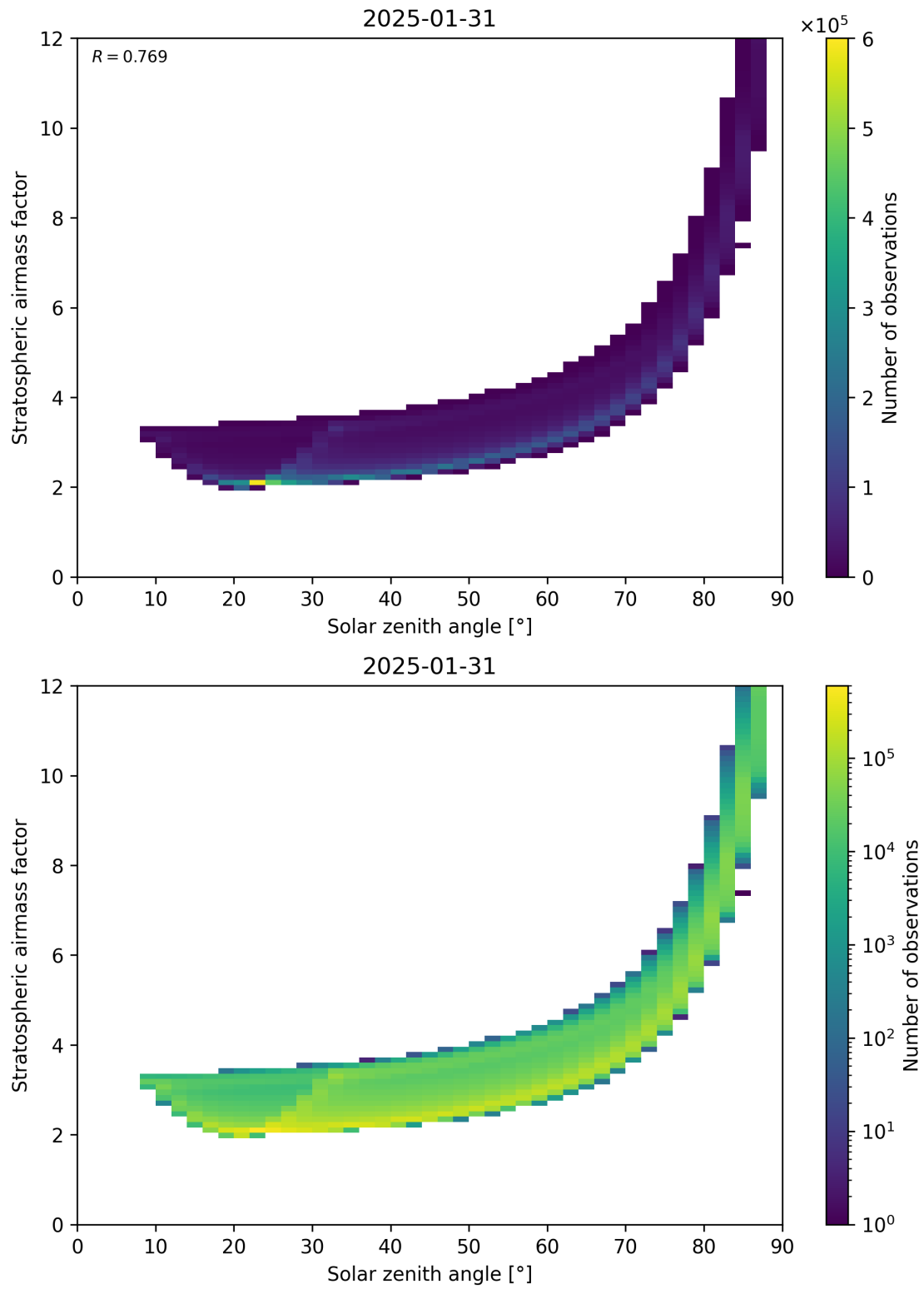
Figure 145: Scatter density plot of “Solar zenith angle” against “Stratospheric airmass factor” for 2025-01-30 to 2025-02-01.
