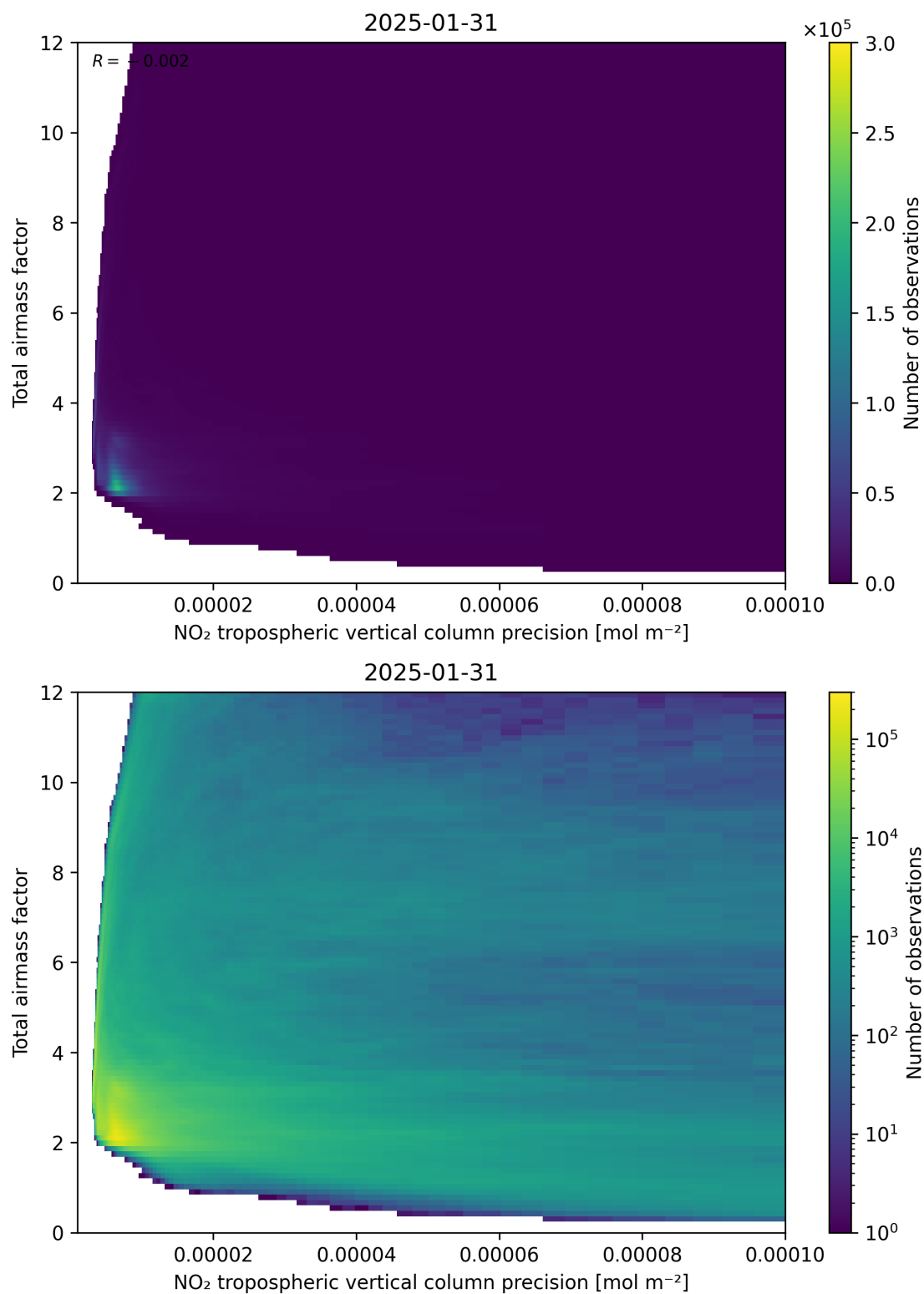
Figure 132: Scatter density plot of “NO 2 tropospheric vertical column precision” against “Total air mass factor” for 2025-01-30 to 2025-02-01.
