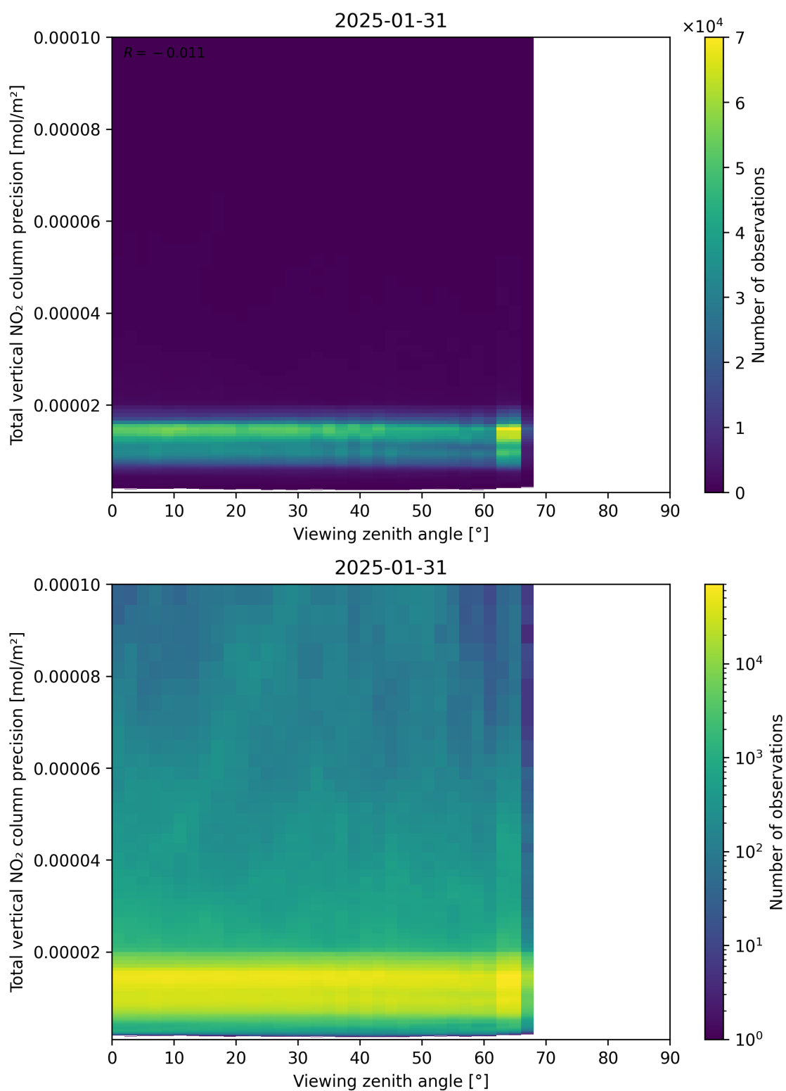
Figure 168: Scatter density plot of “Viewing zenith angle” against “Total vertical NO 2 column precision” for 2025-01-30 to 2025-02-01.
