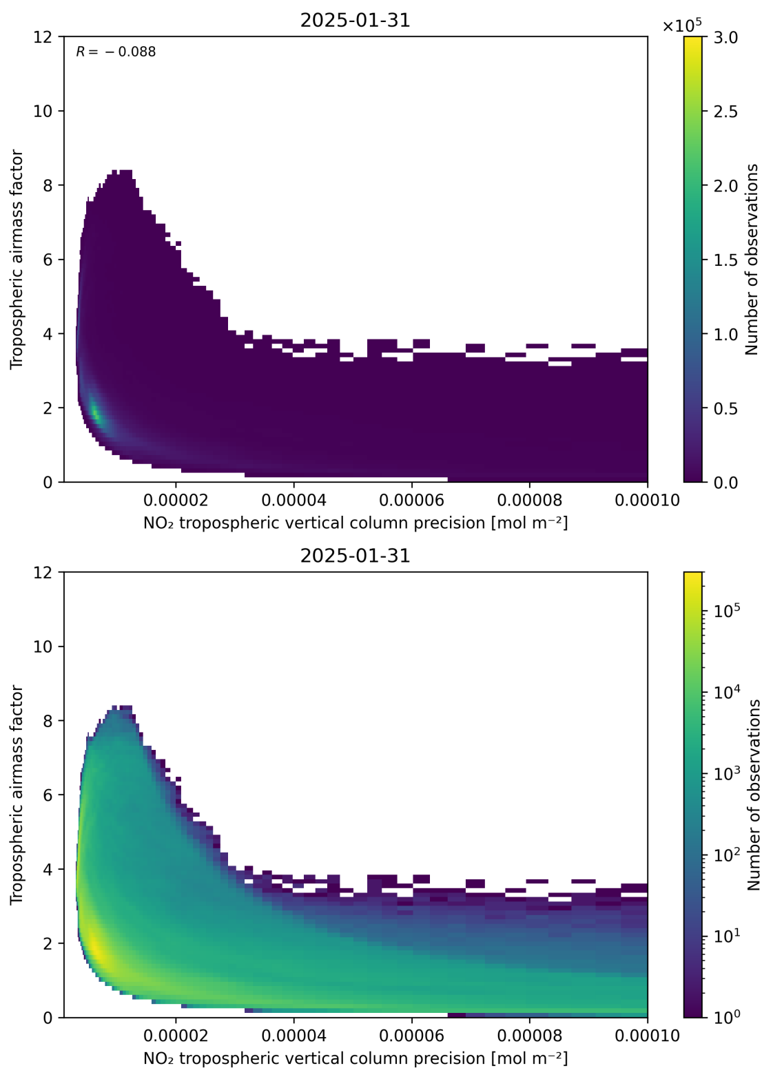
Figure 133: Scatter density plot of “NO 2 tropospheric vertical column precision” against “Tropospheric airmass factor” for 2025-01-30 to 2025-02-01.
