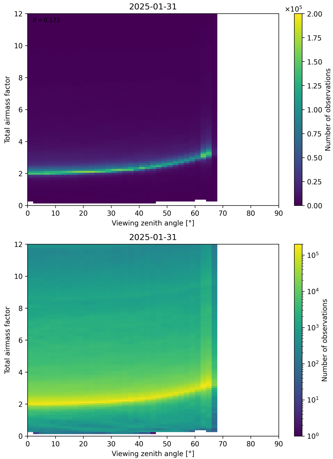
Figure 160: Scatter density plot of “Viewing zenith angle” against “Total airmass factor” for 2025-01-30 to 2025-02-01.
