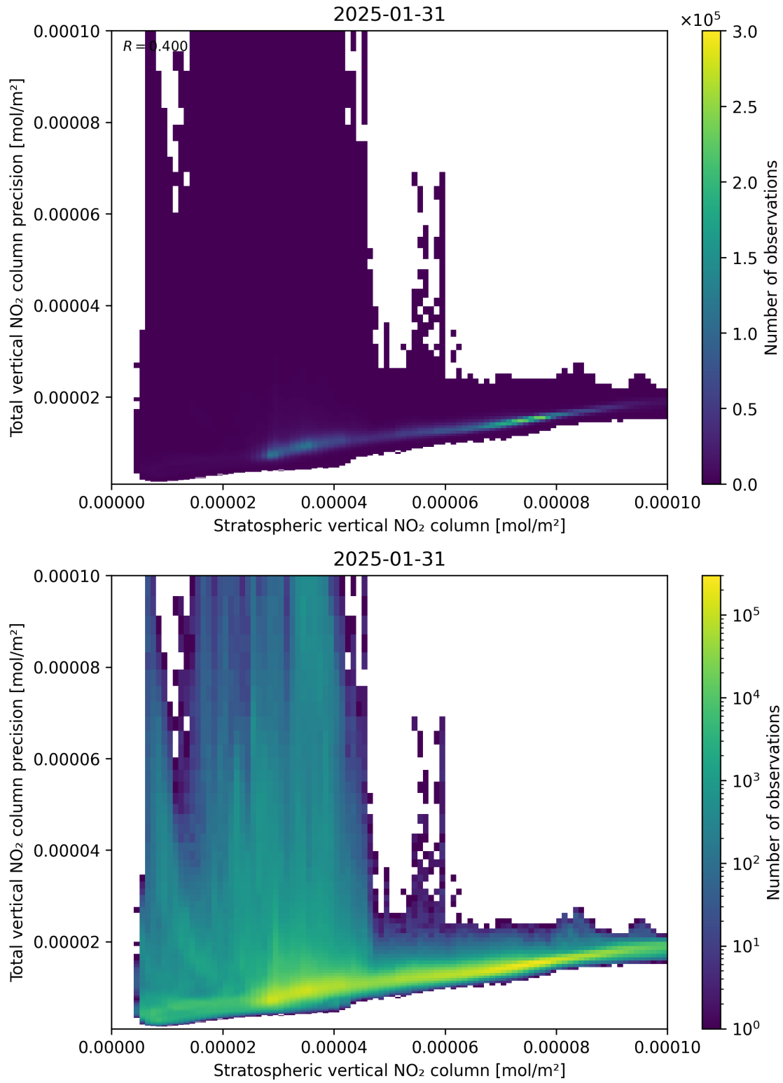
Figure 101: Scatter density plot of “Stratospheric vertical NO 2 column” against “Total vertical NO 2 column precision” for 2025-01-30 to 2025-02-01.
