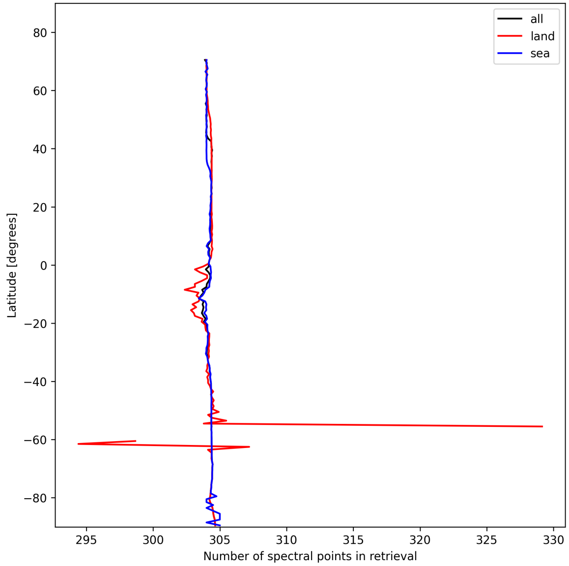
Figure 16: Zonal average of “Number of spectral points in retrieval” for 2025-01-30 to 2025-02-01.
