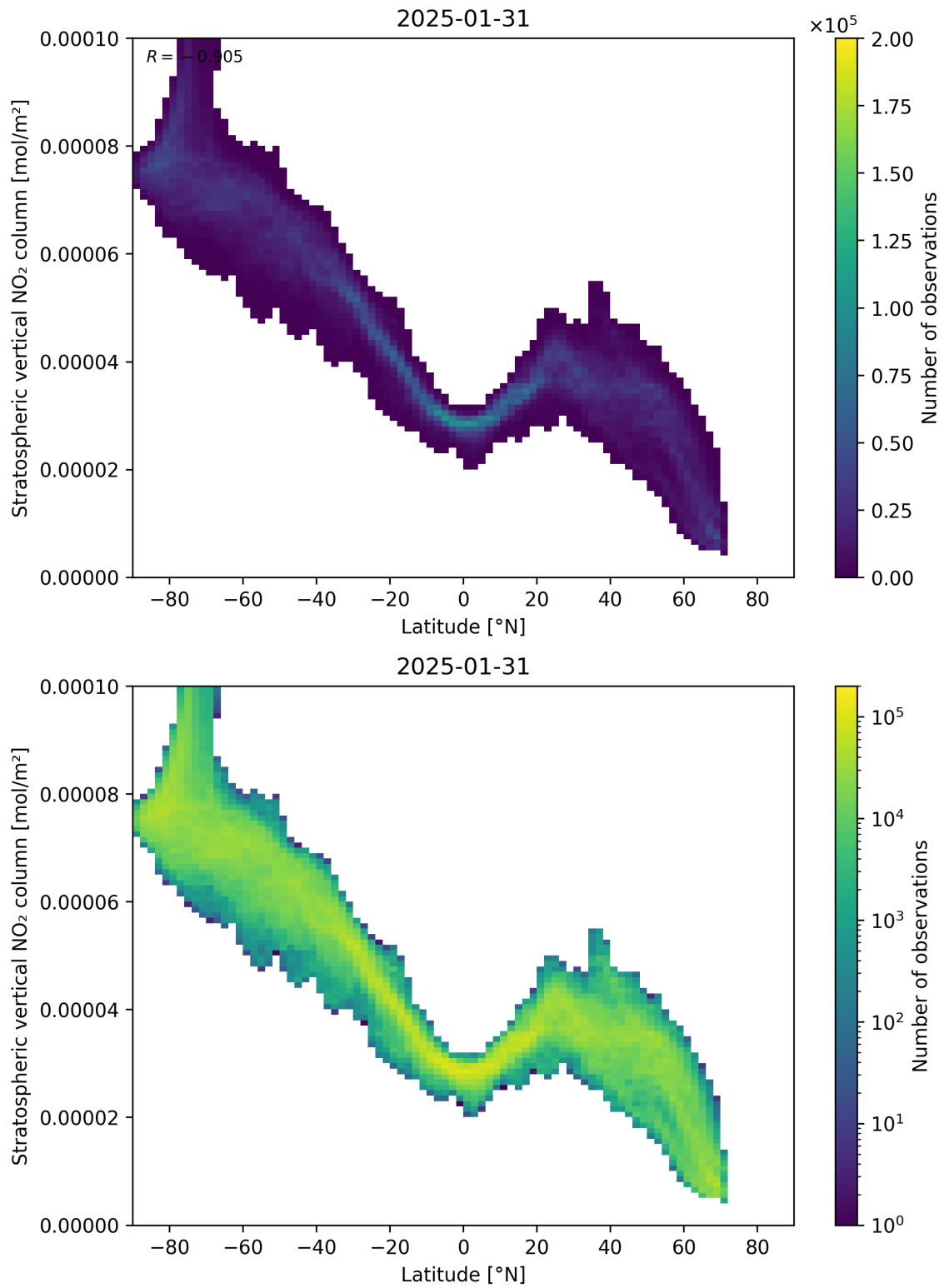
Figure 87: Scatter density plot of “Latitude” against “Stratospheric vertical NO 2 column” for 2025-01-30 to 2025-02-01.
