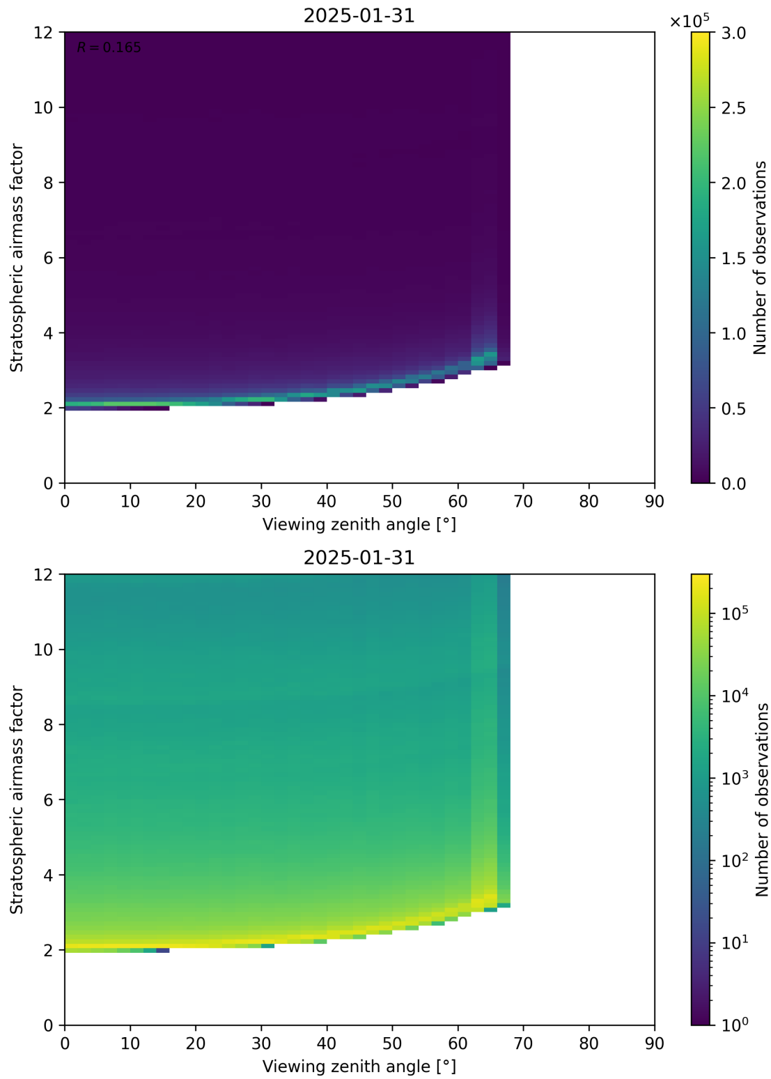
Figure 159: Scatter density plot of “Viewing zenith angle” against “Stratospheric airmass factor” for 2025-01-30 to 2025-02-01.
