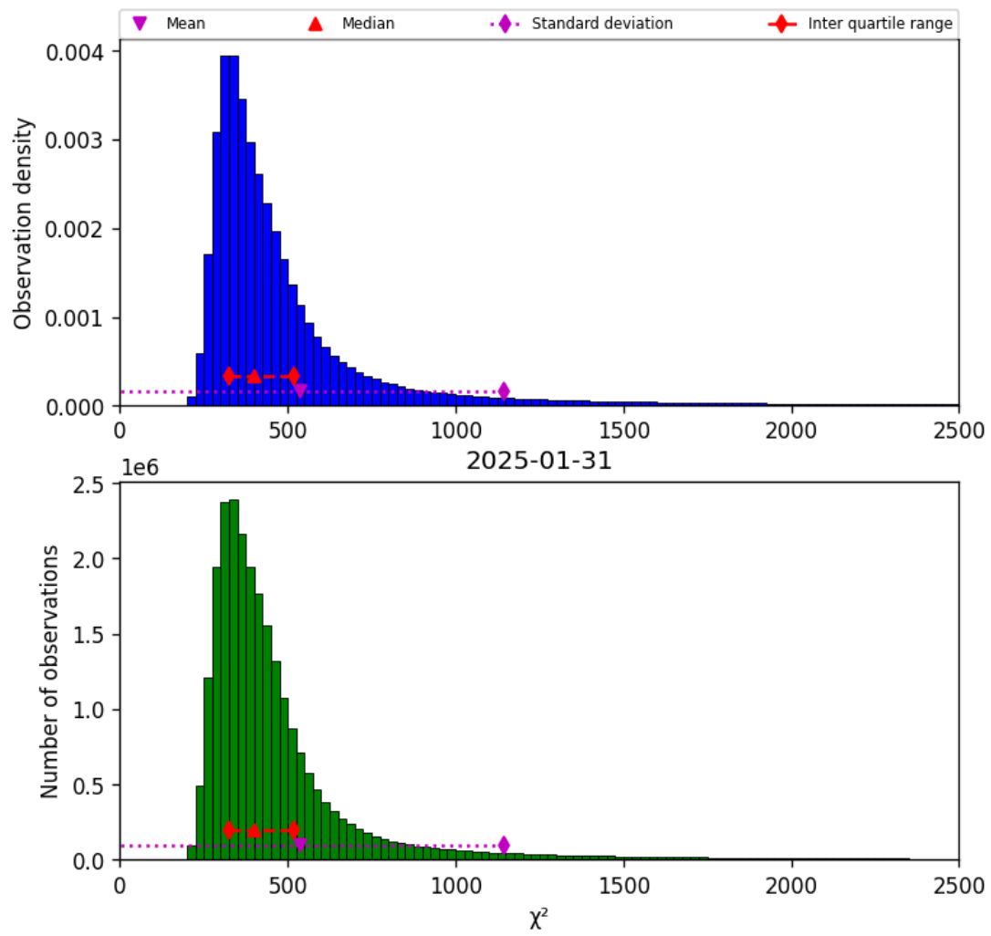
Figure 42: Histogram of “ \chi^2 ” for 2025-01-30 to 2025-02-01
