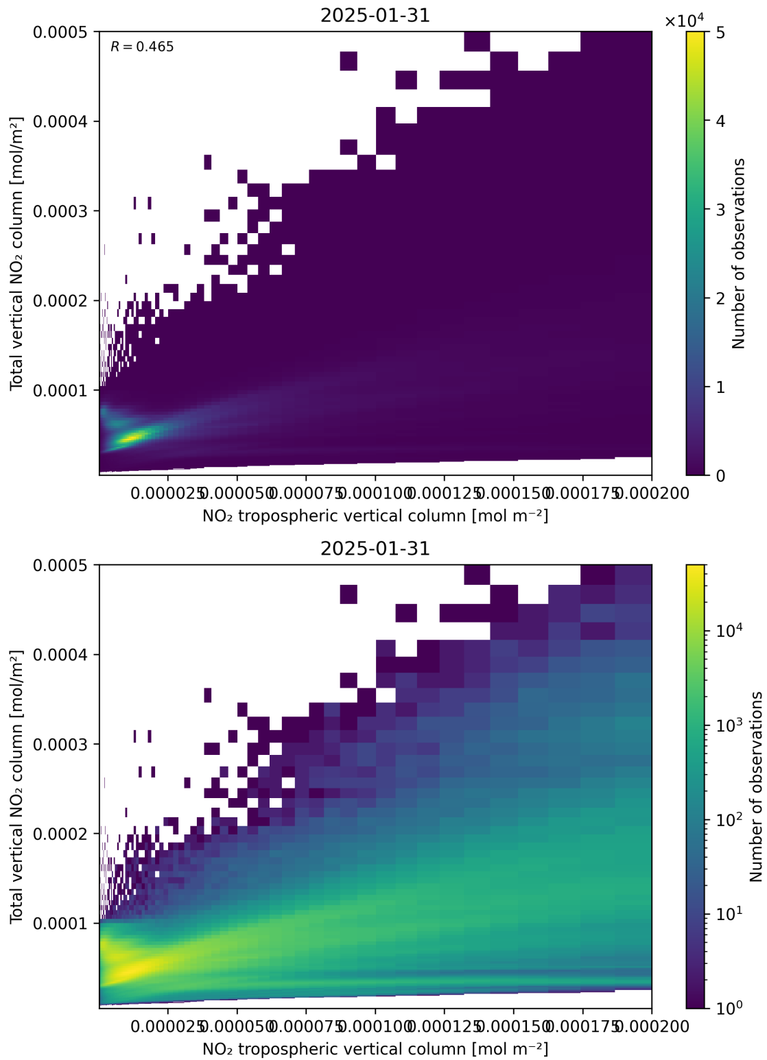
Figure 128: Scatter density plot of “NO 2 tropospheric vertical column” against “Total vertical NO 2 column” for 2025-01-30 to 2025-02-01.
