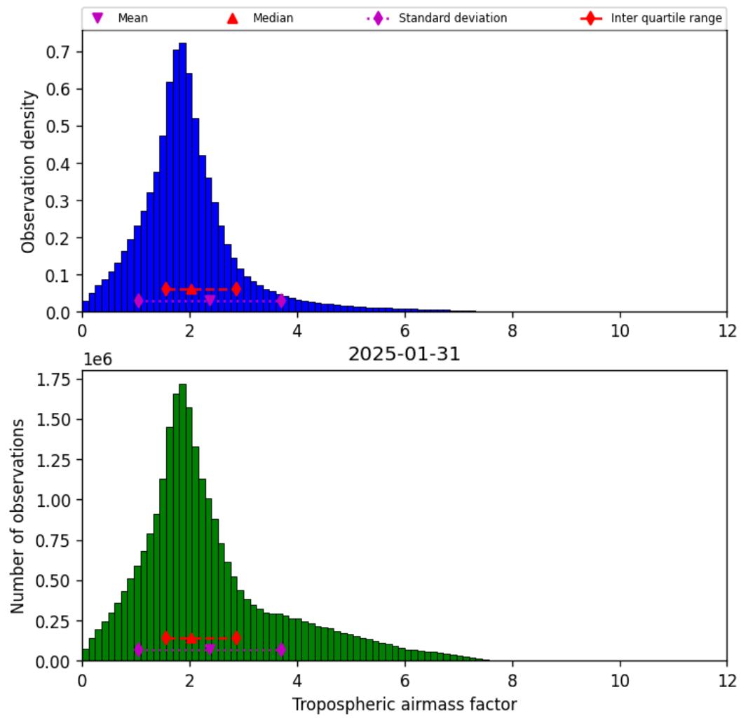
Figure 31: Histogram of “Tropospheric airmass factor” for 2025-01-30 to 2025-02-01
