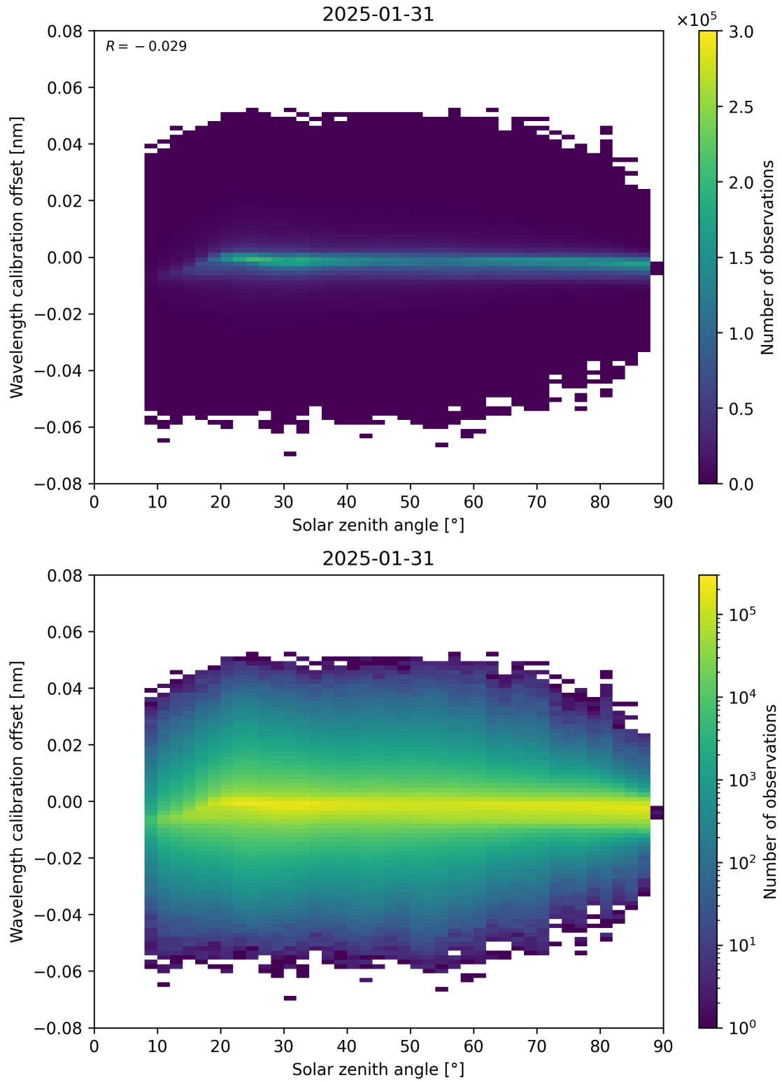
Figure 158: Scatter density plot of “Solar zenith angle” against “Wavelength calibration offset” for 2025-01-30 to 2025-02-01.
