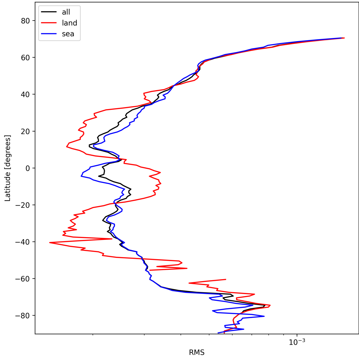
Figure 26: Zonal average of “RMS” for 2025-01-30 to 2025-02-01.
