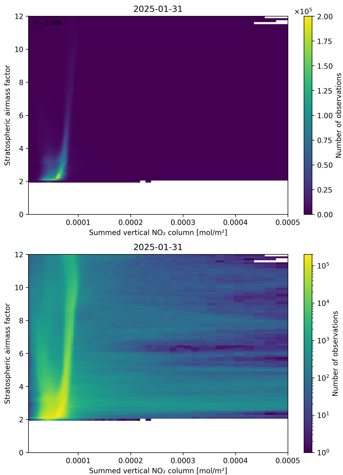
Figure 103: Scatter density plot of “Summed vertical NO 2 column” against “Stratospheric air mass factor” for 2025-01-30 to 2025-02-01.
