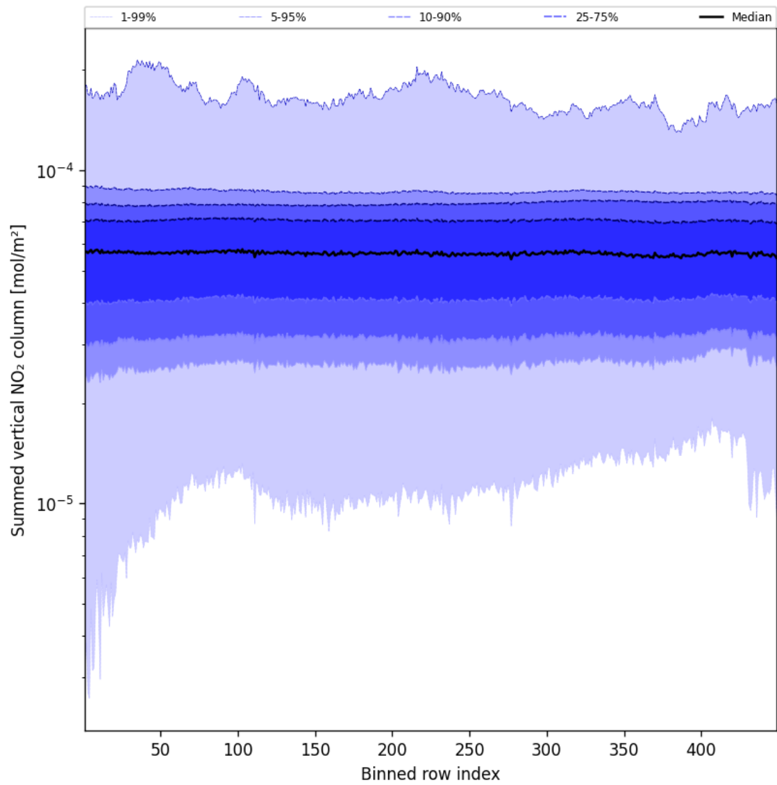
Figure 57: Along track statistics of “Summed vertical NO 2 column” for 2025-01-30 to 2025-02-01
