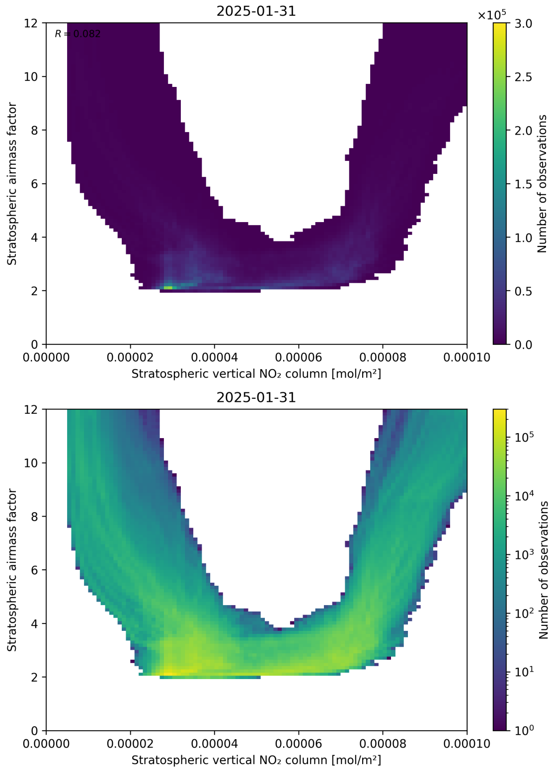
Figure 96: Scatter density plot of “Stratospheric vertical NO 2 column” against “Stratospheric airmass factor” for 2025-01-30 to 2025-02-01.
