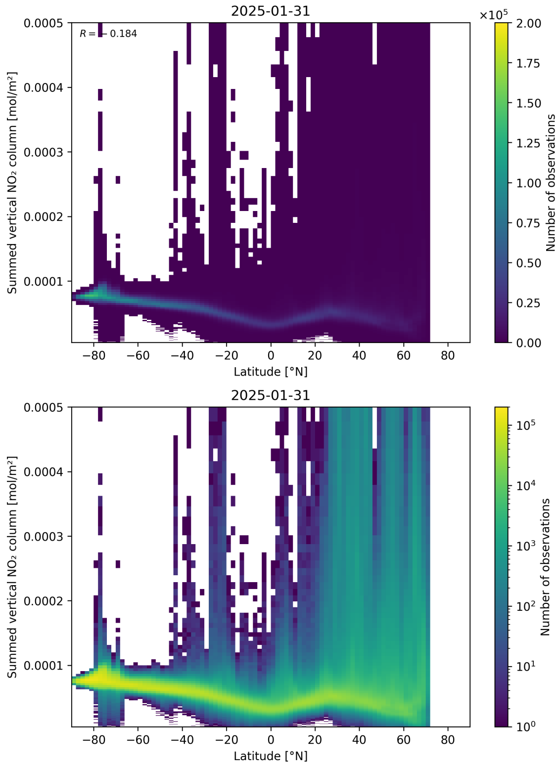
Figure 88: Scatter density plot of “Latitude” against “Summed vertical NO 2 column” for 2025-01-30 to 2025-02-01.
