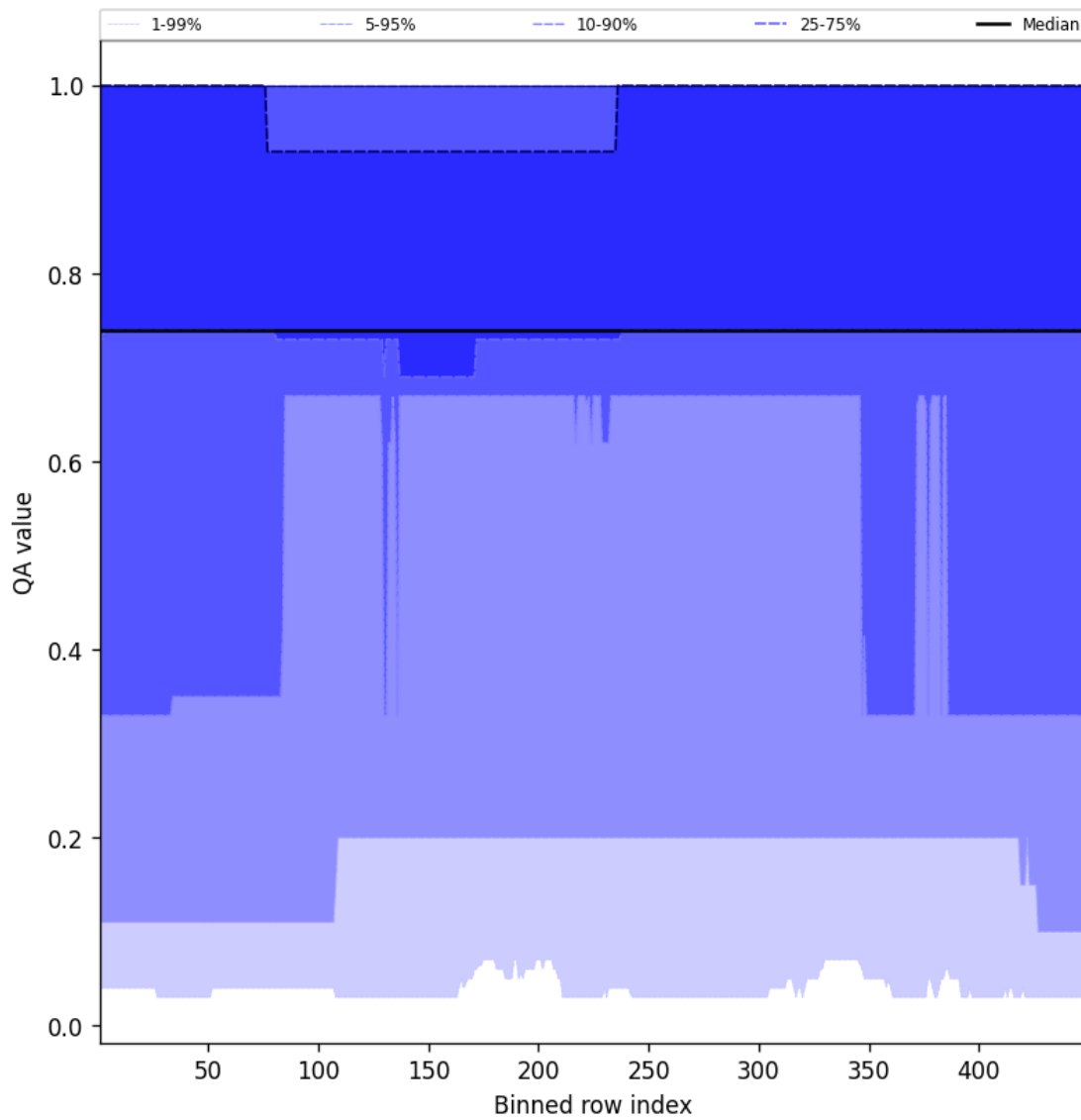
Figure 45: Along track statistics of “QA value” for 2025-01-30 to 2025-02-01
