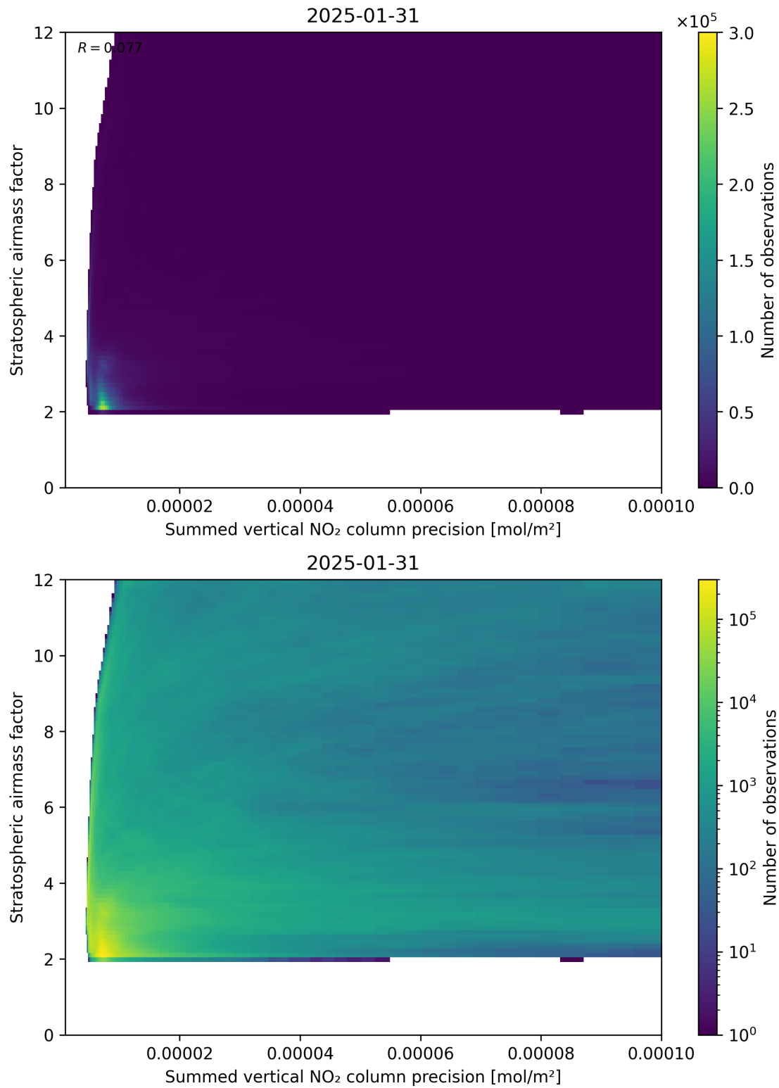
Figure 106: Scatter density plot of “Summed vertical NO 2 column precision” against “Stratospheric airmass factor” for 2025-01-30 to 2025-02-01.
