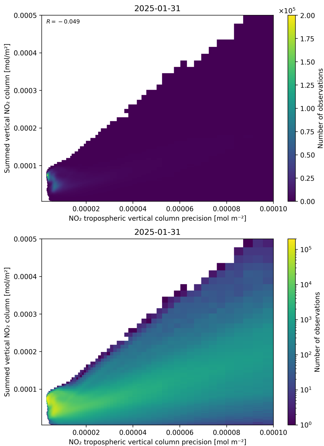
Figure 136: Scatter density plot of “NO 2 tropospheric vertical column precision” against “Summed vertical NO 2 column” for 2025-01-30 to 2025-02-01.
