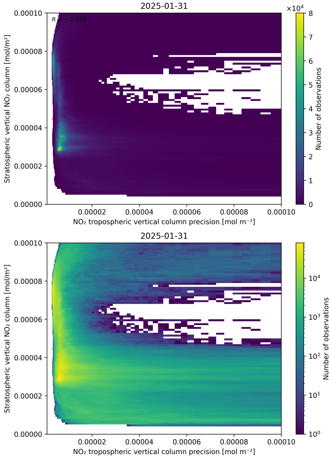
Figure 135: Scatter density plot of “NO 2 tropospheric vertical column precision” against “Stratospheric vertical NO 2 column” for 2025-01-30 to 2025-02-01.
