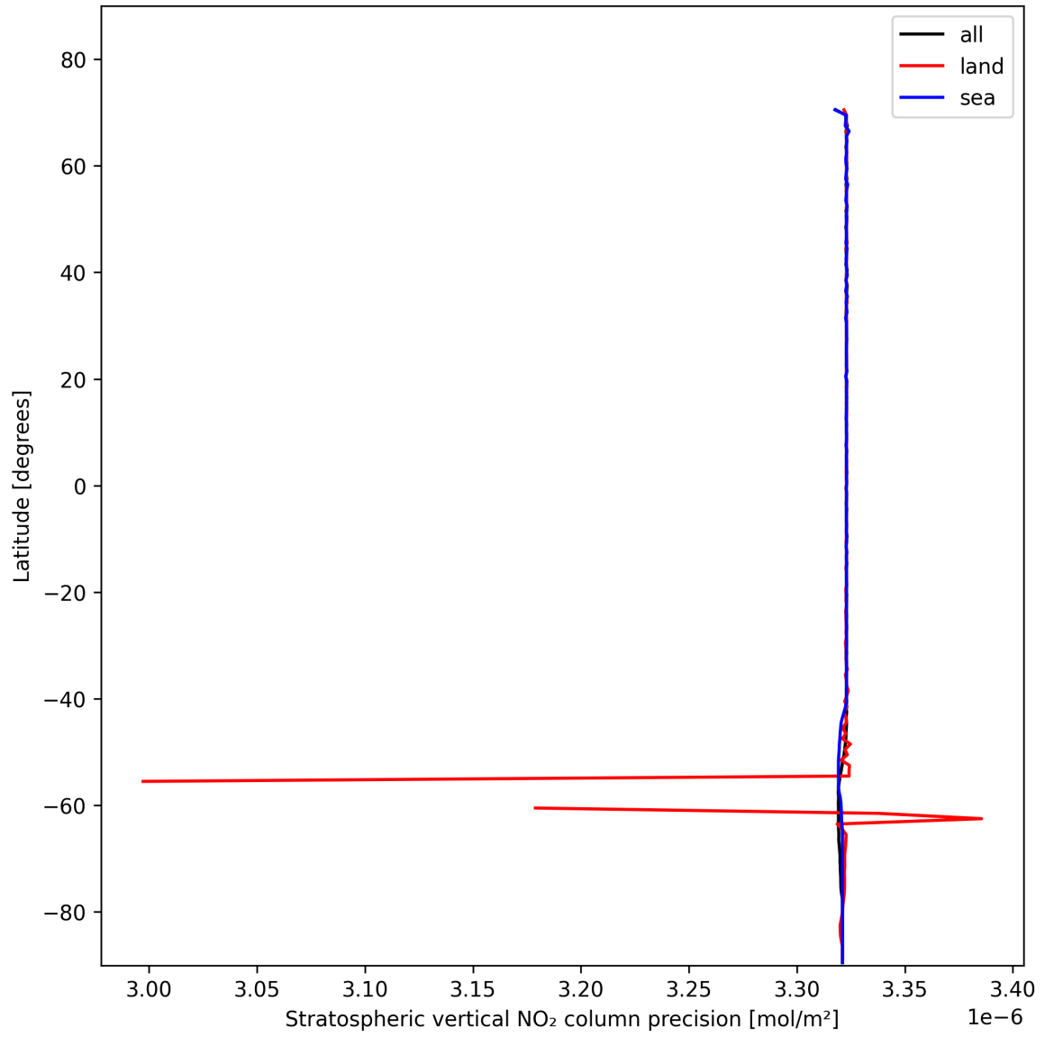
Figure 20: Zonal average of “Stratospheric vertical NO 2 column precision” for 2025-01-30 to 2025-02-01.
