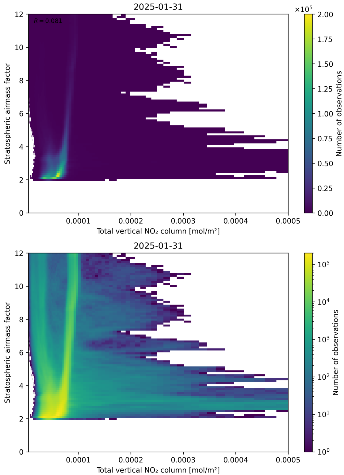
Figure 110: Scatter density plot of “Total vertical NO 2 column” against “Stratospheric airmass factor” for 2025-01-30 to 2025-02-01.
