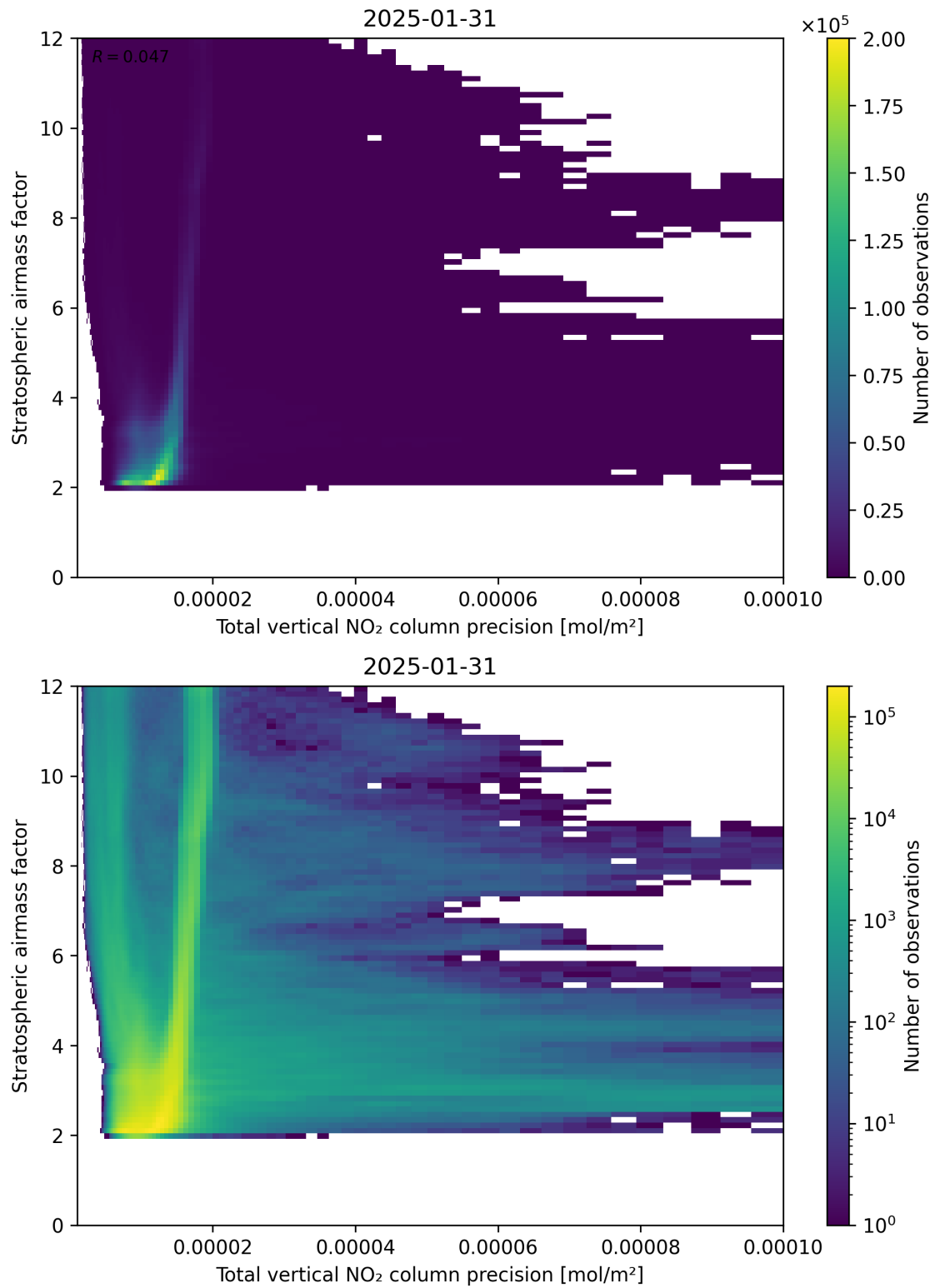
Figure 115: Scatter density plot of “Total vertical NO 2 column precision” against “Stratospheric air mass factor” for 2025-01-30 to 2025-02-01.
