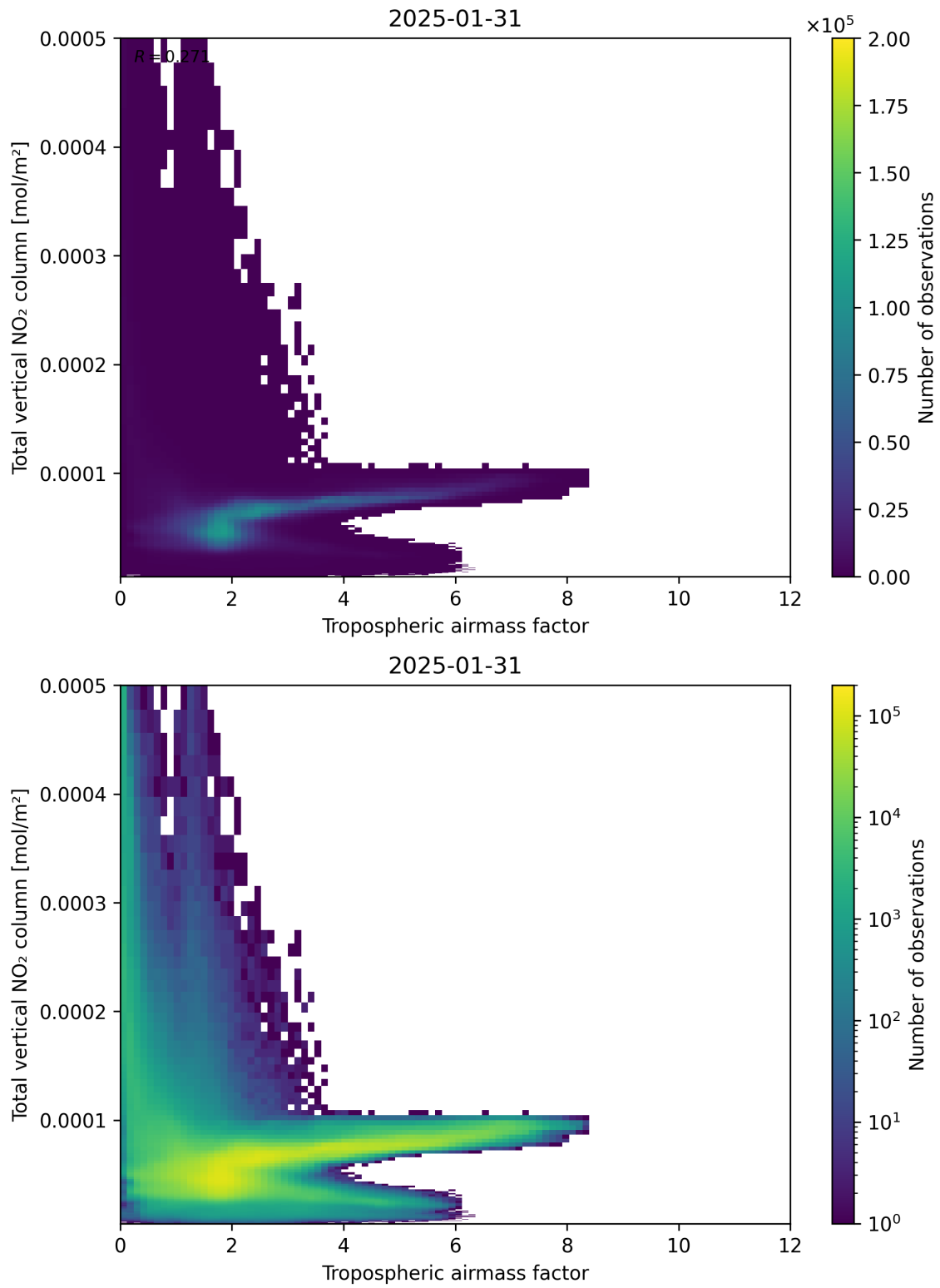
Figure 77: Scatter density plot of “Tropospheric airmass factor” against “Total vertical NO 2 column” for 2025-01-30 to 2025-02-01.
