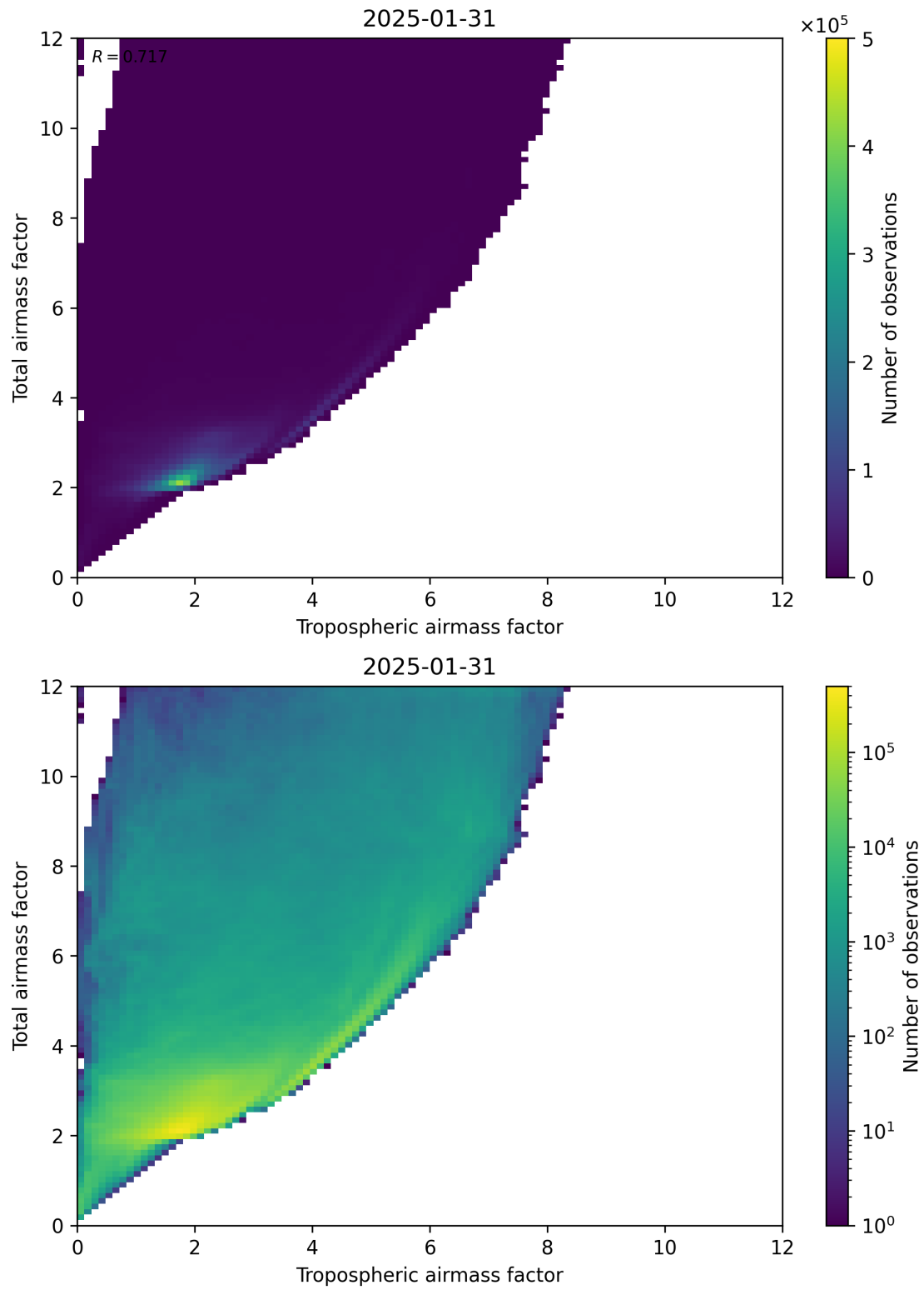
Figure 72: Scatter density plot of “Tropospheric airmass factor” against “Total airmass factor” for 2025-01-30 to 2025-02-01.
