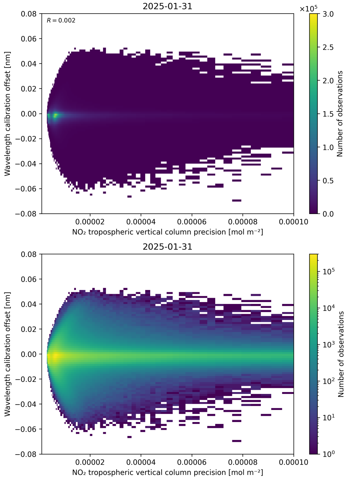
Figure 141: Scatter density plot of “NO 2 tropospheric vertical column precision” against “Wavelength calibration offset” for 2025-01-30 to 2025-02-01.
