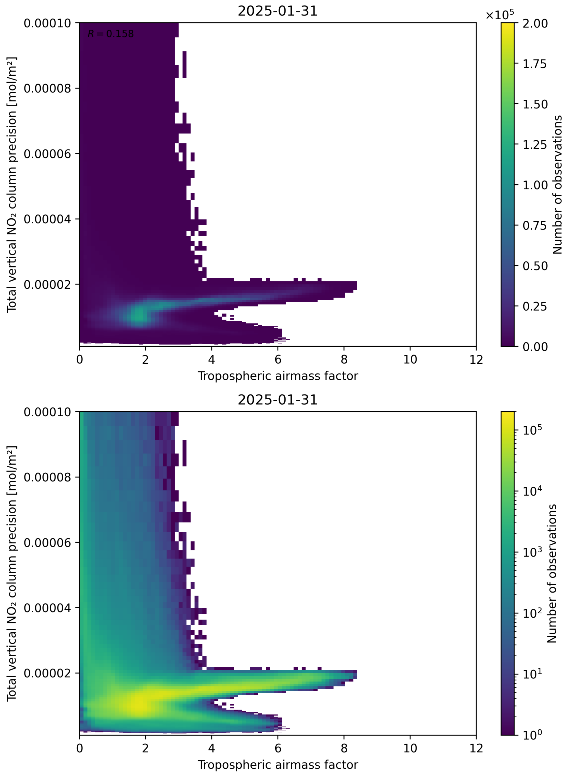
Figure 78: Scatter density plot of “Tropospheric air mass factor” against “Total vertical NO 2 column precision” for 2025-01-30 to 2025-02-01.
