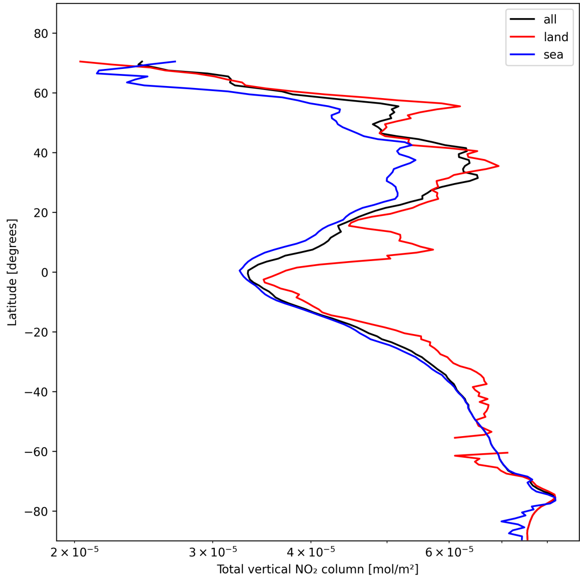
Figure 21: Zonal average of “Total vertical NO 2 column” for 2025-01-30 to 2025-02-01.
