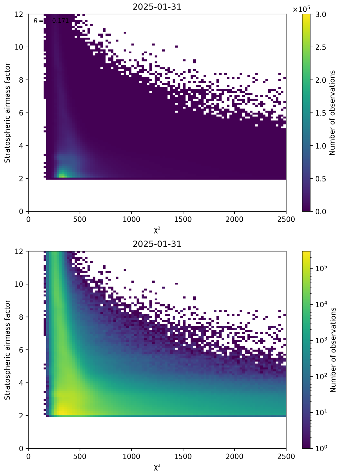
Figure 81: Scatter density plot of “ \chi^2 ” against “Stratospheric airmass factor” for 2025-01-30 to 2025-02-01.
