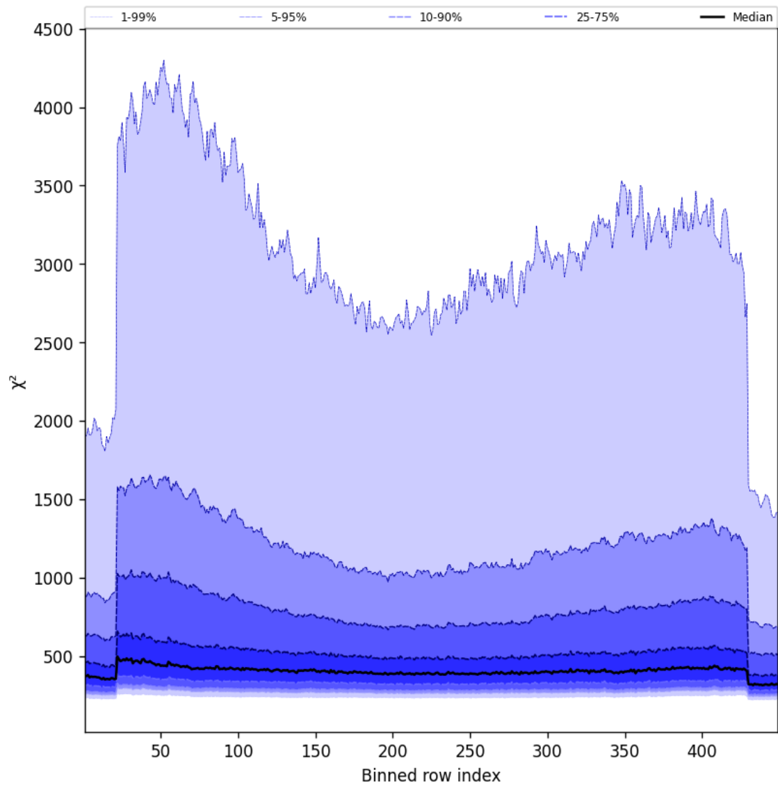
Figure 59: Along track statistics of “ \chi^2 ” for 2025-01-30 to 2025-02-01
