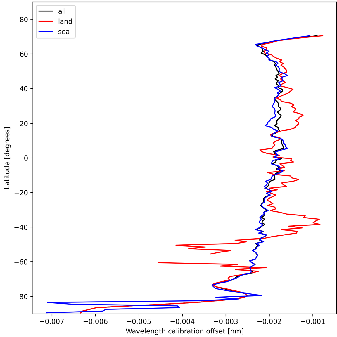
Figure 18: Zonal average of “Wavelength calibration offset” for 2025-01-30 to 2025-02-01.
