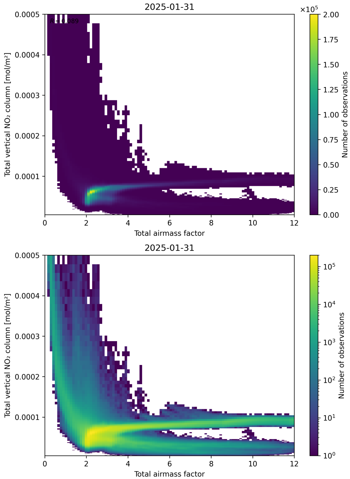
Figure 67: Scatter density plot of “Total airmass factor” against “Total vertical NO 2 column” for 2025-01-30 to 2025-02-01.
