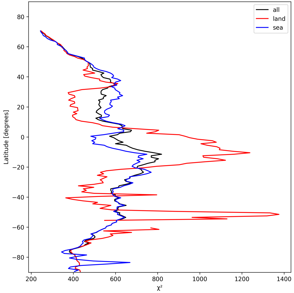
Figure 25: Zonal average of “ \chi^2 ” for 2025-01-30 to 2025-02-01.
