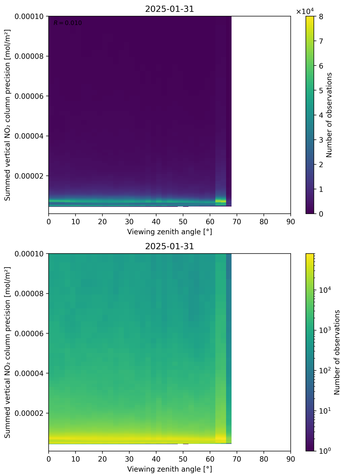
Figure 166: Scatter density plot of “Viewing zenith angle” against “Summed vertical NO 2 column precision” for 2025-01-30 to 2025-02-01.
