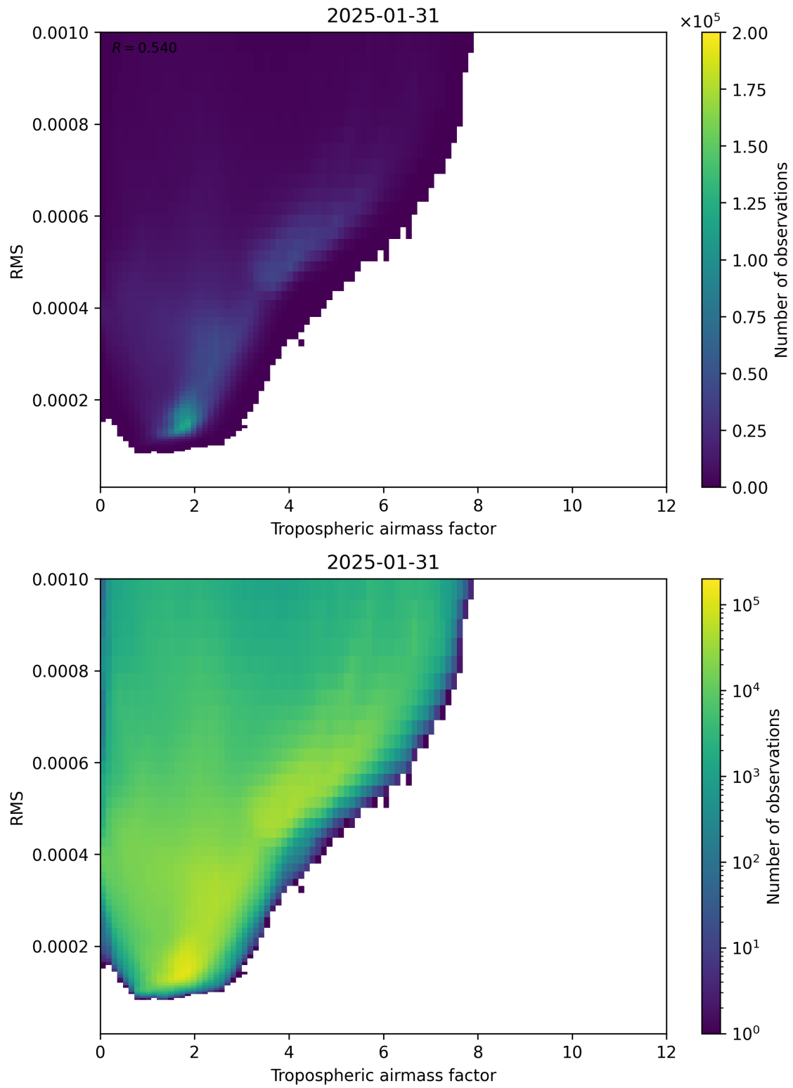
Figure 79: Scatter density plot of “Tropospheric airmass factor” against “RMS” for 2025-01-30 to 2025-02-01.
