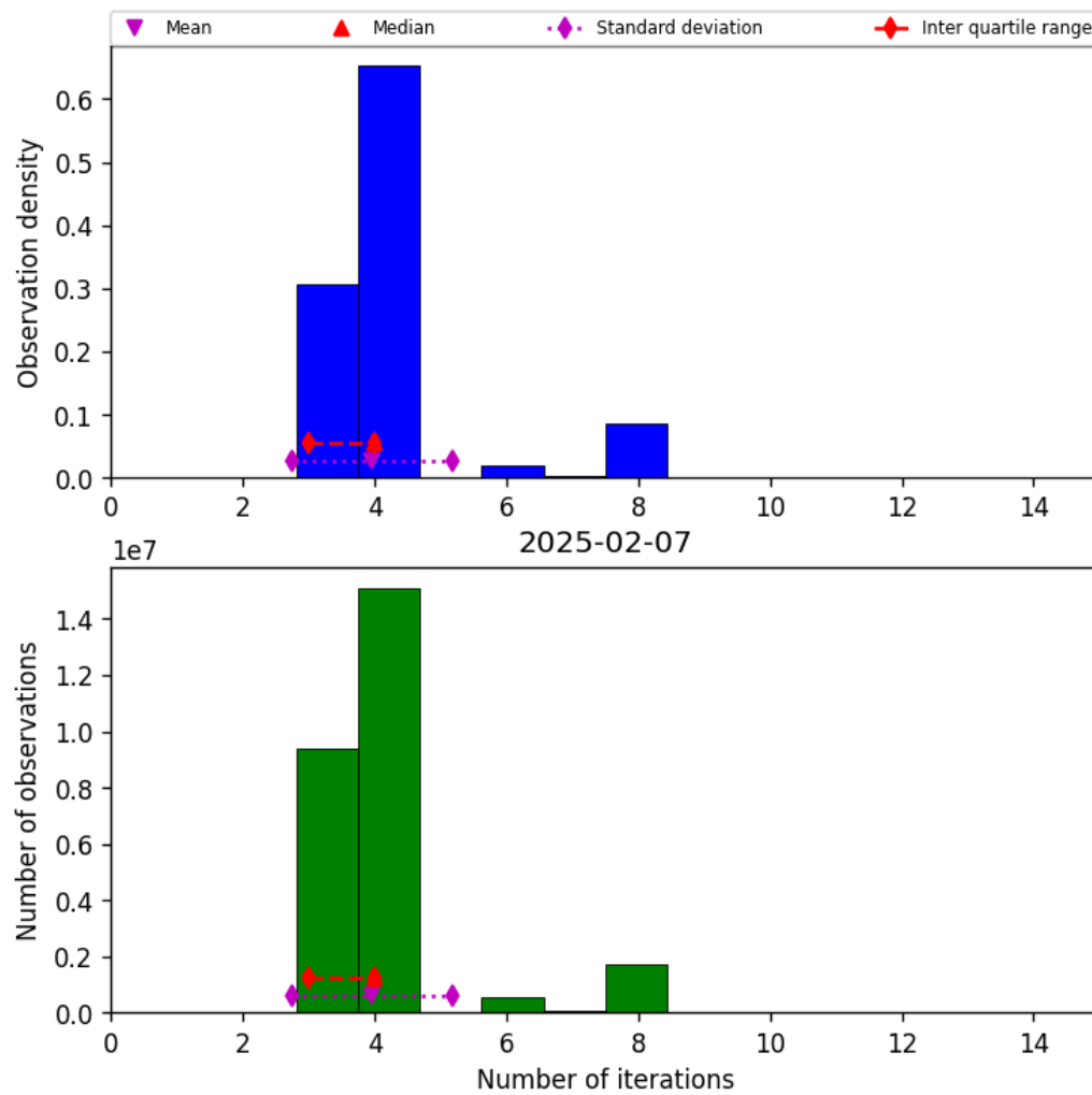
Figure 34: Histogram of “Number of iterations” for 2025-02-06 to 2025-02-08
