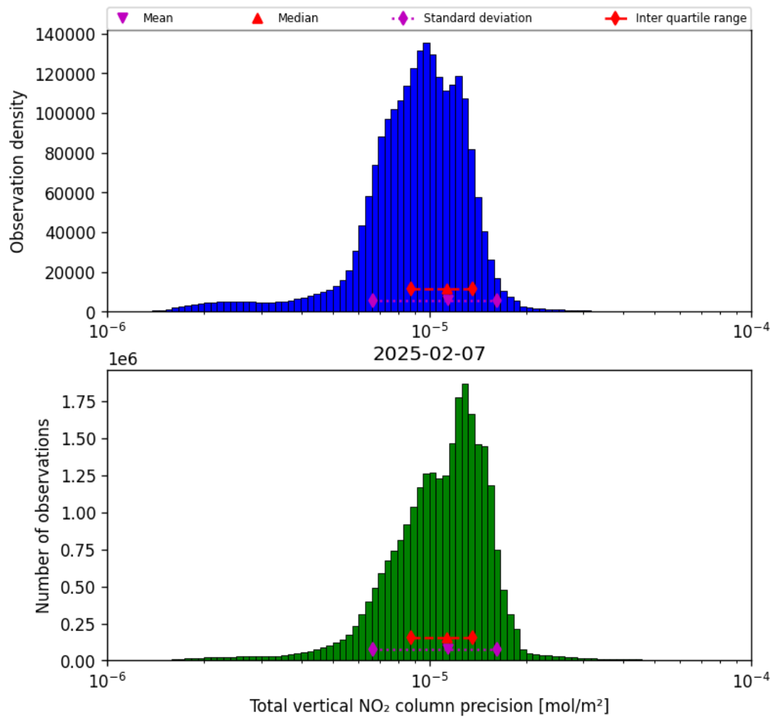
Figure 39: Histogram of “Total vertical NO 2 column precision” for 2025-02-06 to 2025-02-08
