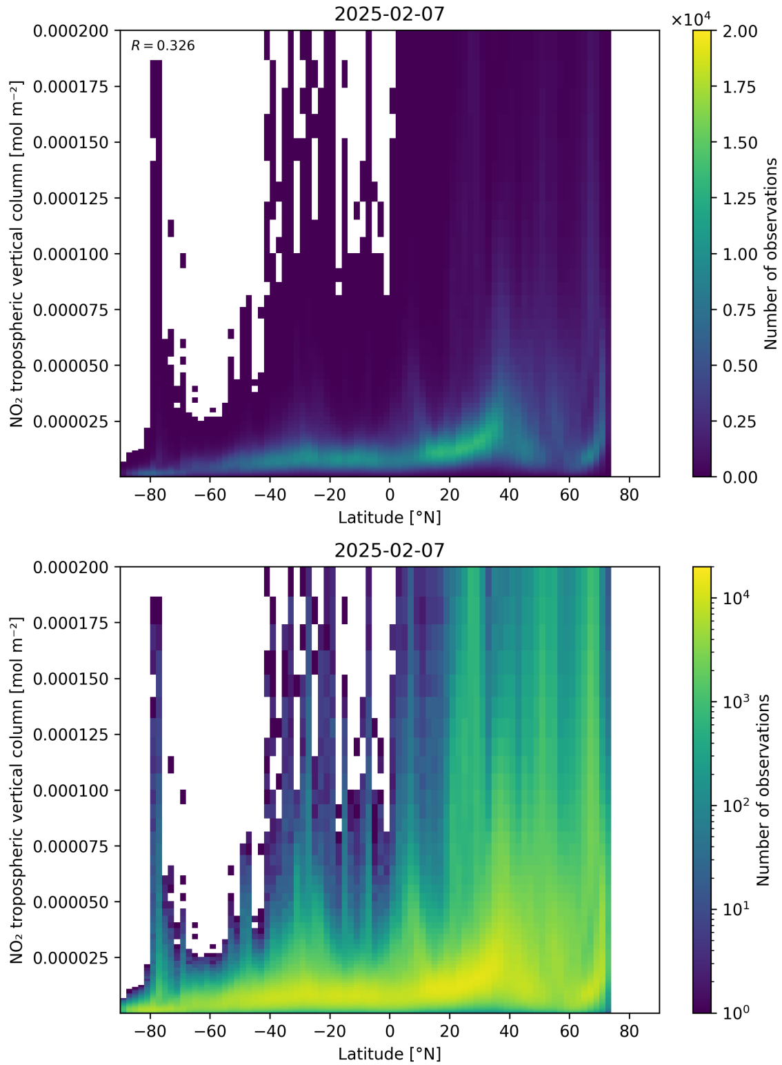
Figure 92: Scatter density plot of “Latitude” against “NO 2 tropospheric vertical column” for 2025-02-06 to 2025-02-08.
