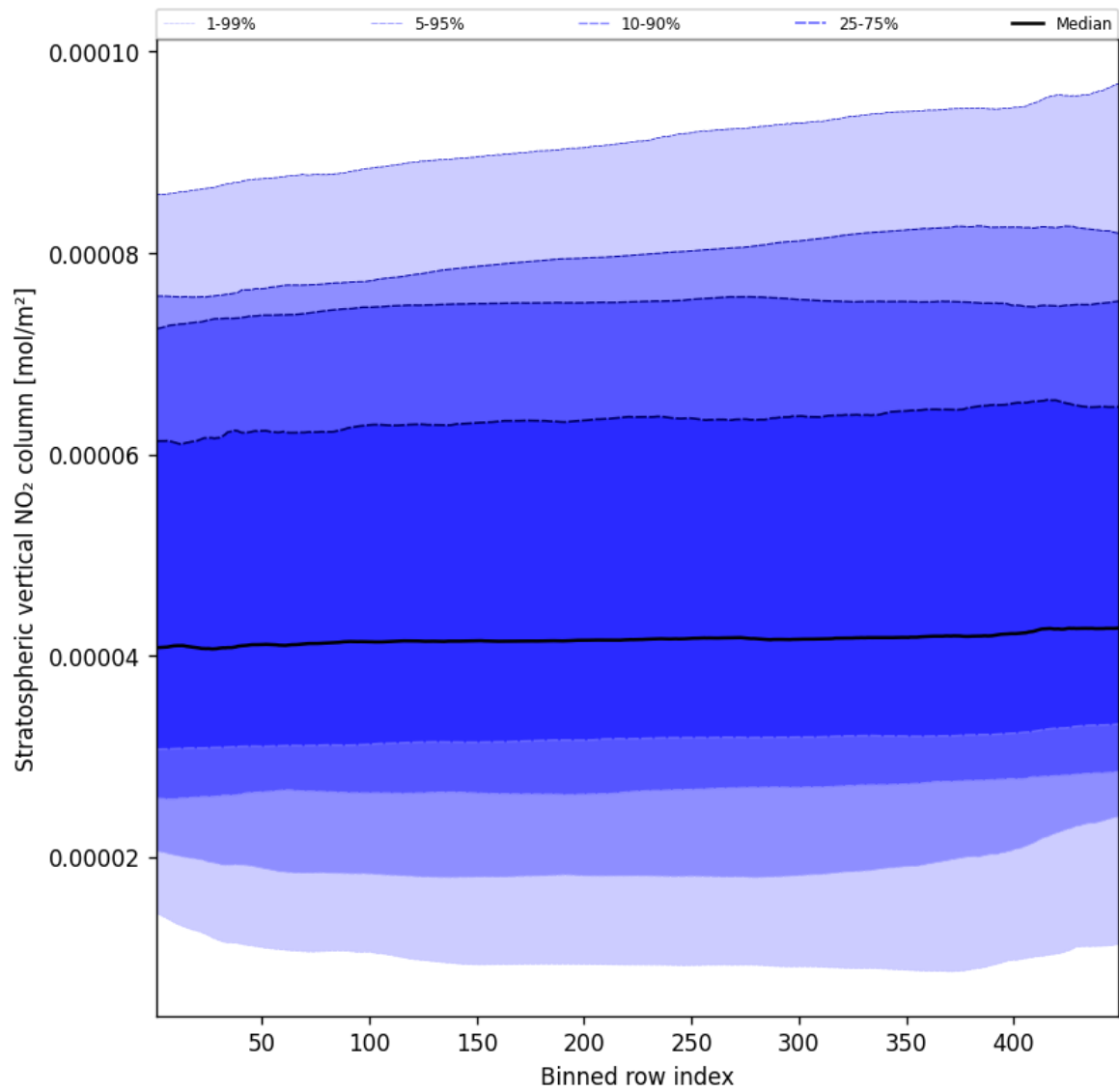
Figure 53: Along track statistics of “Stratospheric vertical NO 2 column” for 2025-02-06 to 2025-02-08
