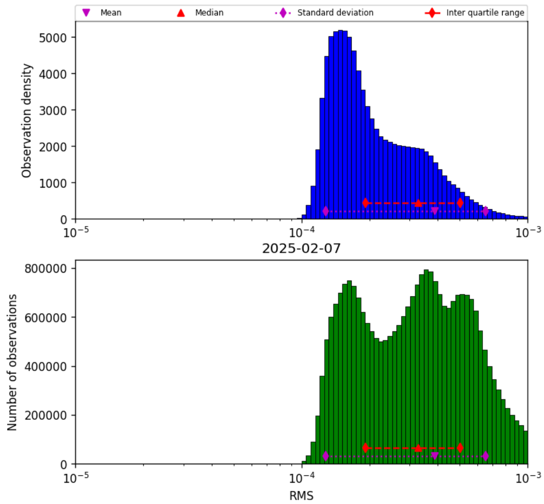
Figure 43: Histogram of “RMS” for 2025-02-06 to 2025-02-08
