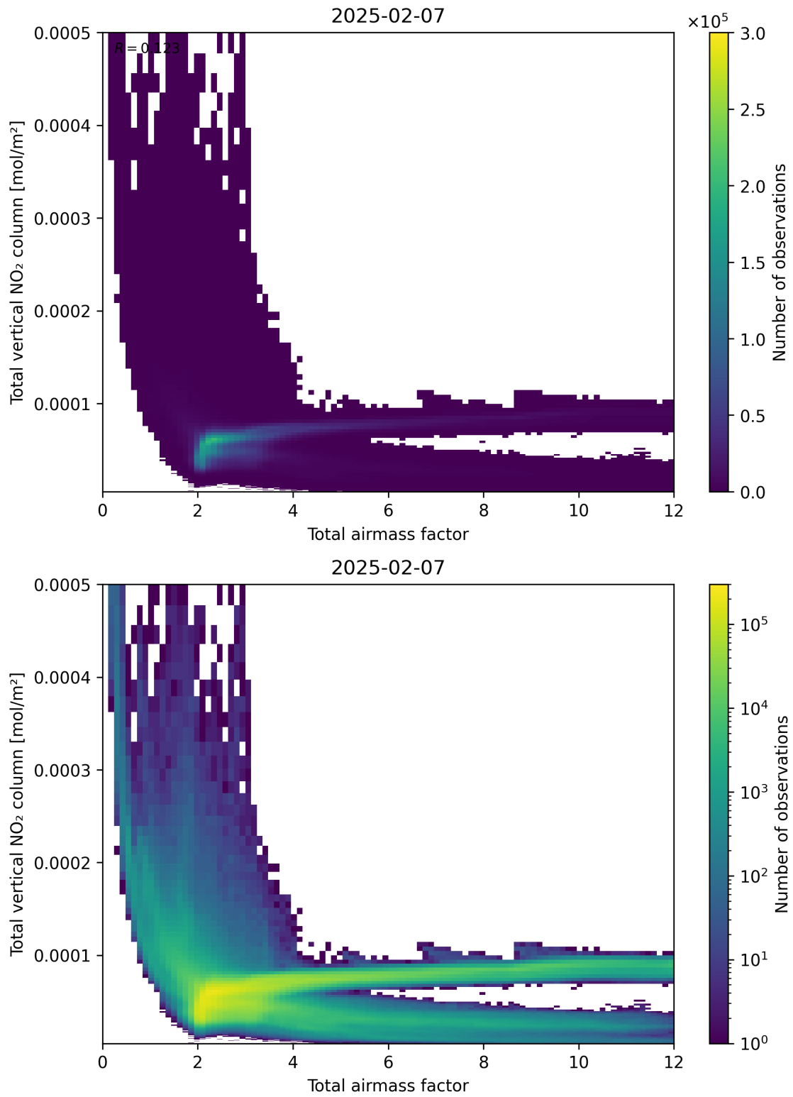
Figure 67: Scatter density plot of “Total airmass factor” against “Total vertical NO 2 column” for 2025-02-06 to 2025-02-08.
