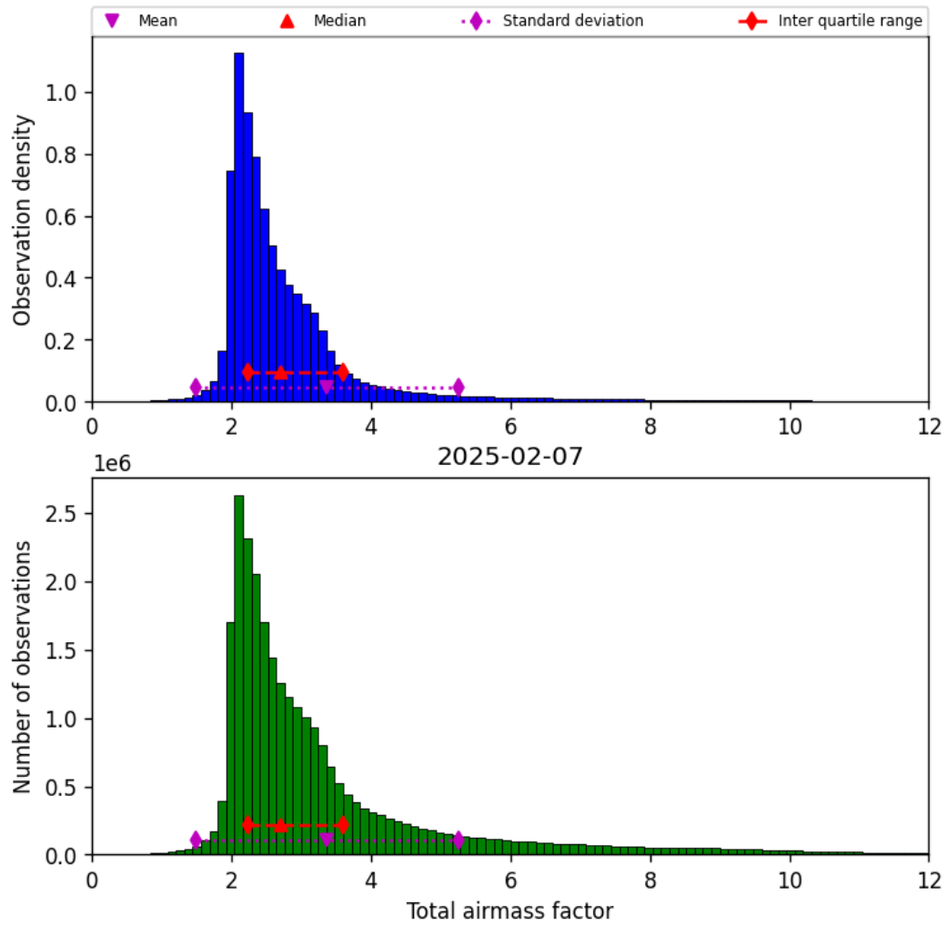
Figure 32: Histogram of “Total airmass factor” for 2025-02-06 to 2025-02-08
