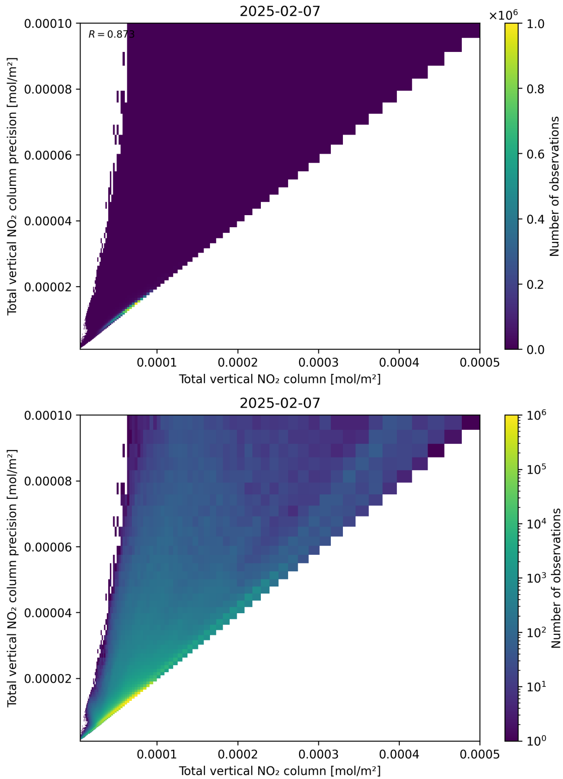
Figure 114: Scatter density plot of “Total vertical NO 2 column” against “Total vertical NO 2 column precision” for 2025-02-06 to 2025-02-08.
