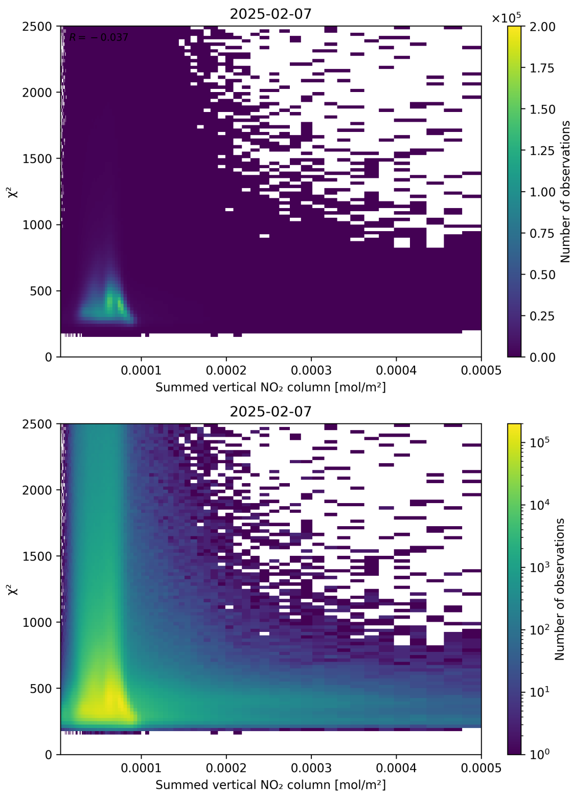
Figure 104: Scatter density plot of “Summed vertical NO 2 column” against “ \chi^2 ” for 2025-02-06 to 2025-02-08.
