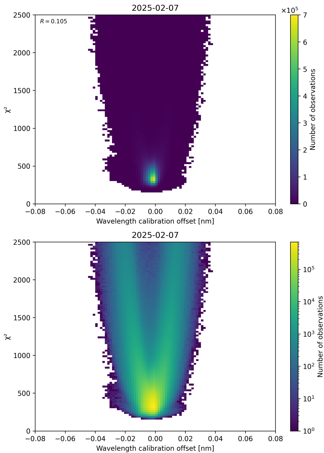
Figure 175: Scatter density plot of “Wavelength calibration offset” against “ \chi^2 ” for 2025-02-06 to 2025-02-08.
