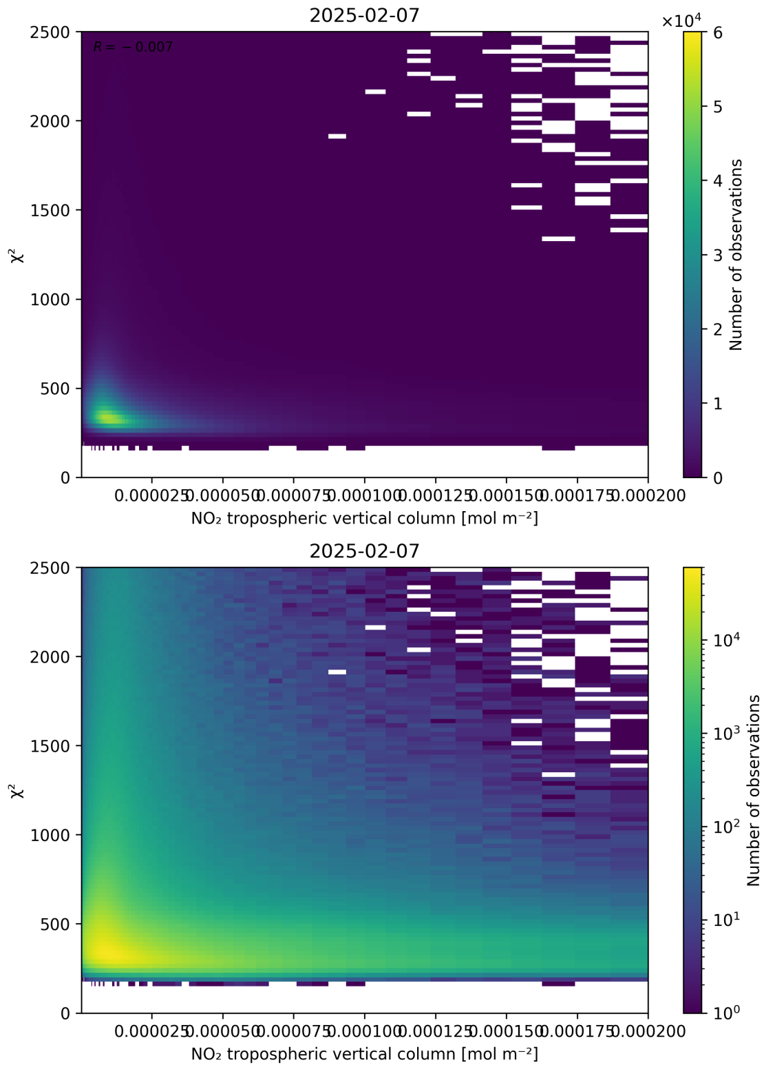
Figure 124: Scatter density plot of “NO 2 tropospheric vertical column” against “ \chi^2 ” for 2025-02-06 to 2025-02-08.
