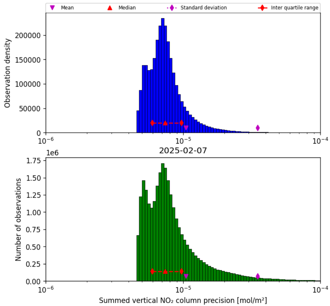
Figure 41: Histogram of "Summed vertical NO 2 column precision" for 2025-02-06 to 2025-02-08
