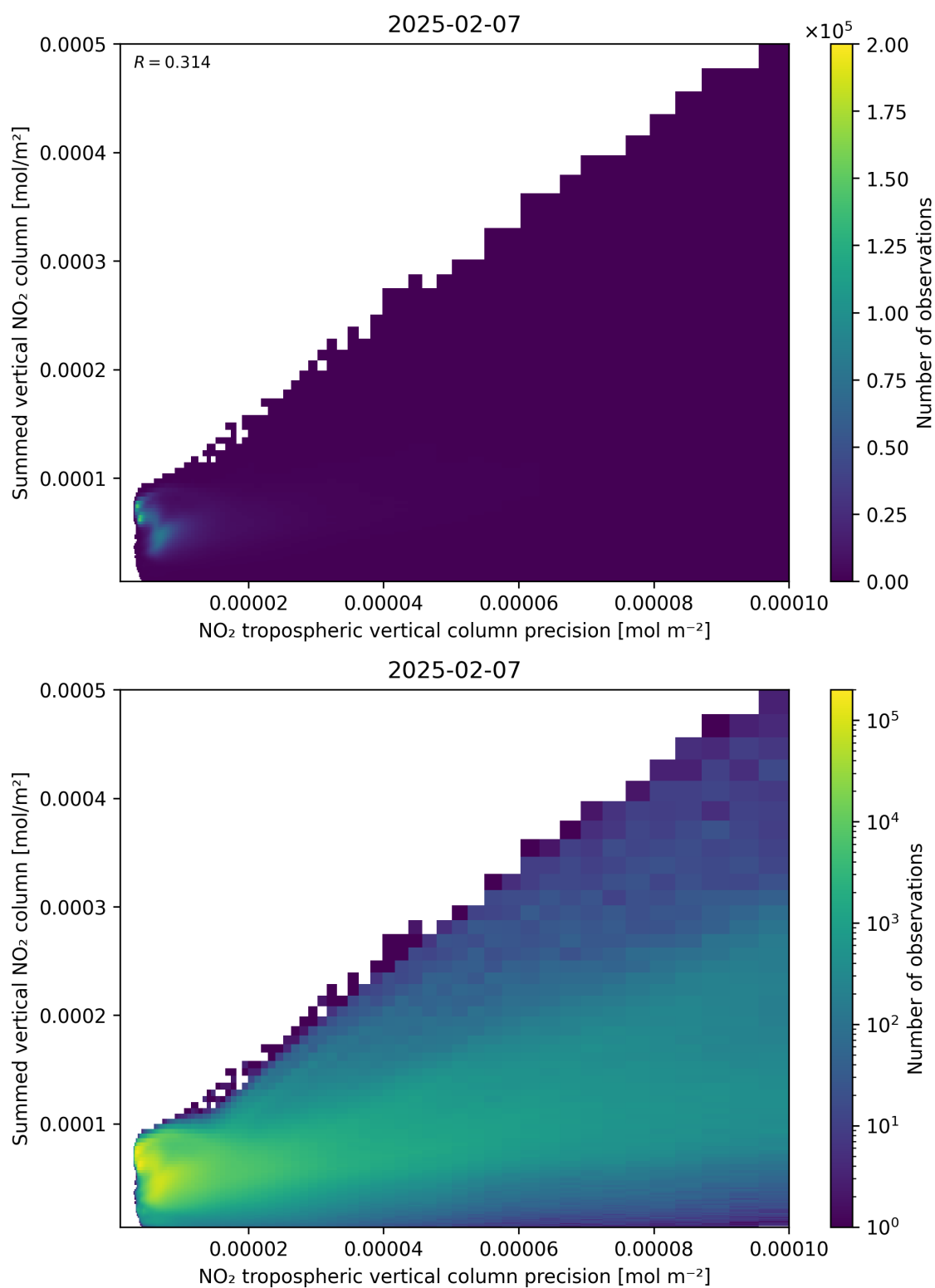
Figure 136: Scatter density plot of “NO 2 tropospheric vertical column precision” against “Summed vertical NO 2 column” for 2025-02-06 to 2025-02-08.
