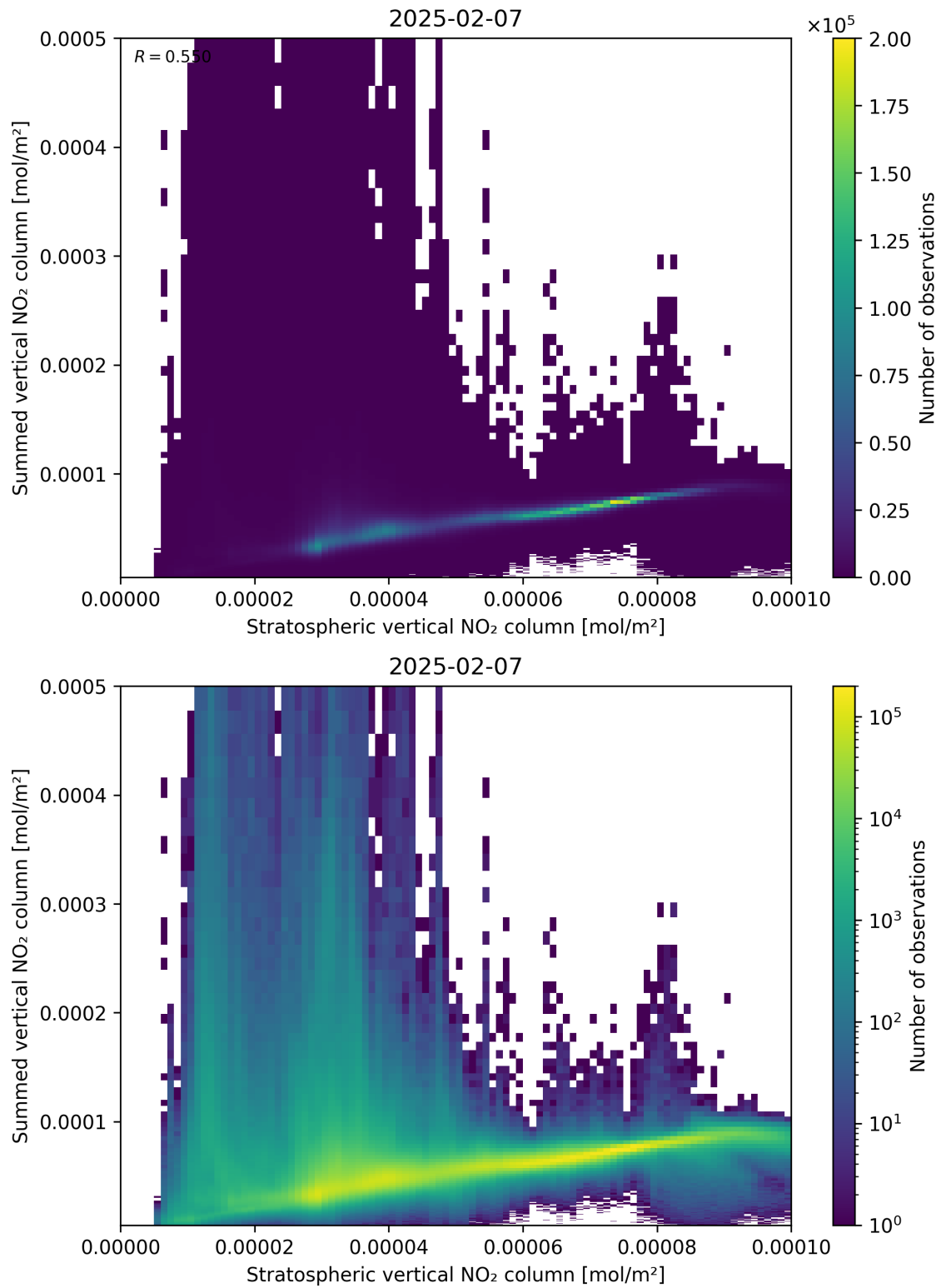
Figure 98: Scatter density plot of “Stratospheric vertical NO 2 column” against “Summed vertical NO 2 column” for 2025-02-06 to 2025-02-08.
