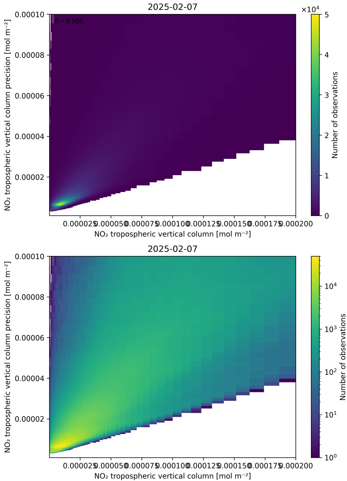
Figure 130: Scatter density plot of “NO 2 tropospheric vertical column” against “NO 2 tropospheric vertical column precision” for 2025-02-06 to 2025-02-08.
