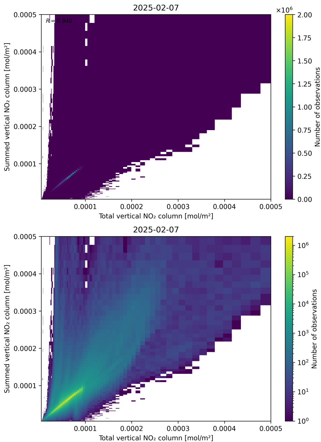
Figure 112: Scatter density plot of “Total vertical NO 2 column” against “Summed vertical NO 2 column” for 2025-02-06 to 2025-02-08.
