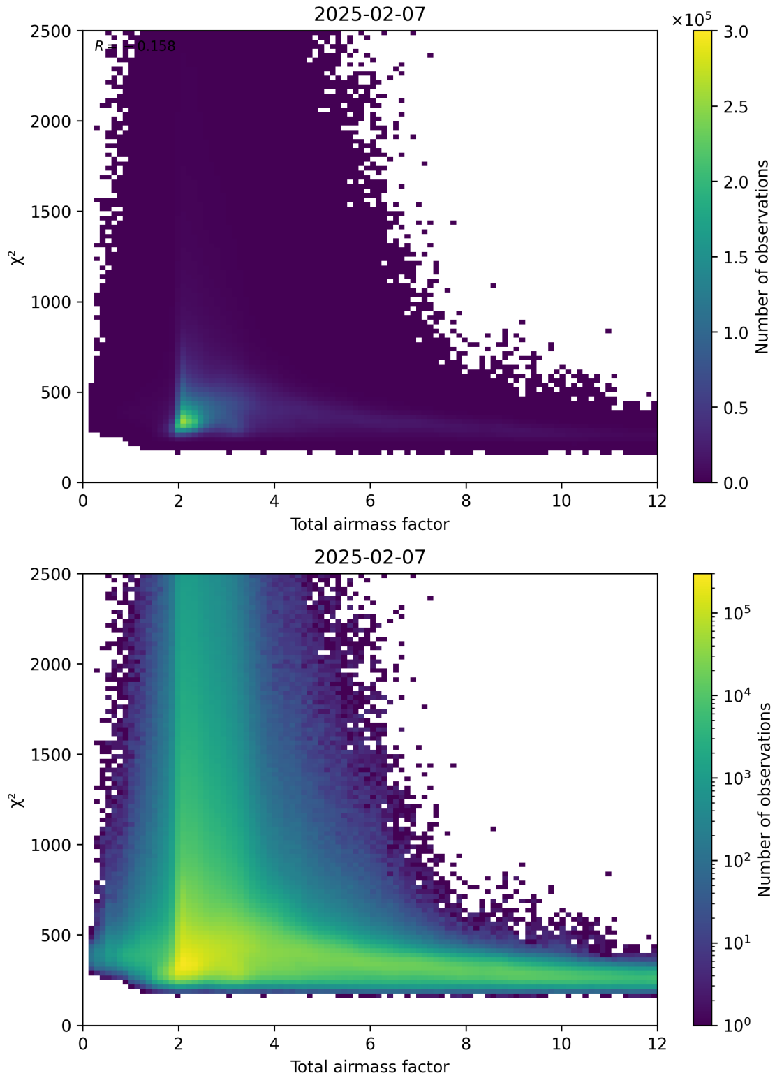
Figure 63: Scatter density plot of “Total airmass factor” against “ \chi^2 ” for 2025-02-06 to 2025-02-08.
