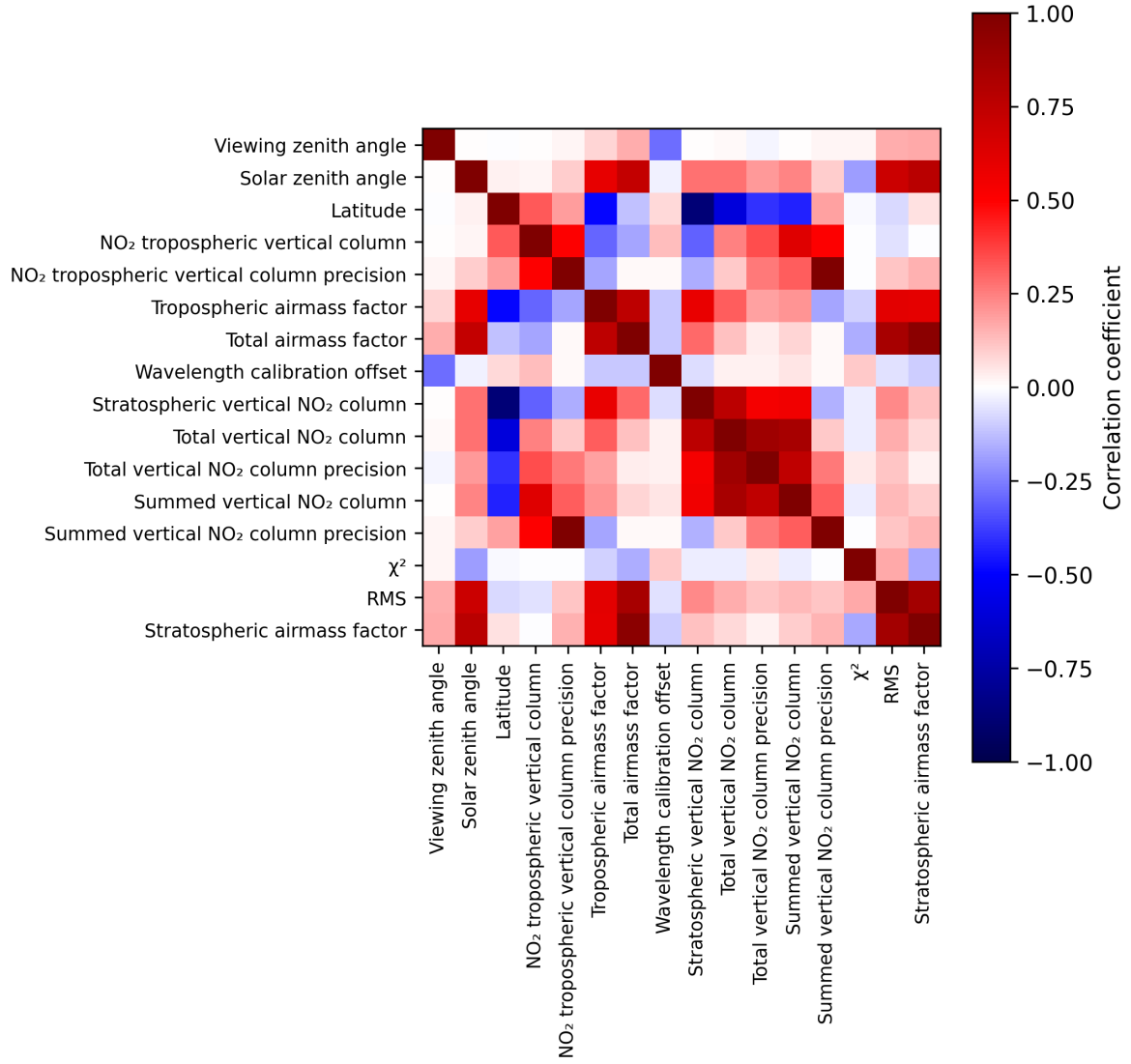
Figure 2: Map of correlation matrix for 2025-02-06 to 2025-02-08.
