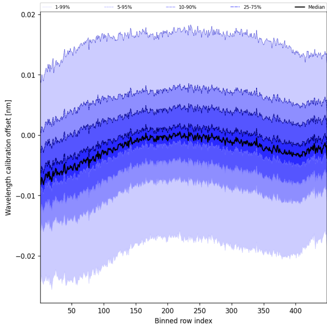
Figure 52: Along track statistics of “Wavelength calibration offset” for 2025-02-06 to 2025-02-08
