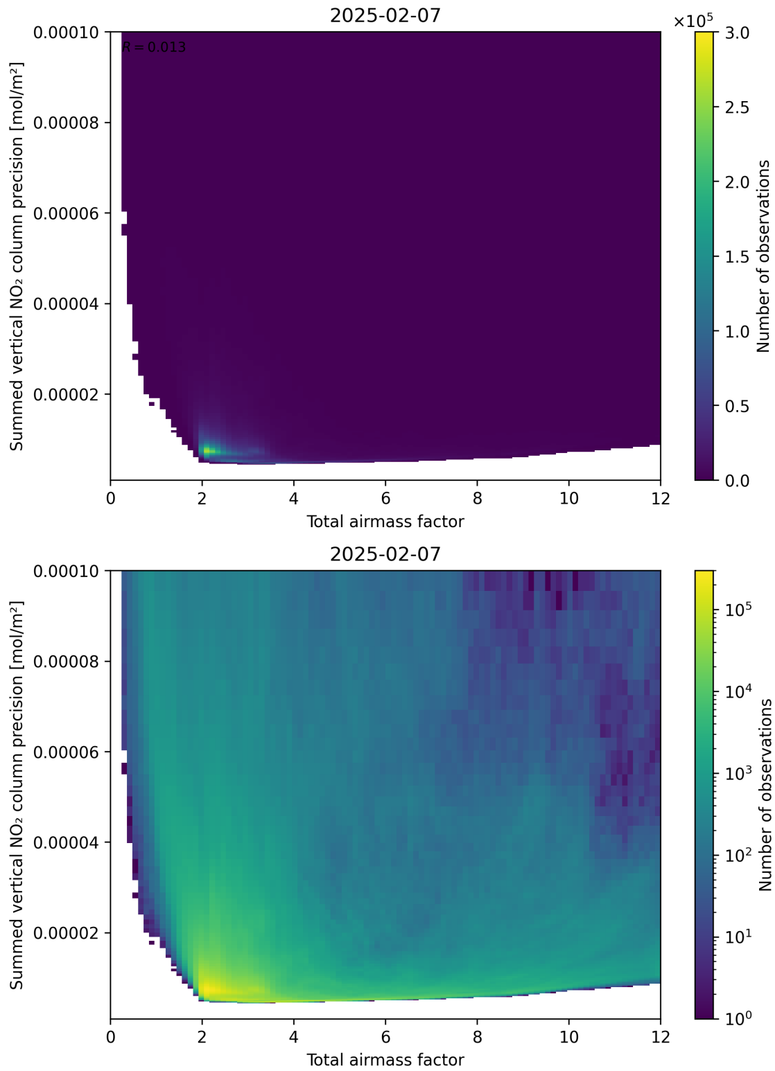
Figure 66: Scatter density plot of “Total airmass factor” against “Summed vertical NO 2 column precision” for 2025-02-06 to 2025-02-08.
