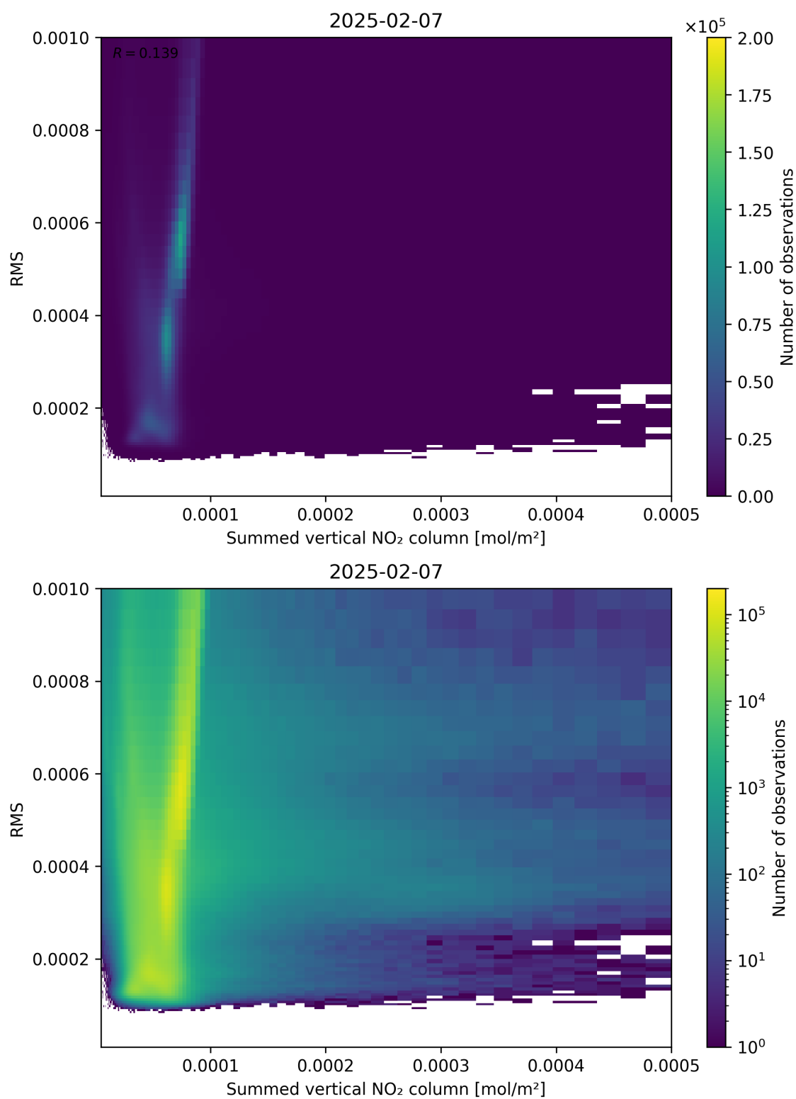
Figure 109: Scatter density plot of “Summed vertical NO 2 column” against “RMS” for 2025-02-06 to 2025-02-08.
