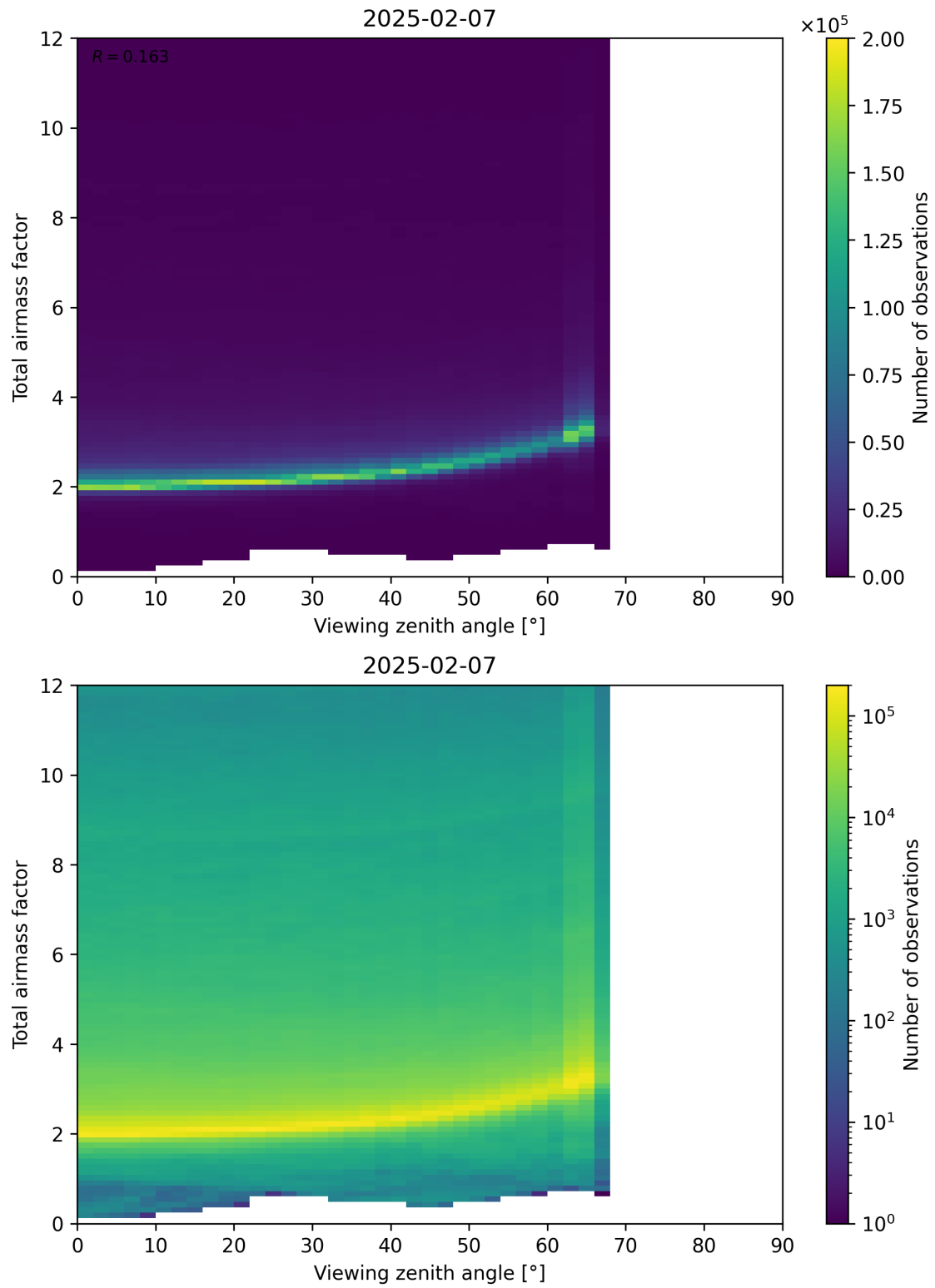
Figure 160: Scatter density plot of “Viewing zenith angle” against “Total airmass factor” for 2025-02-06 to 2025-02-08.
