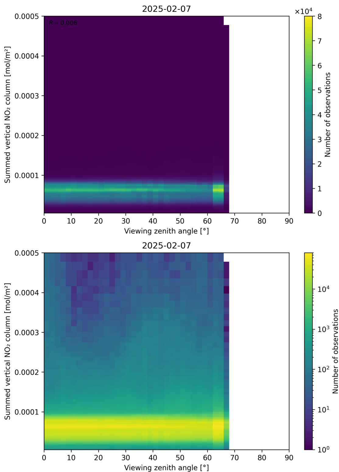
Figure 165: Scatter density plot of “Viewing zenith angle” against “Summed vertical NO 2 column” for 2025-02-06 to 2025-02-08.
