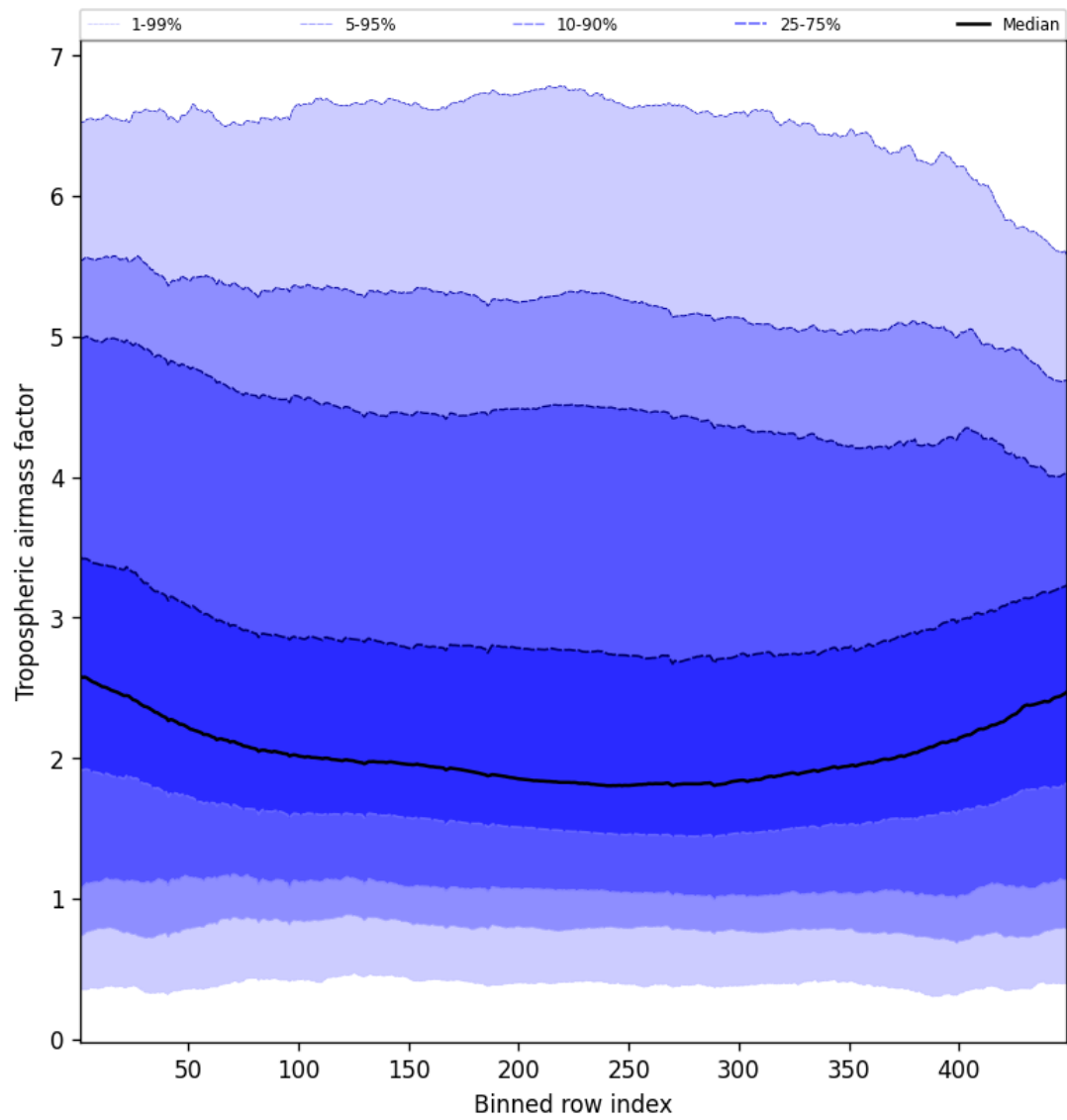
Figure 48: Along track statistics of “Tropospheric air mass factor” for 2025-02-06 to 2025-02-08
