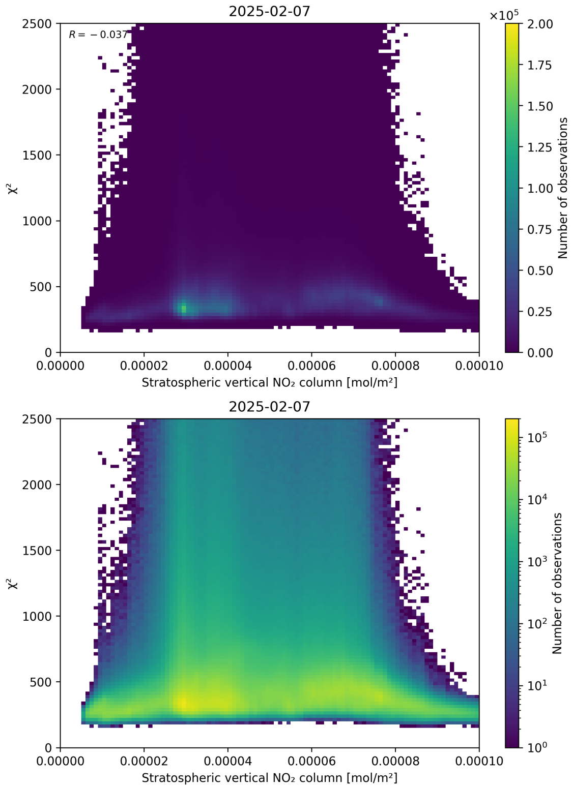
Figure 97: Scatter density plot of “Stratospheric vertical NO 2 column” against “ \chi^2 ” for 2025-02-06 to 2025-02-08.
