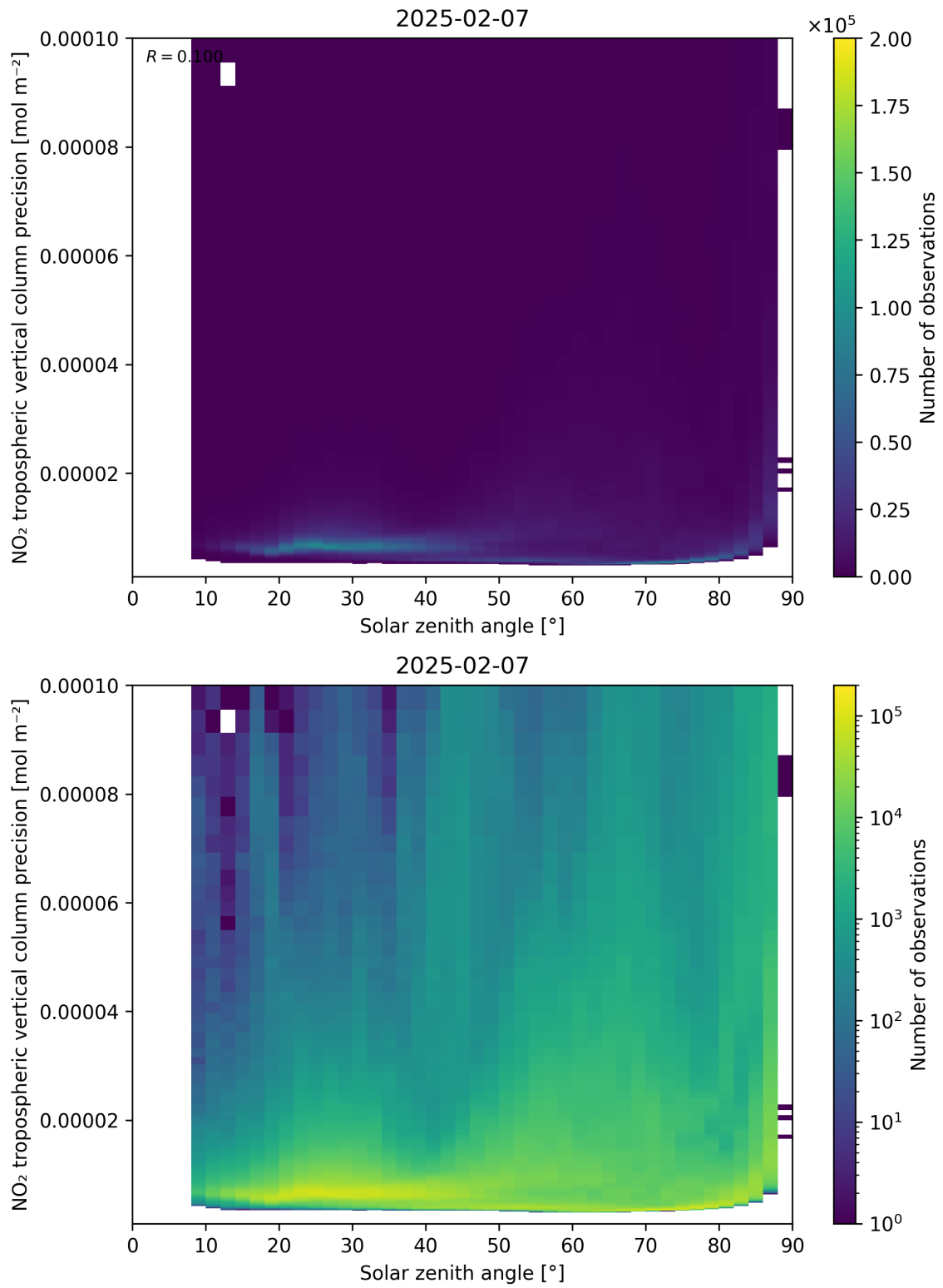
Figure 156: Scatter density plot of “Solar zenith angle” against “NO 2 tropospheric vertical column precision” for 2025-02-06 to 2025-02-08.
