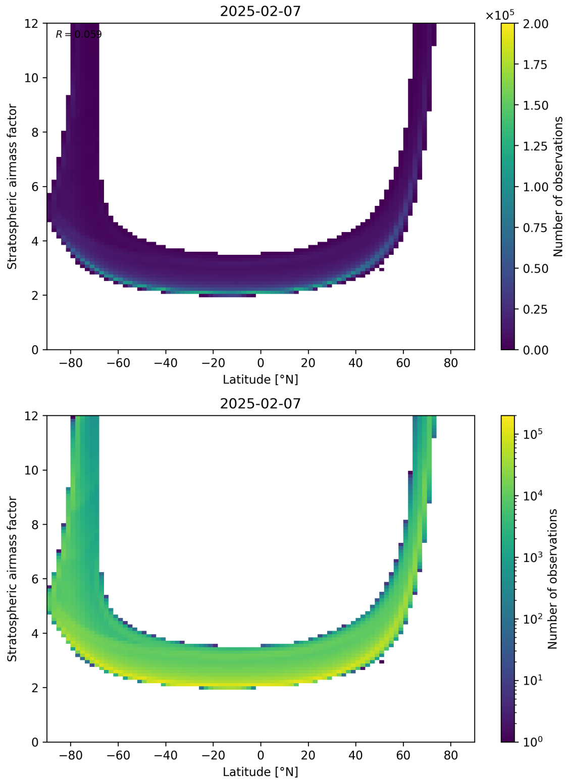
Figure 83: Scatter density plot of “Latitude” against “Stratospheric air mass factor” for 2025-02-06 to 2025-02-08.
