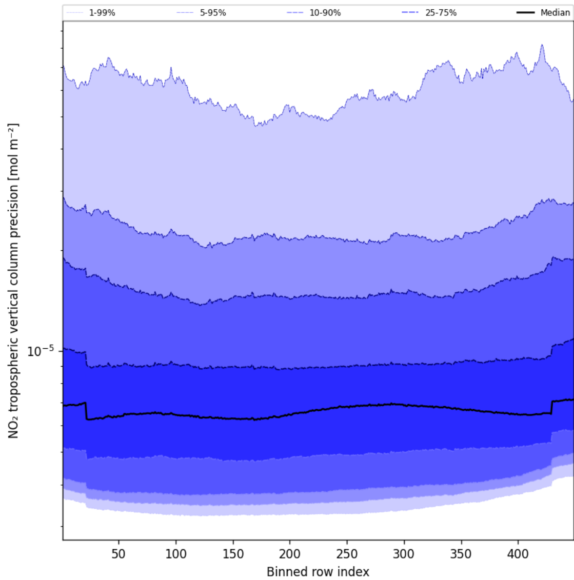
Figure 47: Along track statistics of “NO 2 tropospheric vertical column precision” for 2025-02-06 to 2025-02-08
