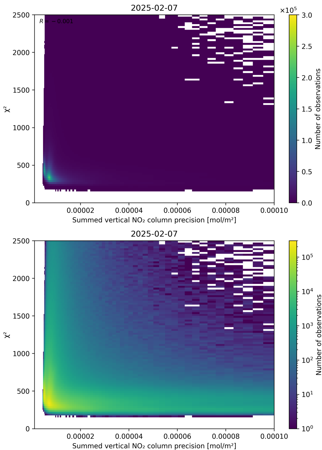
Figure 107: Scatter density plot of “Summed vertical NO 2 column precision” against “ \chi^2 ” for 2025-02-06 to 2025-02-08.
