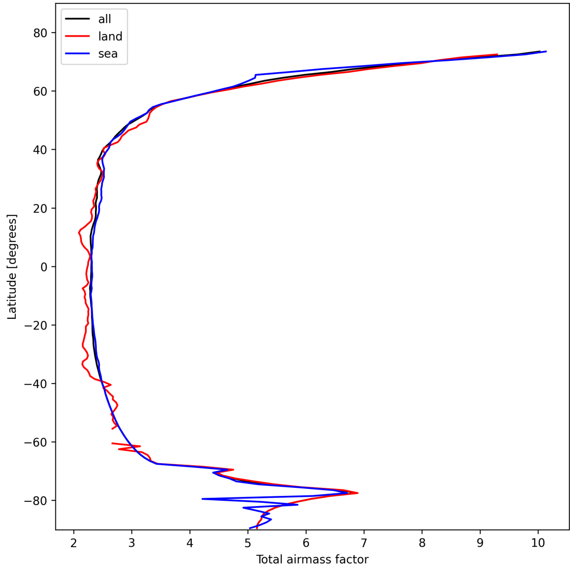
Figure 15: Zonal average of “Total airmass factor” for 2025-02-06 to 2025-02-08.
