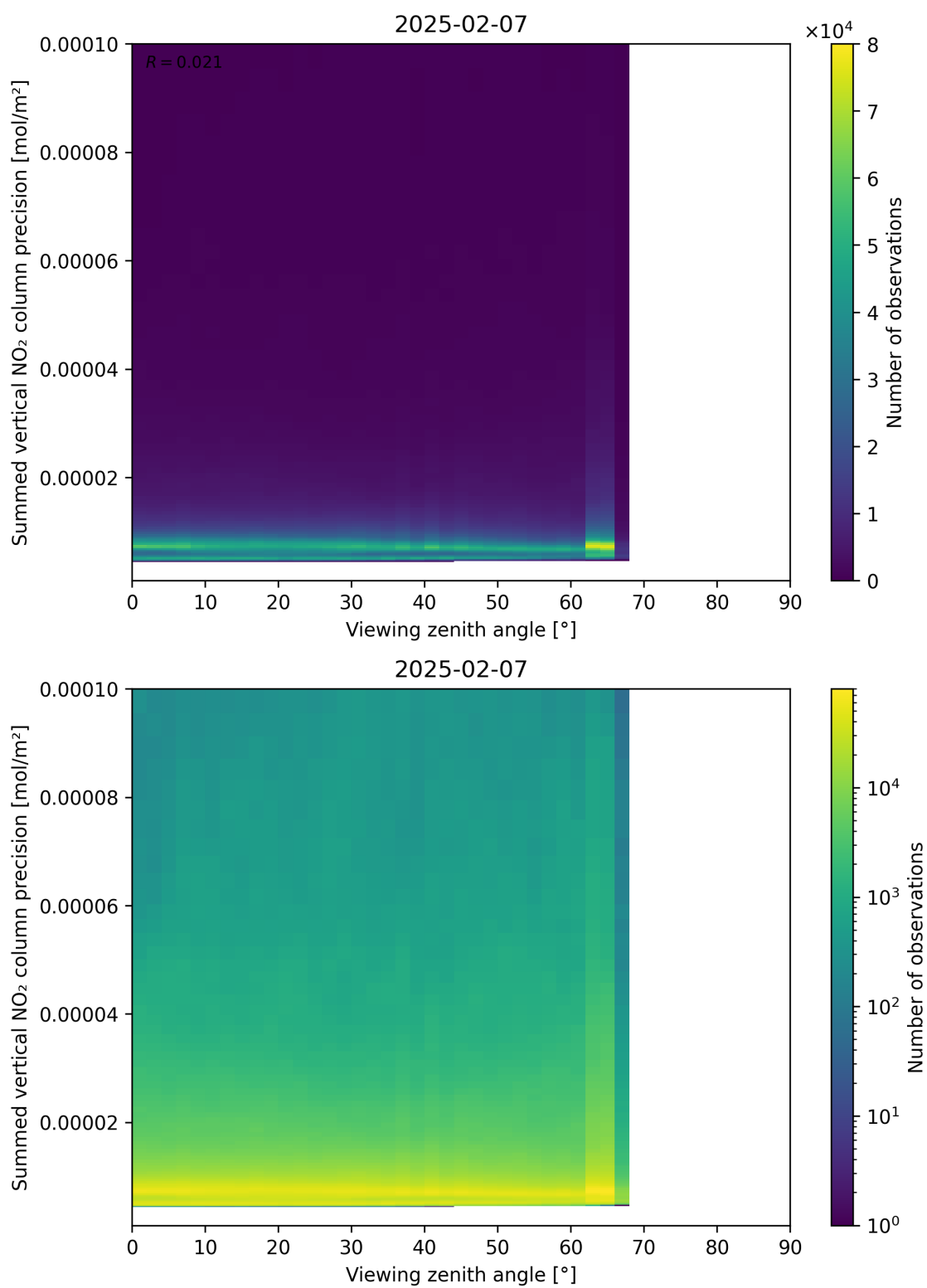
Figure 166: Scatter density plot of “Viewing zenith angle” against “Summed vertical NO 2 column precision” for 2025-02-06 to 2025-02-08.
