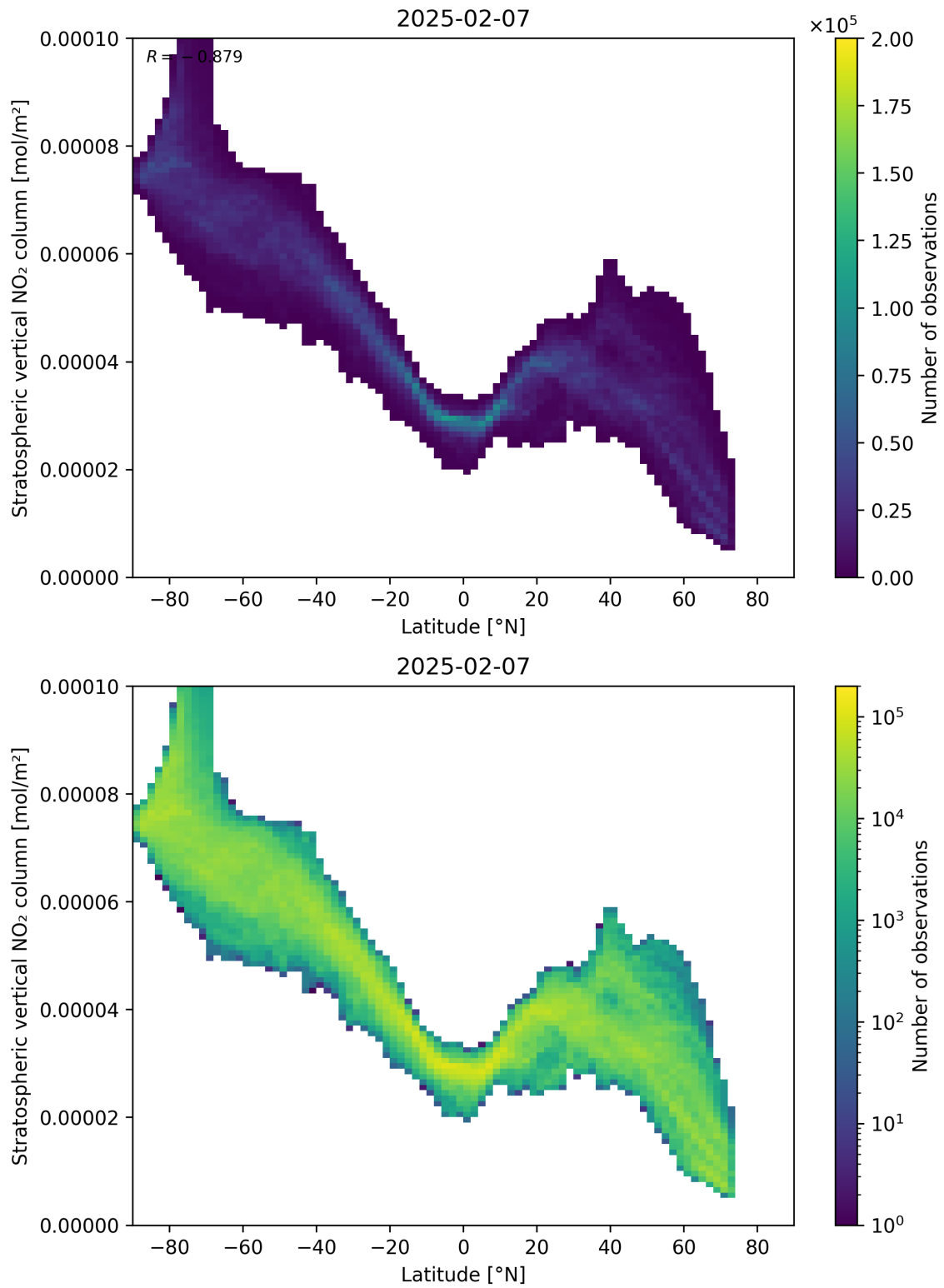
Figure 87: Scatter density plot of “Latitude” against “Stratospheric vertical NO 2 column” for 2025-02-06 to 2025-02-08.
