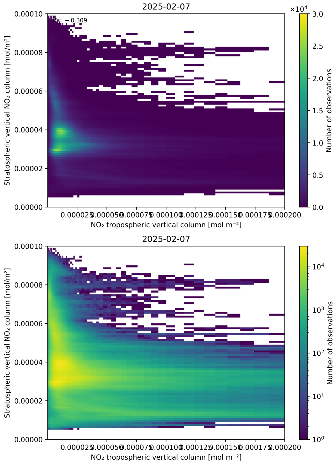
Figure 125: Scatter density plot of “NO 2 tropospheric vertical column” against “Stratospheric vertical NO 2 column” for 2025-02-06 to 2025-02-08.
