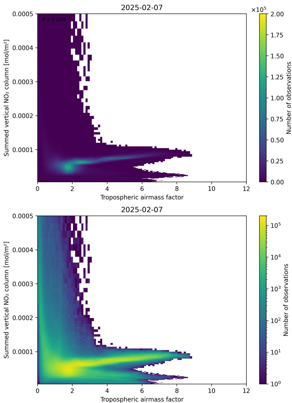
Figure 75: Scatter density plot of “Tropospheric airmass factor” against “Summed vertical NO 2 column” for 2025-02-06 to 2025-02-08.
