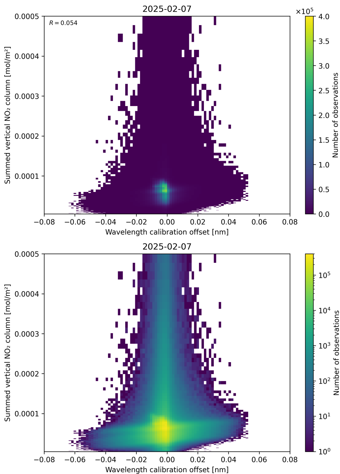
Figure 177: Scatter density plot of “Wavelength calibration offset” against “Summed vertical NO 2 column” for 2025-02-06 to 2025-02-08.
