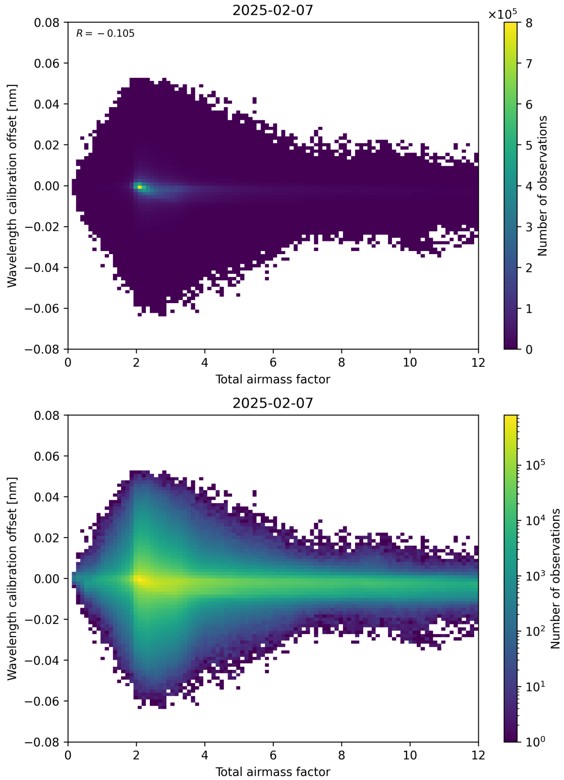
Figure 70: Scatter density plot of “Total airmass factor” against “Wavelength calibration offset” for 2025-02-06 to 2025-02-08.
