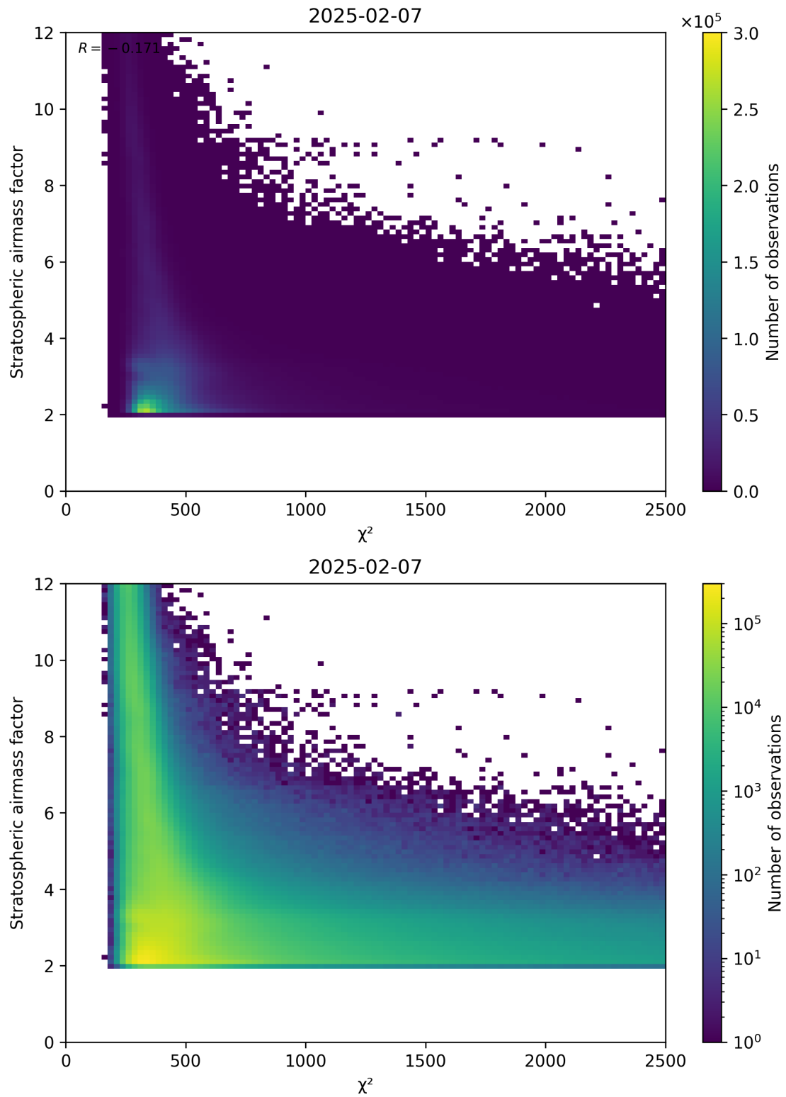
Figure 81: Scatter density plot of “ \chi^2 ” against “Stratospheric airmass factor” for 2025-02-06 to 2025-02-08.
