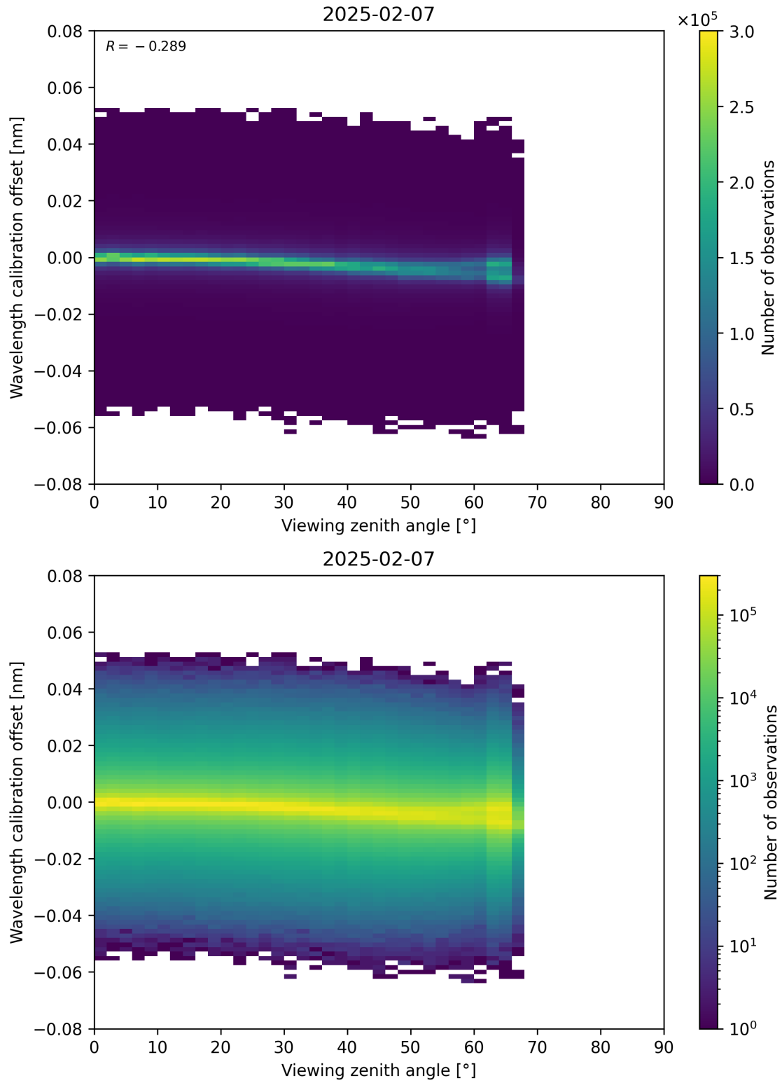
Figure 173: Scatter density plot of “Viewing zenith angle” against “Wavelength calibration offset” for 2025-02-06 to 2025-02-08.
