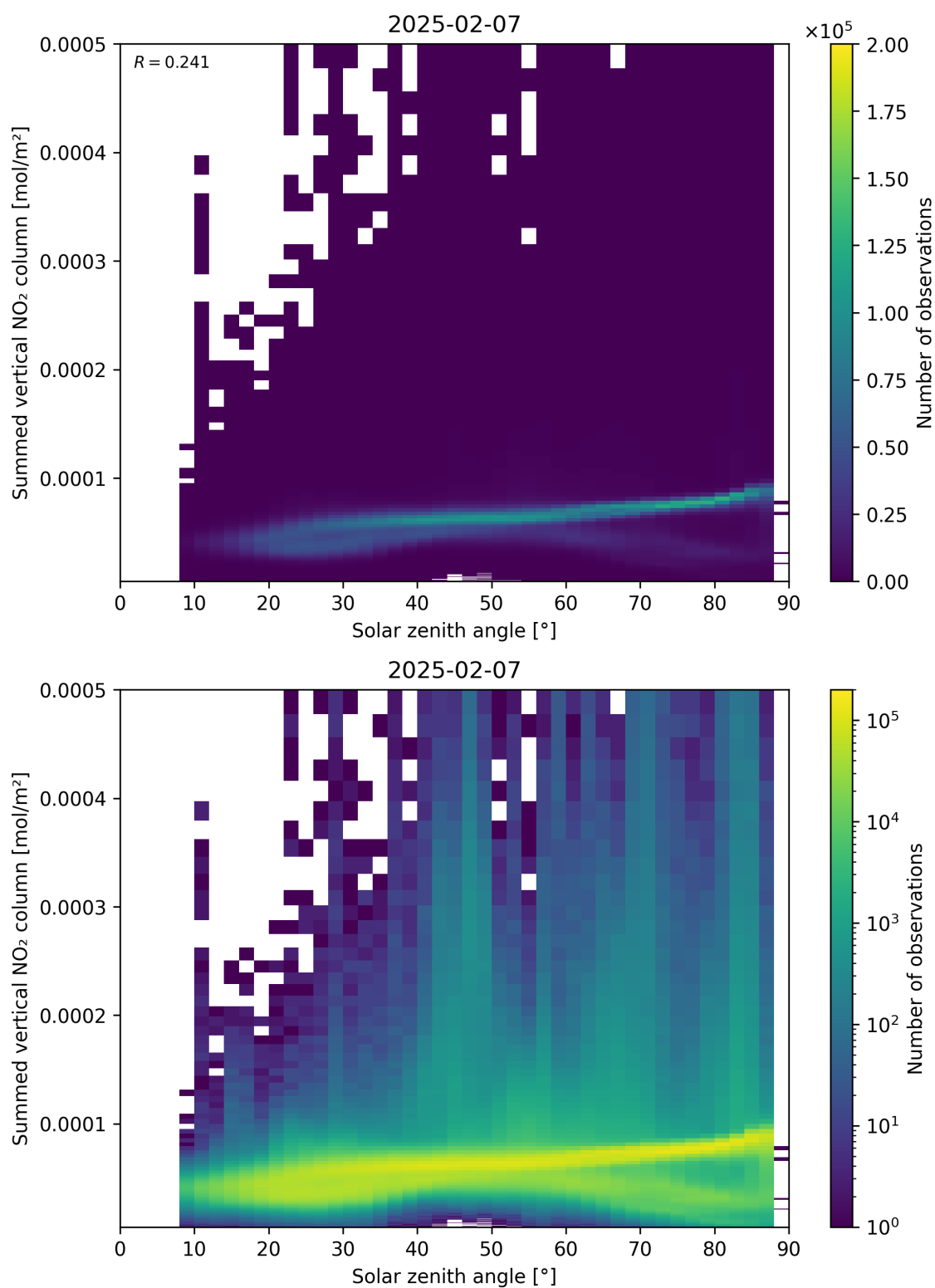
Figure 151: Scatter density plot of “Solar zenith angle” against “Summed vertical NO 2 column” for 2025-02-06 to 2025-02-08.
