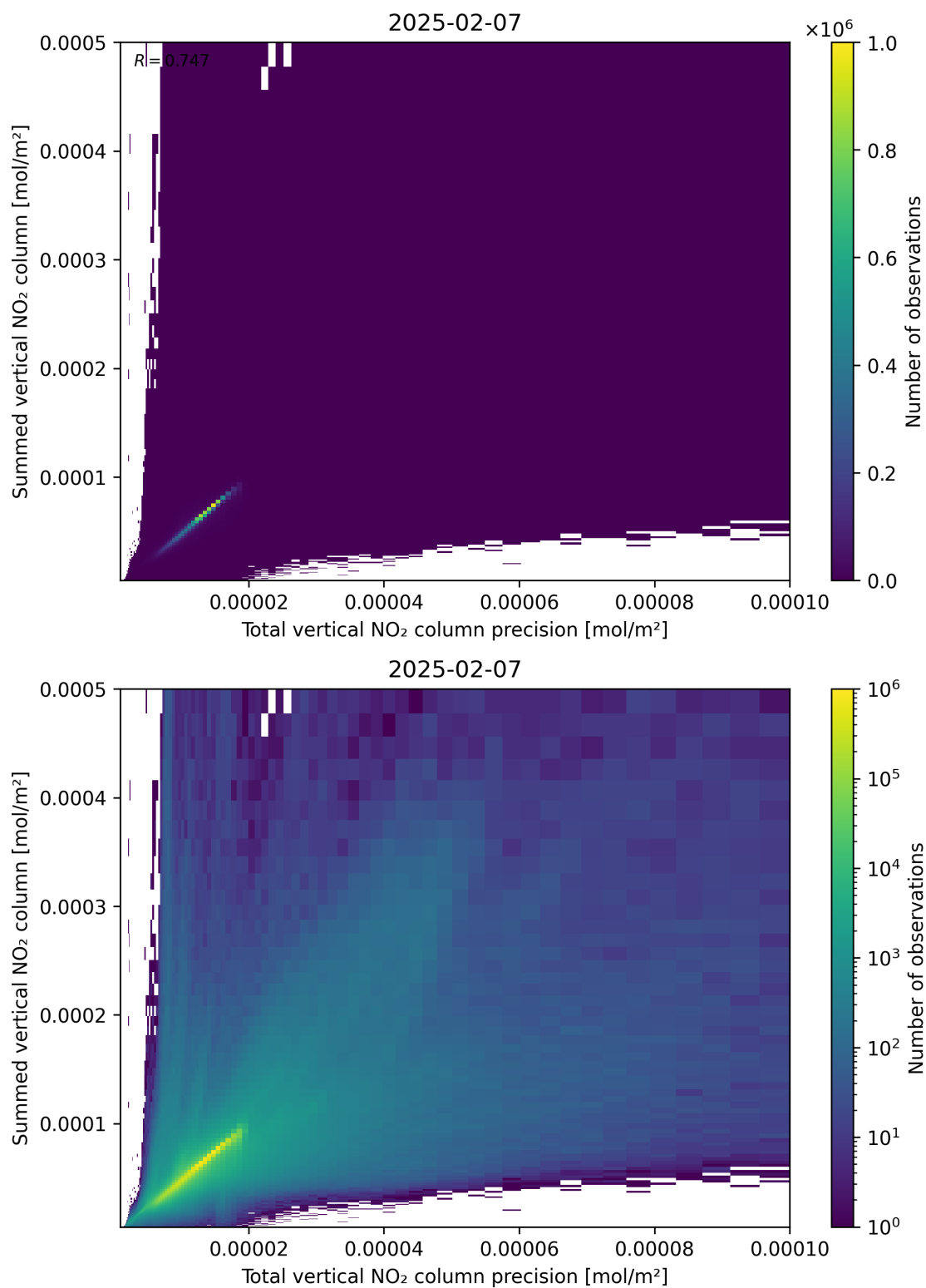
Figure 117: Scatter density plot of “Total vertical NO 2 column precision” against “Summed vertical NO 2 column” for 2025-02-06 to 2025-02-08.
