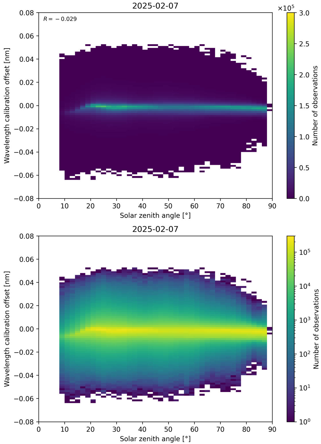
Figure 158: Scatter density plot of “Solar zenith angle” against “Wavelength calibration offset” for 2025-02-06 to 2025-02-08.
