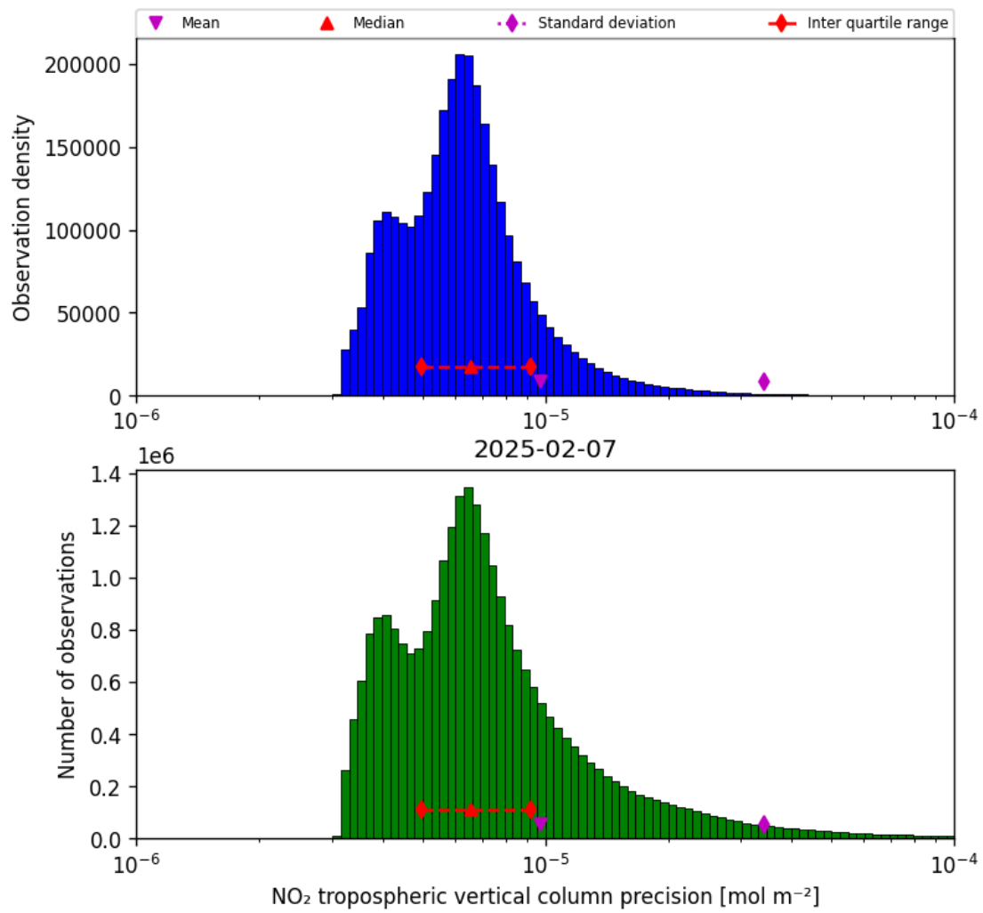
Figure 30: Histogram of “NO 2 tropospheric vertical column precision” for 2025-02-06 to 2025-02-08
