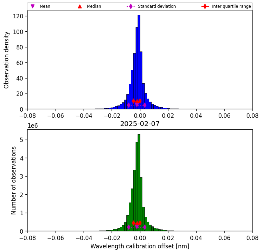
Figure 35: Histogram of “Wavelength calibration offset” for 2025-02-06 to 2025-02-08
