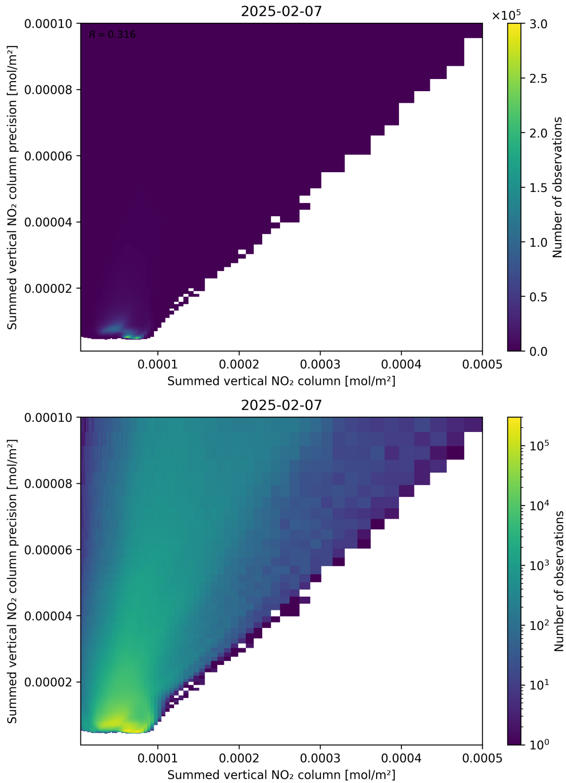
Figure 105: Scatter density plot of “Summed vertical NO 2 column” against “Summed vertical NO 2 column precision” for 2025-02-06 to 2025-02-08.
