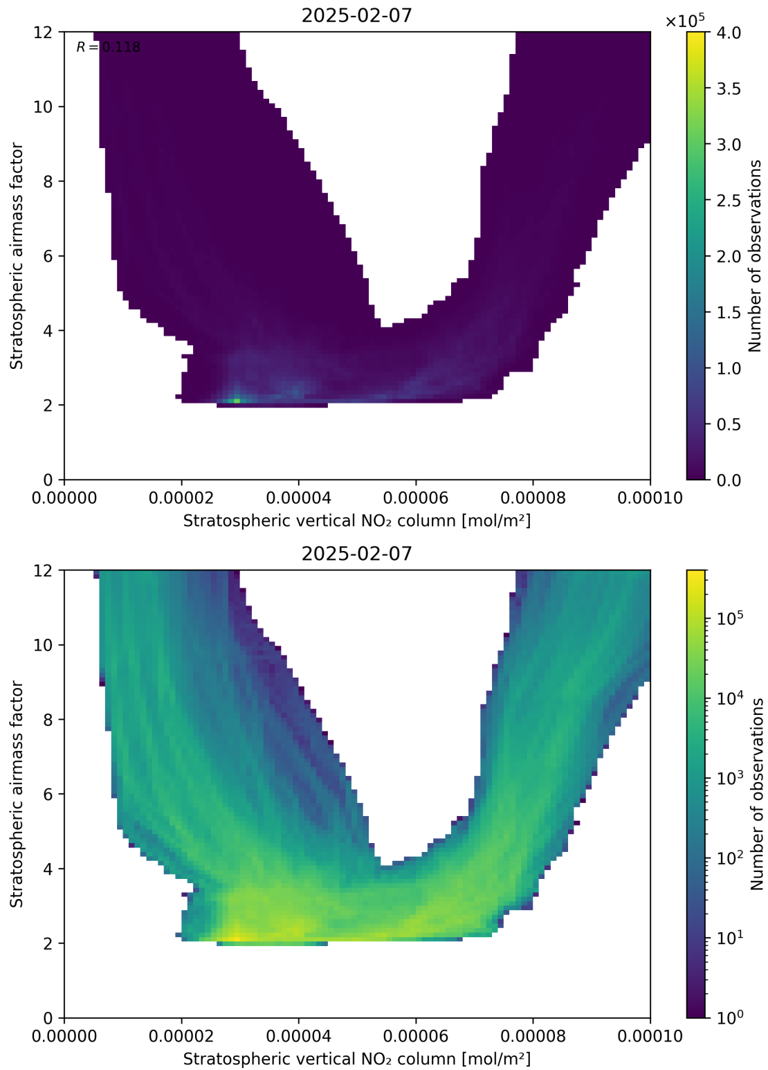
Figure 96: Scatter density plot of “Stratospheric vertical NO 2 column” against “Stratospheric airmass factor” for 2025-02-06 to 2025-02-08.
