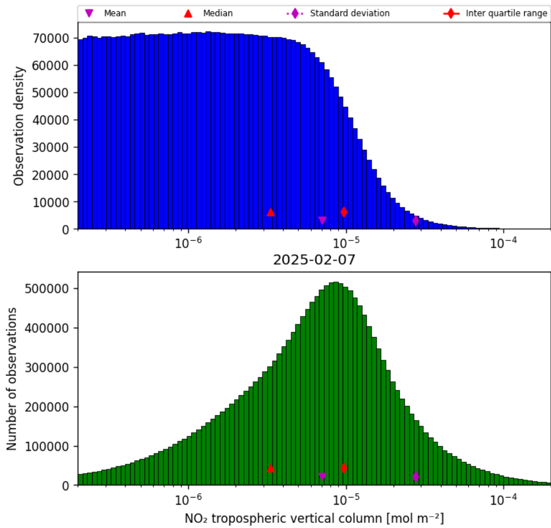
Figure 29: Histogram of “NO 2 tropospheric vertical column” for 2025-02-06 to 2025-02-08
