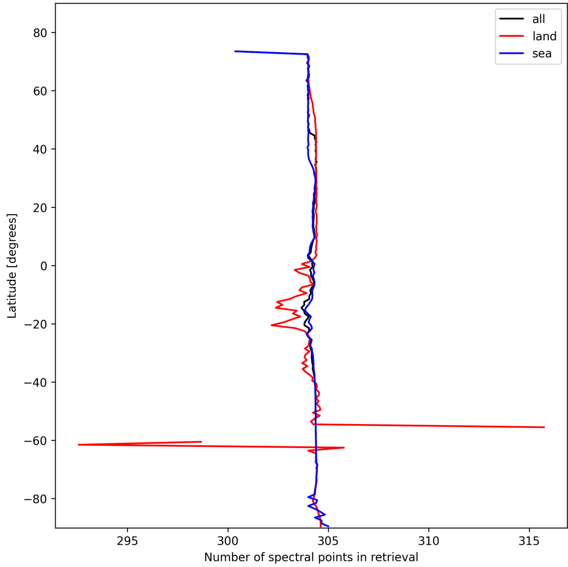
Figure 16: Zonal average of “Number of spectral points in retrieval” for 2025-02-06 to 2025-02-08.
