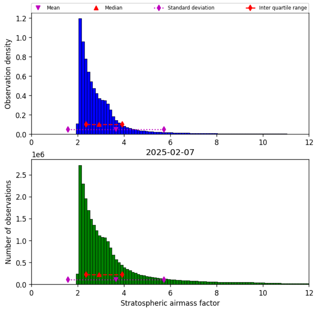
Figure 44: Histogram of “Stratospheric airmass factor” for 2025-02-06 to 2025-02-08
