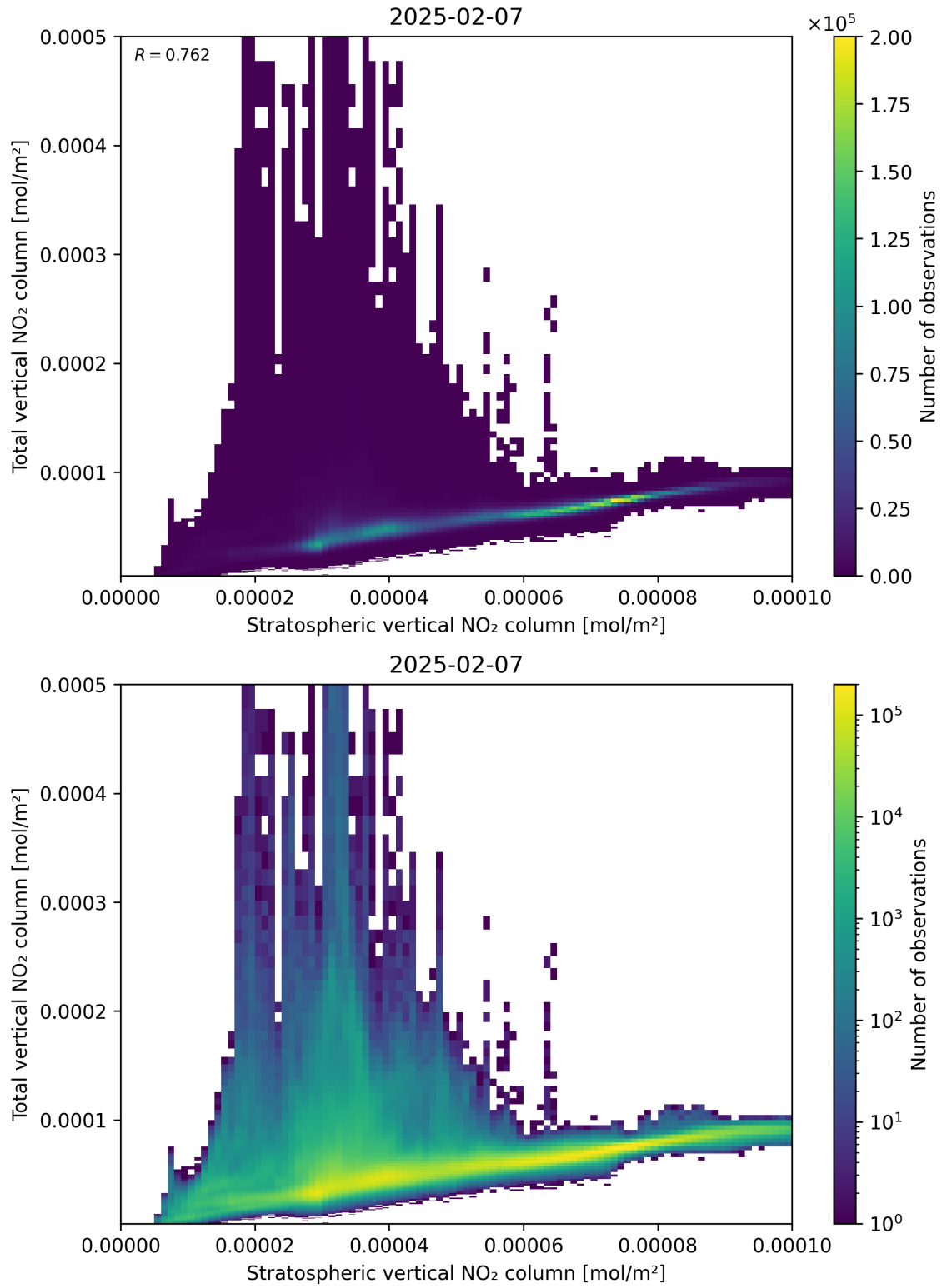
Figure 100: Scatter density plot of “Stratospheric vertical NO 2 column” against “Total vertical NO 2 column” for 2025-02-06 to 2025-02-08.
