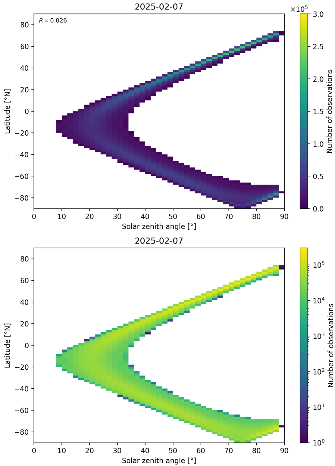
Figure 149: Scatter density plot of “Solar zenith angle” against “Latitude” for 2025-02-06 to 2025-02-08.
