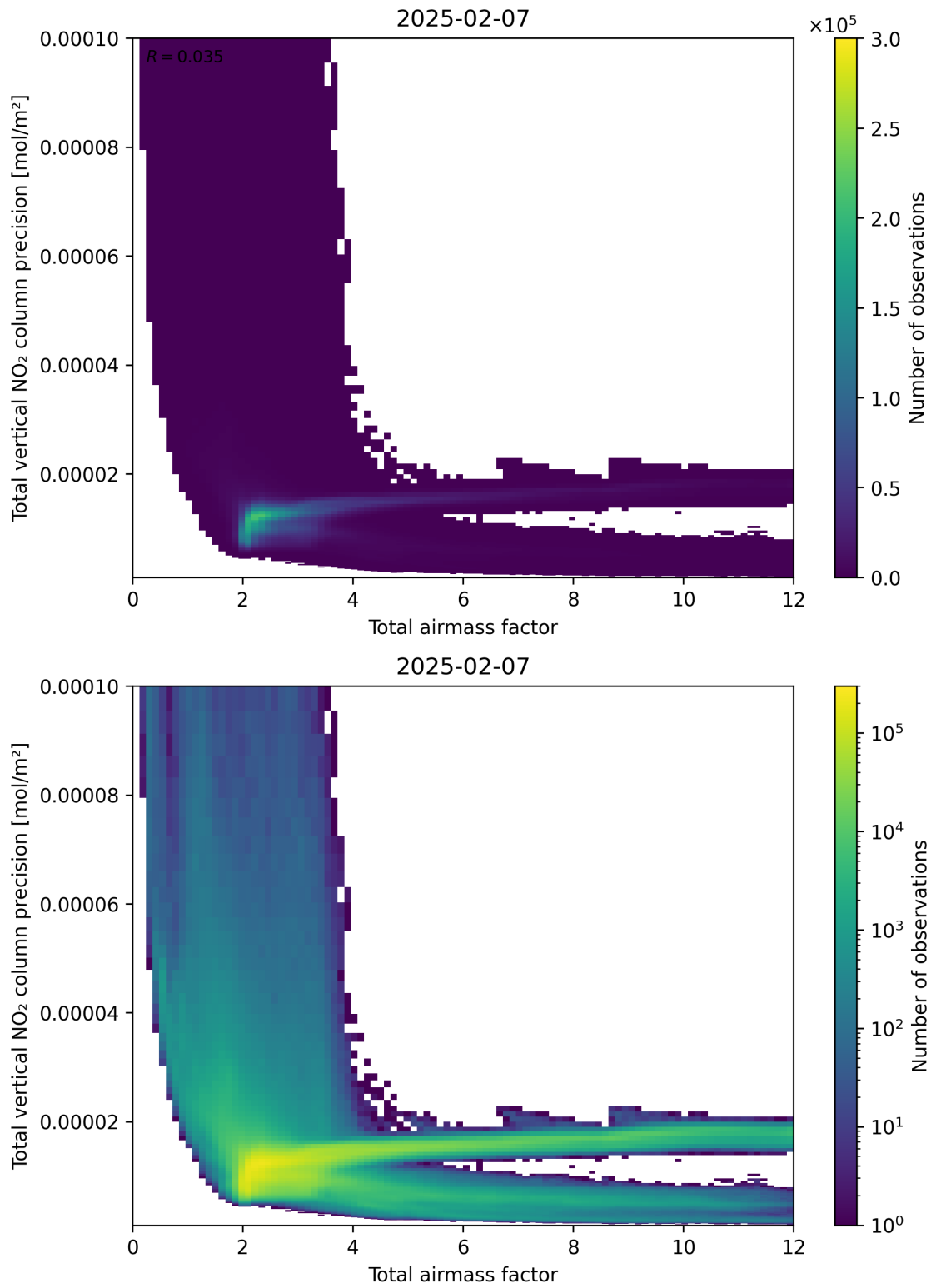
Figure 68: Scatter density plot of “Total airmass factor” against “Total vertical NO 2 column precision” for 2025-02-06 to 2025-02-08.
