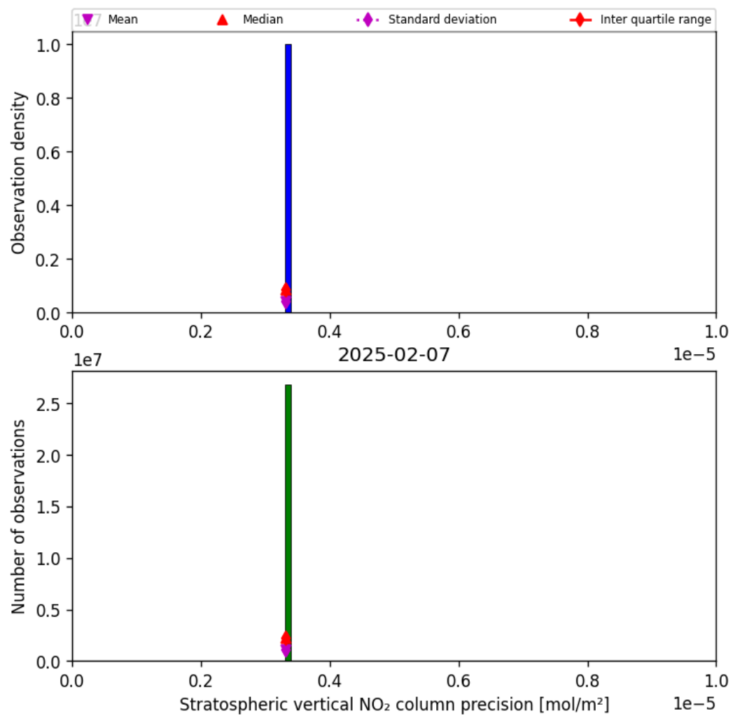
Figure 37: Histogram of “Stratospheric vertical NO 2 column precision” for 2025-02-06 to 2025-02-08
