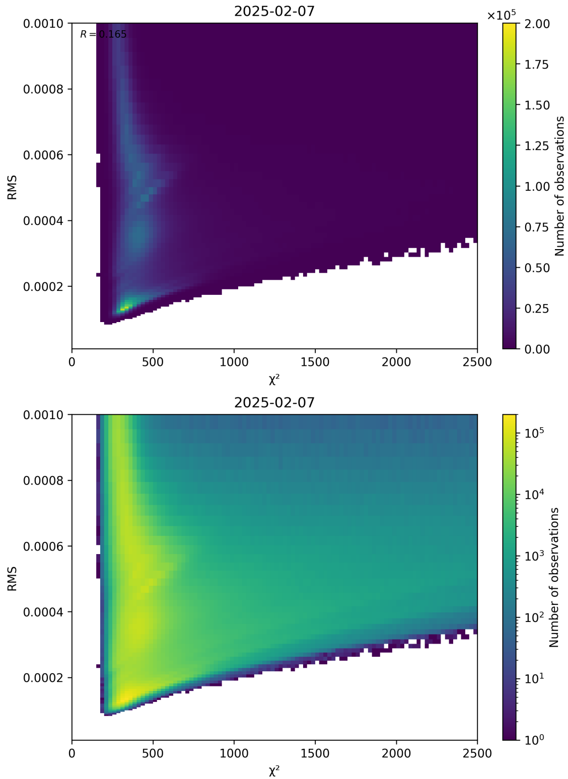
Figure 82: Scatter density plot of “ \chi^2 ” against “RMS” for 2025-02-06 to 2025-02-08.
