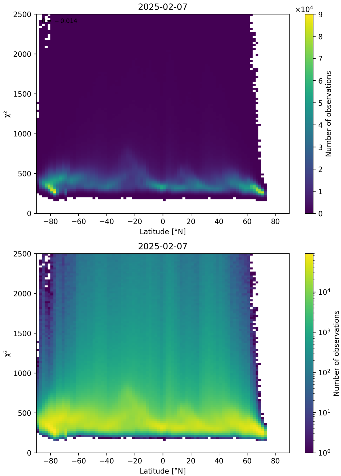
Figure 86: Scatter density plot of “Latitude” against “ \chi^2 ” for 2025-02-06 to 2025-02-08.
