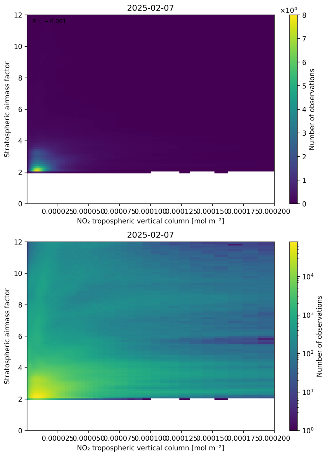
Figure 121: Scatter density plot of “NO 2 tropospheric vertical column” against “Stratospheric airmass factor” for 2025-02-06 to 2025-02-08.
