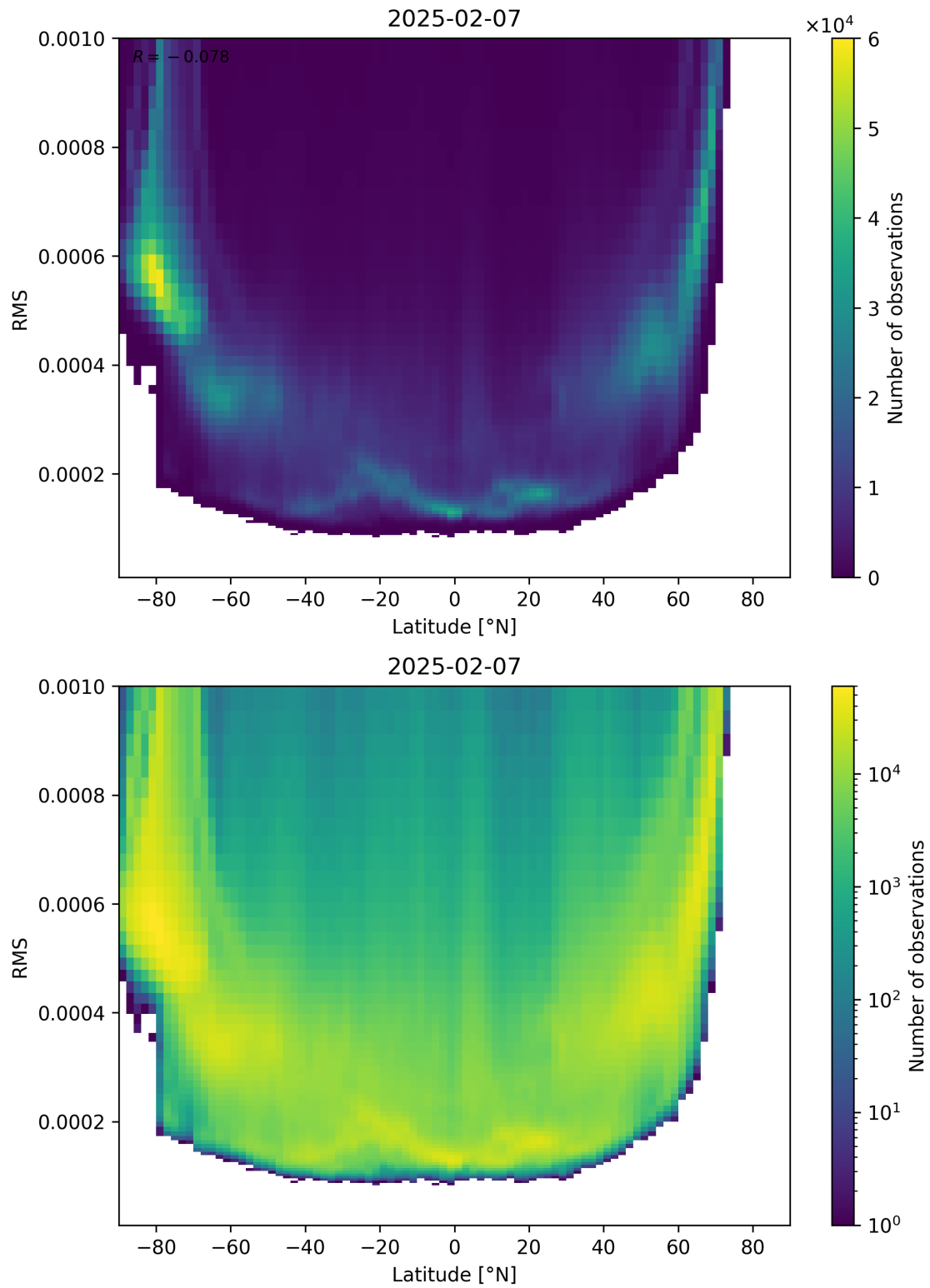
Figure 94: Scatter density plot of “Latitude” against “RMS” for 2025-02-06 to 2025-02-08.
