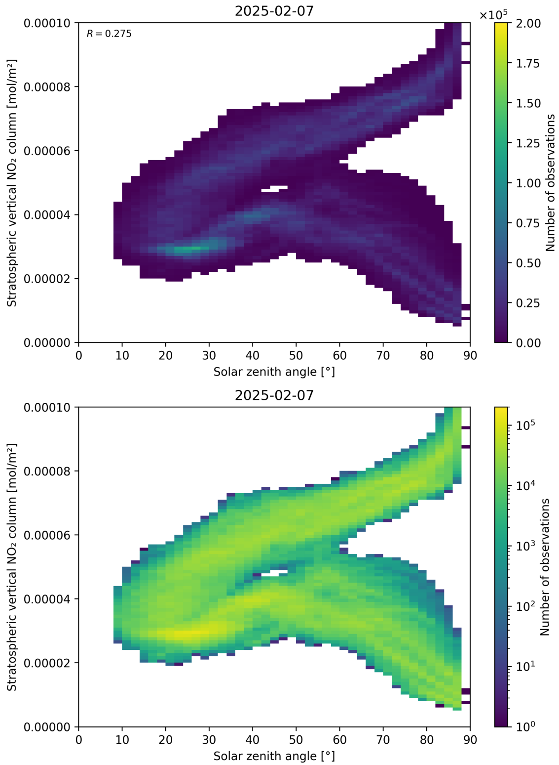
Figure 150: Scatter density plot of “Solar zenith angle” against “Stratospheric vertical NO 2 column” for 2025-02-06 to 2025-02-08.
