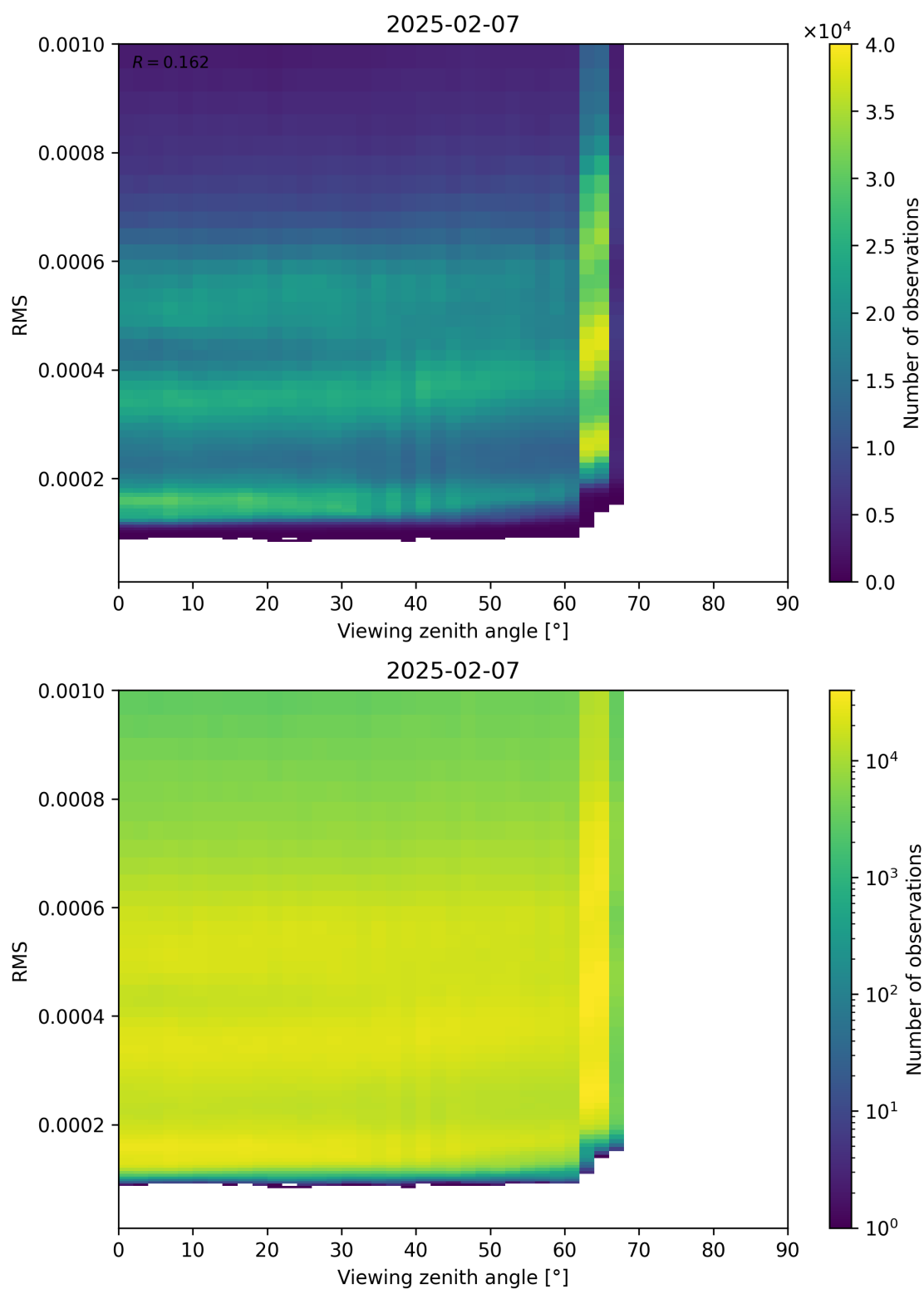
Figure 171: Scatter density plot of “Viewing zenith angle” against “RMS” for 2025-02-06 to 2025-02-08.
