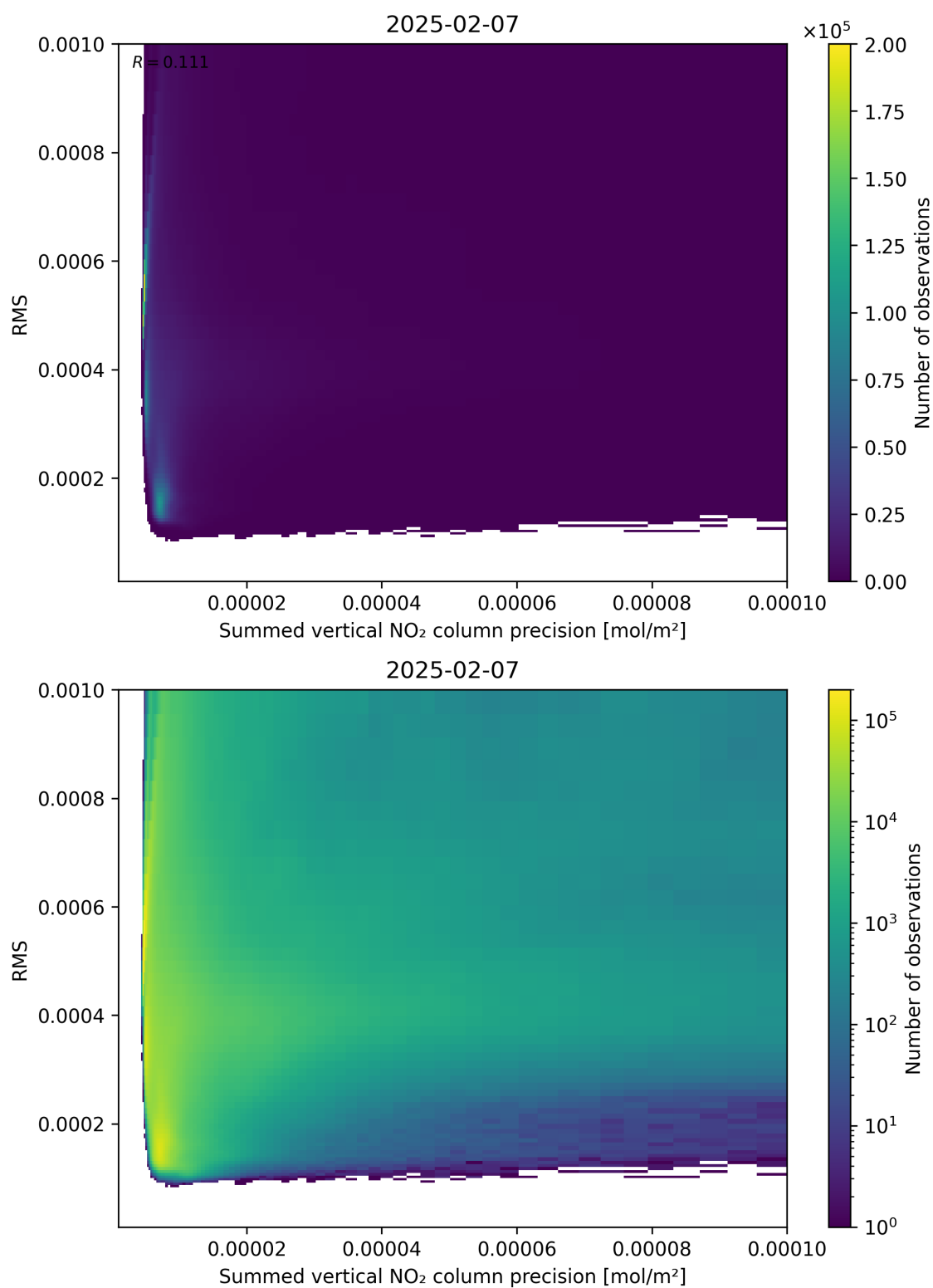
Figure 108: Scatter density plot of “Summed vertical NO 2 column precision” against “RMS” for 2025-02-06 to 2025-02-08.
