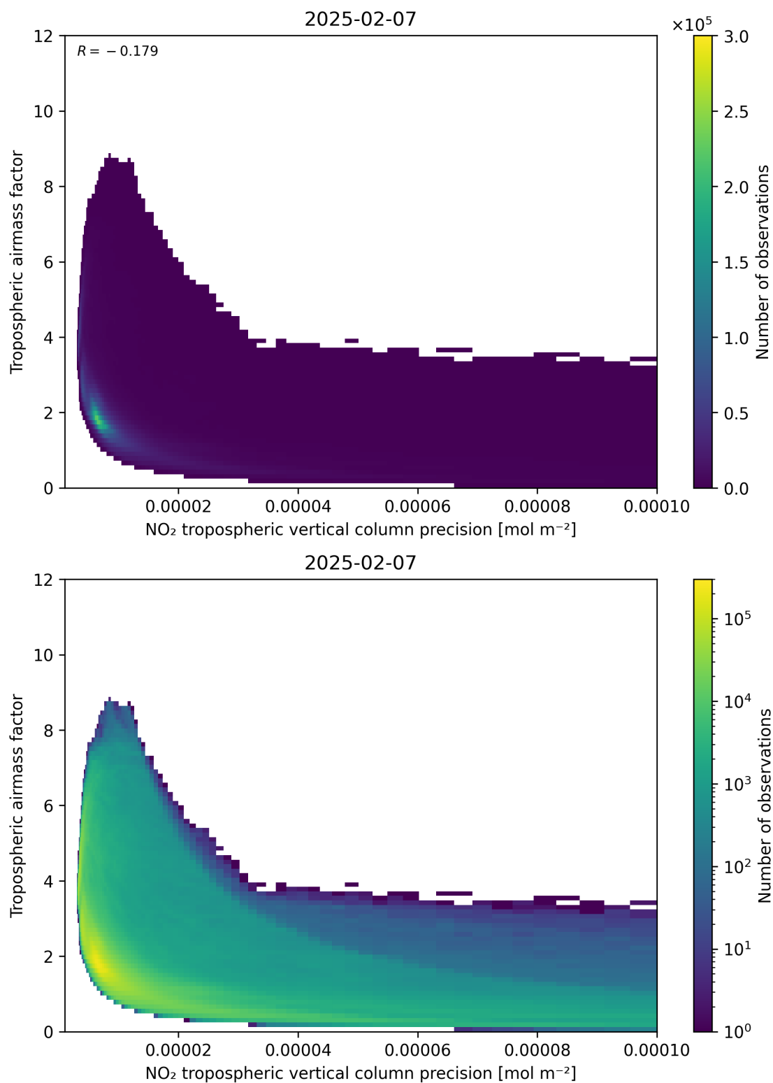
Figure 133: Scatter density plot of “NO 2 tropospheric vertical column precision” against “Tropospheric airmass factor” for 2025-02-06 to 2025-02-08.
