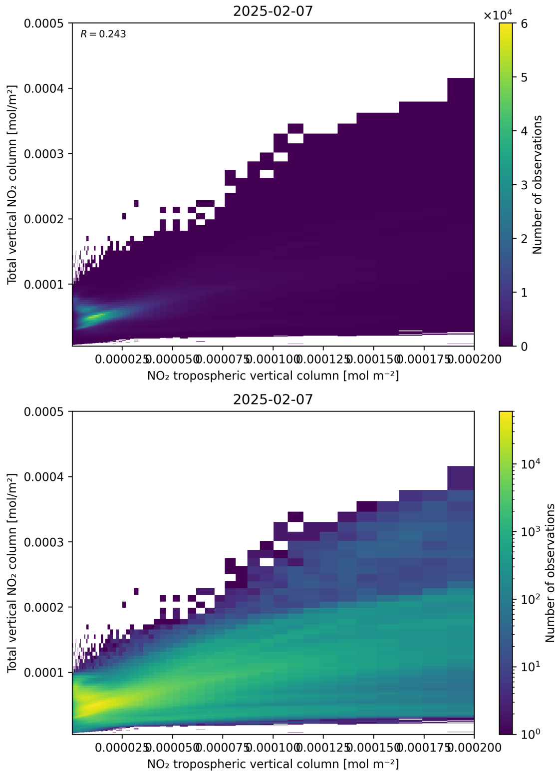
Figure 128: Scatter density plot of “NO 2 tropospheric vertical column” against “Total vertical NO 2 column” for 2025-02-06 to 2025-02-08.
