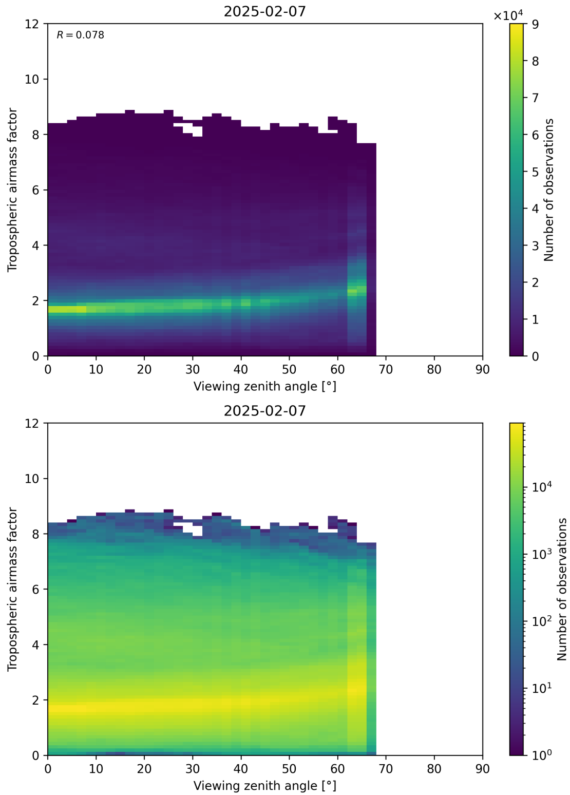
Figure 161: Scatter density plot of “Viewing zenith angle” against “Tropospheric airmass factor” for 2025-02-06 to 2025-02-08.
