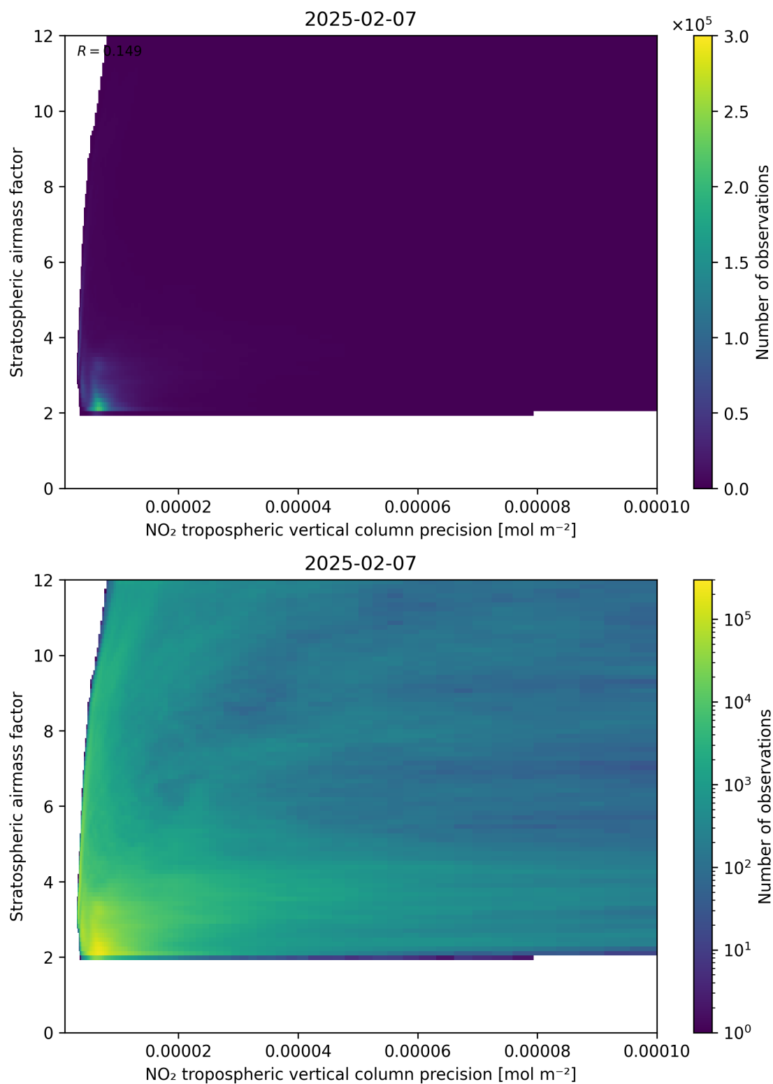
Figure 131: Scatter density plot of “NO 2 tropospheric vertical column precision” against “Stratospheric airmass factor” for 2025-02-06 to 2025-02-08.
