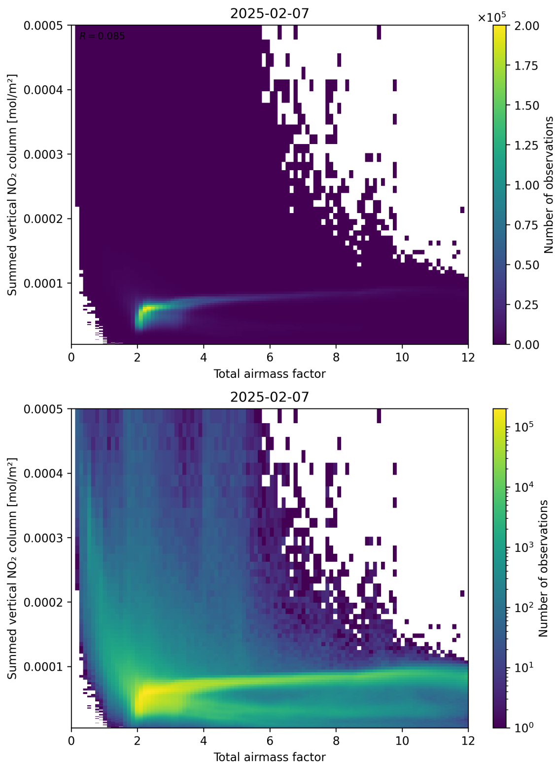
Figure 65: Scatter density plot of “Total airmass factor” against “Summed vertical NO 2 column” for 2025-02-06 to 2025-02-08.
