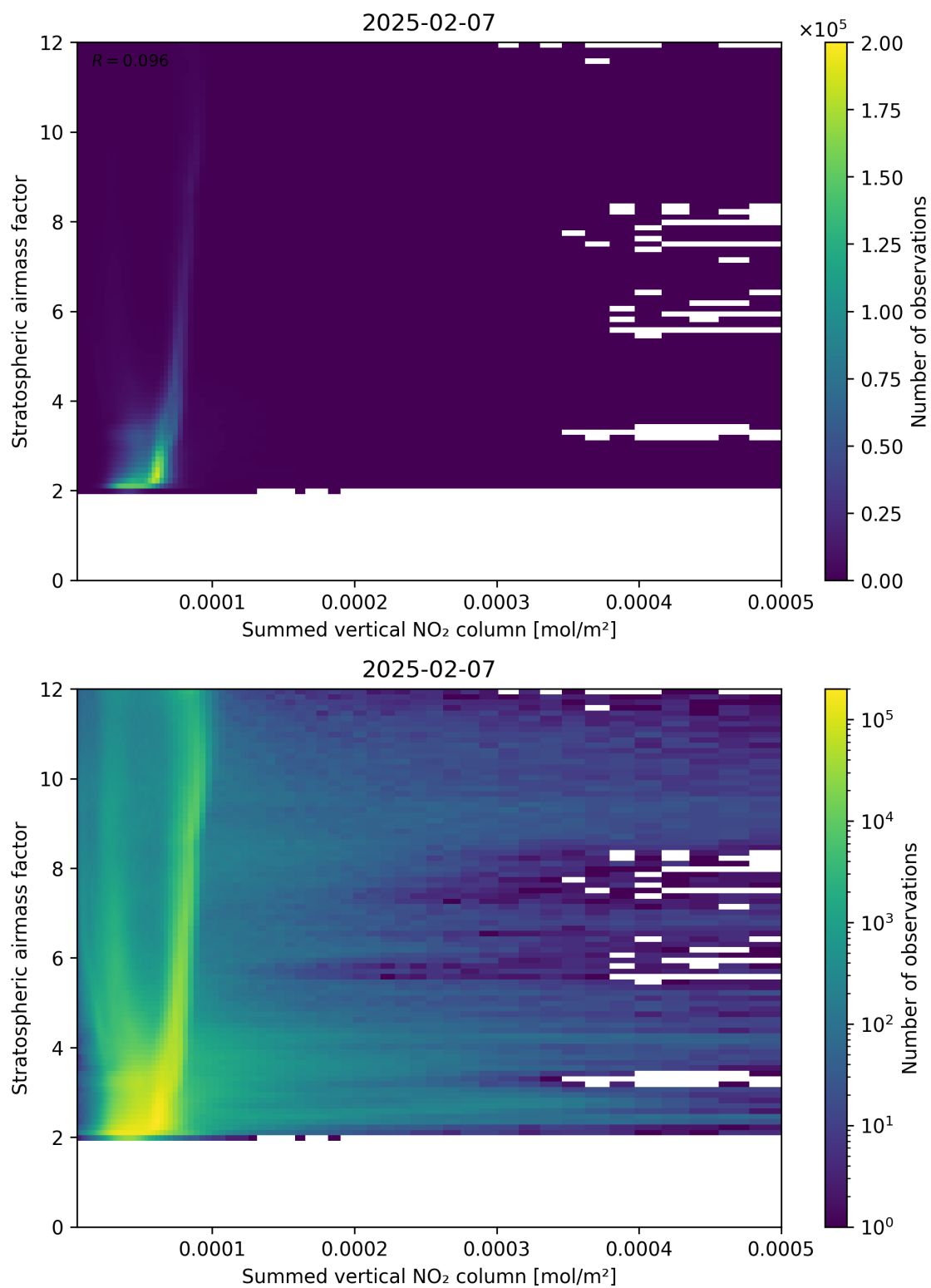
Figure 103: Scatter density plot of “Summed vertical NO 2 column” against “Stratospheric airmass factor” for 2025-02-06 to 2025-02-08.
