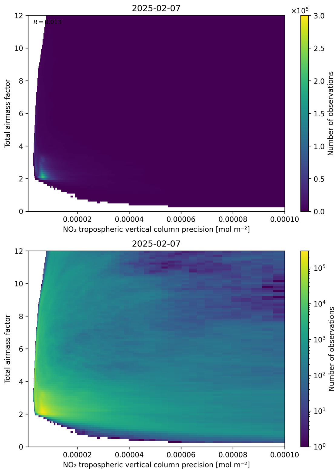
Figure 132: Scatter density plot of “NO 2 tropospheric vertical column precision” against “Total airmass factor” for 2025-02-06 to 2025-02-08.
