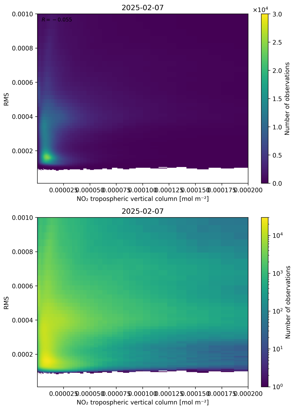
Figure 142: Scatter density plot of “NO 2 tropospheric vertical column” against “RMS” for 2025-02-06 to 2025-02-08.
