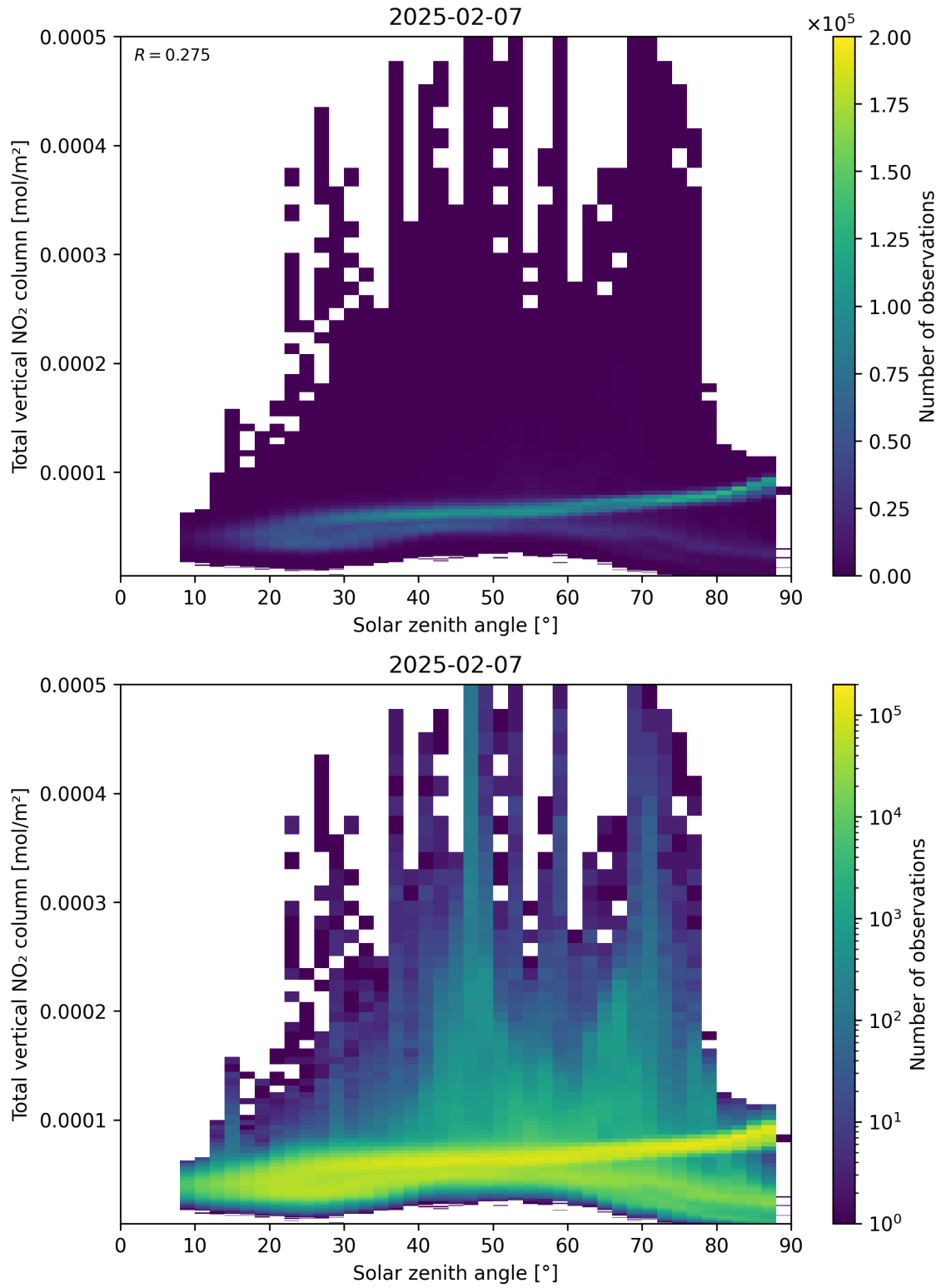
Figure 153: Scatter density plot of “Solar zenith angle” against “Total vertical NO 2 column” for 2025-02-06 to 2025-02-08.
