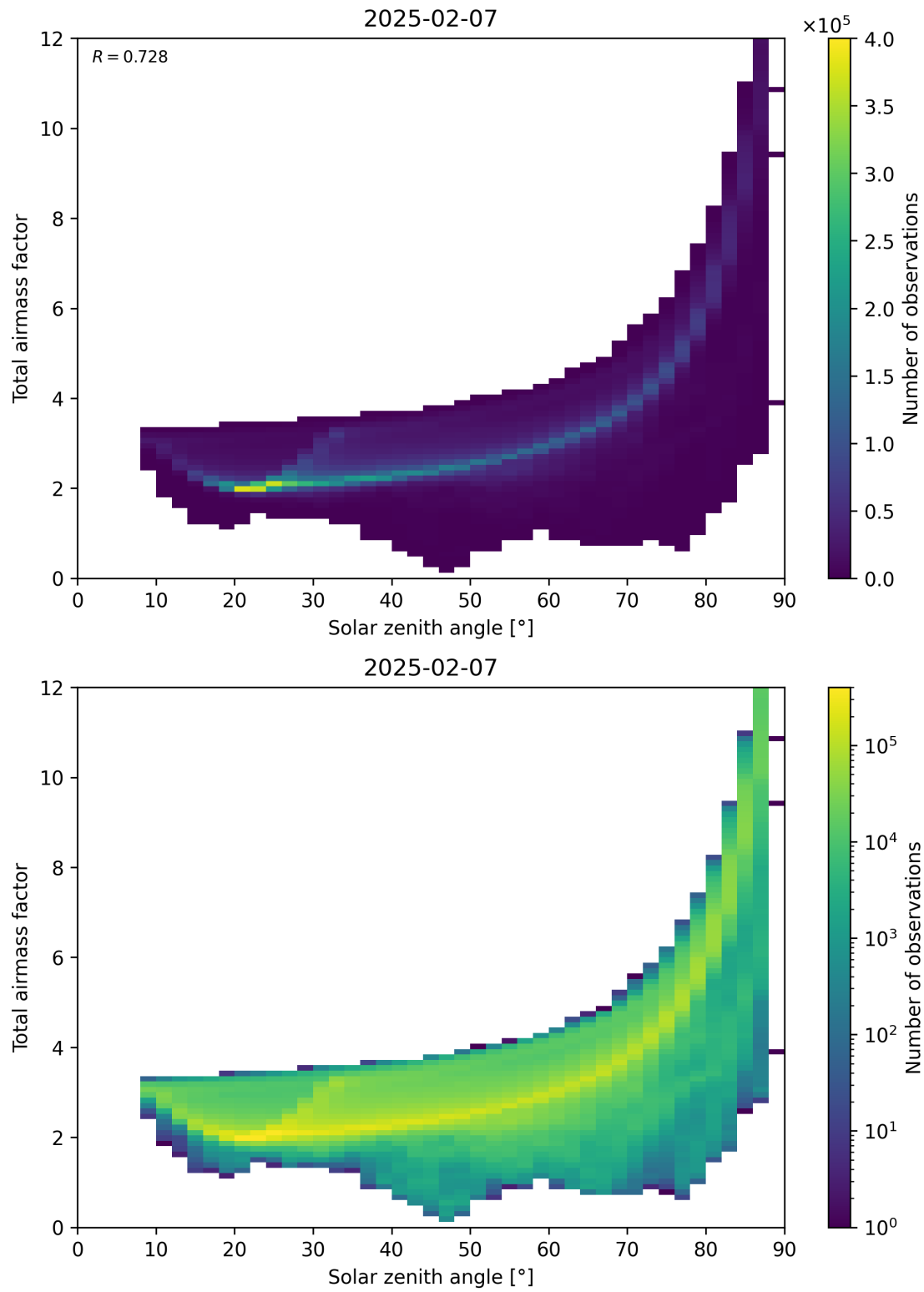
Figure 146: Scatter density plot of “Solar zenith angle” against “Total air mass factor” for 2025-02-06 to 2025-02-08.
