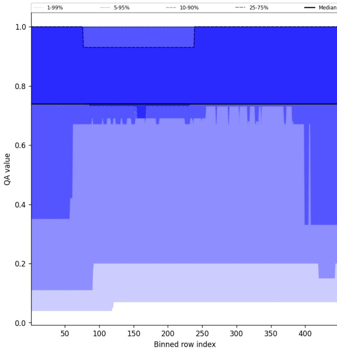
Figure 45: Along track statistics of “QA value” for 2025-02-06 to 2025-02-08
