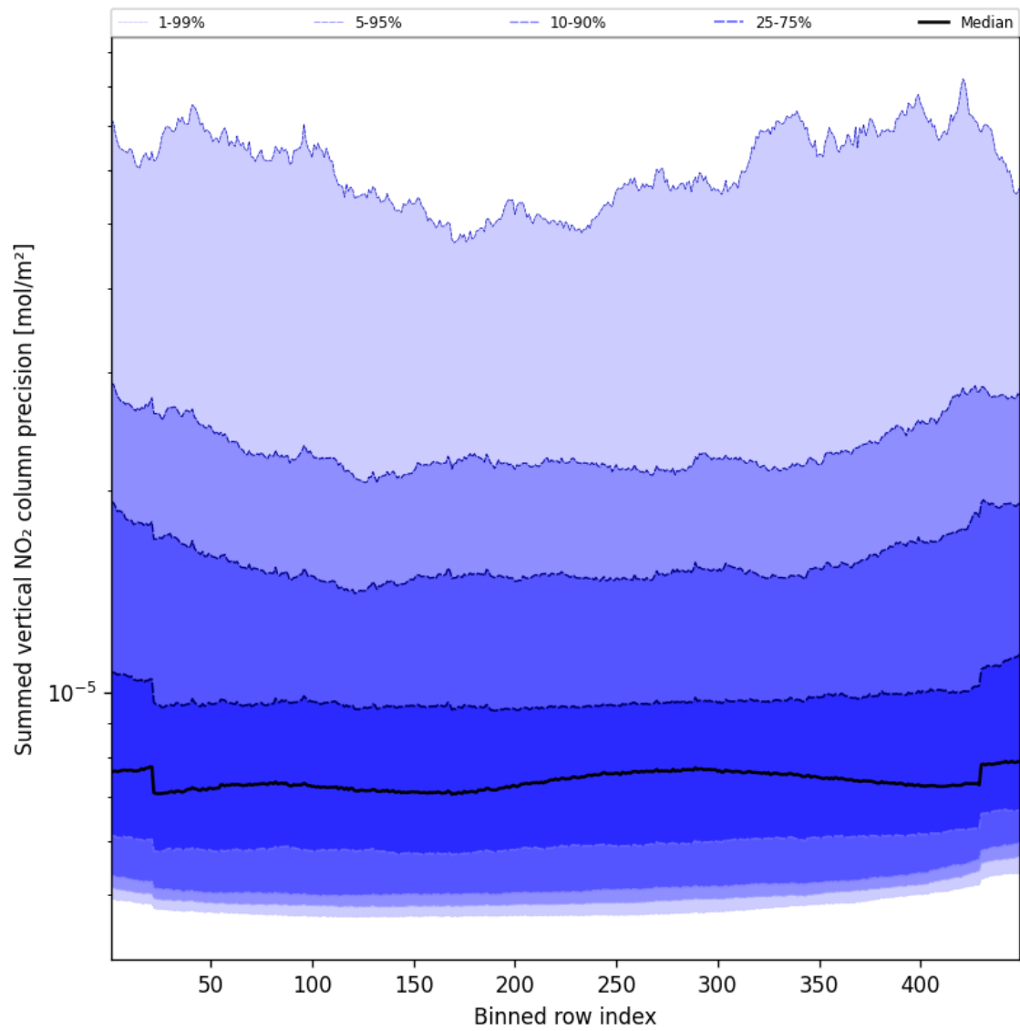
Figure 58: Along track statistics of “Summed vertical NO 2 column precision” for 2025-02-06 to 2025-02-08
