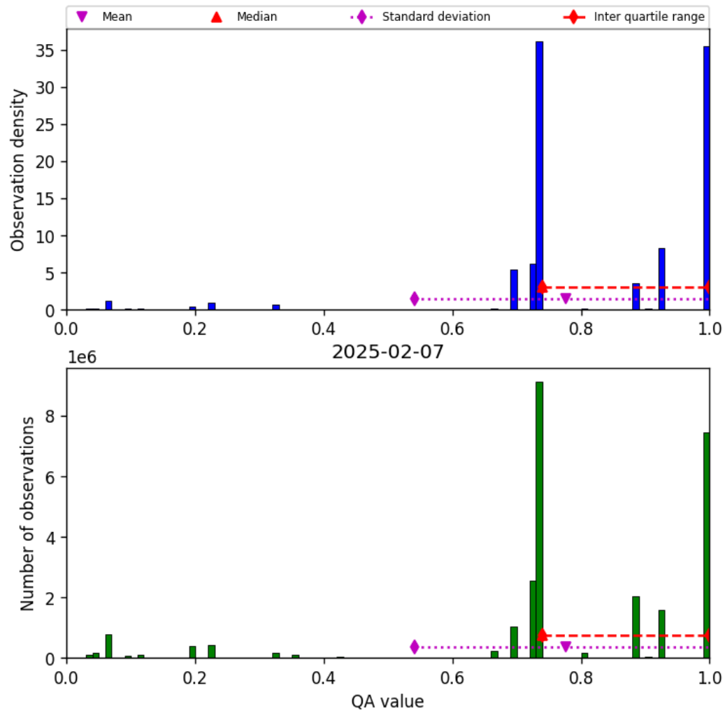
Figure 28: Histogram of “QA value” for 2025-02-06 to 2025-02-08
