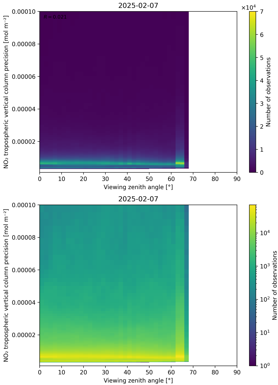
Figure 170: Scatter density plot of “Viewing zenith angle” against “NO 2 tropospheric vertical column precision” for 2025-02-06 to 2025-02-08.
