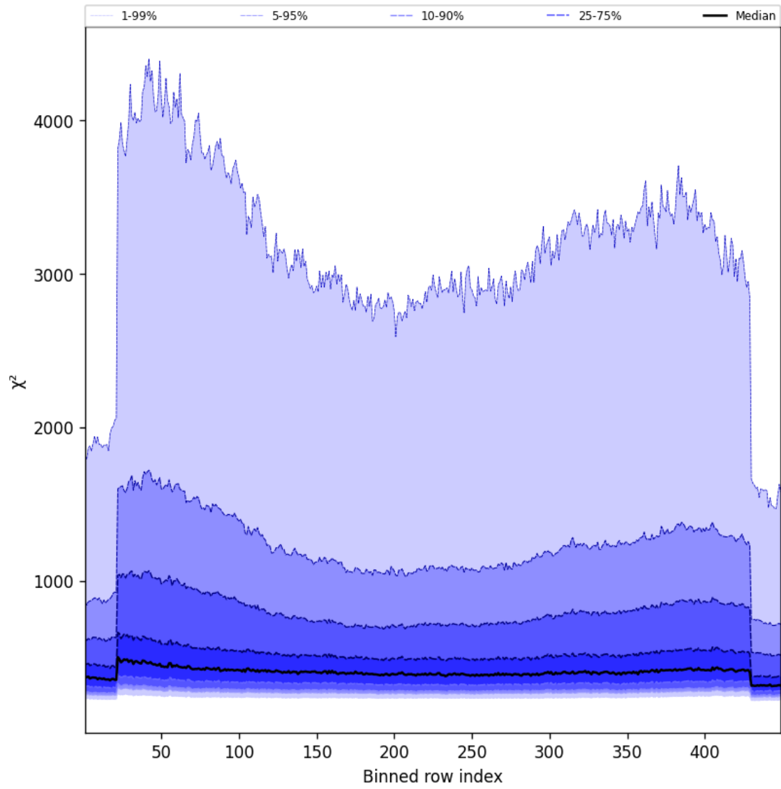
Figure 59: Along track statistics of “ \chi^2 ” for 2025-02-06 to 2025-02-08
