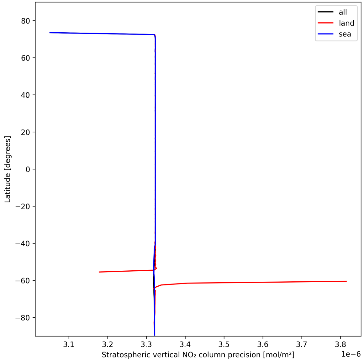
Figure 20: Zonal average of “Stratospheric vertical NO 2 column precision” for 2025-02-06 to 2025-02-08.
