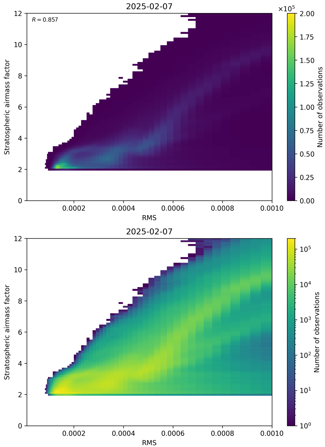
Figure 144: Scatter density plot of “RMS” against “Stratospheric airmass factor” for 2025-02-06 to 2025-02-08.
