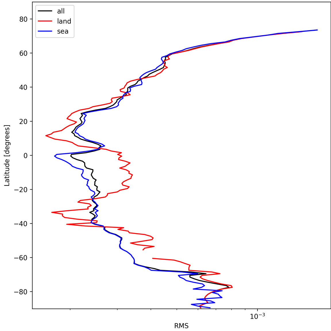
Figure 26: Zonal average of “RMS” for 2025-02-06 to 2025-02-08.
