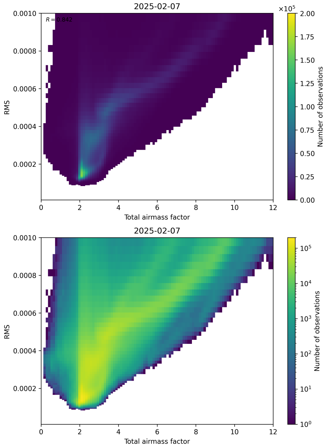
Figure 69: Scatter density plot of “Total airmass factor” against “RMS” for 2025-02-06 to 2025-02-08.
