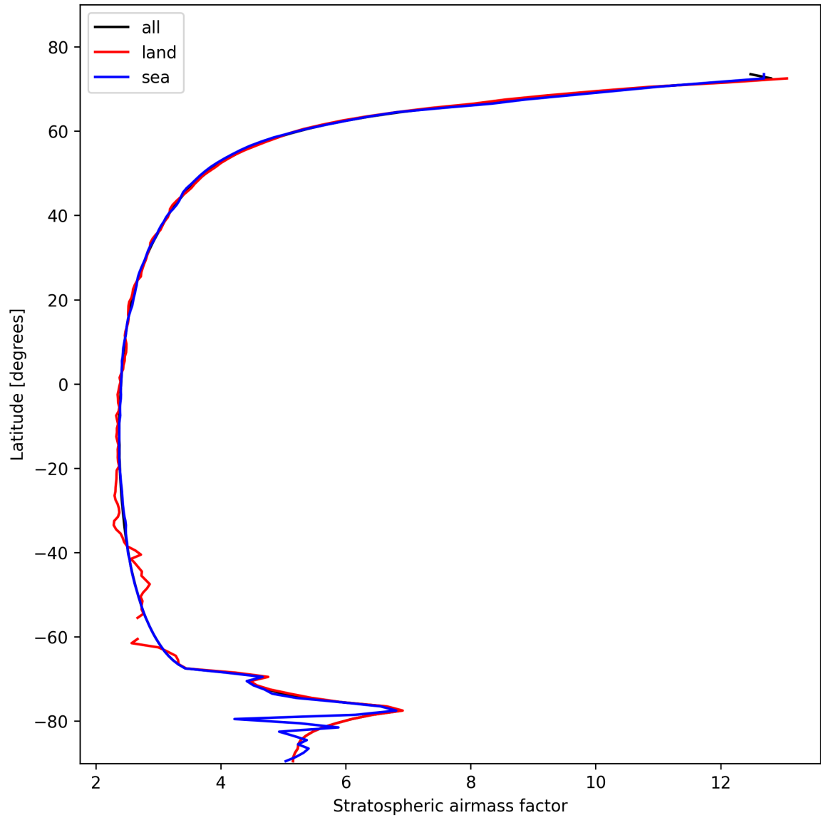
Figure 27: Zonal average of “Stratospheric air mass factor” for 2025-02-06 to 2025-02-08.
