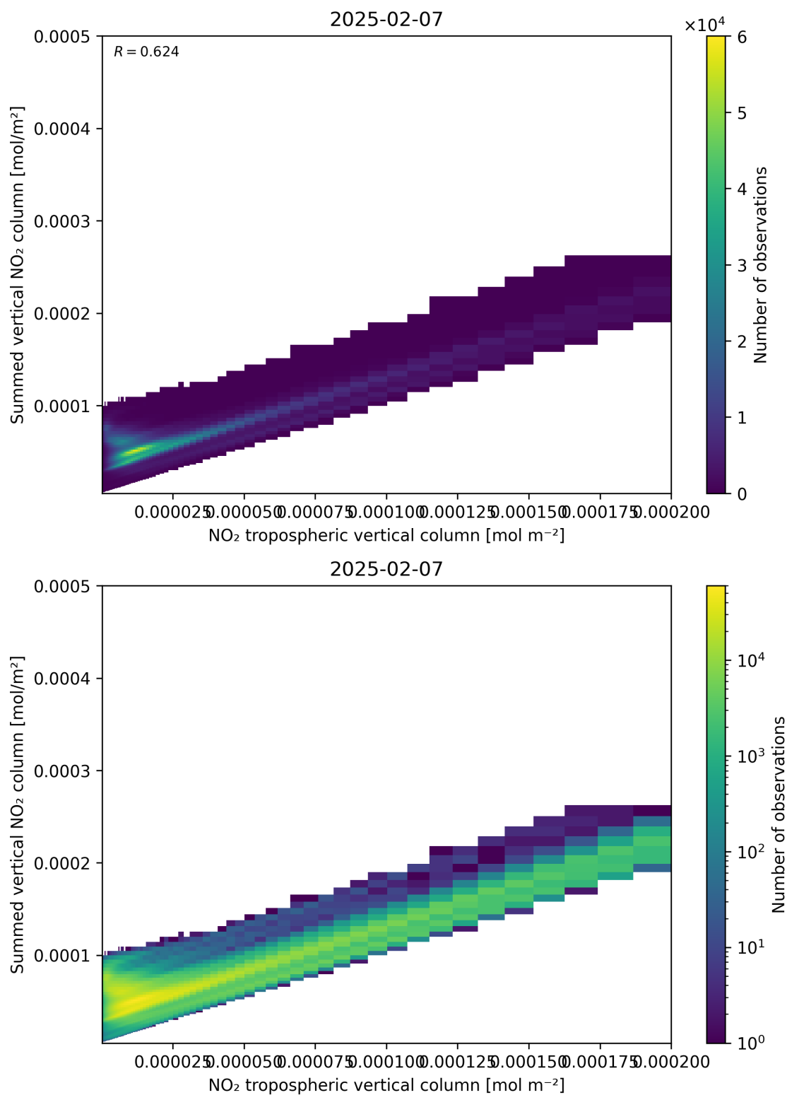
Figure 126: Scatter density plot of “NO 2 tropospheric vertical column” against “Summed vertical NO 2 column” for 2025-02-06 to 2025-02-08.
