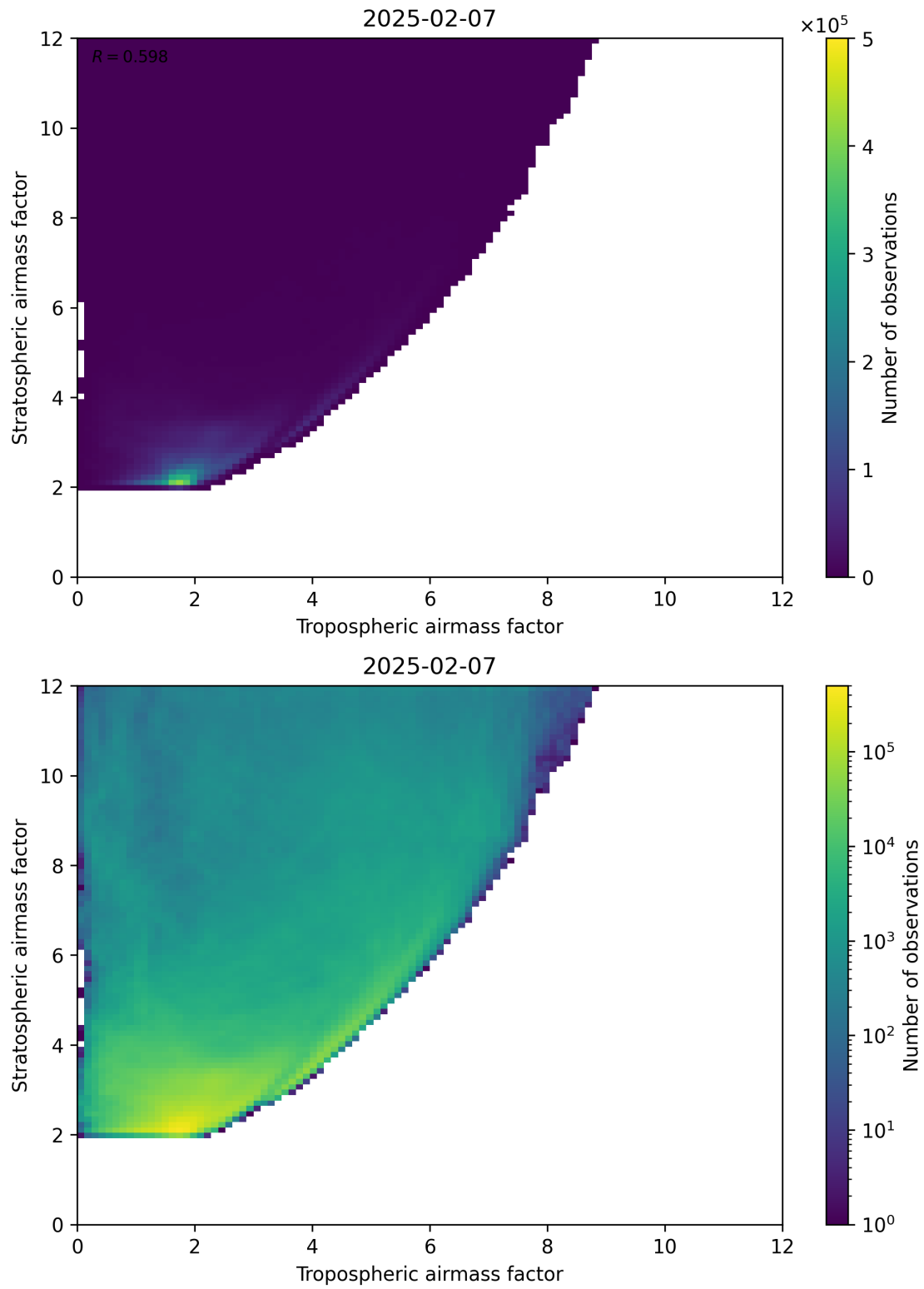
Figure 71: Scatter density plot of “Tropospheric airmass factor” against “Stratospheric airmass factor” for 2025-02-06 to 2025-02-08.
