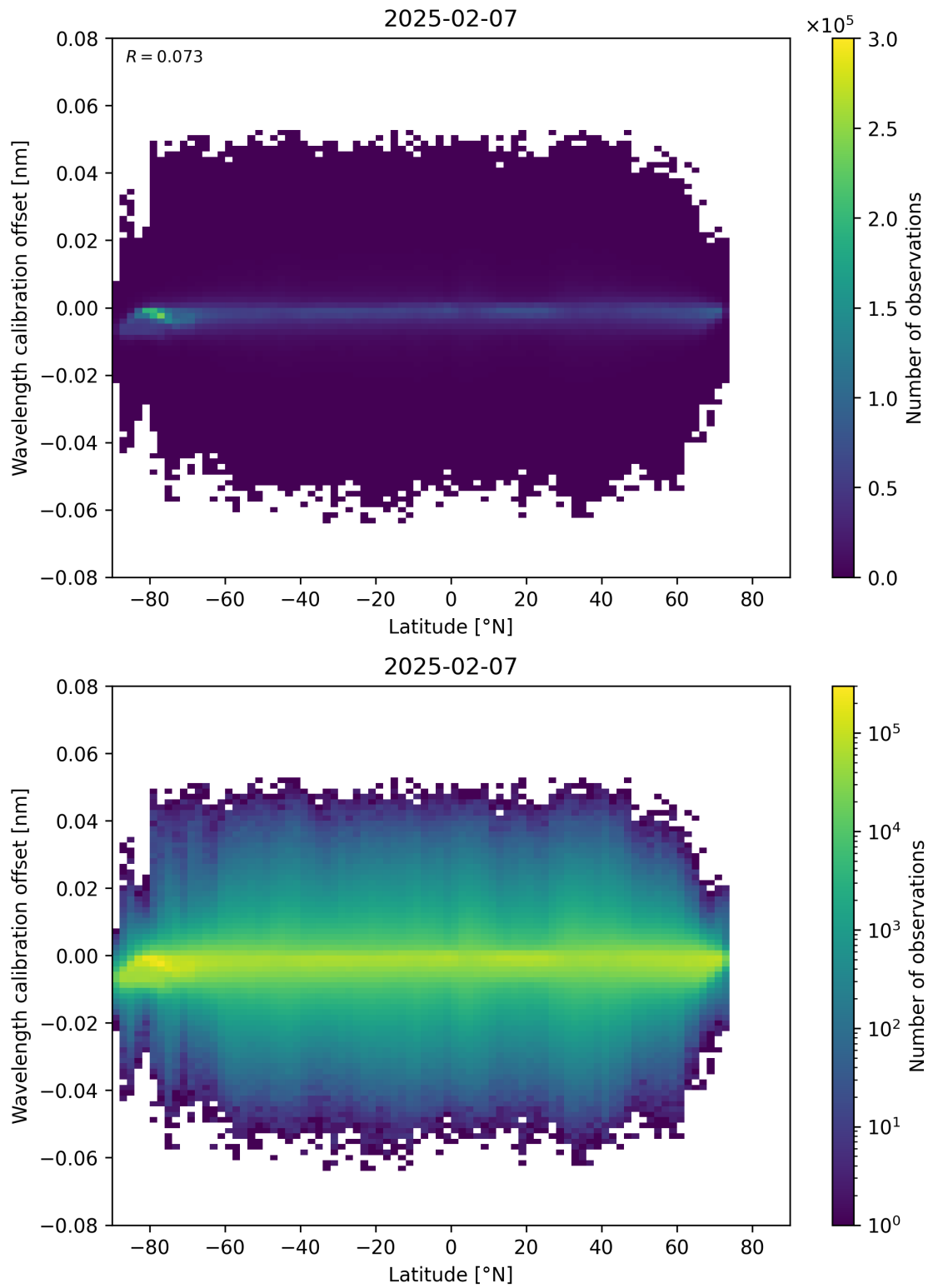
Figure 95: Scatter density plot of “Latitude” against “Wavelength calibration offset” for 2025-02-06 to 2025-02-08.
