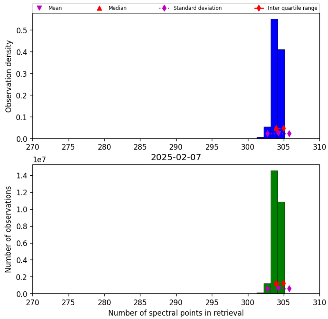
Figure 33: Histogram of “Number of spectral points in retrieval” for 2025-02-06 to 2025-02-08
