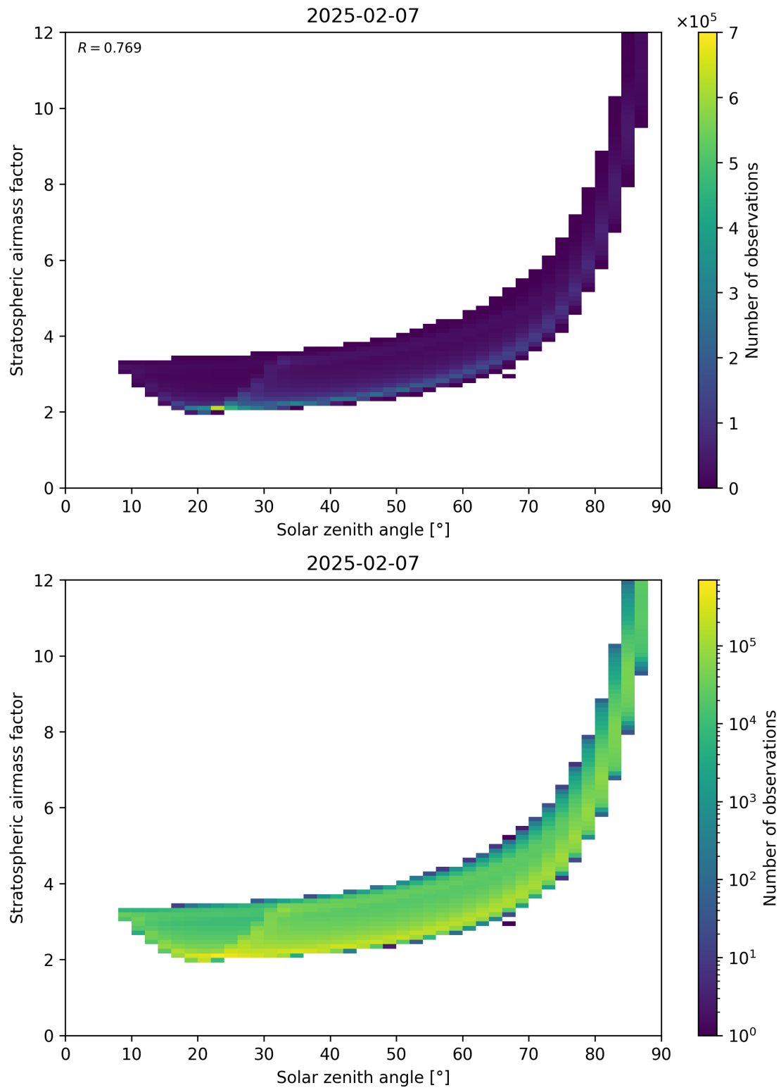
Figure 145: Scatter density plot of “Solar zenith angle” against “Stratospheric airmass factor” for 2025-02-06 to 2025-02-08.
