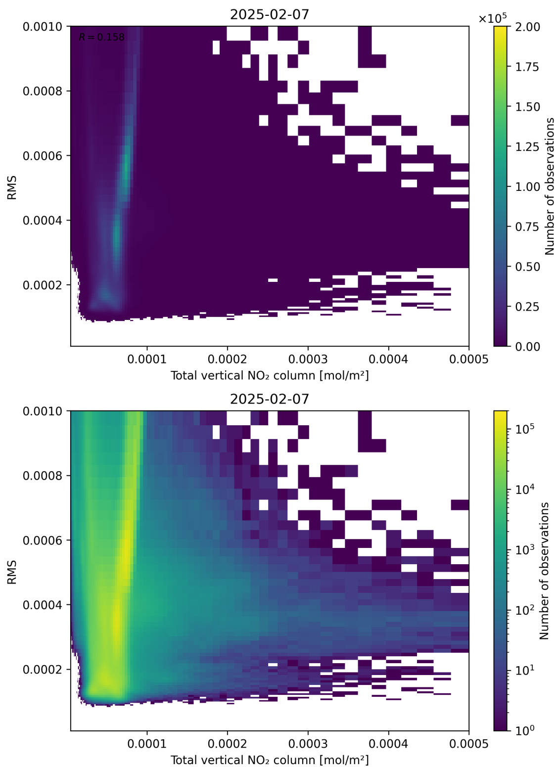
Figure 120: Scatter density plot of “Total vertical NO 2 column” against “RMS” for 2025-02-06 to 2025-02-08.
