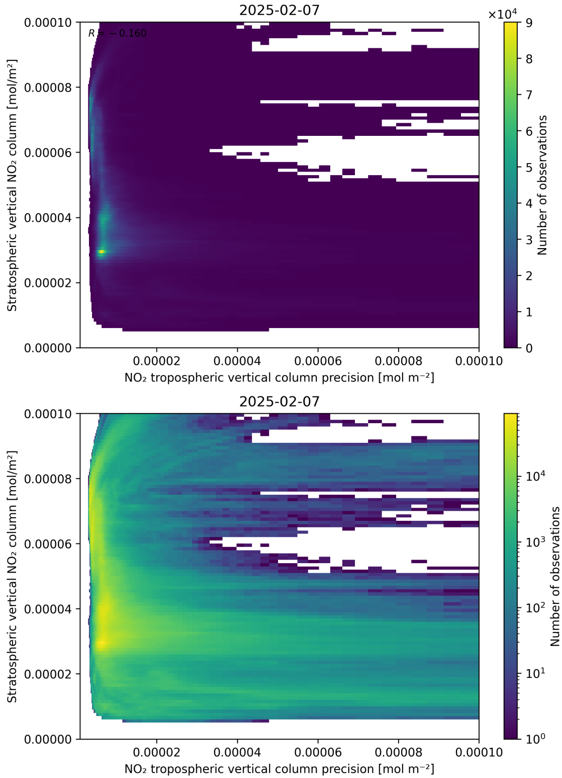
Figure 135: Scatter density plot of “NO 2 tropospheric vertical column precision” against “Stratospheric vertical NO 2 column” for 2025-02-06 to 2025-02-08.
