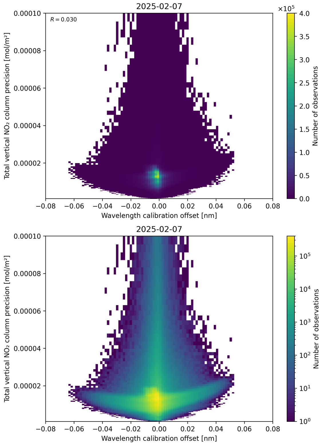
Figure 180: Scatter density plot of “Wavelength calibration offset” against “Total vertical NO 2 column precision” for 2025-02-06 to 2025-02-08.
