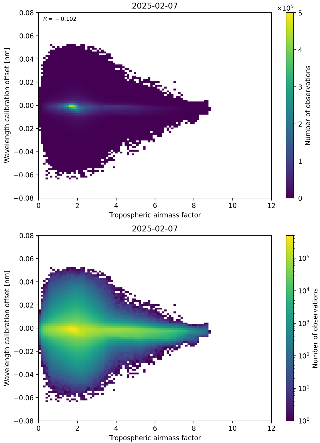
Figure 80: Scatter density plot of “Tropospheric airmass factor” against “Wavelength calibration offset” for 2025-02-06 to 2025-02-08.
