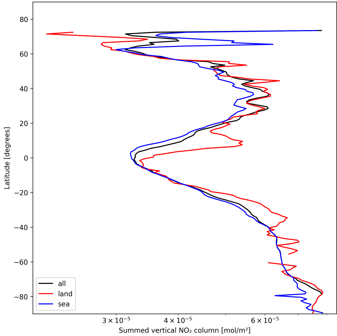
Figure 23: Zonal average of “Summed vertical NO 2 column” for 2025-02-06 to 2025-02-08.
