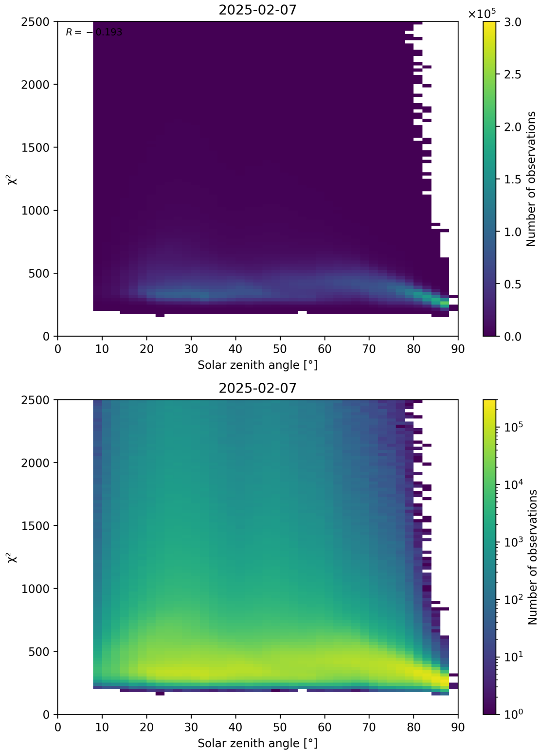
Figure 148: Scatter density plot of “Solar zenith angle” against “ \chi^2 ” for 2025-02-06 to 2025-02-08.
