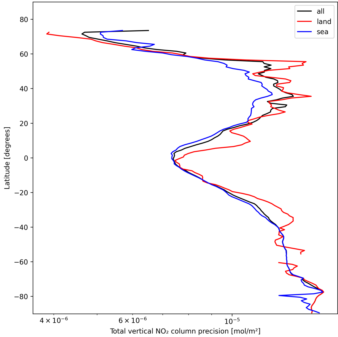
Figure 22: Zonal average of “Total vertical NO 2 column precision” for 2025-02-06 to 2025-02-08.
