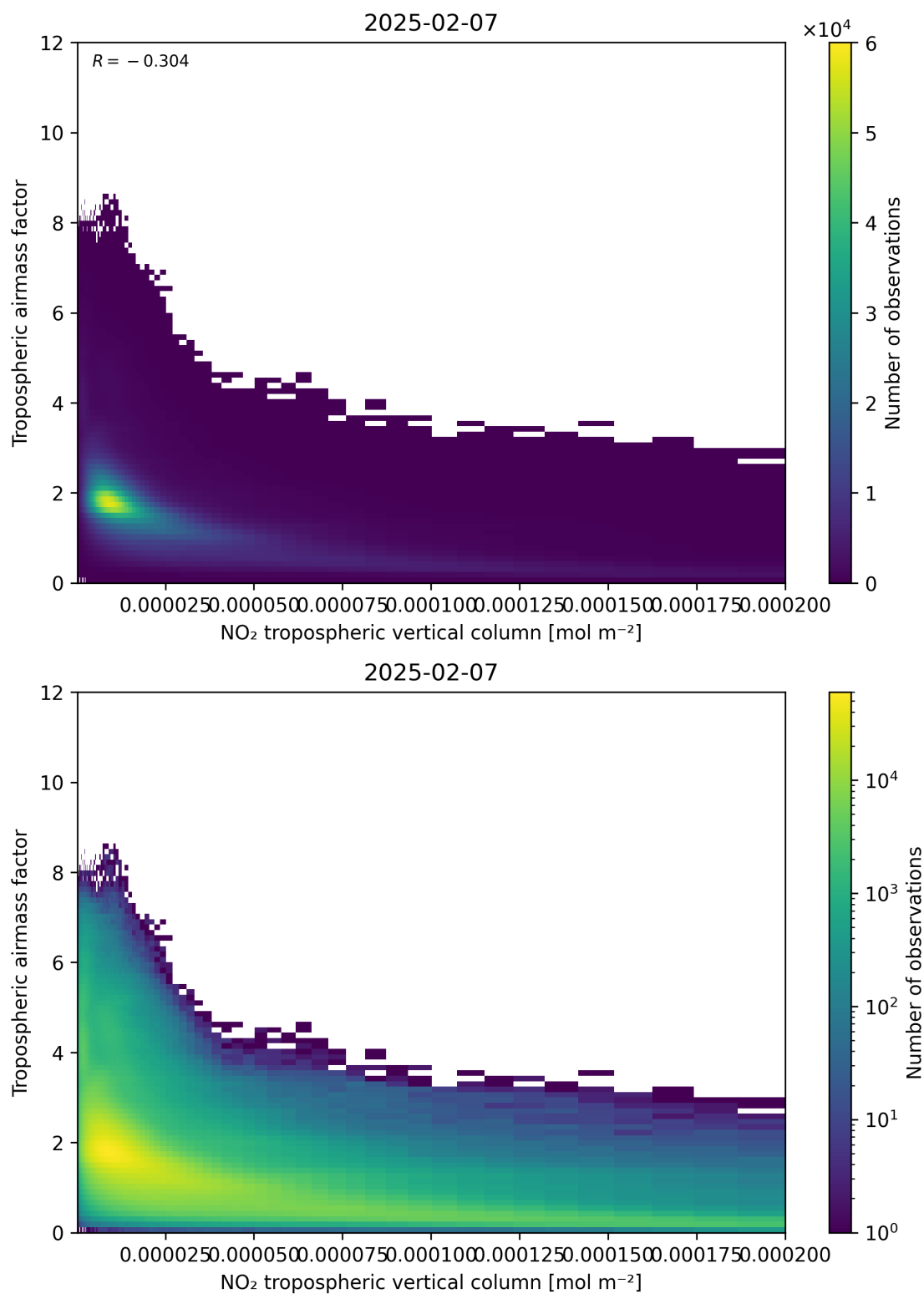
Figure 123: Scatter density plot of “NO 2 tropospheric vertical column” against “Tropospheric air mass factor” for 2025-02-06 to 2025-02-08.
