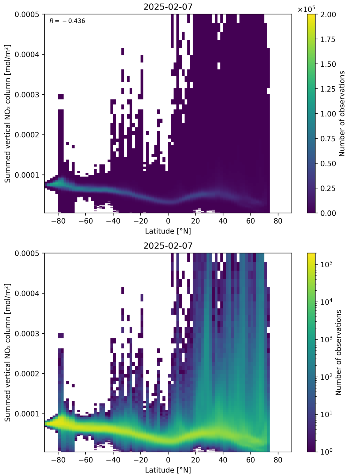
Figure 88: Scatter density plot of “Latitude” against “Summed vertical NO 2 column” for 2025-02-06 to 2025-02-08.
