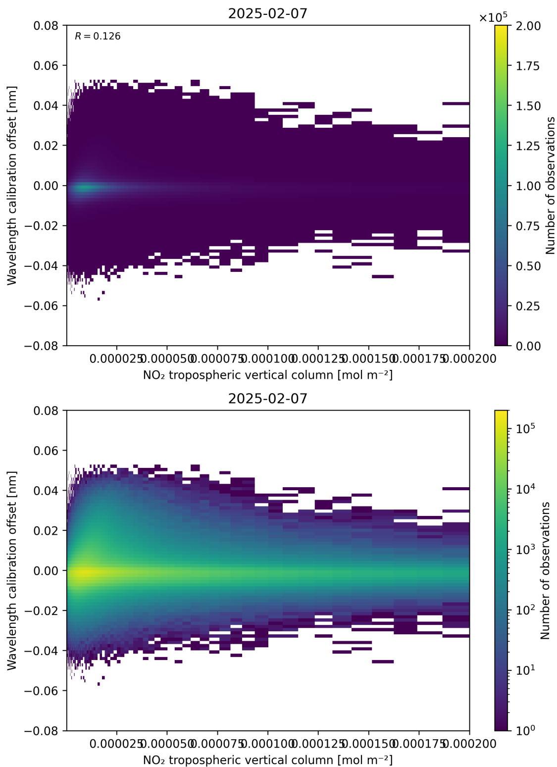
Figure 143: Scatter density plot of “NO 2 tropospheric vertical column” against “Wavelength calibration offset” for 2025-02-06 to 2025-02-08.
