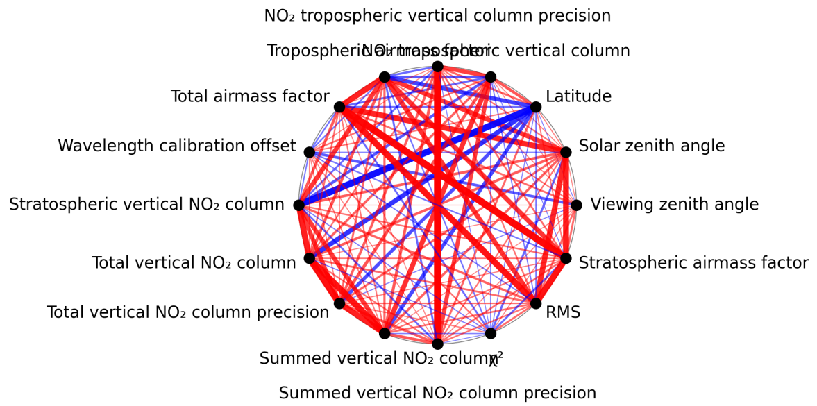
Figure 1: Map of correlation graph for 2025-02-06 to 2025-02-08.
