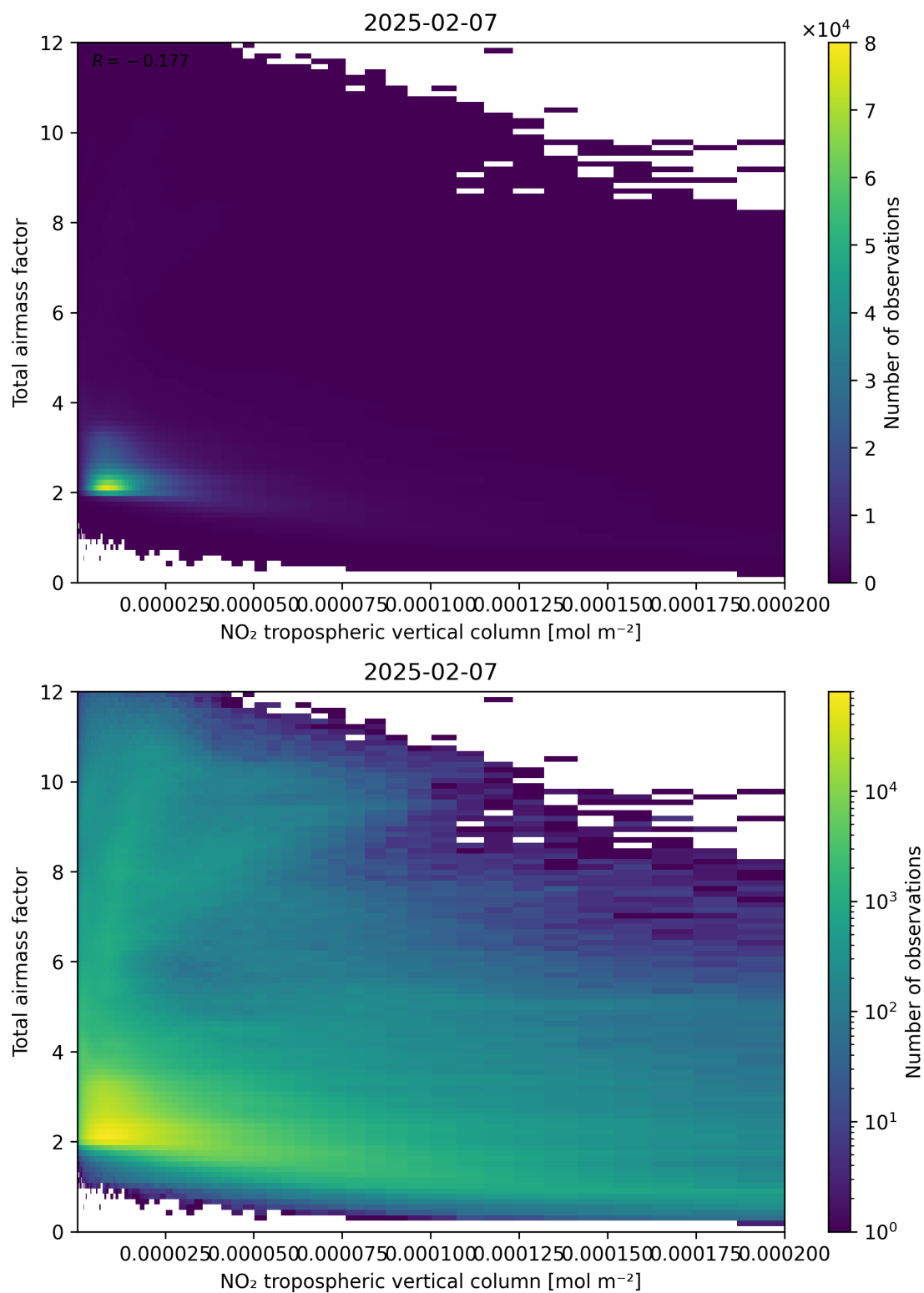
Figure 122: Scatter density plot of “NO 2 tropospheric vertical column” against “Total air mass factor” for 2025-02-06 to 2025-02-08.
