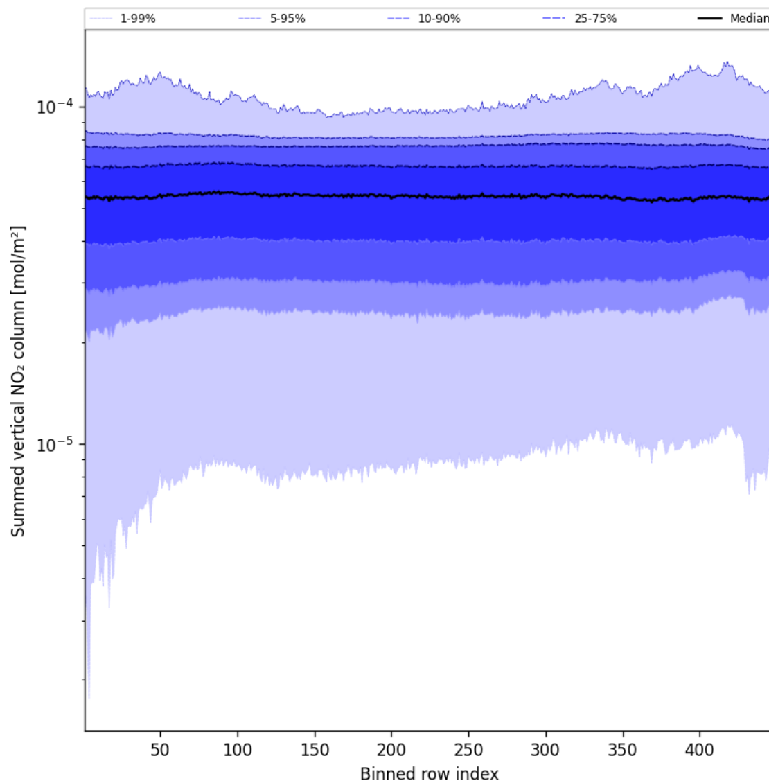
Figure 57: Along track statistics of “Summed vertical NO 2 column” for 2025-02-06 to 2025-02-08
