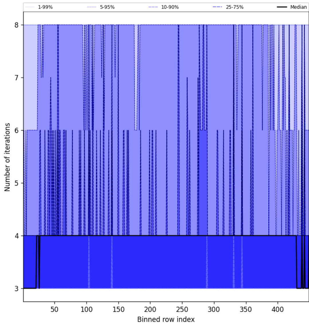
Figure 51: Along track statistics of “Number of iterations” for 2025-02-06 to 2025-02-08
