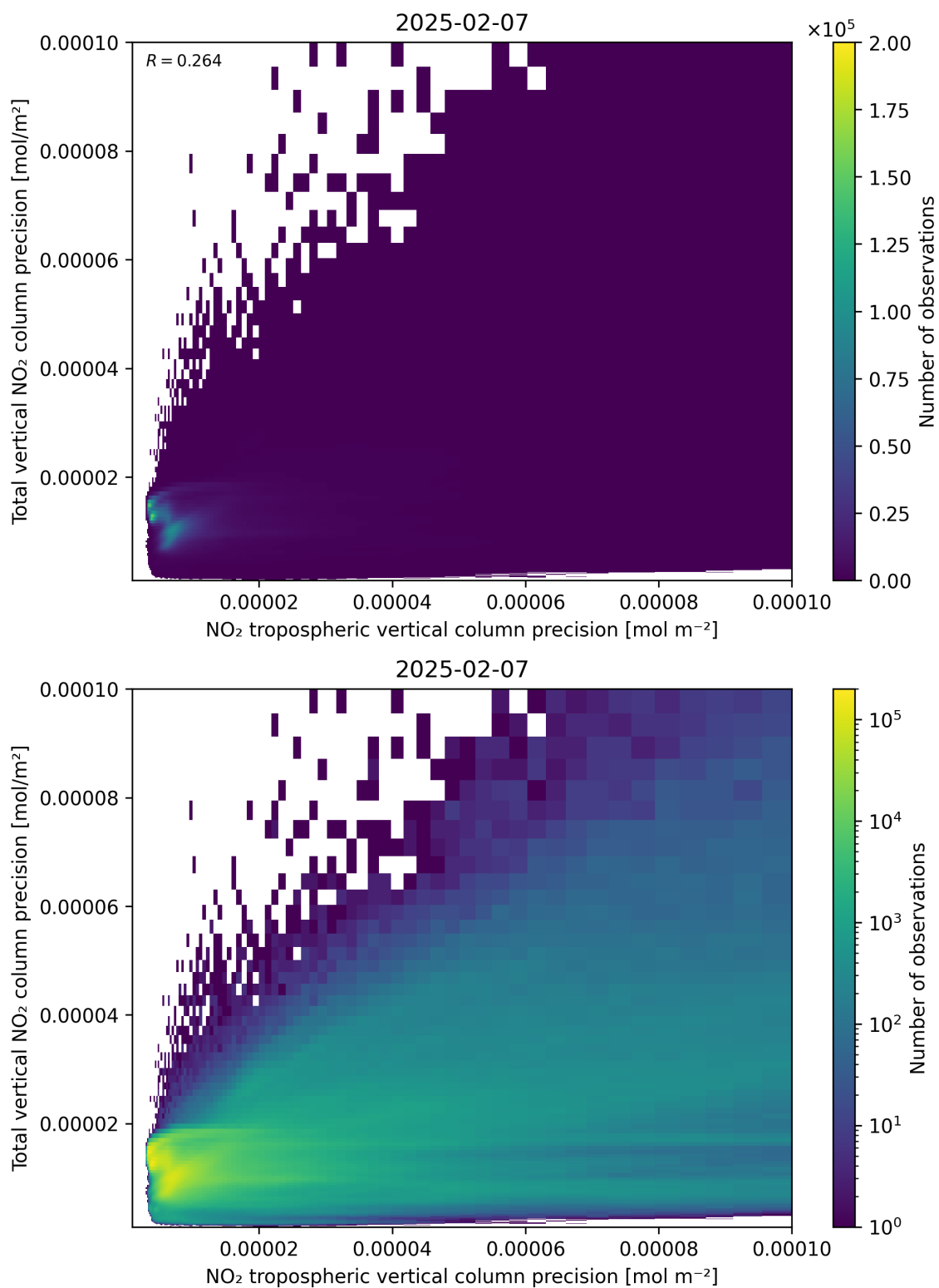
Figure 139: Scatter density plot of “NO 2 tropospheric vertical column precision” against “Total vertical NO 2 column precision” for 2025-02-06 to 2025-02-08.
