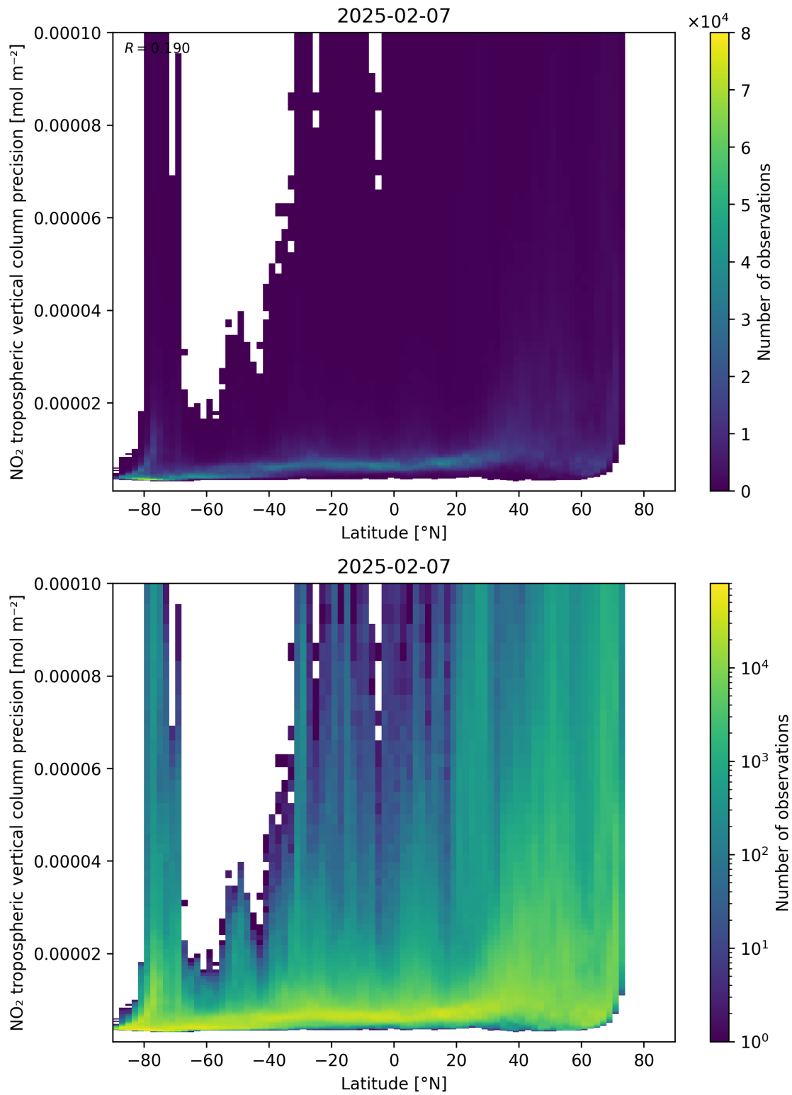
Figure 93: Scatter density plot of “Latitude” against “NO 2 tropospheric vertical column precision” for 2025-02-06 to 2025-02-08.
