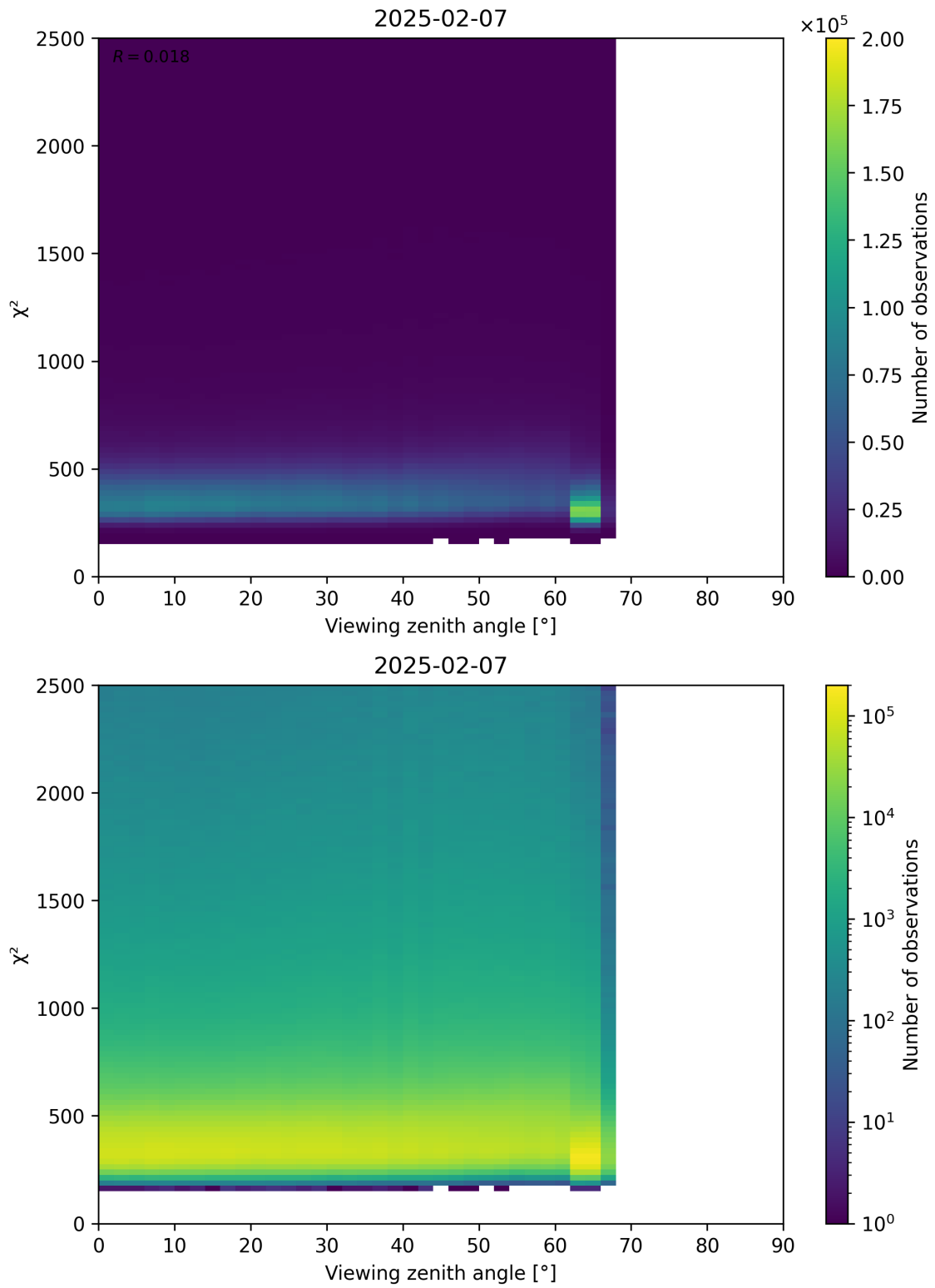
Figure 162: Scatter density plot of “Viewing zenith angle” against “ \chi^2 ” for 2025-02-06 to 2025-02-08.
