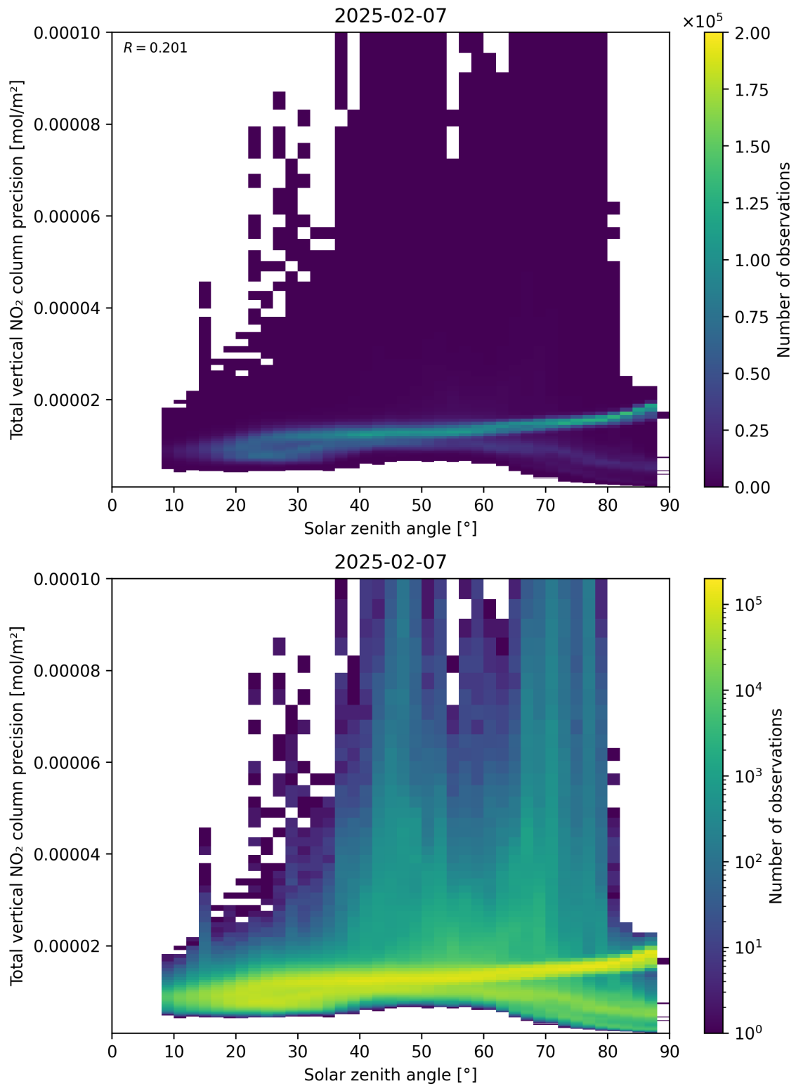
Figure 154: Scatter density plot of “Solar zenith angle” against “Total vertical NO 2 column precision” for 2025-02-06 to 2025-02-08.
