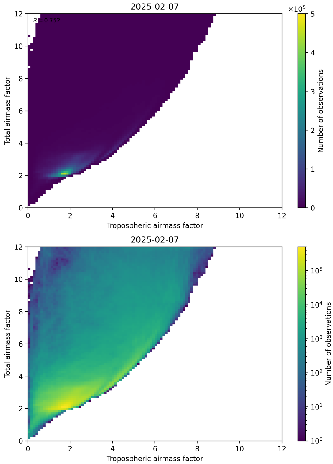
Figure 72: Scatter density plot of “Tropospheric airmass factor” against “Total airmass factor” for 2025-02-06 to 2025-02-08.
