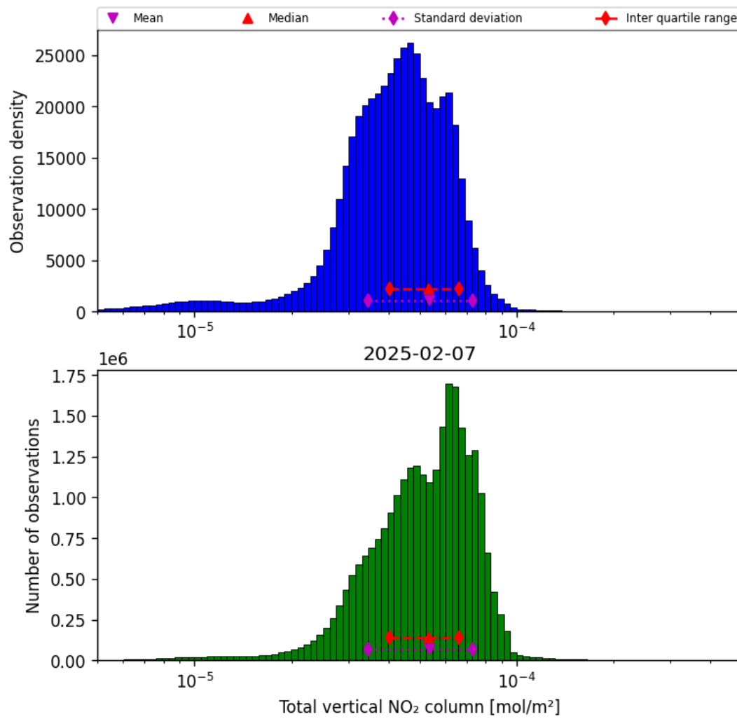
Figure 38: Histogram of “Total vertical NO 2 column” for 2025-02-06 to 2025-02-08
