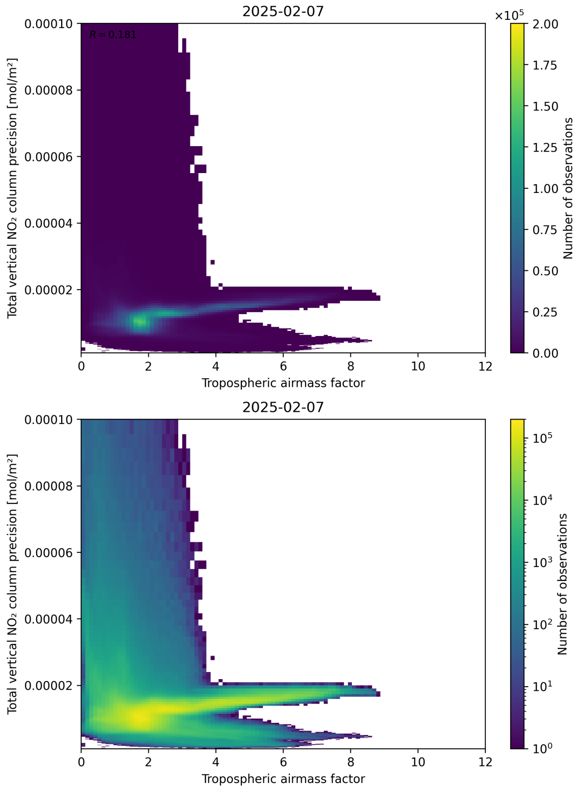
Figure 78: Scatter density plot of “Tropospheric air mass factor” against “Total vertical NO 2 column precision” for 2025-02-06 to 2025-02-08.
