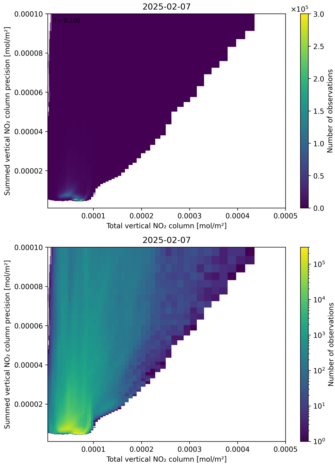
Figure 113: Scatter density plot of “Total vertical NO 2 column” against “Summed vertical NO 2 column precision” for 2025-02-06 to 2025-02-08.
