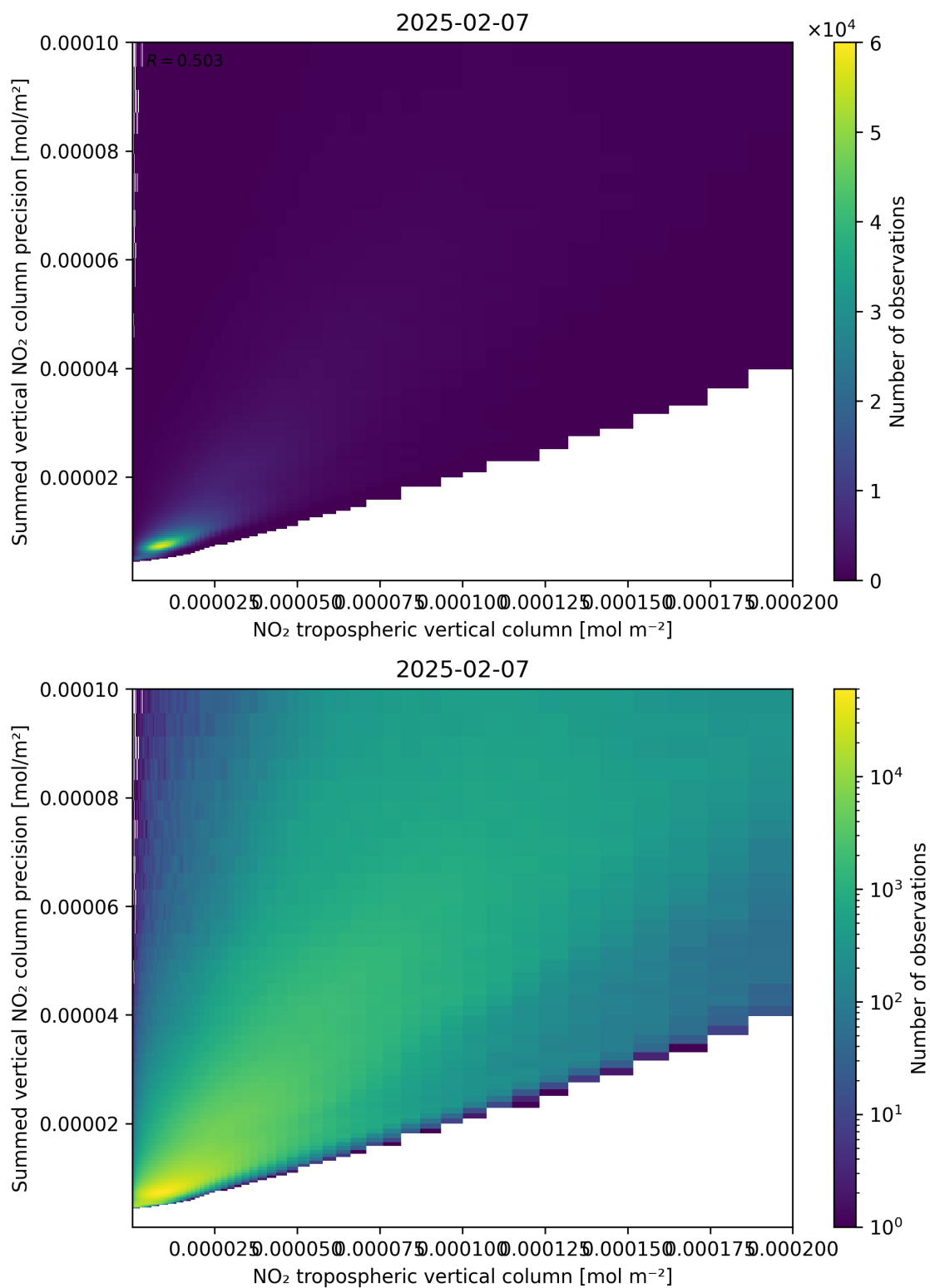
Figure 127: Scatter density plot of “NO 2 tropospheric vertical column” against “Summed vertical NO 2 column precision” for 2025-02-06 to 2025-02-08.
