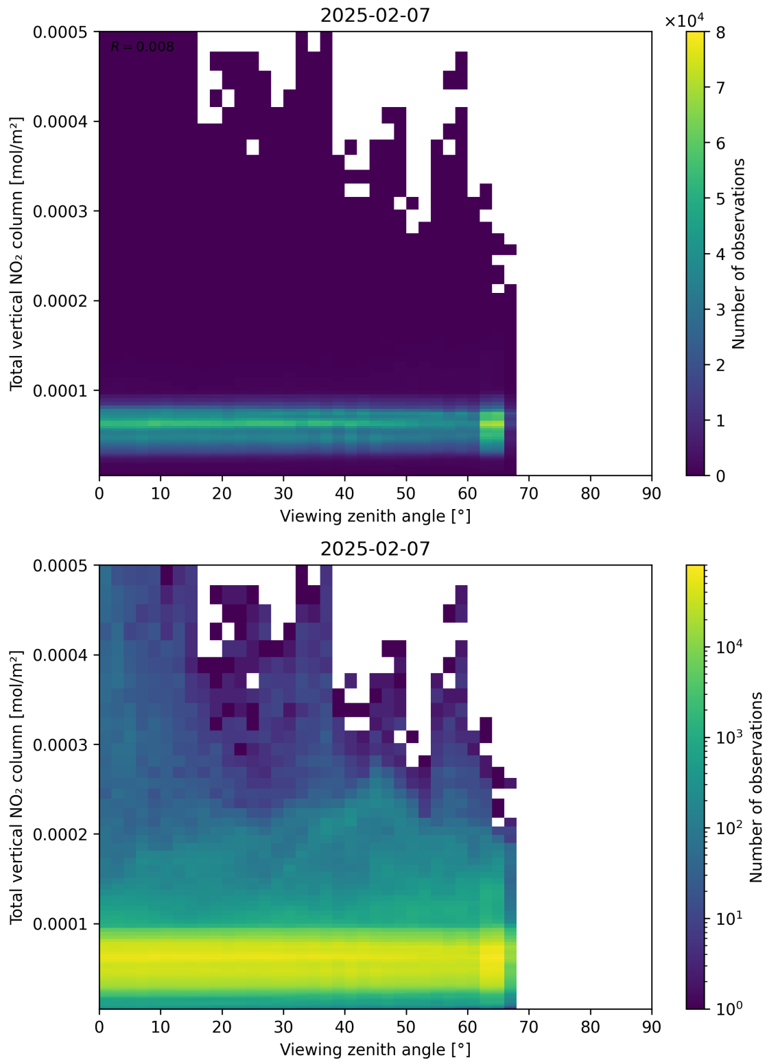
Figure 167: Scatter density plot of “Viewing zenith angle” against “Total vertical NO 2 column” for 2025-02-06 to 2025-02-08.
