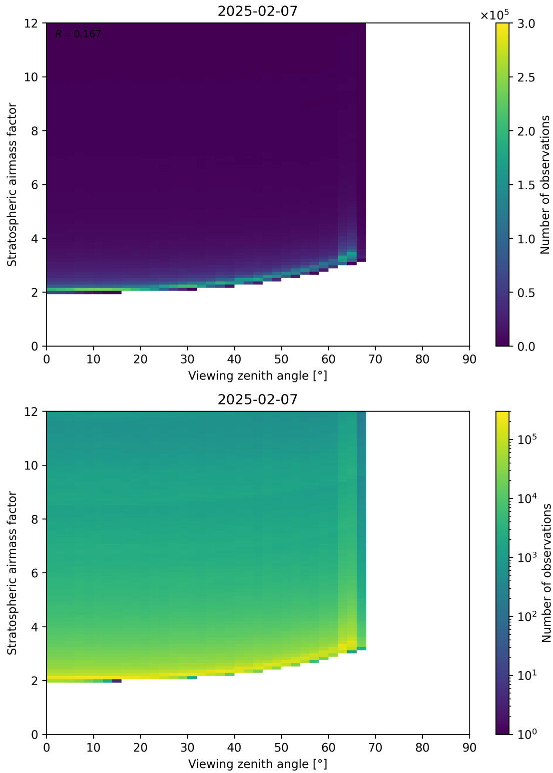
Figure 159: Scatter density plot of “Viewing zenith angle” against “Stratospheric airmass factor” for 2025-02-06 to 2025-02-08.
