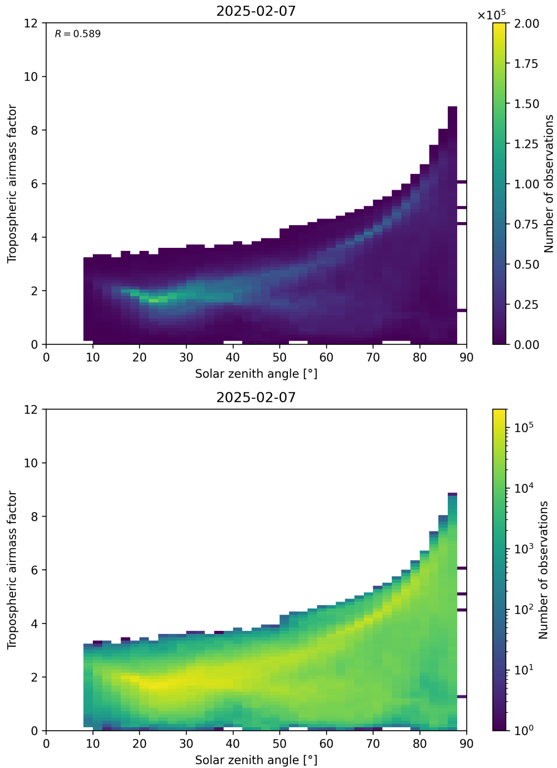
Figure 147: Scatter density plot of “Solar zenith angle” against “Tropospheric airmass factor” for 2025-02-06 to 2025-02-08.
