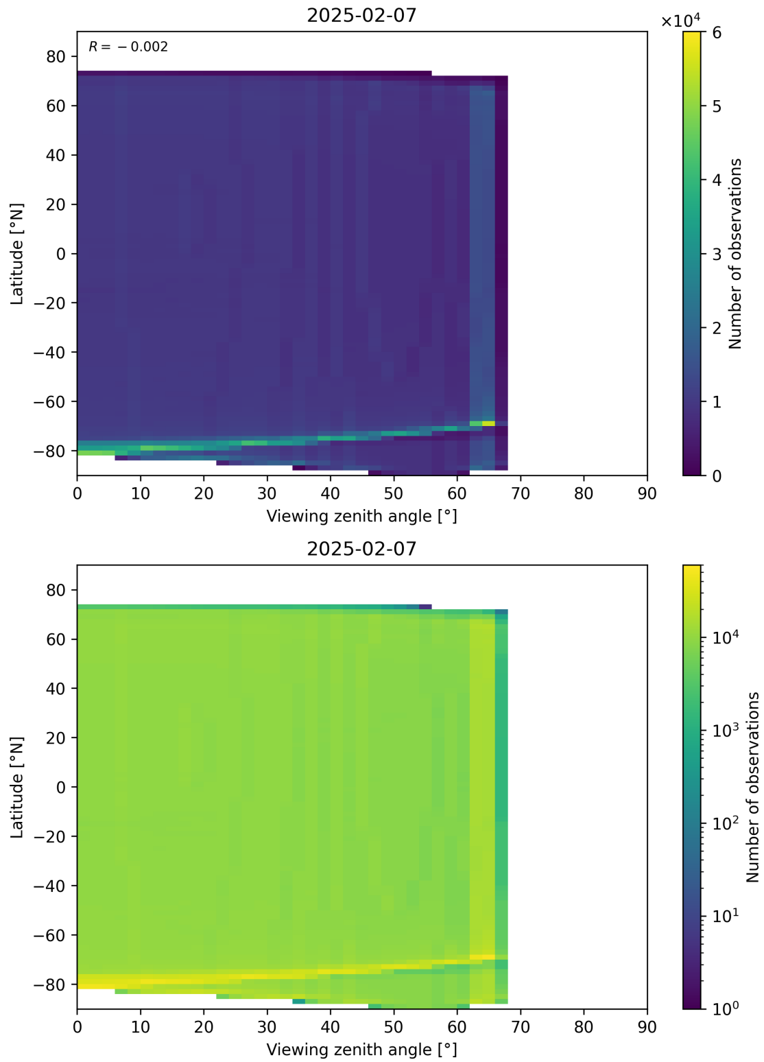
Figure 163: Scatter density plot of “Viewing zenith angle” against “Latitude” for 2025-02-06 to 2025-02-08.
