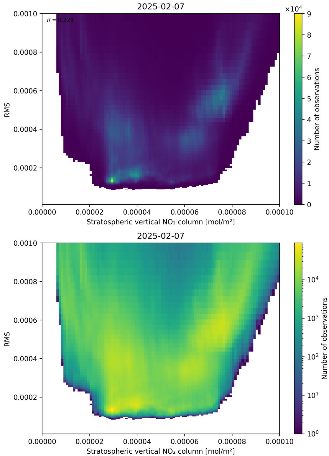
Figure 102: Scatter density plot of “Stratospheric vertical NO 2 column” against “RMS” for 2025-02-06 to 2025-02-08.
