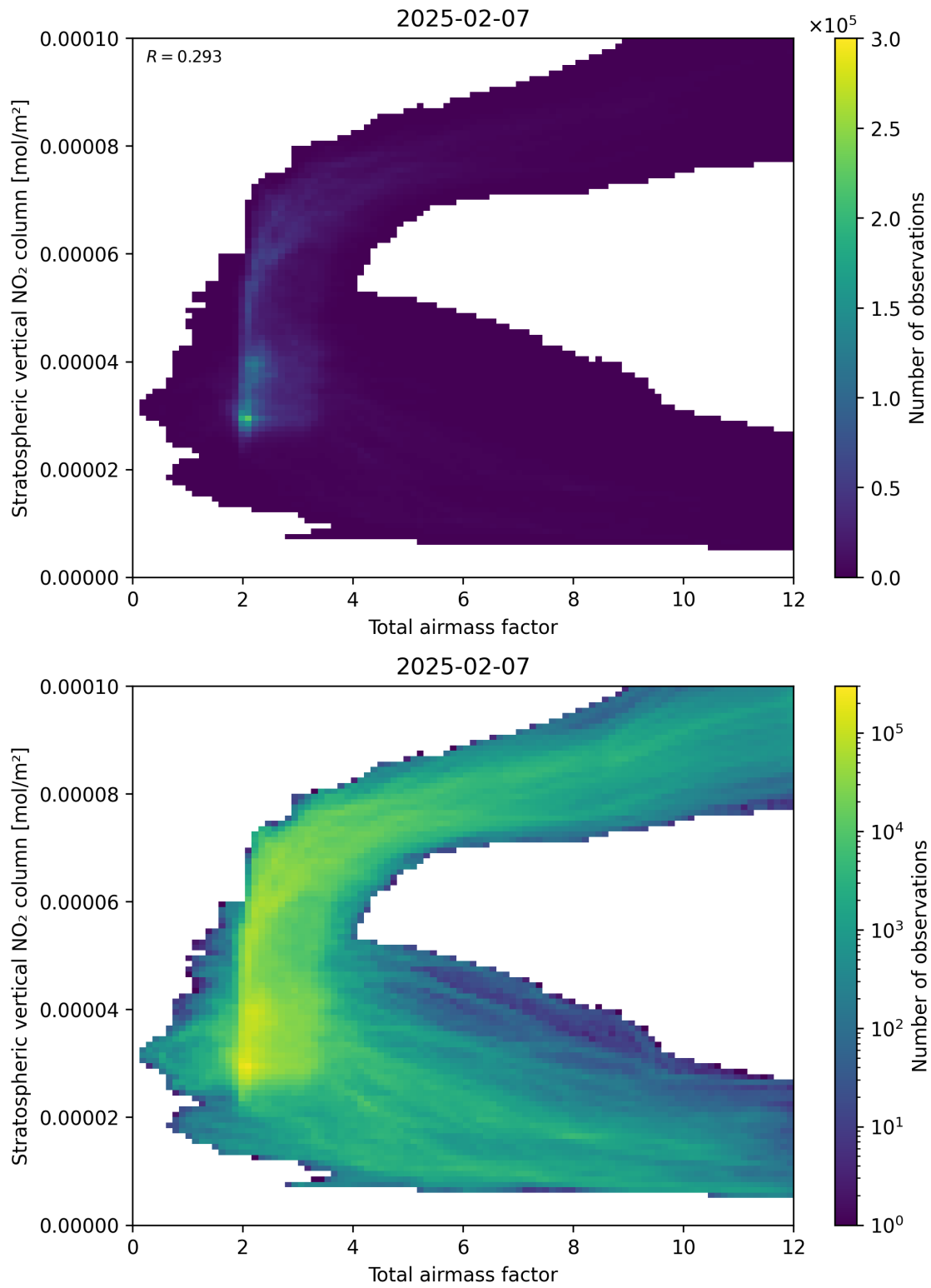
Figure 64: Scatter density plot of “Total airmass factor” against “Stratospheric vertical NO 2 column” for 2025-02-06 to 2025-02-08.
