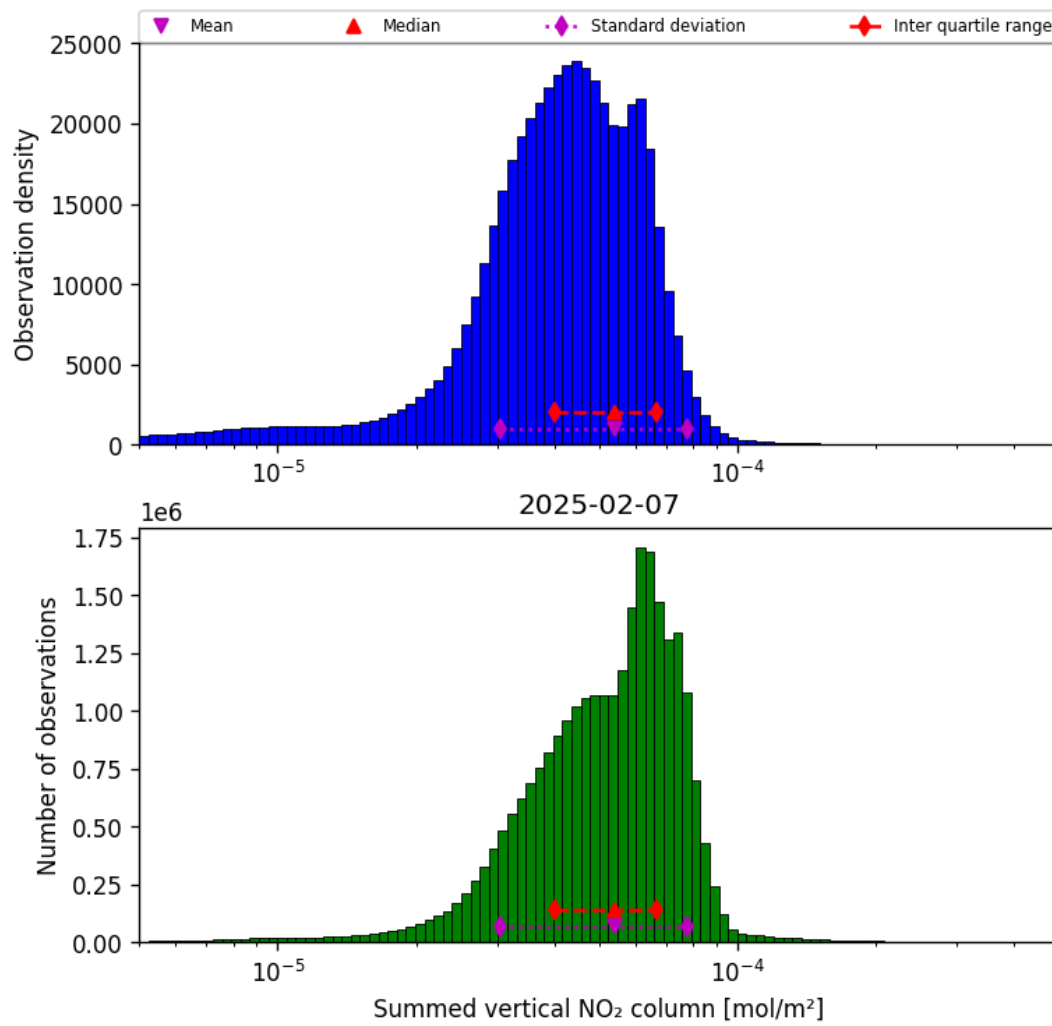
Figure 40: Histogram of “Summed vertical NO 2 column” for 2025-02-06 to 2025-02-08
