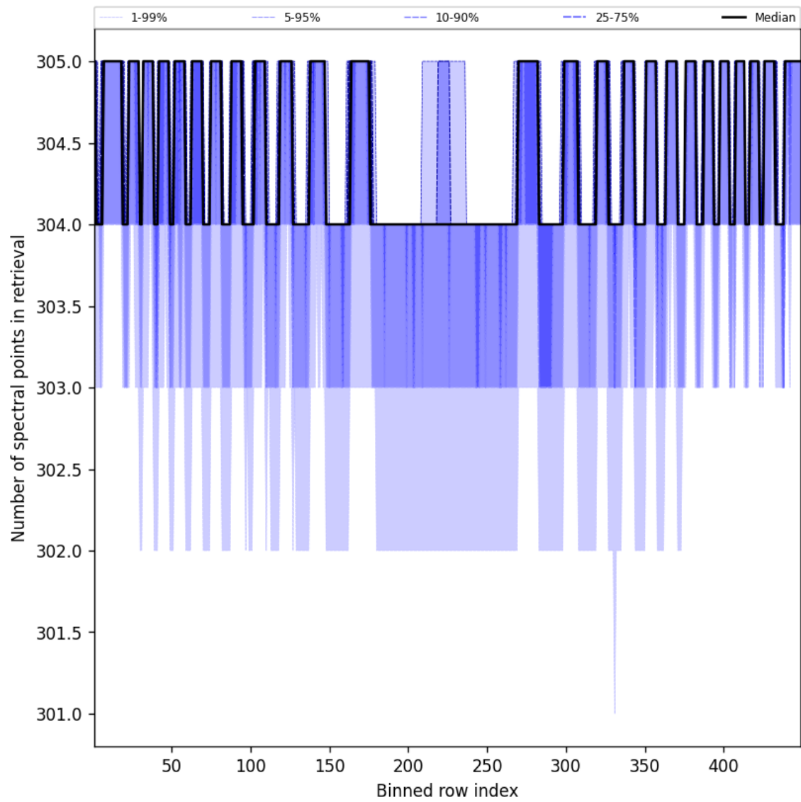
Figure 50: Along track statistics of “Number of spectral points in retrieval” for 2025-02-06 to 2025-02-08
