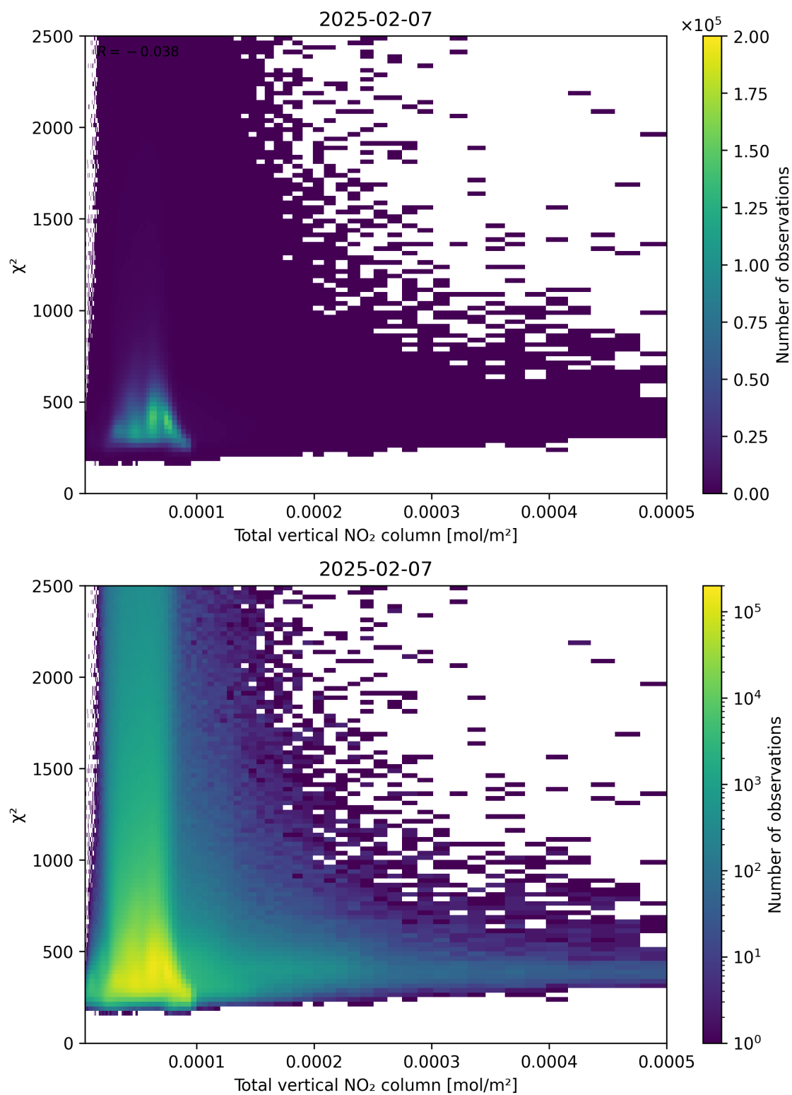
Figure 111: Scatter density plot of “Total vertical NO 2 column” against “ \chi^2 ” for 2025-02-06 to 2025-02-08.
