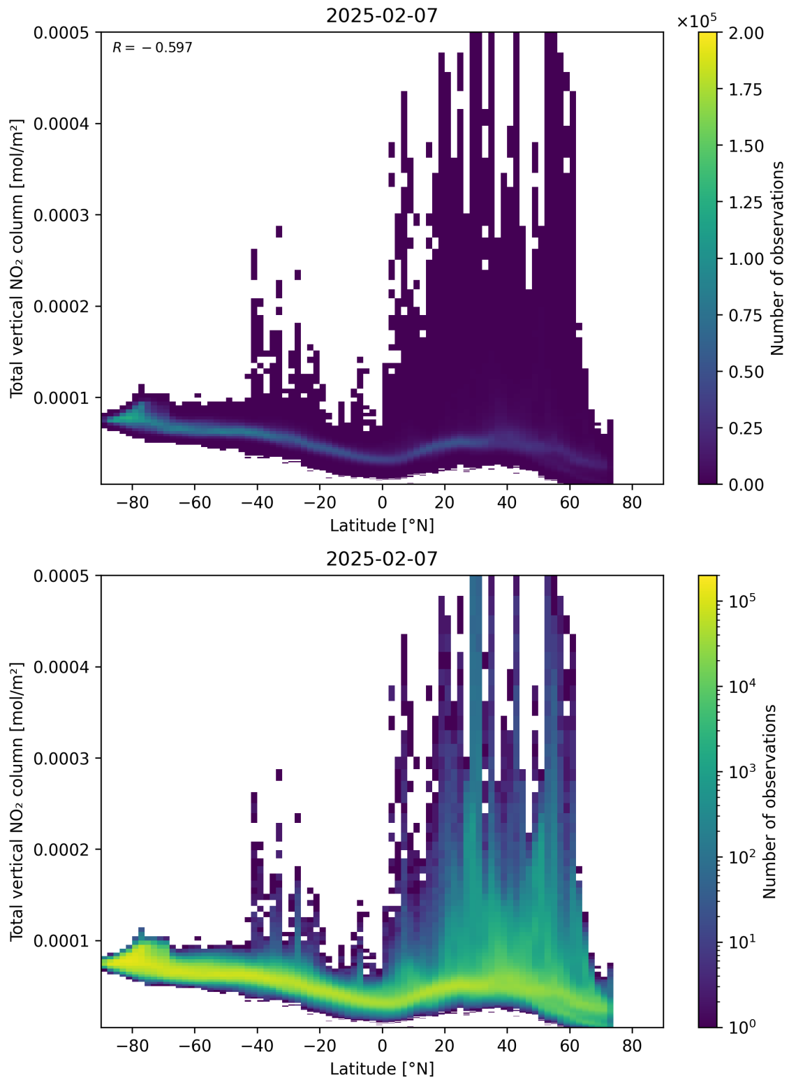
Figure 90: Scatter density plot of “Latitude” against “Total vertical NO 2 column” for 2025-02-06 to 2025-02-08.
