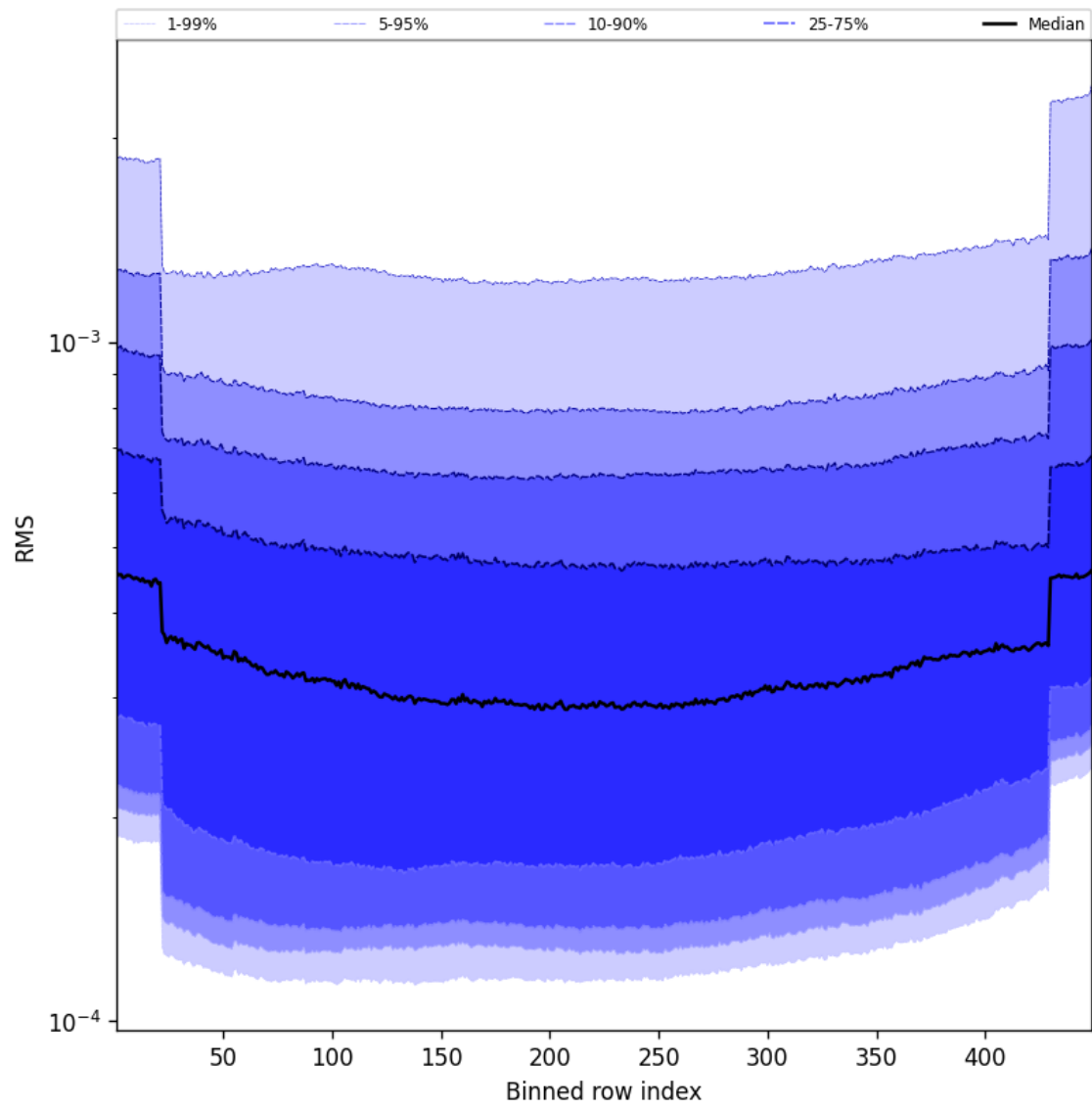
Figure 60: Along track statistics of “RMS” for 2025-02-06 to 2025-02-08
