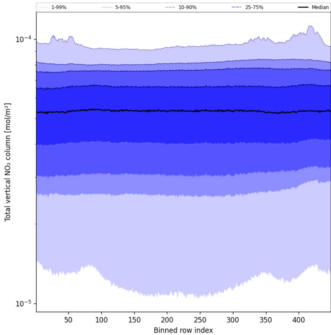
Figure 55: Along track statistics of “Total vertical NO 2 column” for 2025-02-06 to 2025-02-08
