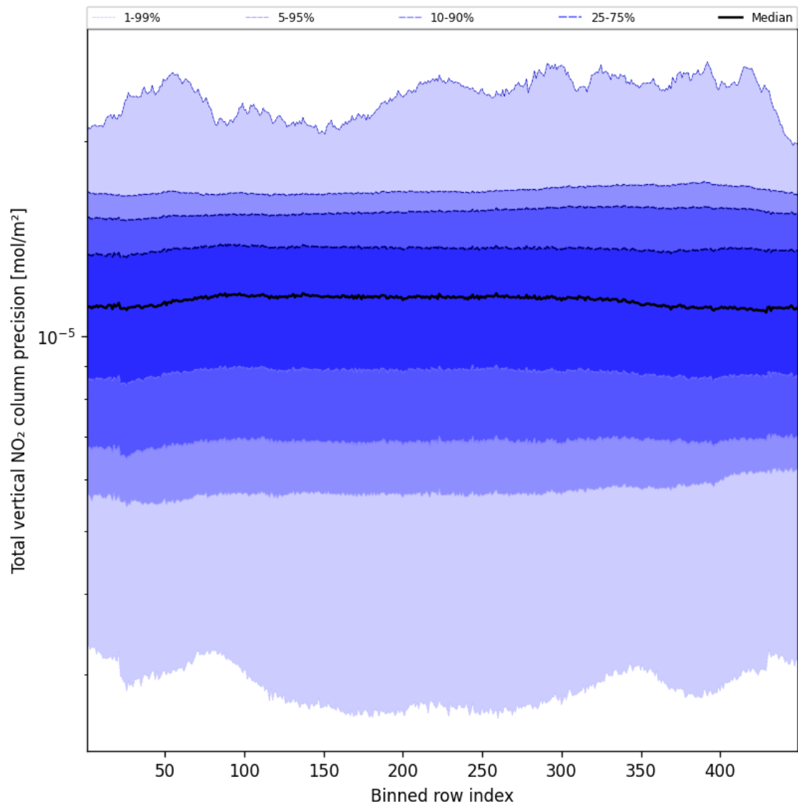
Figure 56: Along track statistics of “Total vertical NO 2 column precision” for 2025-02-06 to 2025-02-08
