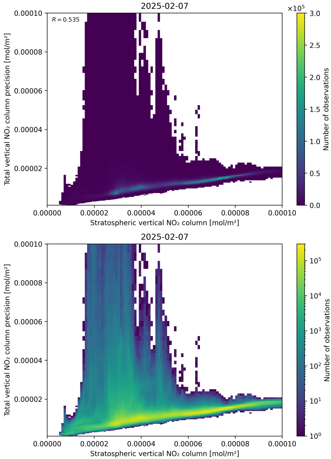
Figure 101: Scatter density plot of “Stratospheric vertical NO 2 column” against “Total vertical NO 2 column precision” for 2025-02-06 to 2025-02-08.
