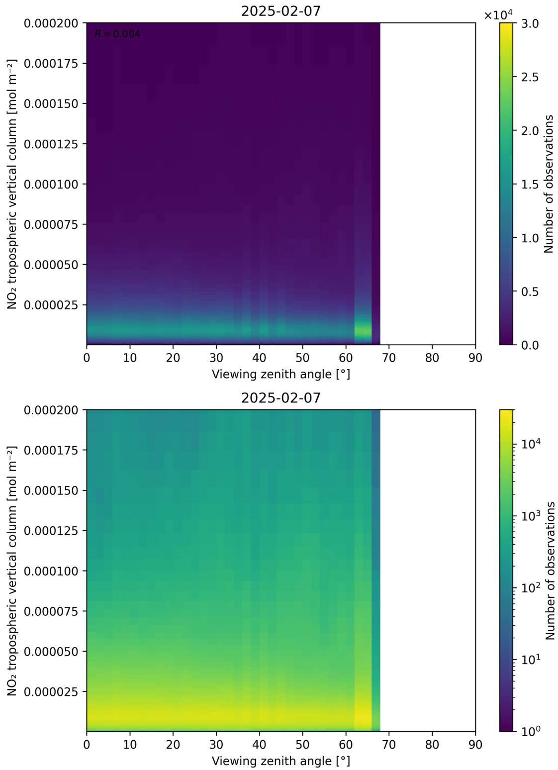
Figure 169: Scatter density plot of “Viewing zenith angle” against “NO 2 tropospheric vertical column” for 2025-02-06 to 2025-02-08.
