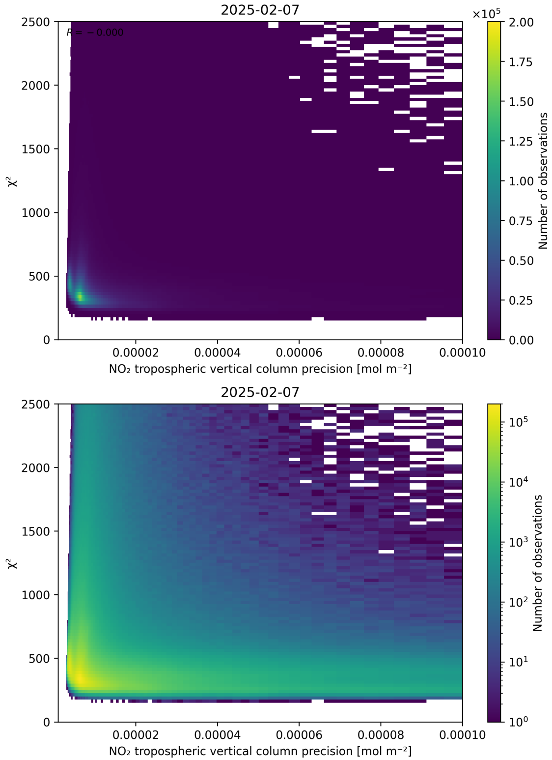
Figure 134: Scatter density plot of “NO 2 tropospheric vertical column precision” against “ \chi^2 ” for 2025-02-06 to 2025-02-08.
