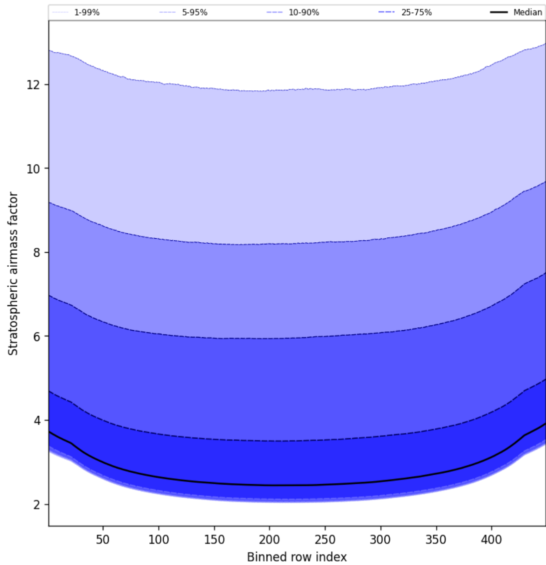
Figure 61: Along track statistics of “Stratospheric airmass factor” for 2025-02-06 to 2025-02-08
