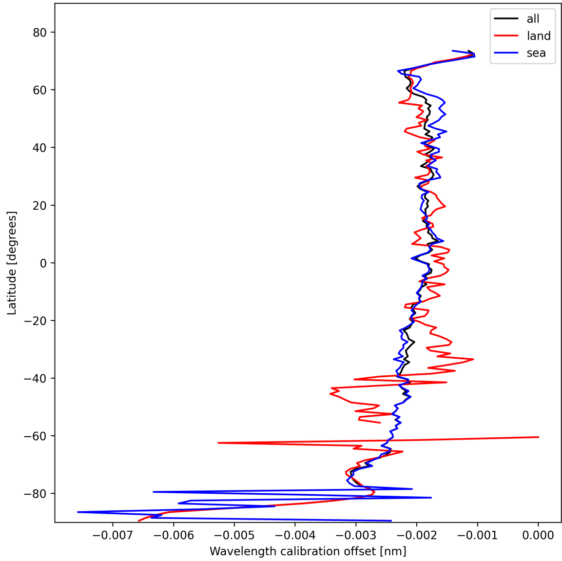
Figure 18: Zonal average of “Wavelength calibration offset” for 2025-02-06 to 2025-02-08.
