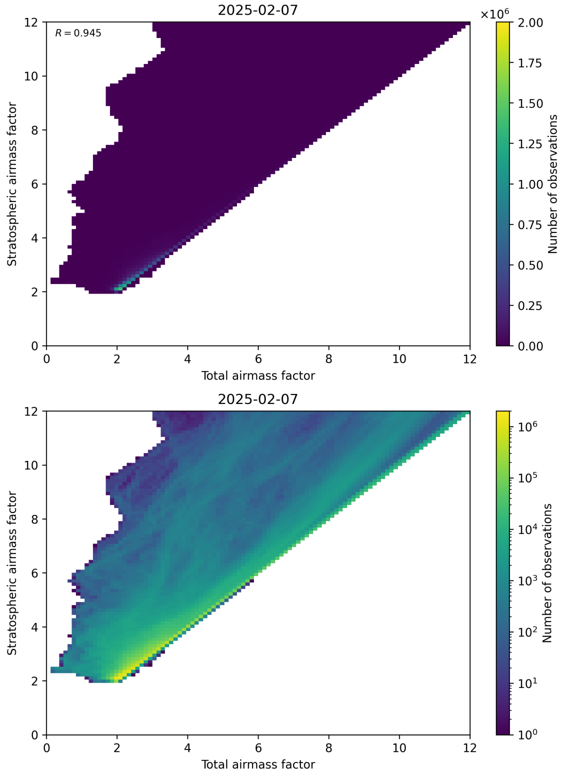
Figure 62: Scatter density plot of “Total airmass factor” against “Stratospheric airmass factor” for 2025-02-06 to 2025-02-08.
