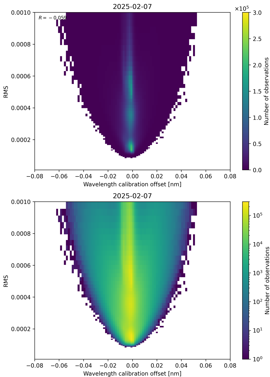
Figure 181: Scatter density plot of “Wavelength calibration offset” against “RMS” for 2025-02-06 to 2025-02-08.
