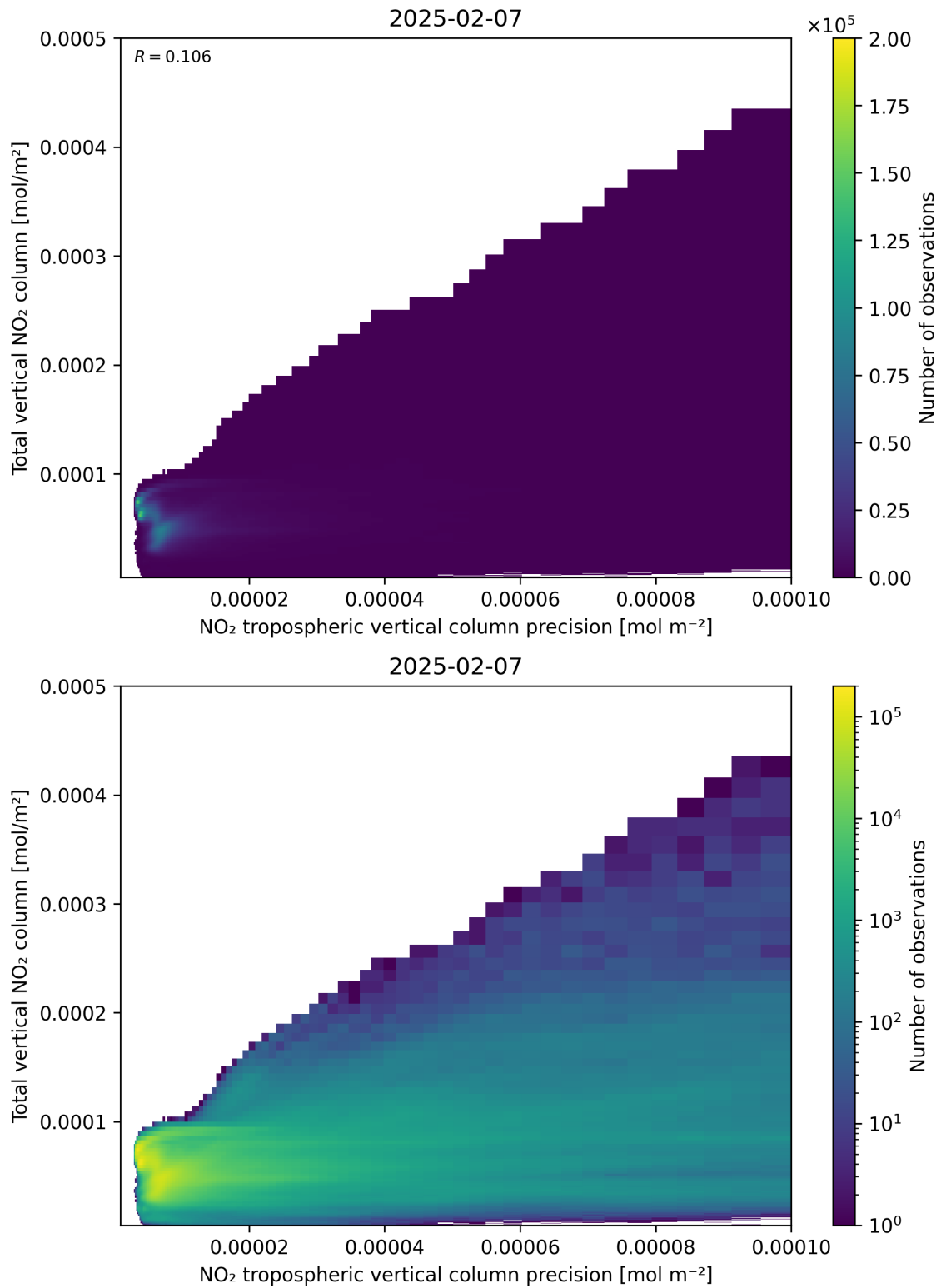
Figure 138: Scatter density plot of “NO 2 tropospheric vertical column precision” against “Total vertical NO 2 column” for 2025-02-06 to 2025-02-08.
