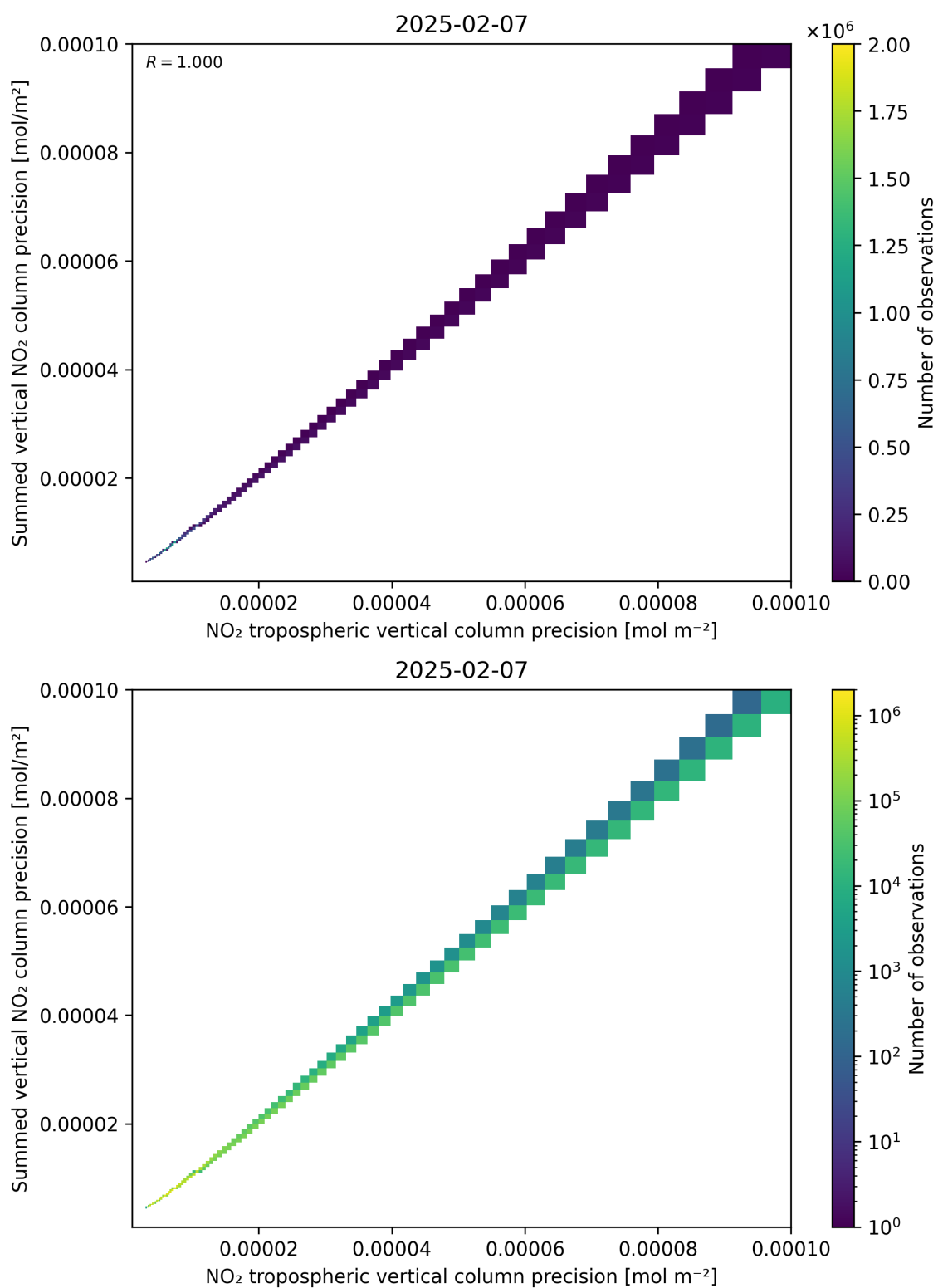
Figure 137: Scatter density plot of “NO 2 tropospheric vertical column precision” against “Summed vertical NO 2 column precision” for 2025-02-06 to 2025-02-08.
