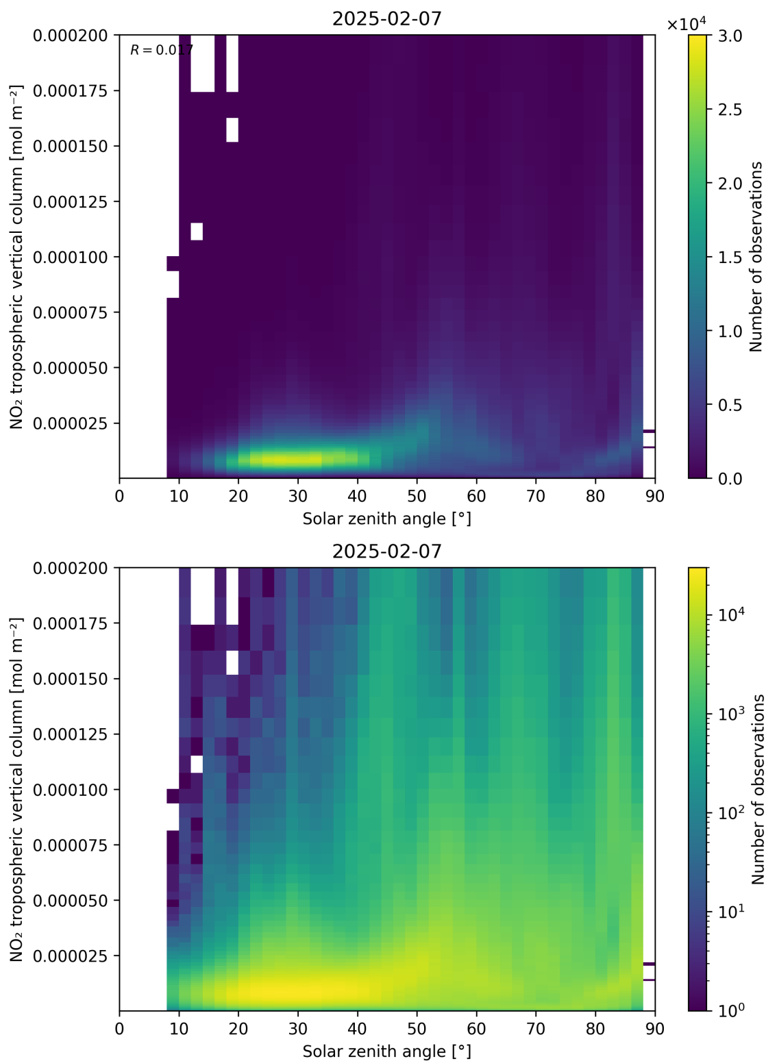
Figure 155: Scatter density plot of “Solar zenith angle” against “NO 2 tropospheric vertical column” for 2025-02-06 to 2025-02-08.
