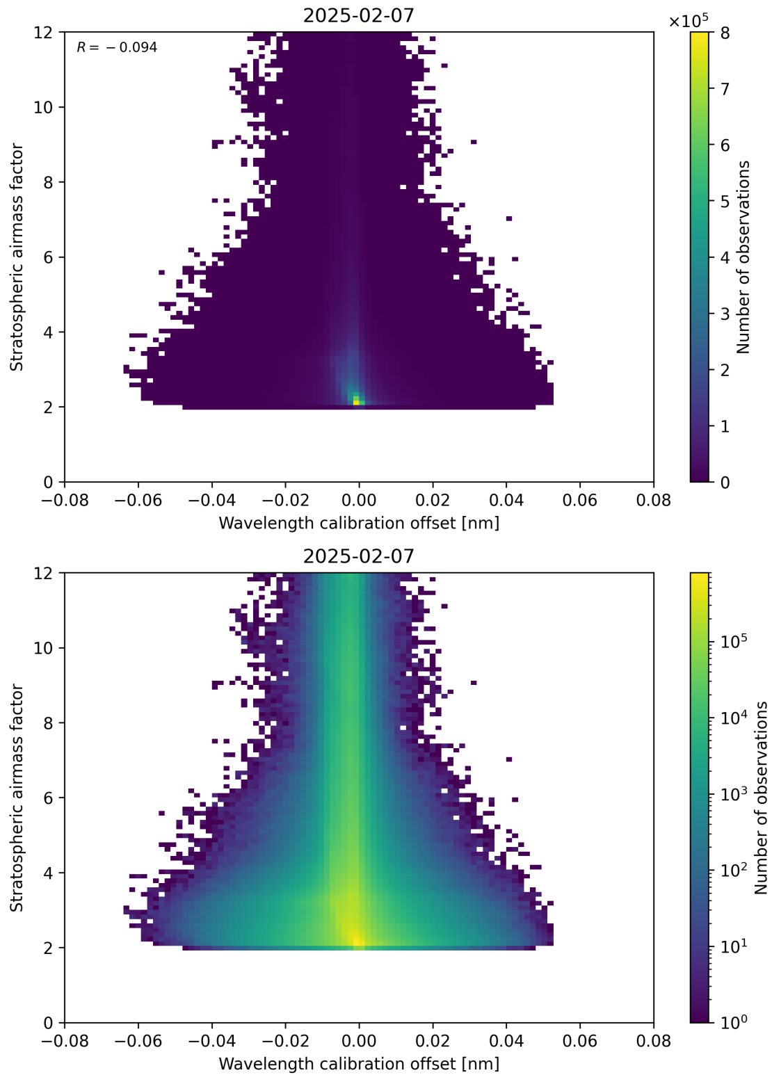
Figure 174: Scatter density plot of “Wavelength calibration offset” against “Stratospheric airmass factor” for 2025-02-06 to 2025-02-08.
