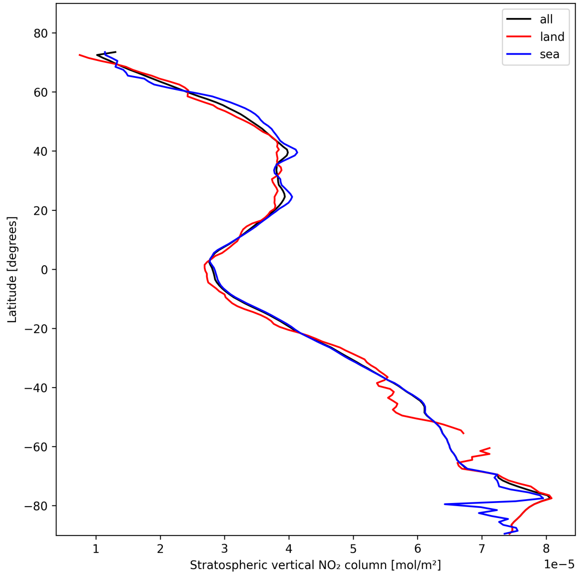
Figure 19: Zonal average of “Stratospheric vertical NO 2 column” for 2025-02-06 to 2025-02-08.
