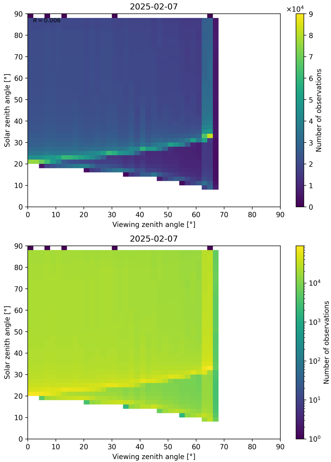
Figure 172: Scatter density plot of “Viewing zenith angle” against “Solar zenith angle” for 2025-02-06 to 2025-02-08.
