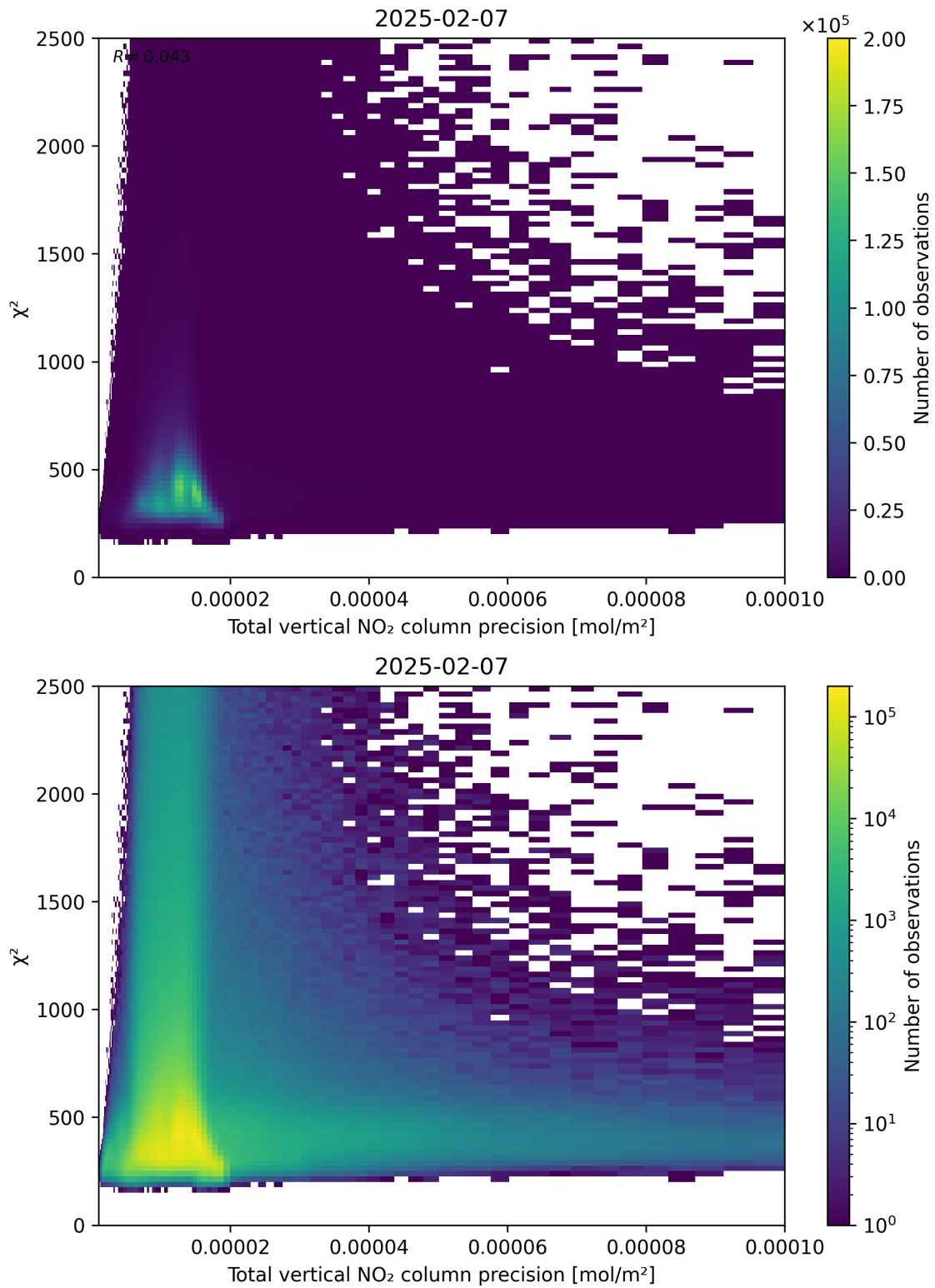
Figure 116: Scatter density plot of “Total vertical NO 2 column precision” against “ \chi^2 ” for 2025-02-06 to 2025-02-08.
