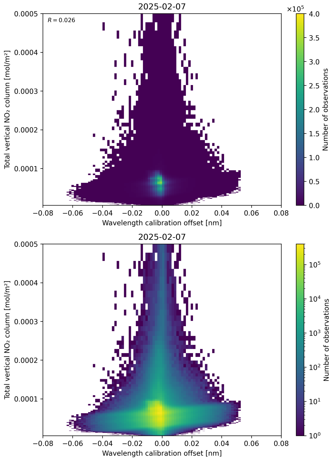
Figure 179: Scatter density plot of “Wavelength calibration offset” against “Total vertical NO 2 column” for 2025-02-06 to 2025-02-08.
