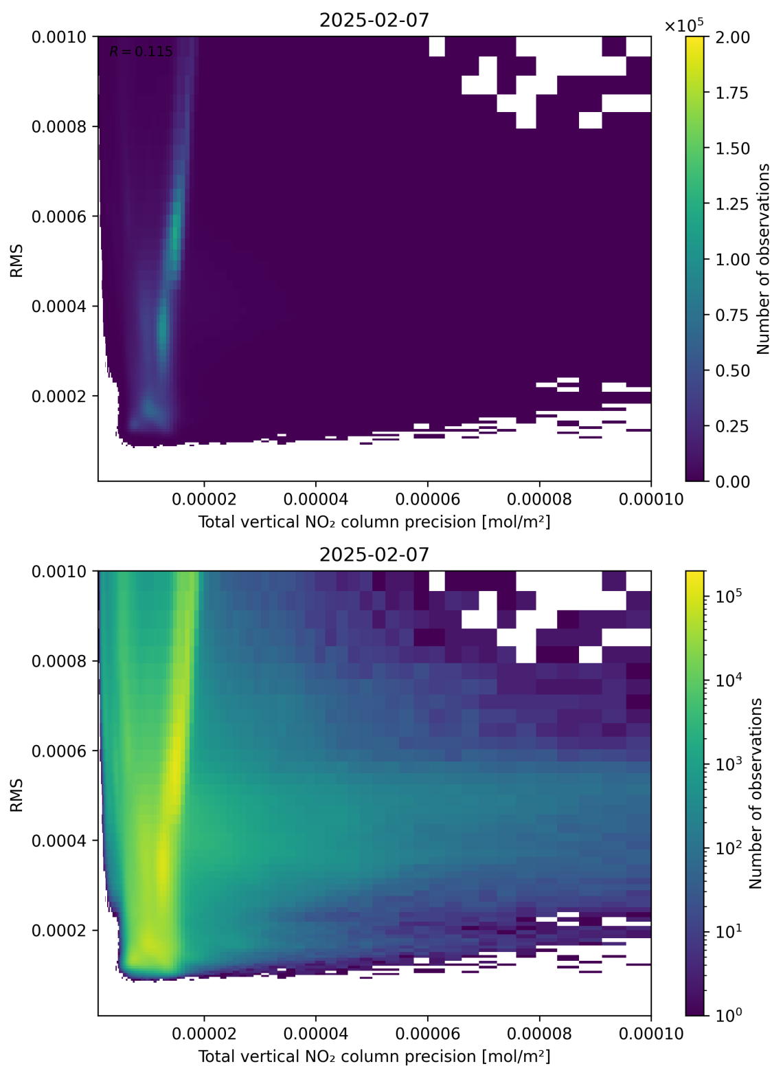
Figure 119: Scatter density plot of “Total vertical NO 2 column precision” against “RMS” for 2025-02-06 to 2025-02-08.
