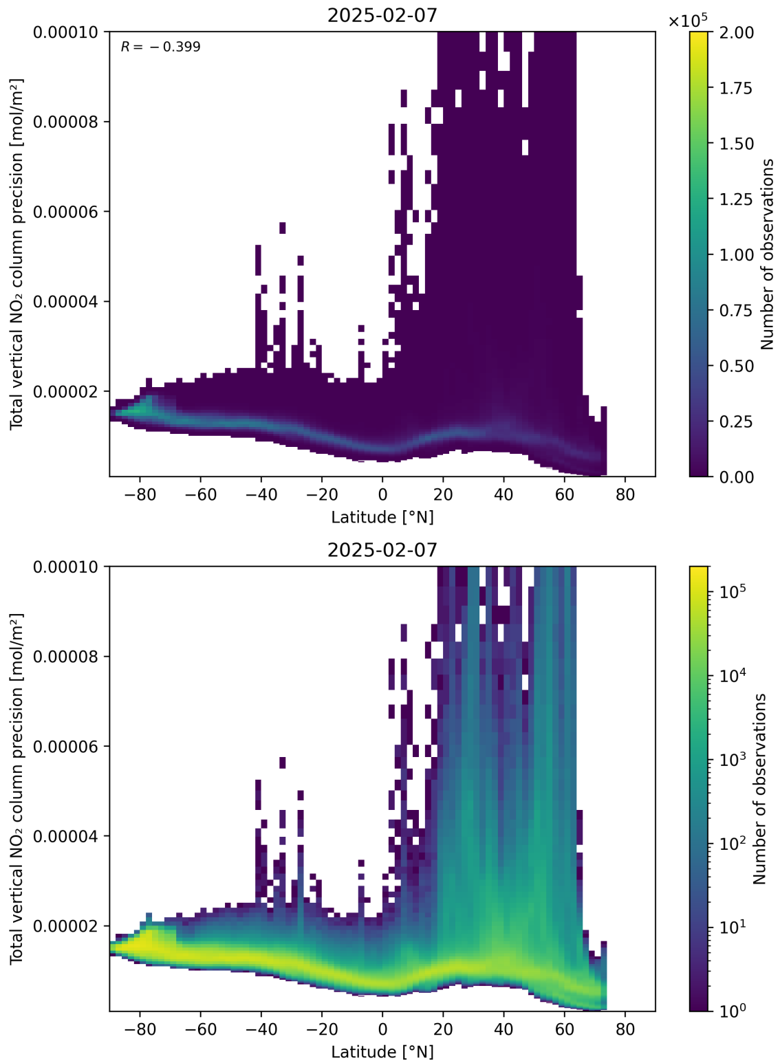
Figure 91: Scatter density plot of “Latitude” against “Total vertical NO 2 column precision” for 2025-02-06 to 2025-02-08.
