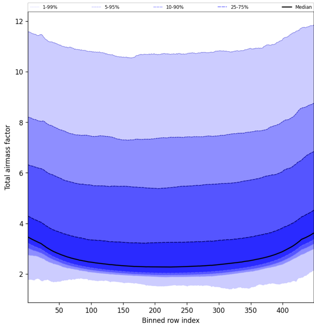
Figure 49: Along track statistics of “Total airmass factor” for 2025-02-06 to 2025-02-08
