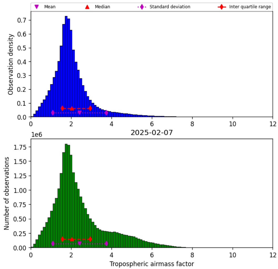
Figure 31: Histogram of “Tropospheric airmass factor” for 2025-02-06 to 2025-02-08
