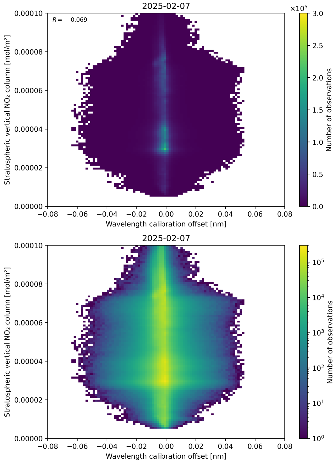
Figure 176: Scatter density plot of “Wavelength calibration offset” against “Stratospheric vertical NO 2 column” for 2025-02-06 to 2025-02-08.
