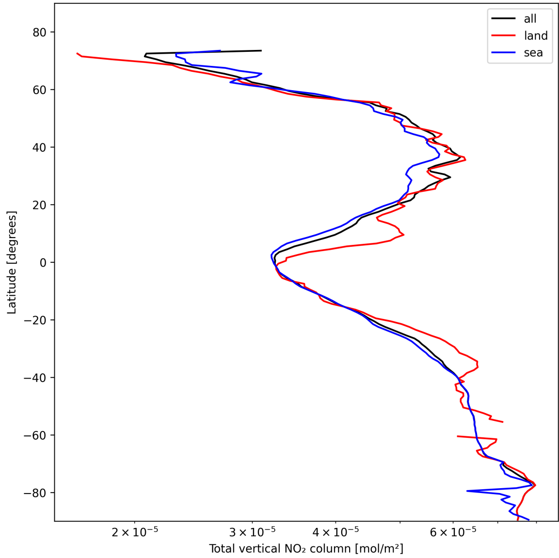
Figure 21: Zonal average of “Total vertical NO 2 column” for 2025-02-06 to 2025-02-08.
