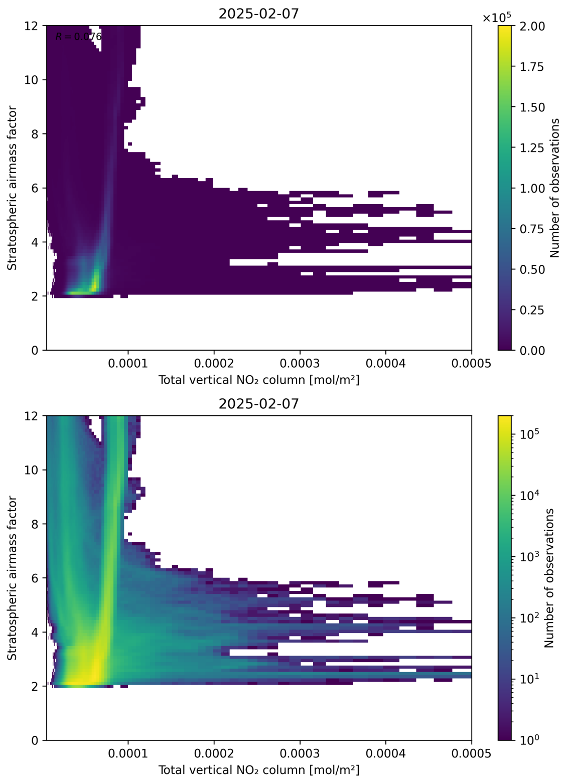
Figure 110: Scatter density plot of “Total vertical NO 2 column” against “Stratospheric airmass factor” for 2025-02-06 to 2025-02-08.
