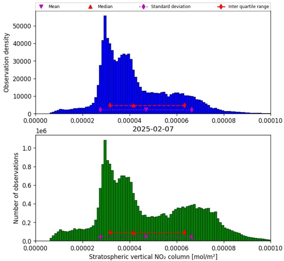
Figure 36: Histogram of “Stratospheric vertical NO 2 column” for 2025-02-06 to 2025-02-08
