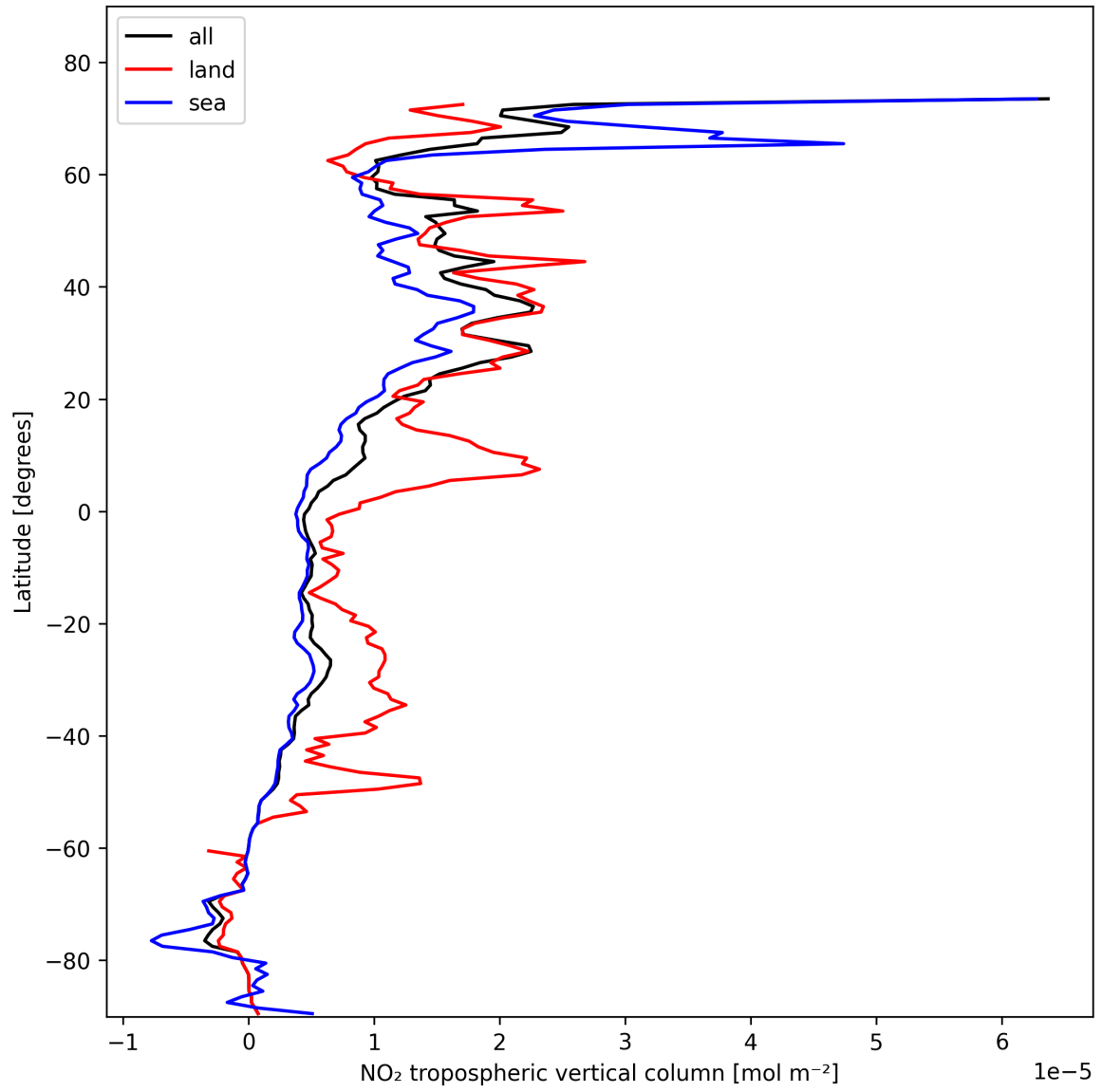
Figure 12: Zonal average of “NO 2 tropospheric vertical column” for 2025-02-06 to 2025-02-08.
