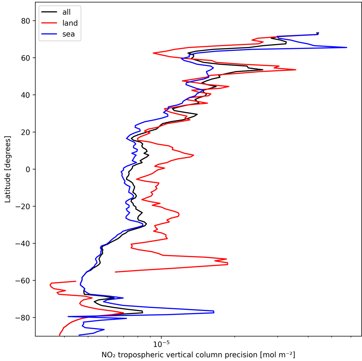
Figure 13: Zonal average of “NO 2 tropospheric vertical column precision” for 2025-02-06 to 2025-02-08.
