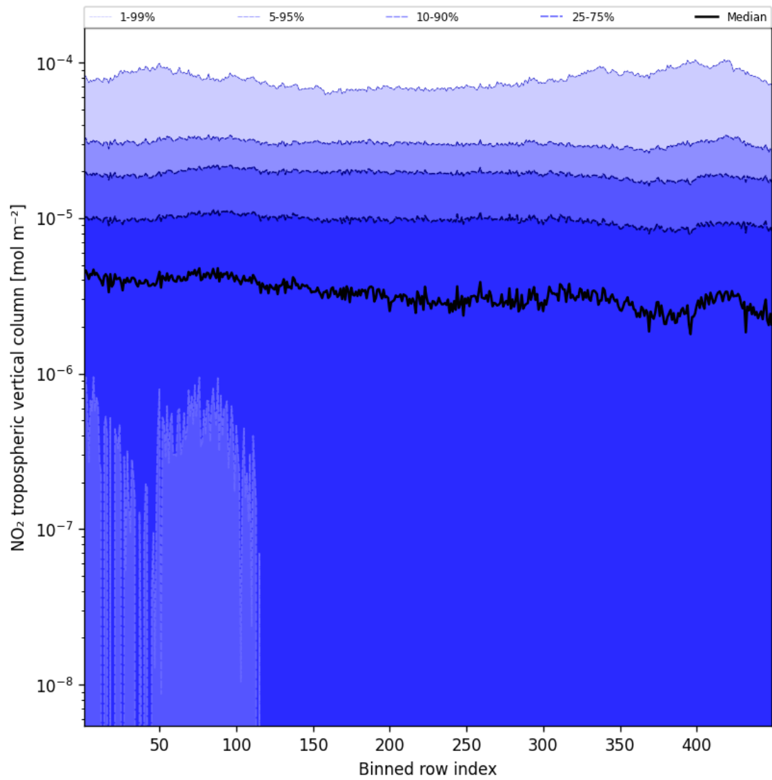
Figure 46: Along track statistics of “NO 2 tropospheric vertical column” for 2025-02-06 to 2025-02-08
