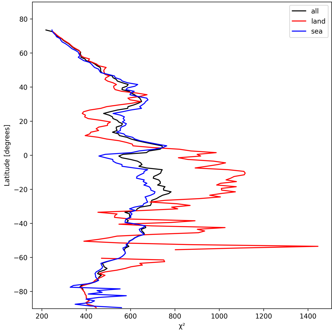
Figure 25: Zonal average of “ \chi^2 ” for 2025-02-06 to 2025-02-08.
