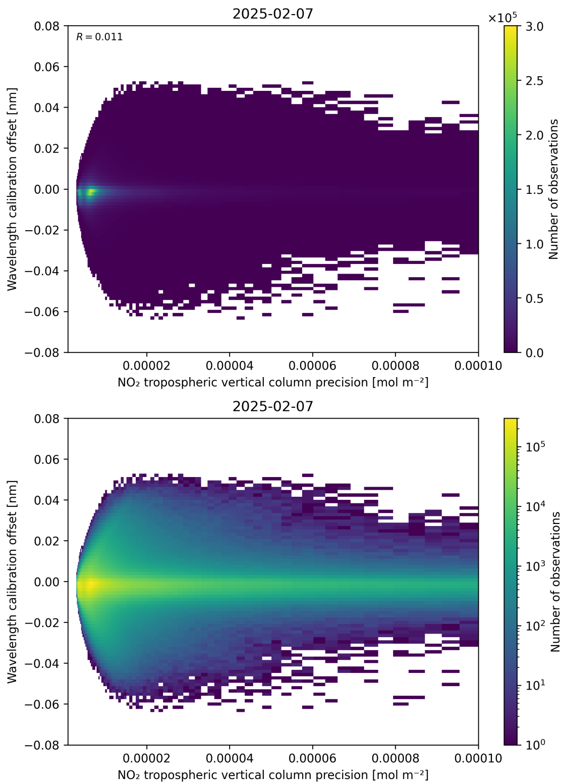
Figure 141: Scatter density plot of “NO 2 tropospheric vertical column precision” against “Wavelength calibration offset” for 2025-02-06 to 2025-02-08.
