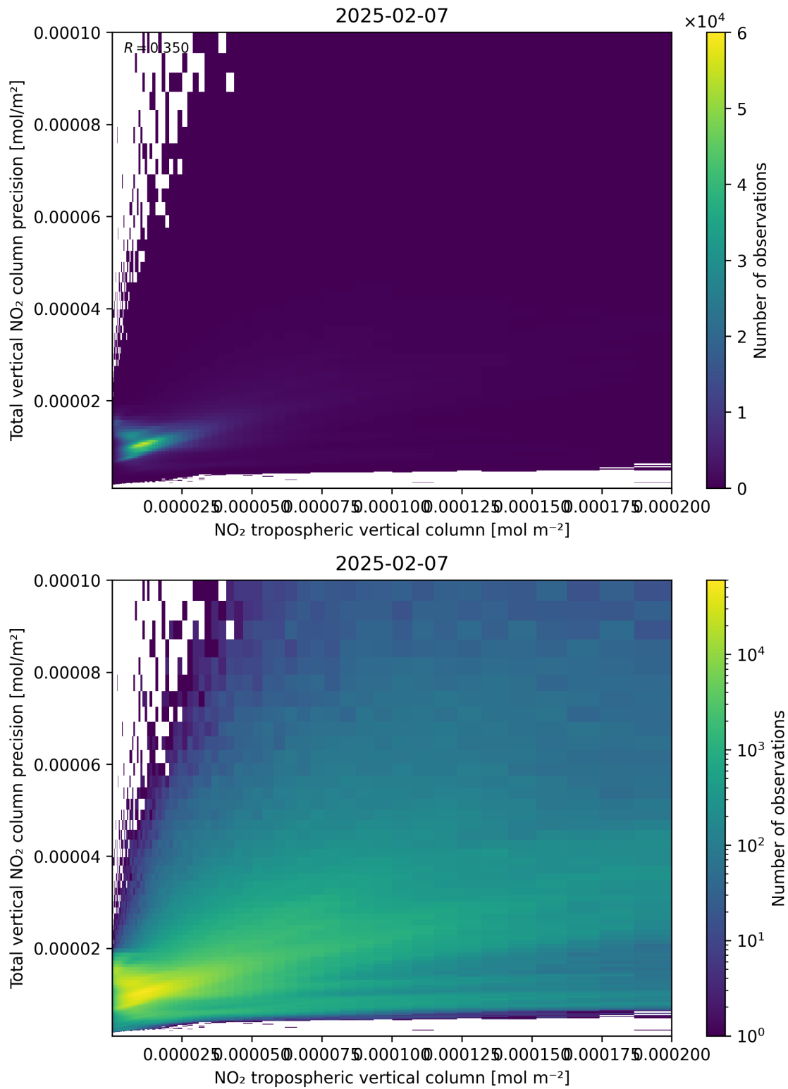
Figure 129: Scatter density plot of “NO 2 tropospheric vertical column” against “Total vertical NO 2 column precision” for 2025-02-06 to 2025-02-08.
