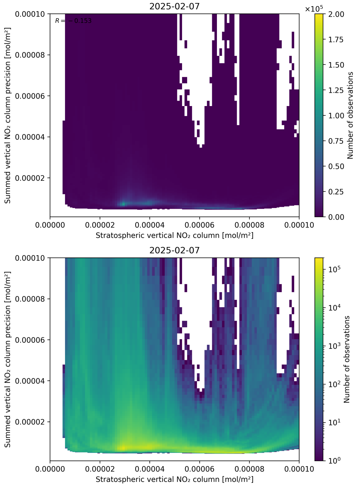
Figure 99: Scatter density plot of “Stratospheric vertical NO 2 column” against “Summed vertical NO 2 column precision” for 2025-02-06 to 2025-02-08.
