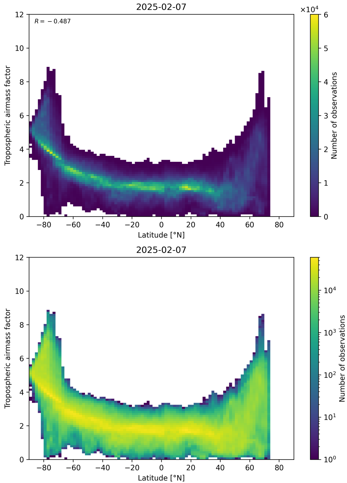
Figure 85: Scatter density plot of “Latitude” against “Tropospheric airmass factor” for 2025-02-06 to 2025-02-08.
