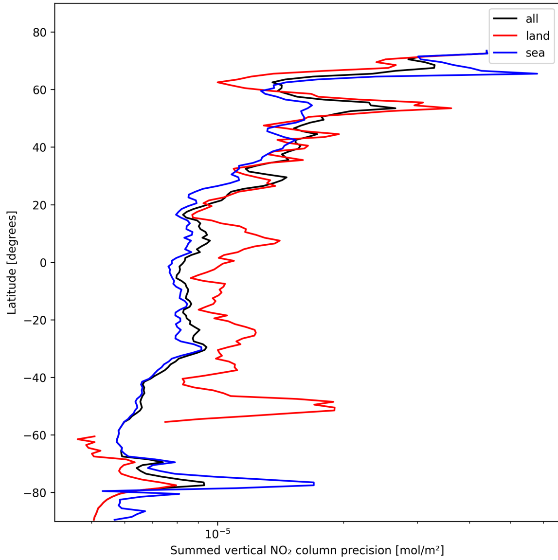
Figure 24: Zonal average of “Summed vertical NO 2 column precision” for 2025-02-06 to 2025-02-08.
