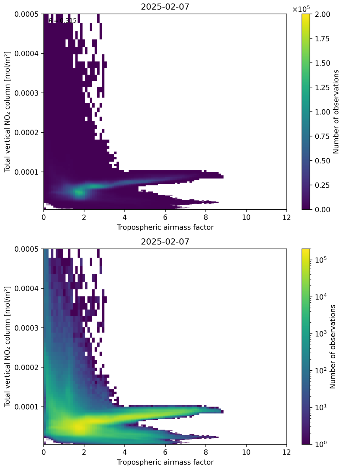
Figure 77: Scatter density plot of “Tropospheric airmass factor” against “Total vertical NO 2 column” for 2025-02-06 to 2025-02-08.
