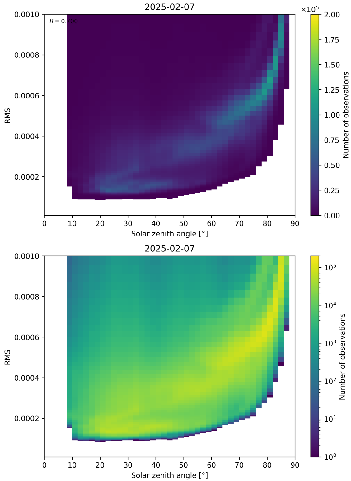
Figure 157: Scatter density plot of “Solar zenith angle” against “RMS” for 2025-02-06 to 2025-02-08.
