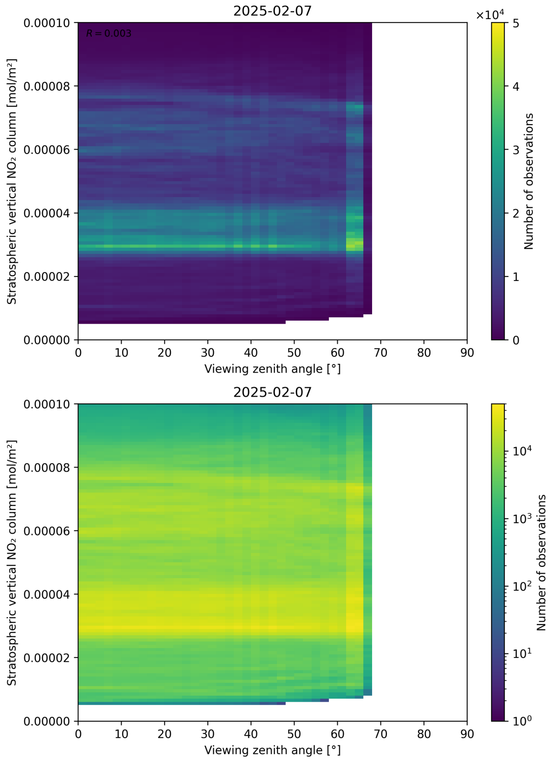
Figure 164: Scatter density plot of “Viewing zenith angle” against “Stratospheric vertical NO 2 column” for 2025-02-06 to 2025-02-08.
