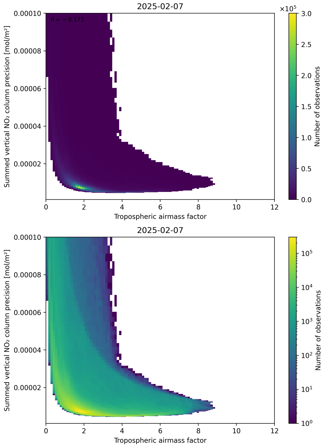
Figure 76: Scatter density plot of “Tropospheric air mass factor” against “Summed vertical NO 2 column precision” for 2025-02-06 to 2025-02-08.
