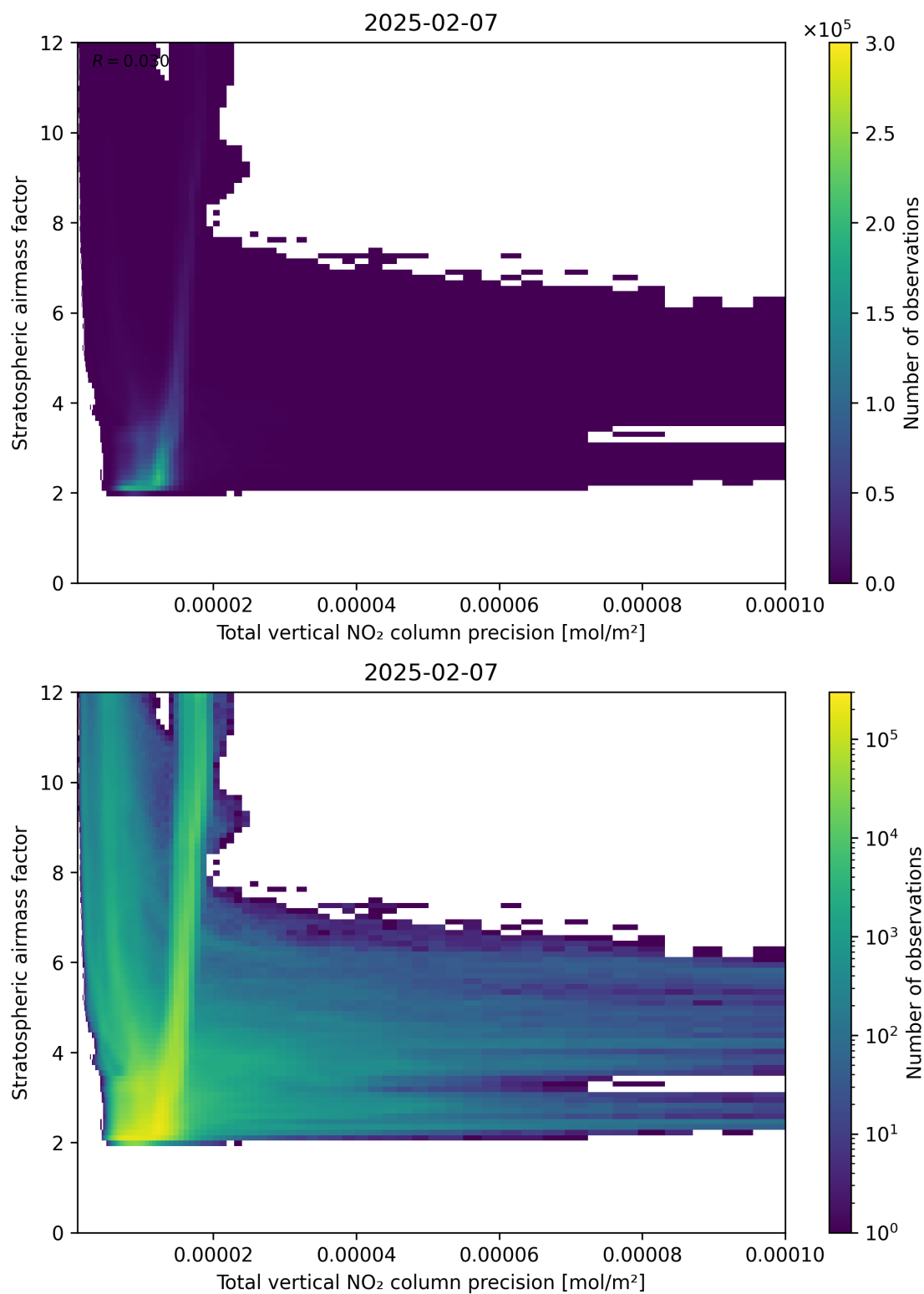
Figure 115: Scatter density plot of “Total vertical NO 2 column precision” against “Stratospheric air mass factor” for 2025-02-06 to 2025-02-08.
