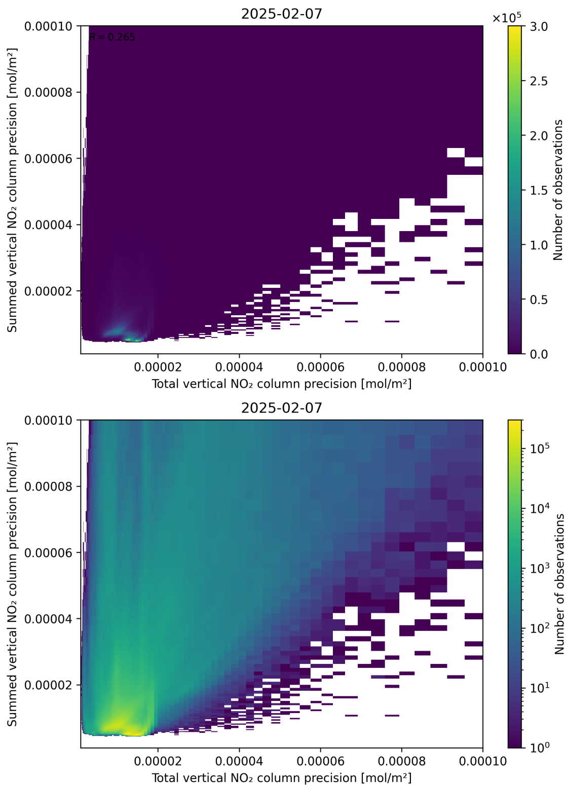
Figure 118: Scatter density plot of “Total vertical NO 2 column precision” against “Summed vertical NO 2 column precision” for 2025-02-06 to 2025-02-08.
