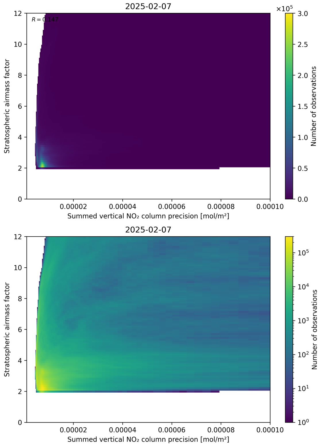
Figure 106: Scatter density plot of “Summed vertical NO 2 column precision” against “Stratospheric airmass factor” for 2025-02-06 to 2025-02-08.
