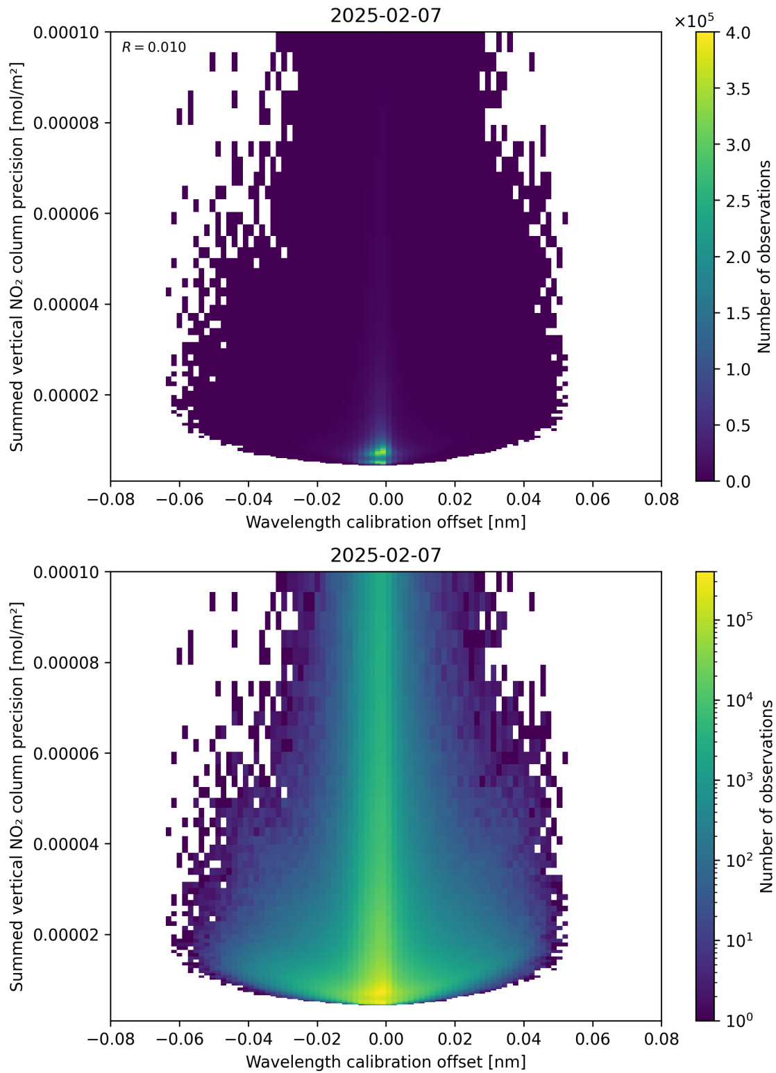
Figure 178: Scatter density plot of “Wavelength calibration offset” against “Summed vertical NO 2 column precision” for 2025-02-06 to 2025-02-08.
