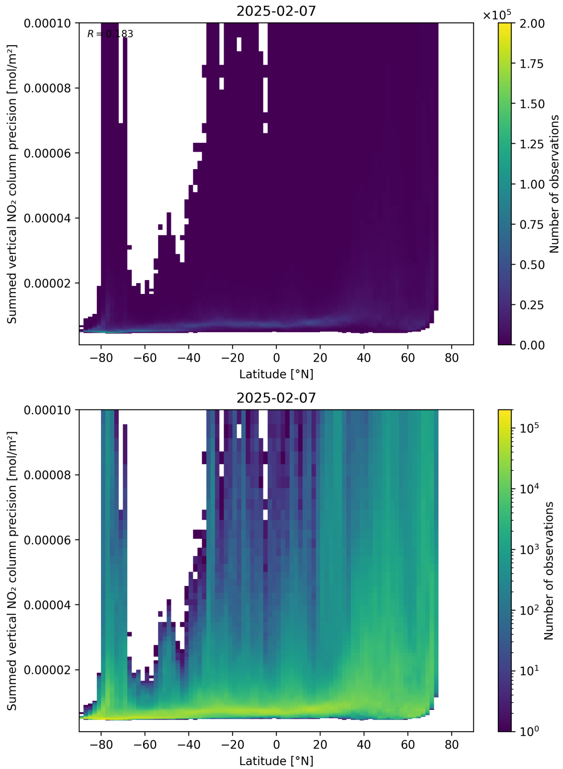
Figure 89: Scatter density plot of “Latitude” against “Summed vertical NO 2 column precision” for 2025-02-06 to 2025-02-08.
