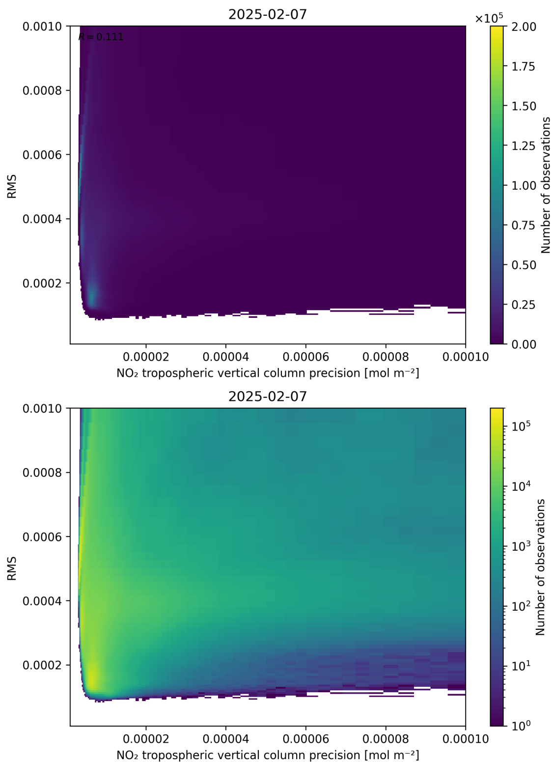
Figure 140: Scatter density plot of “NO 2 tropospheric vertical column precision” against “RMS” for 2025-02-06 to 2025-02-08.
