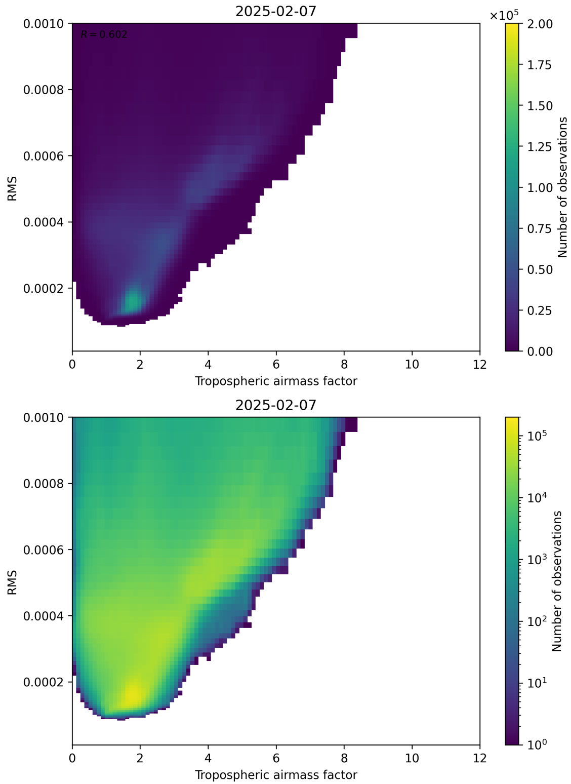
Figure 79: Scatter density plot of “Tropospheric airmass factor” against “RMS” for 2025-02-06 to 2025-02-08.
