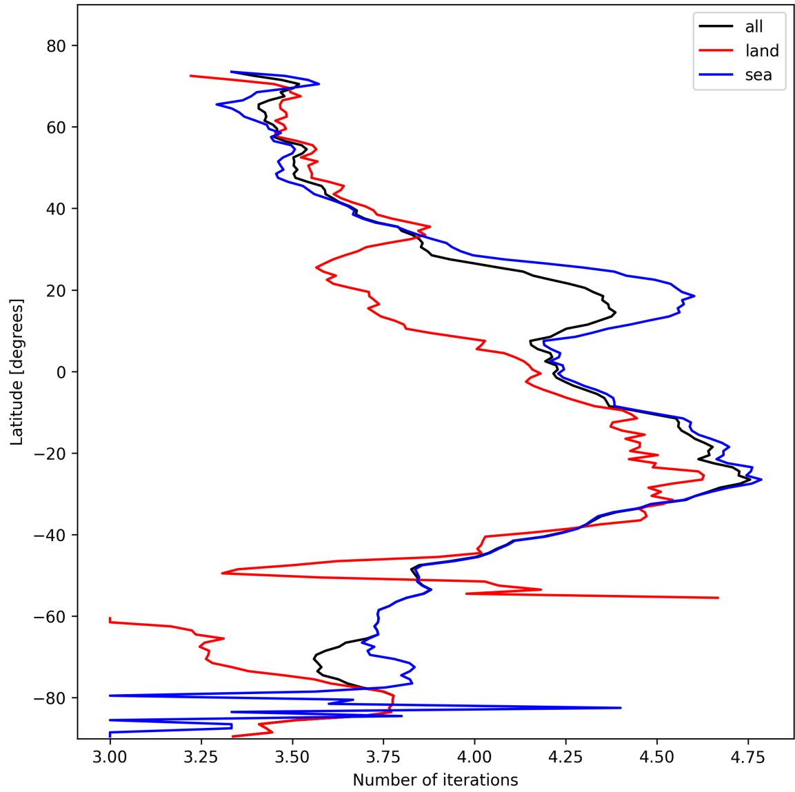
Figure 17: Zonal average of “Number of iterations” for 2025-02-06 to 2025-02-08.
