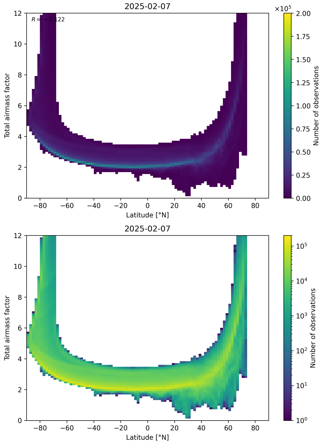
Figure 84: Scatter density plot of “Latitude” against “Total airmass factor” for 2025-02-06 to 2025-02-08.
