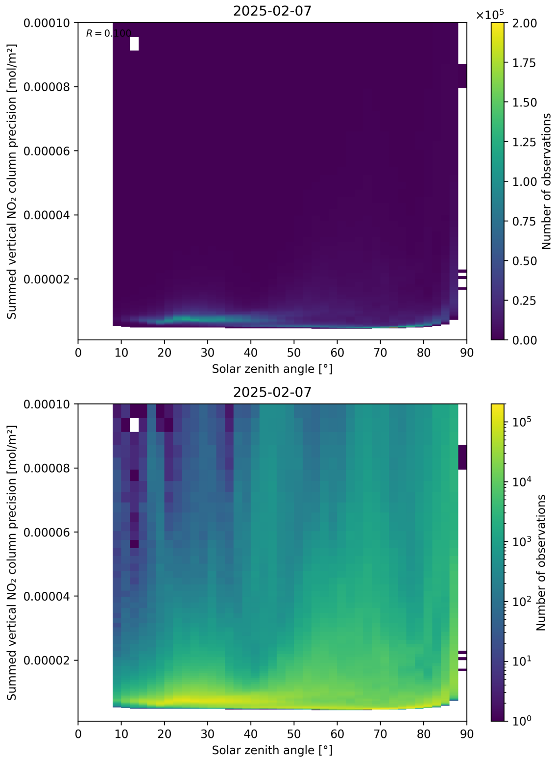
Figure 152: Scatter density plot of “Solar zenith angle” against “Summed vertical NO 2 column precision” for 2025-02-06 to 2025-02-08.
