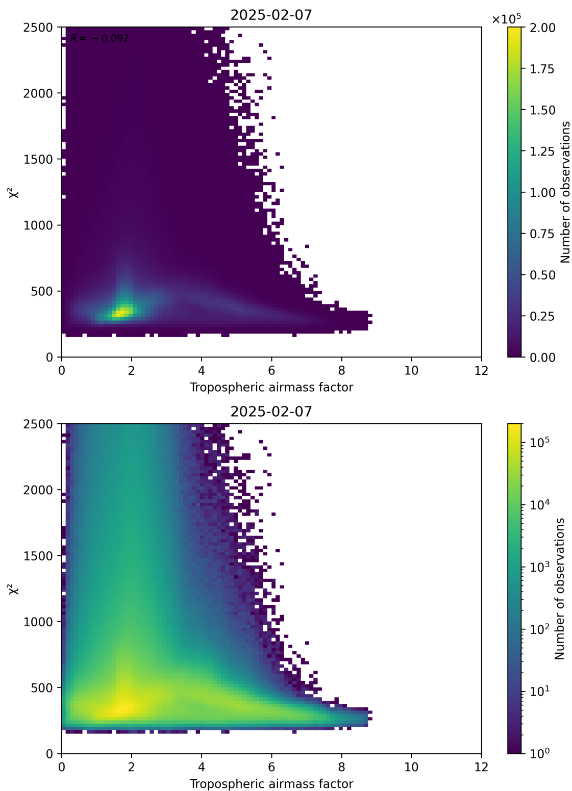
Figure 73: Scatter density plot of “Tropospheric airmass factor” against “ \chi^2 ” for 2025-02-06 to 2025-02-08.
