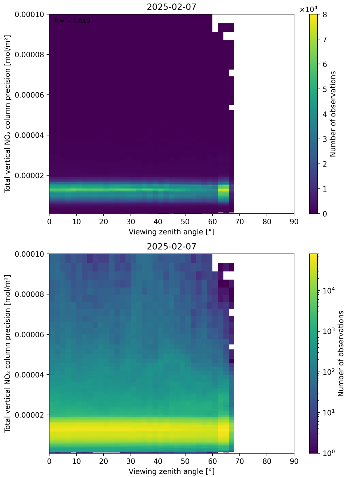
Figure 168: Scatter density plot of “Viewing zenith angle” against “Total vertical NO 2 column precision” for 2025-02-06 to 2025-02-08.
