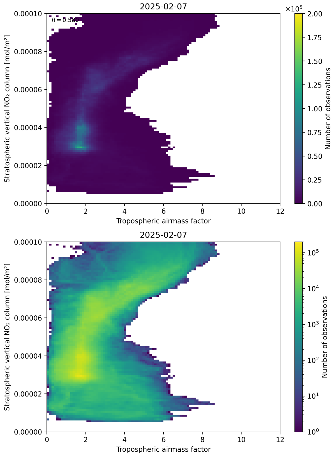
Figure 74: Scatter density plot of “Tropospheric airmass factor” against “Stratospheric vertical NO 2 column” for 2025-02-06 to 2025-02-08.
