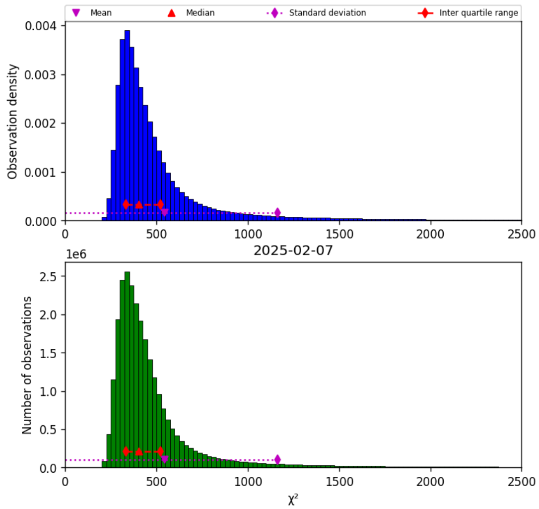
Figure 42: Histogram of “ \chi^2 ” for 2025-02-06 to 2025-02-08
