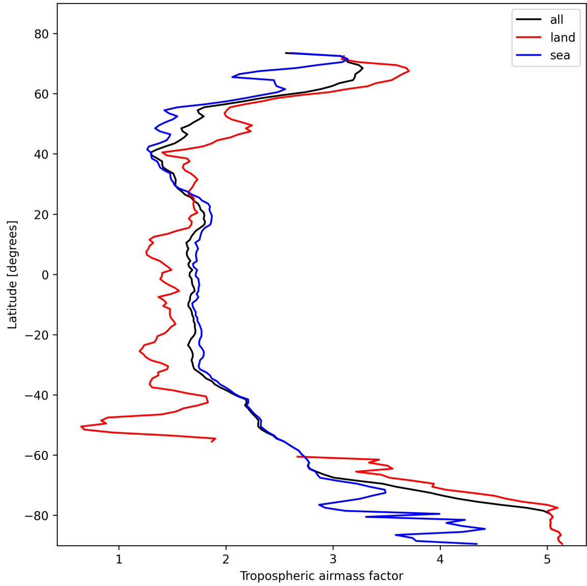
Figure 14: Zonal average of “Tropospheric airmass factor” for 2025-02-06 to 2025-02-08.
