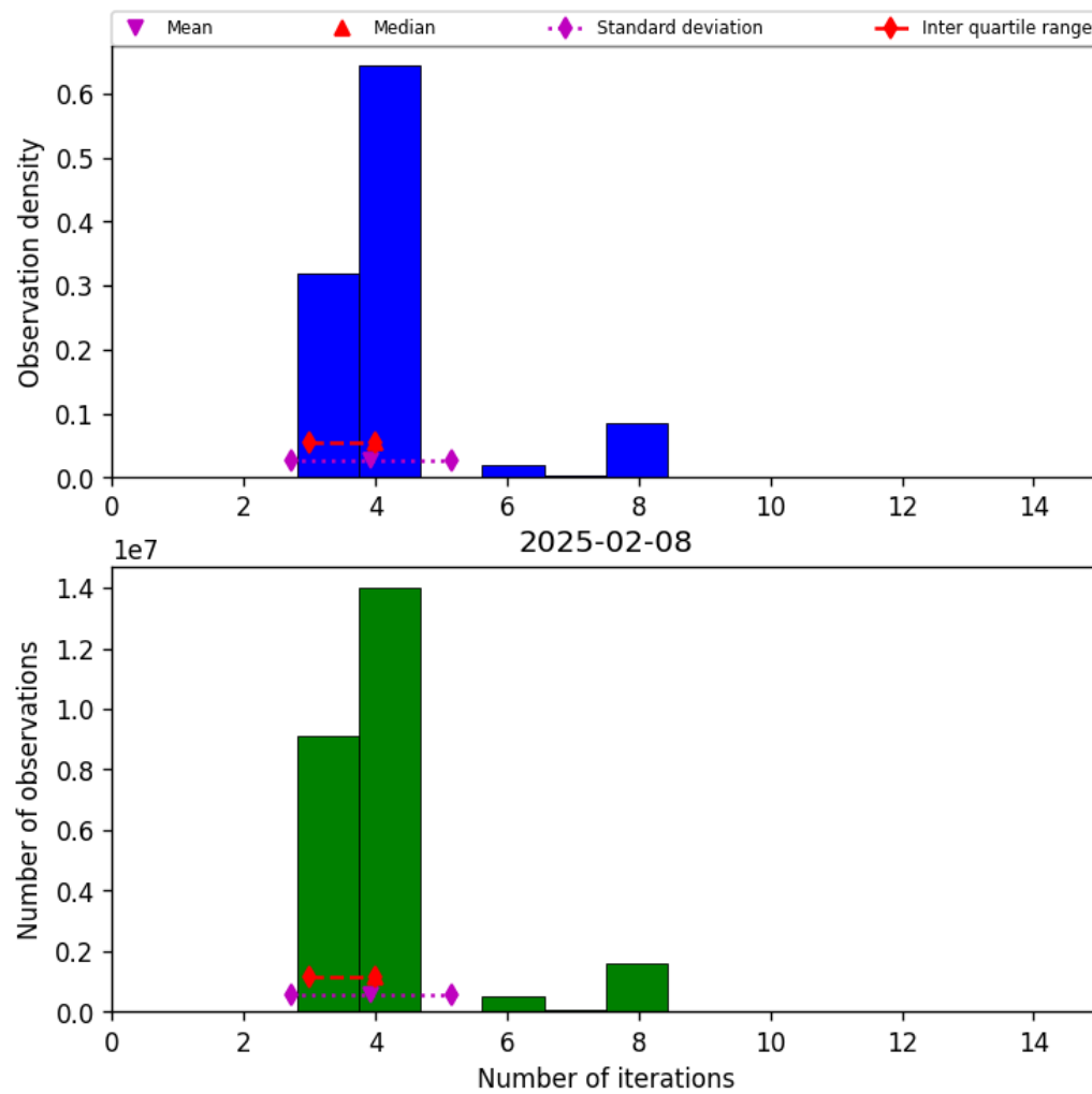
Figure 34: Histogram of “Number of iterations” for 2025-02-08 to 2025-02-09
