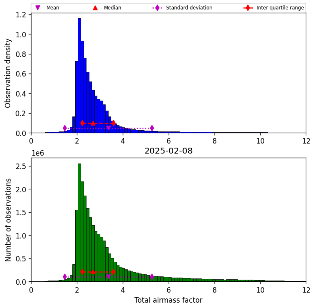
Figure 32: Histogram of “Total airmass factor” for 2025-02-08 to 2025-02-09
