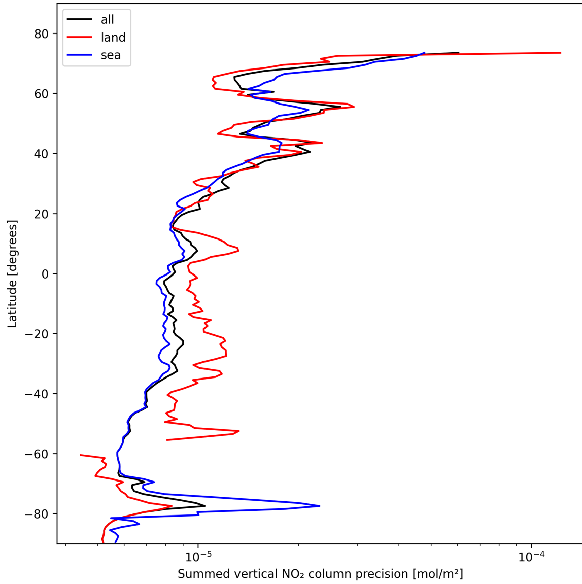
Figure 24: Zonal average of “Summed vertical NO 2 column precision” for 2025-02-08 to 2025-02-09.
