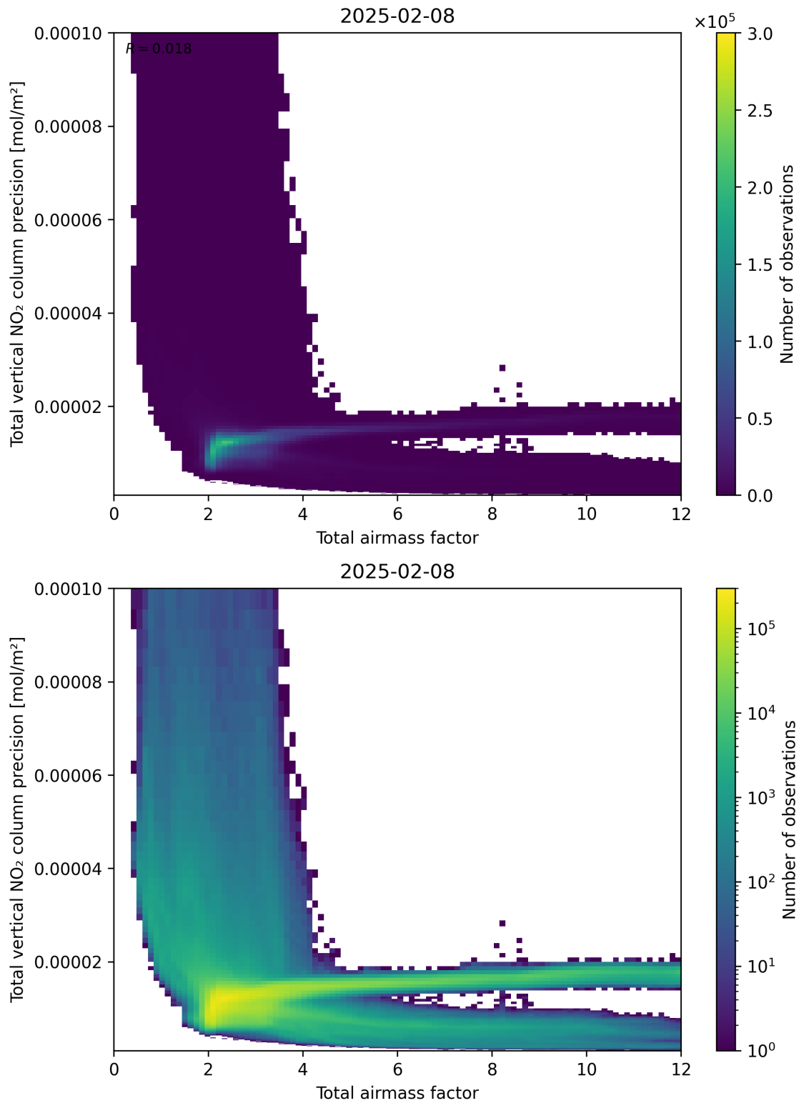
Figure 68: Scatter density plot of “Total airmass factor” against “Total vertical NO 2 column precision” for 2025-02-08 to 2025-02-09.
