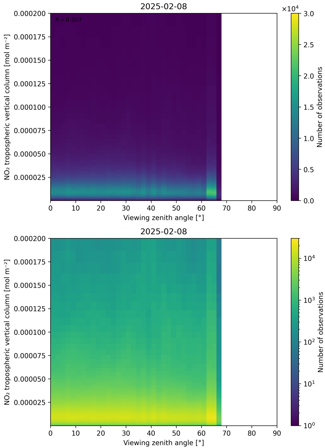
Figure 169: Scatter density plot of “Viewing zenith angle” against “NO 2 tropospheric vertical column” for 2025-02-08 to 2025-02-09.
