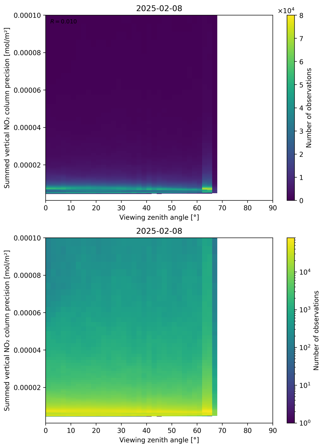
Figure 166: Scatter density plot of “Viewing zenith angle” against “Summed vertical NO 2 column precision” for 2025-02-08 to 2025-02-09.
