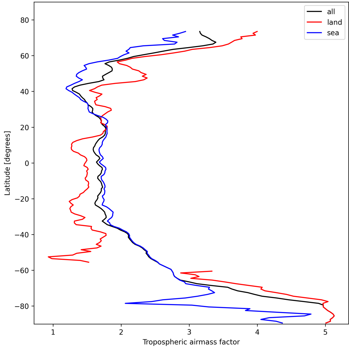
Figure 14: Zonal average of “Tropospheric airmass factor” for 2025-02-08 to 2025-02-09.
