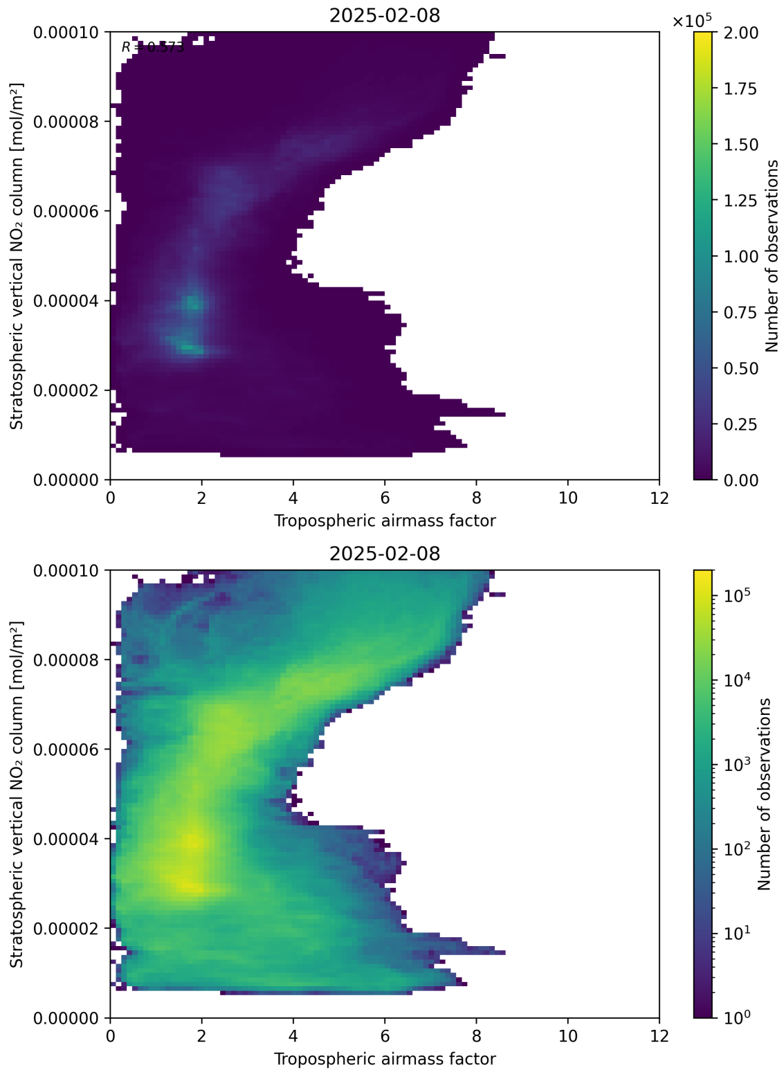
Figure 74: Scatter density plot of “Tropospheric air mass factor” against “Stratospheric vertical NO 2 column” for 2025-02-08 to 2025-02-09.
