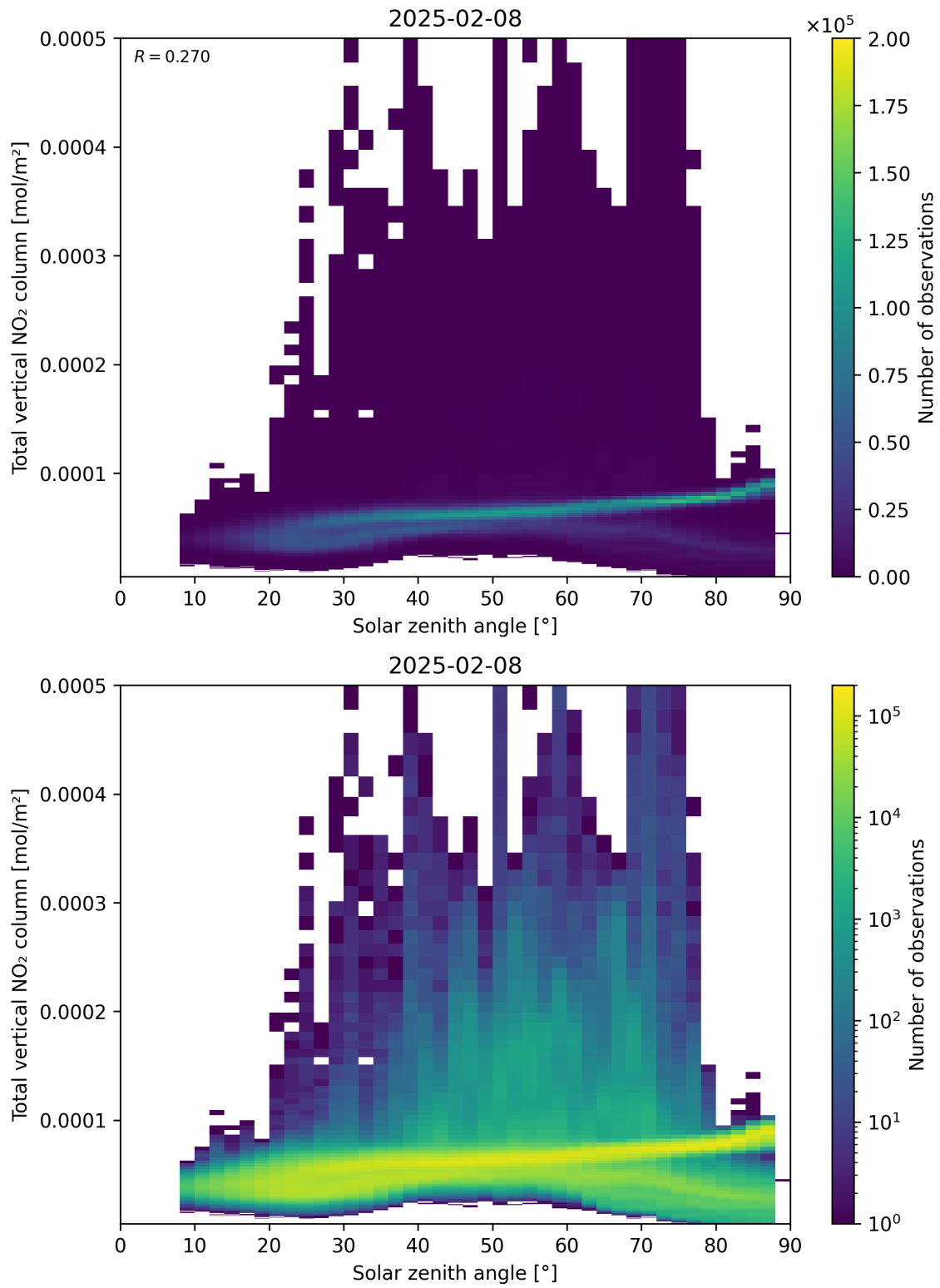
Figure 153: Scatter density plot of “Solar zenith angle” against “Total vertical NO 2 column” for 2025-02-08 to 2025-02-09.
