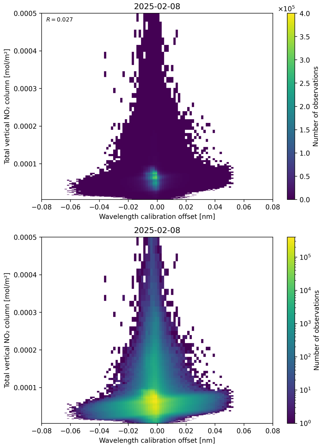
Figure 179: Scatter density plot of “Wavelength calibration offset” against “Total vertical NO 2 column” for 2025-02-08 to 2025-02-09.
