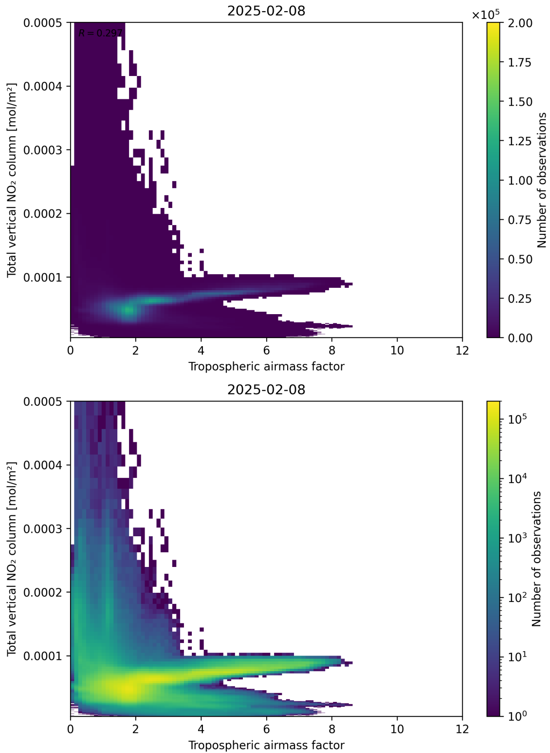
Figure 77: Scatter density plot of “Tropospheric airmass factor” against “Total vertical NO 2 column” for 2025-02-08 to 2025-02-09.
