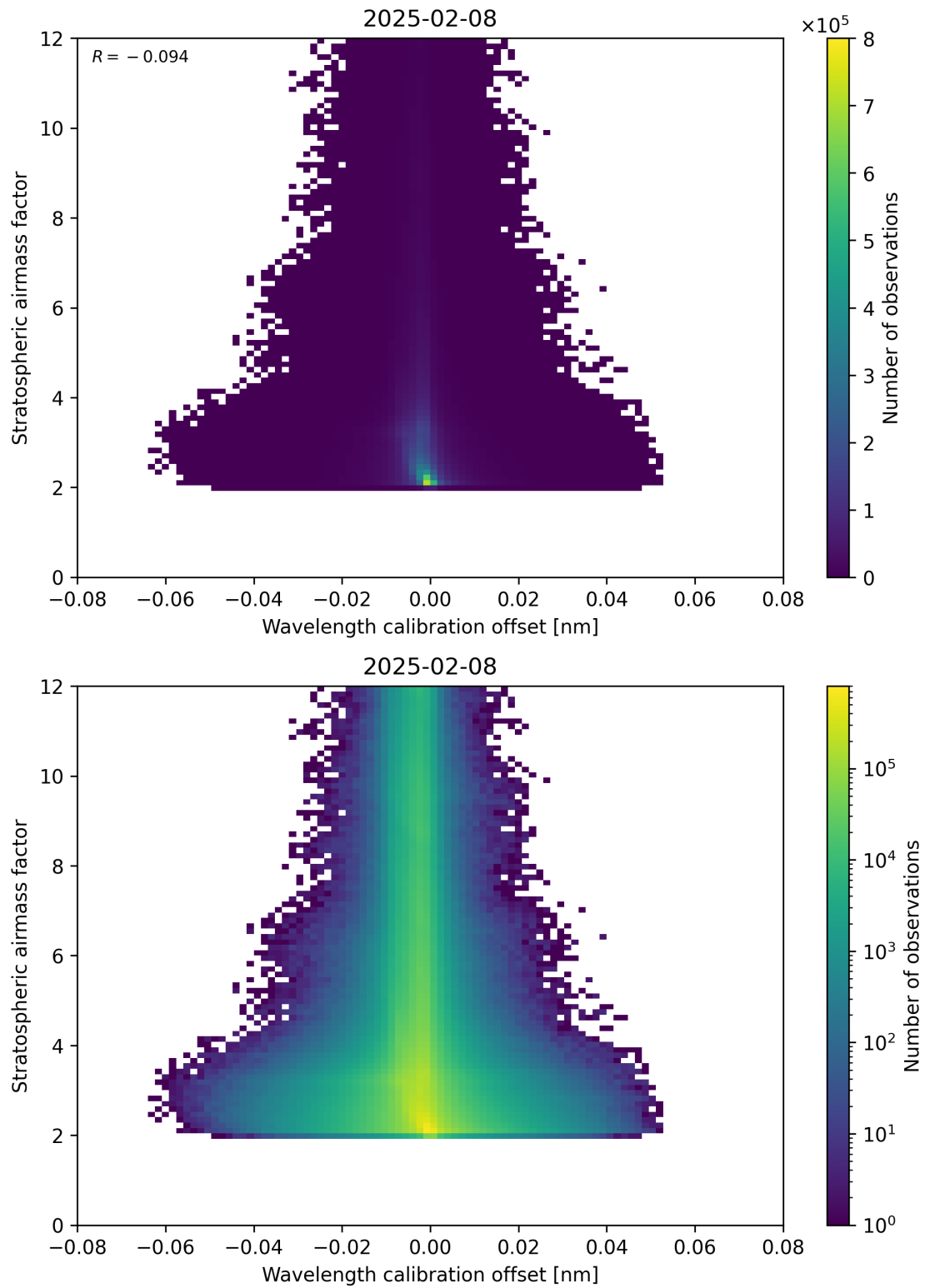
Figure 174: Scatter density plot of “Wavelength calibration offset” against “Stratospheric airmass factor” for 2025-02-08 to 2025-02-09.
