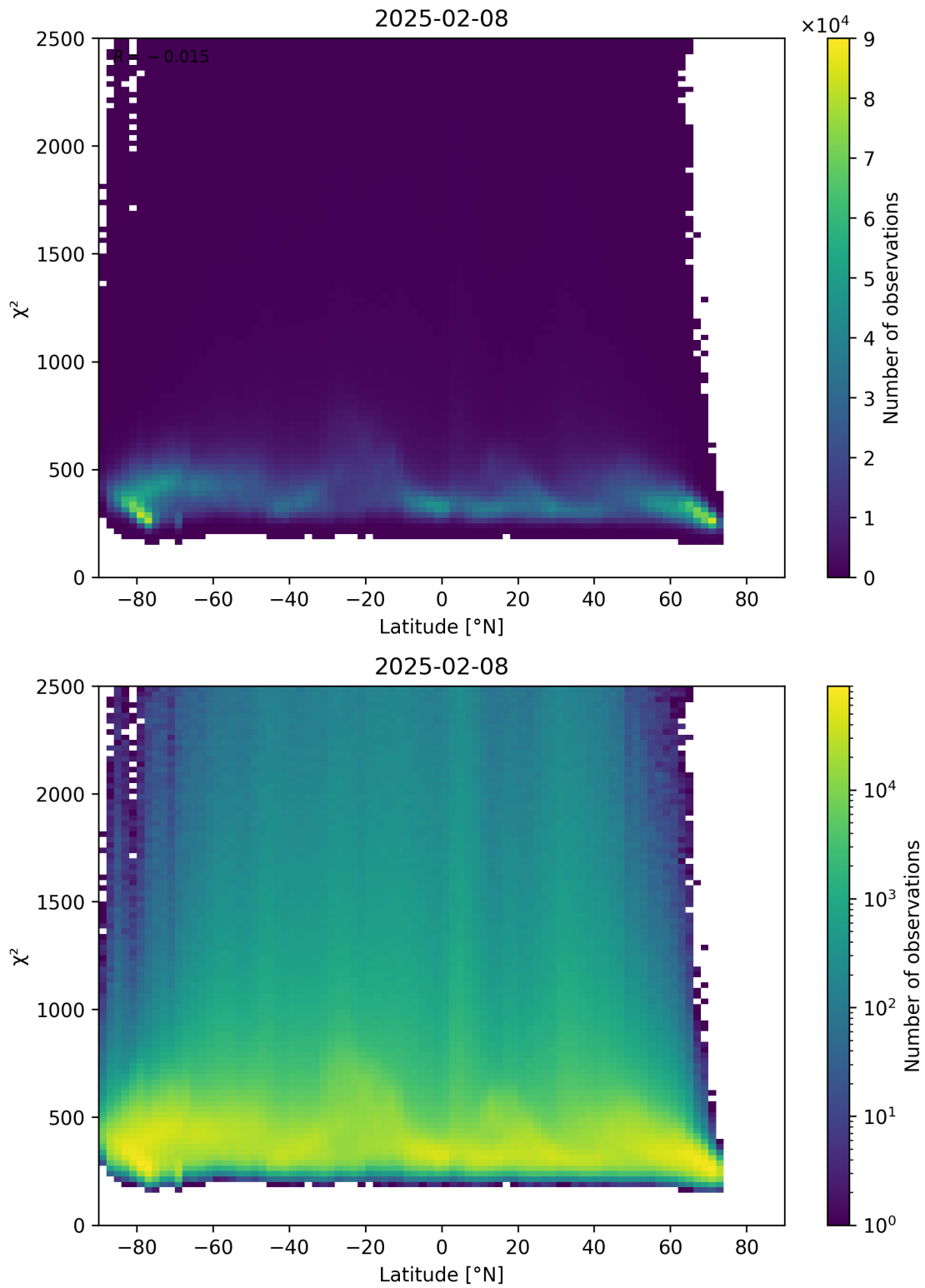
Figure 86: Scatter density plot of “Latitude” against “ \chi^2 ” for 2025-02-08 to 2025-02-09.
