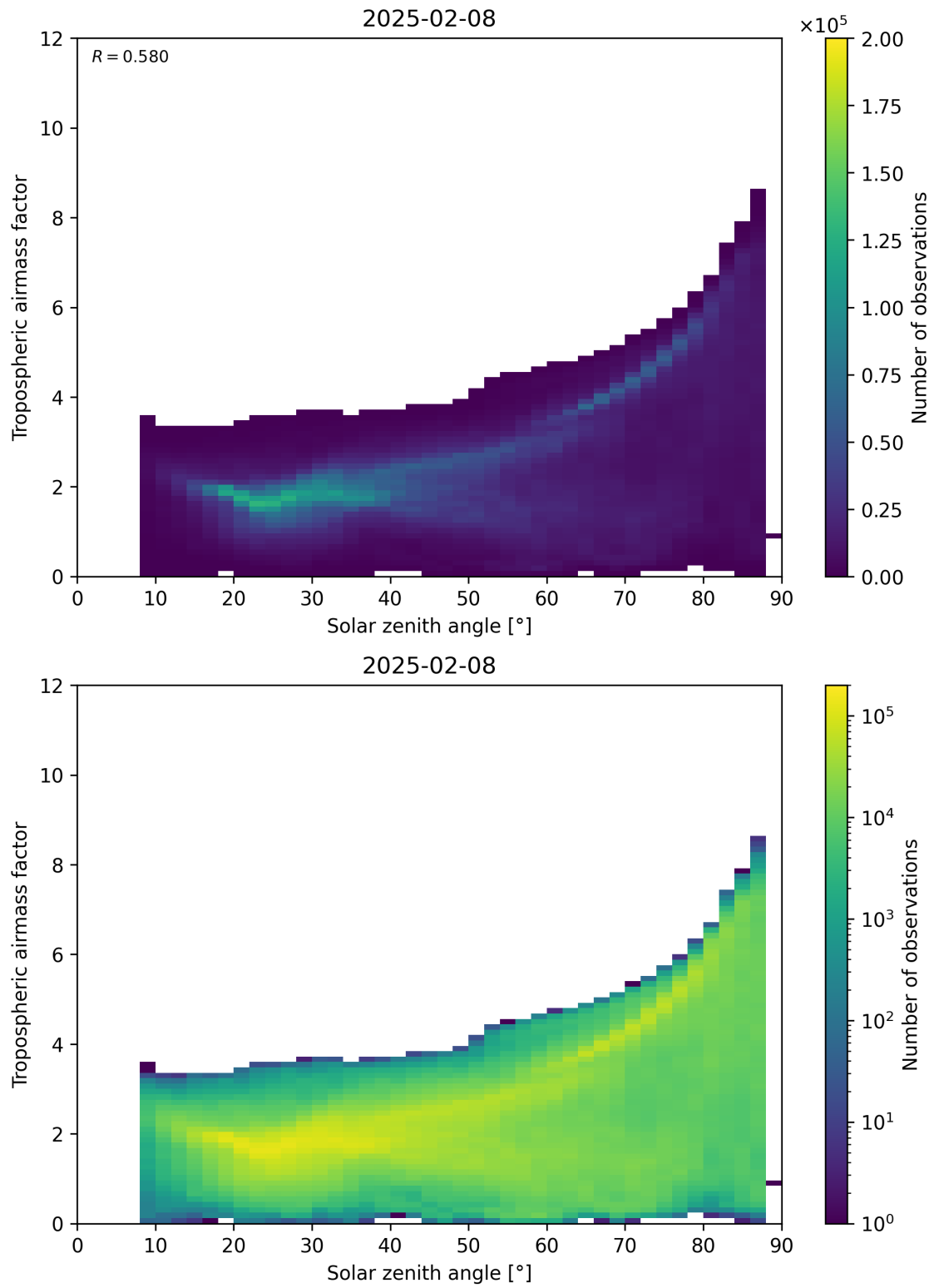
Figure 147: Scatter density plot of “Solar zenith angle” against “Tropospheric airmass factor” for 2025-02-08 to 2025-02-09.
