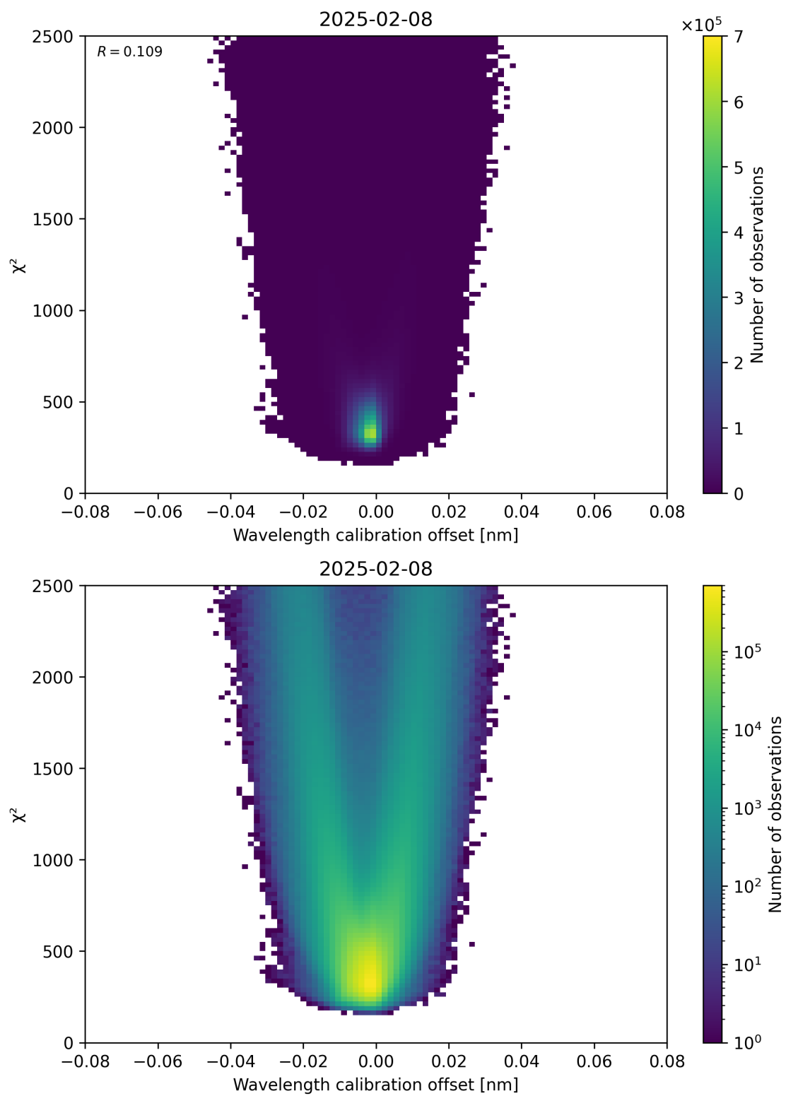
Figure 175: Scatter density plot of “Wavelength calibration offset” against “ \chi^2 ” for 2025-02-08 to 2025-02-09.
