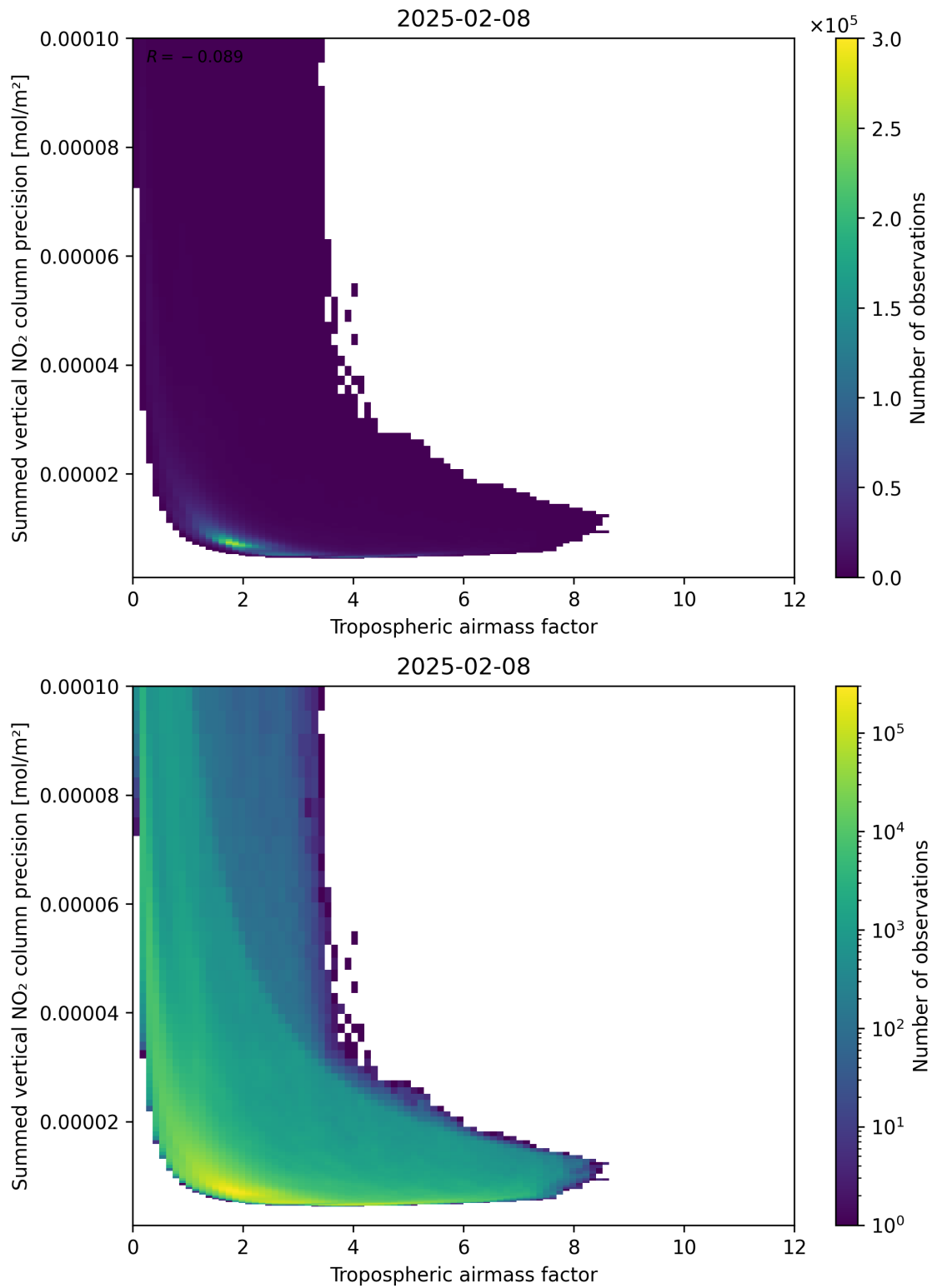
Figure 76: Scatter density plot of “Tropospheric air mass factor” against “Summed vertical NO 2 column precision” for 2025-02-08 to 2025-02-09.
