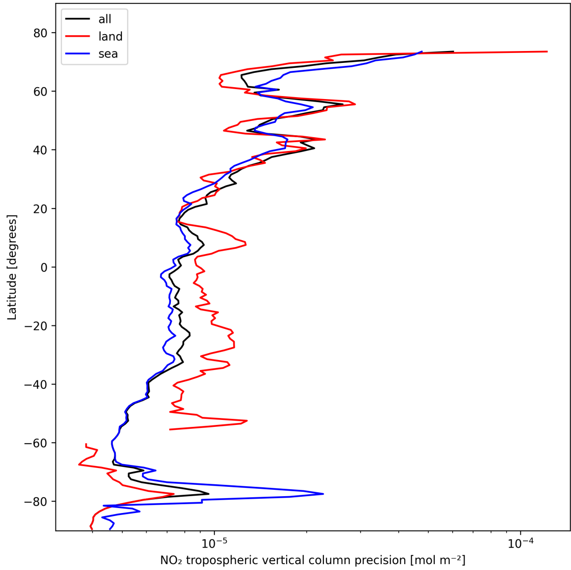
Figure 13: Zonal average of "NO 2 tropospheric vertical column precision" for 2025-02-08 to 2025-02-09.
