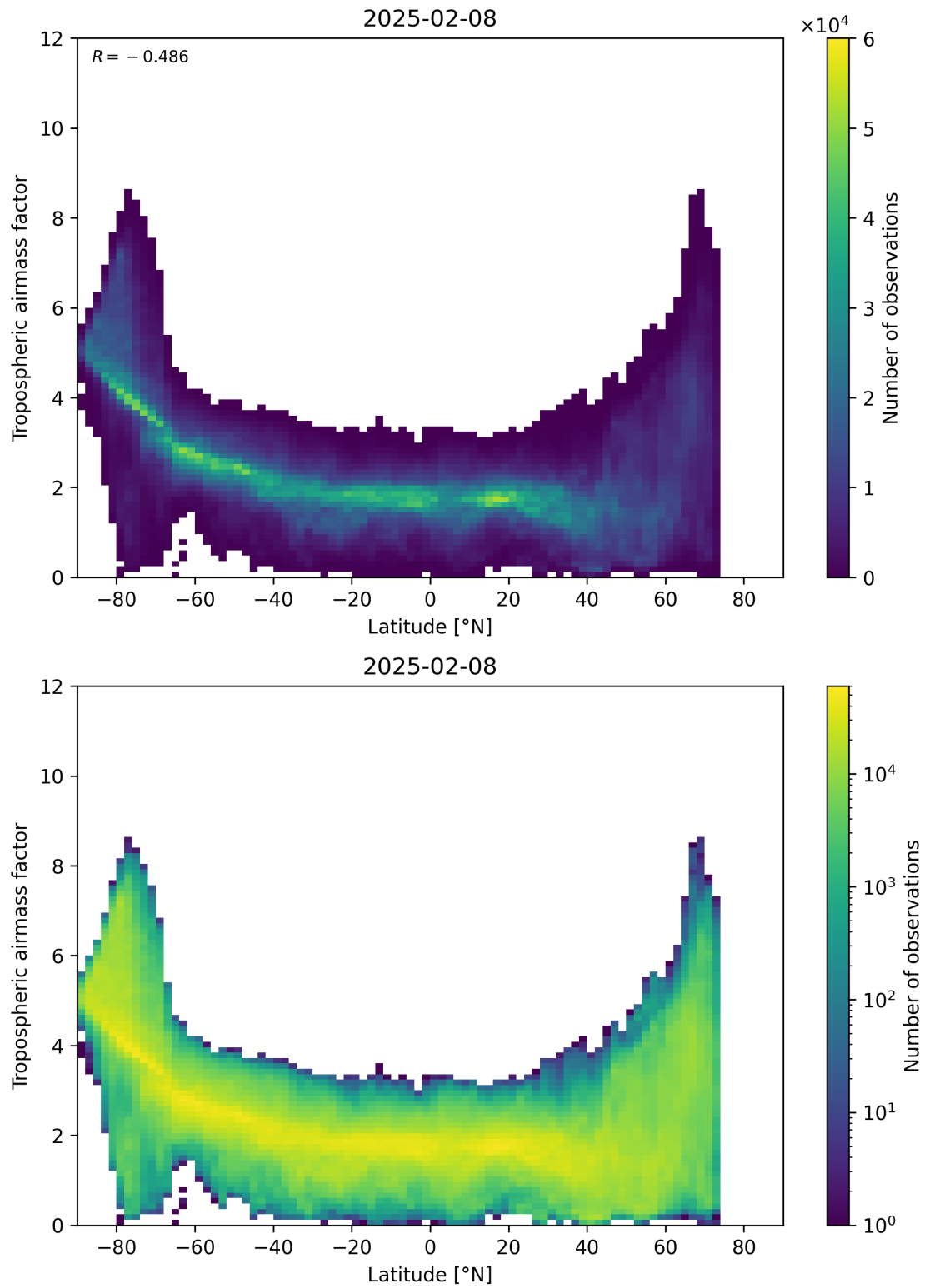
Figure 85: Scatter density plot of “Latitude” against “Tropospheric airmass factor” for 2025-02-08 to 2025-02-09.
