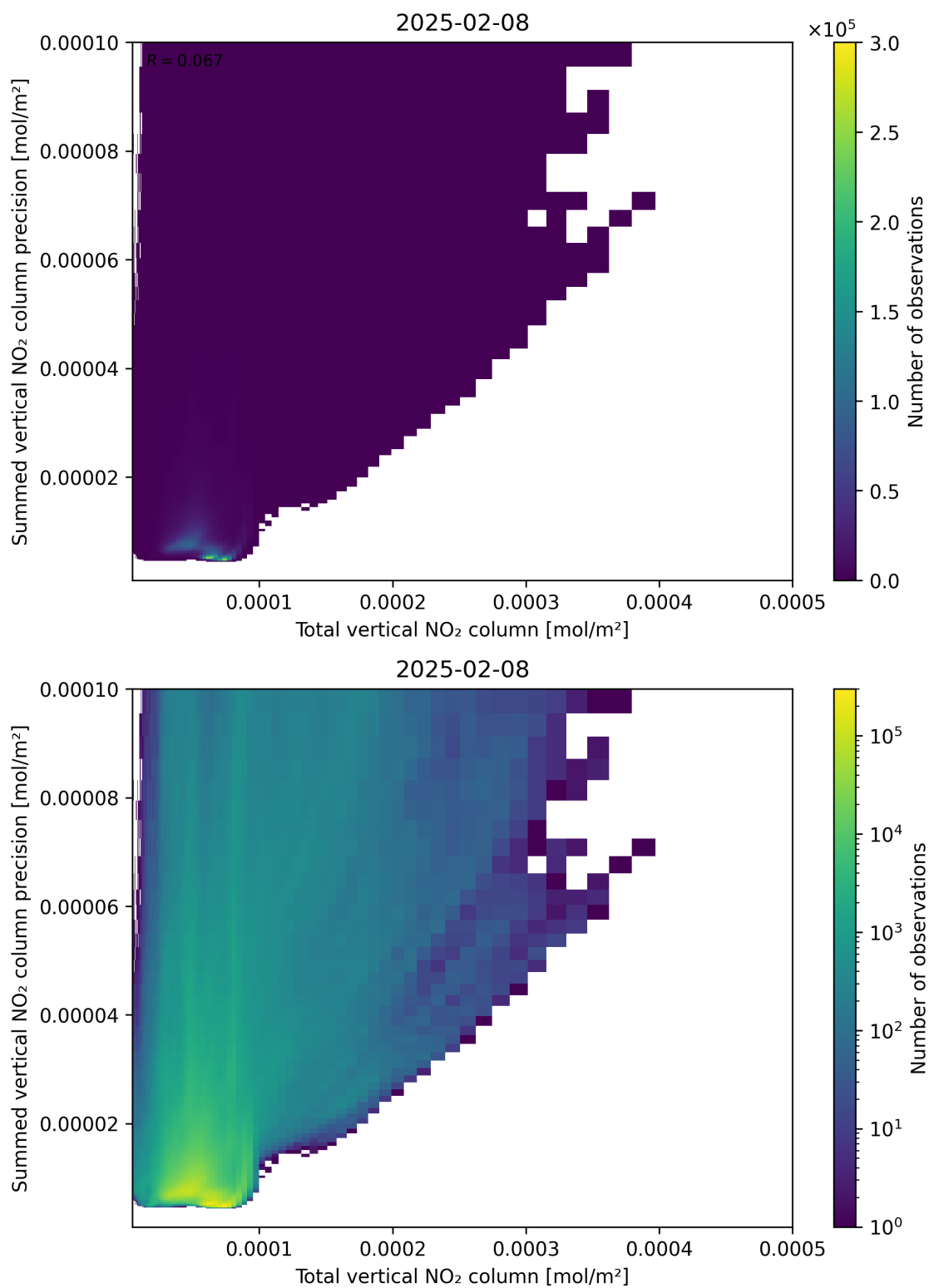
Figure 113: Scatter density plot of “Total vertical NO 2 column” against “Summed vertical NO 2 column precision” for 2025-02-08 to 2025-02-09.
