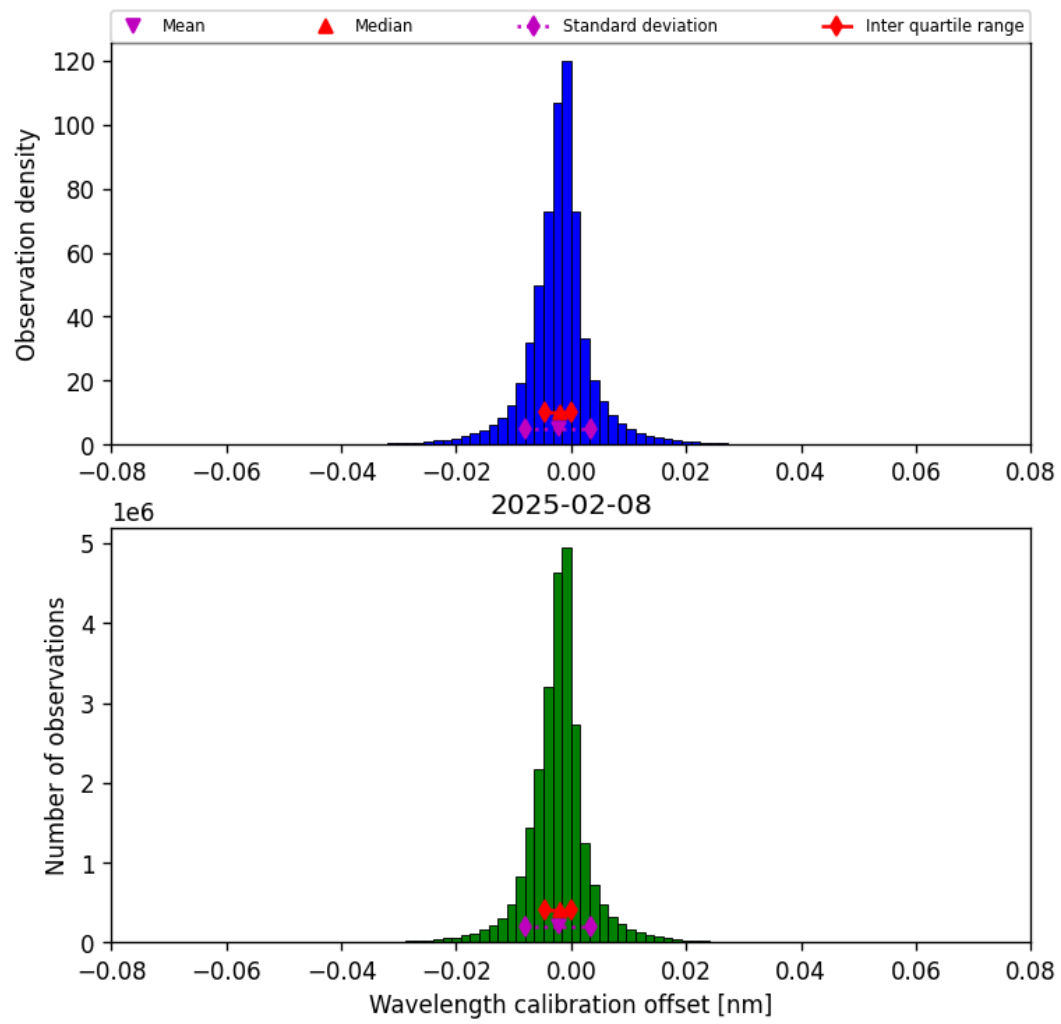
Figure 35: Histogram of “Wavelength calibration offset” for 2025-02-08 to 2025-02-09
