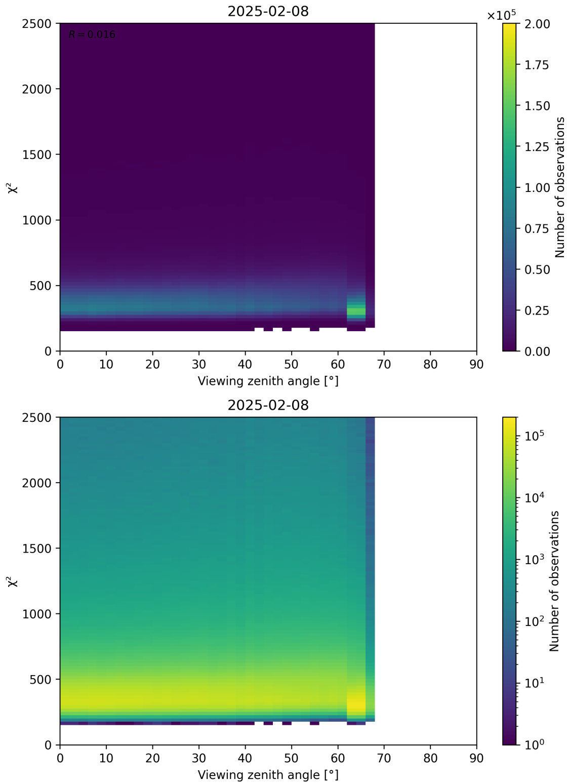
Figure 162: Scatter density plot of “Viewing zenith angle” against “ \chi^2 ” for 2025-02-08 to 2025-02-09.
