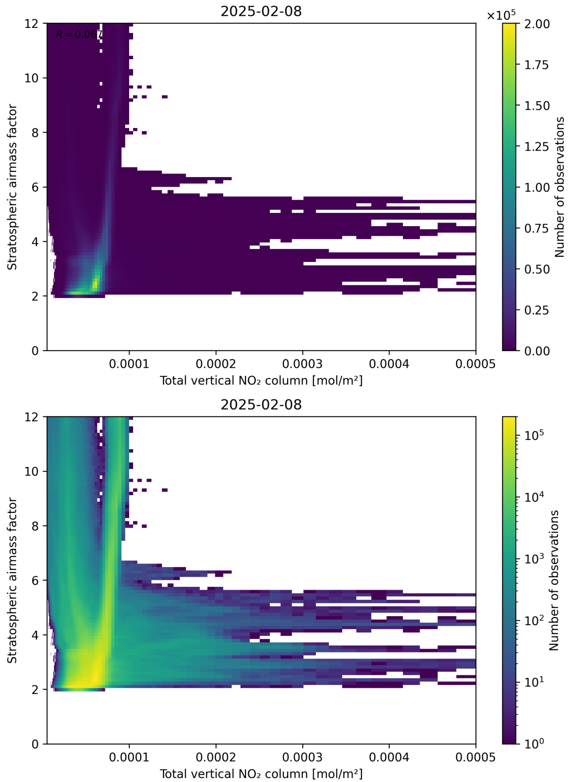
Figure 110: Scatter density plot of “Total vertical NO 2 column” against “Stratospheric air mass factor” for 2025-02-08 to 2025-02-09.
