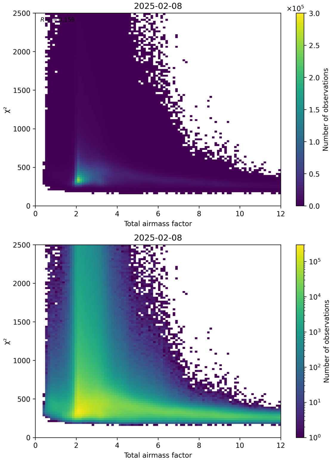
Figure 63: Scatter density plot of “Total airmass factor” against “ \chi^2 ” for 2025-02-08 to 2025-02-09.
