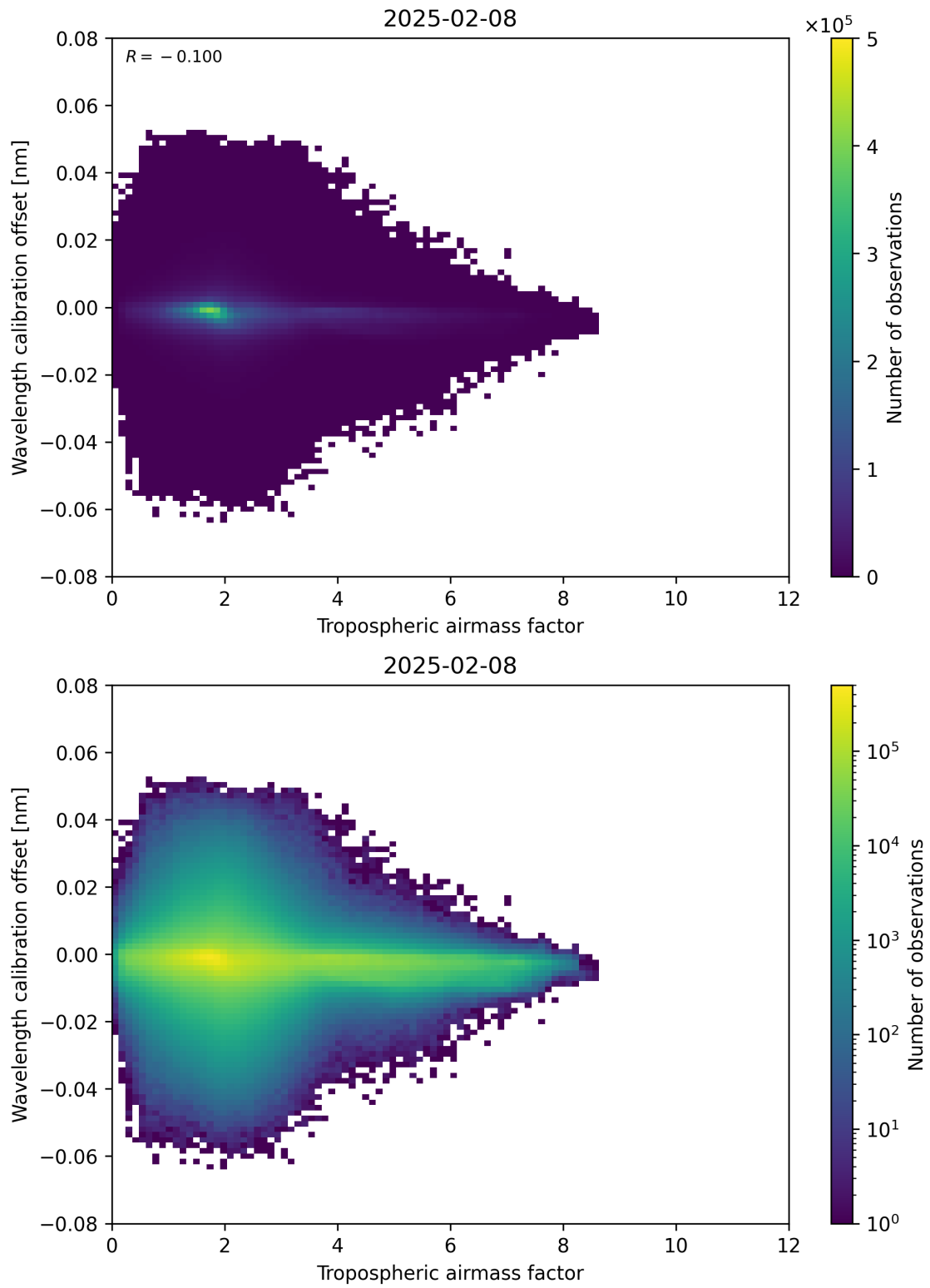
Figure 80: Scatter density plot of “Tropospheric air mass factor” against “Wavelength calibration offset” for 2025-02-08 to 2025-02-09.
