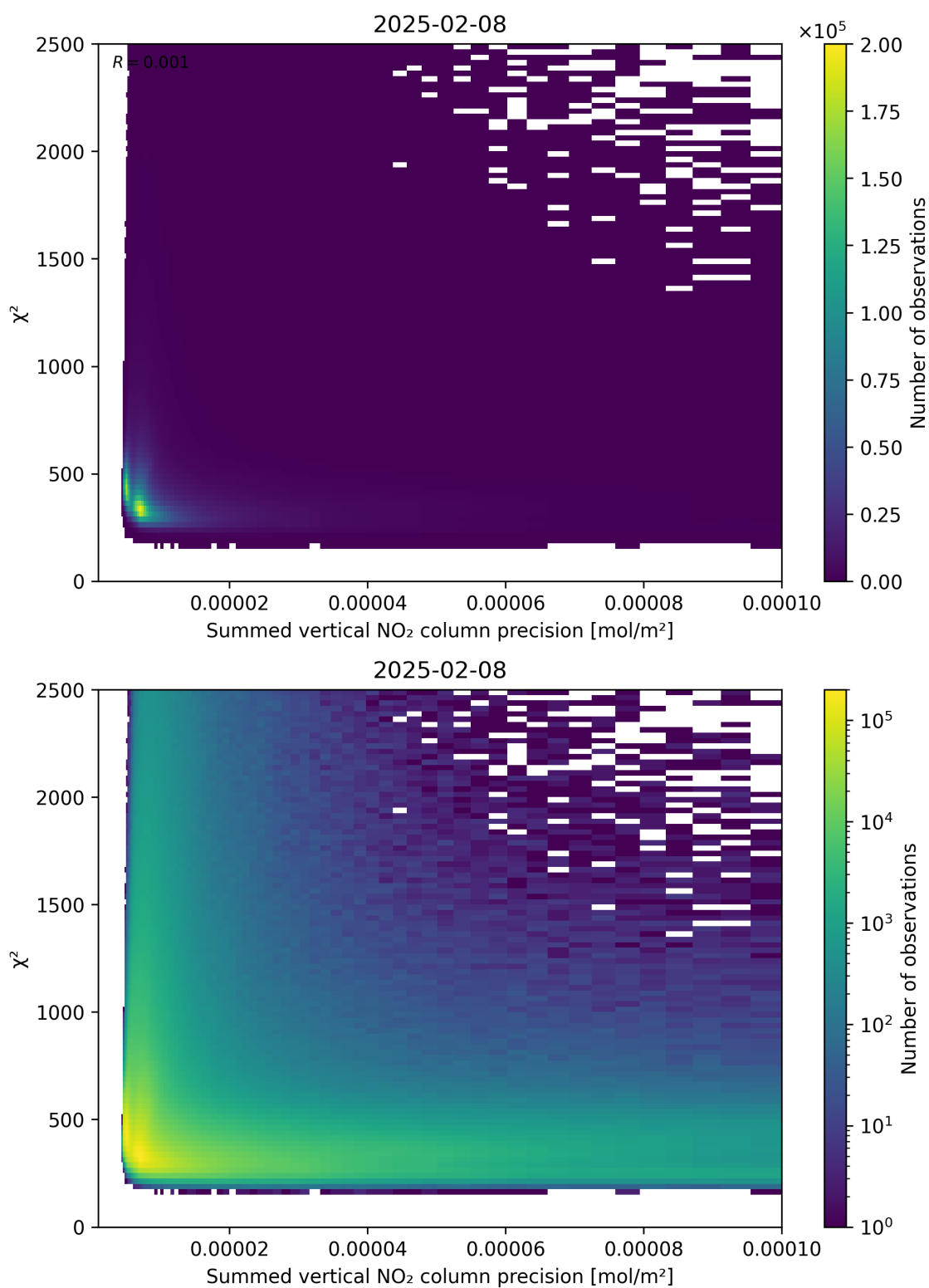
Figure 107: Scatter density plot of “Summed vertical NO 2 column precision” against “ \chi^2 ” for 2025-02-08 to 2025-02-09.
