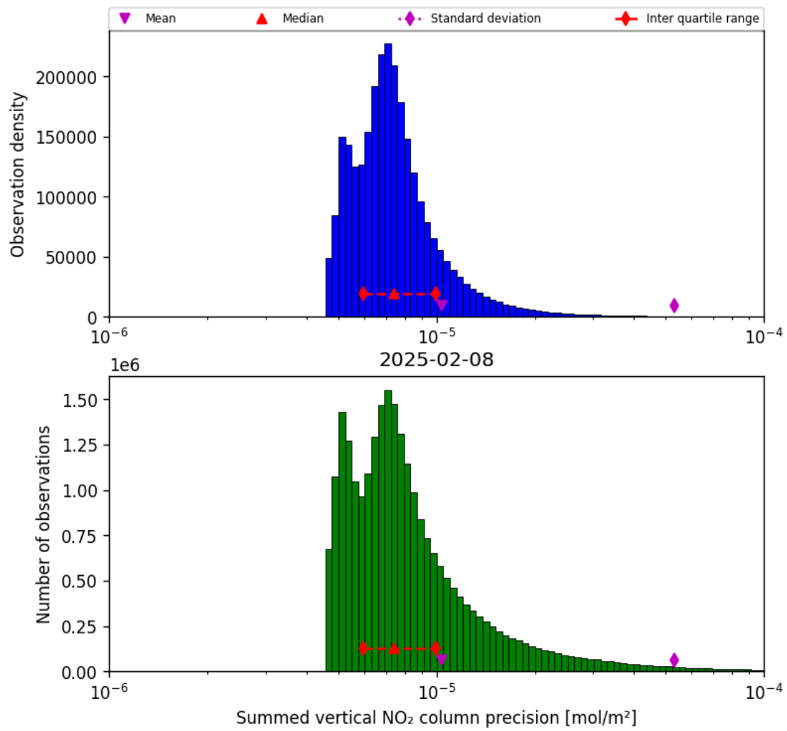
Figure 41: Histogram of “Summed vertical NO 2 column precision” for 2025-02-08 to 2025-02-09
