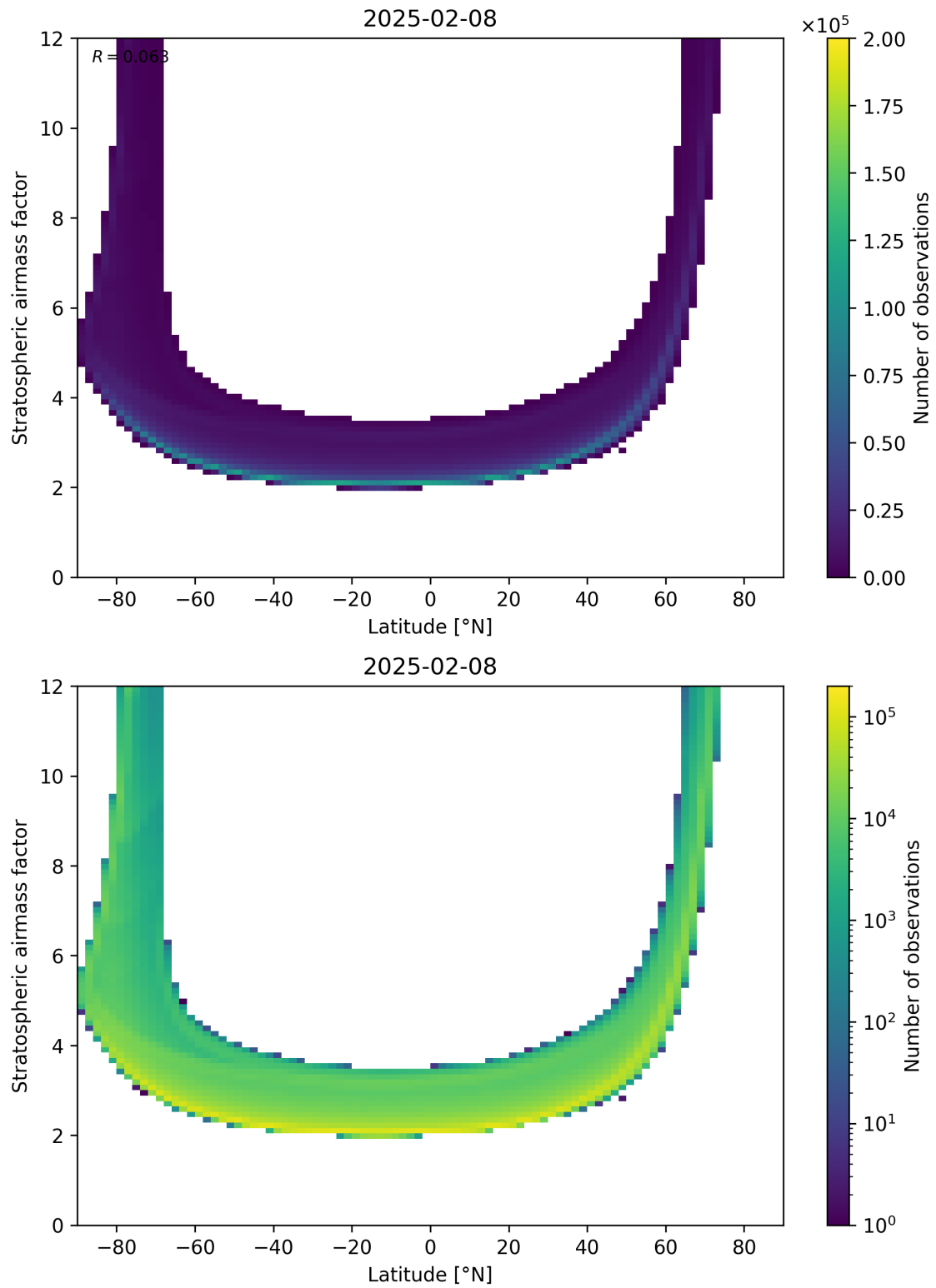
Figure 83: Scatter density plot of “Latitude” against “Stratospheric airmass factor” for 2025-02-08 to 2025-02-09.
