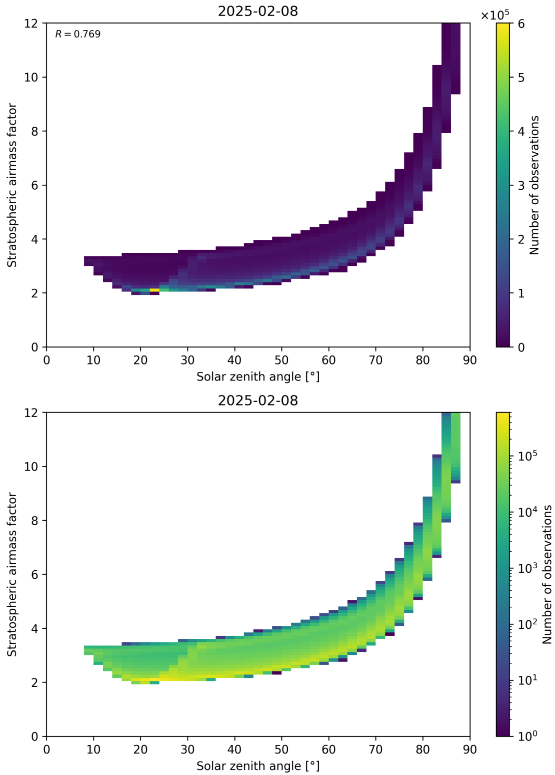
Figure 145: Scatter density plot of “Solar zenith angle” against “Stratospheric airmass factor” for 2025-02-08 to 2025-02-09.
