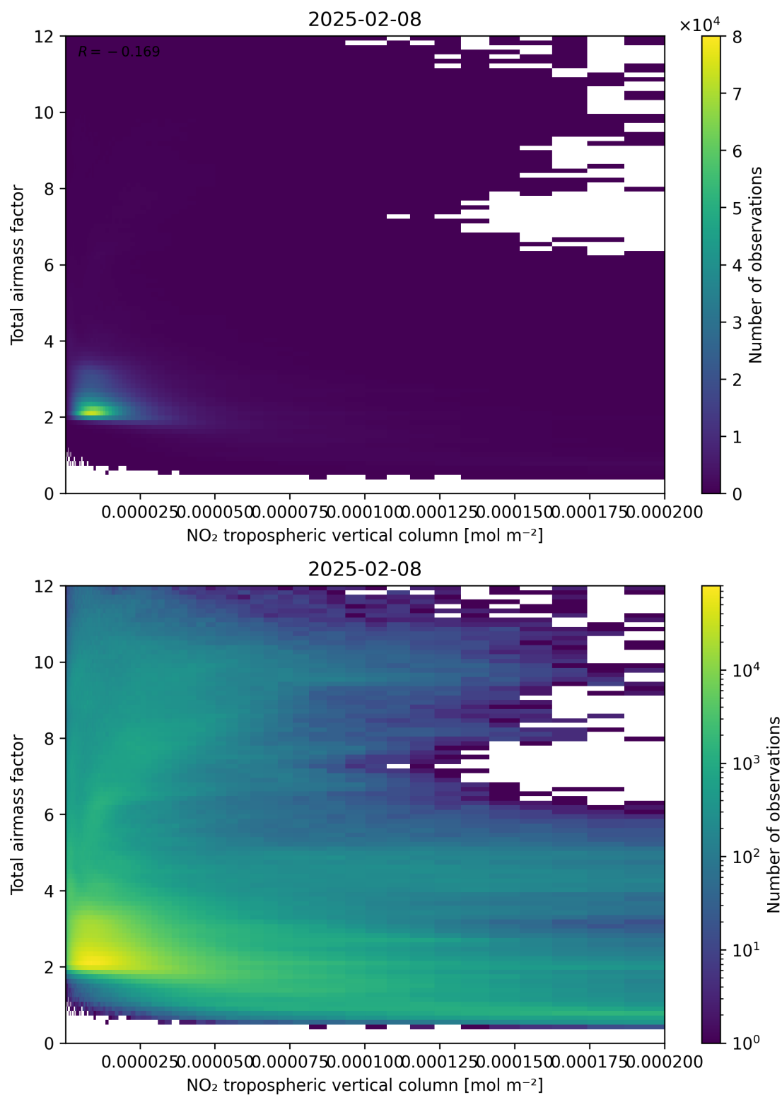
Figure 122: Scatter density plot of “NO 2 tropospheric vertical column” against “Total air mass factor” for 2025-02-08 to 2025-02-09.
