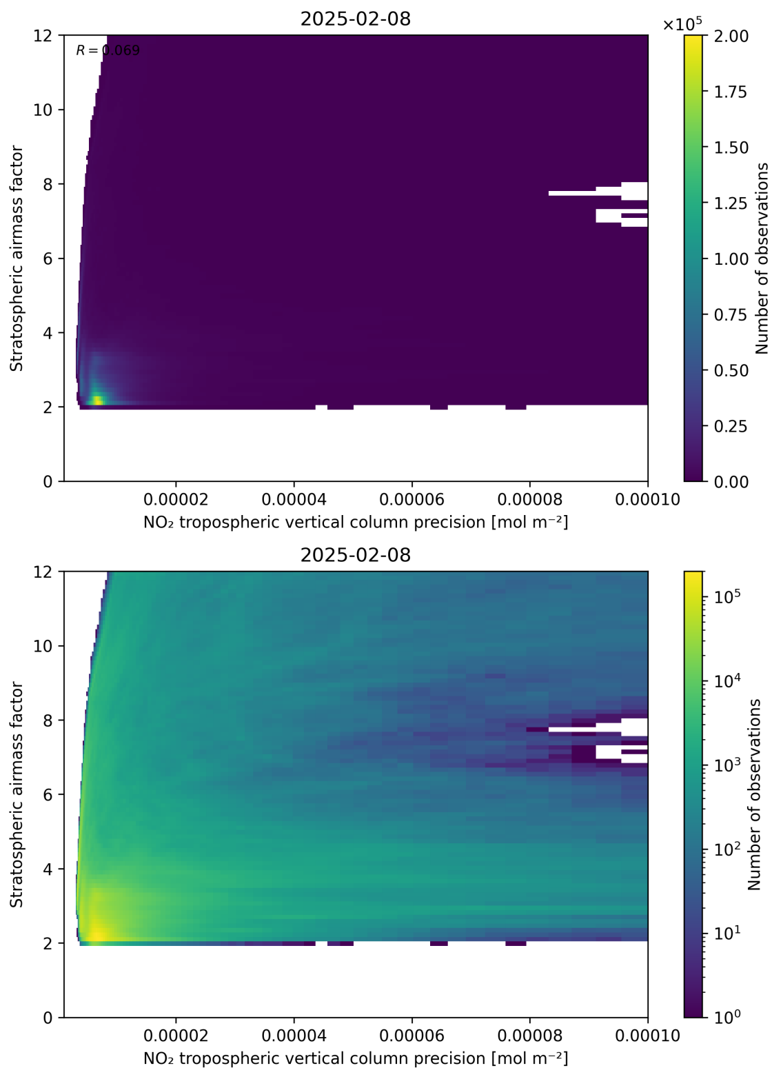
Figure 131: Scatter density plot of “NO 2 tropospheric vertical column precision” against “Stratospheric airmass factor” for 2025-02-08 to 2025-02-09.
