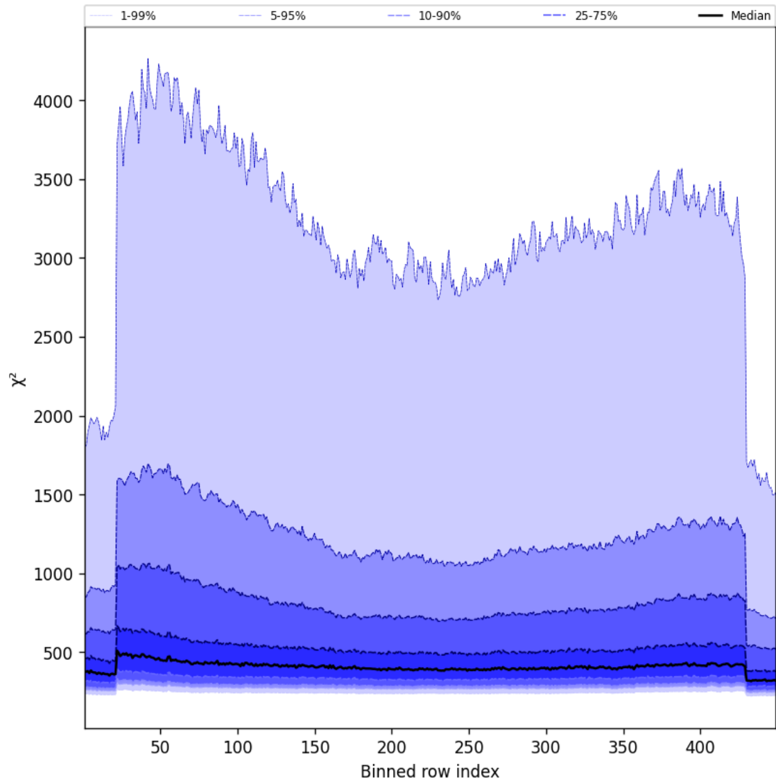
Figure 59: Along track statistics of “ \chi^2 ” for 2025-02-08 to 2025-02-09
