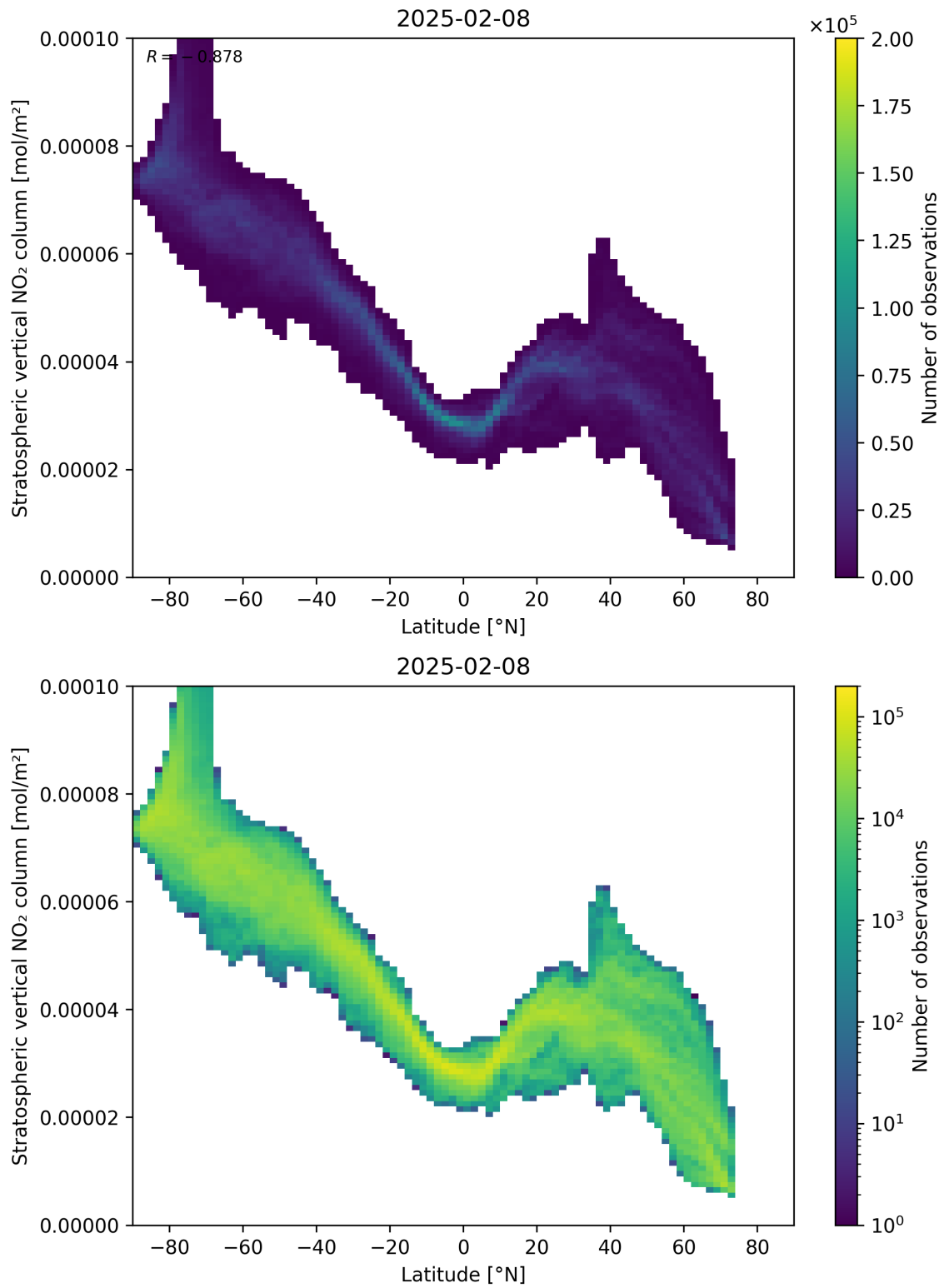
Figure 87: Scatter density plot of “Latitude” against “Stratospheric vertical NO 2 column” for 2025-02-08 to 2025-02-09.
