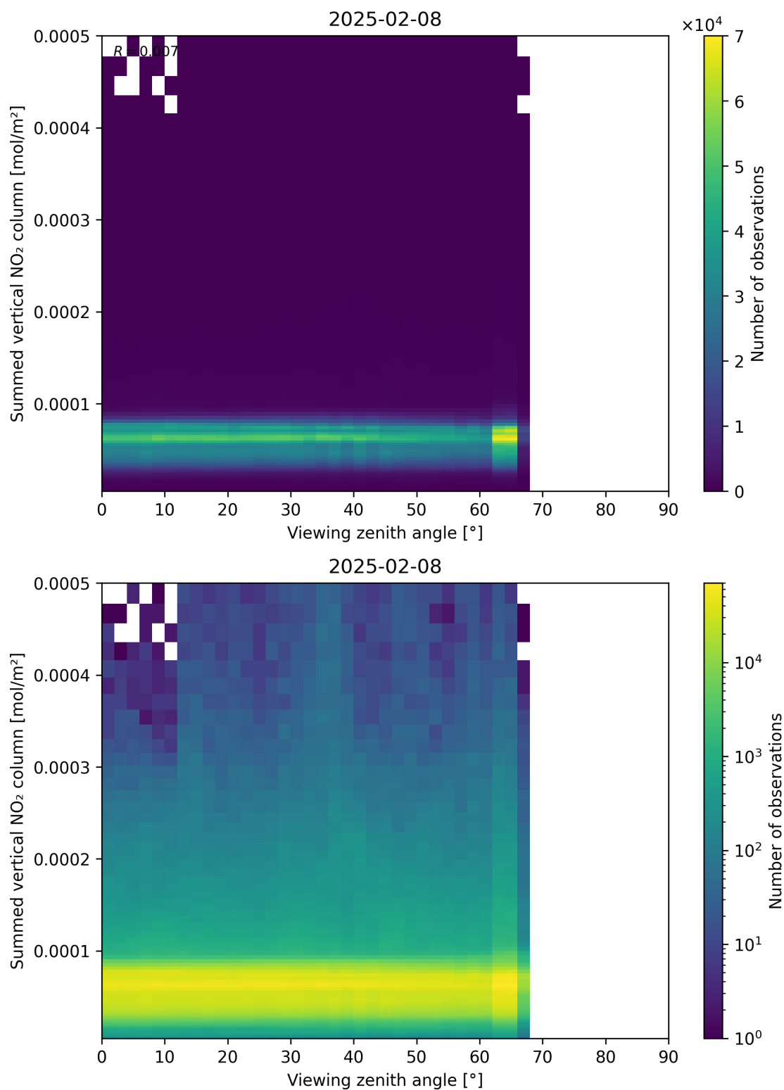
Figure 165: Scatter density plot of “Viewing zenith angle” against “Summed vertical NO 2 column” for 2025-02-08 to 2025-02-09.
