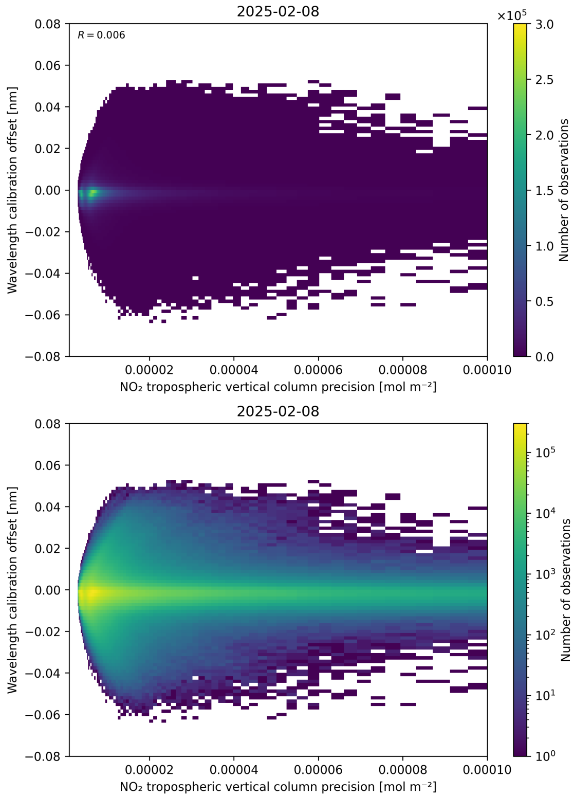
Figure 141: Scatter density plot of “NO 2 tropospheric vertical column precision” against “Wavelength calibration offset” for 2025-02-08 to 2025-02-09.
