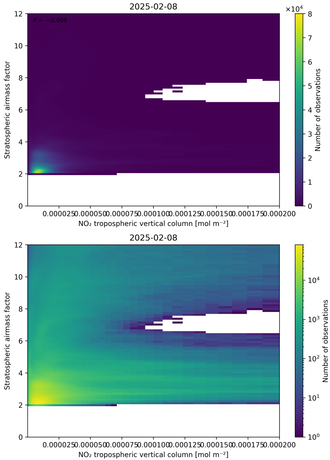
Figure 121: Scatter density plot of “NO 2 tropospheric vertical column” against “Stratospheric air mass factor” for 2025-02-08 to 2025-02-09.
