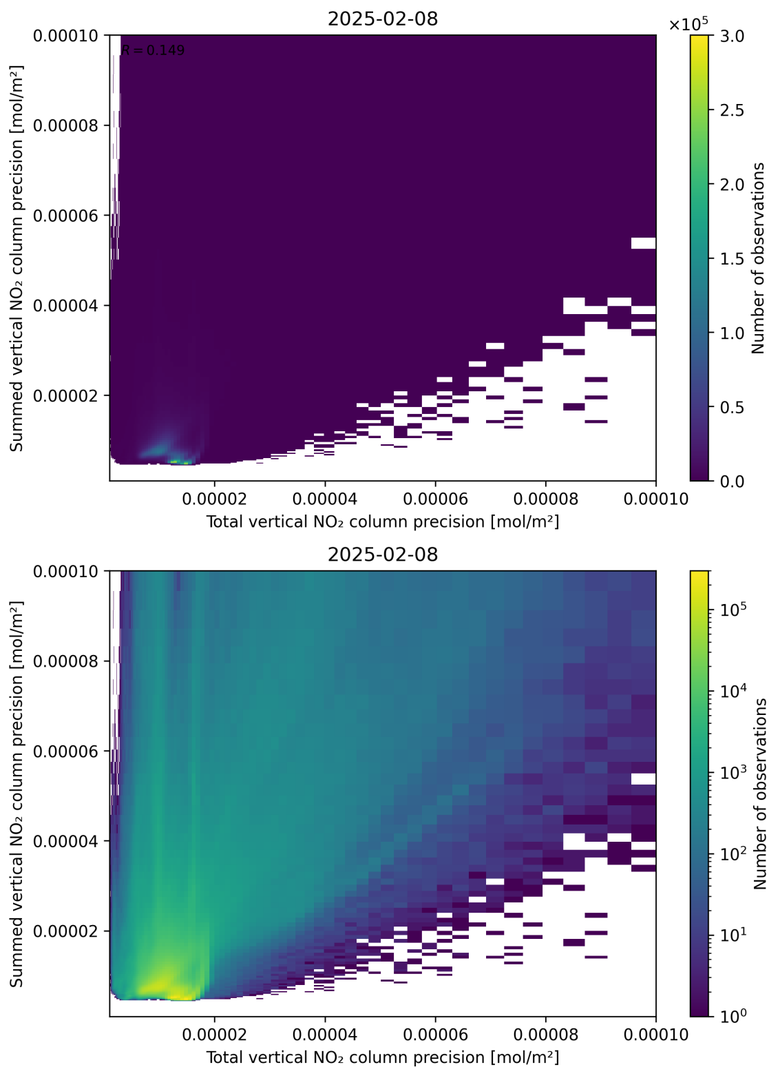
Figure 118: Scatter density plot of “Total vertical NO 2 column precision” against “Summed vertical NO 2 column precision” for 2025-02-08 to 2025-02-09.
