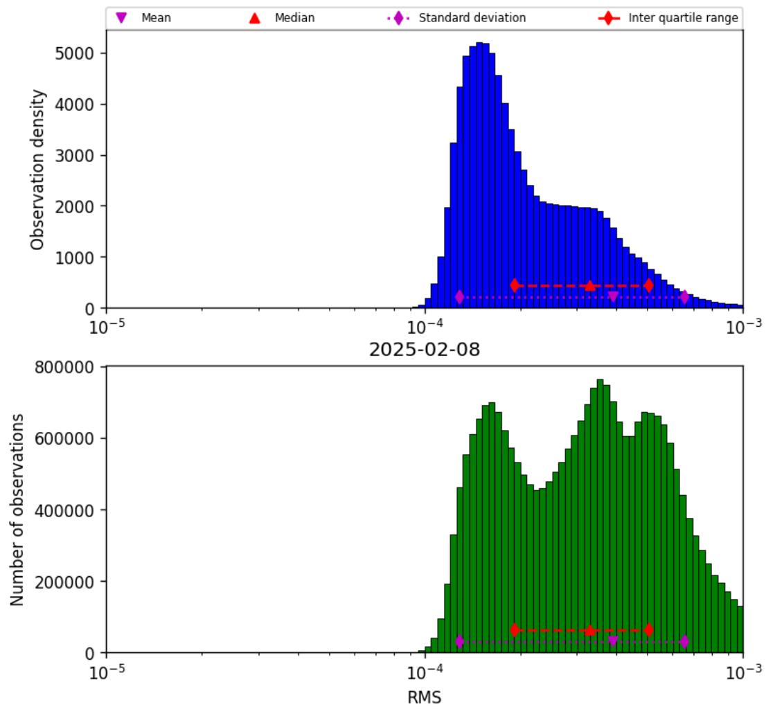
Figure 43: Histogram of “RMS” for 2025-02-08 to 2025-02-09
