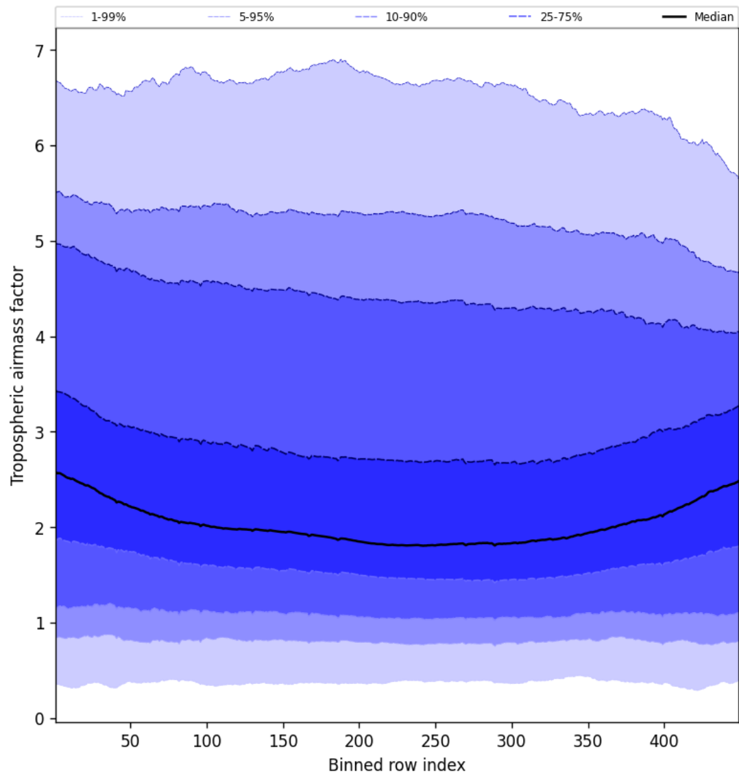
Figure 48: Along track statistics of “Tropospheric airmass factor” for 2025-02-08 to 2025-02-09
