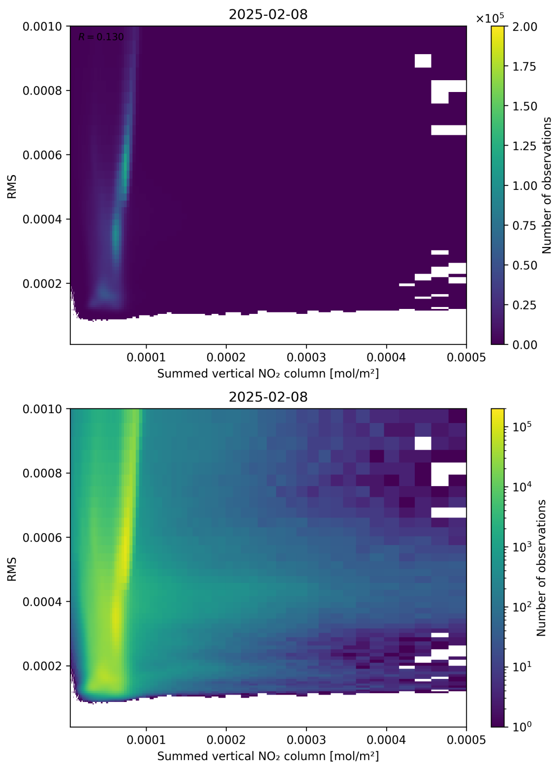
Figure 109: Scatter density plot of “Summed vertical NO 2 column” against “RMS” for 2025-02-08 to 2025-02-09.
