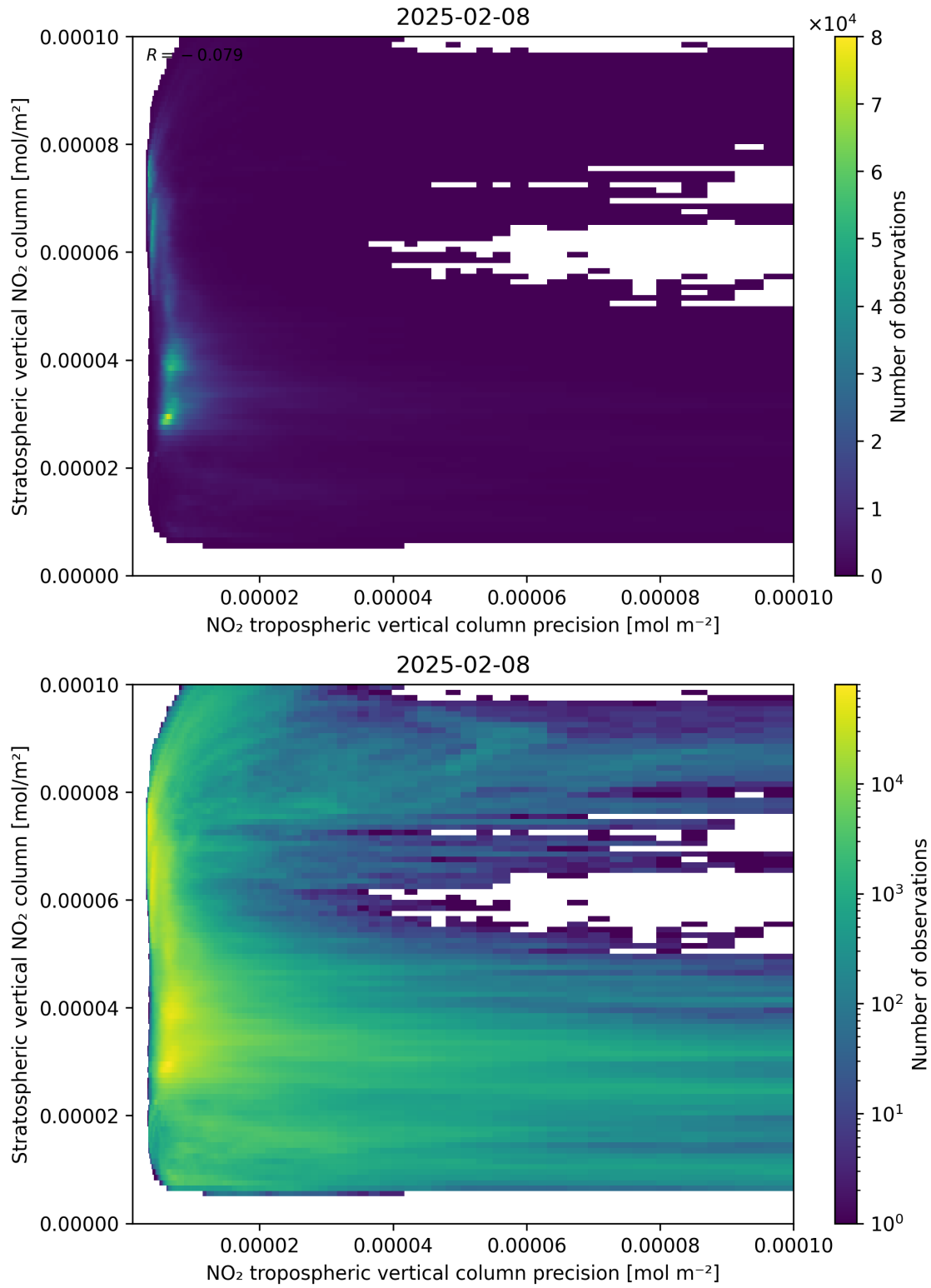
Figure 135: Scatter density plot of “NO 2 tropospheric vertical column precision” against “Stratospheric vertical NO 2 column” for 2025-02-08 to 2025-02-09.
