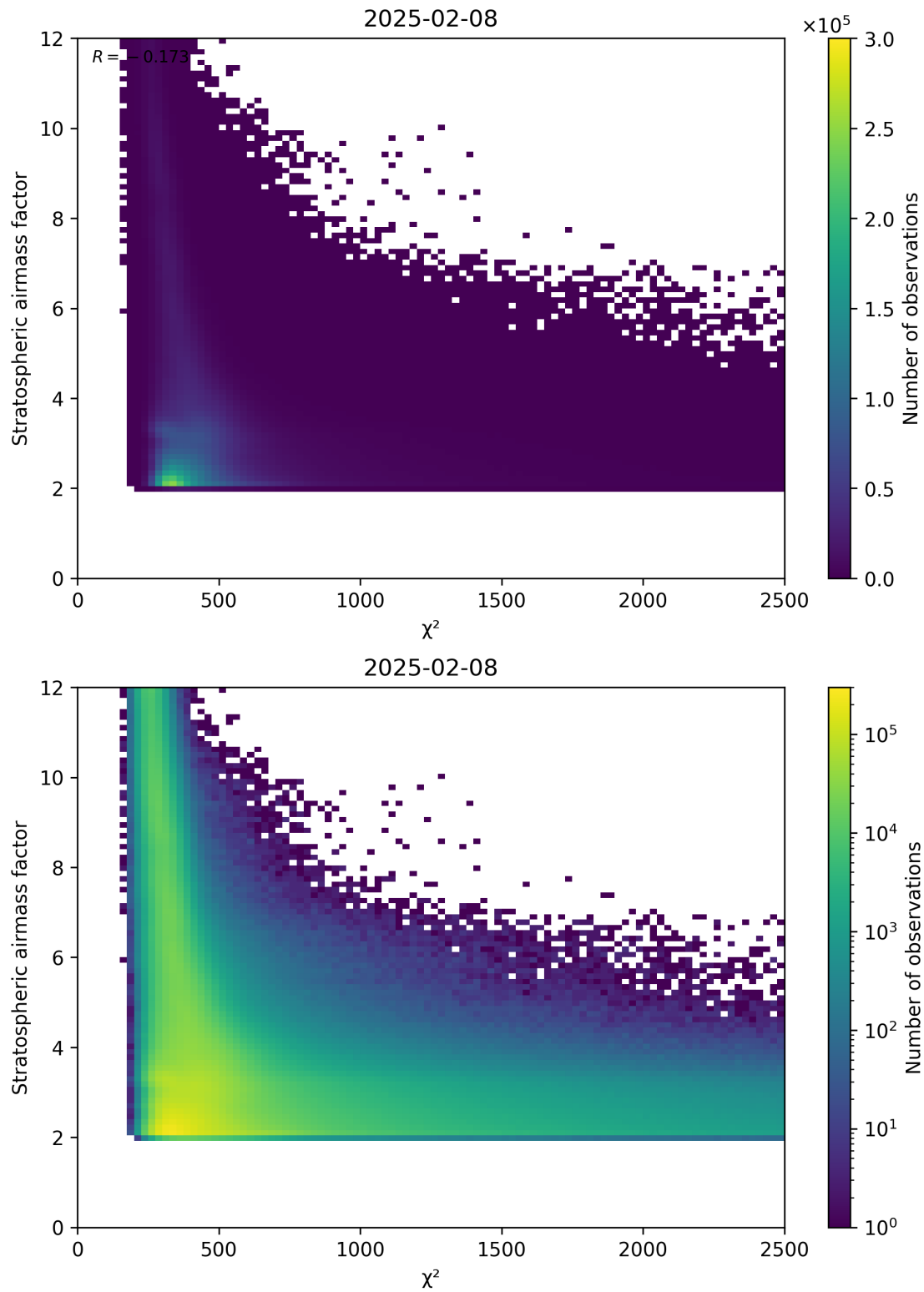
Figure 81: Scatter density plot of “ \chi^2 ” against “Stratospheric airmass factor” for 2025-02-08 to 2025-02-09.
