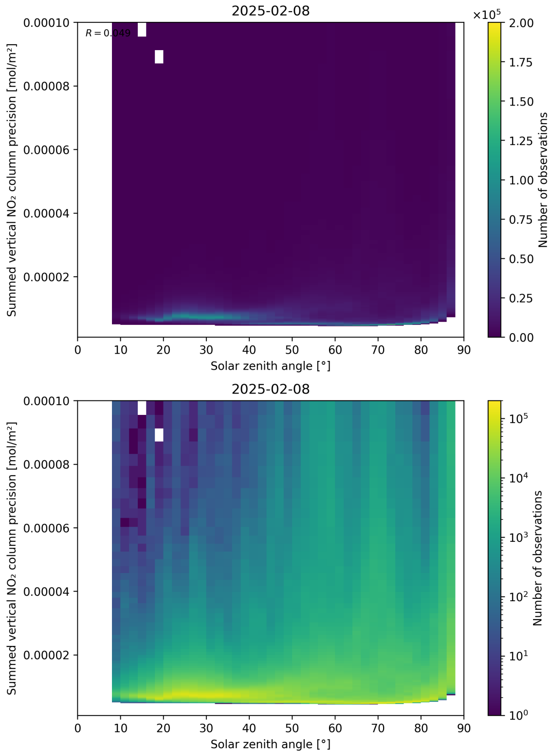
Figure 152: Scatter density plot of “Solar zenith angle” against “Summed vertical NO 2 column precision” for 2025-02-08 to 2025-02-09.
