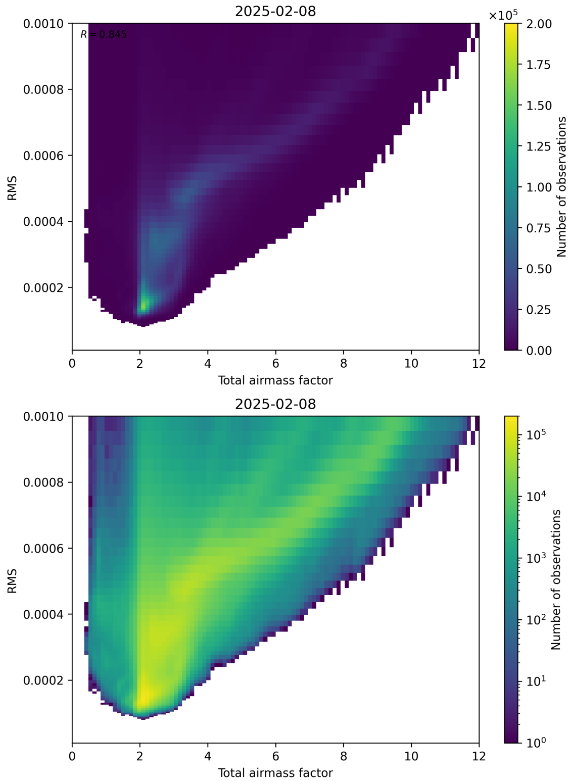
Figure 69: Scatter density plot of “Total airmass factor” against “RMS” for 2025-02-08 to 2025-02-09.
