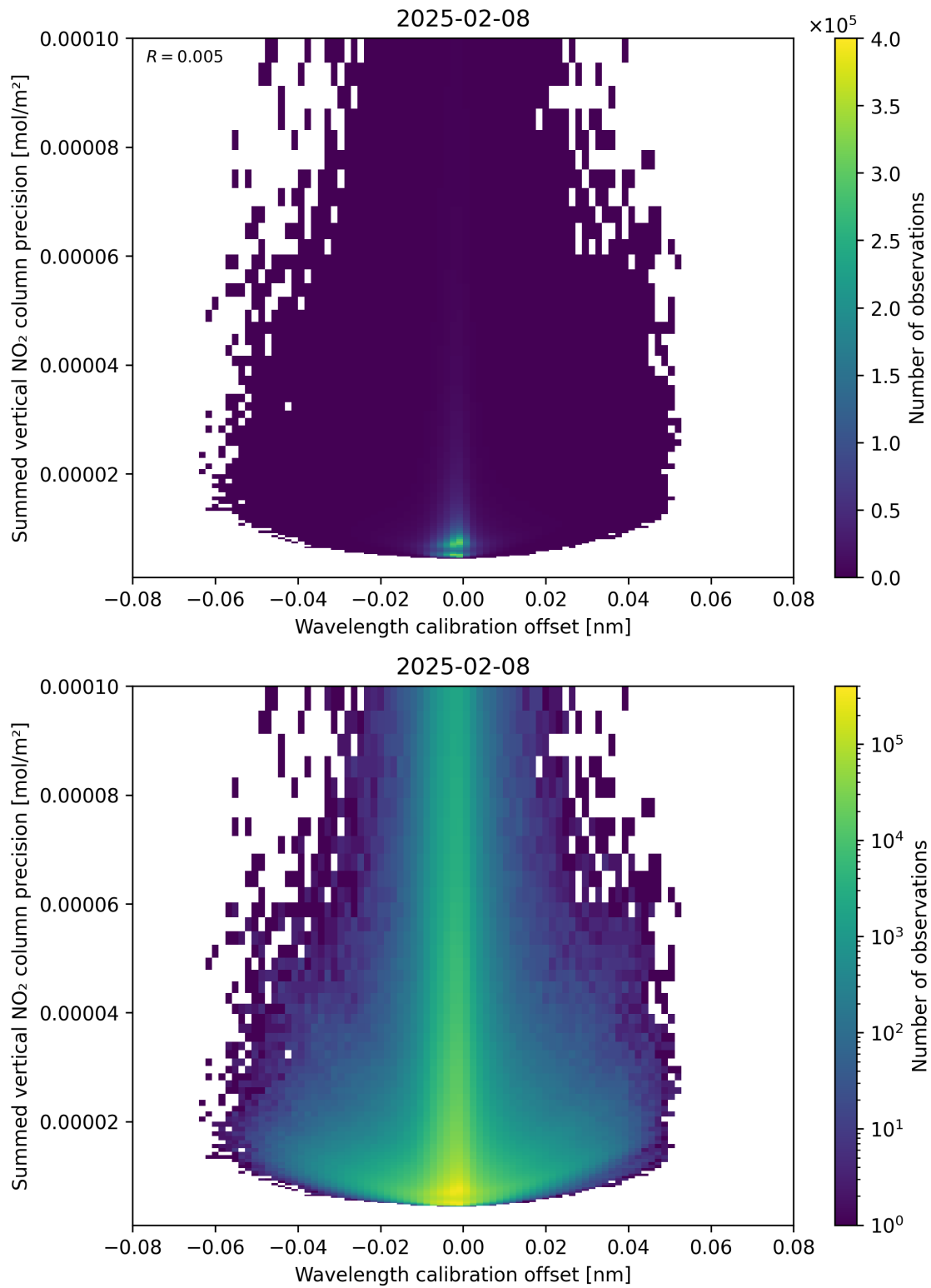
Figure 178: Scatter density plot of “Wavelength calibration offset” against “Summed vertical NO 2 column precision” for 2025-02-08 to 2025-02-09.
