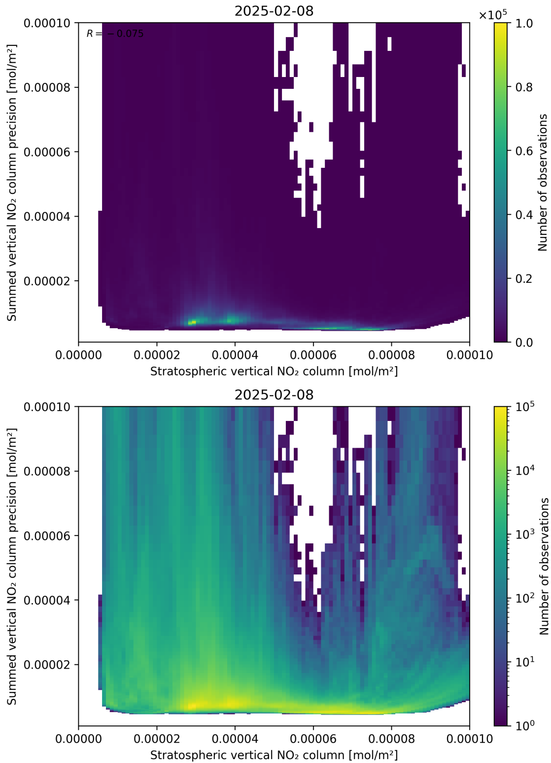
Figure 99: Scatter density plot of “Stratospheric vertical NO 2 column” against “Summed vertical NO 2 column precision” for 2025-02-08 to 2025-02-09.
