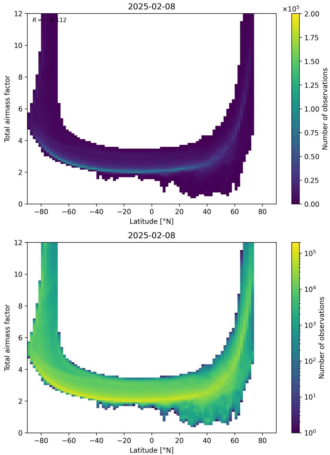
Figure 84: Scatter density plot of “Latitude” against “Total airmass factor” for 2025-02-08 to 2025-02-09.
