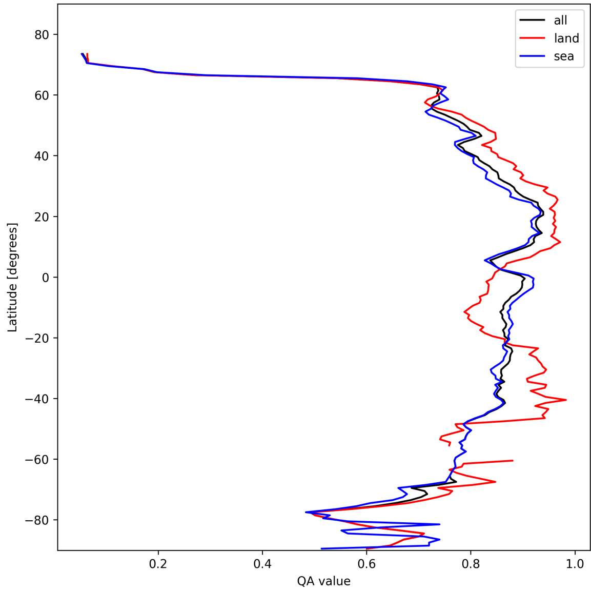
Figure 11: Zonal average of “QA value” for 2025-02-08 to 2025-02-09.
