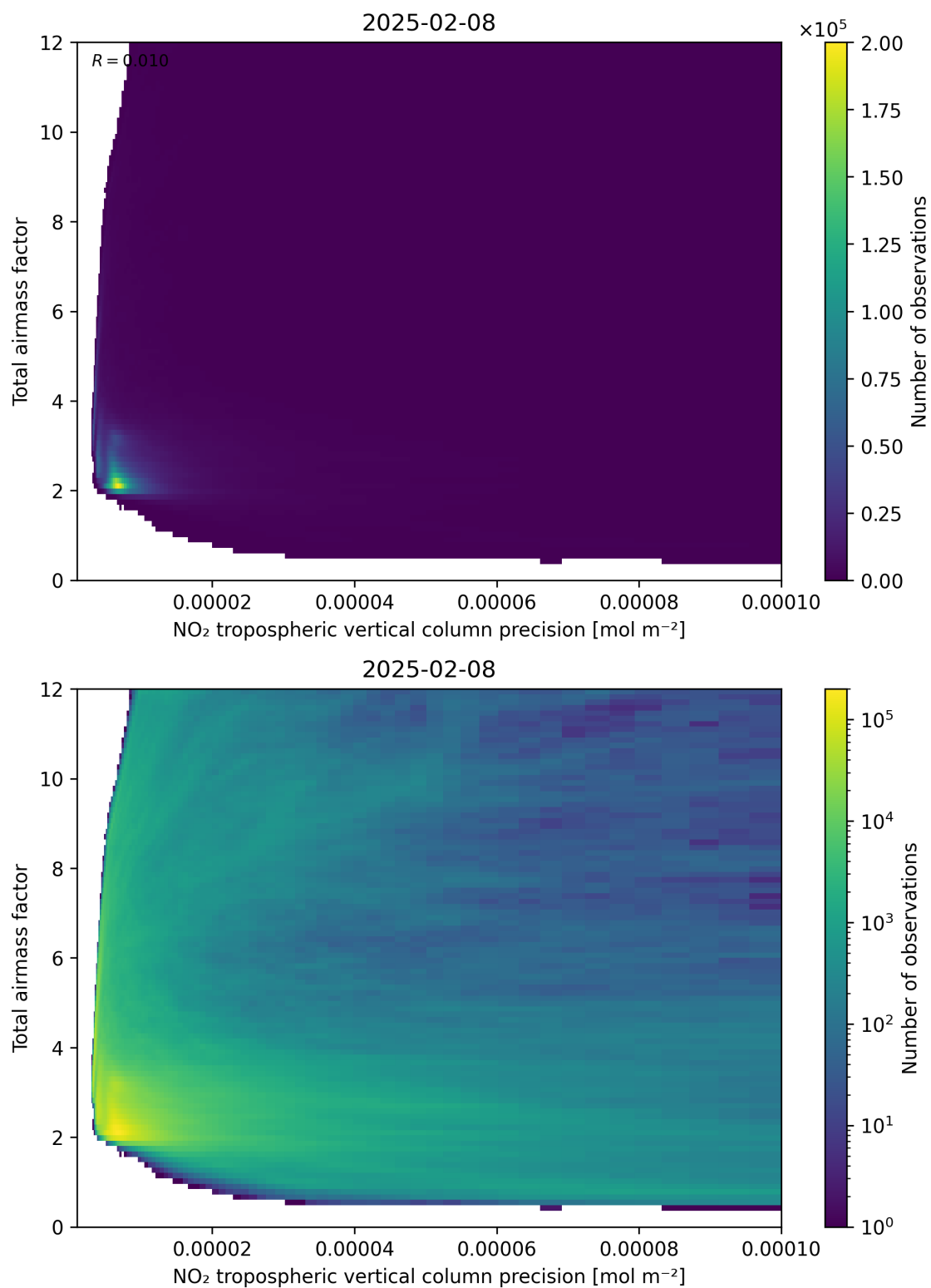
Figure 132: Scatter density plot of “NO 2 tropospheric vertical column precision” against “Total air mass factor” for 2025-02-08 to 2025-02-09.
