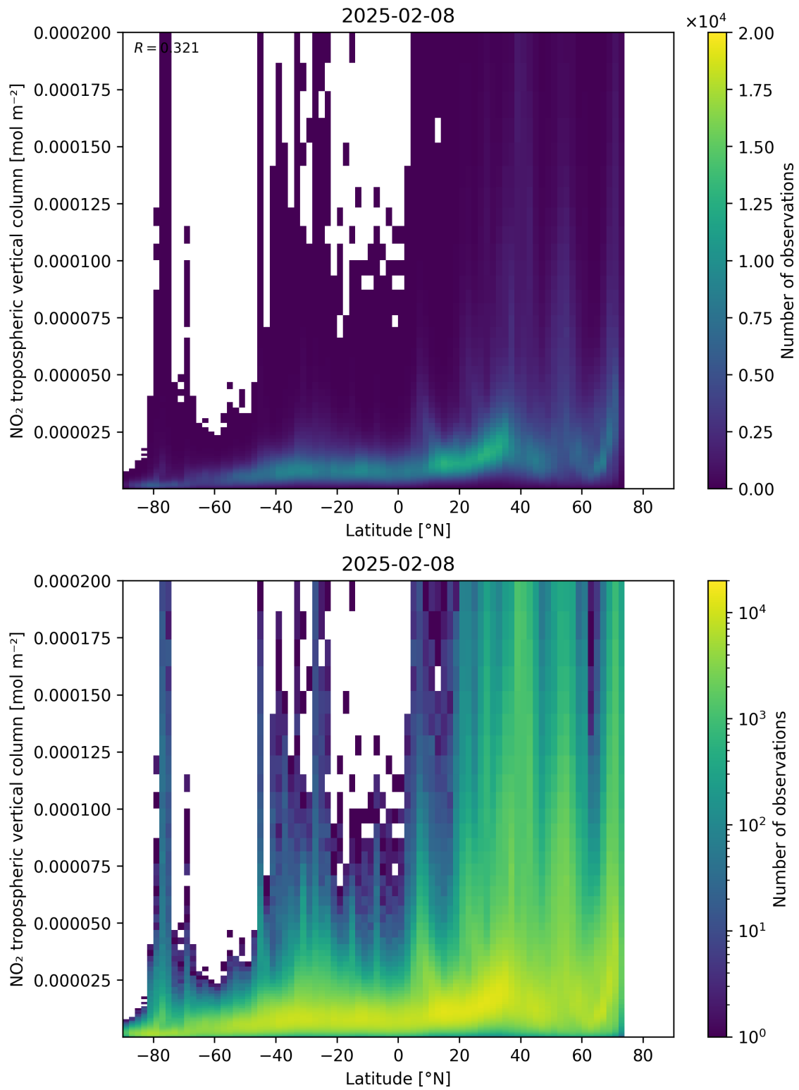
Figure 92: Scatter density plot of “Latitude” against “NO 2 tropospheric vertical column” for 2025-02-08 to 2025-02-09.
