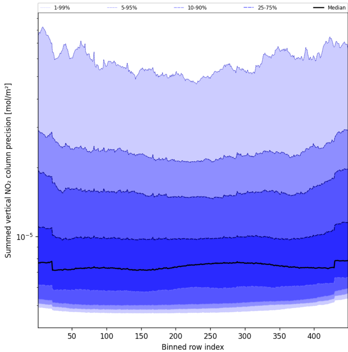
Figure 58: Along track statistics of “Summed vertical NO 2 column precision” for 2025-02-08 to 2025-02-09
