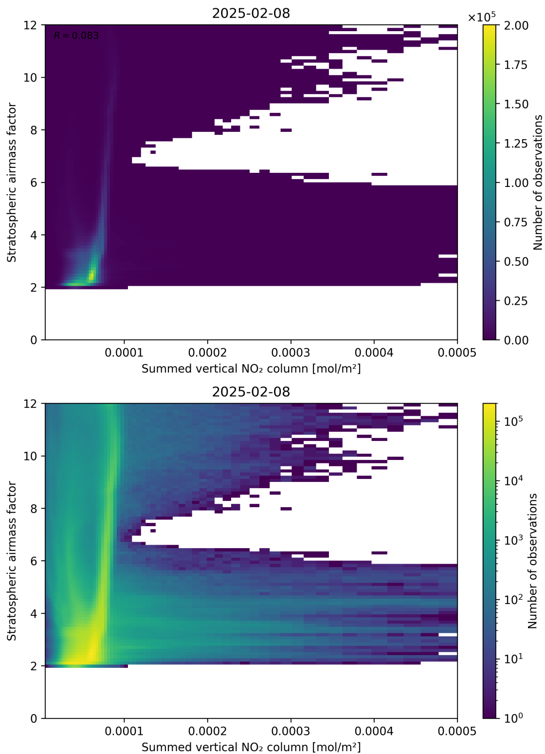
Figure 103: Scatter density plot of “Summed vertical NO 2 column” against “Stratospheric air mass factor” for 2025-02-08 to 2025-02-09.
