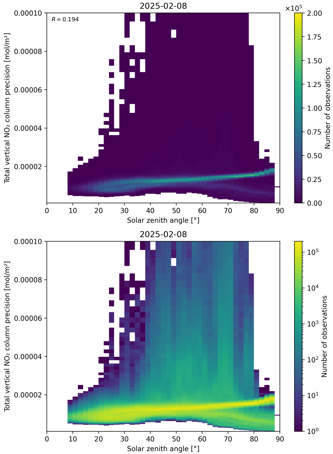
Figure 154: Scatter density plot of “Solar zenith angle” against “Total vertical NO 2 column precision” for 2025-02-08 to 2025-02-09.
