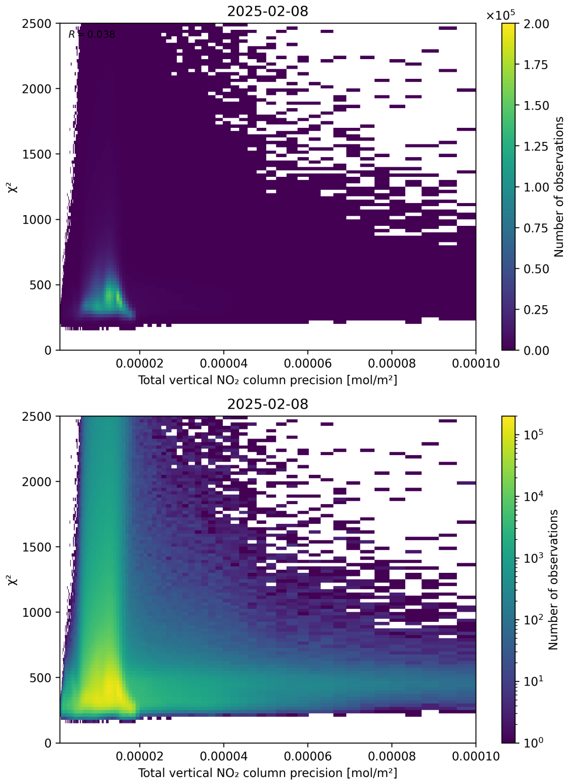
Figure 116: Scatter density plot of “Total vertical NO 2 column precision” against “ \chi^2 ” for 2025-02-08 to 2025-02-09.
