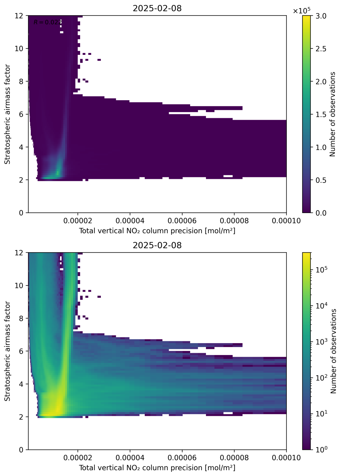
Figure 115: Scatter density plot of “Total vertical NO 2 column precision” against “Stratospheric air mass factor” for 2025-02-08 to 2025-02-09.
