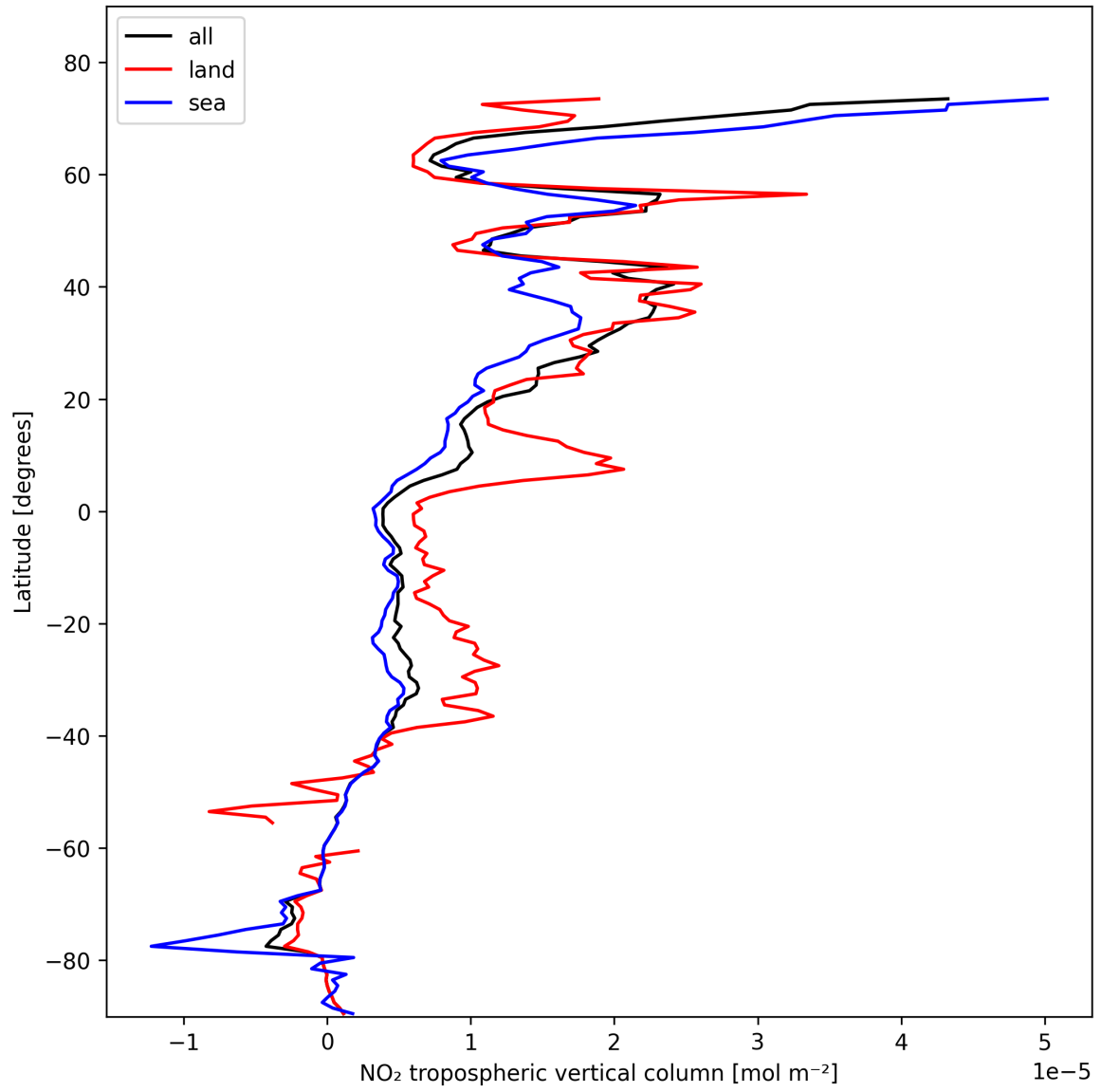
Figure 12: Zonal average of “NO 2 tropospheric vertical column” for 2025-02-08 to 2025-02-09.
