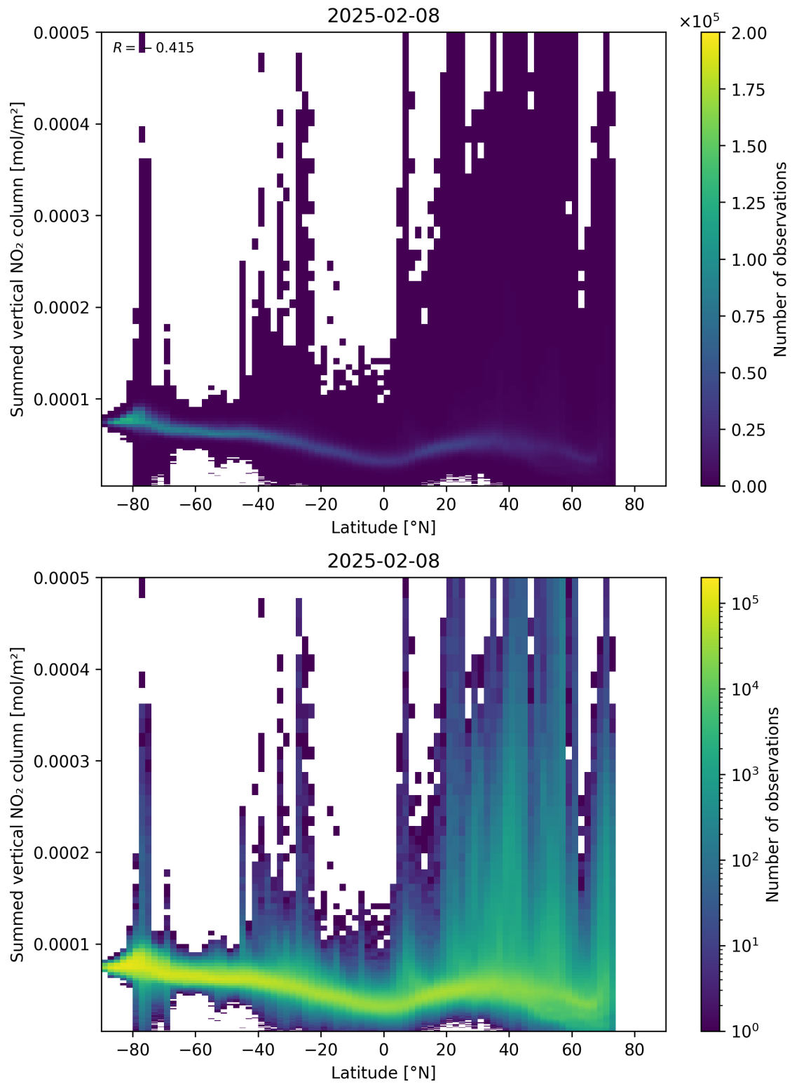
Figure 88: Scatter density plot of “Latitude” against “Summed vertical NO 2 column” for 2025-02-08 to 2025-02-09.
