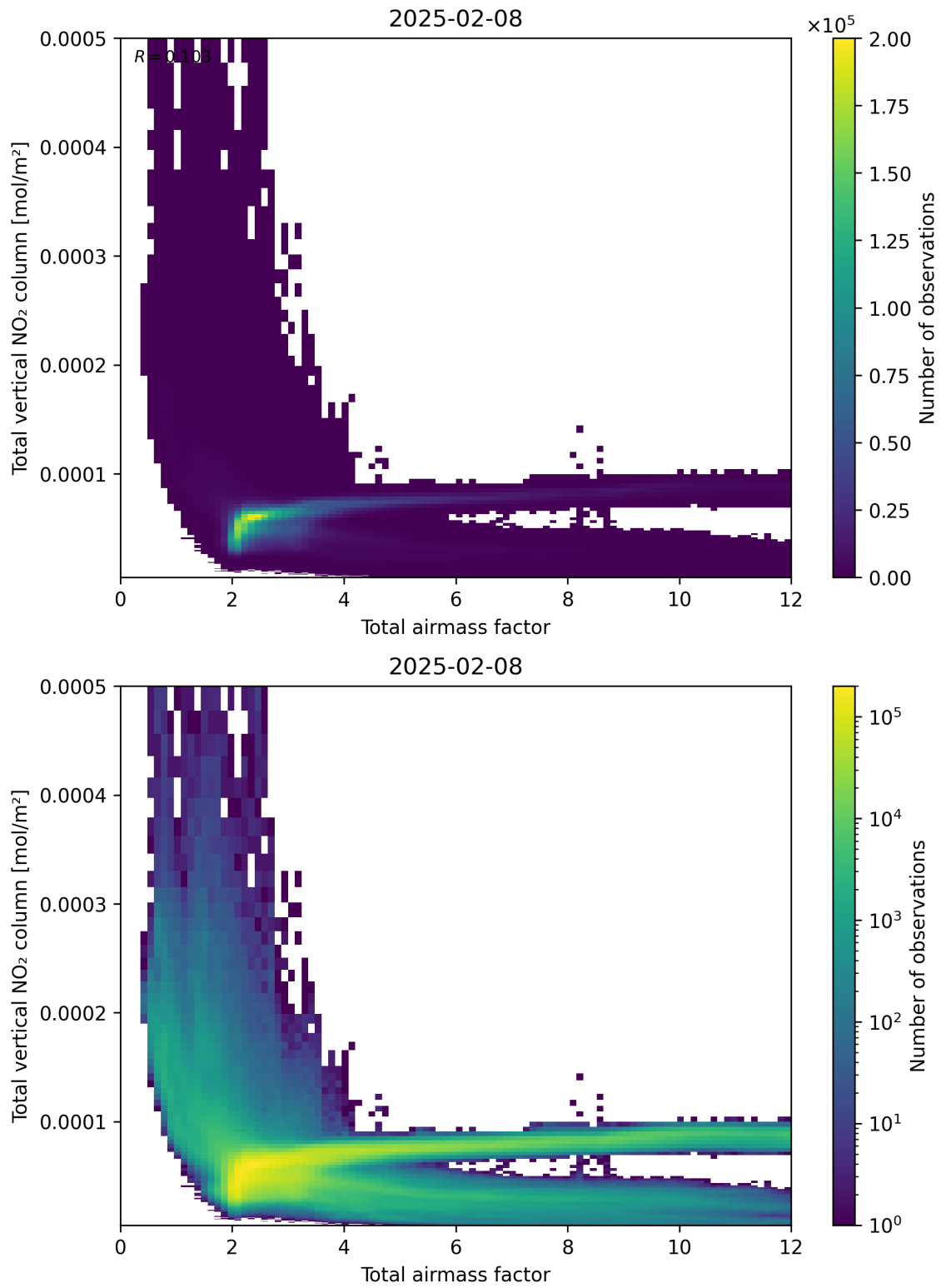
Figure 67: Scatter density plot of “Total airmass factor” against “Total vertical NO 2 column” for 2025-02-08 to 2025-02-09.
