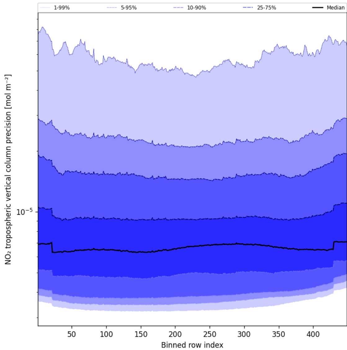
Figure 47: Along track statistics of “NO 2 tropospheric vertical column precision” for 2025-02-08 to 2025-02-09
