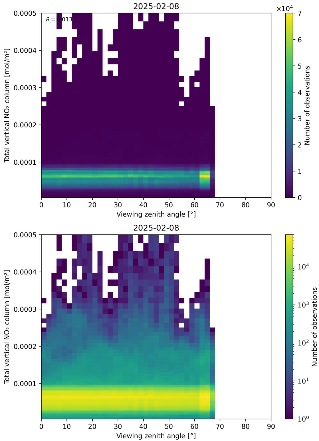
Figure 167: Scatter density plot of “Viewing zenith angle” against “Total vertical NO 2 column” for 2025-02-08 to 2025-02-09.
