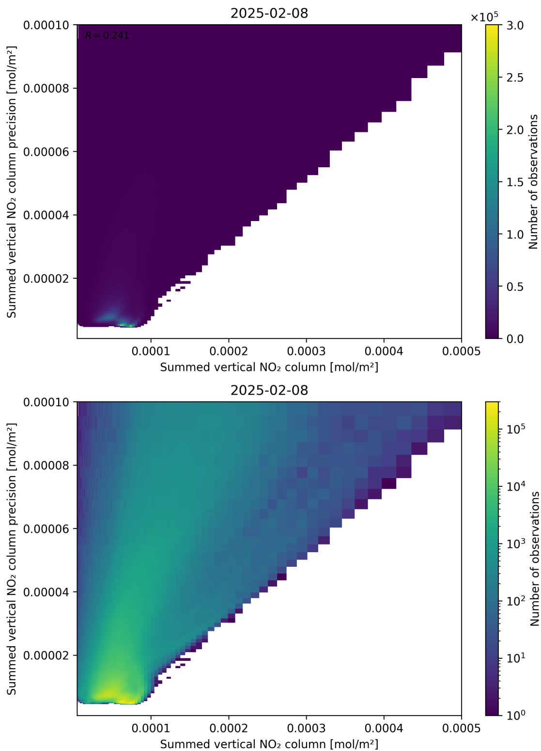
Figure 105: Scatter density plot of “Summed vertical NO 2 column” against “Summed vertical NO 2 column precision” for 2025-02-08 to 2025-02-09.
