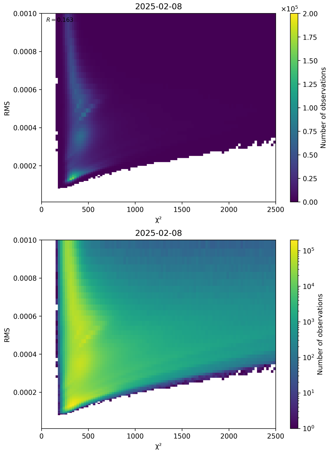
Figure 82: Scatter density plot of “ \chi^2 ” against “RMS” for 2025-02-08 to 2025-02-09.
