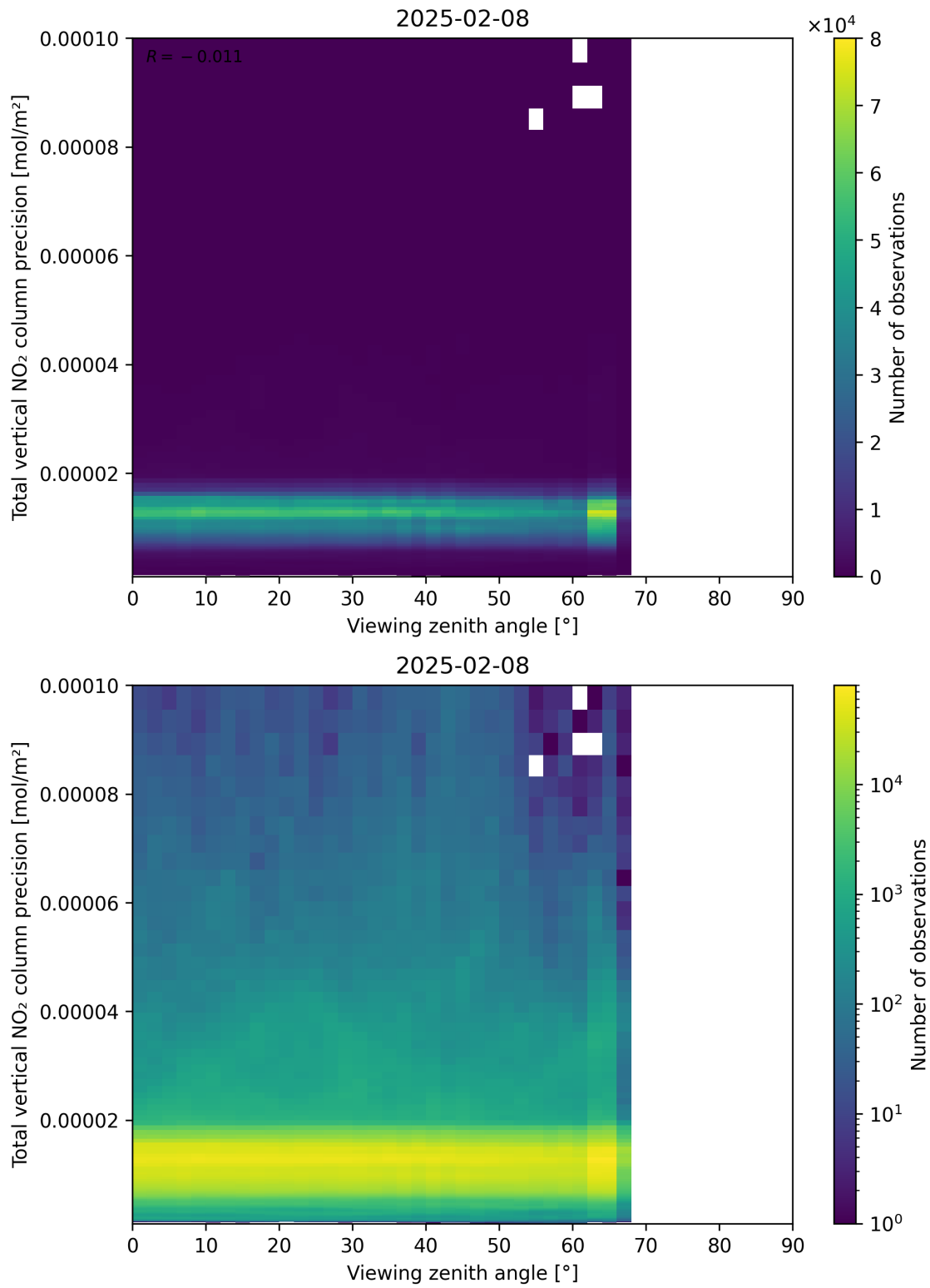
Figure 168: Scatter density plot of “Viewing zenith angle” against “Total vertical NO 2 column precision” for 2025-02-08 to 2025-02-09.
