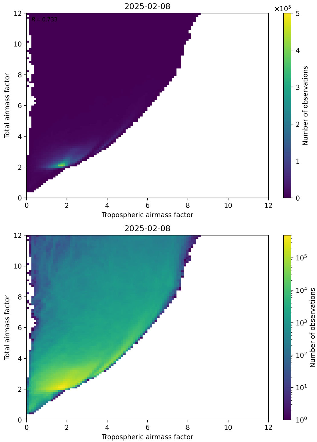
Figure 72: Scatter density plot of “Tropospheric airmass factor” against “Total airmass factor” for 2025-02-08 to 2025-02-09.
