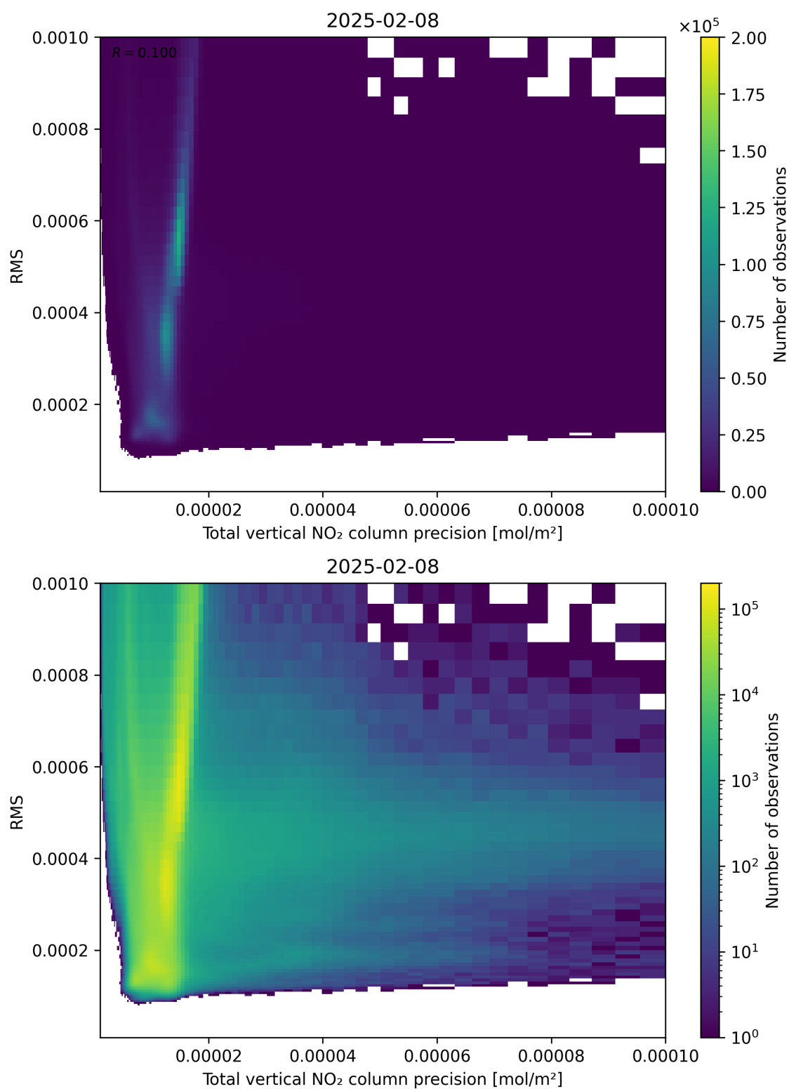
Figure 119: Scatter density plot of “Total vertical NO 2 column precision” against “RMS” for 2025-02-08 to 2025-02-09.
