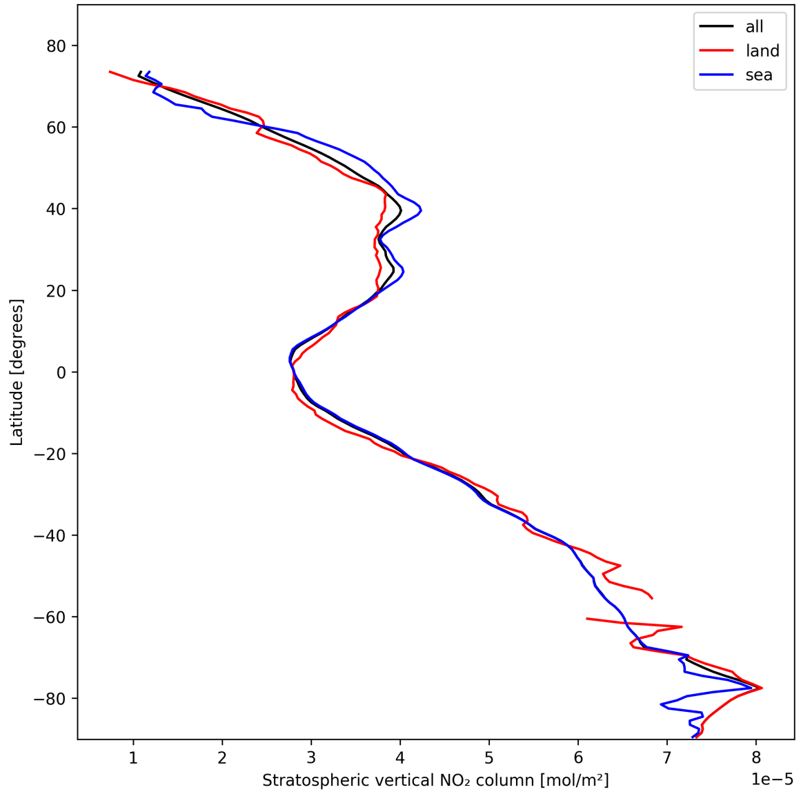
Figure 19: Zonal average of “Stratospheric vertical NO 2 column” for 2025-02-08 to 2025-02-09.
