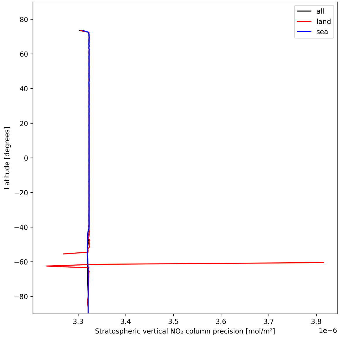
Figure 20: Zonal average of “Stratospheric vertical NO 2 column precision” for 2025-02-08 to 2025-02-09.
