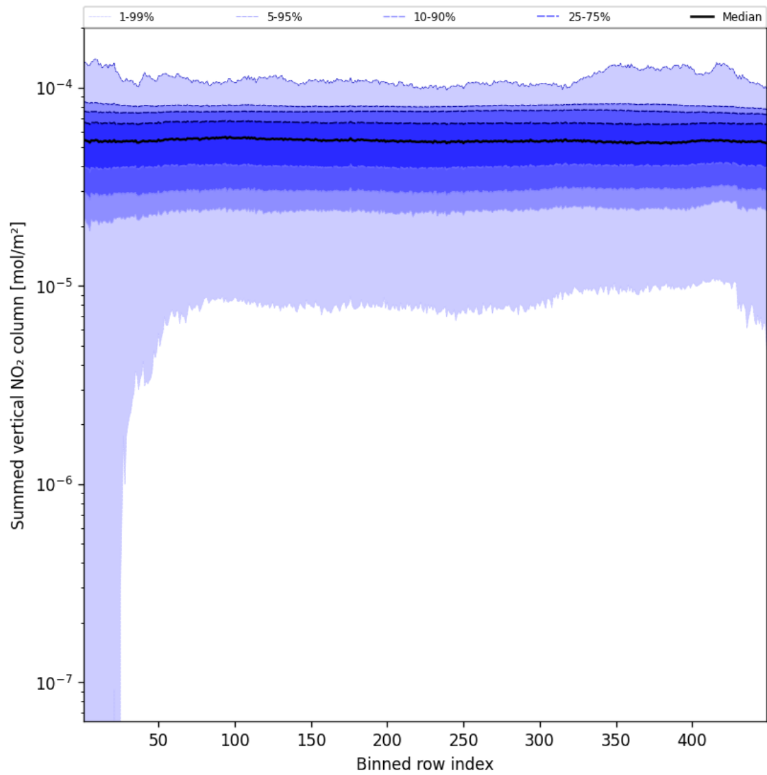
Figure 57: Along track statistics of “Summed vertical NO 2 column” for 2025-02-08 to 2025-02-09
