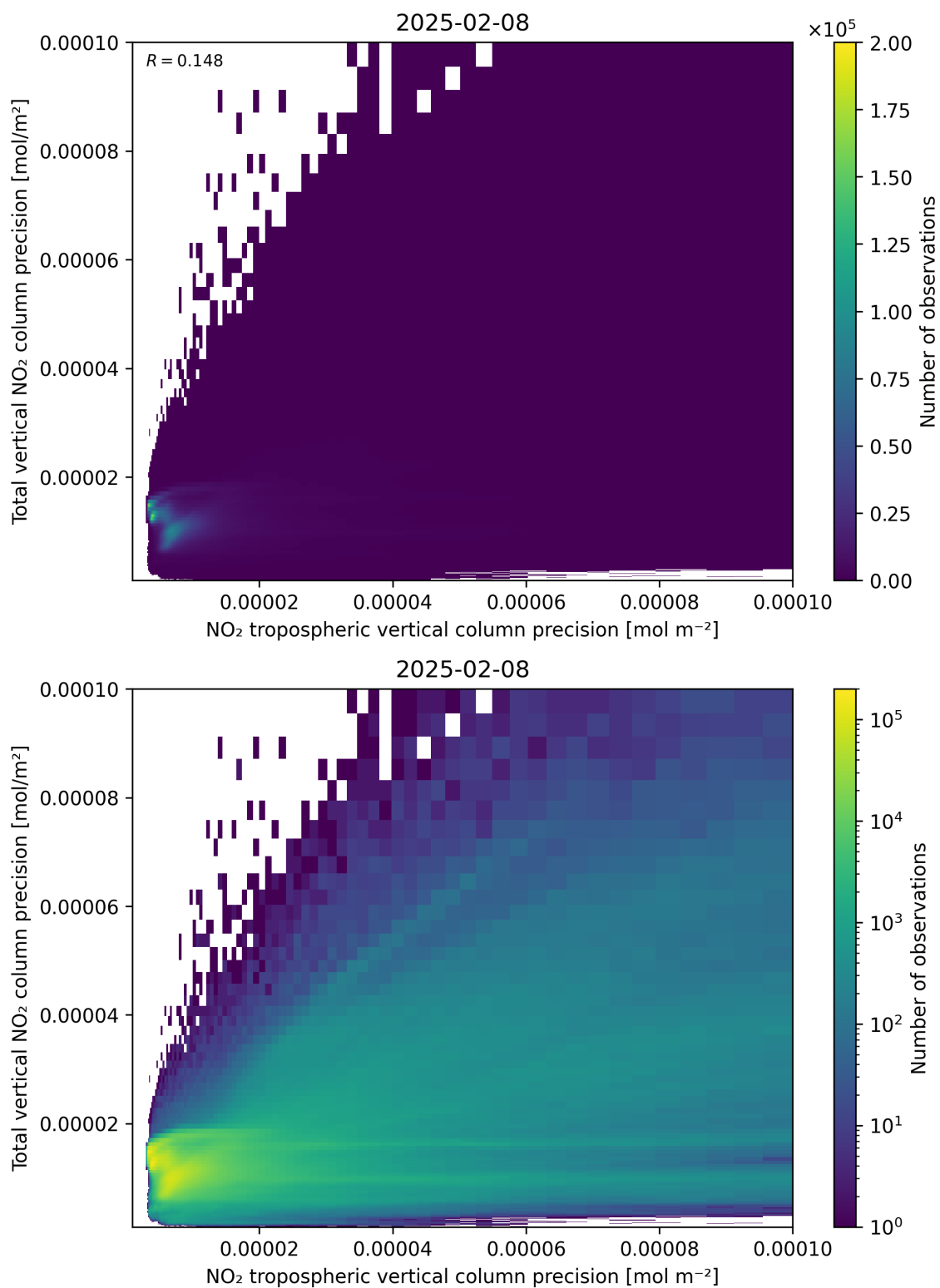
Figure 139: Scatter density plot of “NO 2 tropospheric vertical column precision” against “Total vertical NO 2 column precision” for 2025-02-08 to 2025-02-09.
