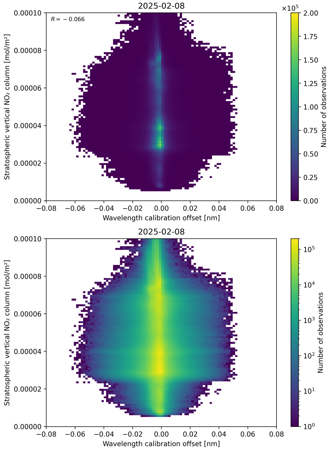
Figure 176: Scatter density plot of “Wavelength calibration offset” against “Stratospheric vertical NO 2 column” for 2025-02-08 to 2025-02-09.
