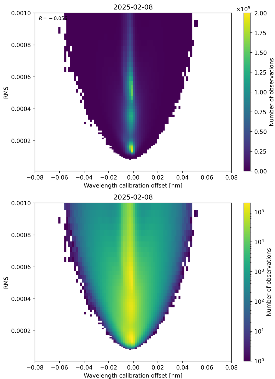
Figure 181: Scatter density plot of “Wavelength calibration offset” against “RMS” for 2025-02-08 to 2025-02-09.
