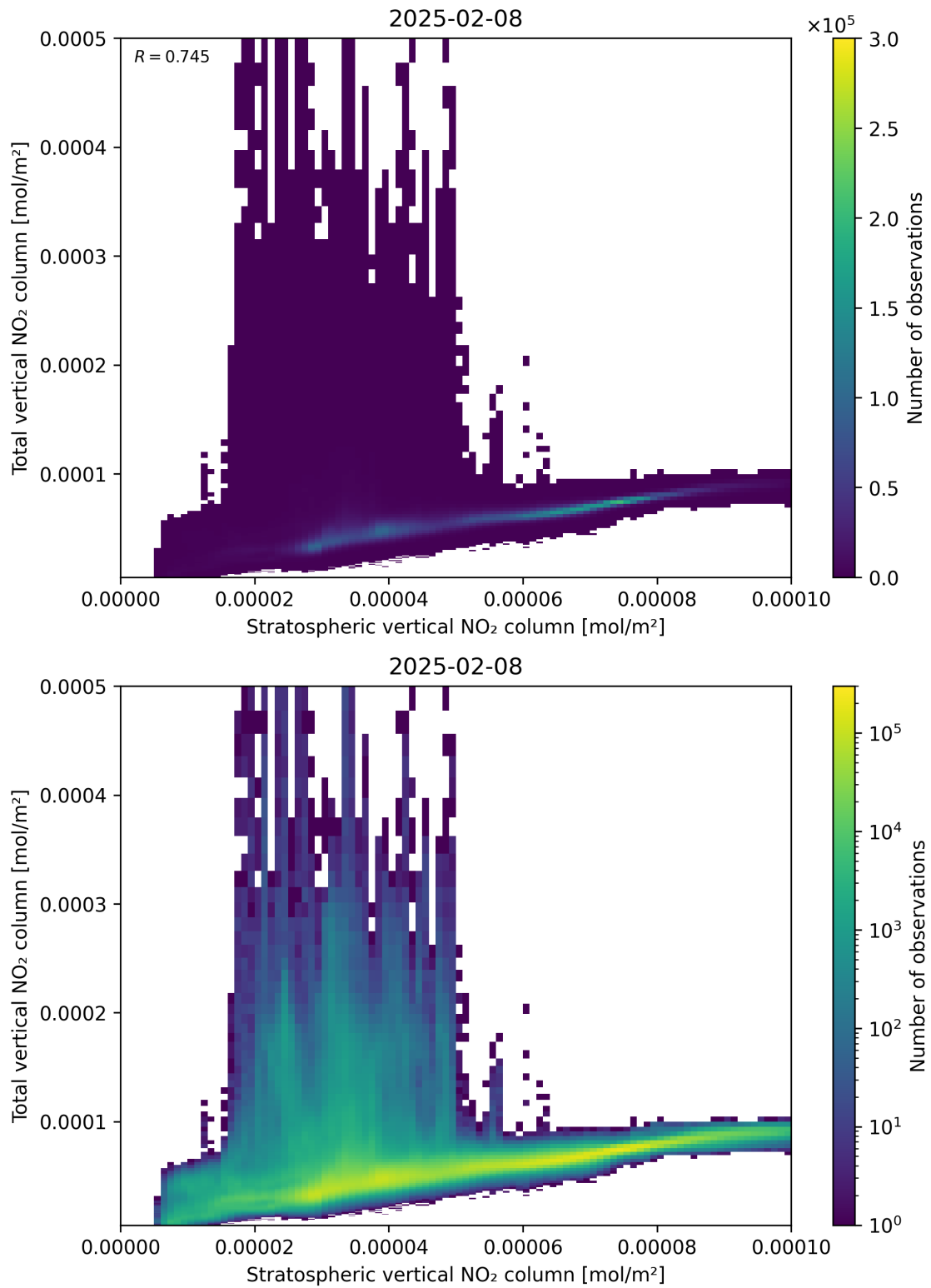
Figure 100: Scatter density plot of “Stratospheric vertical NO 2 column” against “Total vertical NO 2 column” for 2025-02-08 to 2025-02-09.
