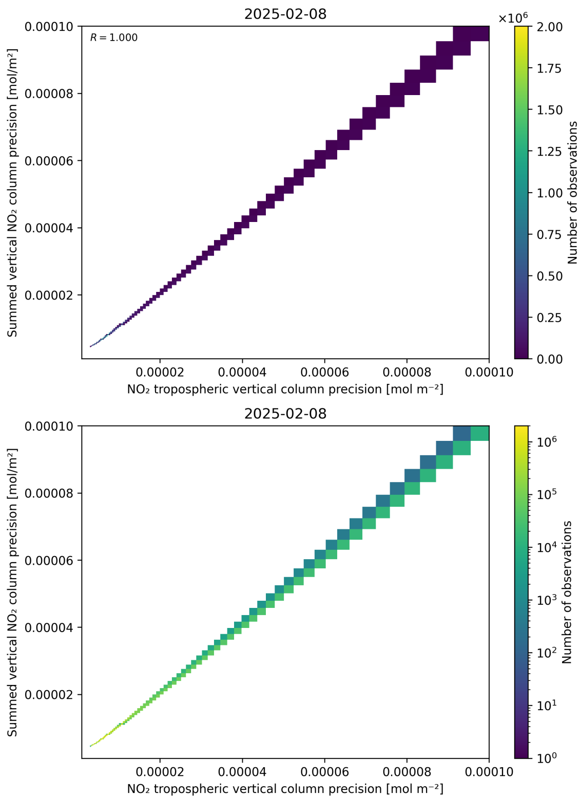
Figure 137: Scatter density plot of “NO 2 tropospheric vertical column precision” against “Summed vertical NO 2 column precision” for 2025-02-08 to 2025-02-09.
