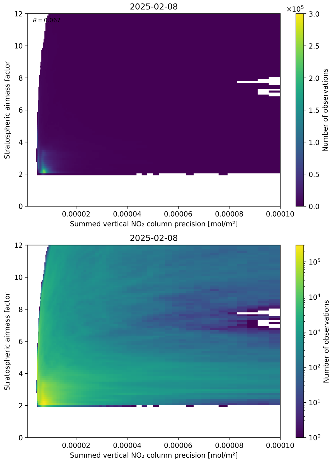
Figure 106: Scatter density plot of “Summed vertical NO 2 column precision” against “Stratospheric airmass factor” for 2025-02-08 to 2025-02-09.
