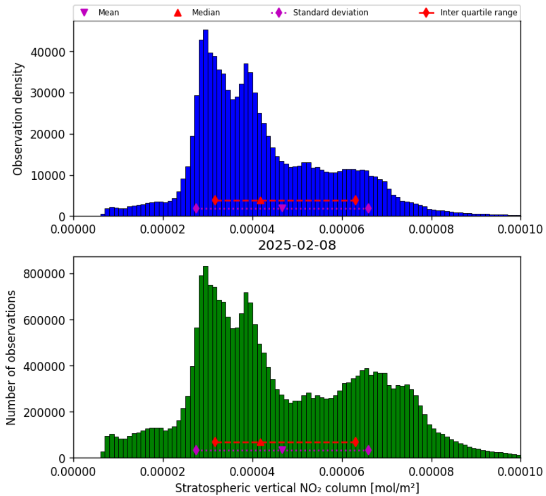
Figure 36: Histogram of “Stratospheric vertical NO 2 column” for 2025-02-08 to 2025-02-09
