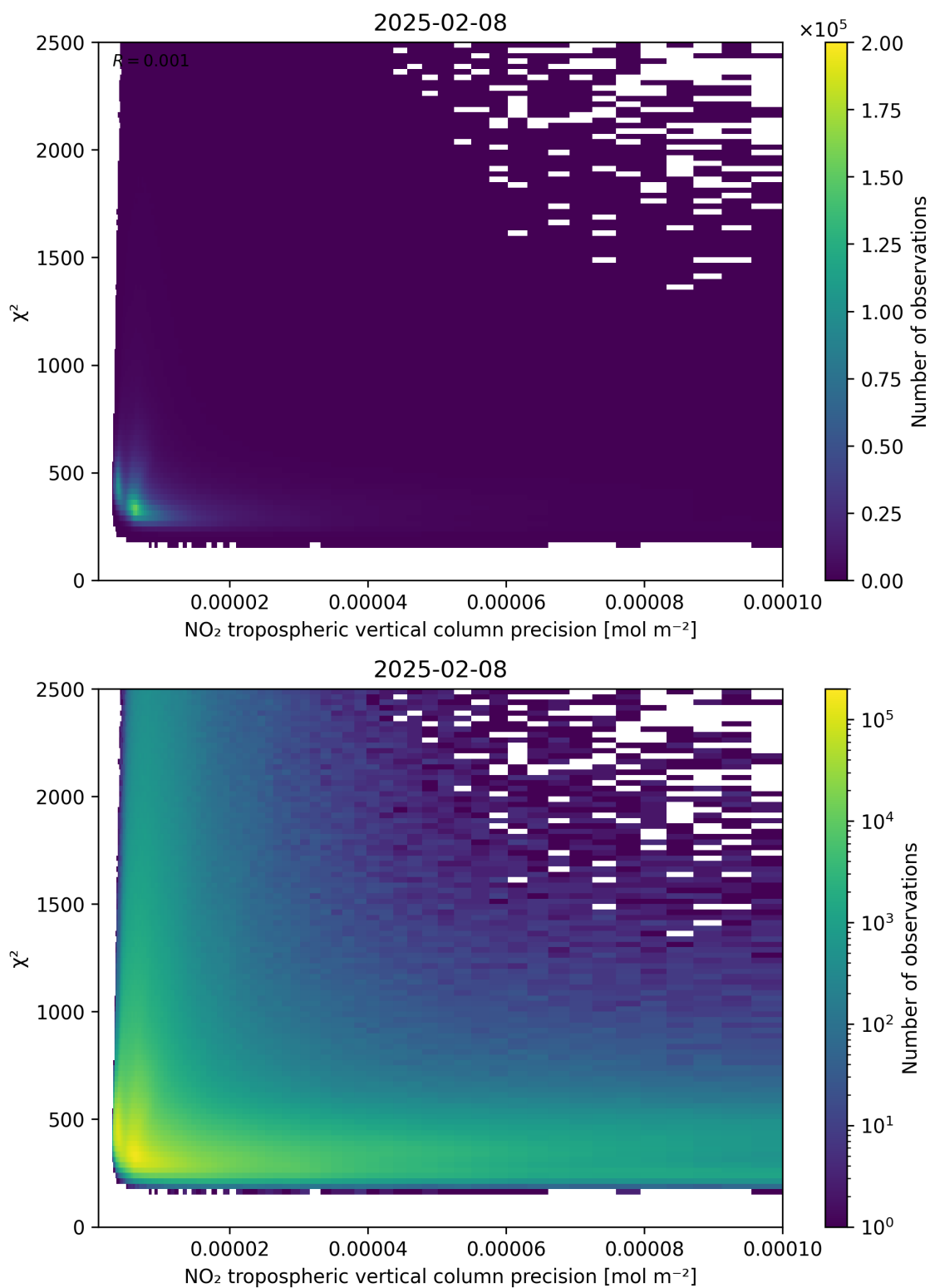
Figure 134: Scatter density plot of “NO 2 tropospheric vertical column precision” against “ \chi^2 ” for 2025-02-08 to 2025-02-09.
