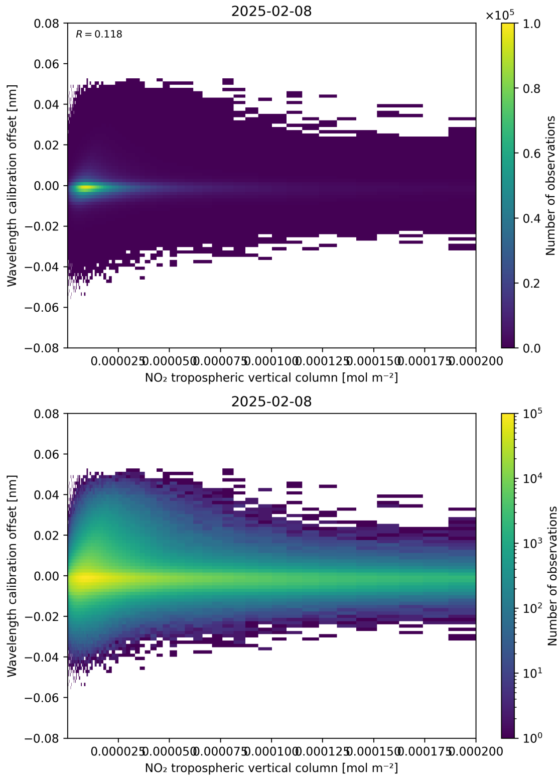
Figure 143: Scatter density plot of “NO 2 tropospheric vertical column” against “Wavelength calibration offset” for 2025-02-08 to 2025-02-09.
