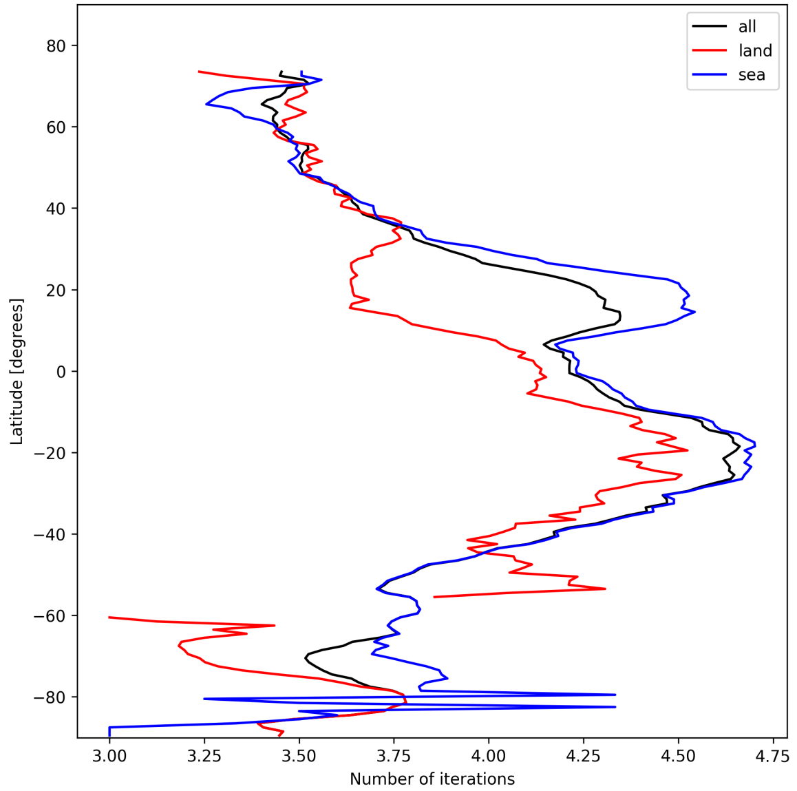
Figure 17: Zonal average of “Number of iterations” for 2025-02-08 to 2025-02-09.
