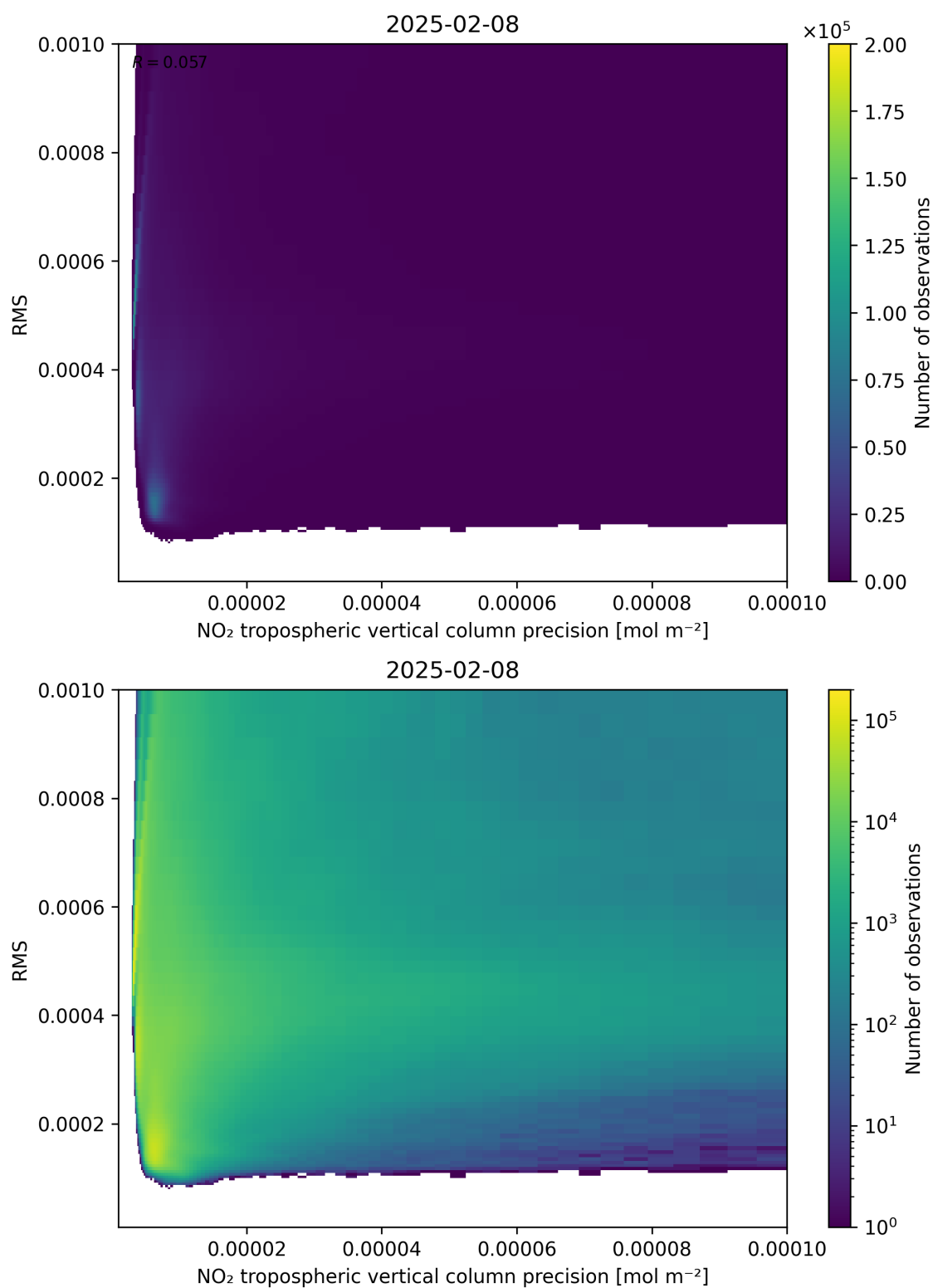
Figure 140: Scatter density plot of “NO 2 tropospheric vertical column precision” against “RMS” for 2025-02-08 to 2025-02-09.
