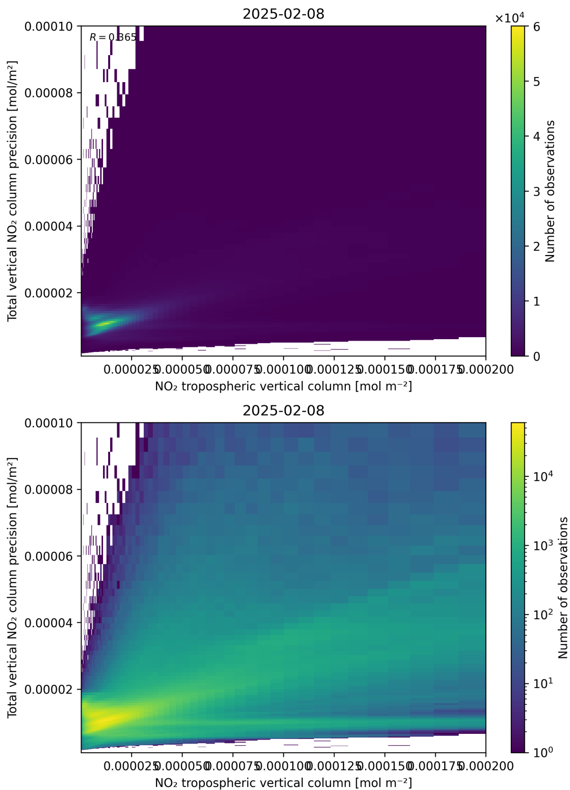
Figure 129: Scatter density plot of “NO 2 tropospheric vertical column” against “Total vertical NO 2 column precision” for 2025-02-08 to 2025-02-09.
