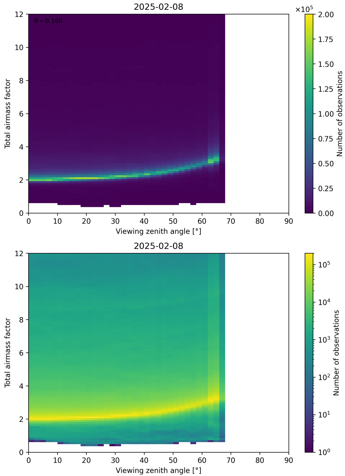
Figure 160: Scatter density plot of “Viewing zenith angle” against “Total airmass factor” for 2025-02-08 to 2025-02-09.
