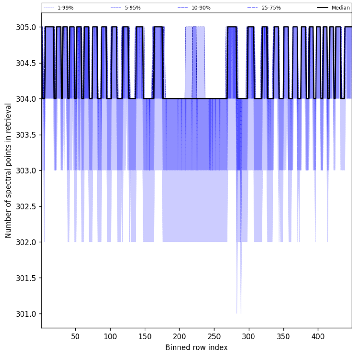
Figure 50: Along track statistics of “Number of spectral points in retrieval” for 2025-02-08 to 2025-02-09
