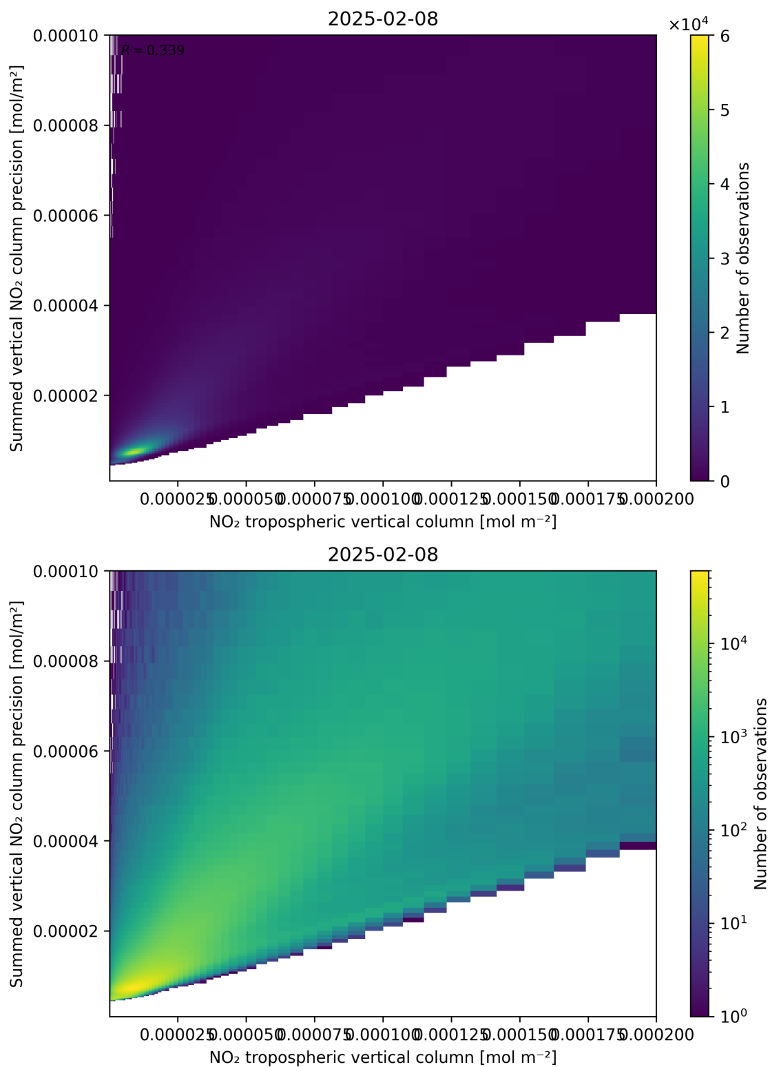
Figure 127: Scatter density plot of “NO 2 tropospheric vertical column” against “Summed vertical NO 2 column precision” for 2025-02-08 to 2025-02-09.
