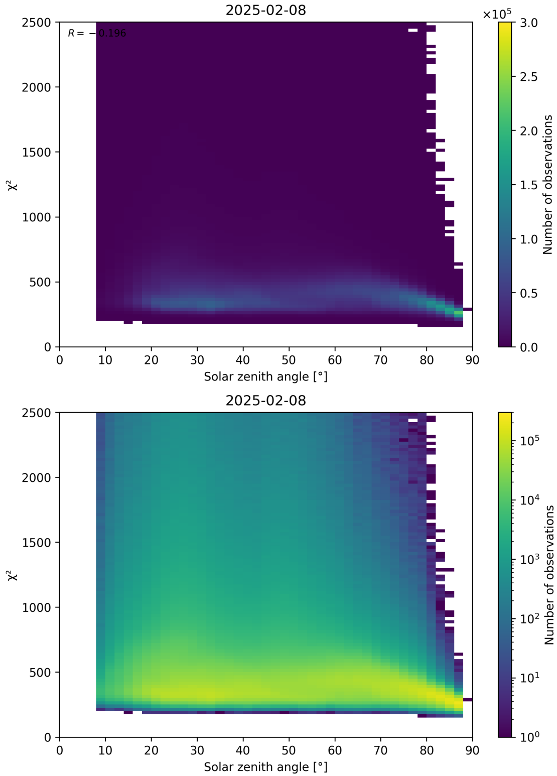
Figure 148: Scatter density plot of “Solar zenith angle” against “ \chi^2 ” for 2025-02-08 to 2025-02-09.
