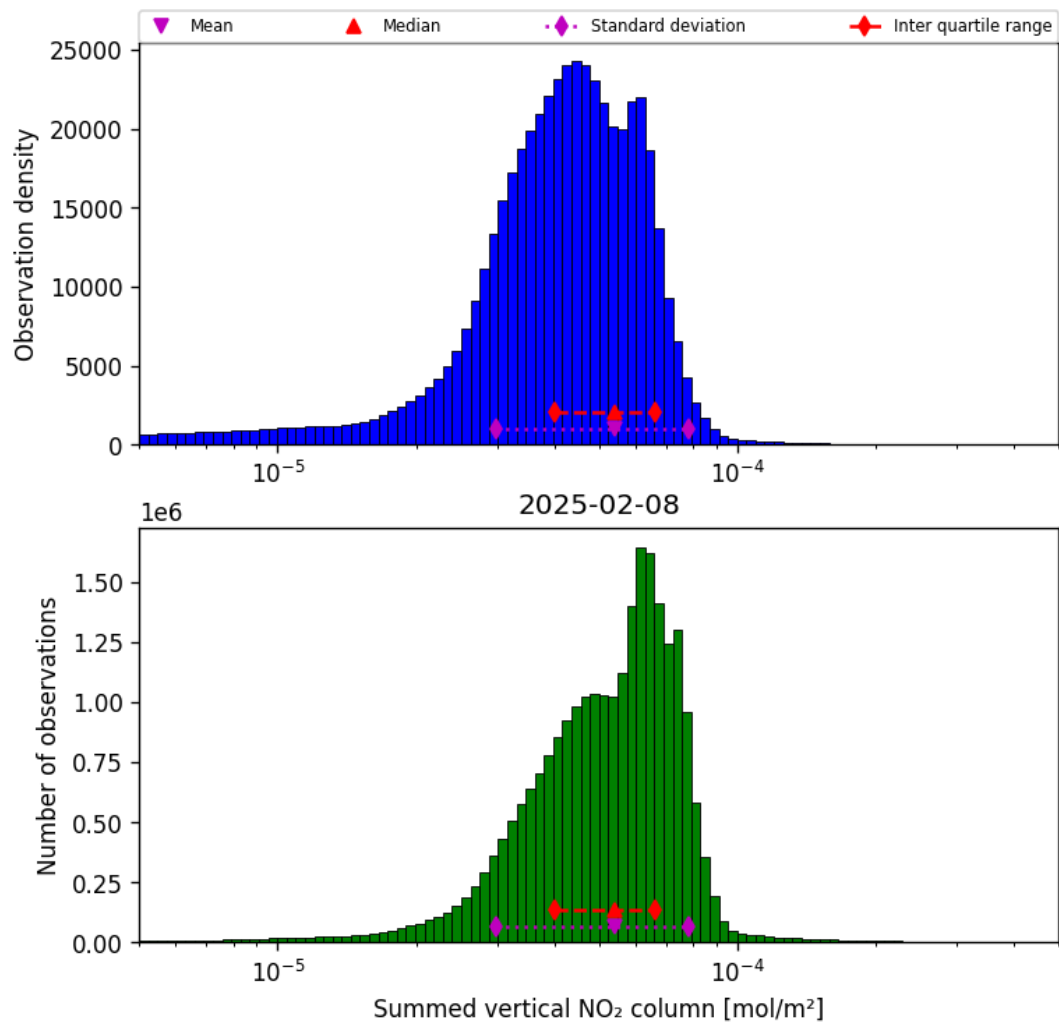
Figure 40: Histogram of "Summed vertical NO 2 column" for 2025-02-08 to 2025-02-09
