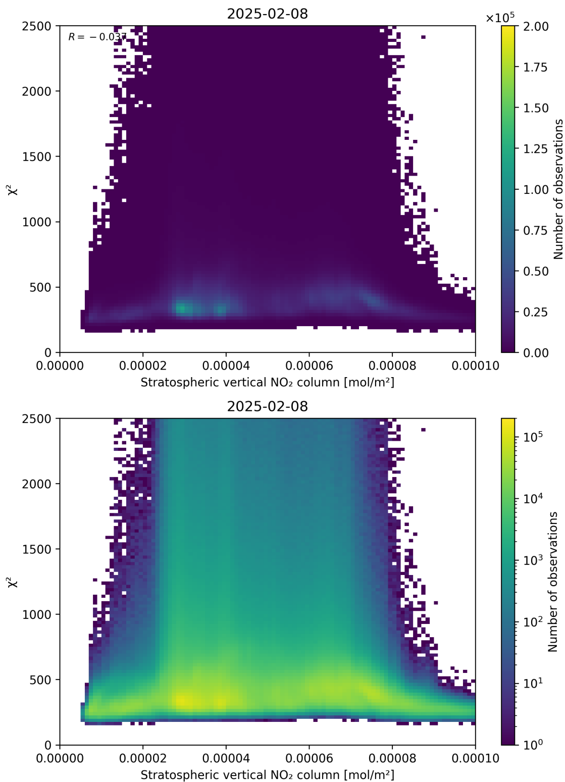
Figure 97: Scatter density plot of “Stratospheric vertical NO 2 column” against “ \chi^2 ” for 2025-02-08 to 2025-02-09.
