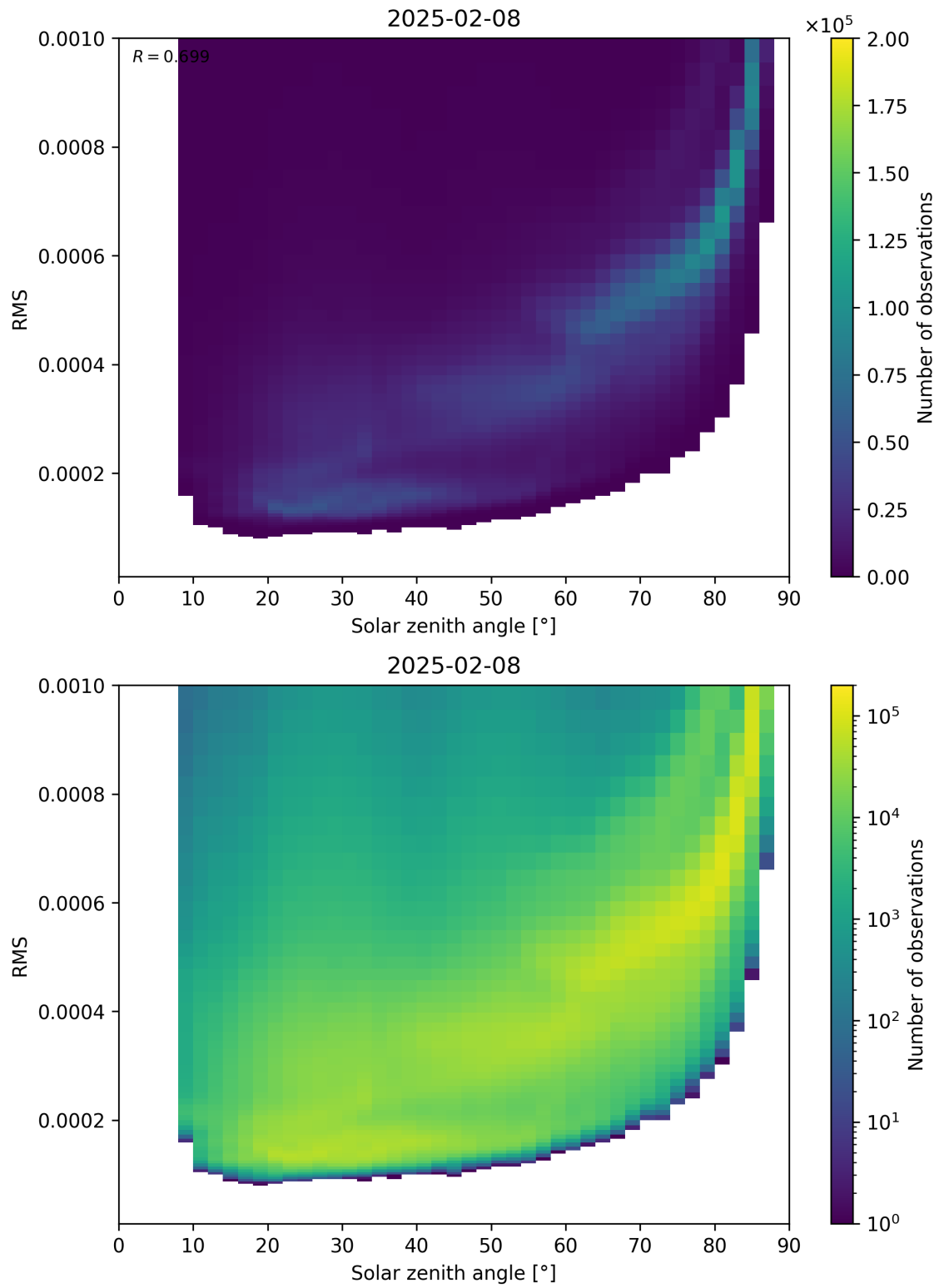
Figure 157: Scatter density plot of “Solar zenith angle” against “RMS” for 2025-02-08 to 2025-02-09.
