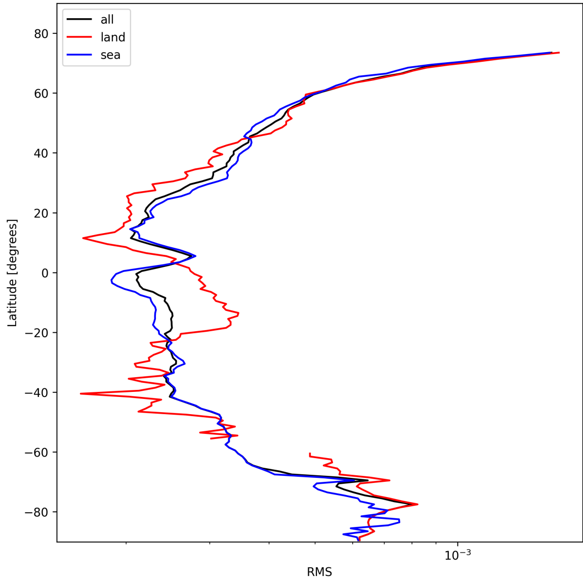
Figure 26: Zonal average of “RMS” for 2025-02-08 to 2025-02-09.
