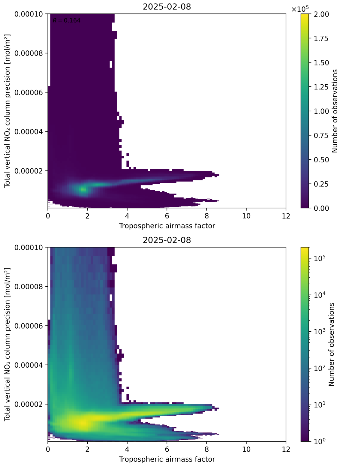
Figure 78: Scatter density plot of “Tropospheric air mass factor” against “Total vertical NO 2 column precision” for 2025-02-08 to 2025-02-09.
