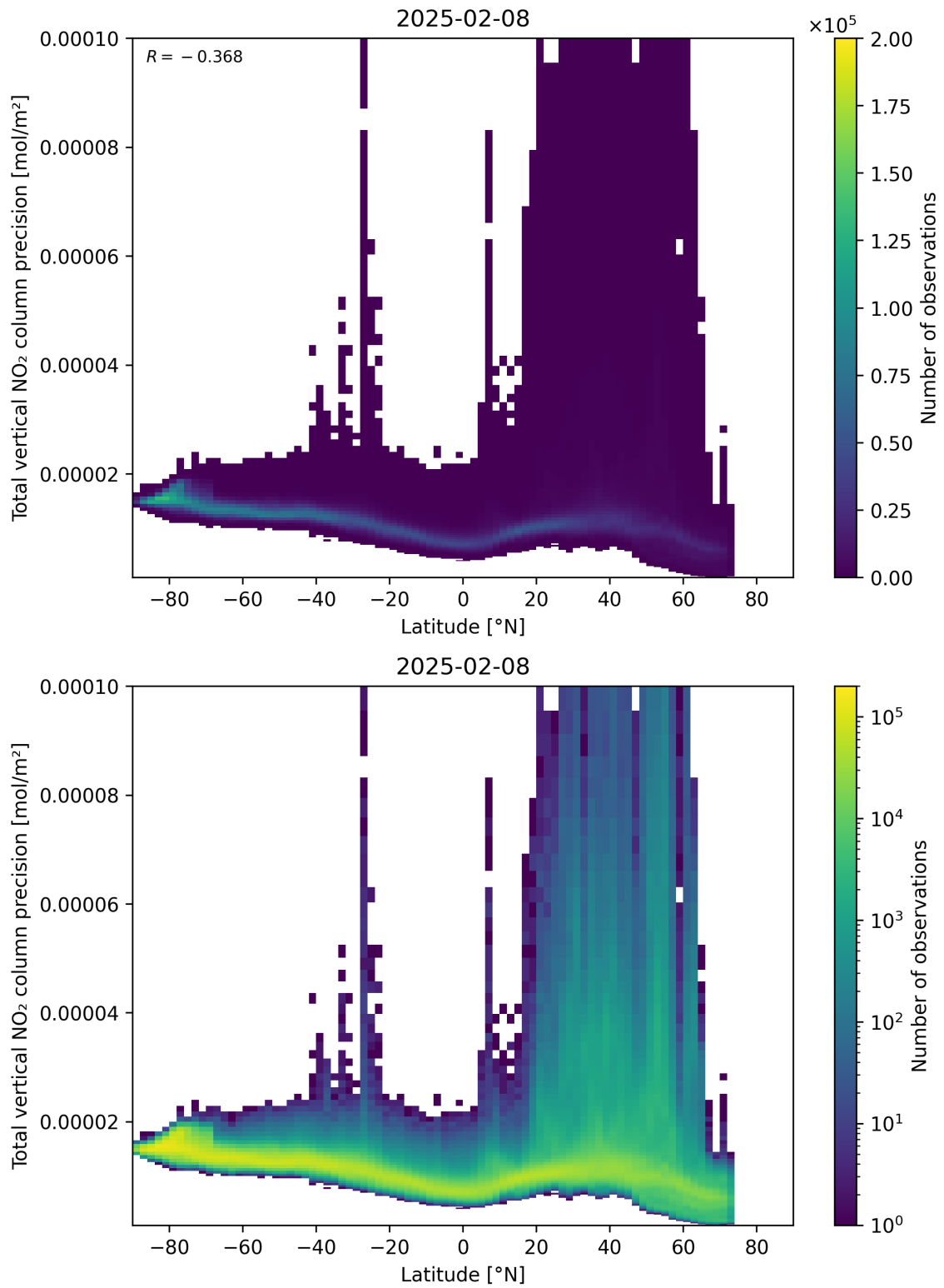
Figure 91: Scatter density plot of “Latitude” against “Total vertical NO 2 column precision” for 2025-02-08 to 2025-02-09.
