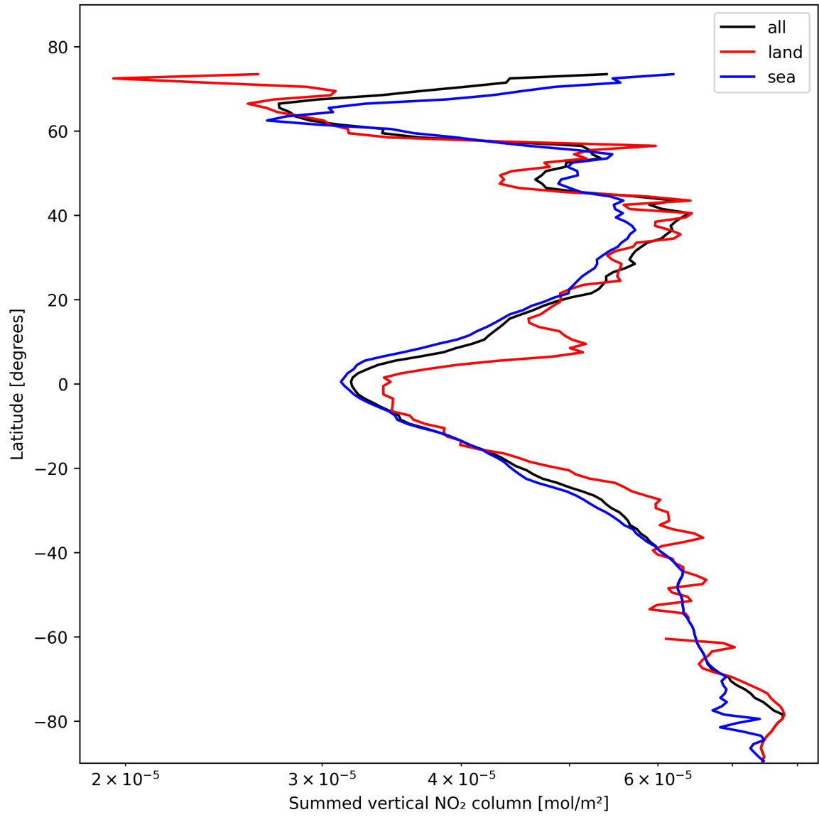
Figure 23: Zonal average of “Summed vertical NO 2 column” for 2025-02-08 to 2025-02-09.
