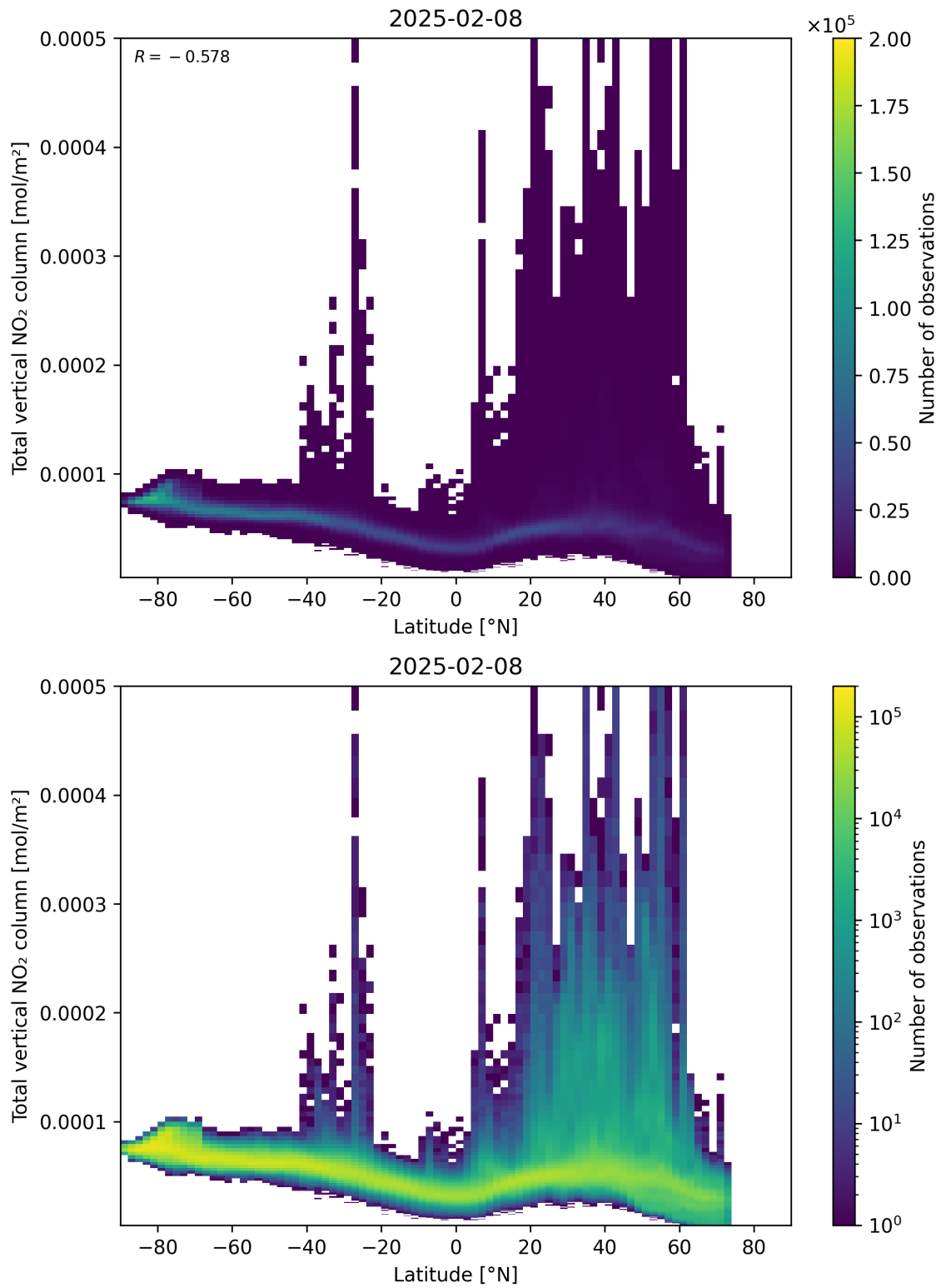
Figure 90: Scatter density plot of “Latitude” against “Total vertical NO 2 column” for 2025-02-08 to 2025-02-09.
