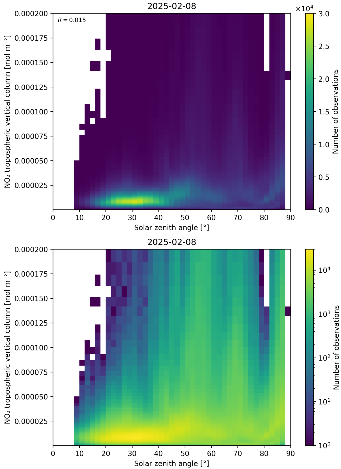
Figure 155: Scatter density plot of “Solar zenith angle” against “NO 2 tropospheric vertical column” for 2025-02-08 to 2025-02-09.
