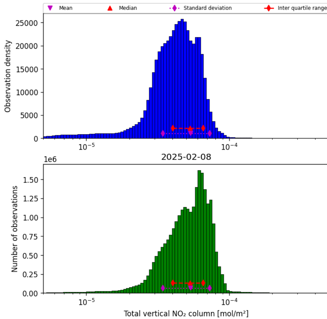
Figure 38: Histogram of “Total vertical NO 2 column” for 2025-02-08 to 2025-02-09
