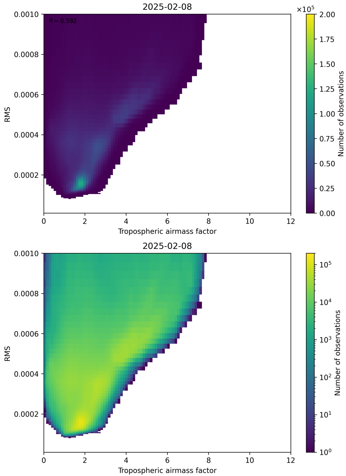
Figure 79: Scatter density plot of “Tropospheric airmass factor” against “RMS” for 2025-02-08 to 2025-02-09.
