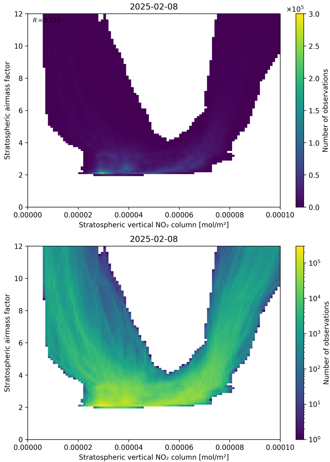
Figure 96: Scatter density plot of “Stratospheric vertical NO 2 column” against “Stratospheric airmass factor” for 2025-02-08 to 2025-02-09.
