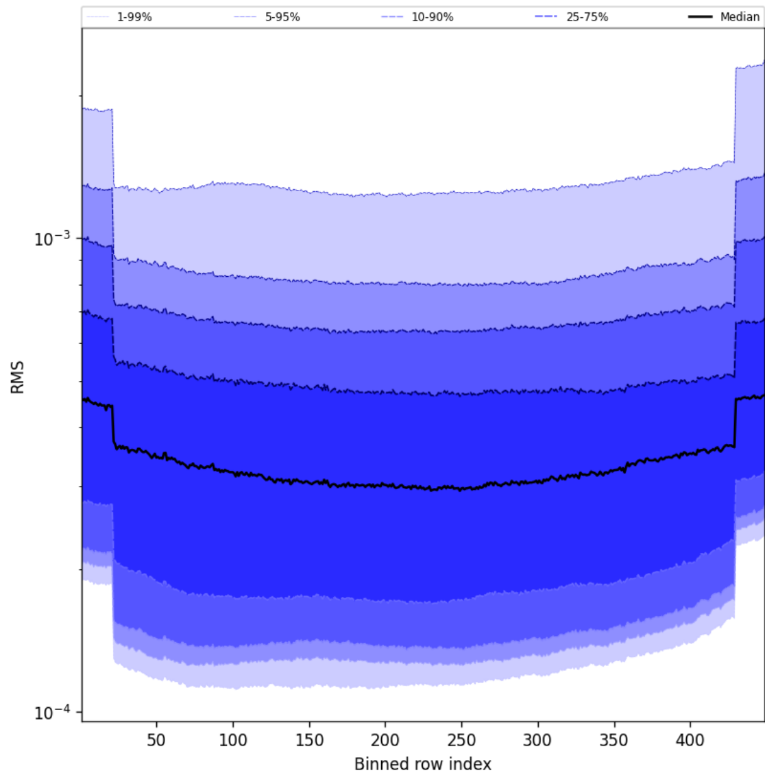
Figure 60: Along track statistics of “RMS” for 2025-02-08 to 2025-02-09
