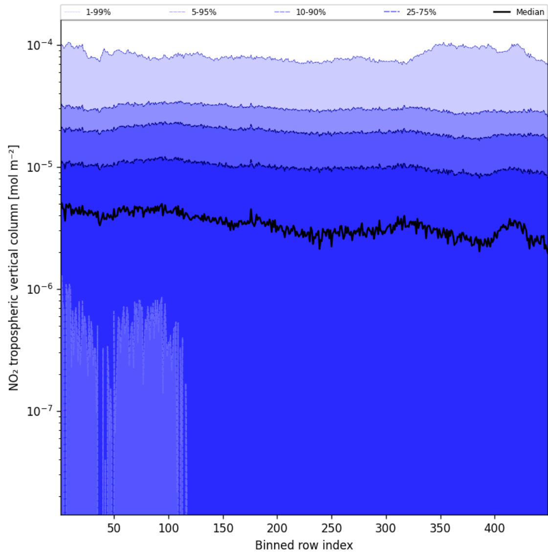
Figure 46: Along track statistics of “NO 2 tropospheric vertical column” for 2025-02-08 to 2025-02-09
