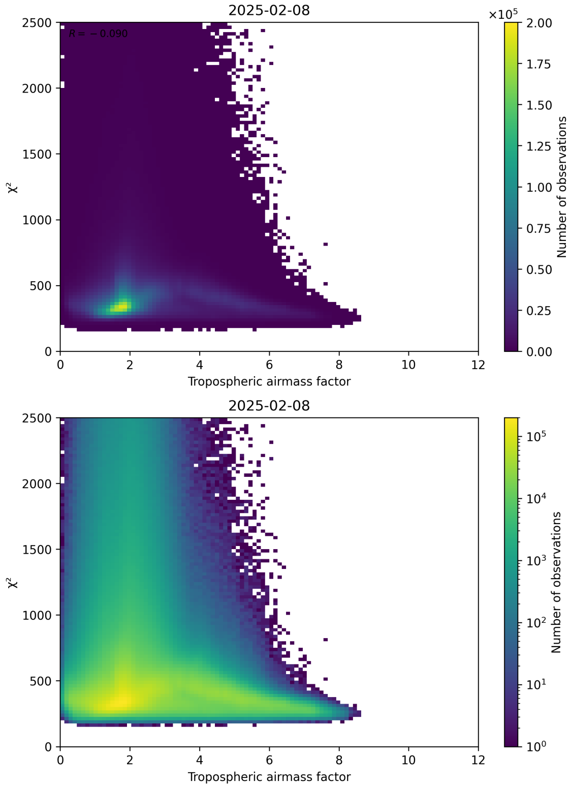
Figure 73: Scatter density plot of “Tropospheric airmass factor” against “ \chi^2 ” for 2025-02-08 to 2025-02-09.
