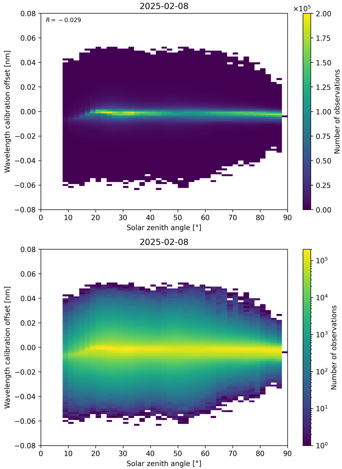
Figure 158: Scatter density plot of “Solar zenith angle” against “Wavelength calibration offset” for 2025-02-08 to 2025-02-09.
