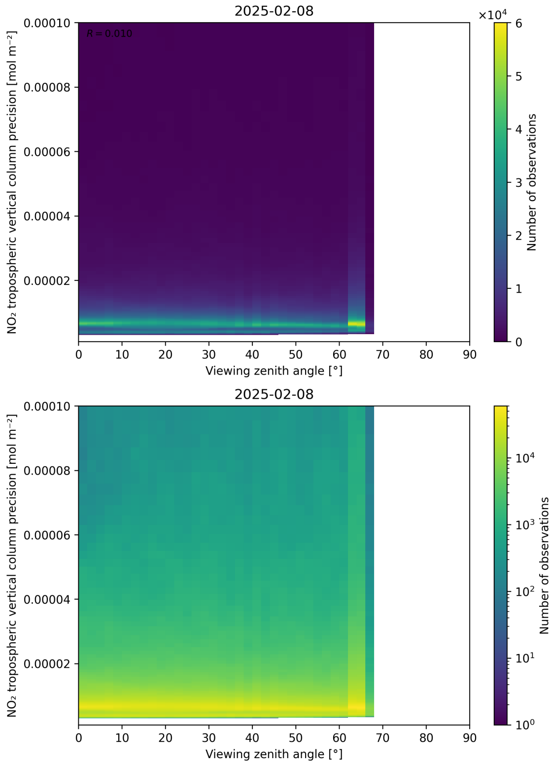
Figure 170: Scatter density plot of “Viewing zenith angle” against “NO 2 tropospheric vertical column precision” for 2025-02-08 to 2025-02-09.
