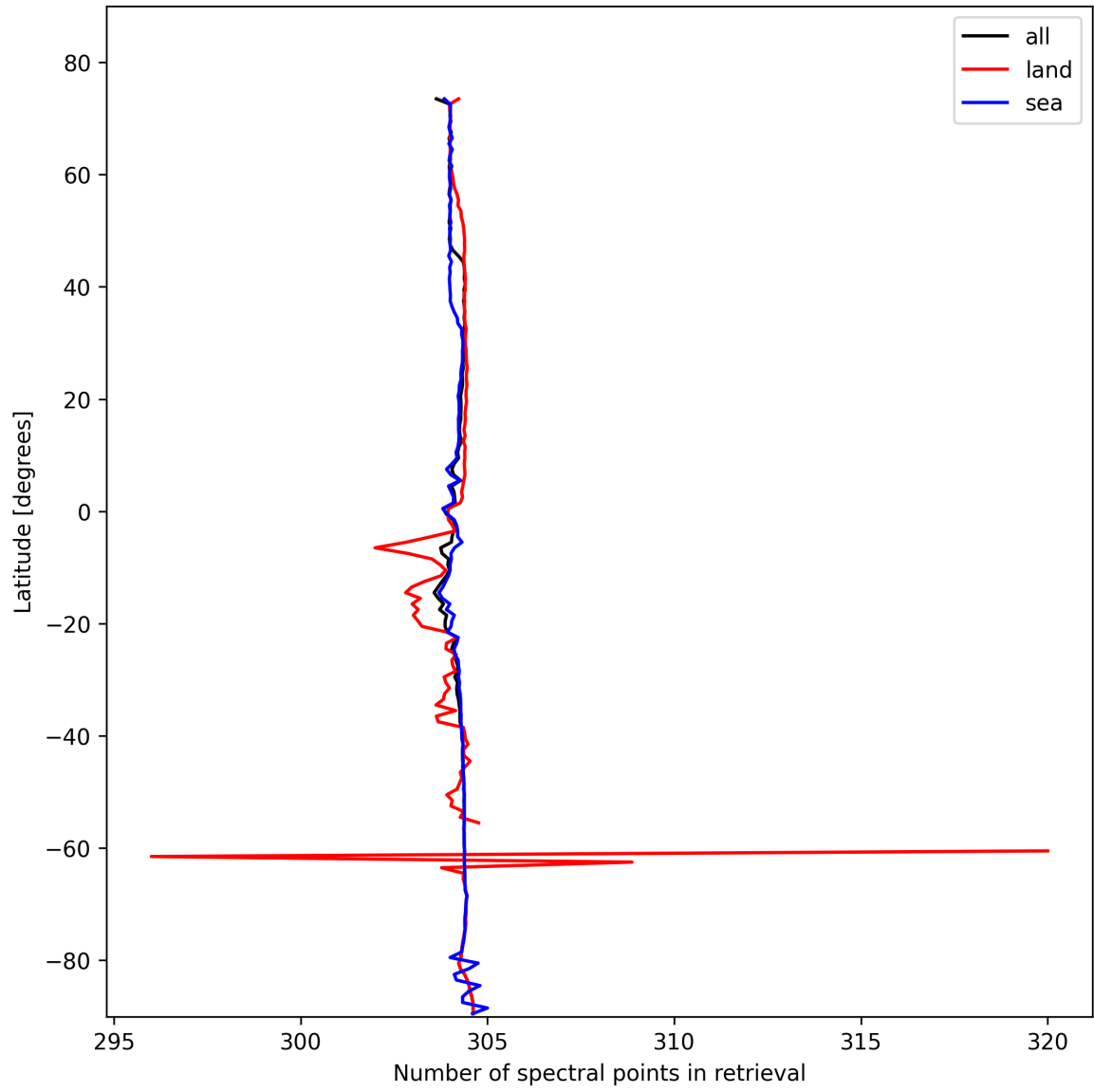
Figure 16: Zonal average of “Number of spectral points in retrieval” for 2025-02-08 to 2025-02-09.
