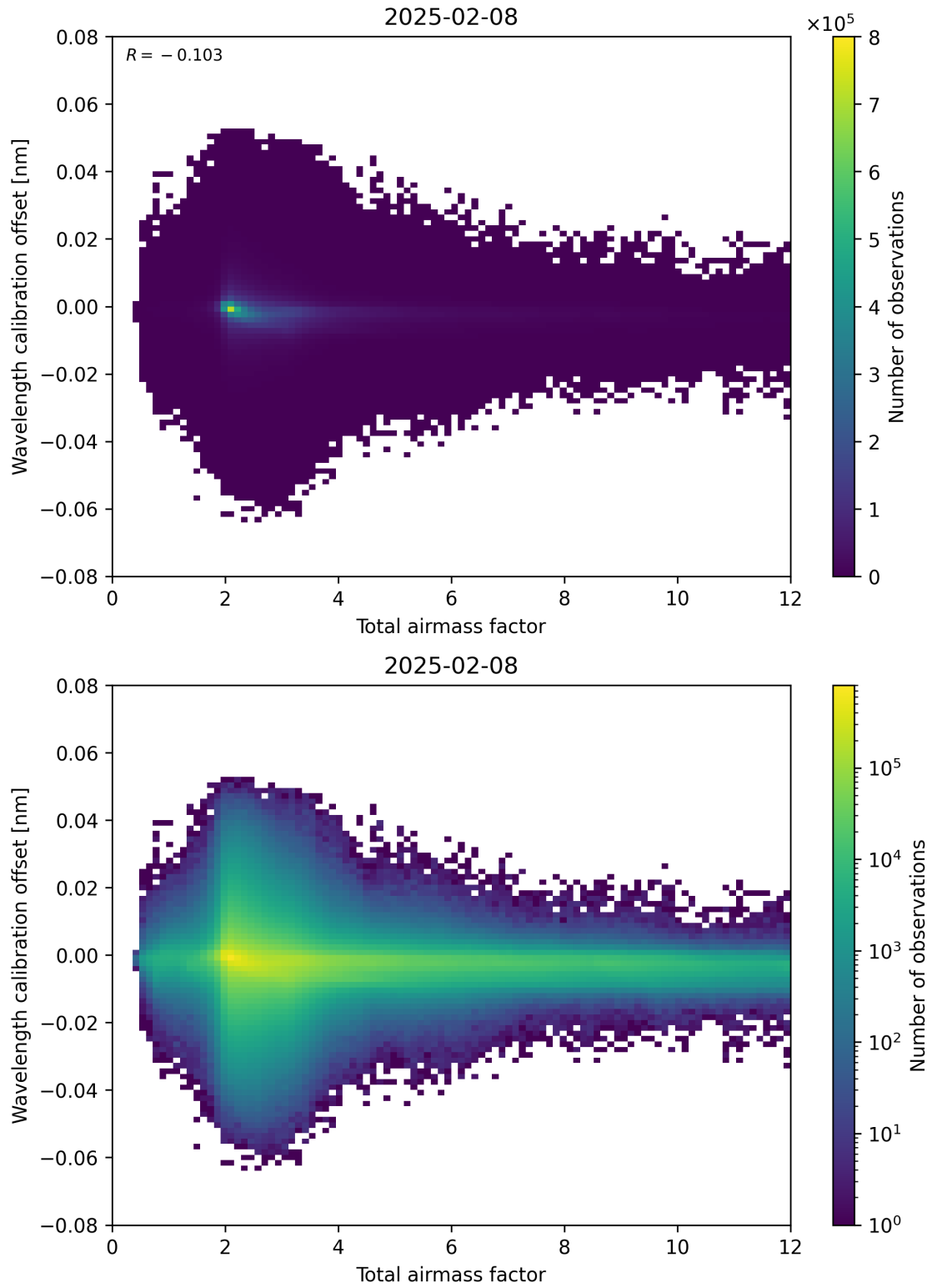
Figure 70: Scatter density plot of “Total airmass factor” against “Wavelength calibration offset” for 2025-02-08 to 2025-02-09.
