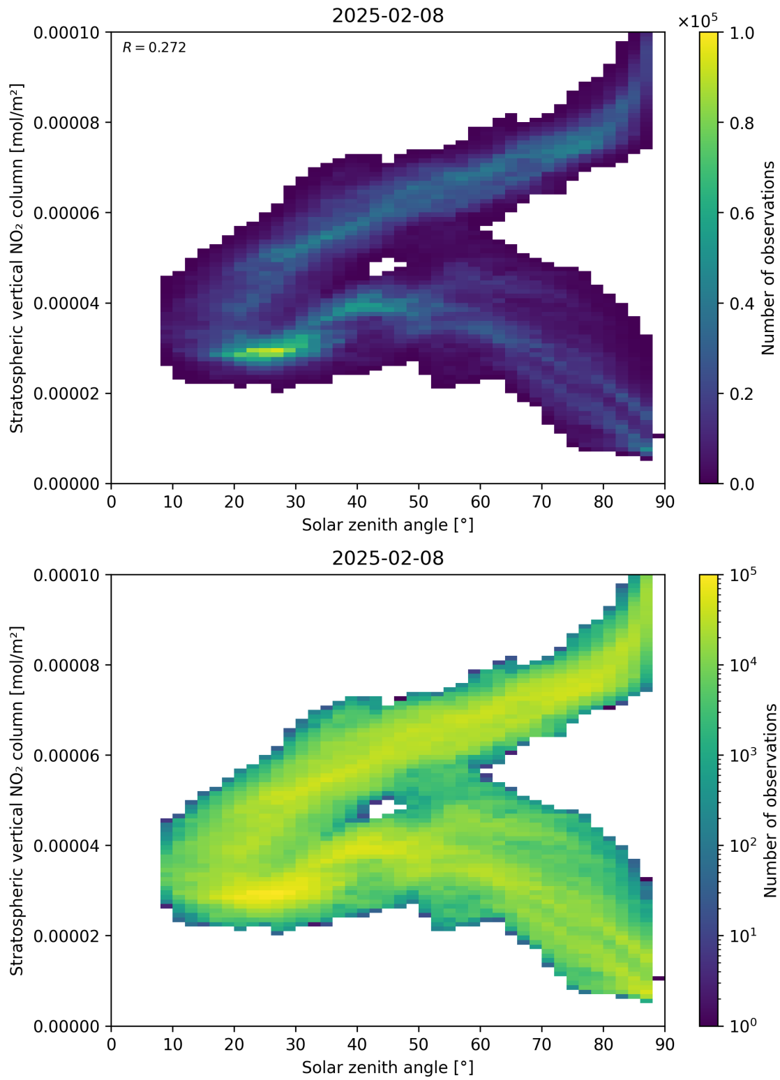
Figure 150: Scatter density plot of “Solar zenith angle” against “Stratospheric vertical NO 2 column” for 2025-02-08 to 2025-02-09.
