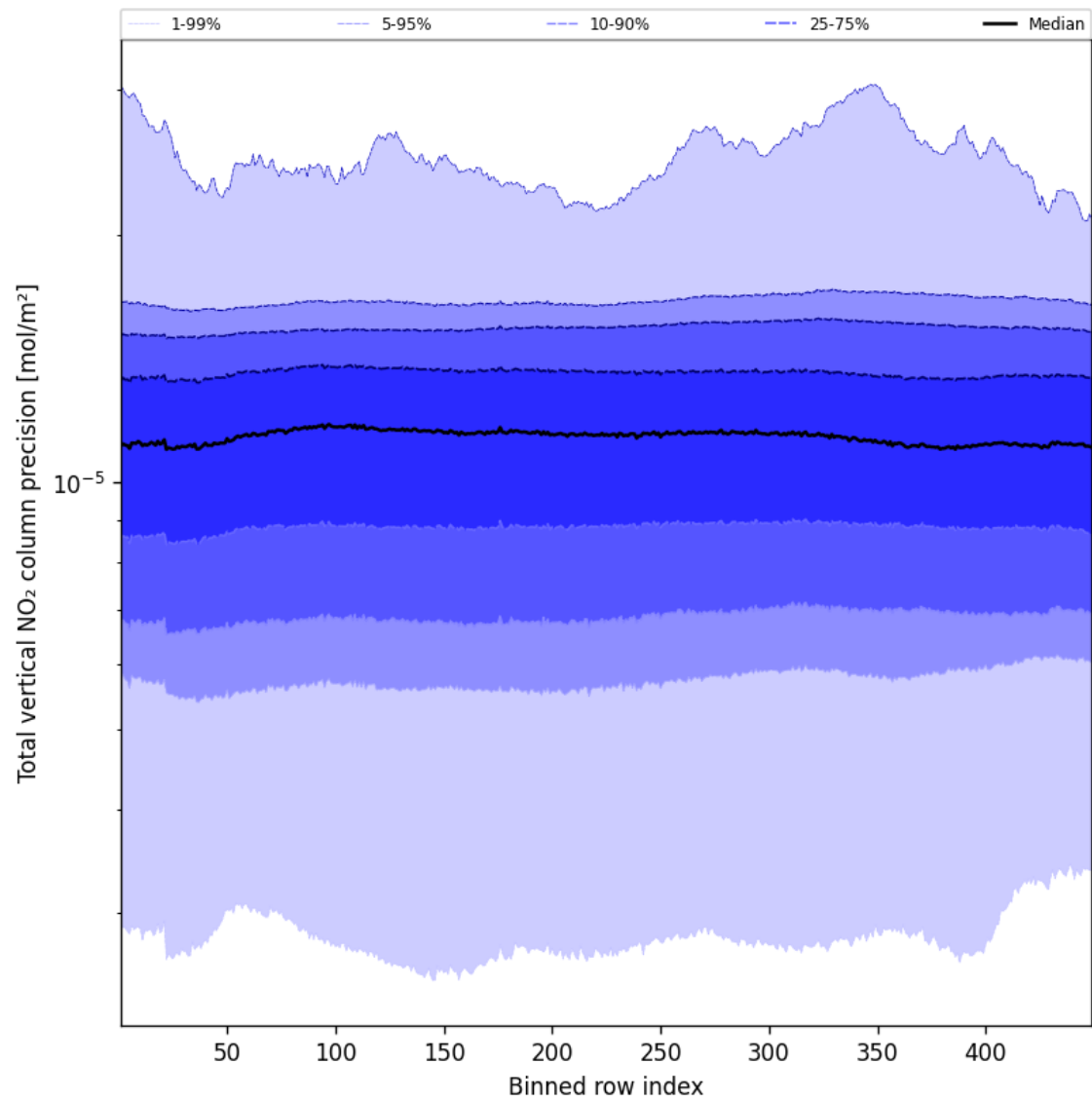
Figure 56: Along track statistics of “Total vertical NO 2 column precision” for 2025-02-08 to 2025-02-09
