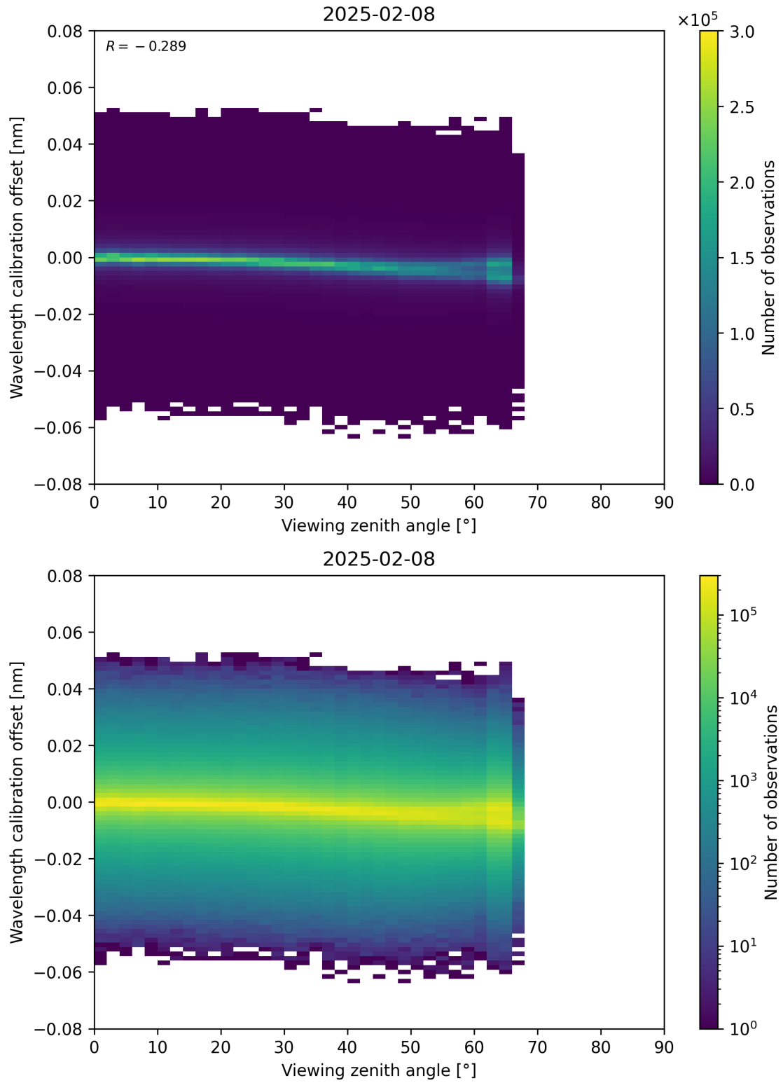
Figure 173: Scatter density plot of “Viewing zenith angle” against “Wavelength calibration offset” for 2025-02-08 to 2025-02-09.
