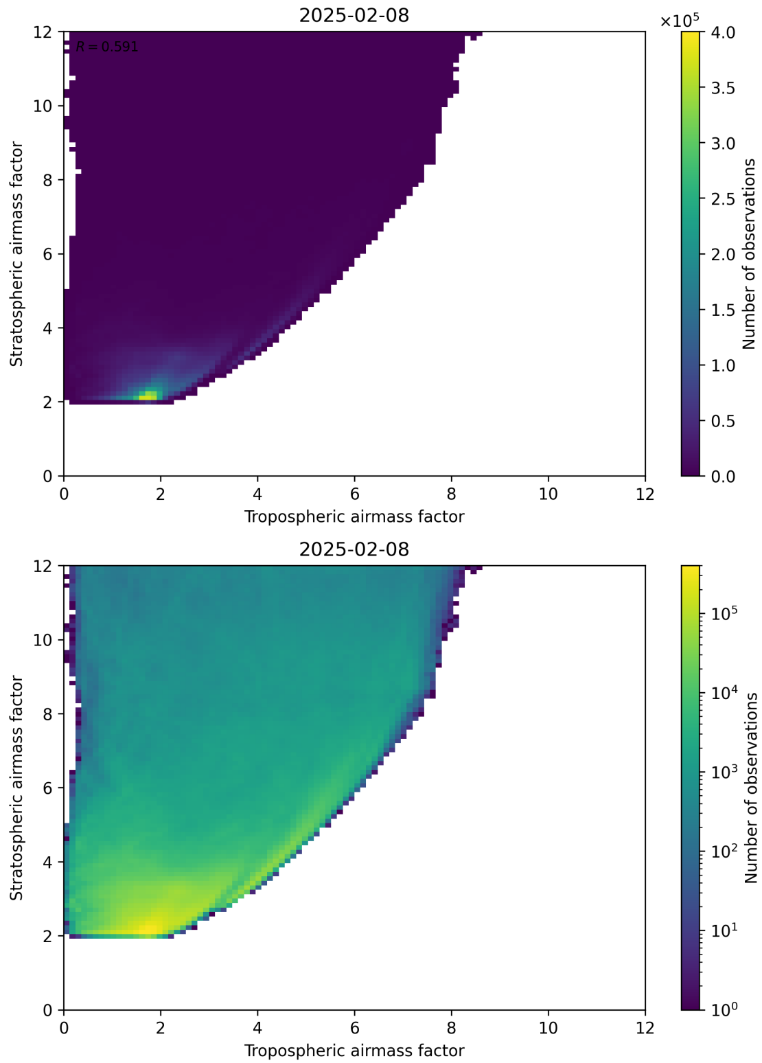
Figure 71: Scatter density plot of “Tropospheric airmass factor” against “Stratospheric airmass factor” for 2025-02-08 to 2025-02-09.
