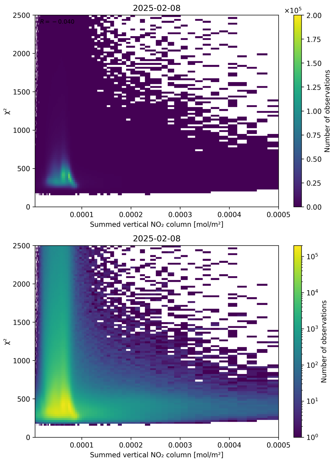
Figure 104: Scatter density plot of “Summed vertical NO 2 column” against “ \chi^2 ” for 2025-02-08 to 2025-02-09.
