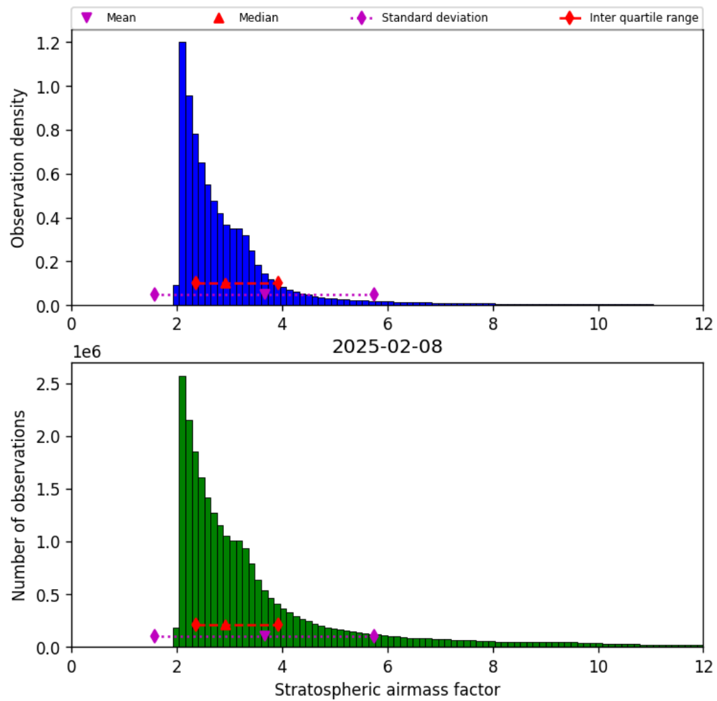
Figure 44: Histogram of “Stratospheric airmass factor” for 2025-02-08 to 2025-02-09
