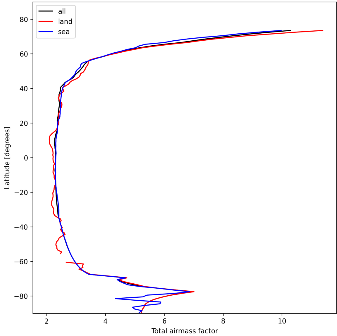
Figure 15: Zonal average of “Total airmass factor” for 2025-02-08 to 2025-02-09.
