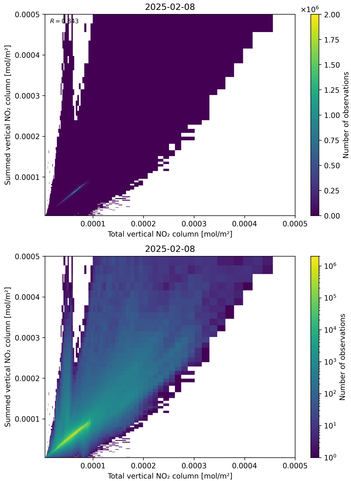
Figure 112: Scatter density plot of “Total vertical NO 2 column” against “Summed vertical NO 2 column” for 2025-02-08 to 2025-02-09.
