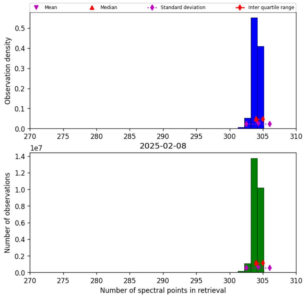
Figure 33: Histogram of “Number of spectral points in retrieval” for 2025-02-08 to 2025-02-09
