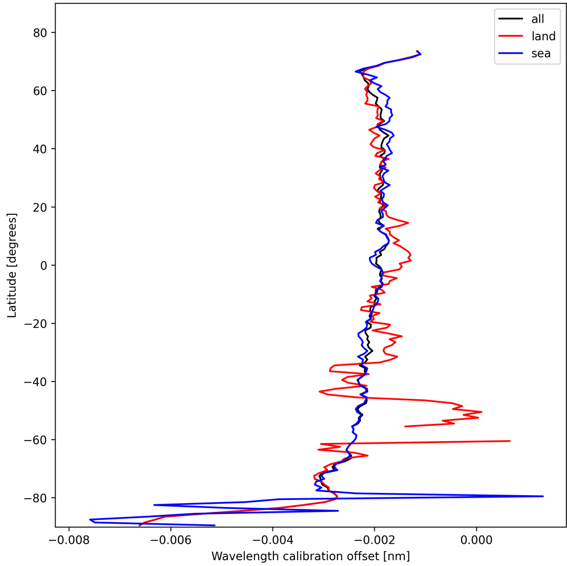
Figure 18: Zonal average of “Wavelength calibration offset” for 2025-02-08 to 2025-02-09.
