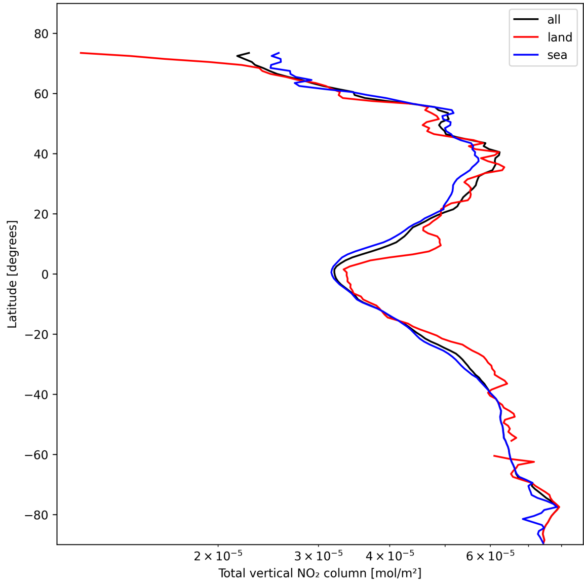
Figure 21: Zonal average of “Total vertical NO 2 column” for 2025-02-08 to 2025-02-09.
