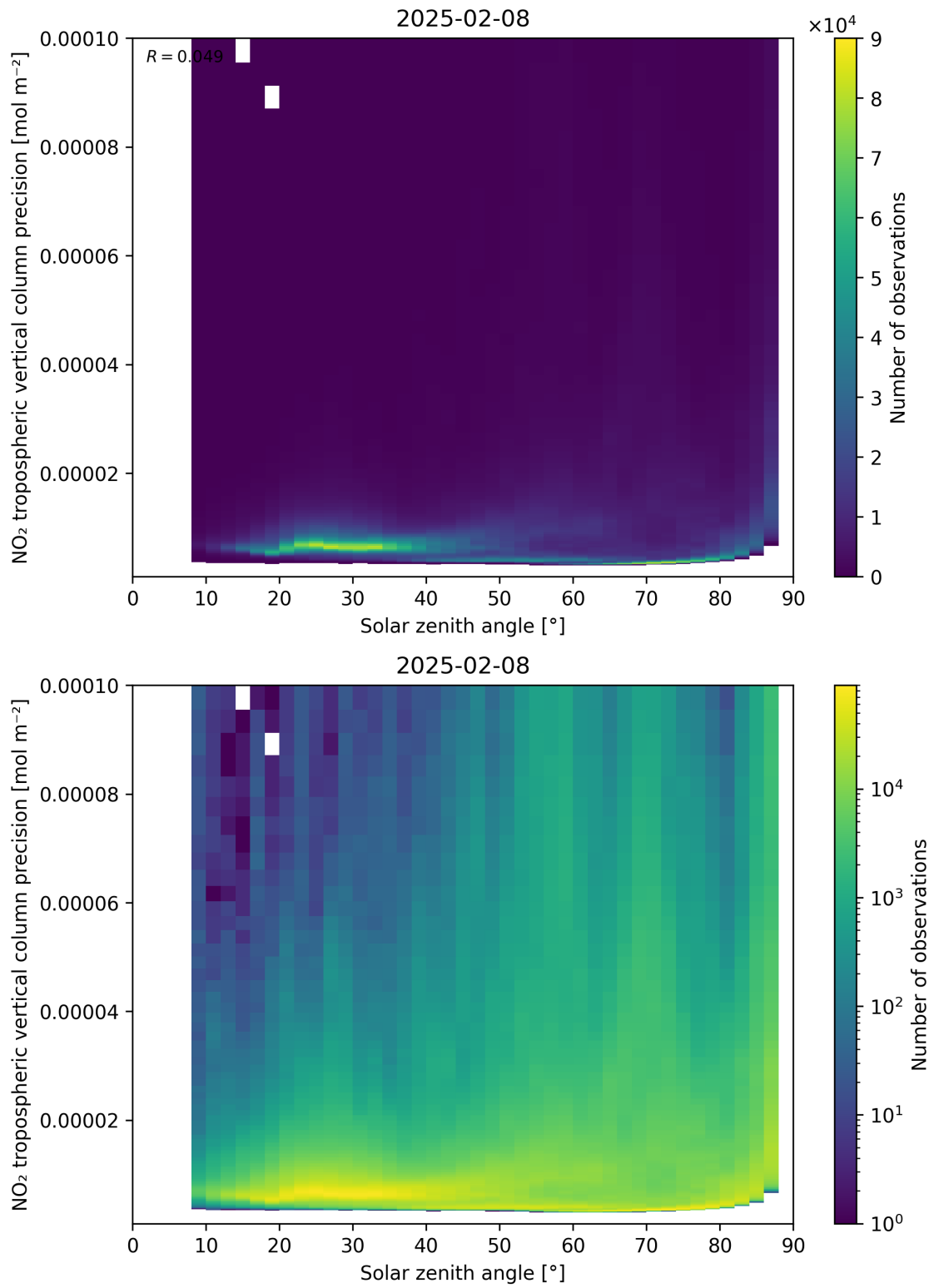
Figure 156: Scatter density plot of “Solar zenith angle” against “NO 2 tropospheric vertical column precision” for 2025-02-08 to 2025-02-09.
