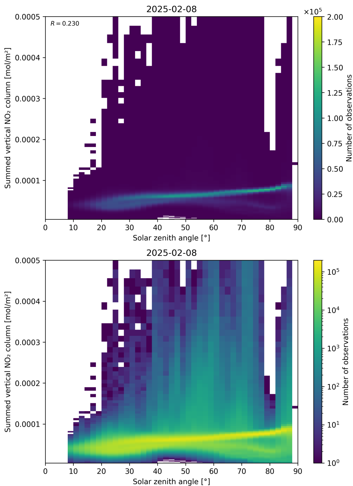
Figure 151: Scatter density plot of “Solar zenith angle” against “Summed vertical NO 2 column” for 2025-02-08 to 2025-02-09.
