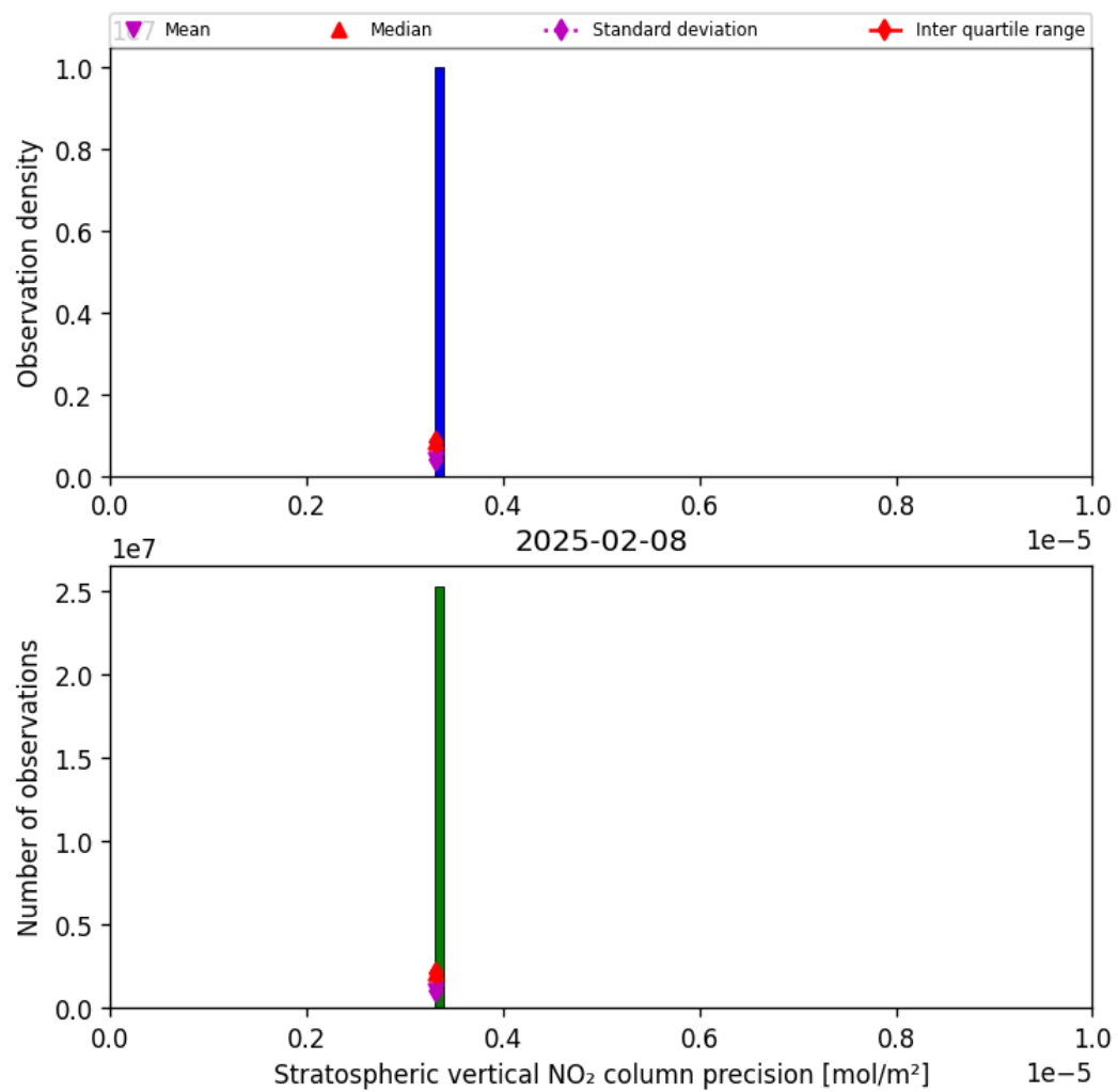
Figure 37: Histogram of “Stratospheric vertical NO 2 column precision” for 2025-02-08 to 2025-02-09
