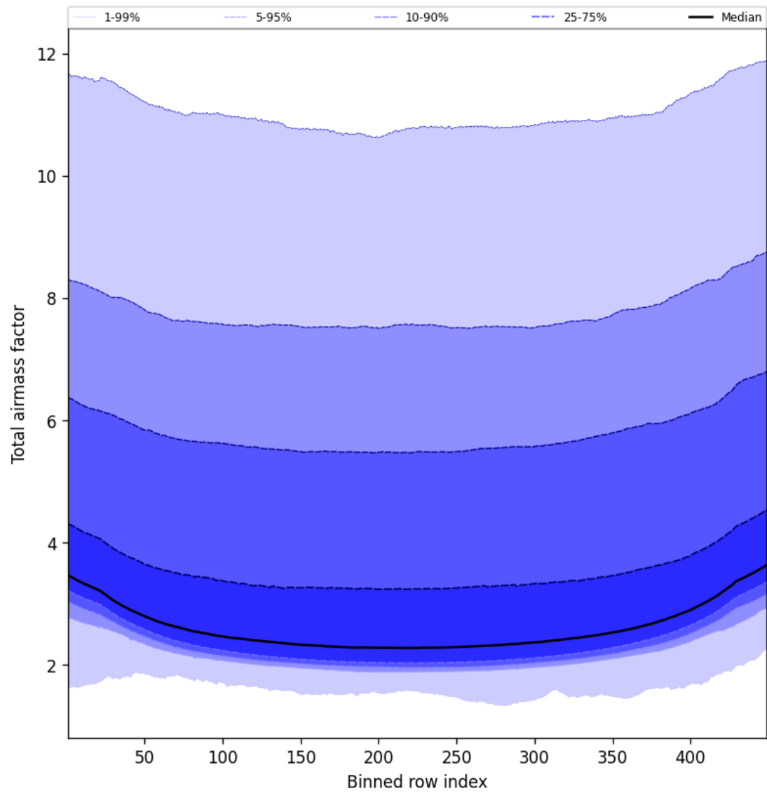
Figure 49: Along track statistics of “Total airmass factor” for 2025-02-08 to 2025-02-09
