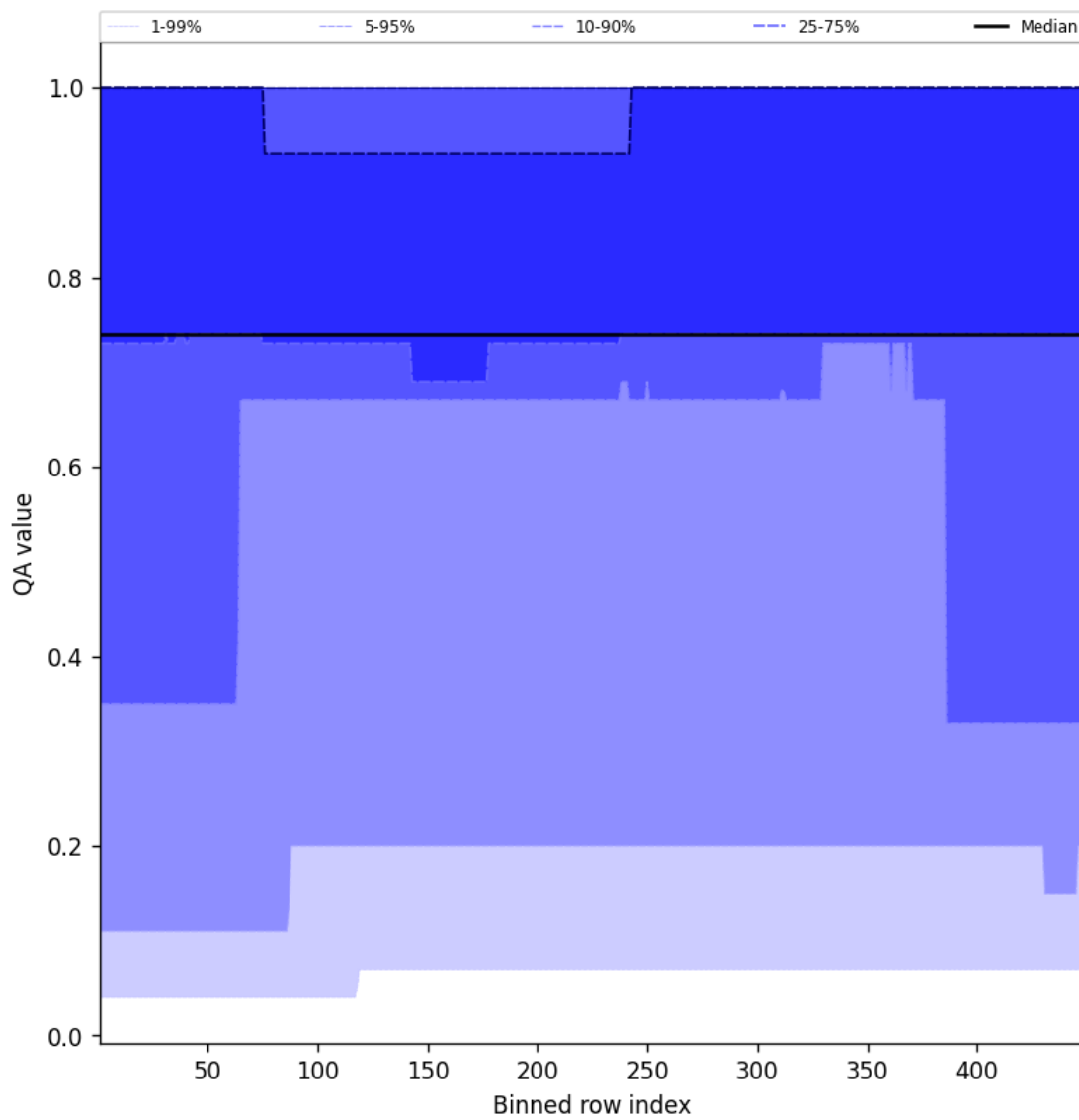
Figure 45: Along track statistics of “QA value” for 2025-02-08 to 2025-02-09
