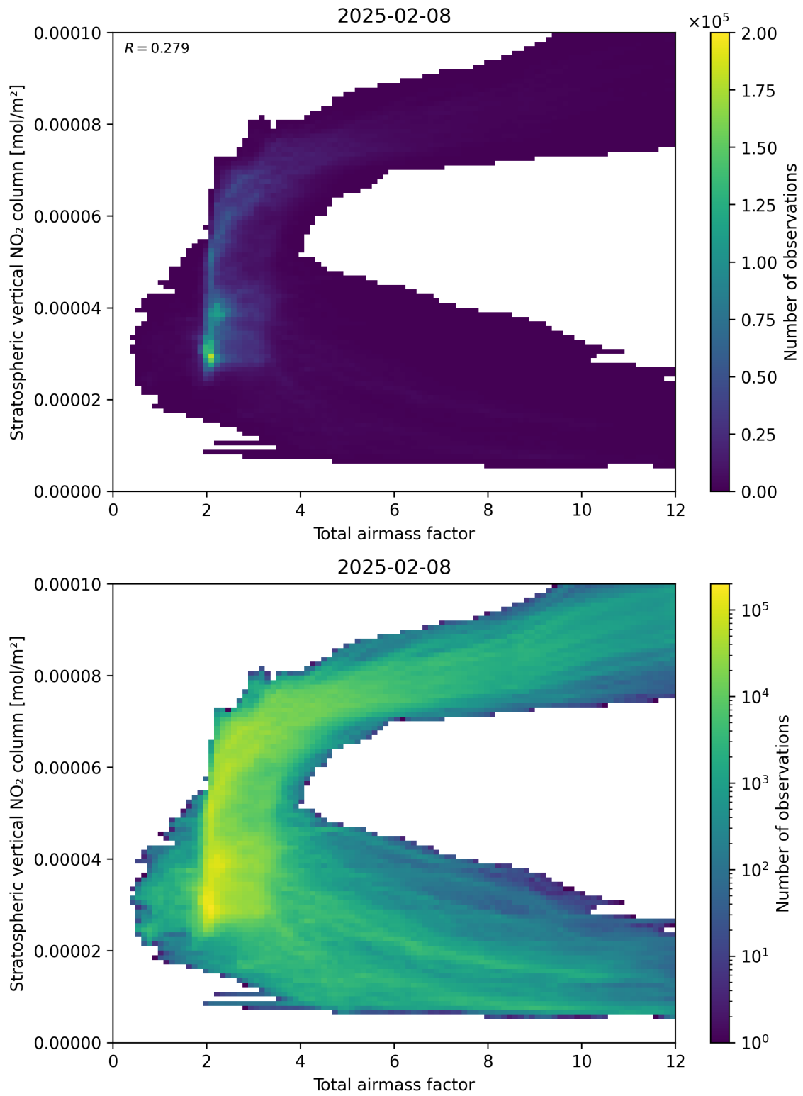
Figure 64: Scatter density plot of “Total airmass factor” against “Stratospheric vertical NO 2 column” for 2025-02-08 to 2025-02-09.
