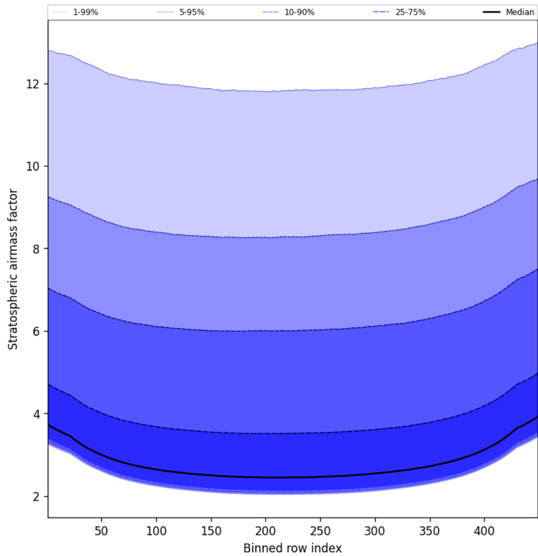
Figure 61: Along track statistics of “Stratospheric airmass factor” for 2025-02-08 to 2025-02-09
