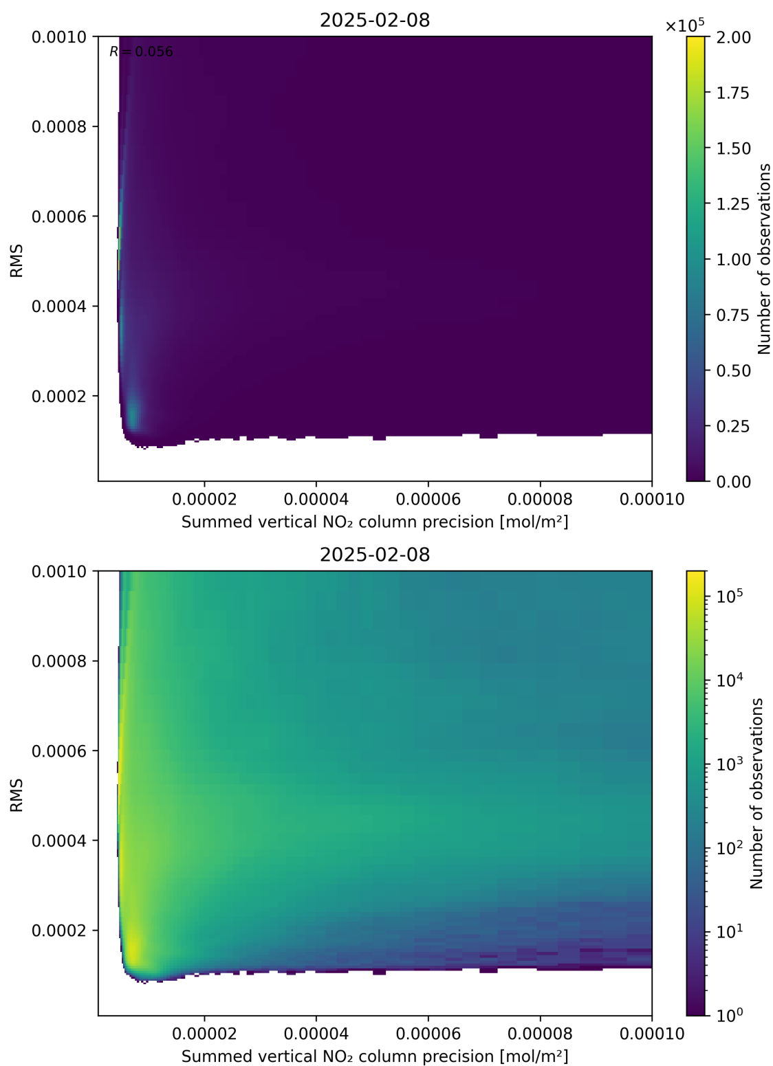
Figure 108: Scatter density plot of “Summed vertical NO 2 column precision” against “RMS” for 2025-02-08 to 2025-02-09.
