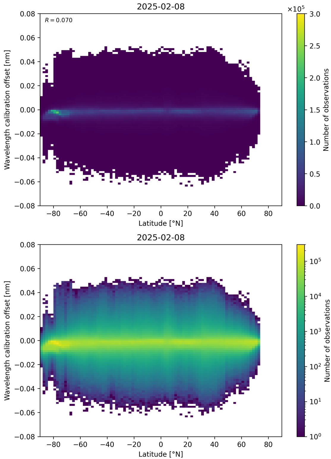
Figure 95: Scatter density plot of “Latitude” against “Wavelength calibration offset” for 2025-02-08 to 2025-02-09.
