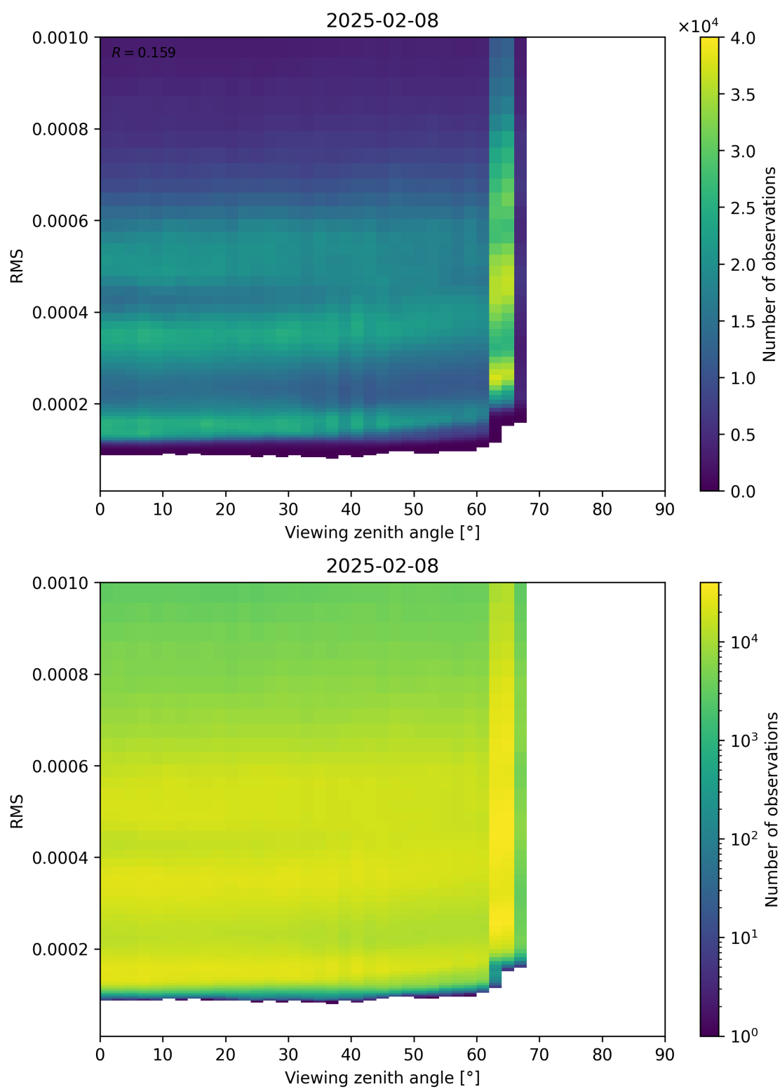
Figure 171: Scatter density plot of “Viewing zenith angle” against “RMS” for 2025-02-08 to 2025-02-09.
