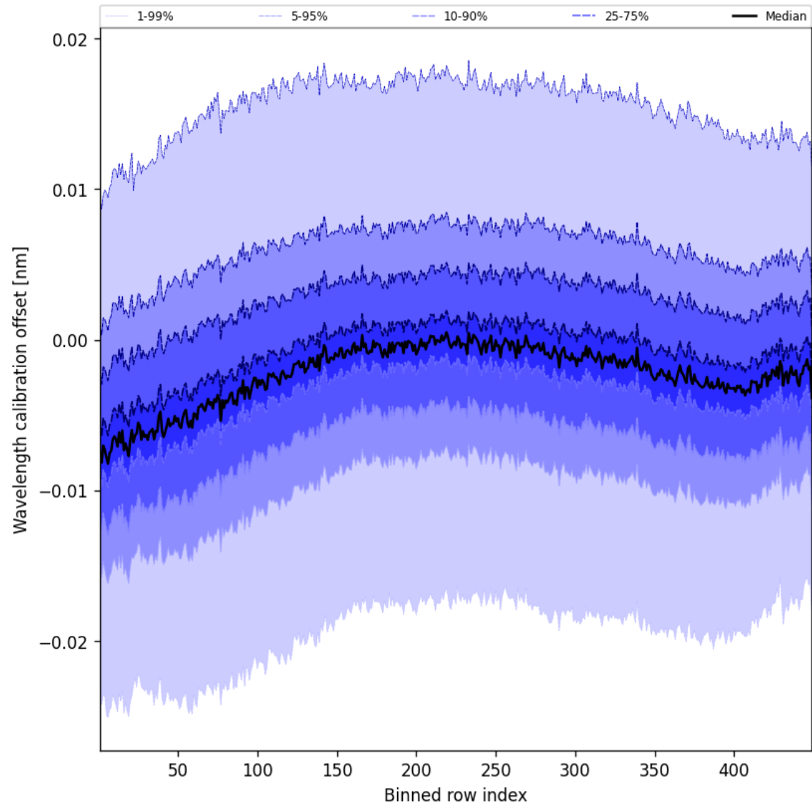
Figure 52: Along track statistics of “Wavelength calibration offset” for 2025-02-08 to 2025-02-09
