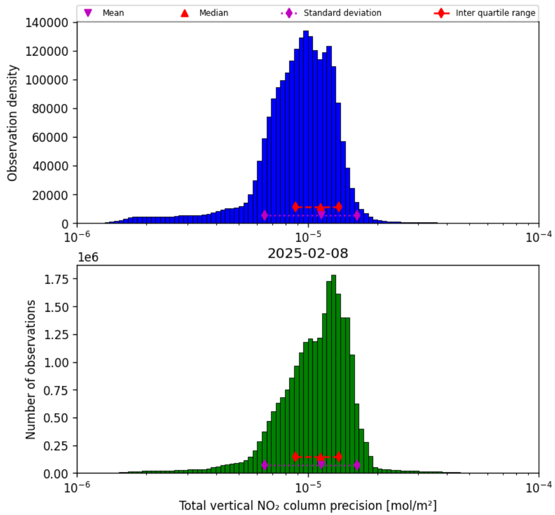
Figure 39: Histogram of “Total vertical NO 2 column precision” for 2025-02-08 to 2025-02-09
