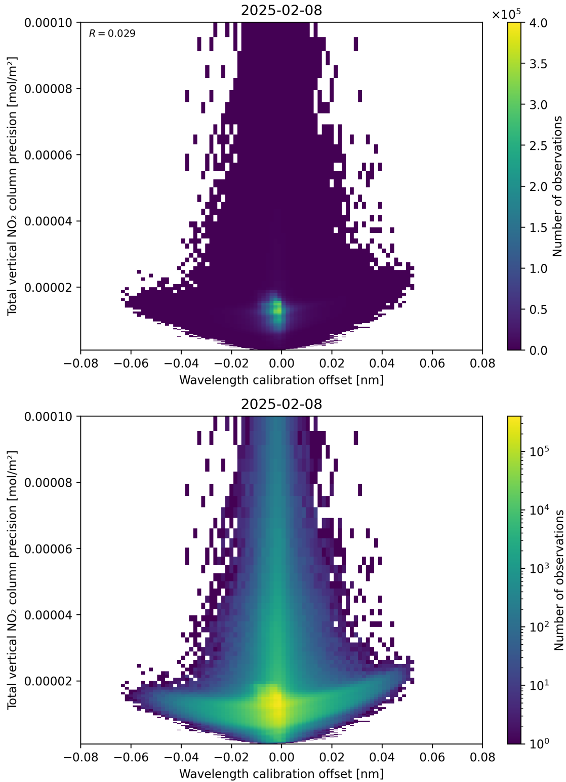
Figure 180: Scatter density plot of “Wavelength calibration offset” against “Total vertical NO 2 column precision” for 2025-02-08 to 2025-02-09.
