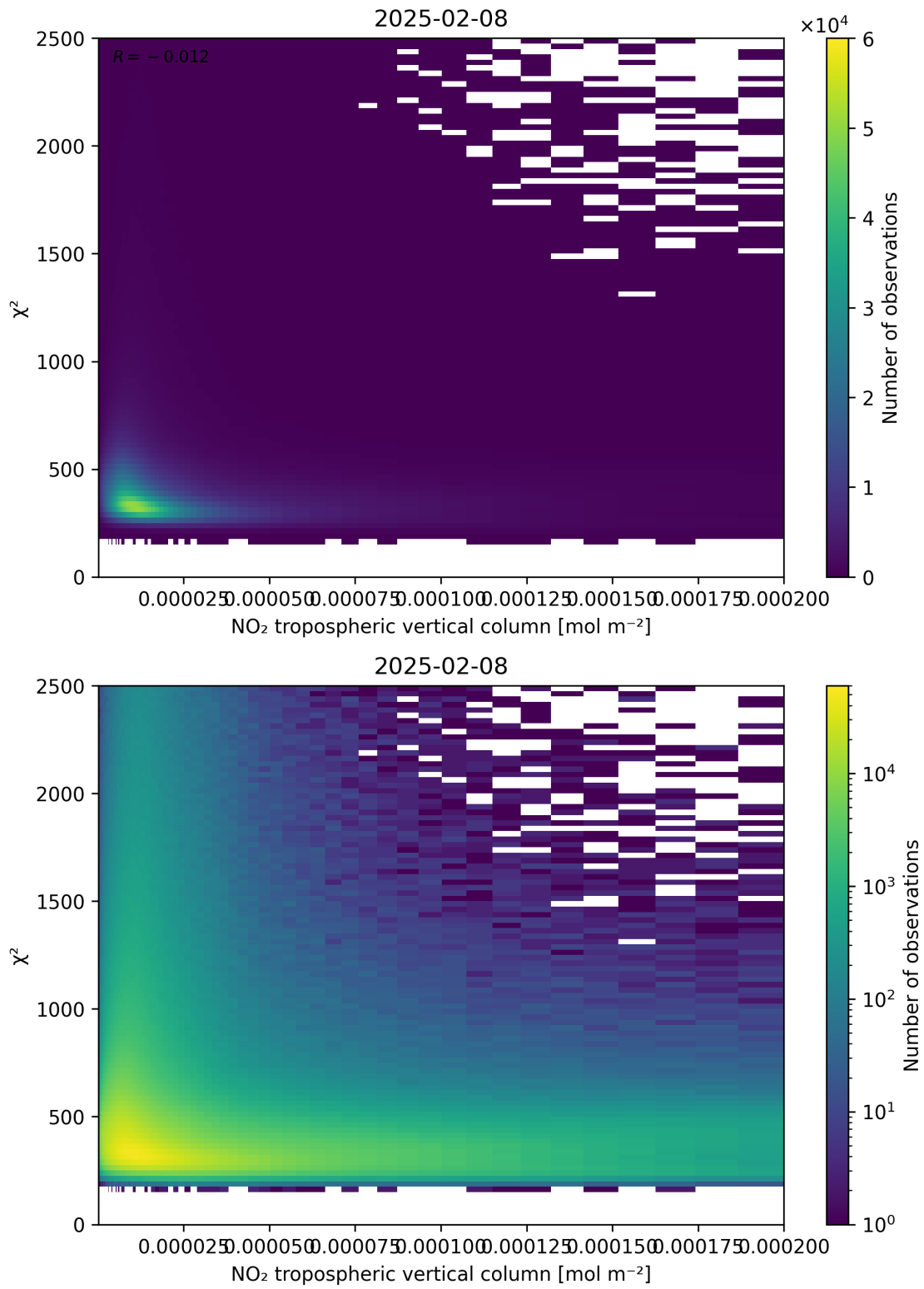
Figure 124: Scatter density plot of “NO 2 tropospheric vertical column” against “ \chi^2 ” for 2025-02-08 to 2025-02-09.
