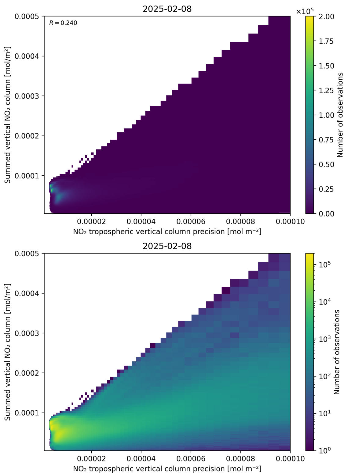
Figure 136: Scatter density plot of “NO 2 tropospheric vertical column precision” against “Summed vertical NO 2 column” for 2025-02-08 to 2025-02-09.
