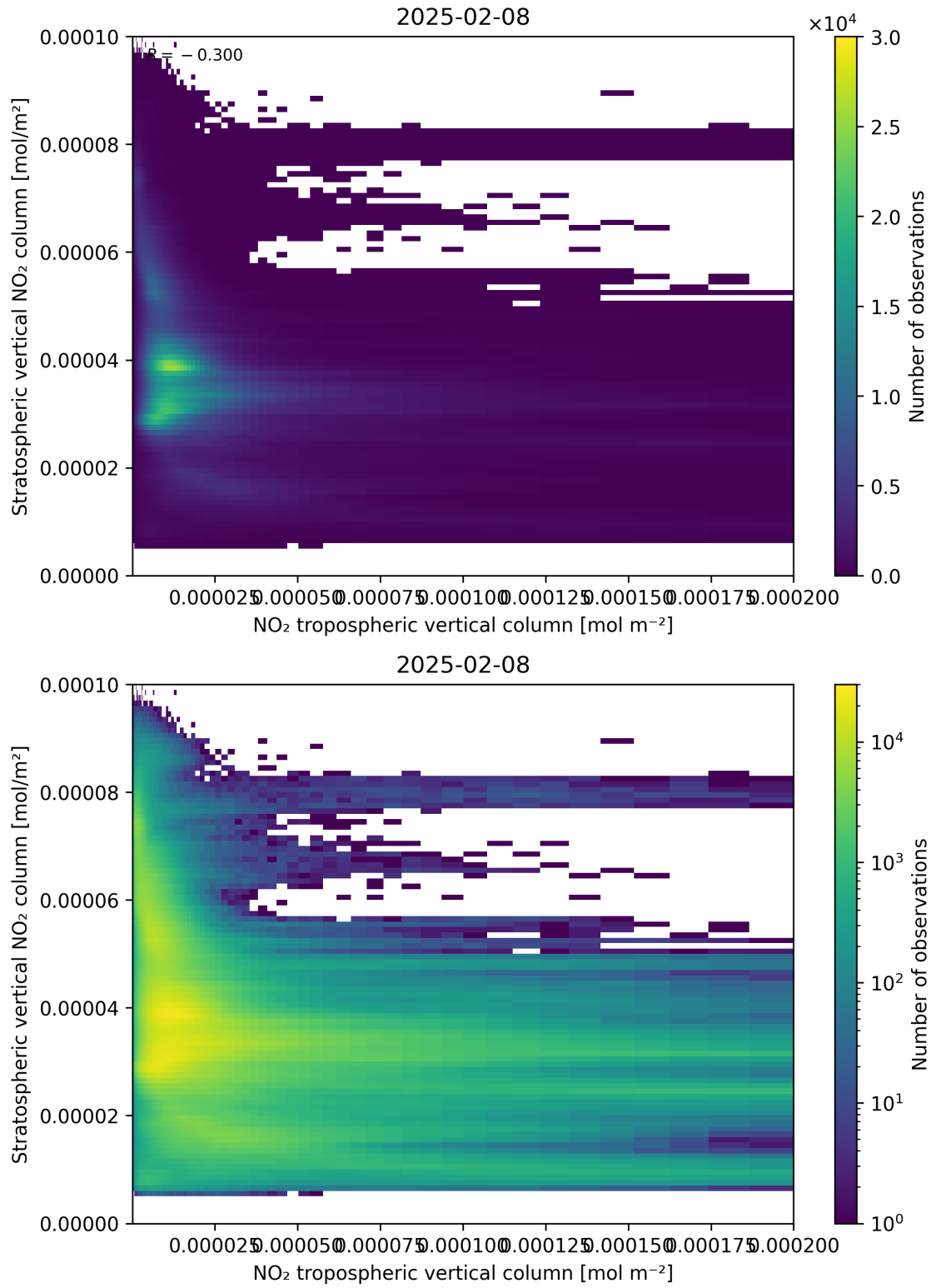
Figure 125: Scatter density plot of “NO 2 tropospheric vertical column” against “Stratospheric vertical NO 2 column” for 2025-02-08 to 2025-02-09.
