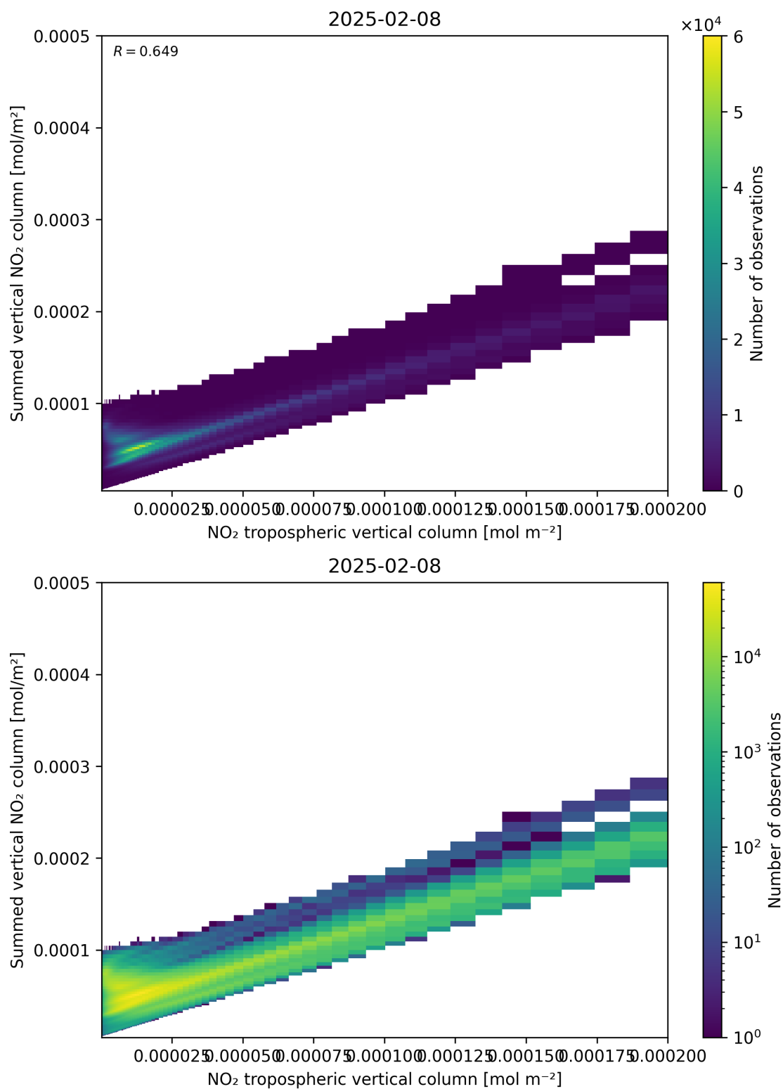
Figure 126: Scatter density plot of “NO 2 tropospheric vertical column” against “Summed vertical NO 2 column” for 2025-02-08 to 2025-02-09.
