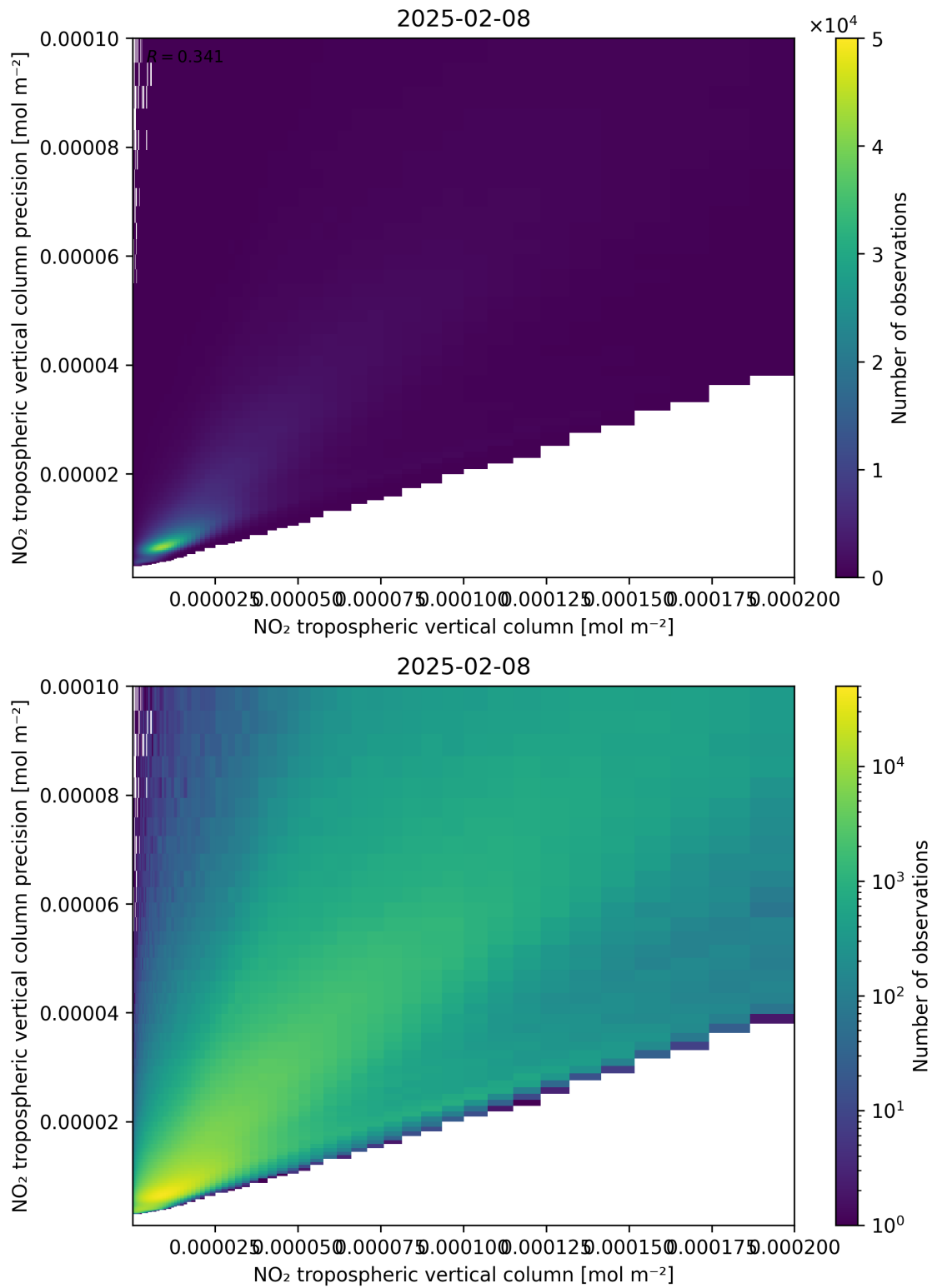
Figure 130: Scatter density plot of “NO 2 tropospheric vertical column” against “NO 2 tropospheric vertical column precision” for 2025-02-08 to 2025-02-09.
