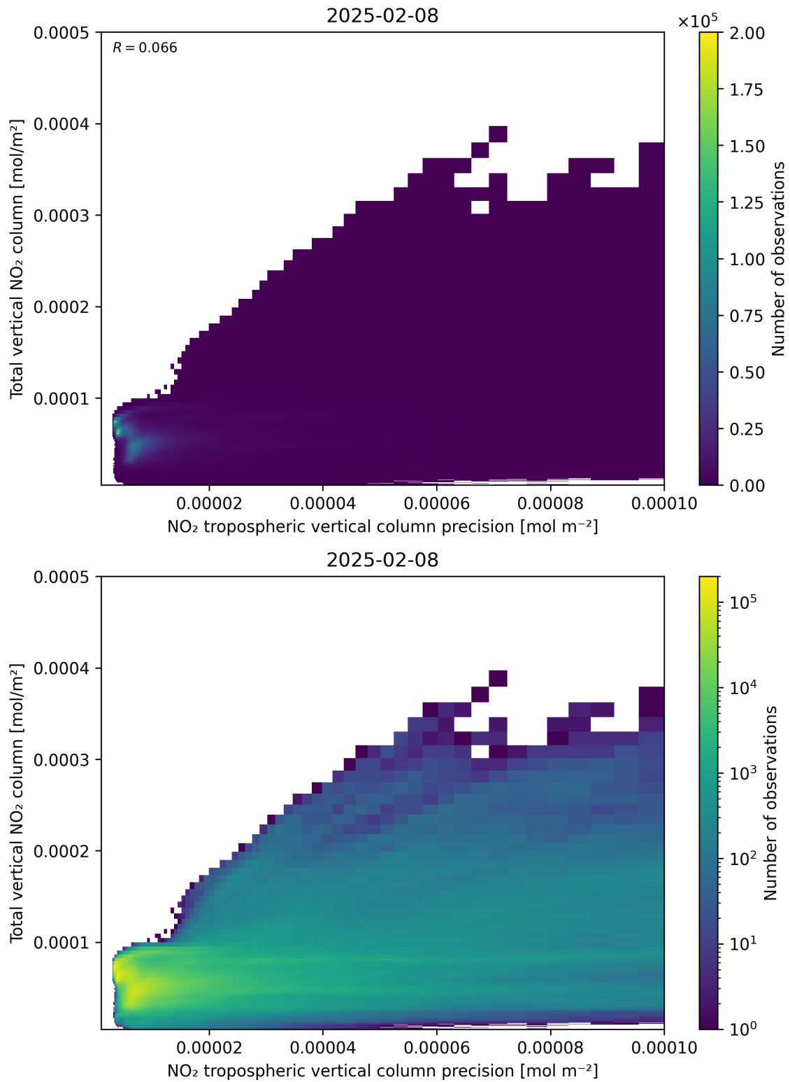
Figure 138: Scatter density plot of “NO 2 tropospheric vertical column precision” against “Total vertical NO 2 column” for 2025-02-08 to 2025-02-09.
