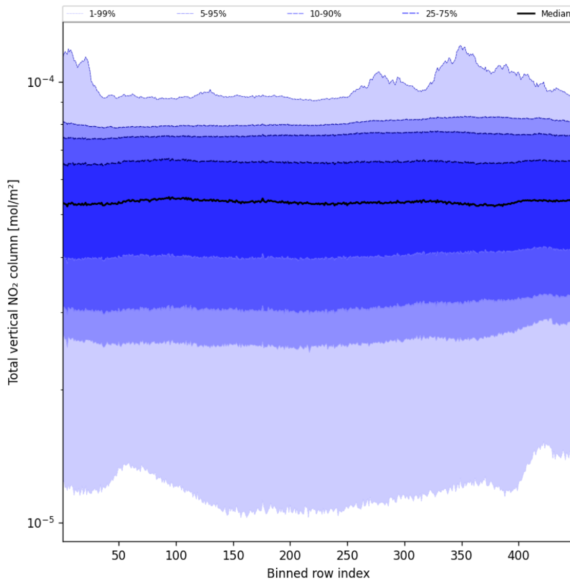
Figure 55: Along track statistics of “Total vertical NO 2 column” for 2025-02-08 to 2025-02-09
