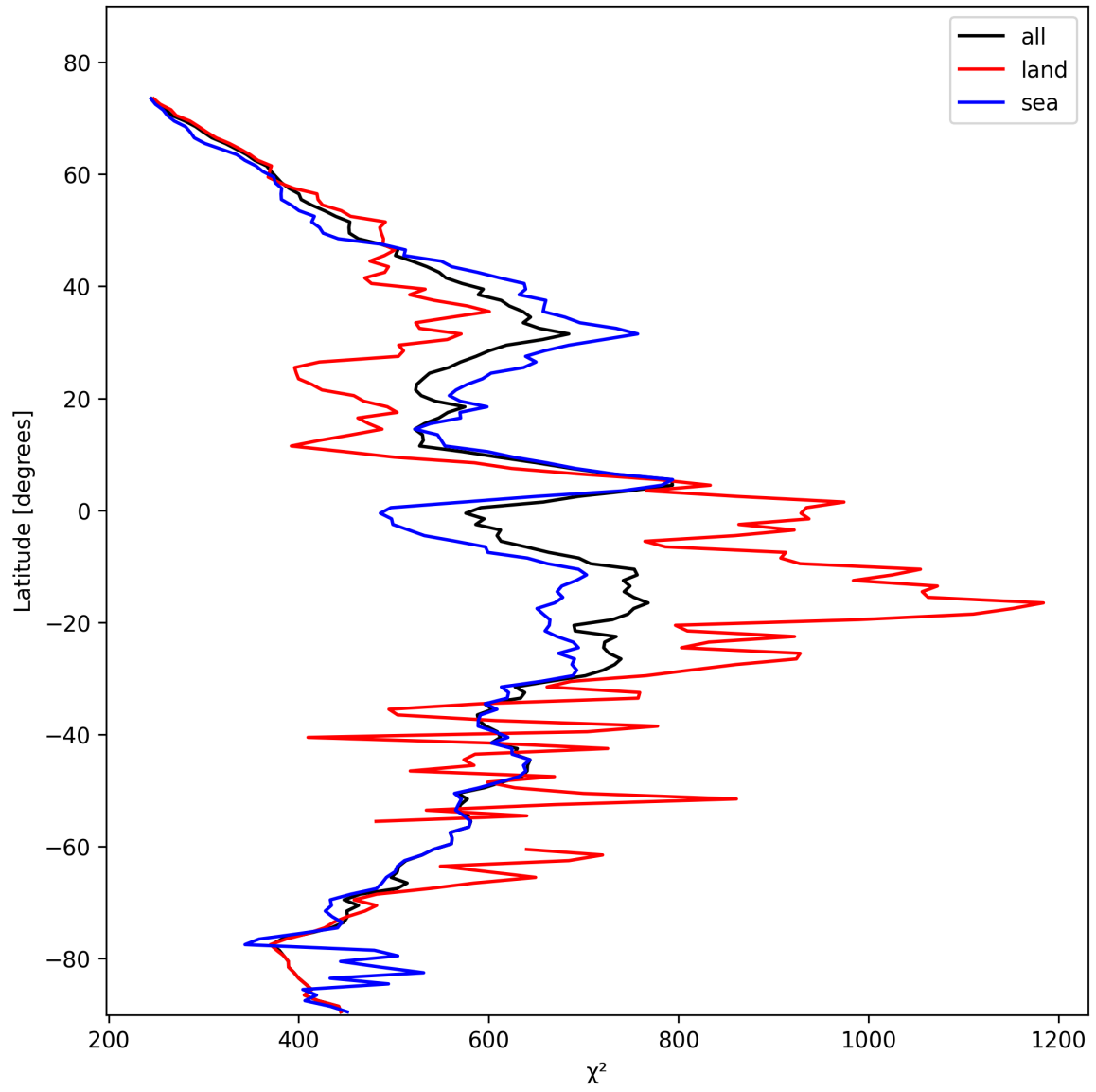
Figure 25: Zonal average of “ \chi^2 ” for 2025-02-08 to 2025-02-09.
