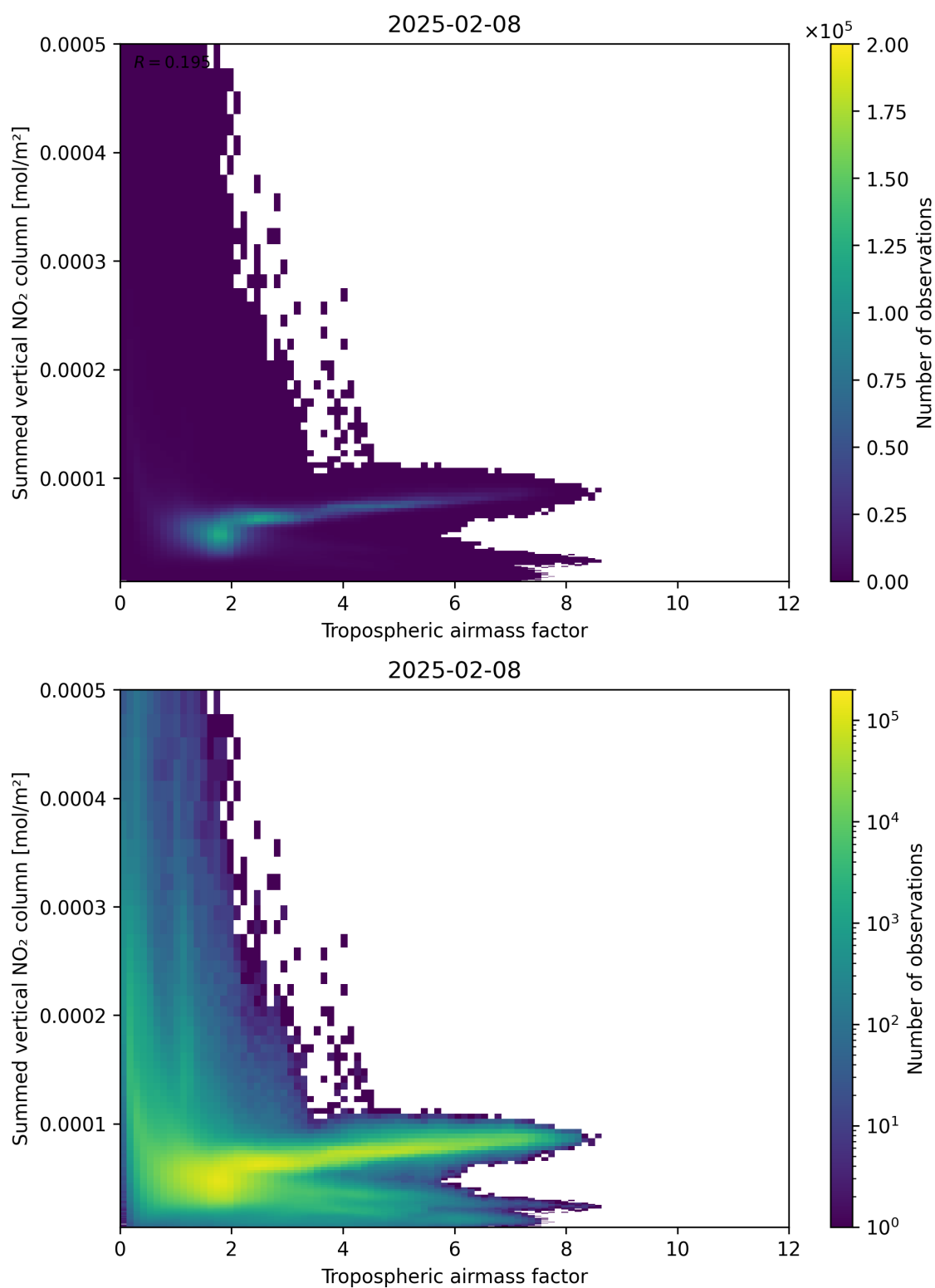
Figure 75: Scatter density plot of “Tropospheric air mass factor” against “Summed vertical NO 2 column” for 2025-02-08 to 2025-02-09.
