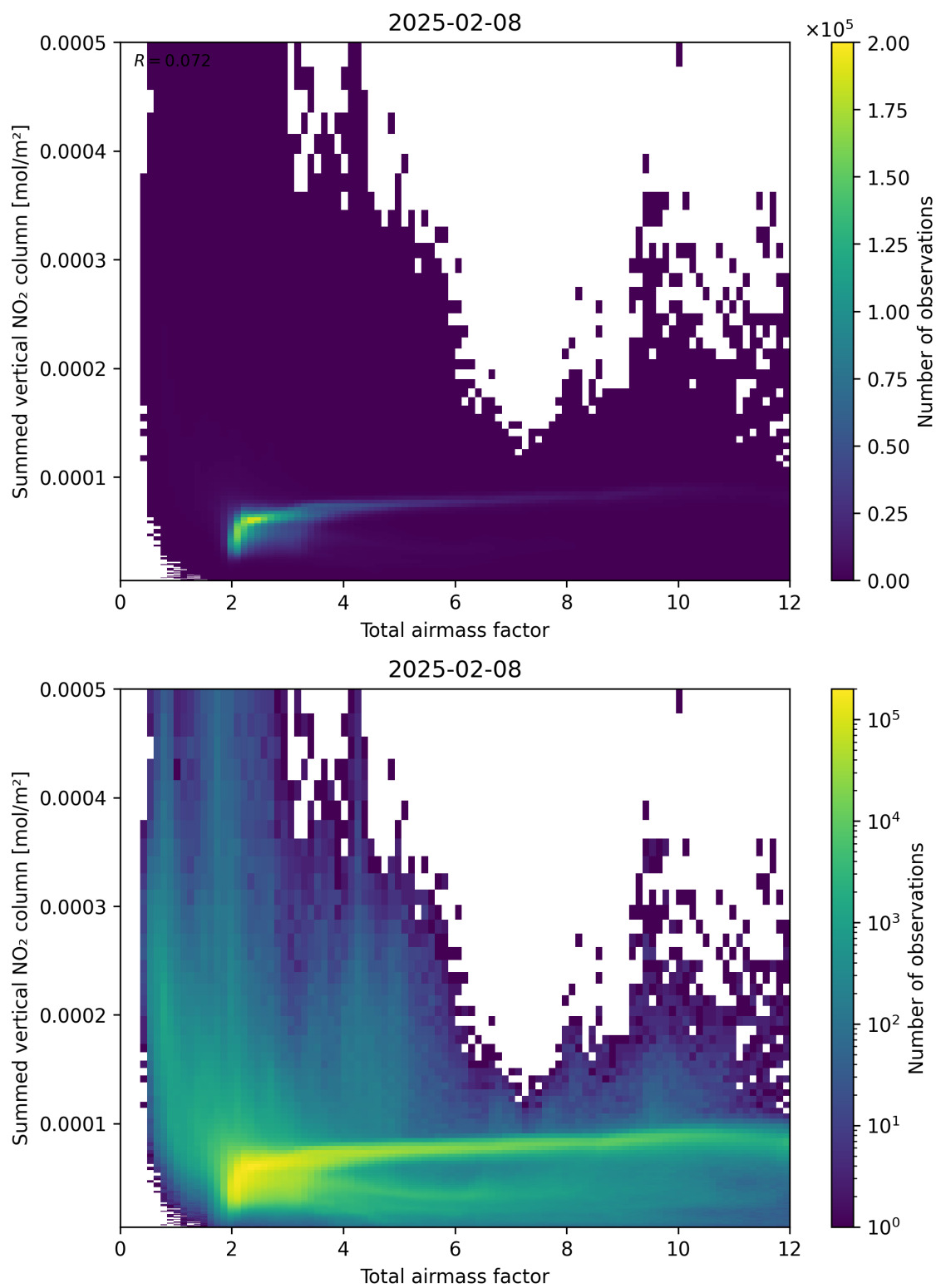
Figure 65: Scatter density plot of “Total airmass factor” against “Summed vertical NO 2 column” for 2025-02-08 to 2025-02-09.
