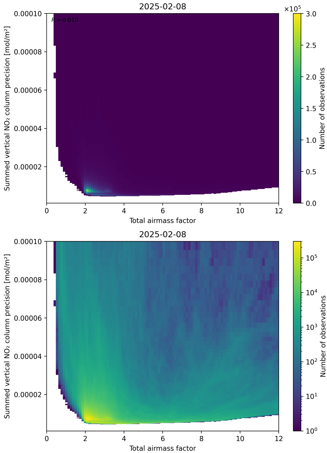
Figure 66: Scatter density plot of “Total airmass factor” against “Summed vertical NO 2 column precision” for 2025-02-08 to 2025-02-09.
