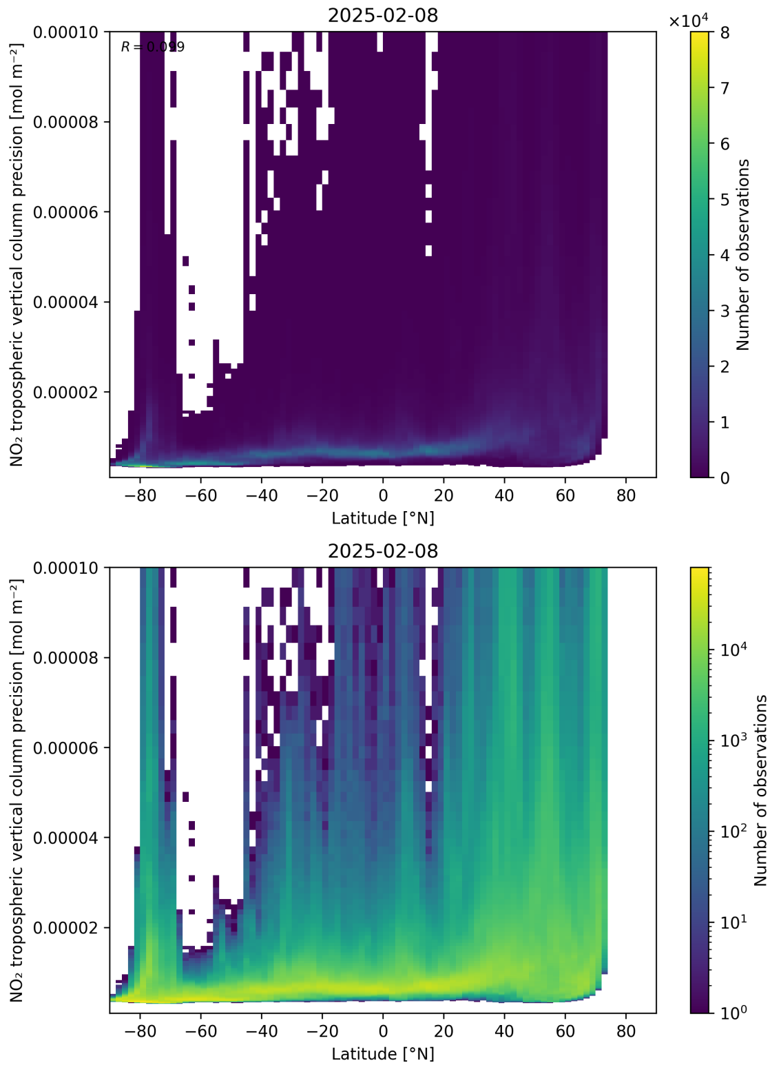
Figure 93: Scatter density plot of “Latitude” against “NO 2 tropospheric vertical column precision” for 2025-02-08 to 2025-02-09.
