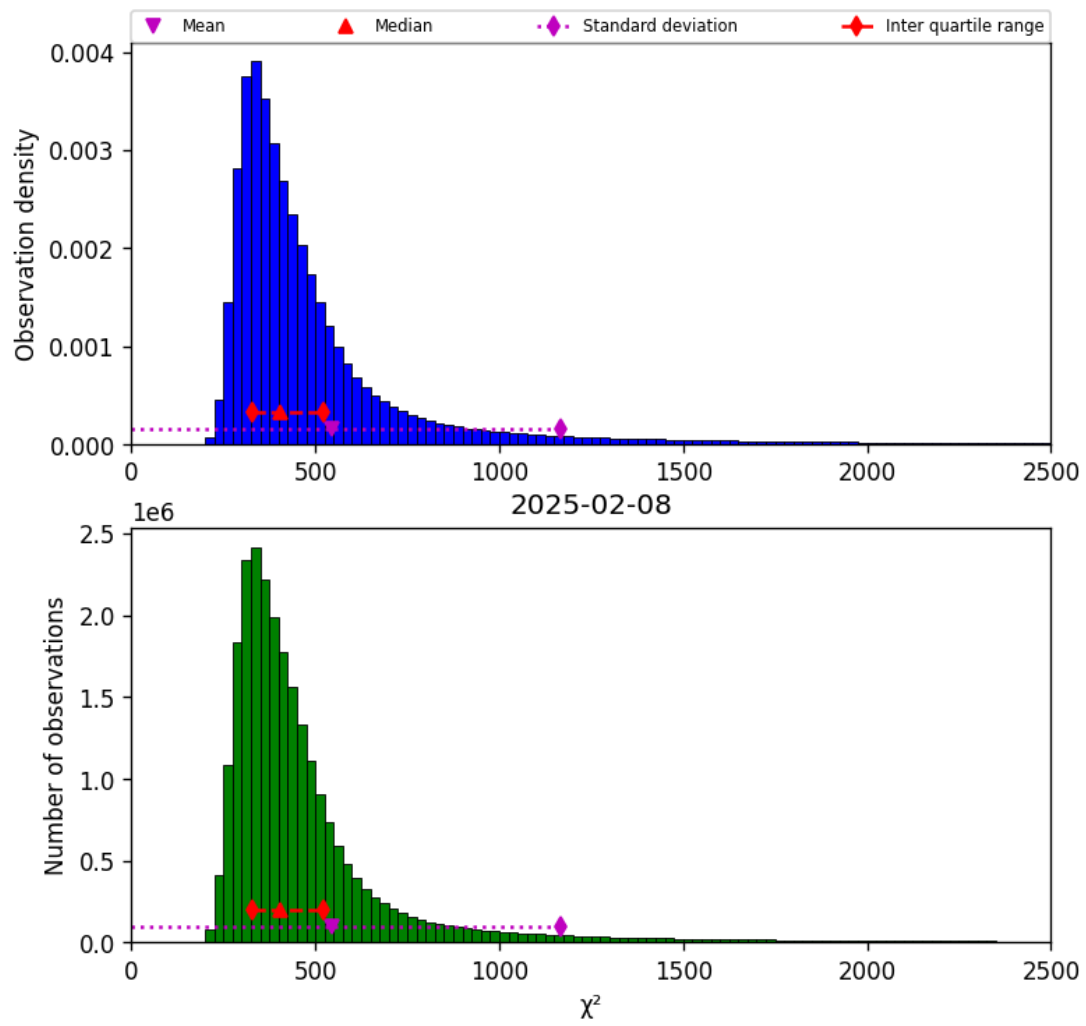
Figure 42: Histogram of “ \chi^2 ” for 2025-02-08 to 2025-02-09
