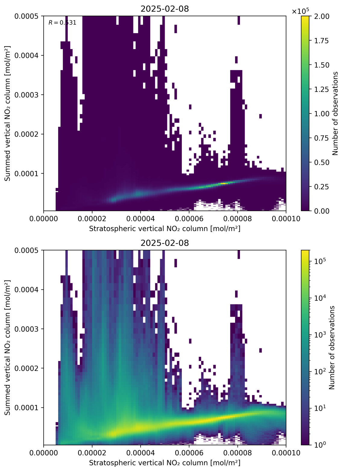
Figure 98: Scatter density plot of “Stratospheric vertical NO 2 column” against “Summed vertical NO 2 column” for 2025-02-08 to 2025-02-09.
