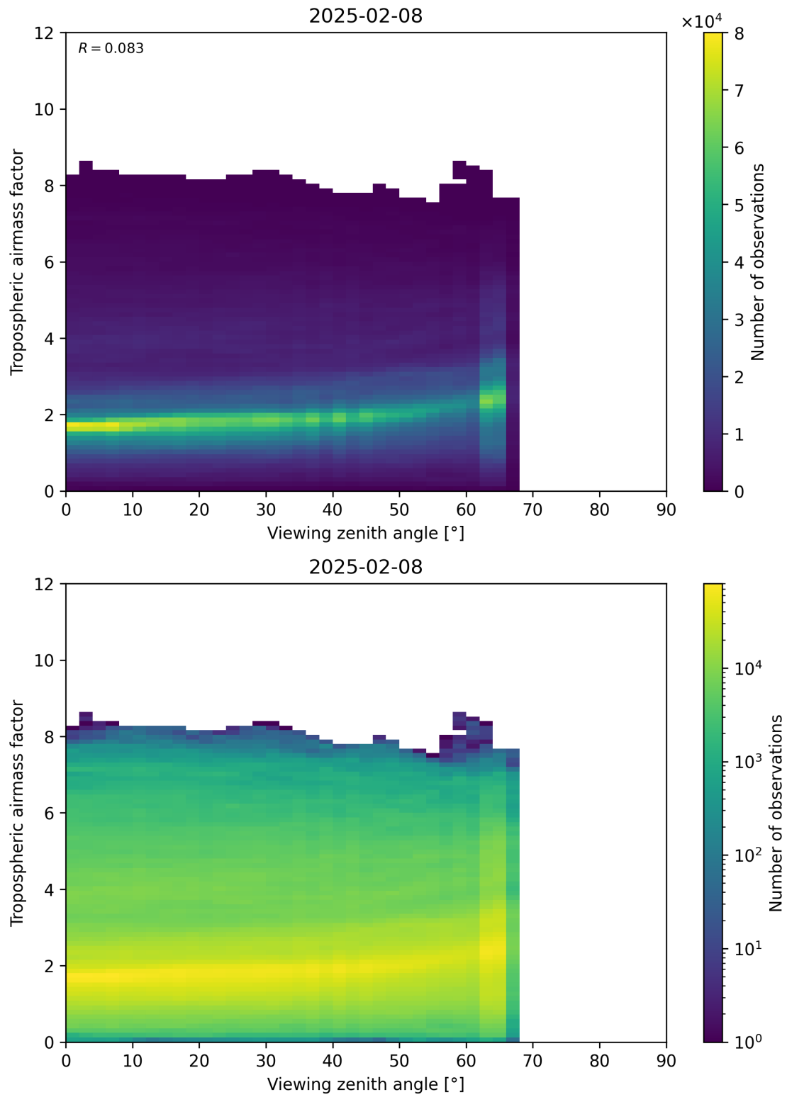
Figure 161: Scatter density plot of “Viewing zenith angle” against “Tropospheric airmass factor” for 2025-02-08 to 2025-02-09.
