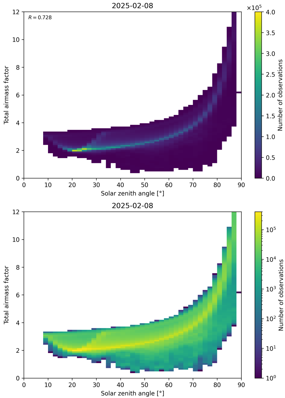
Figure 146: Scatter density plot of “Solar zenith angle” against “Total air mass factor” for 2025-02-08 to 2025-02-09.
