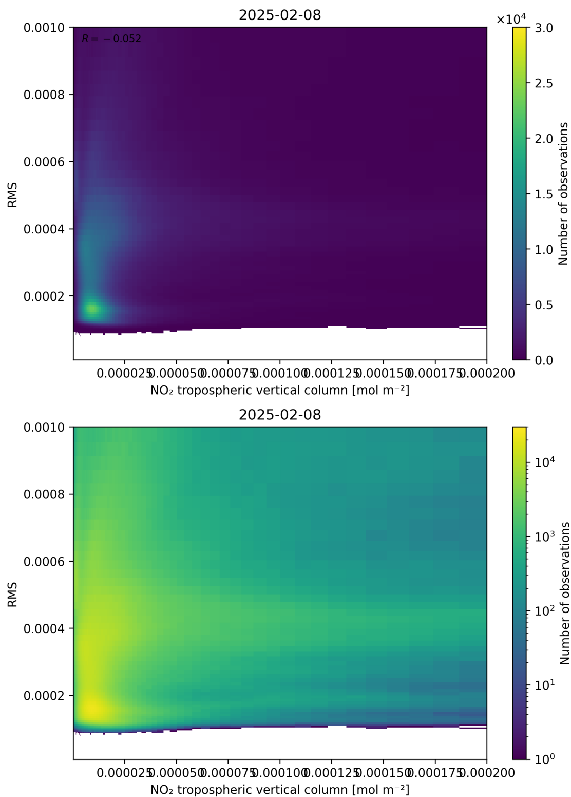
Figure 142: Scatter density plot of “NO 2 tropospheric vertical column” against “RMS” for 2025-02-08 to 2025-02-09.
