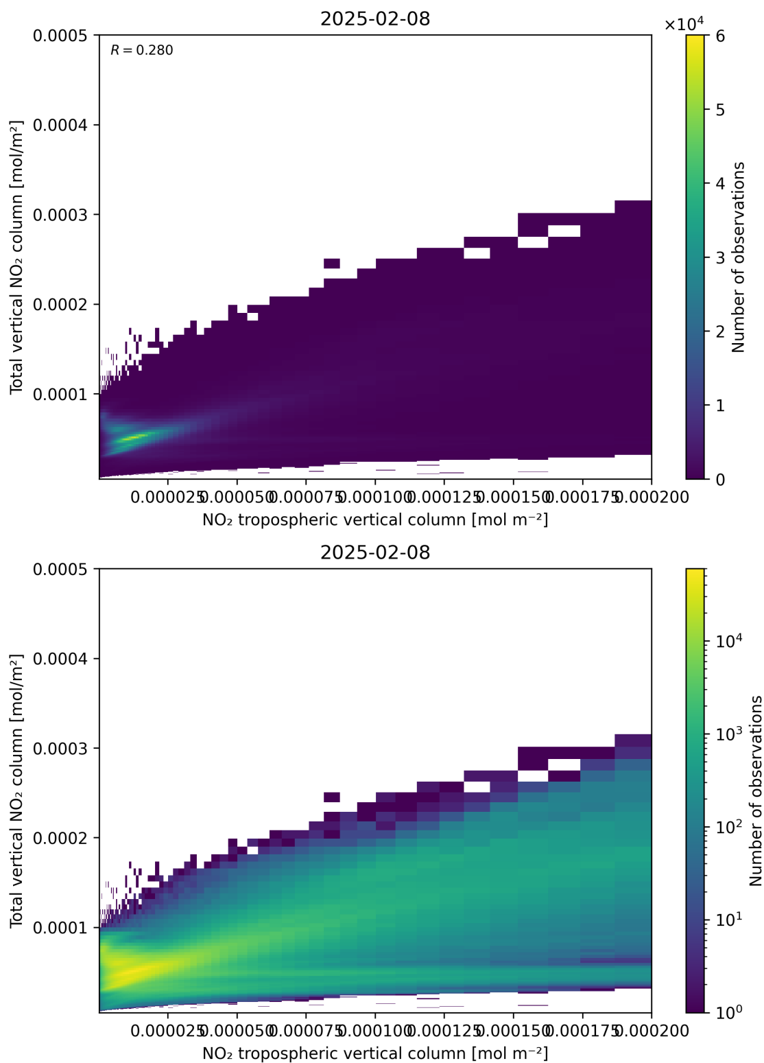
Figure 128: Scatter density plot of “NO 2 tropospheric vertical column” against “Total vertical NO 2 column” for 2025-02-08 to 2025-02-09.
