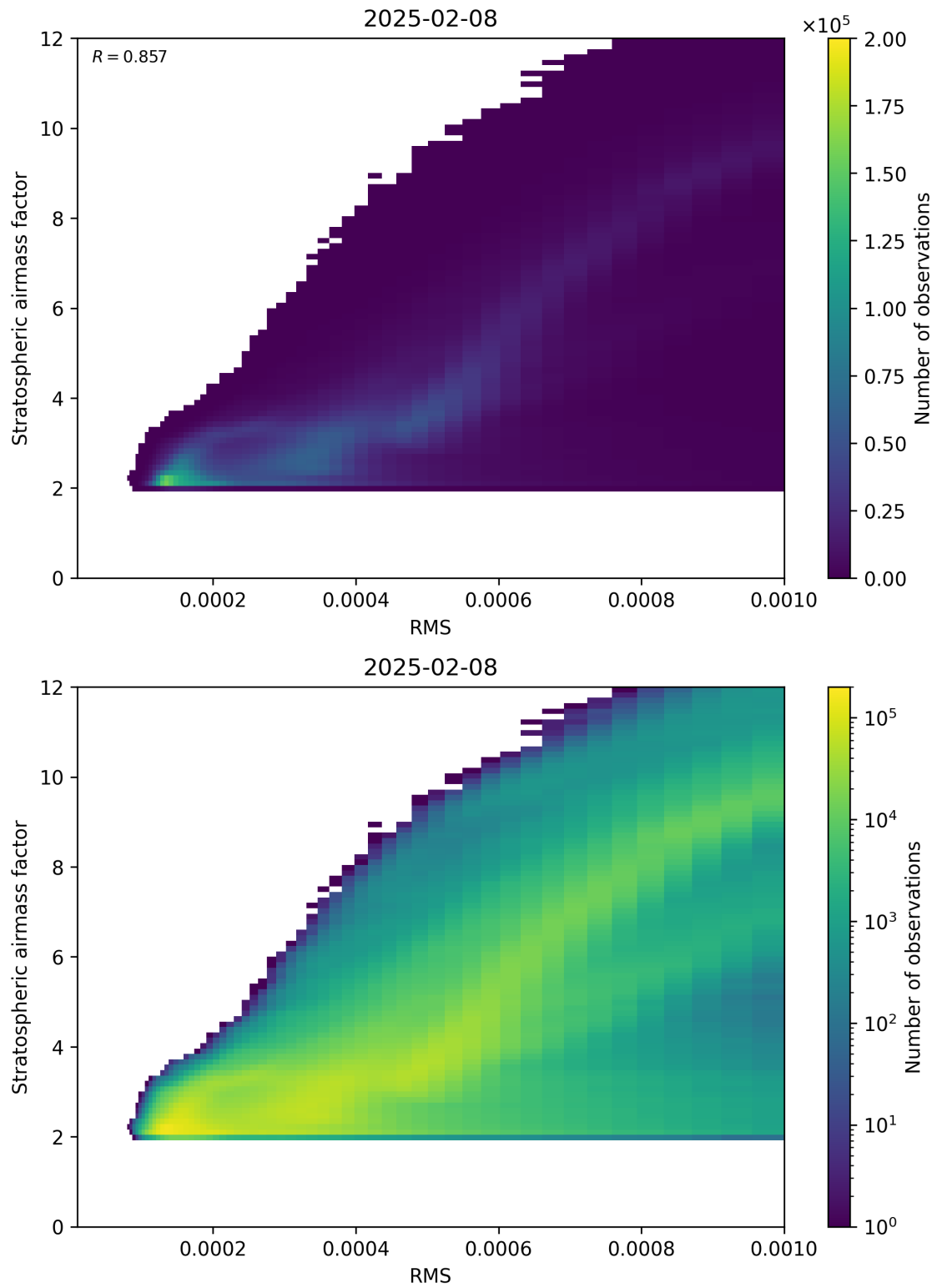
Figure 144: Scatter density plot of “RMS” against “Stratospheric airmass factor” for 2025-02-08 to 2025-02-09.
