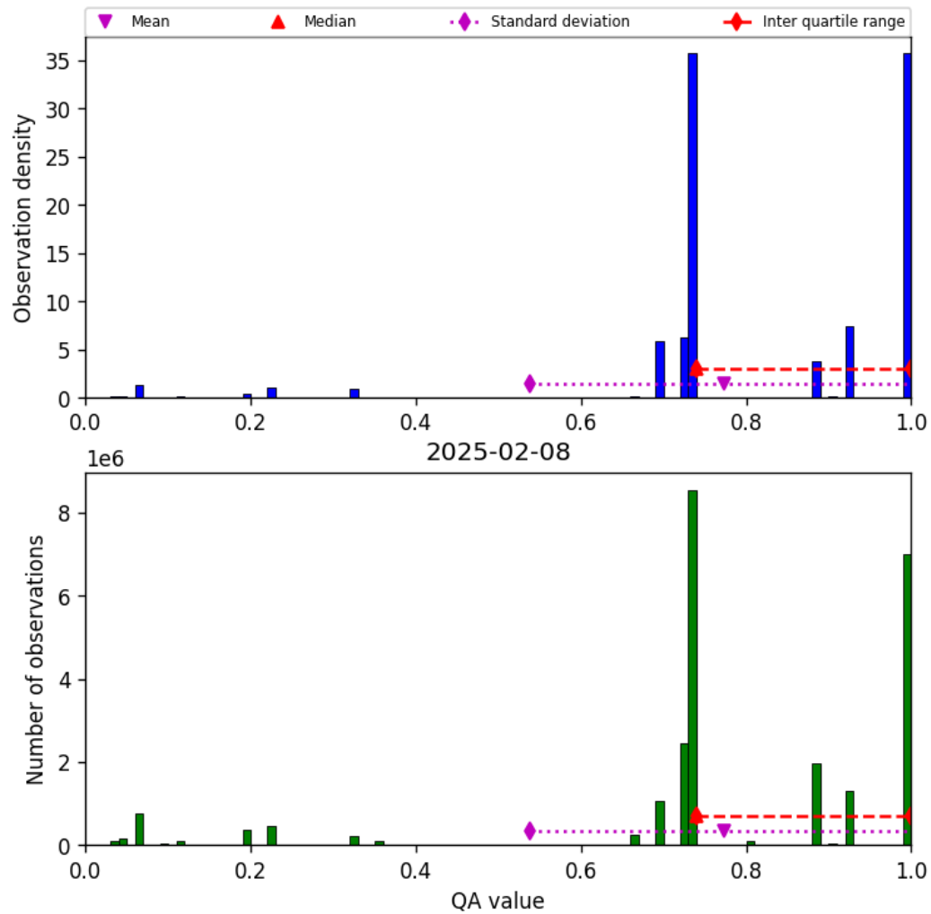
Figure 28: Histogram of “QA value” for 2025-02-08 to 2025-02-09
