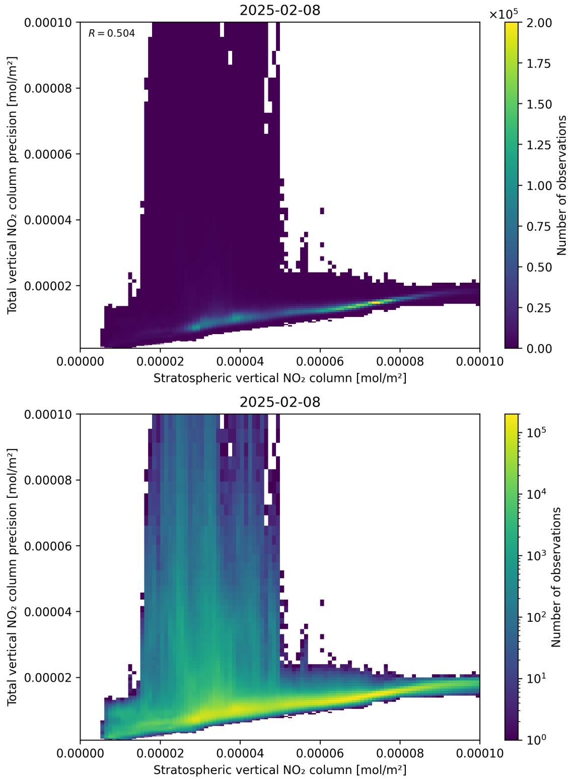
Figure 101: Scatter density plot of “Stratospheric vertical NO 2 column” against “Total vertical NO 2 column precision” for 2025-02-08 to 2025-02-09.
