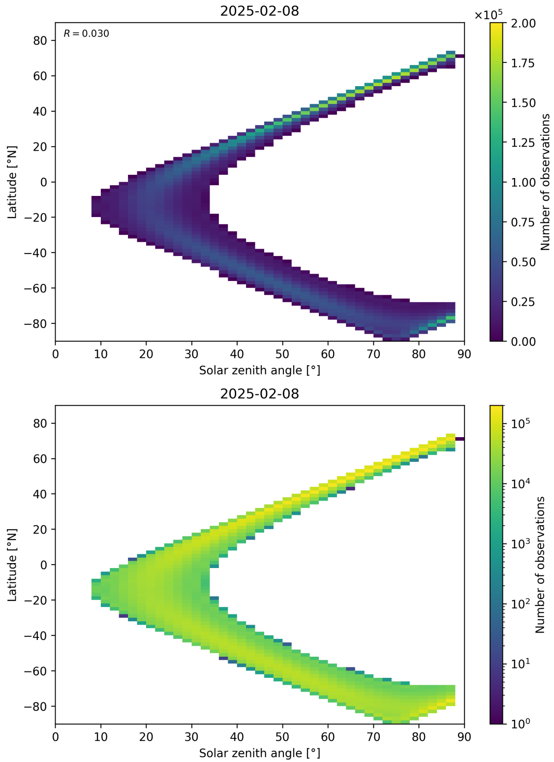
Figure 149: Scatter density plot of “Solar zenith angle” against “Latitude” for 2025-02-08 to 2025-02-09.
