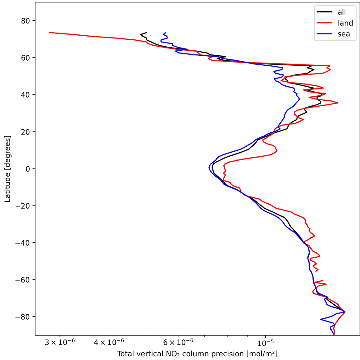
Figure 22: Zonal average of “Total vertical NO 2 column precision” for 2025-02-08 to 2025-02-09.
