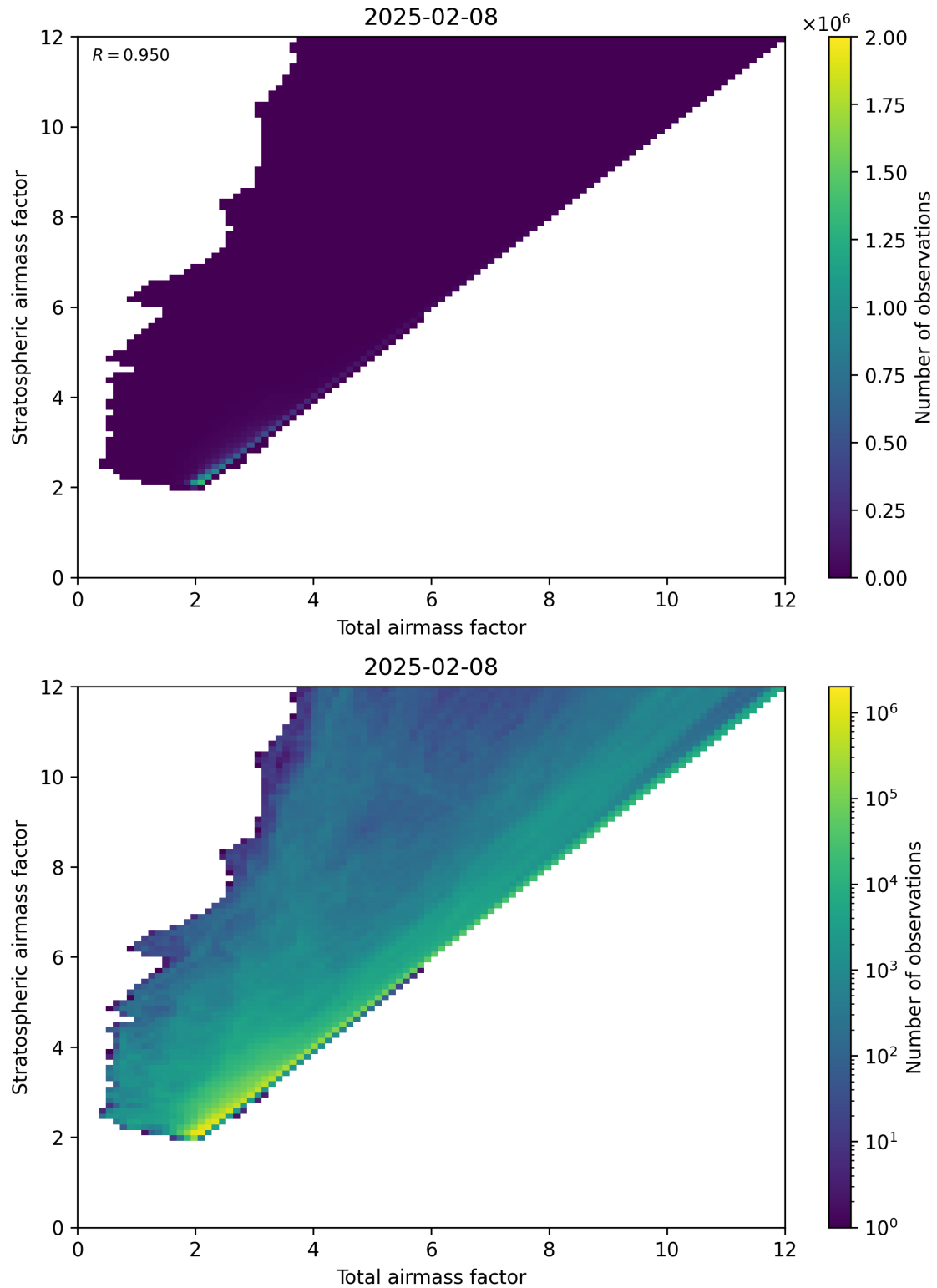
Figure 62: Scatter density plot of “Total airmass factor” against “Stratospheric airmass factor” for 2025-02-08 to 2025-02-09.
