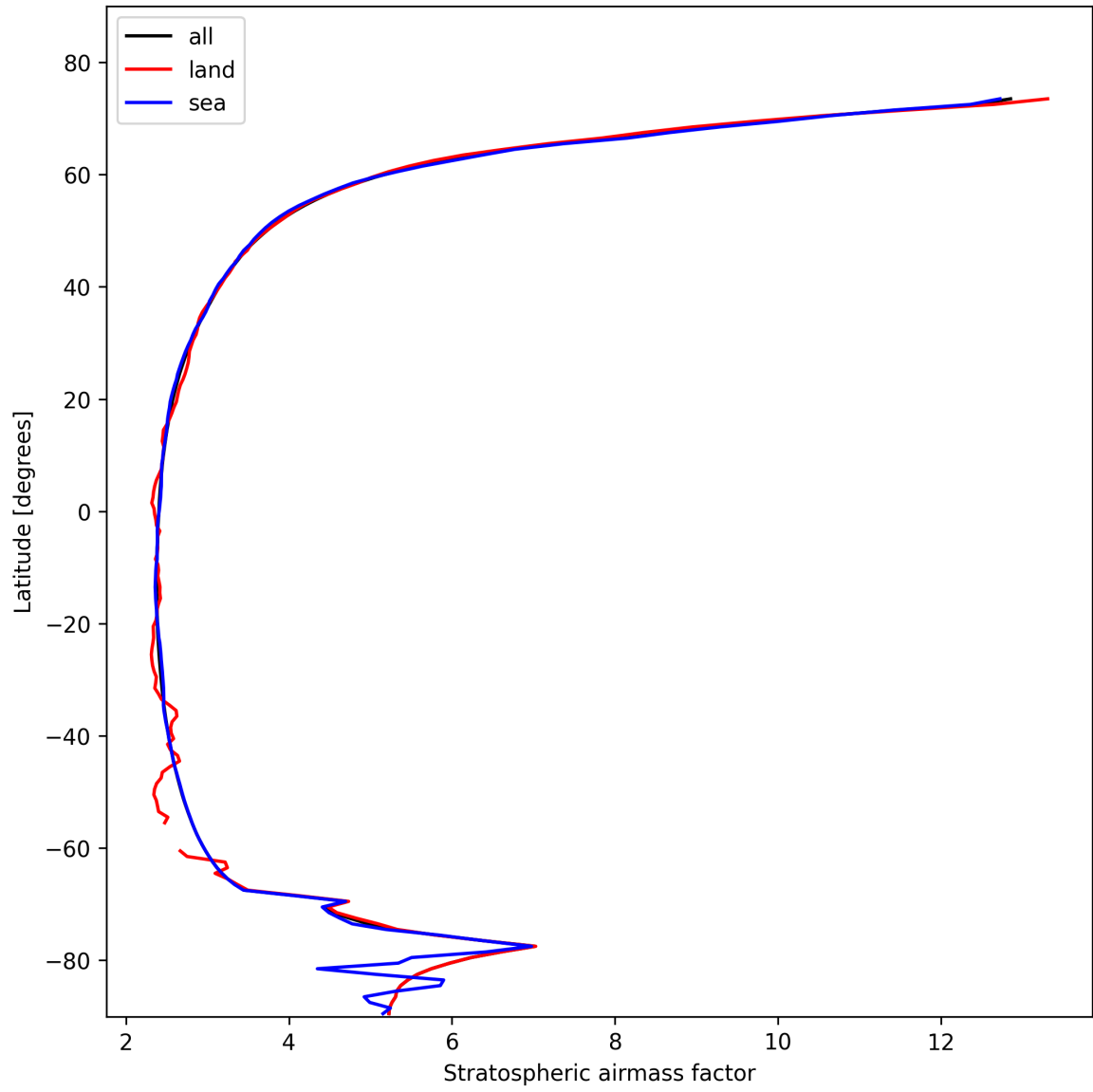
Figure 27: Zonal average of “Stratospheric air mass factor” for 2025-02-08 to 2025-02-09.
