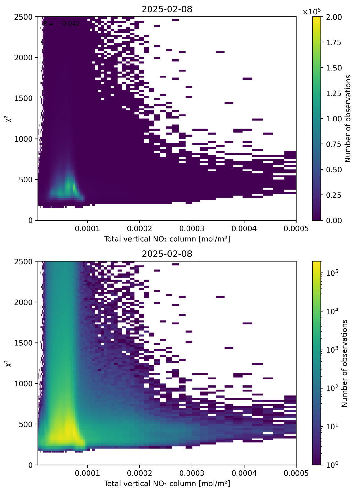
Figure 111: Scatter density plot of “Total vertical NO 2 column” against “ \chi^2 ” for 2025-02-08 to 2025-02-09.
