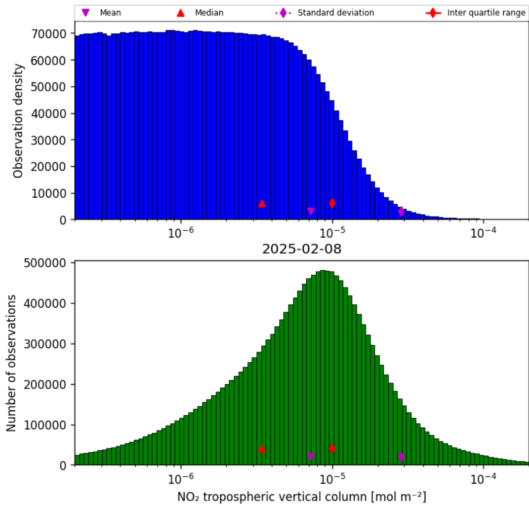
Figure 29: Histogram of “NO 2 tropospheric vertical column” for 2025-02-08 to 2025-02-09
