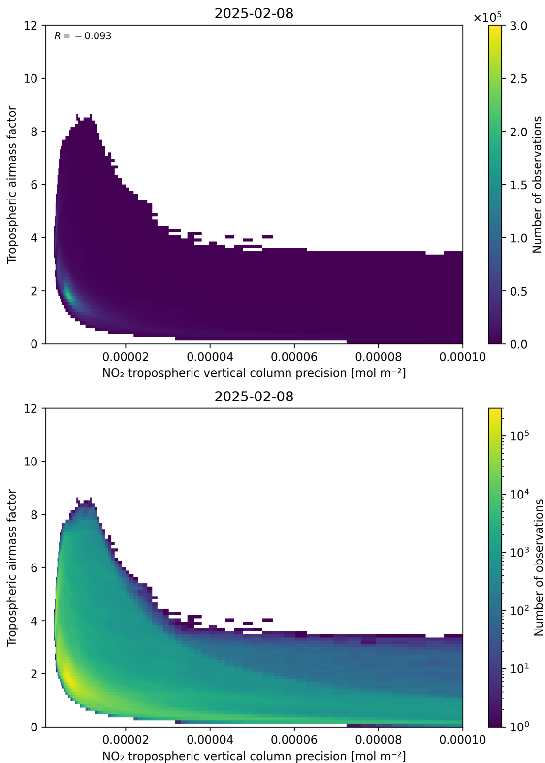
Figure 133: Scatter density plot of “NO 2 tropospheric vertical column precision” against “Tropospheric airmass factor” for 2025-02-08 to 2025-02-09.
