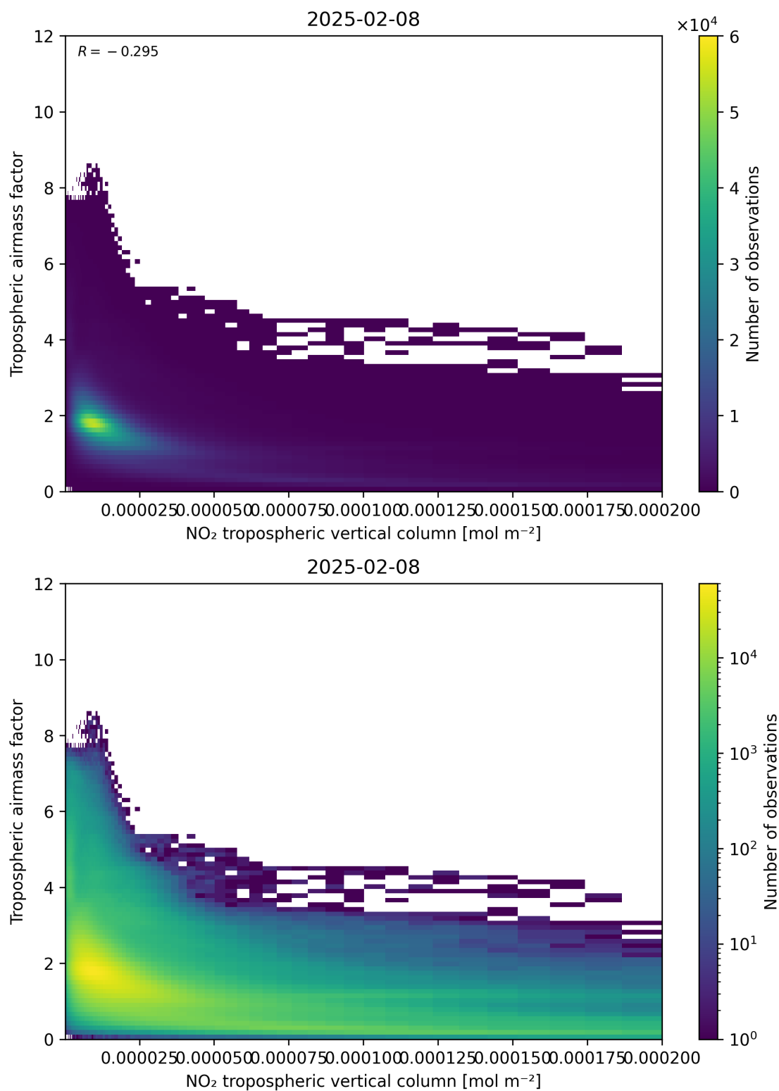
Figure 123: Scatter density plot of “NO 2 tropospheric vertical column” against “Tropospheric air mass factor” for 2025-02-08 to 2025-02-09.
