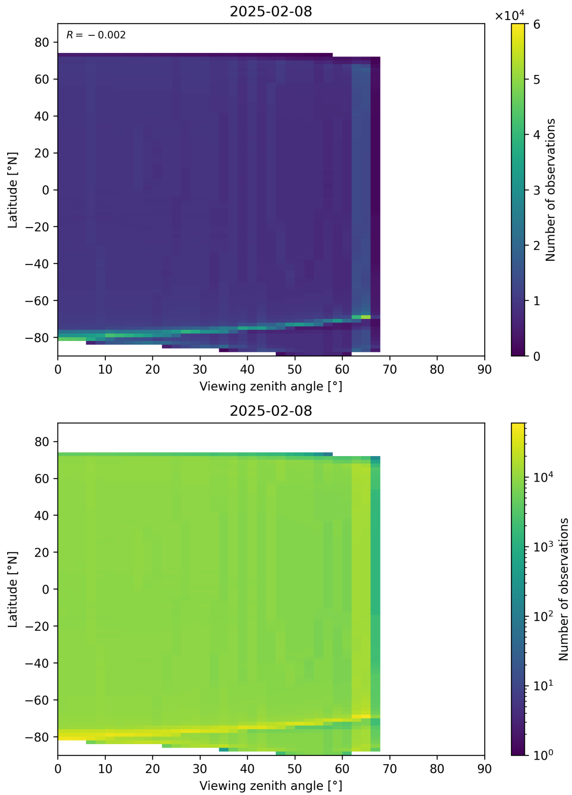
Figure 163: Scatter density plot of “Viewing zenith angle” against “Latitude” for 2025-02-08 to 2025-02-09.
