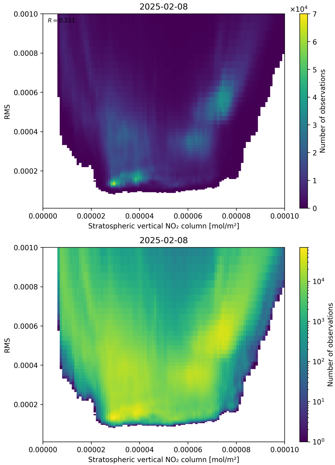
Figure 102: Scatter density plot of “Stratospheric vertical NO 2 column” against “RMS” for 2025-02-08 to 2025-02-09.
