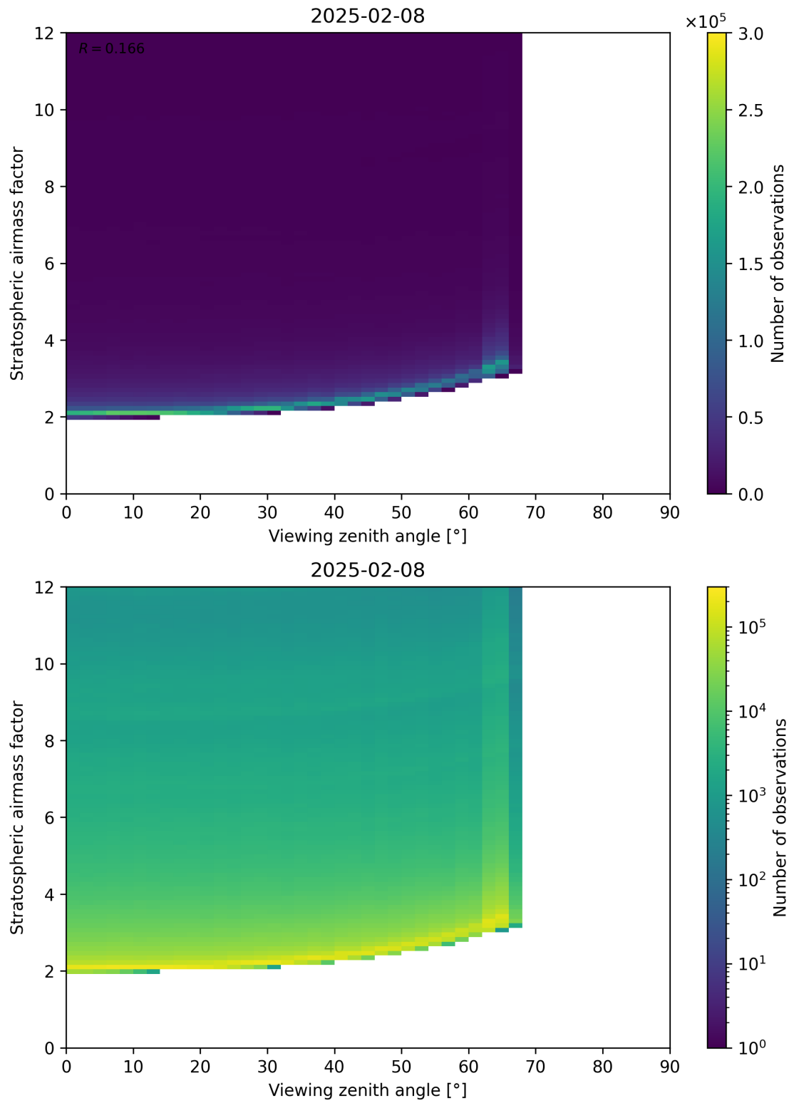
Figure 159: Scatter density plot of “Viewing zenith angle” against “Stratospheric airmass factor” for 2025-02-08 to 2025-02-09.
