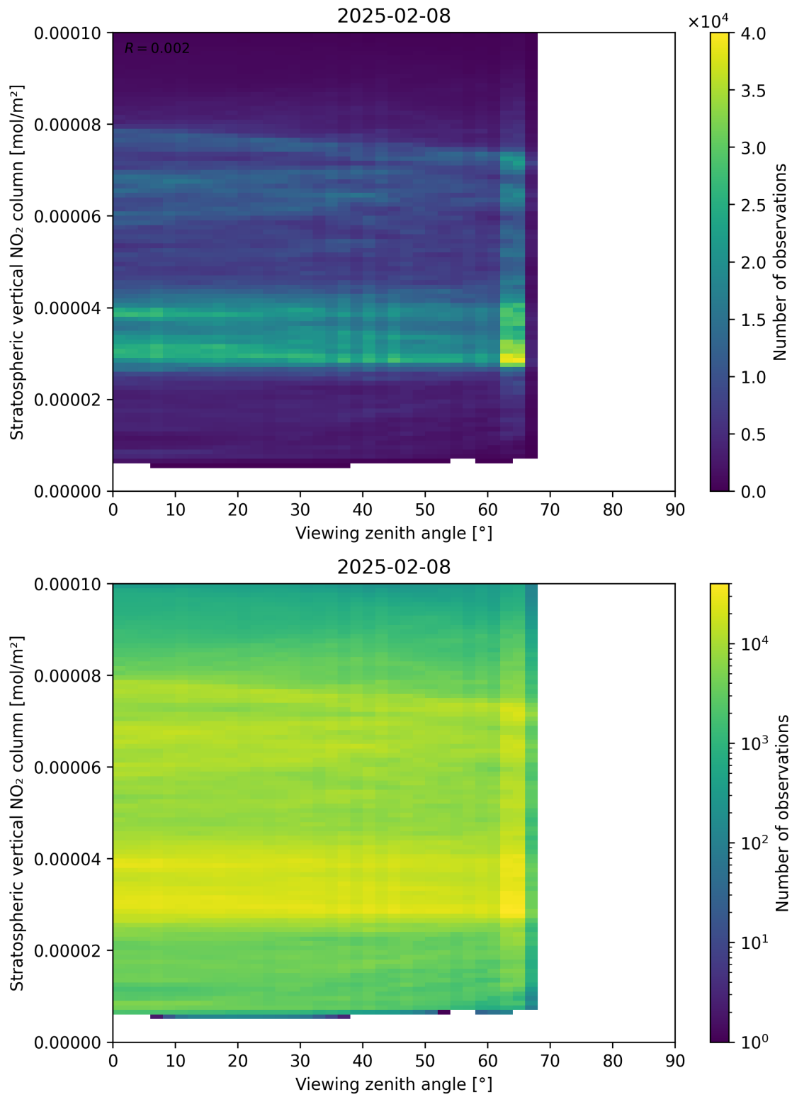
Figure 164: Scatter density plot of “Viewing zenith angle” against “Stratospheric vertical NO 2 column” for 2025-02-08 to 2025-02-09.
