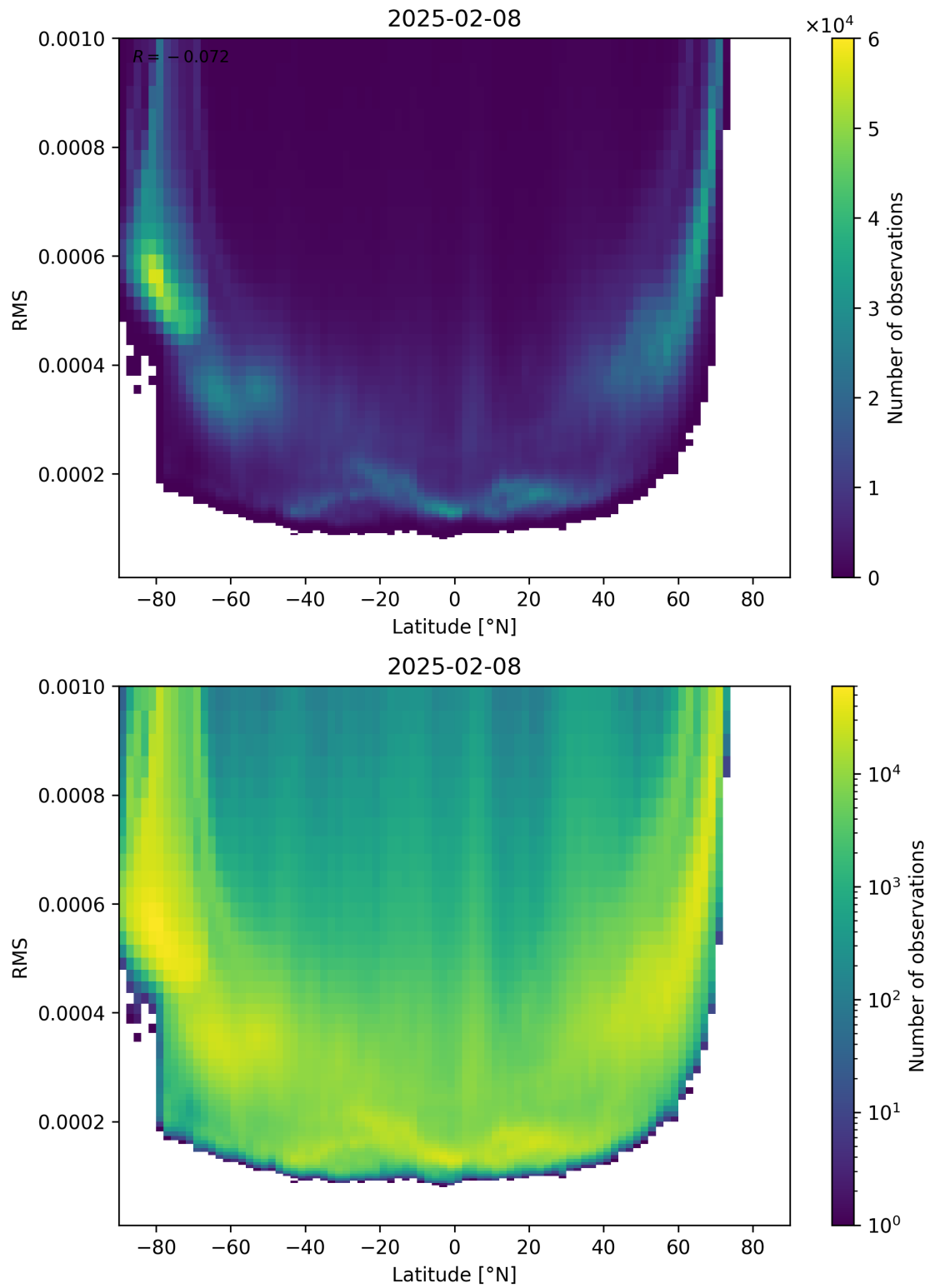
Figure 94: Scatter density plot of “Latitude” against “RMS” for 2025-02-08 to 2025-02-09.
