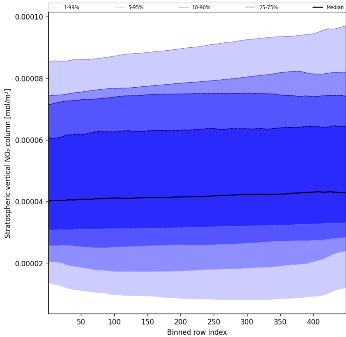
Figure 53: Along track statistics of “Stratospheric vertical NO 2 column” for 2025-02-08 to 2025-02-09
