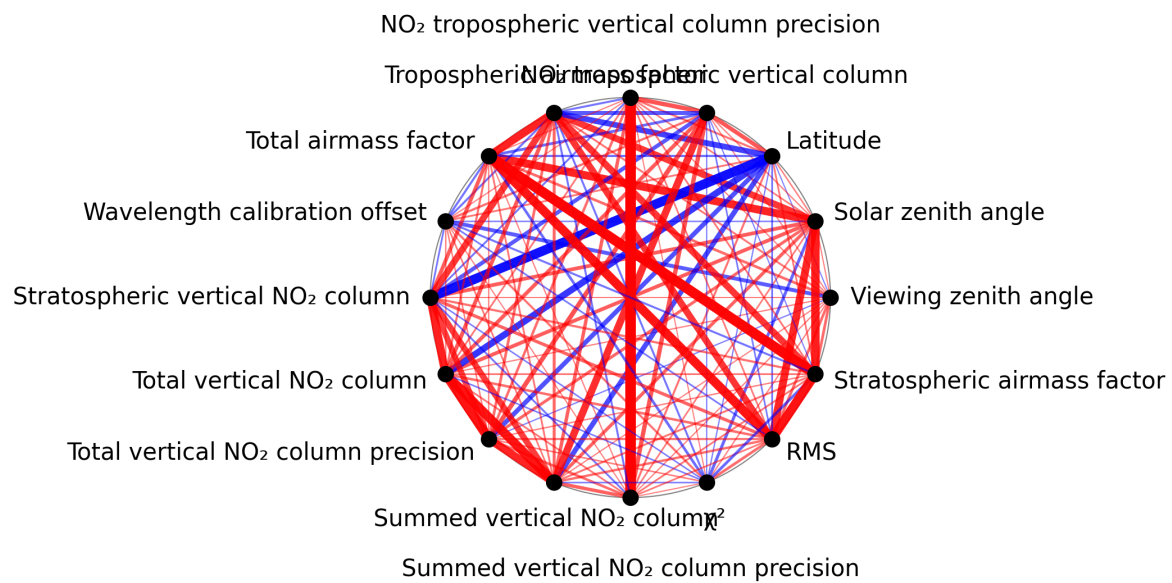
Figure 1: Map of correlation graph for 2025-02-08 to 2025-02-09.
