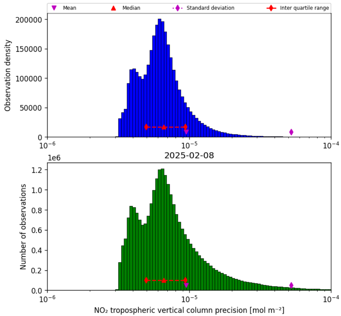
Figure 30: Histogram of “NO 2 tropospheric vertical column precision” for 2025-02-08 to 2025-02-09
