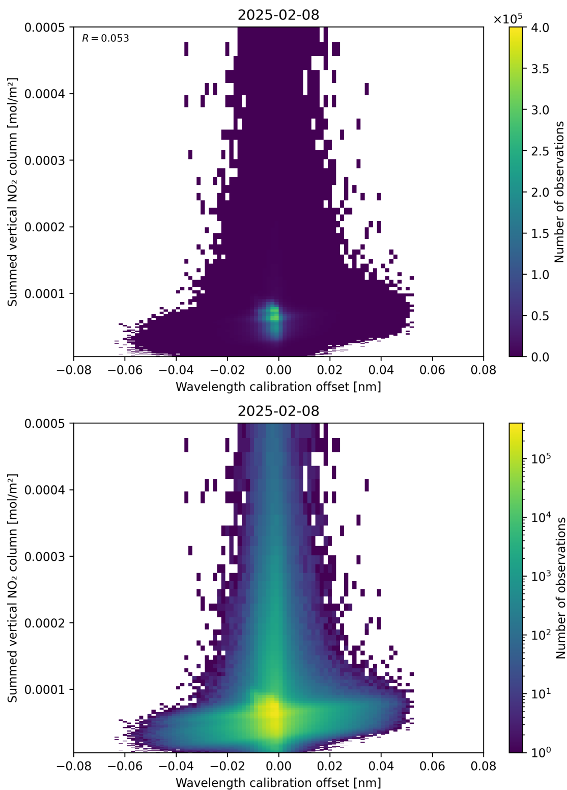
Figure 177: Scatter density plot of “Wavelength calibration offset” against “Summed vertical NO 2 column” for 2025-02-08 to 2025-02-09.
