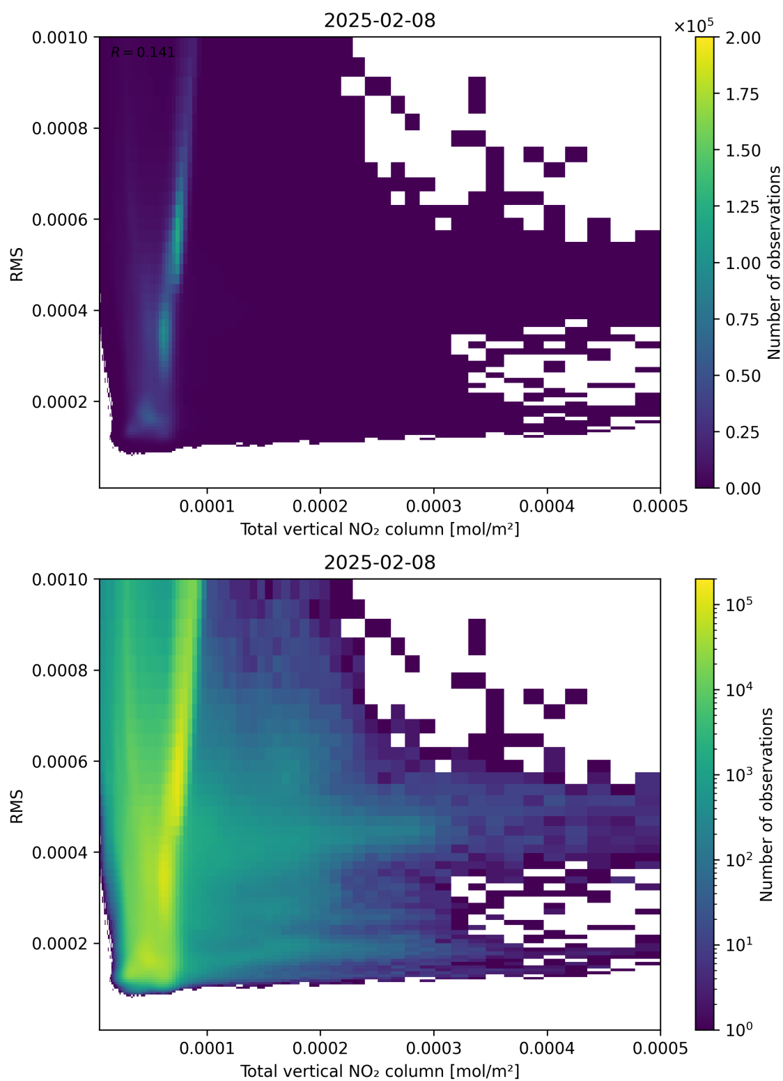
Figure 120: Scatter density plot of “Total vertical NO 2 column” against “RMS” for 2025-02-08 to 2025-02-09.
