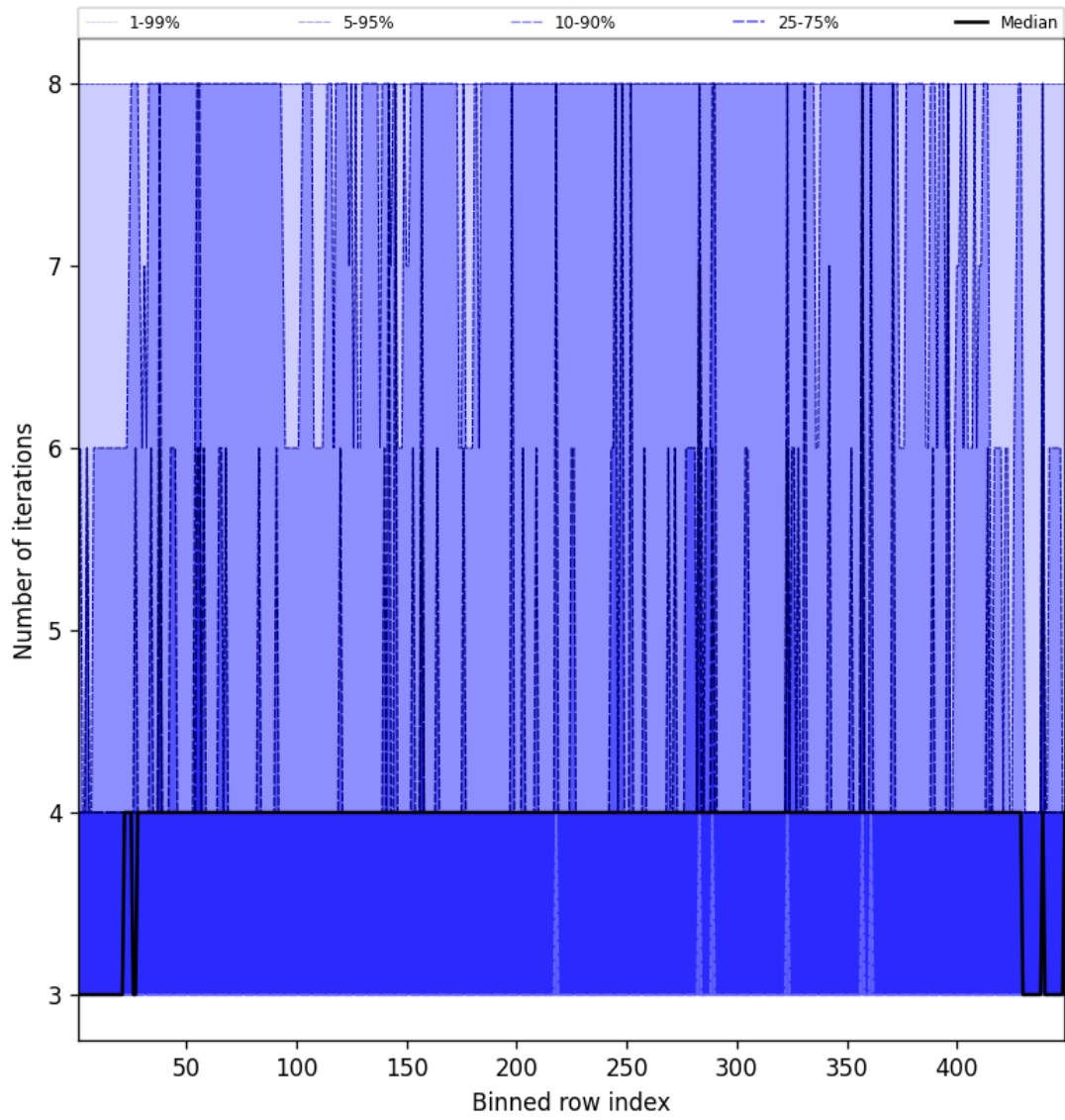
Figure 51: Along track statistics of “Number of iterations” for 2025-02-08 to 2025-02-09
