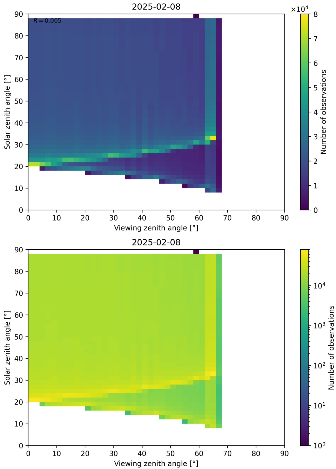
Figure 172: Scatter density plot of “Viewing zenith angle” against “Solar zenith angle” for 2025-02-08 to 2025-02-09.
