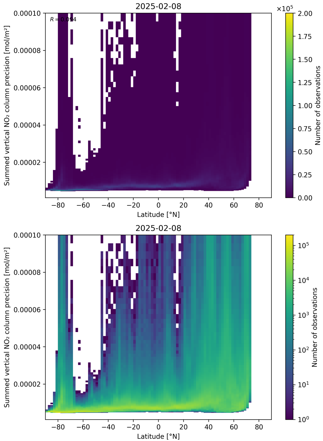
Figure 89: Scatter density plot of “Latitude” against “Summed vertical NO 2 column precision” for 2025-02-08 to 2025-02-09.
