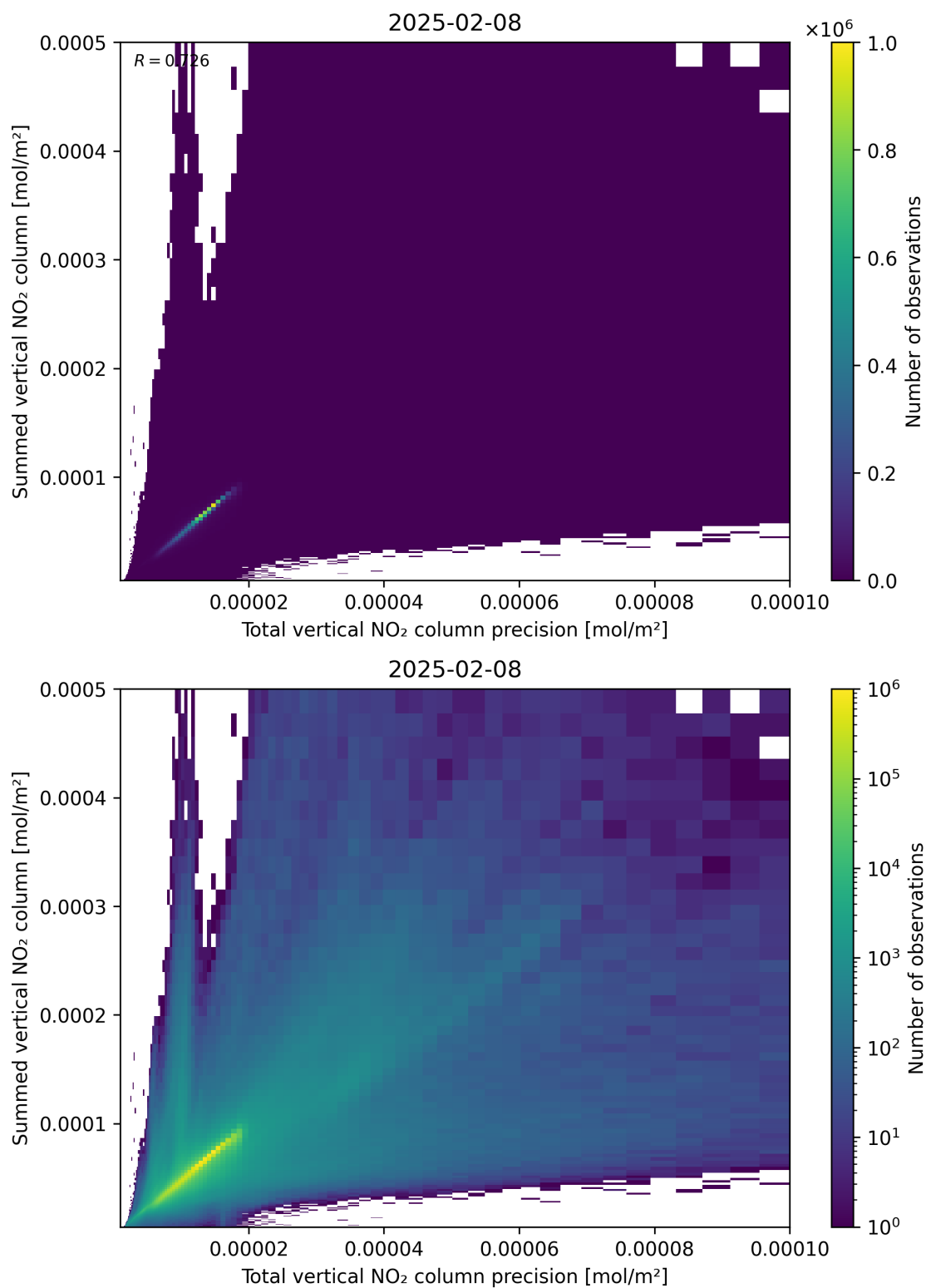
Figure 117: Scatter density plot of “Total vertical NO 2 column precision” against “Summed vertical NO 2 column” for 2025-02-08 to 2025-02-09.
