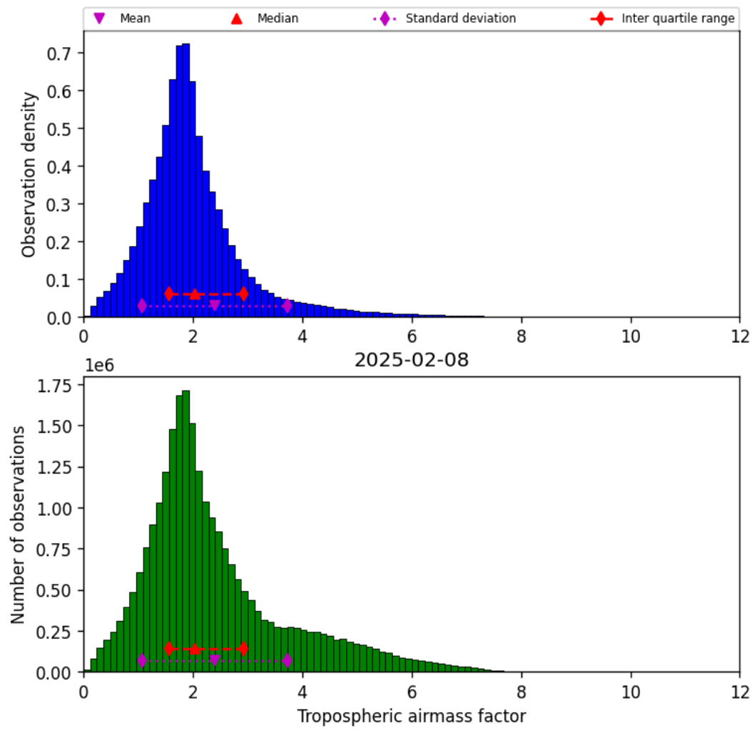
Figure 31: Histogram of “Tropospheric airmass factor” for 2025-02-08 to 2025-02-09
