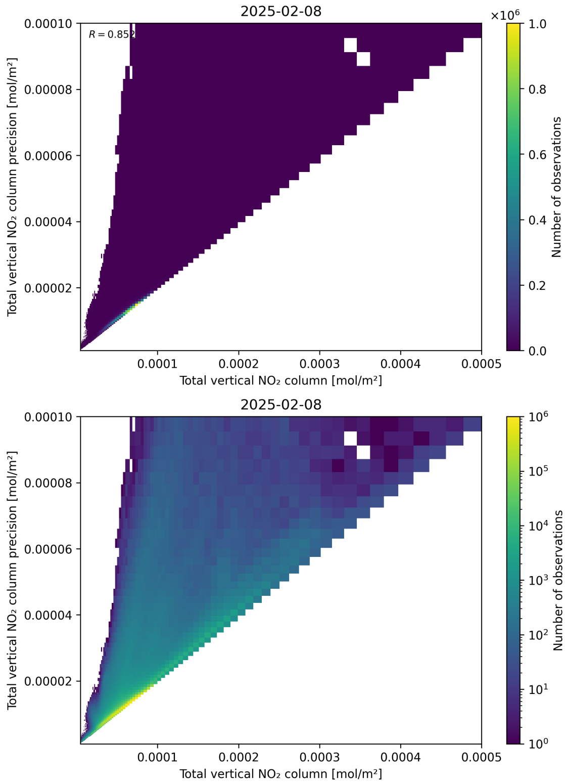
Figure 114: Scatter density plot of “Total vertical NO 2 column” against “Total vertical NO 2 column precision” for 2025-02-08 to 2025-02-09.
