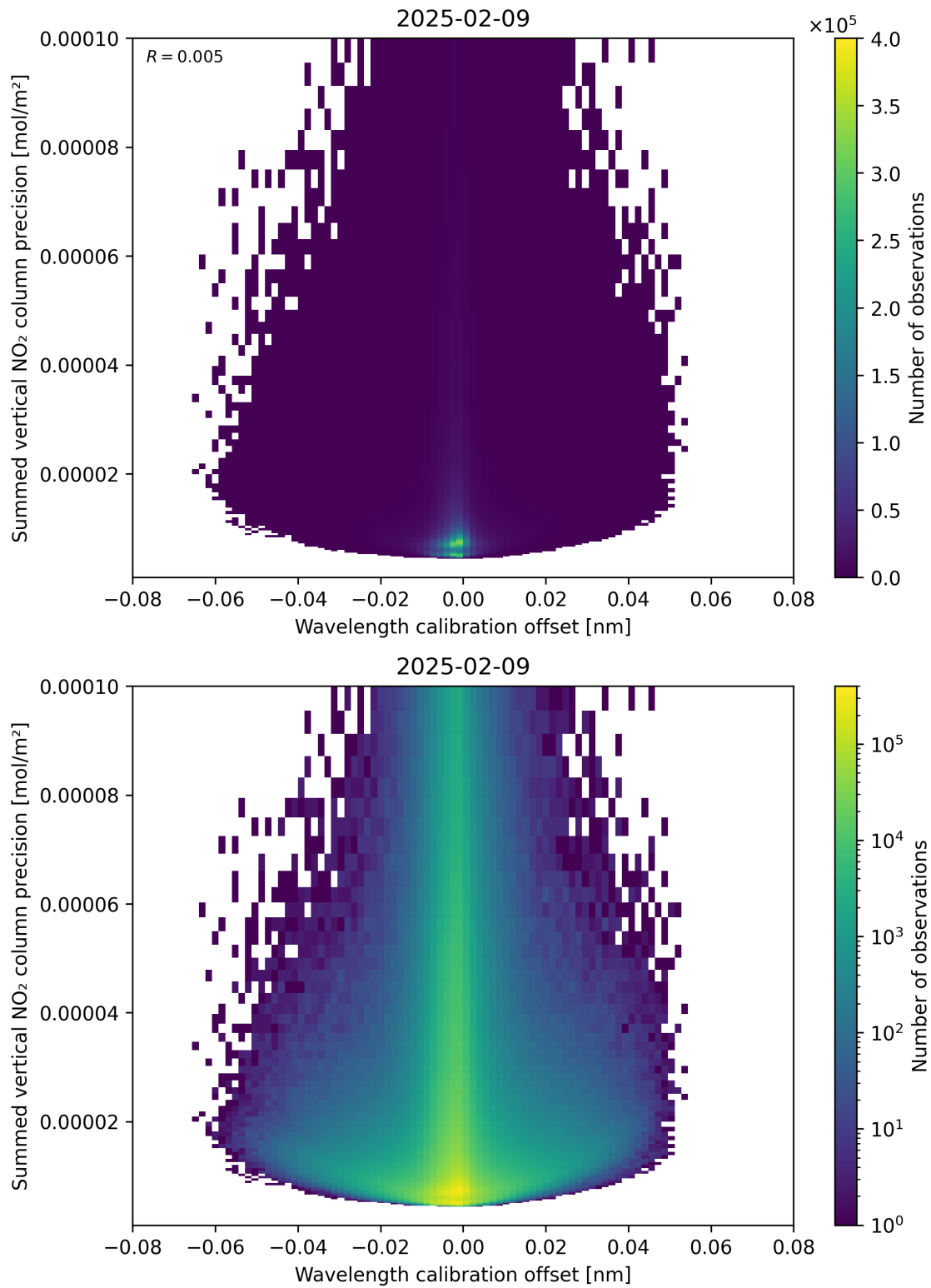
Figure 178: Scatter density plot of “Wavelength calibration offset” against “Summed vertical NO 2 column precision” for 2025-02-08 to 2025-02-10.
