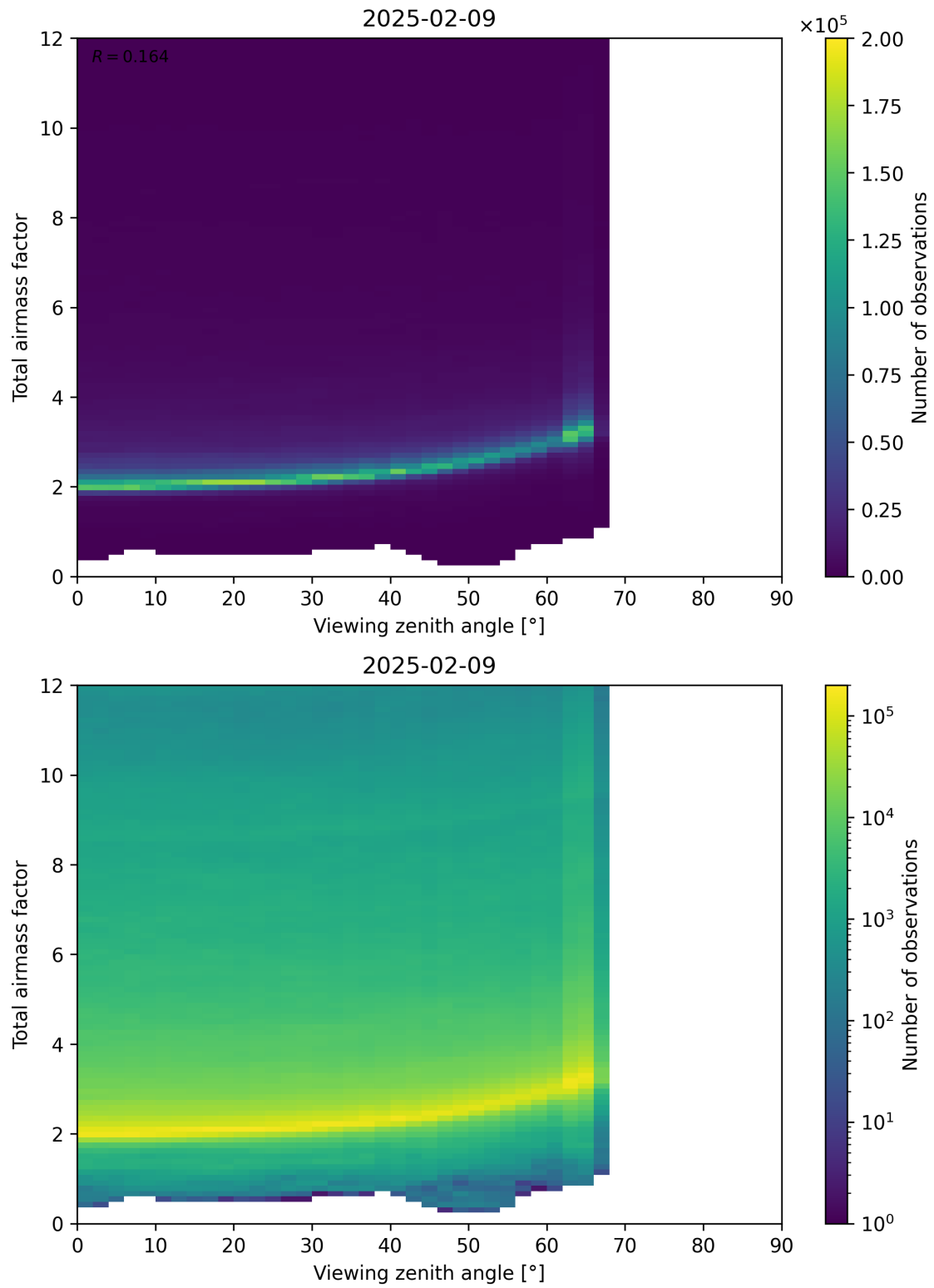
Figure 160: Scatter density plot of “Viewing zenith angle” against “Total airmass factor” for 2025-02-08 to 2025-02-10.
