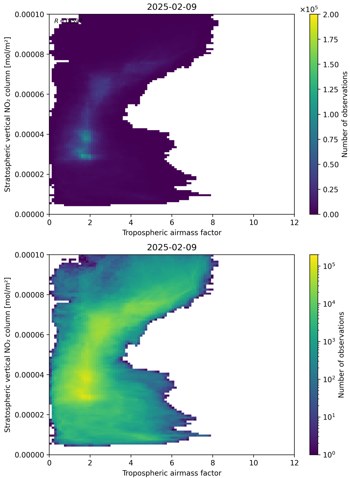
Figure 74: Scatter density plot of “Tropospheric air mass factor” against “Stratospheric vertical NO 2 column” for 2025-02-08 to 2025-02-10.
