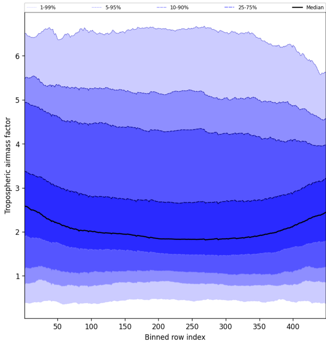
Figure 48: Along track statistics of “Tropospheric airmass factor” for 2025-02-08 to 2025-02-10
