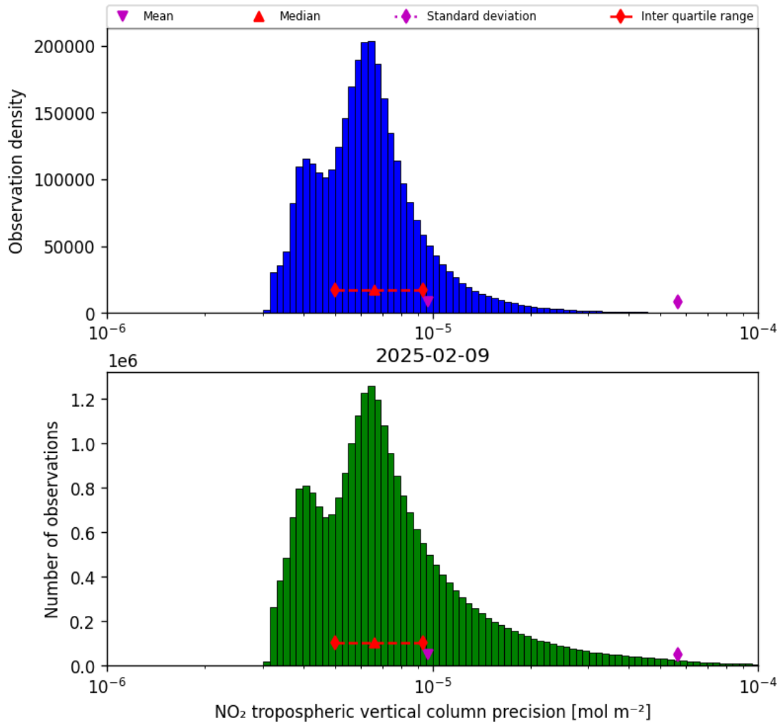
Figure 30: Histogram of “NO 2 tropospheric vertical column precision” for 2025-02-08 to 2025-02-10
