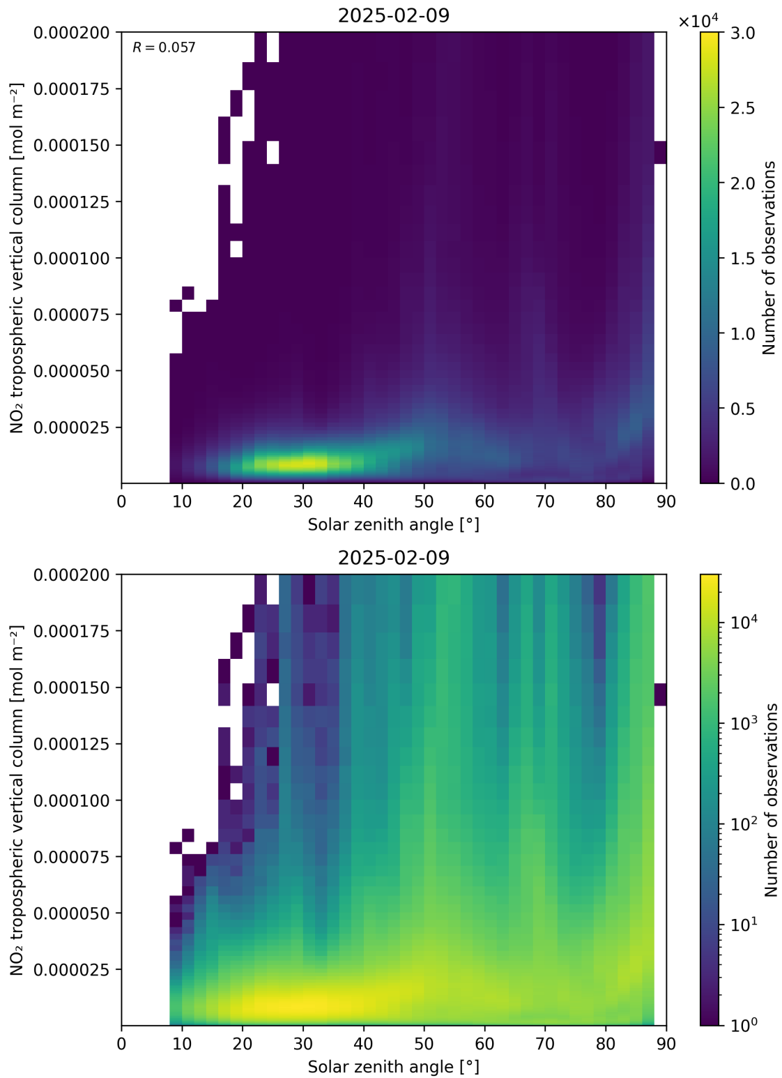
Figure 155: Scatter density plot of “Solar zenith angle” against “NO 2 tropospheric vertical column” for 2025-02-08 to 2025-02-10.
