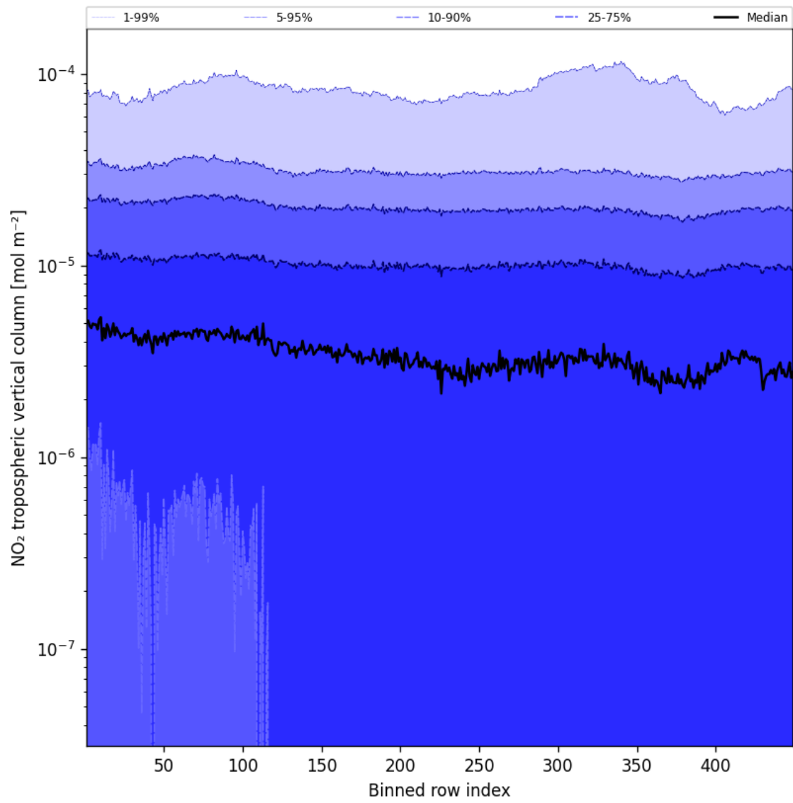
Figure 46: Along track statistics of “NO 2 tropospheric vertical column” for 2025-02-08 to 2025-02-10
