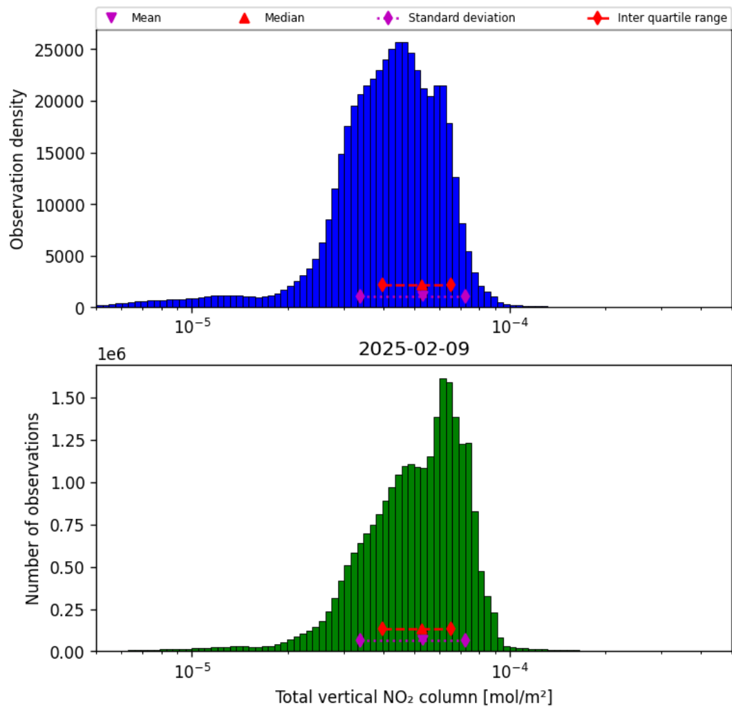
Figure 38: Histogram of “Total vertical NO 2 column” for 2025-02-08 to 2025-02-10
