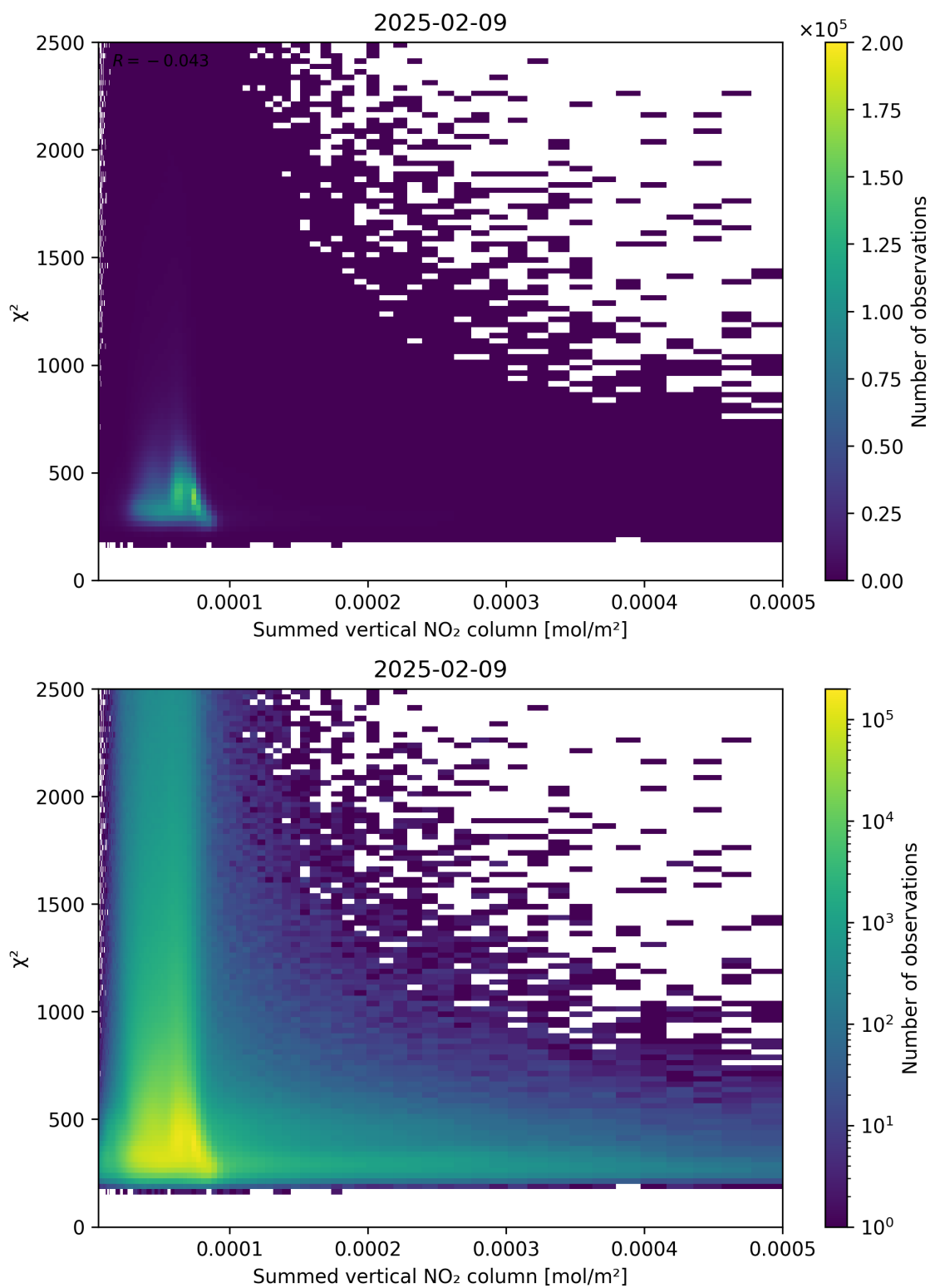
Figure 104: Scatter density plot of “Summed vertical NO 2 column” against “ \chi^2 ” for 2025-02-08 to 2025-02-10.
