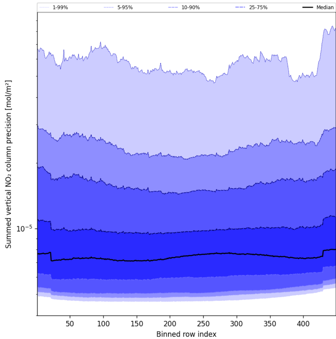
Figure 58: Along track statistics of “Summed vertical NO 2 column precision” for 2025-02-08 to 2025-02-10
