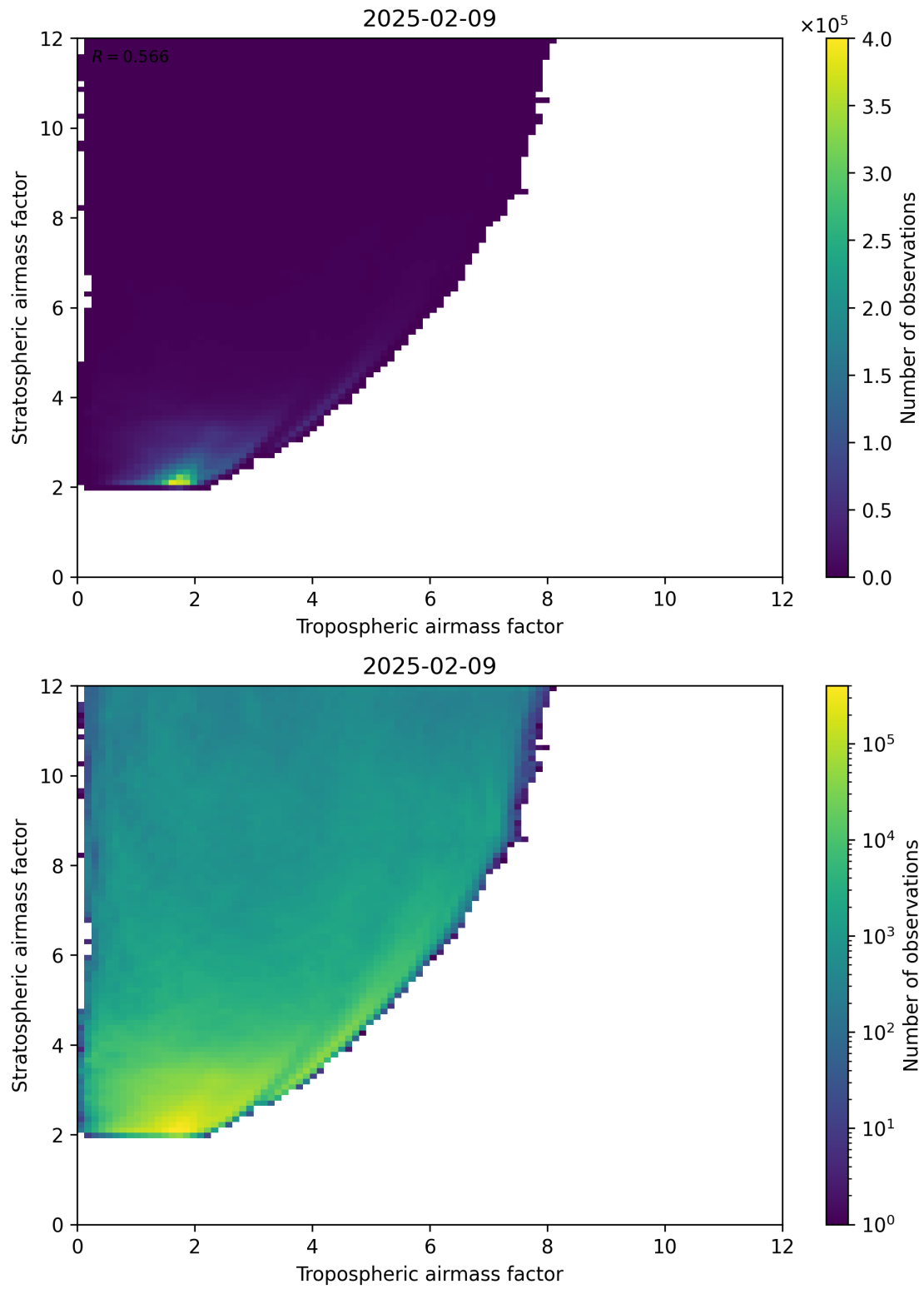
Figure 71: Scatter density plot of “Tropospheric airmass factor” against “Stratospheric airmass factor” for 2025-02-08 to 2025-02-10.
