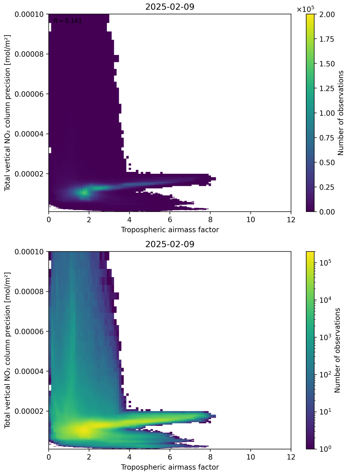
Figure 78: Scatter density plot of “Tropospheric air mass factor” against “Total vertical NO 2 column precision” for 2025-02-08 to 2025-02-10.
