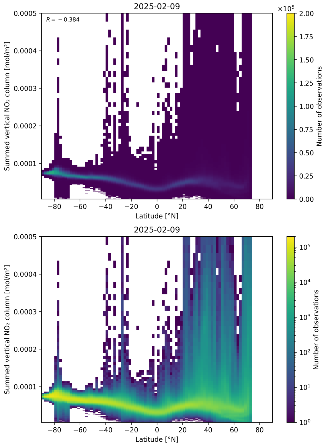
Figure 88: Scatter density plot of “Latitude” against “Summed vertical NO 2 column” for 2025-02-08 to 2025-02-10.
