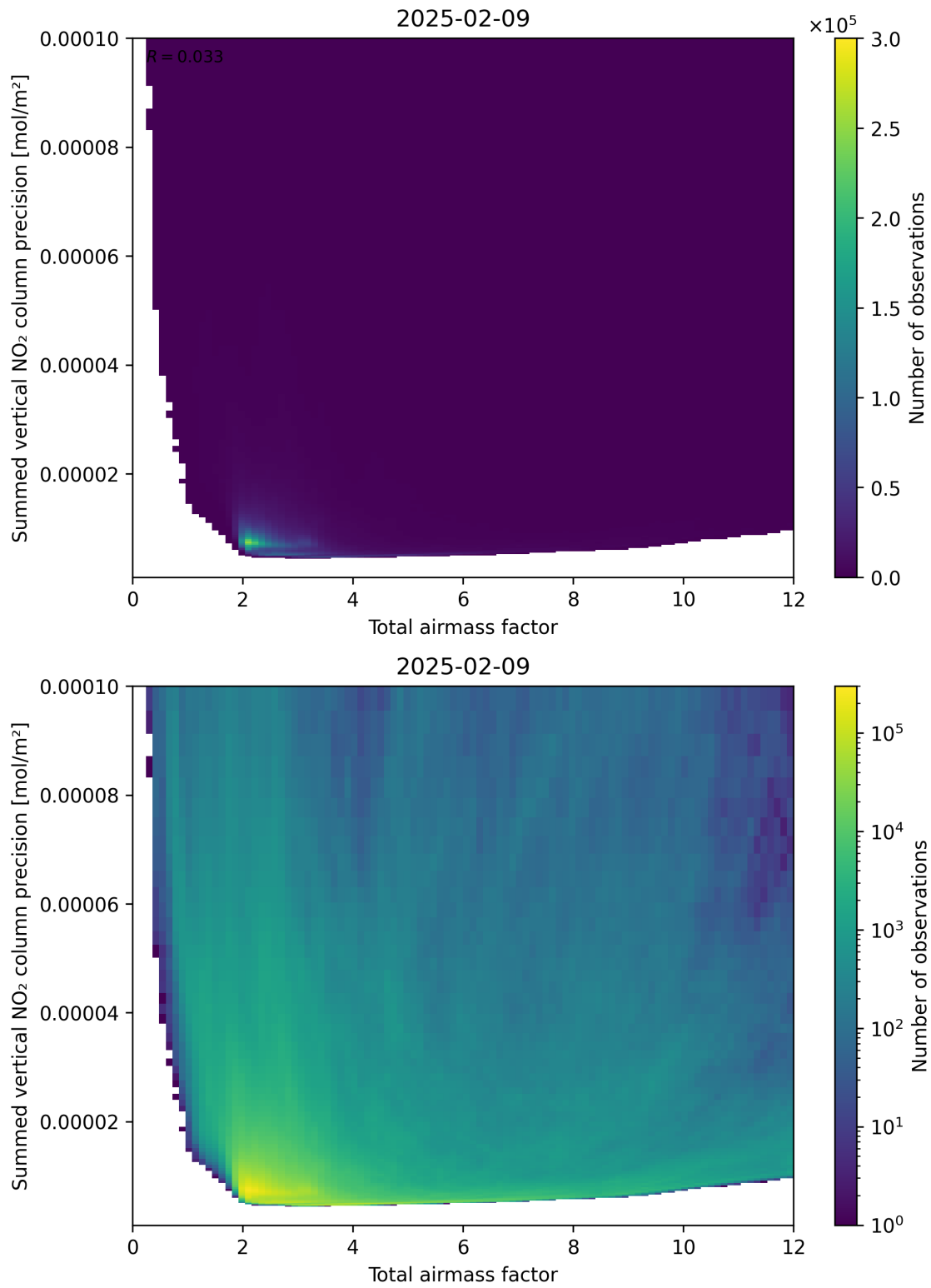
Figure 66: Scatter density plot of “Total airmass factor” against “Summed vertical NO 2 column precision” for 2025-02-08 to 2025-02-10.
