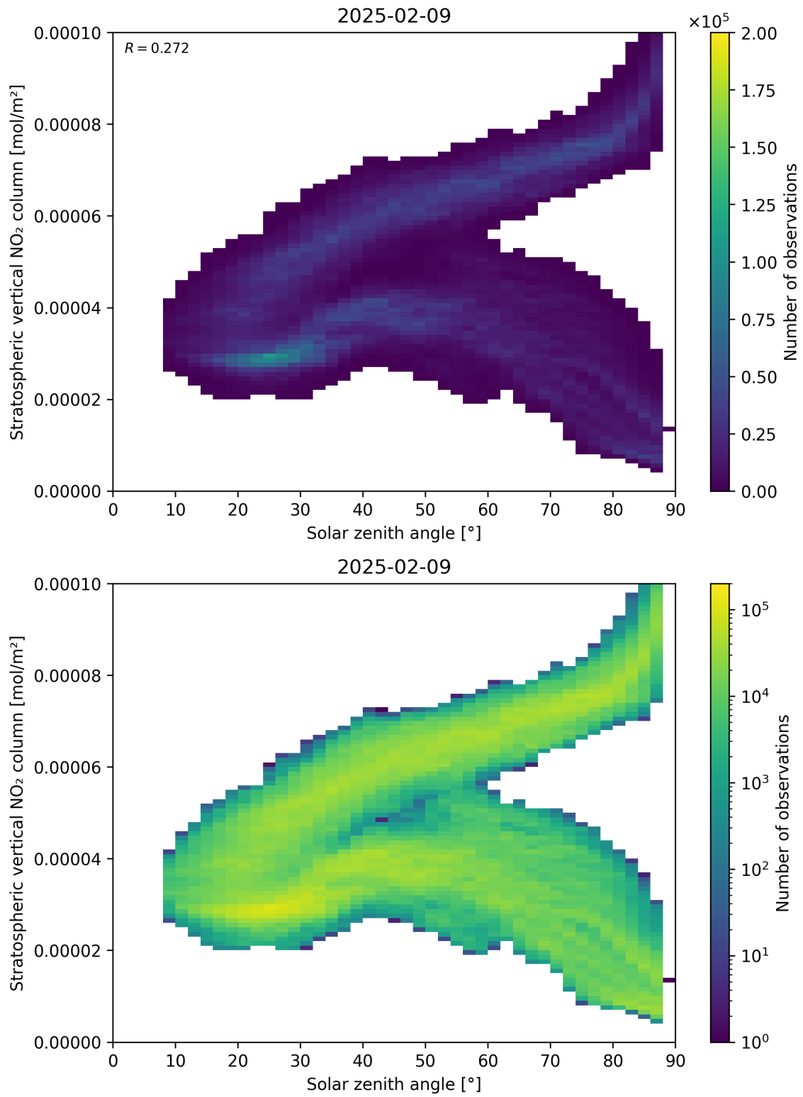
Figure 150: Scatter density plot of “Solar zenith angle” against “Stratospheric vertical NO 2 column” for 2025-02-08 to 2025-02-10.
