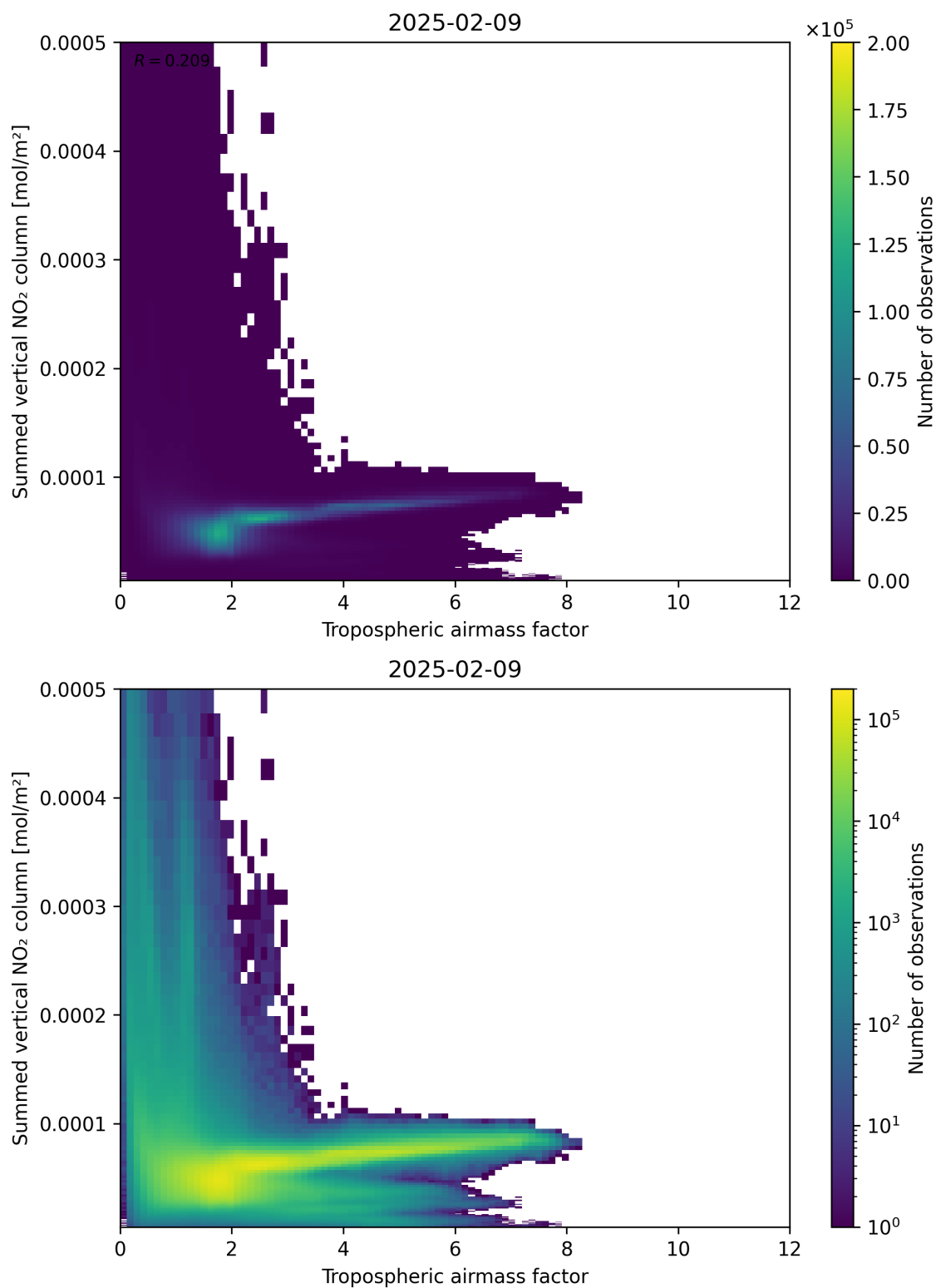
Figure 75: Scatter density plot of “Tropospheric air mass factor” against “Summed vertical NO 2 column” for 2025-02-08 to 2025-02-10.
