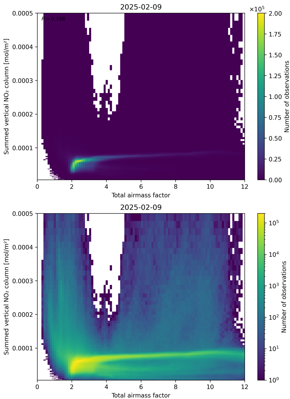
Figure 65: Scatter density plot of “Total airmass factor” against “Summed vertical NO 2 column” for 2025-02-08 to 2025-02-10.
