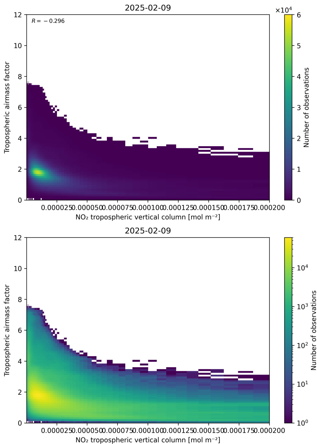
Figure 123: Scatter density plot of “NO 2 tropospheric vertical column” against “Tropospheric air mass factor” for 2025-02-08 to 2025-02-10.
