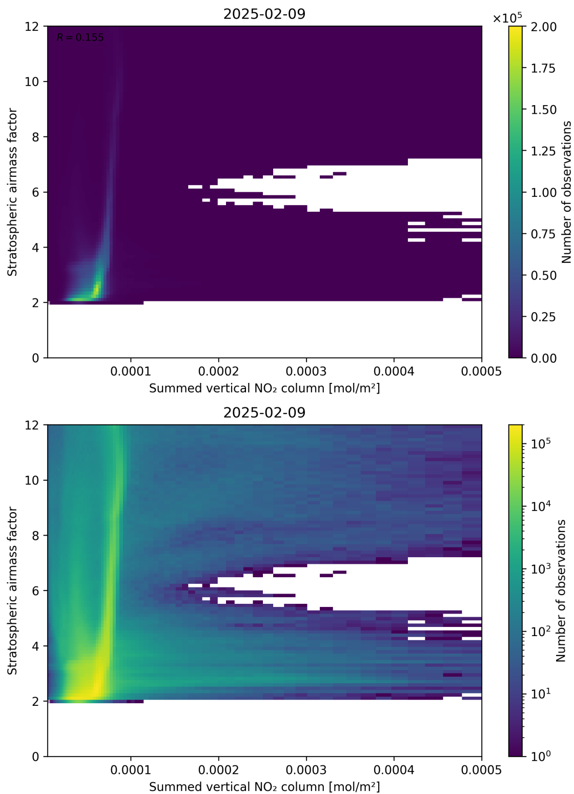
Figure 103: Scatter density plot of “Summed vertical NO 2 column” against “Stratospheric air mass factor” for 2025-02-08 to 2025-02-10.
