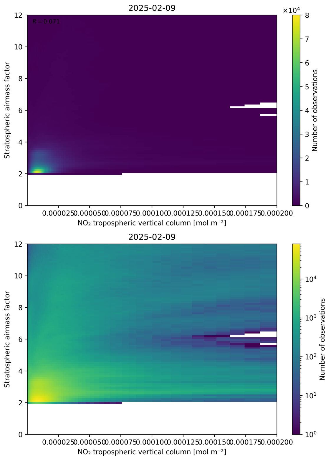
Figure 121: Scatter density plot of “NO 2 tropospheric vertical column” against “Stratospheric air mass factor” for 2025-02-08 to 2025-02-10.
