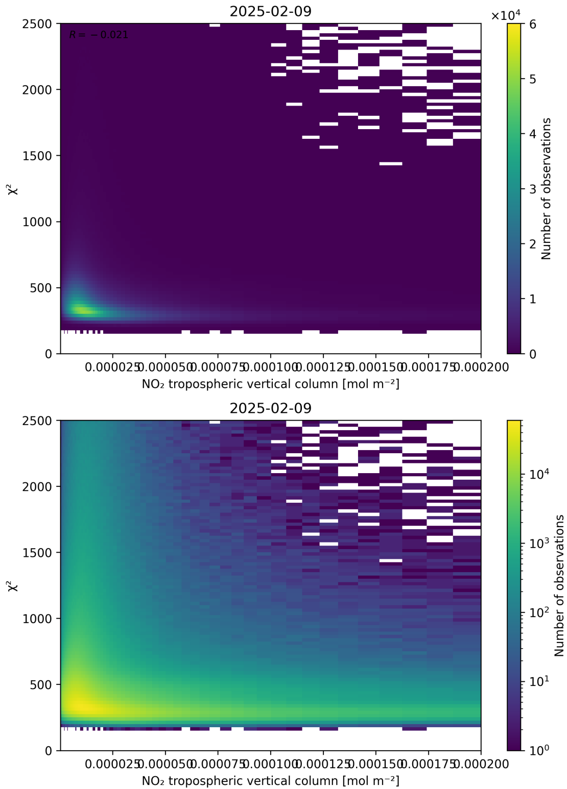
Figure 124: Scatter density plot of “NO 2 tropospheric vertical column” against “ \chi^2 ” for 2025-02-08 to 2025-02-10.
