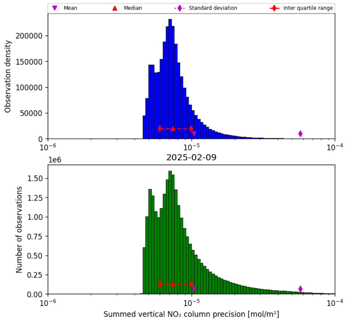
Figure 41: Histogram of “Summed vertical NO 2 column precision” for 2025-02-08 to 2025-02-10
