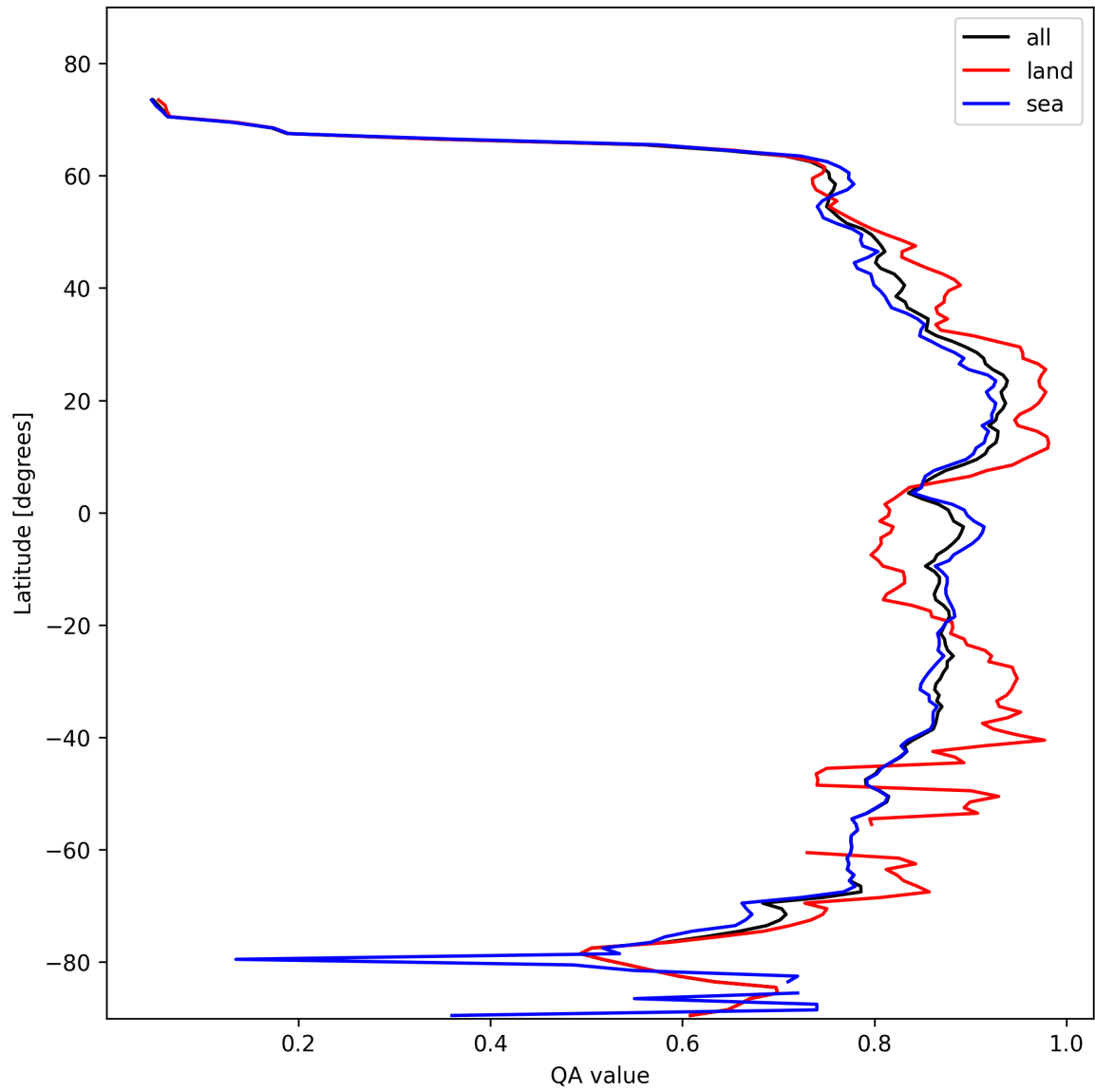
Figure 11: Zonal average of “QA value” for 2025-02-08 to 2025-02-10.
