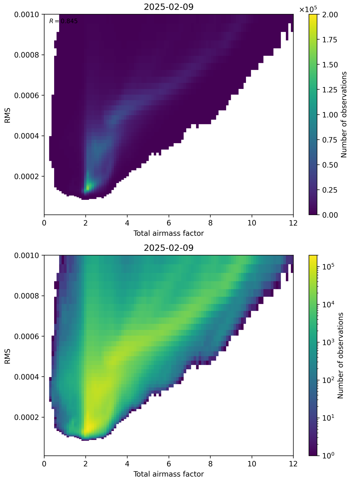
Figure 69: Scatter density plot of “Total airmass factor” against “RMS” for 2025-02-08 to 2025-02-10.
