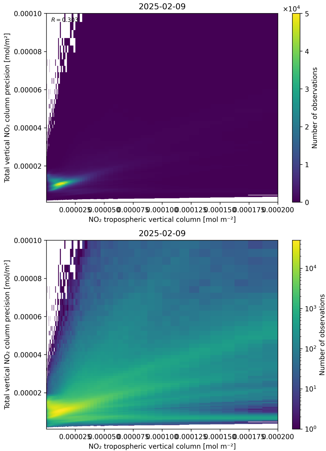
Figure 129: Scatter density plot of “NO 2 tropospheric vertical column” against “Total vertical NO 2 column precision” for 2025-02-08 to 2025-02-10.
