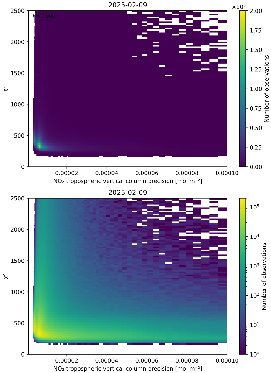
Figure 134: Scatter density plot of “NO 2 tropospheric vertical column precision” against “ \chi^2 ” for 2025-02-08 to 2025-02-10.
