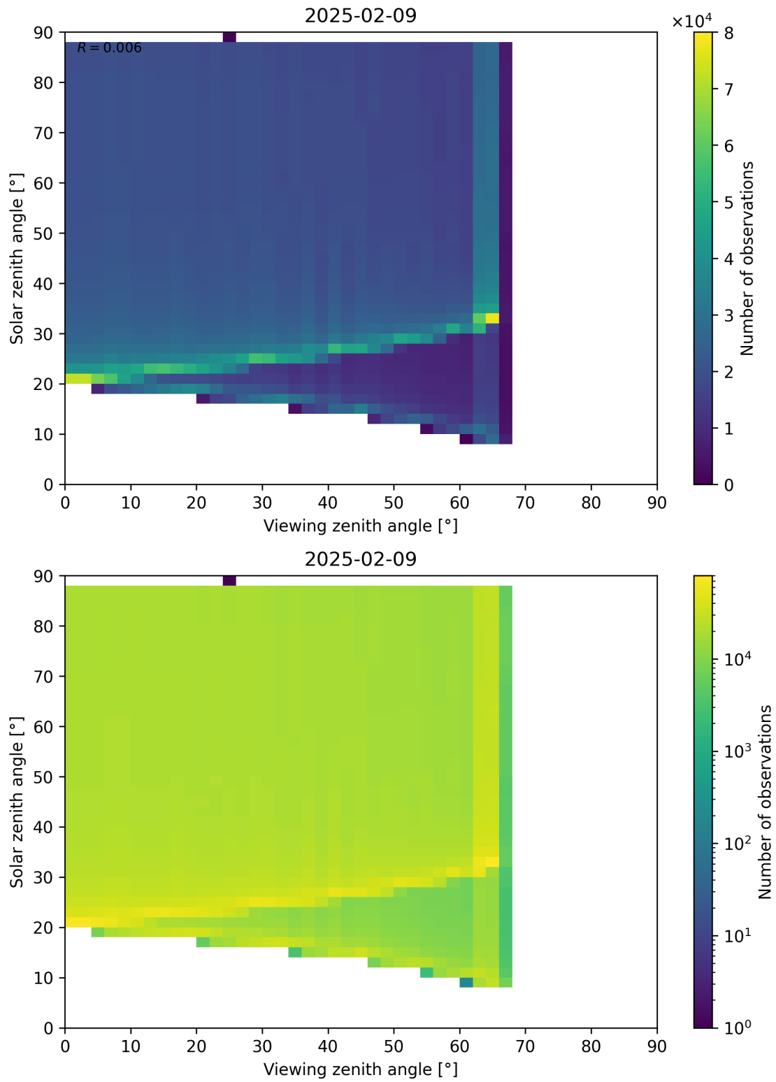
Figure 172: Scatter density plot of “Viewing zenith angle” against “Solar zenith angle” for 2025-02-08 to 2025-02-10.
