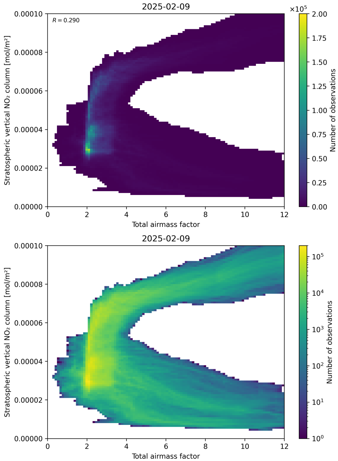
Figure 64: Scatter density plot of “Total airmass factor” against “Stratospheric vertical \text{NO}_2 column” for 2025-02-08 to 2025-02-10.
