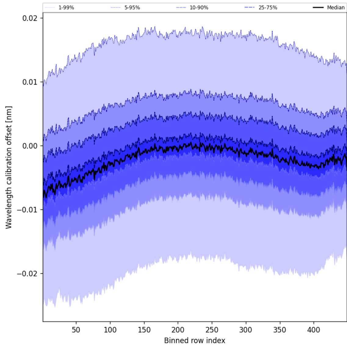
Figure 52: Along track statistics of “Wavelength calibration offset” for 2025-02-08 to 2025-02-10
