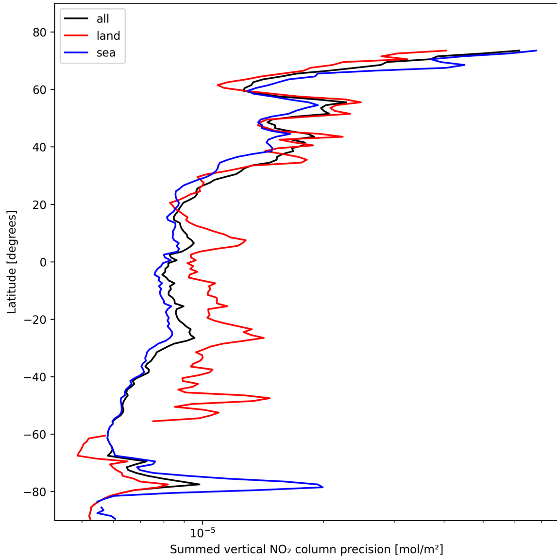
Figure 24: Zonal average of “Summed vertical NO 2 column precision” for 2025-02-08 to 2025-02-10.
