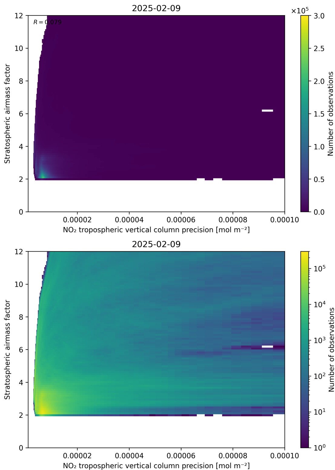
Figure 131: Scatter density plot of “NO 2 tropospheric vertical column precision” against “Stratospheric airmass factor” for 2025-02-08 to 2025-02-10.
