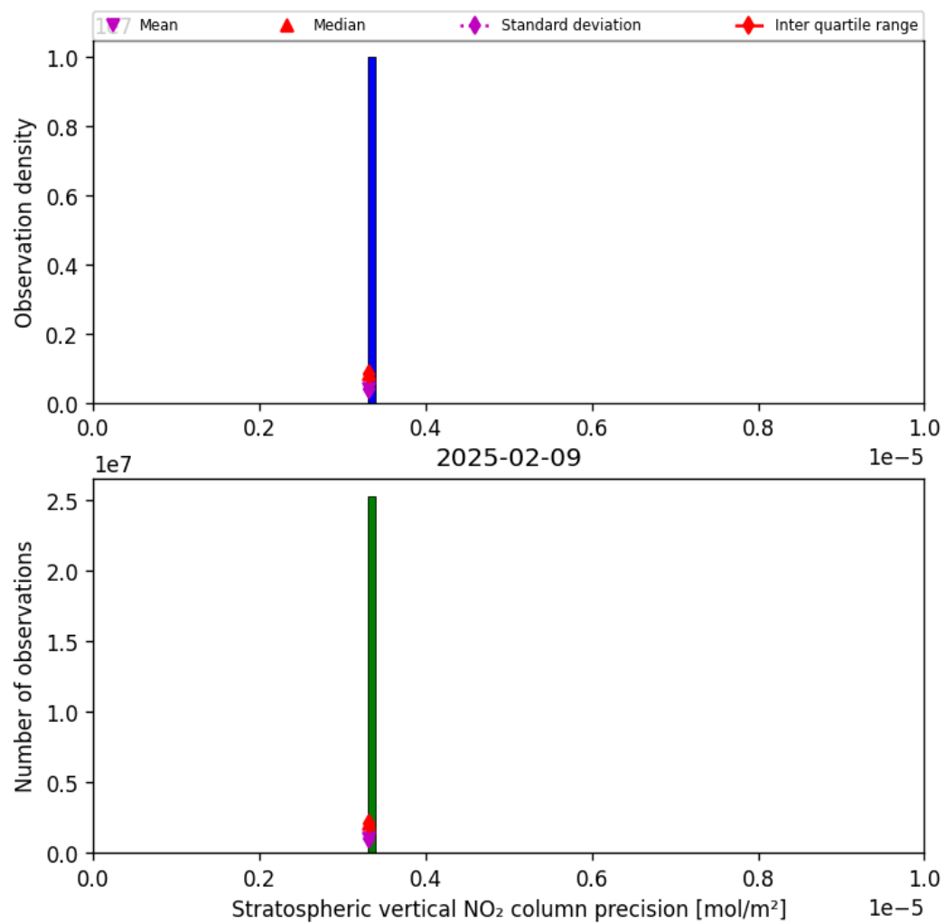
Figure 37: Histogram of “Stratospheric vertical NO 2 column precision” for 2025-02-08 to 2025-02-10
