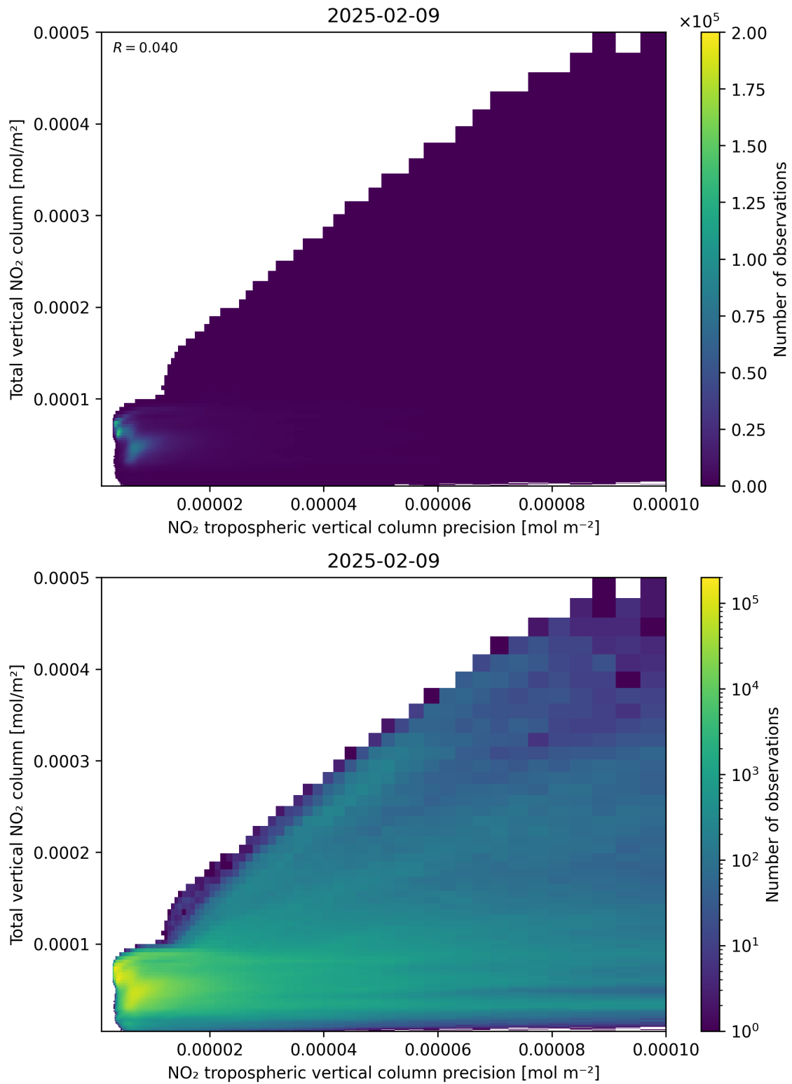
Figure 138: Scatter density plot of “NO 2 tropospheric vertical column precision” against “Total vertical NO 2 column” for 2025-02-08 to 2025-02-10.
