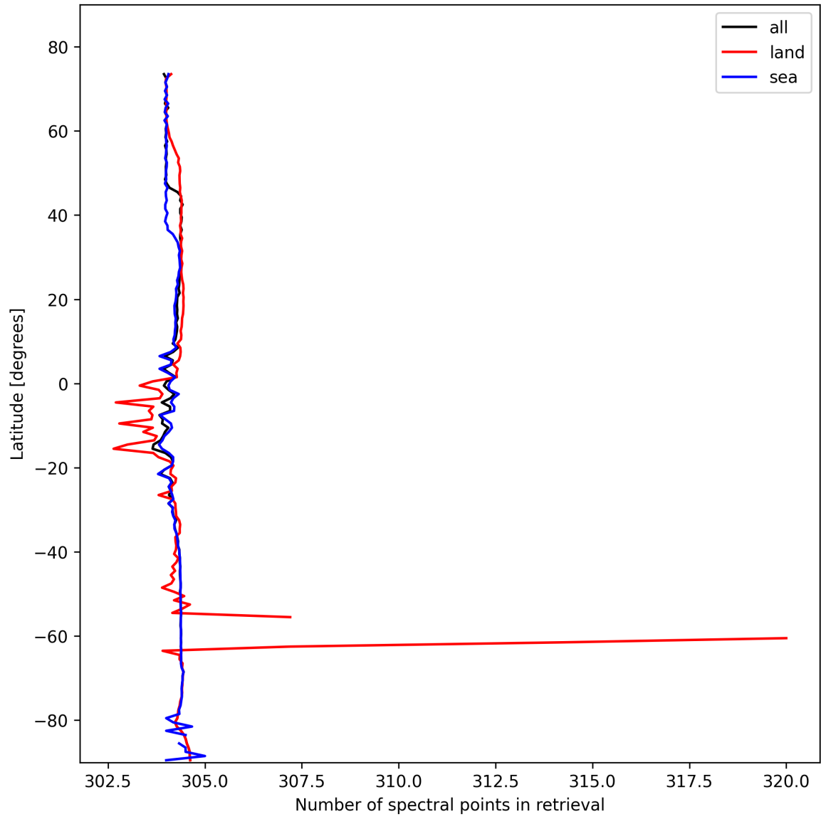
Figure 16: Zonal average of “Number of spectral points in retrieval” for 2025-02-08 to 2025-02-10.
