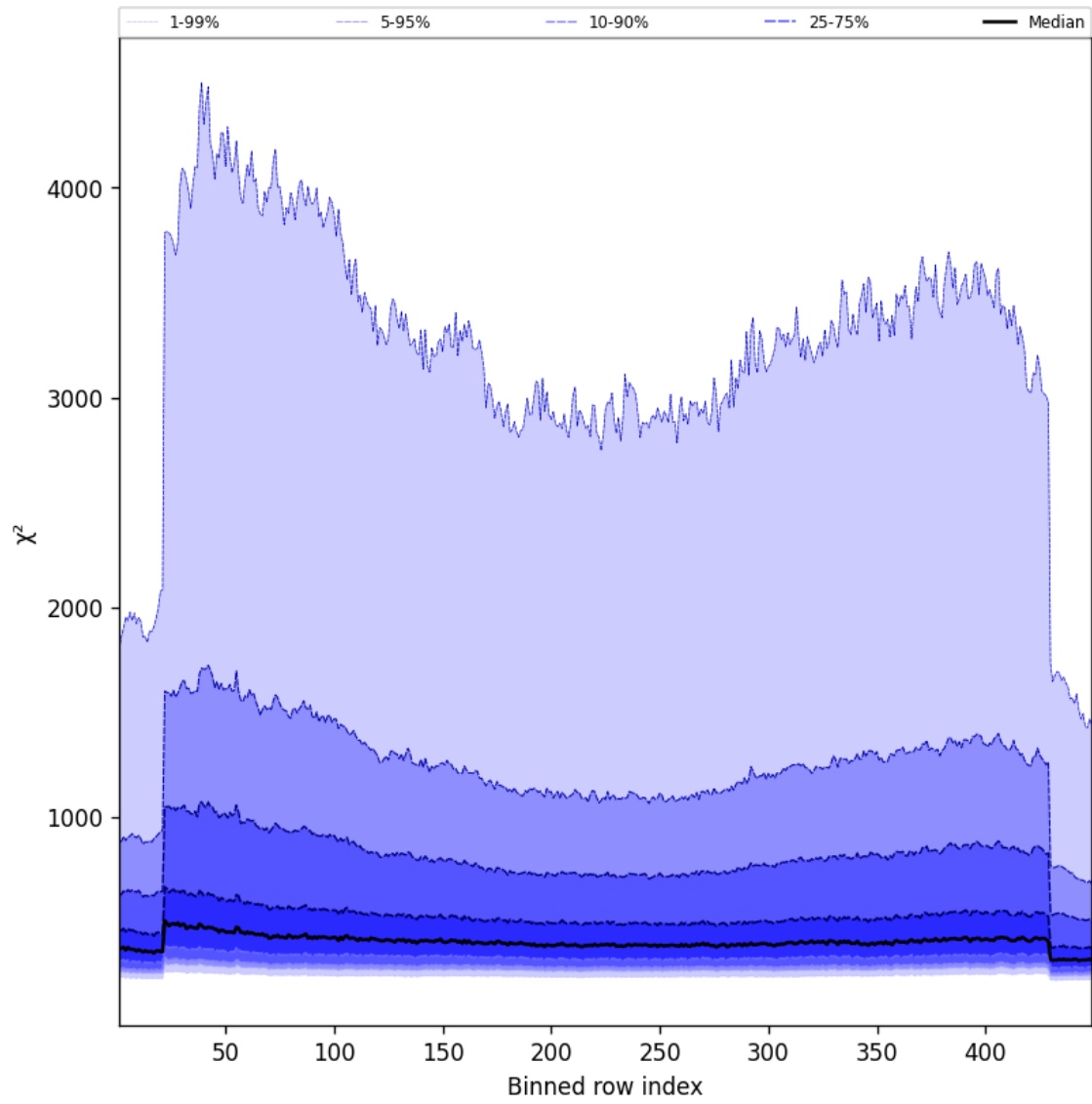
Figure 59: Along track statistics of “ \chi^2 ” for 2025-02-08 to 2025-02-10
