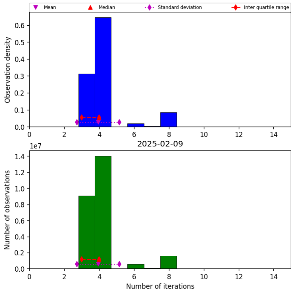
Figure 34: Histogram of “Number of iterations” for 2025-02-08 to 2025-02-10
