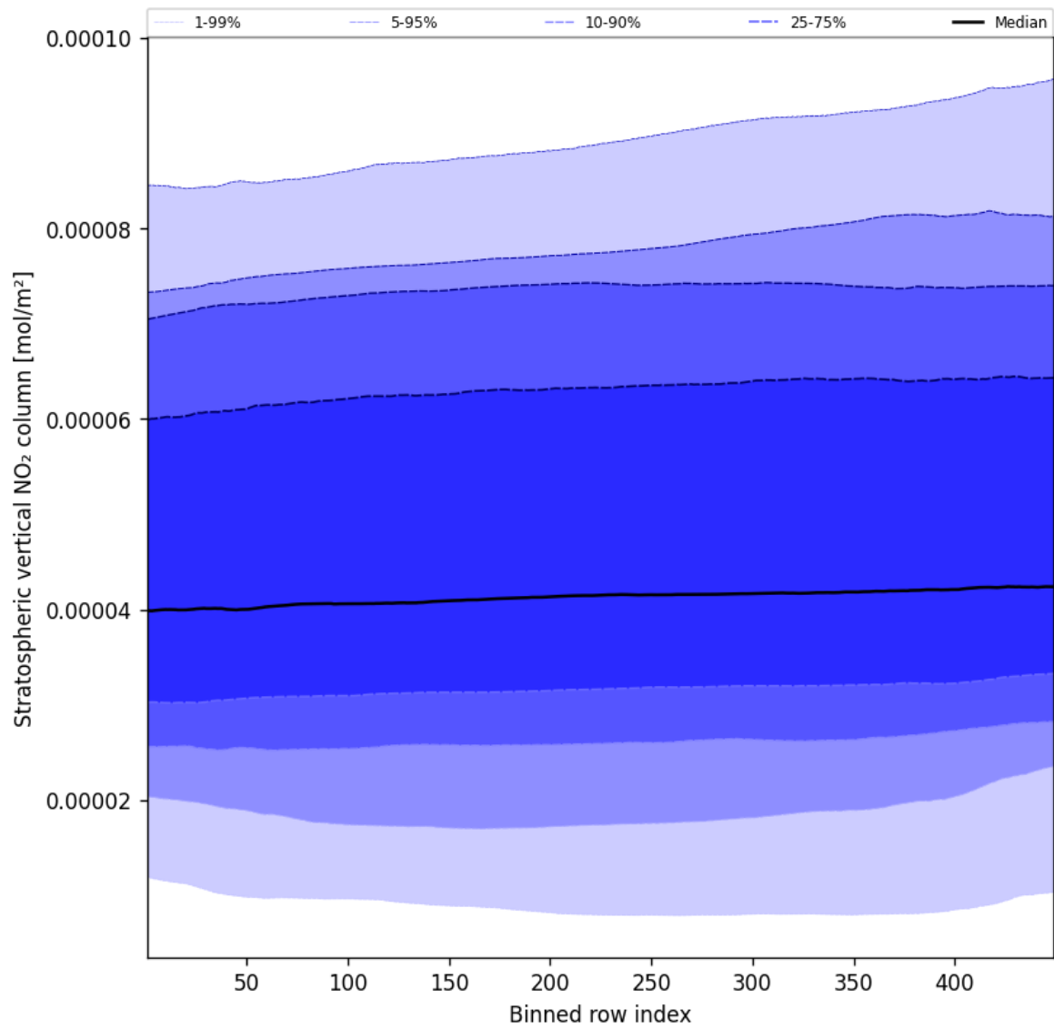
Figure 53: Along track statistics of “Stratospheric vertical NO 2 column” for 2025-02-08 to 2025-02-10
