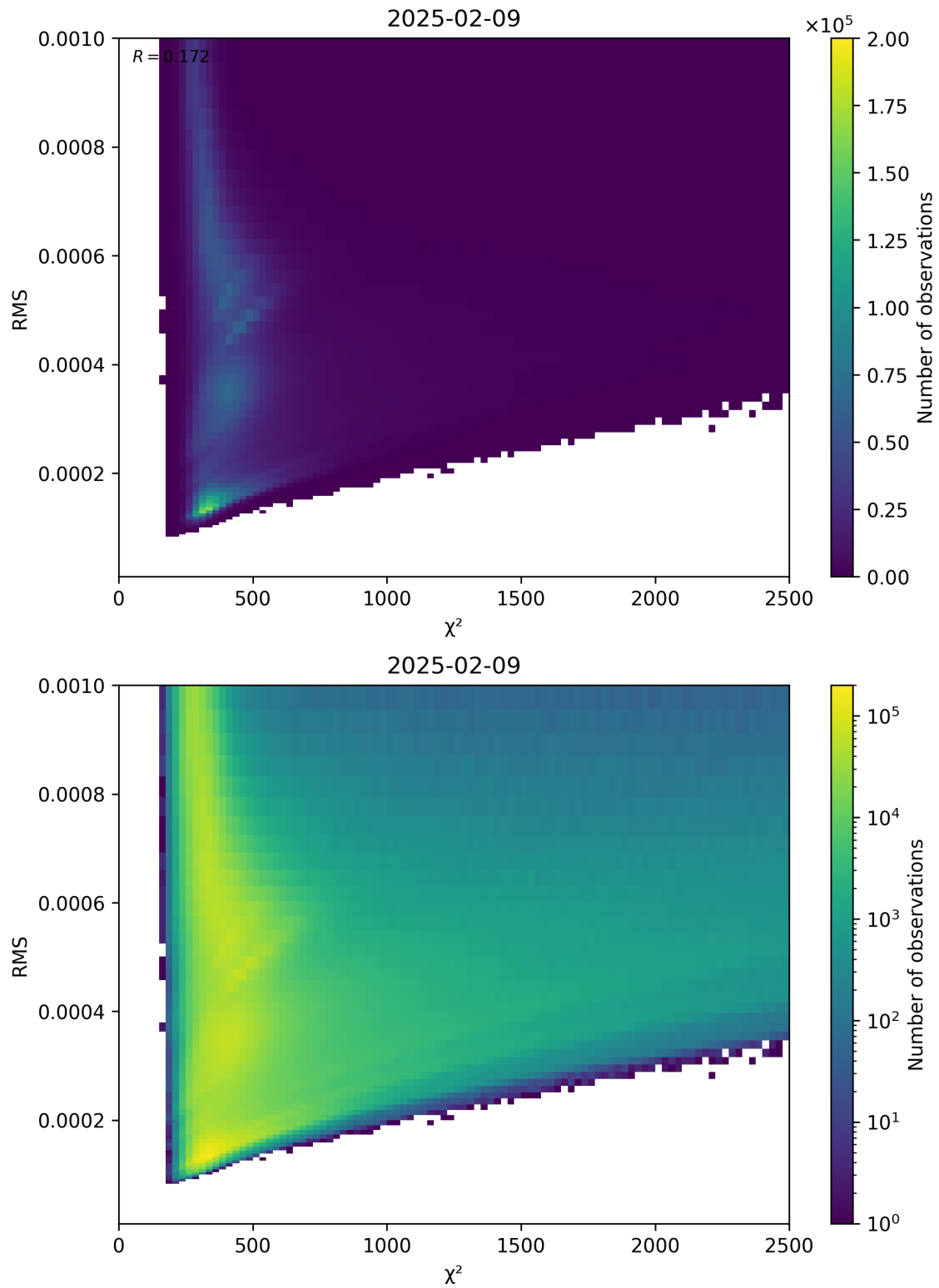
Figure 82: Scatter density plot of “ \chi^2 ” against “RMS” for 2025-02-08 to 2025-02-10.
