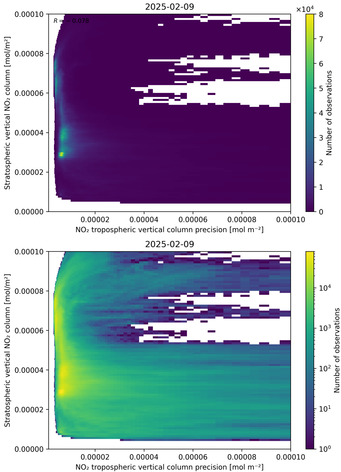
Figure 135: Scatter density plot of “NO 2 tropospheric vertical column precision” against “Stratospheric vertical NO 2 column” for 2025-02-08 to 2025-02-10.
