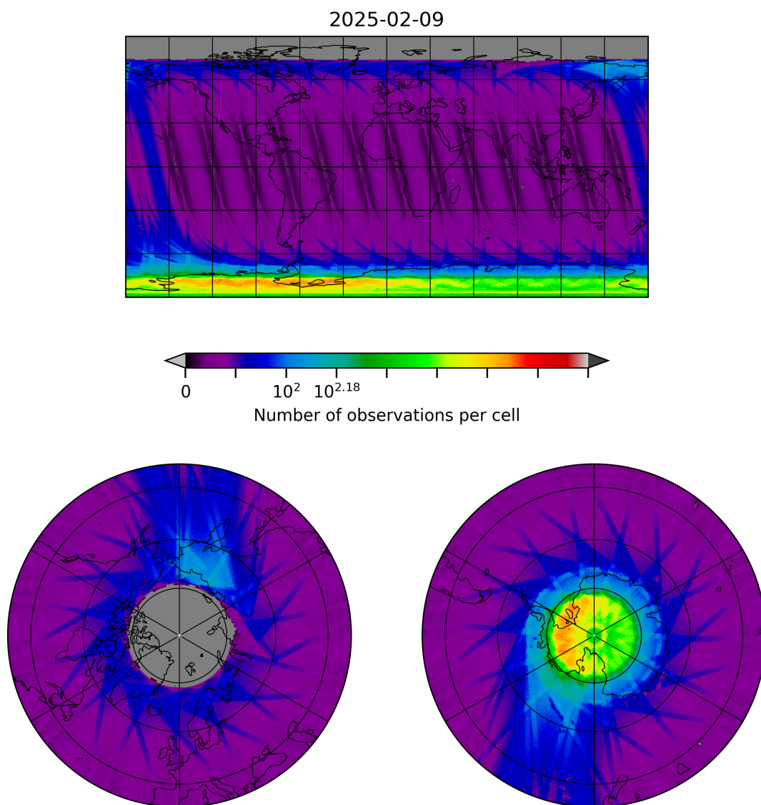
Figure 10: Map of the number of observations for 2025-02-08 to 2025-02-10
