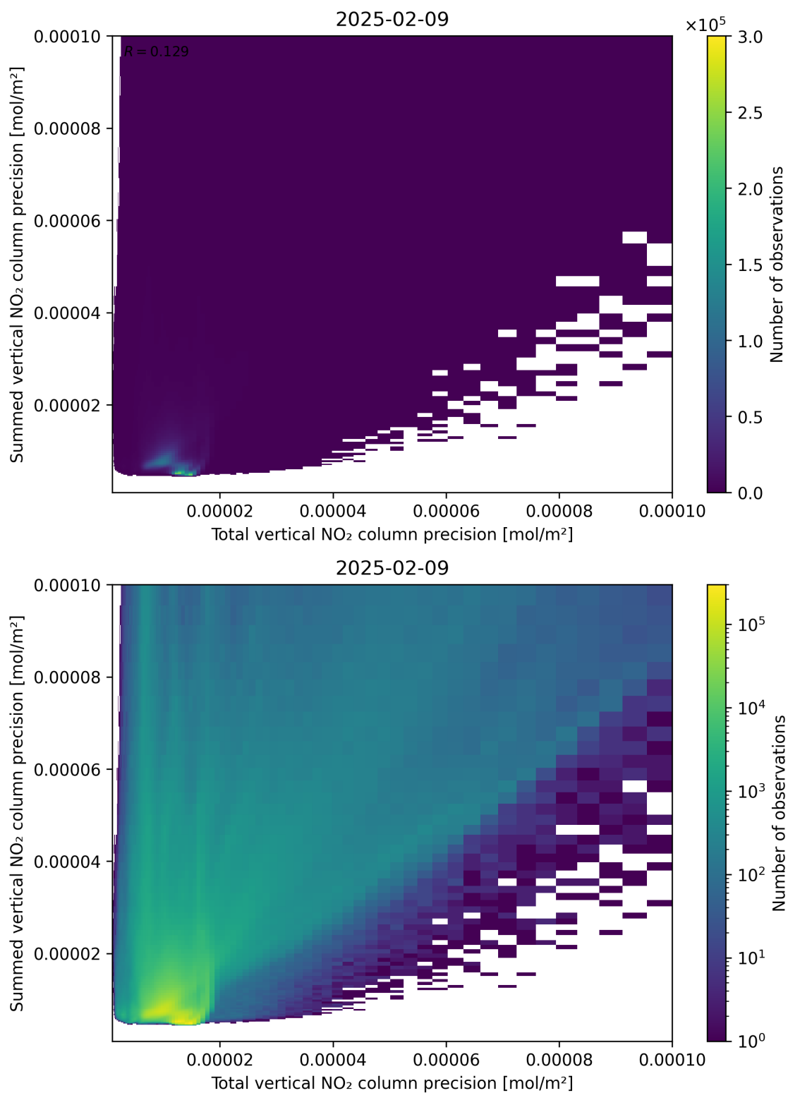
Figure 118: Scatter density plot of “Total vertical NO 2 column precision” against “Summed vertical NO 2 column precision” for 2025-02-08 to 2025-02-10.
