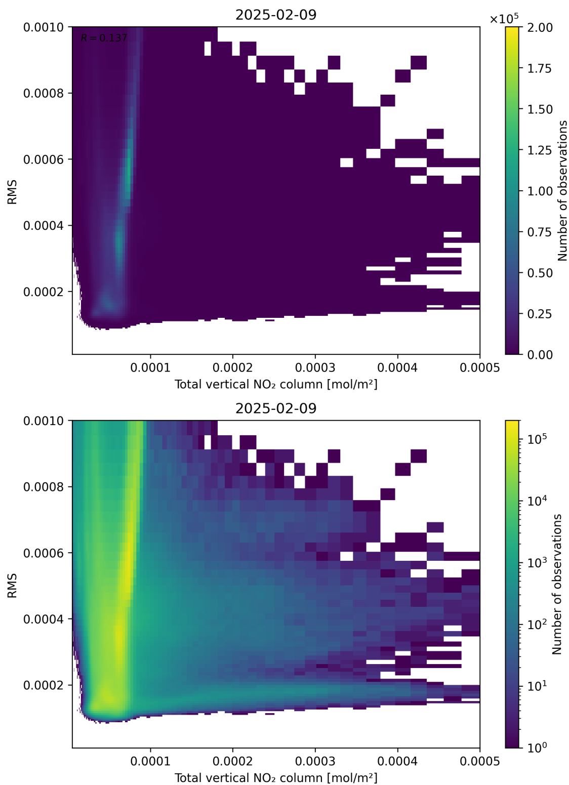
Figure 120: Scatter density plot of “Total vertical NO 2 column” against “RMS” for 2025-02-08 to 2025-02-10.
