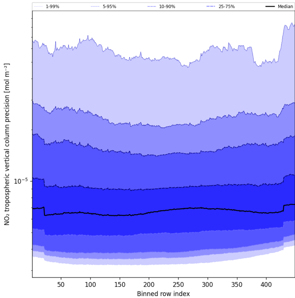
Figure 47: Along track statistics of “NO 2 tropospheric vertical column precision” for 2025-02-08 to 2025-02-10
