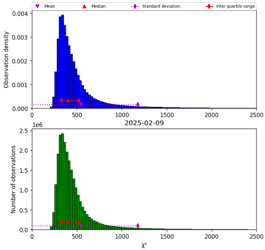
Figure 42: Histogram of “ \chi^2 ” for 2025-02-08 to 2025-02-10
