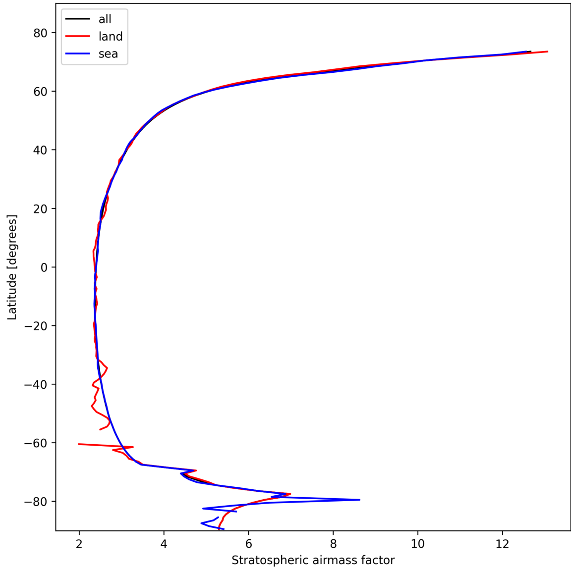
Figure 27: Zonal average of “Stratospheric air mass factor” for 2025-02-08 to 2025-02-10.
