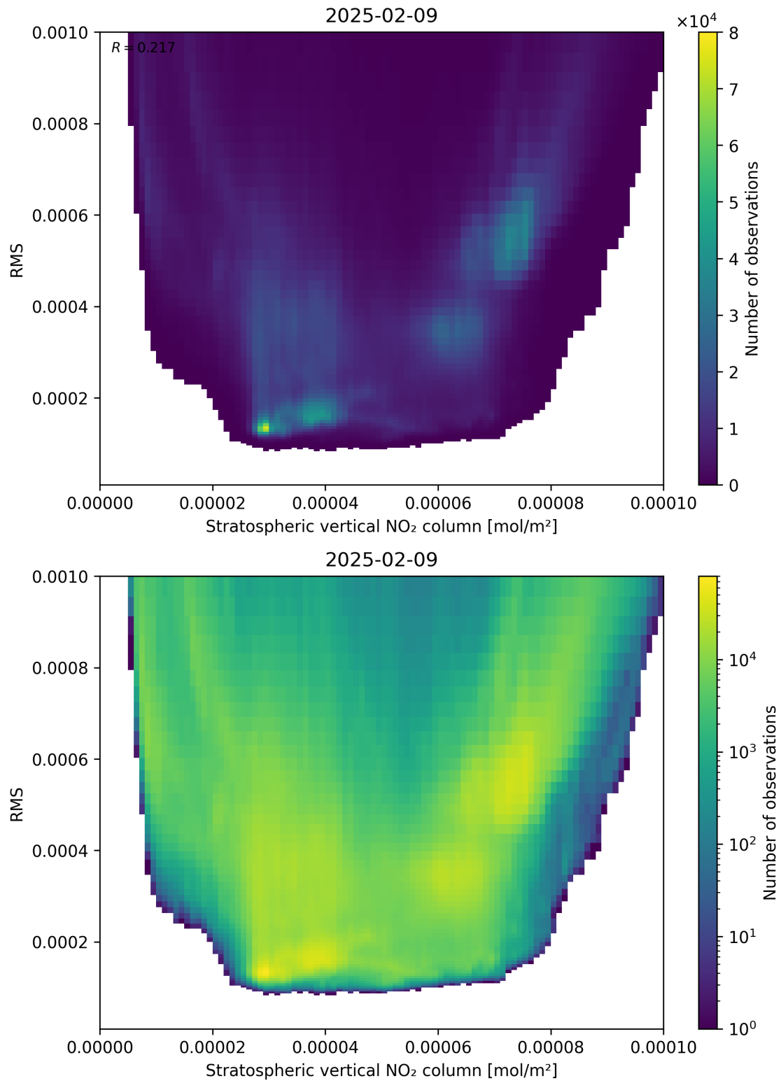
Figure 102: Scatter density plot of “Stratospheric vertical NO 2 column” against “RMS” for 2025-02-08 to 2025-02-10.
