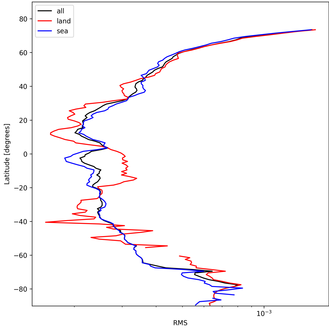
Figure 26: Zonal average of “RMS” for 2025-02-08 to 2025-02-10.
