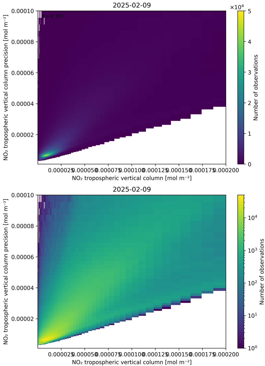
Figure 130: Scatter density plot of “NO 2 tropospheric vertical column” against “NO 2 tropospheric vertical column precision” for 2025-02-08 to 2025-02-10.
