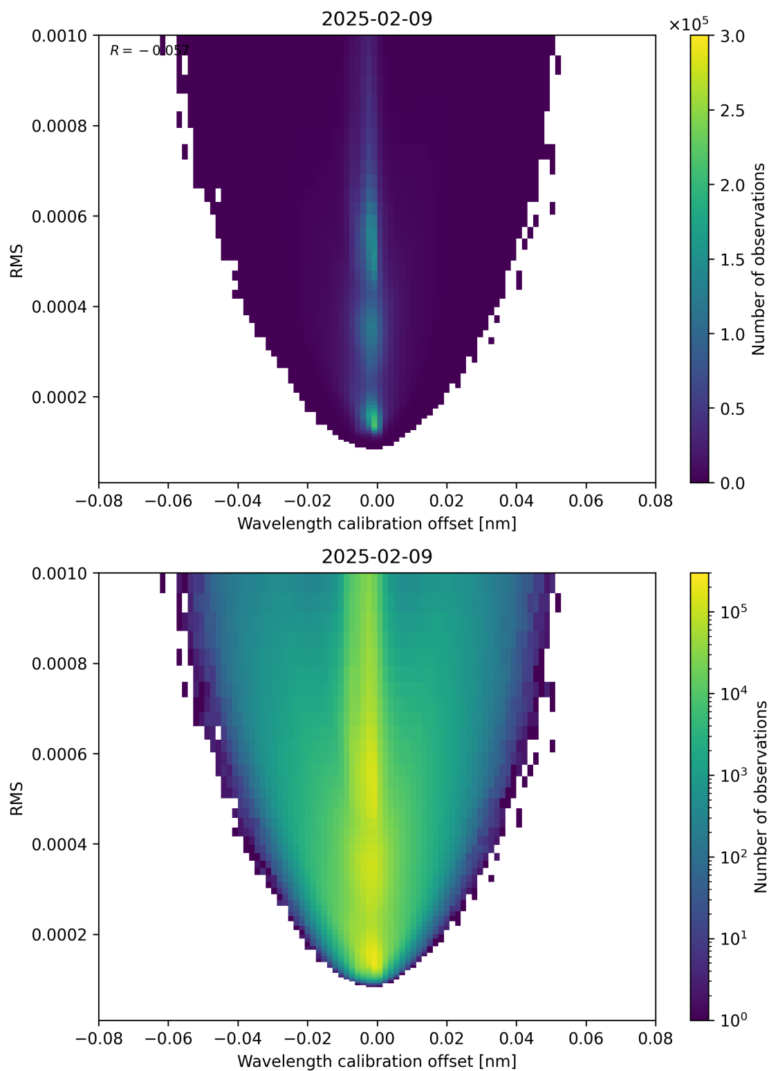
Figure 181: Scatter density plot of “Wavelength calibration offset” against “RMS” for 2025-02-08 to 2025-02-10.
