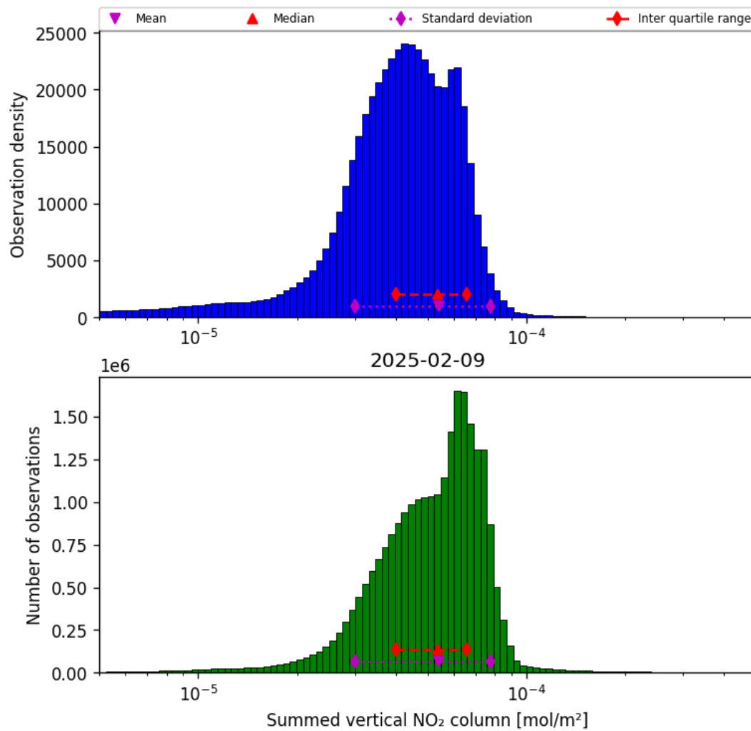
Figure 40: Histogram of “Summed vertical NO 2 column” for 2025-02-08 to 2025-02-10
