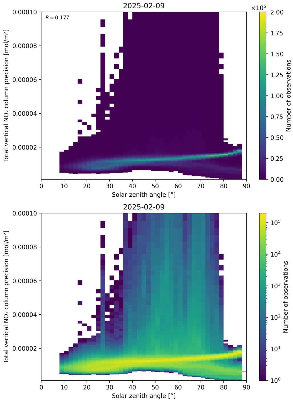
Figure 154: Scatter density plot of “Solar zenith angle” against “Total vertical NO 2 column precision” for 2025-02-08 to 2025-02-10.
