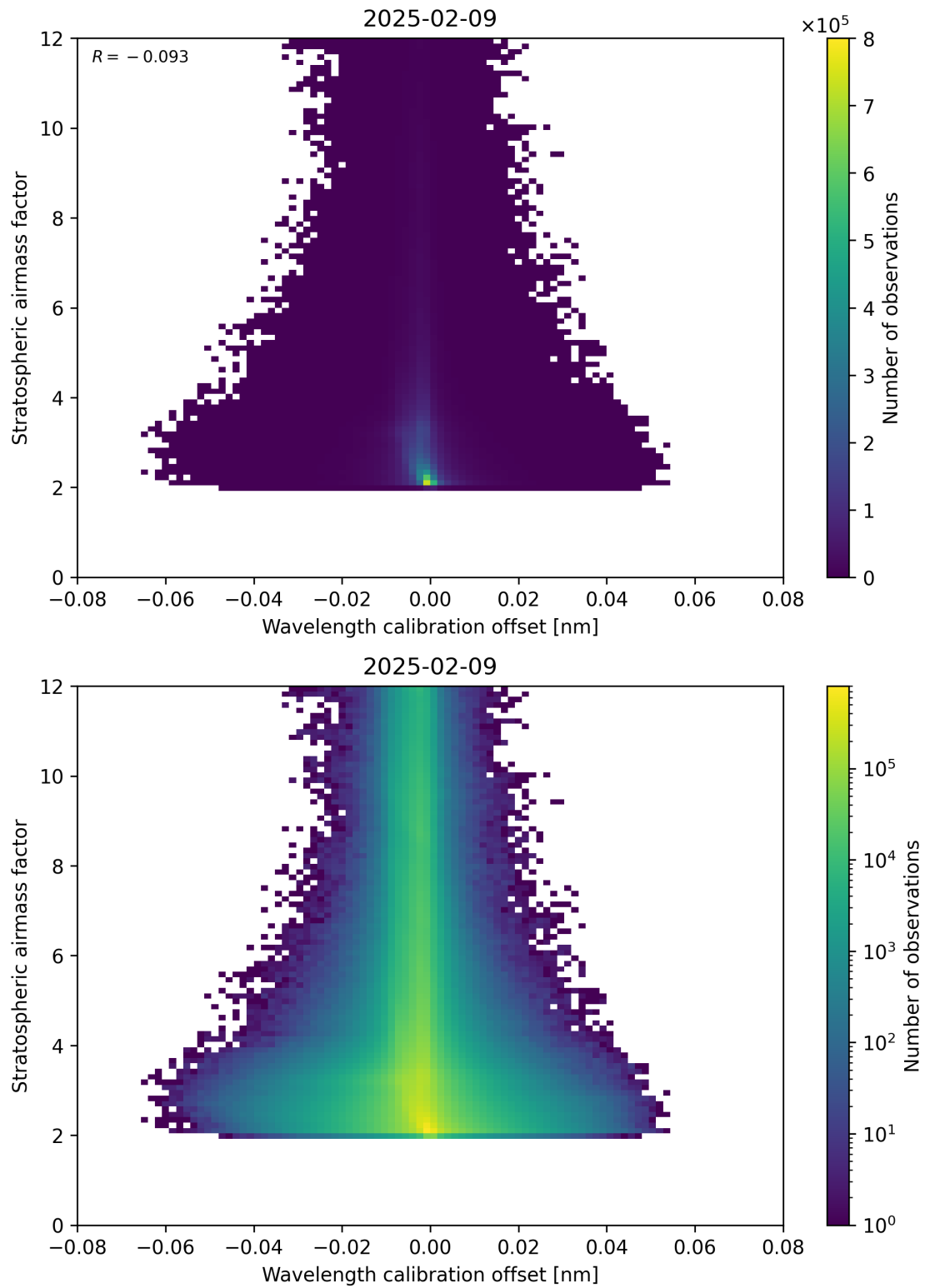
Figure 174: Scatter density plot of “Wavelength calibration offset” against “Stratospheric airmass factor” for 2025-02-08 to 2025-02-10.
