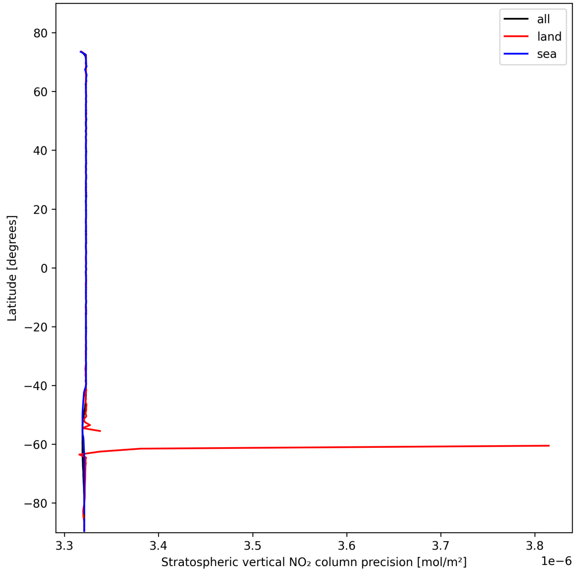
Figure 20: Zonal average of “Stratospheric vertical NO 2 column precision” for 2025-02-08 to 2025-02-10.
