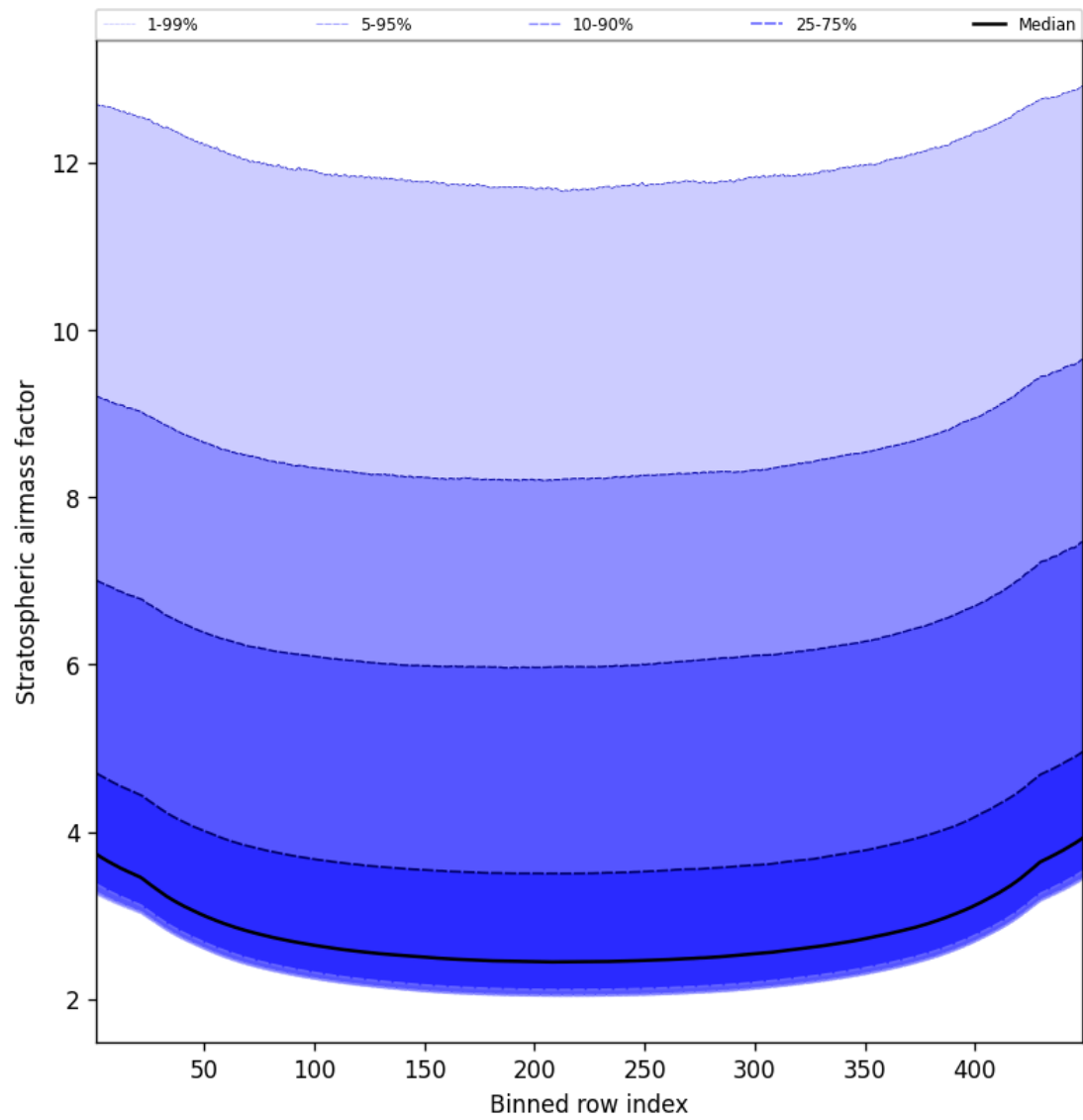
Figure 61: Along track statistics of “Stratospheric airmass factor” for 2025-02-08 to 2025-02-10
