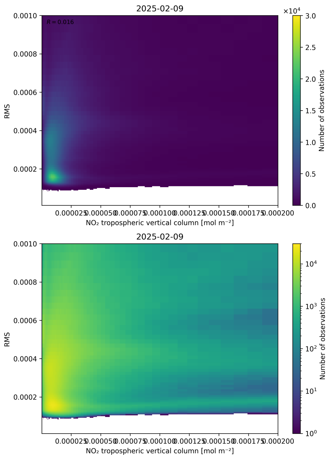
Figure 142: Scatter density plot of “NO 2 tropospheric vertical column” against “RMS” for 2025-02-08 to 2025-02-10.
