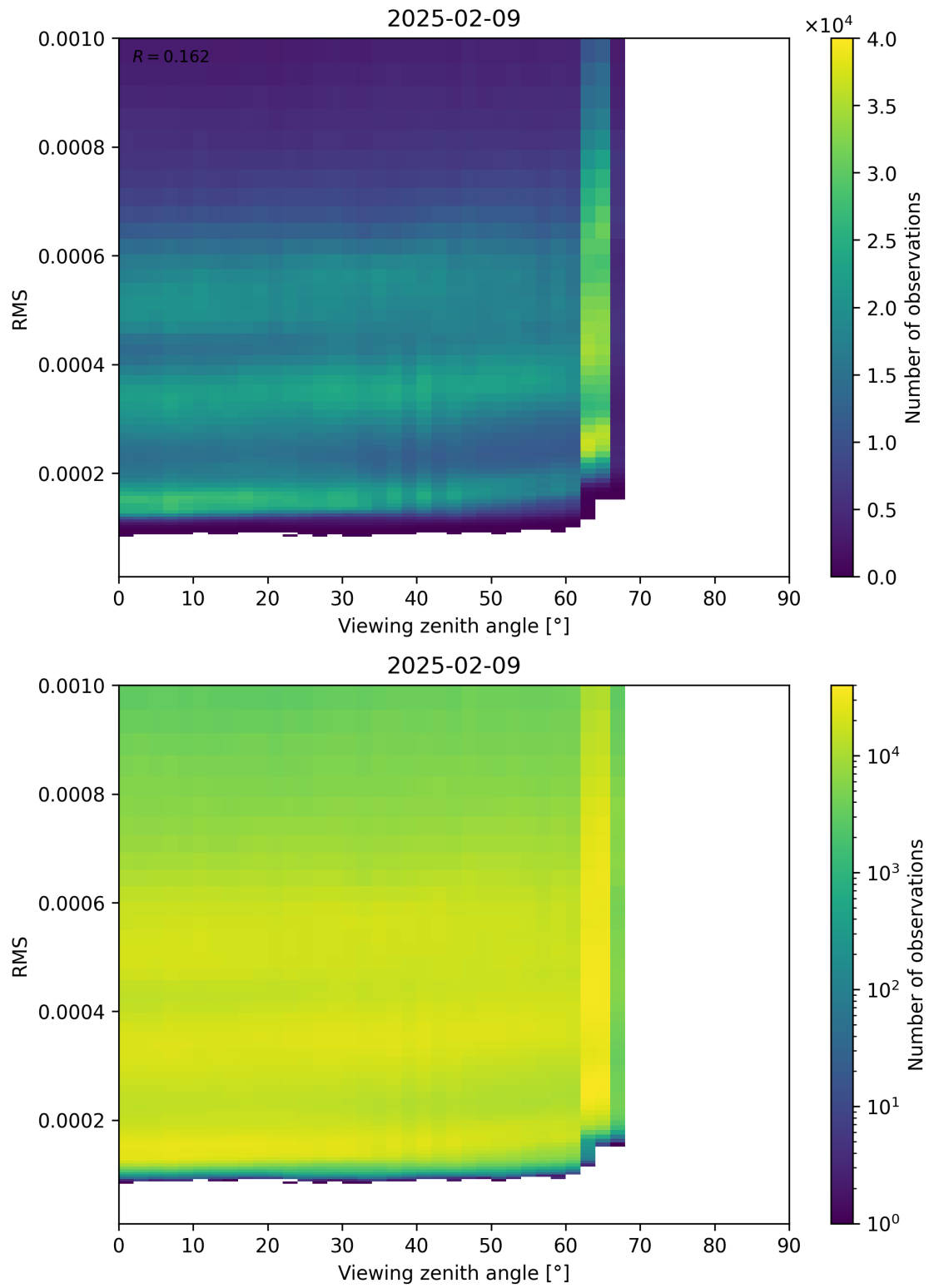
Figure 171: Scatter density plot of “Viewing zenith angle” against “RMS” for 2025-02-08 to 2025-02-10.
