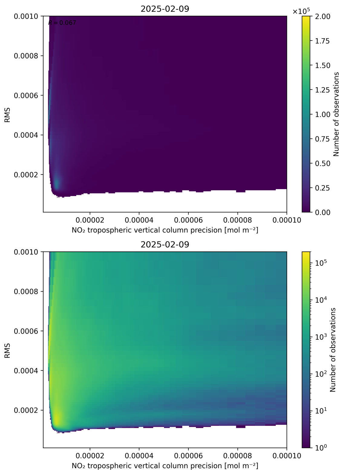
Figure 140: Scatter density plot of “NO 2 tropospheric vertical column precision” against “RMS” for 2025-02-08 to 2025-02-10.
