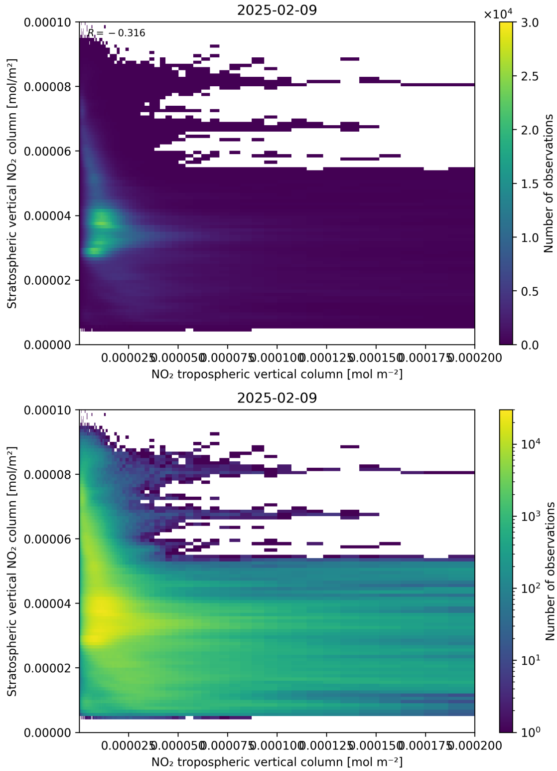
Figure 125: Scatter density plot of “NO 2 tropospheric vertical column” against “Stratospheric vertical NO 2 column” for 2025-02-08 to 2025-02-10.
