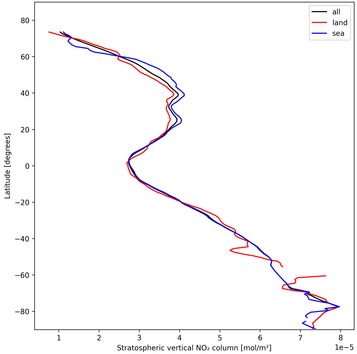
Figure 19: Zonal average of “Stratospheric vertical NO 2 column” for 2025-02-08 to 2025-02-10.
