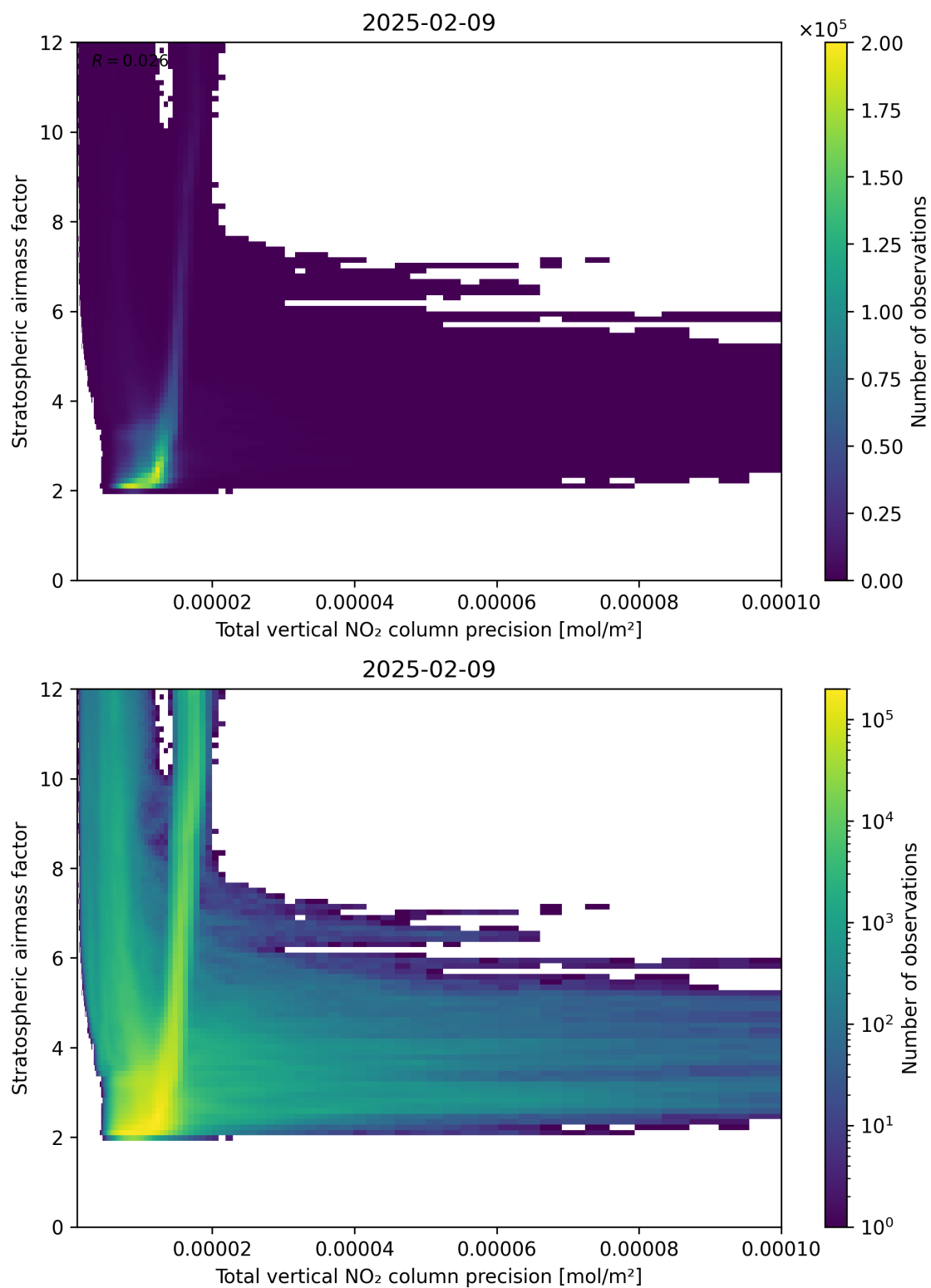
Figure 115: Scatter density plot of “Total vertical NO 2 column precision” against “Stratospheric air mass factor” for 2025-02-08 to 2025-02-10.
