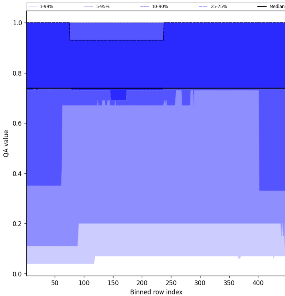
Figure 45: Along track statistics of “QA value” for 2025-02-08 to 2025-02-10
