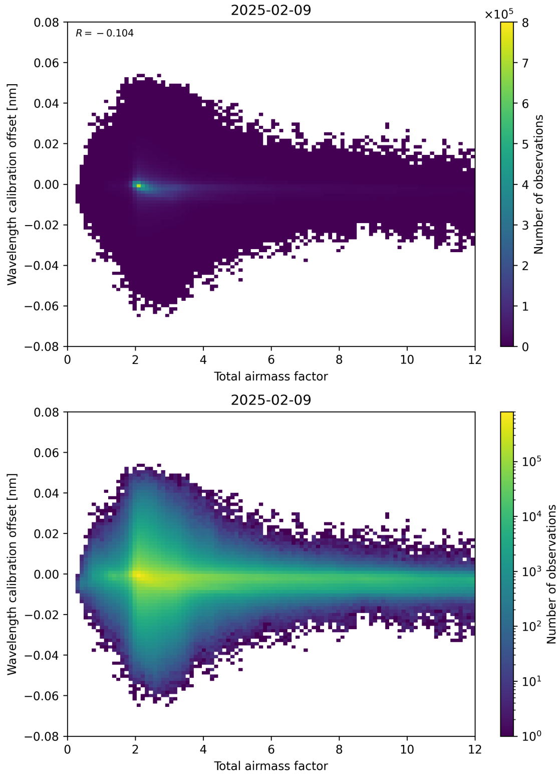
Figure 70: Scatter density plot of “Total airmass factor” against “Wavelength calibration offset” for 2025-02-08 to 2025-02-10.
