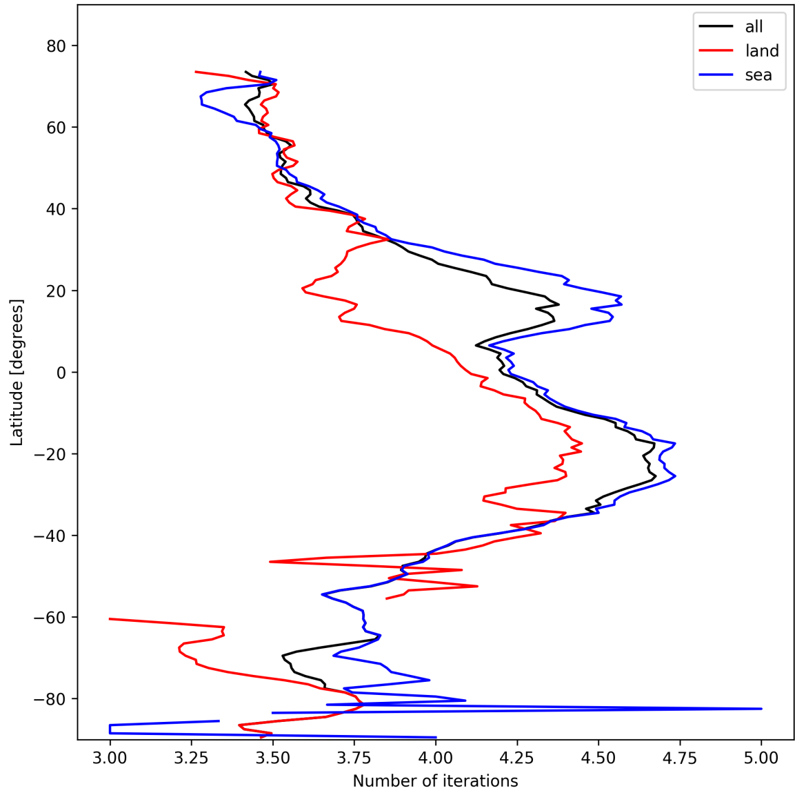
Figure 17: Zonal average of “Number of iterations” for 2025-02-08 to 2025-02-10.
