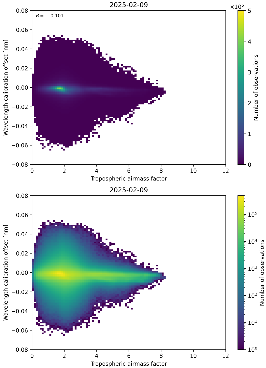
Figure 80: Scatter density plot of “Tropospheric airmass factor” against “Wavelength calibration offset” for 2025-02-08 to 2025-02-10.
