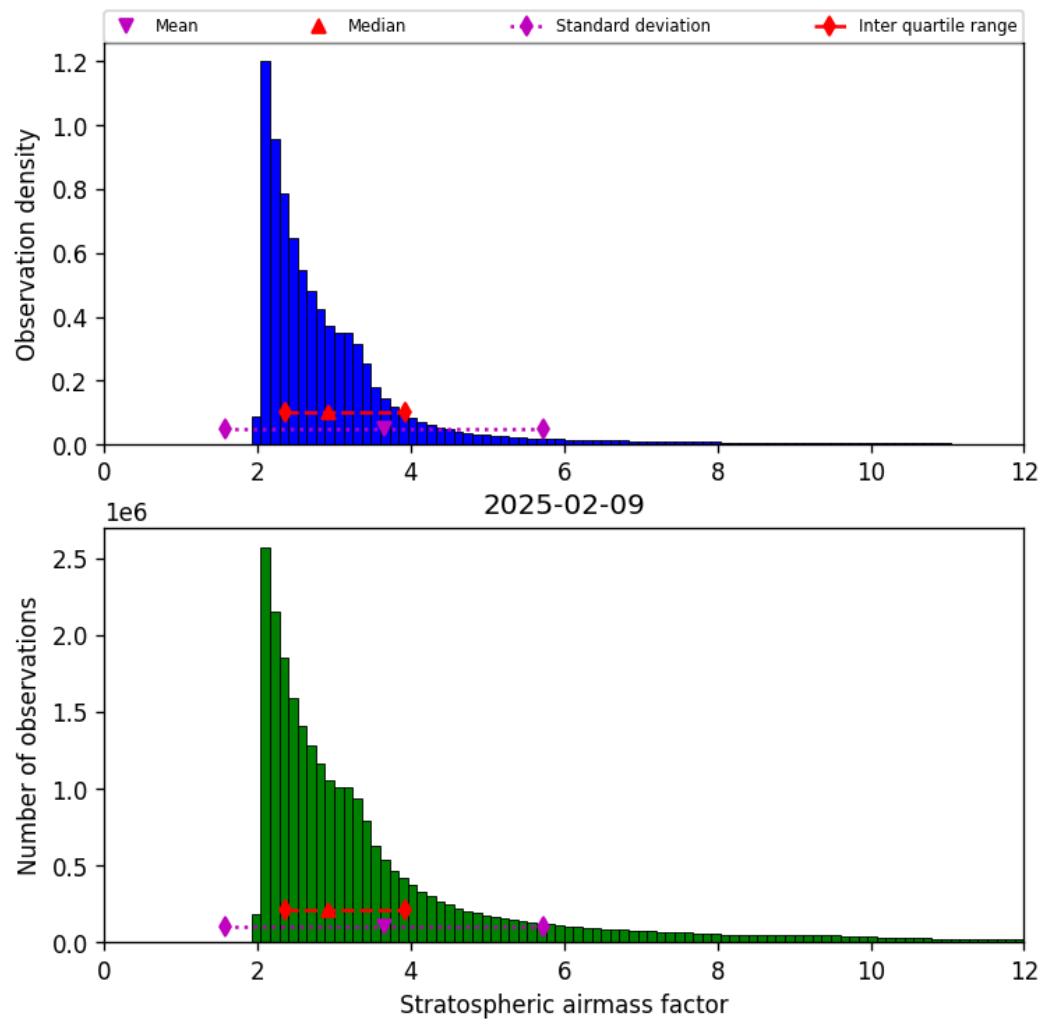
Figure 44: Histogram of “Stratospheric airmass factor” for 2025-02-08 to 2025-02-10
