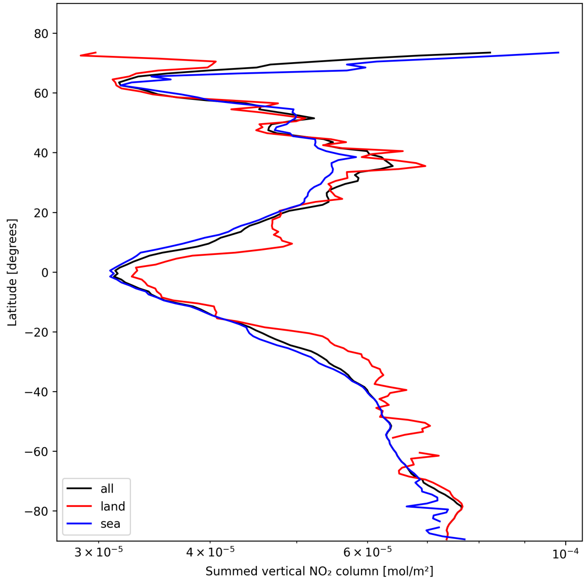
Figure 23: Zonal average of “Summed vertical NO 2 column” for 2025-02-08 to 2025-02-10.
