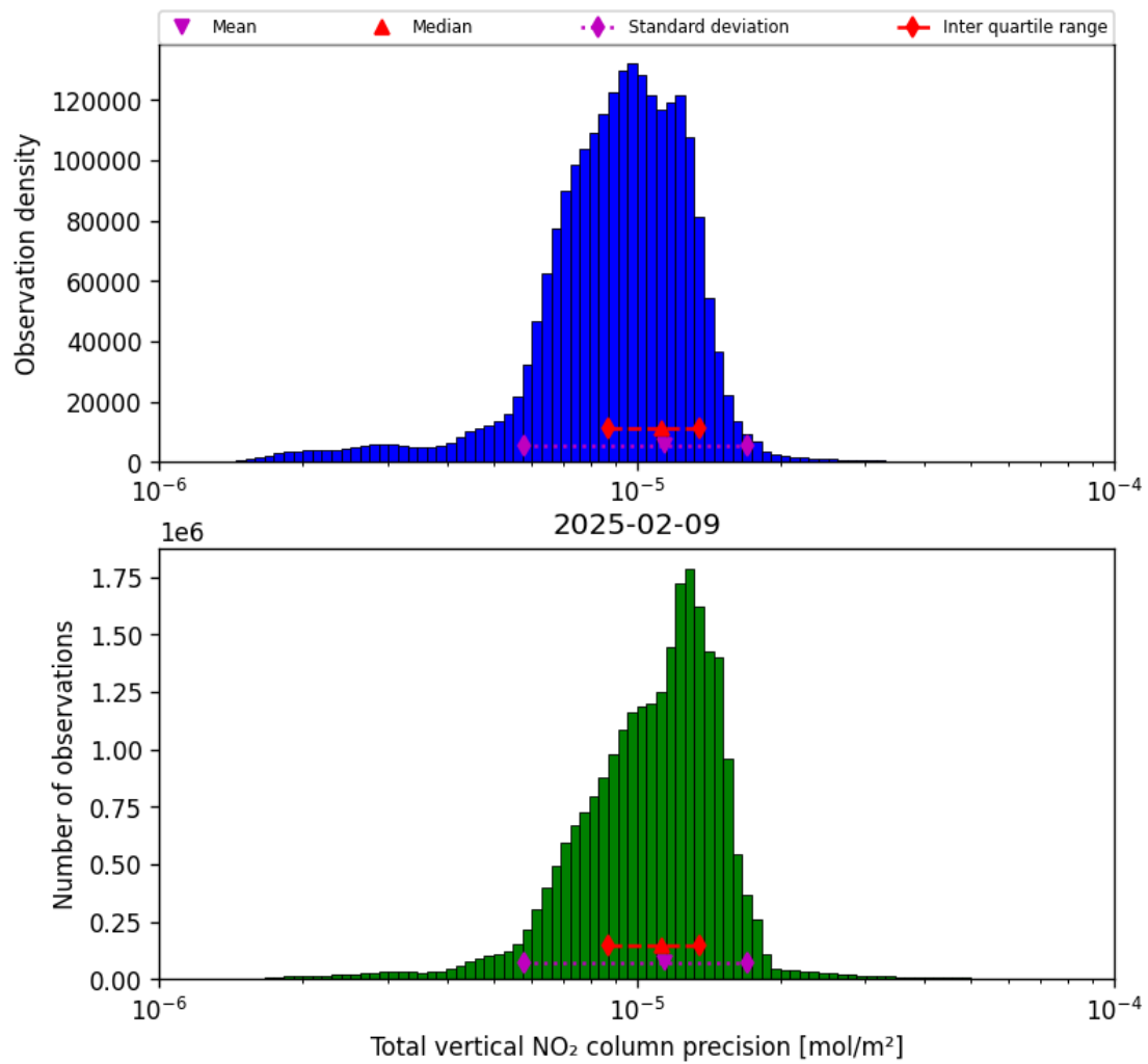
Figure 39: Histogram of “Total vertical NO 2 column precision” for 2025-02-08 to 2025-02-10
