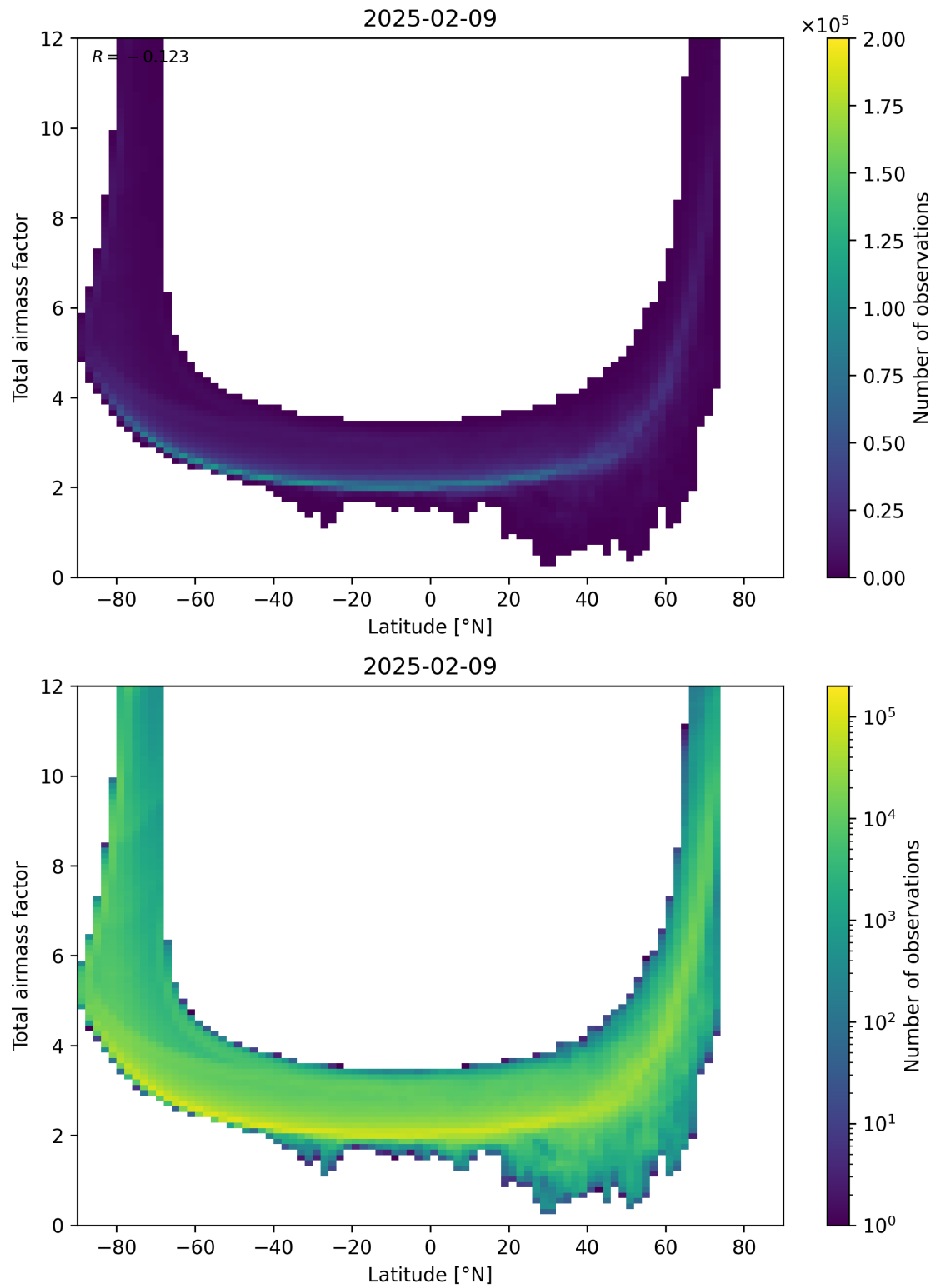
Figure 84: Scatter density plot of “Latitude” against “Total airmass factor” for 2025-02-08 to 2025-02-10.
