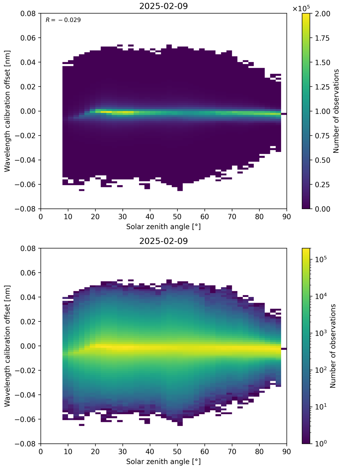
Figure 158: Scatter density plot of “Solar zenith angle” against “Wavelength calibration offset” for 2025-02-08 to 2025-02-10.
