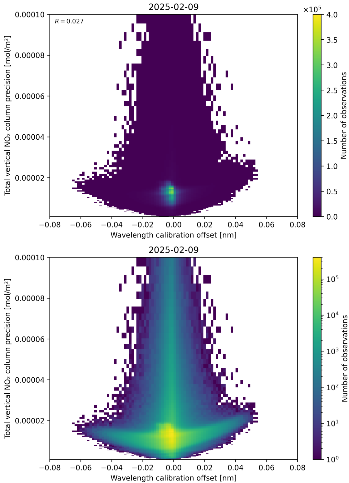
Figure 180: Scatter density plot of “Wavelength calibration offset” against “Total vertical NO 2 column precision” for 2025-02-08 to 2025-02-10.
