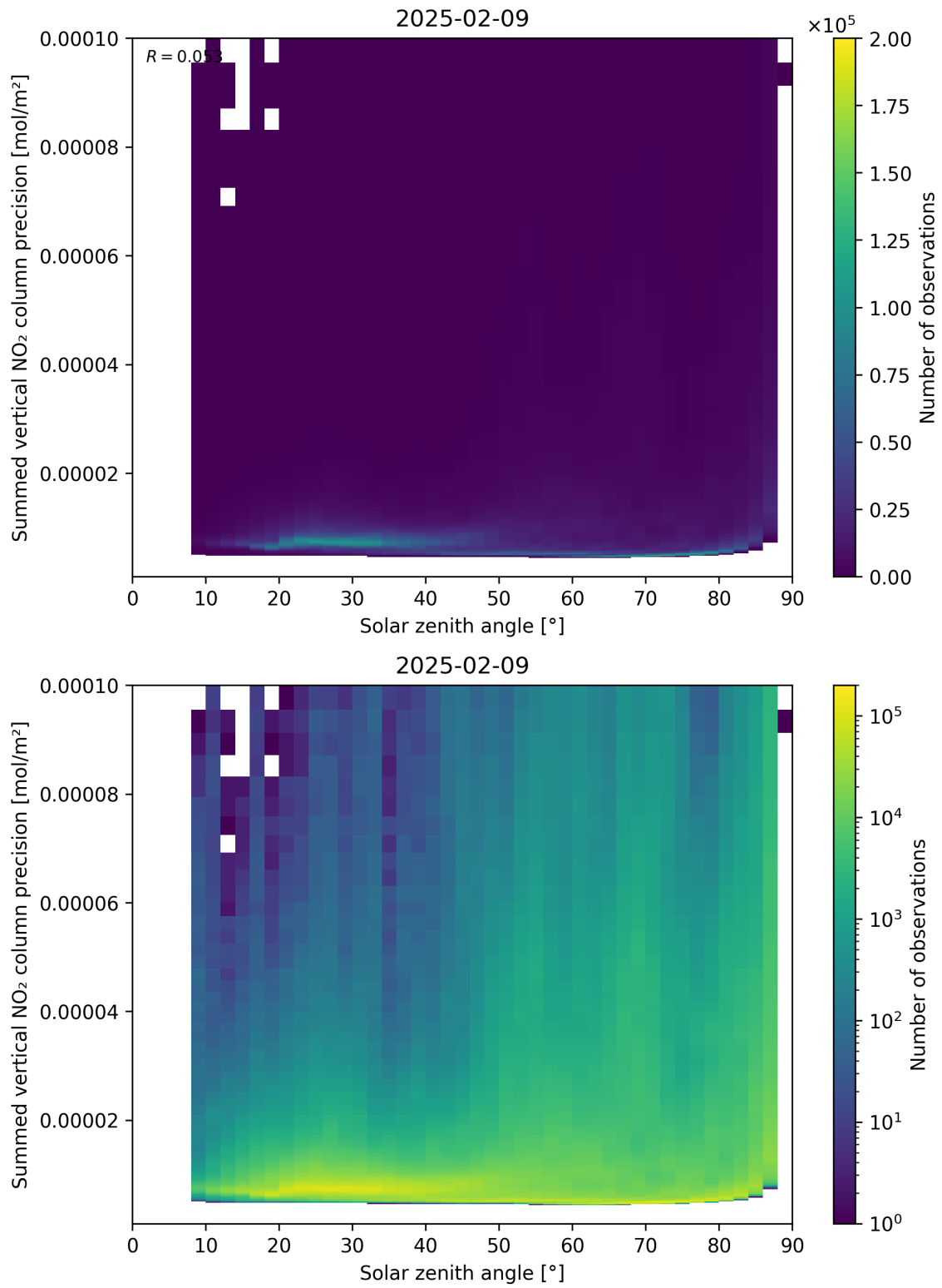
Figure 152: Scatter density plot of “Solar zenith angle” against “Summed vertical NO 2 column precision” for 2025-02-08 to 2025-02-10.
