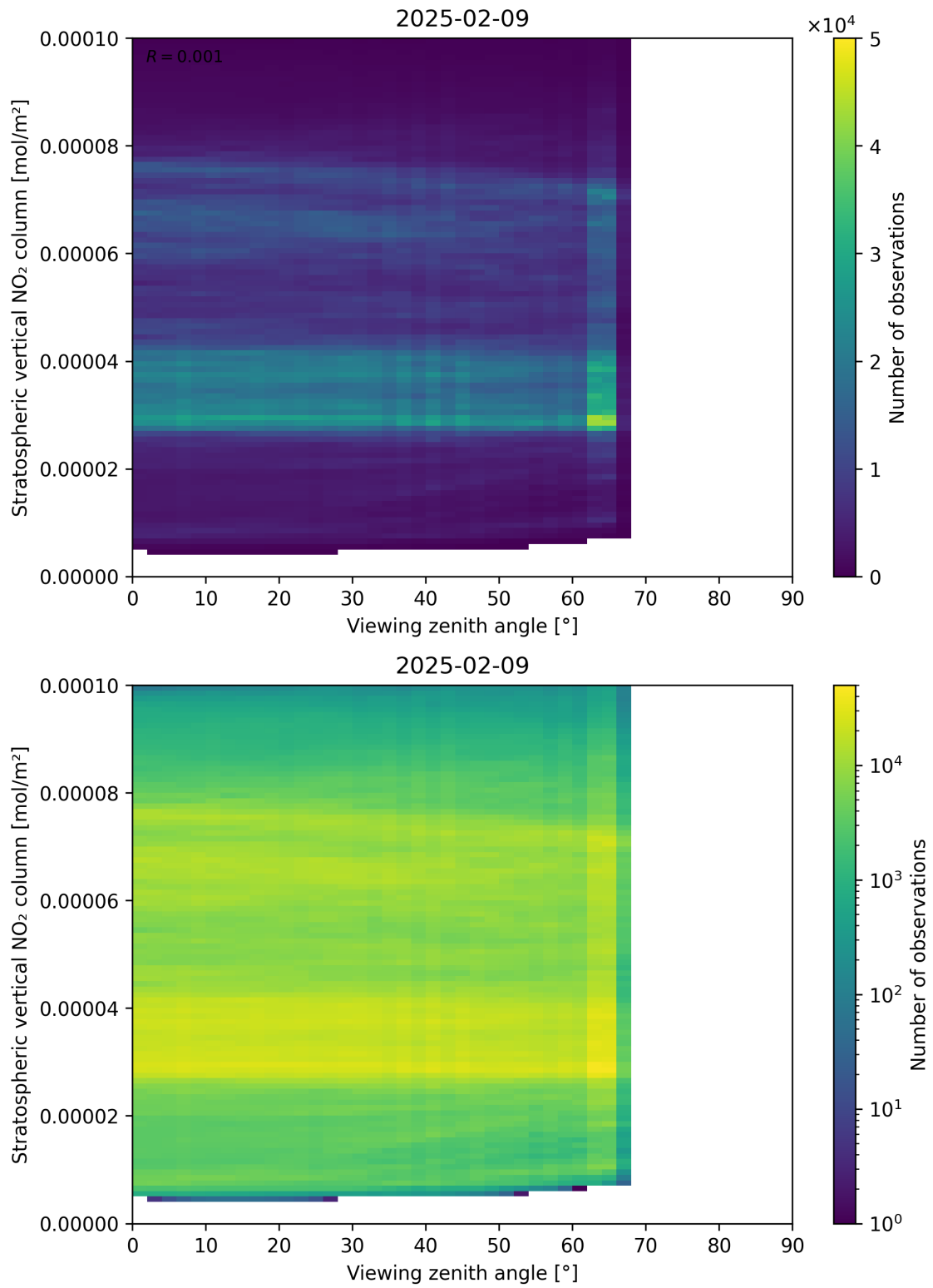
Figure 164: Scatter density plot of “Viewing zenith angle” against “Stratospheric vertical NO 2 column” for 2025-02-08 to 2025-02-10.
