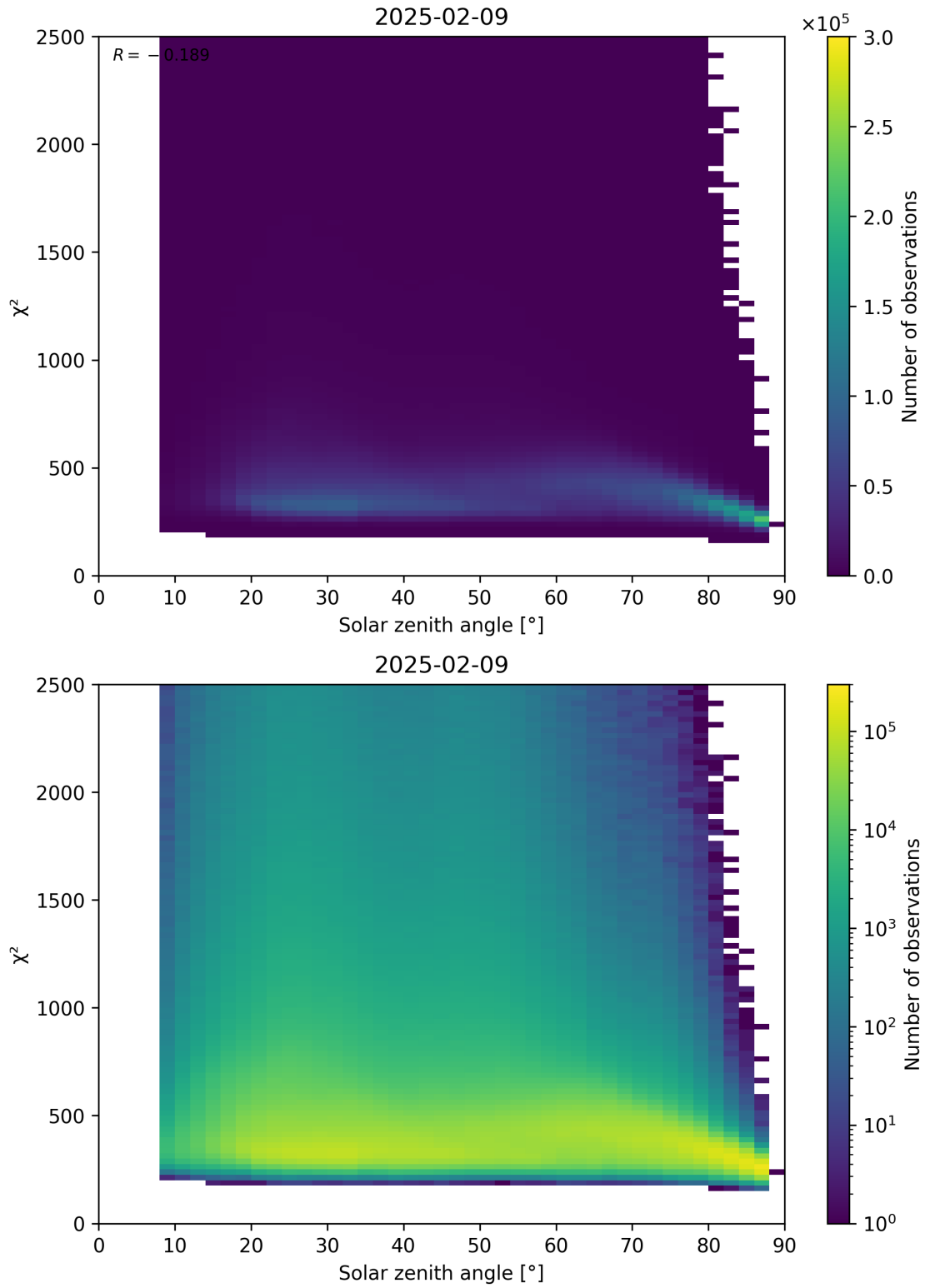
Figure 148: Scatter density plot of “Solar zenith angle” against “ \chi^2 ” for 2025-02-08 to 2025-02-10.
