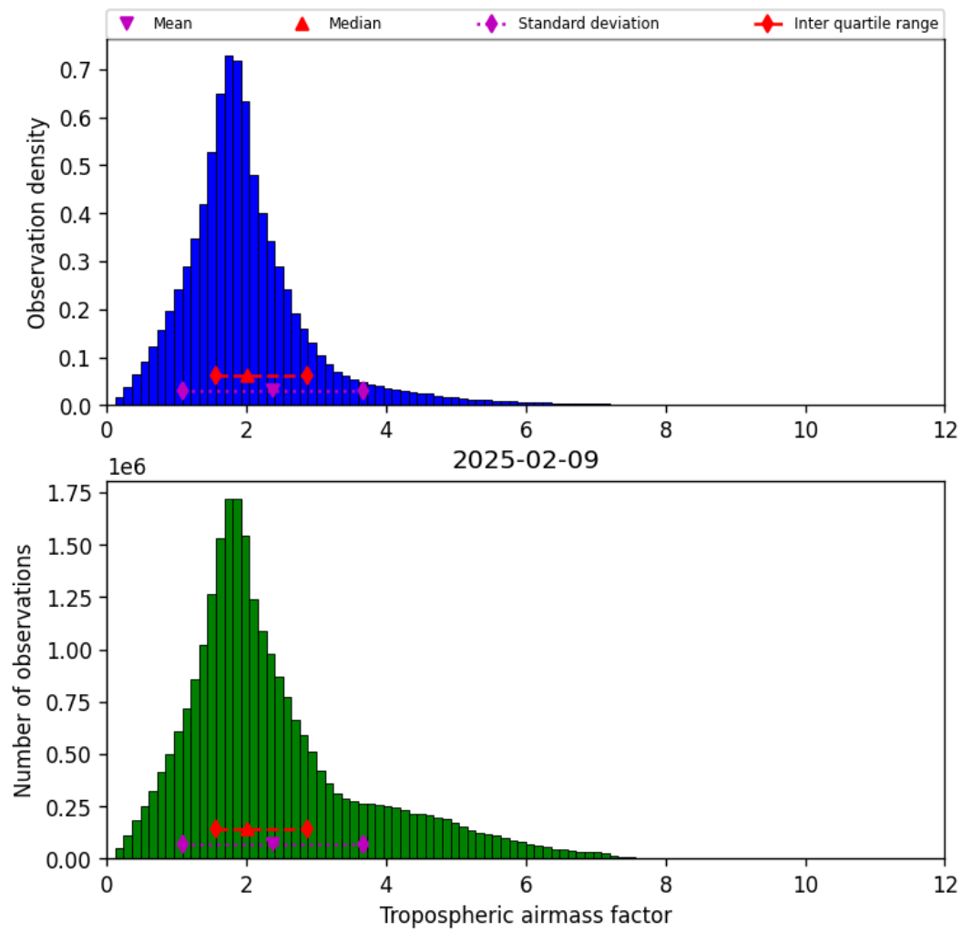
Figure 31: Histogram of “Tropospheric airmass factor” for 2025-02-08 to 2025-02-10
