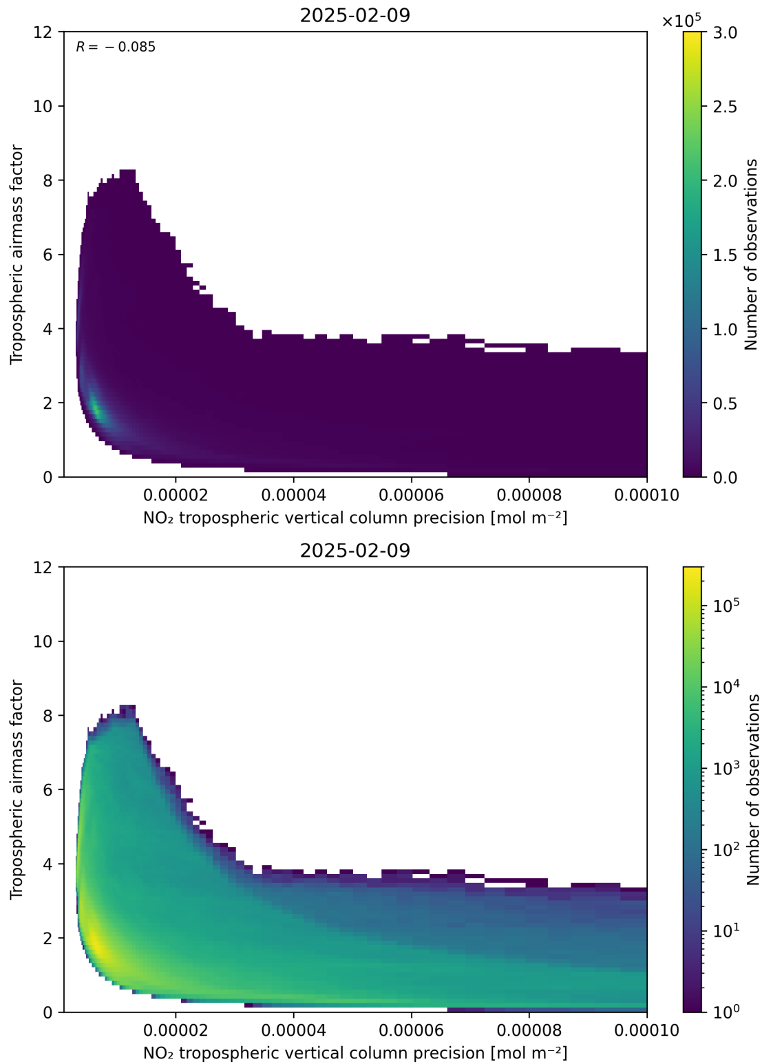
Figure 133: Scatter density plot of “NO 2 tropospheric vertical column precision” against “Tropospheric air mass factor” for 2025-02-08 to 2025-02-10.
