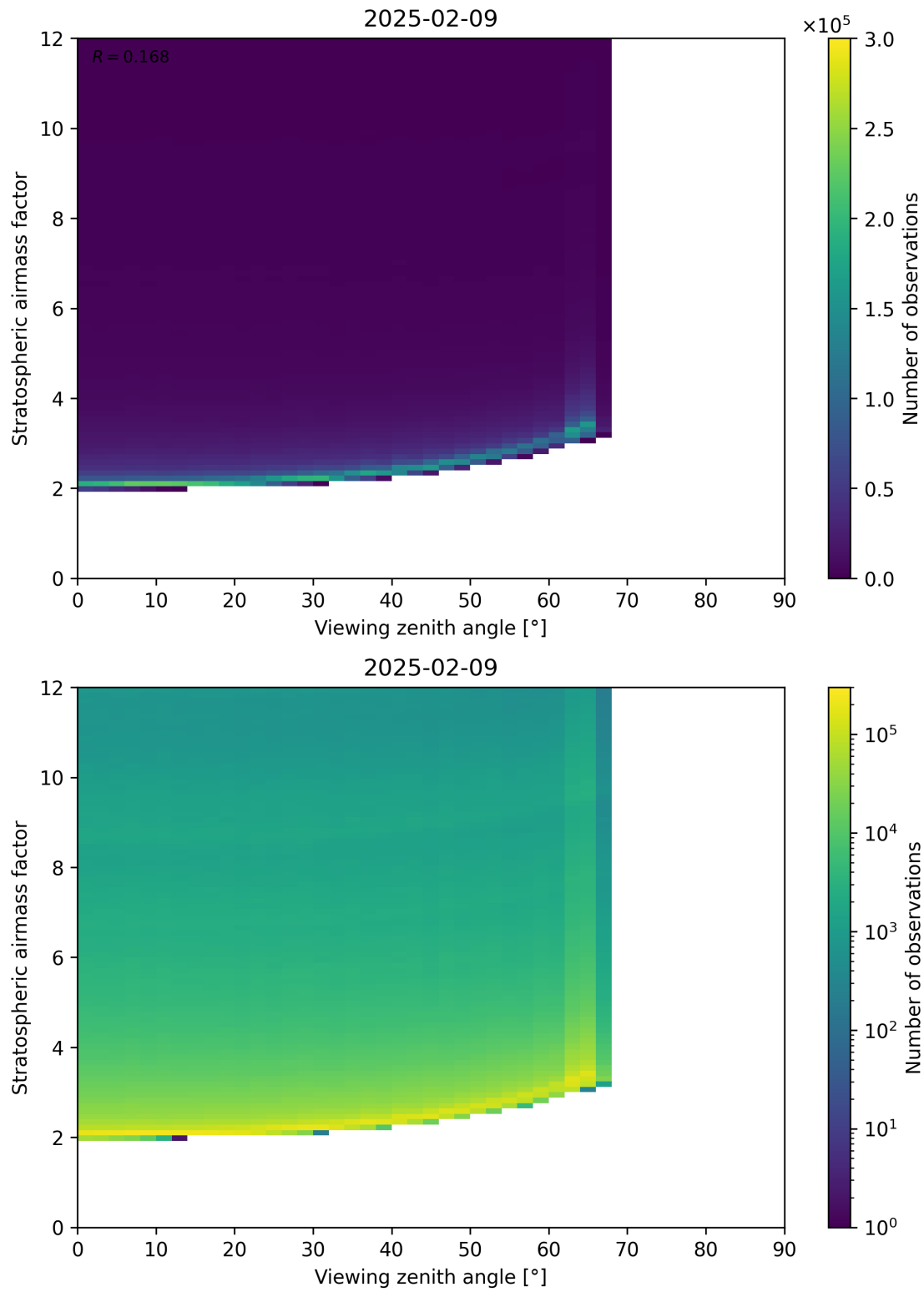
Figure 159: Scatter density plot of “Viewing zenith angle” against “Stratospheric airmass factor” for 2025-02-08 to 2025-02-10.
