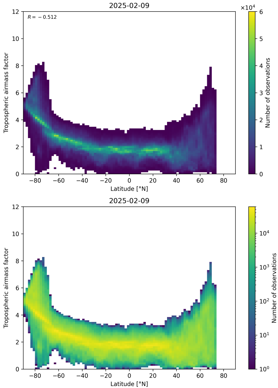
Figure 85: Scatter density plot of “Latitude” against “Tropospheric airmass factor” for 2025-02-08 to 2025-02-10.
