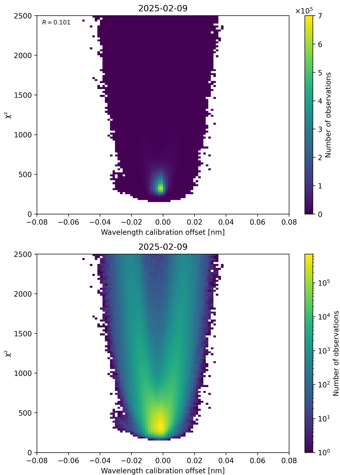
Figure 175: Scatter density plot of “Wavelength calibration offset” against “ \chi^2 ” for 2025-02-08 to 2025-02-10.
