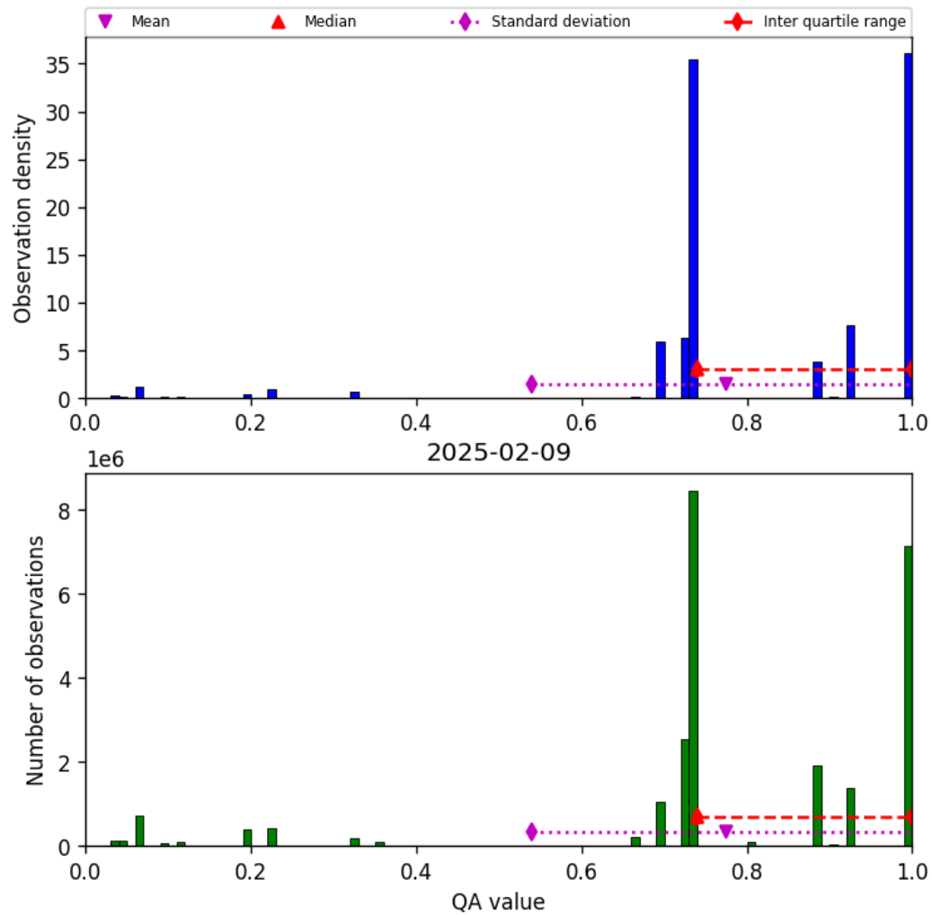
Figure 28: Histogram of “QA value” for 2025-02-08 to 2025-02-10
