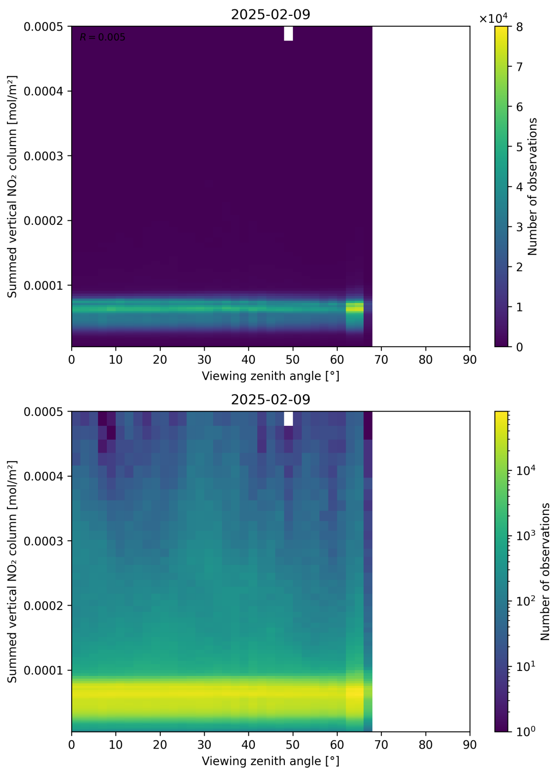
Figure 165: Scatter density plot of “Viewing zenith angle” against “Summed vertical NO 2 column” for 2025-02-08 to 2025-02-10.
