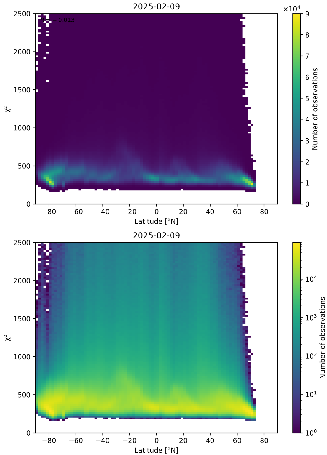
Figure 86: Scatter density plot of “Latitude” against “ \chi^2 ” for 2025-02-08 to 2025-02-10.
