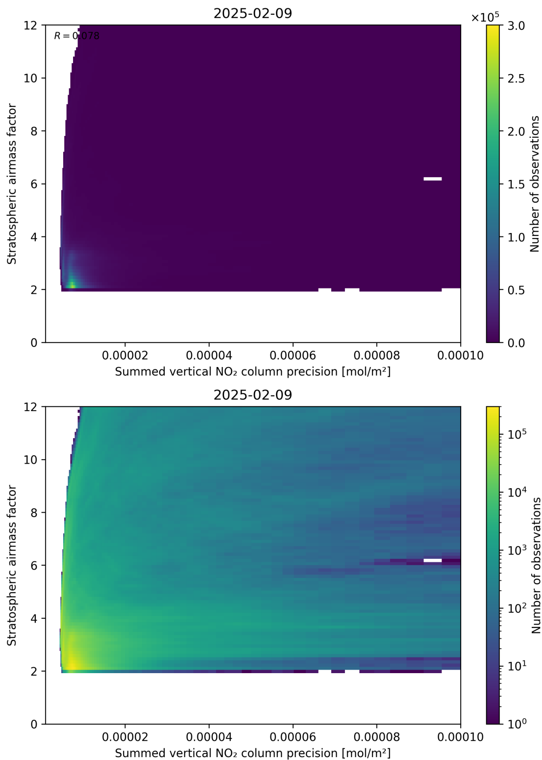
Figure 106: Scatter density plot of “Summed vertical NO 2 column precision” against “Stratospheric airmass factor” for 2025-02-08 to 2025-02-10.
