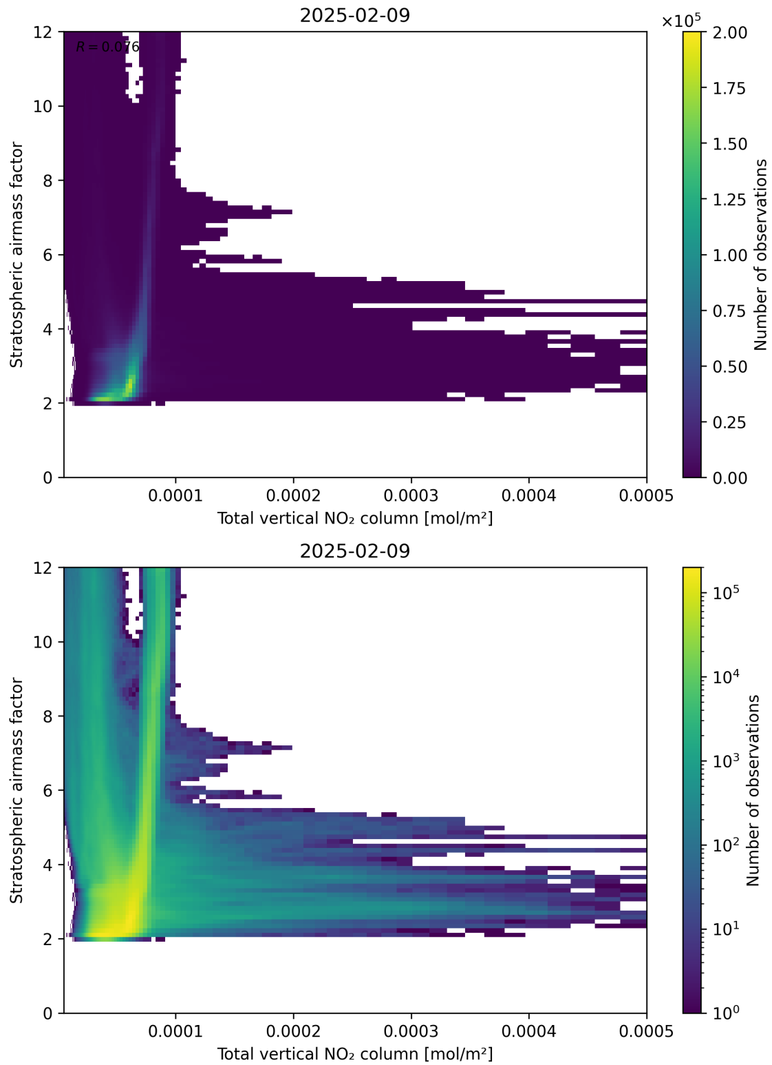
Figure 110: Scatter density plot of “Total vertical NO 2 column” against “Stratospheric airmass factor” for 2025-02-08 to 2025-02-10.
