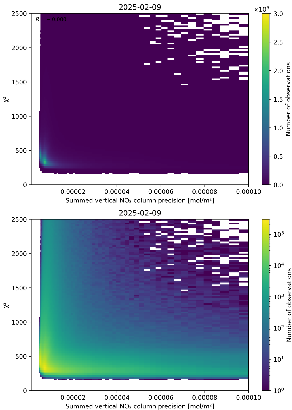
Figure 107: Scatter density plot of “Summed vertical NO 2 column precision” against “ \chi^2 ” for 2025-02-08 to 2025-02-10.
