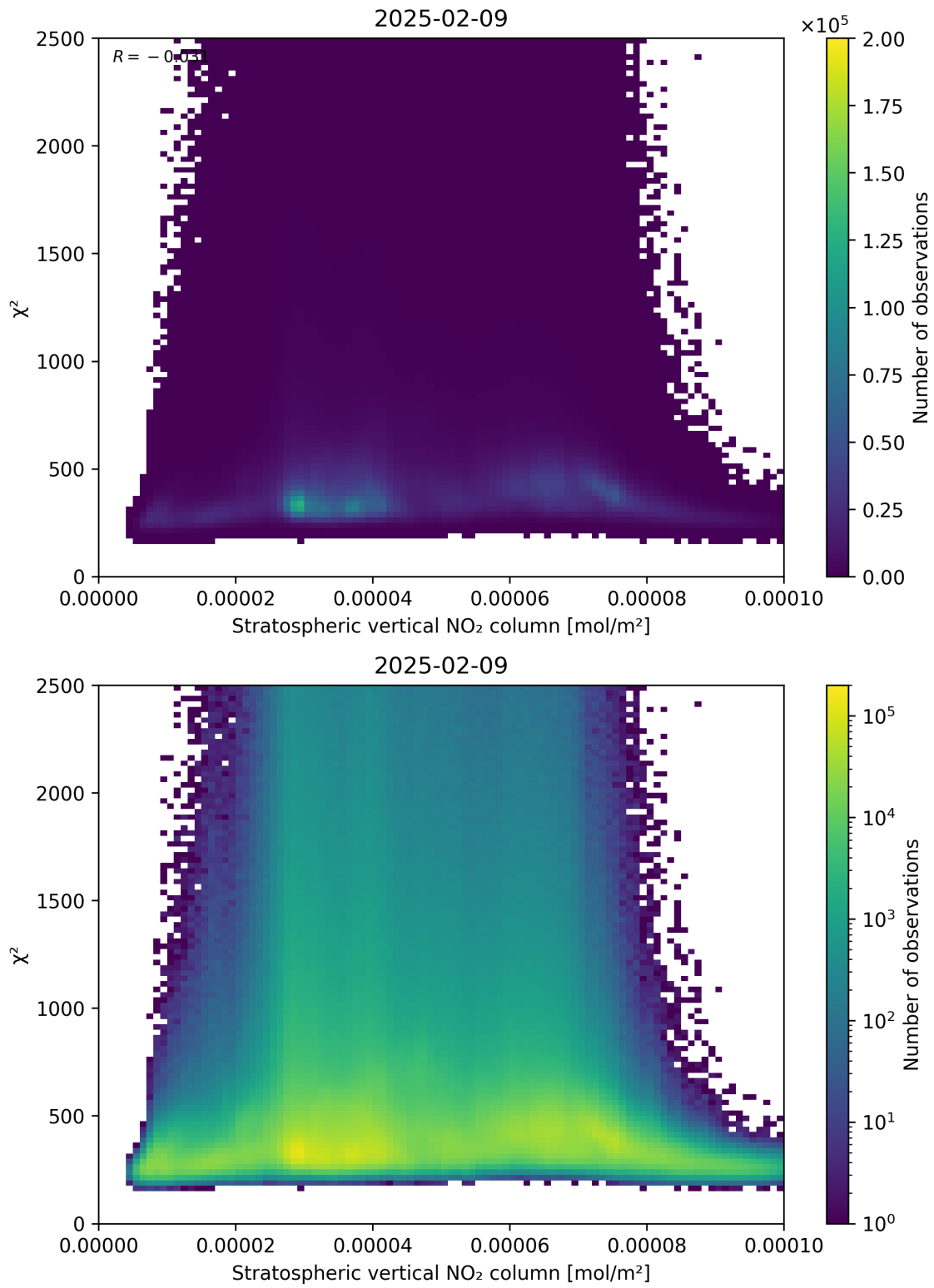
Figure 97: Scatter density plot of “Stratospheric vertical NO 2 column” against “ \chi^2 ” for 2025-02-08 to 2025-02-10.
