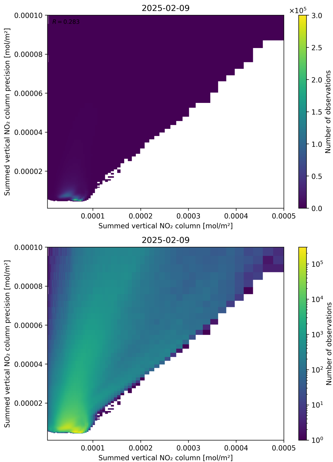
Figure 105: Scatter density plot of “Summed vertical NO 2 column” against “Summed vertical NO 2 column precision” for 2025-02-08 to 2025-02-10.
