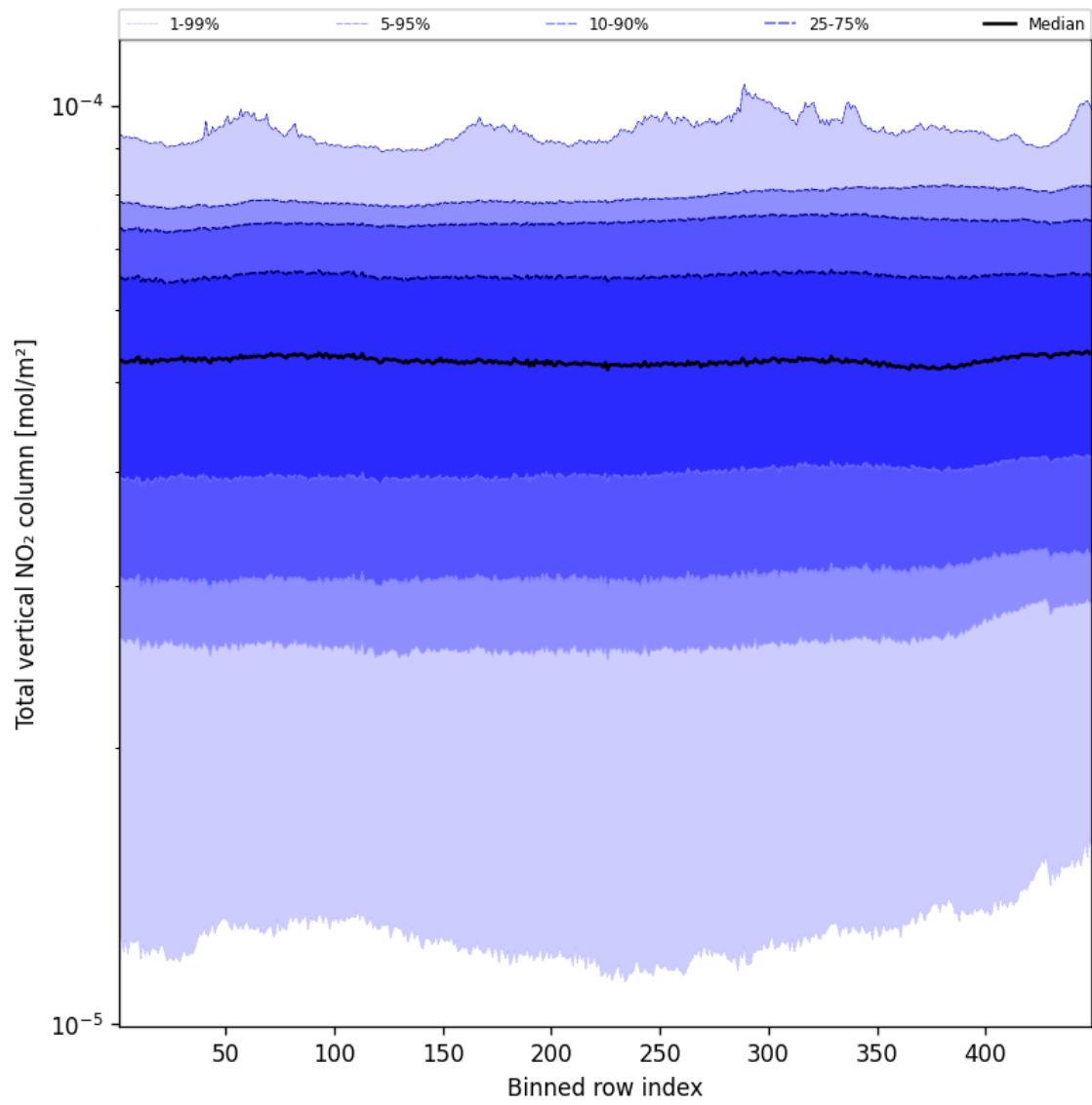
Figure 55: Along track statistics of “Total vertical NO 2 column” for 2025-02-08 to 2025-02-10
