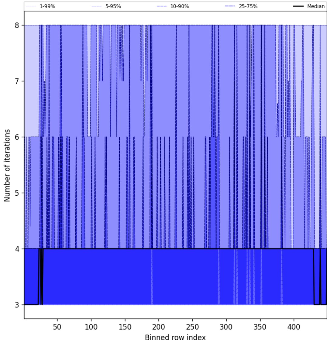
Figure 51: Along track statistics of “Number of iterations” for 2025-02-08 to 2025-02-10
