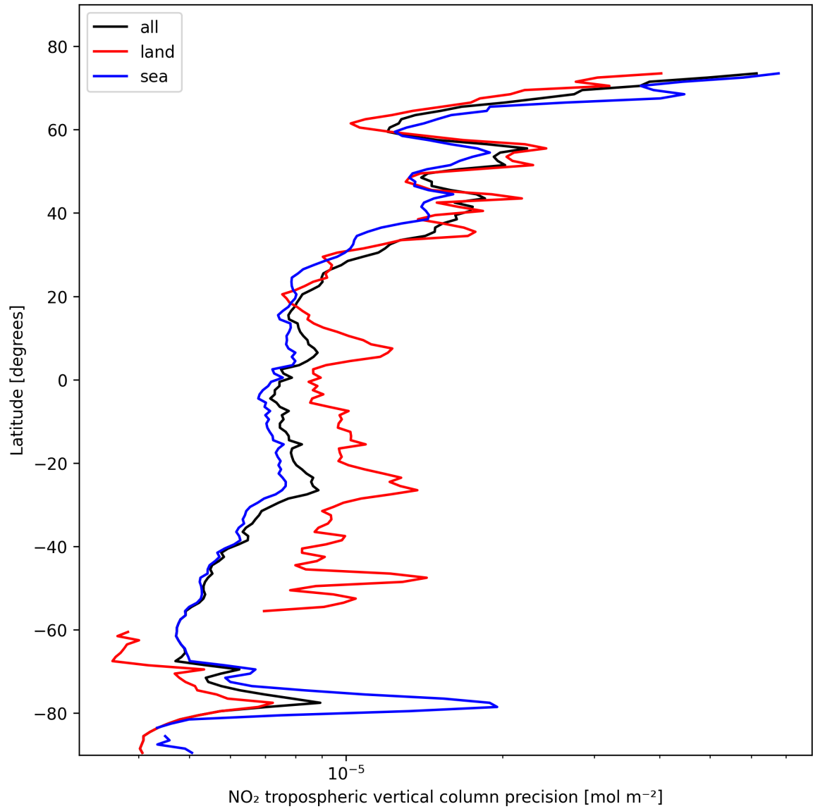
Figure 13: Zonal average of “NO 2 tropospheric vertical column precision” for 2025-02-08 to 2025-02-10.
