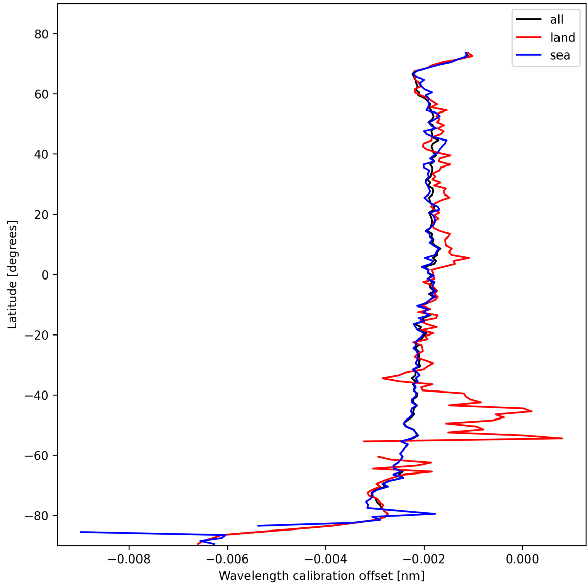
Figure 18: Zonal average of “Wavelength calibration offset” for 2025-02-08 to 2025-02-10.
