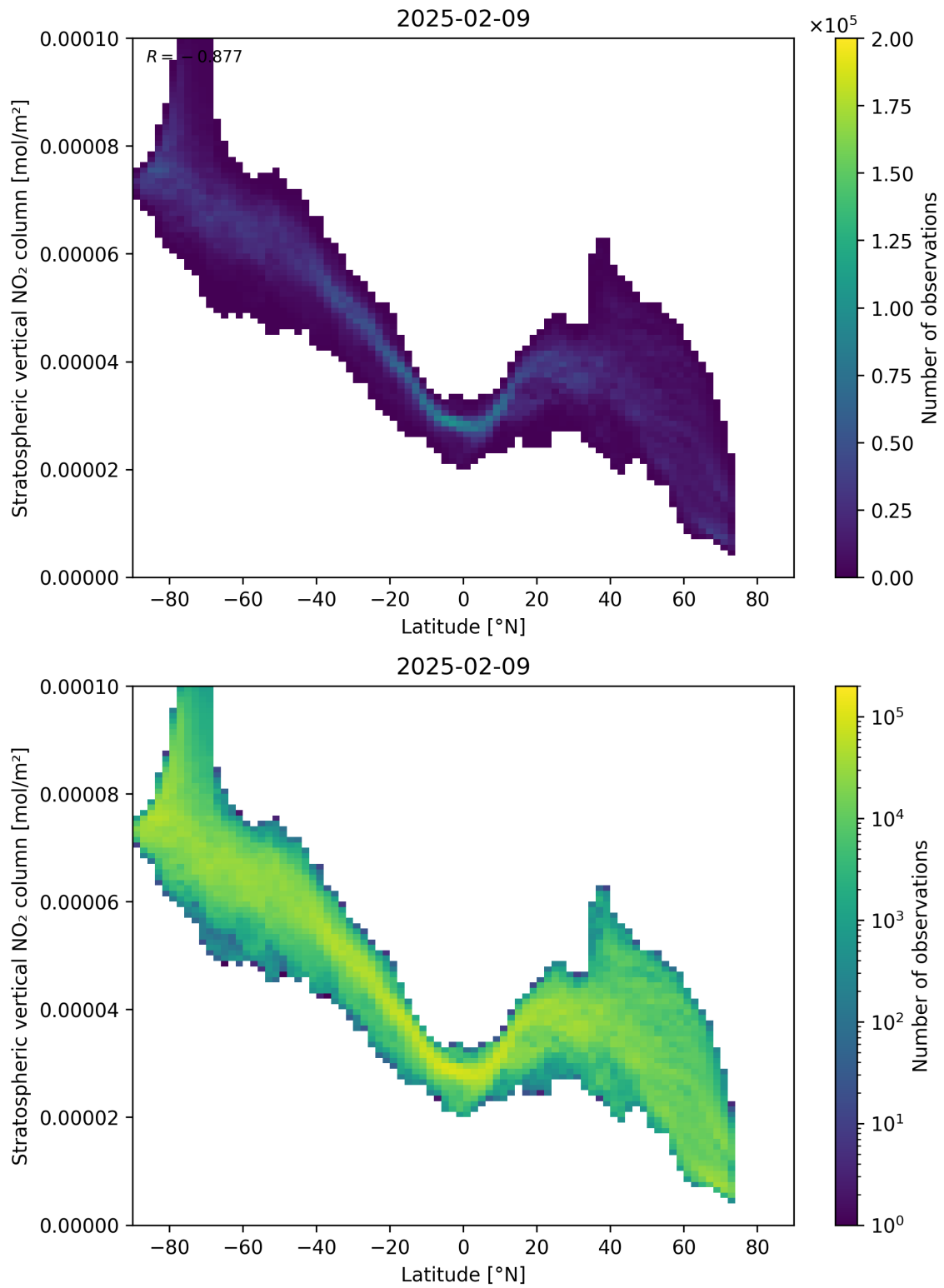
Figure 87: Scatter density plot of “Latitude” against “Stratospheric vertical NO 2 column” for 2025-02-08 to 2025-02-10.
