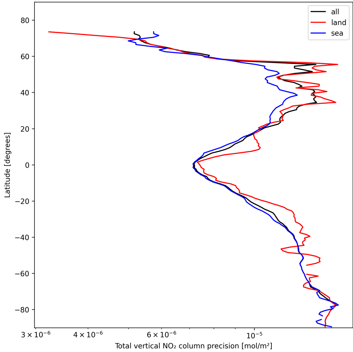
Figure 22: Zonal average of “Total vertical NO 2 column precision” for 2025-02-08 to 2025-02-10.
