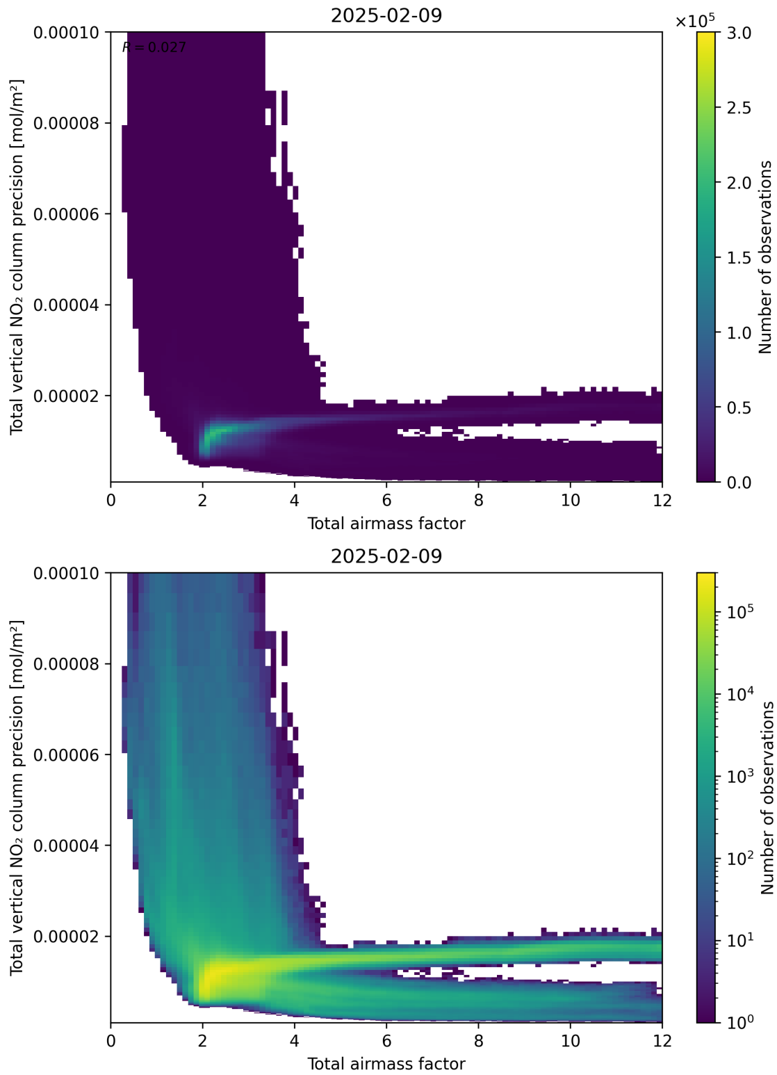
Figure 68: Scatter density plot of “Total airmass factor” against “Total vertical NO 2 column precision” for 2025-02-08 to 2025-02-10.
