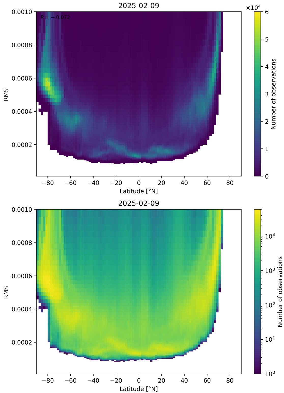
Figure 94: Scatter density plot of “Latitude” against “RMS” for 2025-02-08 to 2025-02-10.
