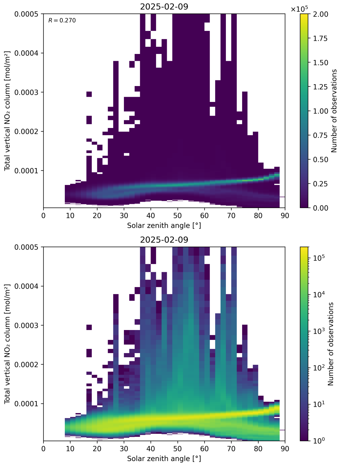
Figure 153: Scatter density plot of “Solar zenith angle” against “Total vertical NO 2 column” for 2025-02-08 to 2025-02-10.
