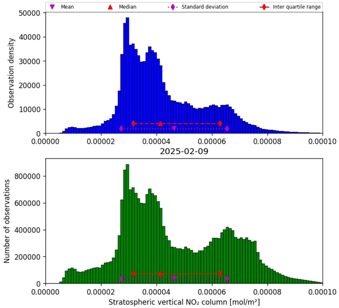
Figure 36: Histogram of “Stratospheric vertical NO 2 column” for 2025-02-08 to 2025-02-10
