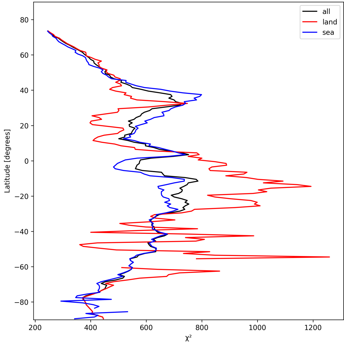
Figure 25: Zonal average of “ \chi^2 ” for 2025-02-08 to 2025-02-10.
