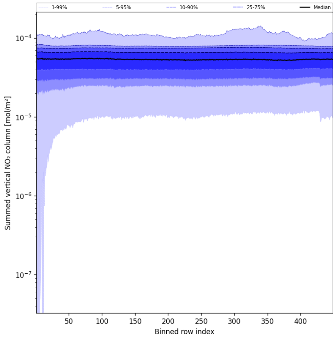
Figure 57: Along track statistics of “Summed vertical NO 2 column” for 2025-02-08 to 2025-02-10
