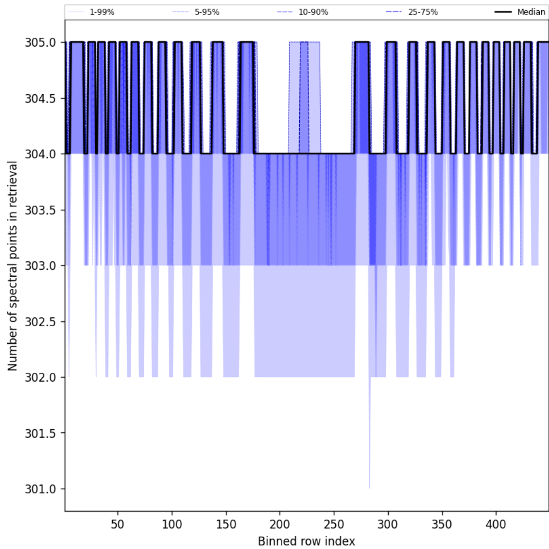
Figure 50: Along track statistics of “Number of spectral points in retrieval” for 2025-02-08 to 2025-02-10
