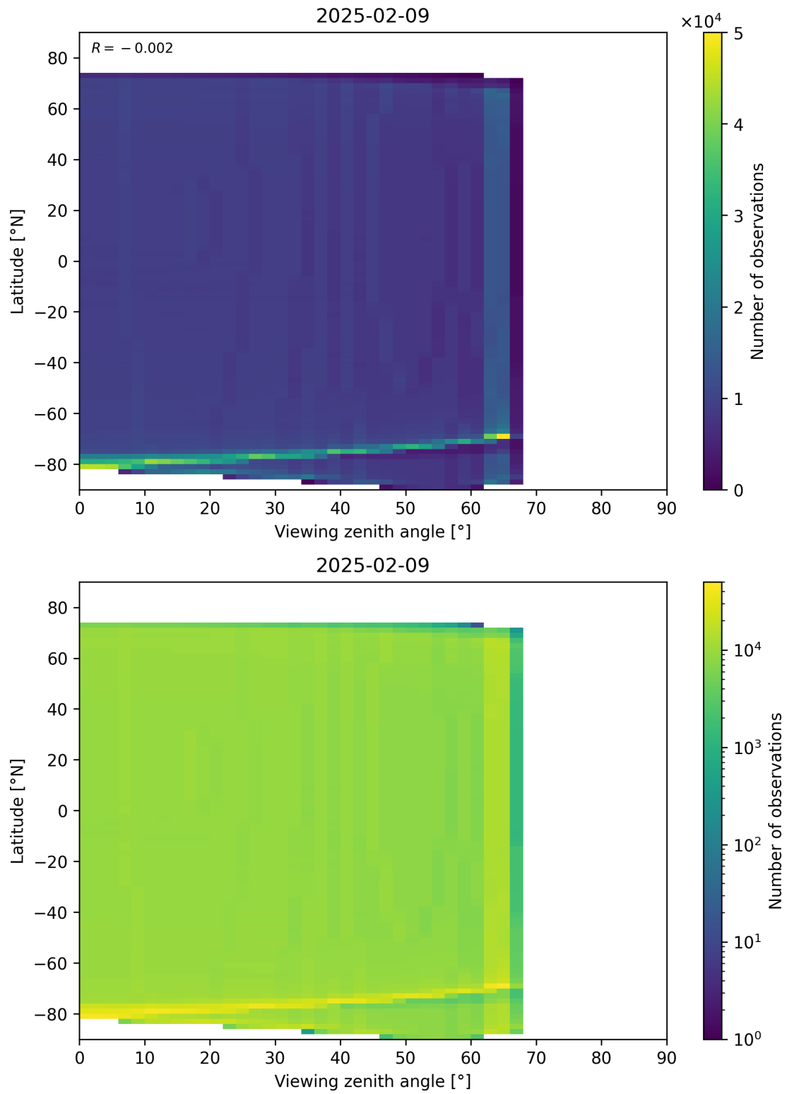
Figure 163: Scatter density plot of “Viewing zenith angle” against “Latitude” for 2025-02-08 to 2025-02-10.
