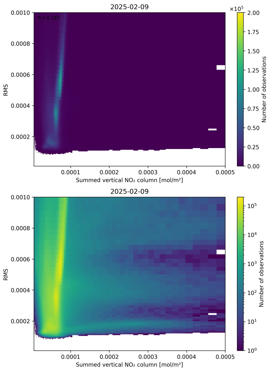
Figure 109: Scatter density plot of “Summed vertical NO 2 column” against “RMS” for 2025-02-08 to 2025-02-10.
