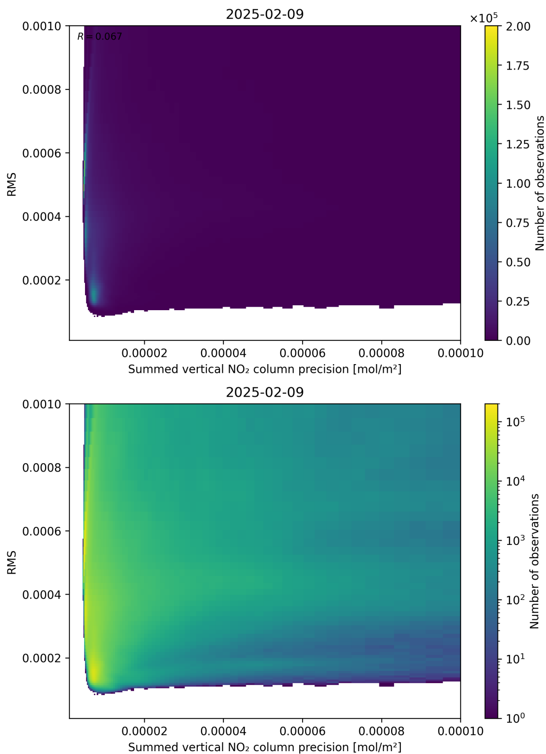
Figure 108: Scatter density plot of “Summed vertical NO 2 column precision” against “RMS” for 2025-02-08 to 2025-02-10.
