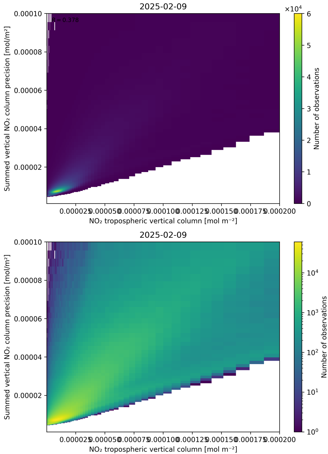
Figure 127: Scatter density plot of “NO 2 tropospheric vertical column” against “Summed vertical NO 2 column precision” for 2025-02-08 to 2025-02-10.
