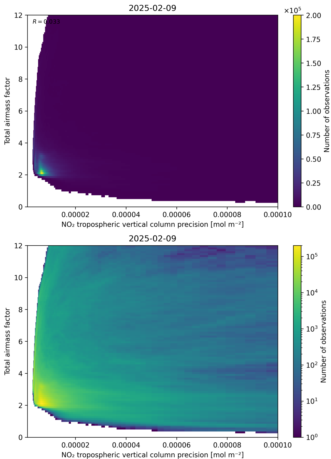
Figure 132: Scatter density plot of “NO 2 tropospheric vertical column precision” against “Total air mass factor” for 2025-02-08 to 2025-02-10.
