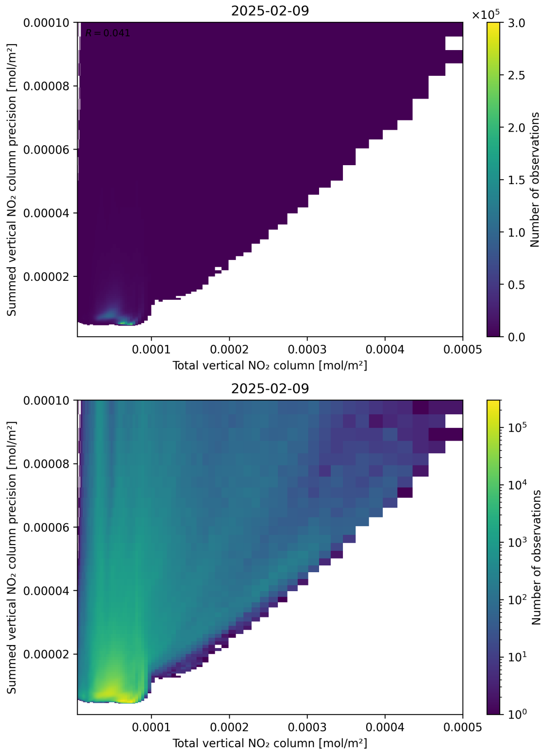
Figure 113: Scatter density plot of “Total vertical NO 2 column” against “Summed vertical NO 2 column precision” for 2025-02-08 to 2025-02-10.
