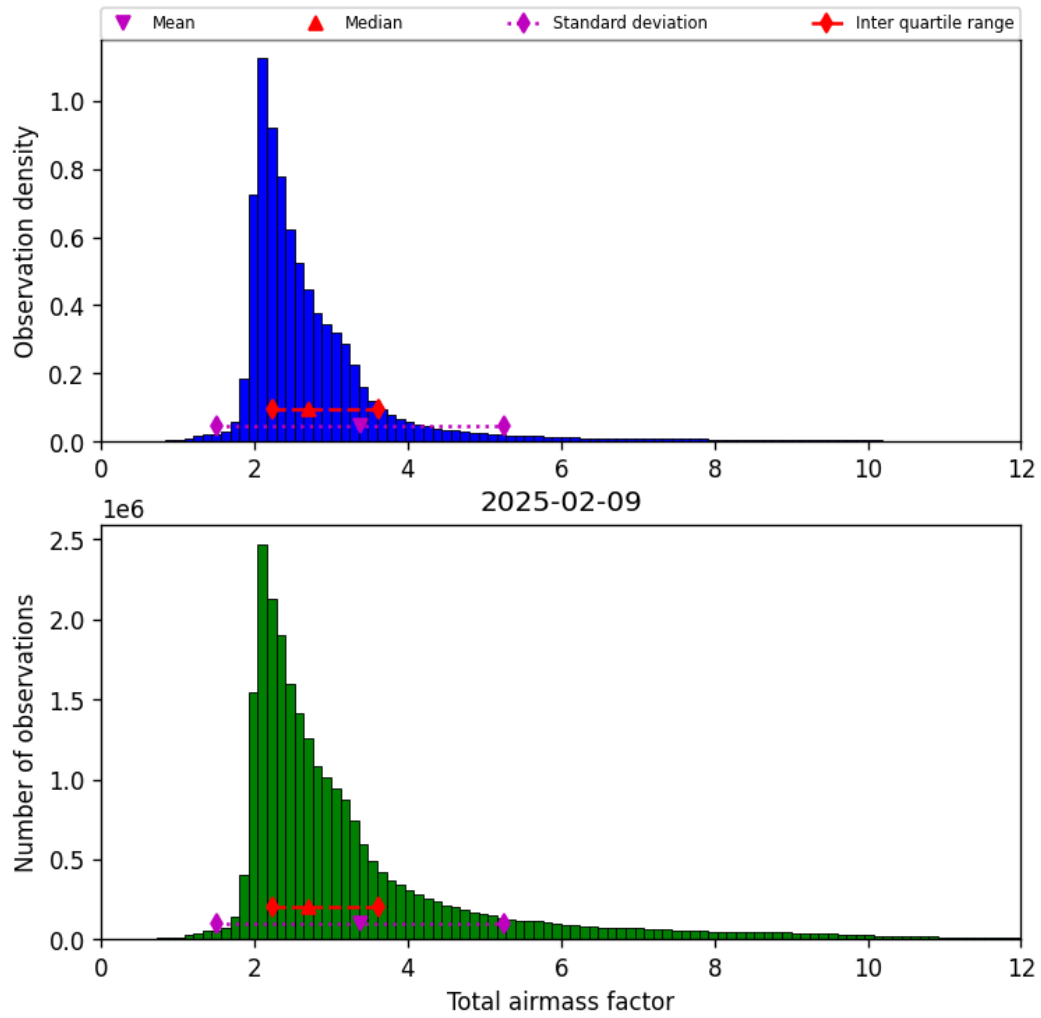
Figure 32: Histogram of “Total airmass factor” for 2025-02-08 to 2025-02-10
