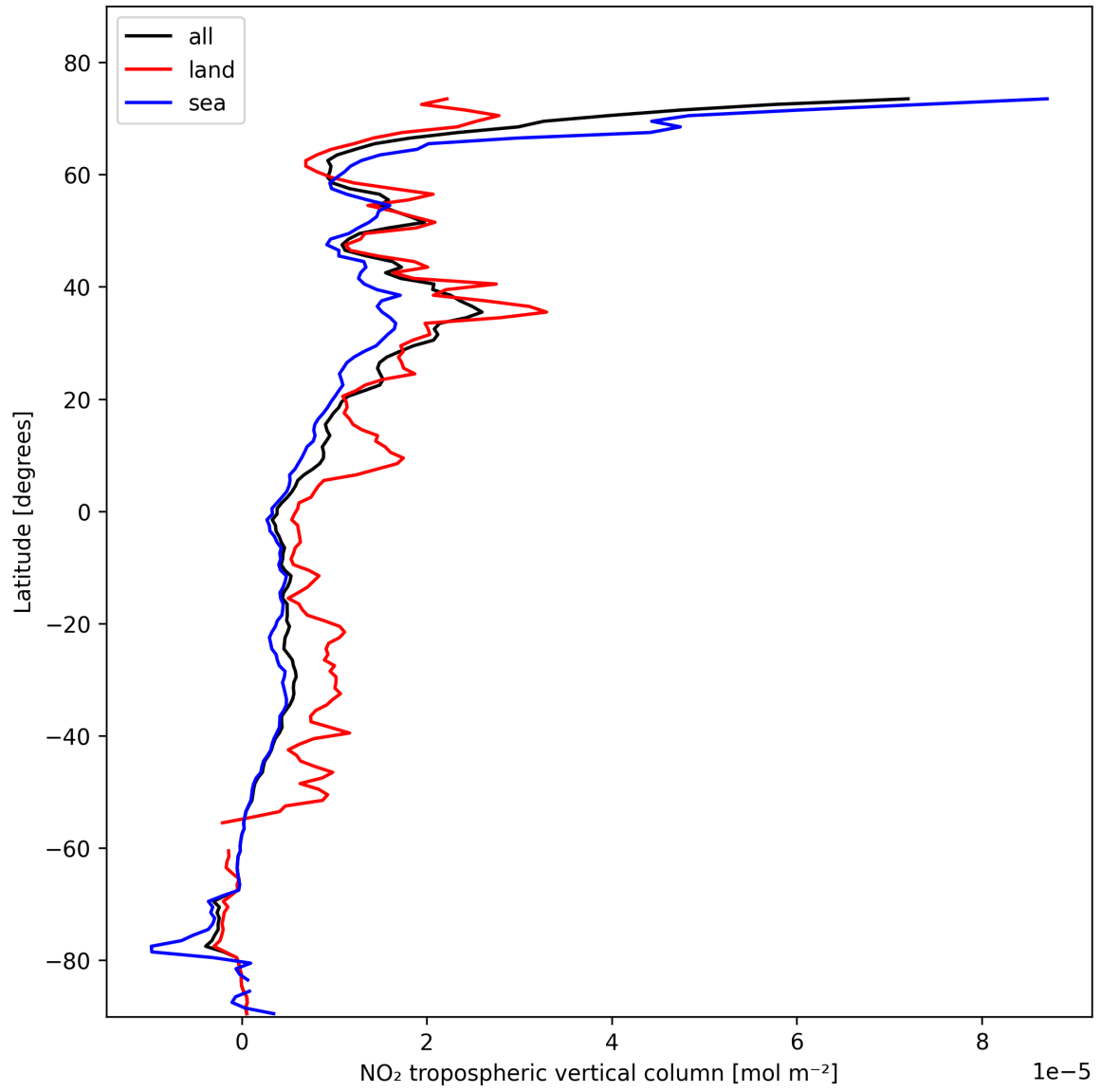
Figure 12: Zonal average of “NO 2 tropospheric vertical column” for 2025-02-08 to 2025-02-10.
