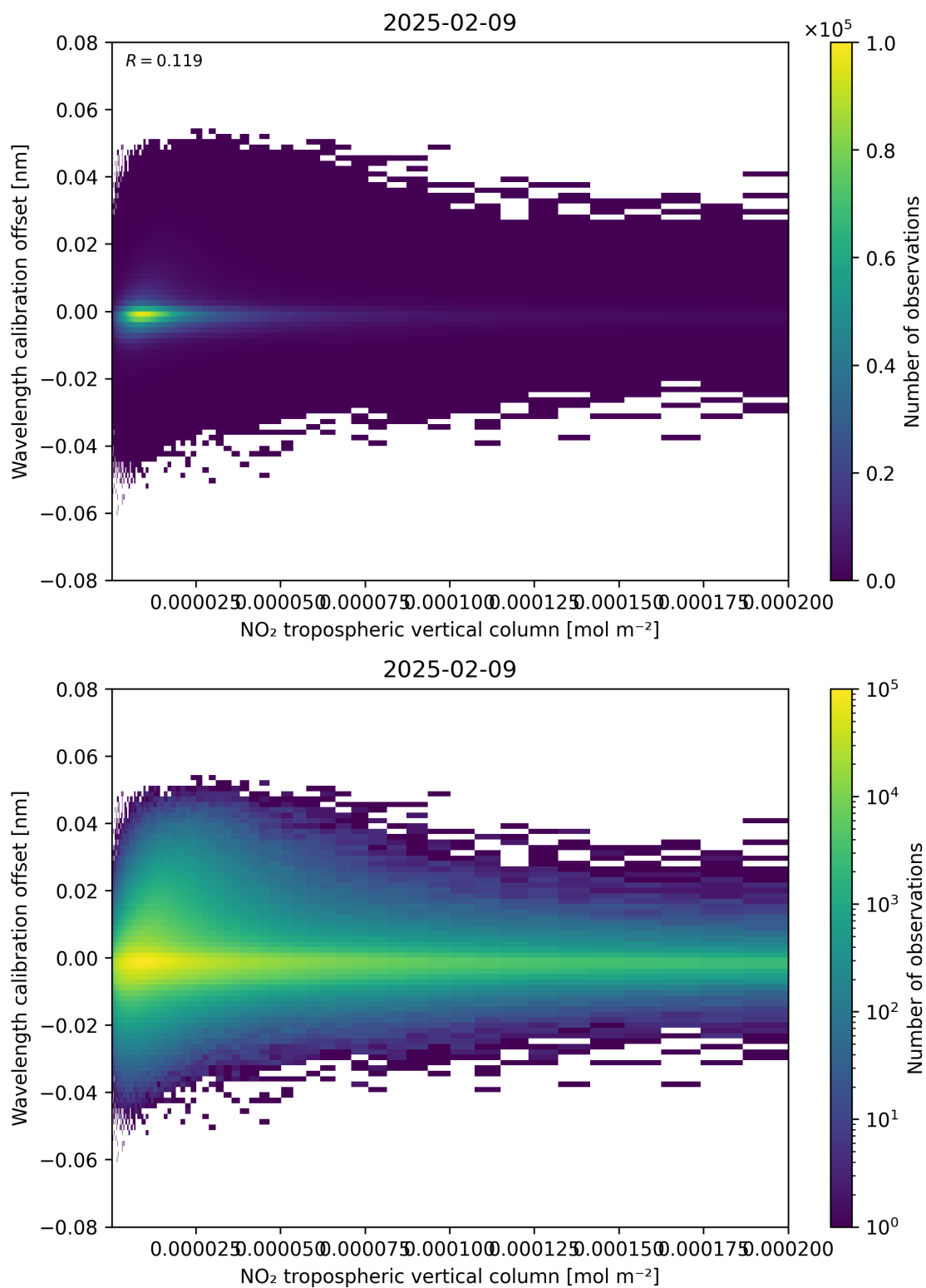
Figure 143: Scatter density plot of “NO 2 tropospheric vertical column” against “Wavelength calibration offset” for 2025-02-08 to 2025-02-10.
