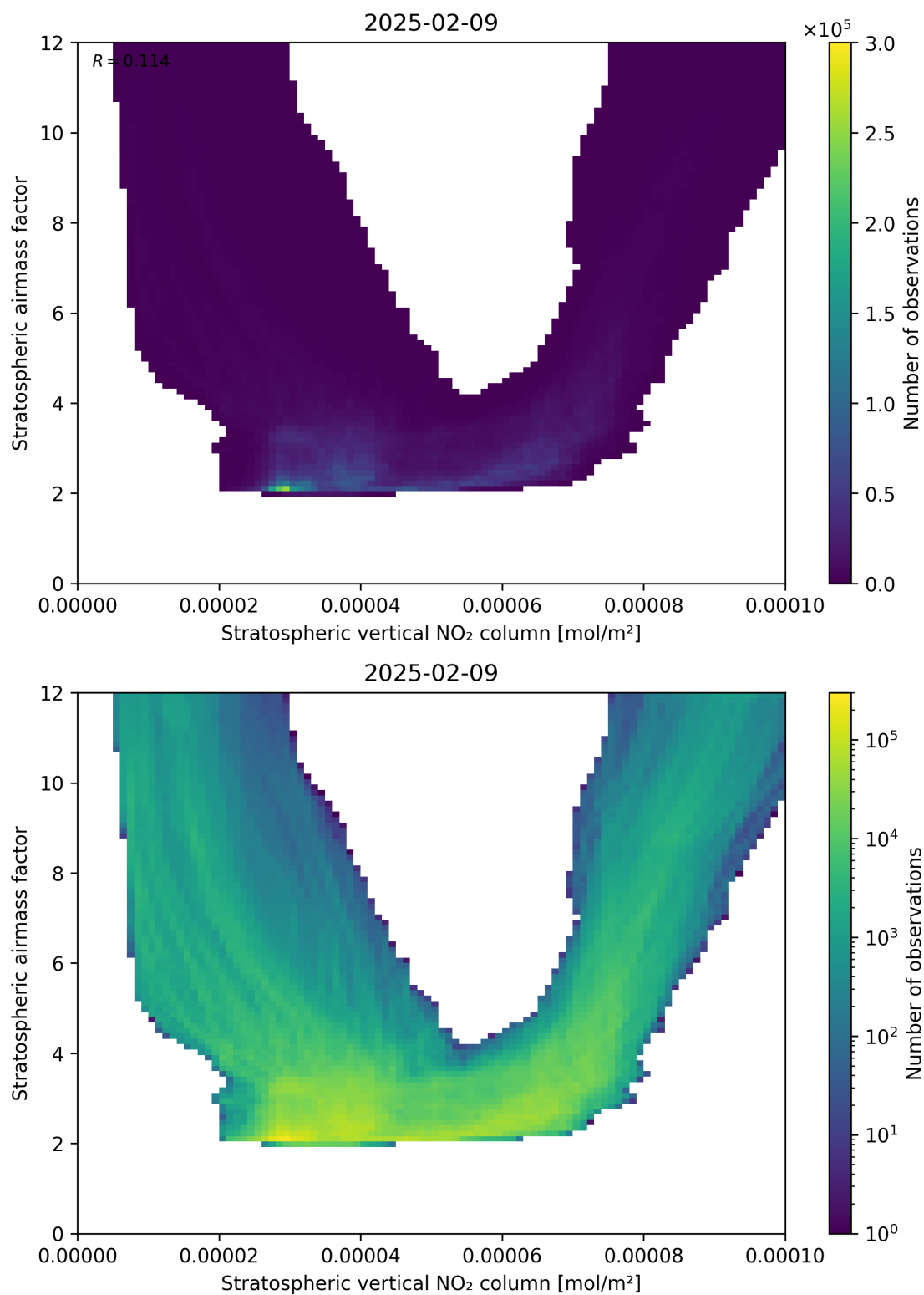
Figure 96: Scatter density plot of “Stratospheric vertical NO 2 column” against “Stratospheric airmass factor” for 2025-02-08 to 2025-02-10.
