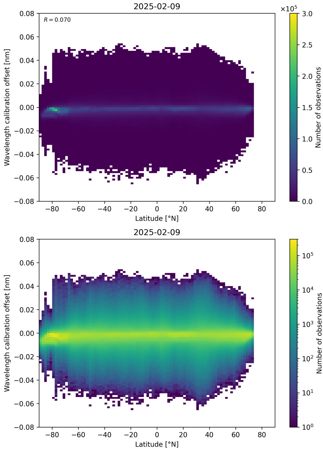
Figure 95: Scatter density plot of “Latitude” against “Wavelength calibration offset” for 2025-02-08 to 2025-02-10.
