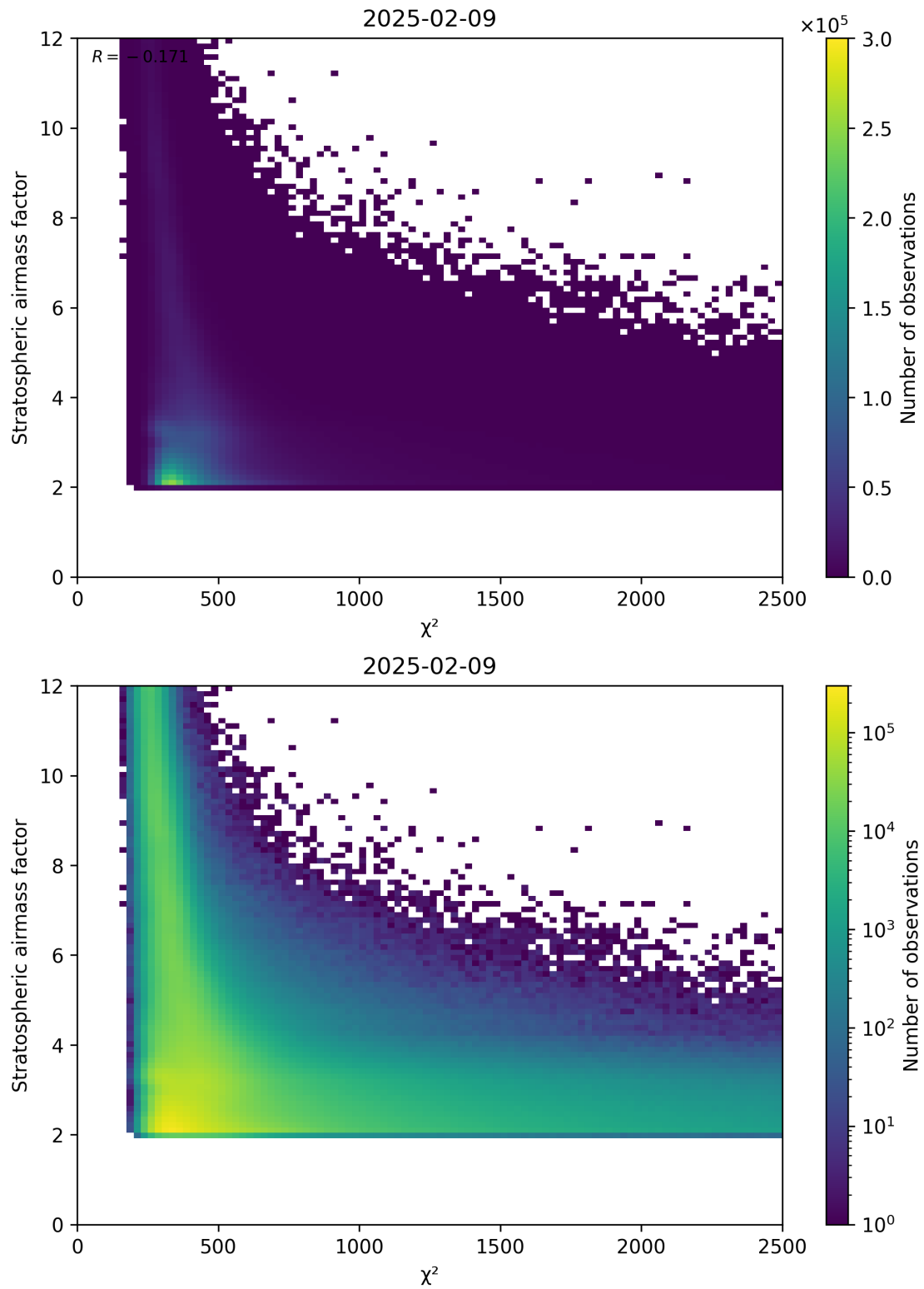
Figure 81: Scatter density plot of “ \chi^2 ” against “Stratospheric airmass factor” for 2025-02-08 to 2025-02-10.
