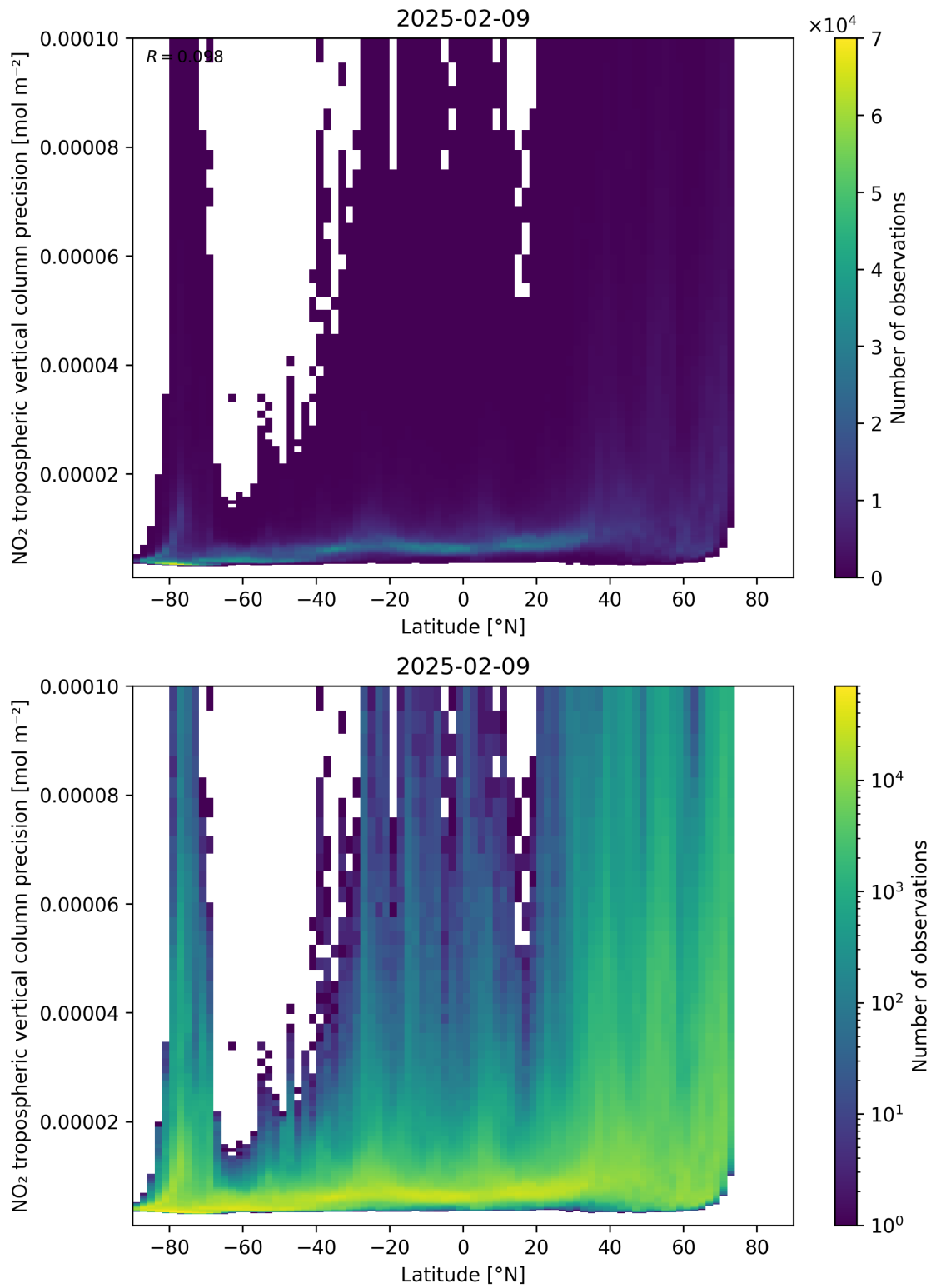
Figure 93: Scatter density plot of “Latitude” against “NO 2 tropospheric vertical column precision” for 2025-02-08 to 2025-02-10.
