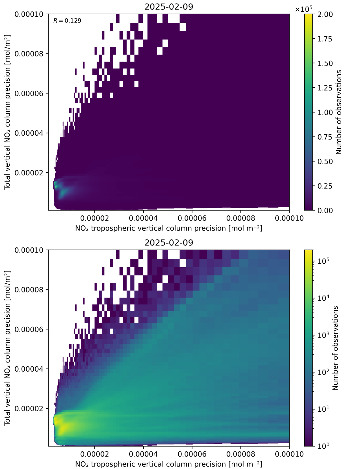
Figure 139: Scatter density plot of “NO 2 tropospheric vertical column precision” against “Total vertical NO 2 column precision” for 2025-02-08 to 2025-02-10.
