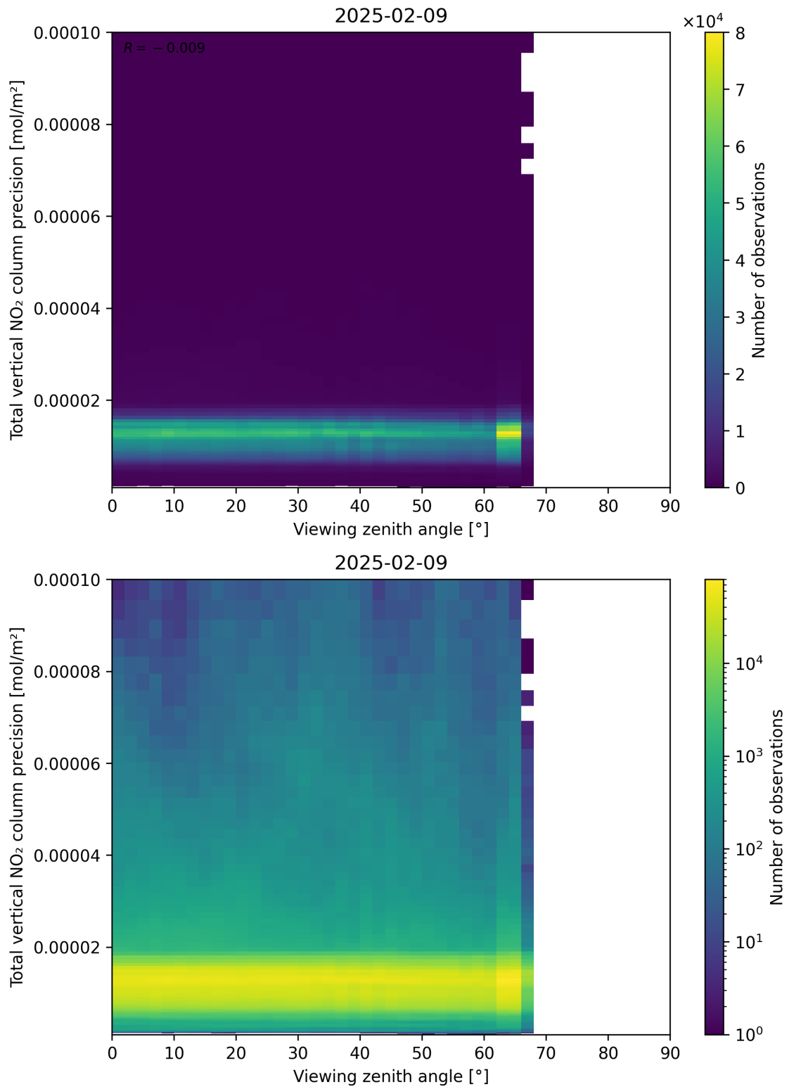
Figure 168: Scatter density plot of “Viewing zenith angle” against “Total vertical NO 2 column precision” for 2025-02-08 to 2025-02-10.
