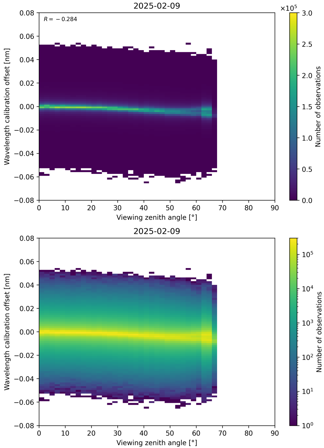
Figure 173: Scatter density plot of “Viewing zenith angle” against “Wavelength calibration offset” for 2025-02-08 to 2025-02-10.
