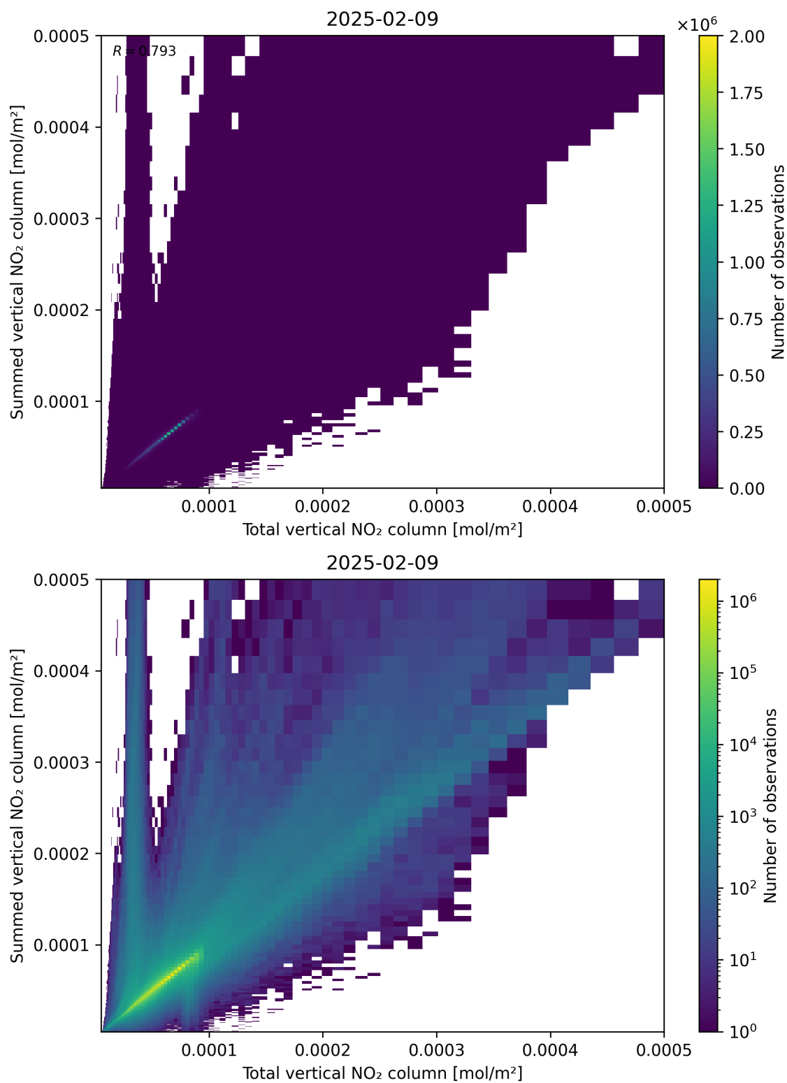
Figure 112: Scatter density plot of “Total vertical NO 2 column” against “Summed vertical NO 2 column” for 2025-02-08 to 2025-02-10.
