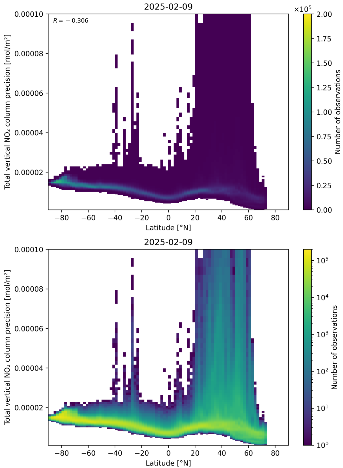
Figure 91: Scatter density plot of “Latitude” against “Total vertical NO 2 column precision” for 2025-02-08 to 2025-02-10.
