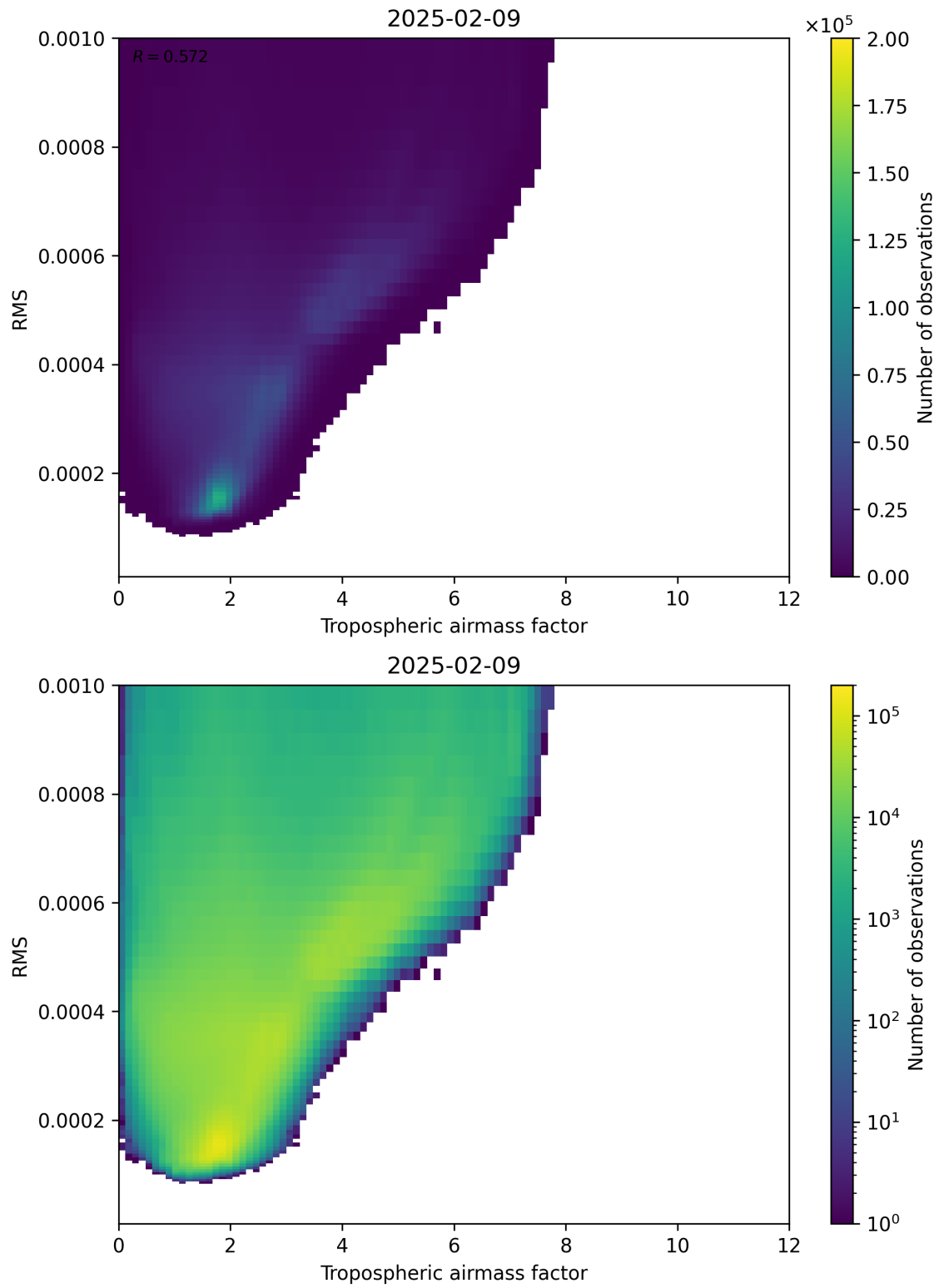
Figure 79: Scatter density plot of “Tropospheric airmass factor” against “RMS” for 2025-02-08 to 2025-02-10.
