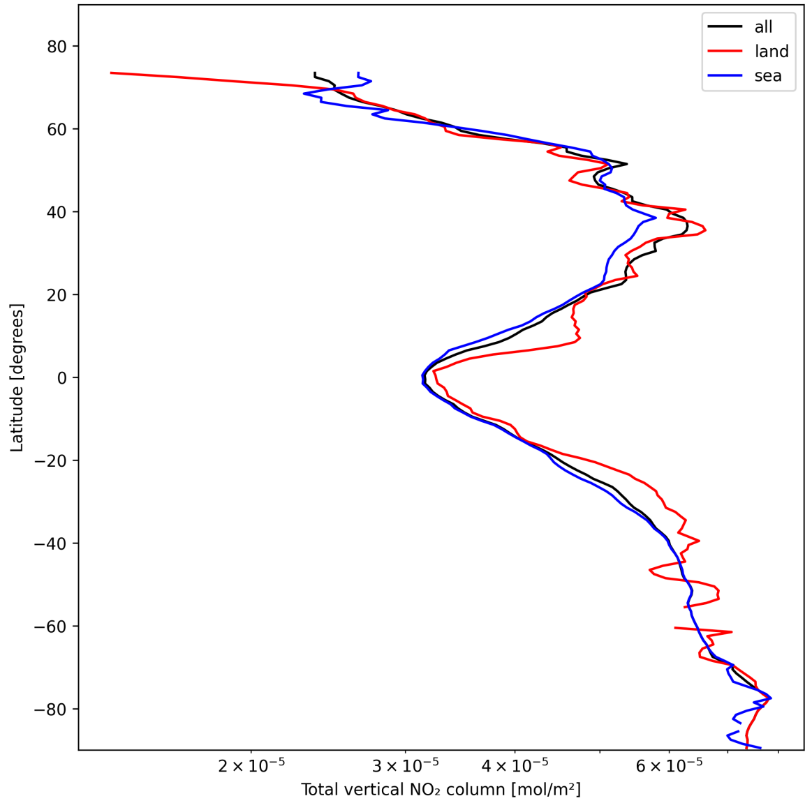
Figure 21: Zonal average of “Total vertical NO 2 column” for 2025-02-08 to 2025-02-10.
