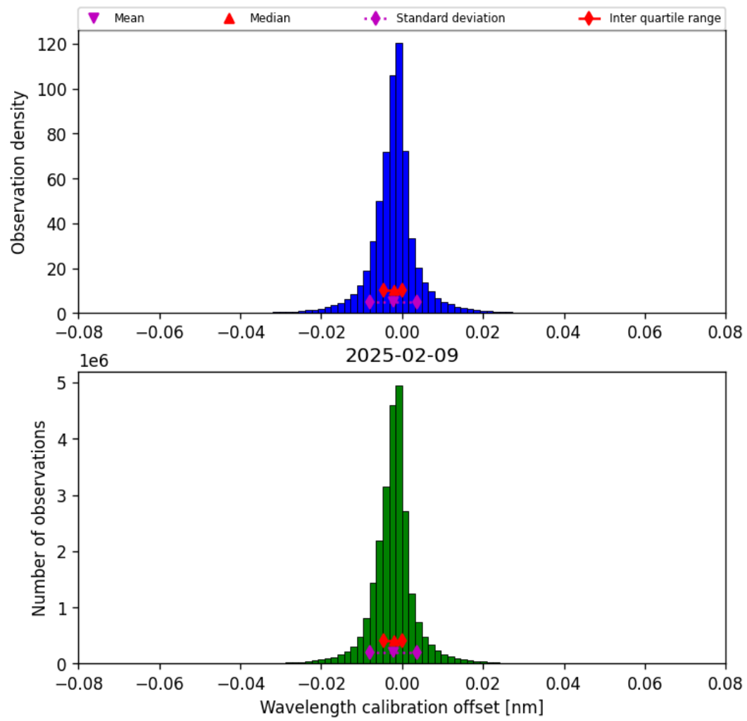
Figure 35: Histogram of “Wavelength calibration offset” for 2025-02-08 to 2025-02-10
