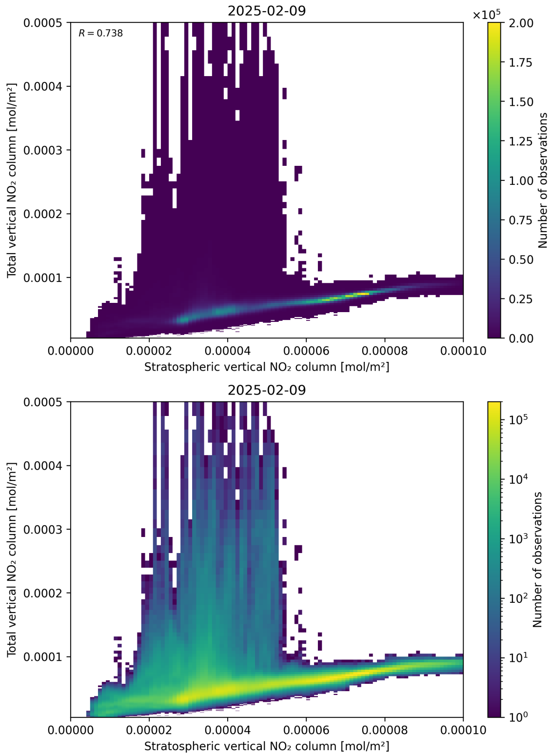
Figure 100: Scatter density plot of “Stratospheric vertical NO 2 column” against “Total vertical NO 2 column” for 2025-02-08 to 2025-02-10.
