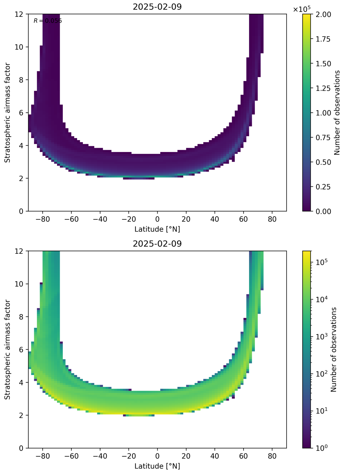
Figure 83: Scatter density plot of “Latitude” against “Stratospheric air mass factor” for 2025-02-08 to 2025-02-10.
