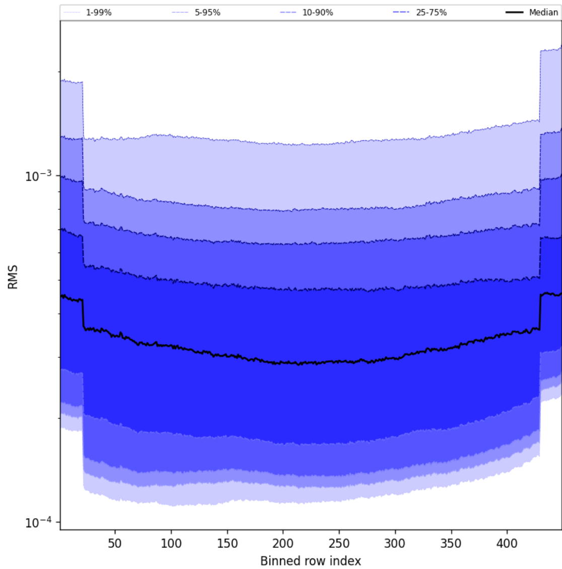
Figure 60: Along track statistics of “RMS” for 2025-02-08 to 2025-02-10
