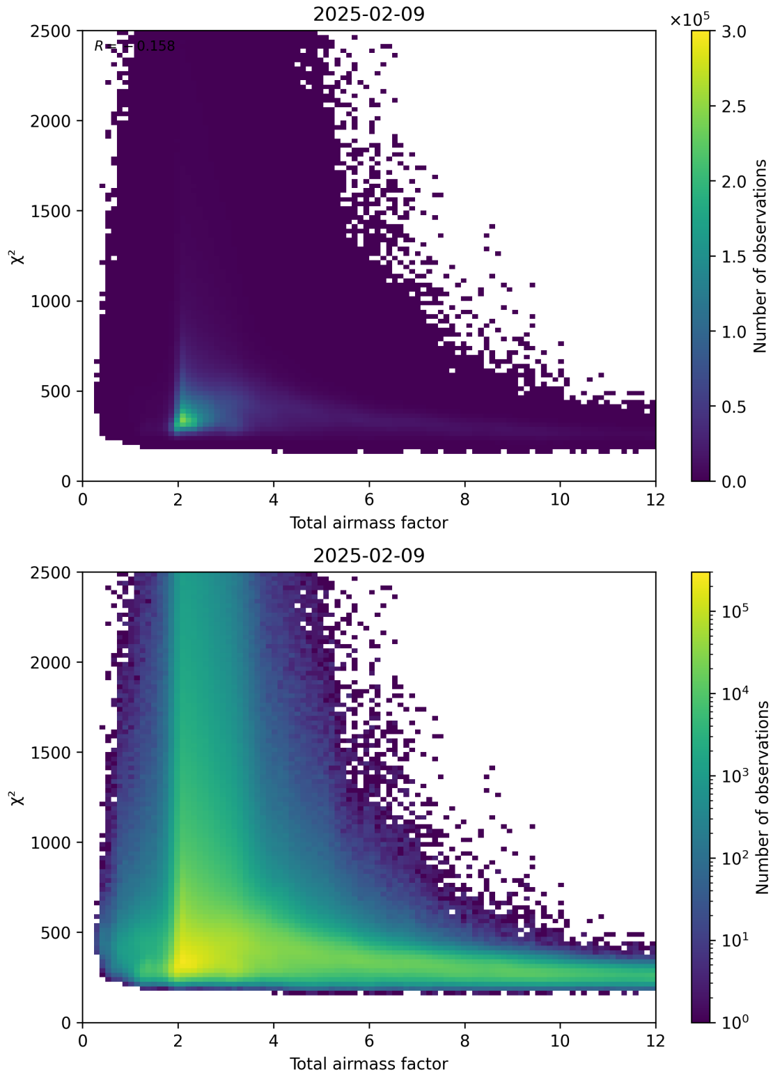
Figure 63: Scatter density plot of “Total airmass factor” against “ \chi^2 ” for 2025-02-08 to 2025-02-10.
