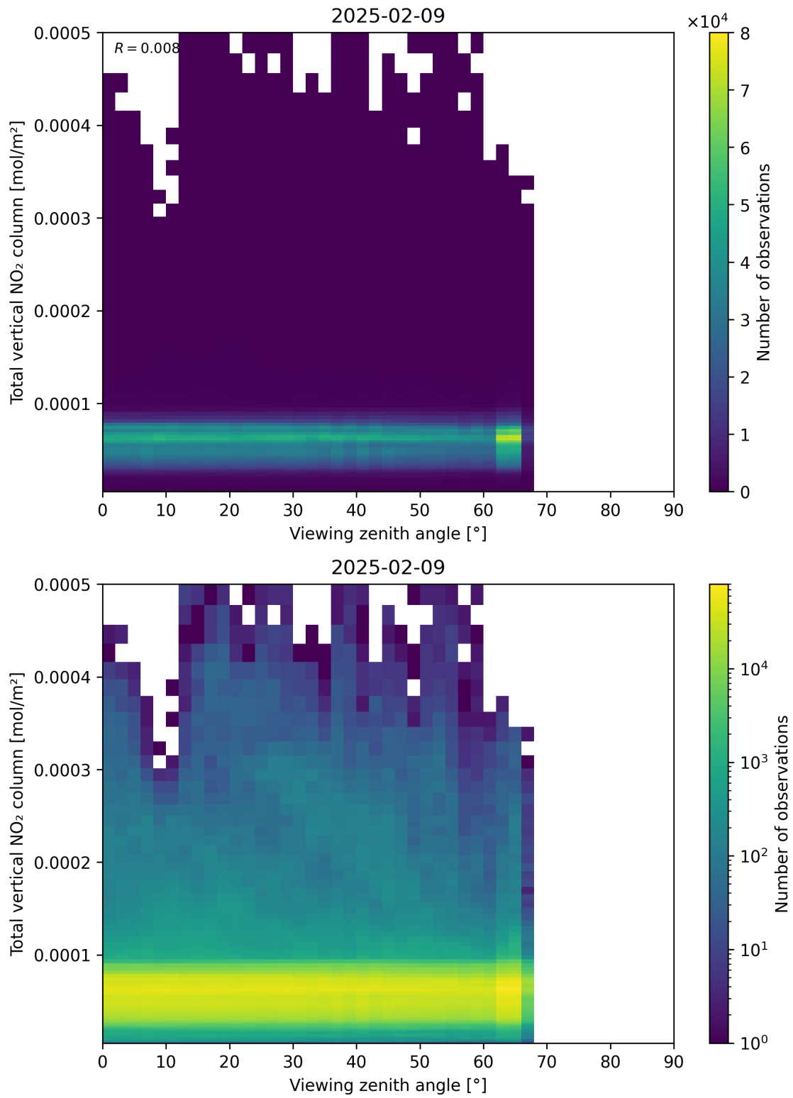
Figure 167: Scatter density plot of “Viewing zenith angle” against “Total vertical NO 2 column” for 2025-02-08 to 2025-02-10.
