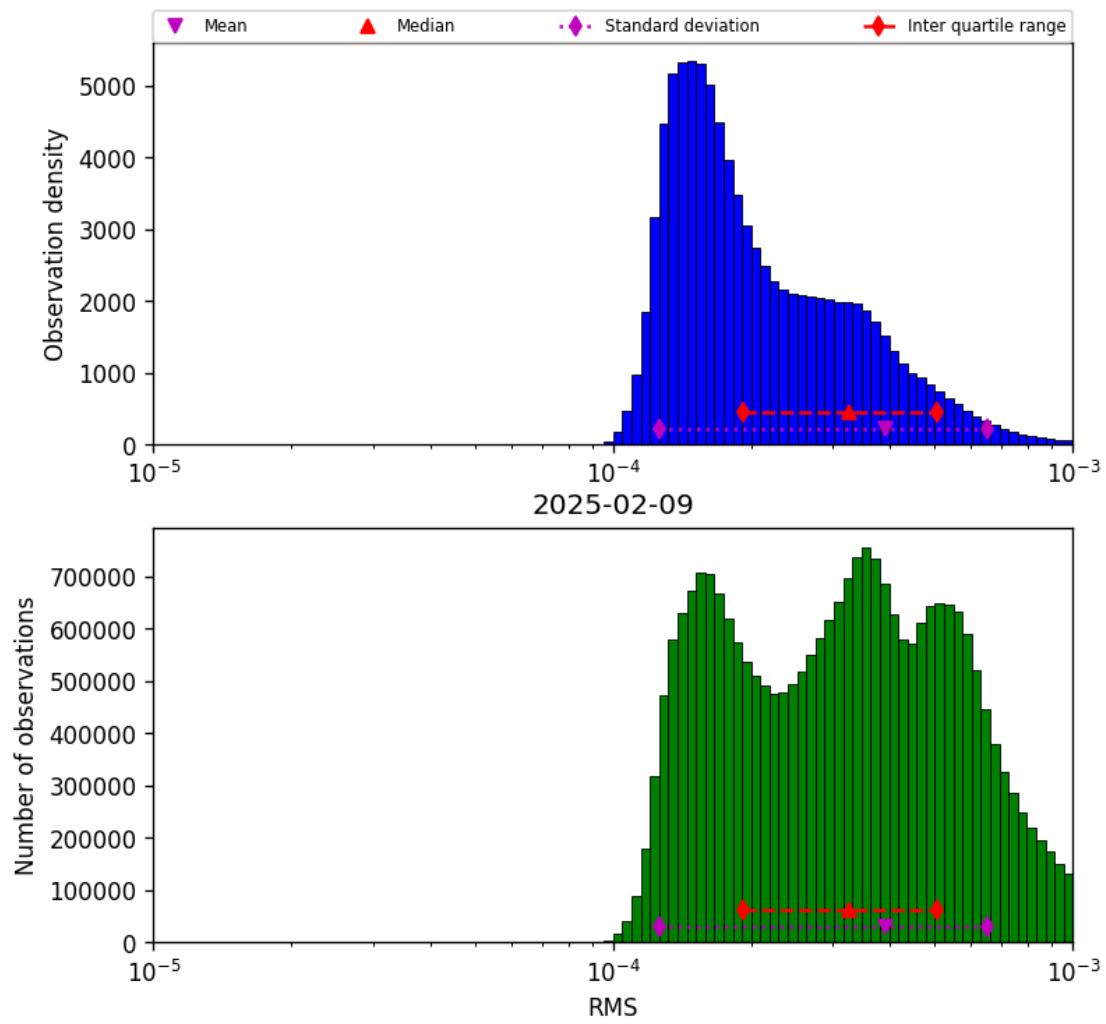
Figure 43: Histogram of “RMS” for 2025-02-08 to 2025-02-10
