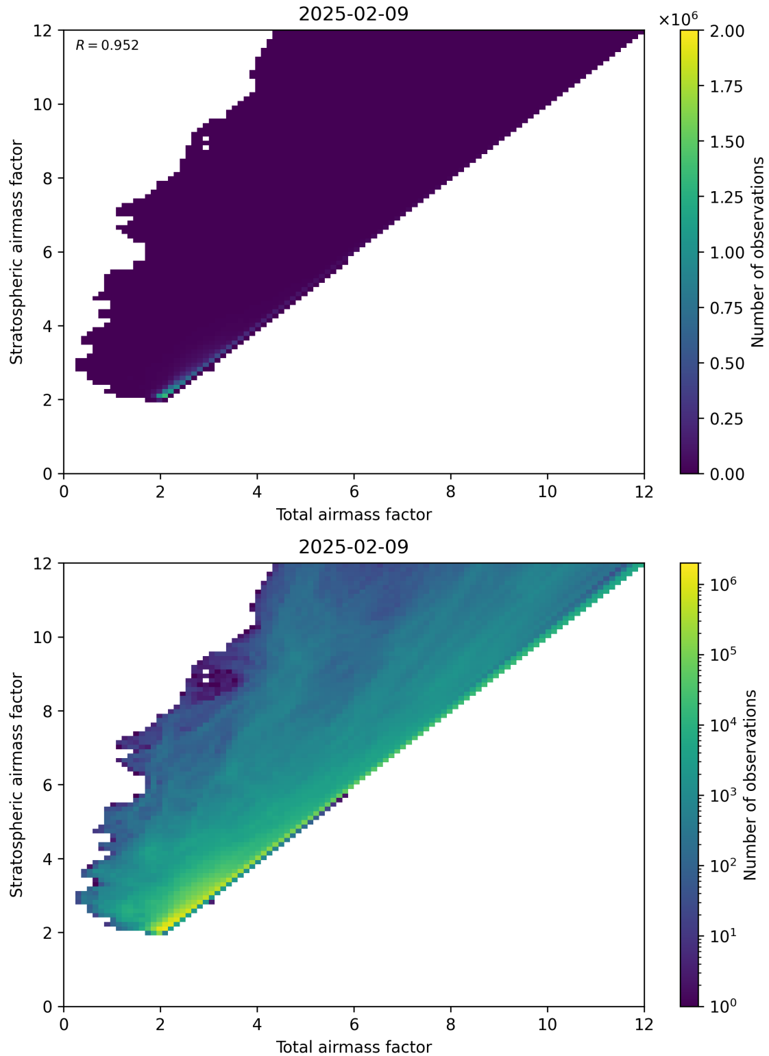
Figure 62: Scatter density plot of “Total airmass factor” against “Stratospheric airmass factor” for 2025-02-08 to 2025-02-10.
