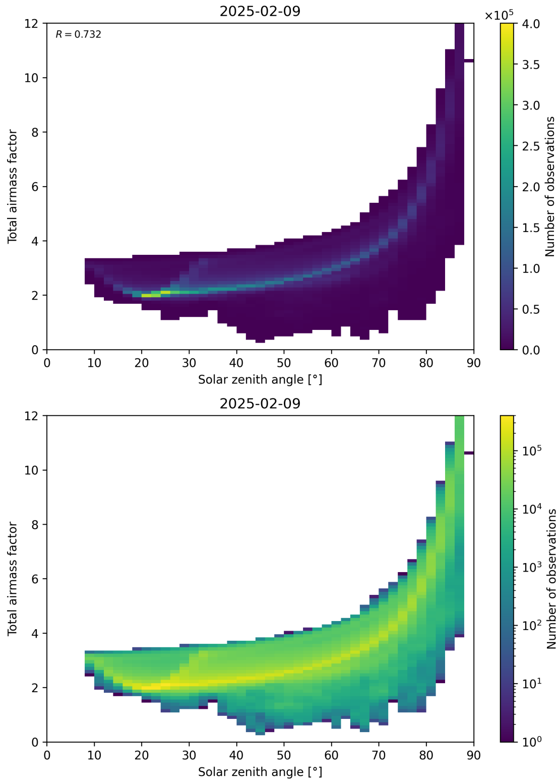
Figure 146: Scatter density plot of “Solar zenith angle” against “Total air mass factor” for 2025-02-08 to 2025-02-10.
