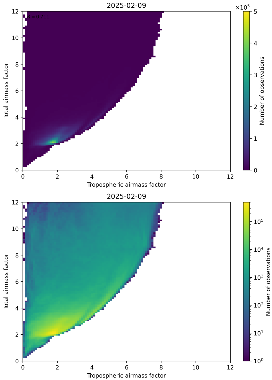
Figure 72: Scatter density plot of “Tropospheric airmass factor” against “Total airmass factor” for 2025-02-08 to 2025-02-10.
