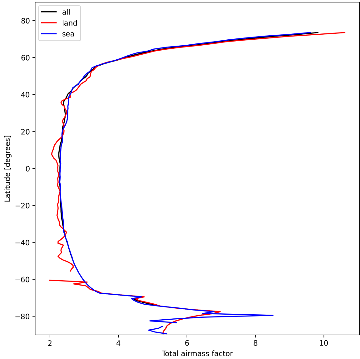
Figure 15: Zonal average of “Total airmass factor” for 2025-02-08 to 2025-02-10.
