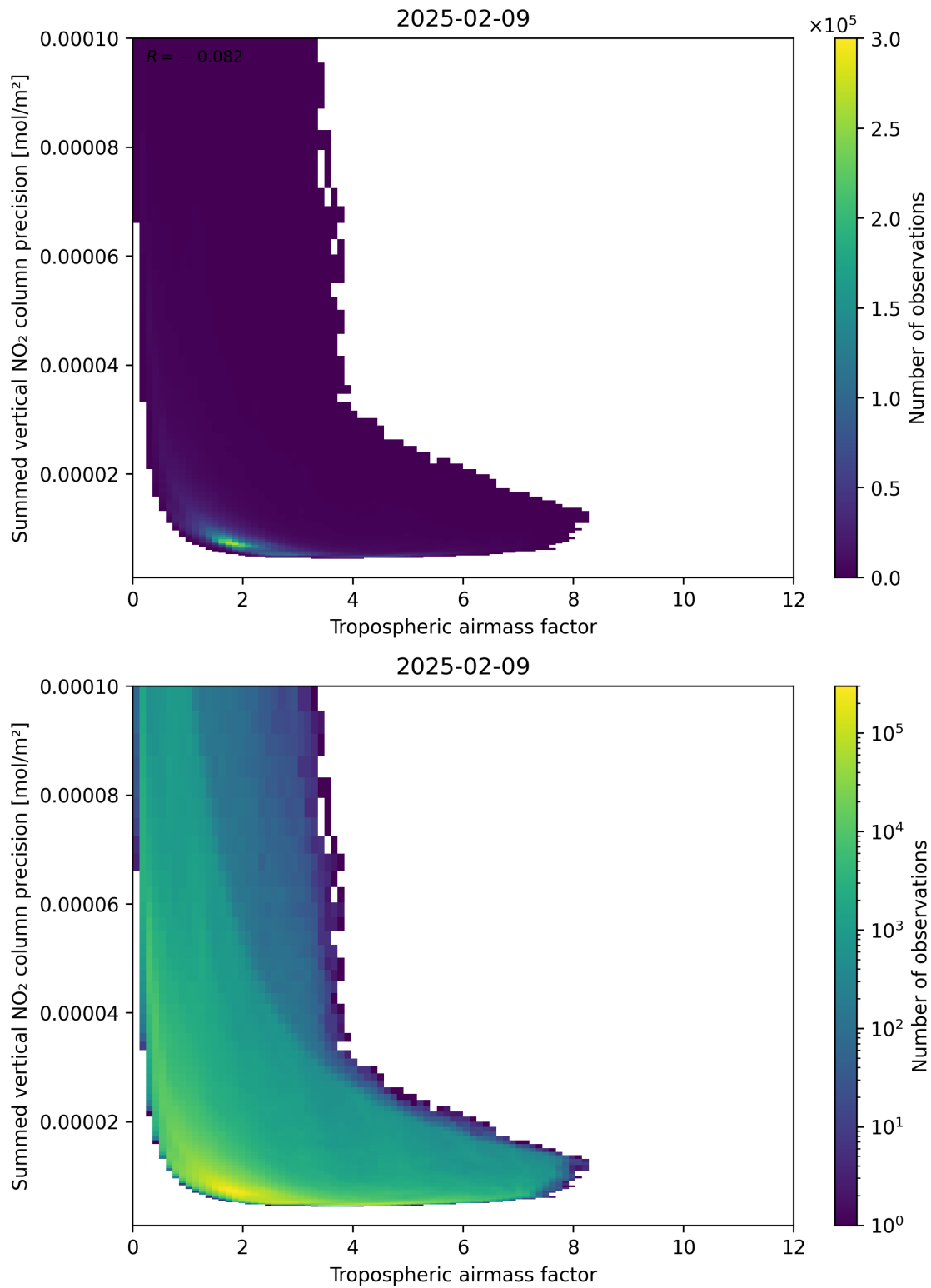
Figure 76: Scatter density plot of “Tropospheric air mass factor” against “Summed vertical NO 2 column precision” for 2025-02-08 to 2025-02-10.
