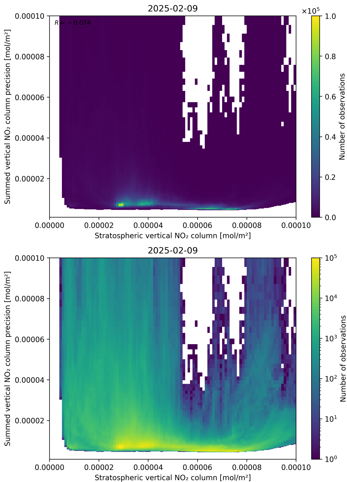
Figure 99: Scatter density plot of “Stratospheric vertical NO 2 column” against “Summed vertical NO 2 column precision” for 2025-02-08 to 2025-02-10.
