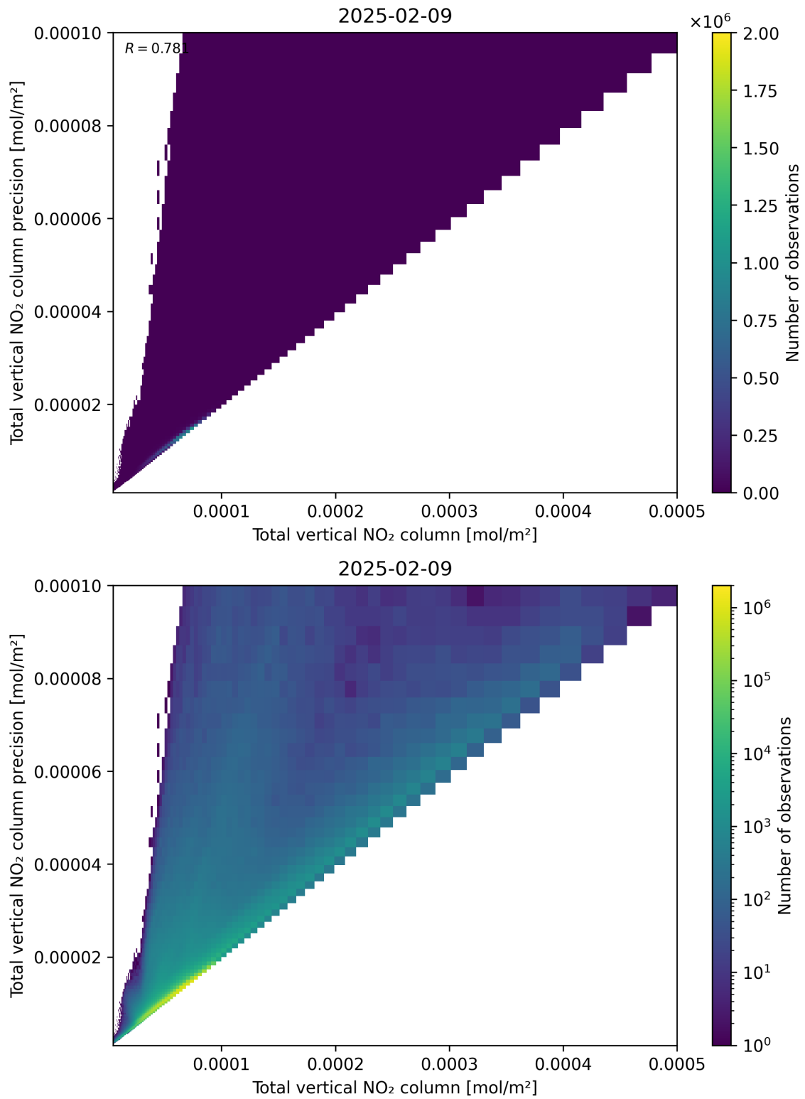
Figure 114: Scatter density plot of “Total vertical NO 2 column” against “Total vertical NO 2 column precision” for 2025-02-08 to 2025-02-10.
