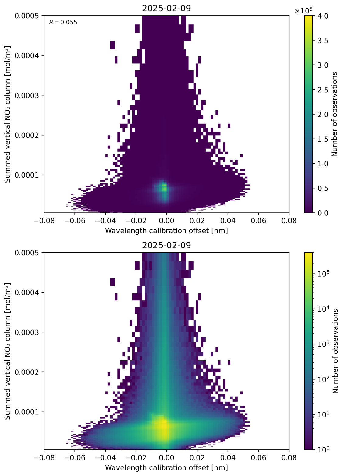
Figure 177: Scatter density plot of “Wavelength calibration offset” against “Summed vertical NO 2 column” for 2025-02-08 to 2025-02-10.
