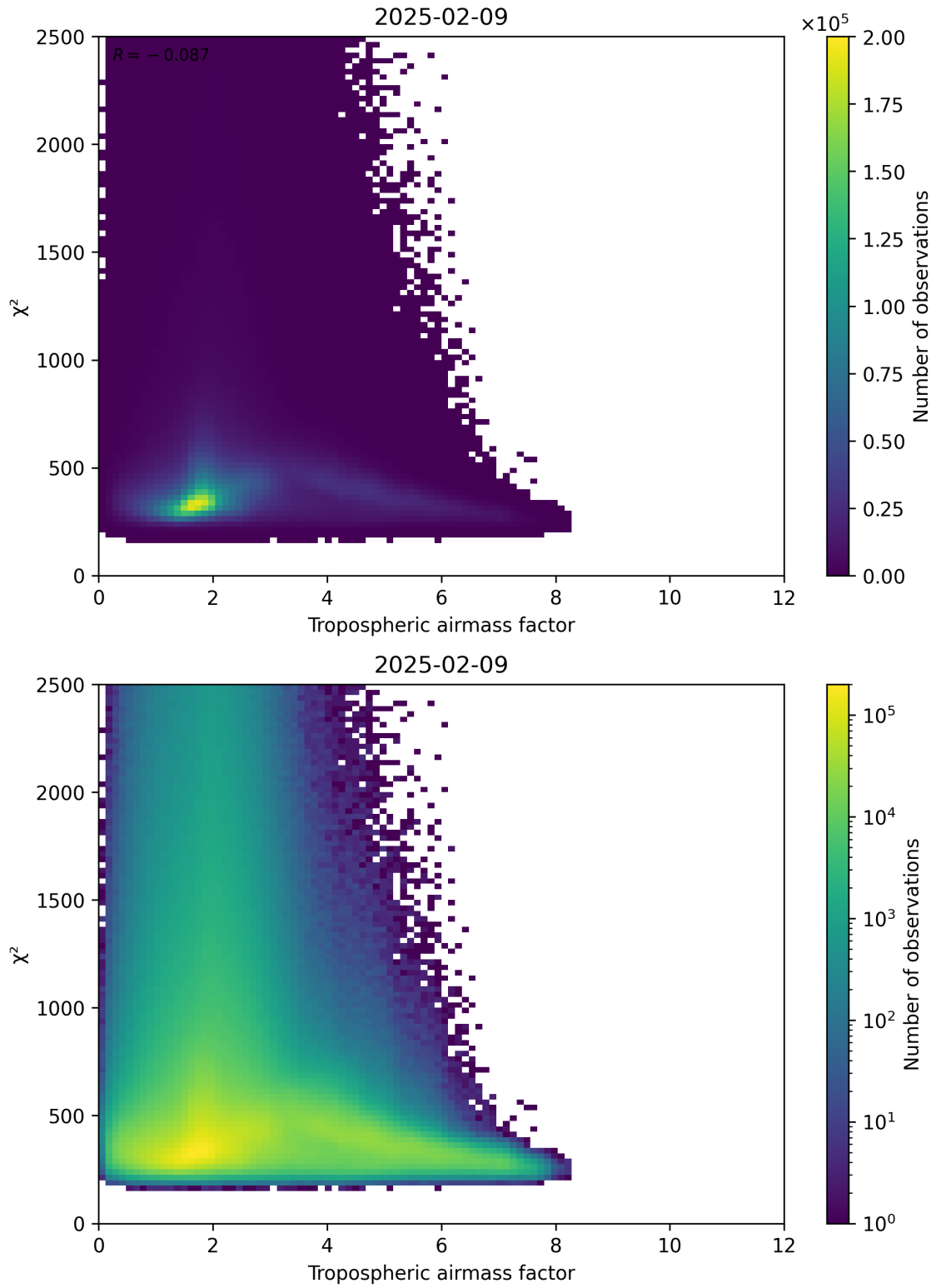
Figure 73: Scatter density plot of “Tropospheric airmass factor” against “ \chi^2 ” for 2025-02-08 to 2025-02-10.
