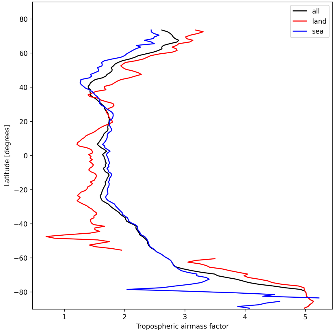
Figure 14: Zonal average of “Tropospheric airmass factor” for 2025-02-08 to 2025-02-10.
