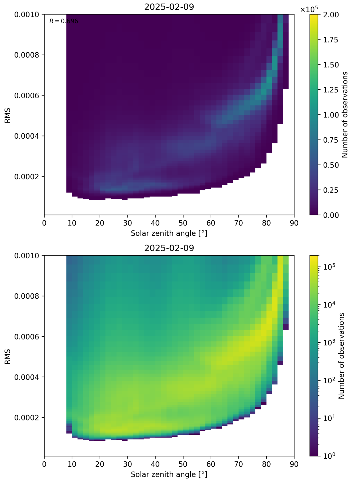
Figure 157: Scatter density plot of “Solar zenith angle” against “RMS” for 2025-02-08 to 2025-02-10.
