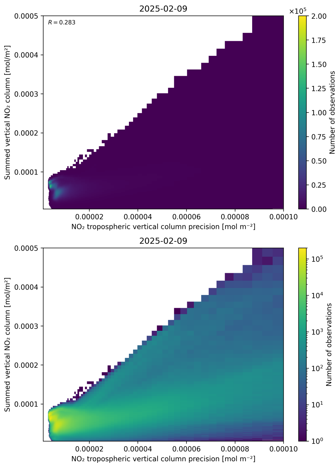
Figure 136: Scatter density plot of “NO 2 tropospheric vertical column precision” against “Summed vertical NO 2 column” for 2025-02-08 to 2025-02-10.
