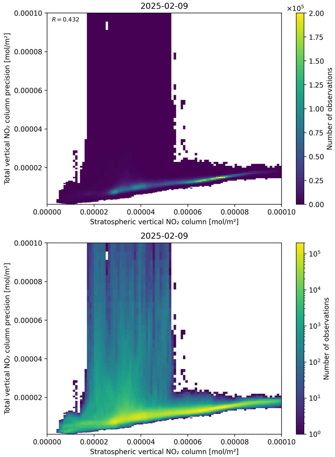
Figure 101: Scatter density plot of “Stratospheric vertical NO 2 column” against “Total vertical NO 2 column precision” for 2025-02-08 to 2025-02-10.
