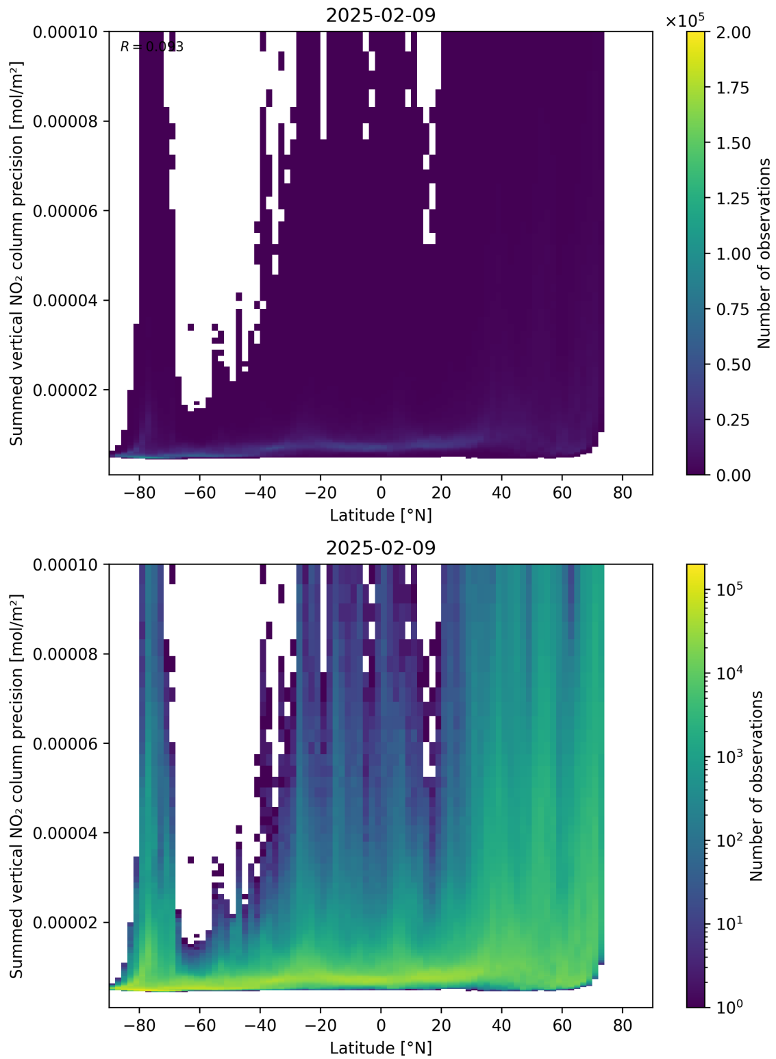
Figure 89: Scatter density plot of “Latitude” against “Summed vertical NO 2 column precision” for 2025-02-08 to 2025-02-10.
