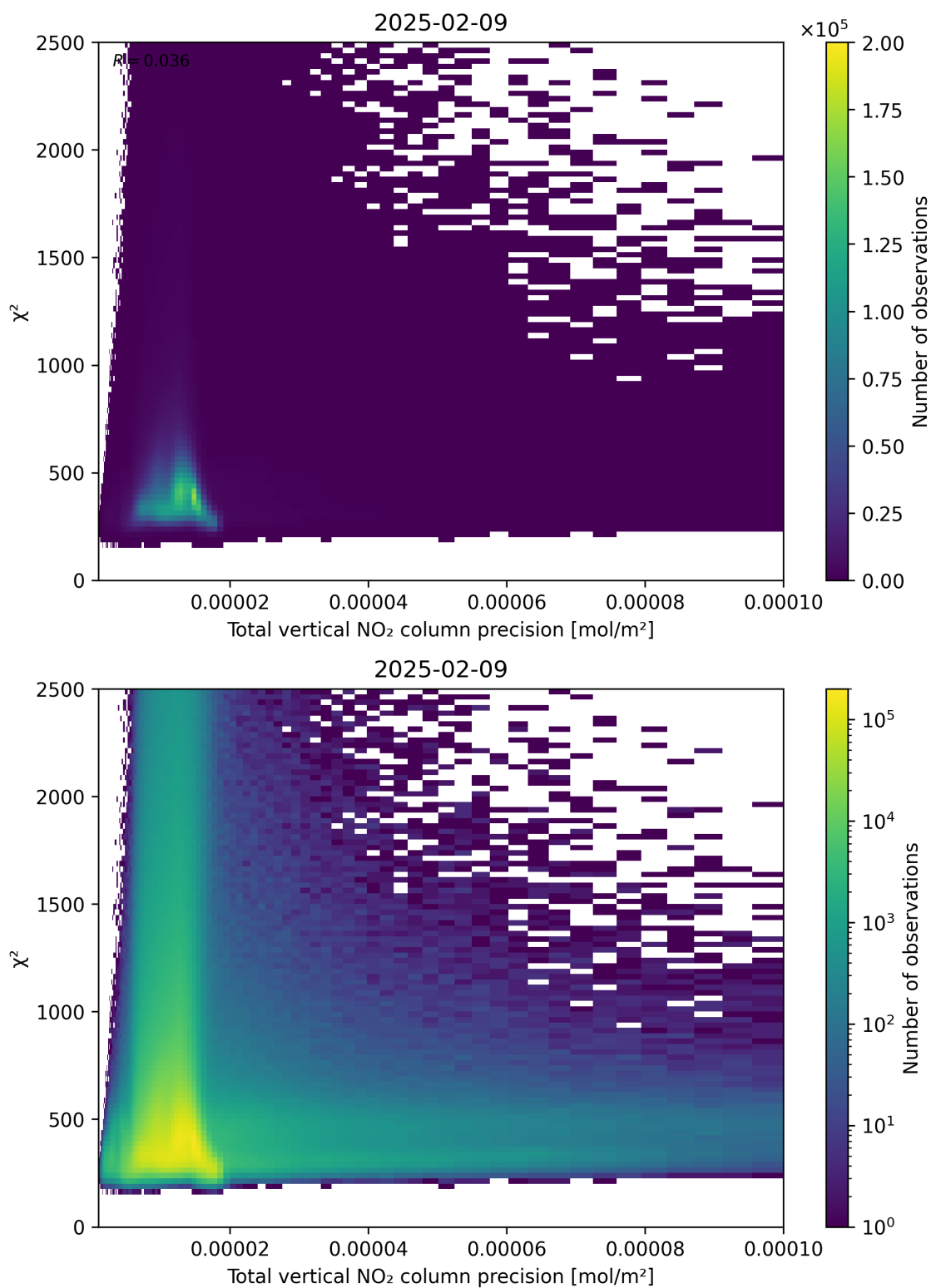
Figure 116: Scatter density plot of “Total vertical NO 2 column precision” against “ \chi^2 ” for 2025-02-08 to 2025-02-10.
