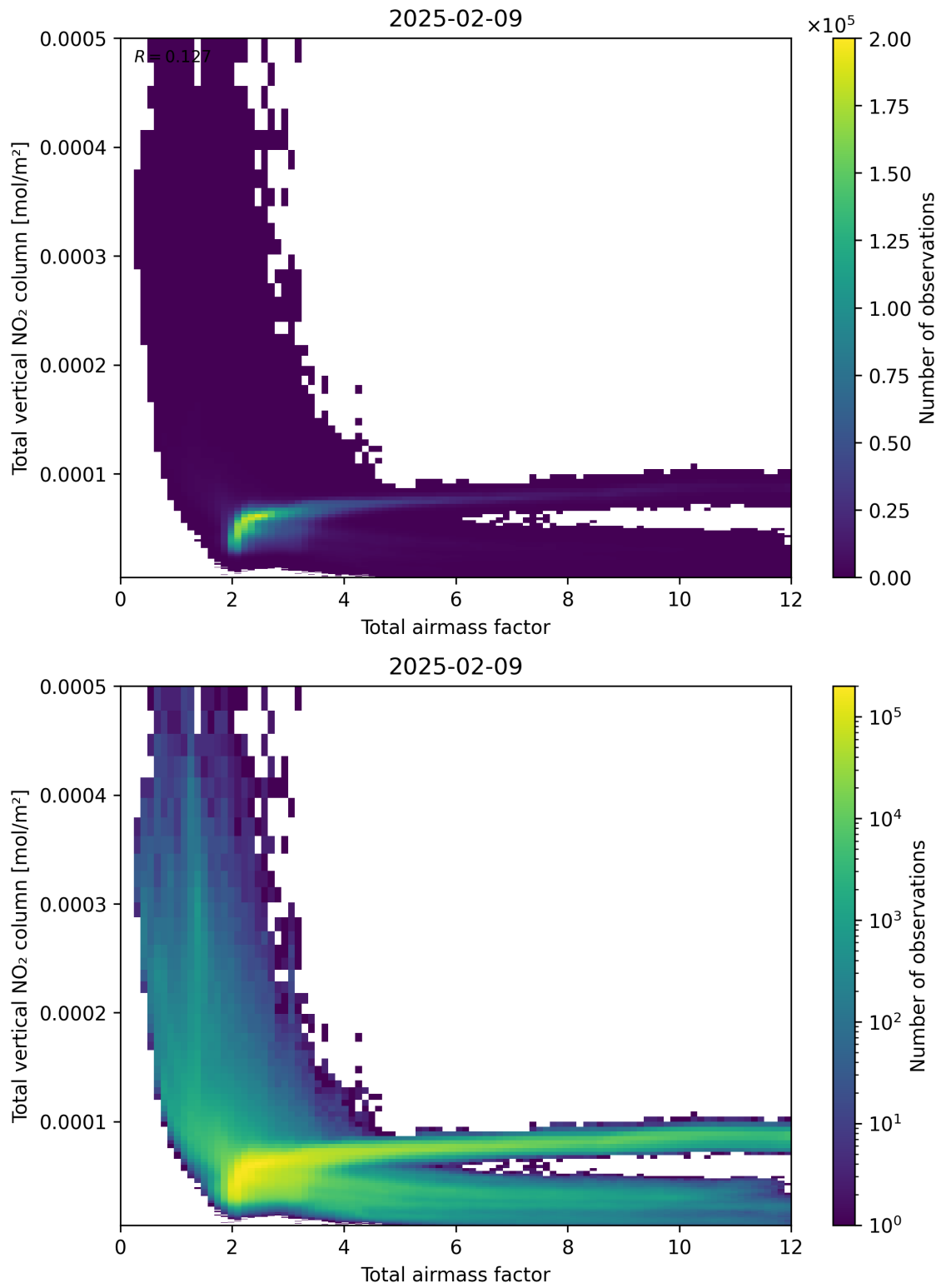
Figure 67: Scatter density plot of “Total airmass factor” against “Total vertical NO 2 column” for 2025-02-08 to 2025-02-10.
