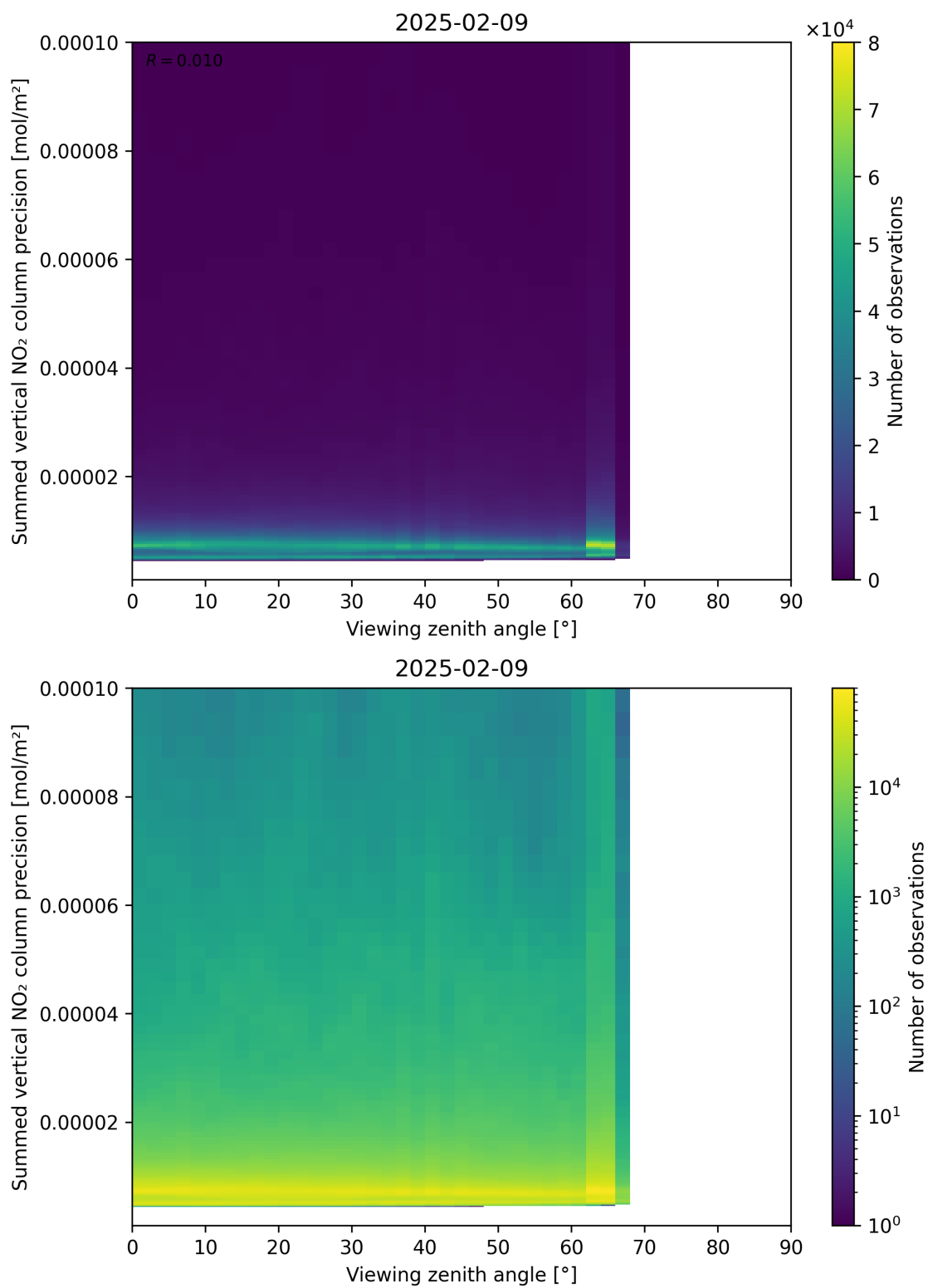
Figure 166: Scatter density plot of “Viewing zenith angle” against “Summed vertical NO 2 column precision” for 2025-02-08 to 2025-02-10.
