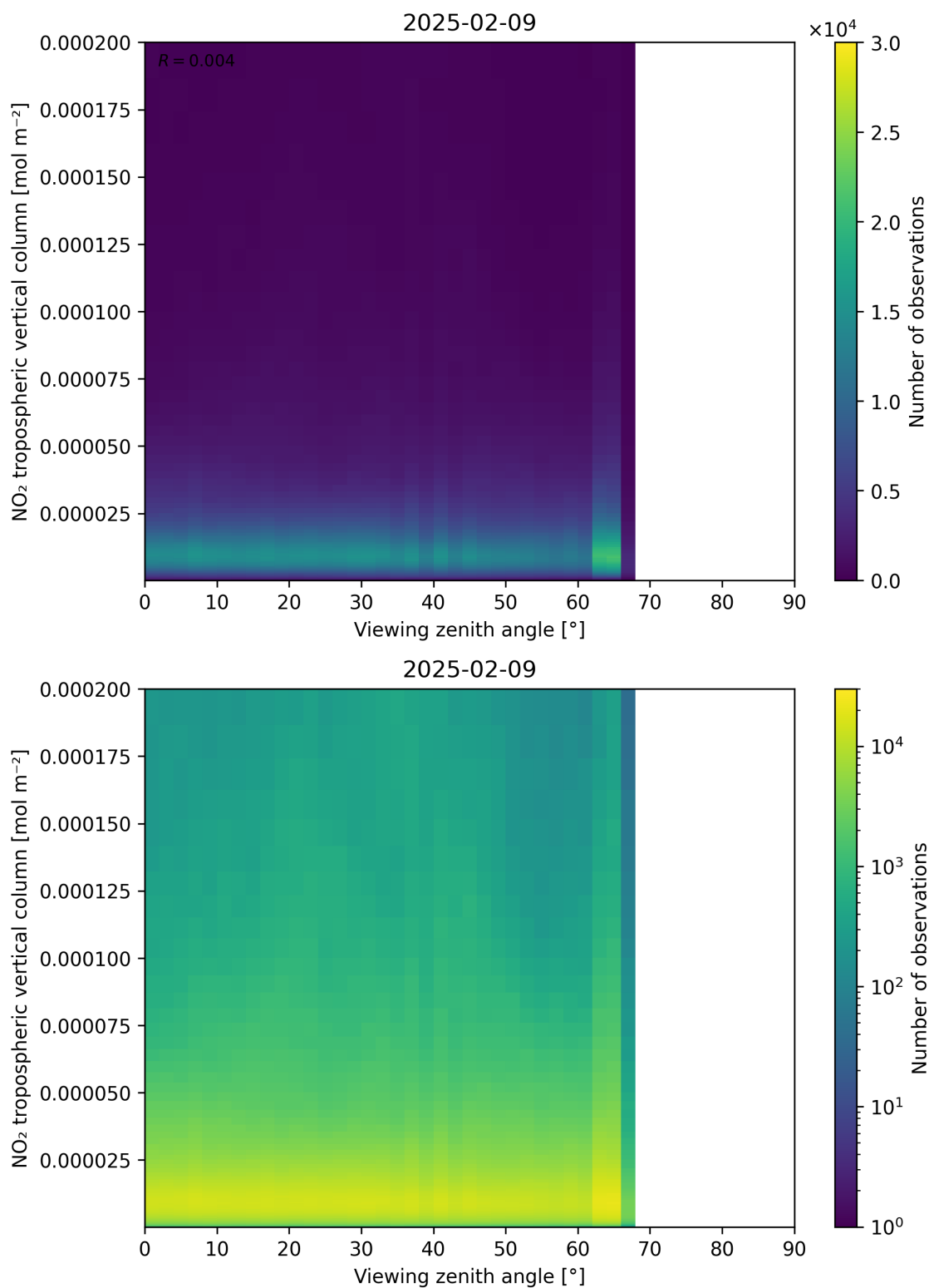
Figure 169: Scatter density plot of “Viewing zenith angle” against “NO 2 tropospheric vertical column” for 2025-02-08 to 2025-02-10.
