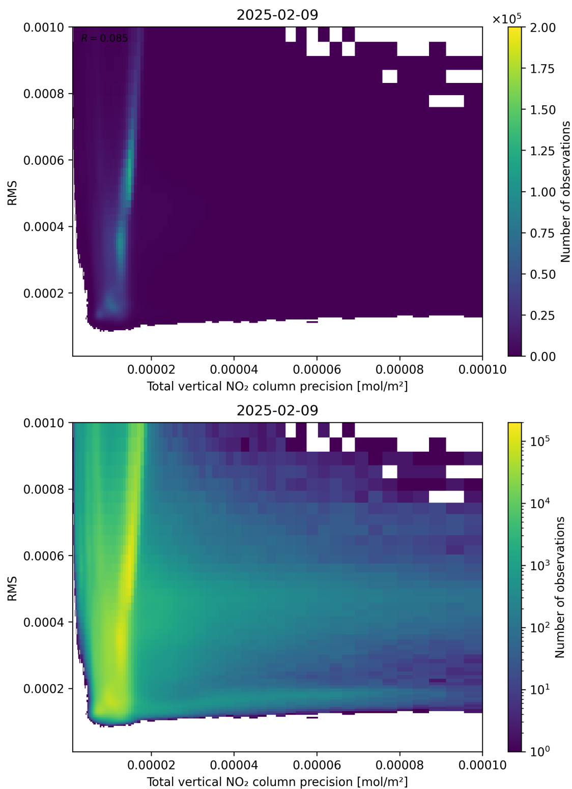
Figure 119: Scatter density plot of “Total vertical NO 2 column precision” against “RMS” for 2025-02-08 to 2025-02-10.
