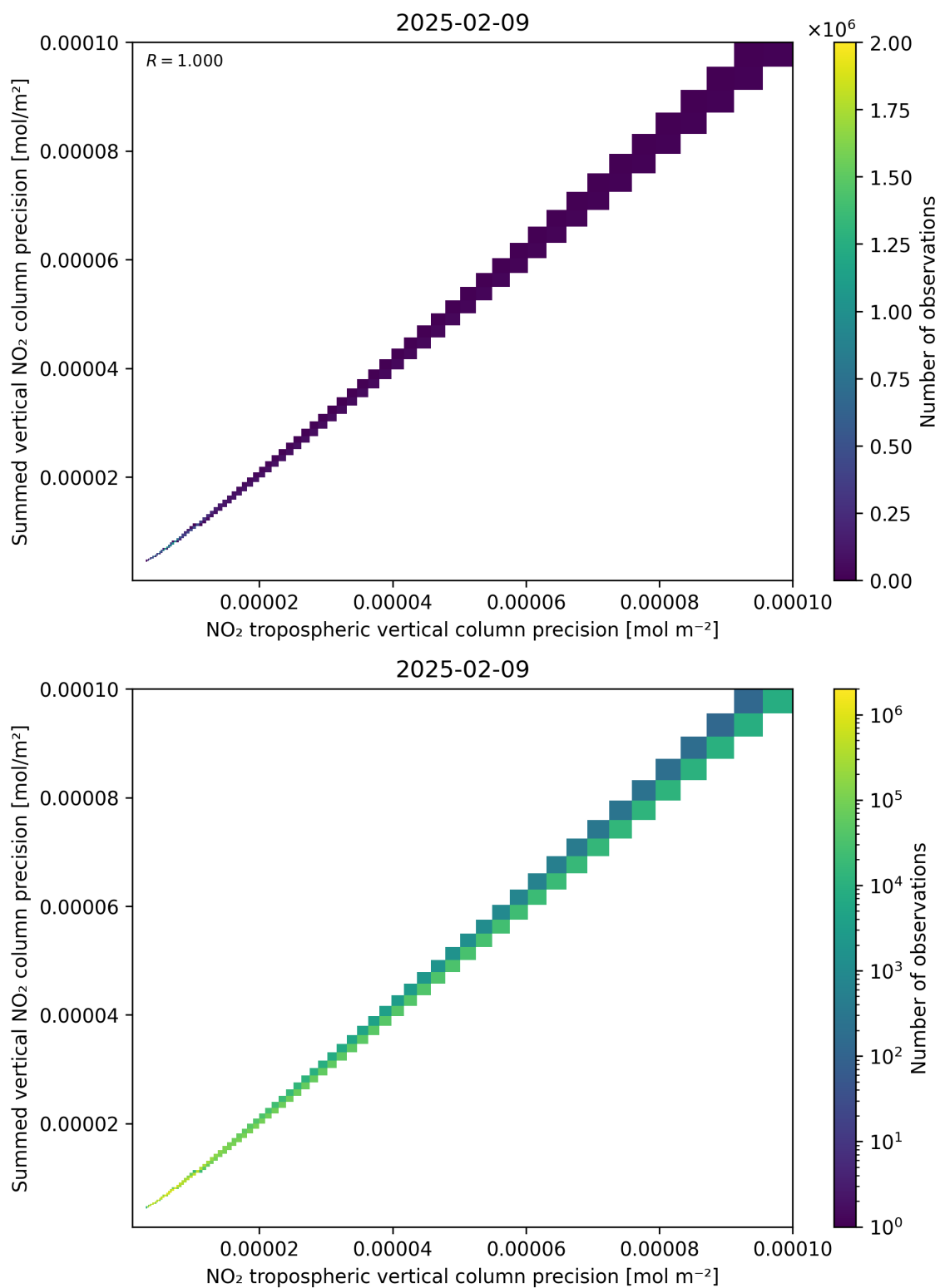
Figure 137: Scatter density plot of “NO 2 tropospheric vertical column precision” against “Summed vertical NO 2 column precision” for 2025-02-08 to 2025-02-10.
