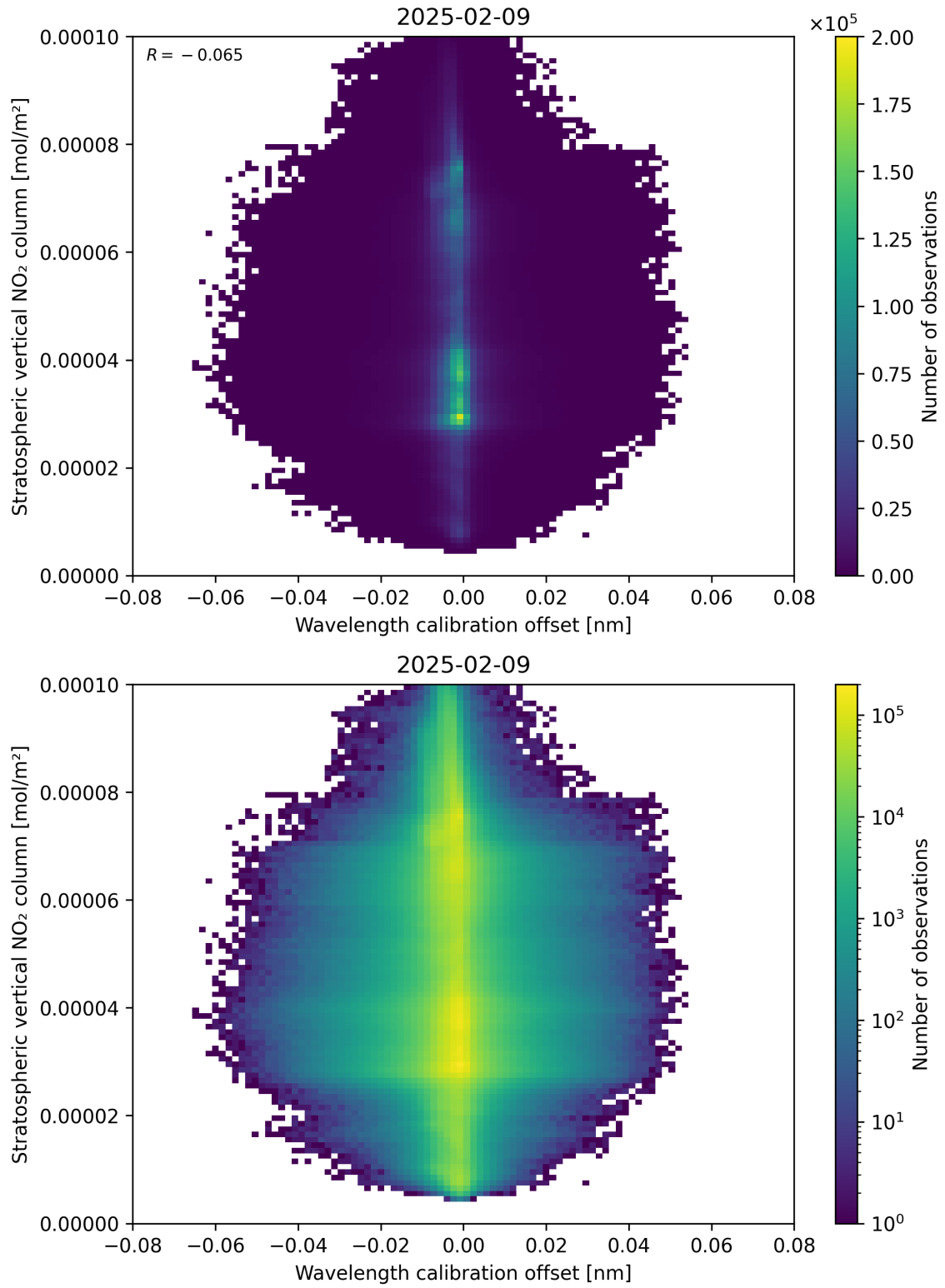
Figure 176: Scatter density plot of “Wavelength calibration offset” against “Stratospheric vertical NO 2 column” for 2025-02-08 to 2025-02-10.
