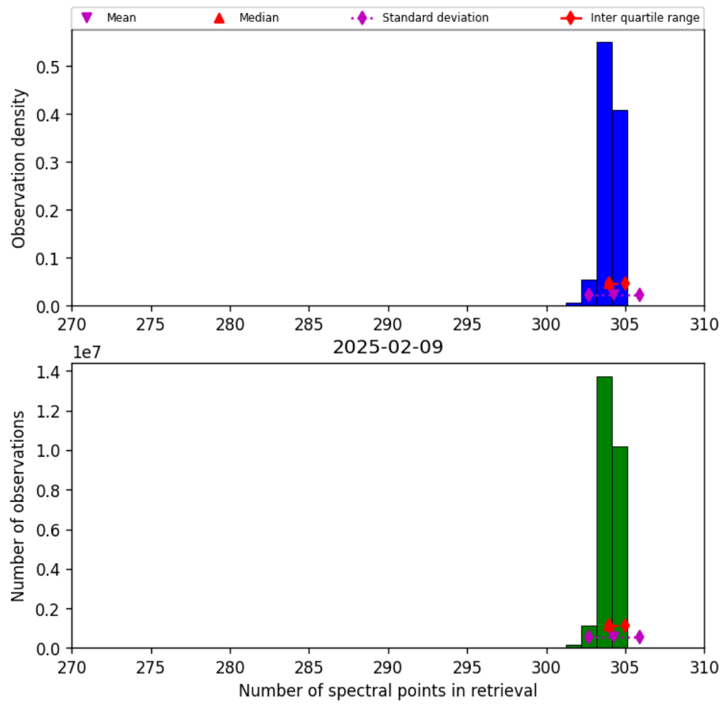
Figure 33: Histogram of “Number of spectral points in retrieval” for 2025-02-08 to 2025-02-10
