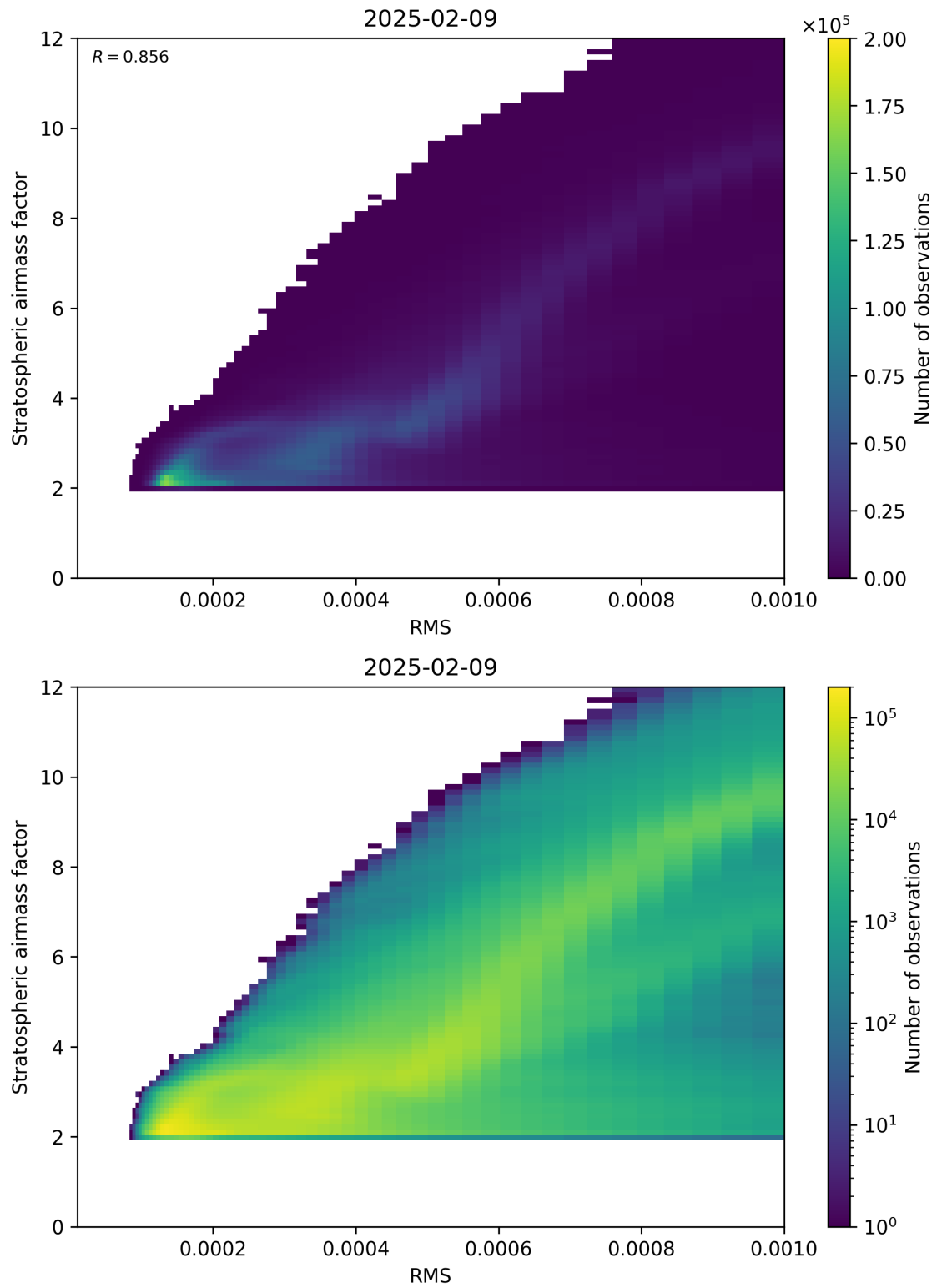
Figure 144: Scatter density plot of “RMS” against “Stratospheric airmass factor” for 2025-02-08 to 2025-02-10.
