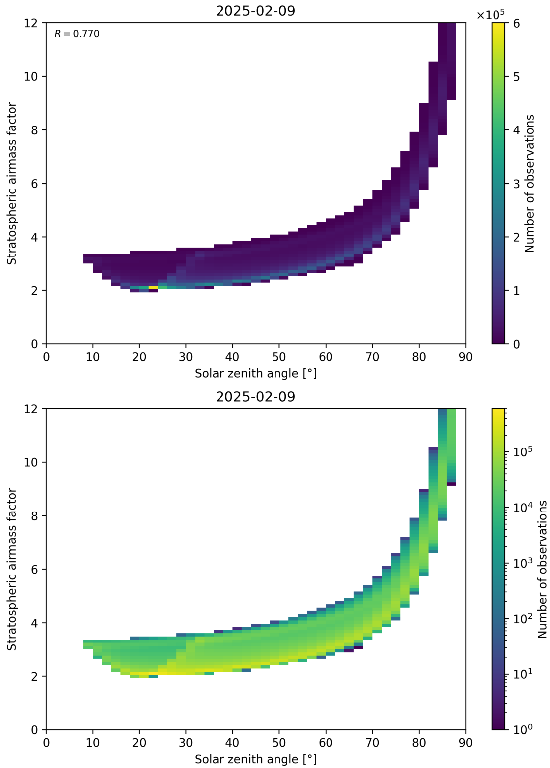
Figure 145: Scatter density plot of “Solar zenith angle” against “Stratospheric airmass factor” for 2025-02-08 to 2025-02-10.
