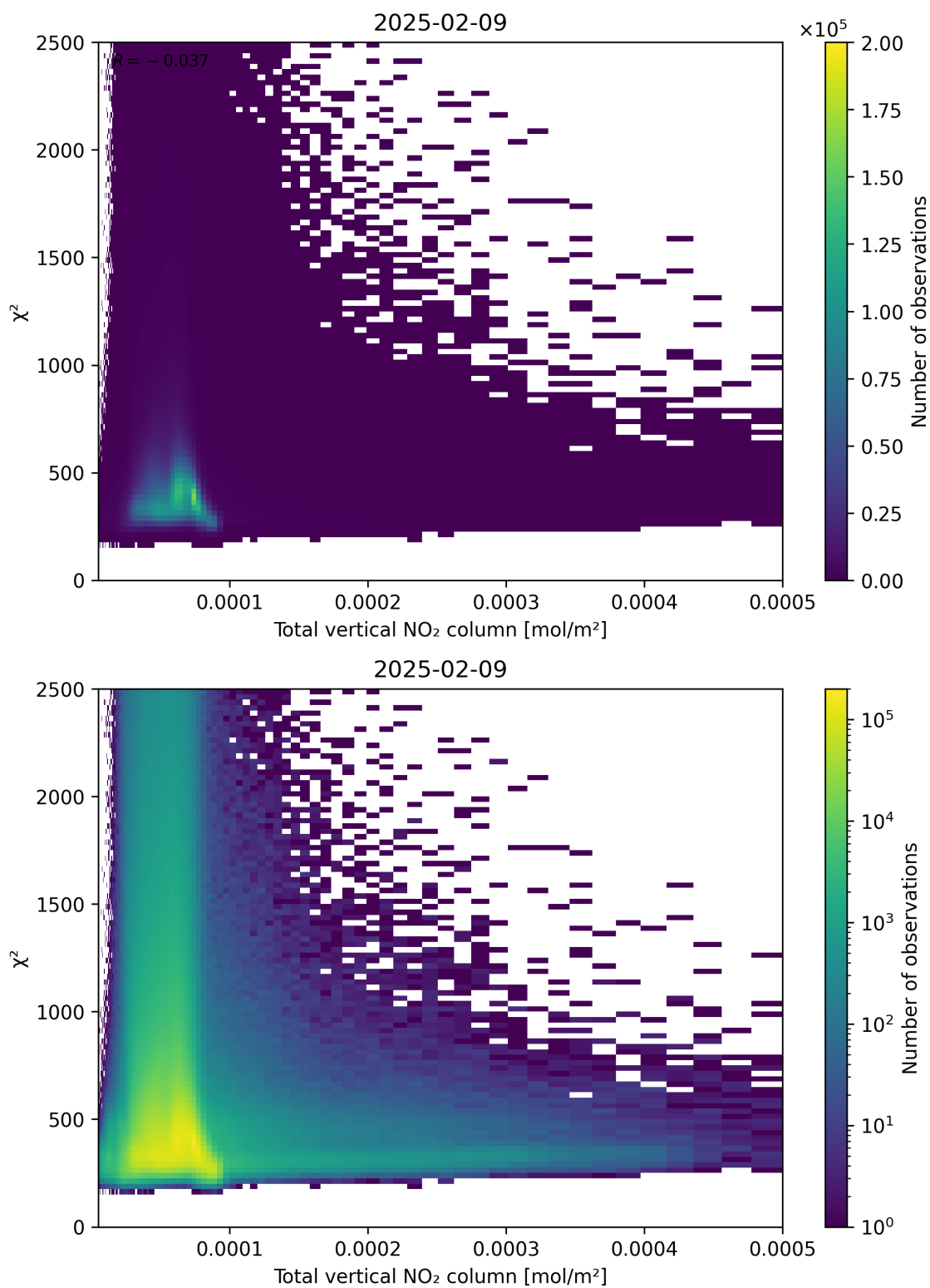
Figure 111: Scatter density plot of “Total vertical NO 2 column” against “ \chi^2 ” for 2025-02-08 to 2025-02-10.
