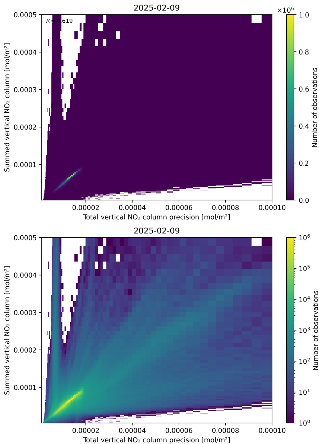
Figure 117: Scatter density plot of “Total vertical NO 2 column precision” against “Summed vertical NO 2 column” for 2025-02-08 to 2025-02-10.
