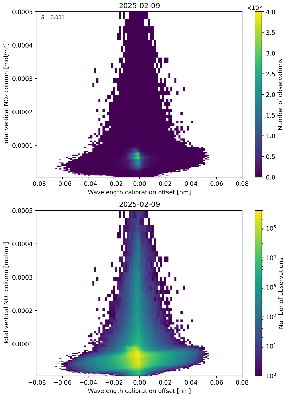
Figure 179: Scatter density plot of “Wavelength calibration offset” against “Total vertical NO 2 column” for 2025-02-08 to 2025-02-10.
