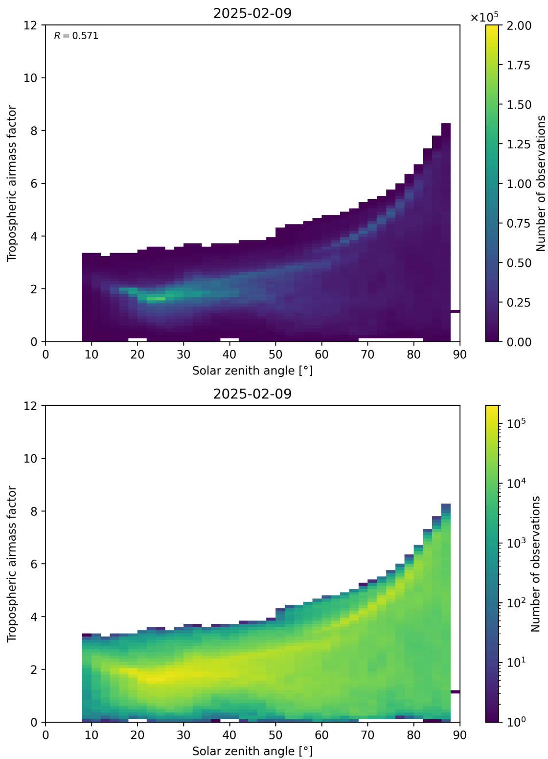
Figure 147: Scatter density plot of “Solar zenith angle” against “Tropospheric airmass factor” for 2025-02-08 to 2025-02-10.
