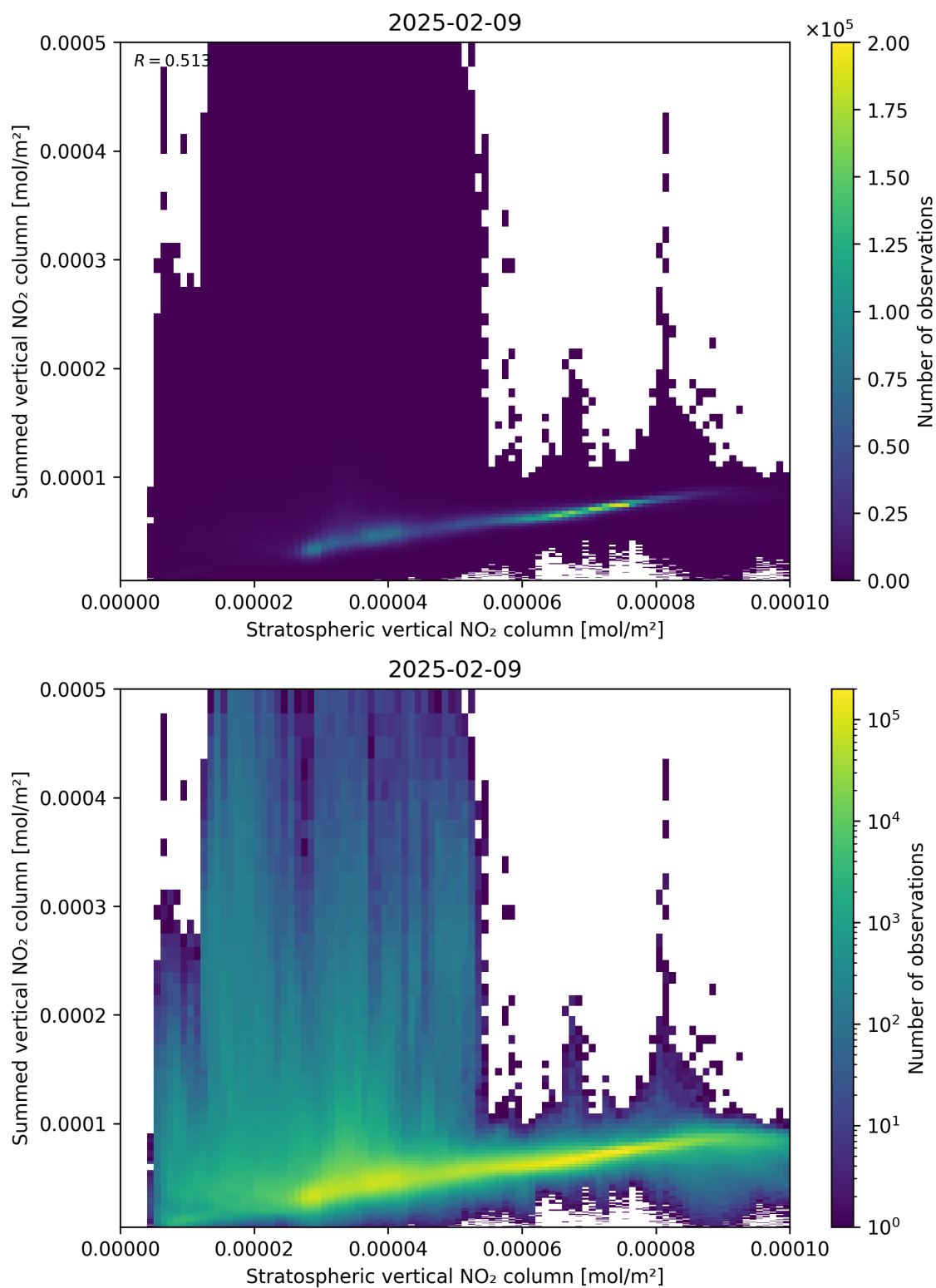
Figure 98: Scatter density plot of “Stratospheric vertical NO 2 column” against “Summed vertical NO 2 column” for 2025-02-08 to 2025-02-10.
