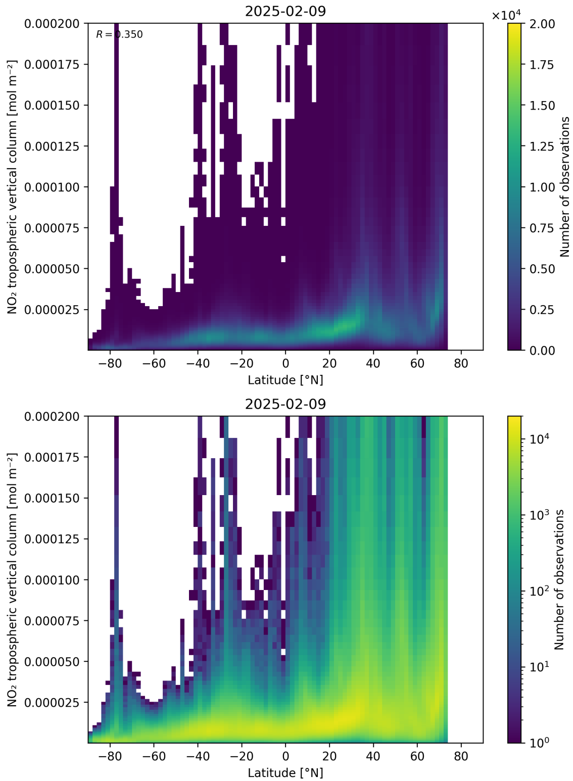
Figure 92: Scatter density plot of “Latitude” against “NO 2 tropospheric vertical column” for 2025-02-08 to 2025-02-10.
