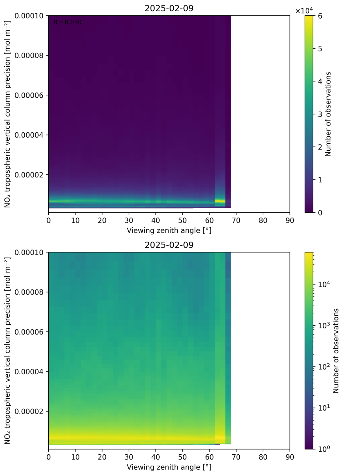
Figure 170: Scatter density plot of “Viewing zenith angle” against “NO 2 tropospheric vertical column precision” for 2025-02-08 to 2025-02-10.
