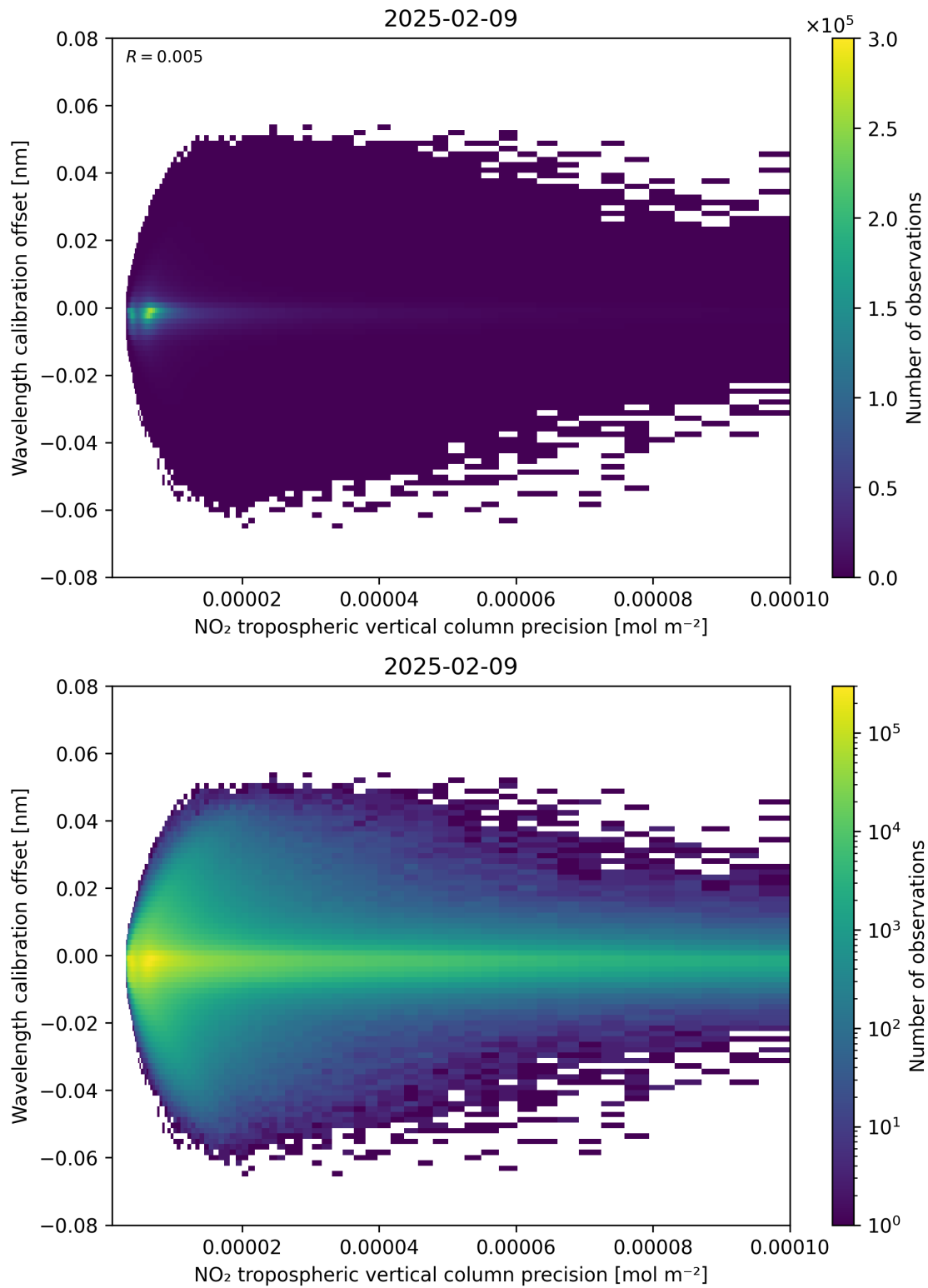
Figure 141: Scatter density plot of “NO 2 tropospheric vertical column precision” against “Wavelength calibration offset” for 2025-02-08 to 2025-02-10.
