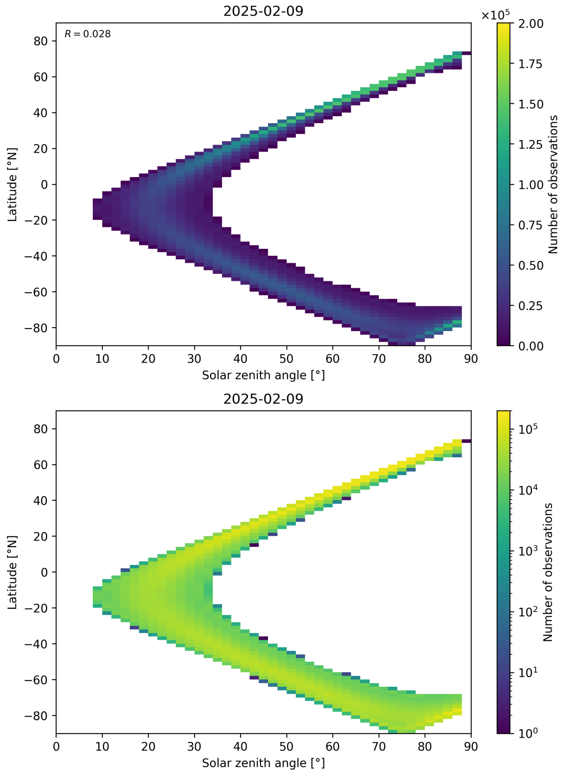
Figure 149: Scatter density plot of “Solar zenith angle” against “Latitude” for 2025-02-08 to 2025-02-10.
