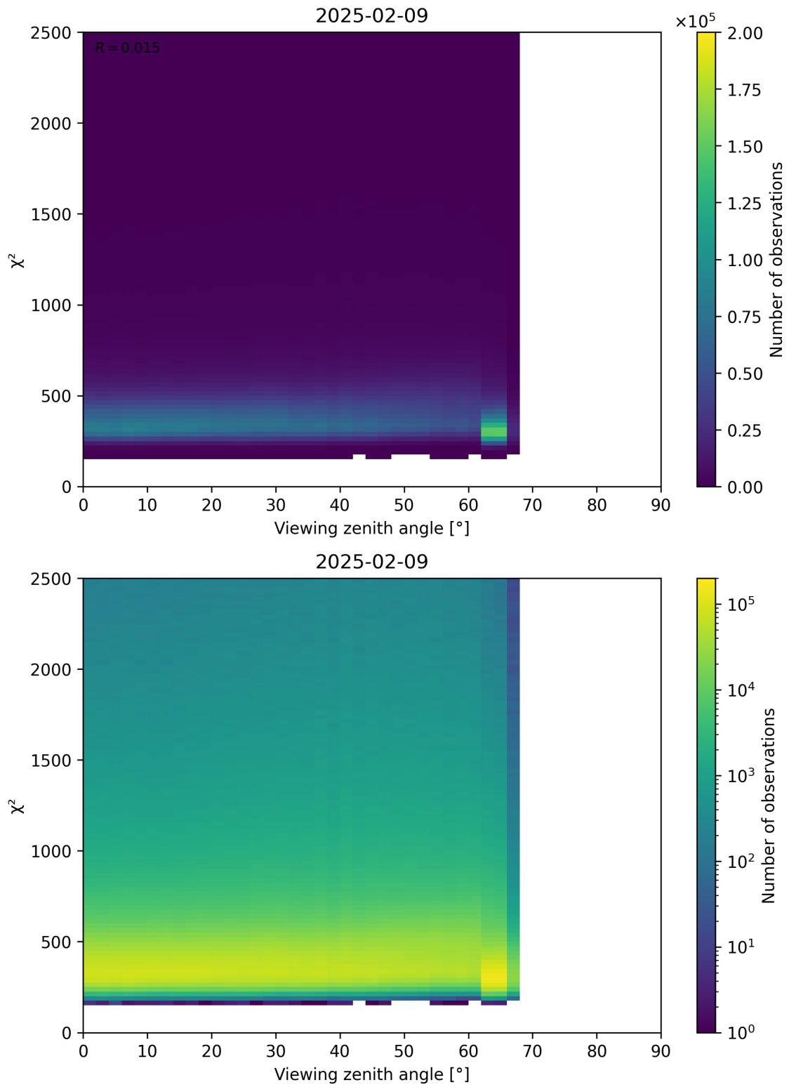
Figure 162: Scatter density plot of “Viewing zenith angle” against “ \chi^2 ” for 2025-02-08 to 2025-02-10.
