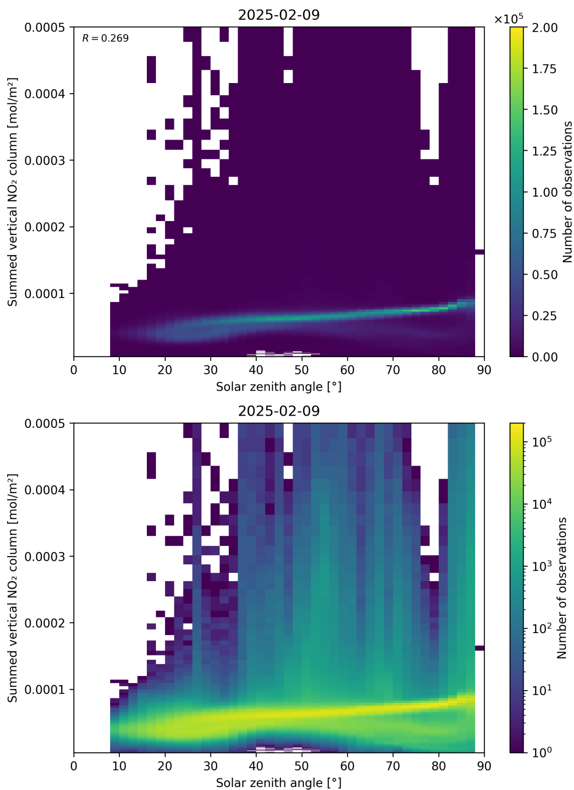
Figure 151: Scatter density plot of “Solar zenith angle” against “Summed vertical NO 2 column” for 2025-02-08 to 2025-02-10.
