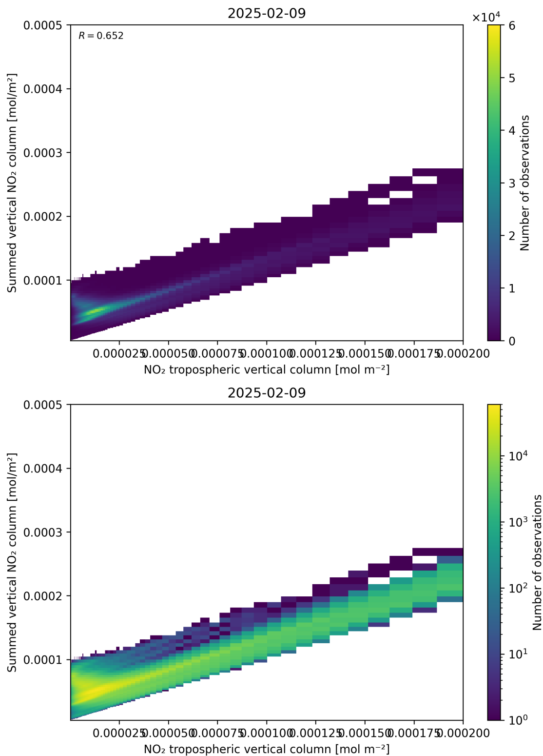
Figure 126: Scatter density plot of “NO 2 tropospheric vertical column” against “Summed vertical NO 2 column” for 2025-02-08 to 2025-02-10.
