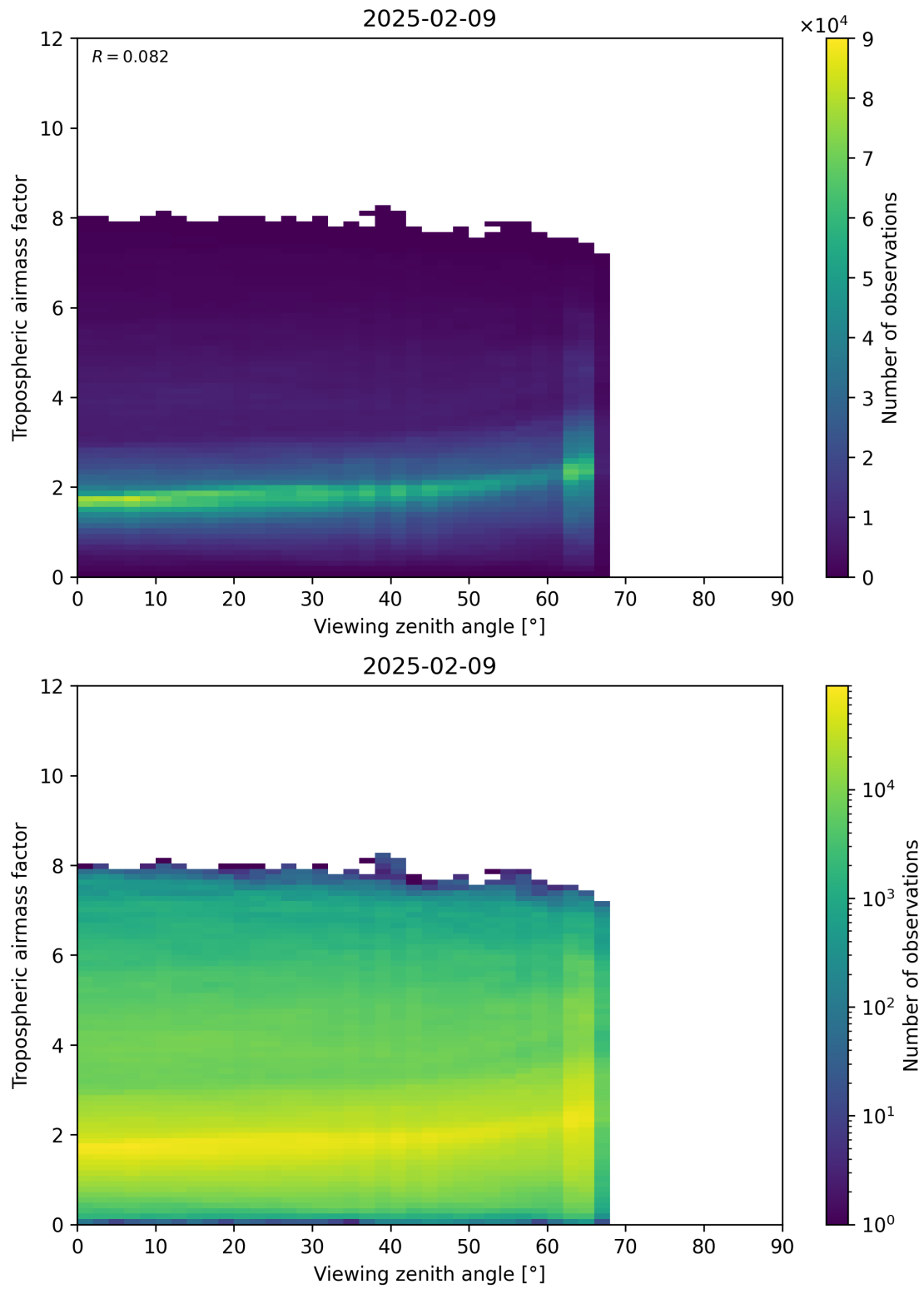
Figure 161: Scatter density plot of “Viewing zenith angle” against “Tropospheric airmass factor” for 2025-02-08 to 2025-02-10.
