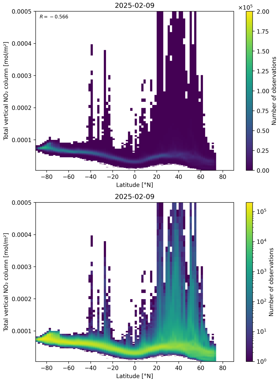
Figure 90: Scatter density plot of “Latitude” against “Total vertical NO 2 column” for 2025-02-08 to 2025-02-10.
