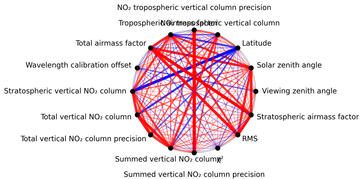
Figure 1: Map of correlation graph for 2025-02-08 to 2025-02-10.
