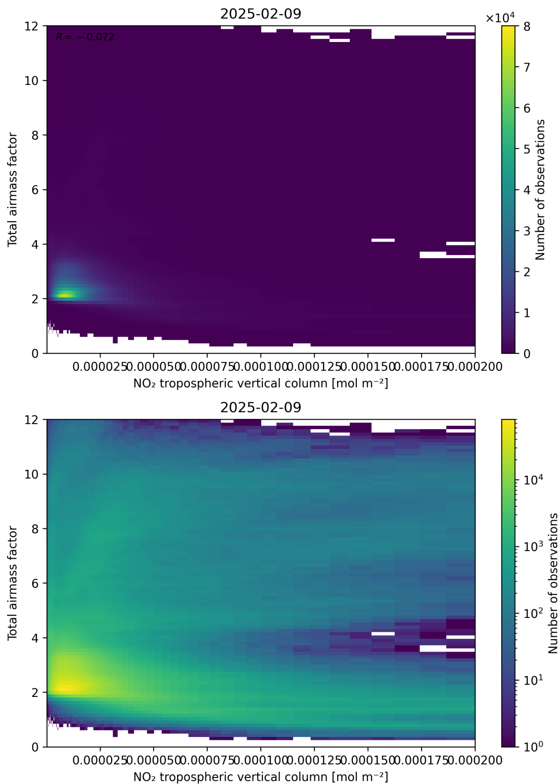
Figure 122: Scatter density plot of “NO 2 tropospheric vertical column” against “Total air mass factor” for 2025-02-08 to 2025-02-10.
