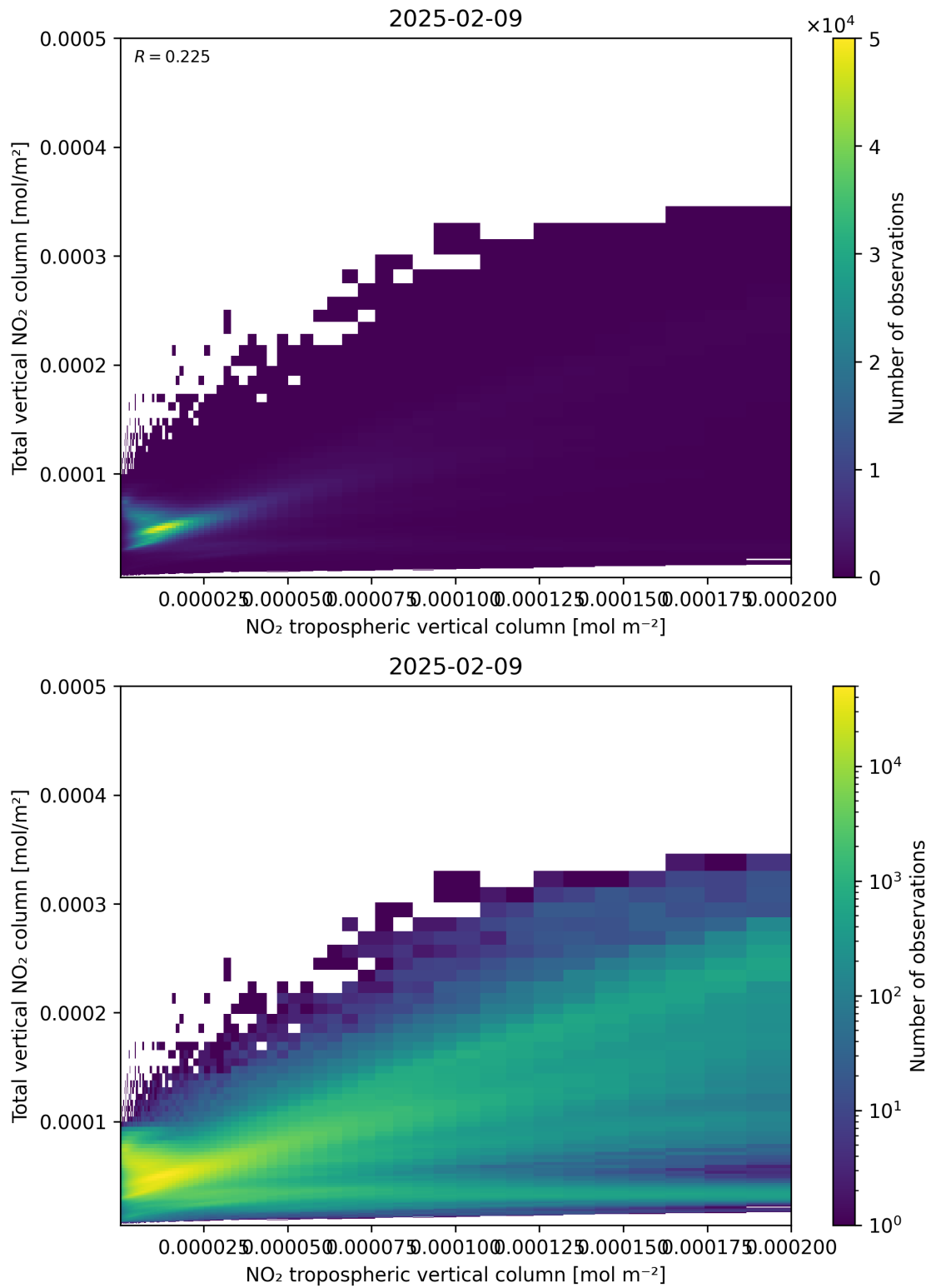
Figure 128: Scatter density plot of “NO 2 tropospheric vertical column” against “Total vertical NO 2 column” for 2025-02-08 to 2025-02-10.
