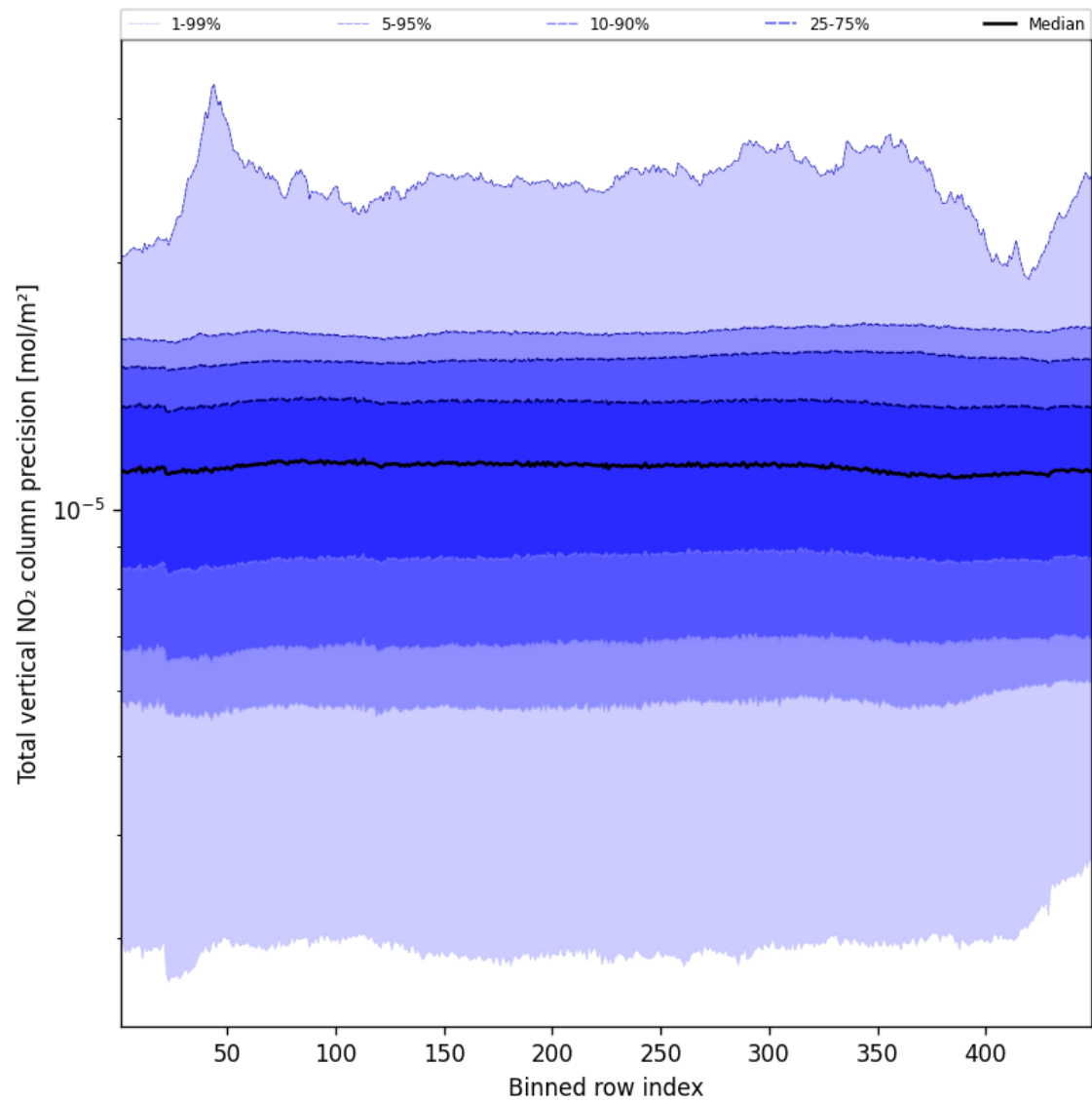
Figure 56: Along track statistics of “Total vertical NO 2 column precision” for 2025-02-08 to 2025-02-10
