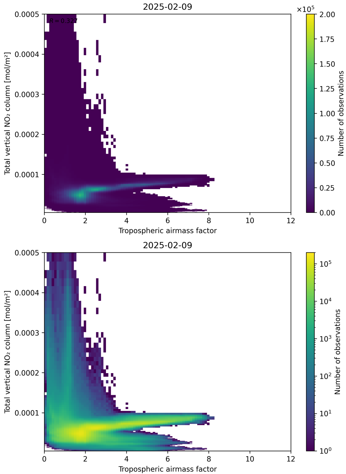
Figure 77: Scatter density plot of “Tropospheric airmass factor” against “Total vertical NO 2 column” for 2025-02-08 to 2025-02-10.
