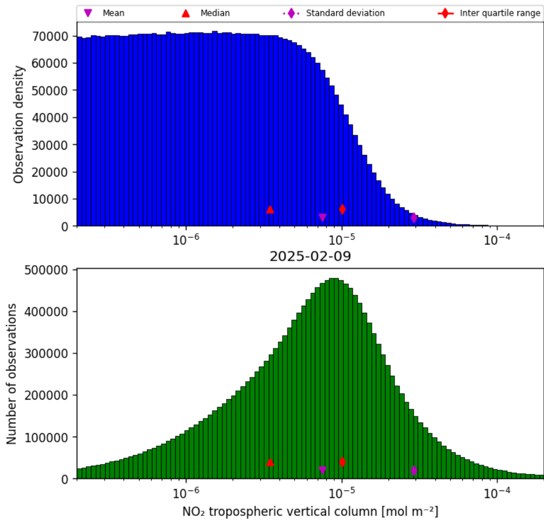
Figure 29: Histogram of “NO 2 tropospheric vertical column” for 2025-02-08 to 2025-02-10
