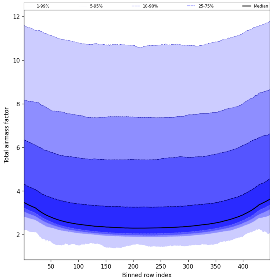
Figure 49: Along track statistics of “Total airmass factor” for 2025-02-08 to 2025-02-10
