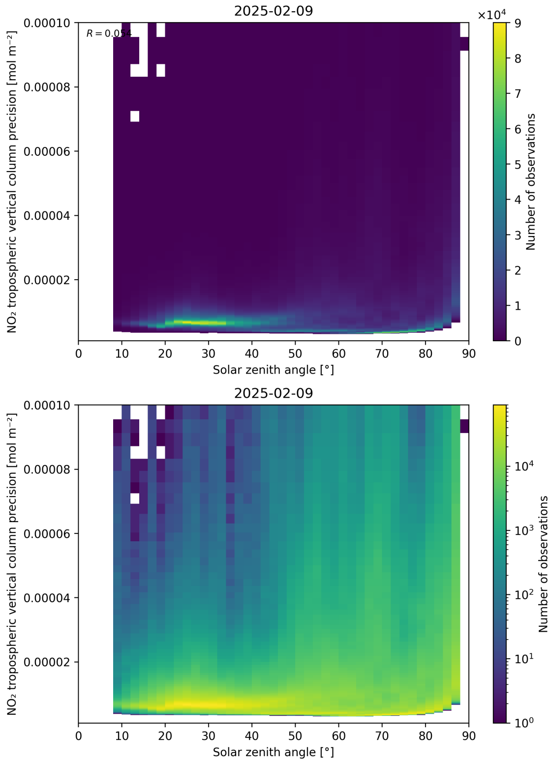
Figure 156: Scatter density plot of “Solar zenith angle” against “NO 2 tropospheric vertical column precision” for 2025-02-08 to 2025-02-10.
