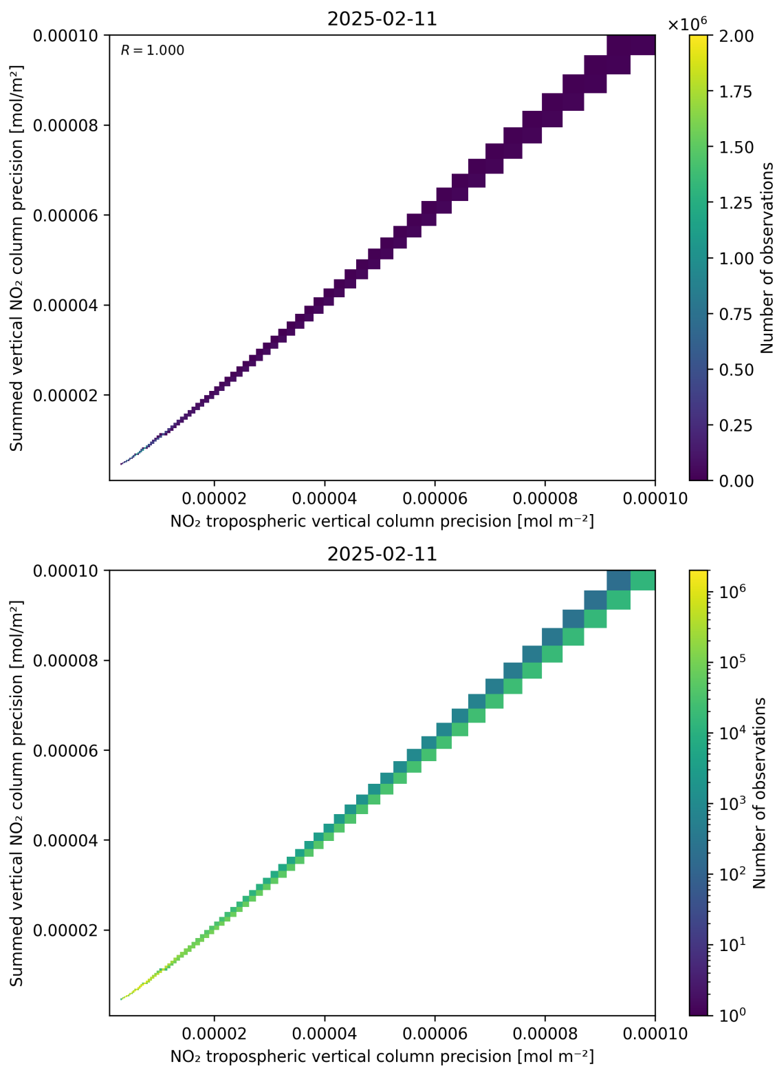
Figure 137: Scatter density plot of “NO 2 tropospheric vertical column precision” against “Summed vertical NO 2 column precision” for 2025-02-10 to 2025-02-12.
