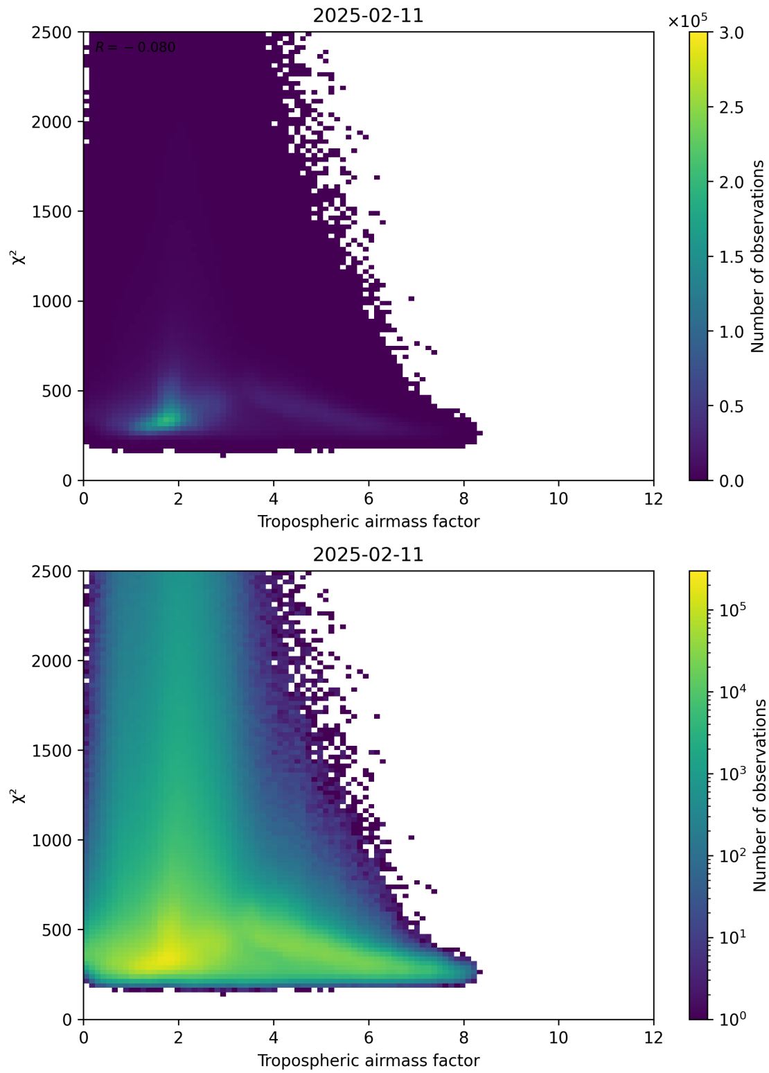
Figure 73: Scatter density plot of “Tropospheric airmass factor” against “ \chi^2 ” for 2025-02-10 to 2025-02-12.
