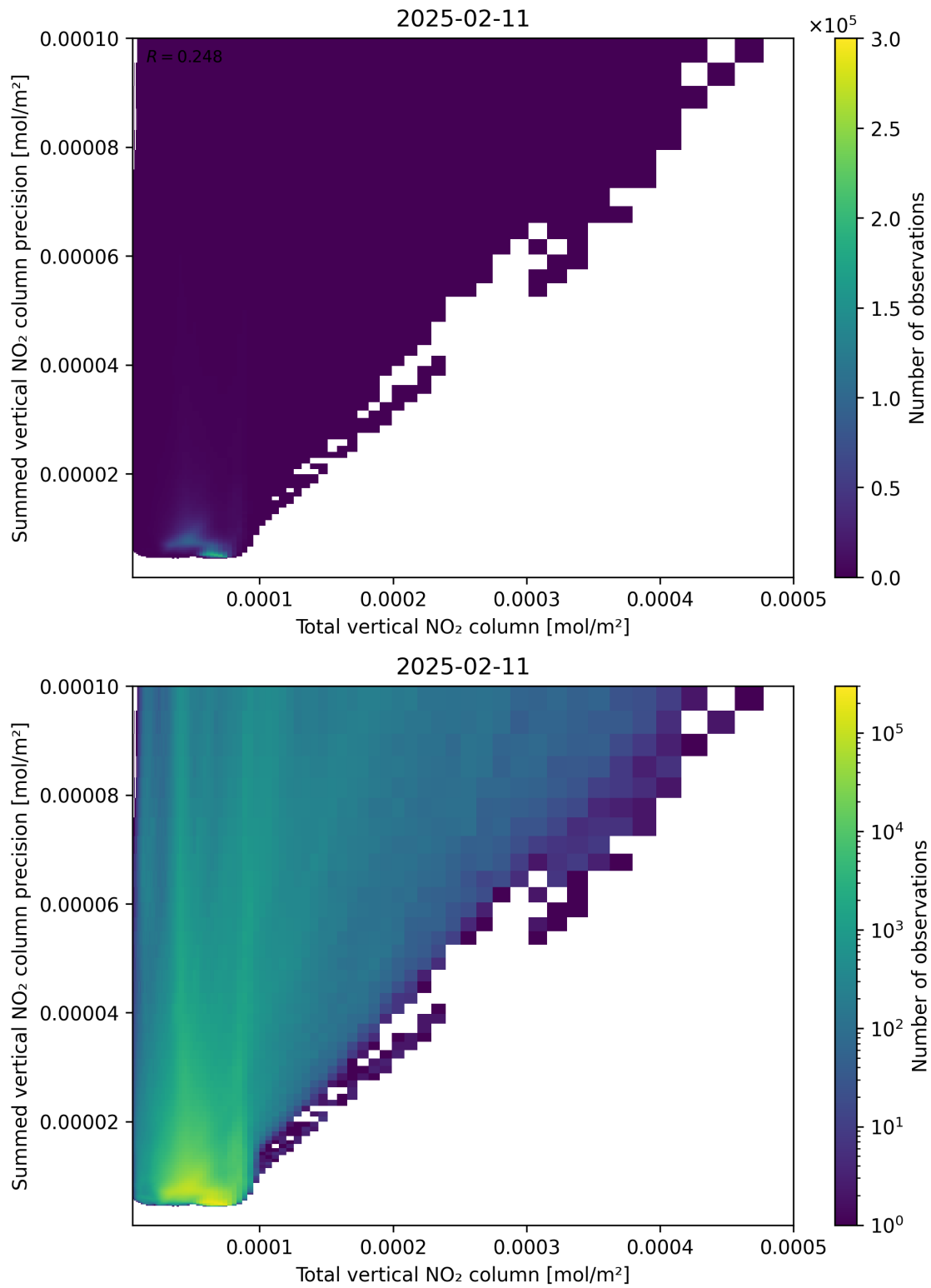
Figure 113: Scatter density plot of “Total vertical NO 2 column” against “Summed vertical NO 2 column precision” for 2025-02-10 to 2025-02-12.
