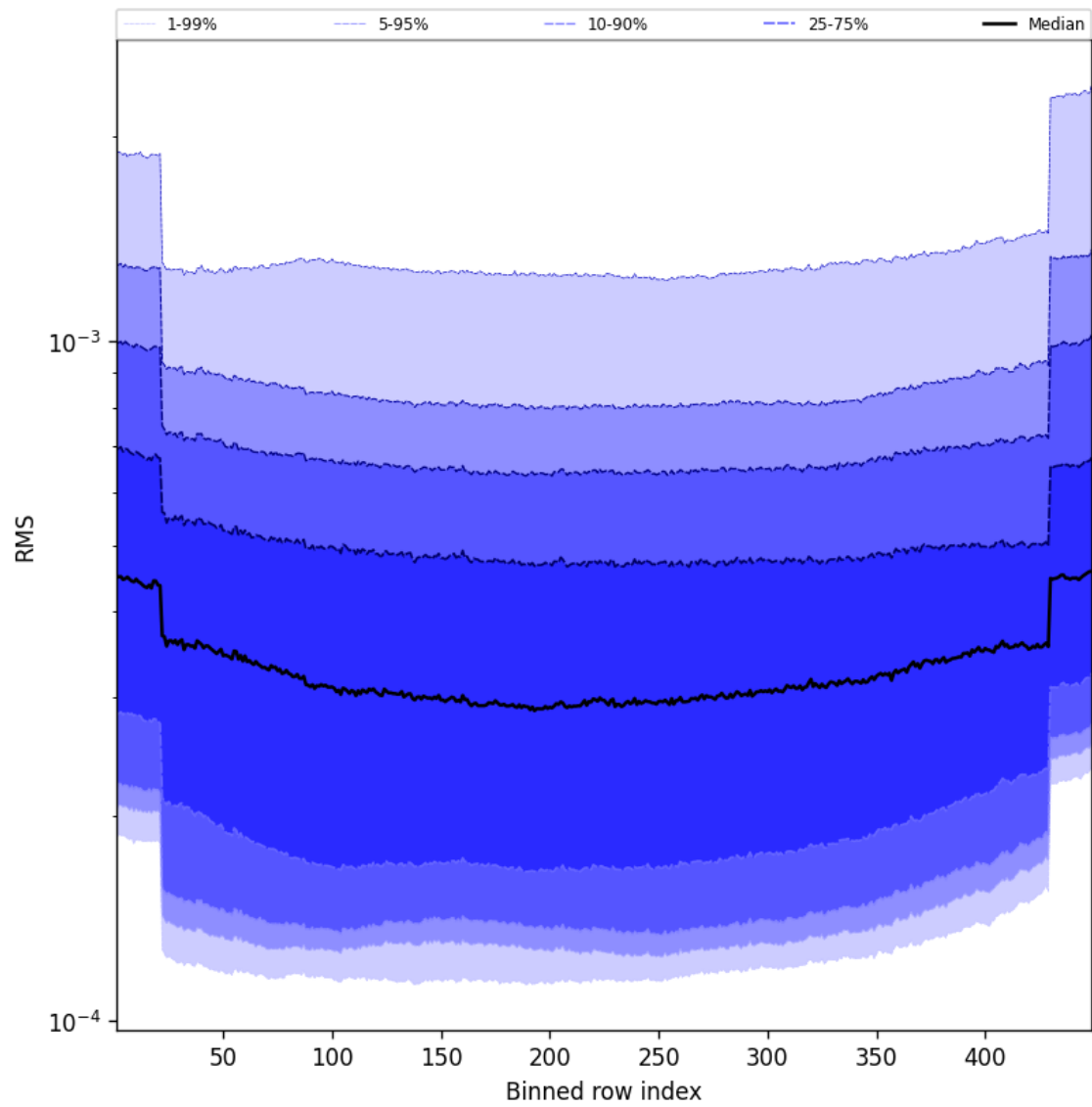
Figure 60: Along track statistics of “RMS” for 2025-02-10 to 2025-02-12
