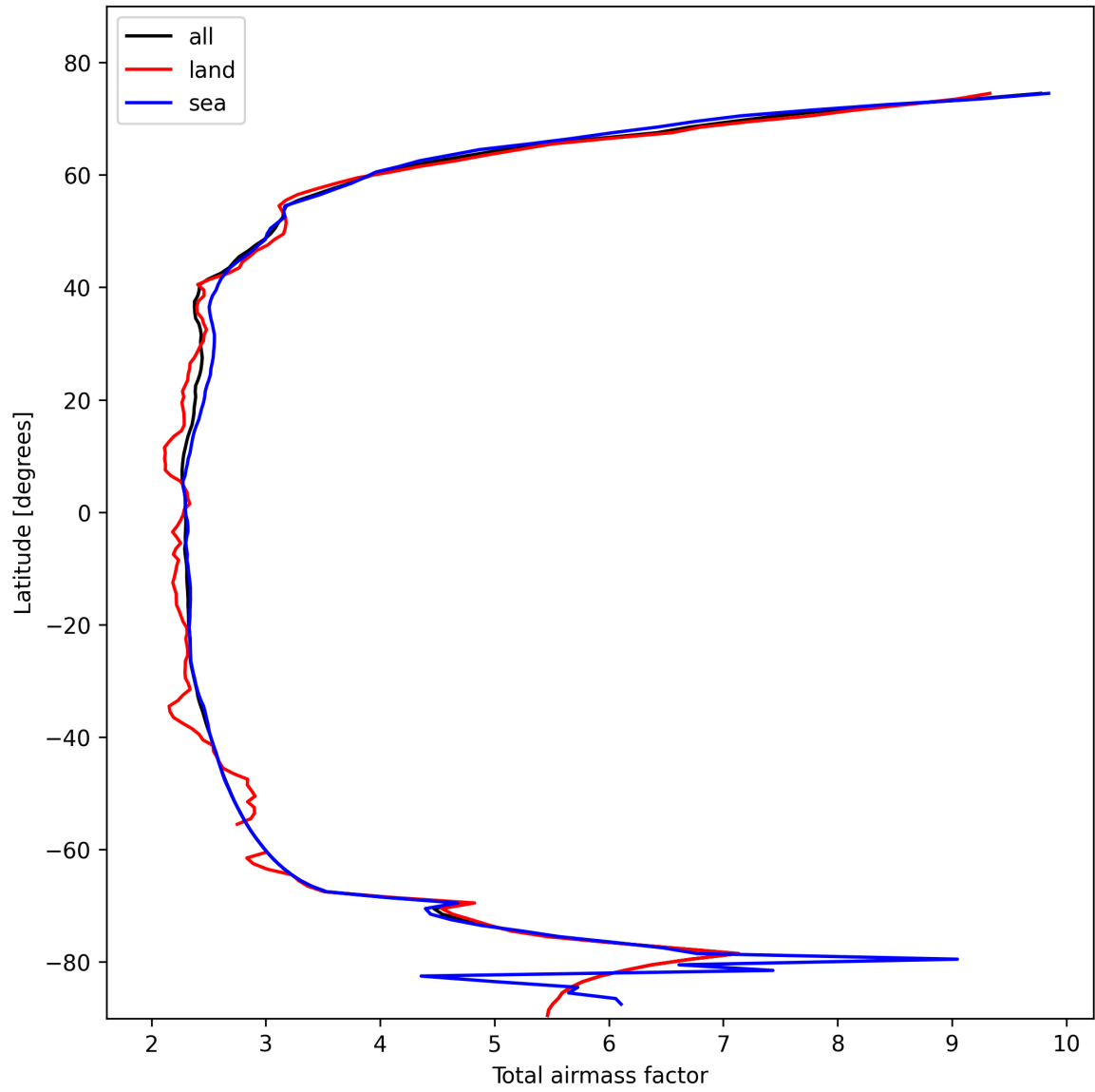
Figure 15: Zonal average of “Total airmass factor” for 2025-02-10 to 2025-02-12.
