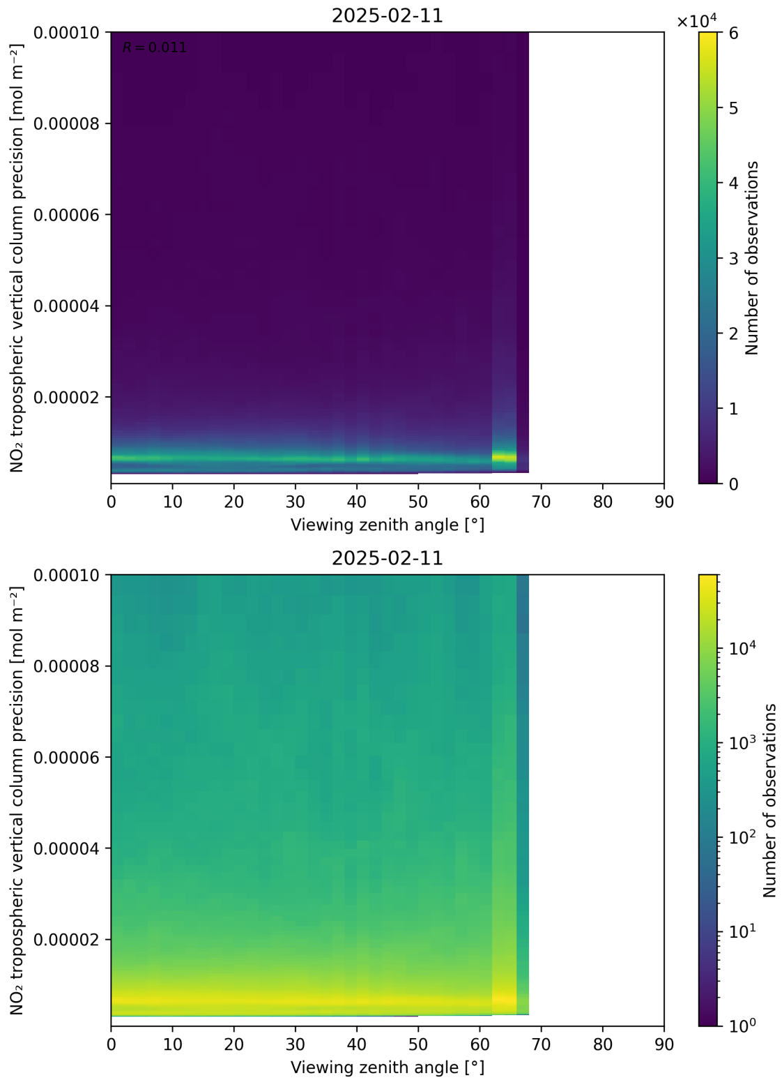
Figure 170: Scatter density plot of “Viewing zenith angle” against “NO 2 tropospheric vertical column precision” for 2025-02-10 to 2025-02-12.
