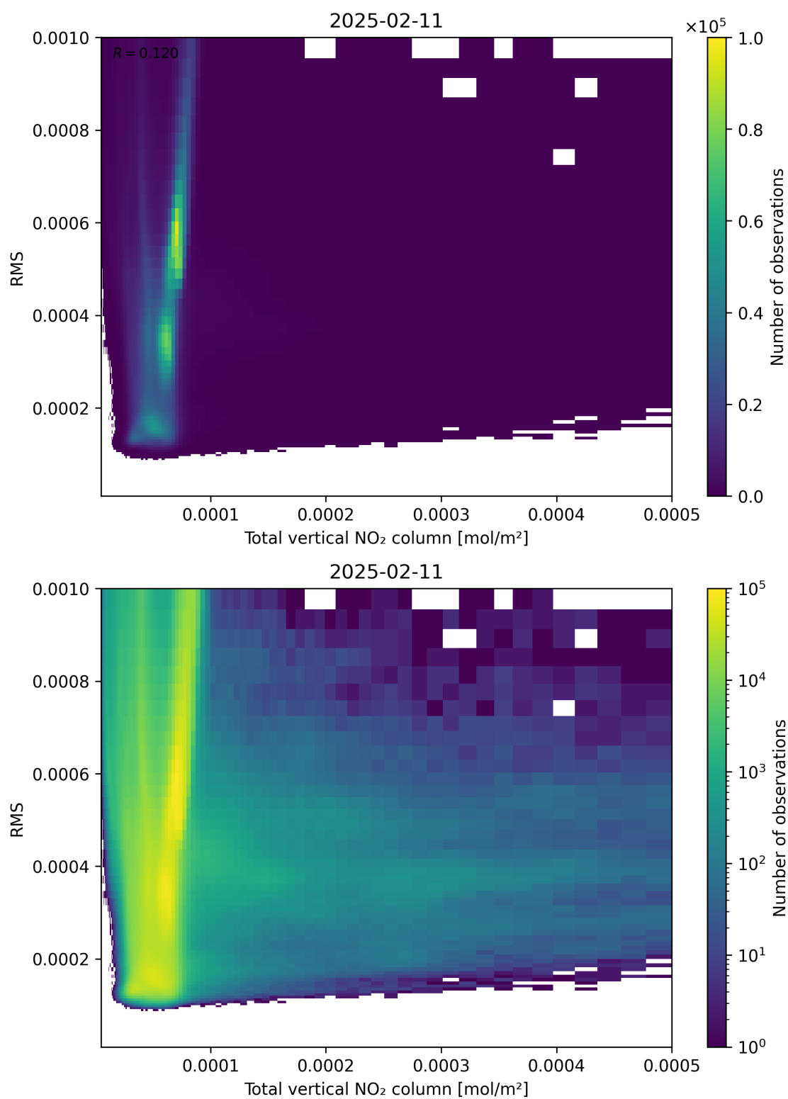
Figure 120: Scatter density plot of “Total vertical NO 2 column” against “RMS” for 2025-02-10 to 2025-02-12.
