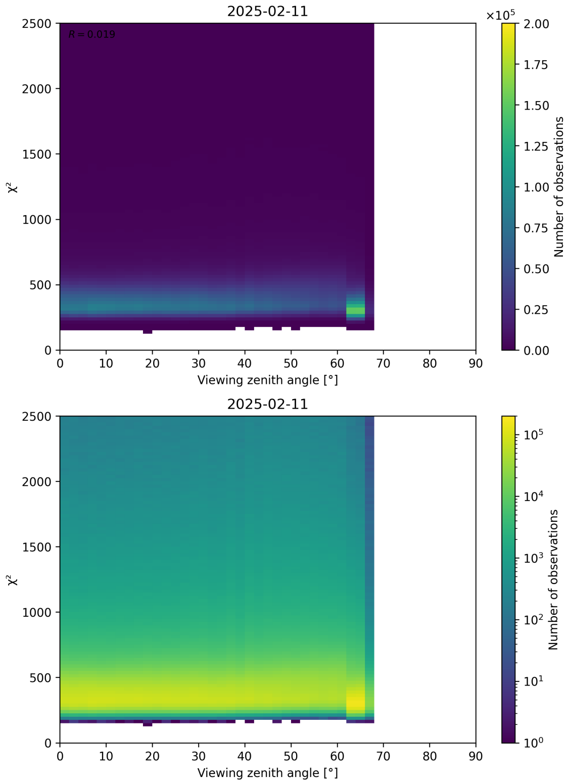
Figure 162: Scatter density plot of “Viewing zenith angle” against “ \chi^2 ” for 2025-02-10 to 2025-02-12.
