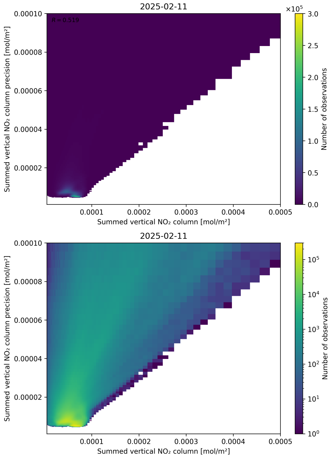
Figure 105: Scatter density plot of “Summed vertical NO 2 column” against “Summed vertical NO 2 column precision” for 2025-02-10 to 2025-02-12.
