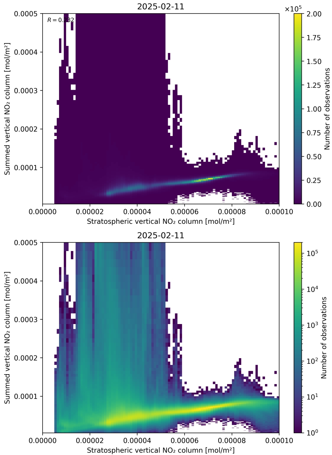
Figure 98: Scatter density plot of “Stratospheric vertical NO 2 column” against “Summed vertical NO 2 column” for 2025-02-10 to 2025-02-12.
