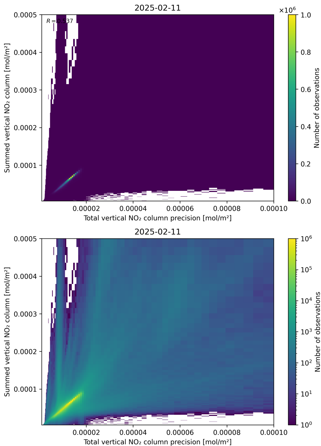
Figure 117: Scatter density plot of “Total vertical NO 2 column precision” against “Summed vertical NO 2 column” for 2025-02-10 to 2025-02-12.
