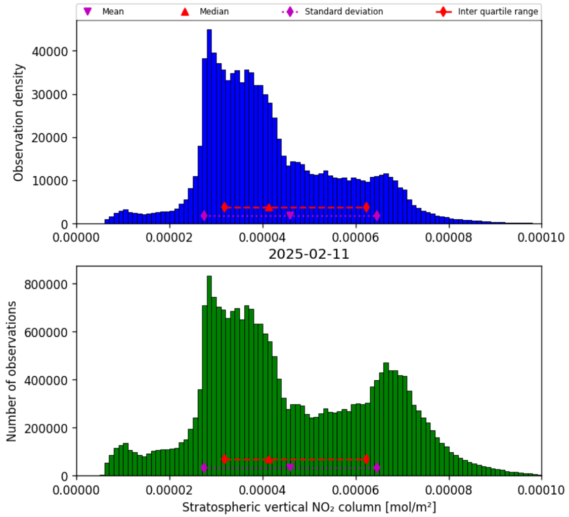
Figure 36: Histogram of “Stratospheric vertical NO 2 column” for 2025-02-10 to 2025-02-12
