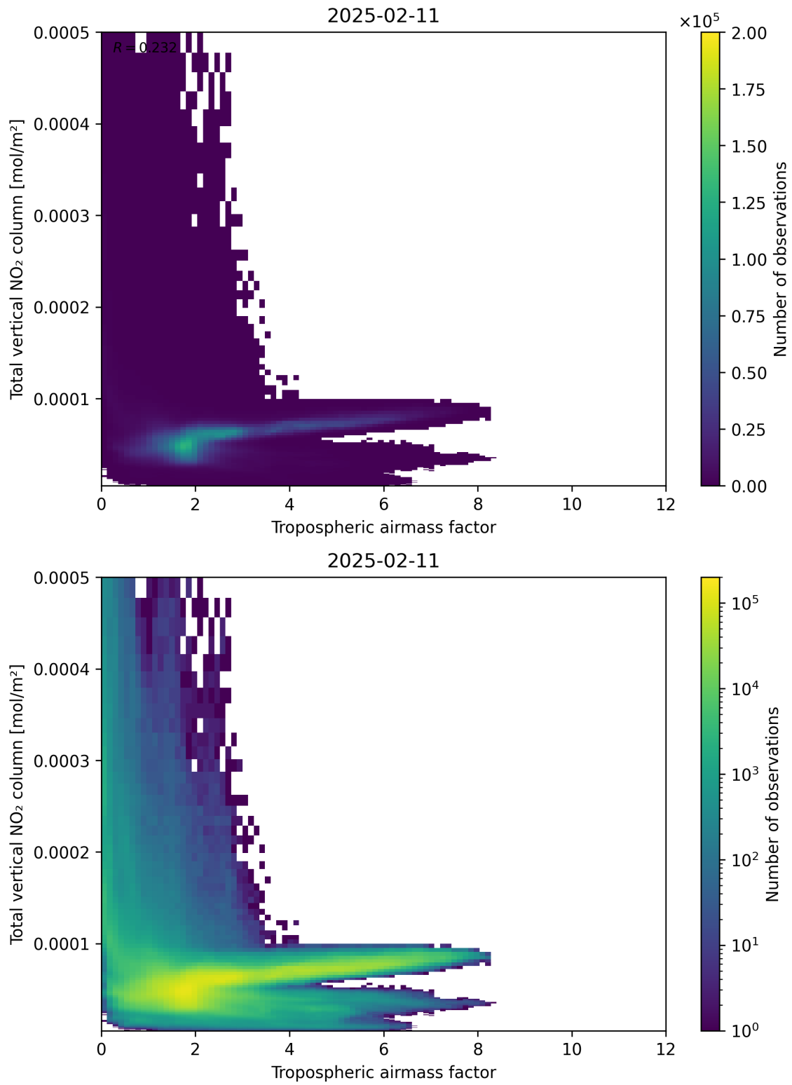
Figure 77: Scatter density plot of “Tropospheric airmass factor” against “Total vertical NO 2 column” for 2025-02-10 to 2025-02-12.
