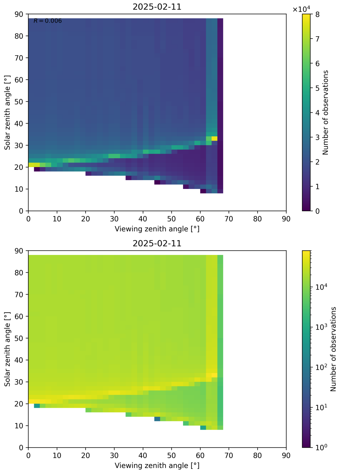
Figure 172: Scatter density plot of “Viewing zenith angle” against “Solar zenith angle” for 2025-02-10 to 2025-02-12.
