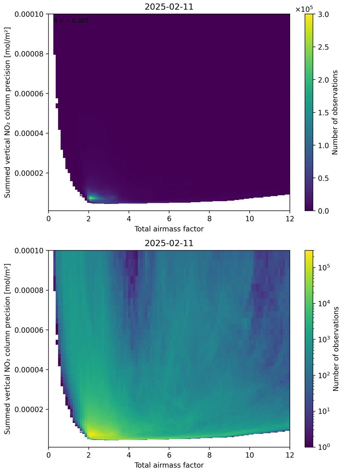
Figure 66: Scatter density plot of “Total airmass factor” against “Summed vertical NO 2 column precision” for 2025-02-10 to 2025-02-12.
