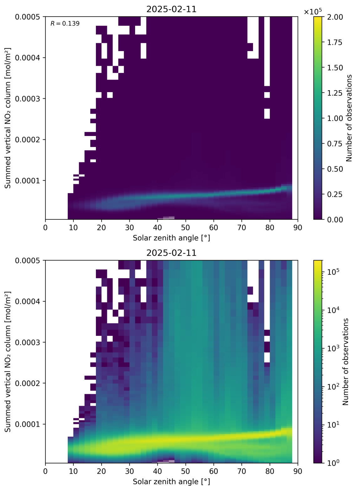
Figure 151: Scatter density plot of “Solar zenith angle” against “Summed vertical NO 2 column” for 2025-02-10 to 2025-02-12.
