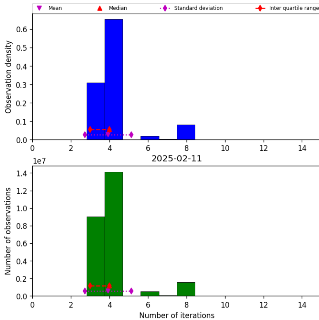
Figure 34: Histogram of “Number of iterations” for 2025-02-10 to 2025-02-12
