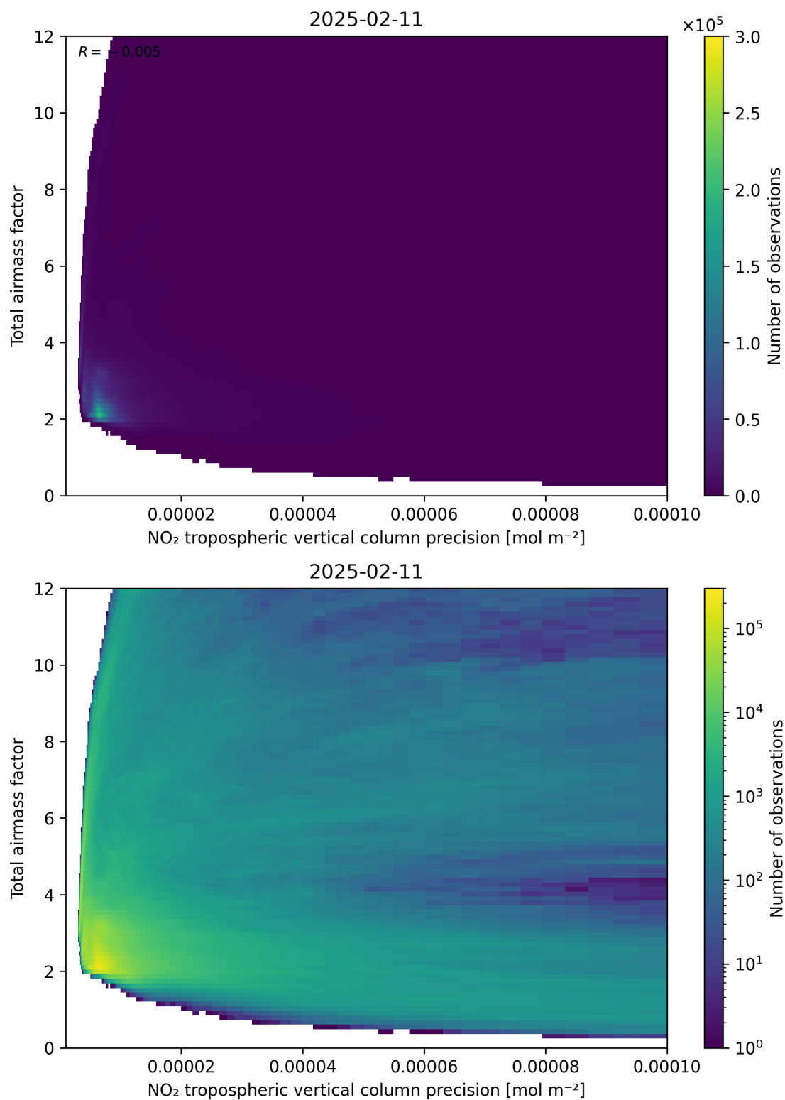
Figure 132: Scatter density plot of “NO 2 tropospheric vertical column precision” against “Total air mass factor” for 2025-02-10 to 2025-02-12.
