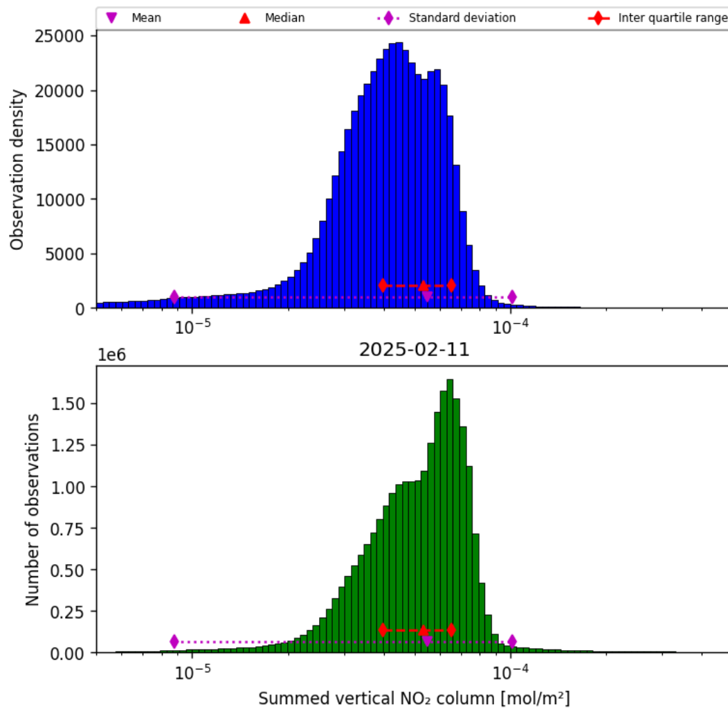
Figure 40: Histogram of “Summed vertical NO 2 column” for 2025-02-10 to 2025-02-12
