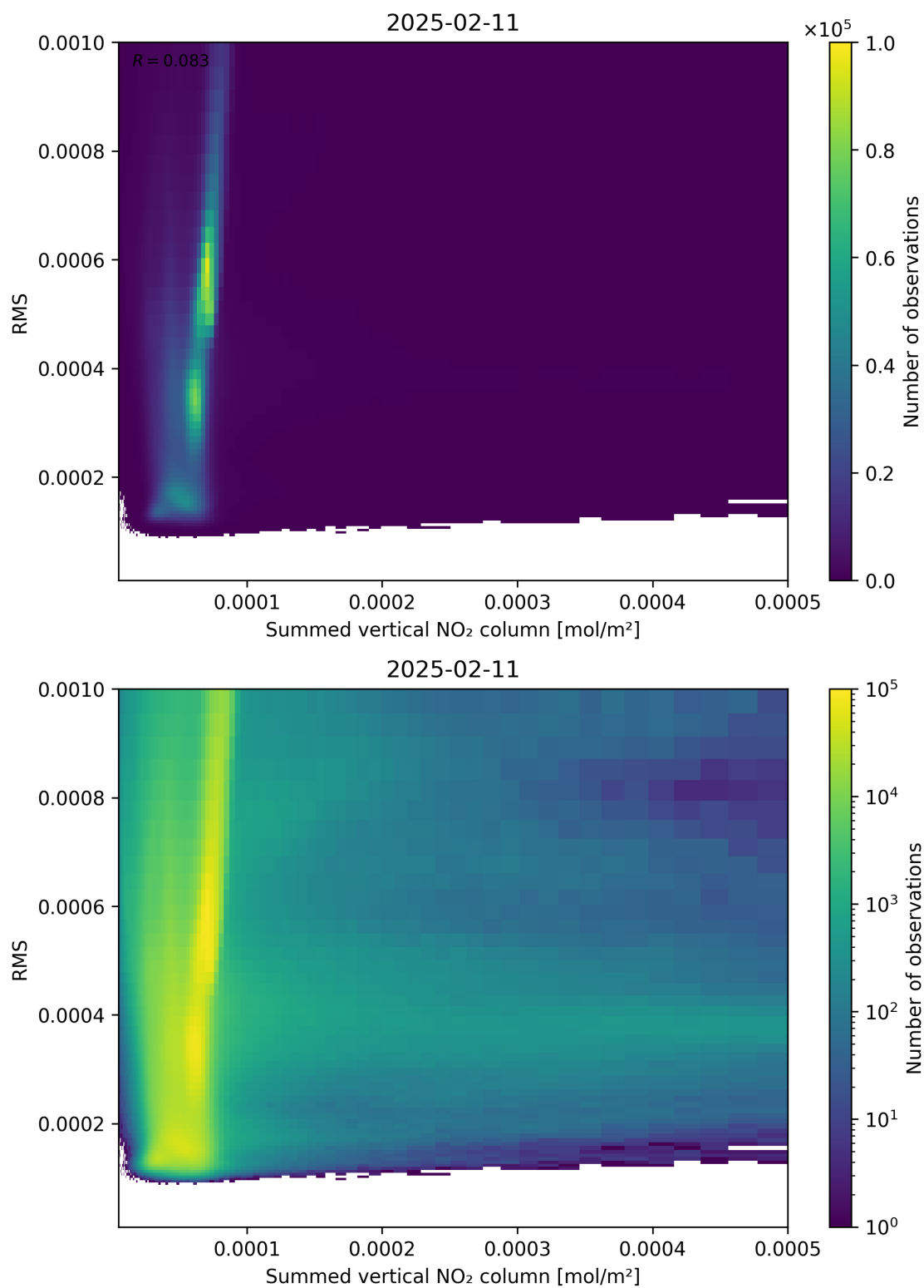
Figure 109: Scatter density plot of “Summed vertical NO 2 column” against “RMS” for 2025-02-10 to 2025-02-12.
