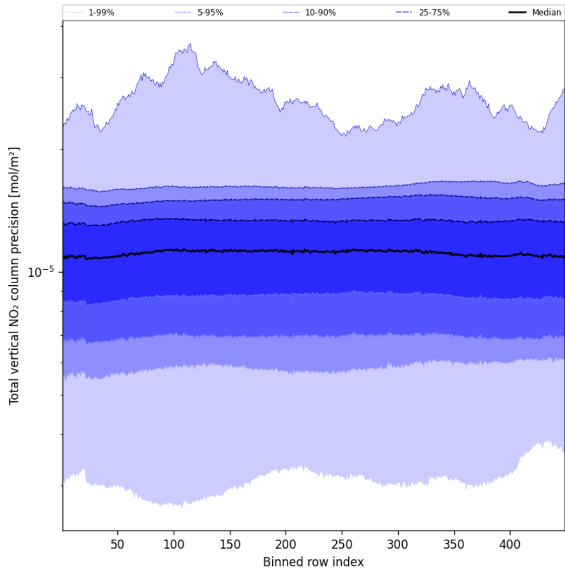
Figure 56: Along track statistics of “Total vertical NO 2 column precision” for 2025-02-10 to 2025-02-12
