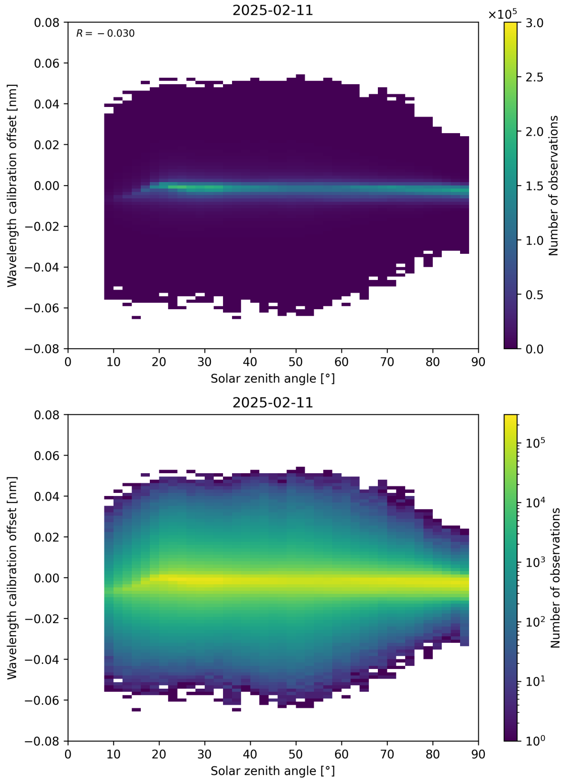
Figure 158: Scatter density plot of “Solar zenith angle” against “Wavelength calibration offset” for 2025-02-10 to 2025-02-12.
