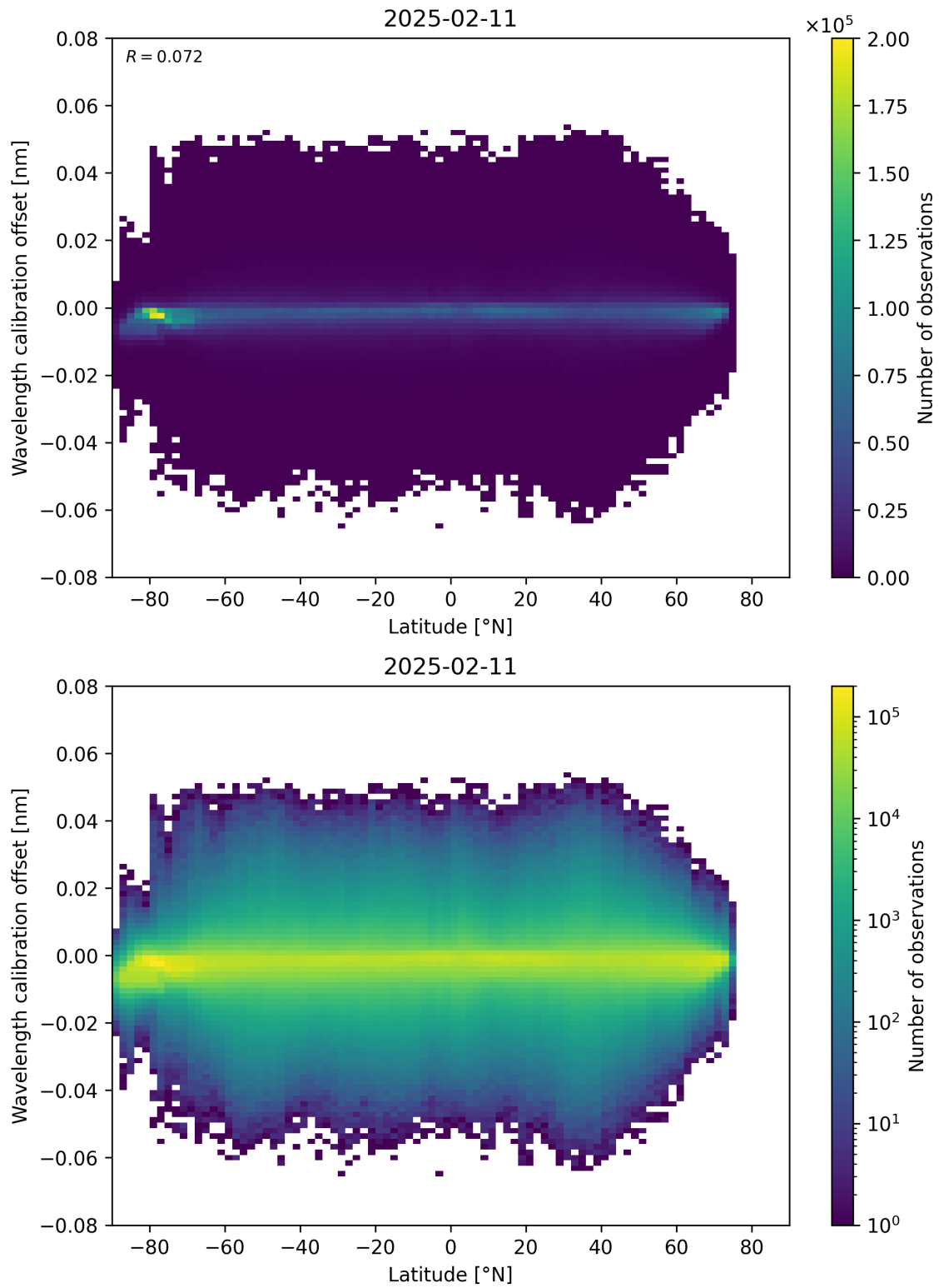
Figure 95: Scatter density plot of “Latitude” against “Wavelength calibration offset” for 2025-02-10 to 2025-02-12.
