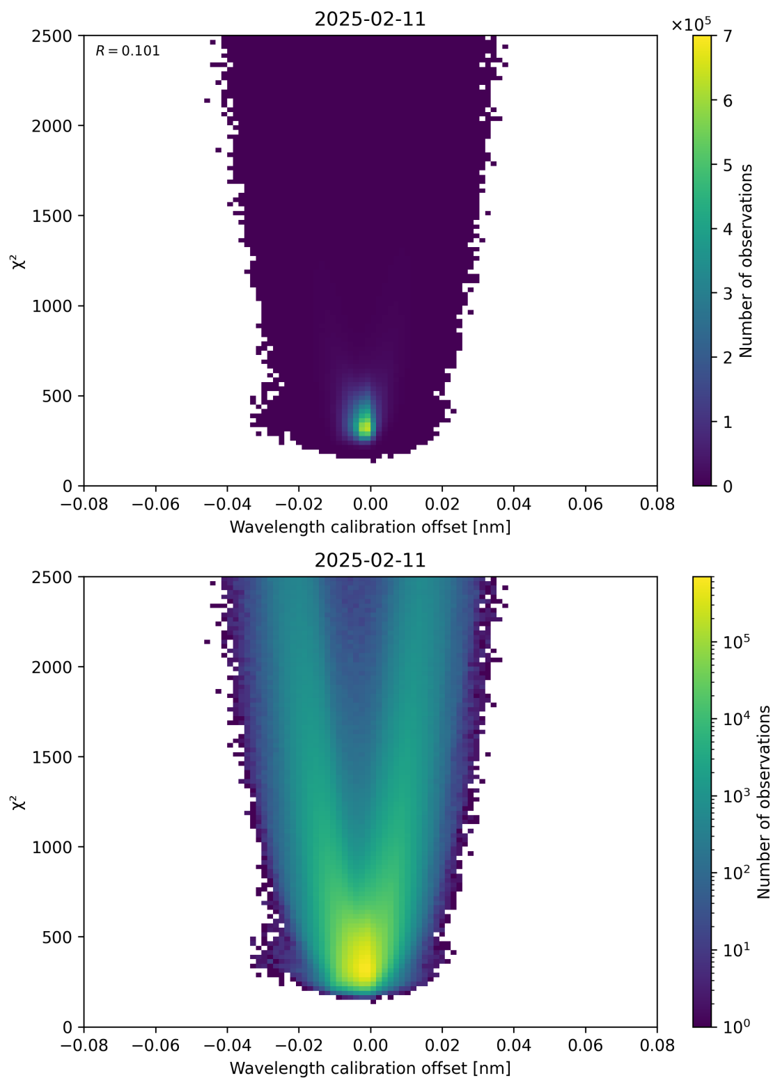
Figure 175: Scatter density plot of “Wavelength calibration offset” against “ \chi^2 ” for 2025-02-10 to 2025-02-12.
