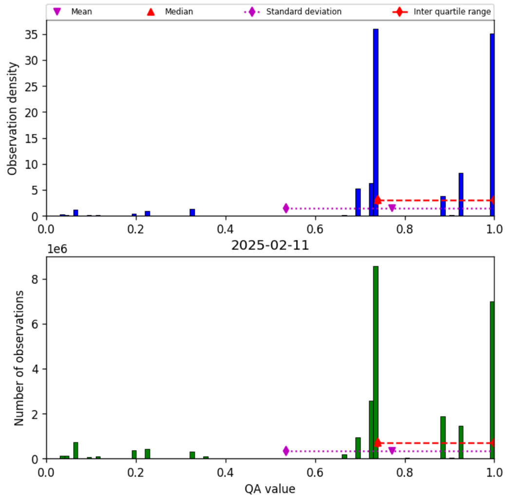
Figure 28: Histogram of “QA value” for 2025-02-10 to 2025-02-12
