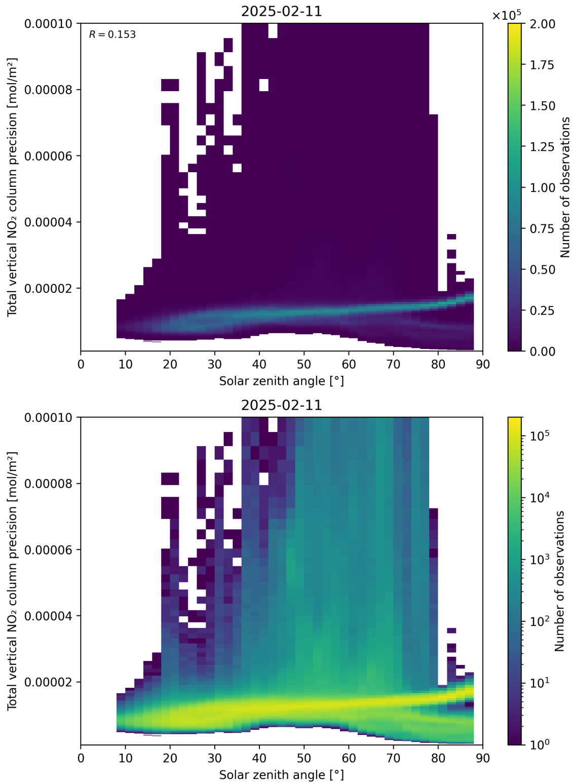
Figure 154: Scatter density plot of “Solar zenith angle” against “Total vertical NO 2 column precision” for 2025-02-10 to 2025-02-12.
