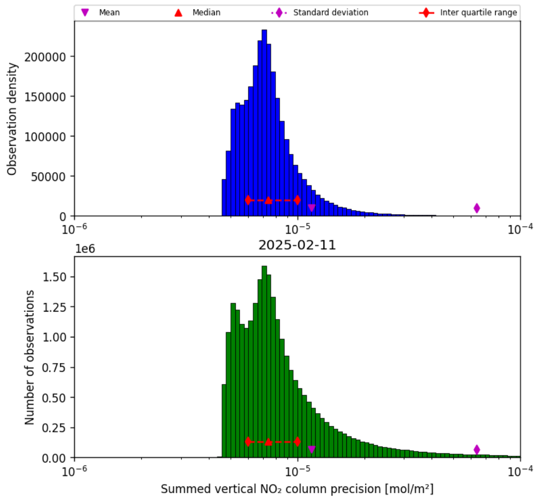
Figure 41: Histogram of “Summed vertical NO 2 column precision” for 2025-02-10 to 2025-02-12
