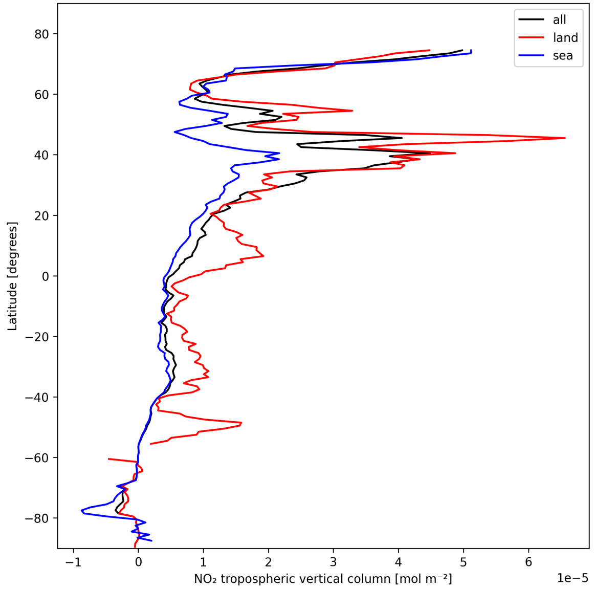
Figure 12: Zonal average of “NO 2 tropospheric vertical column” for 2025-02-10 to 2025-02-12.
