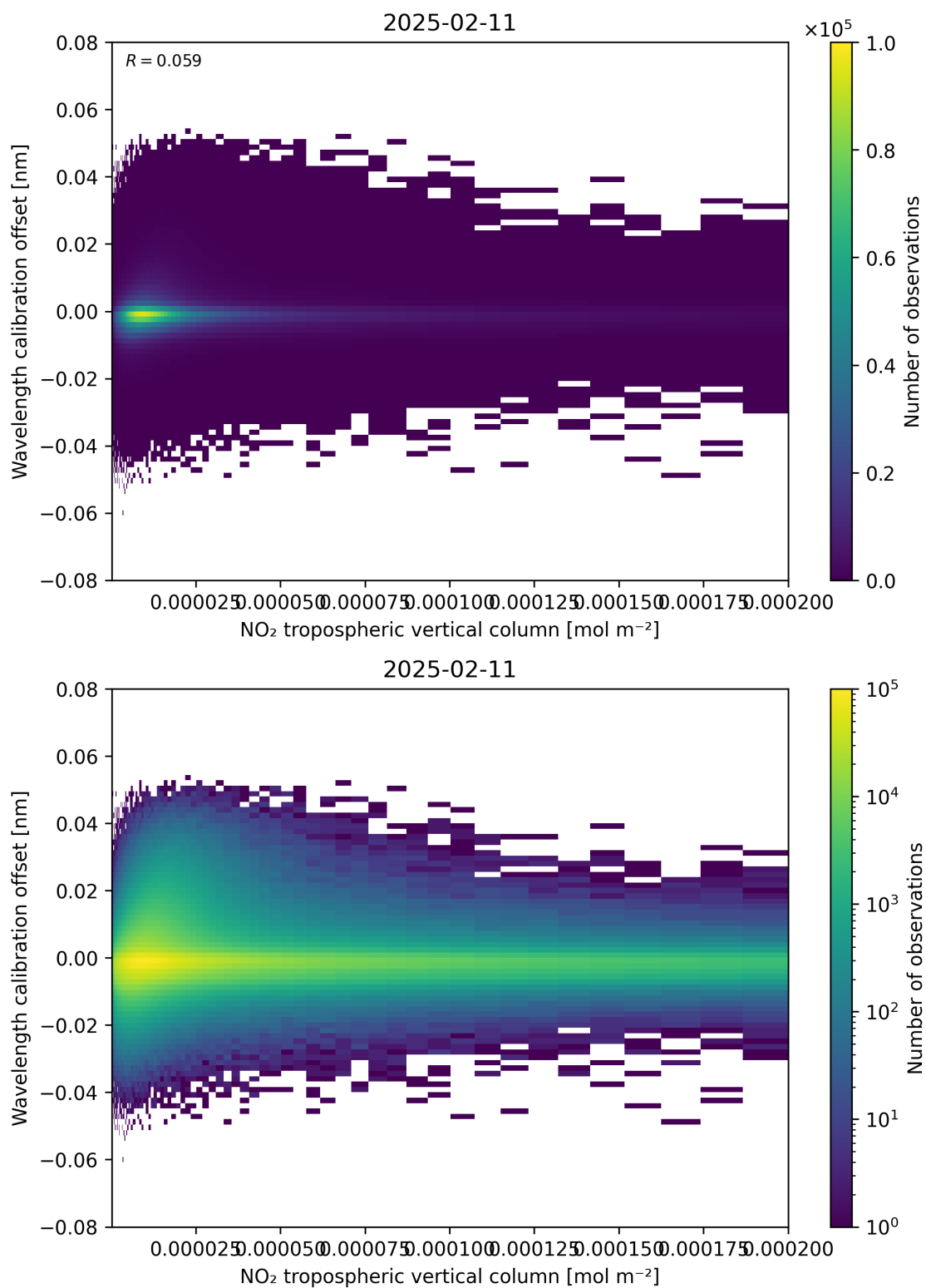
Figure 143: Scatter density plot of “NO 2 tropospheric vertical column” against “Wavelength calibration offset” for 2025-02-10 to 2025-02-12.
