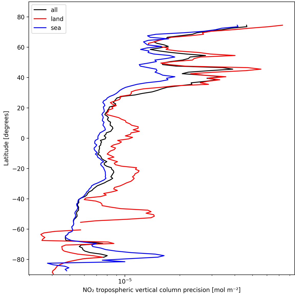
Figure 13: Zonal average of "NO 2 tropospheric vertical column precision" for 2025-02-10 to 2025-02-12.
