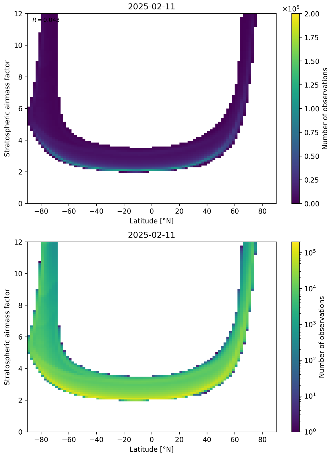
Figure 83: Scatter density plot of “Latitude” against “Stratospheric airmass factor” for 2025-02-10 to 2025-02-12.
