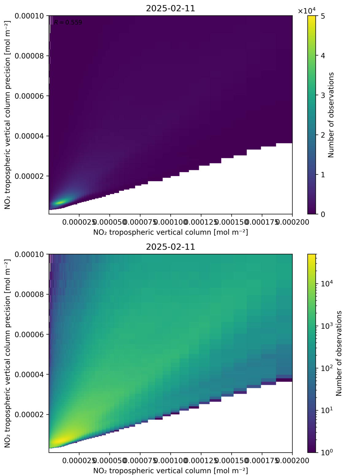
Figure 130: Scatter density plot of “NO 2 tropospheric vertical column” against “NO 2 tropospheric vertical column precision” for 2025-02-10 to 2025-02-12.
