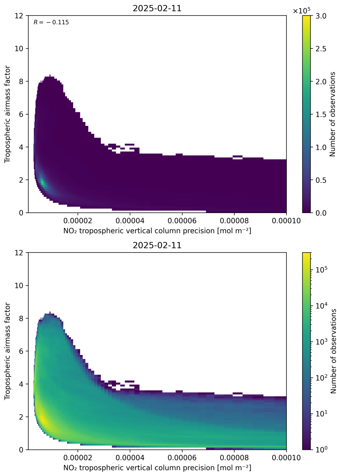
Figure 133: Scatter density plot of “NO 2 tropospheric vertical column precision” against “Tropospheric air mass factor” for 2025-02-10 to 2025-02-12.
