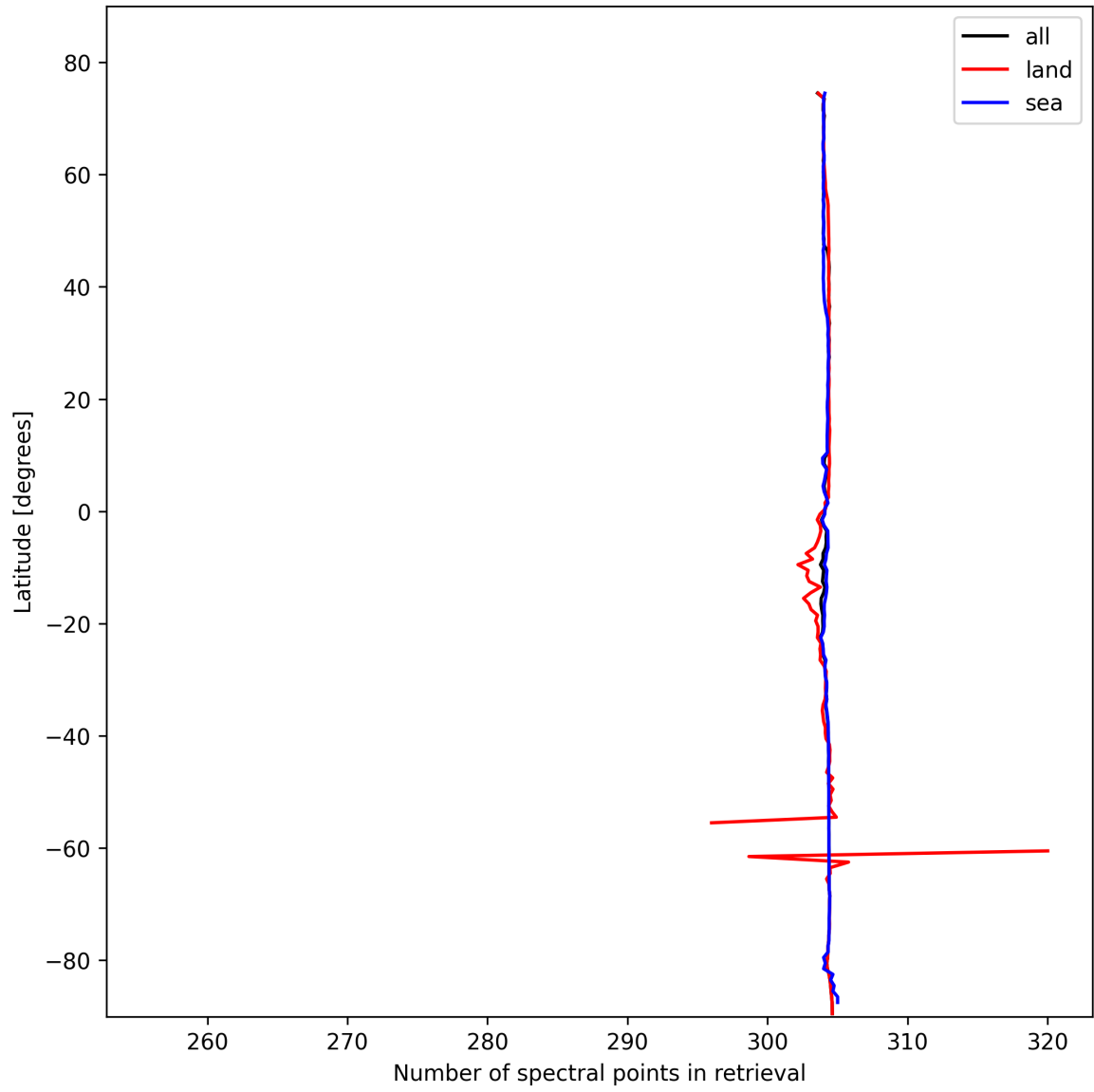
Figure 16: Zonal average of “Number of spectral points in retrieval” for 2025-02-10 to 2025-02-12.
