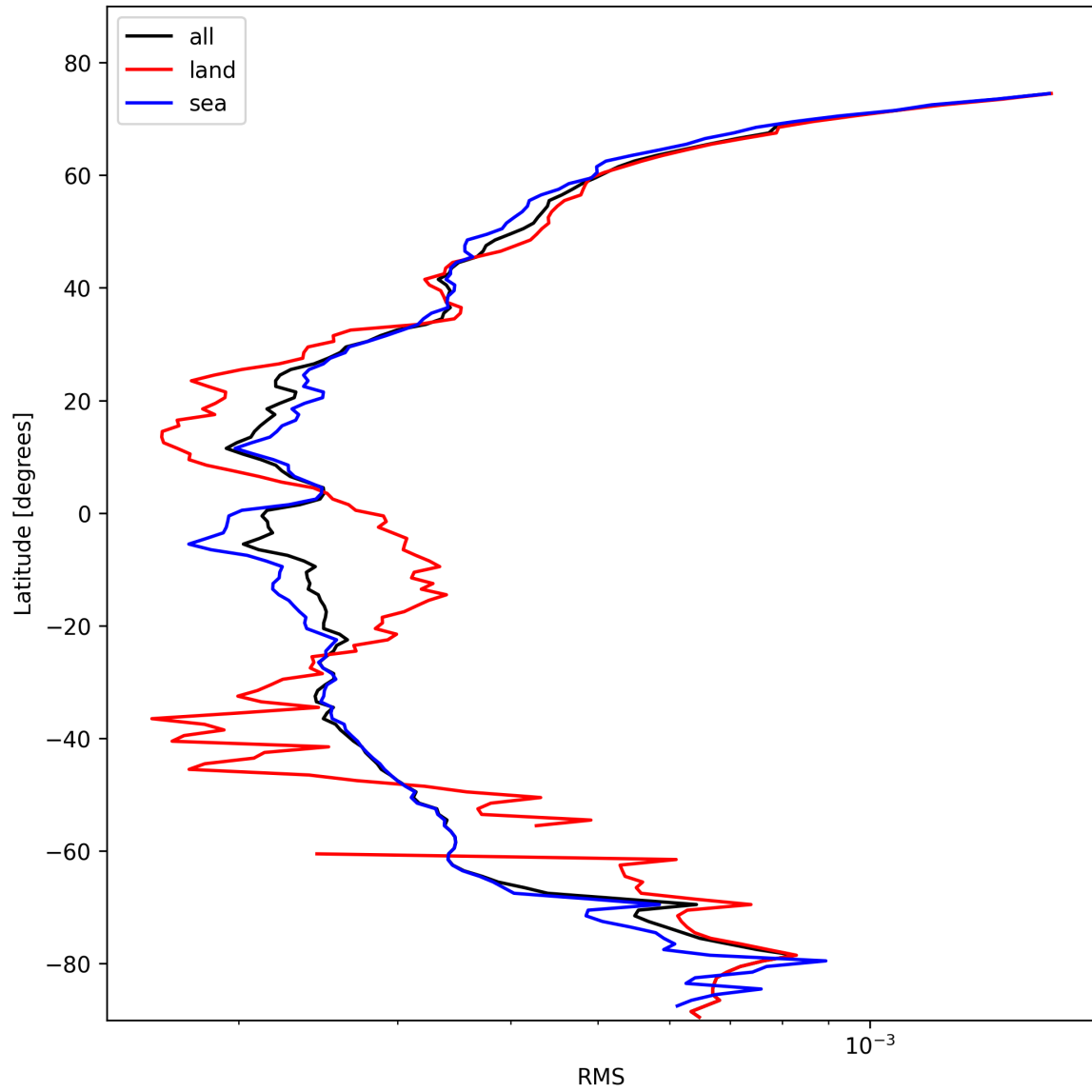
Figure 26: Zonal average of “RMS” for 2025-02-10 to 2025-02-12.
