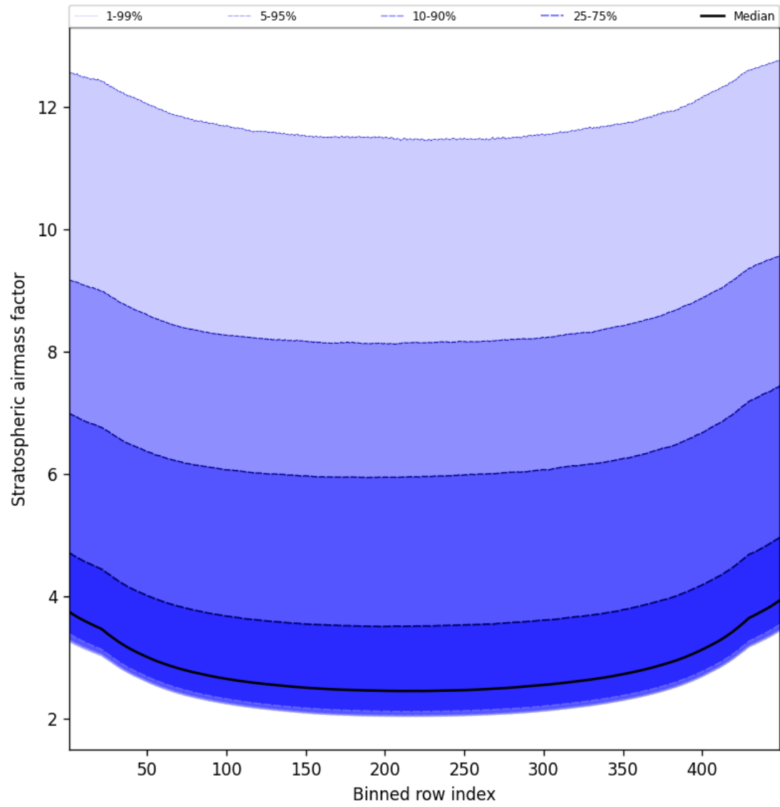
Figure 61: Along track statistics of “Stratospheric airmass factor” for 2025-02-10 to 2025-02-12
