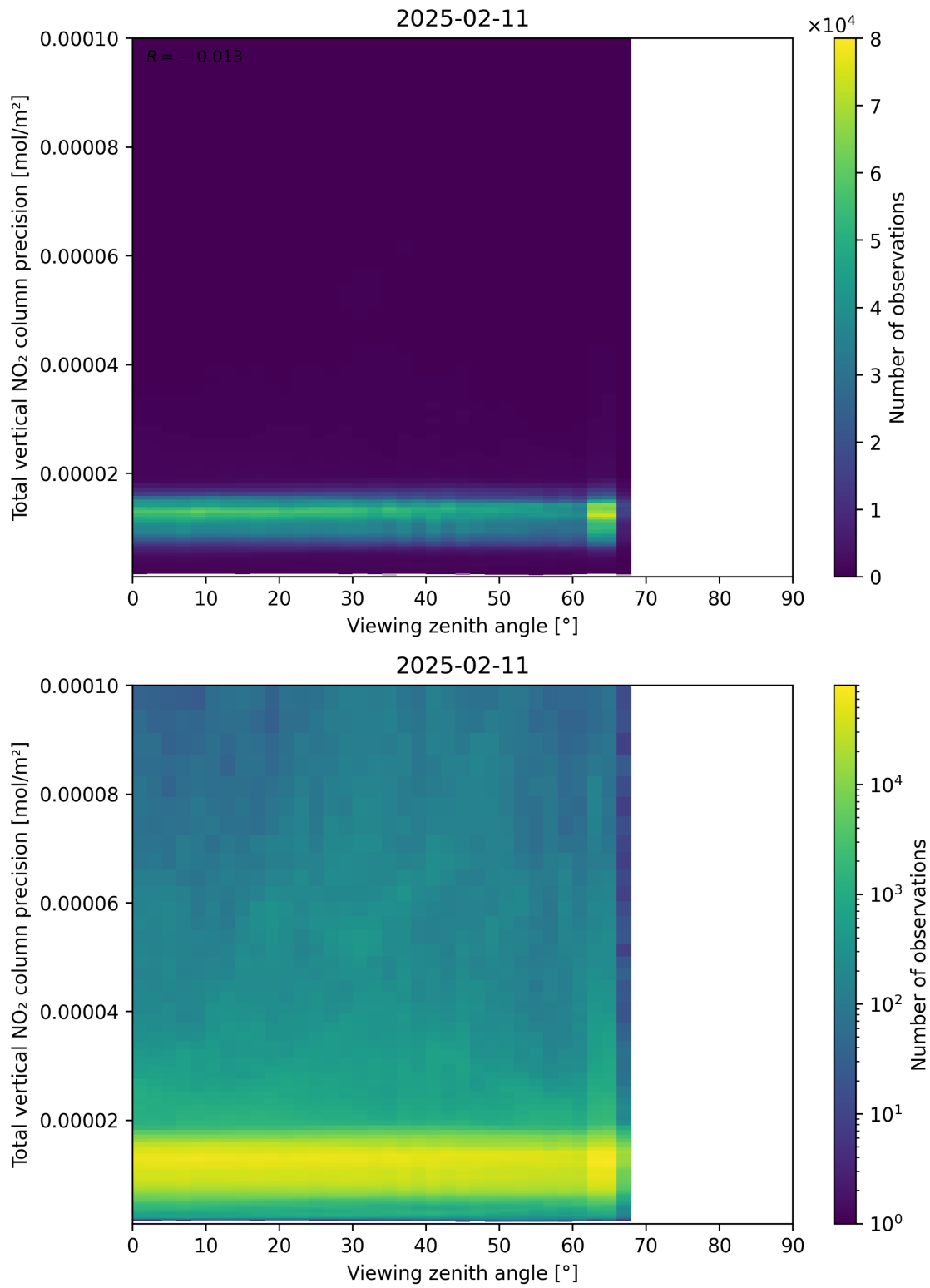
Figure 168: Scatter density plot of “Viewing zenith angle” against “Total vertical NO 2 column precision” for 2025-02-10 to 2025-02-12.
