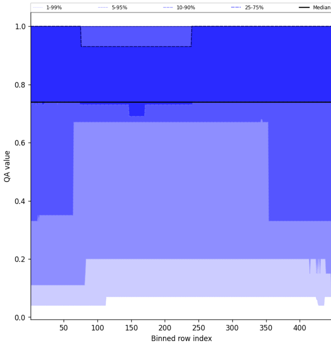
Figure 45: Along track statistics of “QA value” for 2025-02-10 to 2025-02-12
