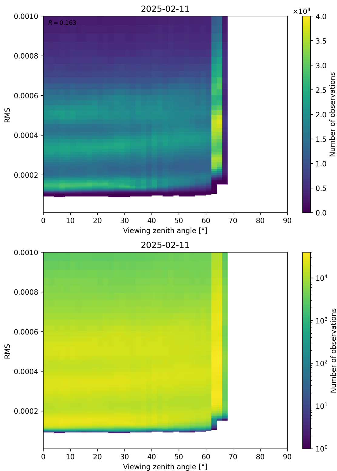
Figure 171: Scatter density plot of “Viewing zenith angle” against “RMS” for 2025-02-10 to 2025-02-12.
