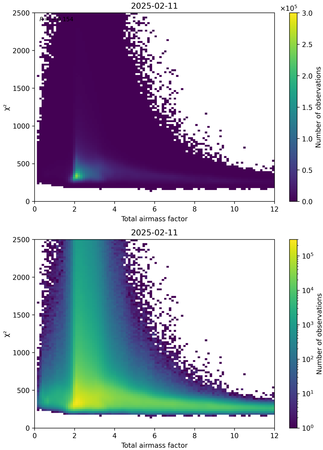
Figure 63: Scatter density plot of “Total airmass factor” against “ \chi^2 ” for 2025-02-10 to 2025-02-12.
