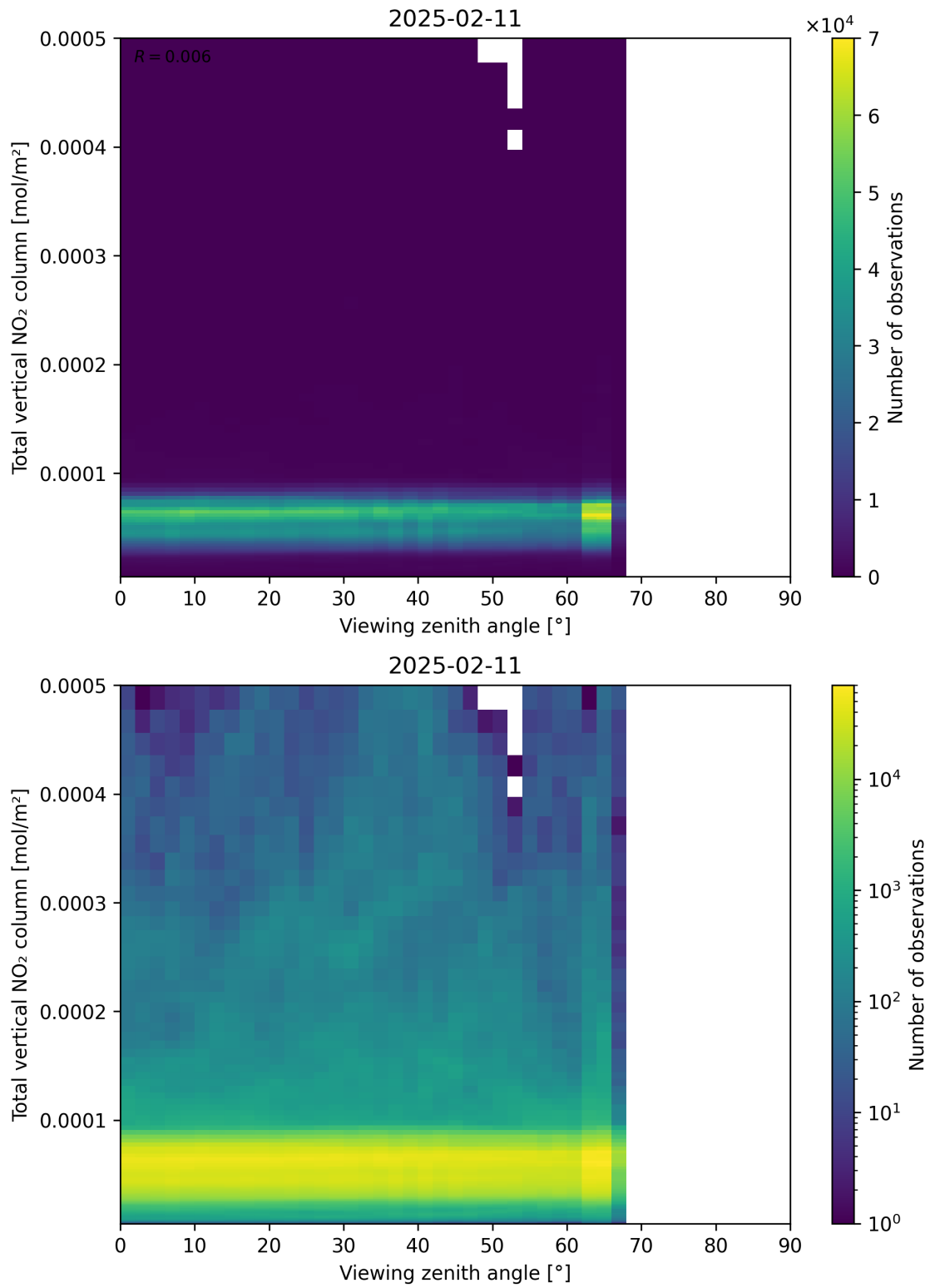
Figure 167: Scatter density plot of “Viewing zenith angle” against “Total vertical NO 2 column” for 2025-02-10 to 2025-02-12.
