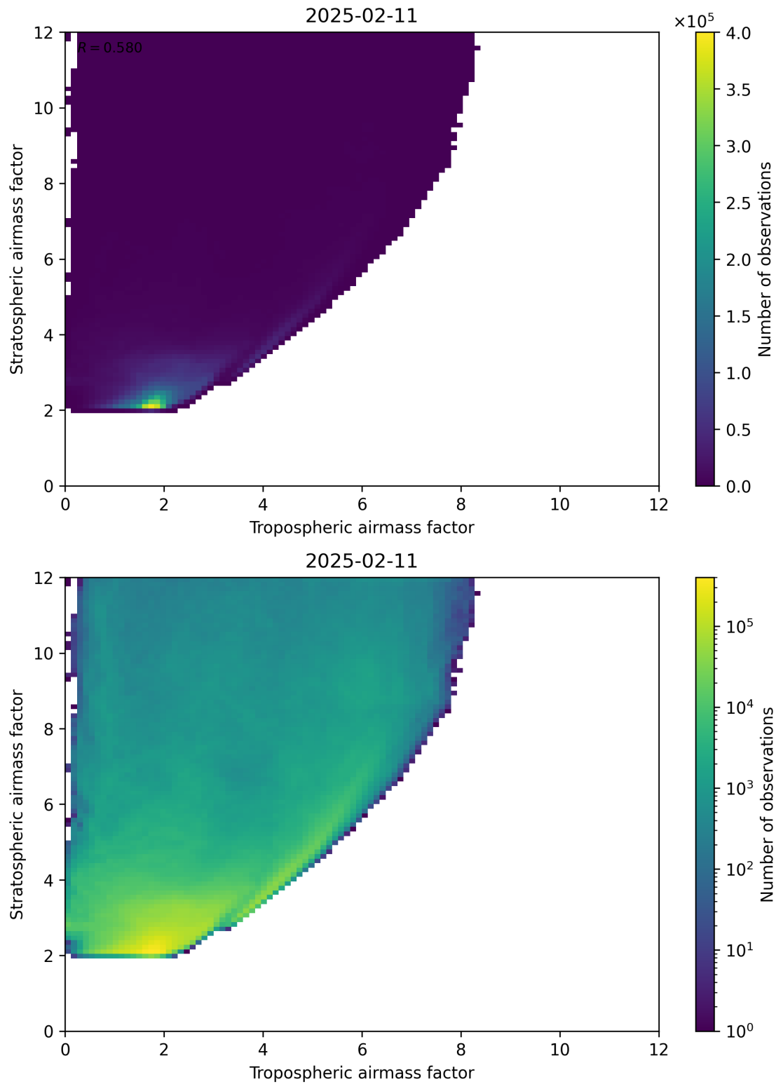
Figure 71: Scatter density plot of “Tropospheric airmass factor” against “Stratospheric airmass factor” for 2025-02-10 to 2025-02-12.
