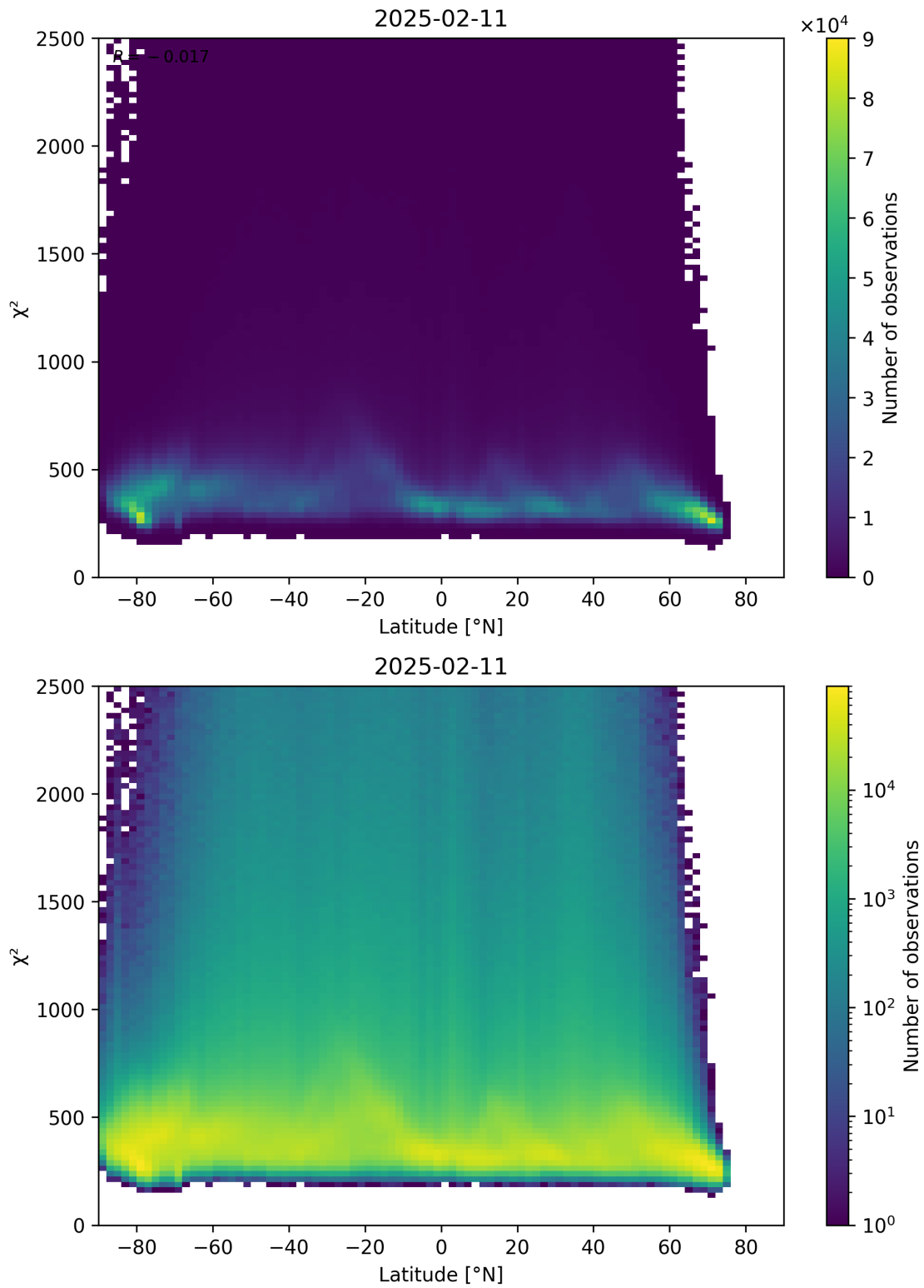
Figure 86: Scatter density plot of “Latitude” against “ \chi^2 ” for 2025-02-10 to 2025-02-12.
