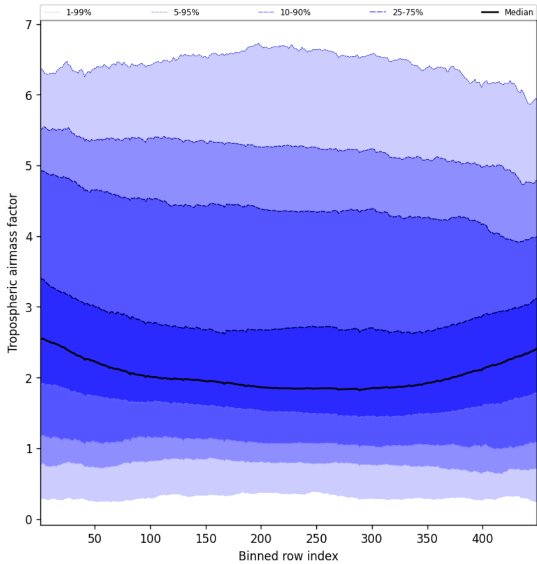
Figure 48: Along track statistics of “Tropospheric airmass factor” for 2025-02-10 to 2025-02-12
