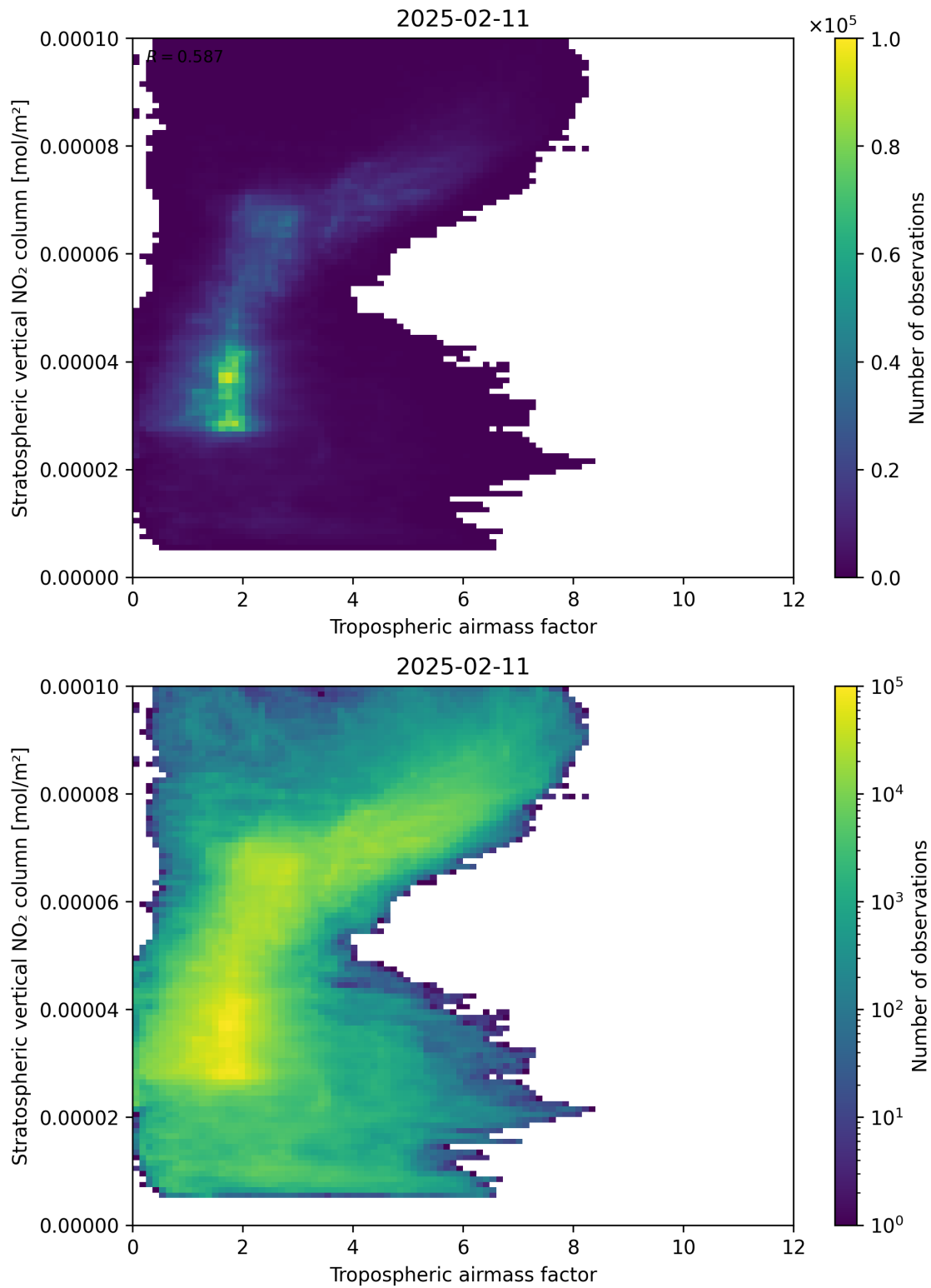
Figure 74: Scatter density plot of “Tropospheric air mass factor” against “Stratospheric vertical NO 2 column” for 2025-02-10 to 2025-02-12.
