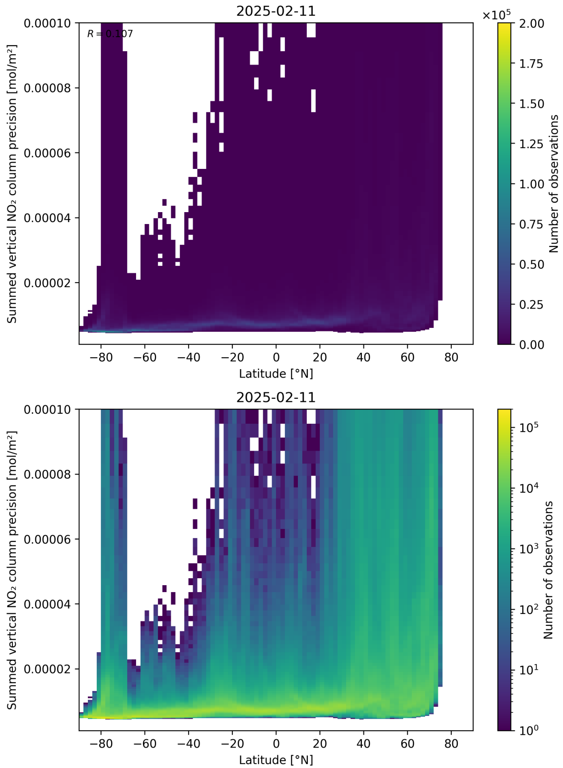
Figure 89: Scatter density plot of “Latitude” against “Summed vertical NO 2 column precision” for 2025-02-10 to 2025-02-12.
