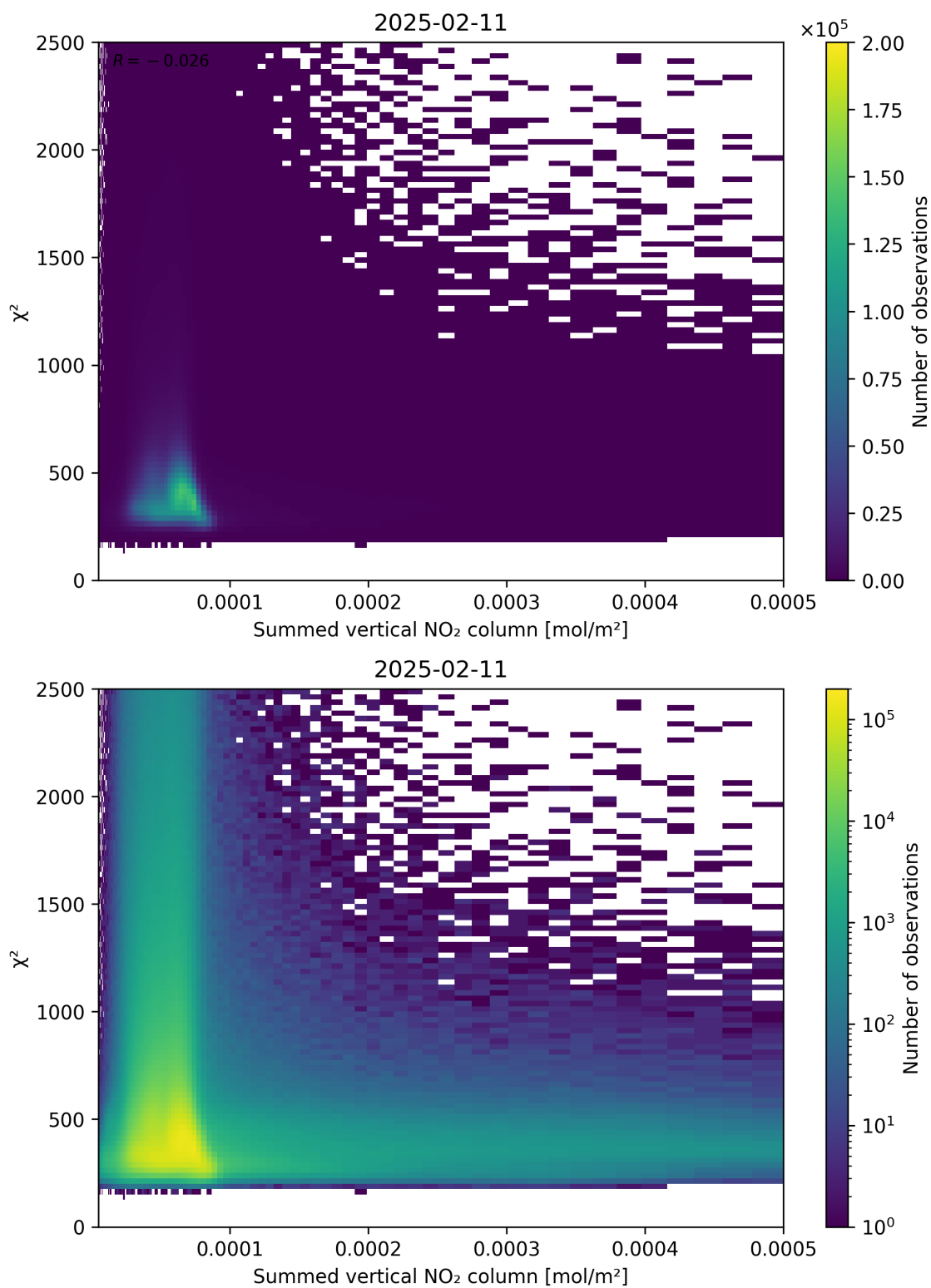
Figure 104: Scatter density plot of “Summed vertical NO 2 column” against “ \chi^2 ” for 2025-02-10 to 2025-02-12.
