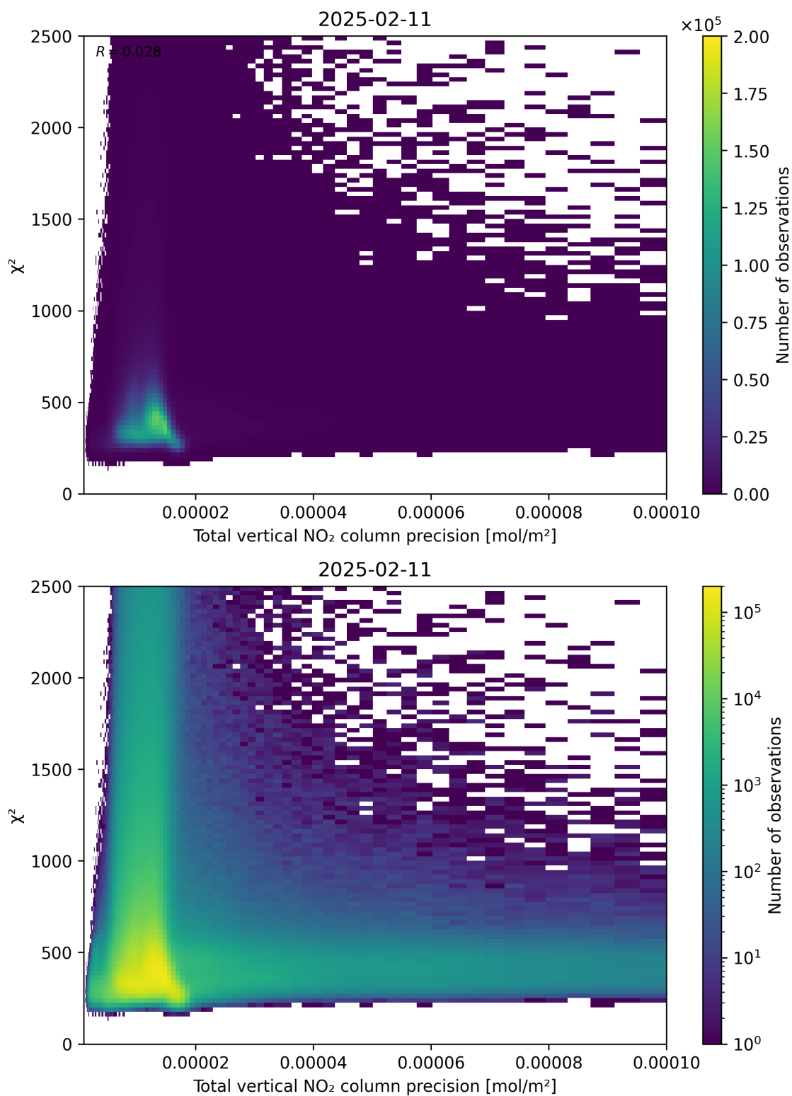
Figure 116: Scatter density plot of “Total vertical NO 2 column precision” against “ \chi^2 ” for 2025-02-10 to 2025-02-12.
