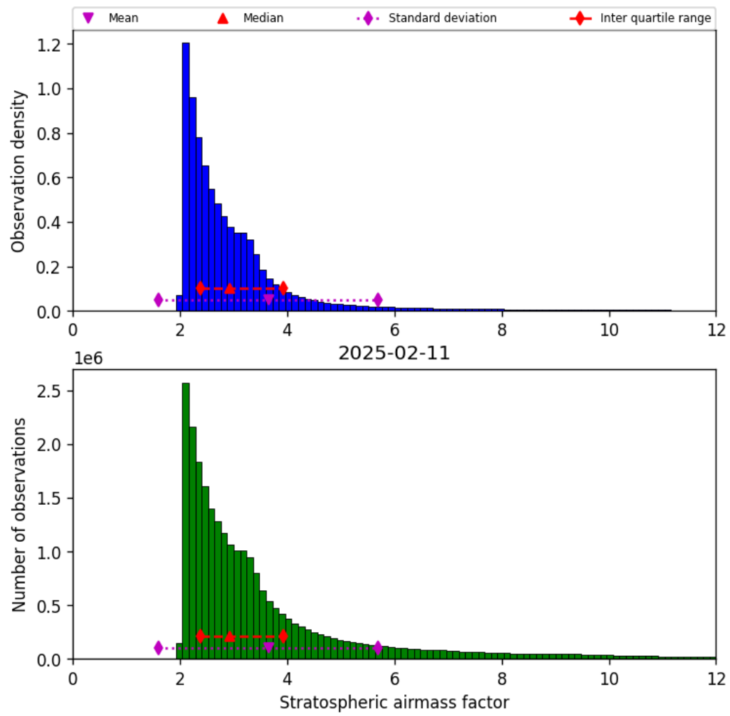
Figure 44: Histogram of “Stratospheric airmass factor” for 2025-02-10 to 2025-02-12
