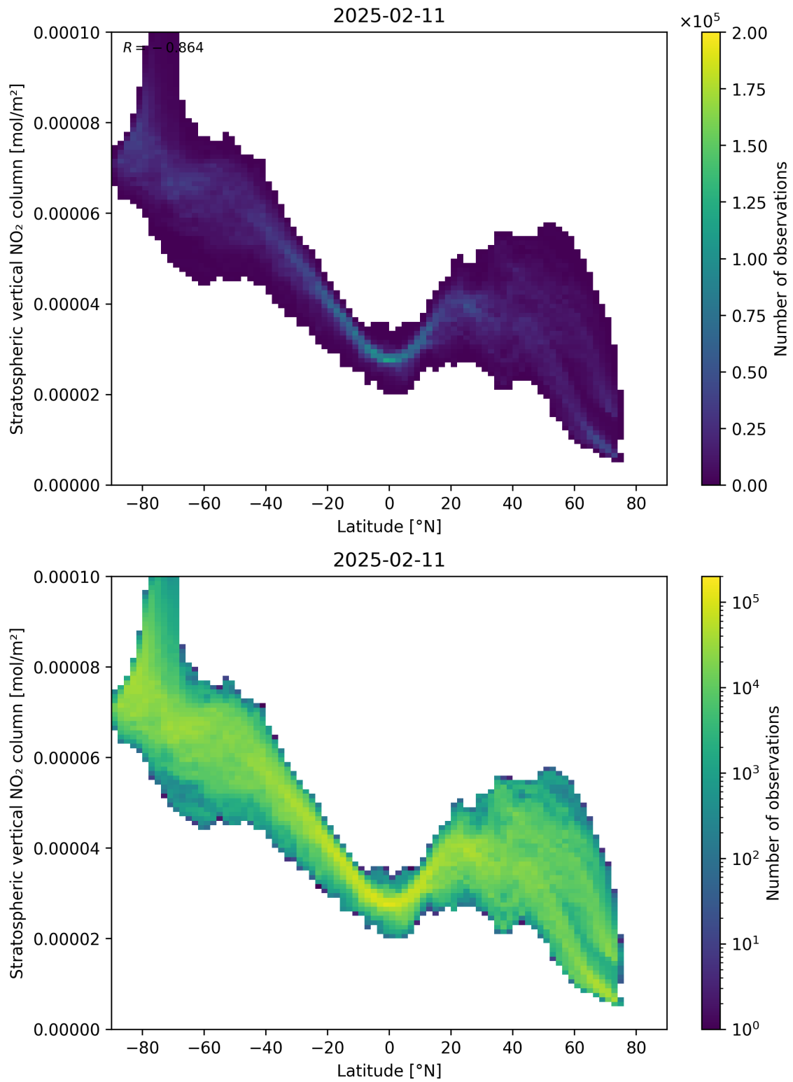
Figure 87: Scatter density plot of “Latitude” against “Stratospheric vertical NO 2 column” for 2025-02-10 to 2025-02-12.
