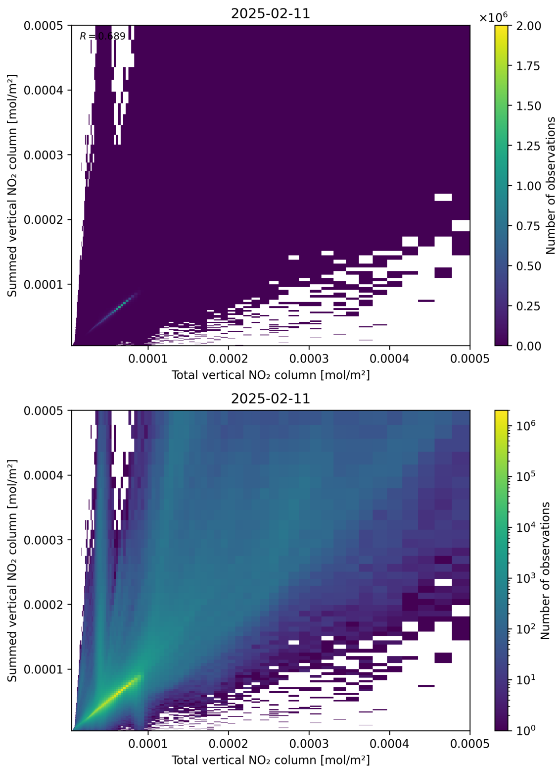
Figure 112: Scatter density plot of “Total vertical NO 2 column” against “Summed vertical NO 2 column” for 2025-02-10 to 2025-02-12.
