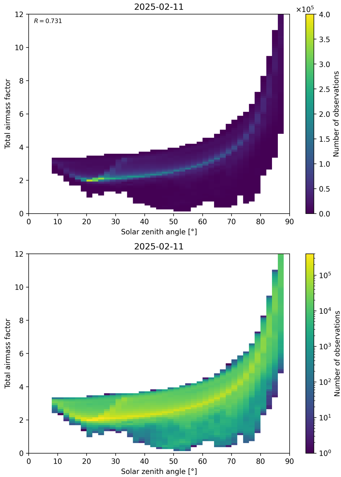
Figure 146: Scatter density plot of “Solar zenith angle” against “Total air mass factor” for 2025-02-10 to 2025-02-12.
