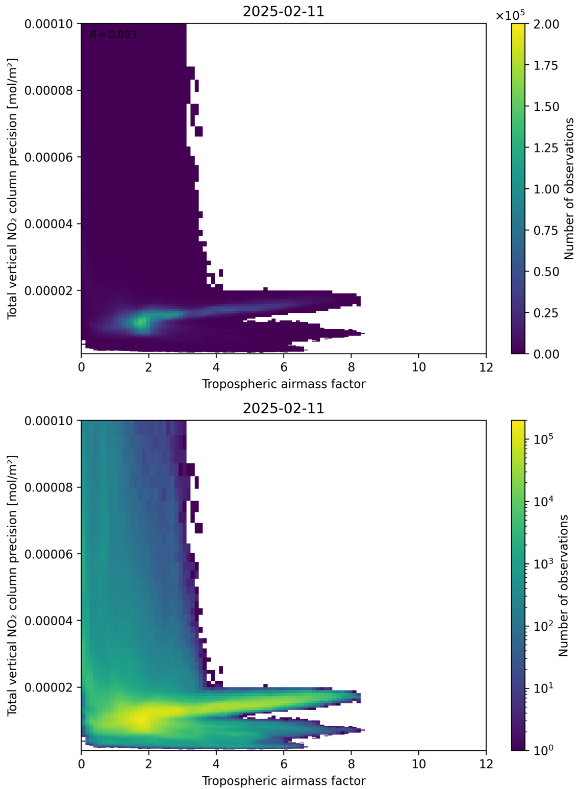
Figure 78: Scatter density plot of “Tropospheric air mass factor” against “Total vertical NO 2 column precision” for 2025-02-10 to 2025-02-12.
