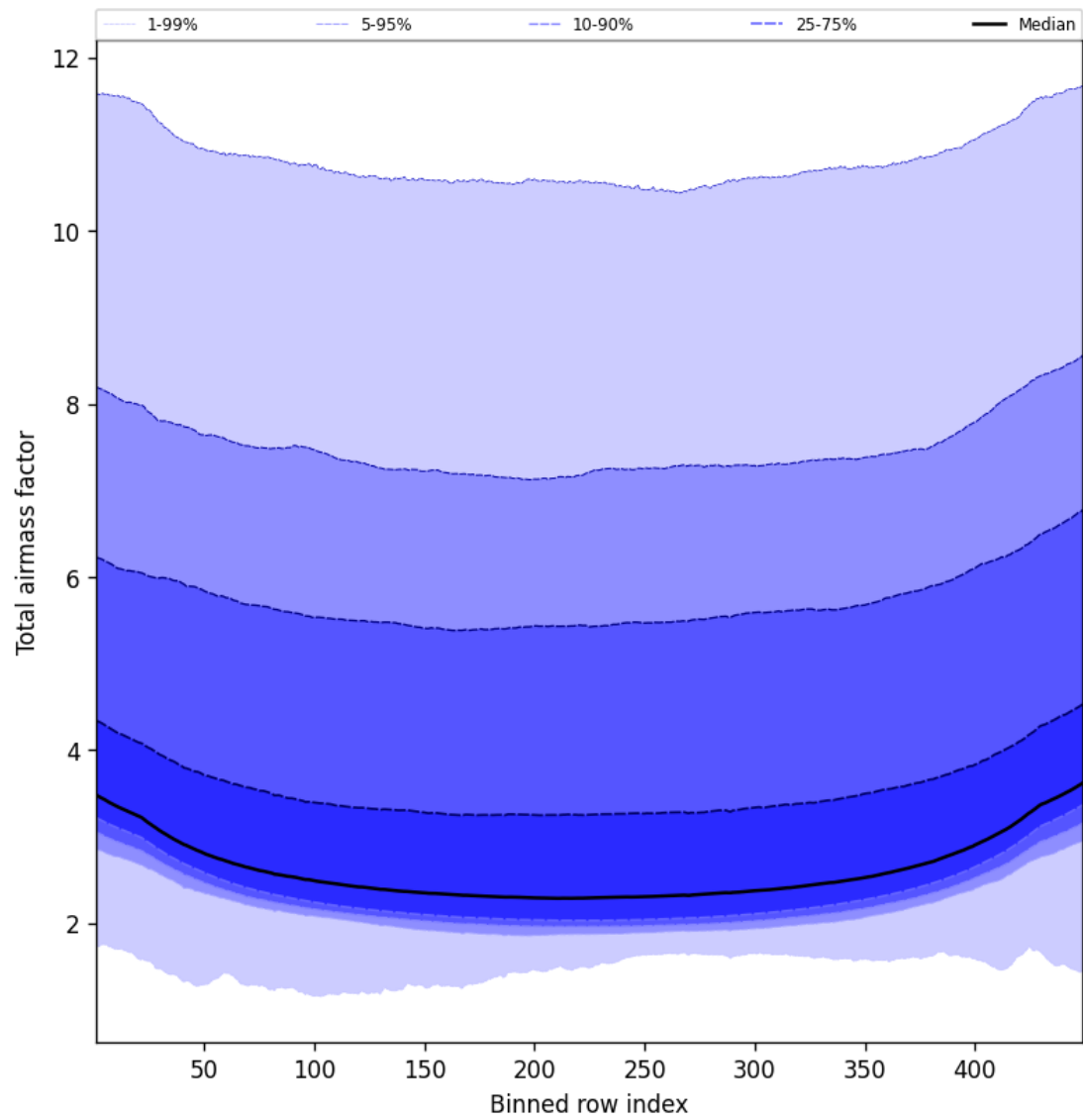
Figure 49: Along track statistics of “Total airmass factor” for 2025-02-10 to 2025-02-12
