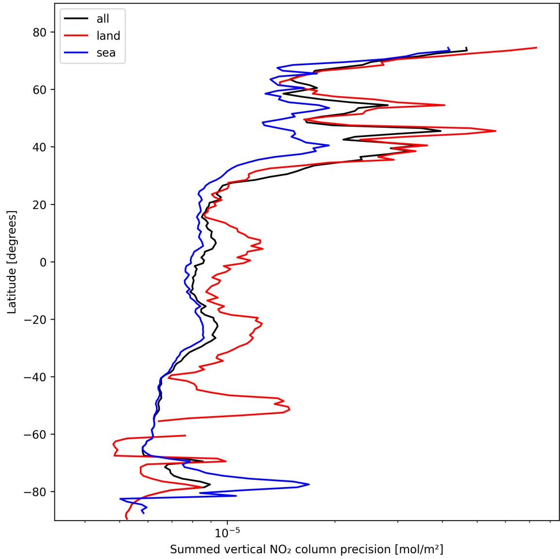
Figure 24: Zonal average of “Summed vertical NO 2 column precision” for 2025-02-10 to 2025-02-12.
