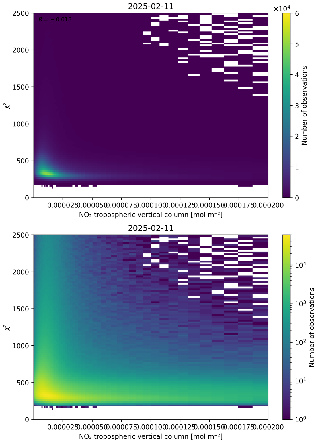
Figure 124: Scatter density plot of “NO 2 tropospheric vertical column” against “ \chi^2 ” for 2025-02-10 to 2025-02-12.
