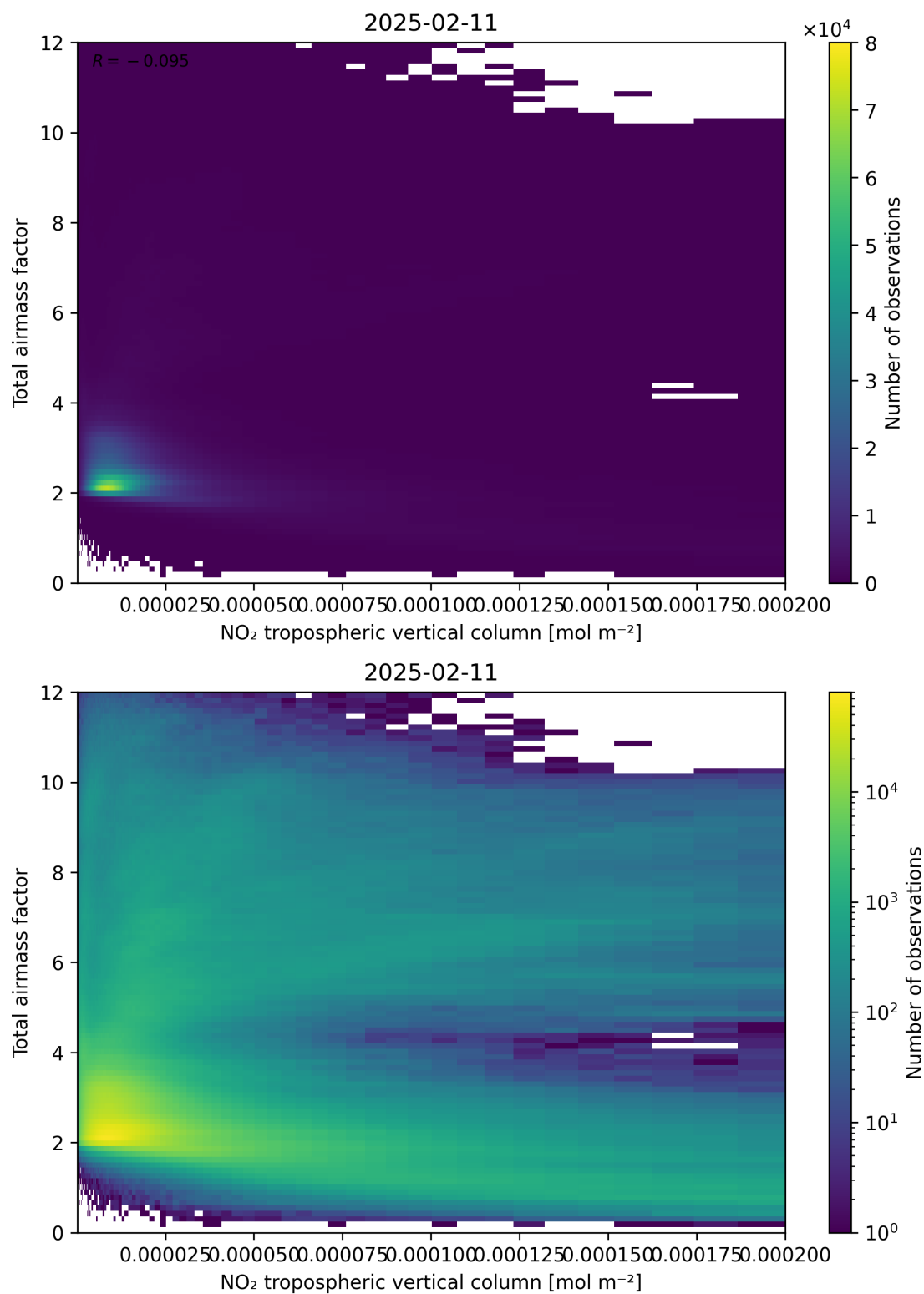
Figure 122: Scatter density plot of “NO 2 tropospheric vertical column” against “Total air mass factor” for 2025-02-10 to 2025-02-12.
