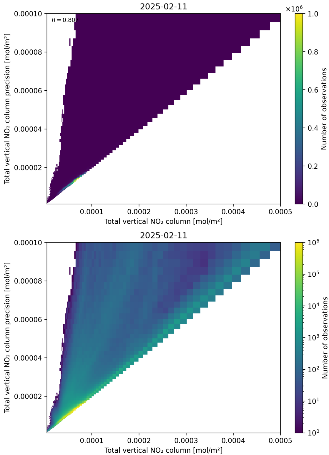
Figure 114: Scatter density plot of “Total vertical NO 2 column” against “Total vertical NO 2 column precision” for 2025-02-10 to 2025-02-12.
