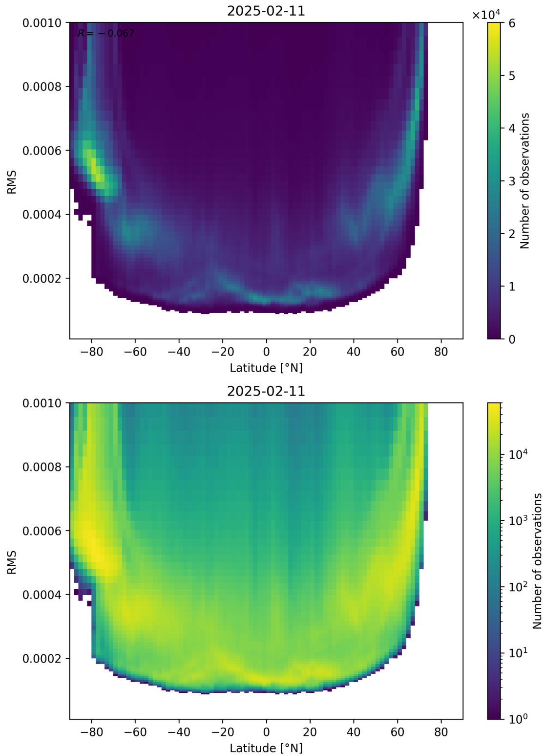
Figure 94: Scatter density plot of “Latitude” against “RMS” for 2025-02-10 to 2025-02-12.
