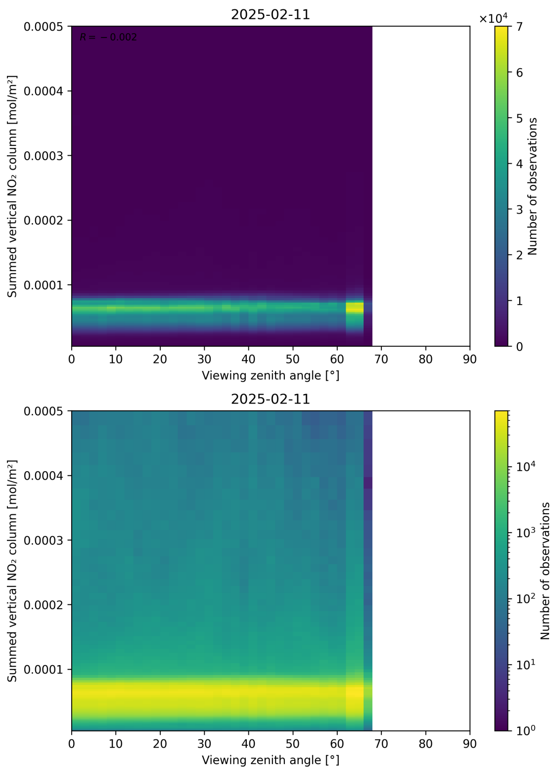
Figure 165: Scatter density plot of “Viewing zenith angle” against “Summed vertical NO 2 column” for 2025-02-10 to 2025-02-12.
