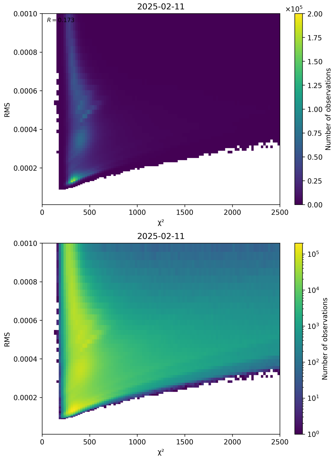
Figure 82: Scatter density plot of “ \chi^2 ” against “RMS” for 2025-02-10 to 2025-02-12.
