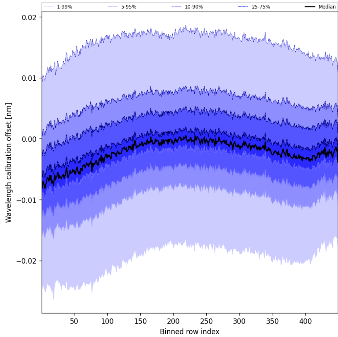
Figure 52: Along track statistics of “Wavelength calibration offset” for 2025-02-10 to 2025-02-12
