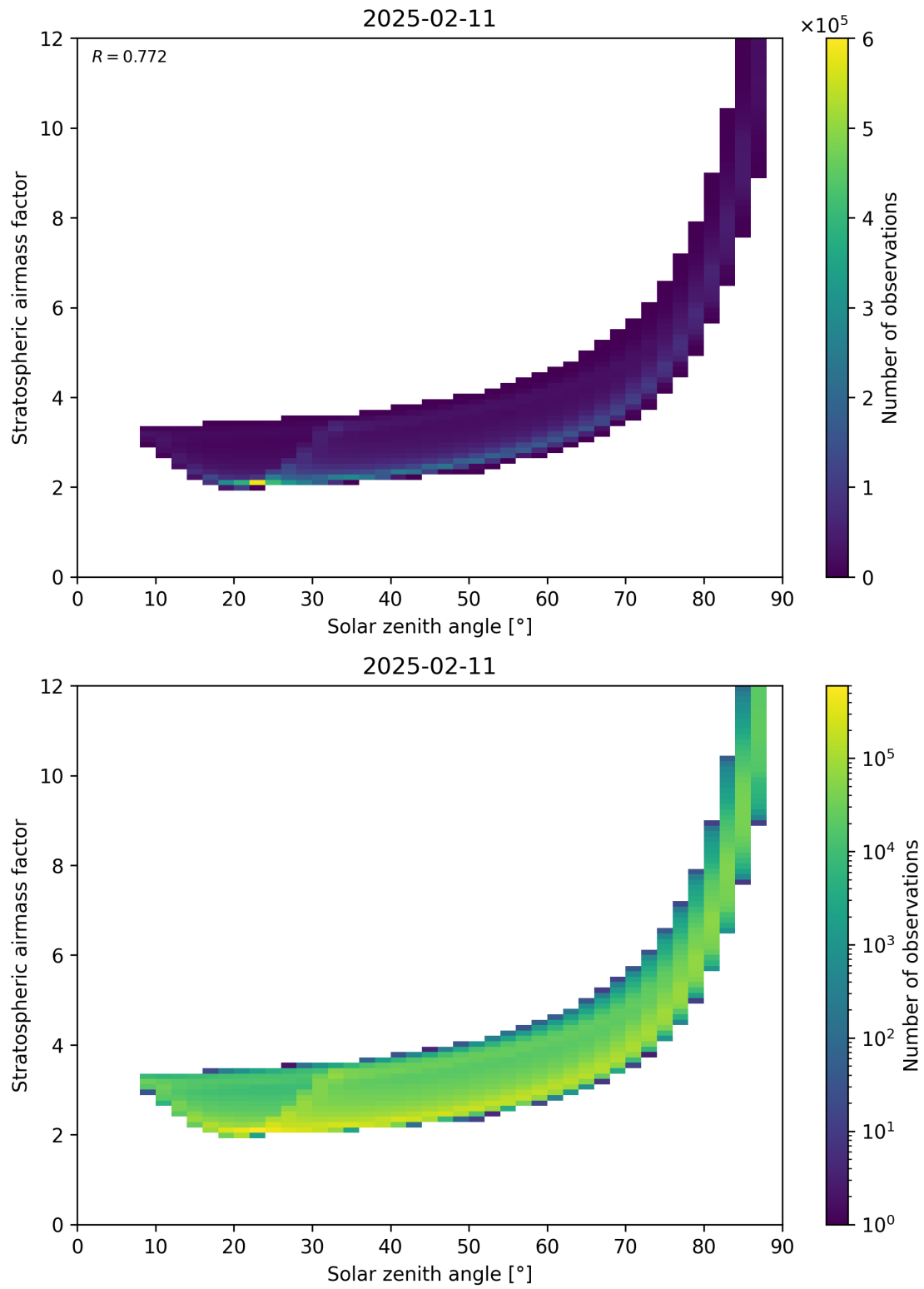
Figure 145: Scatter density plot of “Solar zenith angle” against “Stratospheric airmass factor” for 2025-02-10 to 2025-02-12.
