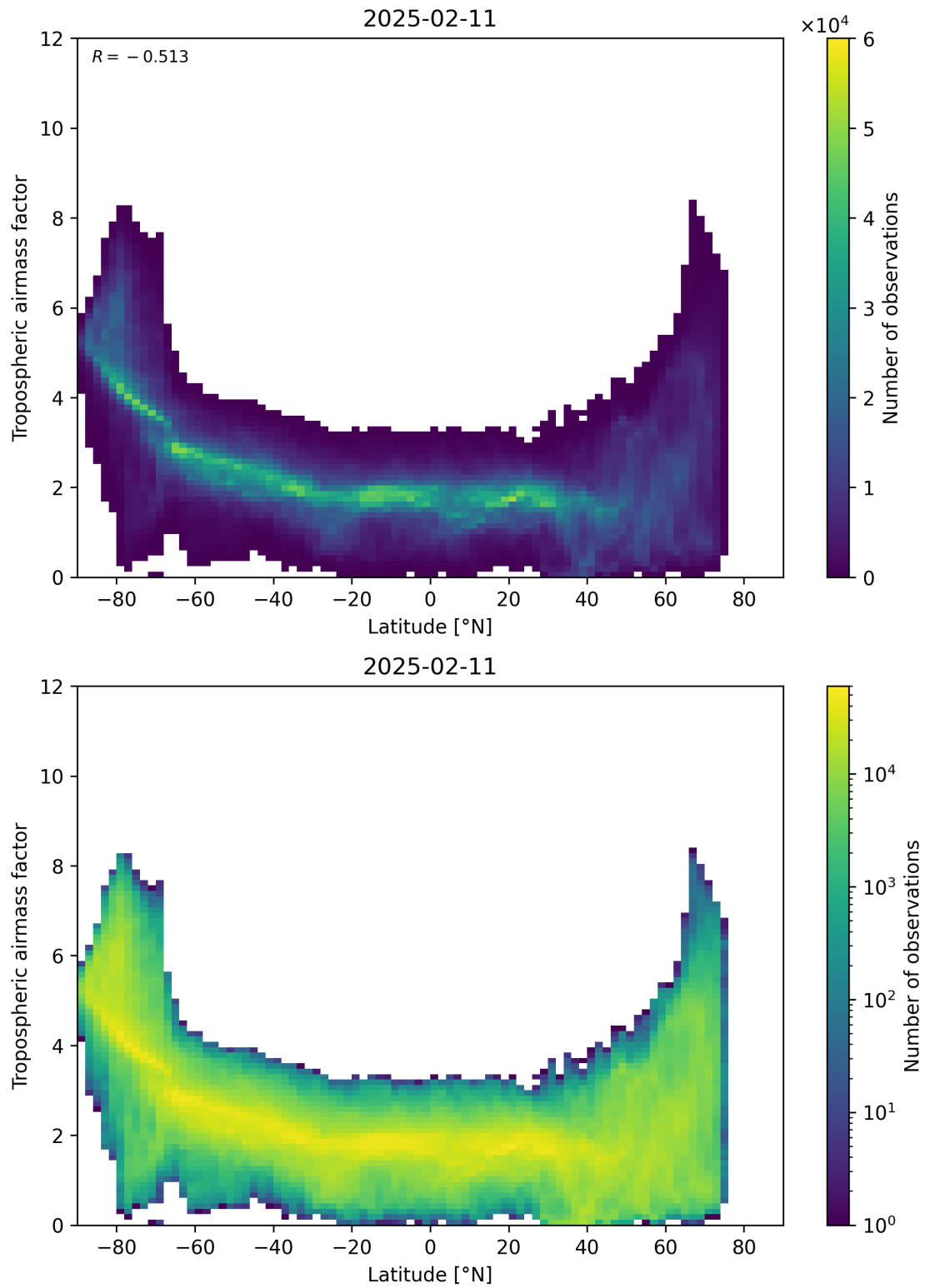
Figure 85: Scatter density plot of “Latitude” against “Tropospheric airmass factor” for 2025-02-10 to 2025-02-12.
