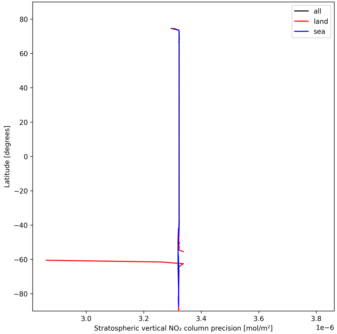
Figure 20: Zonal average of “Stratospheric vertical NO 2 column precision” for 2025-02-10 to 2025-02-12.
