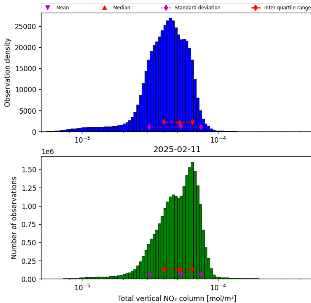
Figure 38: Histogram of “Total vertical NO 2 column” for 2025-02-10 to 2025-02-12
