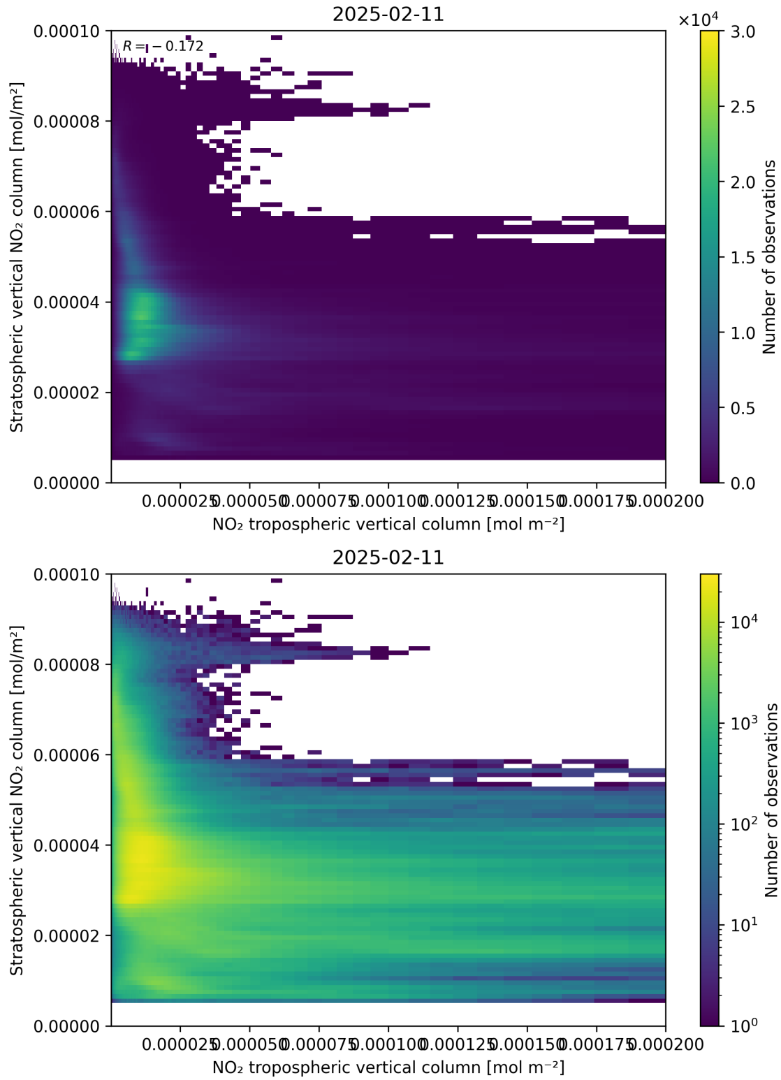
Figure 125: Scatter density plot of “NO 2 tropospheric vertical column” against “Stratospheric vertical NO 2 column” for 2025-02-10 to 2025-02-12.
