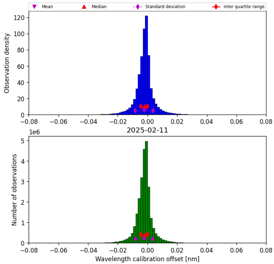
Figure 35: Histogram of “Wavelength calibration offset” for 2025-02-10 to 2025-02-12
