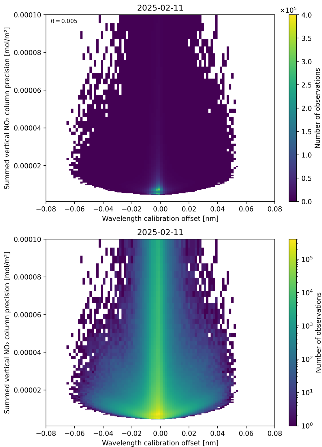
Figure 178: Scatter density plot of “Wavelength calibration offset” against “Summed vertical NO 2 column precision” for 2025-02-10 to 2025-02-12.
