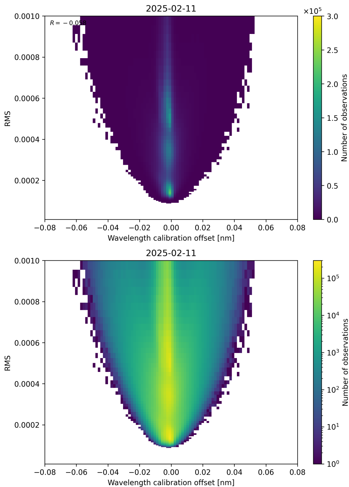
Figure 181: Scatter density plot of “Wavelength calibration offset” against “RMS” for 2025-02-10 to 2025-02-12.
