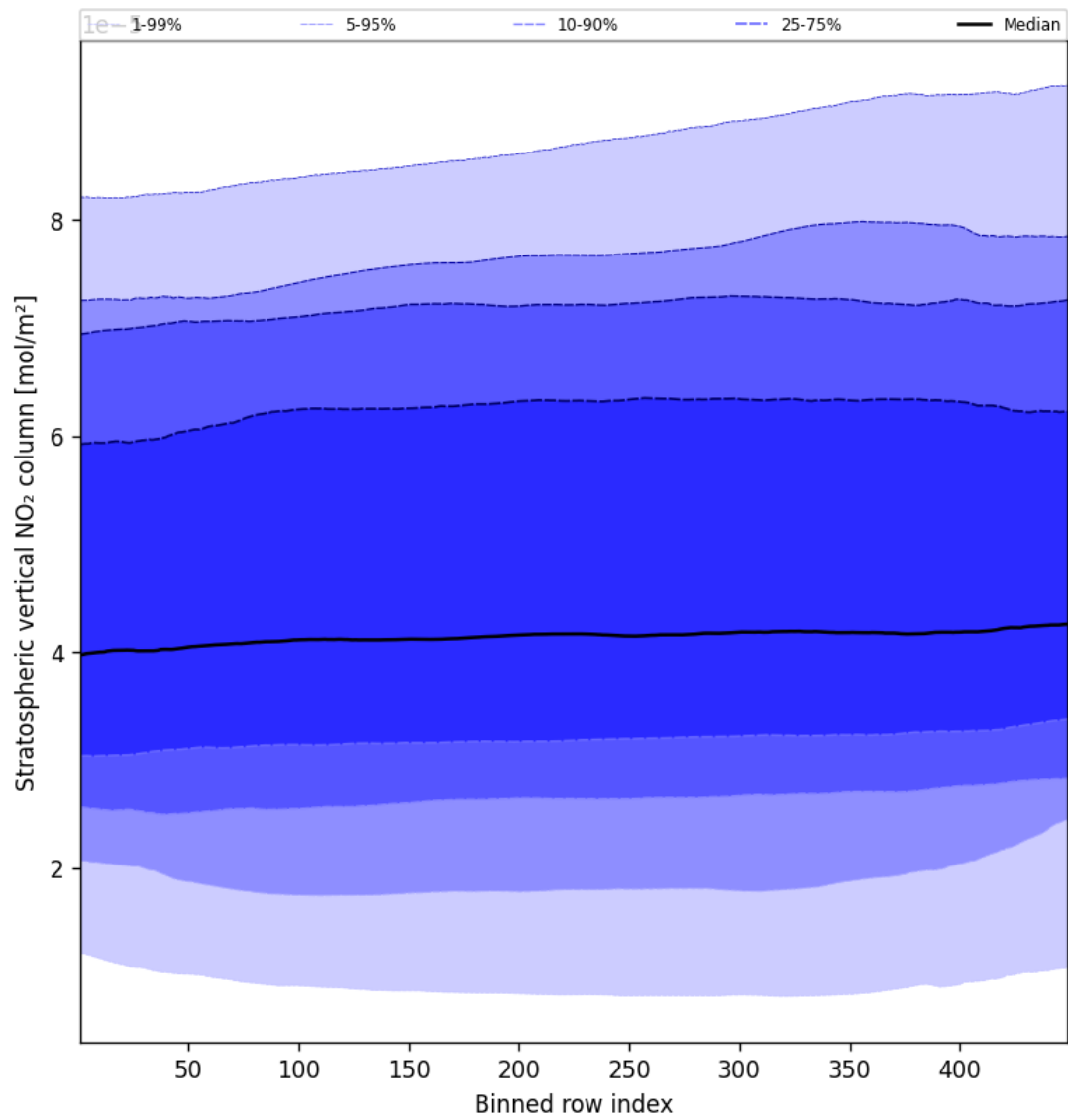
Figure 53: Along track statistics of “Stratospheric vertical NO 2 column” for 2025-02-10 to 2025-02-12
