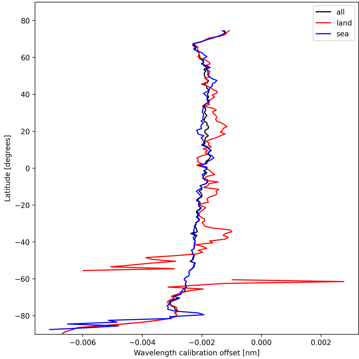
Figure 18: Zonal average of “Wavelength calibration offset” for 2025-02-10 to 2025-02-12.
