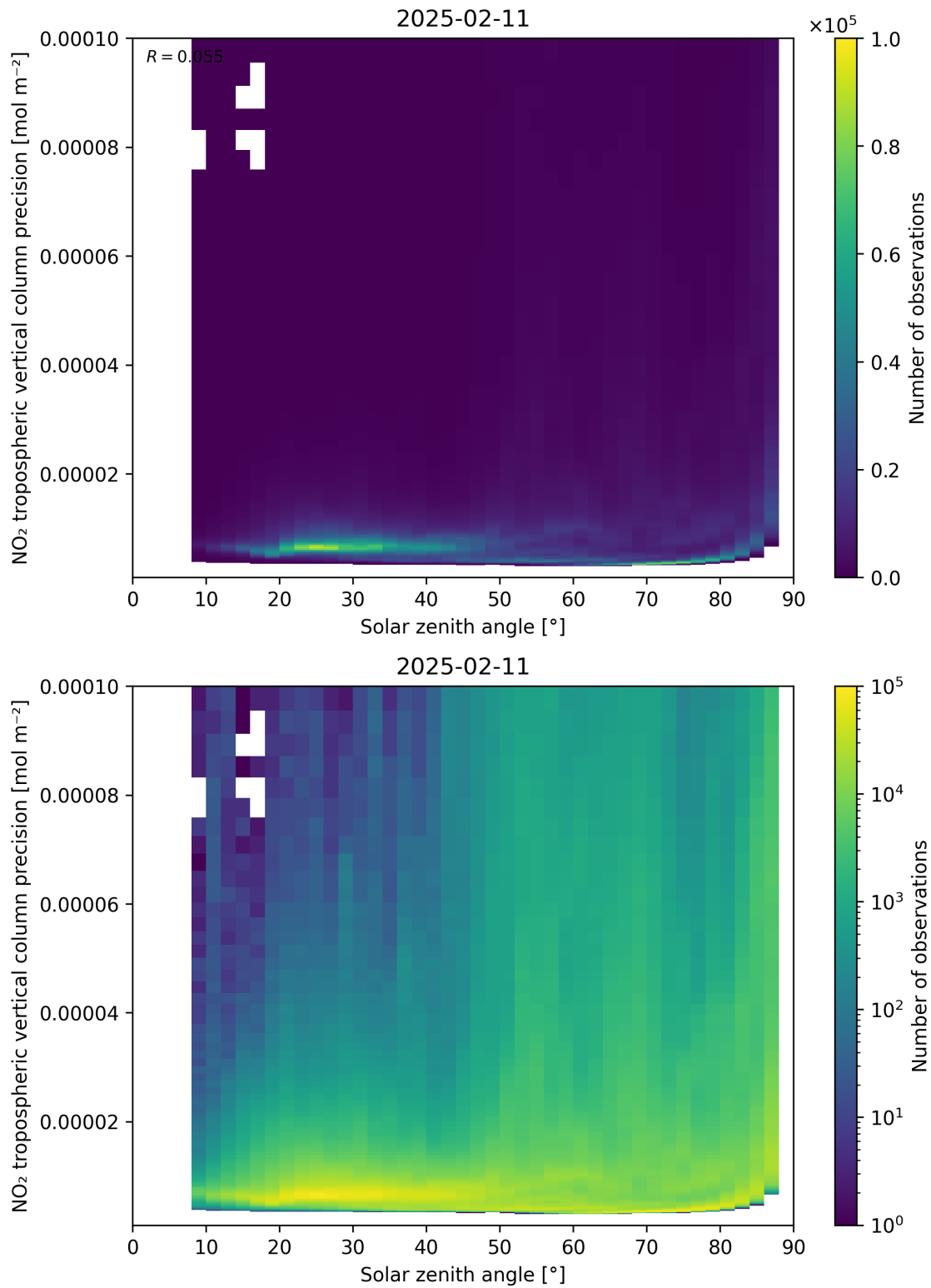
Figure 156: Scatter density plot of “Solar zenith angle” against “NO 2 tropospheric vertical column precision” for 2025-02-10 to 2025-02-12.
