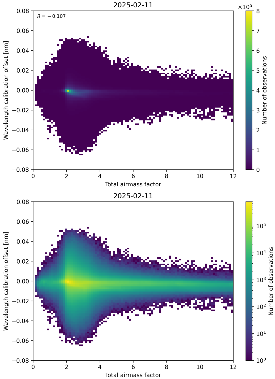
Figure 70: Scatter density plot of “Total airmass factor” against “Wavelength calibration offset” for 2025-02-10 to 2025-02-12.
