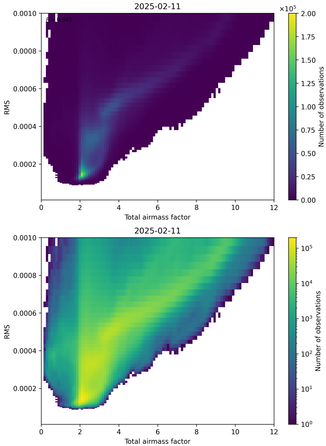
Figure 69: Scatter density plot of “Total airmass factor” against “RMS” for 2025-02-10 to 2025-02-12.
