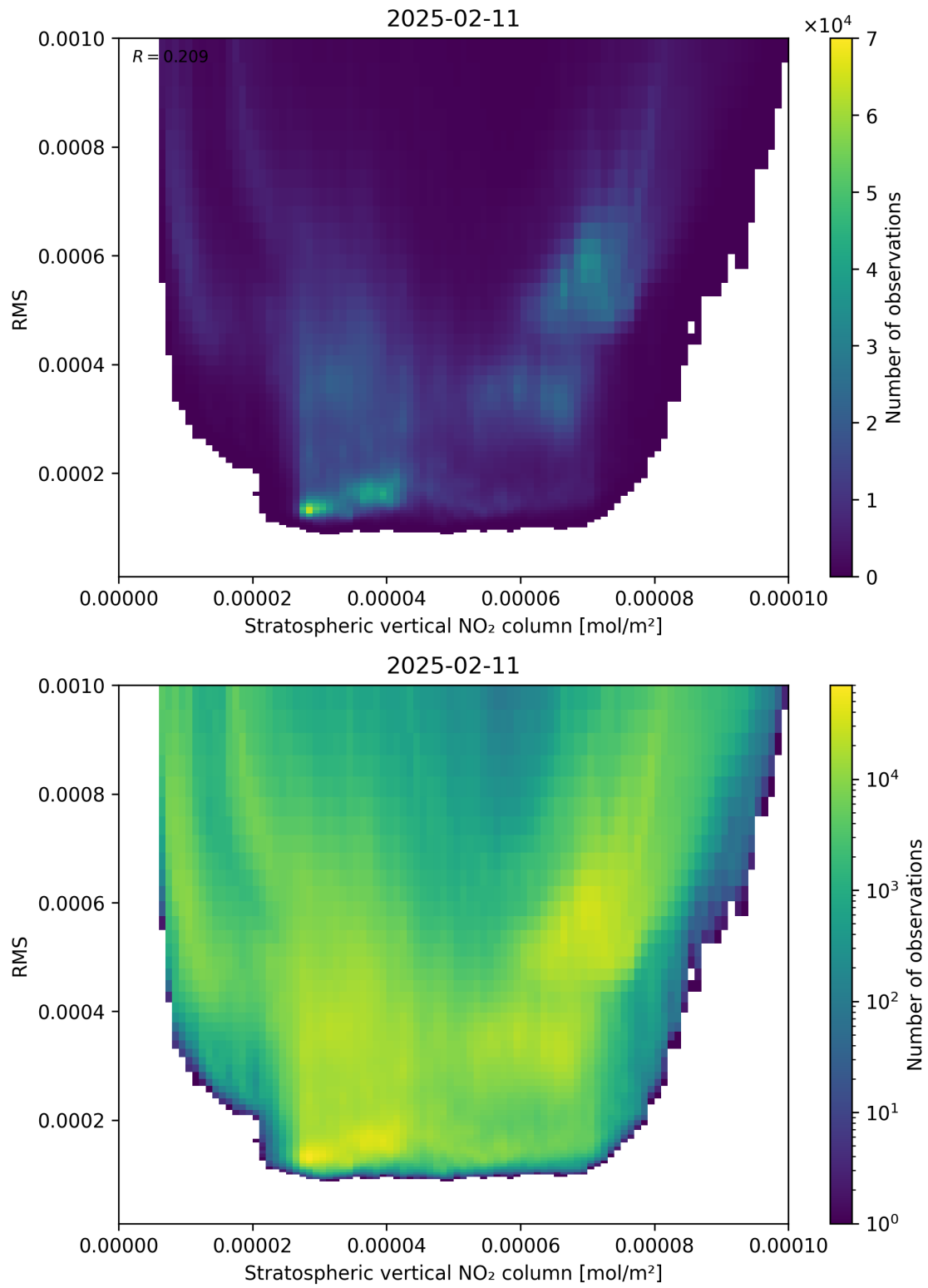
Figure 102: Scatter density plot of “Stratospheric vertical NO 2 column” against “RMS” for 2025-02-10 to 2025-02-12.
