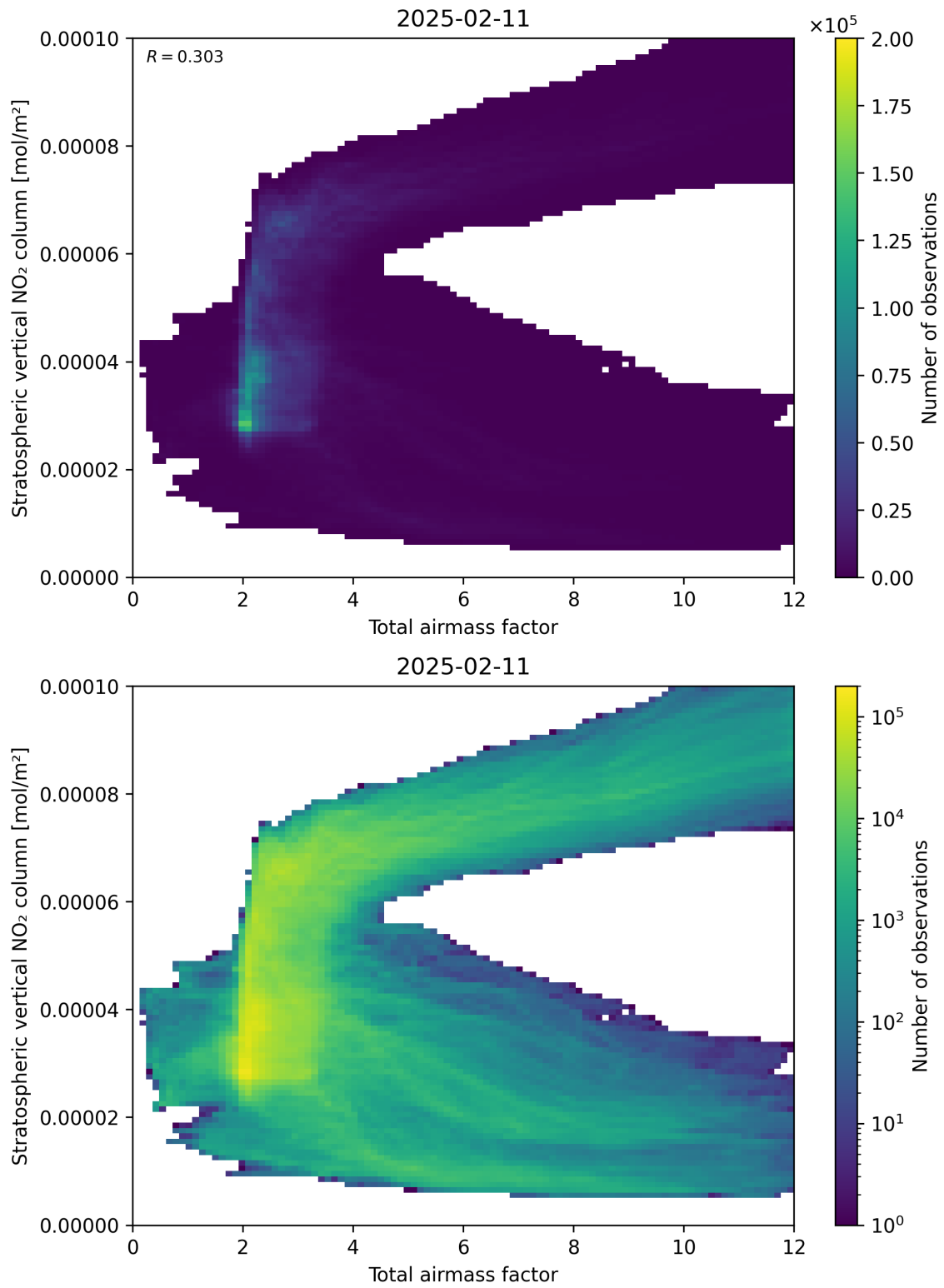
Figure 64: Scatter density plot of “Total airmass factor” against “Stratospheric vertical NO 2 column” for 2025-02-10 to 2025-02-12.
