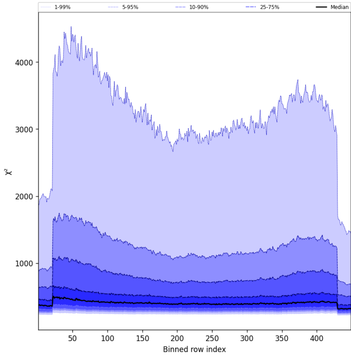
Figure 59: Along track statistics of “ \chi^2 ” for 2025-02-10 to 2025-02-12
