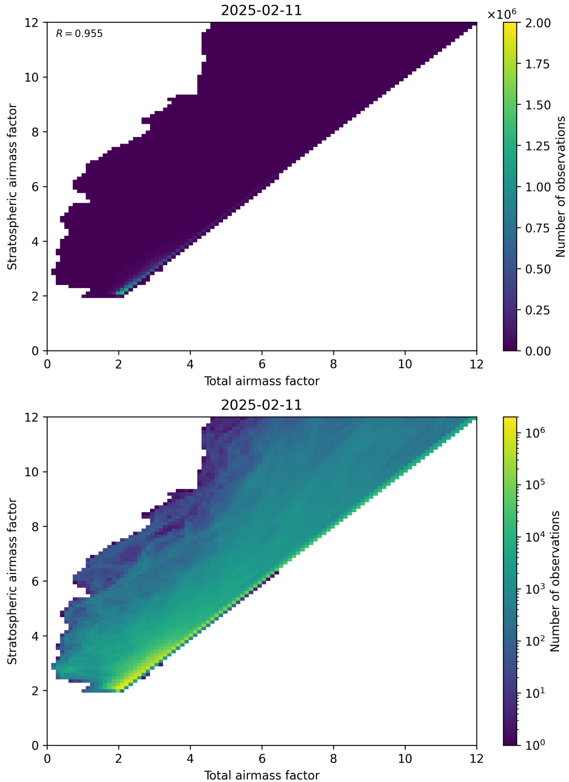
Figure 62: Scatter density plot of “Total airmass factor” against “Stratospheric airmass factor” for 2025-02-10 to 2025-02-12.
