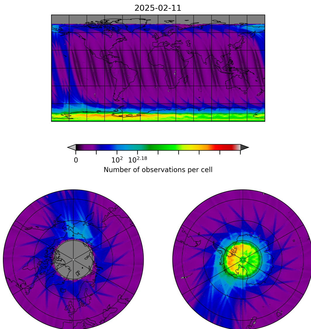
Figure 10: Map of the number of observations for 2025-02-10 to 2025-02-12
