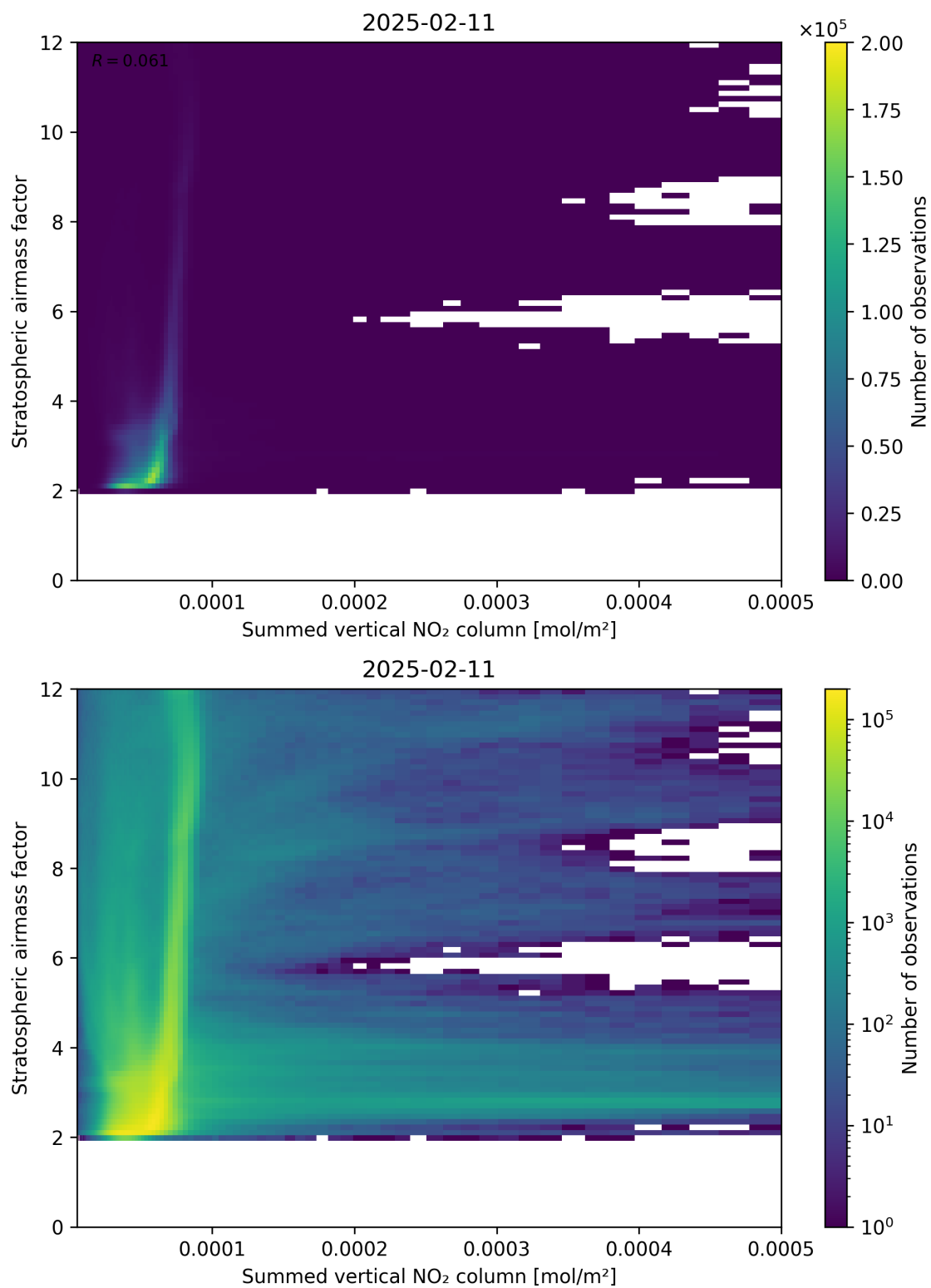
Figure 103: Scatter density plot of “Summed vertical NO 2 column” against “Stratospheric airmass factor” for 2025-02-10 to 2025-02-12.
