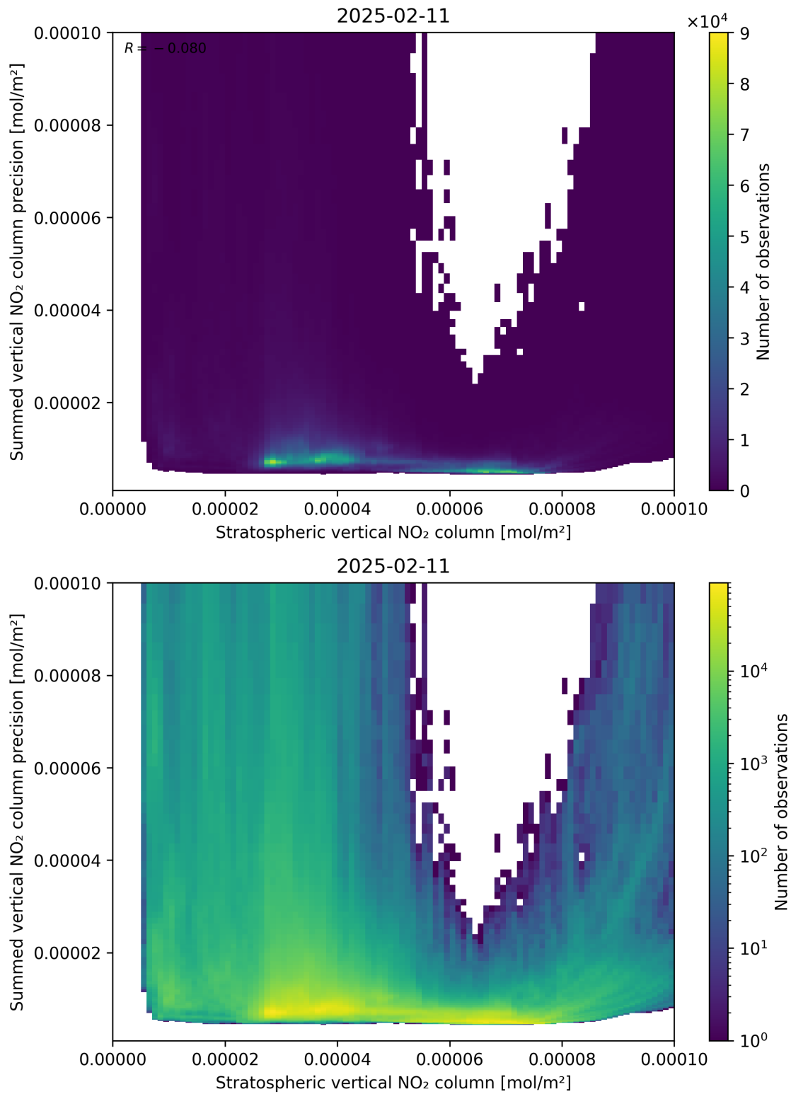
Figure 99: Scatter density plot of “Stratospheric vertical NO 2 column” against “Summed vertical NO 2 column precision” for 2025-02-10 to 2025-02-12.
