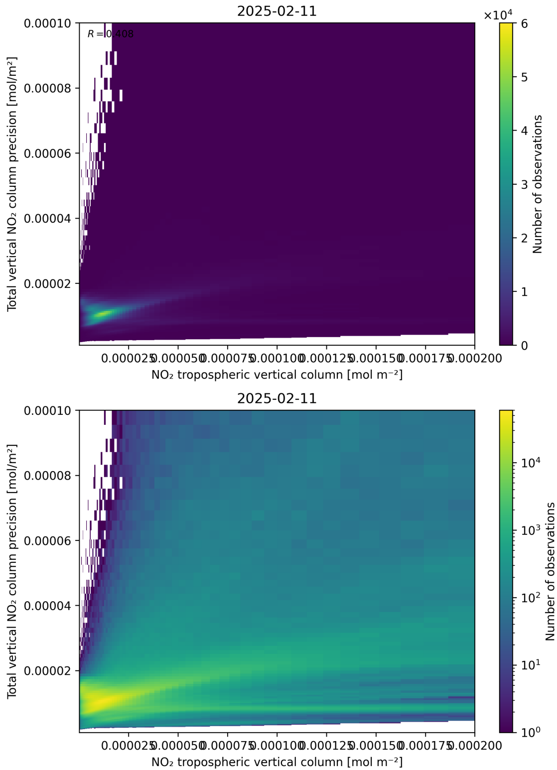
Figure 129: Scatter density plot of “NO 2 tropospheric vertical column” against “Total vertical NO 2 column precision” for 2025-02-10 to 2025-02-12.
