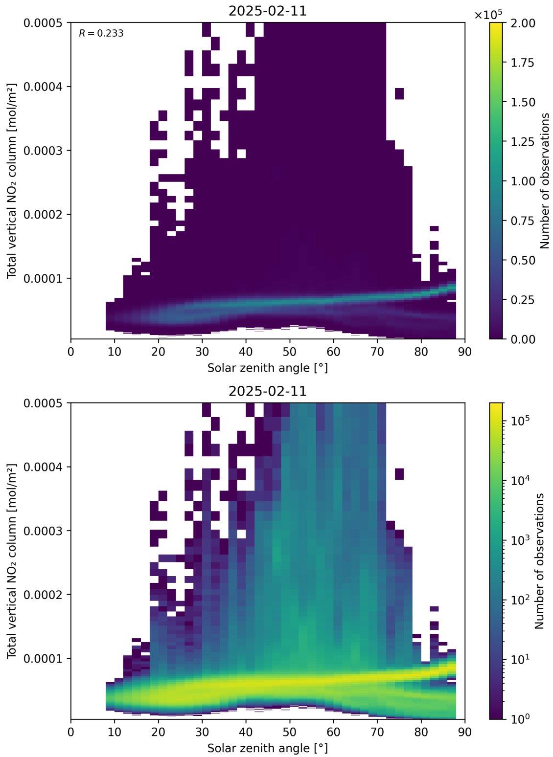
Figure 153: Scatter density plot of “Solar zenith angle” against “Total vertical NO 2 column” for 2025-02-10 to 2025-02-12.
