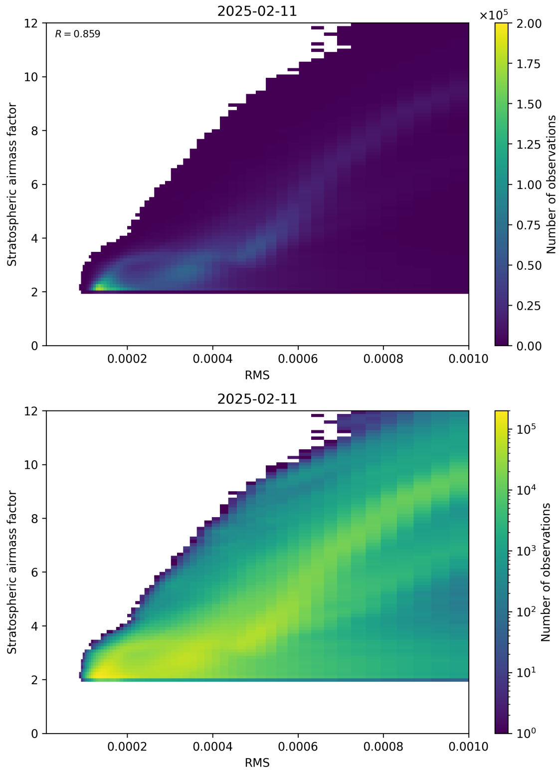
Figure 144: Scatter density plot of “RMS” against “Stratospheric airmass factor” for 2025-02-10 to 2025-02-12.
