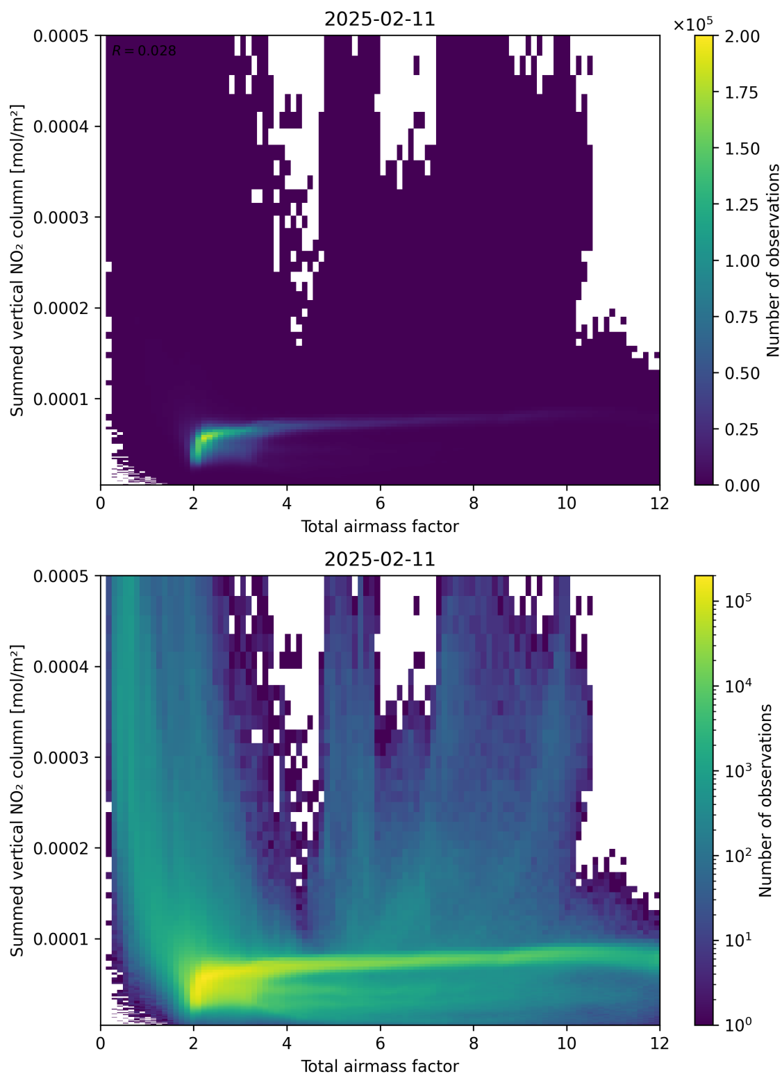
Figure 65: Scatter density plot of “Total airmass factor” against “Summed vertical NO 2 column” for 2025-02-10 to 2025-02-12.
