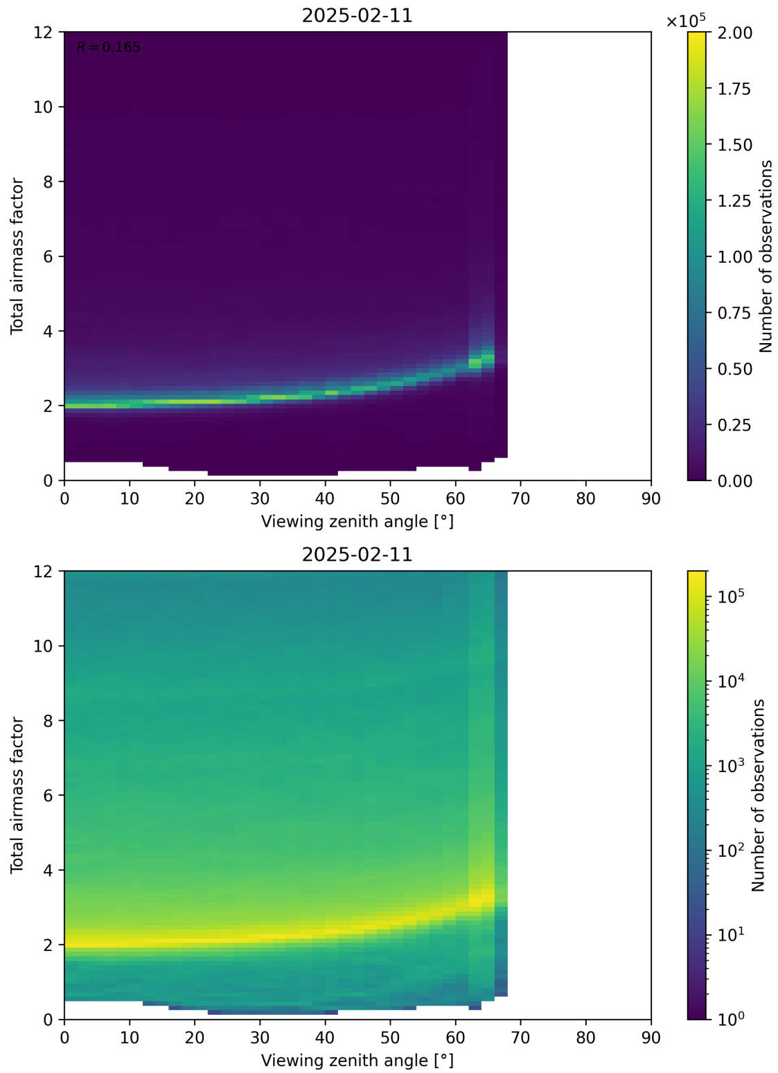
Figure 160: Scatter density plot of “Viewing zenith angle” against “Total airmass factor” for 2025-02-10 to 2025-02-12.
