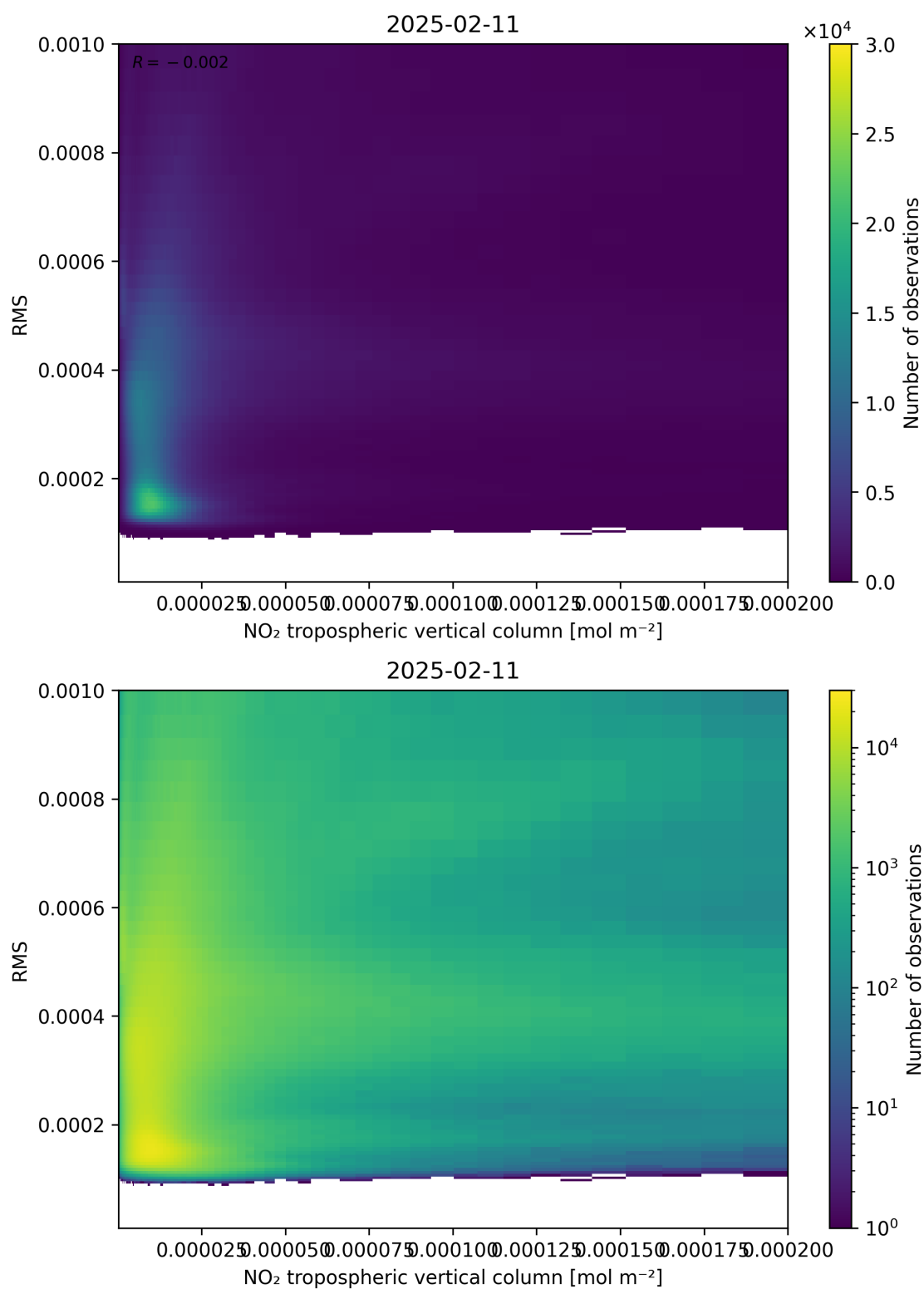
Figure 142: Scatter density plot of “NO 2 tropospheric vertical column” against “RMS” for 2025-02-10 to 2025-02-12.
