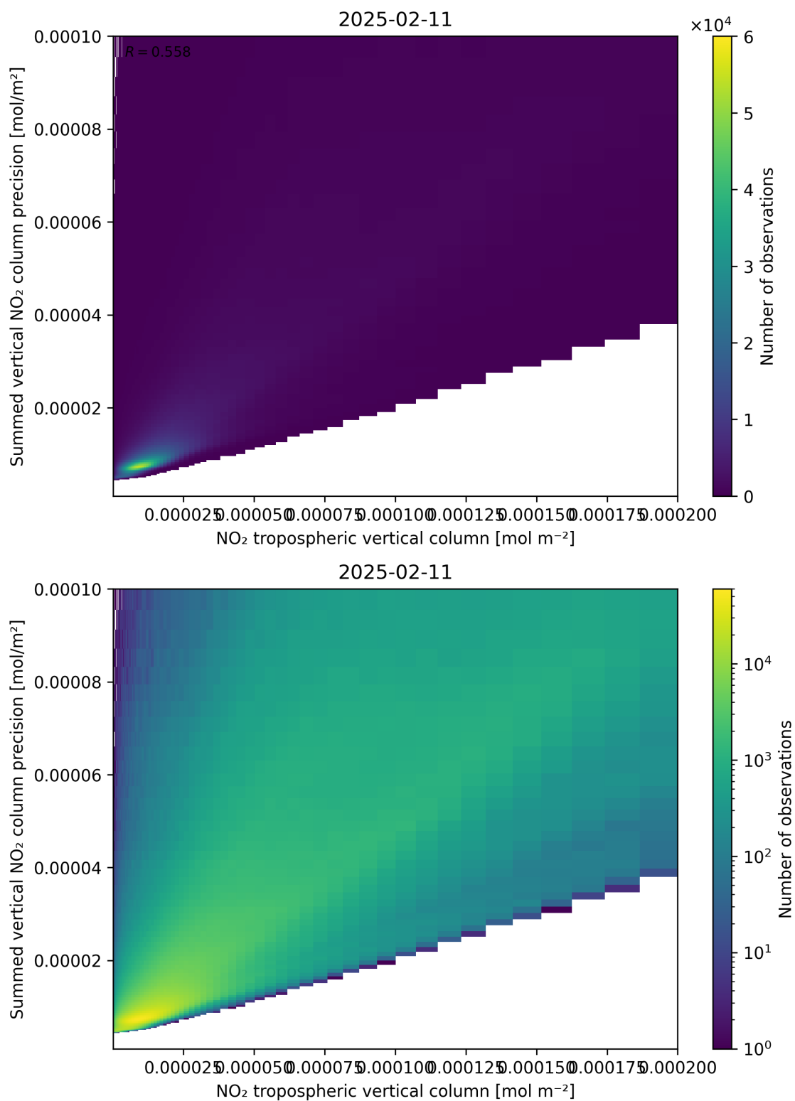
Figure 127: Scatter density plot of “NO 2 tropospheric vertical column” against “Summed vertical NO 2 column precision” for 2025-02-10 to 2025-02-12.
