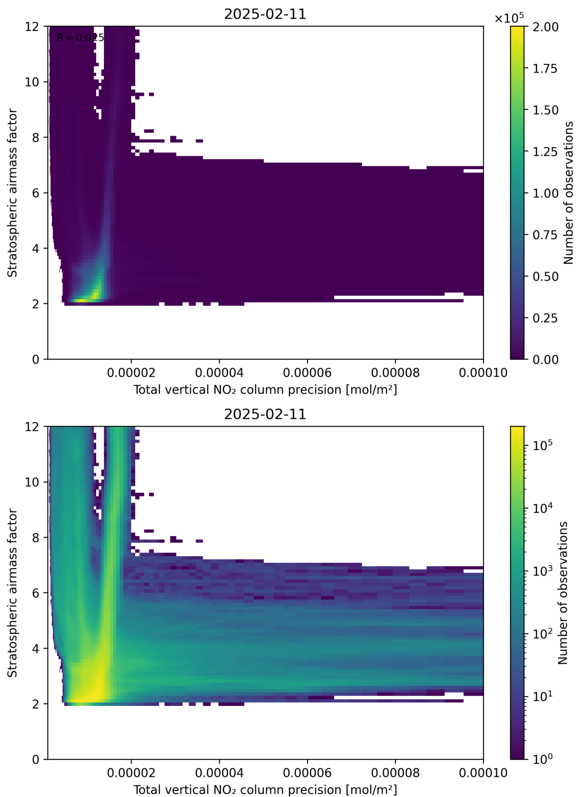
Figure 115: Scatter density plot of “Total vertical NO 2 column precision” against “Stratospheric air mass factor” for 2025-02-10 to 2025-02-12.
