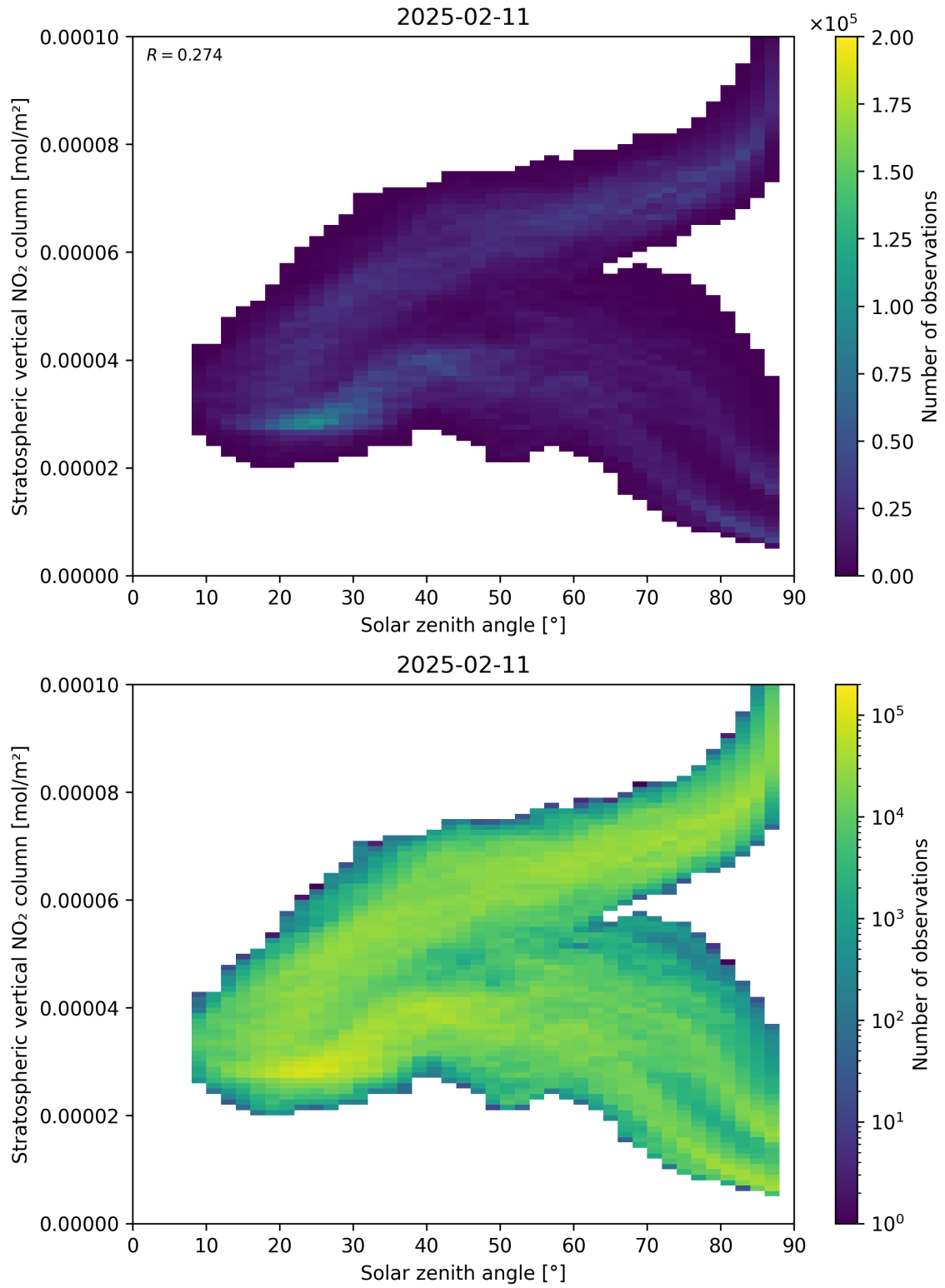
Figure 150: Scatter density plot of “Solar zenith angle” against “Stratospheric vertical NO 2 column” for 2025-02-10 to 2025-02-12.
