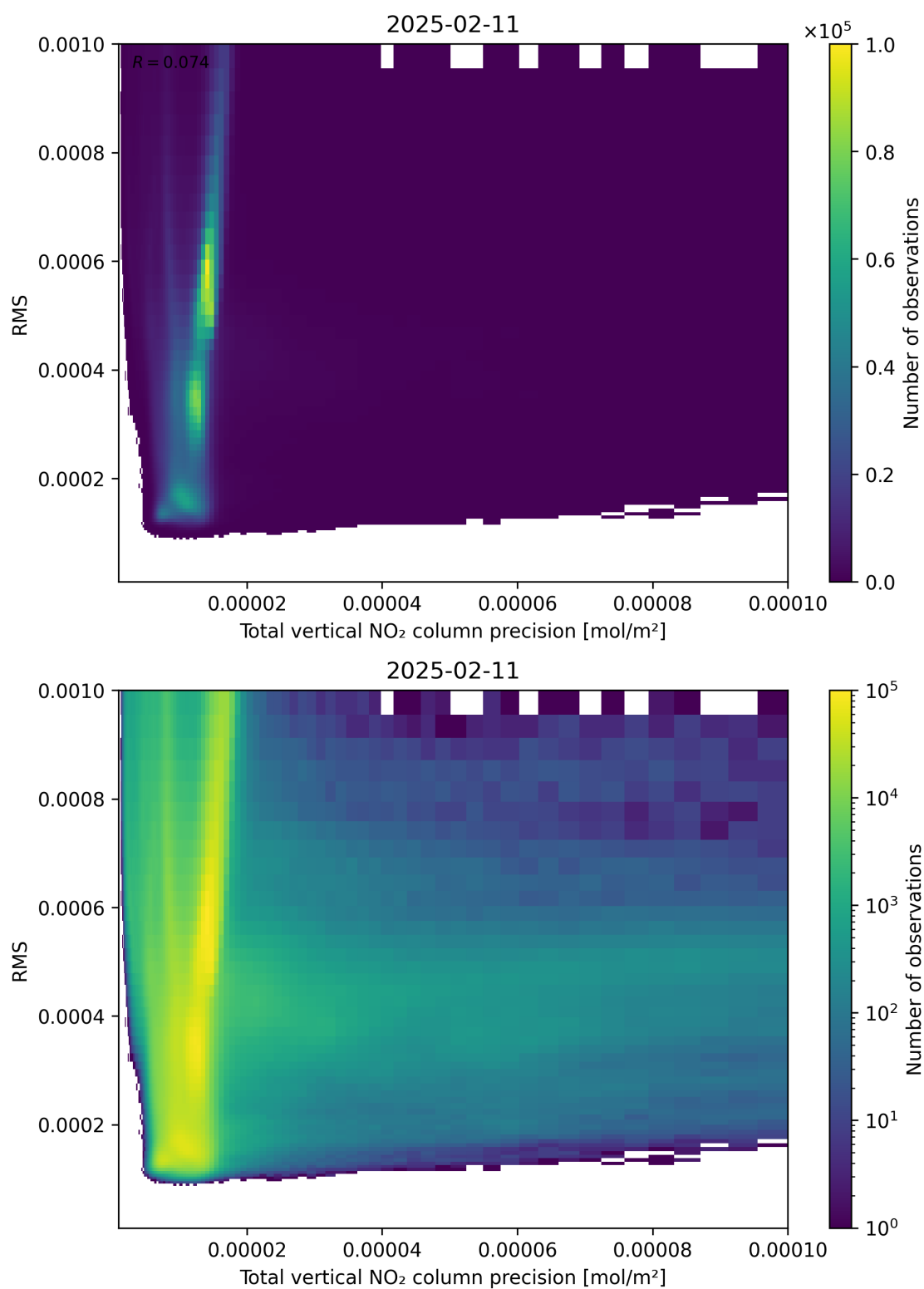
Figure 119: Scatter density plot of “Total vertical NO 2 column precision” against “RMS” for 2025-02-10 to 2025-02-12.
