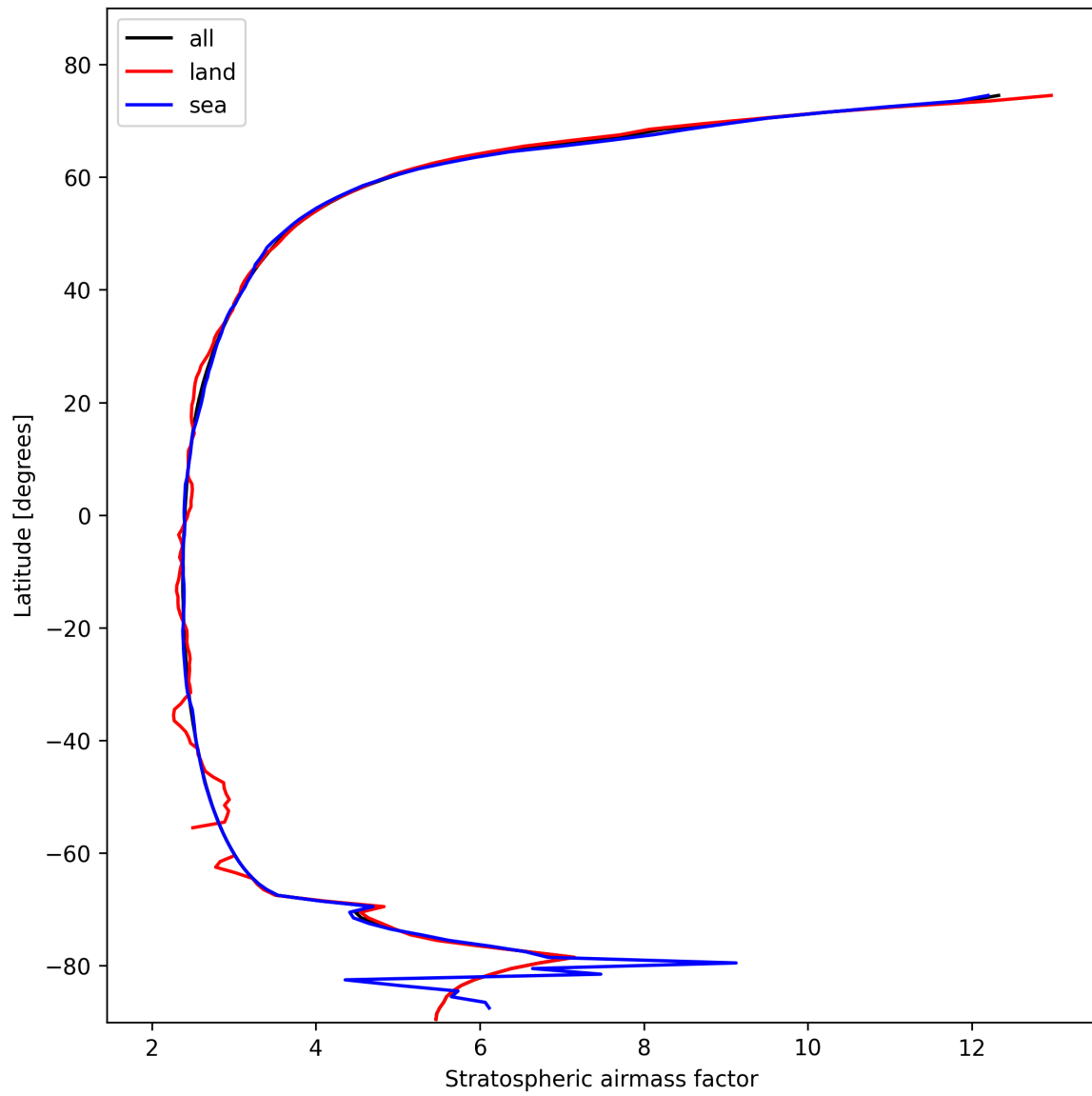
Figure 27: Zonal average of “Stratospheric airmass factor” for 2025-02-10 to 2025-02-12.
