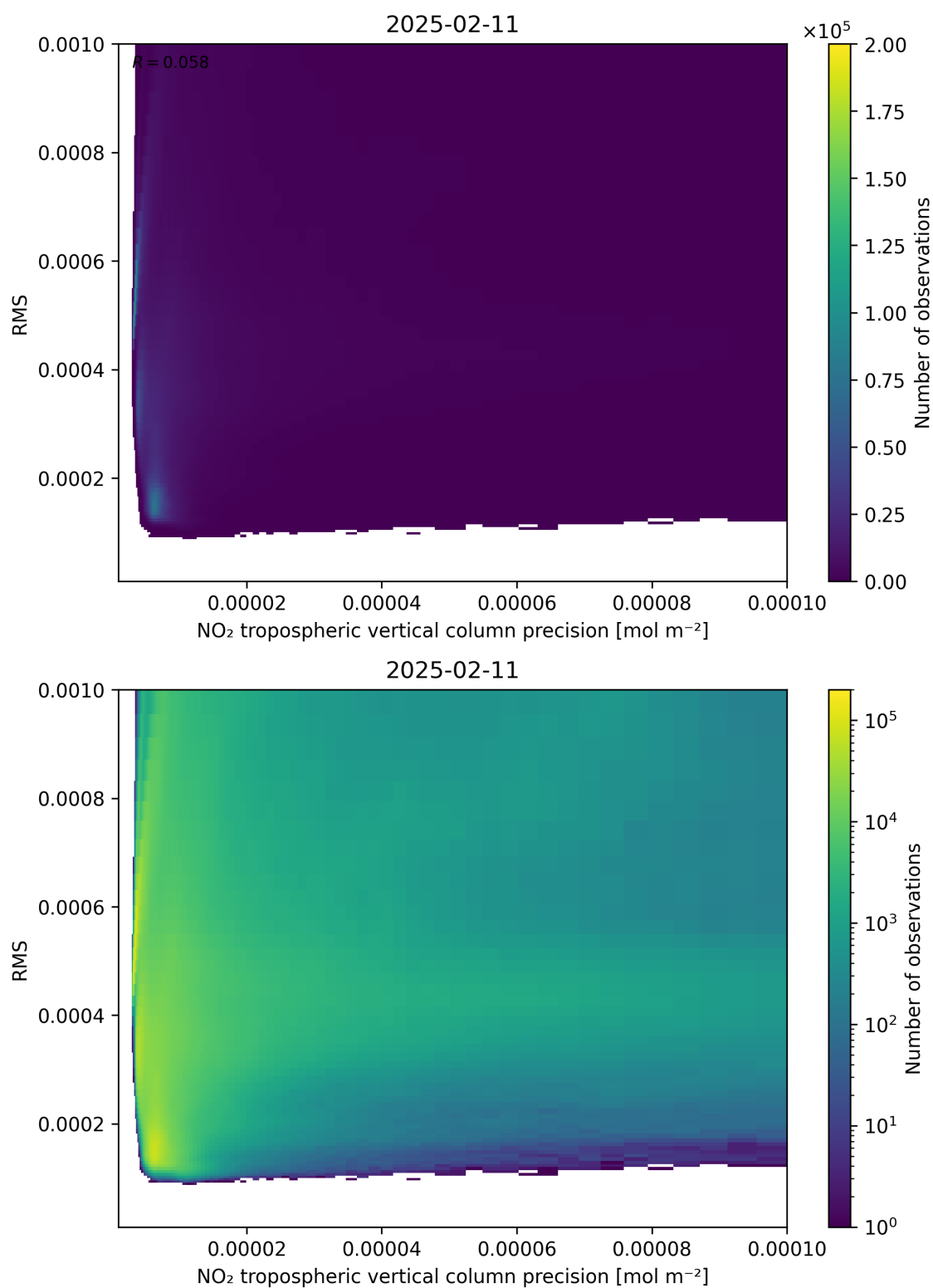
Figure 140: Scatter density plot of “NO 2 tropospheric vertical column precision” against “RMS” for 2025-02-10 to 2025-02-12.
