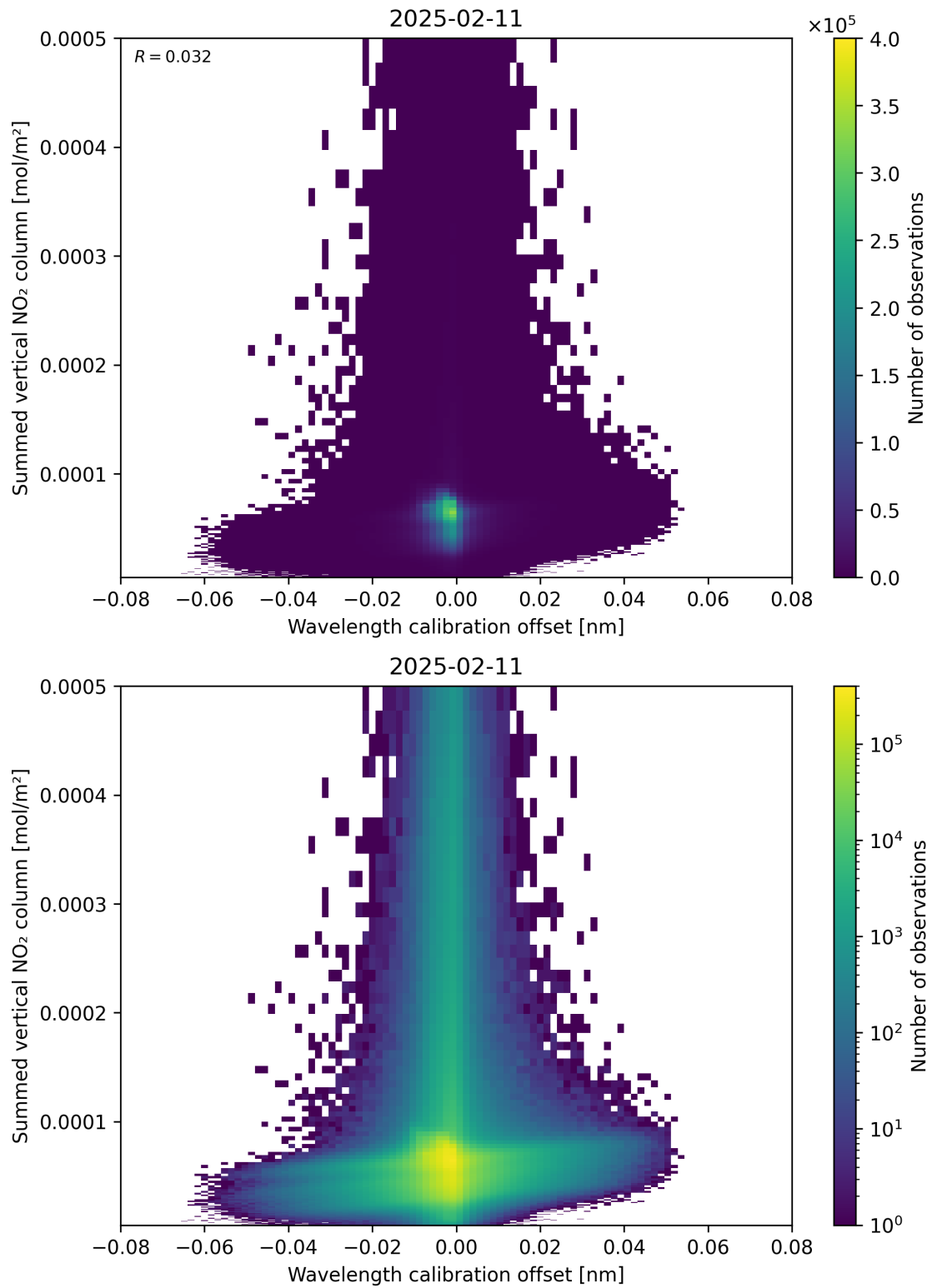
Figure 177: Scatter density plot of “Wavelength calibration offset” against “Summed vertical NO 2 column” for 2025-02-10 to 2025-02-12.
