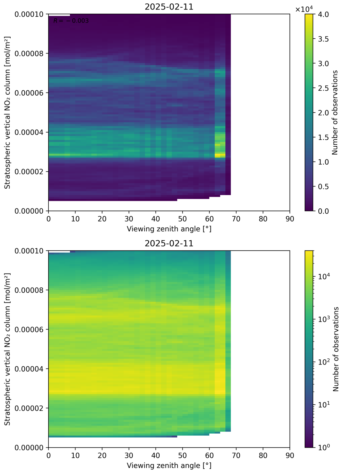
Figure 164: Scatter density plot of “Viewing zenith angle” against “Stratospheric vertical NO 2 column” for 2025-02-10 to 2025-02-12.
