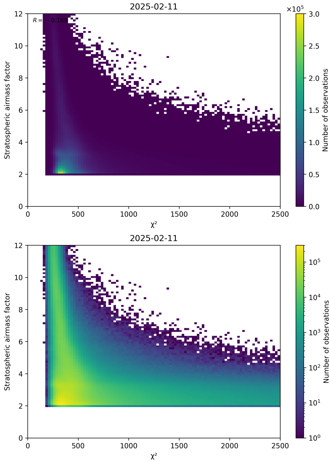
Figure 81: Scatter density plot of “ \chi^2 ” against “Stratospheric airmass factor” for 2025-02-10 to 2025-02-12.
