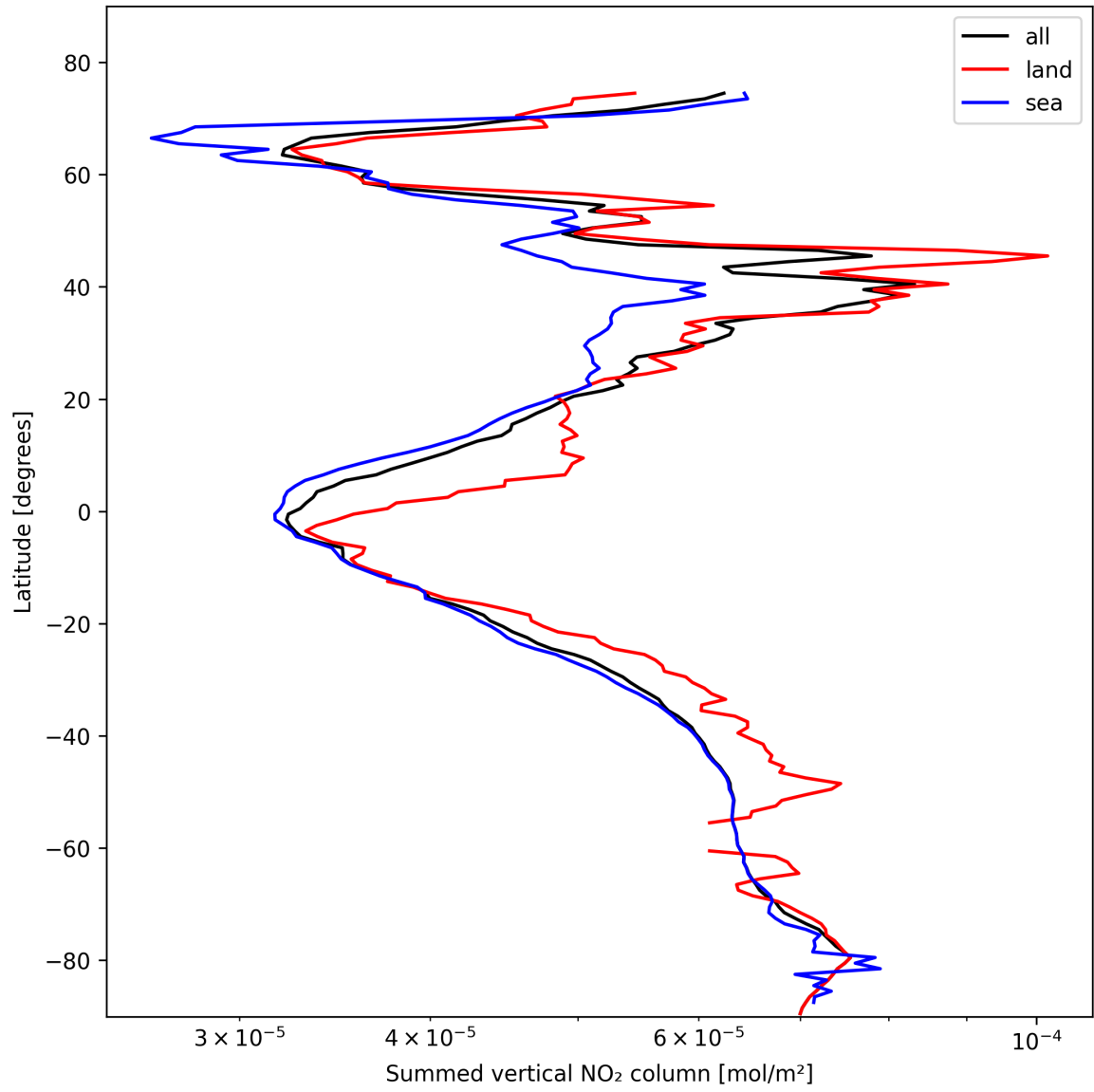
Figure 23: Zonal average of “Summed vertical NO 2 column” for 2025-02-10 to 2025-02-12.
