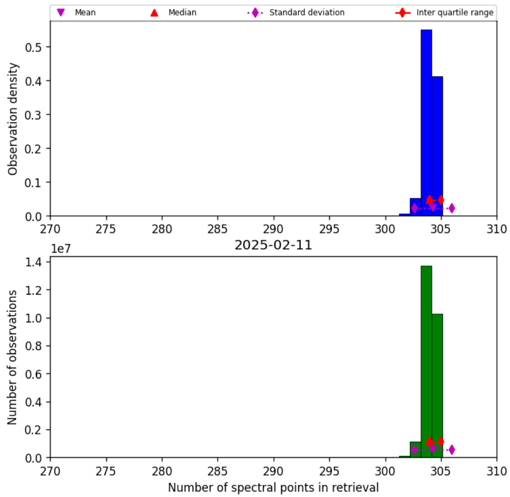
Figure 33: Histogram of “Number of spectral points in retrieval” for 2025-02-10 to 2025-02-12
