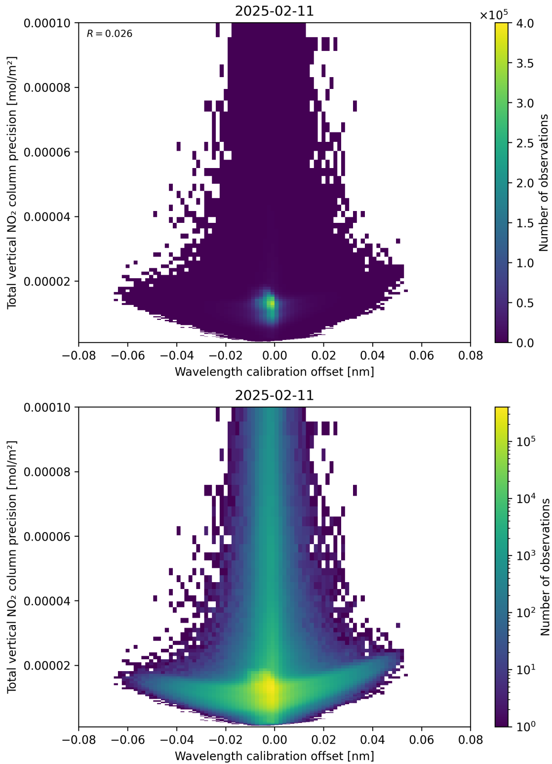
Figure 180: Scatter density plot of “Wavelength calibration offset” against “Total vertical NO 2 column precision” for 2025-02-10 to 2025-02-12.
