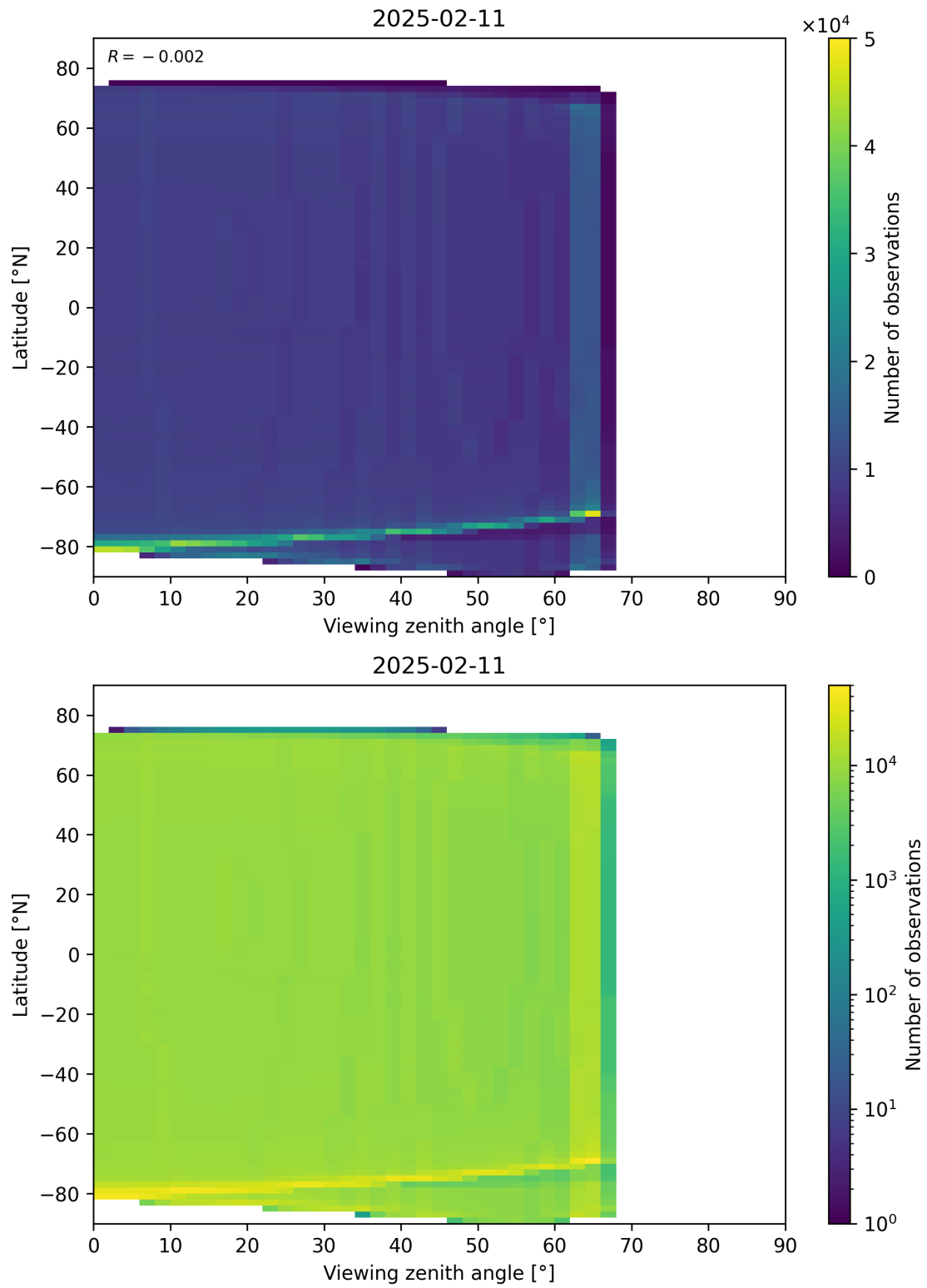
Figure 163: Scatter density plot of “Viewing zenith angle” against “Latitude” for 2025-02-10 to 2025-02-12.
