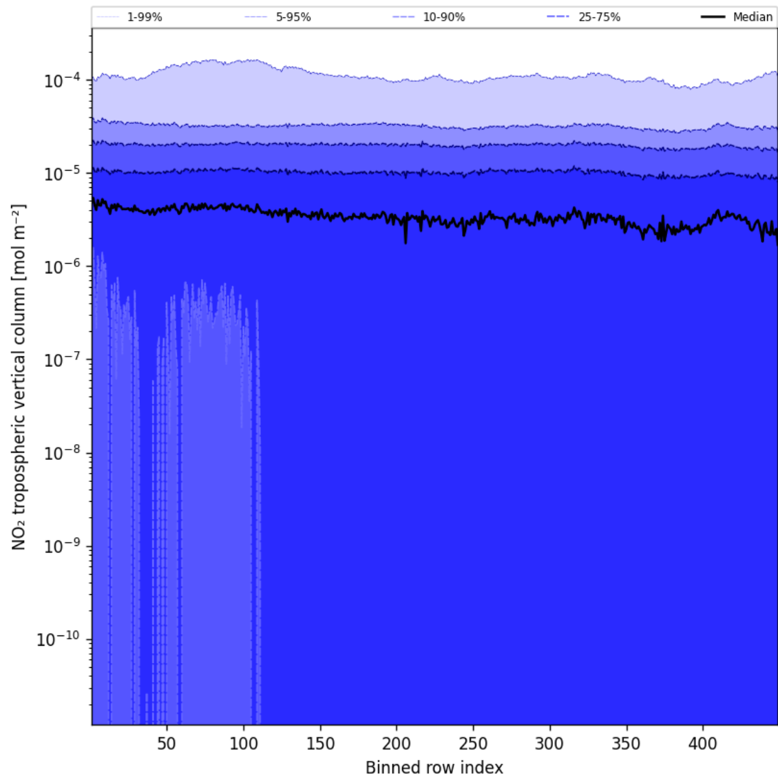
Figure 46: Along track statistics of “NO 2 tropospheric vertical column” for 2025-02-10 to 2025-02-12
