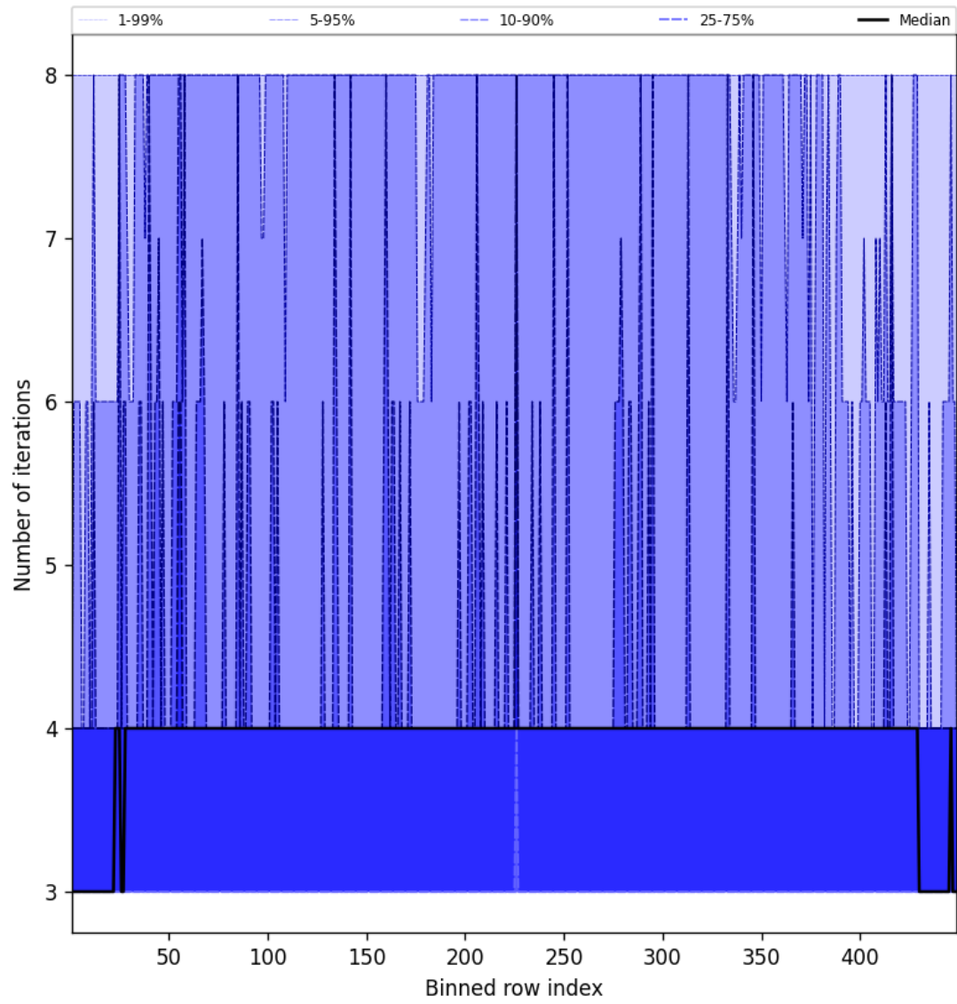
Figure 51: Along track statistics of “Number of iterations” for 2025-02-10 to 2025-02-12
