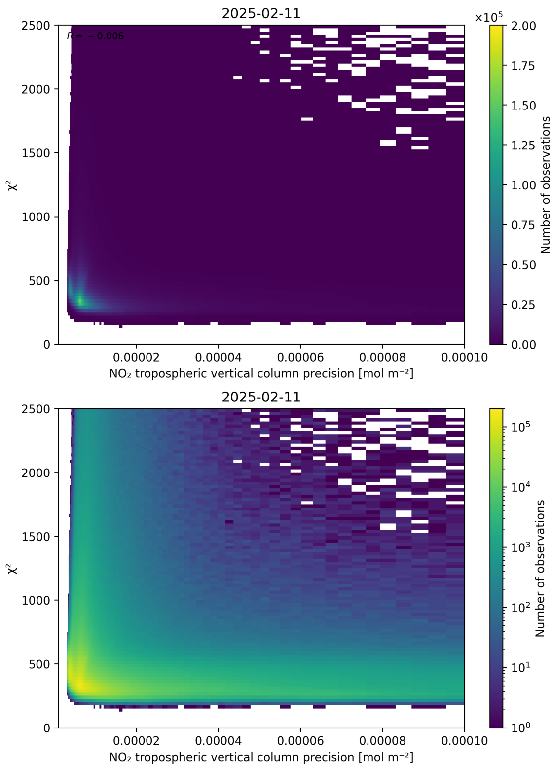
Figure 134: Scatter density plot of “NO 2 tropospheric vertical column precision” against “ \chi^2 ” for 2025-02-10 to 2025-02-12.
