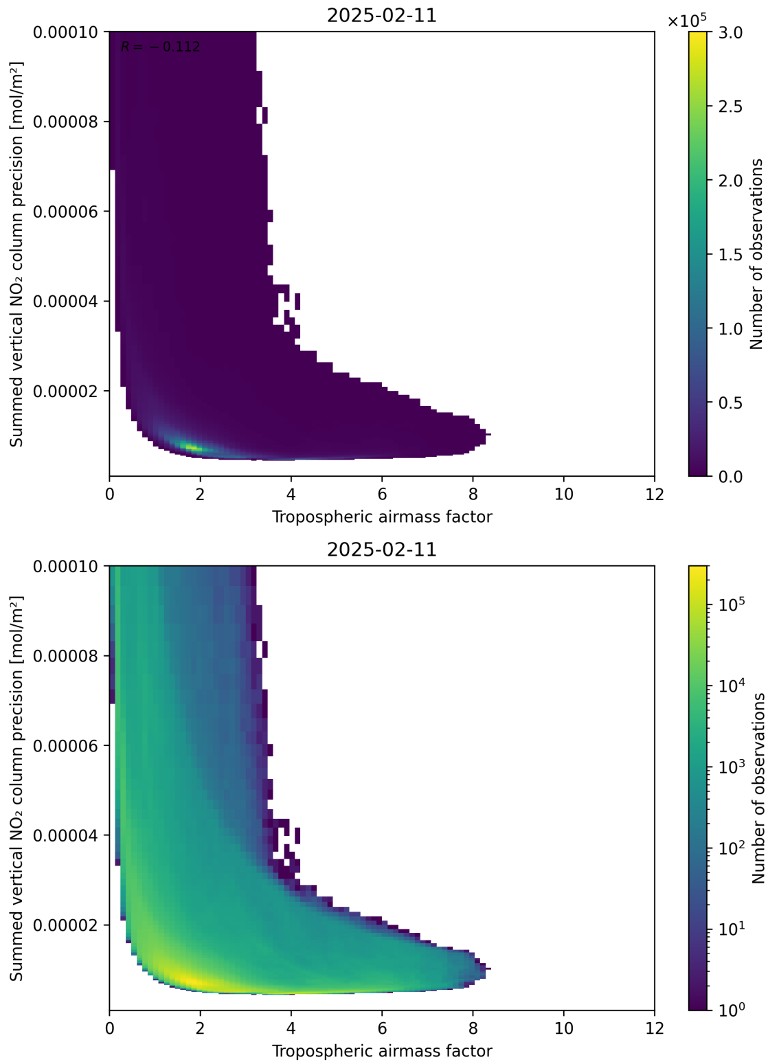
Figure 76: Scatter density plot of “Tropospheric air mass factor” against “Summed vertical NO 2 column precision” for 2025-02-10 to 2025-02-12.
