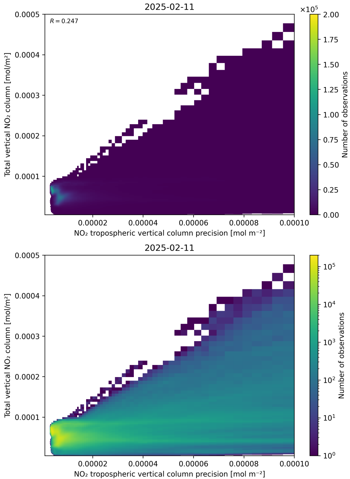
Figure 138: Scatter density plot of “NO 2 tropospheric vertical column precision” against “Total vertical NO 2 column” for 2025-02-10 to 2025-02-12.
