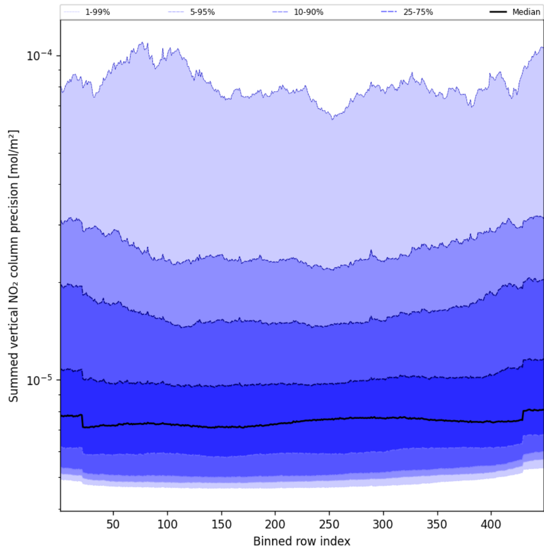
Figure 58: Along track statistics of “Summed vertical NO 2 column precision” for 2025-02-10 to 2025-02-12
