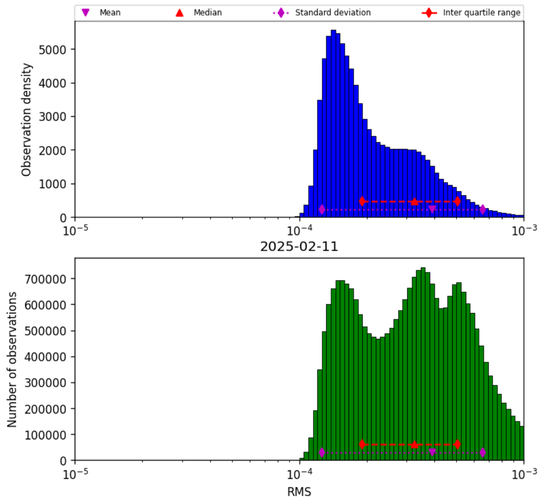
Figure 43: Histogram of “RMS” for 2025-02-10 to 2025-02-12
