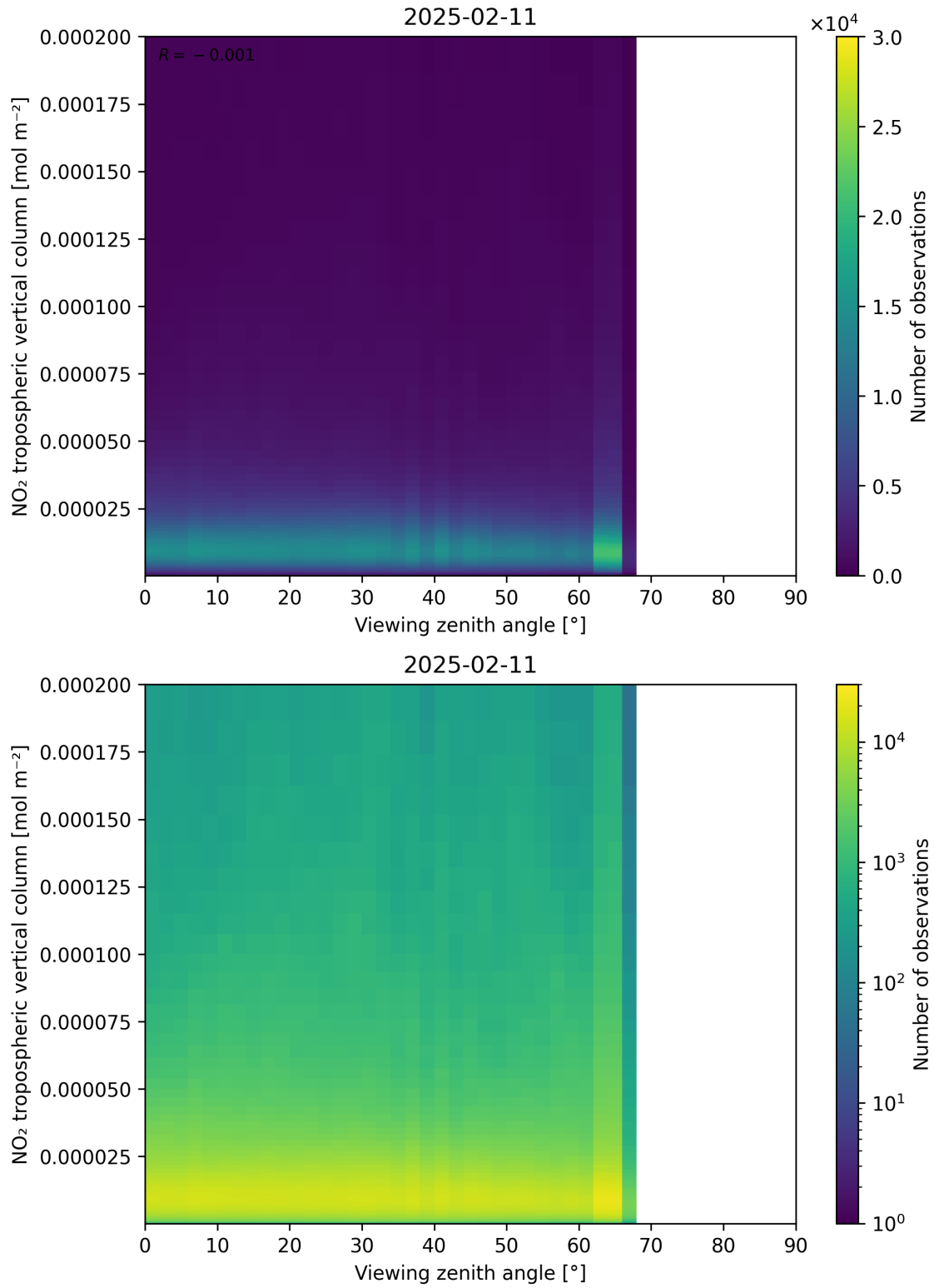
Figure 169: Scatter density plot of “Viewing zenith angle” against “NO 2 tropospheric vertical column” for 2025-02-10 to 2025-02-12.
