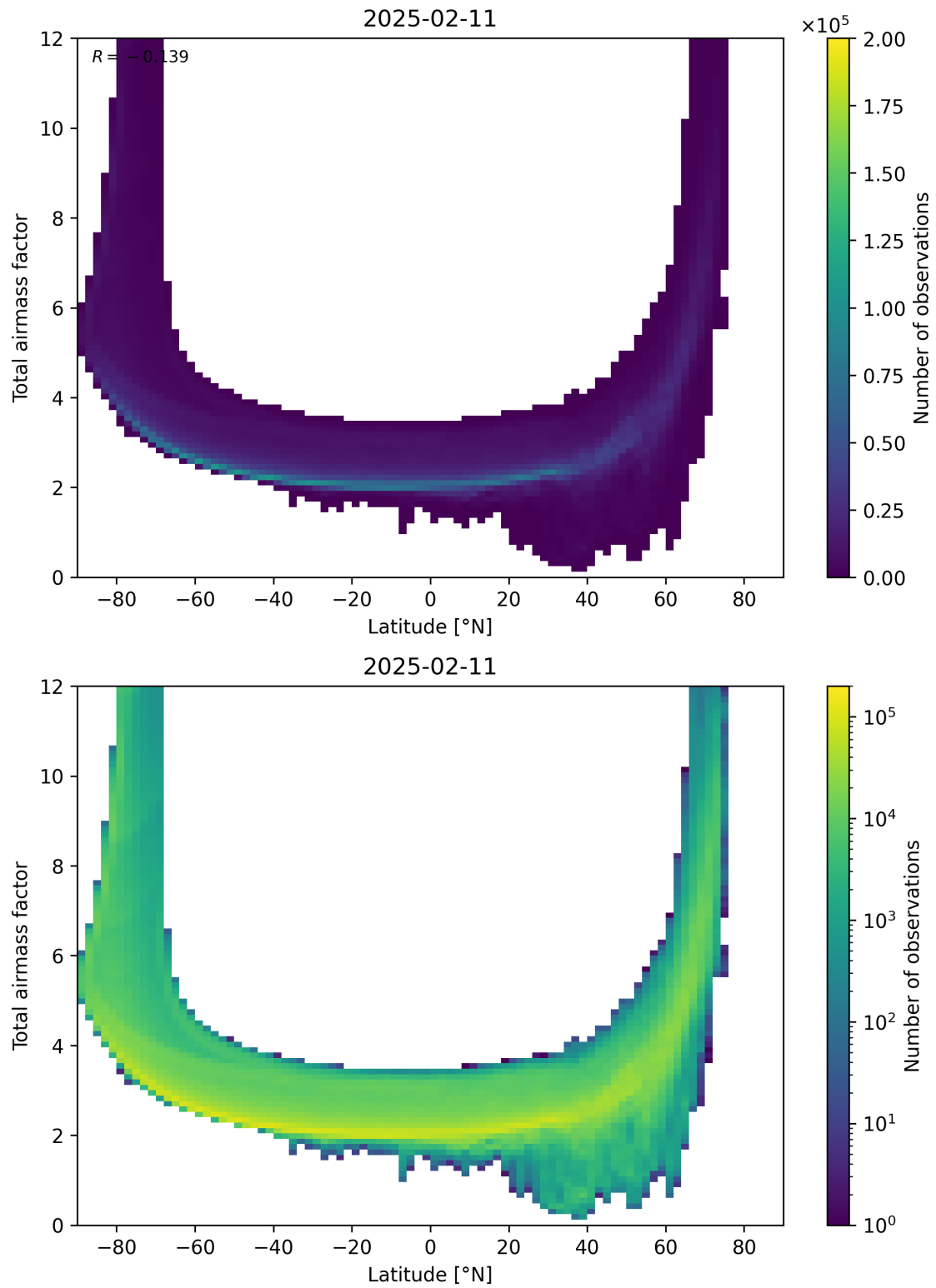
Figure 84: Scatter density plot of “Latitude” against “Total airmass factor” for 2025-02-10 to 2025-02-12.
