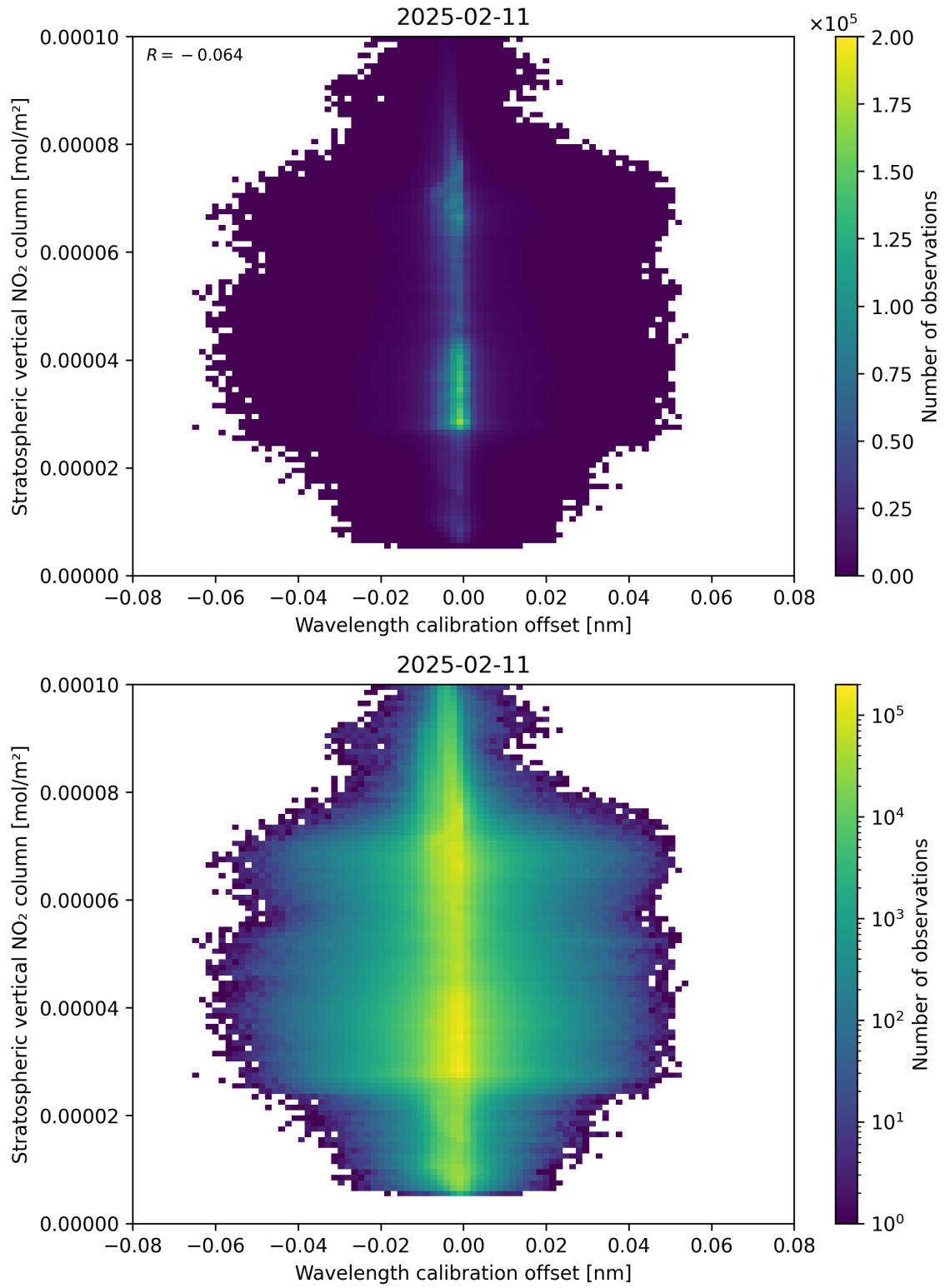
Figure 176: Scatter density plot of “Wavelength calibration offset” against “Stratospheric vertical NO 2 column” for 2025-02-10 to 2025-02-12.
