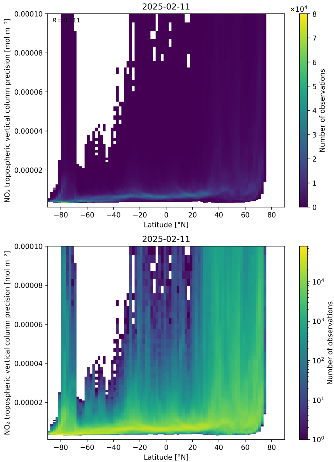
Figure 93: Scatter density plot of “Latitude” against “NO 2 tropospheric vertical column precision” for 2025-02-10 to 2025-02-12.
