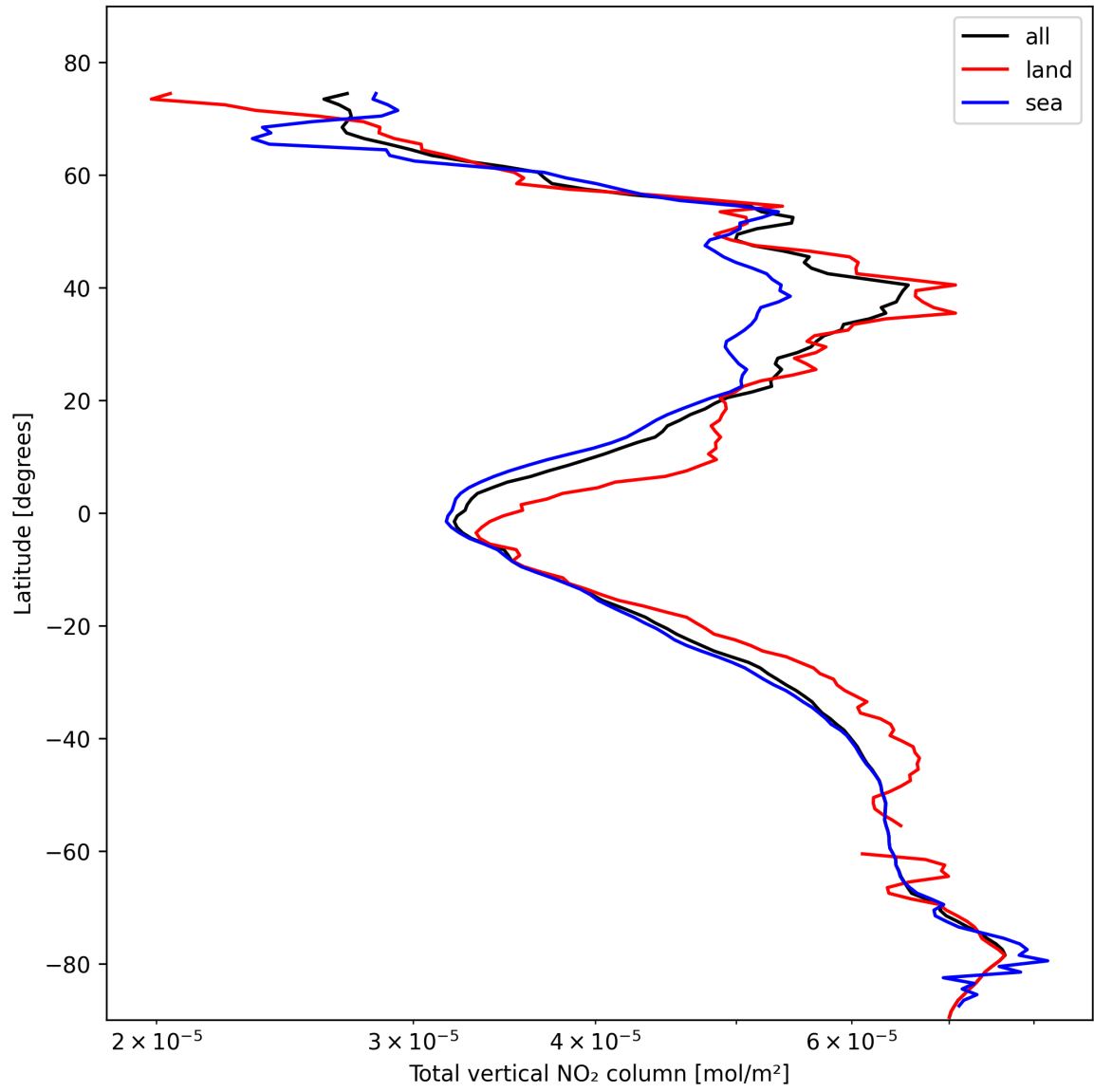
Figure 21: Zonal average of “Total vertical NO 2 column” for 2025-02-10 to 2025-02-12.
