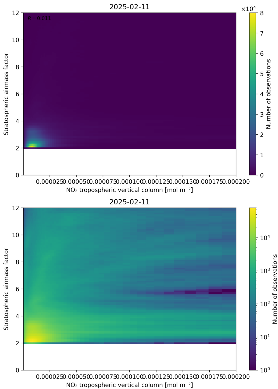
Figure 121: Scatter density plot of “NO 2 tropospheric vertical column” against “Stratospheric airmass factor” for 2025-02-10 to 2025-02-12.
