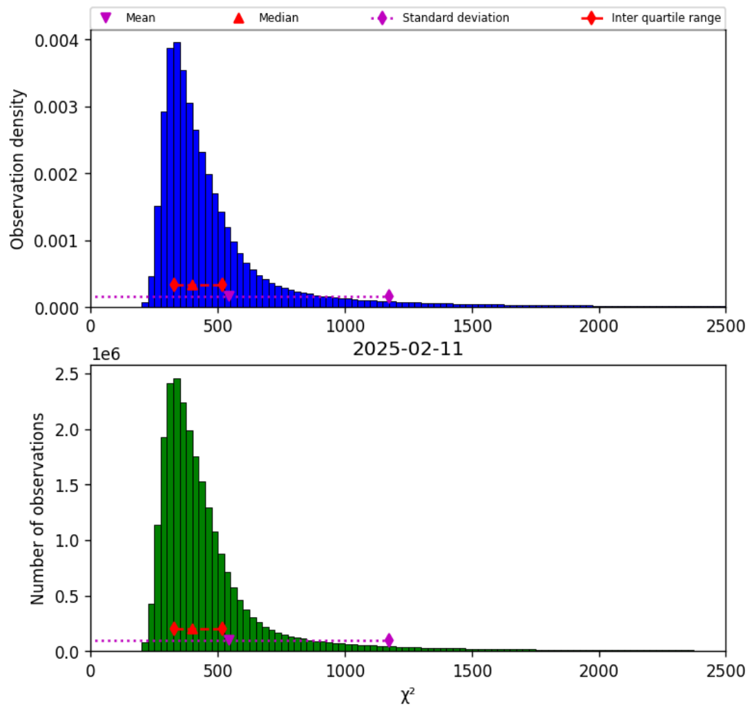
Figure 42: Histogram of “ \chi^2 ” for 2025-02-10 to 2025-02-12
