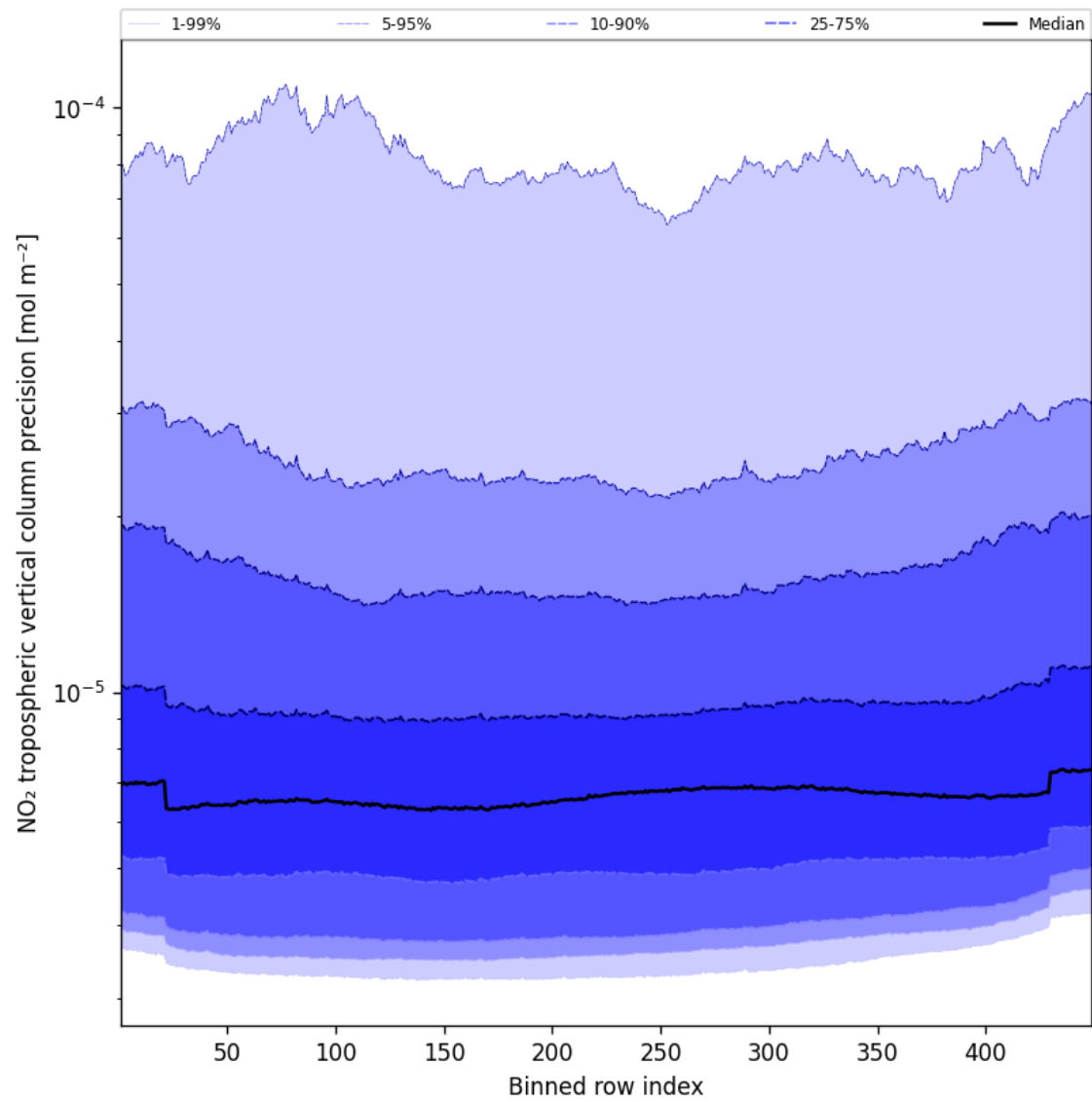
Figure 47: Along track statistics of “NO 2 tropospheric vertical column precision” for 2025-02-10 to 2025-02-12
