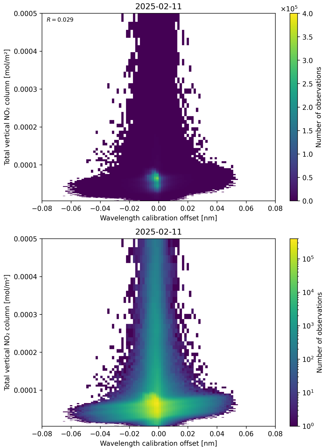
Figure 179: Scatter density plot of “Wavelength calibration offset” against “Total vertical NO 2 column” for 2025-02-10 to 2025-02-12.
