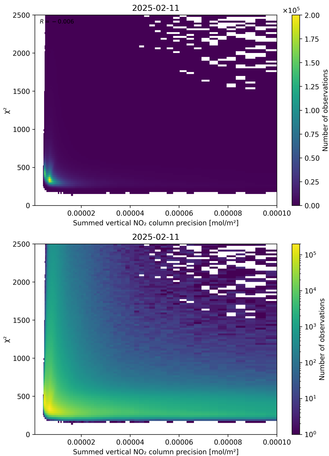
Figure 107: Scatter density plot of “Summed vertical NO 2 column precision” against “ \chi^2 ” for 2025-02-10 to 2025-02-12.
