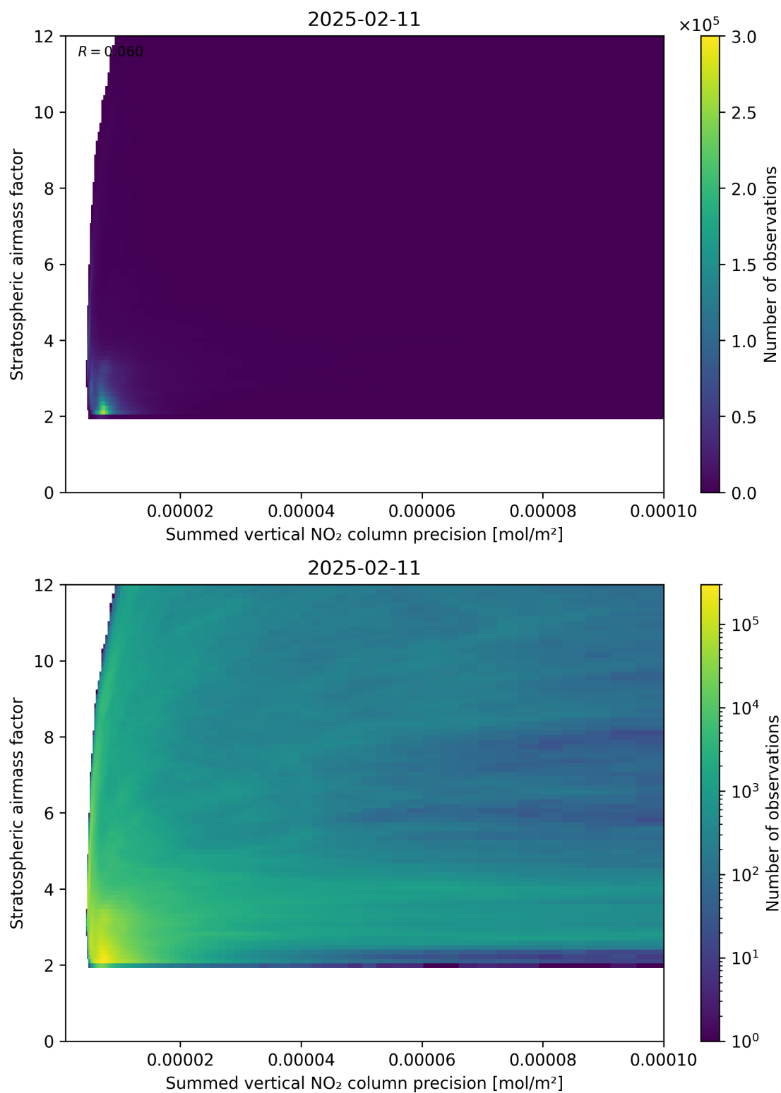
Figure 106: Scatter density plot of “Summed vertical NO 2 column precision” against “Stratospheric airmass factor” for 2025-02-10 to 2025-02-12.
