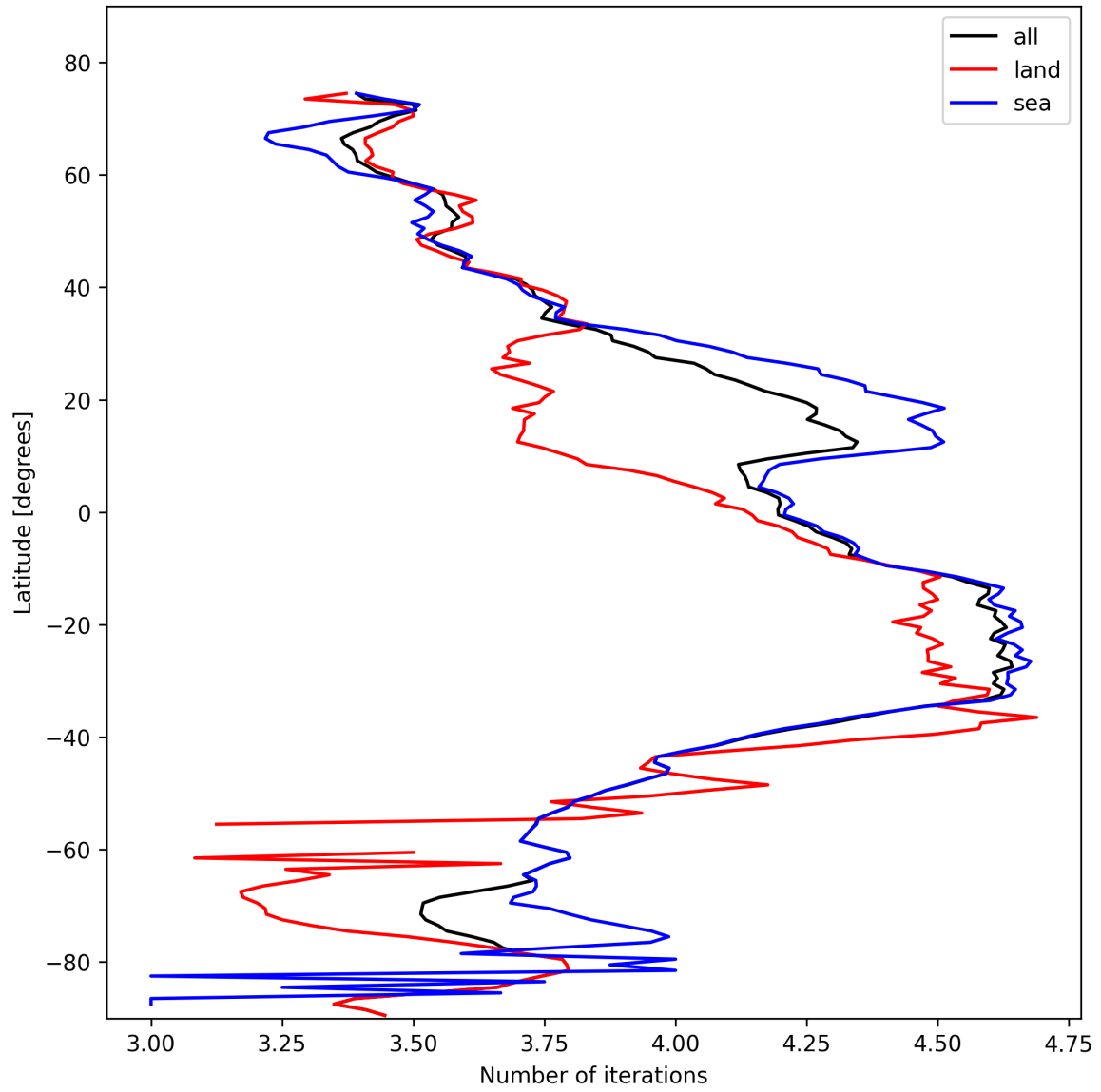
Figure 17: Zonal average of “Number of iterations” for 2025-02-10 to 2025-02-12.
