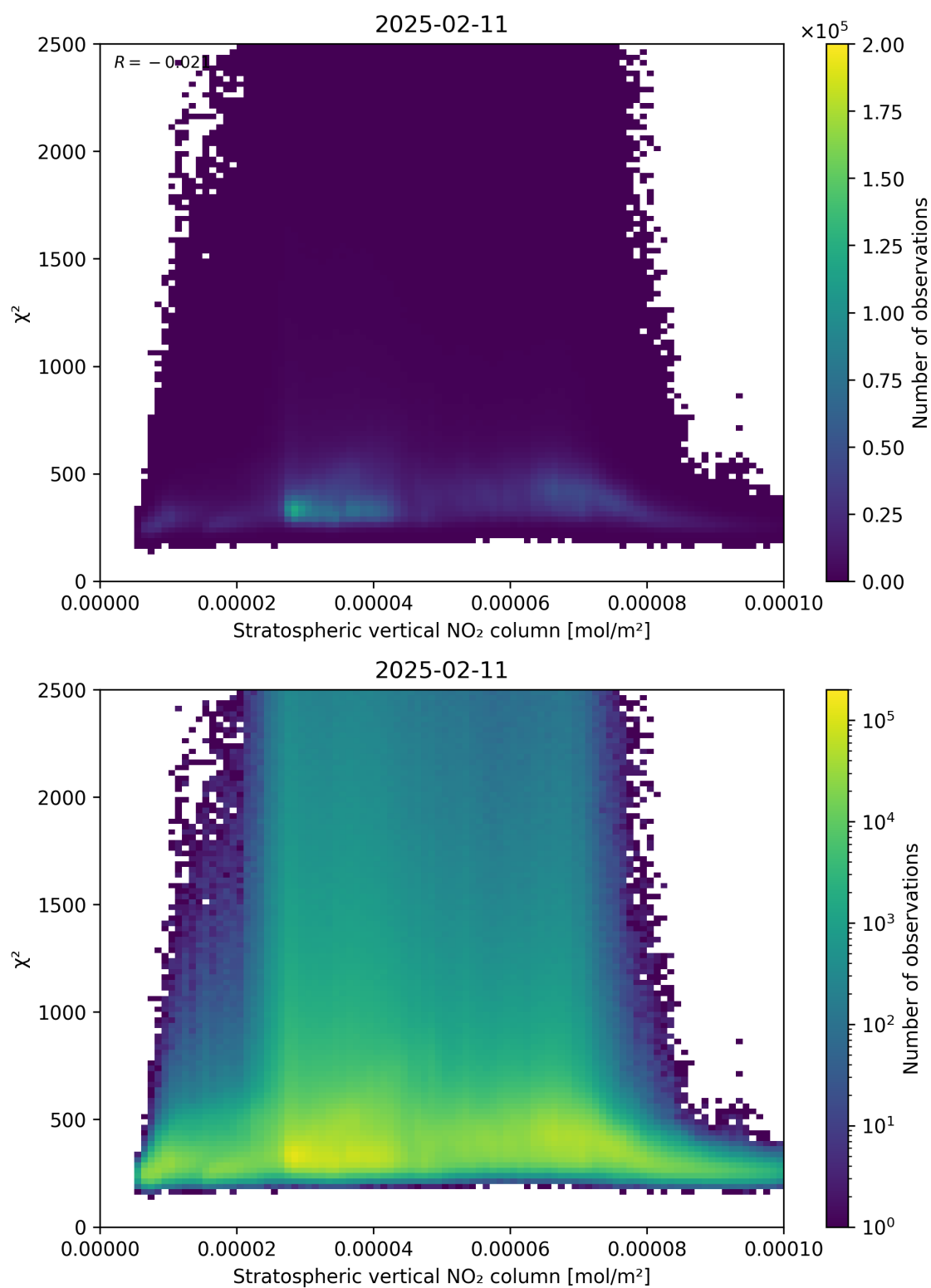
Figure 97: Scatter density plot of “Stratospheric vertical NO 2 column” against “ \chi^2 ” for 2025-02-10 to 2025-02-12.
