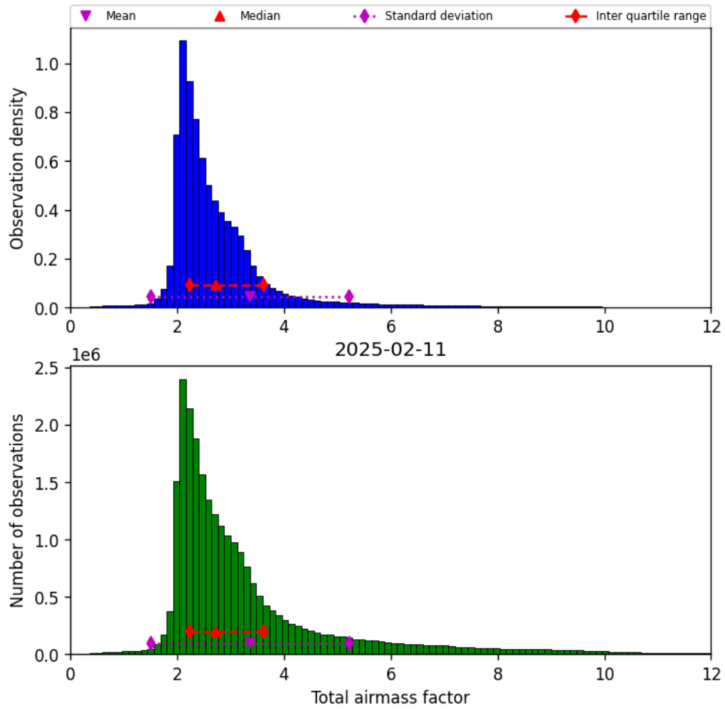
Figure 32: Histogram of “Total airmass factor” for 2025-02-10 to 2025-02-12
