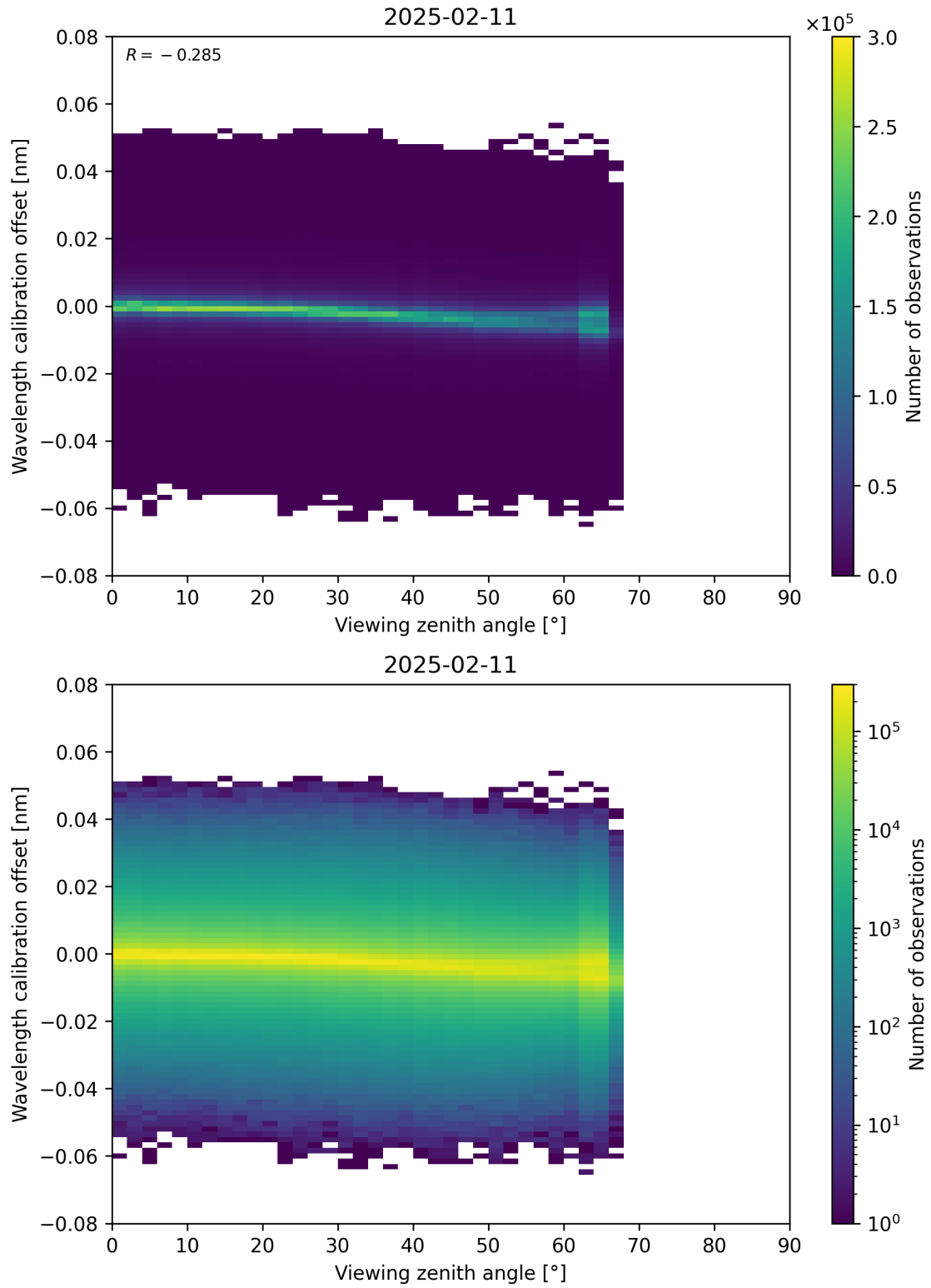
Figure 173: Scatter density plot of “Viewing zenith angle” against “Wavelength calibration offset” for 2025-02-10 to 2025-02-12.
