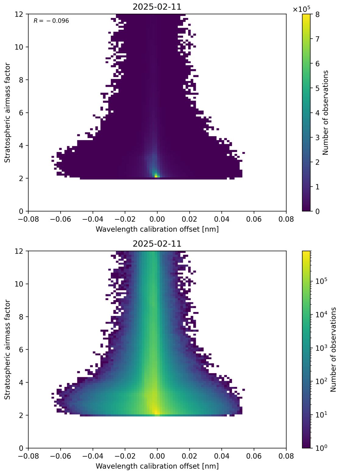
Figure 174: Scatter density plot of “Wavelength calibration offset” against “Stratospheric air mass factor” for 2025-02-10 to 2025-02-12.
