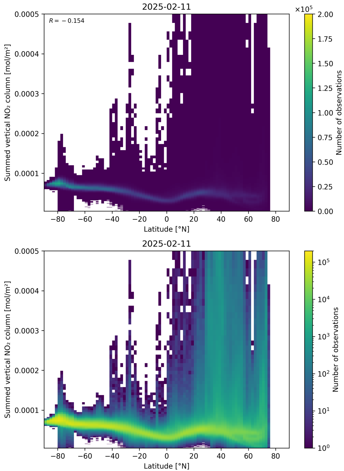
Figure 88: Scatter density plot of “Latitude” against “Summed vertical NO 2 column” for 2025-02-10 to 2025-02-12.
