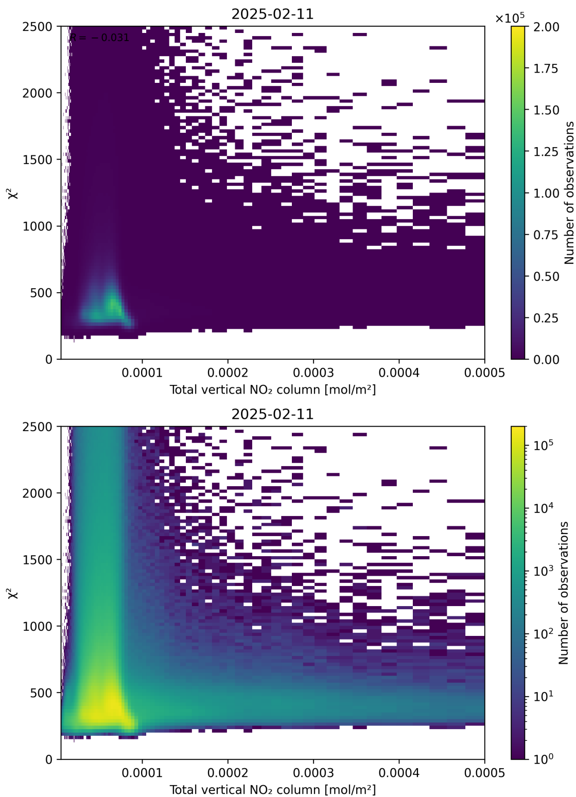
Figure 111: Scatter density plot of “Total vertical NO 2 column” against “ \chi^2 ” for 2025-02-10 to 2025-02-12.
