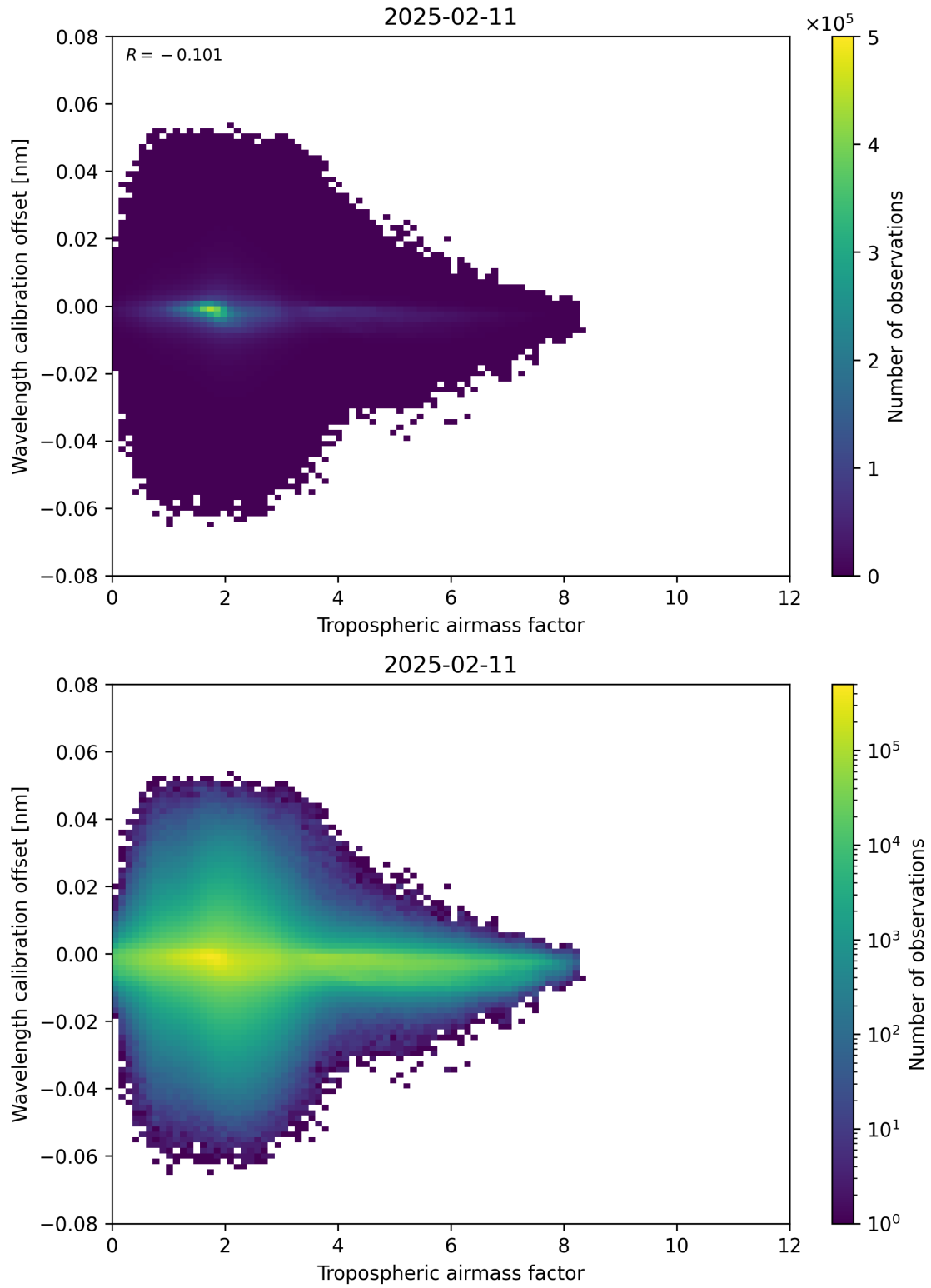
Figure 80: Scatter density plot of “Tropospheric airmass factor” against “Wavelength calibration offset” for 2025-02-10 to 2025-02-12.
