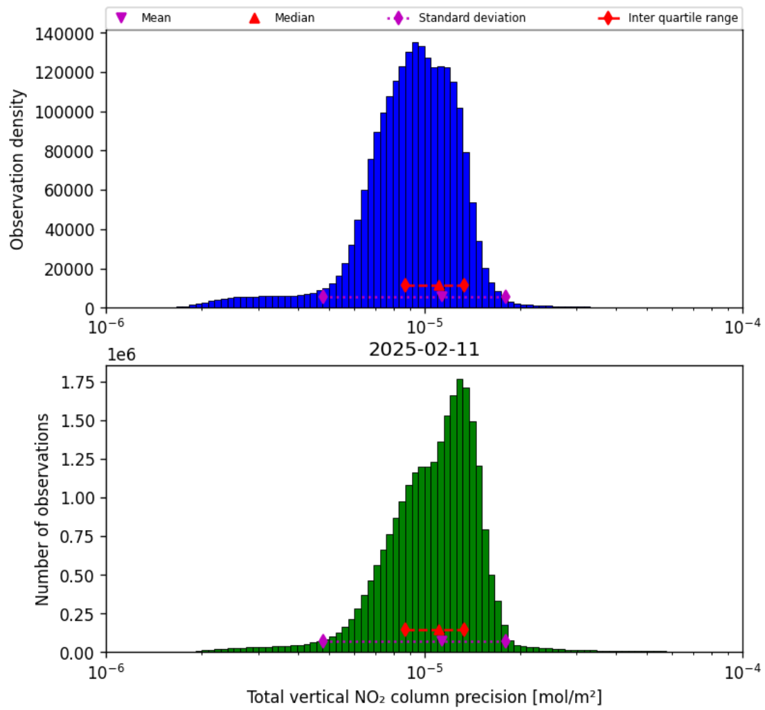
Figure 39: Histogram of “Total vertical NO 2 column precision” for 2025-02-10 to 2025-02-12
