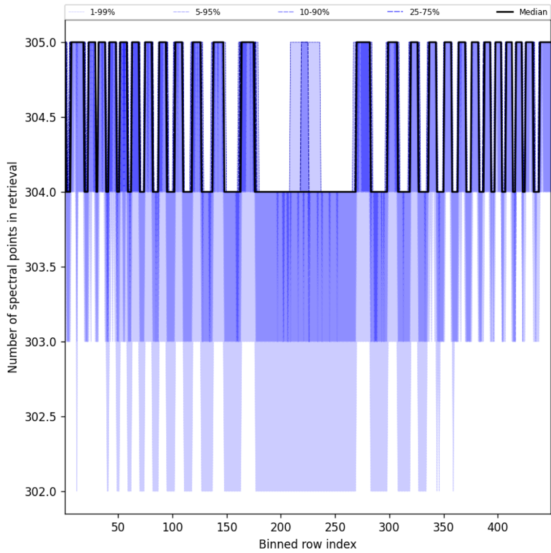
Figure 50: Along track statistics of “Number of spectral points in retrieval” for 2025-02-10 to 2025-02-12
