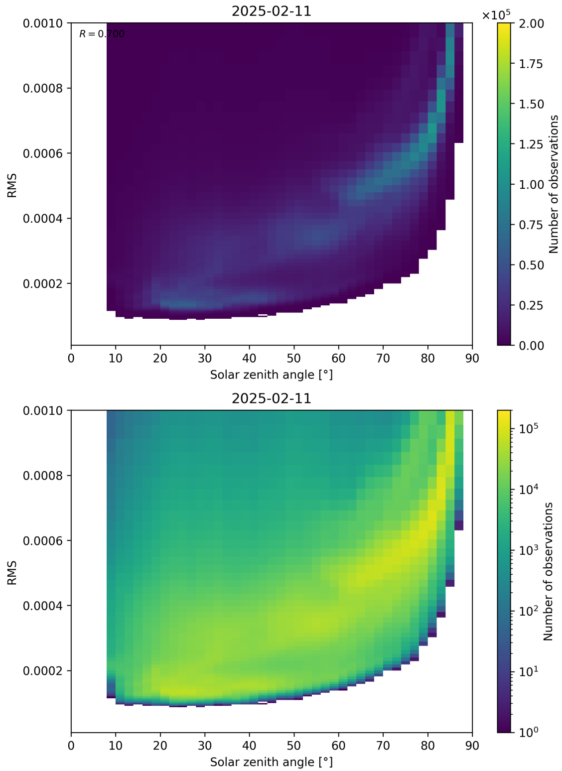
Figure 157: Scatter density plot of “Solar zenith angle” against “RMS” for 2025-02-10 to 2025-02-12.
