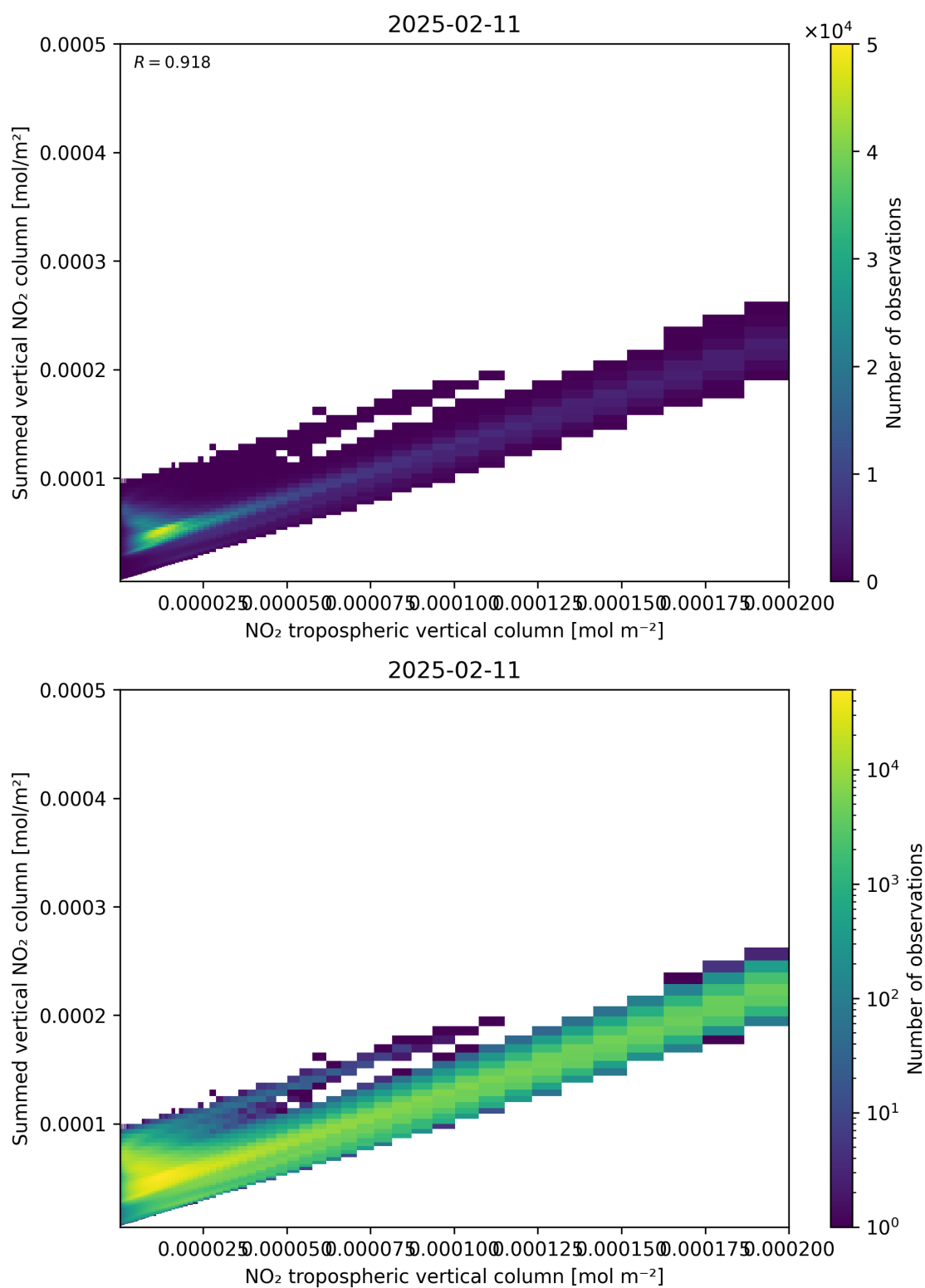
Figure 126: Scatter density plot of “NO 2 tropospheric vertical column” against “Summed vertical NO 2 column” for 2025-02-10 to 2025-02-12.
