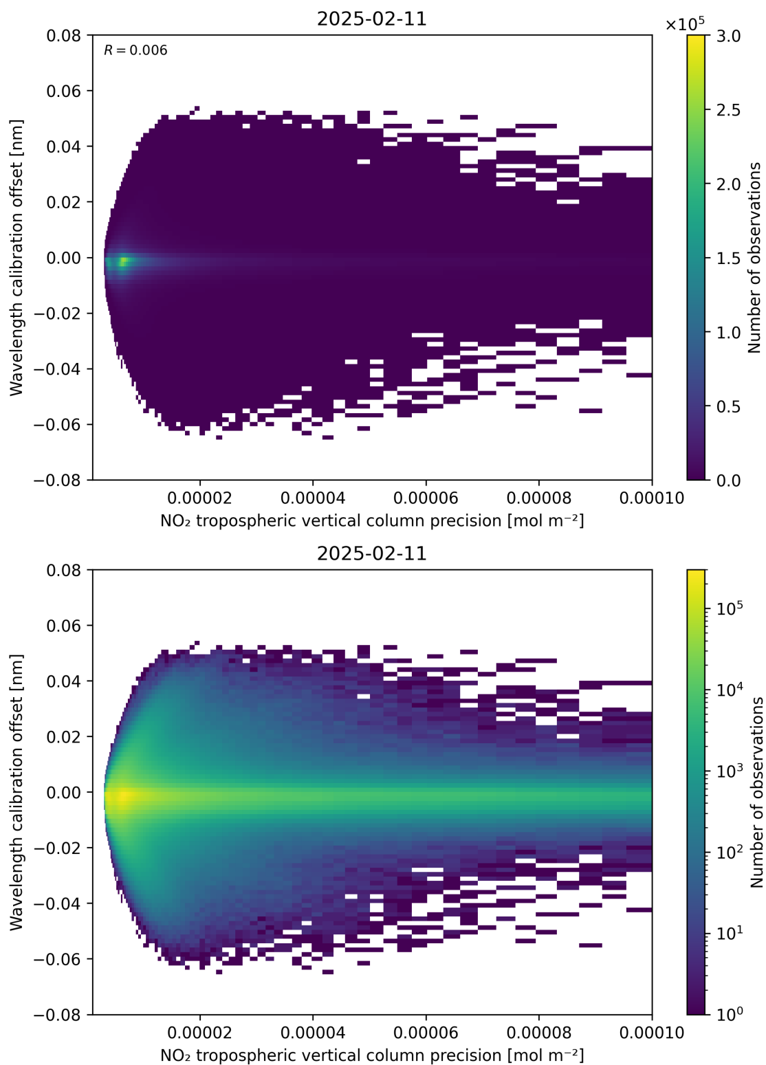
Figure 141: Scatter density plot of “NO 2 tropospheric vertical column precision” against “Wavelength calibration offset” for 2025-02-10 to 2025-02-12.
