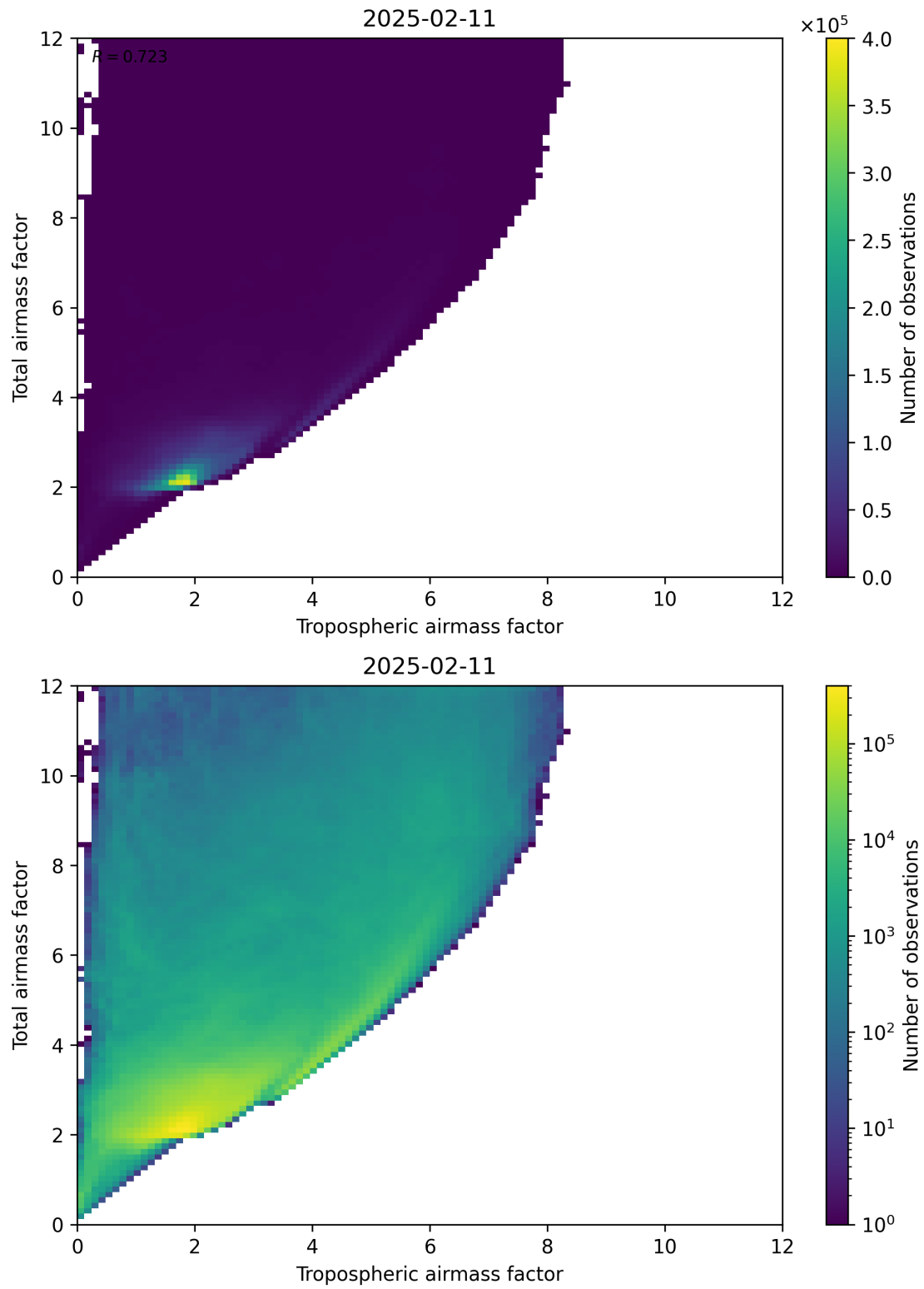
Figure 72: Scatter density plot of “Tropospheric airmass factor” against “Total airmass factor” for 2025-02-10 to 2025-02-12.
