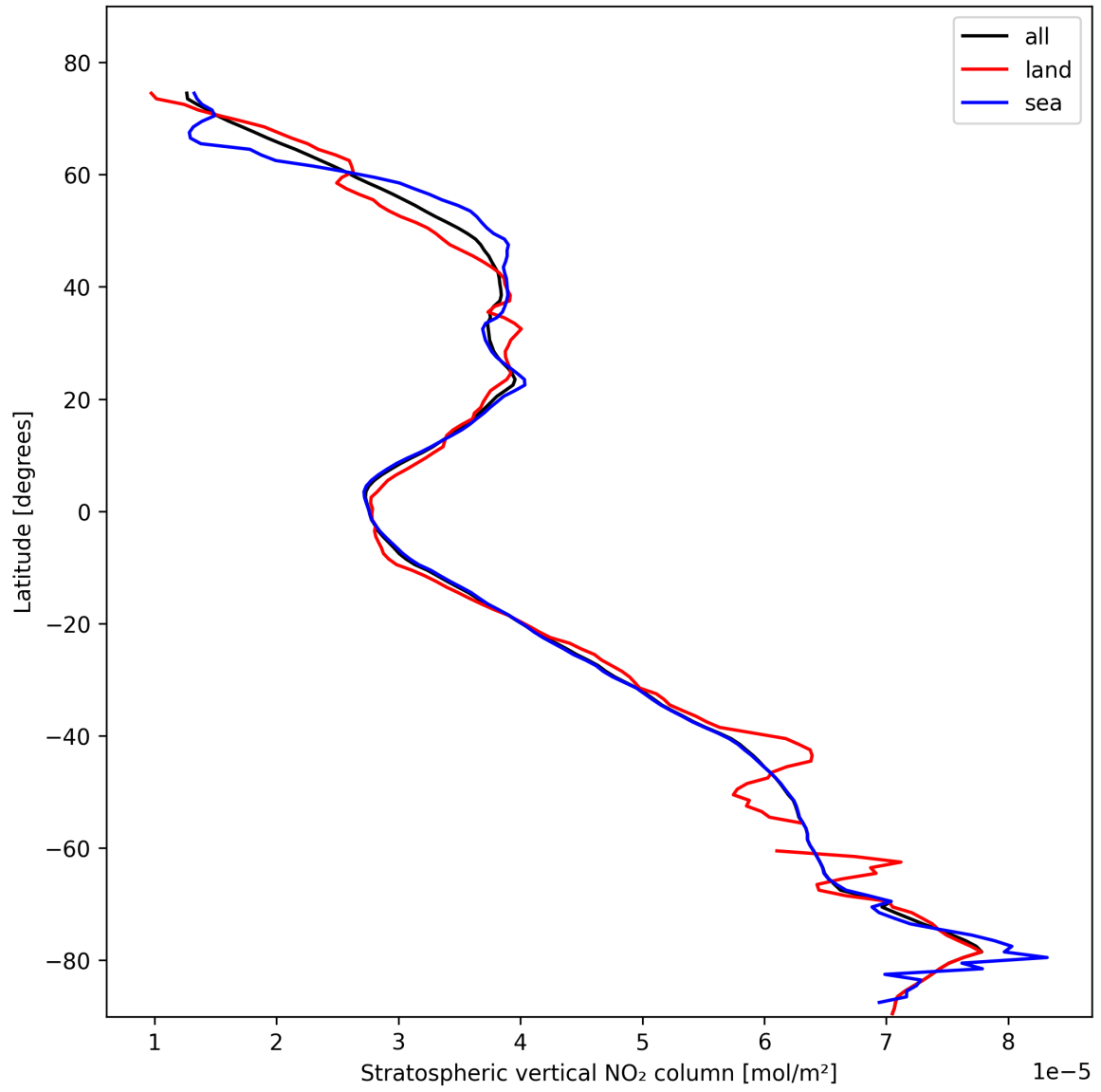
Figure 19: Zonal average of “Stratospheric vertical NO 2 column” for 2025-02-10 to 2025-02-12.
