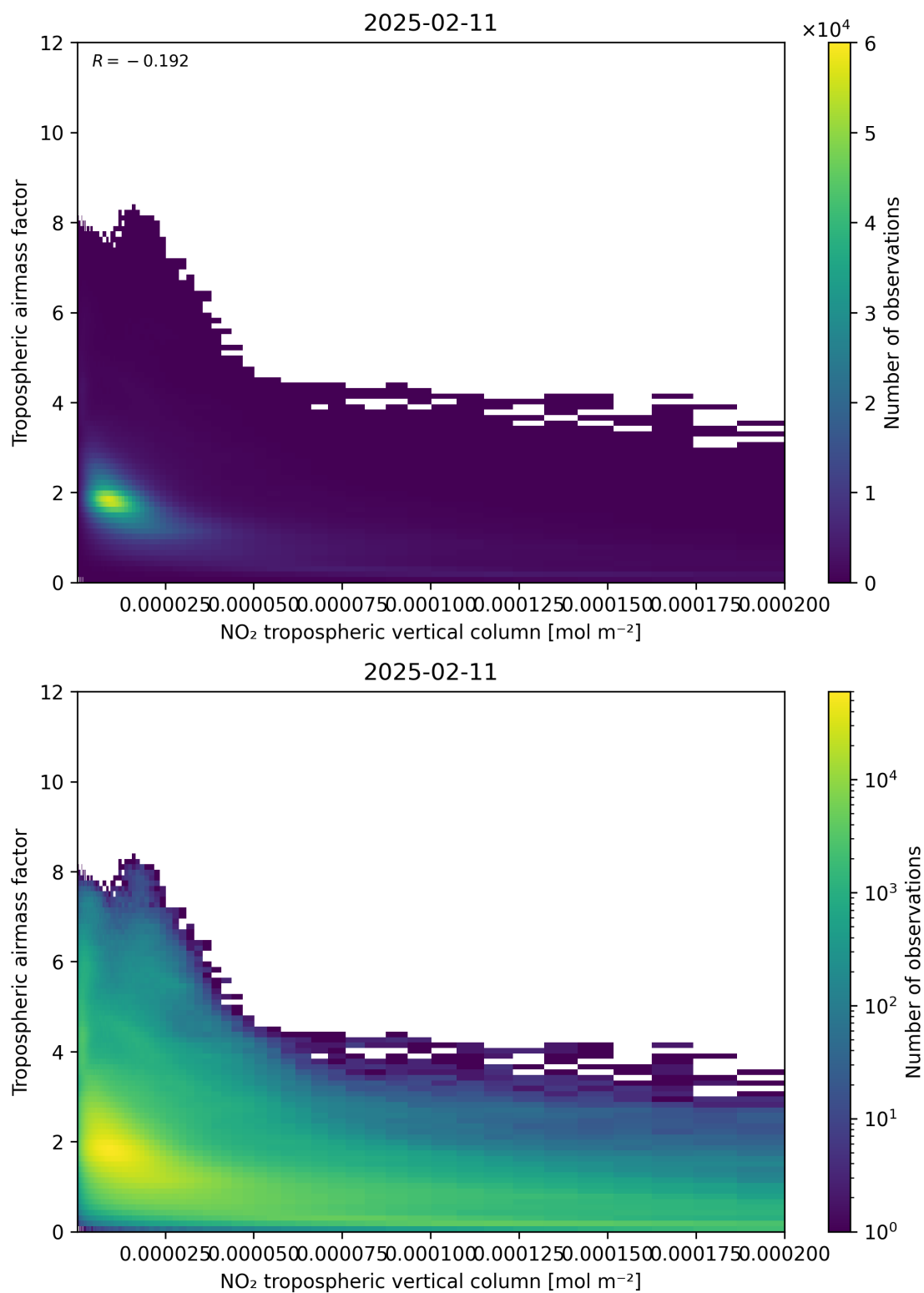
Figure 123: Scatter density plot of “NO 2 tropospheric vertical column” against “Tropospheric air mass factor” for 2025-02-10 to 2025-02-12.
