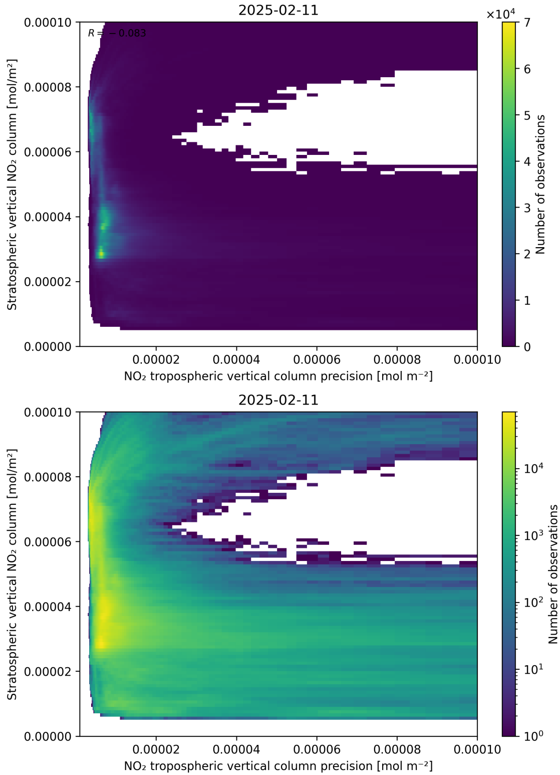
Figure 135: Scatter density plot of “NO 2 tropospheric vertical column precision” against “Stratospheric vertical NO 2 column” for 2025-02-10 to 2025-02-12.
