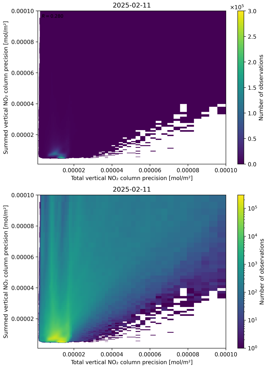
Figure 118: Scatter density plot of “Total vertical NO 2 column precision” against “Summed vertical NO 2 column precision” for 2025-02-10 to 2025-02-12.
