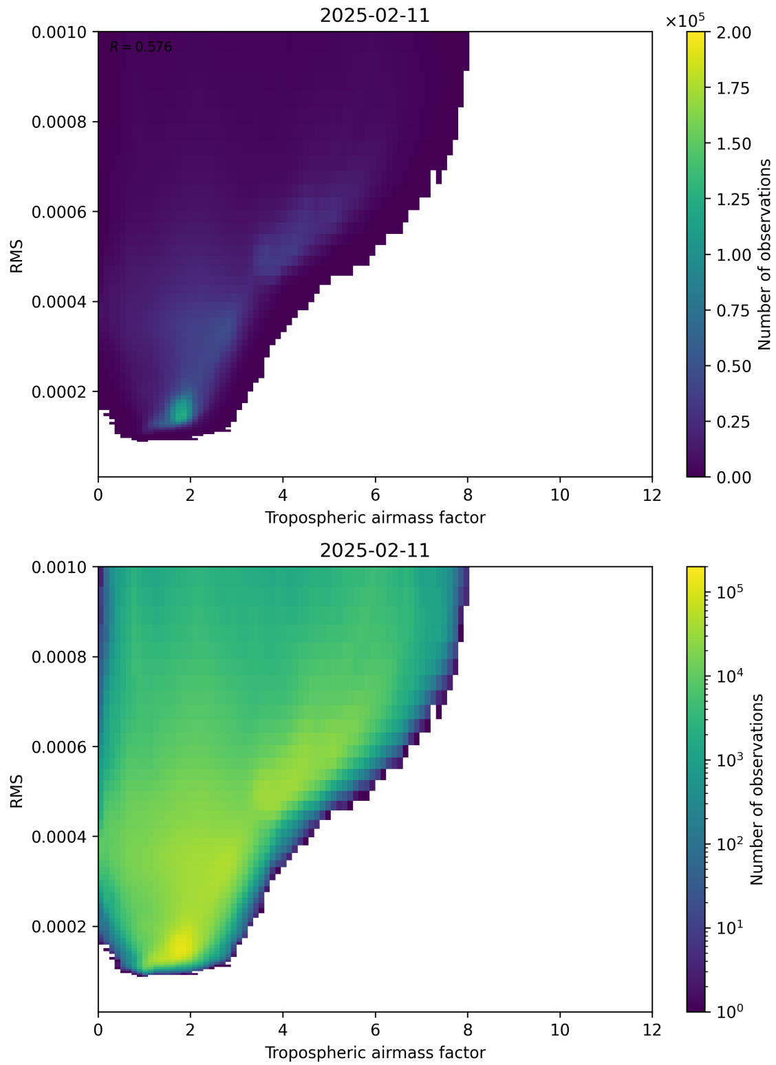
Figure 79: Scatter density plot of “Tropospheric airmass factor” against “RMS” for 2025-02-10 to 2025-02-12.
