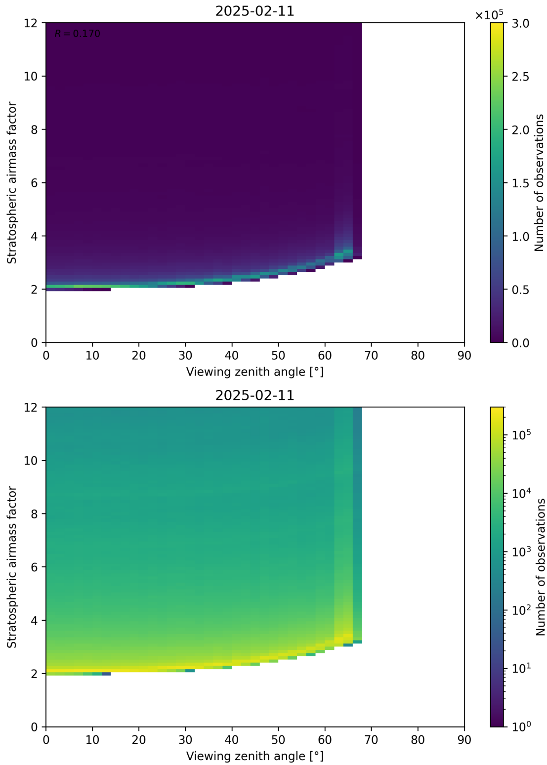
Figure 159: Scatter density plot of “Viewing zenith angle” against “Stratospheric airmass factor” for 2025-02-10 to 2025-02-12.
