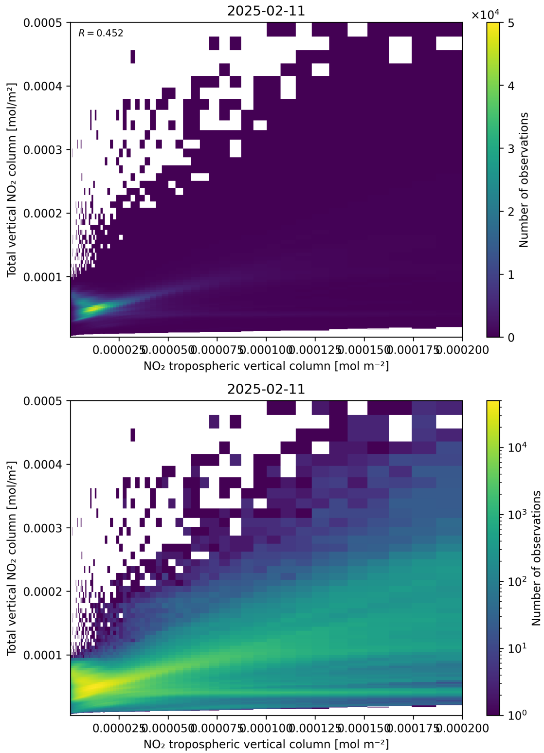
Figure 128: Scatter density plot of “NO 2 tropospheric vertical column” against “Total vertical NO 2 column” for 2025-02-10 to 2025-02-12.
