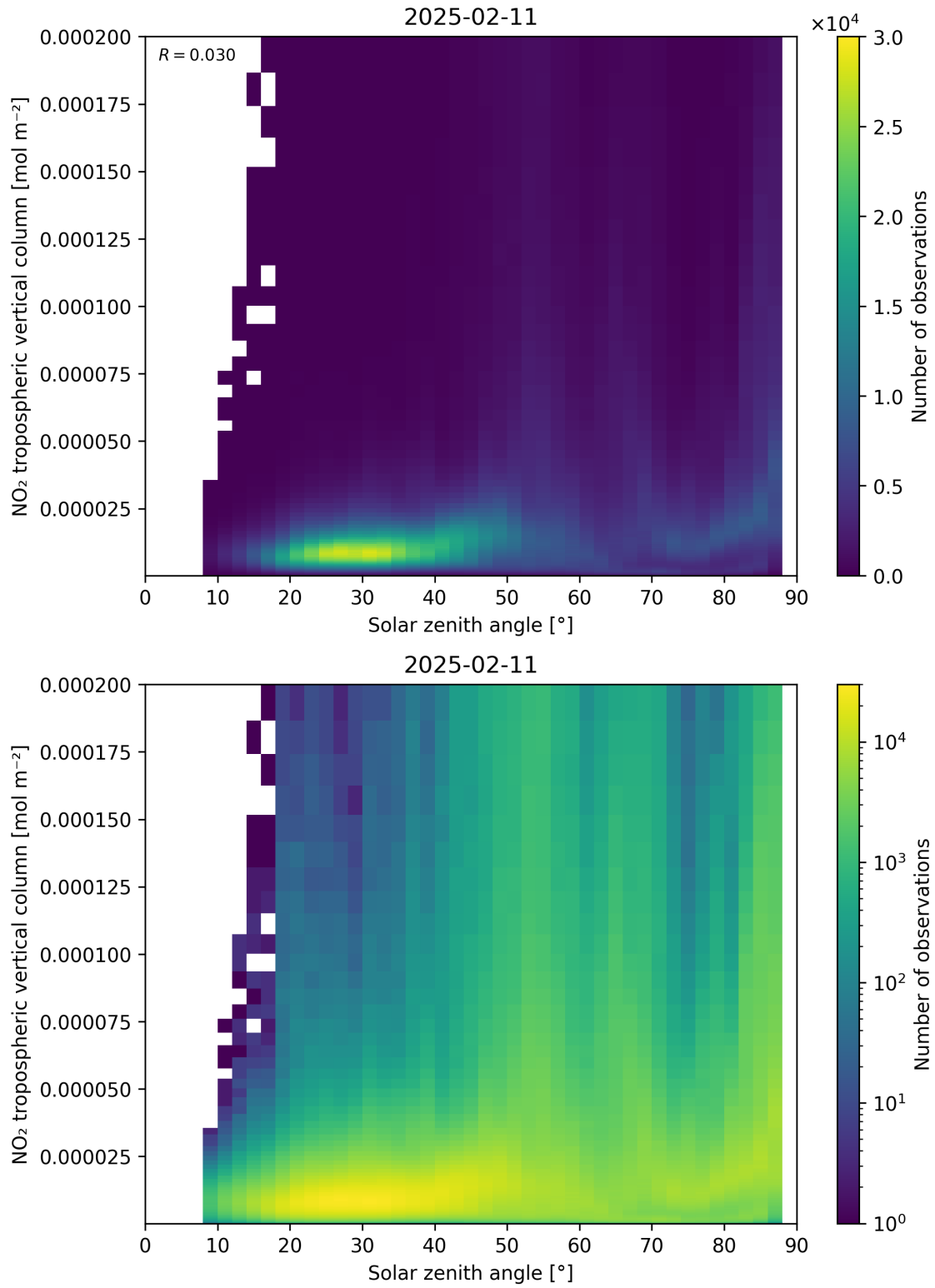
Figure 155: Scatter density plot of “Solar zenith angle” against “NO 2 tropospheric vertical column” for 2025-02-10 to 2025-02-12.
