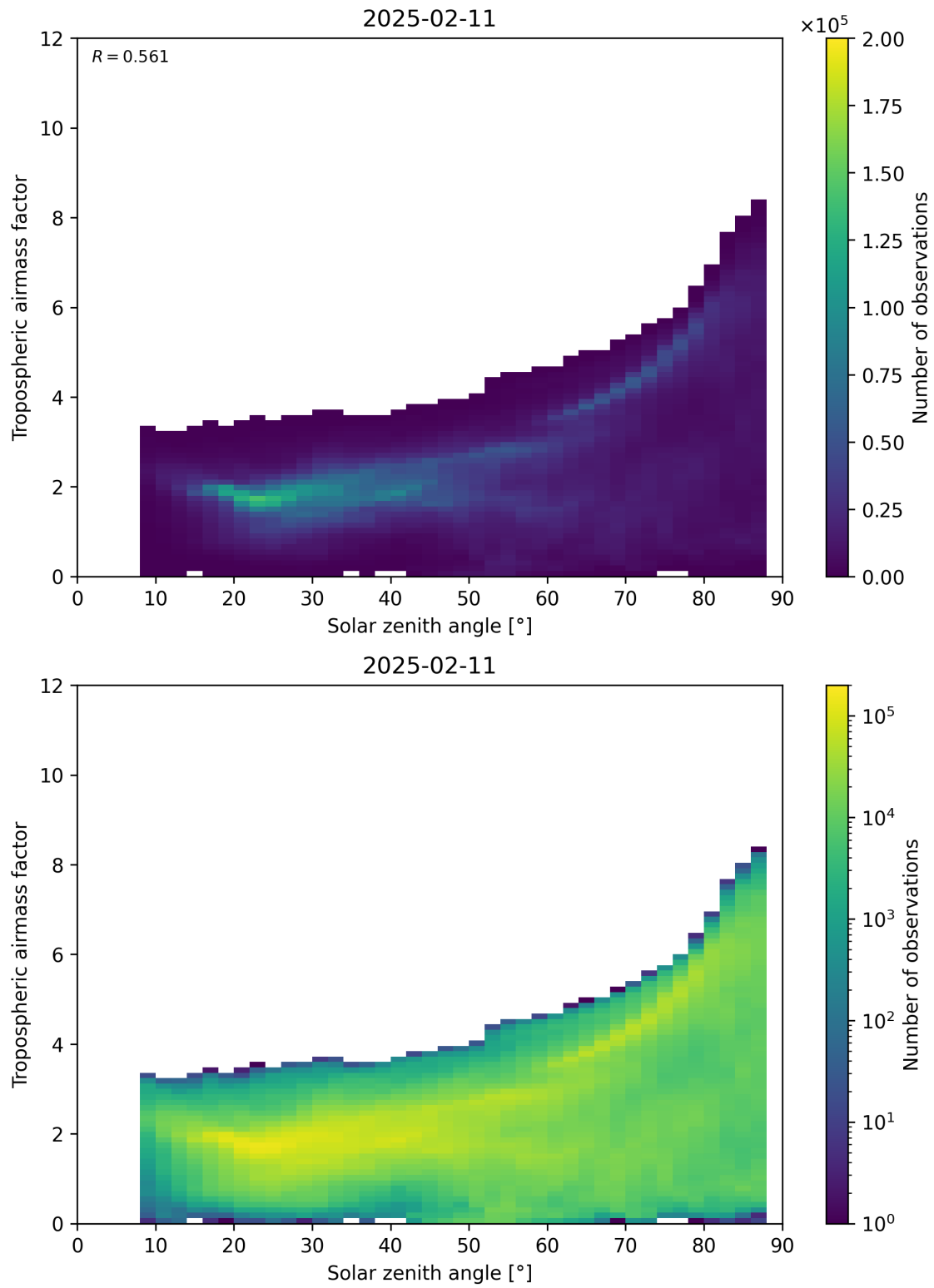
Figure 147: Scatter density plot of “Solar zenith angle” against “Tropospheric airmass factor” for 2025-02-10 to 2025-02-12.
