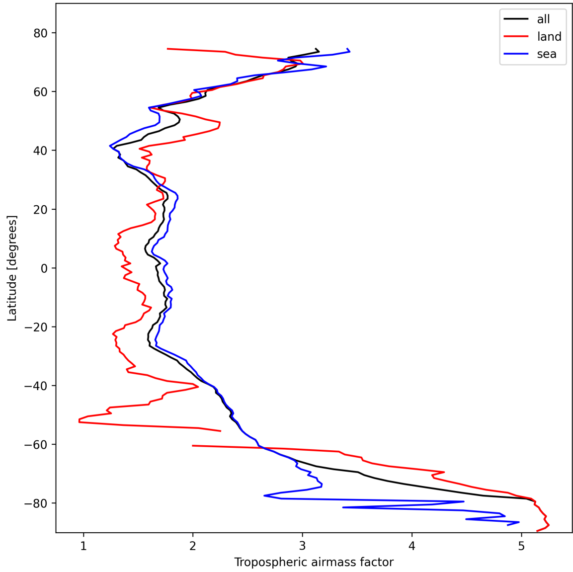
Figure 14: Zonal average of “Tropospheric airmass factor” for 2025-02-10 to 2025-02-12.
