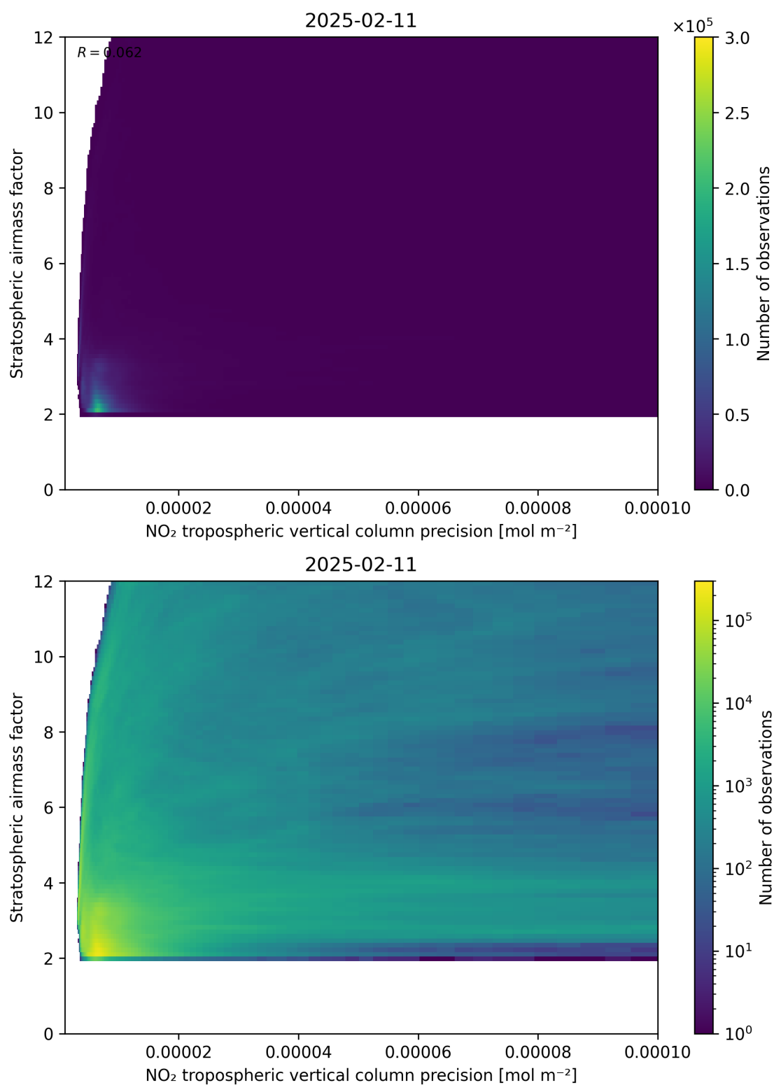
Figure 131: Scatter density plot of “NO 2 tropospheric vertical column precision” against “Stratospheric airmass factor” for 2025-02-10 to 2025-02-12.
