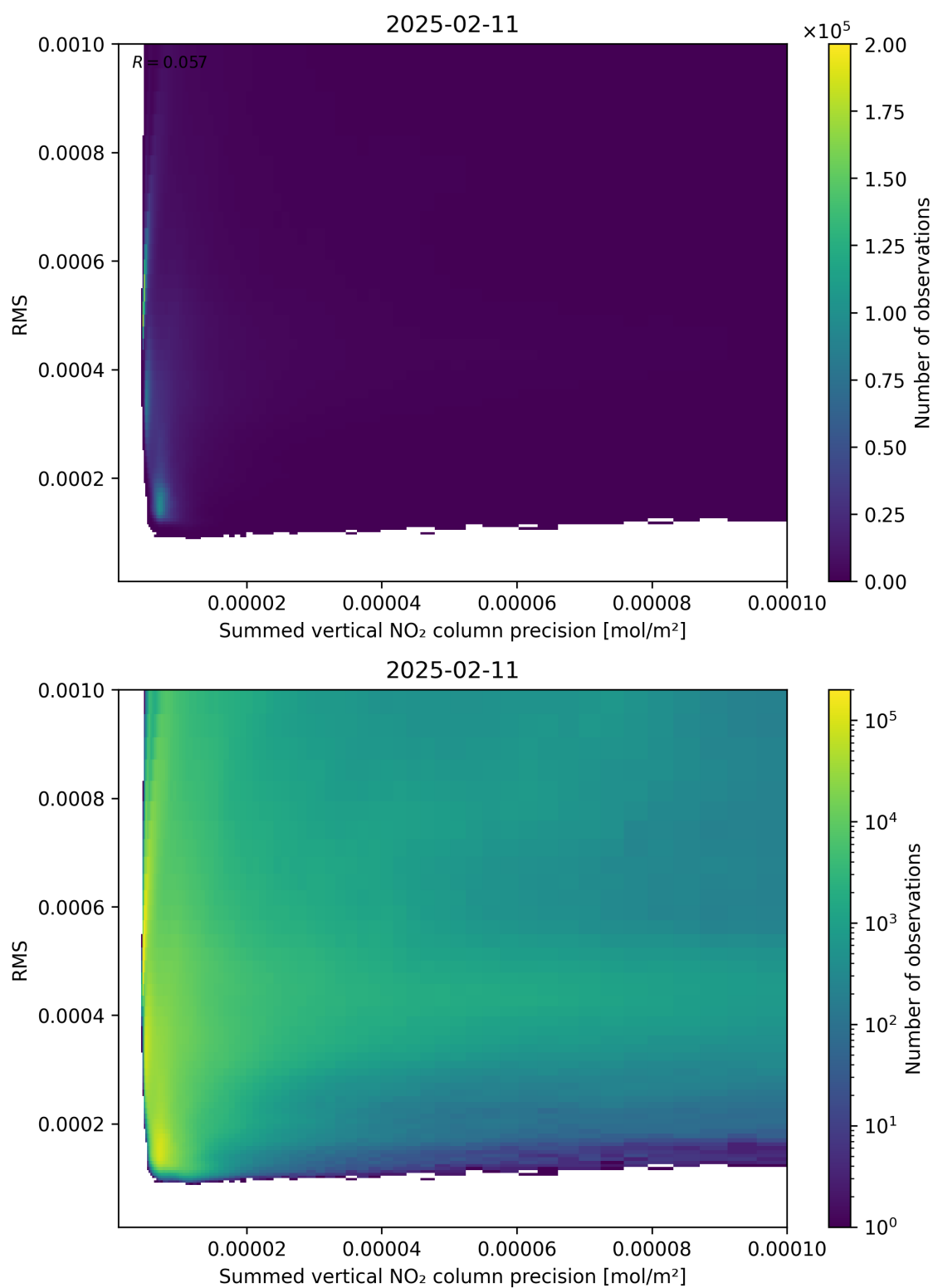
Figure 108: Scatter density plot of “Summed vertical NO 2 column precision” against “RMS” for 2025-02-10 to 2025-02-12.
