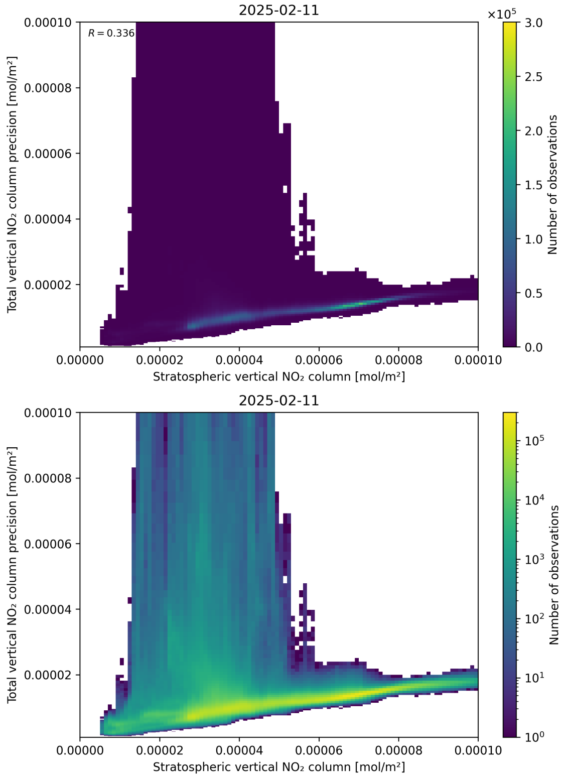
Figure 101: Scatter density plot of “Stratospheric vertical NO 2 column” against “Total vertical NO 2 column precision” for 2025-02-10 to 2025-02-12.
