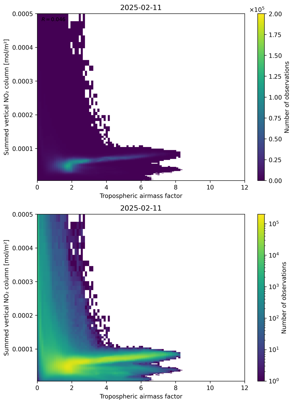
Figure 75: Scatter density plot of “Tropospheric airmass factor” against “Summed vertical NO 2 column” for 2025-02-10 to 2025-02-12.
