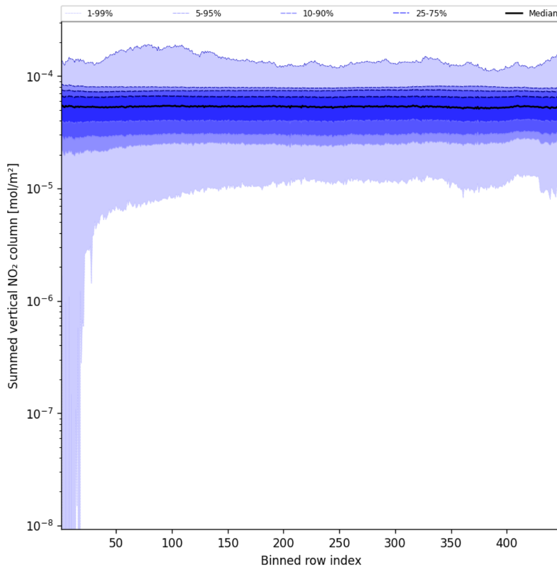
Figure 57: Along track statistics of “Summed vertical NO 2 column” for 2025-02-10 to 2025-02-12
