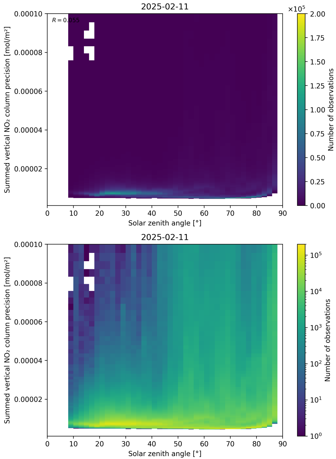
Figure 152: Scatter density plot of “Solar zenith angle” against “Summed vertical NO 2 column precision” for 2025-02-10 to 2025-02-12.
