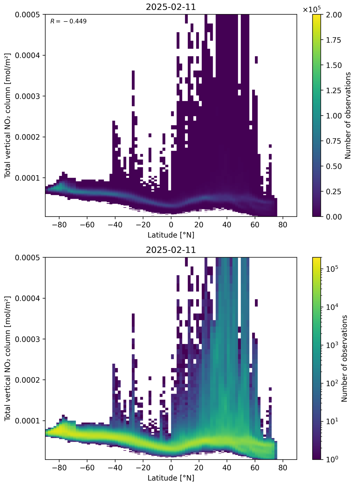
Figure 90: Scatter density plot of “Latitude” against “Total vertical NO 2 column” for 2025-02-10 to 2025-02-12.
