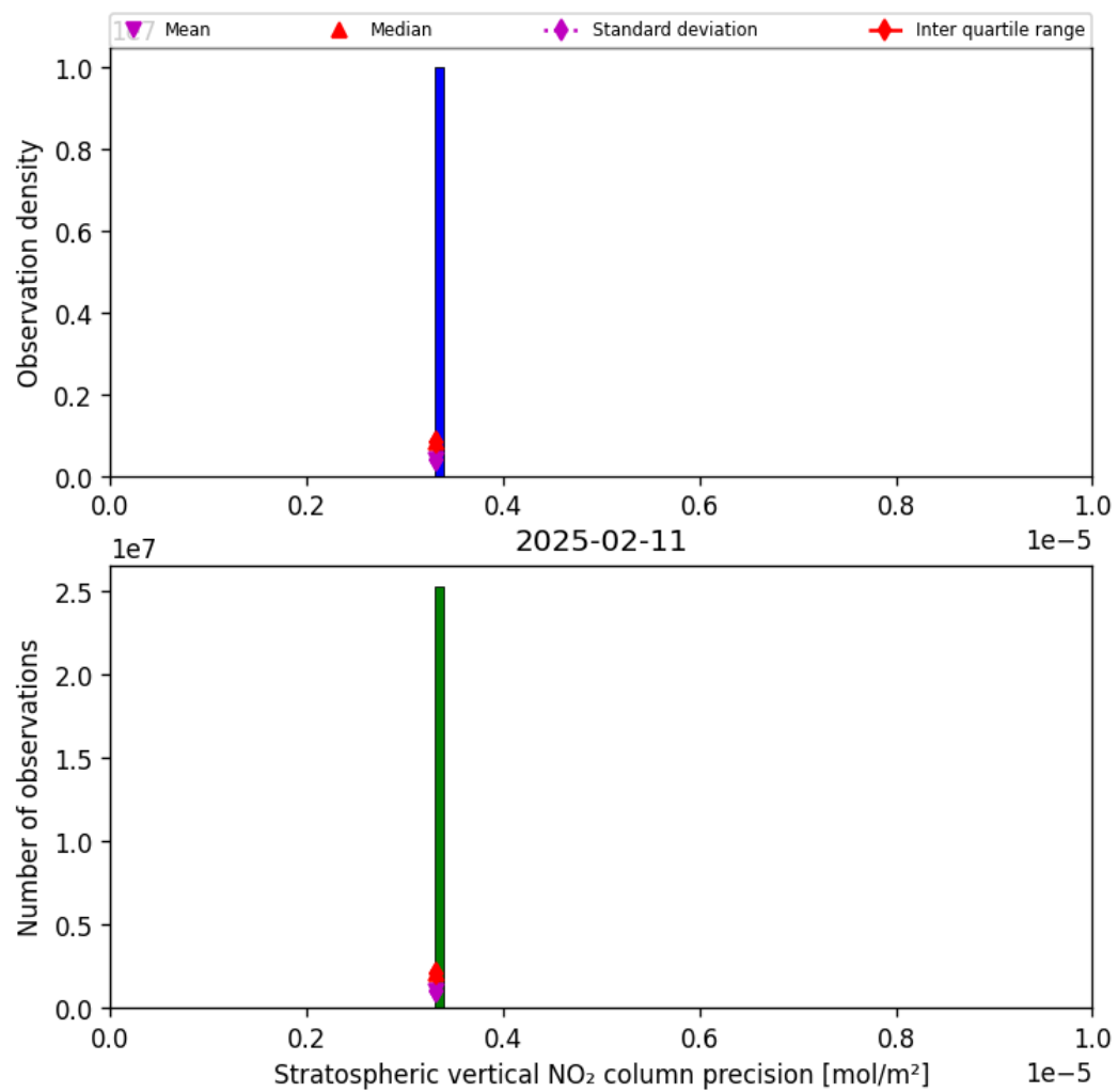
Figure 37: Histogram of “Stratospheric vertical NO 2 column precision” for 2025-02-10 to 2025-02-12
