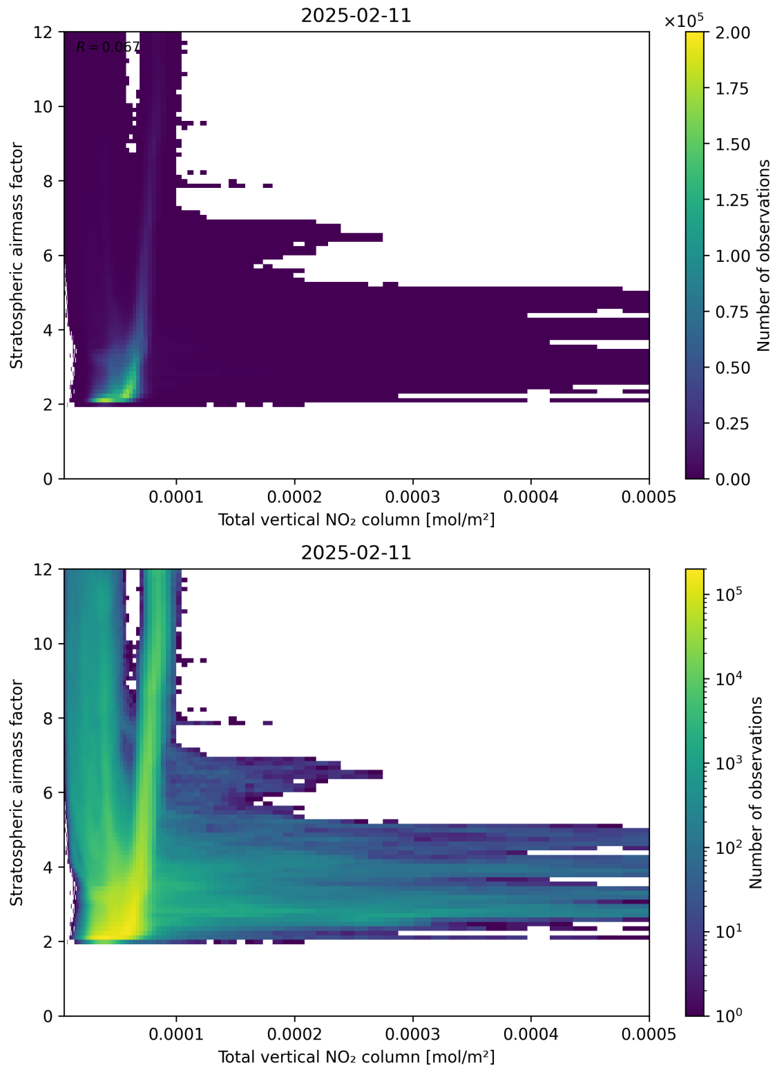
Figure 110: Scatter density plot of “Total vertical NO 2 column” against “Stratospheric airmass factor” for 2025-02-10 to 2025-02-12.
