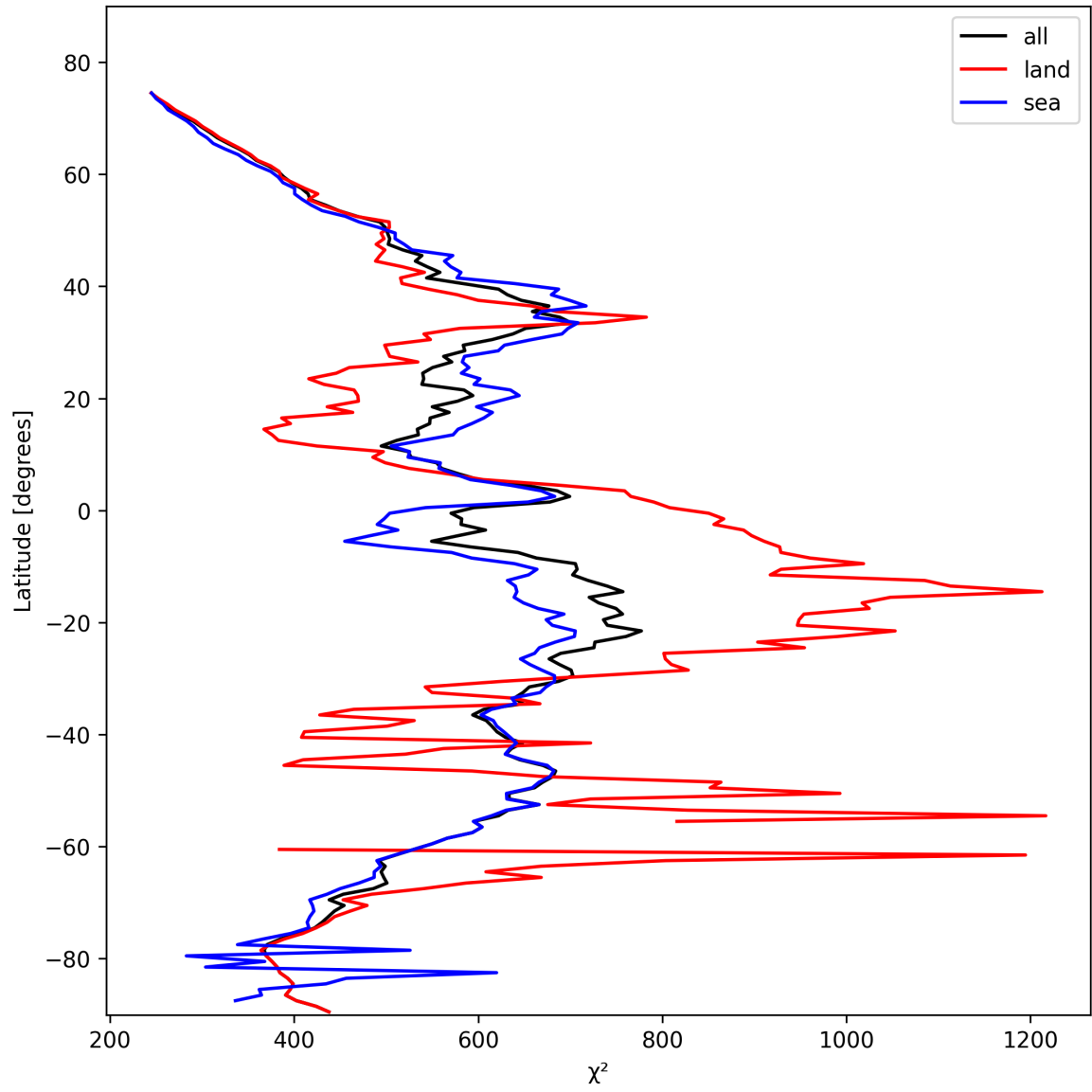
Figure 25: Zonal average of “ \chi^2 ” for 2025-02-10 to 2025-02-12.
