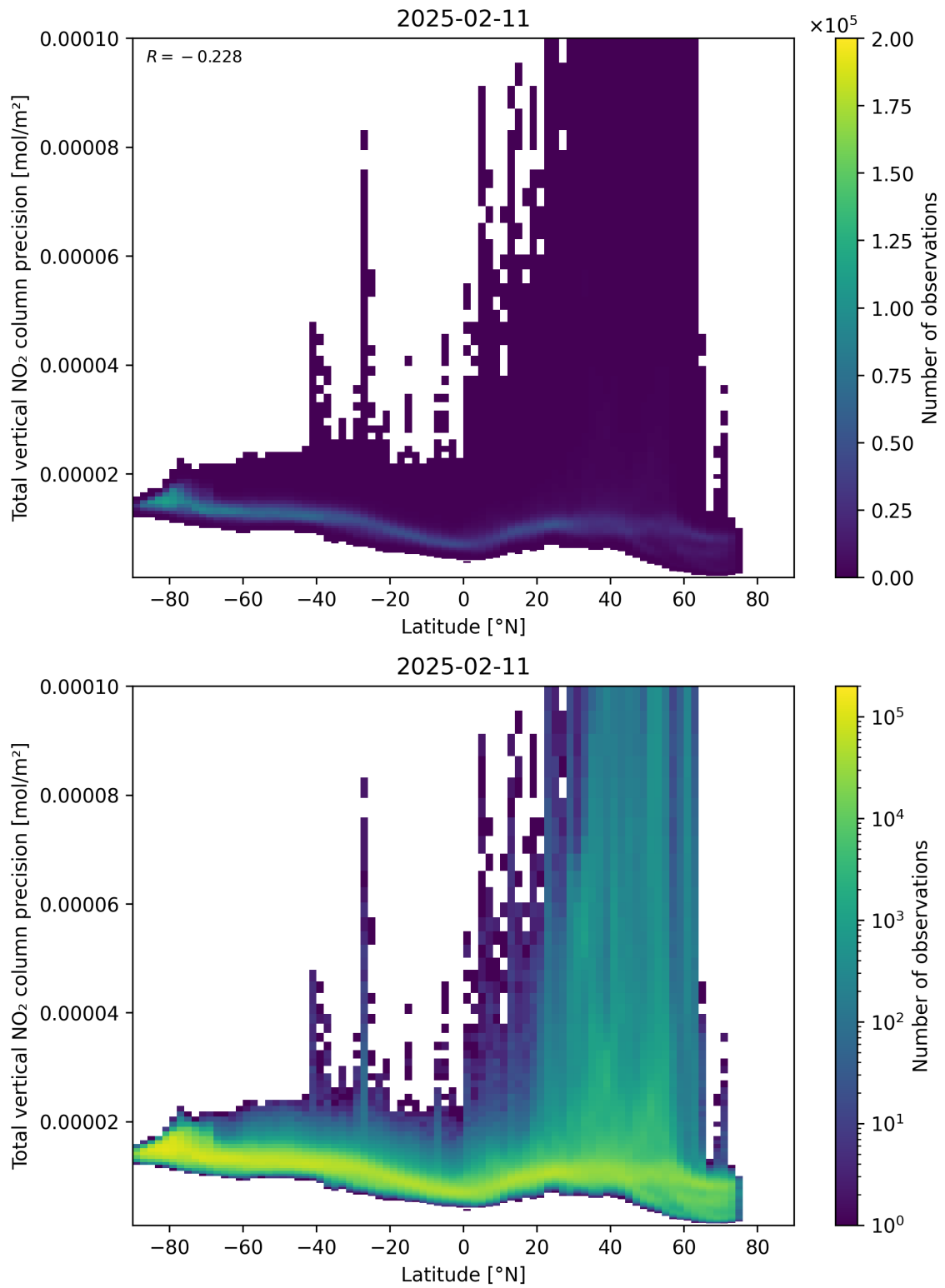
Figure 91: Scatter density plot of “Latitude” against “Total vertical NO 2 column precision” for 2025-02-10 to 2025-02-12.
