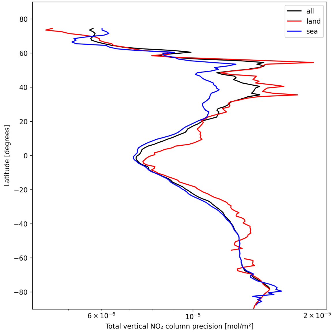
Figure 22: Zonal average of “Total vertical NO 2 column precision” for 2025-02-10 to 2025-02-12.
