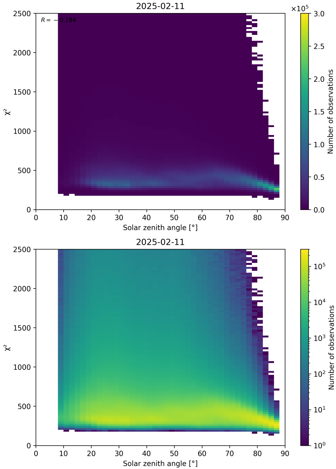
Figure 148: Scatter density plot of “Solar zenith angle” against “ \chi^2 ” for 2025-02-10 to 2025-02-12.
