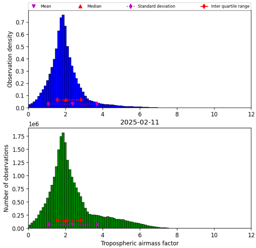
Figure 31: Histogram of “Tropospheric airmass factor” for 2025-02-10 to 2025-02-12
