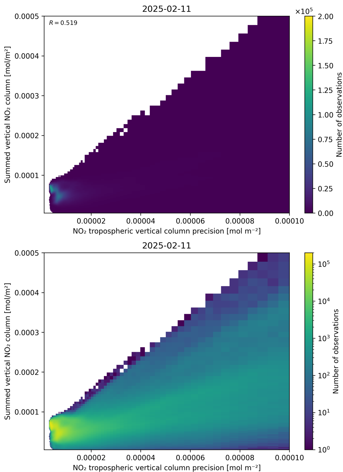
Figure 136: Scatter density plot of “NO 2 tropospheric vertical column precision” against “Summed vertical NO 2 column” for 2025-02-10 to 2025-02-12.
