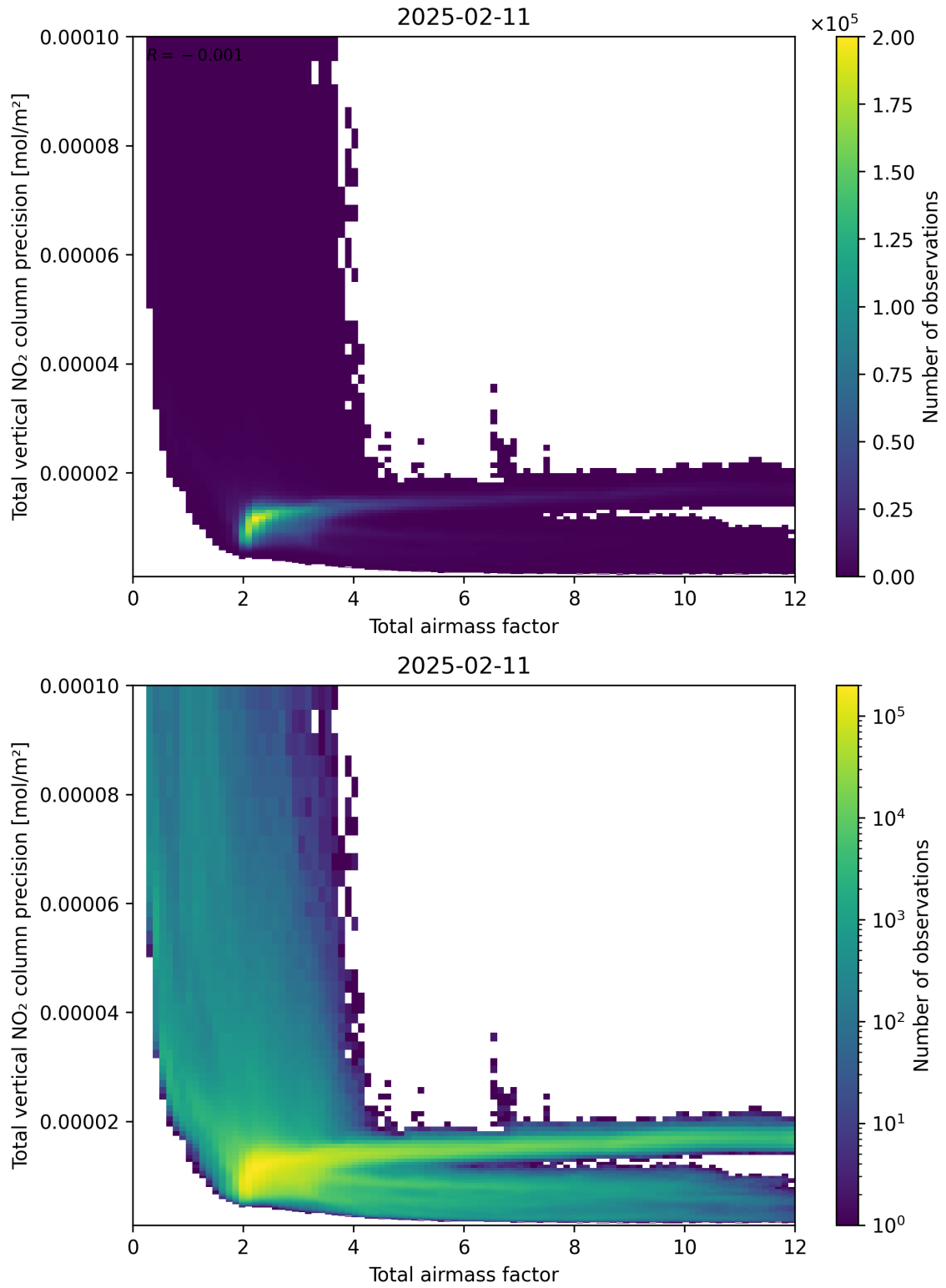
Figure 68: Scatter density plot of “Total airmass factor” against “Total vertical NO 2 column precision” for 2025-02-10 to 2025-02-12.
