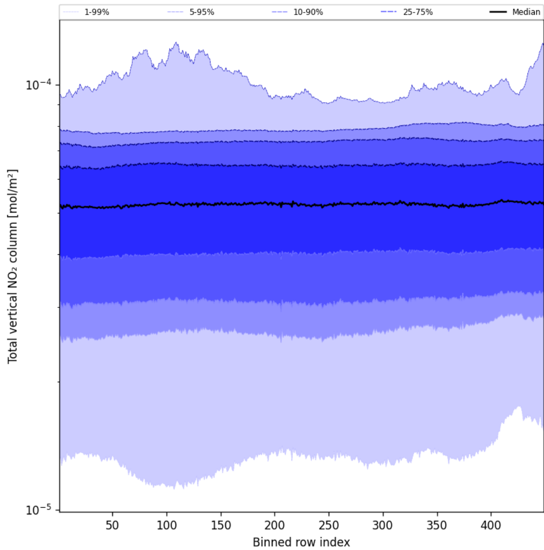
Figure 55: Along track statistics of “Total vertical NO 2 column” for 2025-02-10 to 2025-02-12
