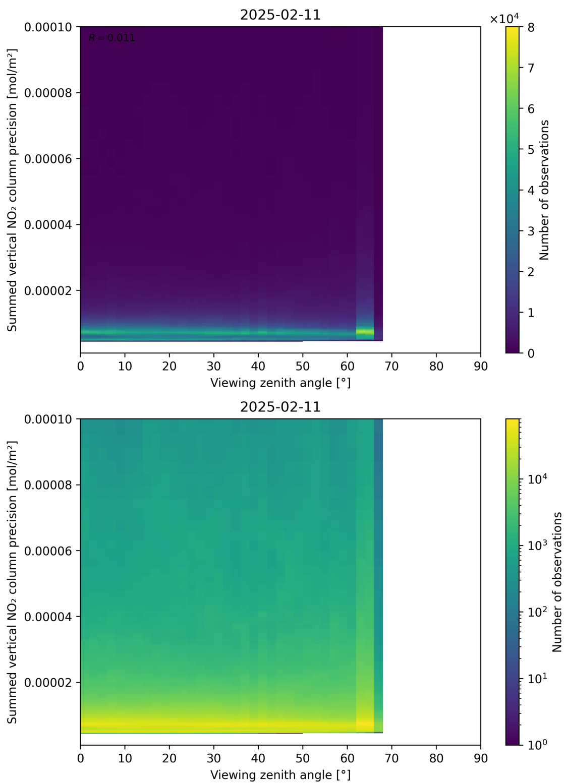
Figure 166: Scatter density plot of “Viewing zenith angle” against “Summed vertical NO 2 column precision” for 2025-02-10 to 2025-02-12.
