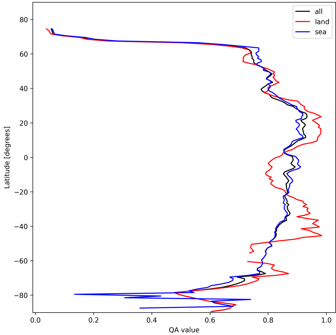
Figure 11: Zonal average of “QA value” for 2025-02-10 to 2025-02-12.
