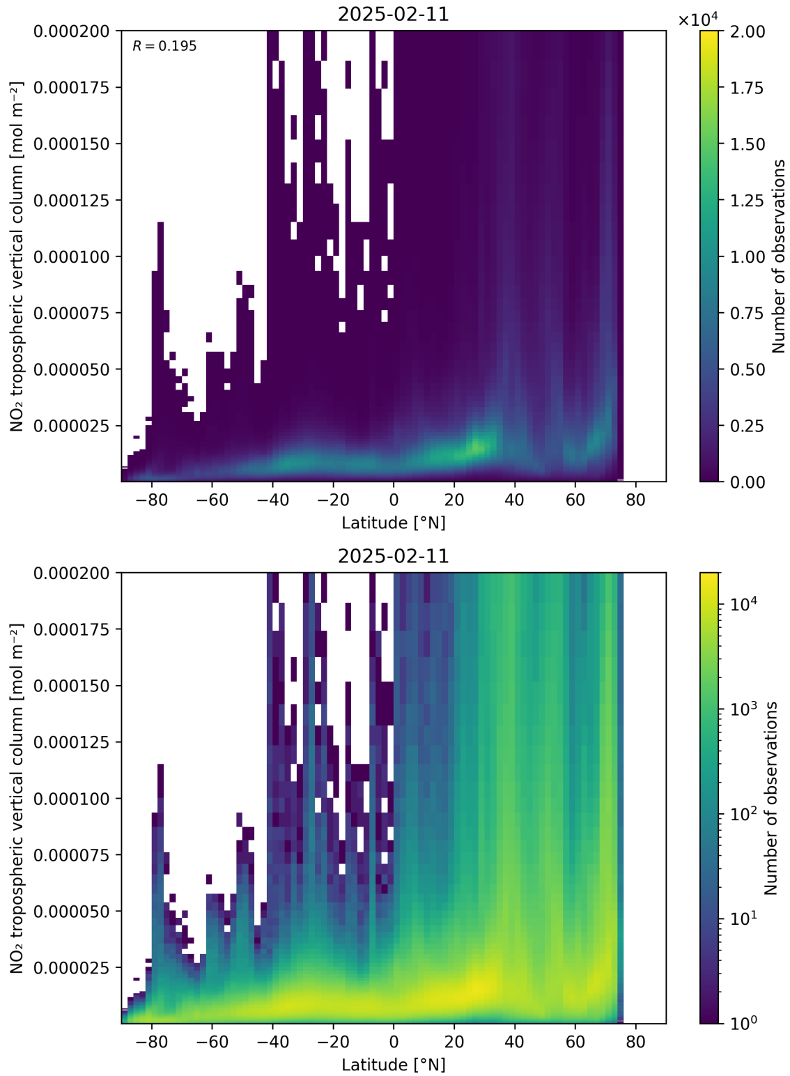
Figure 92: Scatter density plot of “Latitude” against “NO 2 tropospheric vertical column” for 2025-02-10 to 2025-02-12.
