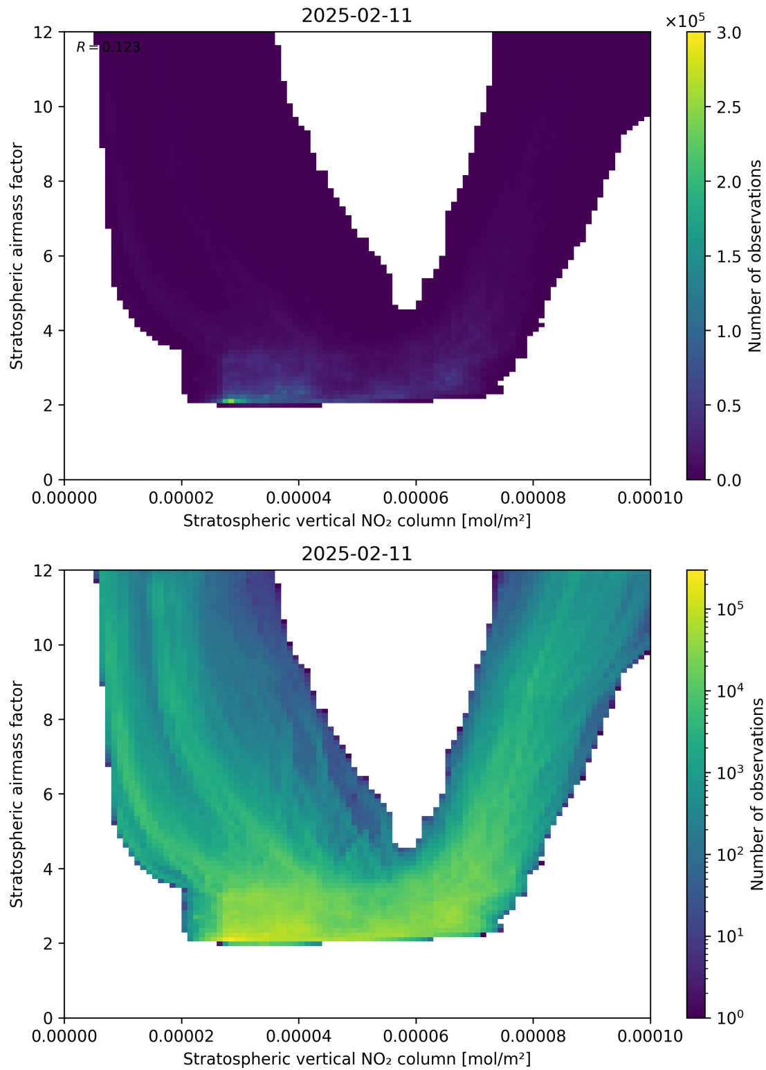
Figure 96: Scatter density plot of “Stratospheric vertical NO 2 column” against “Stratospheric airmass factor” for 2025-02-10 to 2025-02-12.
