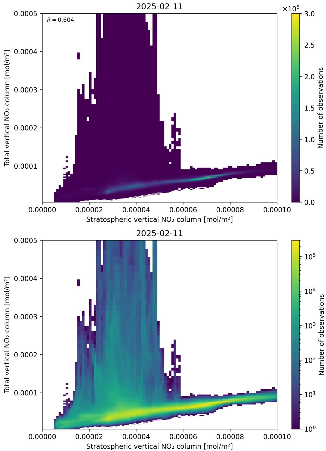
Figure 100: Scatter density plot of “Stratospheric vertical NO 2 column” against “Total vertical NO 2 column” for 2025-02-10 to 2025-02-12.
