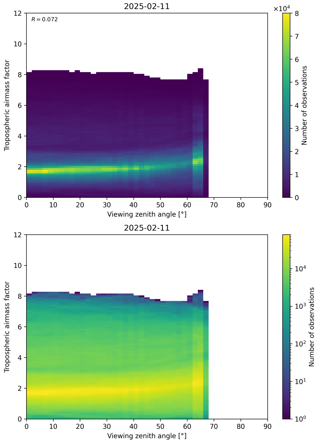
Figure 161: Scatter density plot of “Viewing zenith angle” against “Tropospheric airmass factor” for 2025-02-10 to 2025-02-12.
