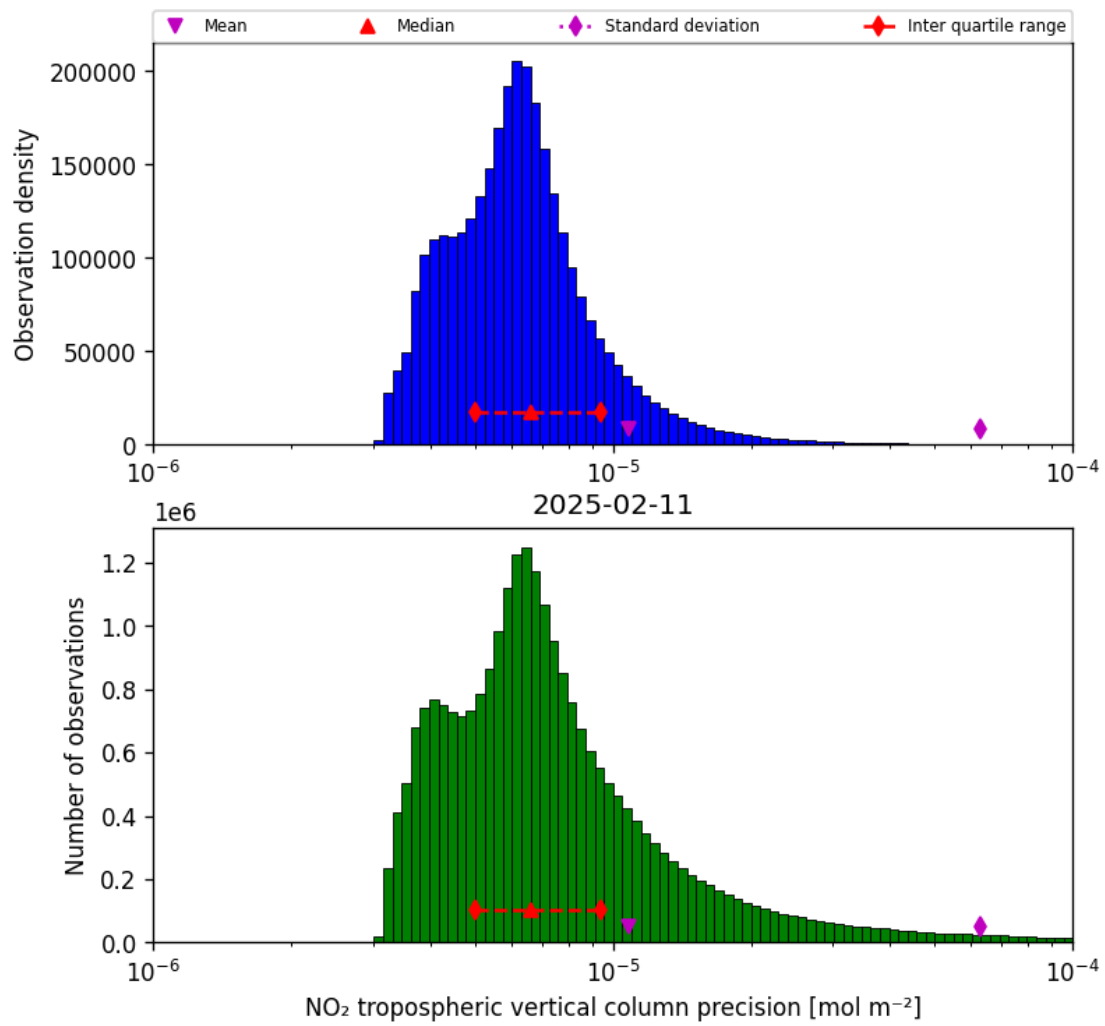
Figure 30: Histogram of “NO 2 tropospheric vertical column precision” for 2025-02-10 to 2025-02-12
