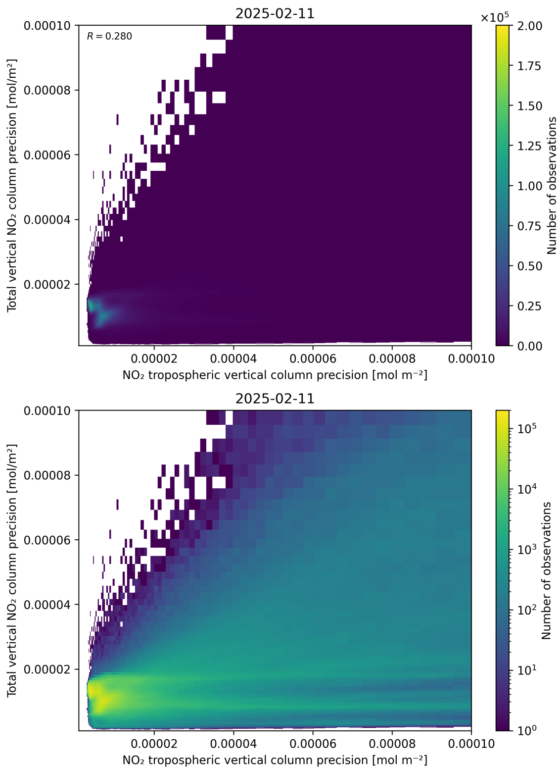
Figure 139: Scatter density plot of “NO 2 tropospheric vertical column precision” against “Total vertical NO 2 column precision” for 2025-02-10 to 2025-02-12.
