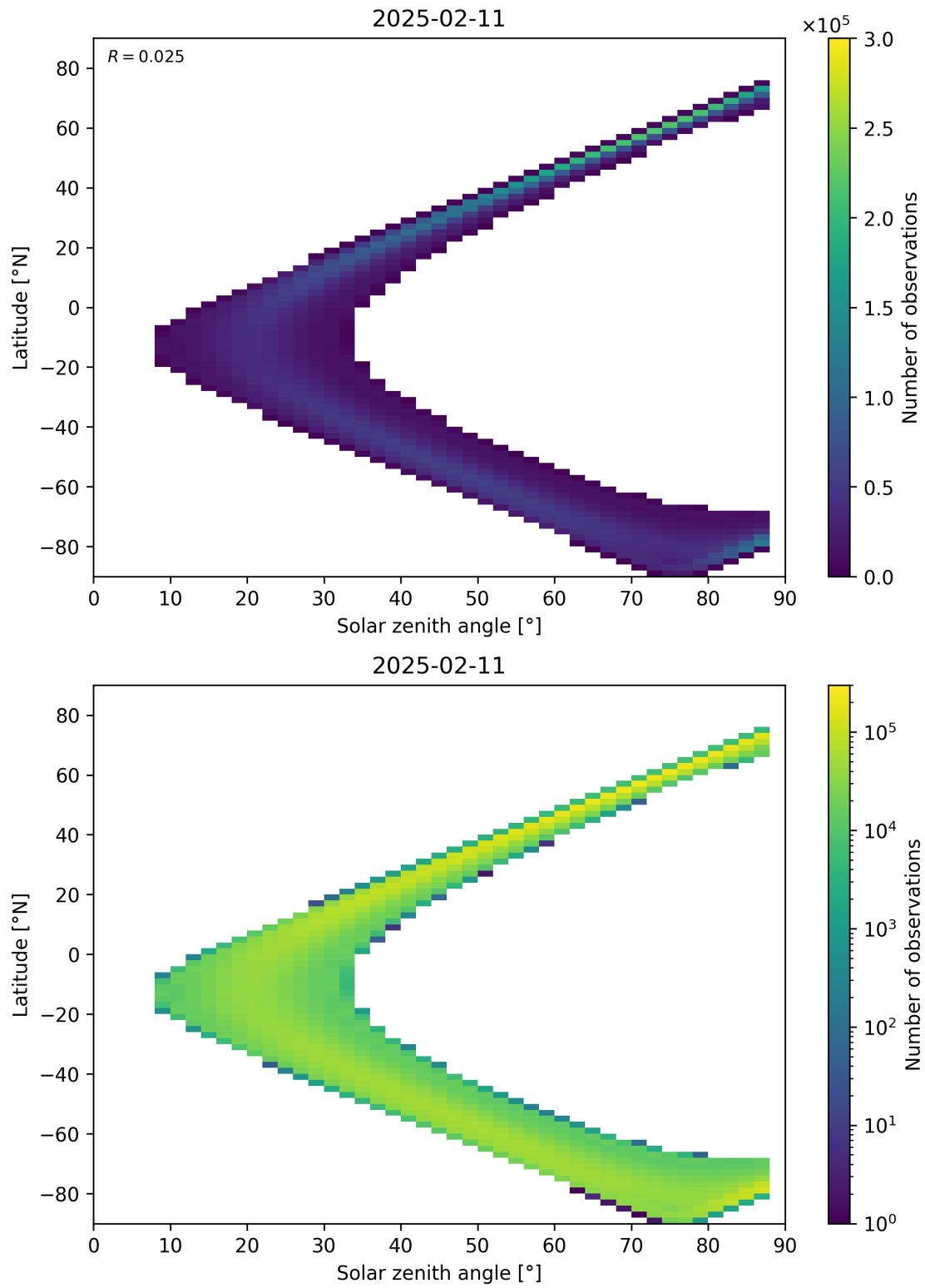
Figure 149: Scatter density plot of “Solar zenith angle” against “Latitude” for 2025-02-10 to 2025-02-12.
