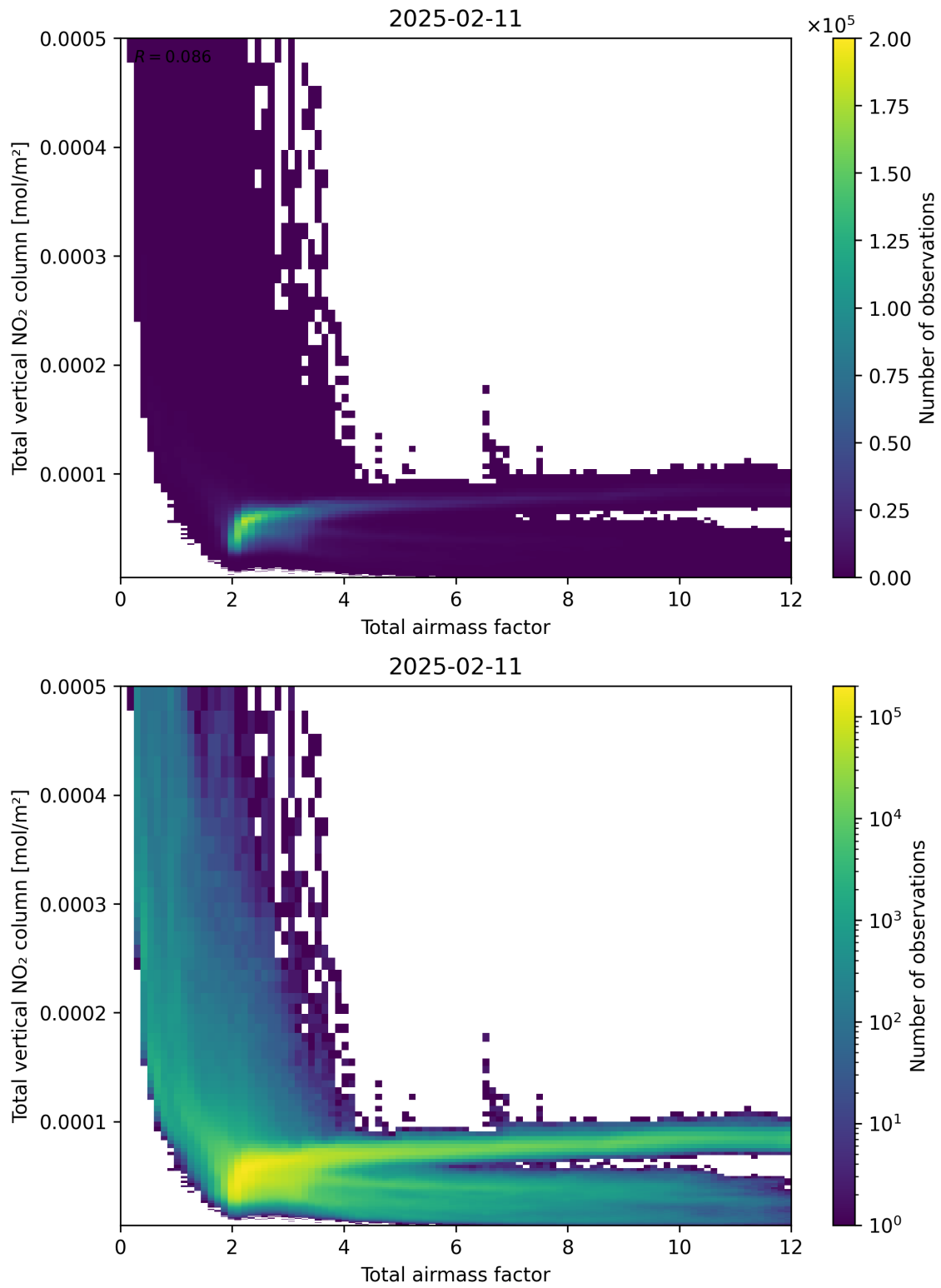
Figure 67: Scatter density plot of “Total airmass factor” against “Total vertical NO 2 column” for 2025-02-10 to 2025-02-12.
