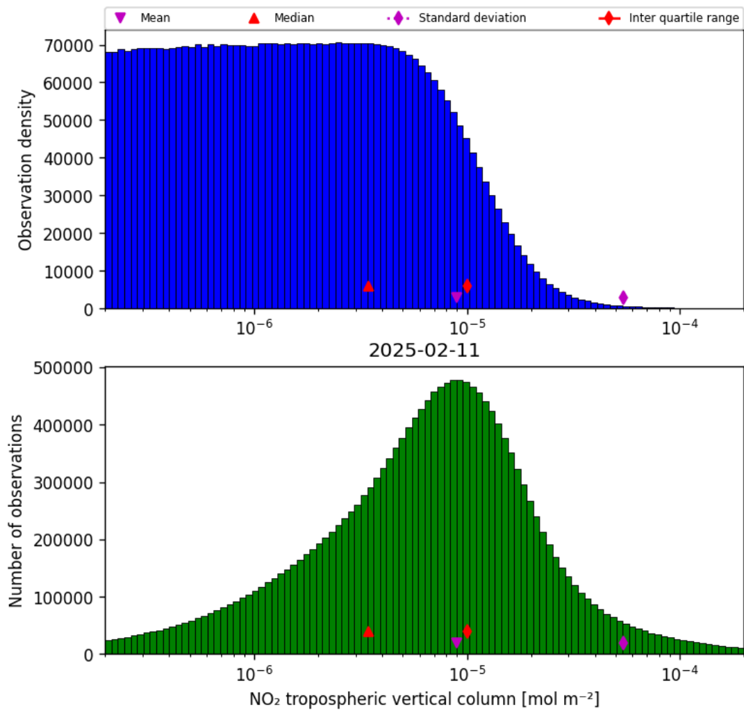
Figure 29: Histogram of “NO 2 tropospheric vertical column” for 2025-02-10 to 2025-02-12
