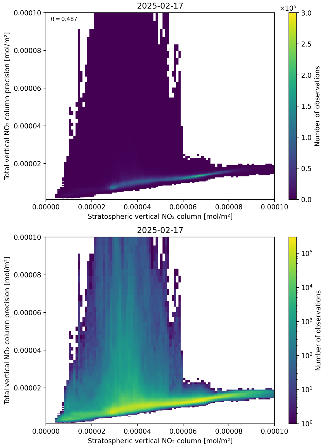
Figure 101: Scatter density plot of “Stratospheric vertical NO 2 column” against “Total vertical NO 2 column precision” for 2025-02-16 to 2025-02-18.
