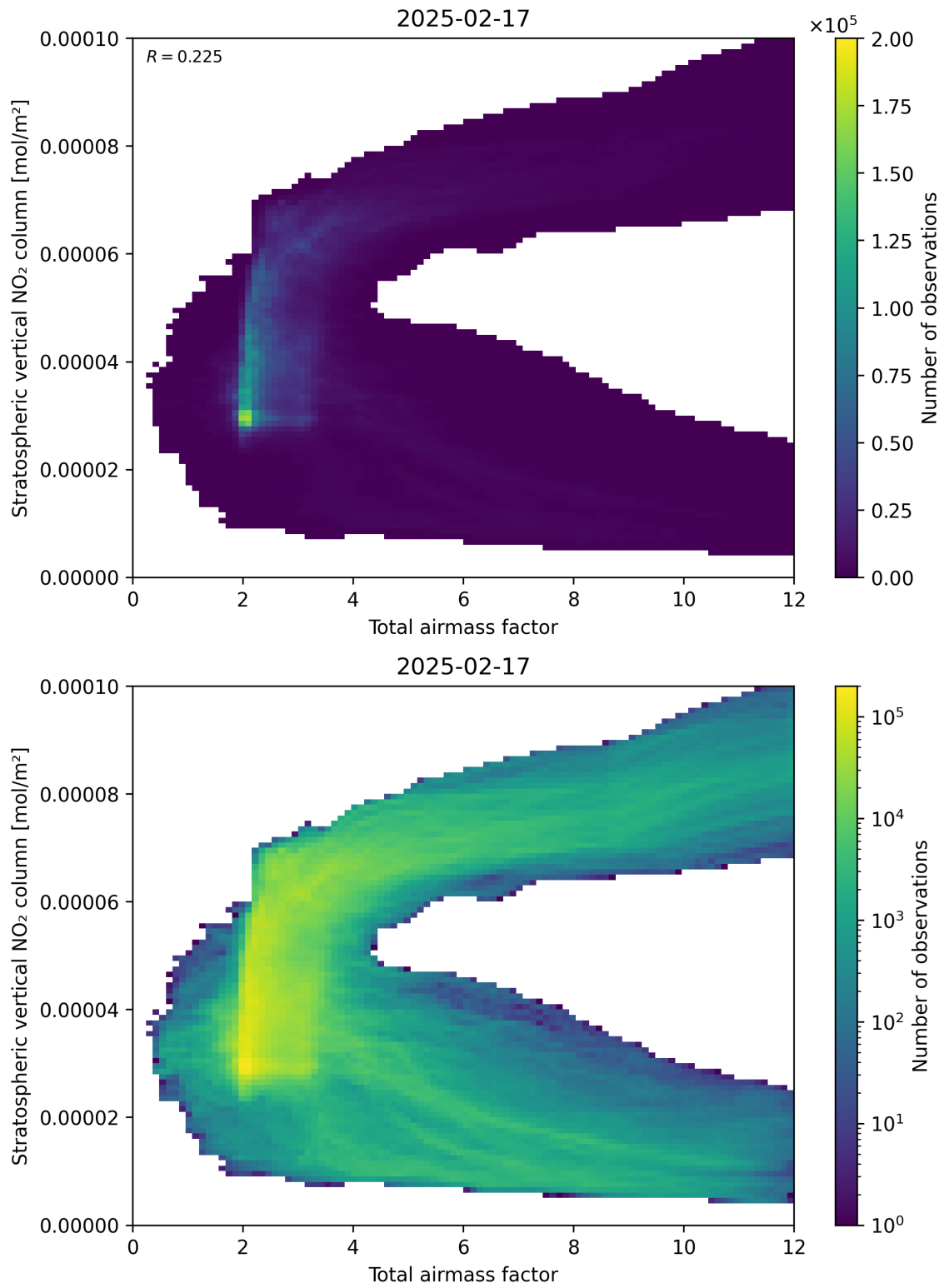
Figure 64: Scatter density plot of “Total airmass factor” against “Stratospheric vertical NO 2 column” for 2025-02-16 to 2025-02-18.
