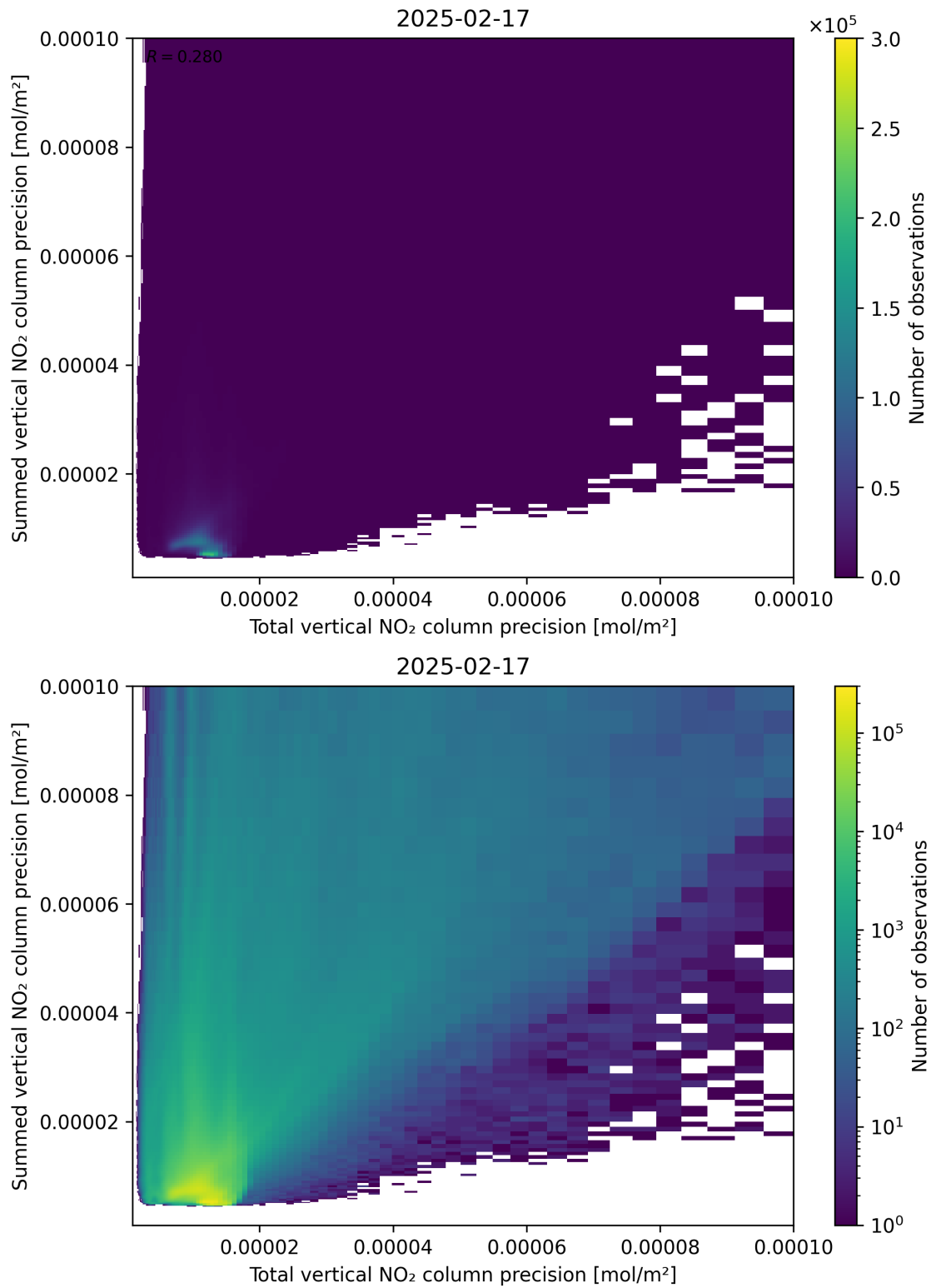
Figure 118: Scatter density plot of “Total vertical NO 2 column precision” against “Summed vertical NO 2 column precision” for 2025-02-16 to 2025-02-18.
