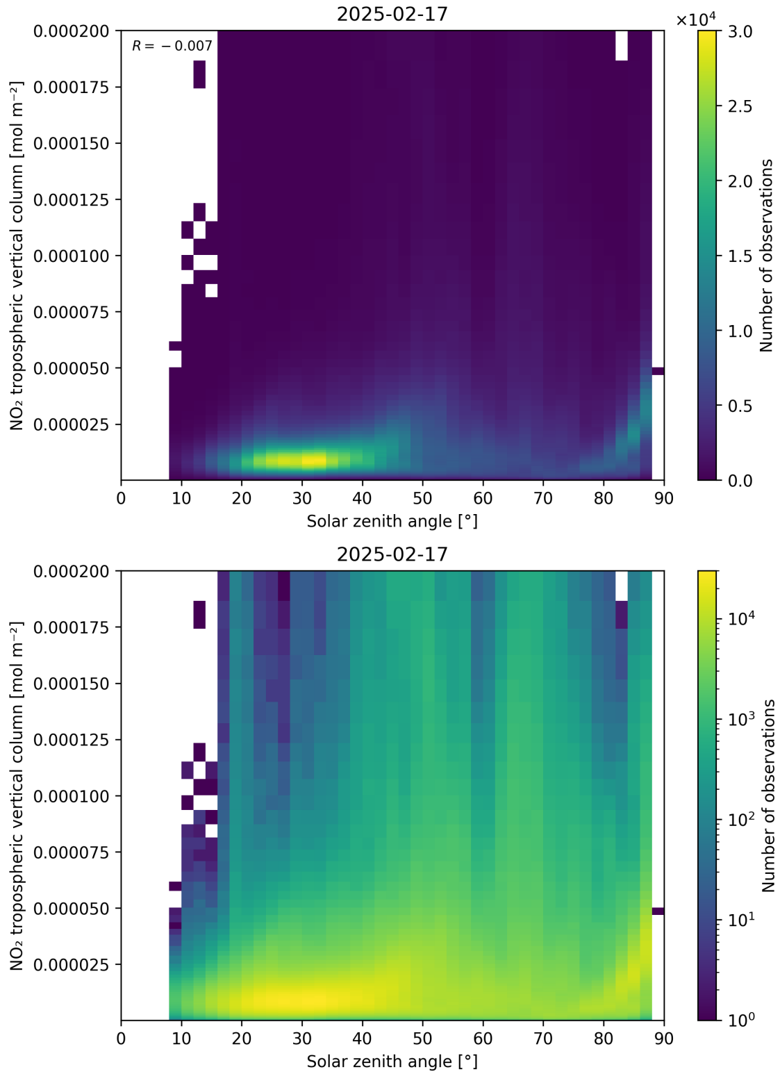
Figure 155: Scatter density plot of “Solar zenith angle” against “NO 2 tropospheric vertical column” for 2025-02-16 to 2025-02-18.
