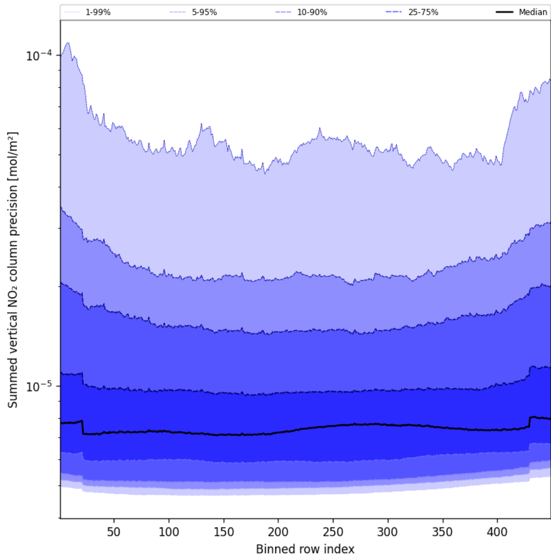
Figure 58: Along track statistics of “Summed vertical NO 2 column precision” for 2025-02-16 to 2025-02-18
