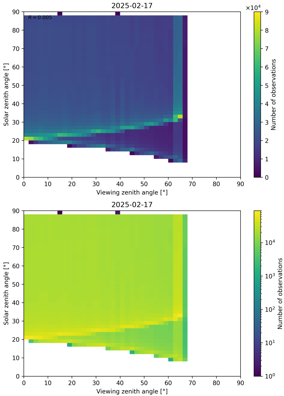
Figure 172: Scatter density plot of “Viewing zenith angle” against “Solar zenith angle” for 2025-02-16 to 2025-02-18.
