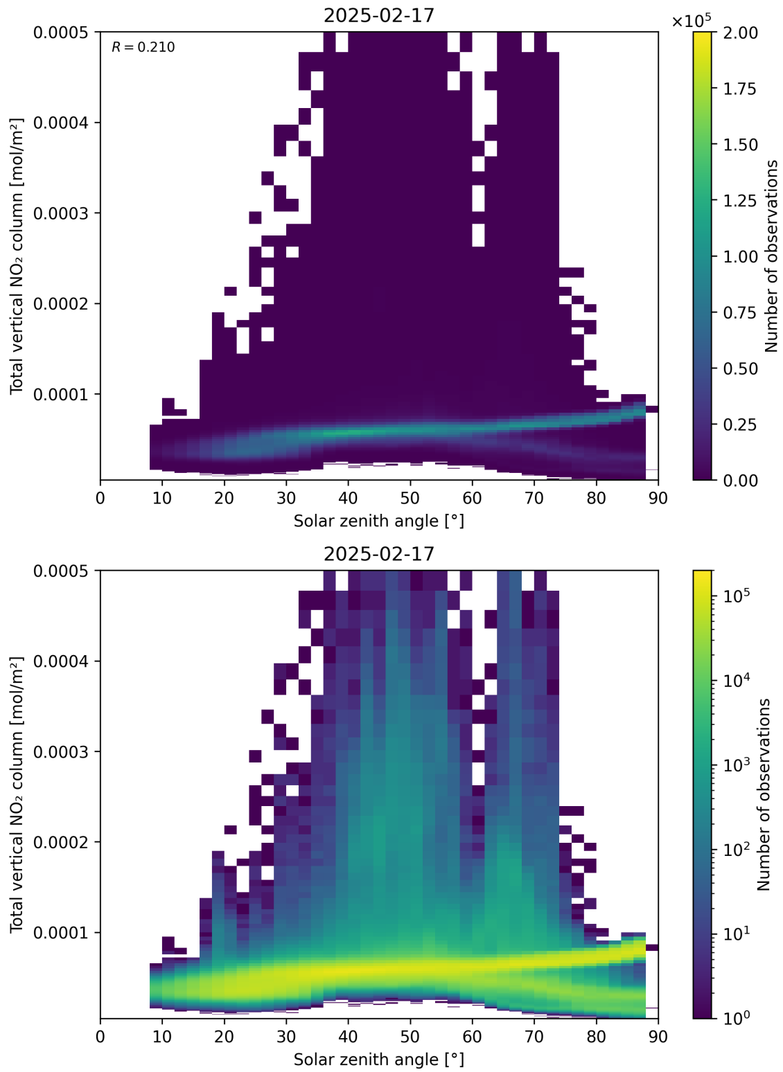
Figure 153: Scatter density plot of “Solar zenith angle” against “Total vertical NO 2 column” for 2025-02-16 to 2025-02-18.
