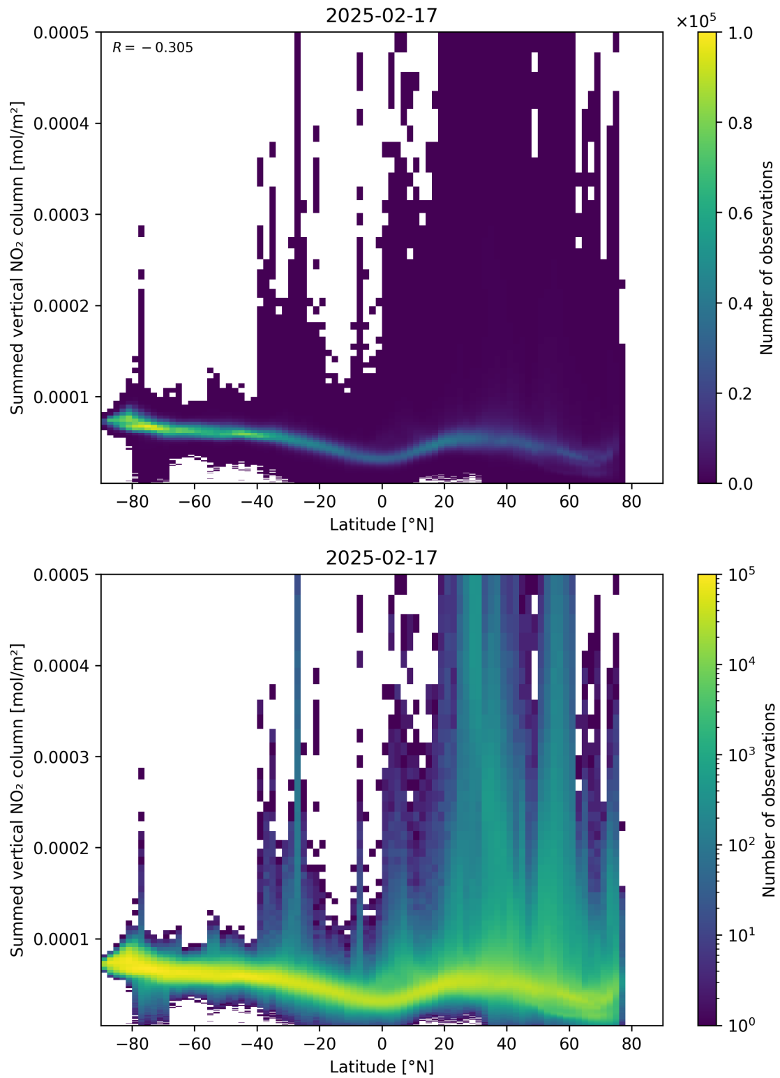
Figure 88: Scatter density plot of “Latitude” against “Summed vertical NO 2 column” for 2025-02-16 to 2025-02-18.
