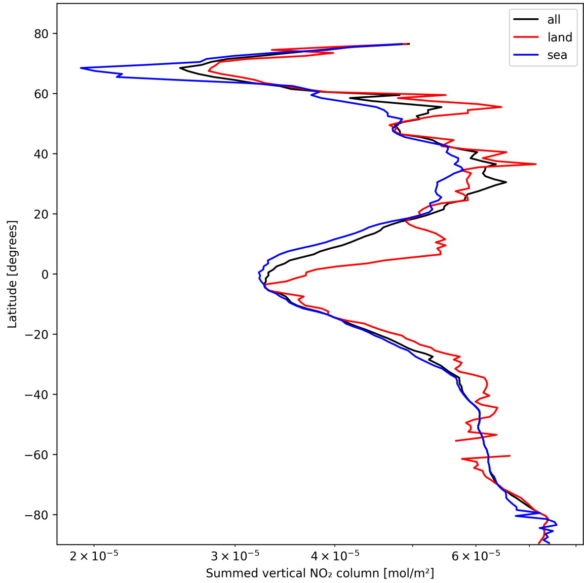
Figure 23: Zonal average of “Summed vertical NO 2 column” for 2025-02-16 to 2025-02-18.
