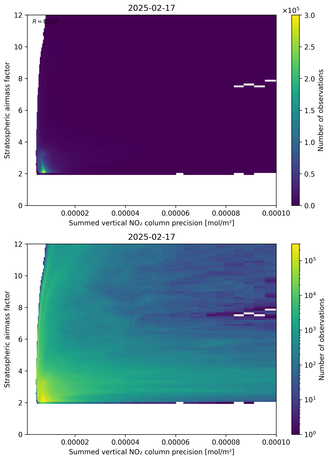
Figure 106: Scatter density plot of “Summed vertical NO 2 column precision” against “Stratospheric airmass factor” for 2025-02-16 to 2025-02-18.
