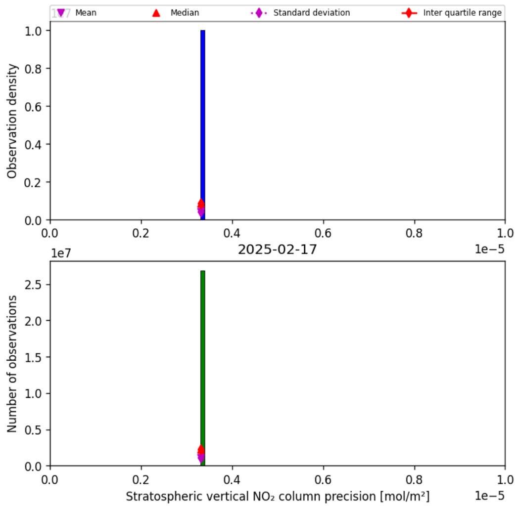
Figure 37: Histogram of “Stratospheric vertical NO 2 column precision” for 2025-02-16 to 2025-02-18
