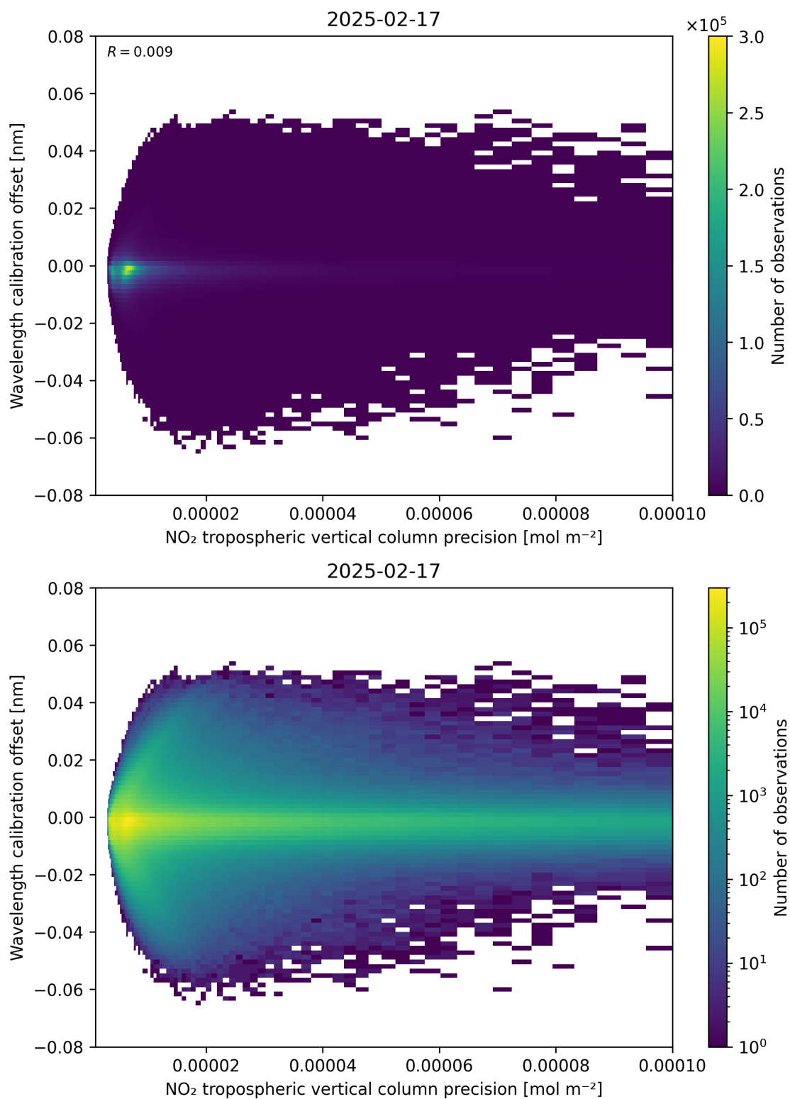
Figure 141: Scatter density plot of “NO 2 tropospheric vertical column precision” against “Wavelength calibration offset” for 2025-02-16 to 2025-02-18.
