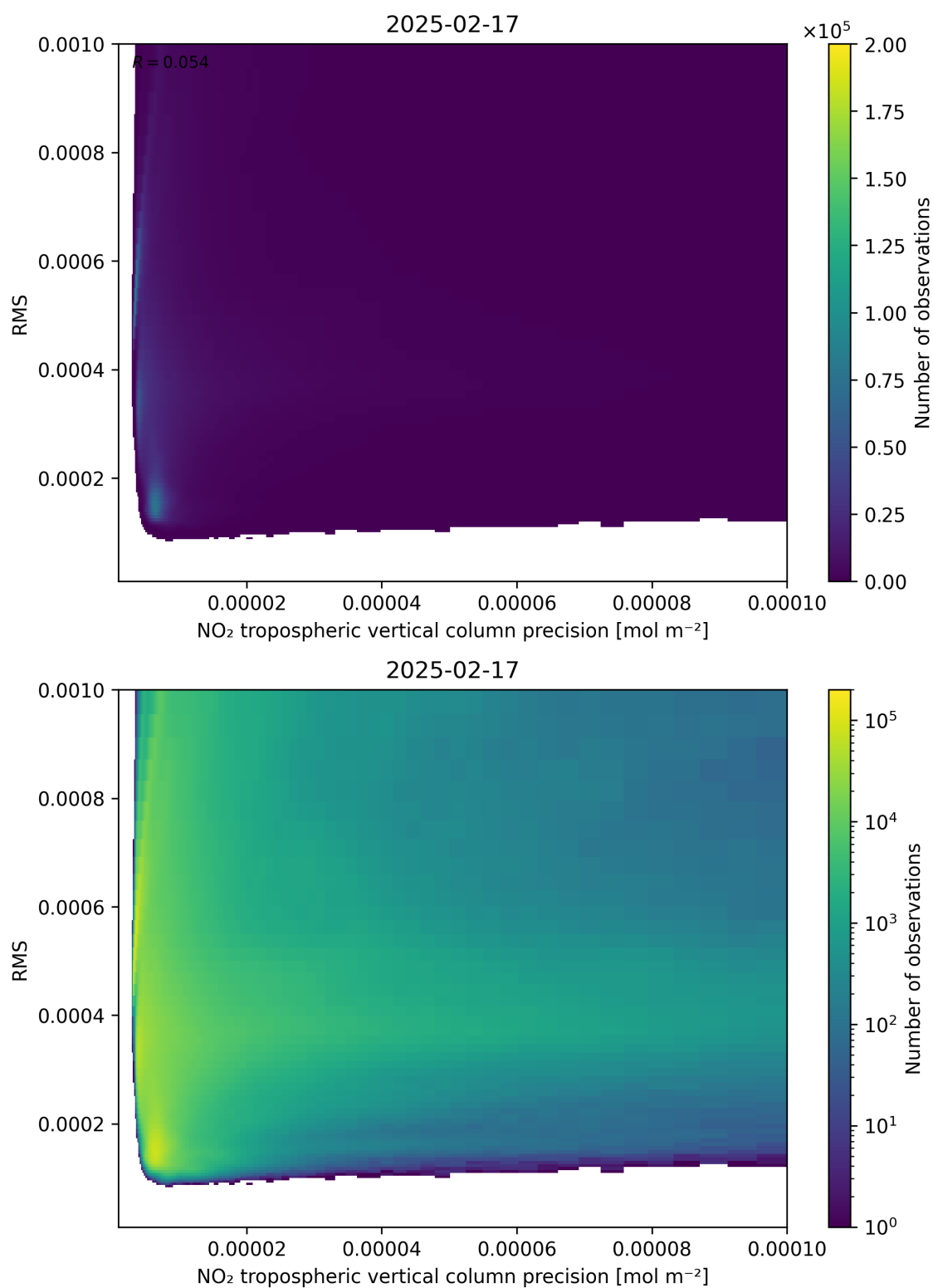
Figure 140: Scatter density plot of “NO 2 tropospheric vertical column precision” against “RMS” for 2025-02-16 to 2025-02-18.
