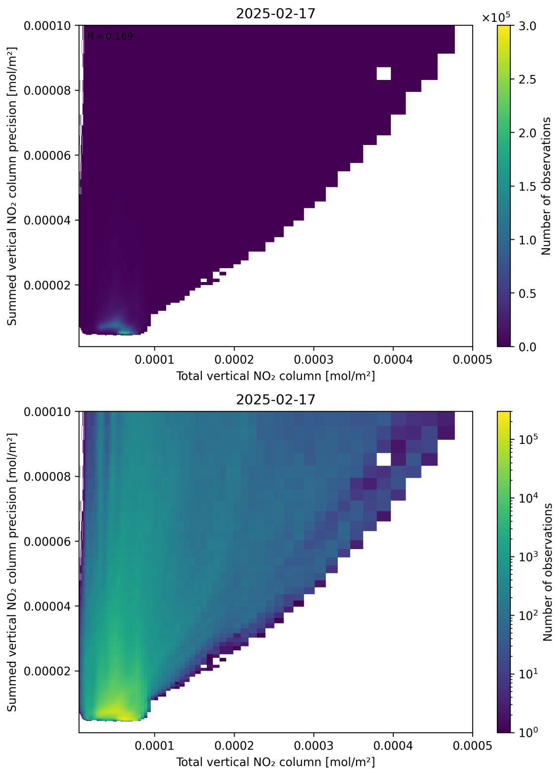
Figure 113: Scatter density plot of “Total vertical NO 2 column” against “Summed vertical NO 2 column precision” for 2025-02-16 to 2025-02-18.
