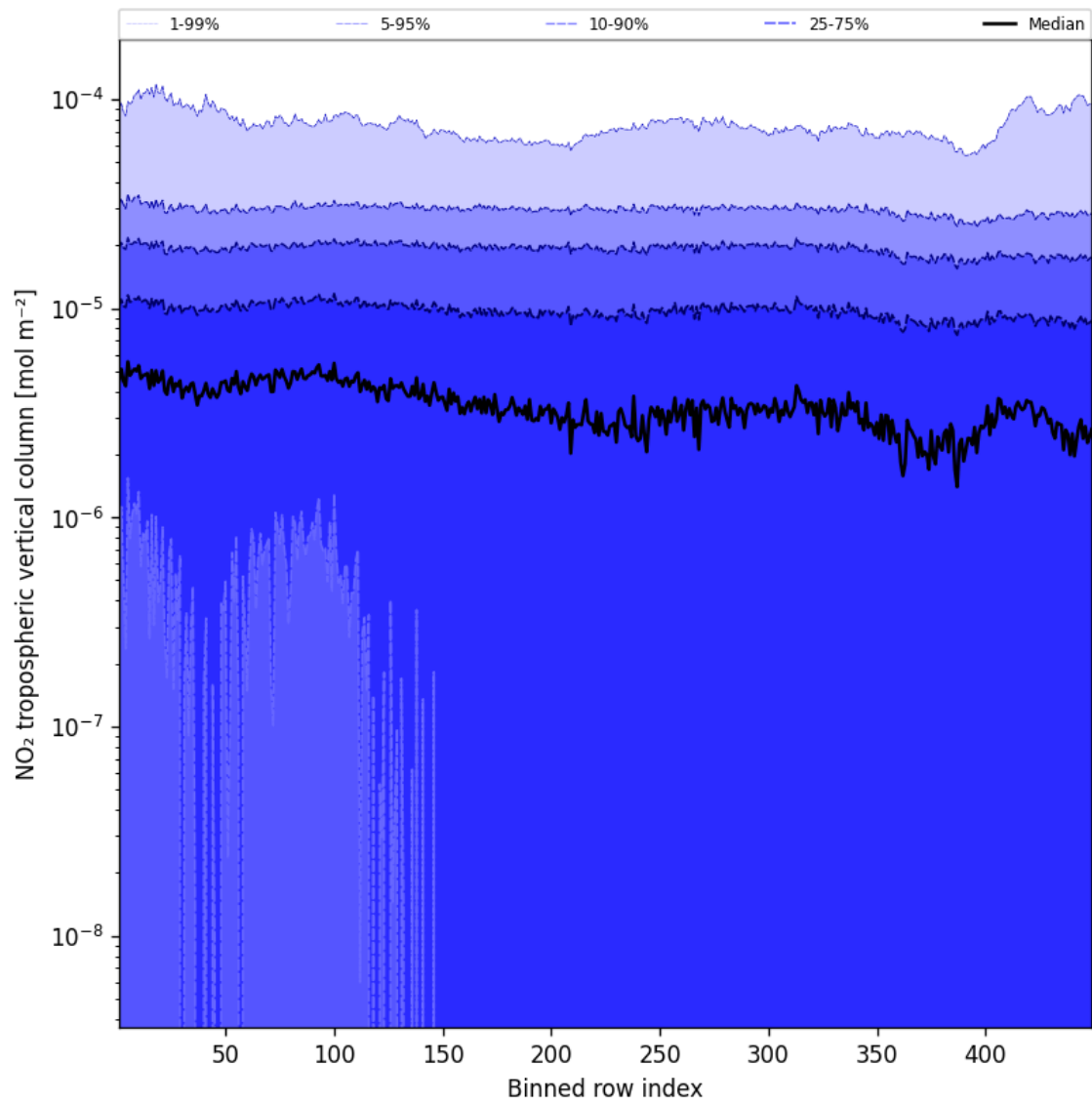
Figure 46: Along track statistics of “NO 2 tropospheric vertical column” for 2025-02-16 to 2025-02-18
