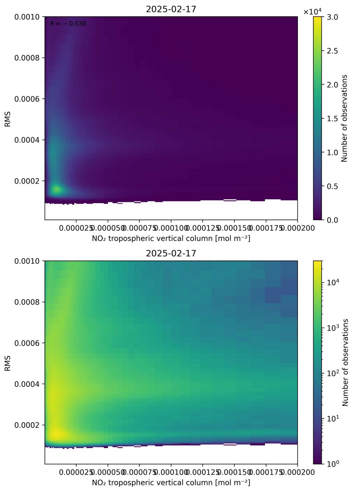
Figure 142: Scatter density plot of “NO 2 tropospheric vertical column” against “RMS” for 2025-02-16 to 2025-02-18.
