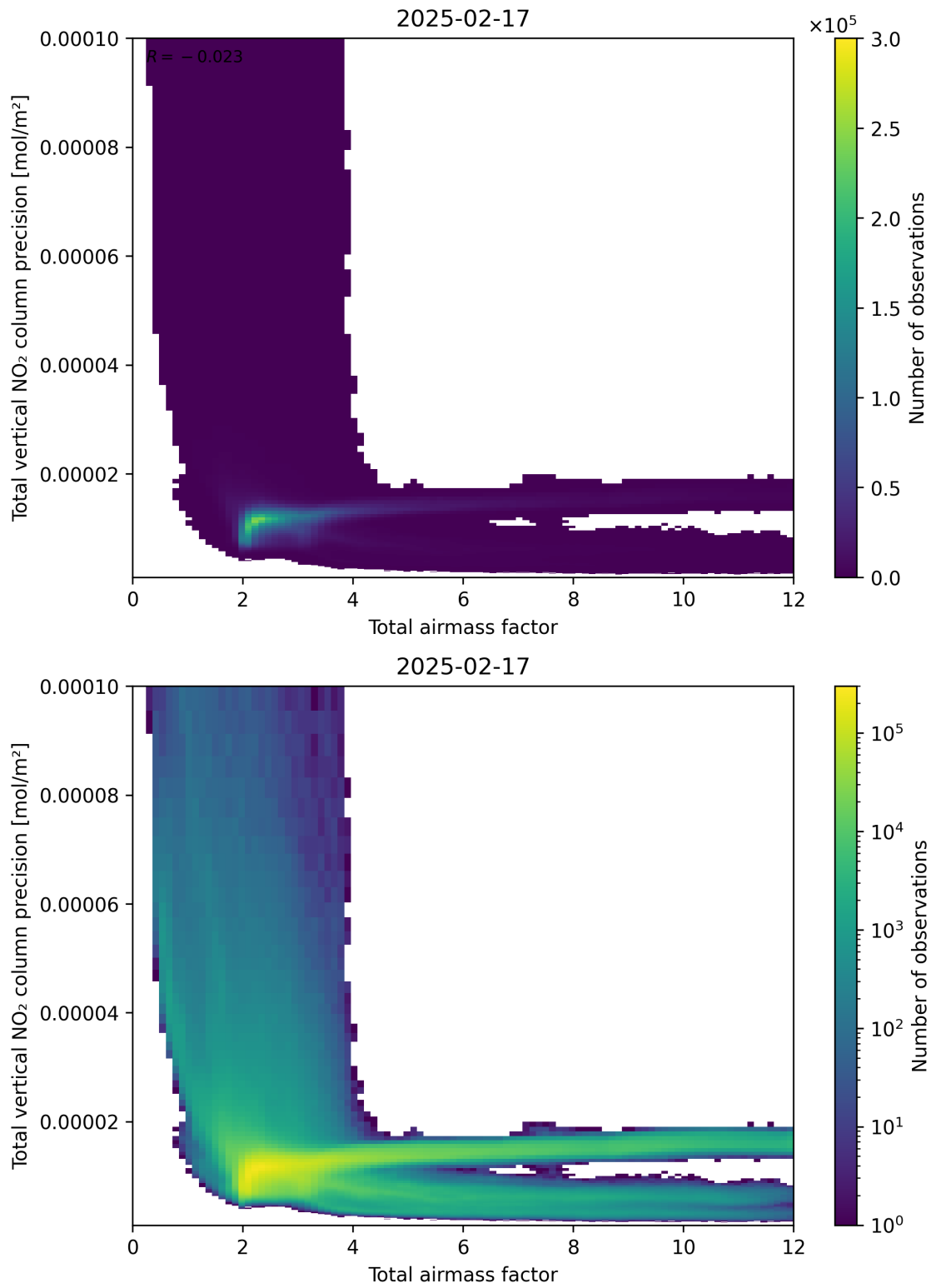
Figure 68: Scatter density plot of “Total airmass factor” against “Total vertical NO 2 column precision” for 2025-02-16 to 2025-02-18.
