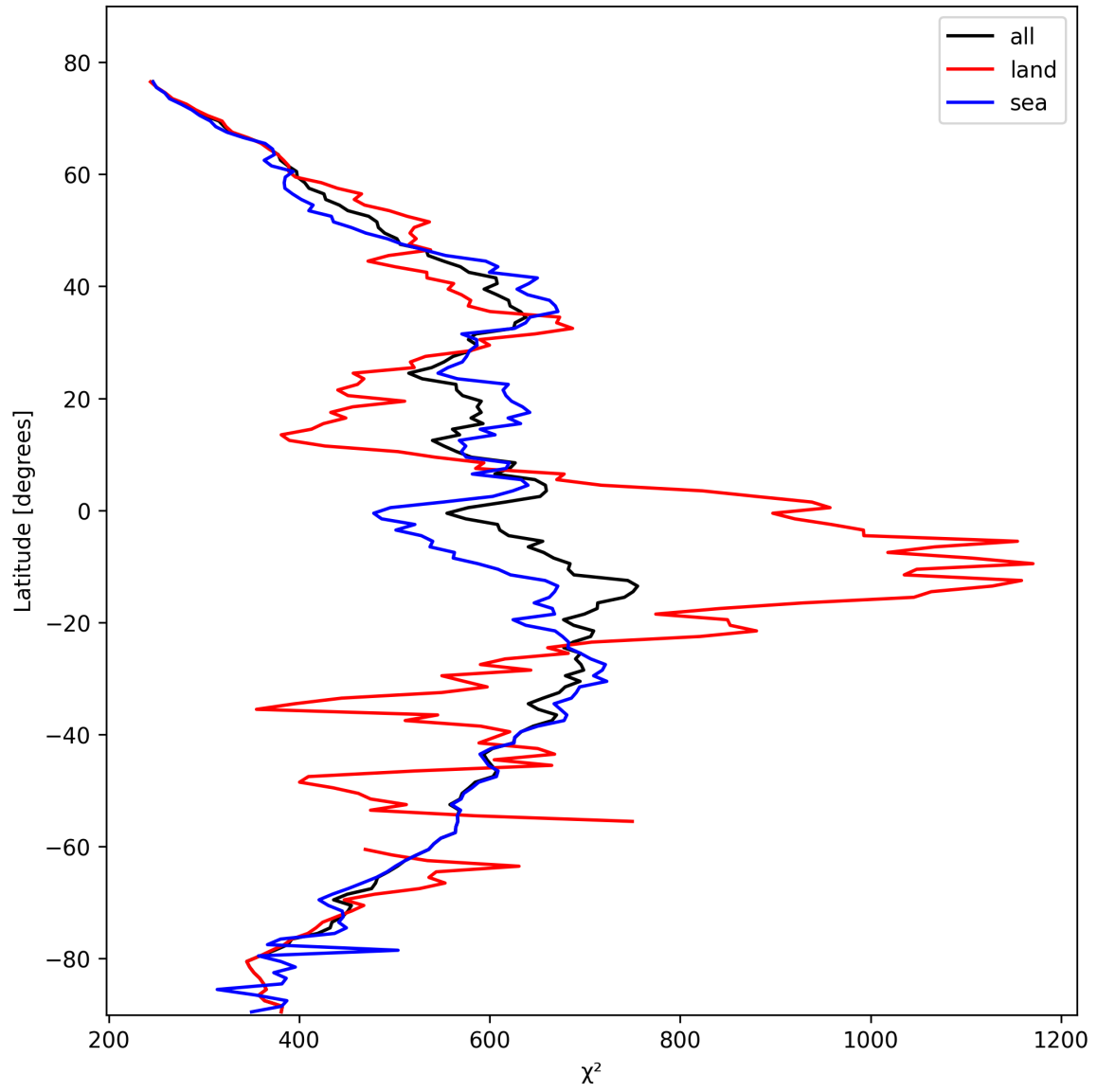
Figure 25: Zonal average of “ \chi^2 ” for 2025-02-16 to 2025-02-18.
