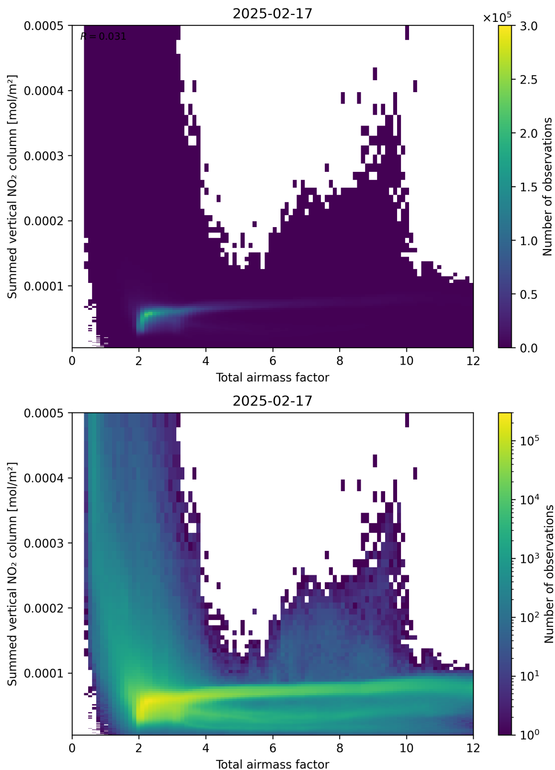
Figure 65: Scatter density plot of “Total airmass factor” against “Summed vertical NO 2 column” for 2025-02-16 to 2025-02-18.
