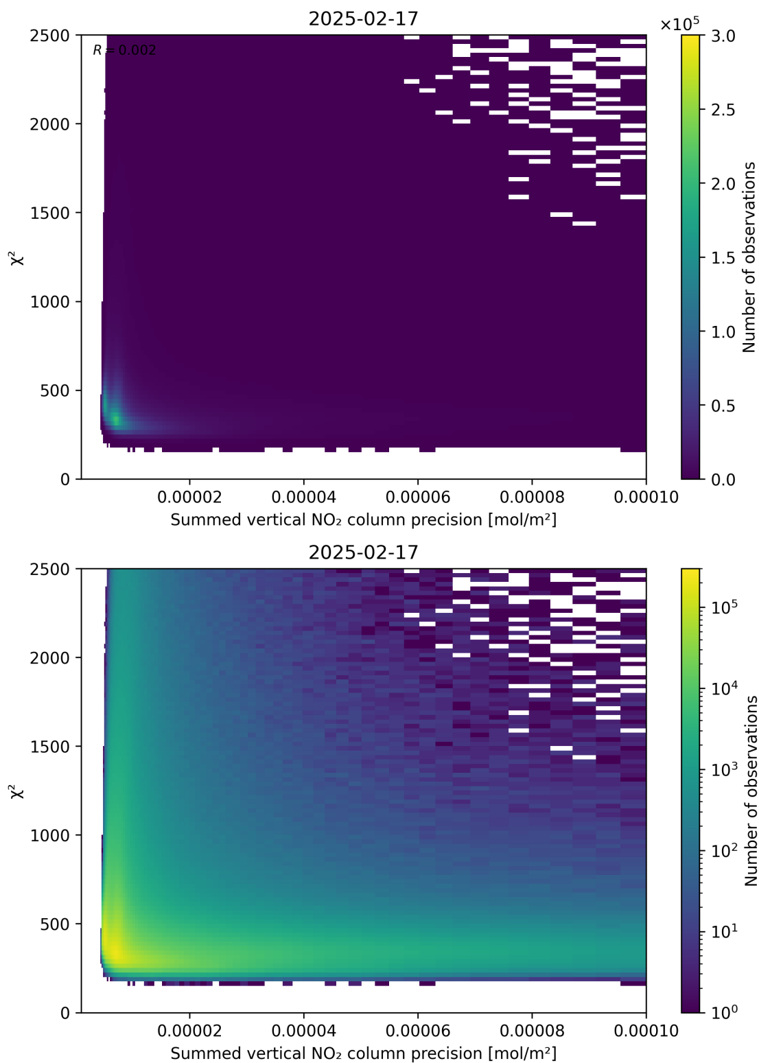
Figure 107: Scatter density plot of “Summed vertical NO 2 column precision” against “ \chi^2 ” for 2025-02-16 to 2025-02-18.
