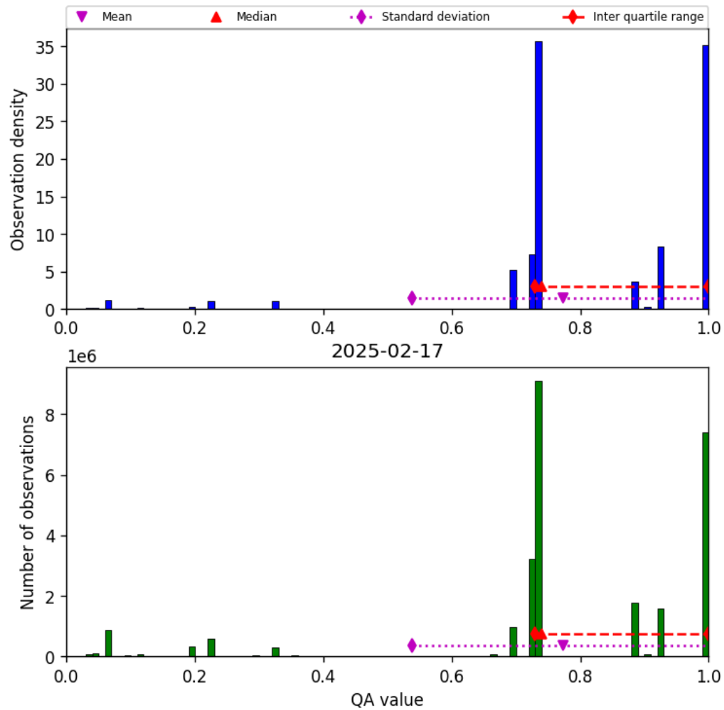
Figure 28: Histogram of “QA value” for 2025-02-16 to 2025-02-18
