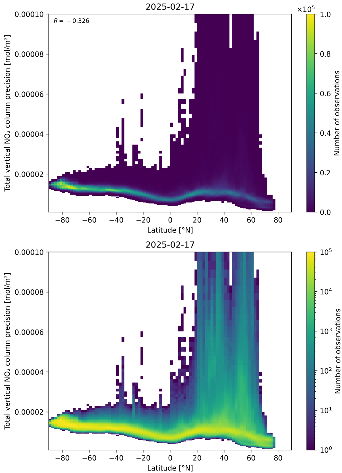
Figure 91: Scatter density plot of “Latitude” against “Total vertical NO 2 column precision” for 2025-02-16 to 2025-02-18.
