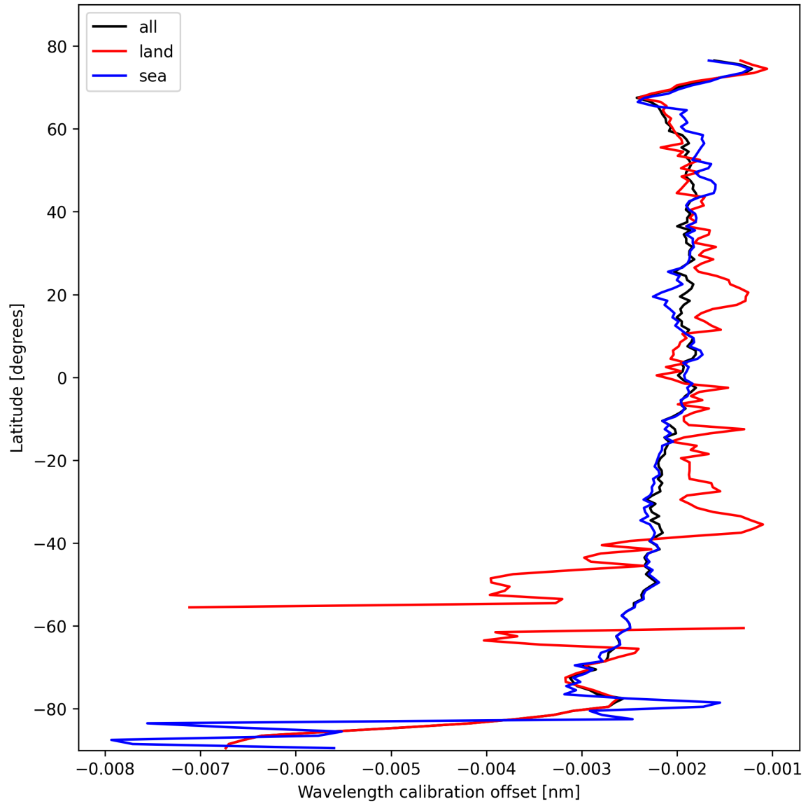
Figure 18: Zonal average of “Wavelength calibration offset” for 2025-02-16 to 2025-02-18.
