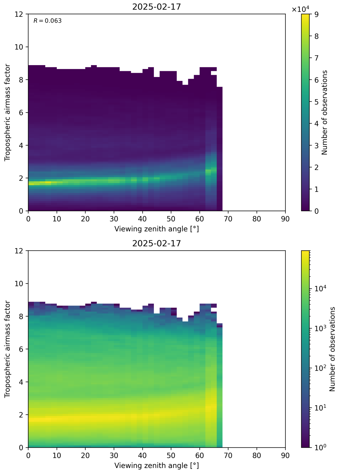
Figure 161: Scatter density plot of “Viewing zenith angle” against “Tropospheric airmass factor” for 2025-02-16 to 2025-02-18.
