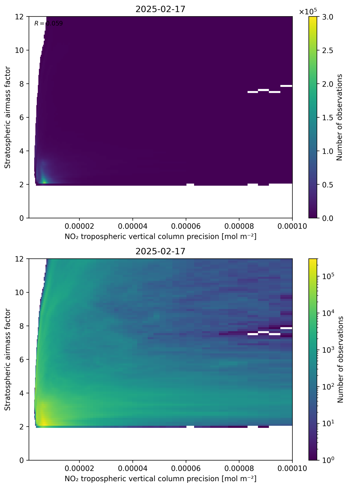
Figure 131: Scatter density plot of “NO 2 tropospheric vertical column precision” against “Stratospheric airmass factor” for 2025-02-16 to 2025-02-18.
