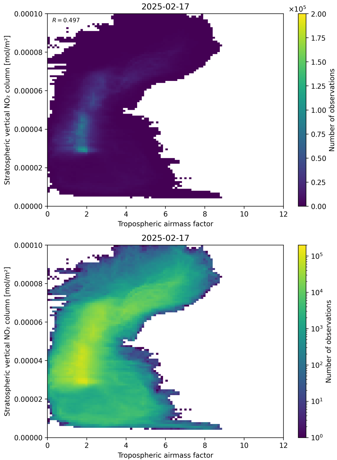
Figure 74: Scatter density plot of “Tropospheric air mass factor” against “Stratospheric vertical NO 2 column” for 2025-02-16 to 2025-02-18.
