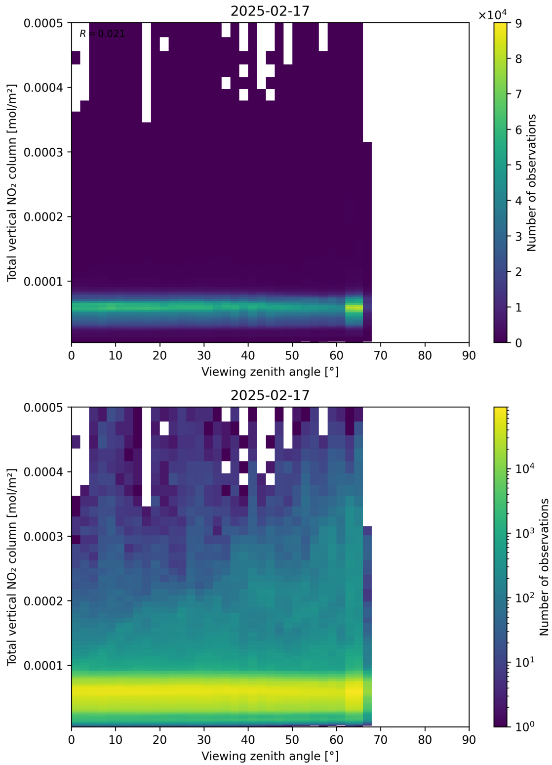
Figure 167: Scatter density plot of “Viewing zenith angle” against “Total vertical NO 2 column” for 2025-02-16 to 2025-02-18.
