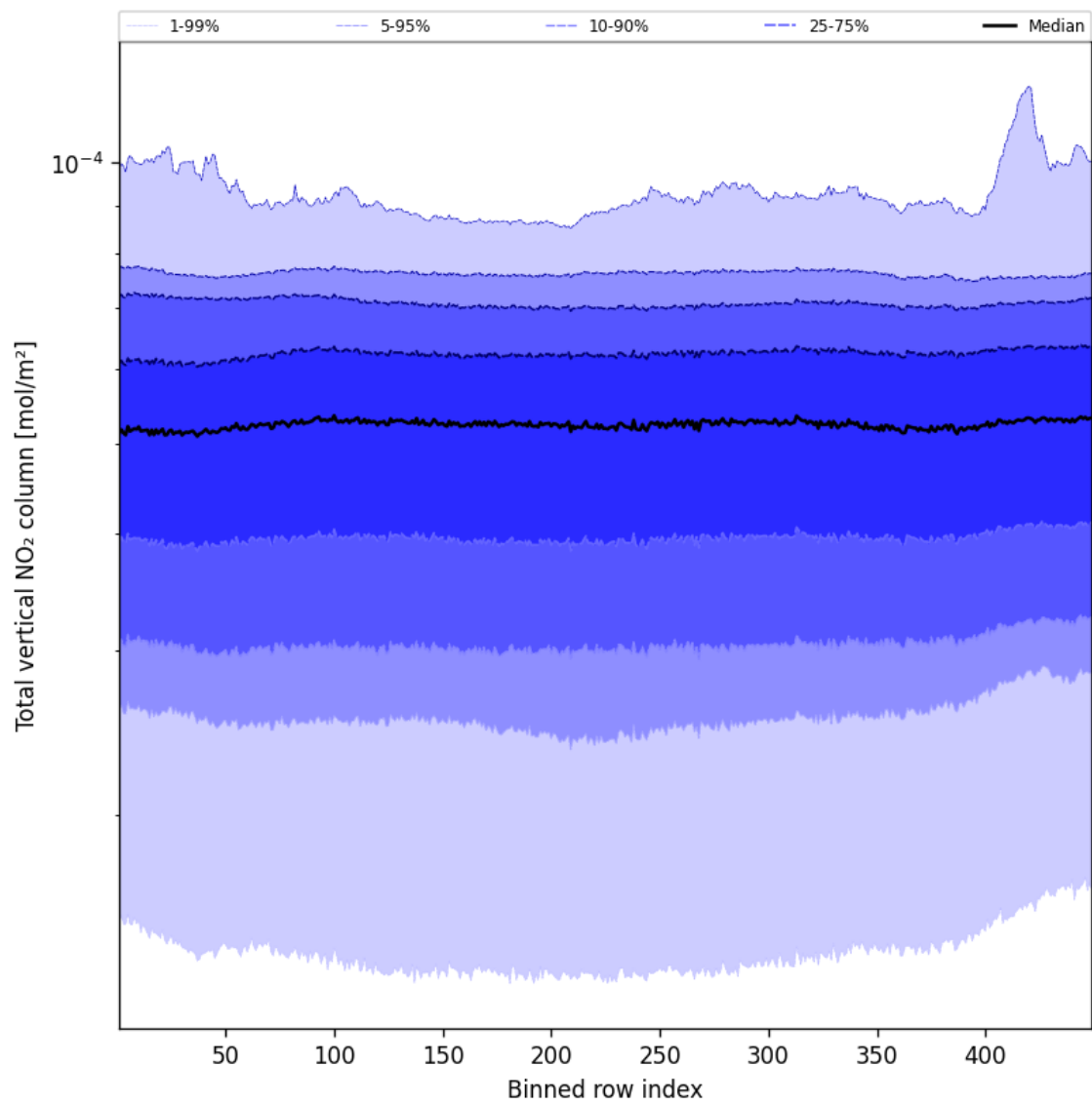
Figure 55: Along track statistics of “Total vertical NO 2 column” for 2025-02-16 to 2025-02-18
