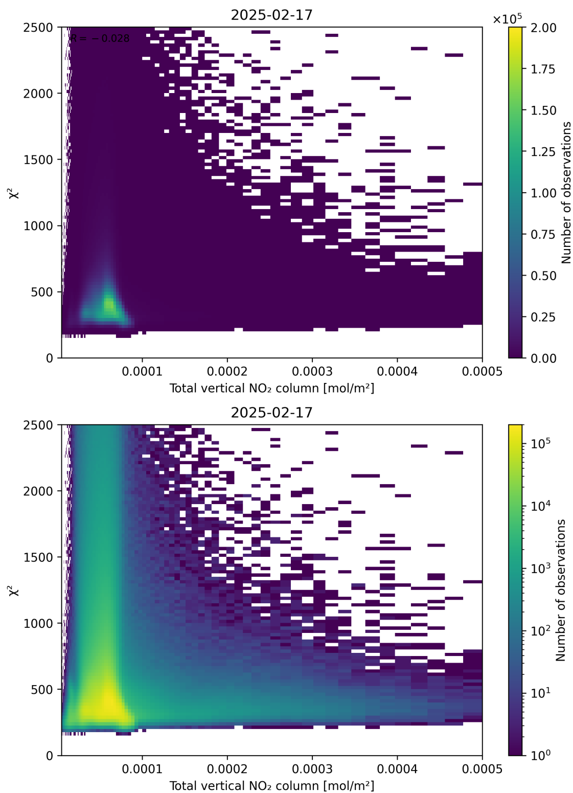
Figure 111: Scatter density plot of “Total vertical NO 2 column” against “ \chi^2 ” for 2025-02-16 to 2025-02-18.
