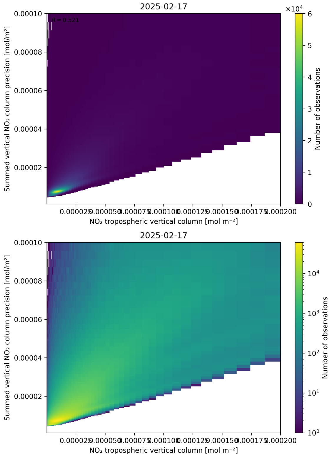
Figure 127: Scatter density plot of “NO 2 tropospheric vertical column” against “Summed vertical NO 2 column precision” for 2025-02-16 to 2025-02-18.
