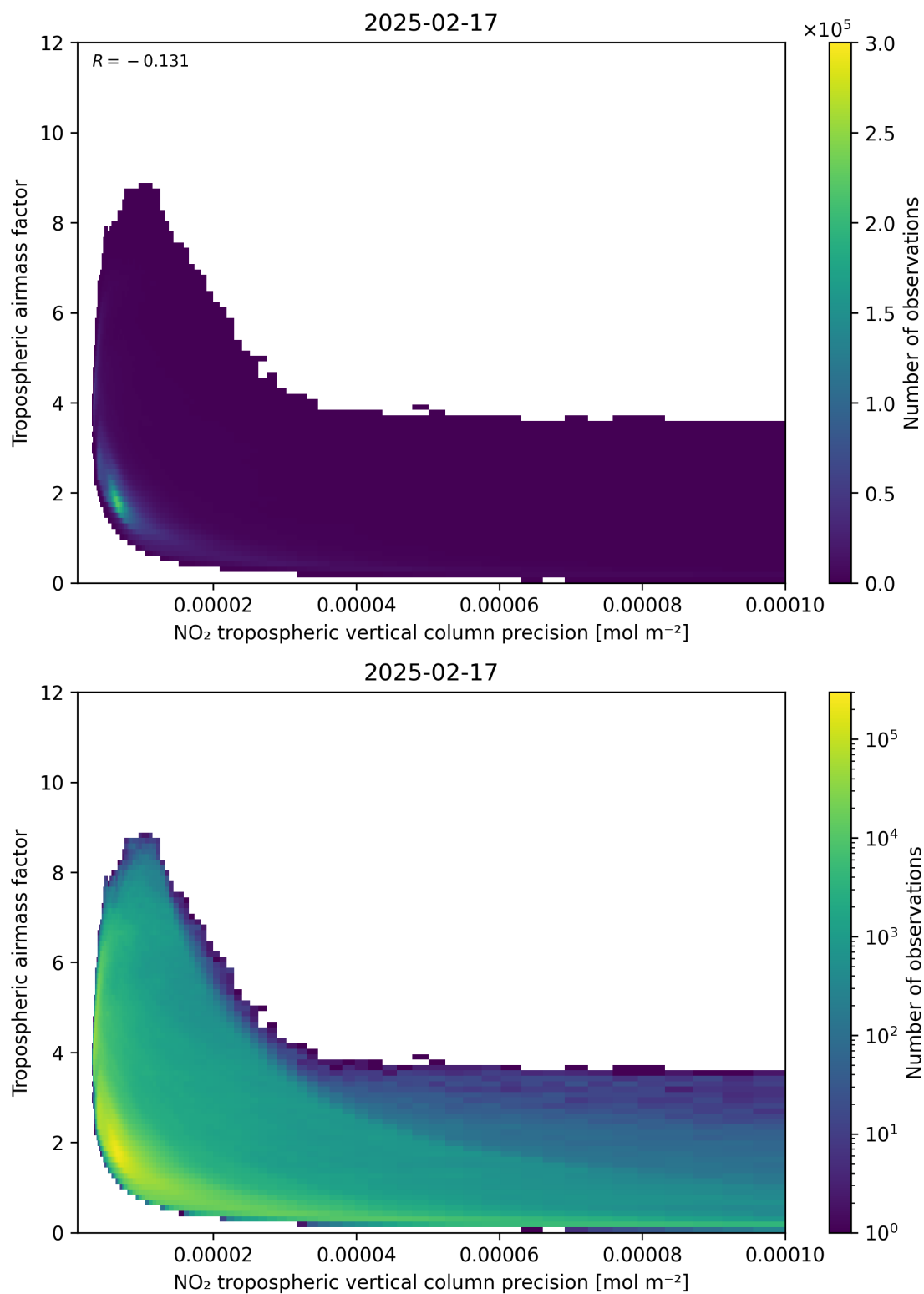
Figure 133: Scatter density plot of “NO 2 tropospheric vertical column precision” against “Tropospheric air mass factor” for 2025-02-16 to 2025-02-18.
