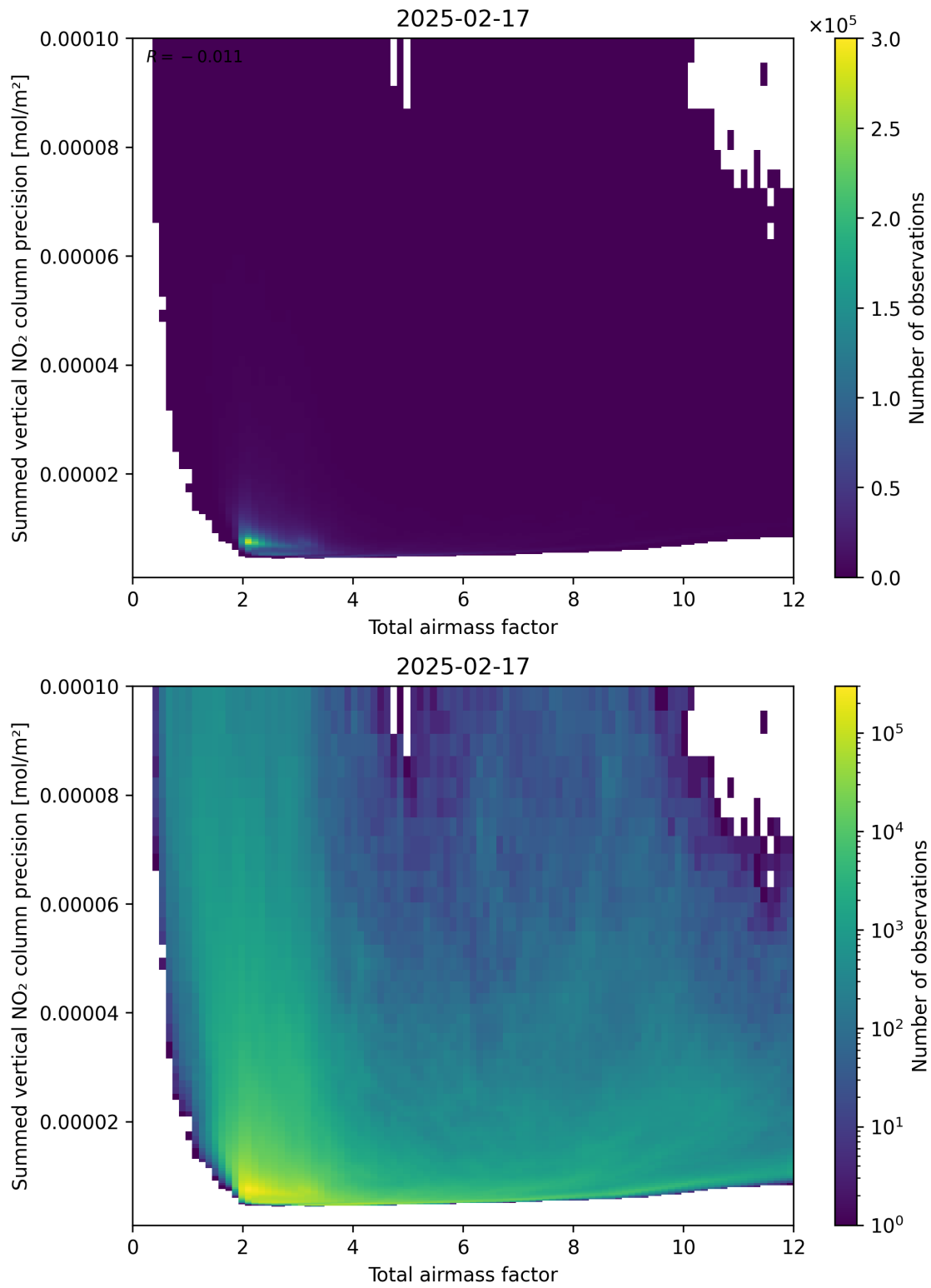
Figure 66: Scatter density plot of “Total airmass factor” against “Summed vertical NO 2 column precision” for 2025-02-16 to 2025-02-18.
