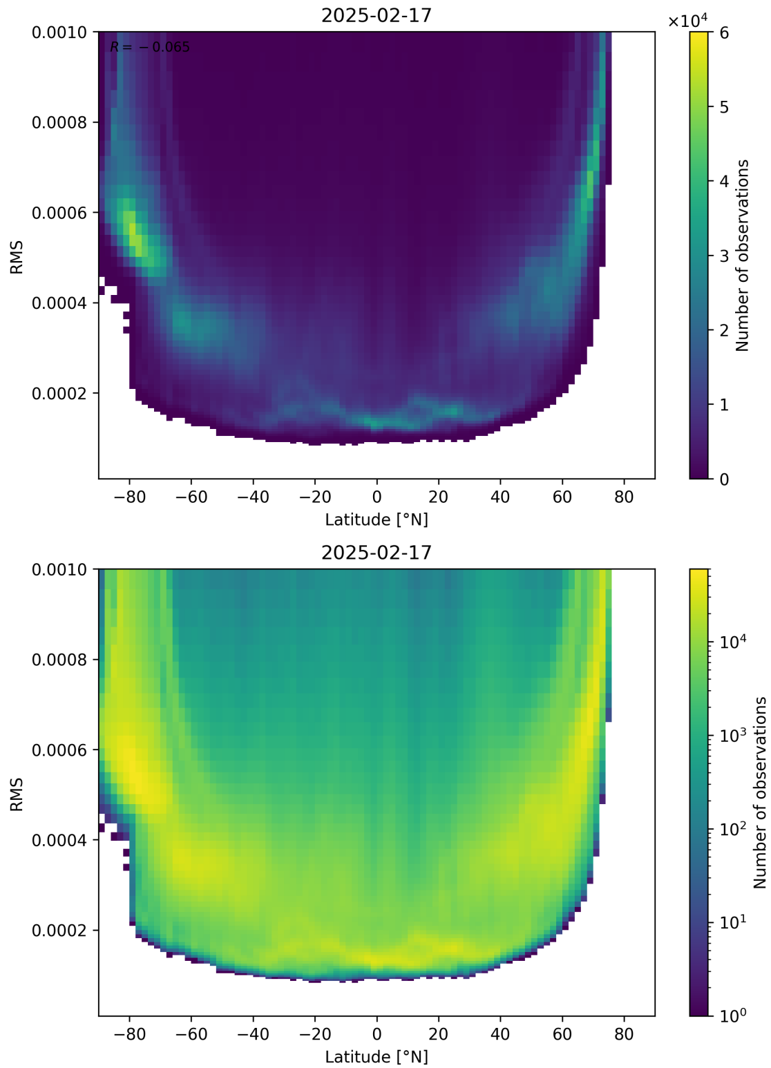
Figure 94: Scatter density plot of “Latitude” against “RMS” for 2025-02-16 to 2025-02-18.
