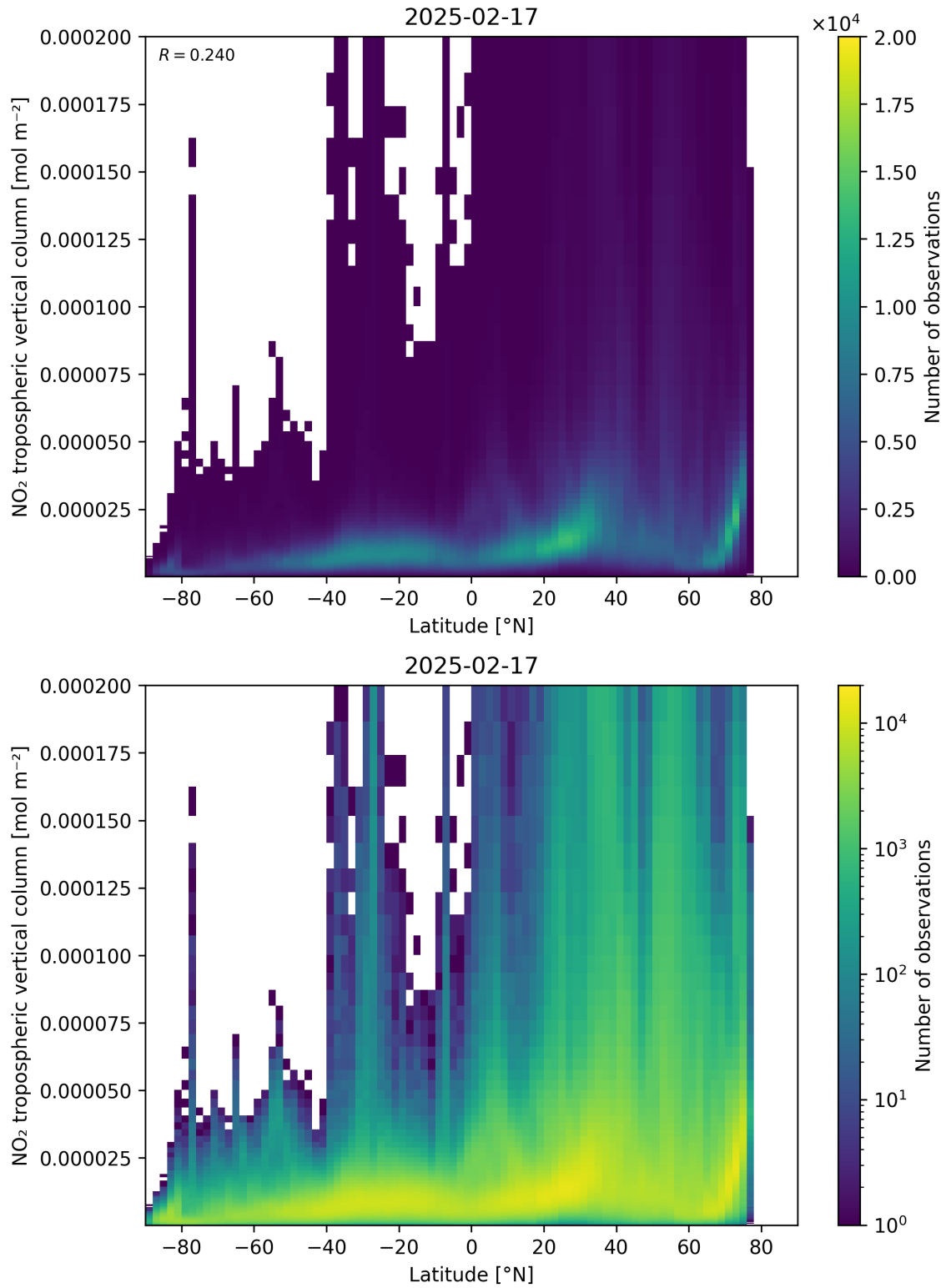
Figure 92: Scatter density plot of “Latitude” against “NO 2 tropospheric vertical column” for 2025-02-16 to 2025-02-18.
