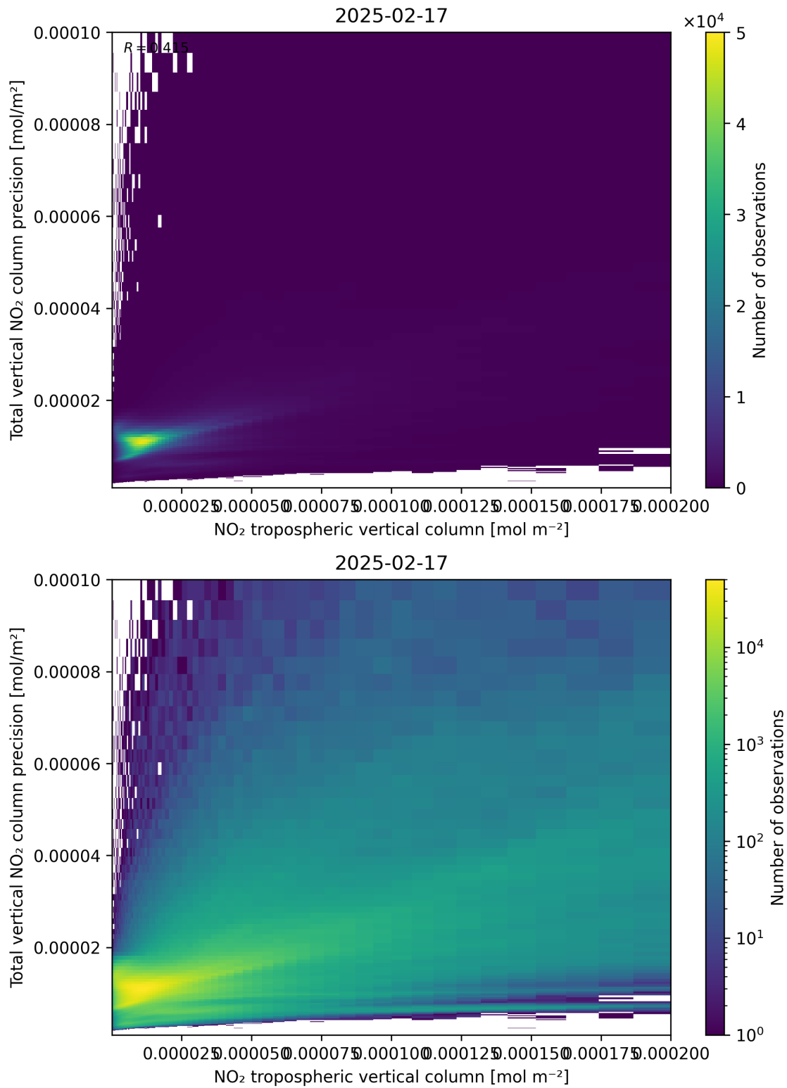
Figure 129: Scatter density plot of “NO 2 tropospheric vertical column” against “Total vertical NO 2 column precision” for 2025-02-16 to 2025-02-18.
