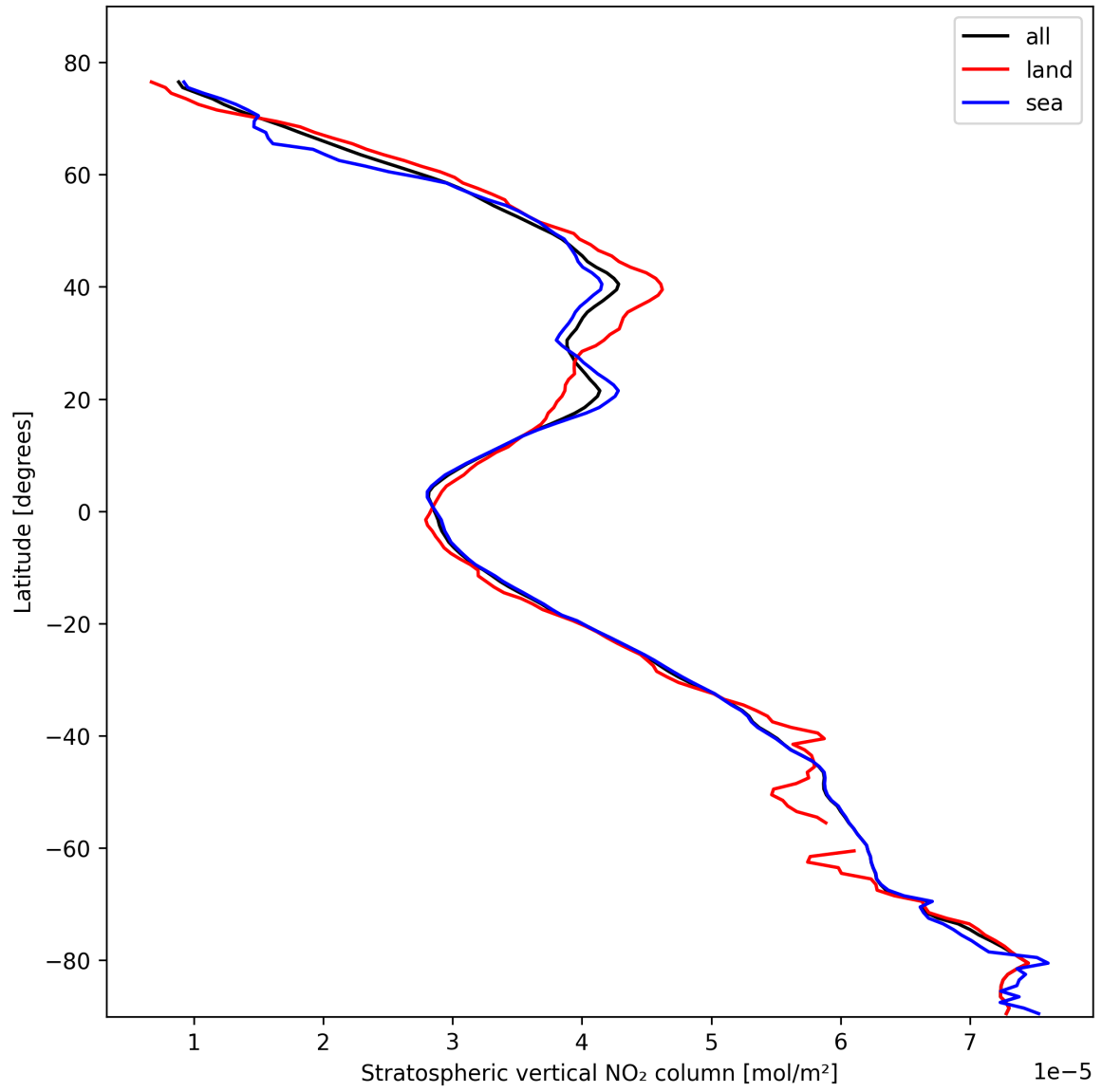
Figure 19: Zonal average of “Stratospheric vertical NO 2 column” for 2025-02-16 to 2025-02-18.
