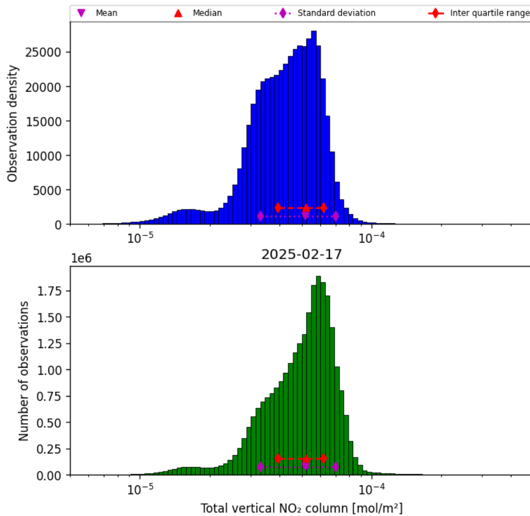
Figure 38: Histogram of “Total vertical NO 2 column” for 2025-02-16 to 2025-02-18
