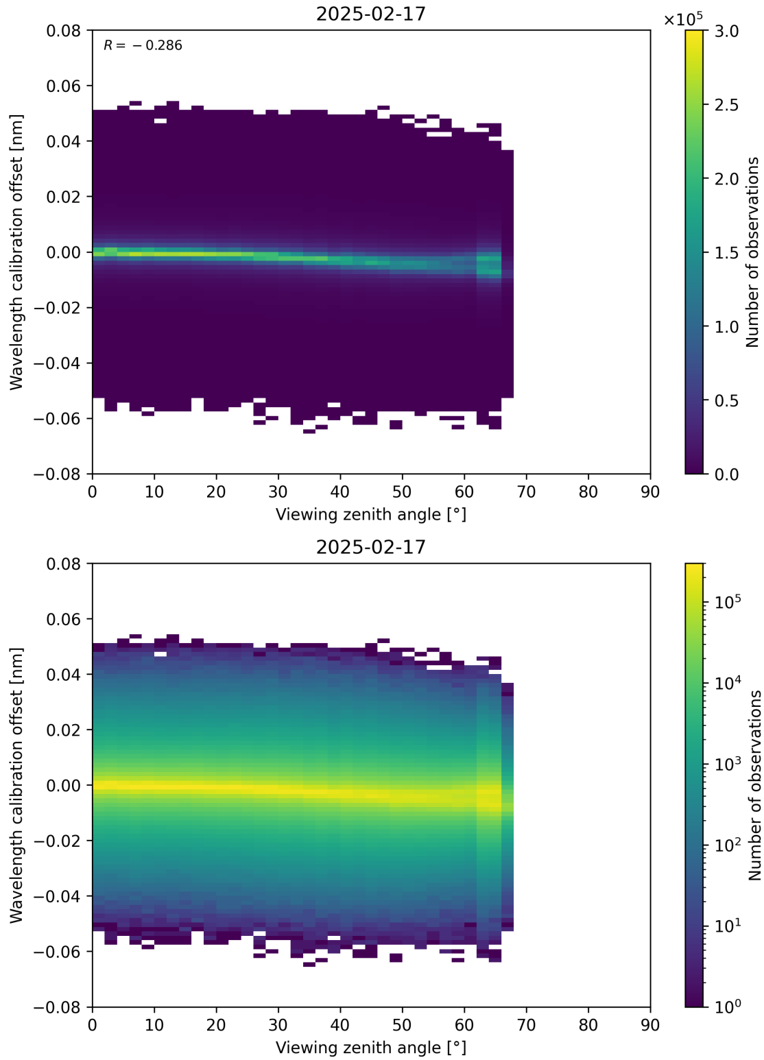
Figure 173: Scatter density plot of “Viewing zenith angle” against “Wavelength calibration offset” for 2025-02-16 to 2025-02-18.
