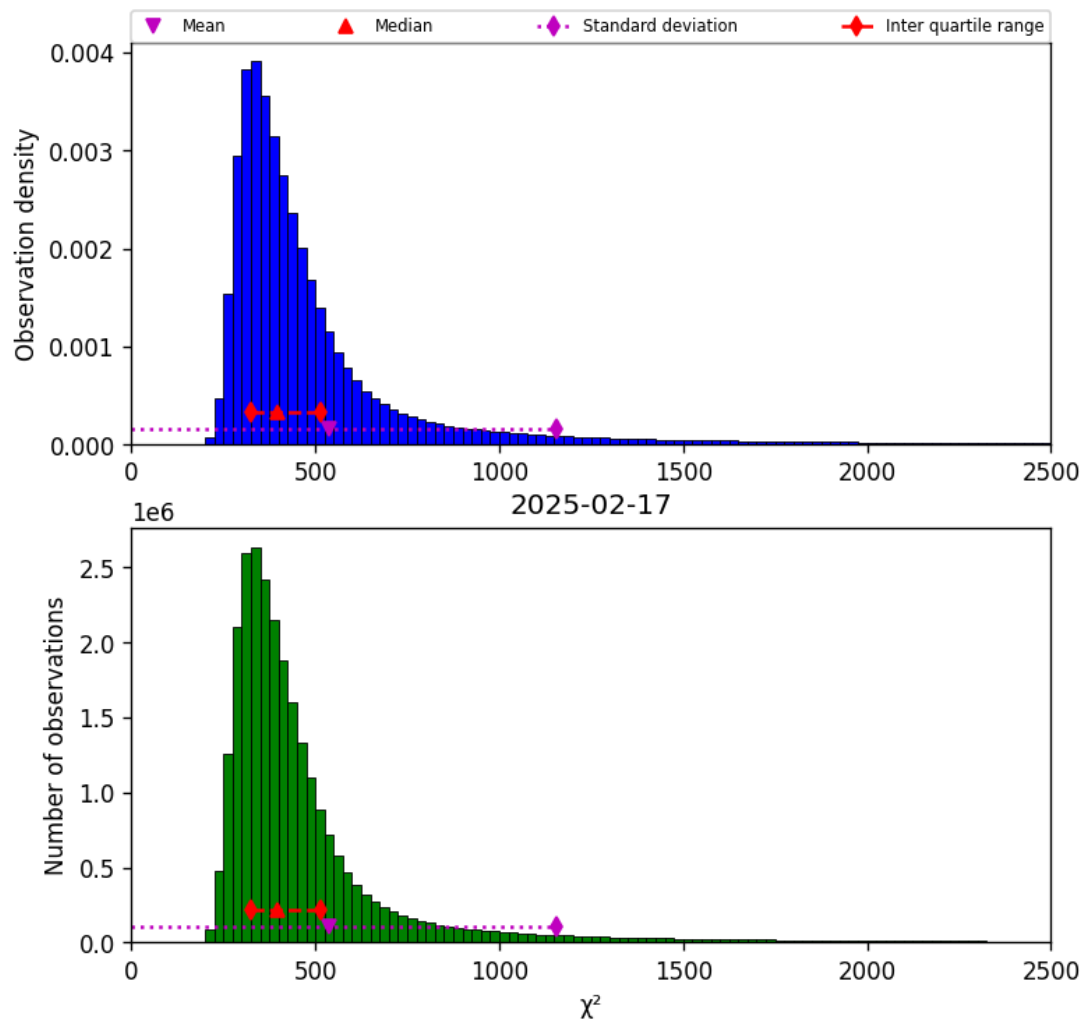
Figure 42: Histogram of “ \chi^2 ” for 2025-02-16 to 2025-02-18
