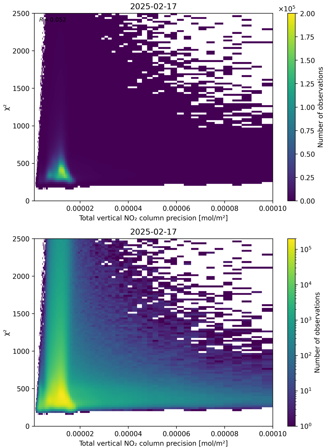
Figure 116: Scatter density plot of “Total vertical NO 2 column precision” against “ \chi^2 ” for 2025-02-16 to 2025-02-18.
