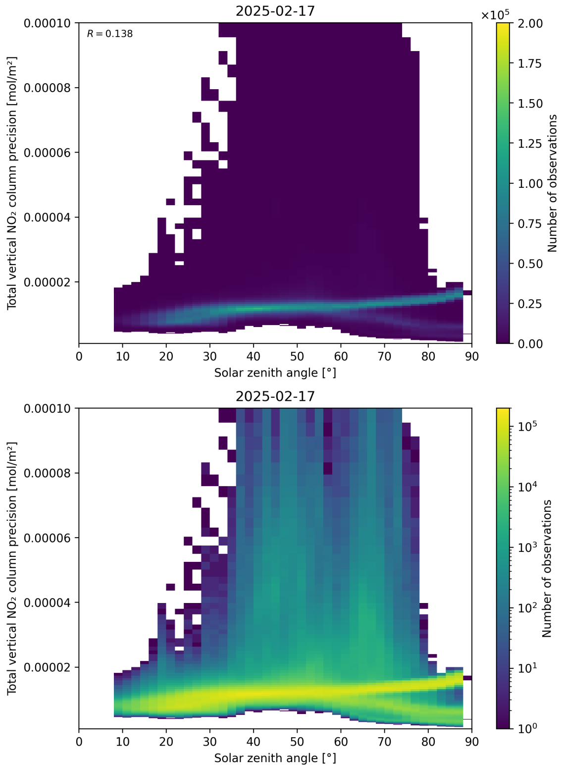
Figure 154: Scatter density plot of “Solar zenith angle” against “Total vertical NO 2 column precision” for 2025-02-16 to 2025-02-18.
