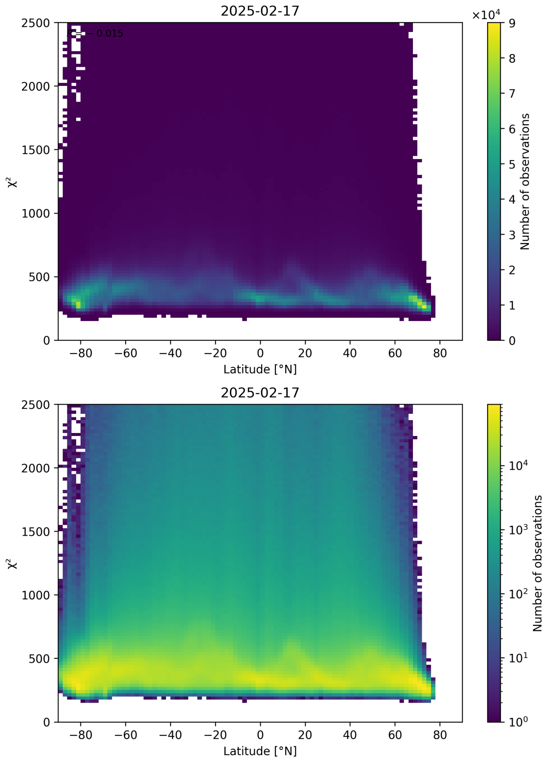
Figure 86: Scatter density plot of “Latitude” against “ \chi^2 ” for 2025-02-16 to 2025-02-18.
