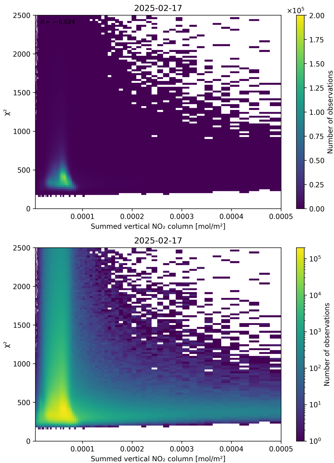
Figure 104: Scatter density plot of “Summed vertical NO 2 column” against “ \chi^2 ” for 2025-02-16 to 2025-02-18.
