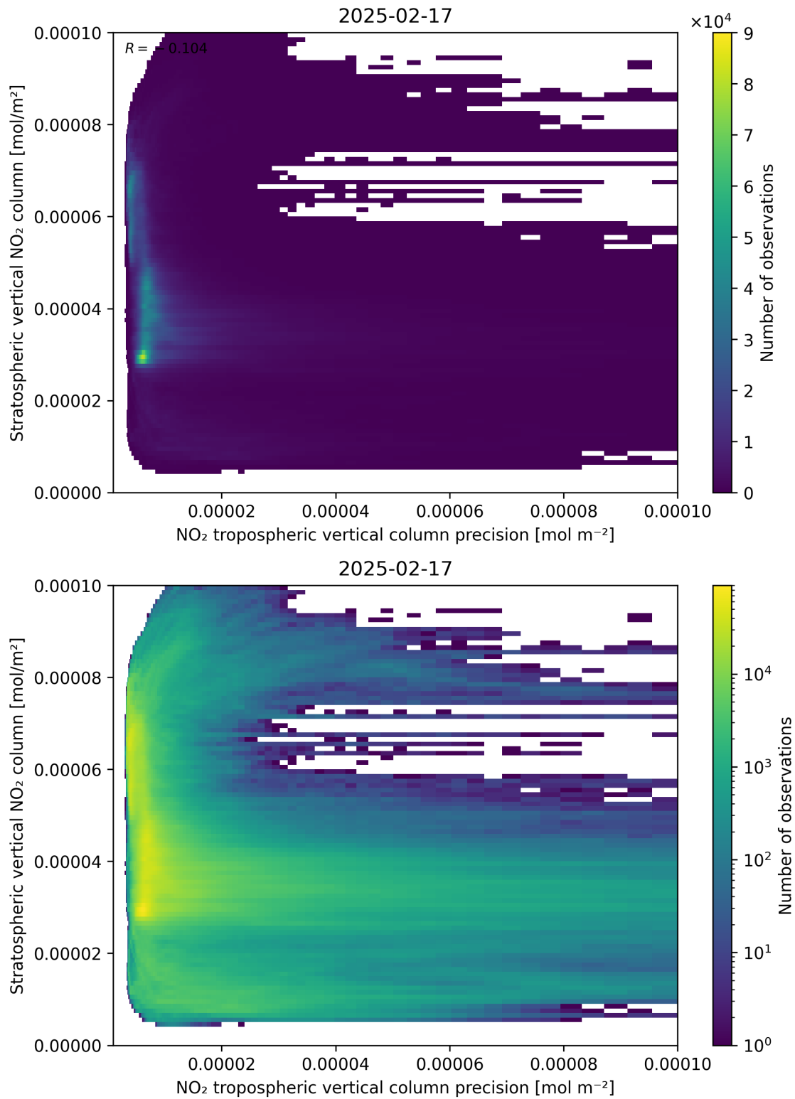
Figure 135: Scatter density plot of “NO 2 tropospheric vertical column precision” against “Stratospheric vertical NO 2 column” for 2025-02-16 to 2025-02-18.
