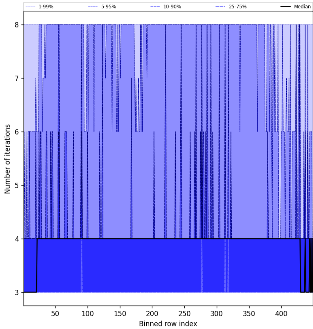
Figure 51: Along track statistics of “Number of iterations” for 2025-02-16 to 2025-02-18
