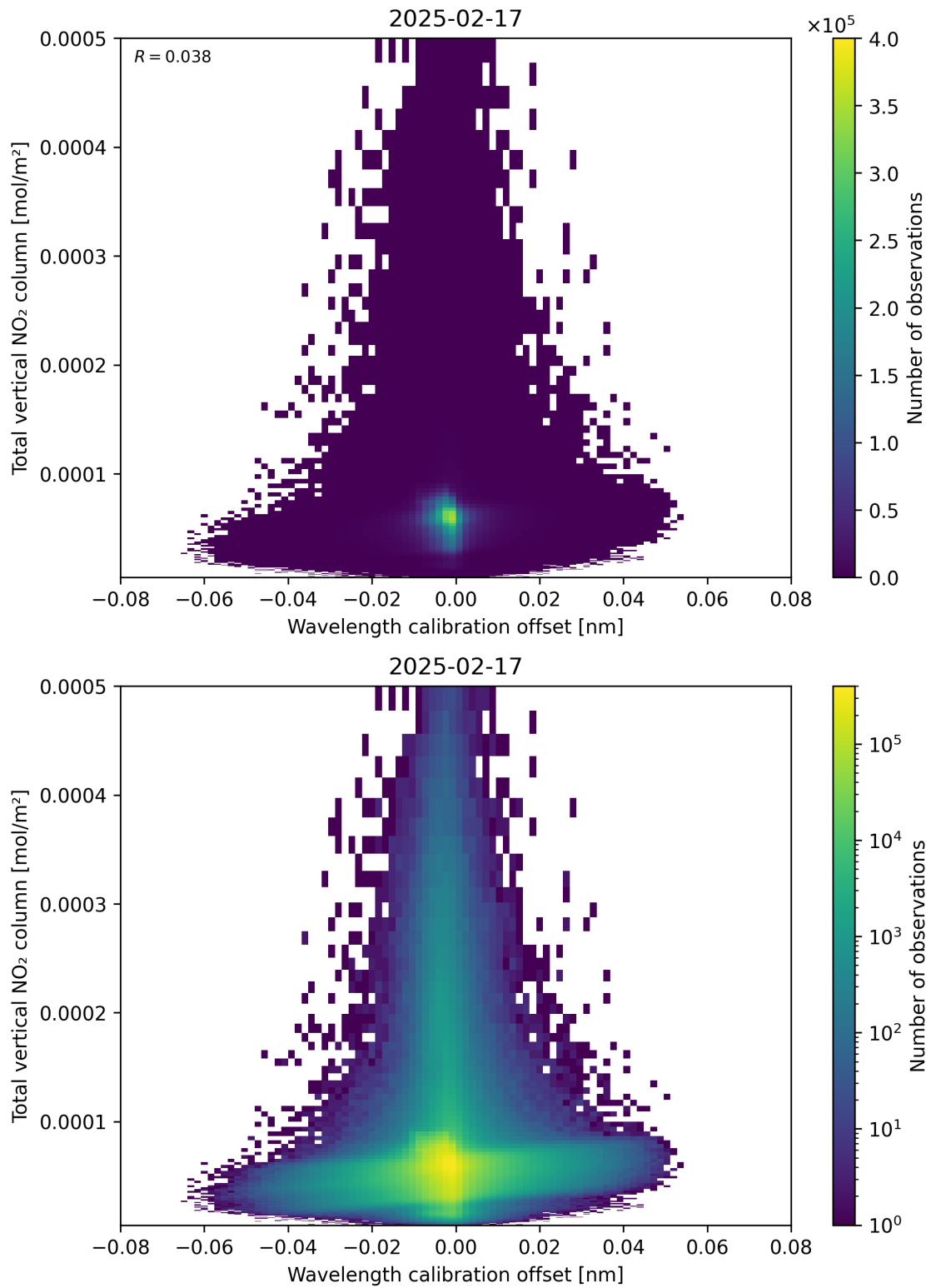
Figure 179: Scatter density plot of “Wavelength calibration offset” against “Total vertical NO 2 column” for 2025-02-16 to 2025-02-18.
