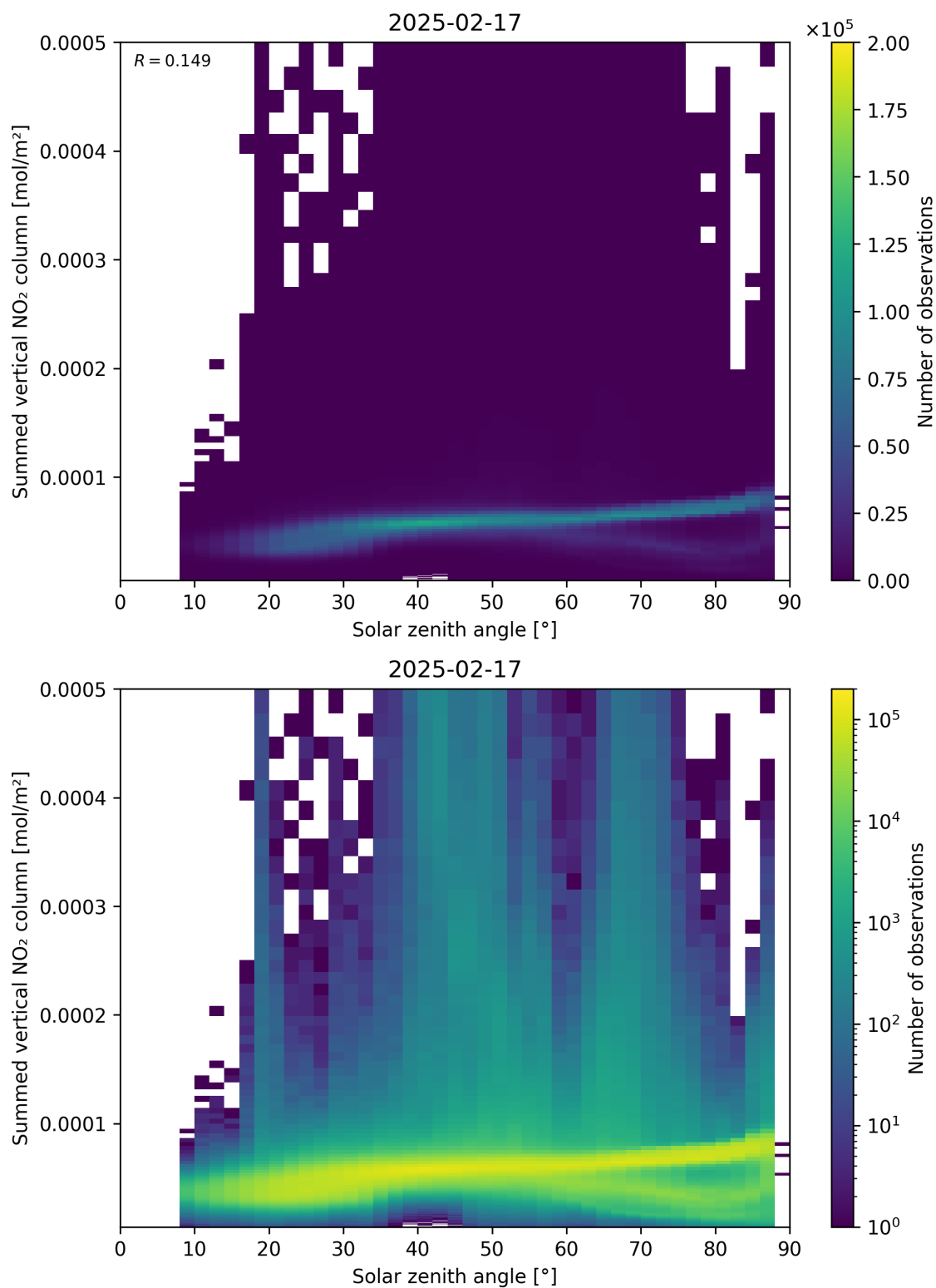
Figure 151: Scatter density plot of “Solar zenith angle” against “Summed vertical NO 2 column” for 2025-02-16 to 2025-02-18.
