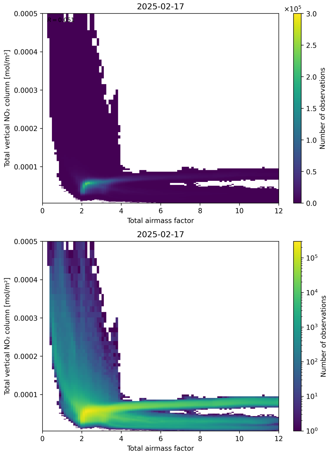
Figure 67: Scatter density plot of “Total airmass factor” against “Total vertical NO 2 column” for 2025-02-16 to 2025-02-18.
