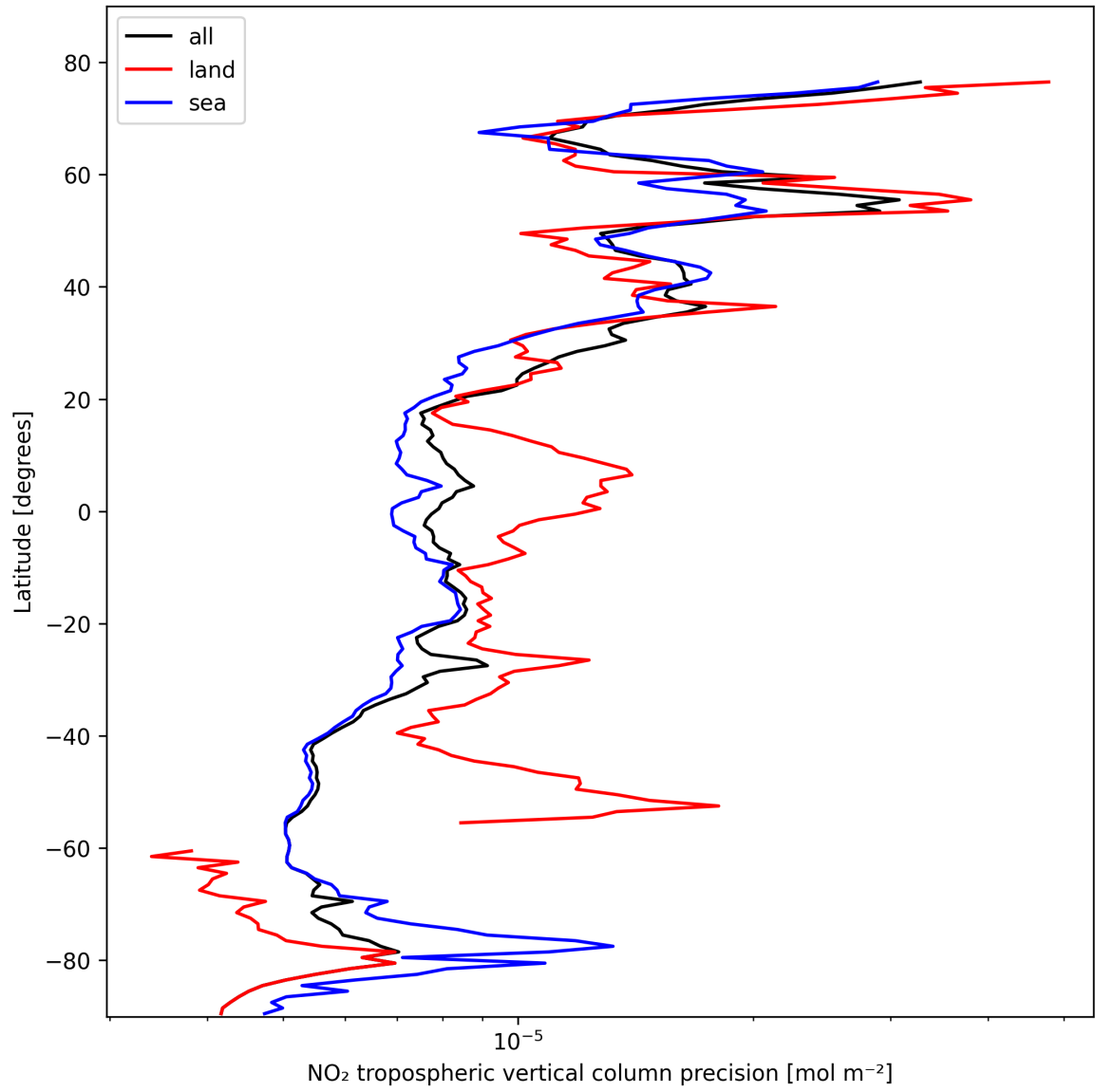
Figure 13: Zonal average of “NO 2 tropospheric vertical column precision” for 2025-02-16 to 2025-02-18.
