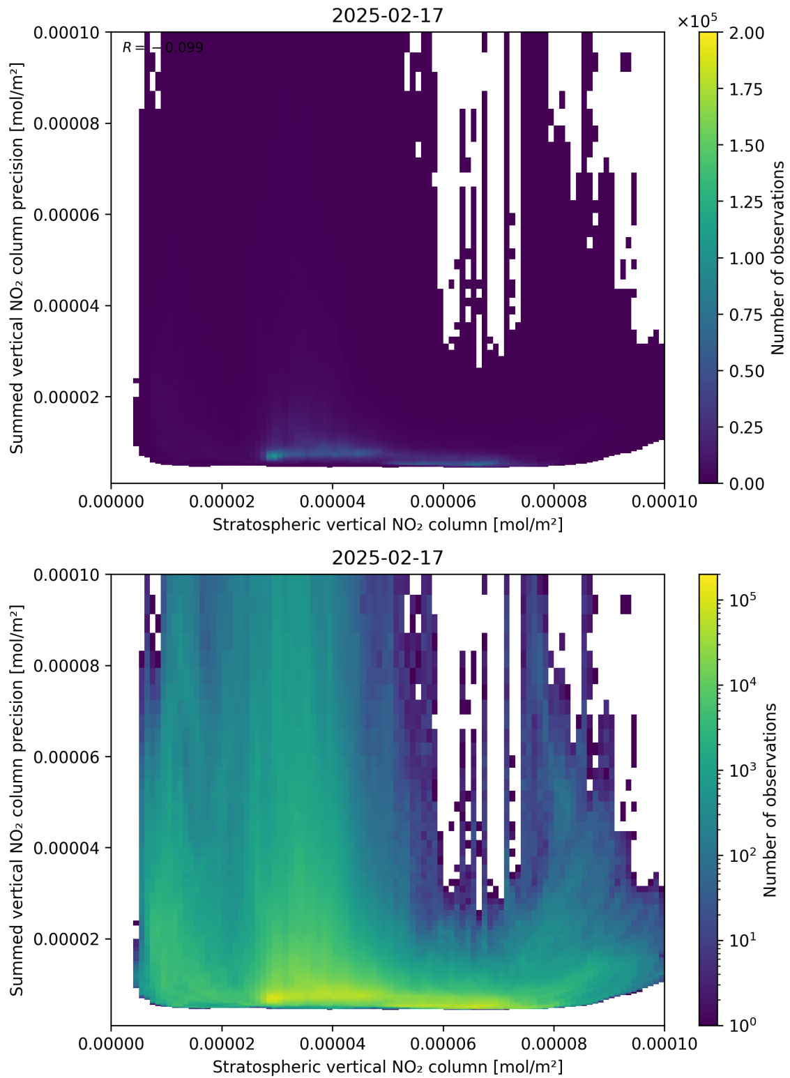
Figure 99: Scatter density plot of “Stratospheric vertical NO 2 column” against “Summed vertical NO 2 column precision” for 2025-02-16 to 2025-02-18.
