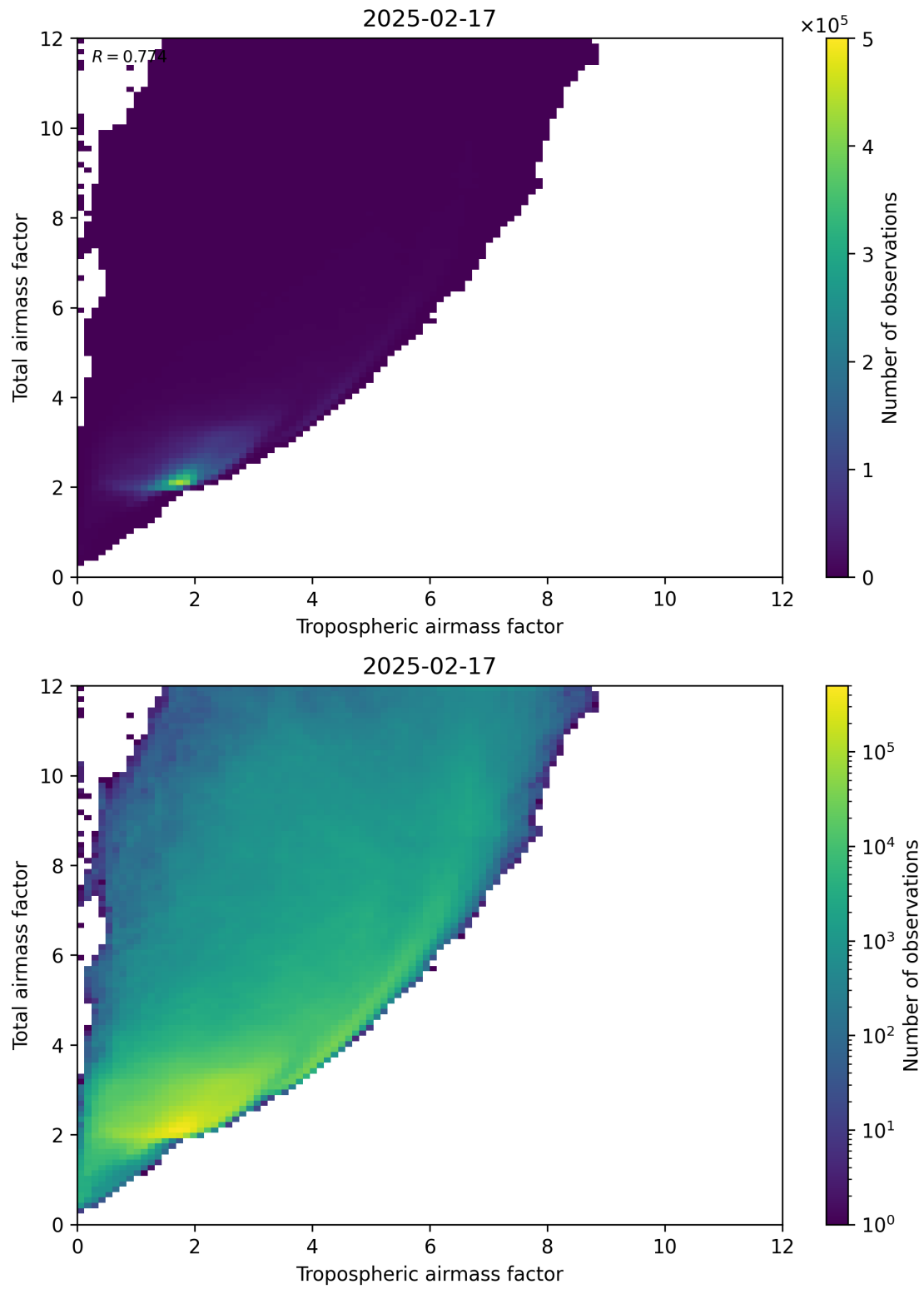
Figure 72: Scatter density plot of “Tropospheric airmass factor” against “Total airmass factor” for 2025-02-16 to 2025-02-18.
