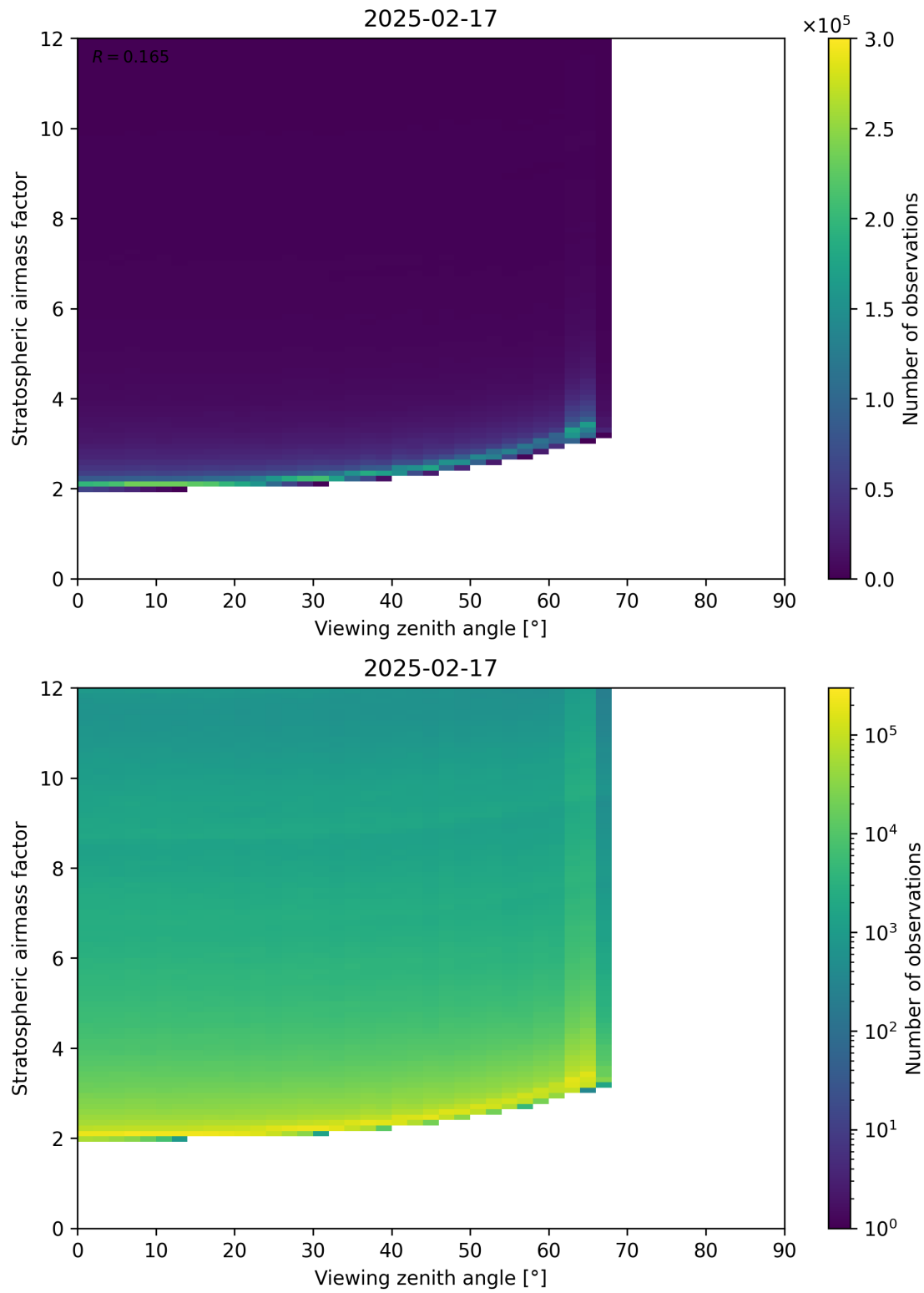
Figure 159: Scatter density plot of “Viewing zenith angle” against “Stratospheric airmass factor” for 2025-02-16 to 2025-02-18.
