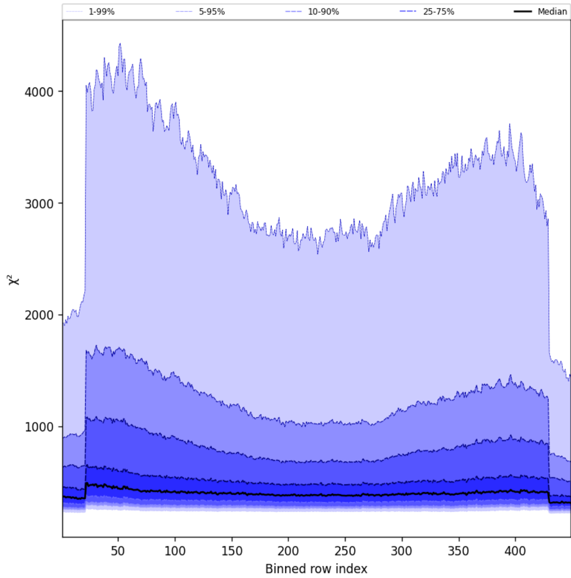
Figure 59: Along track statistics of “ \chi^2 ” for 2025-02-16 to 2025-02-18
