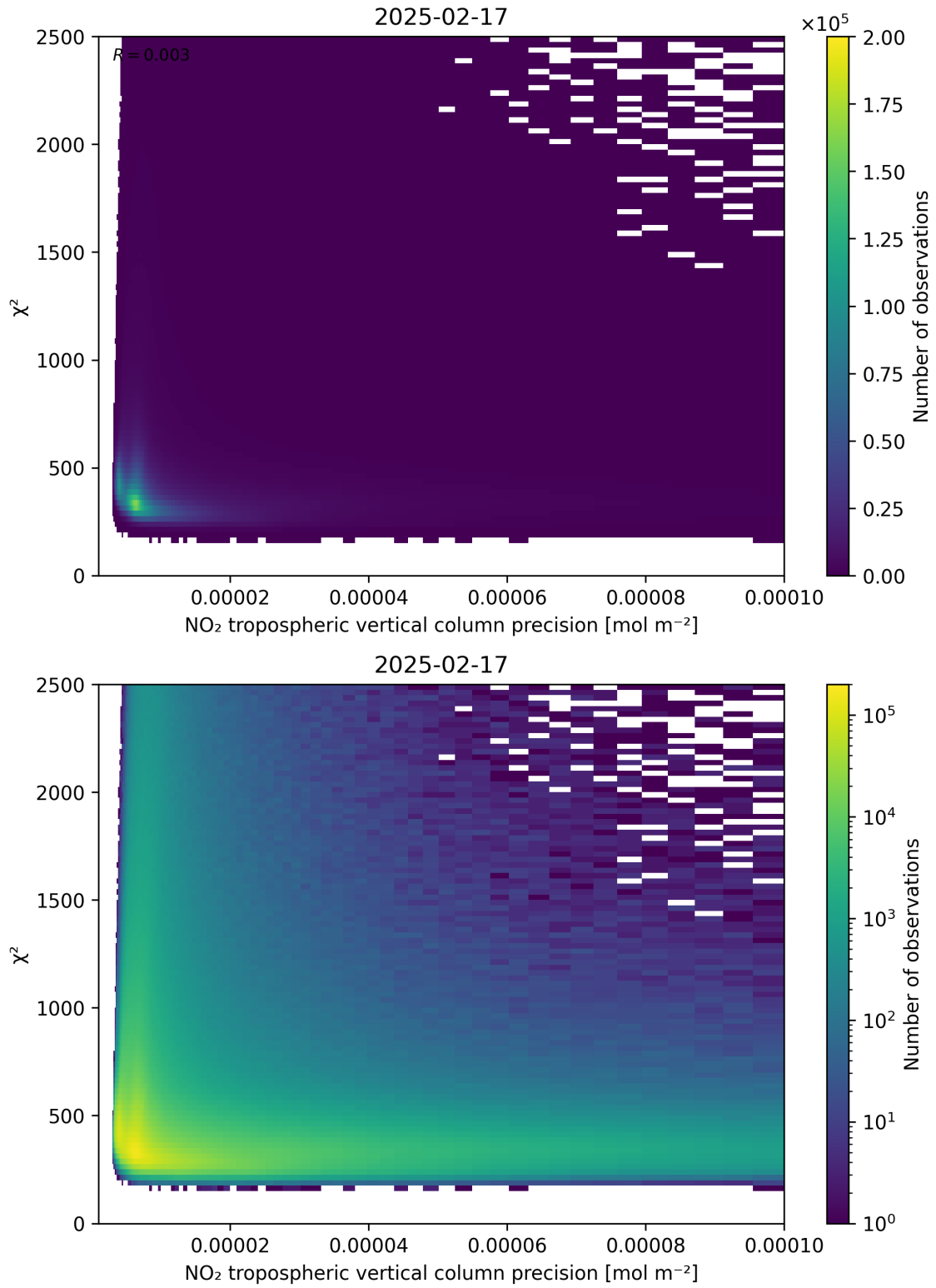
Figure 134: Scatter density plot of “NO 2 tropospheric vertical column precision” against “ \chi^2 ” for 2025-02-16 to 2025-02-18.
