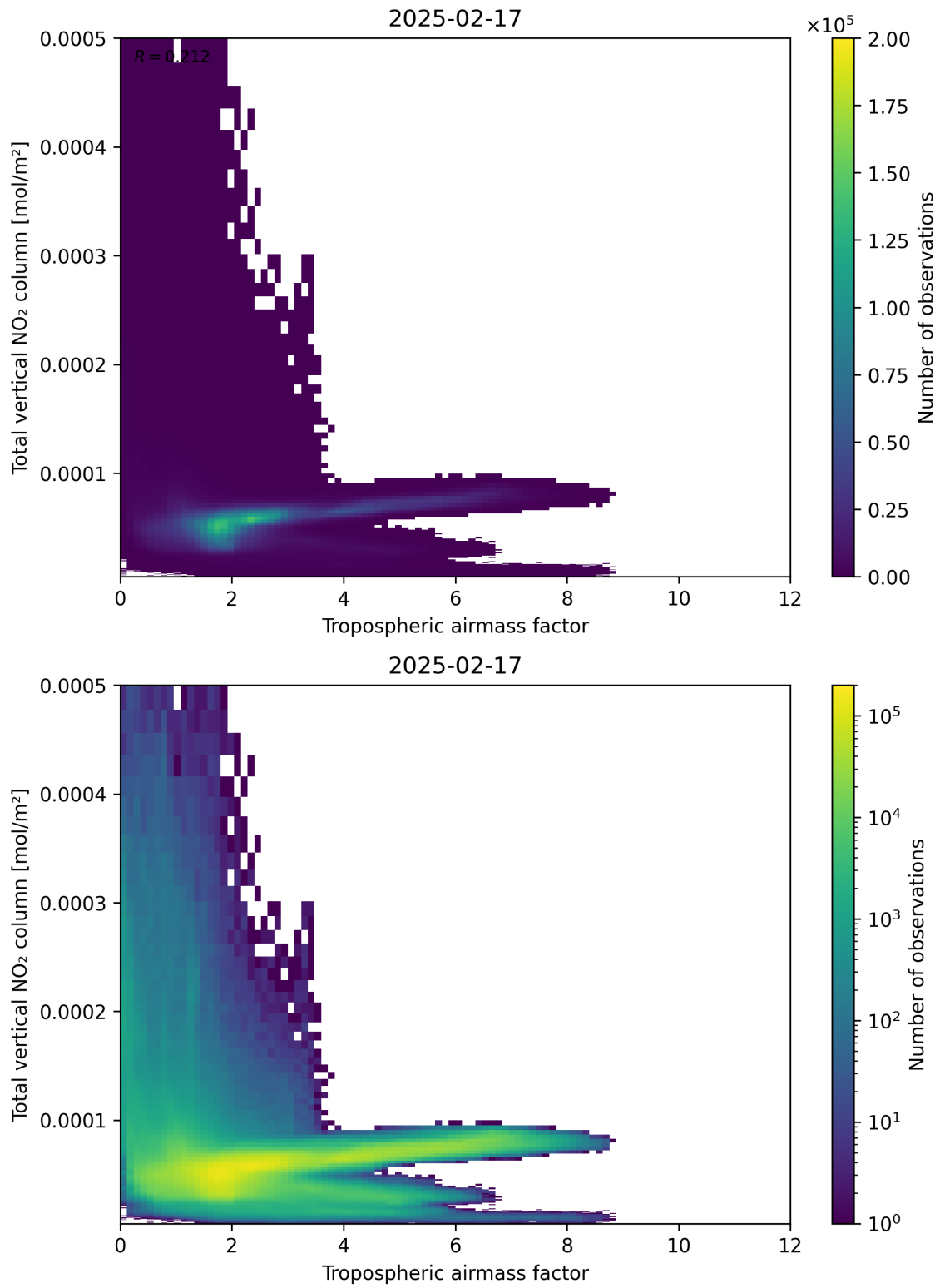
Figure 77: Scatter density plot of “Tropospheric airmass factor” against “Total vertical NO 2 column” for 2025-02-16 to 2025-02-18.
