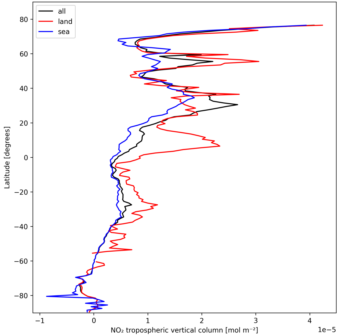
Figure 12: Zonal average of “NO 2 tropospheric vertical column” for 2025-02-16 to 2025-02-18.
