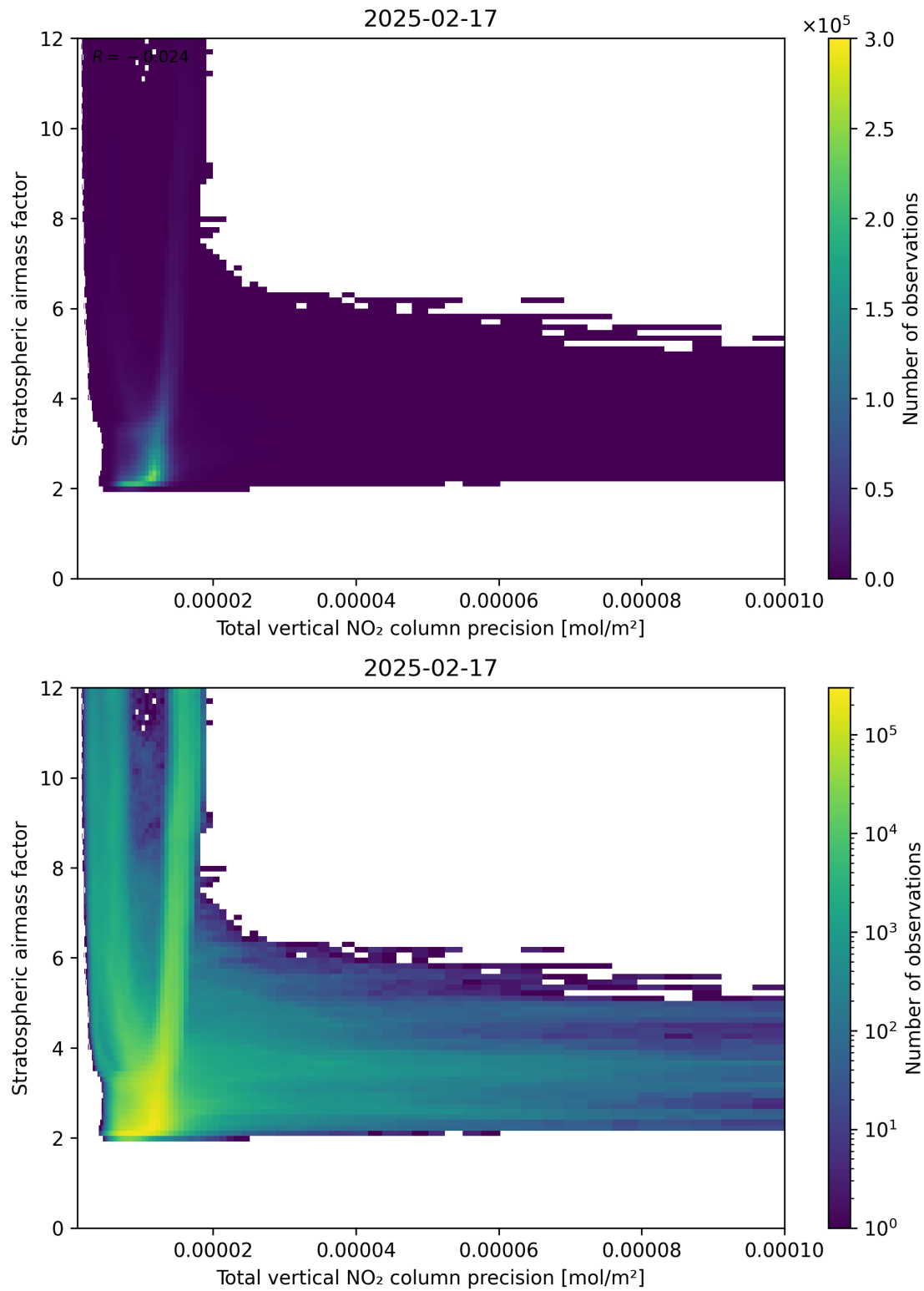
Figure 115: Scatter density plot of “Total vertical NO 2 column precision” against “Stratospheric air mass factor” for 2025-02-16 to 2025-02-18.
