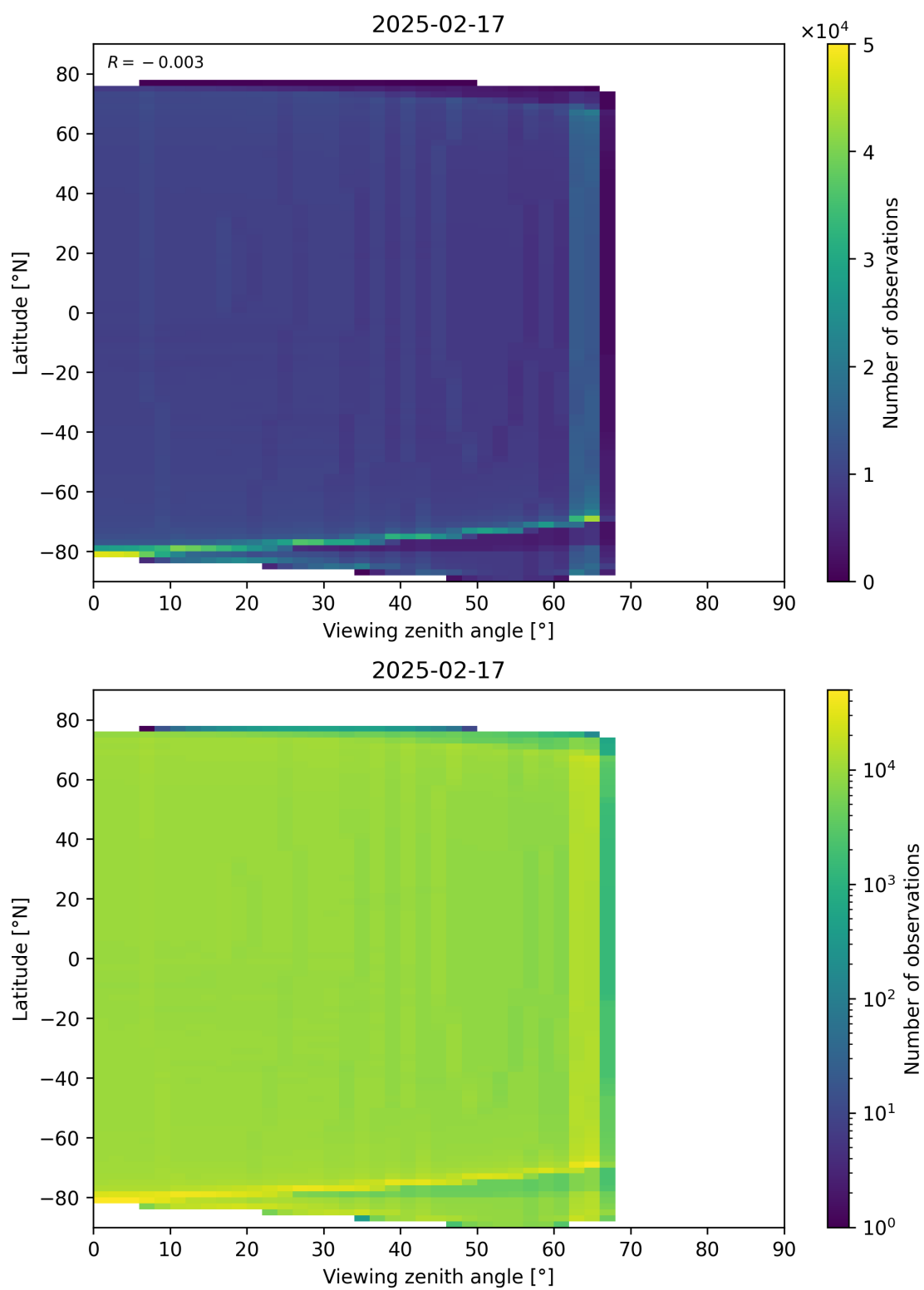
Figure 163: Scatter density plot of “Viewing zenith angle” against “Latitude” for 2025-02-16 to 2025-02-18.
