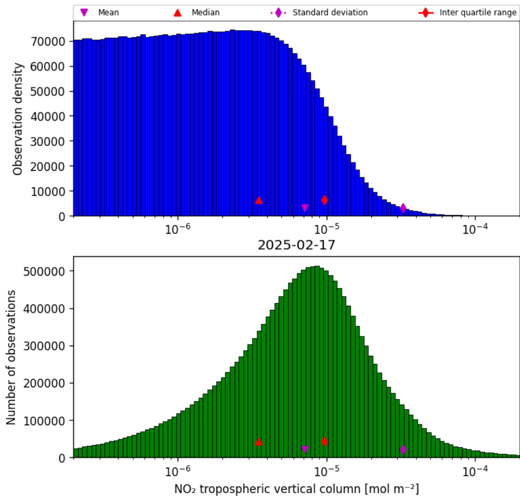
Figure 29: Histogram of “NO 2 tropospheric vertical column” for 2025-02-16 to 2025-02-18
