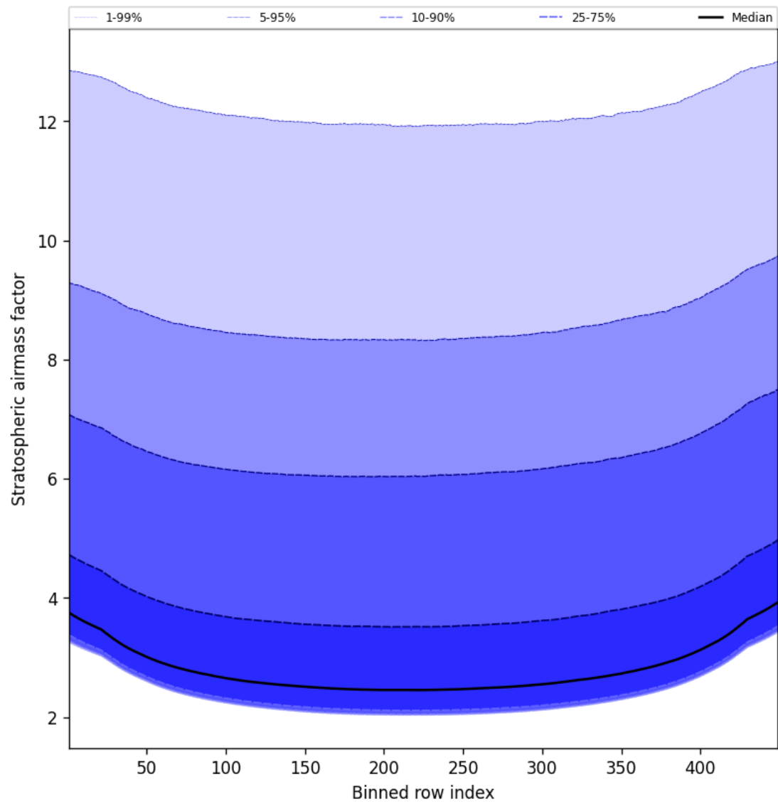
Figure 61: Along track statistics of “Stratospheric air mass factor” for 2025-02-16 to 2025-02-18
