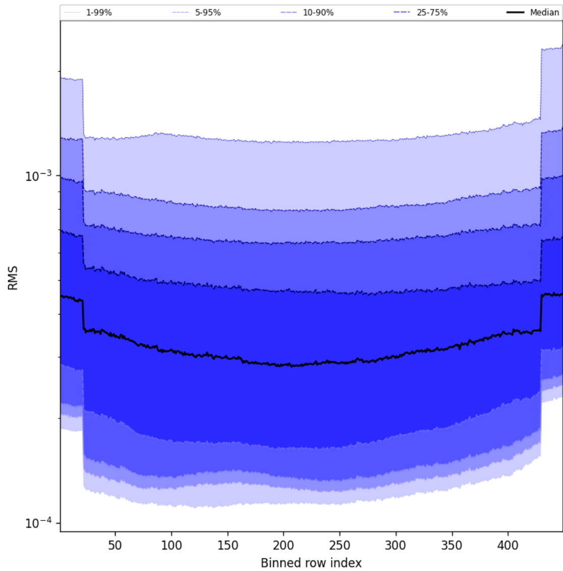
Figure 60: Along track statistics of “RMS” for 2025-02-16 to 2025-02-18
