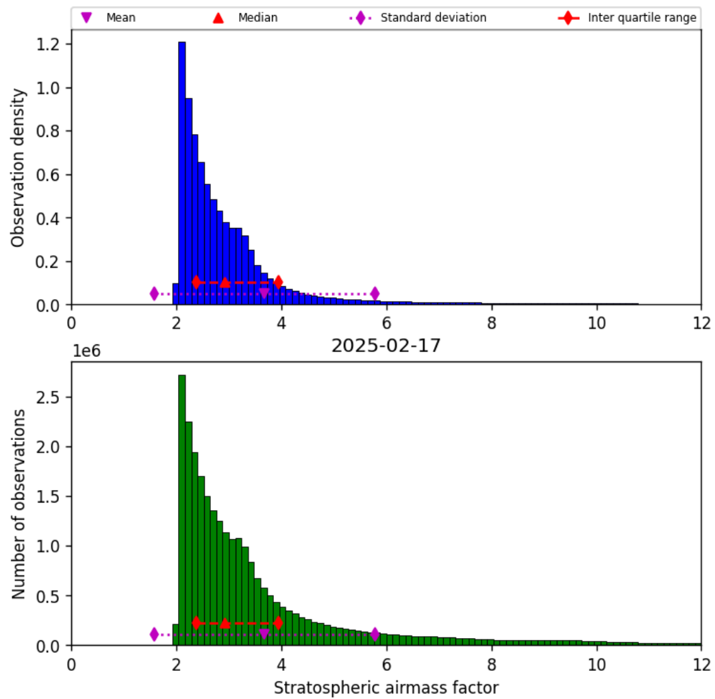
Figure 44: Histogram of “Stratospheric airmass factor” for 2025-02-16 to 2025-02-18
