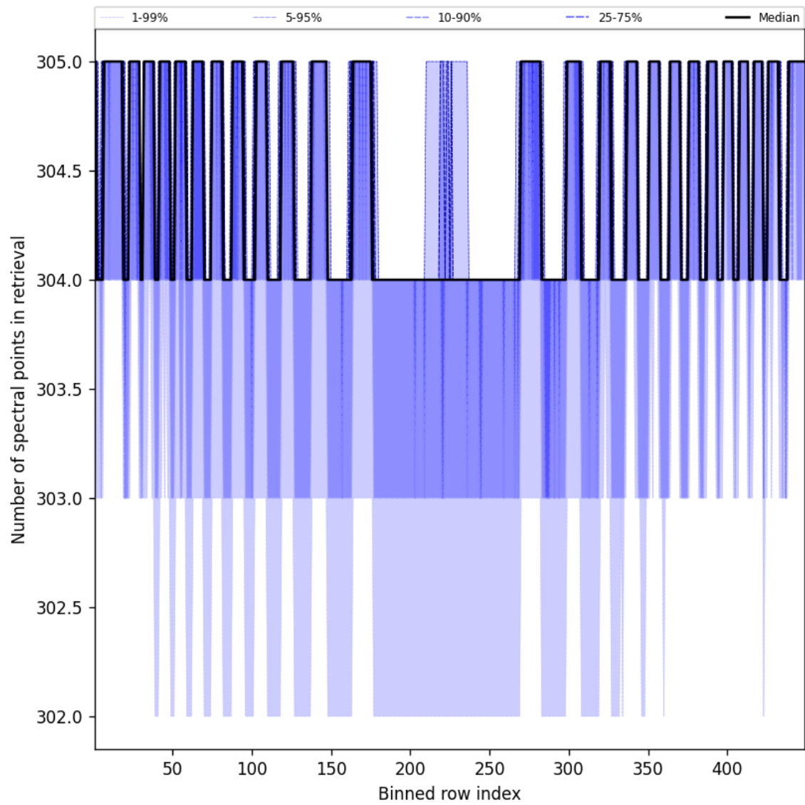
Figure 50: Along track statistics of “Number of spectral points in retrieval” for 2025-02-16 to 2025-02-18
