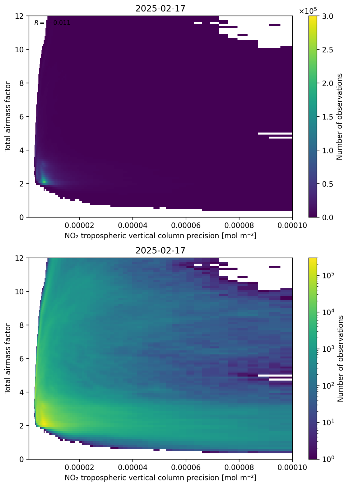
Figure 132: Scatter density plot of “NO 2 tropospheric vertical column precision” against “Total air mass factor” for 2025-02-16 to 2025-02-18.
