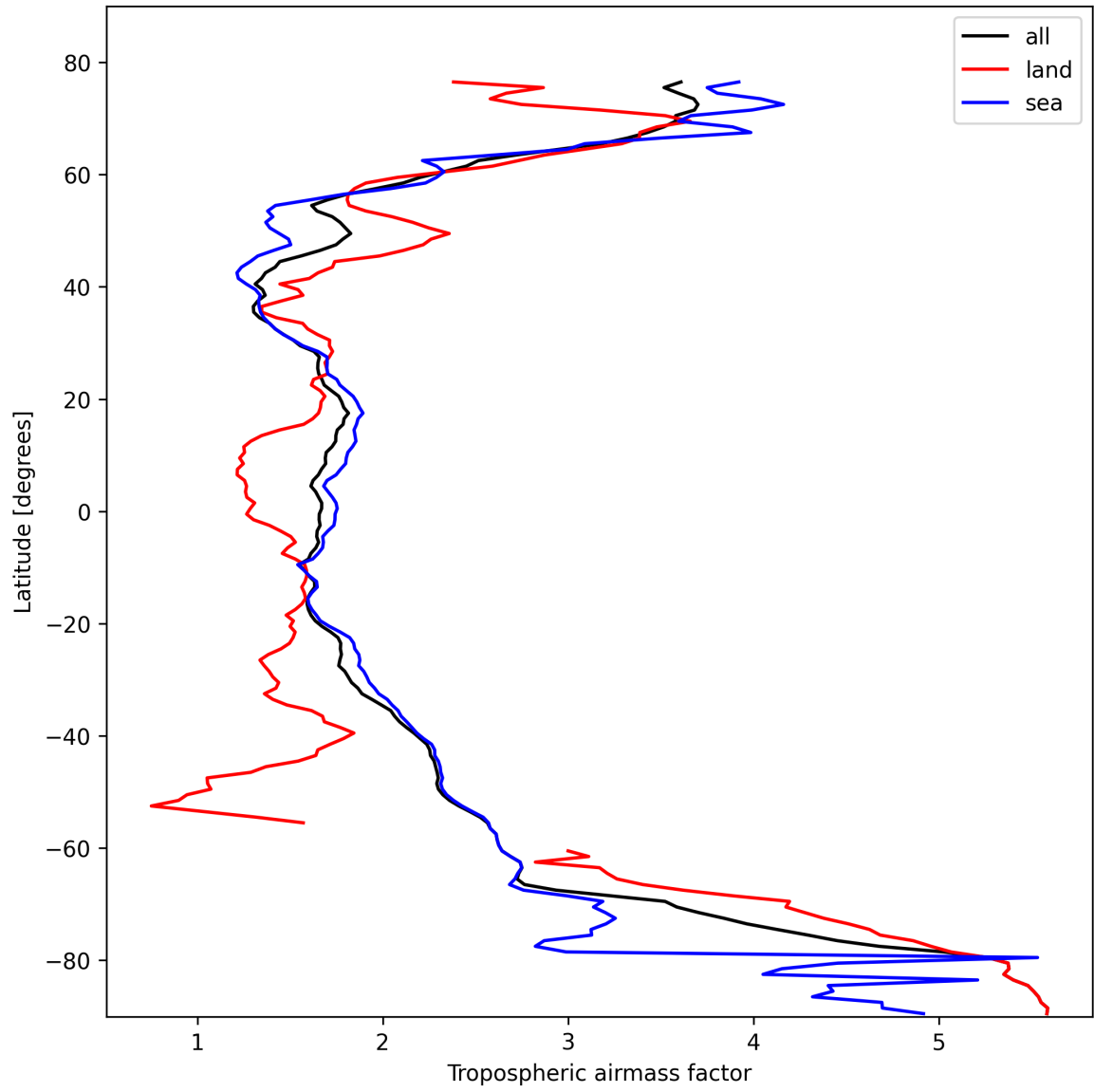
Figure 14: Zonal average of “Tropospheric airmass factor” for 2025-02-16 to 2025-02-18.
