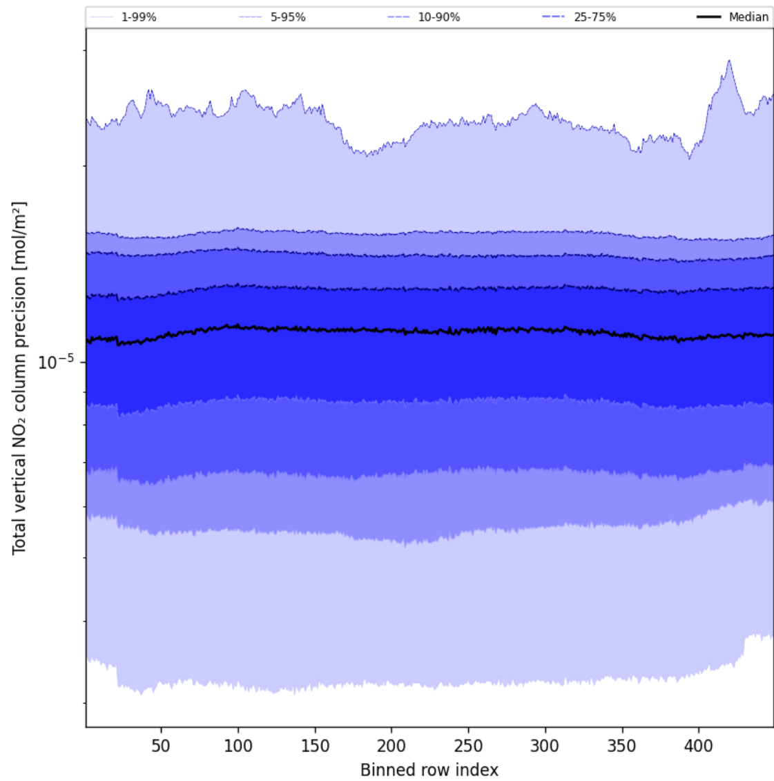
Figure 56: Along track statistics of “Total vertical NO 2 column precision” for 2025-02-16 to 2025-02-18
