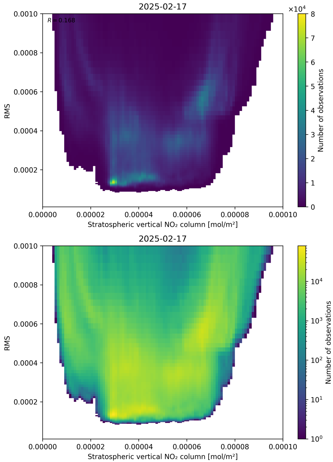
Figure 102: Scatter density plot of “Stratospheric vertical NO 2 column” against “RMS” for 2025-02-16 to 2025-02-18.
