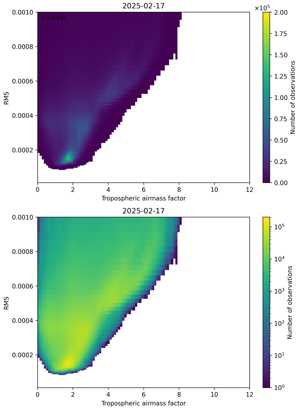
Figure 79: Scatter density plot of “Tropospheric airmass factor” against “RMS” for 2025-02-16 to 2025-02-18.
