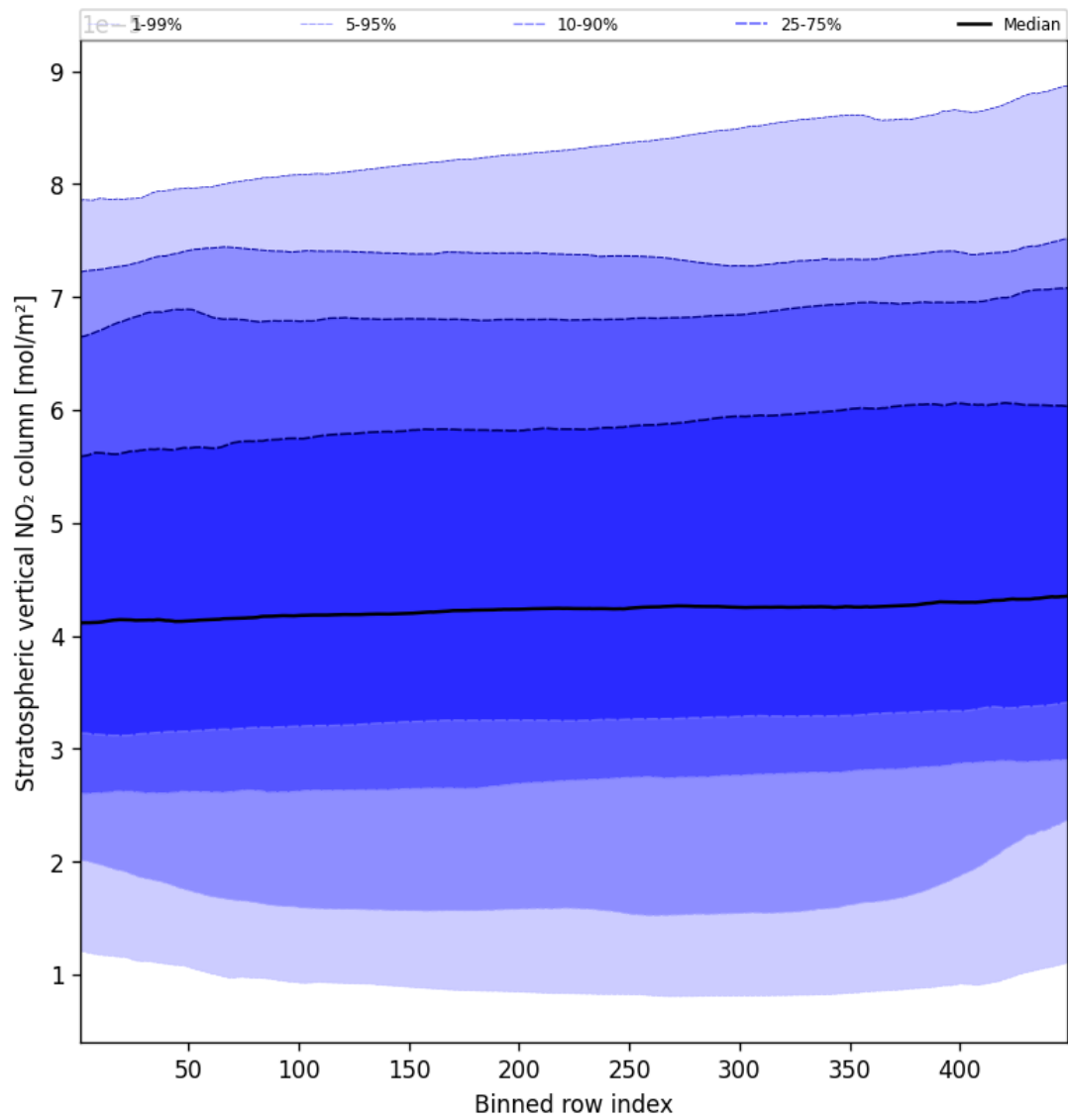
Figure 53: Along track statistics of “Stratospheric vertical NO 2 column” for 2025-02-16 to 2025-02-18
