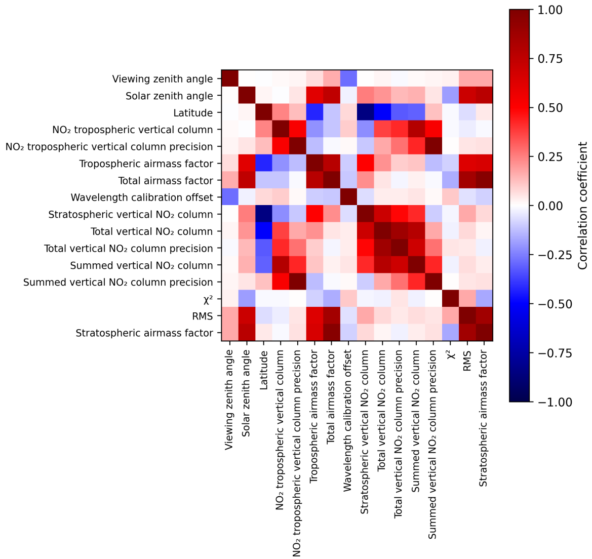
Figure 2: Map of correlation matrix for 2025-02-16 to 2025-02-18.
