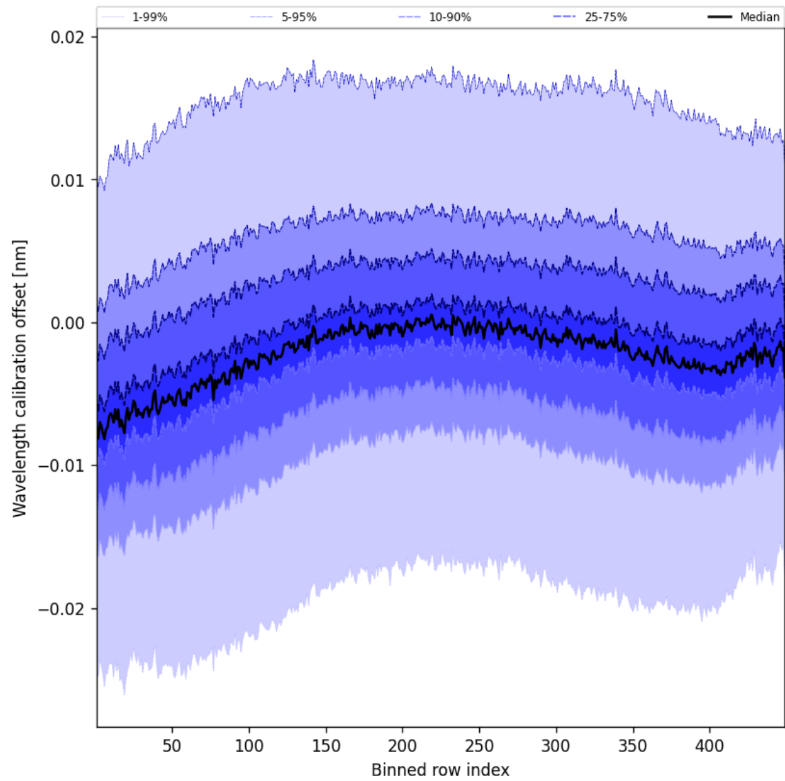
Figure 52: Along track statistics of “Wavelength calibration offset” for 2025-02-16 to 2025-02-18
