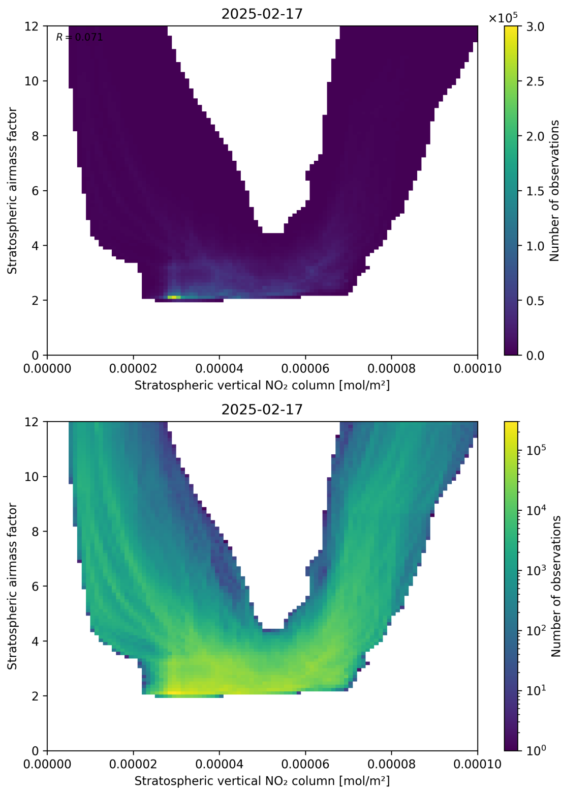
Figure 96: Scatter density plot of “Stratospheric vertical NO 2 column” against “Stratospheric airmass factor” for 2025-02-16 to 2025-02-18.
