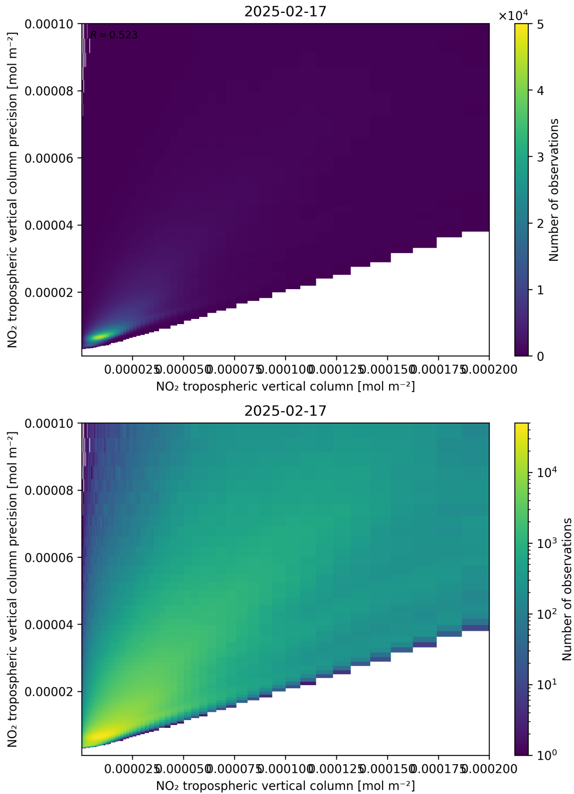
Figure 130: Scatter density plot of “NO 2 tropospheric vertical column” against “NO 2 tropospheric vertical column precision” for 2025-02-16 to 2025-02-18.
