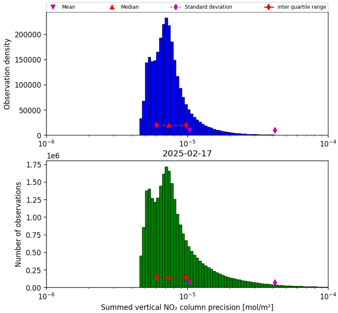
Figure 41: Histogram of “Summed vertical NO 2 column precision” for 2025-02-16 to 2025-02-18
