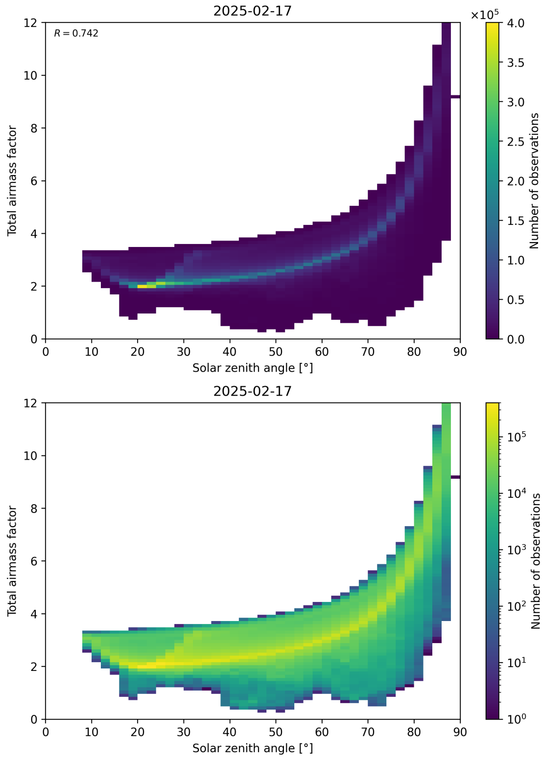
Figure 146: Scatter density plot of “Solar zenith angle” against “Total air mass factor” for 2025-02-16 to 2025-02-18.
