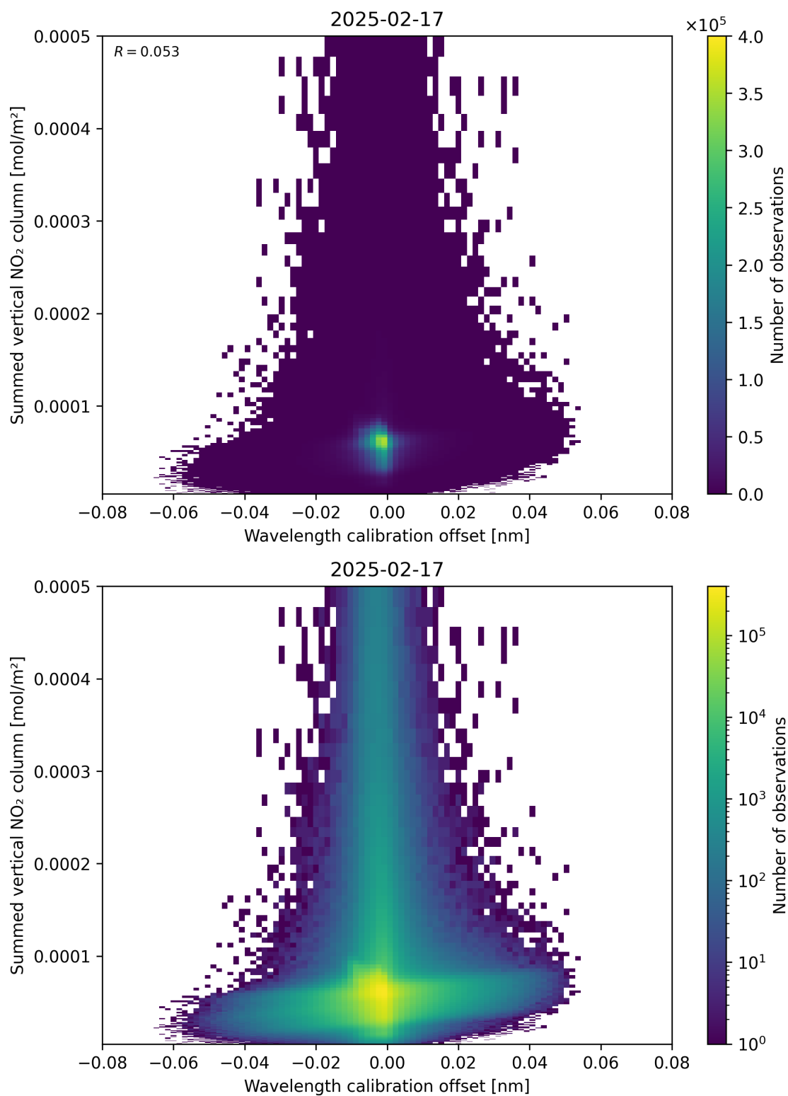
Figure 177: Scatter density plot of “Wavelength calibration offset” against “Summed vertical NO 2 column” for 2025-02-16 to 2025-02-18.
