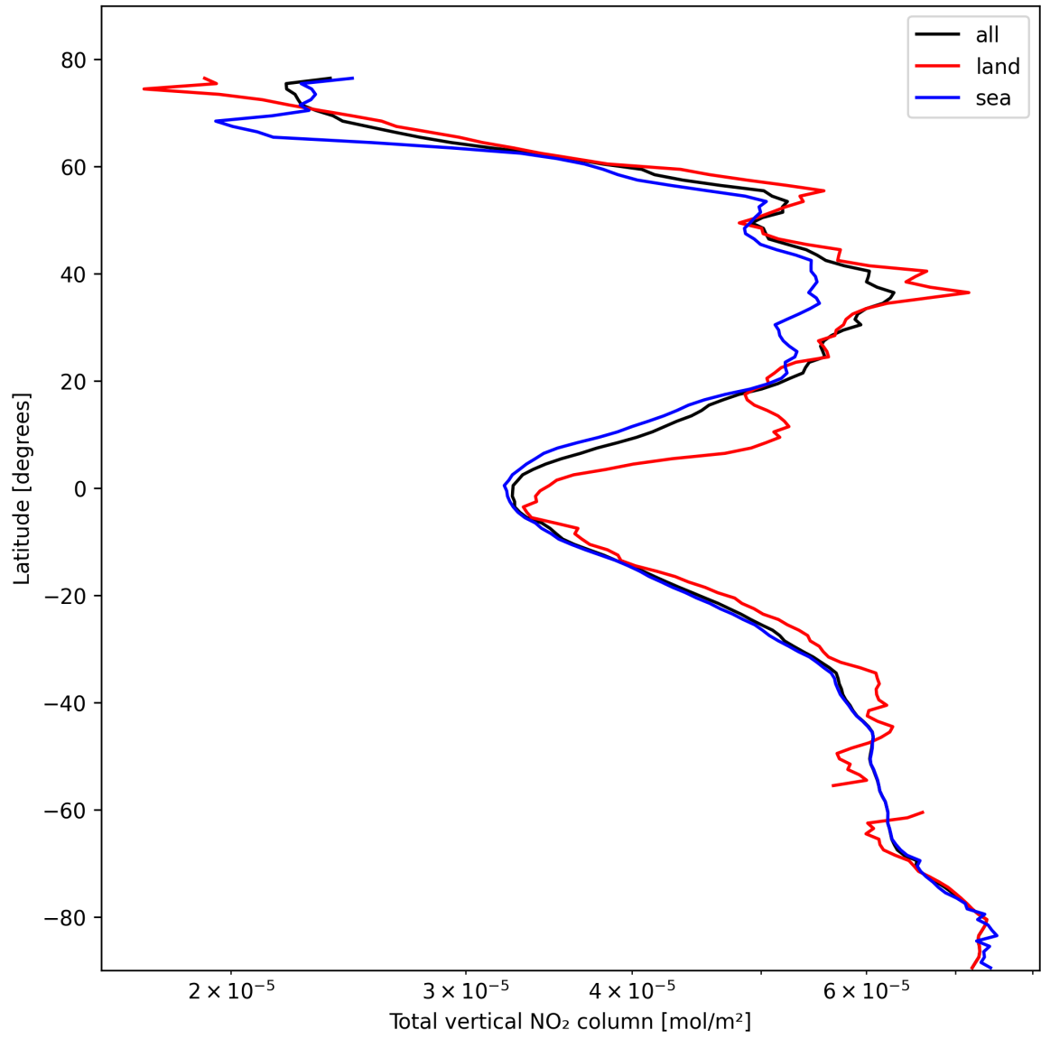
Figure 21: Zonal average of “Total vertical NO 2 column” for 2025-02-16 to 2025-02-18.
