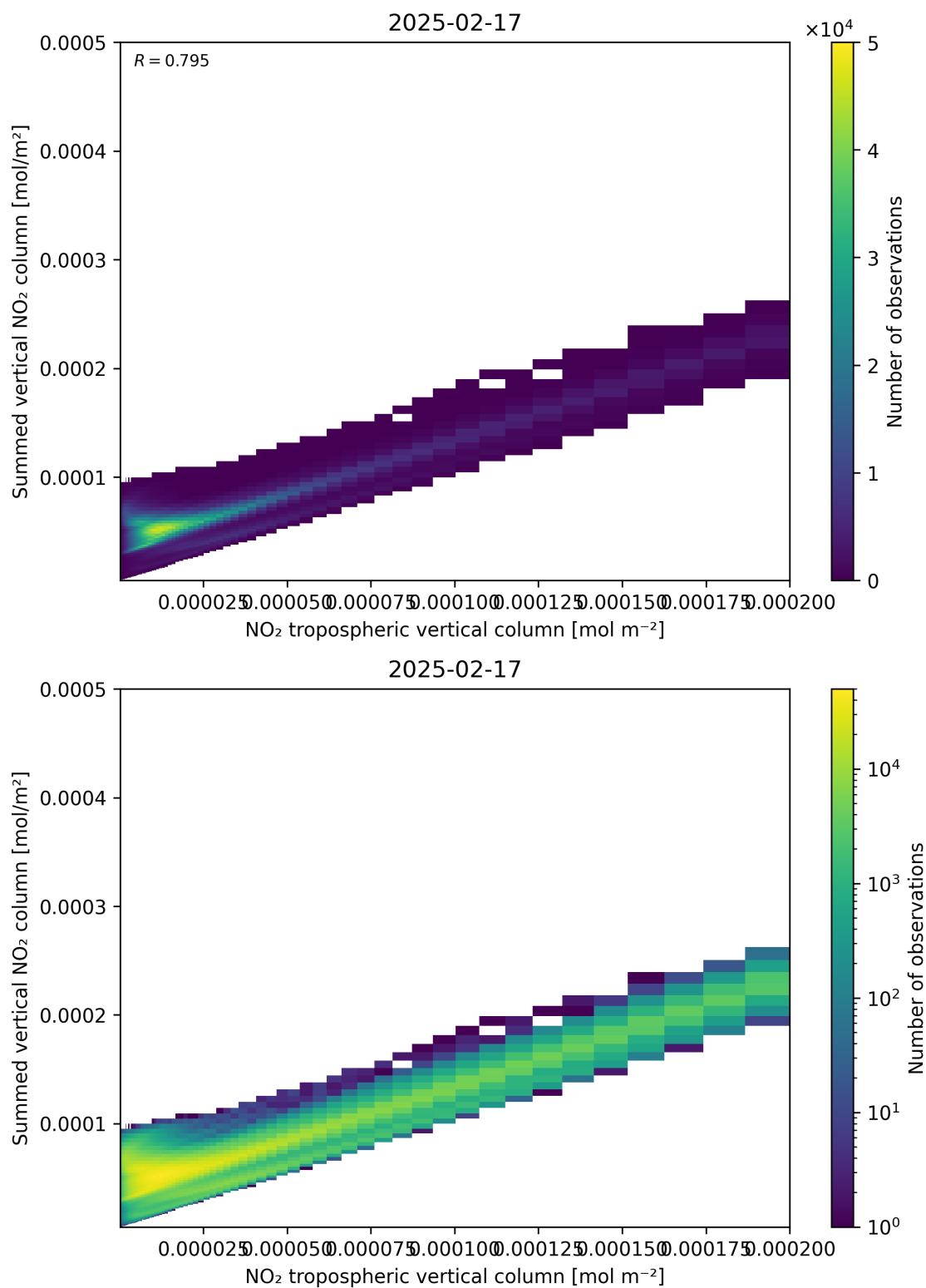
Figure 126: Scatter density plot of “NO 2 tropospheric vertical column” against “Summed vertical NO 2 column” for 2025-02-16 to 2025-02-18.
