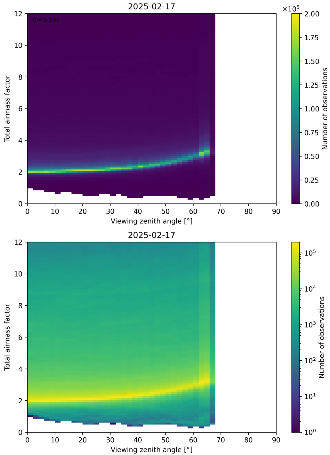
Figure 160: Scatter density plot of “Viewing zenith angle” against “Total airmass factor” for 2025-02-16 to 2025-02-18.
