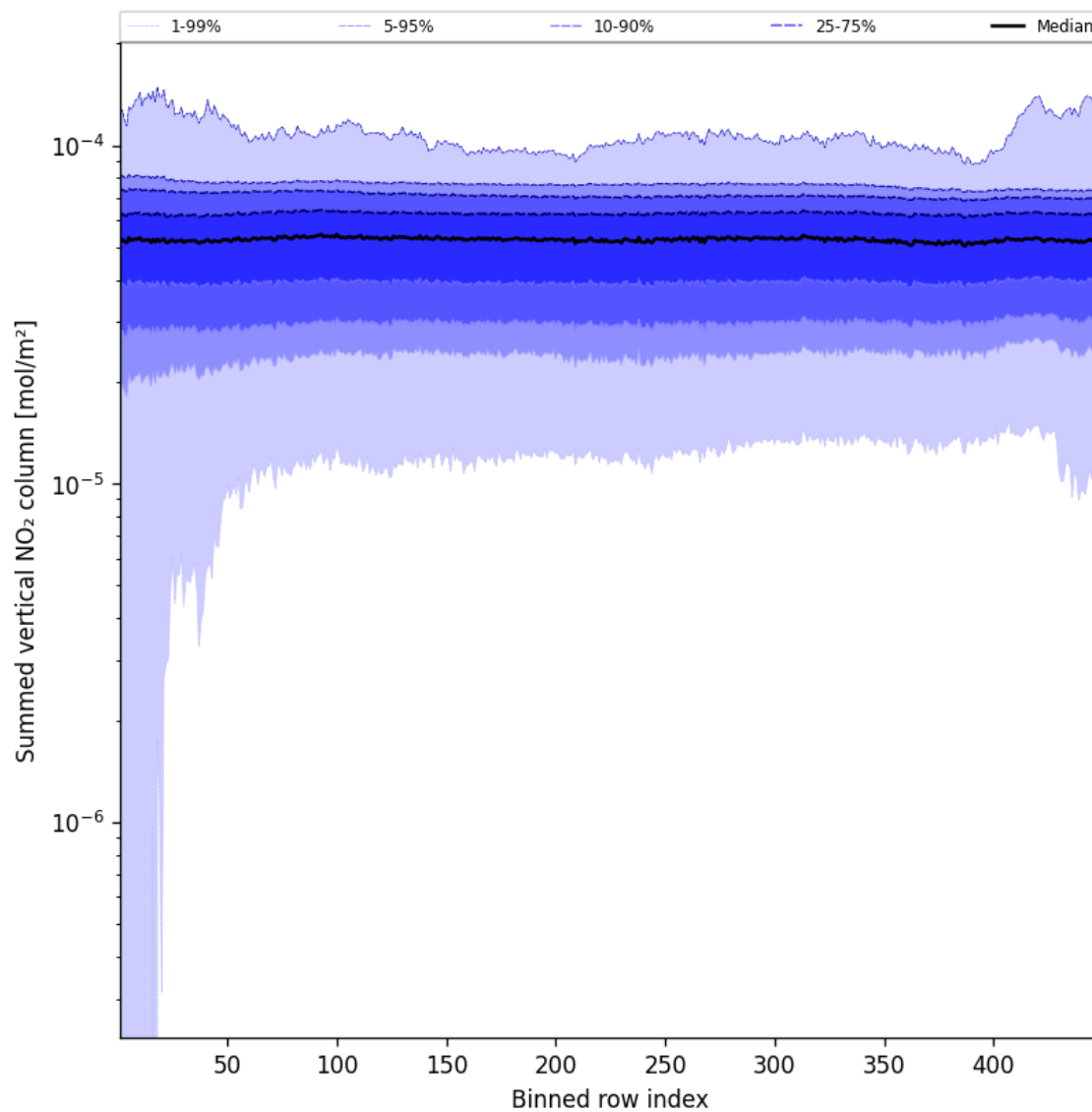
Figure 57: Along track statistics of “Summed vertical NO 2 column” for 2025-02-16 to 2025-02-18
