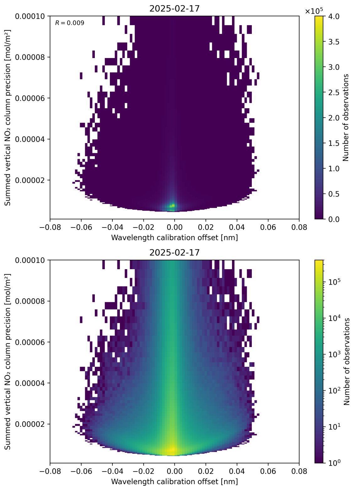
Figure 178: Scatter density plot of “Wavelength calibration offset” against “Summed vertical NO 2 column precision” for 2025-02-16 to 2025-02-18.
