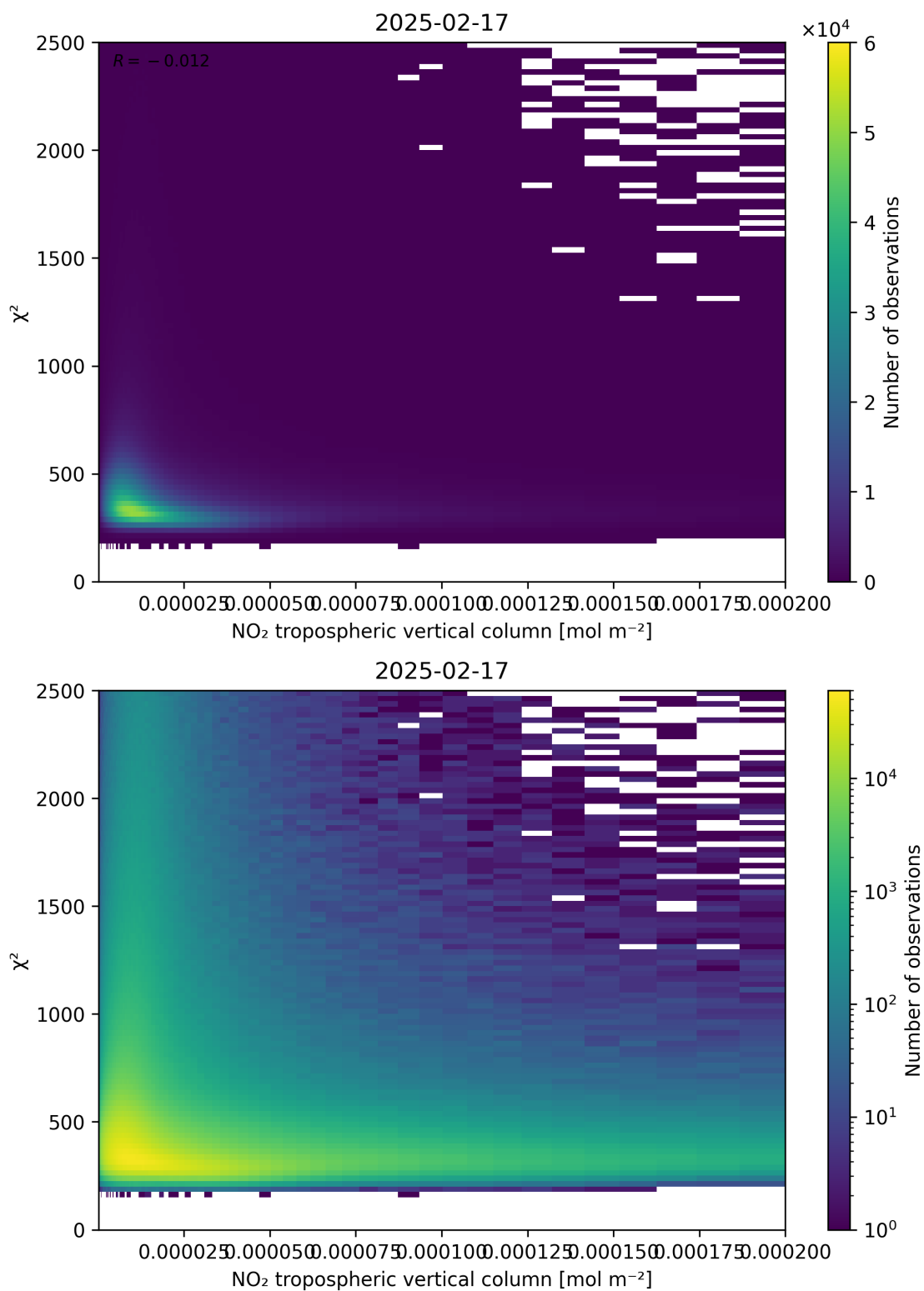
Figure 124: Scatter density plot of “NO 2 tropospheric vertical column” against “ \chi^2 ” for 2025-02-16 to 2025-02-18.
