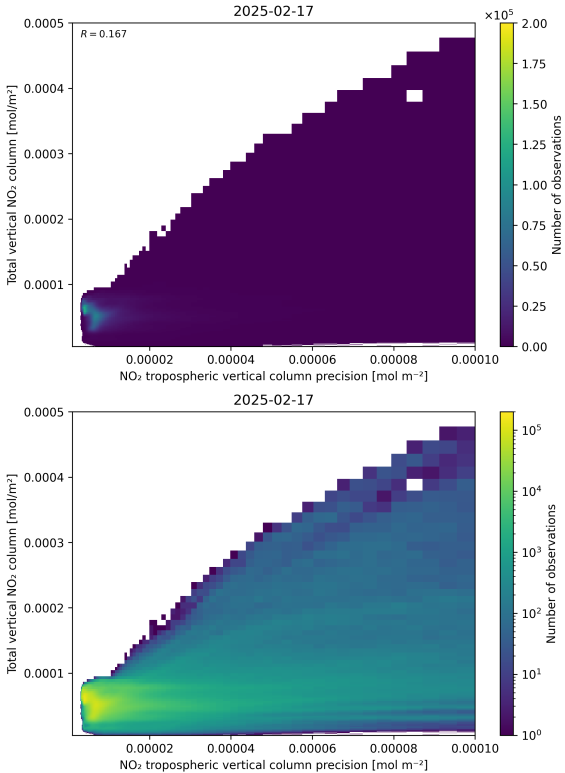
Figure 138: Scatter density plot of “NO 2 tropospheric vertical column precision” against “Total vertical NO 2 column” for 2025-02-16 to 2025-02-18.
