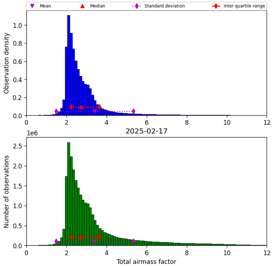
Figure 32: Histogram of “Total airmass factor” for 2025-02-16 to 2025-02-18
