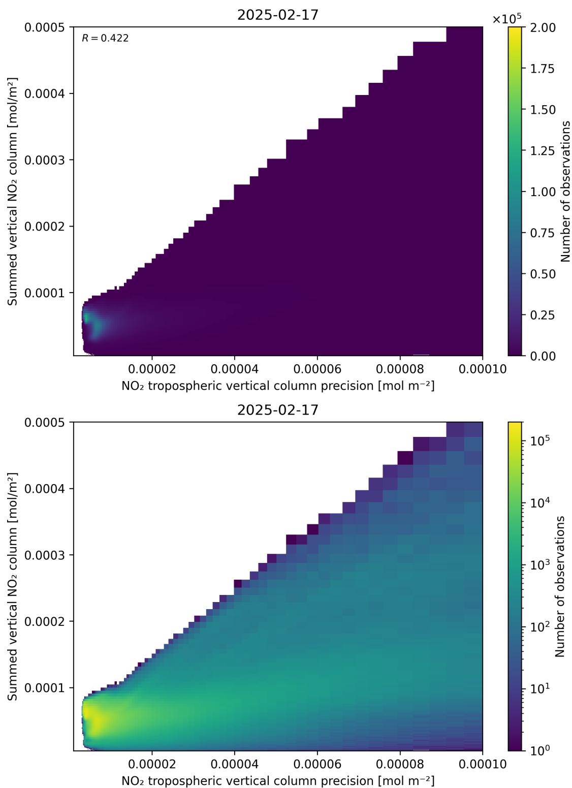
Figure 136: Scatter density plot of “NO 2 tropospheric vertical column precision” against “Summed vertical NO 2 column” for 2025-02-16 to 2025-02-18.
