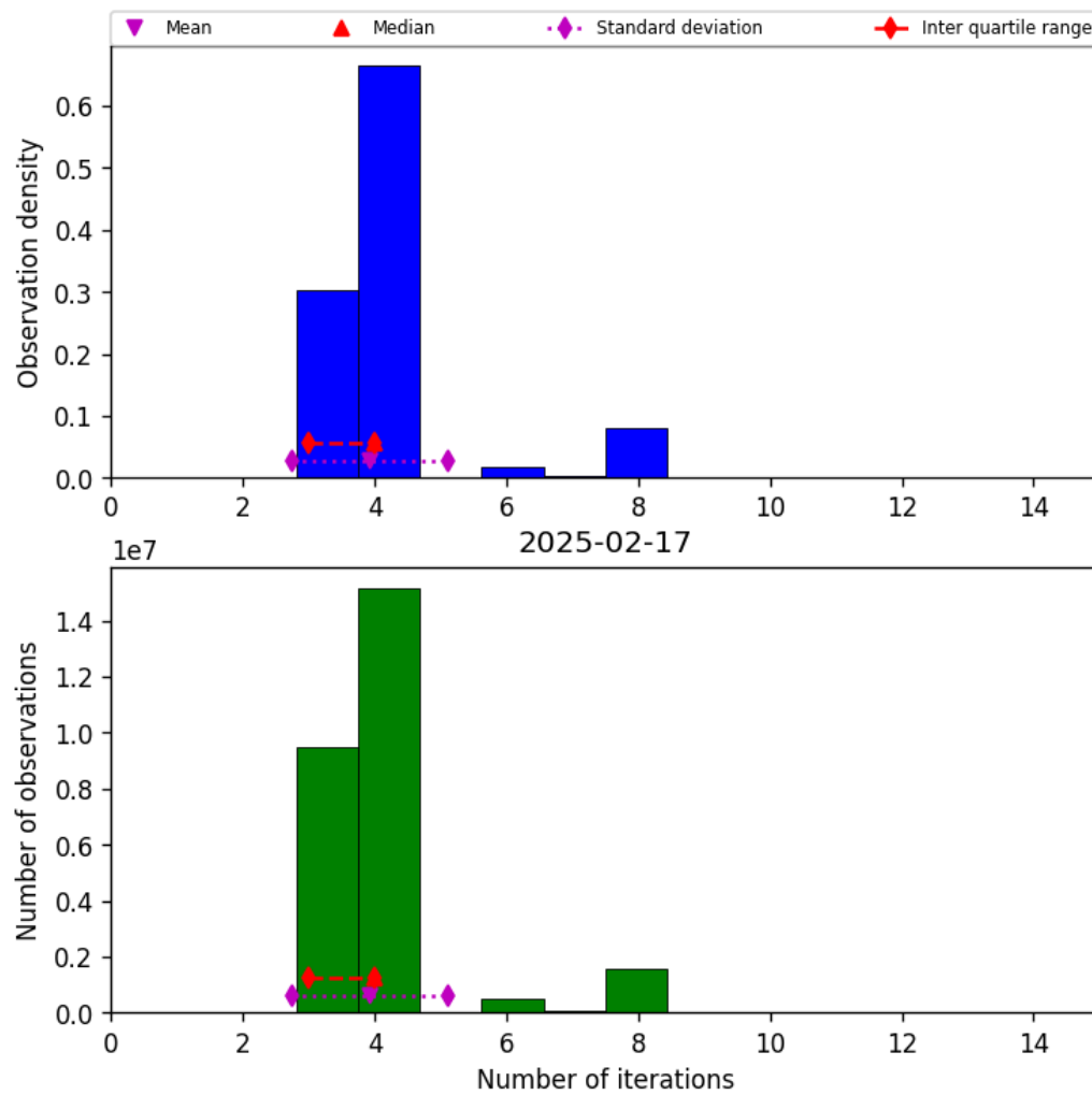
Figure 34: Histogram of “Number of iterations” for 2025-02-16 to 2025-02-18
