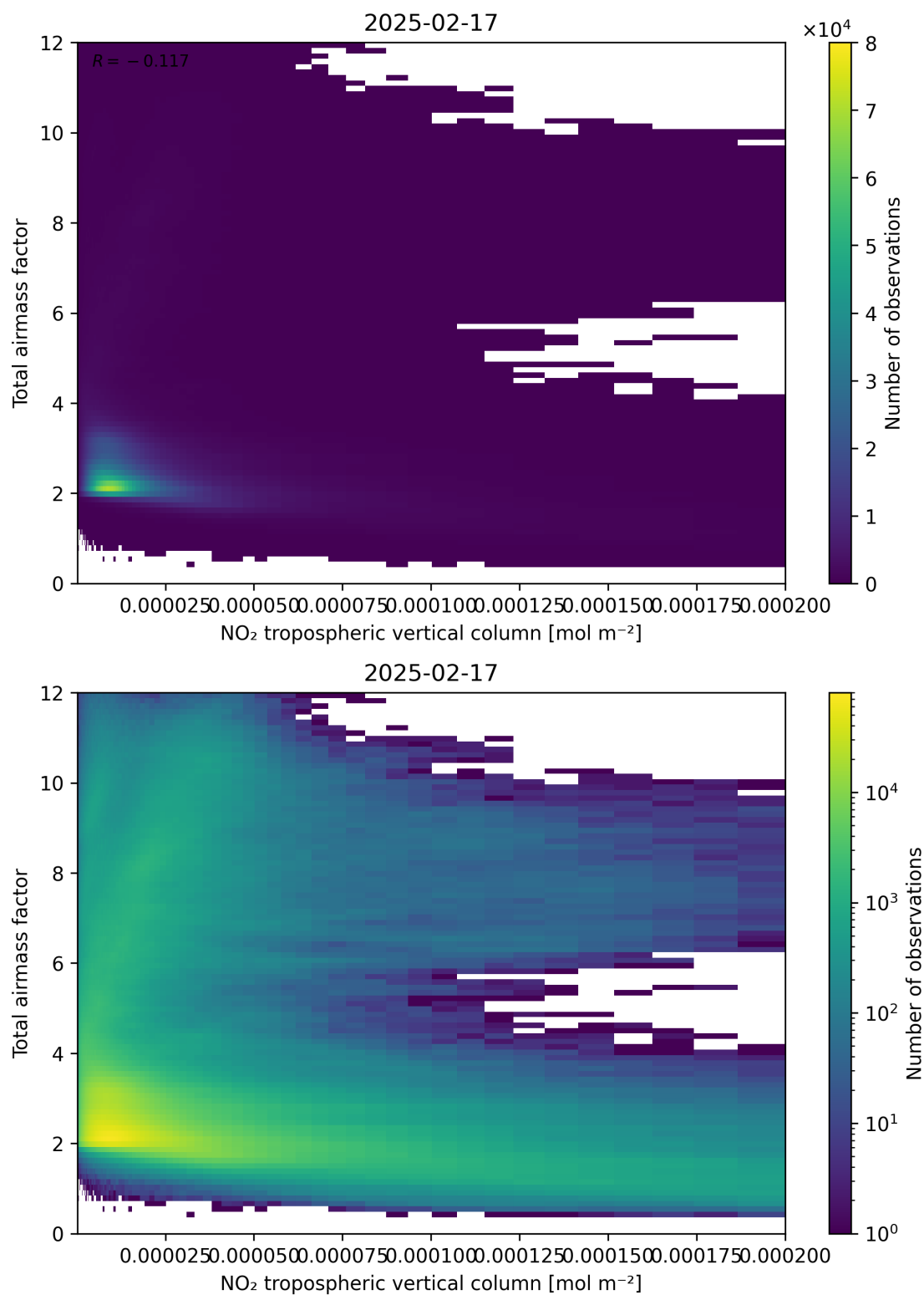
Figure 122: Scatter density plot of “NO 2 tropospheric vertical column” against “Total air mass factor” for 2025-02-16 to 2025-02-18.
