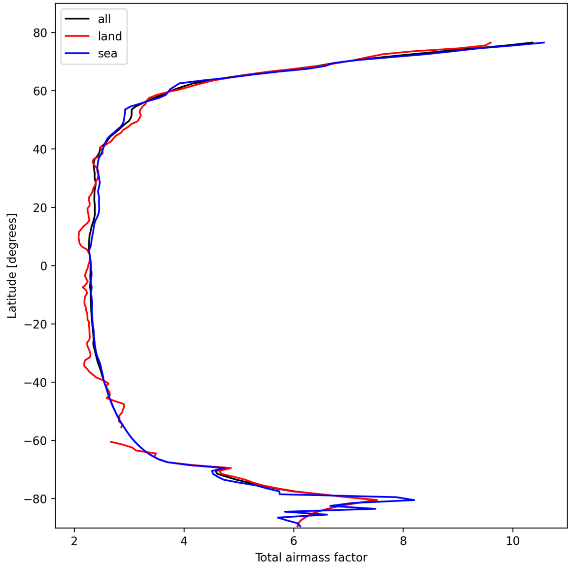
Figure 15: Zonal average of “Total airmass factor” for 2025-02-16 to 2025-02-18.
