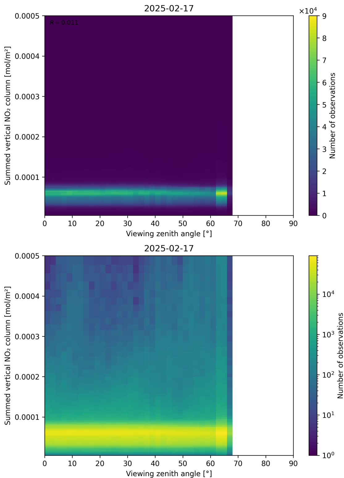
Figure 165: Scatter density plot of “Viewing zenith angle” against “Summed vertical NO 2 column” for 2025-02-16 to 2025-02-18.
