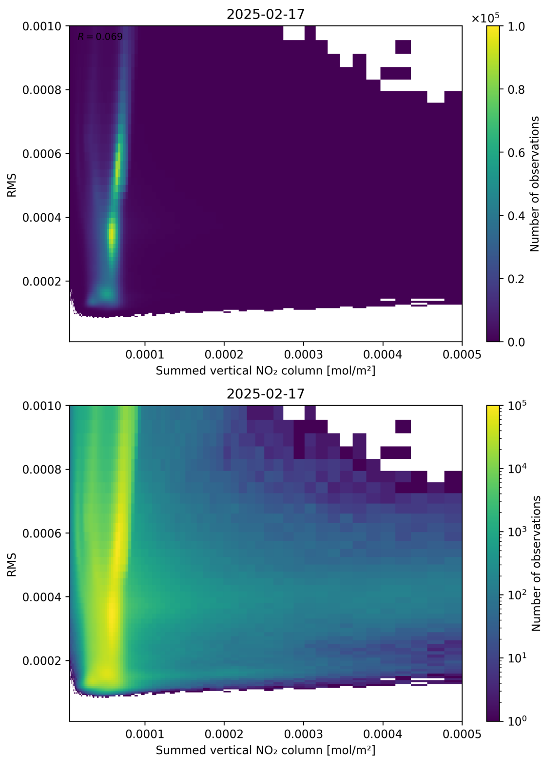
Figure 109: Scatter density plot of “Summed vertical NO 2 column” against “RMS” for 2025-02-16 to 2025-02-18.
