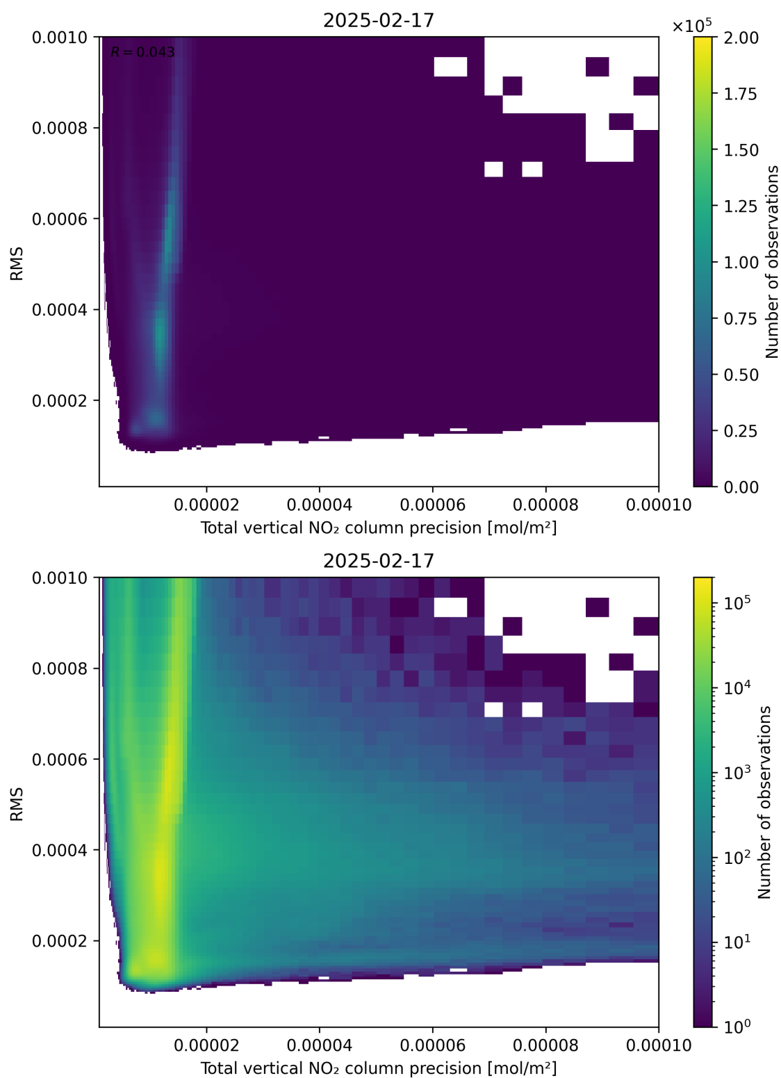
Figure 119: Scatter density plot of “Total vertical NO 2 column precision” against “RMS” for 2025-02-16 to 2025-02-18.
