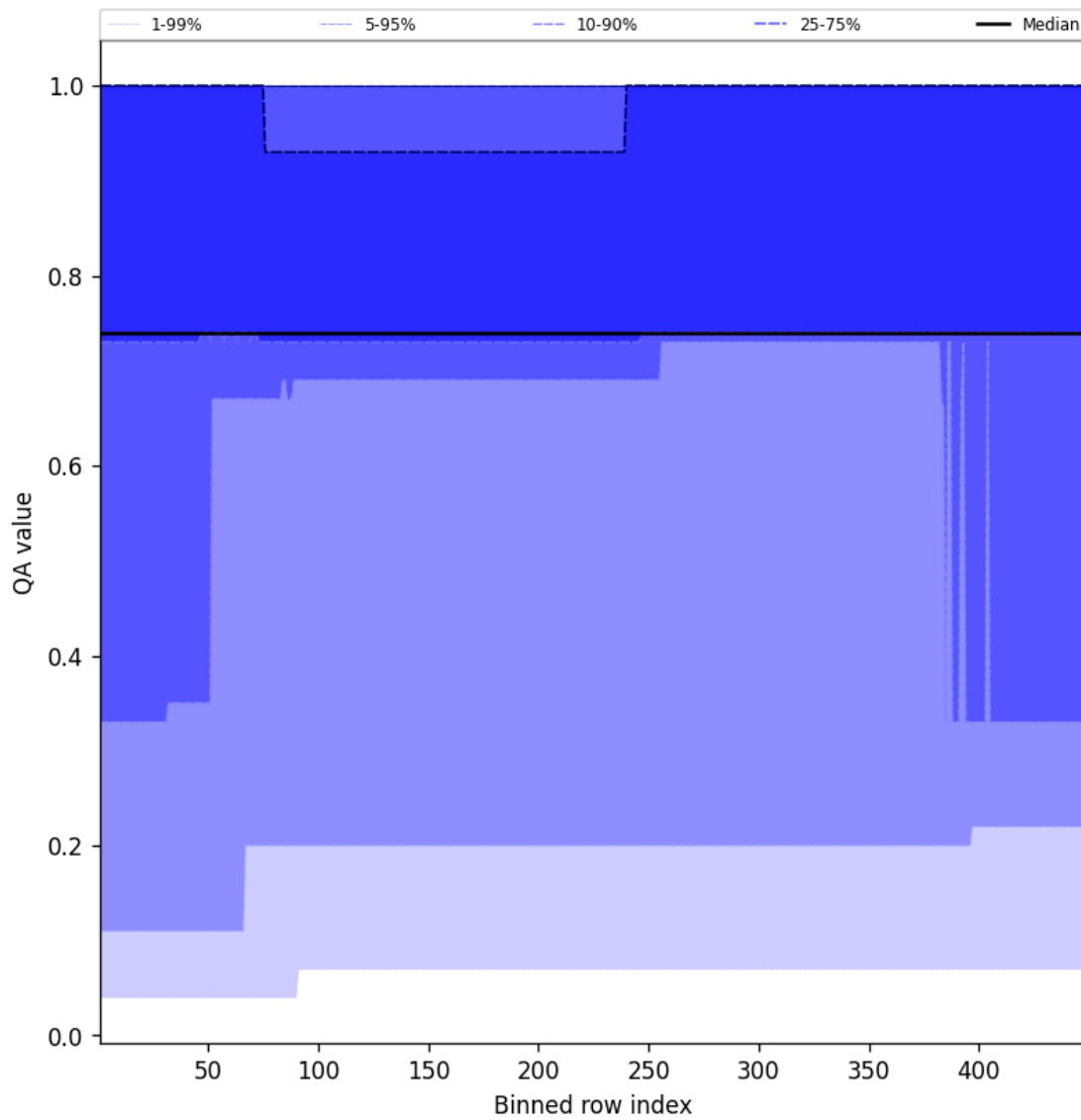
Figure 45: Along track statistics of “QA value” for 2025-02-16 to 2025-02-18
