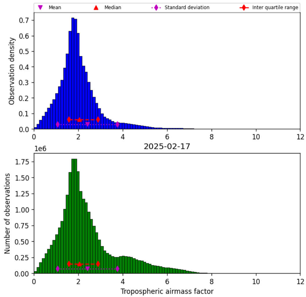
Figure 31: Histogram of “Tropospheric airmass factor” for 2025-02-16 to 2025-02-18
