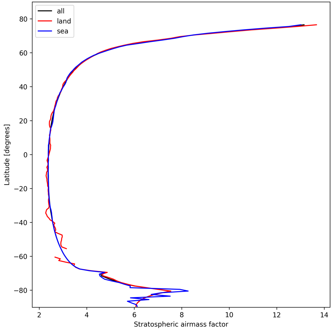
Figure 27: Zonal average of “Stratospheric airmass factor” for 2025-02-16 to 2025-02-18.
