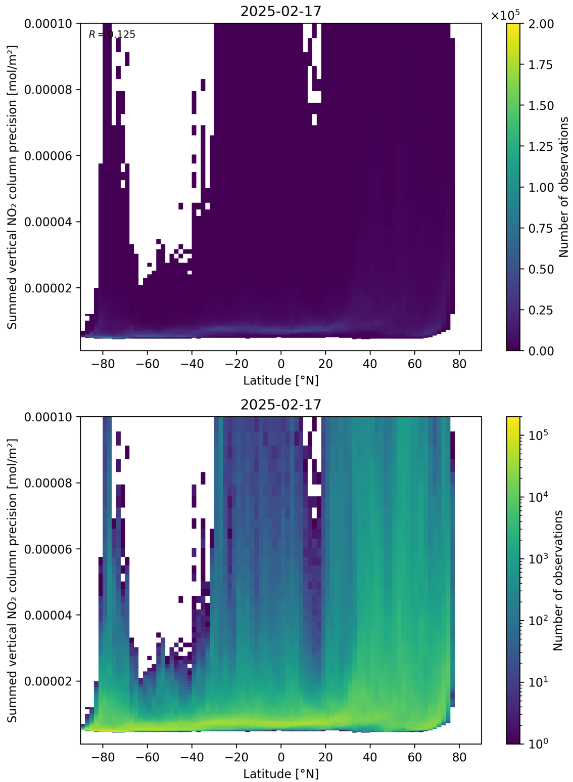
Figure 89: Scatter density plot of “Latitude” against “Summed vertical NO 2 column precision” for 2025-02-16 to 2025-02-18.
