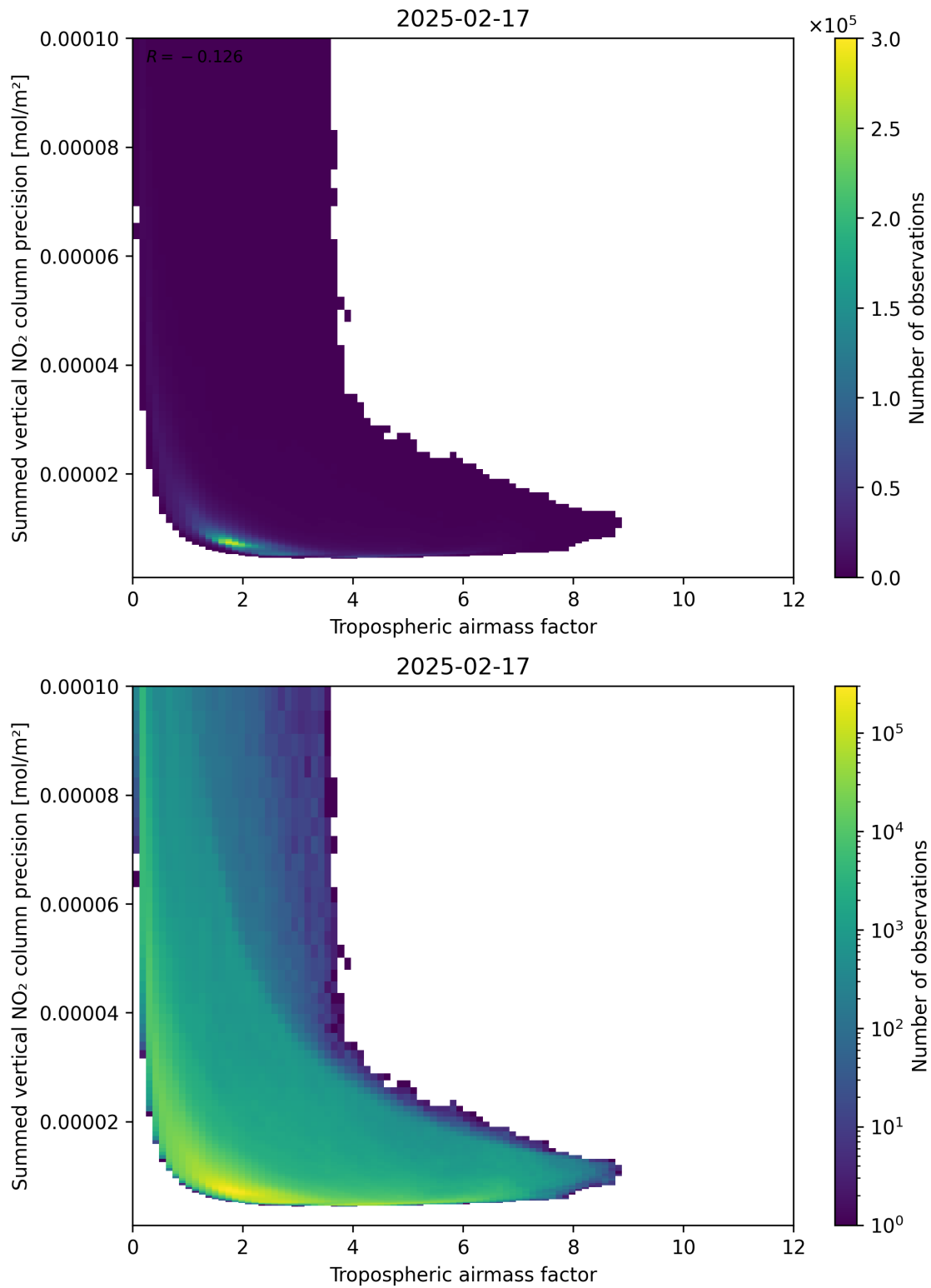
Figure 76: Scatter density plot of “Tropospheric air mass factor” against “Summed vertical NO 2 column precision” for 2025-02-16 to 2025-02-18.
