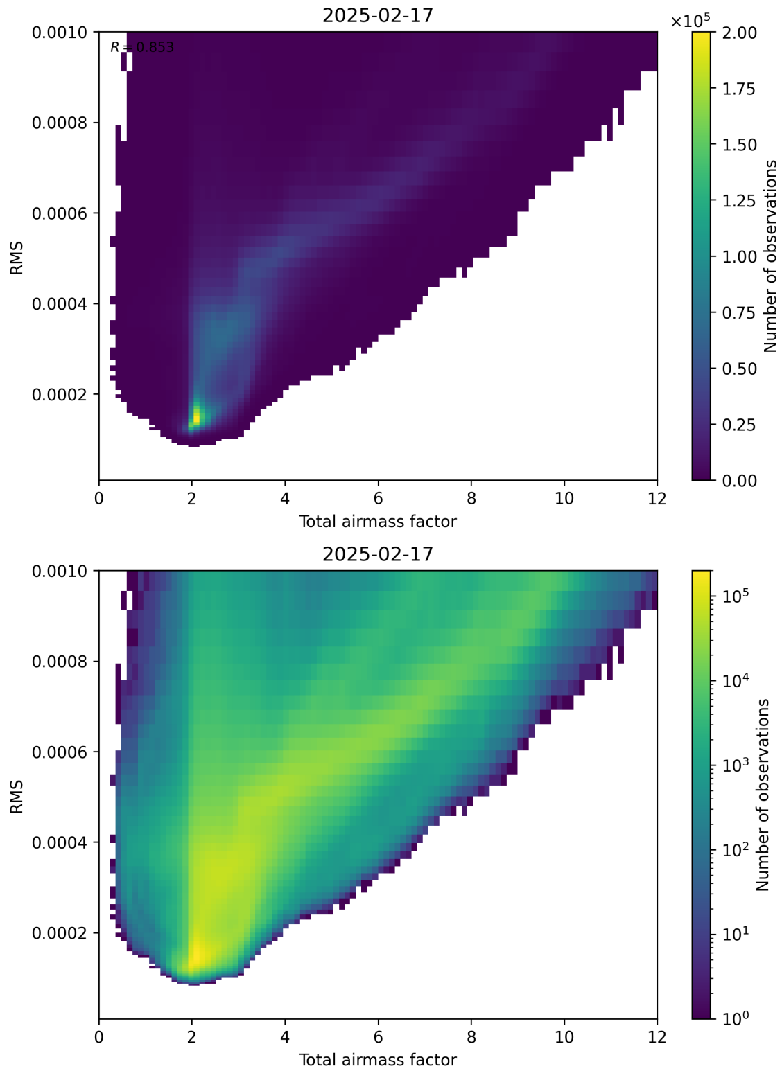
Figure 69: Scatter density plot of “Total airmass factor” against “RMS” for 2025-02-16 to 2025-02-18.
