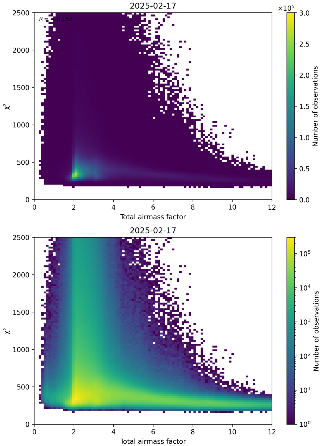
Figure 63: Scatter density plot of “Total airmass factor” against “ \chi^2 ” for 2025-02-16 to 2025-02-18.
