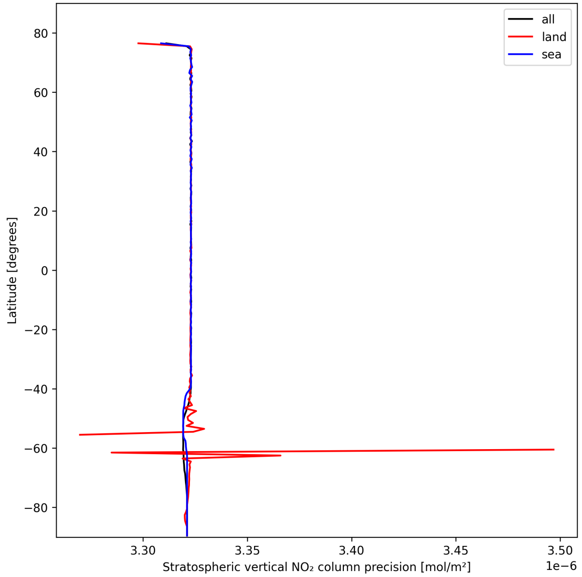
Figure 20: Zonal average of “Stratospheric vertical NO 2 column precision” for 2025-02-16 to 2025-02-18.
