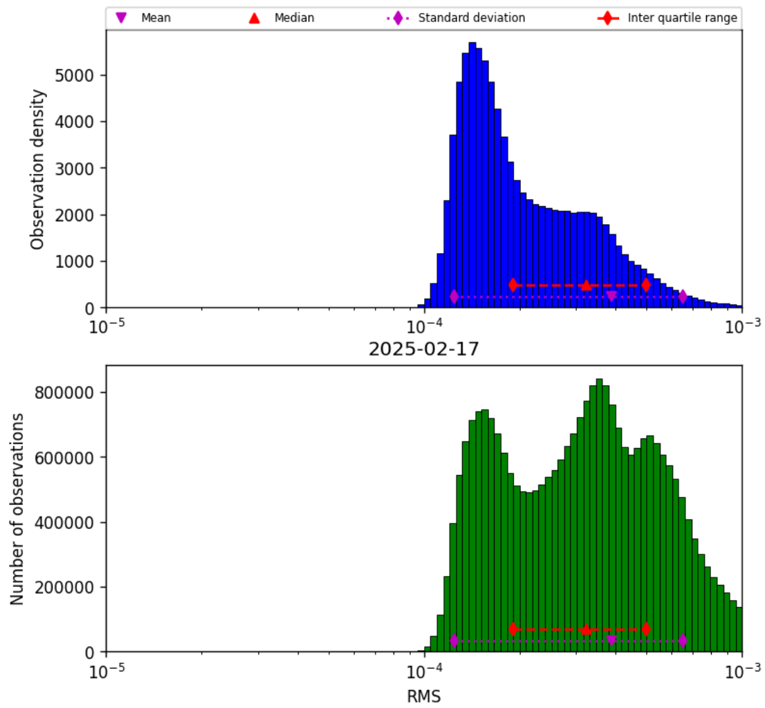
Figure 43: Histogram of “RMS” for 2025-02-16 to 2025-02-18
