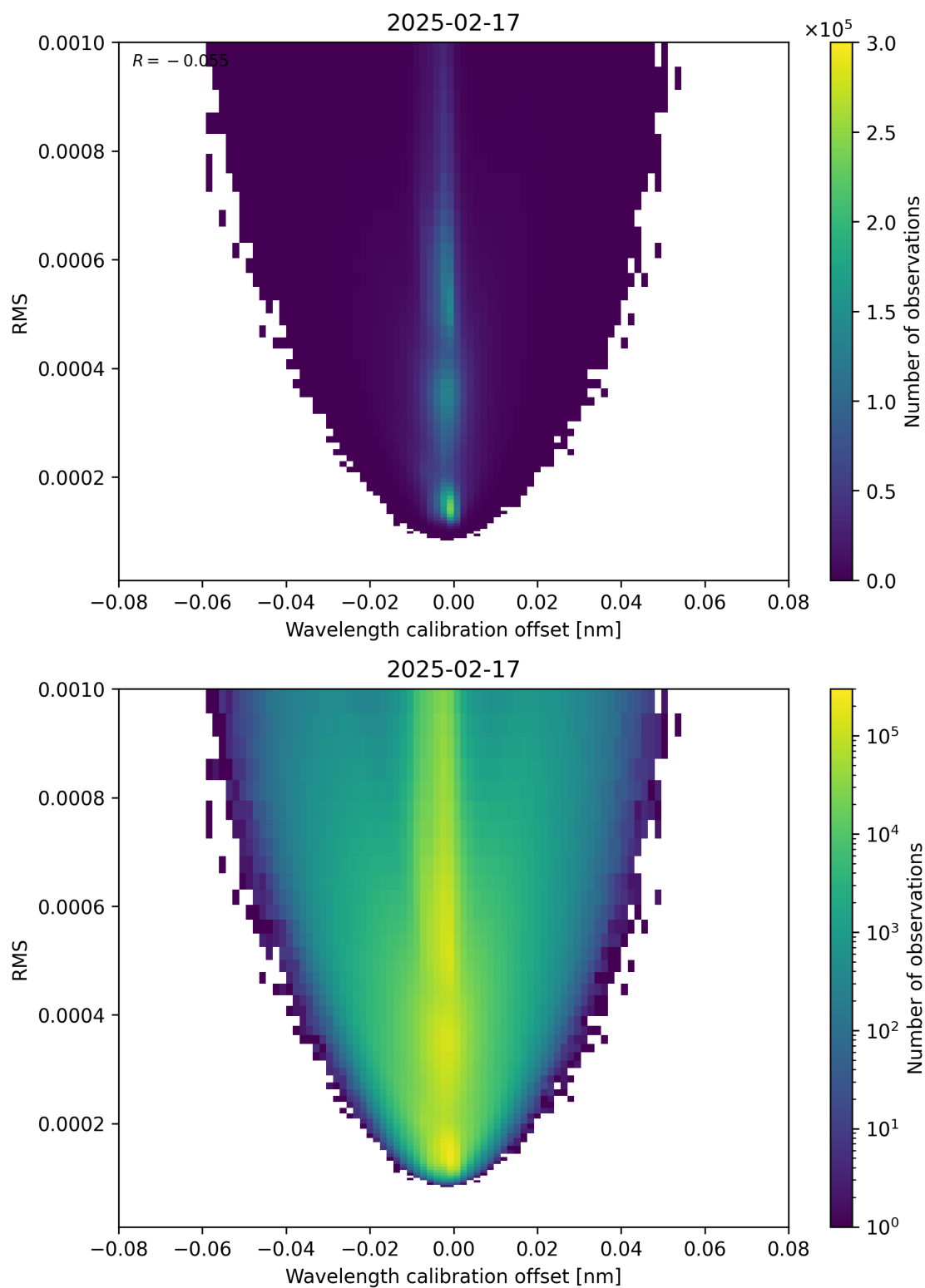
Figure 181: Scatter density plot of “Wavelength calibration offset” against “RMS” for 2025-02-16 to 2025-02-18.
