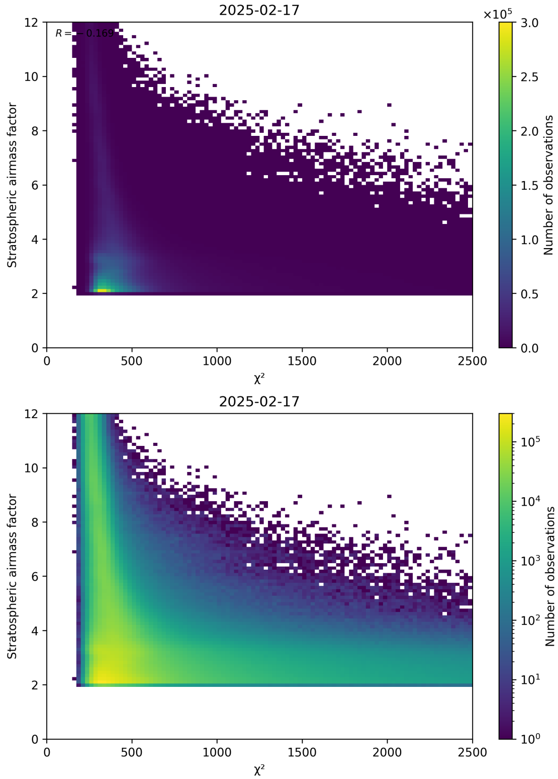
Figure 81: Scatter density plot of “ \chi^2 ” against “Stratospheric airmass factor” for 2025-02-16 to 2025-02-18.
