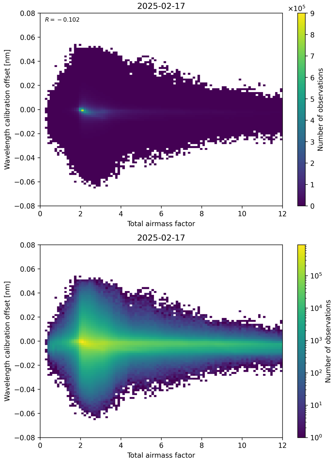
Figure 70: Scatter density plot of “Total airmass factor” against “Wavelength calibration offset” for 2025-02-16 to 2025-02-18.
