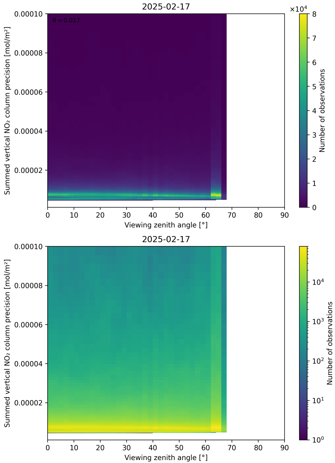
Figure 166: Scatter density plot of “Viewing zenith angle” against “Summed vertical NO 2 column precision” for 2025-02-16 to 2025-02-18.
