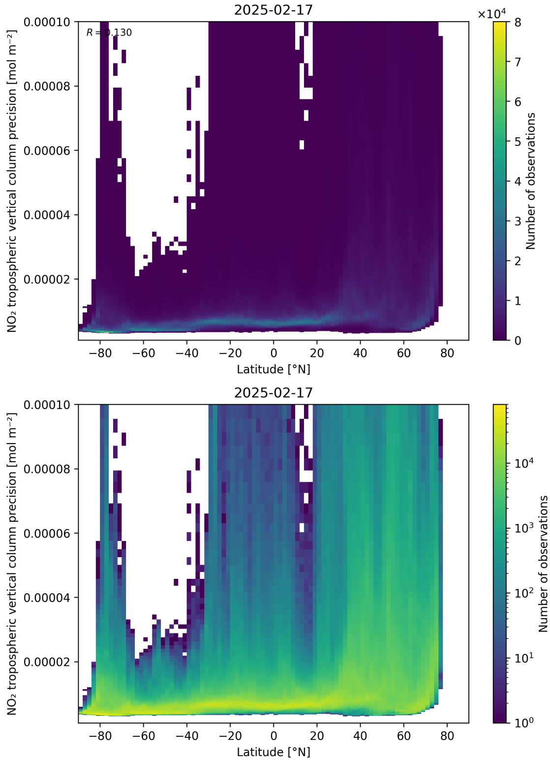
Figure 93: Scatter density plot of “Latitude” against “NO 2 tropospheric vertical column precision” for 2025-02-16 to 2025-02-18.
