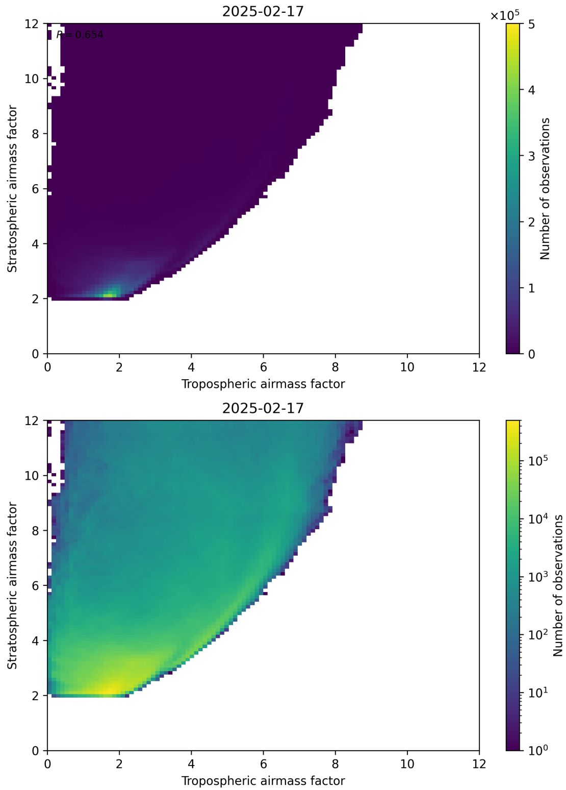
Figure 71: Scatter density plot of “Tropospheric airmass factor” against “Stratospheric airmass factor” for 2025-02-16 to 2025-02-18.
