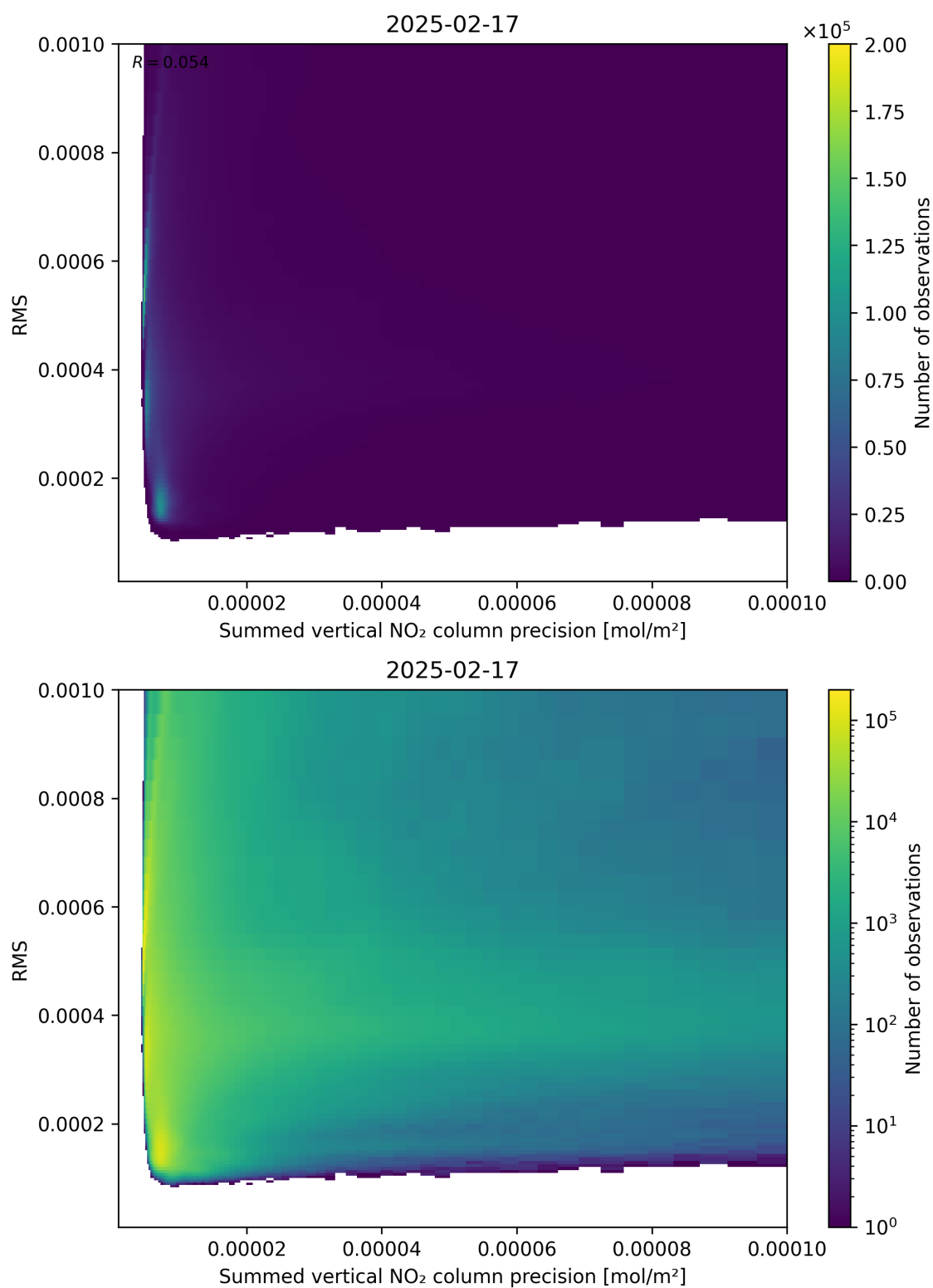
Figure 108: Scatter density plot of “Summed vertical NO 2 column precision” against “RMS” for 2025-02-16 to 2025-02-18.
