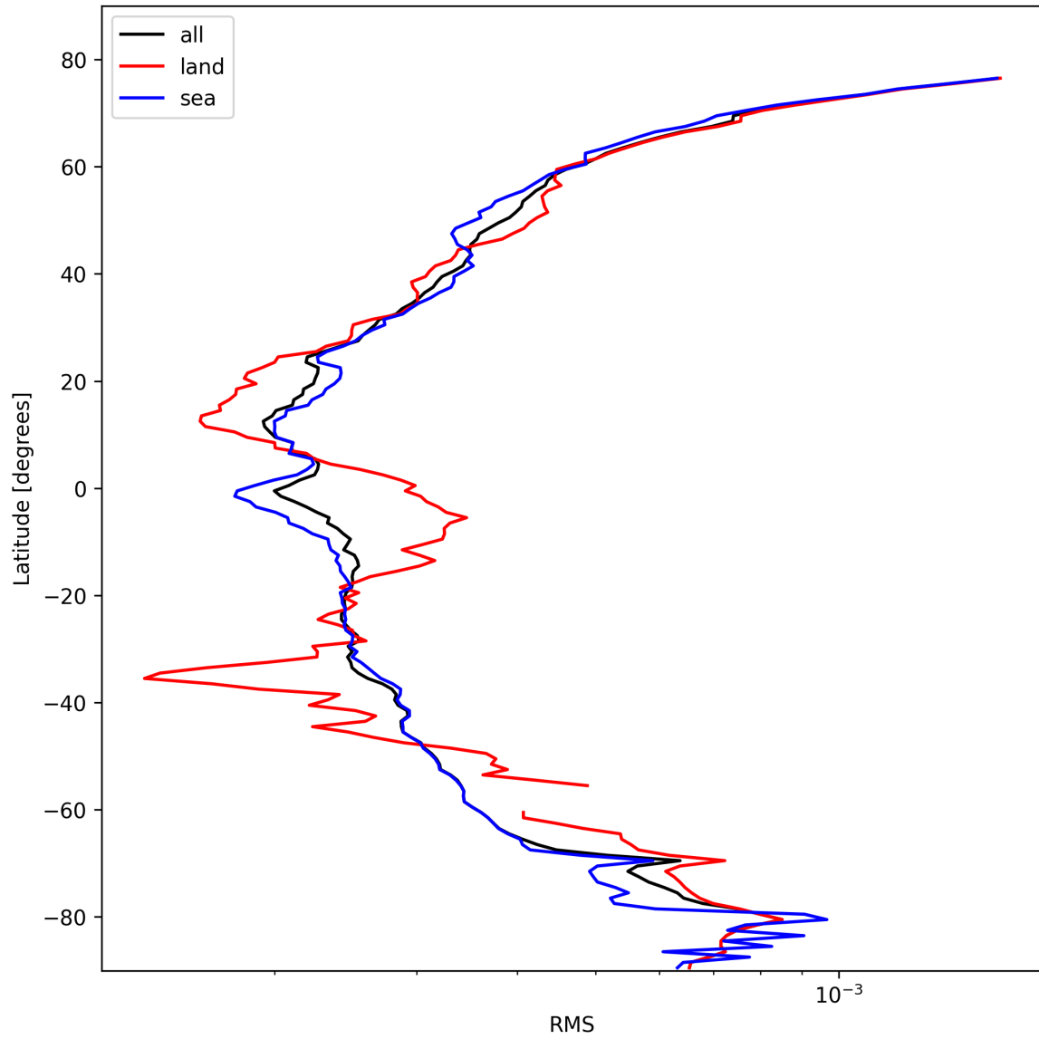
Figure 26: Zonal average of “RMS” for 2025-02-16 to 2025-02-18.
