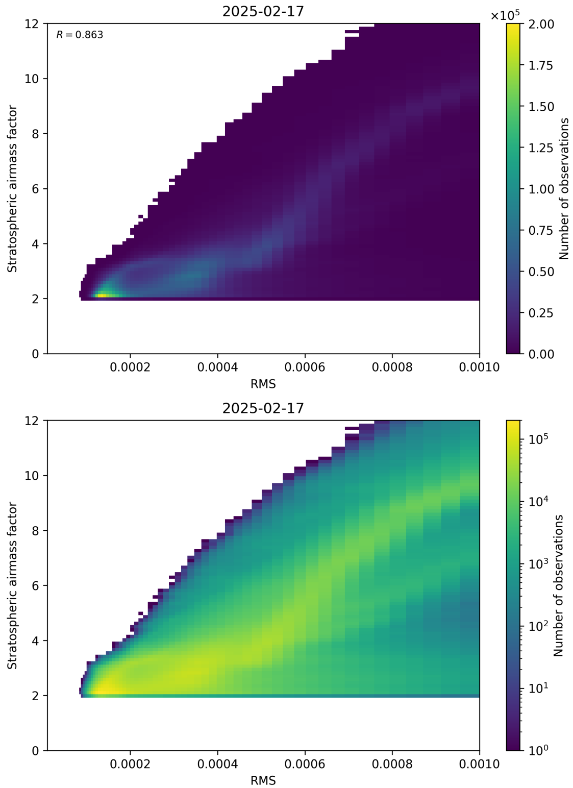
Figure 144: Scatter density plot of “RMS” against “Stratospheric airmass factor” for 2025-02-16 to 2025-02-18.
