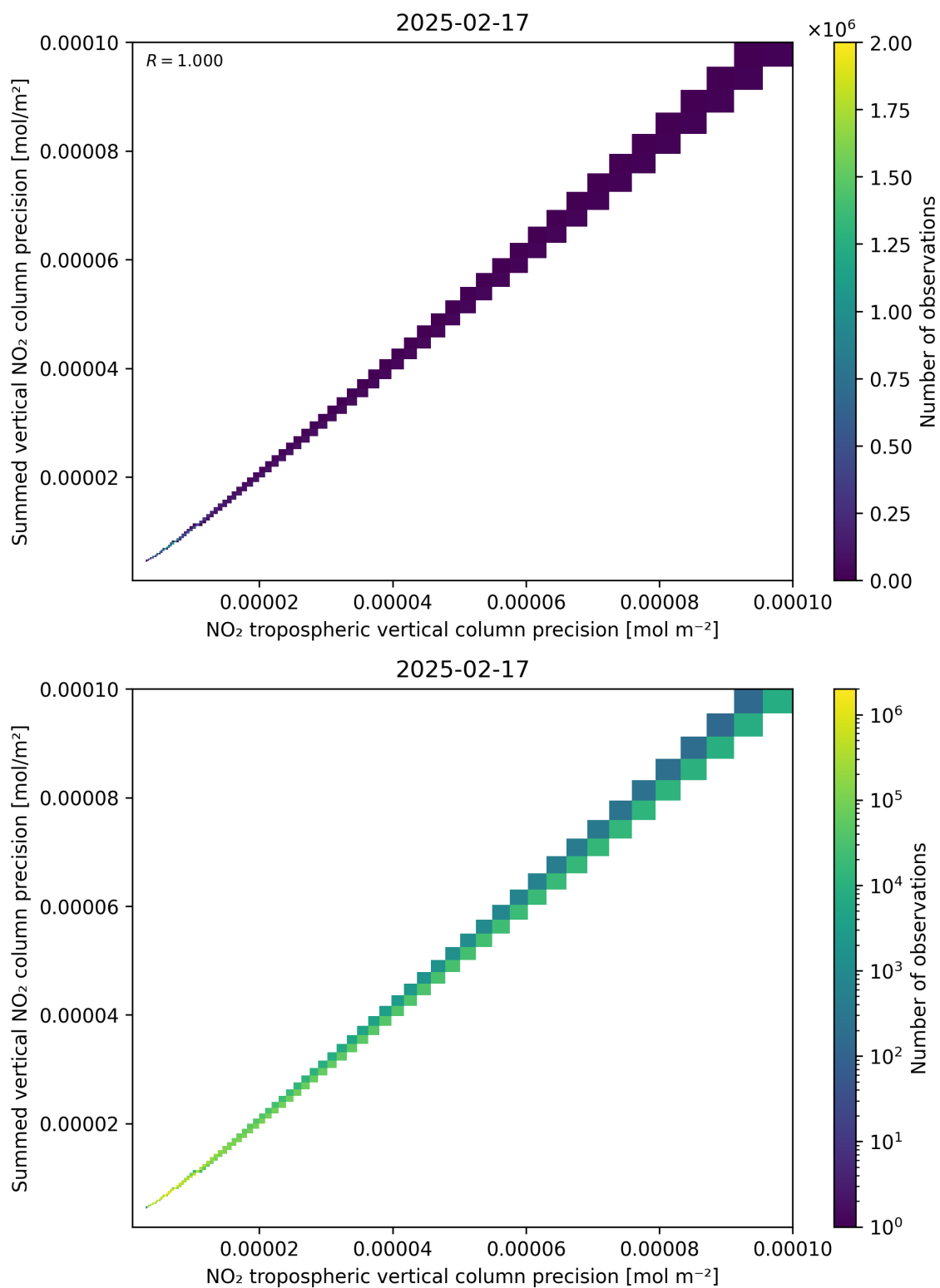
Figure 137: Scatter density plot of “NO 2 tropospheric vertical column precision” against “Summed vertical NO 2 column precision” for 2025-02-16 to 2025-02-18.
