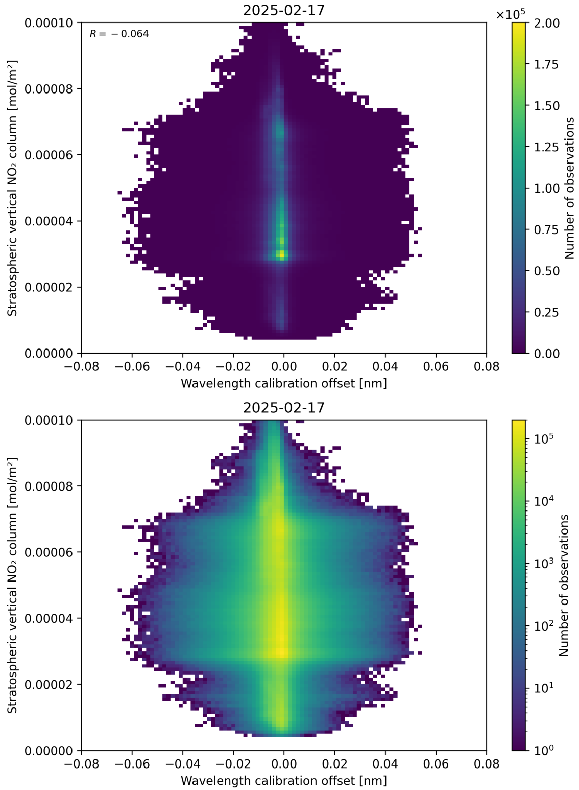
Figure 176: Scatter density plot of “Wavelength calibration offset” against “Stratospheric vertical NO 2 column” for 2025-02-16 to 2025-02-18.
