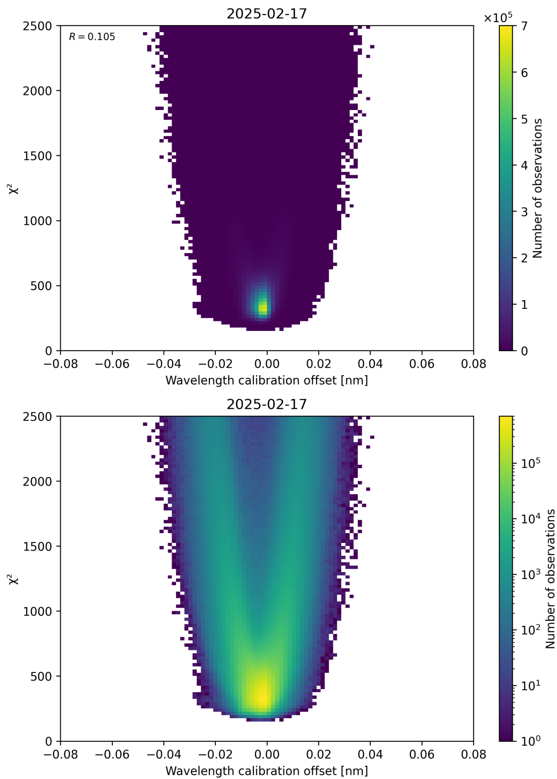
Figure 175: Scatter density plot of “Wavelength calibration offset” against “ \chi^2 ” for 2025-02-16 to 2025-02-18.
