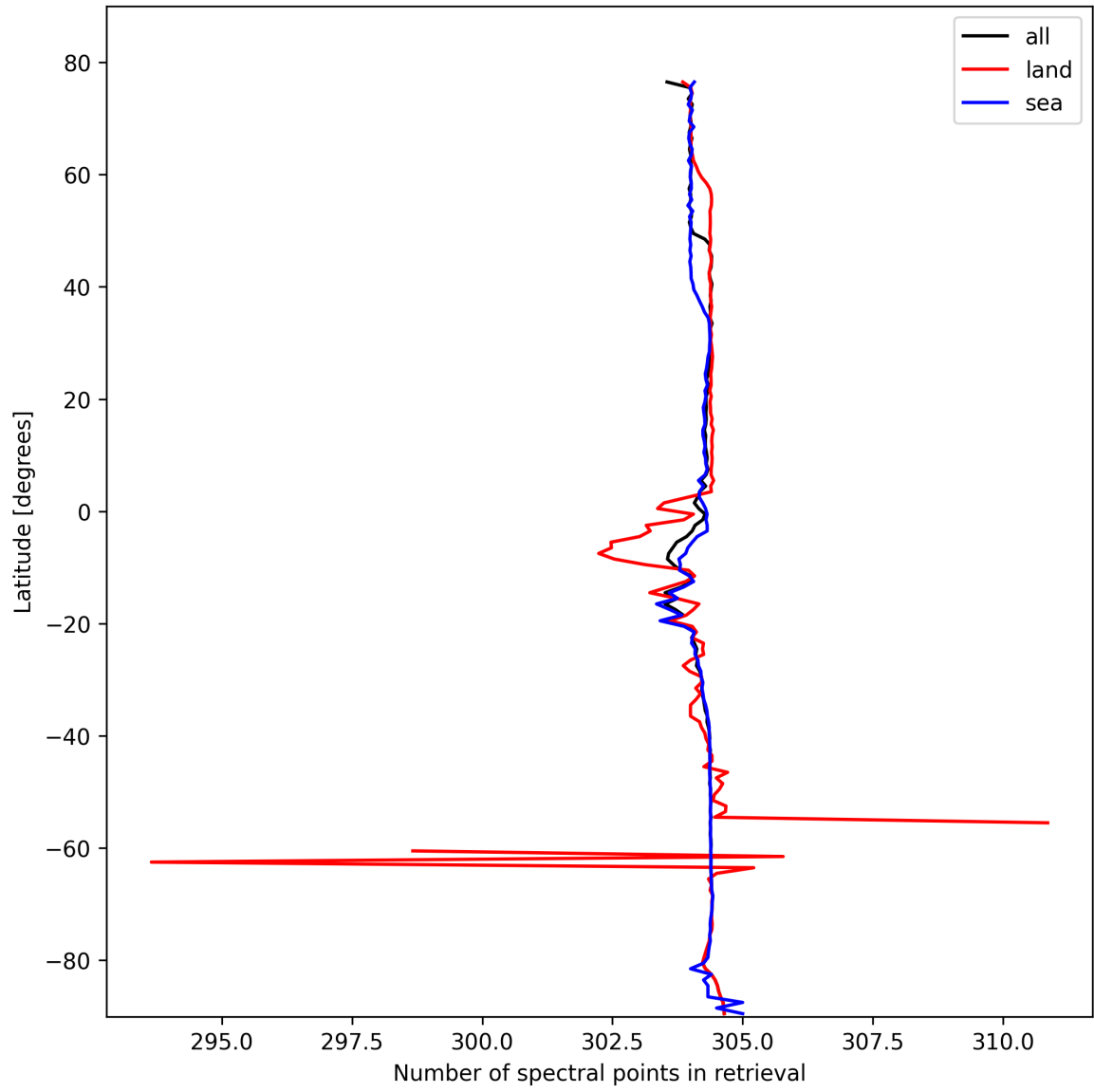
Figure 16: Zonal average of “Number of spectral points in retrieval” for 2025-02-16 to 2025-02-18.
