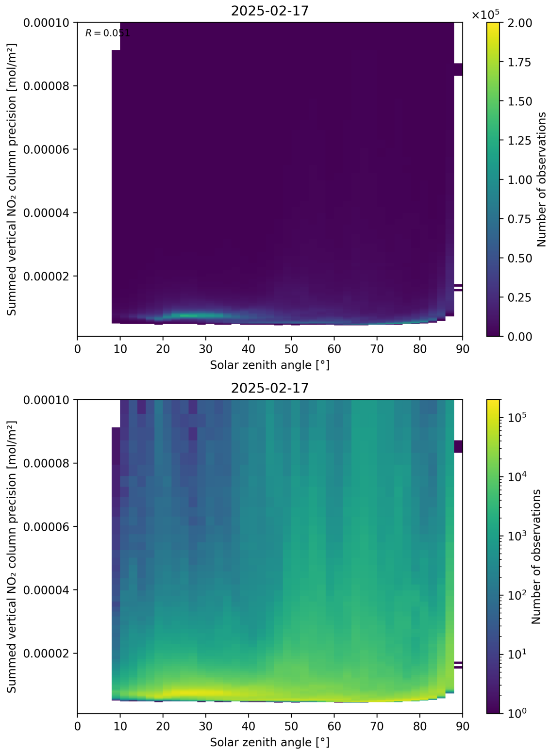
Figure 152: Scatter density plot of “Solar zenith angle” against “Summed vertical NO 2 column precision” for 2025-02-16 to 2025-02-18.
