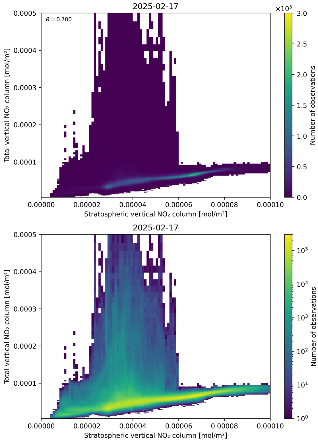
Figure 100: Scatter density plot of “Stratospheric vertical NO 2 column” against “Total vertical NO 2 column” for 2025-02-16 to 2025-02-18.
