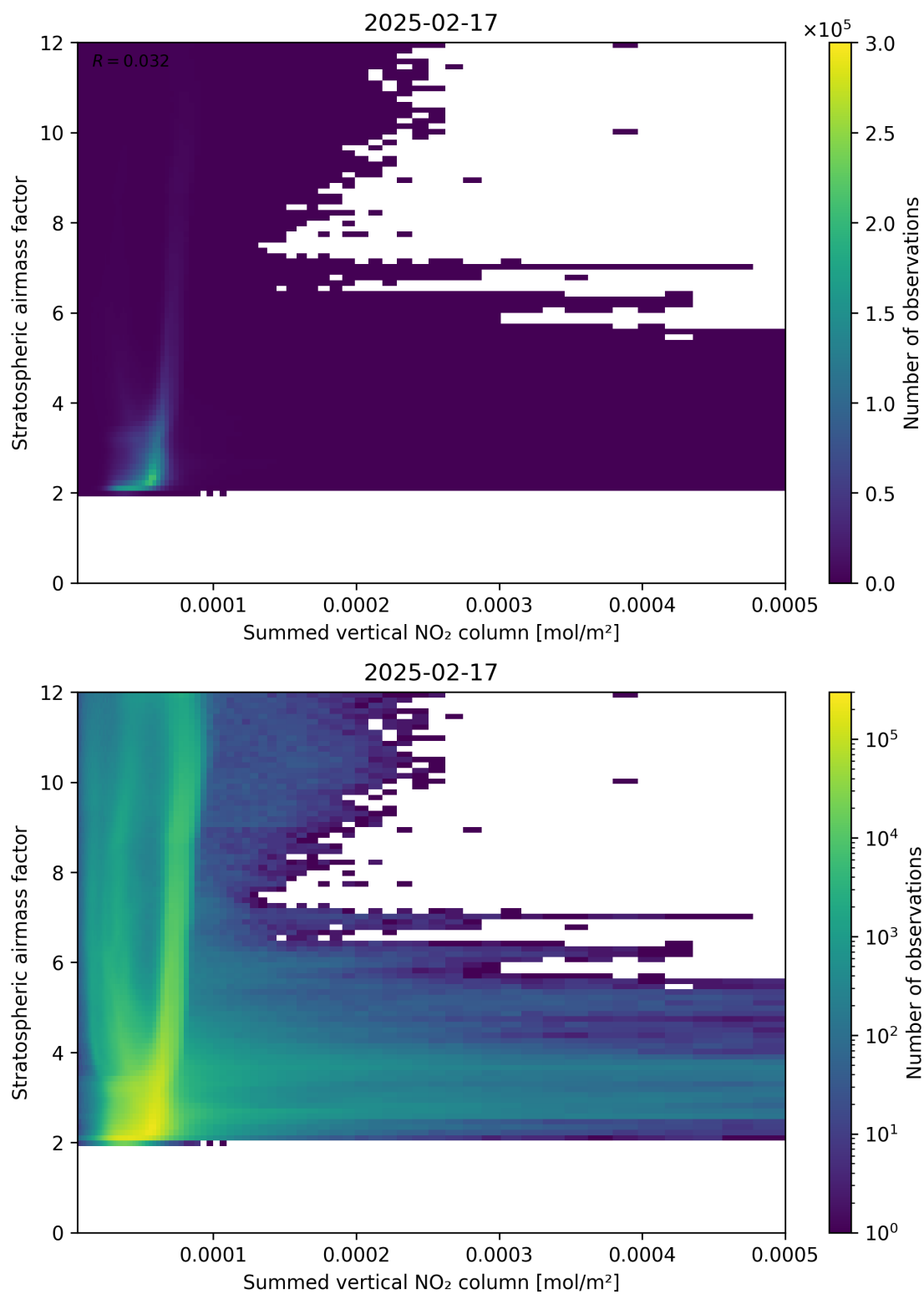
Figure 103: Scatter density plot of “Summed vertical NO 2 column” against “Stratospheric air mass factor” for 2025-02-16 to 2025-02-18.
