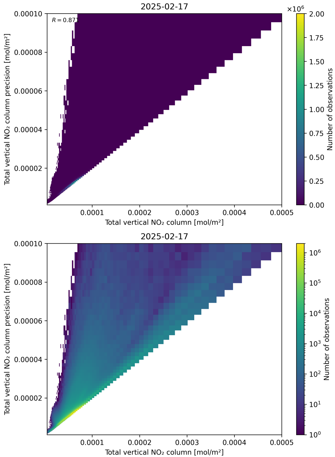
Figure 114: Scatter density plot of “Total vertical NO 2 column” against “Total vertical NO 2 column precision” for 2025-02-16 to 2025-02-18.
