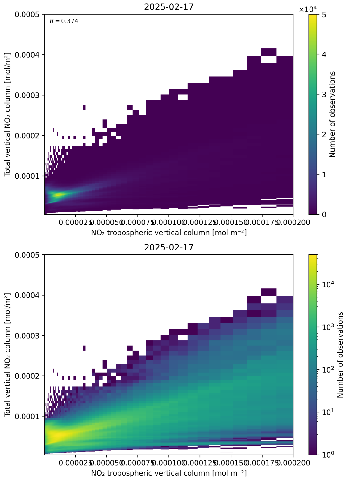
Figure 128: Scatter density plot of “NO 2 tropospheric vertical column” against “Total vertical NO 2 column” for 2025-02-16 to 2025-02-18.
