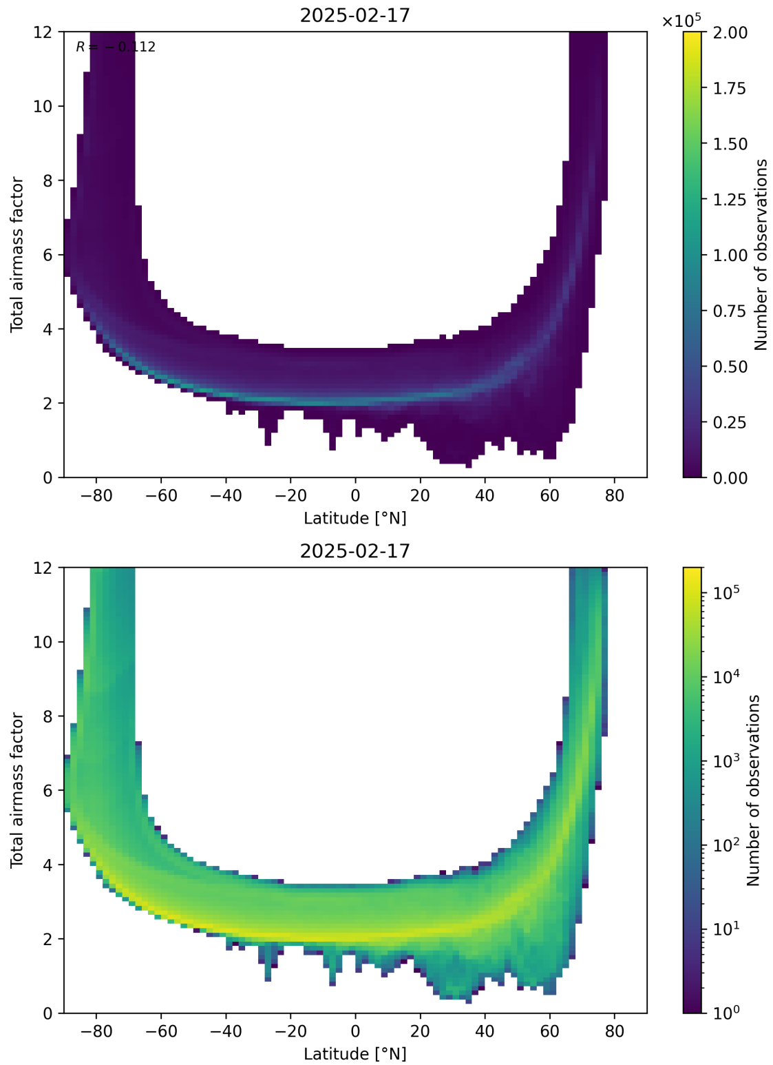
Figure 84: Scatter density plot of “Latitude” against “Total airmass factor” for 2025-02-16 to 2025-02-18.
