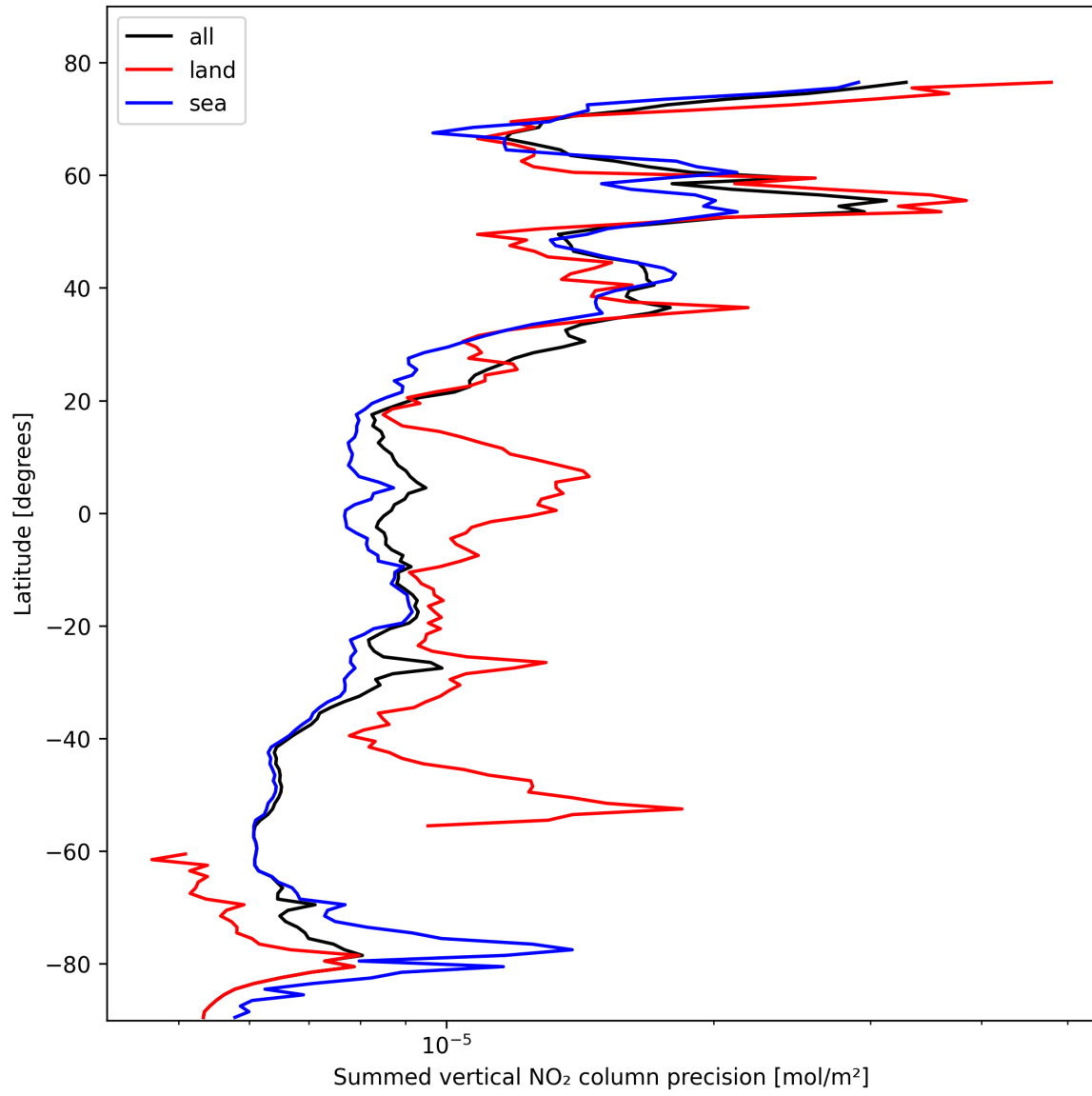
Figure 24: Zonal average of “Summed vertical NO 2 column precision” for 2025-02-16 to 2025-02-18.
