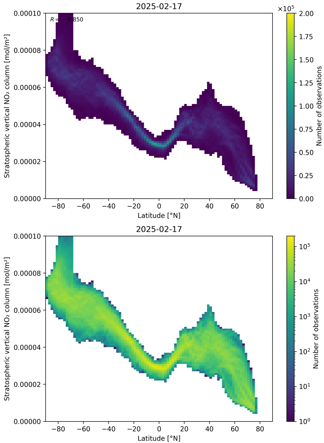
Figure 87: Scatter density plot of “Latitude” against “Stratospheric vertical NO 2 column” for 2025-02-16 to 2025-02-18.
