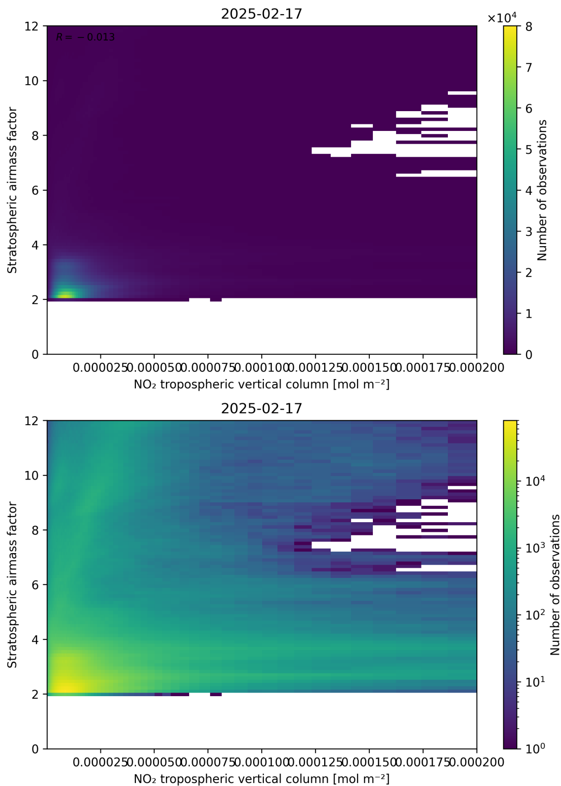
Figure 121: Scatter density plot of “NO 2 tropospheric vertical column” against “Stratospheric airmass factor” for 2025-02-16 to 2025-02-18.
