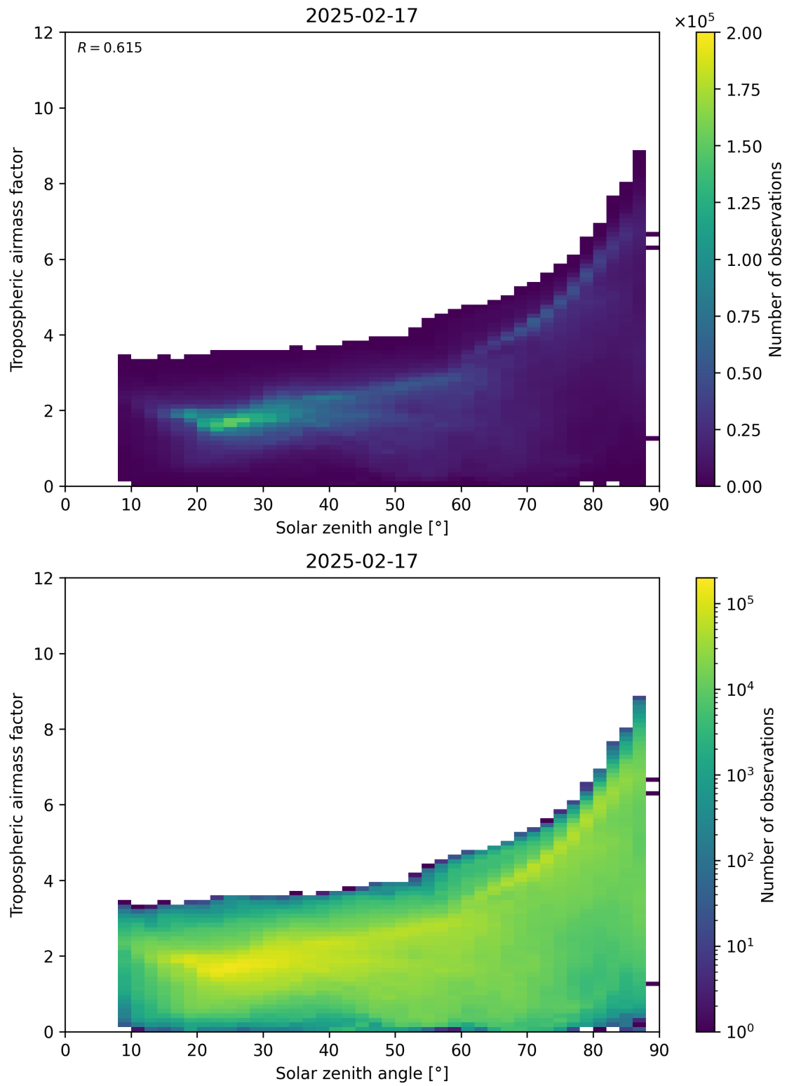
Figure 147: Scatter density plot of “Solar zenith angle” against “Tropospheric airmass factor” for 2025-02-16 to 2025-02-18.
