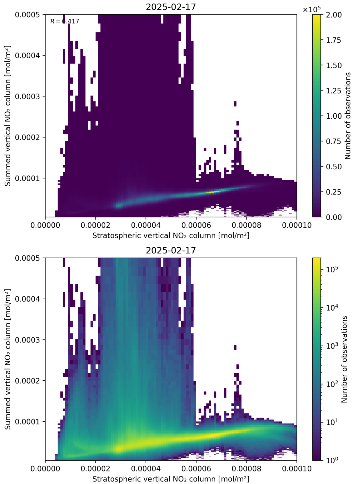
Figure 98: Scatter density plot of “Stratospheric vertical NO 2 column” against “Summed vertical NO 2 column” for 2025-02-16 to 2025-02-18.
