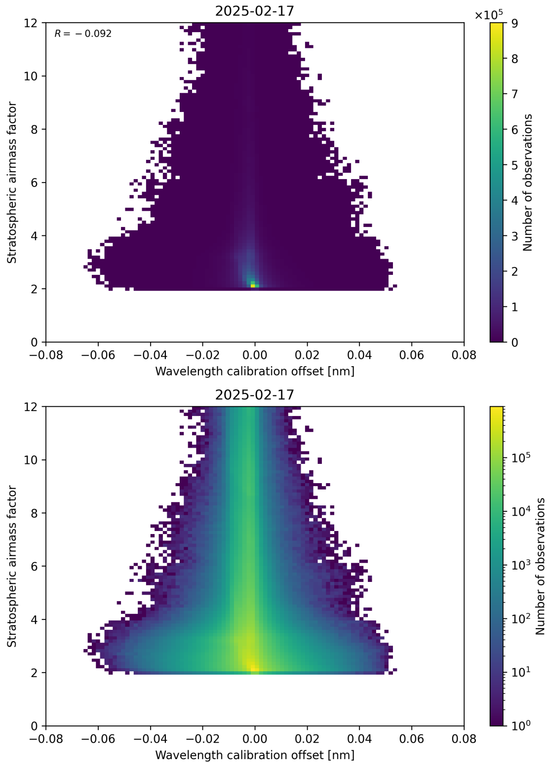
Figure 174: Scatter density plot of “Wavelength calibration offset” against “Stratospheric airmass factor” for 2025-02-16 to 2025-02-18.
