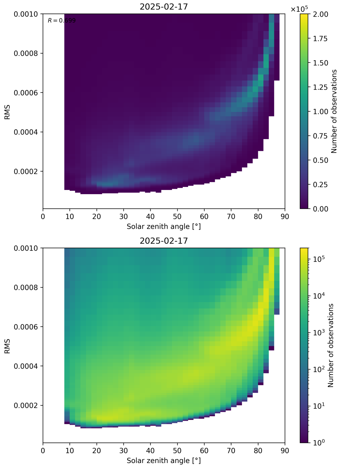
Figure 157: Scatter density plot of “Solar zenith angle” against “RMS” for 2025-02-16 to 2025-02-18.
