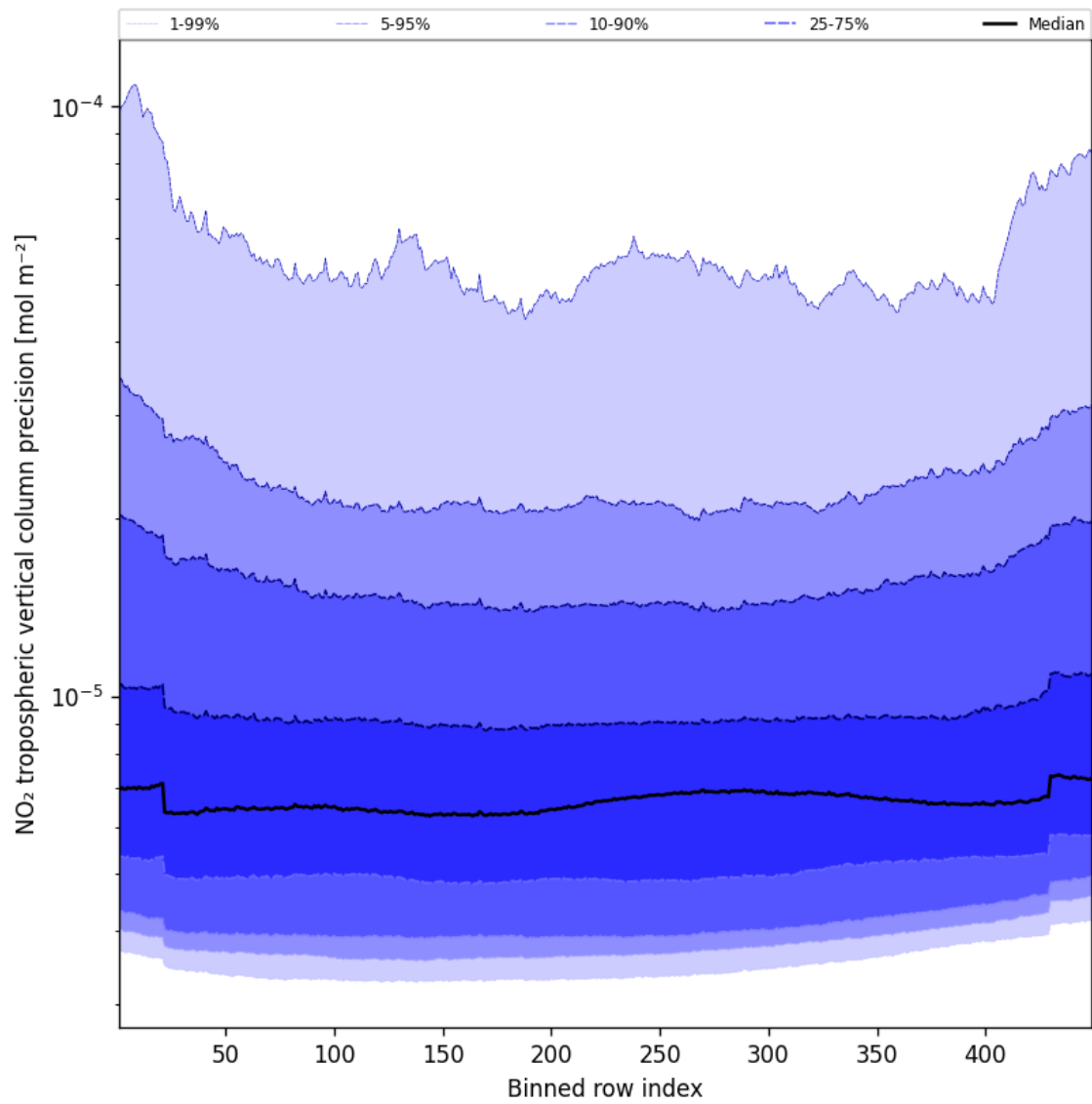
Figure 47: Along track statistics of “NO 2 tropospheric vertical column precision” for 2025-02-16 to 2025-02-18
