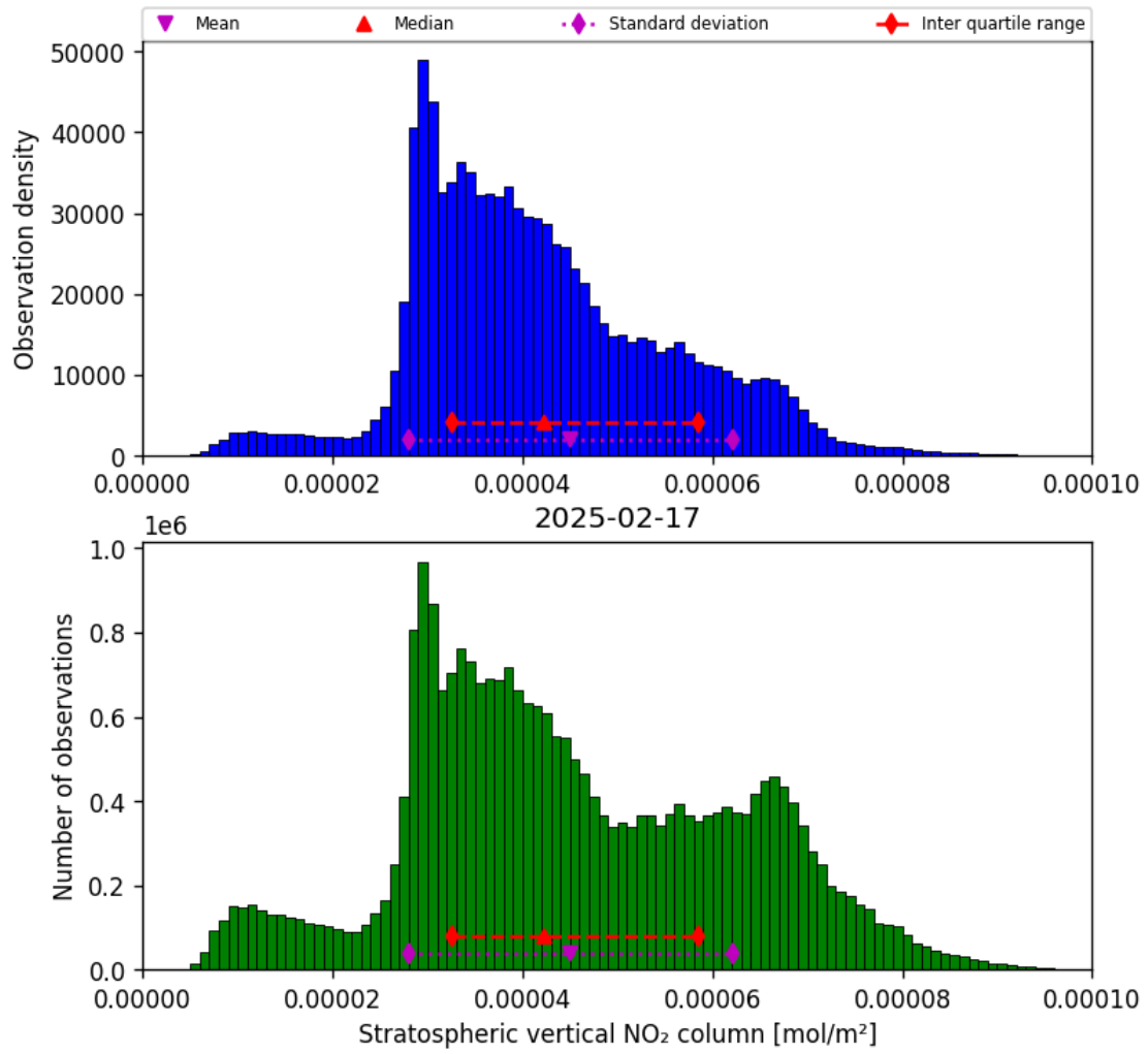
Figure 36: Histogram of “Stratospheric vertical NO 2 column” for 2025-02-16 to 2025-02-18
