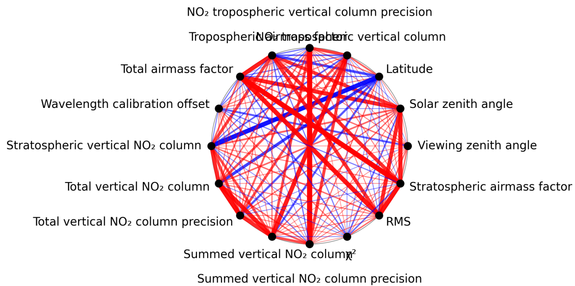
Figure 1: Map of correlation graph for 2025-02-16 to 2025-02-18.
