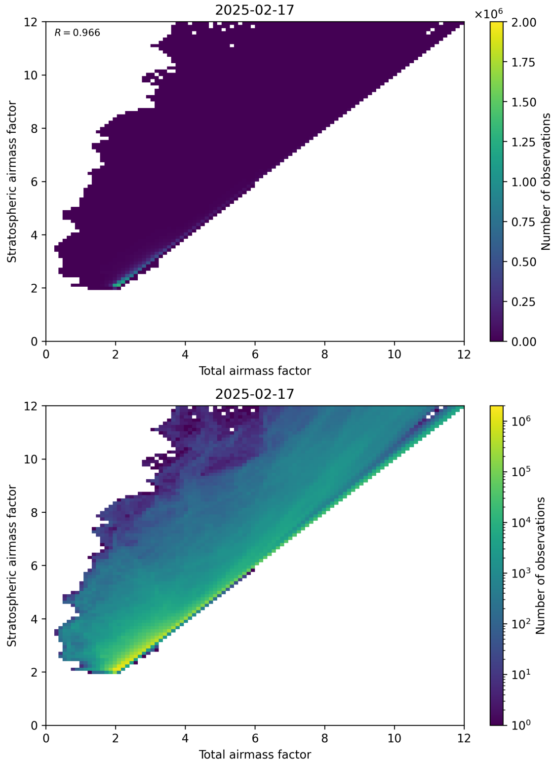
Figure 62: Scatter density plot of “Total airmass factor” against “Stratospheric airmass factor” for 2025-02-16 to 2025-02-18.
