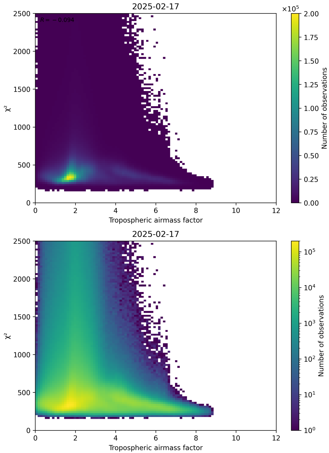
Figure 73: Scatter density plot of “Tropospheric airmass factor” against “ \chi^2 ” for 2025-02-16 to 2025-02-18.
