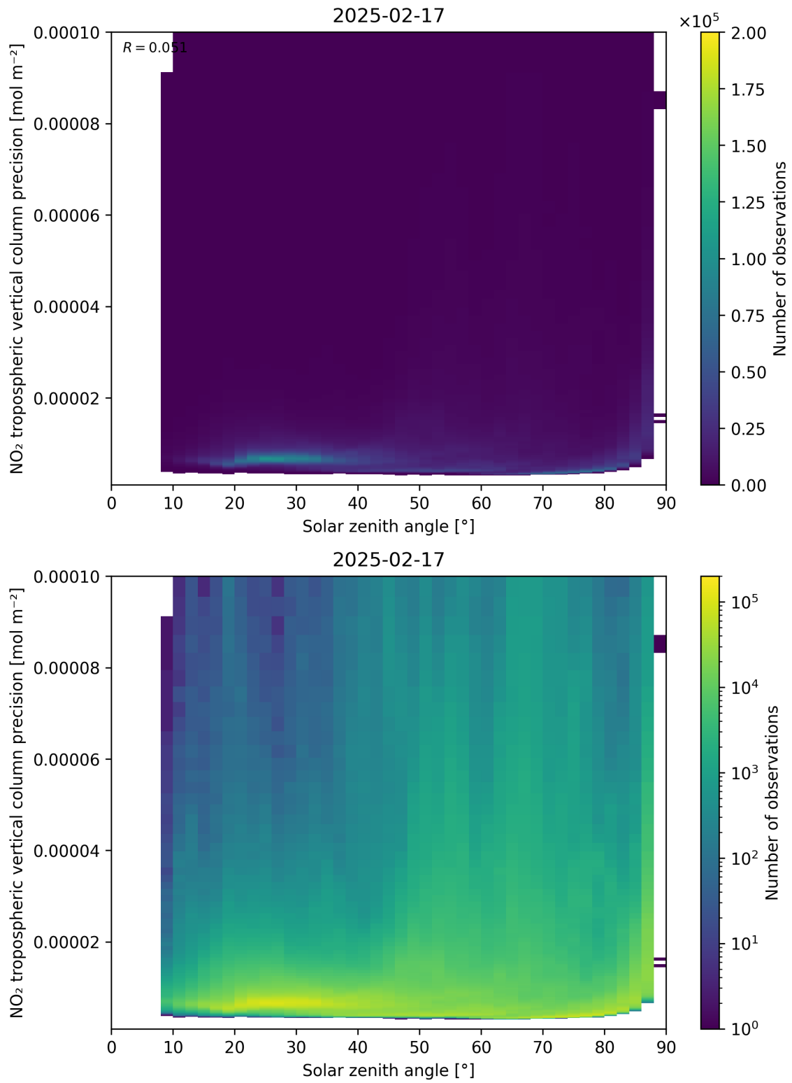
Figure 156: Scatter density plot of “Solar zenith angle” against “NO 2 tropospheric vertical column precision” for 2025-02-16 to 2025-02-18.
