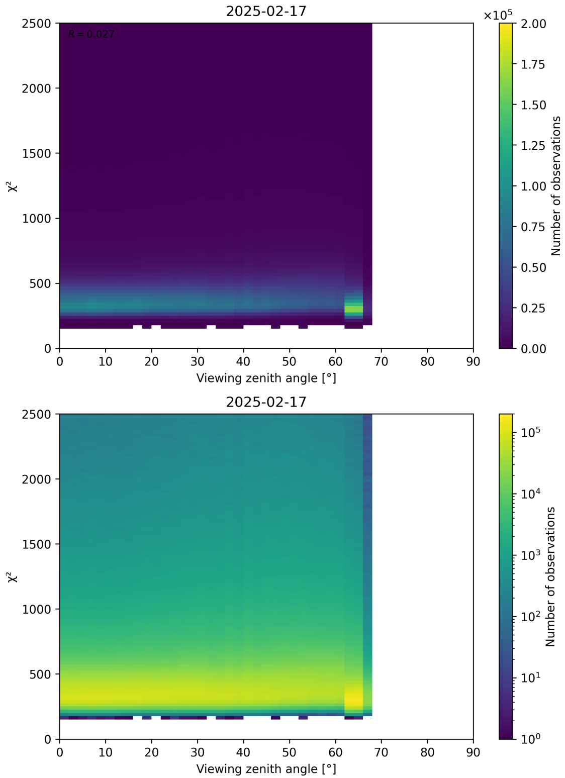
Figure 162: Scatter density plot of “Viewing zenith angle” against “ \chi^2 ” for 2025-02-16 to 2025-02-18.
