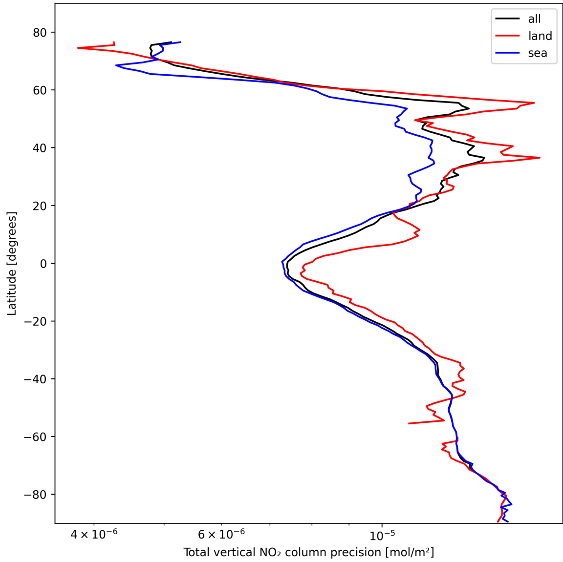
Figure 22: Zonal average of “Total vertical NO 2 column precision” for 2025-02-16 to 2025-02-18.
