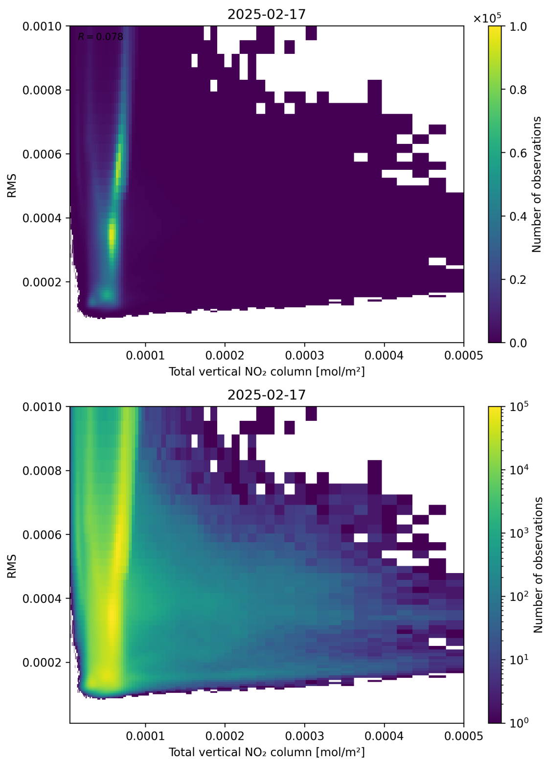
Figure 120: Scatter density plot of “Total vertical NO 2 column” against “RMS” for 2025-02-16 to 2025-02-18.
