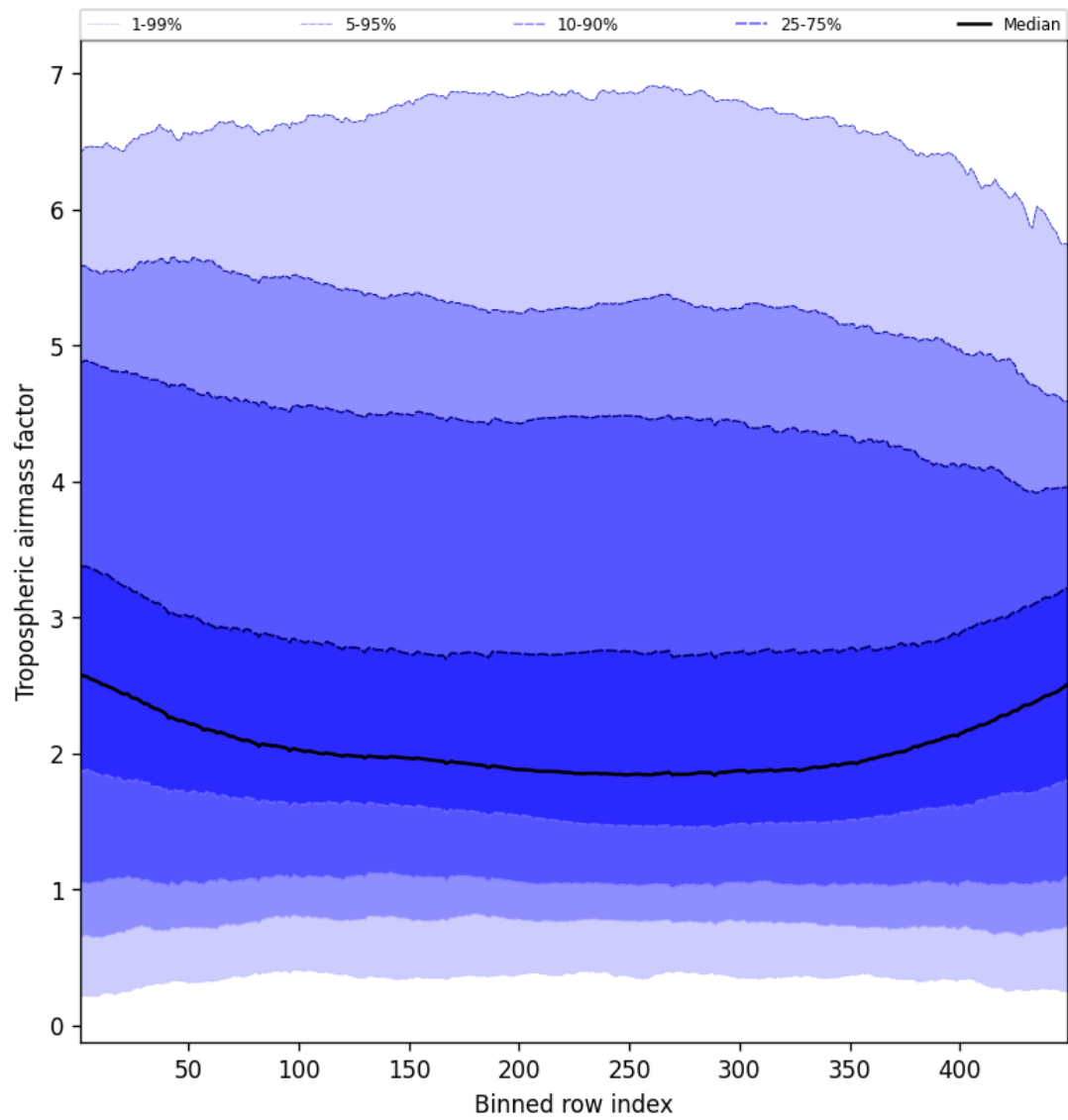
Figure 48: Along track statistics of “Tropospheric air mass factor” for 2025-02-16 to 2025-02-18
