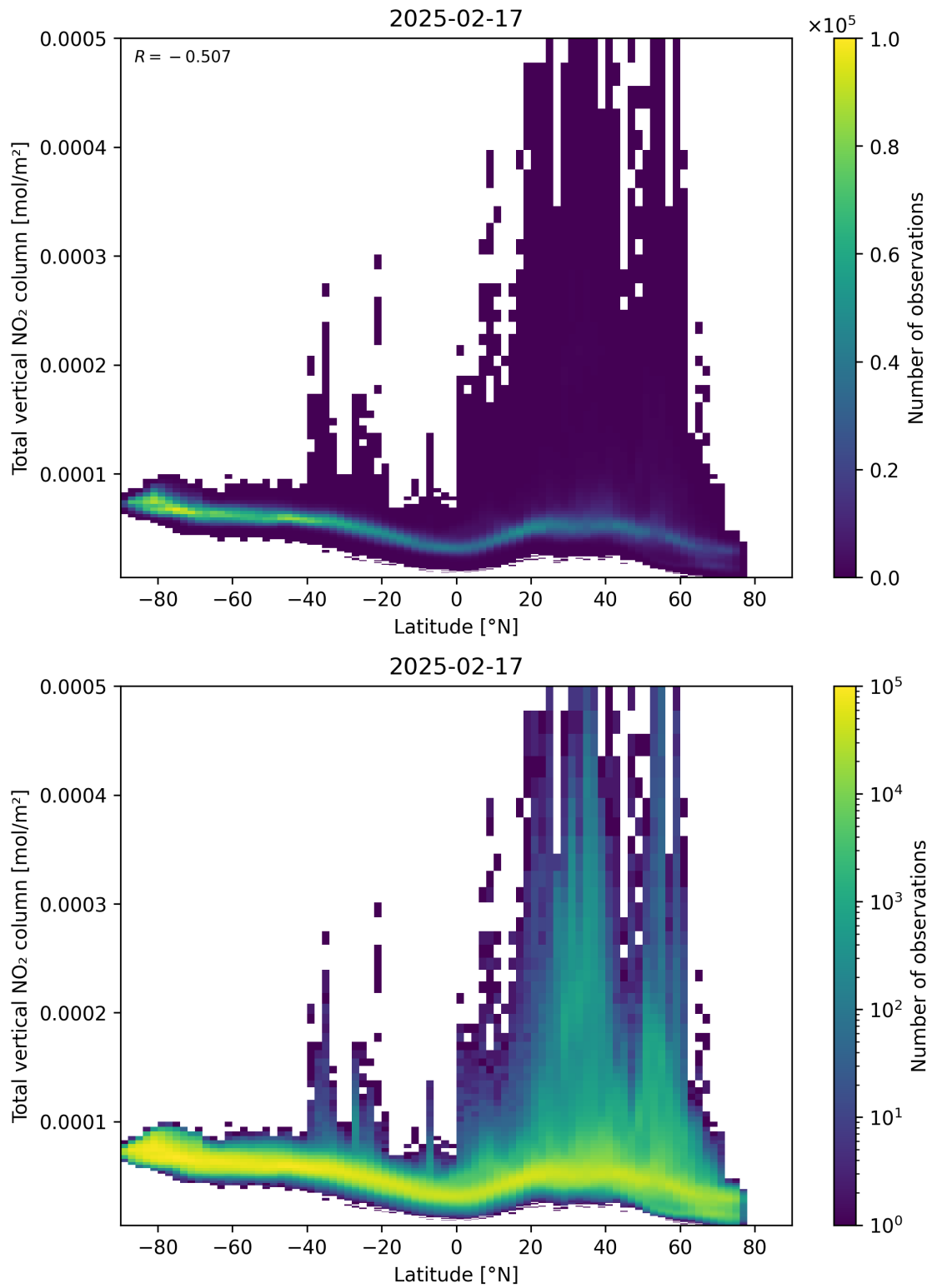
Figure 90: Scatter density plot of “Latitude” against “Total vertical NO 2 column” for 2025-02-16 to 2025-02-18.
