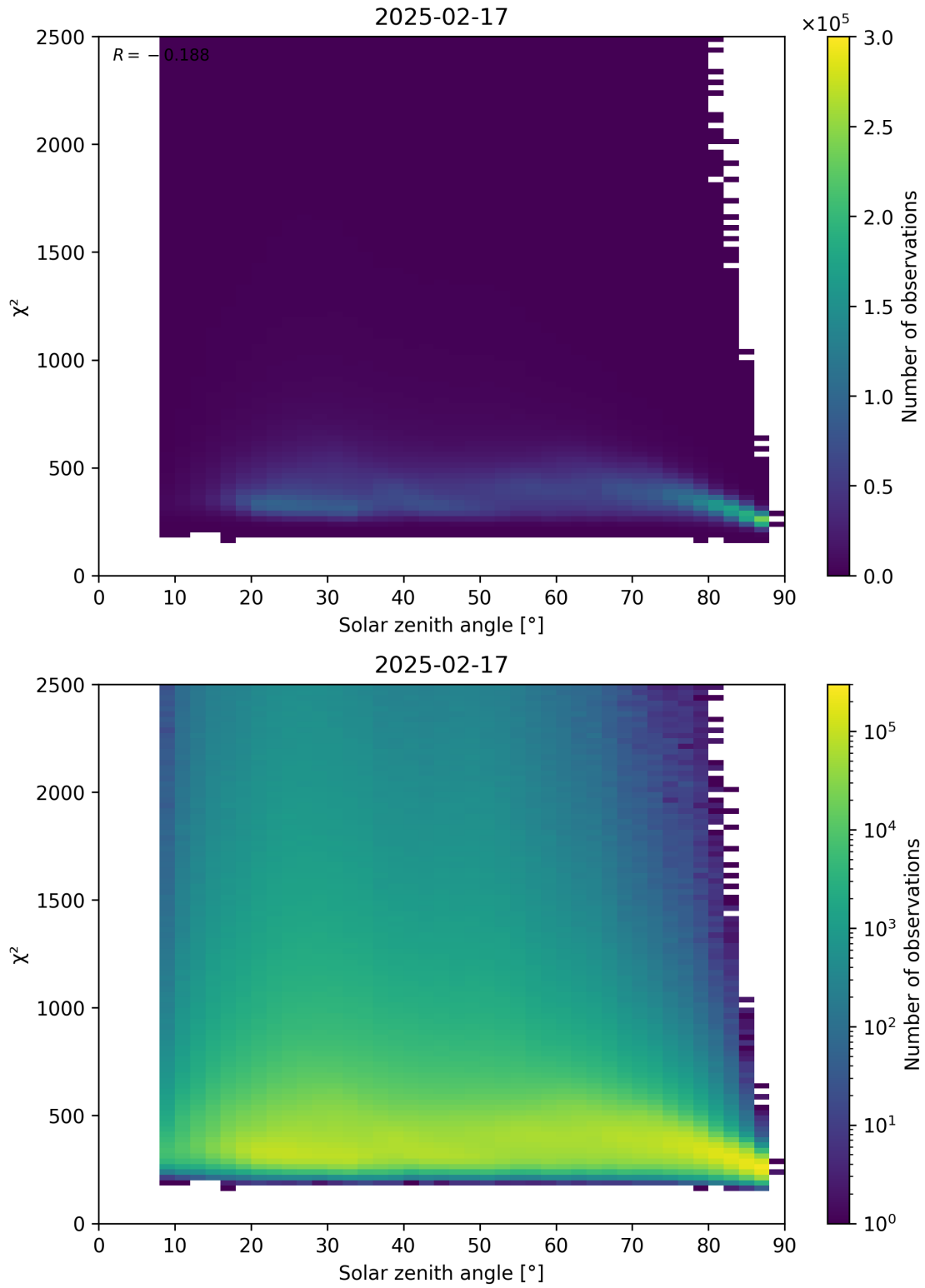
Figure 148: Scatter density plot of “Solar zenith angle” against “ \chi^2 ” for 2025-02-16 to 2025-02-18.
