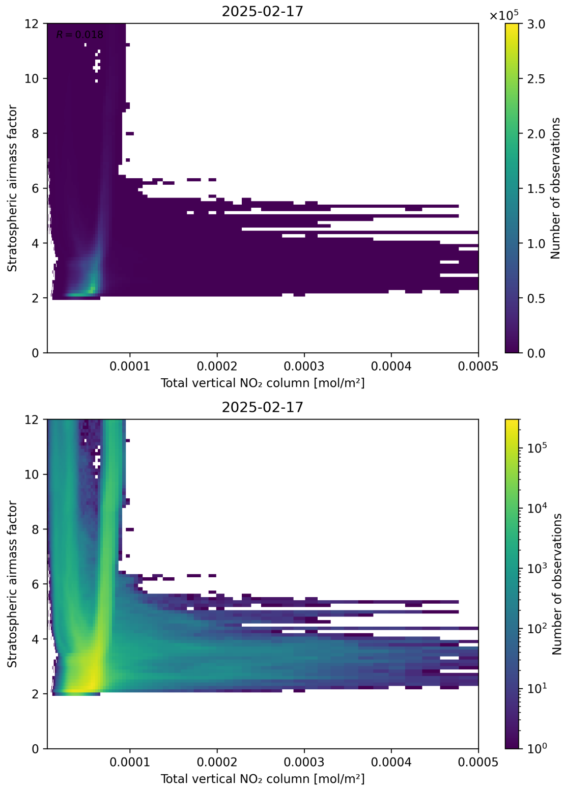
Figure 110: Scatter density plot of “Total vertical NO 2 column” against “Stratospheric airmass factor” for 2025-02-16 to 2025-02-18.
