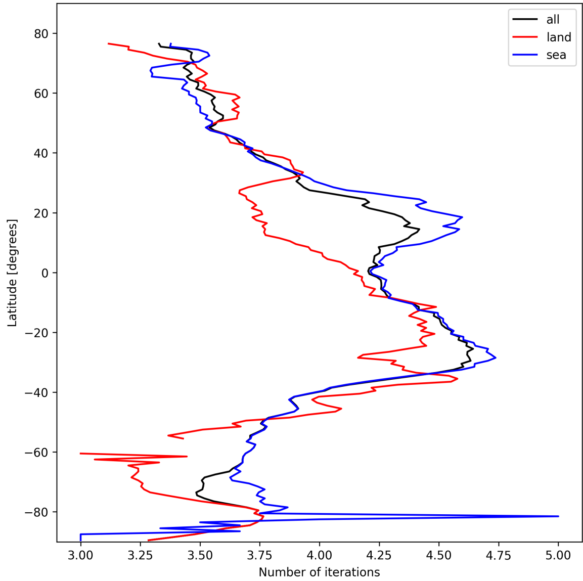
Figure 17: Zonal average of “Number of iterations” for 2025-02-16 to 2025-02-18.
