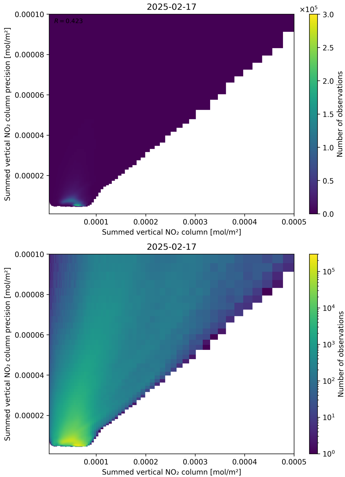
Figure 105: Scatter density plot of “Summed vertical NO 2 column” against “Summed vertical NO 2 column precision” for 2025-02-16 to 2025-02-18.
