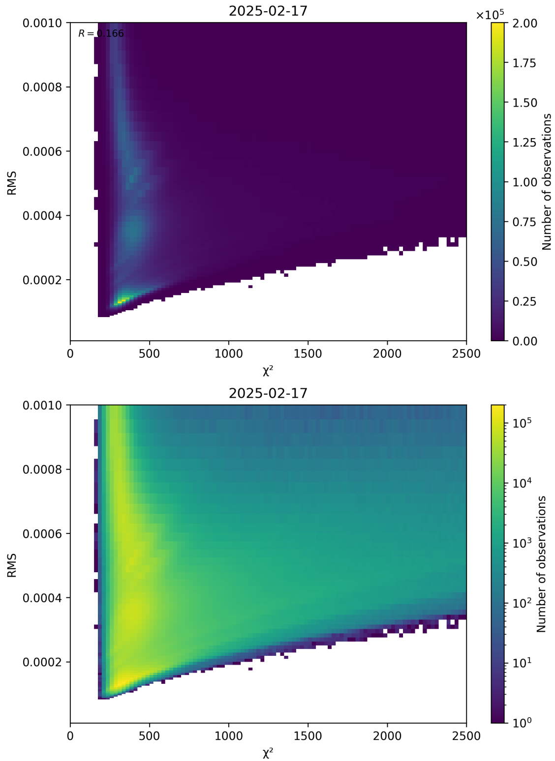
Figure 82: Scatter density plot of “ \chi^2 ” against “RMS” for 2025-02-16 to 2025-02-18.
