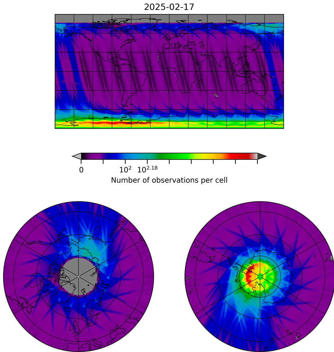
Figure 10: Map of the number of observations for 2025-02-16 to 2025-02-18
