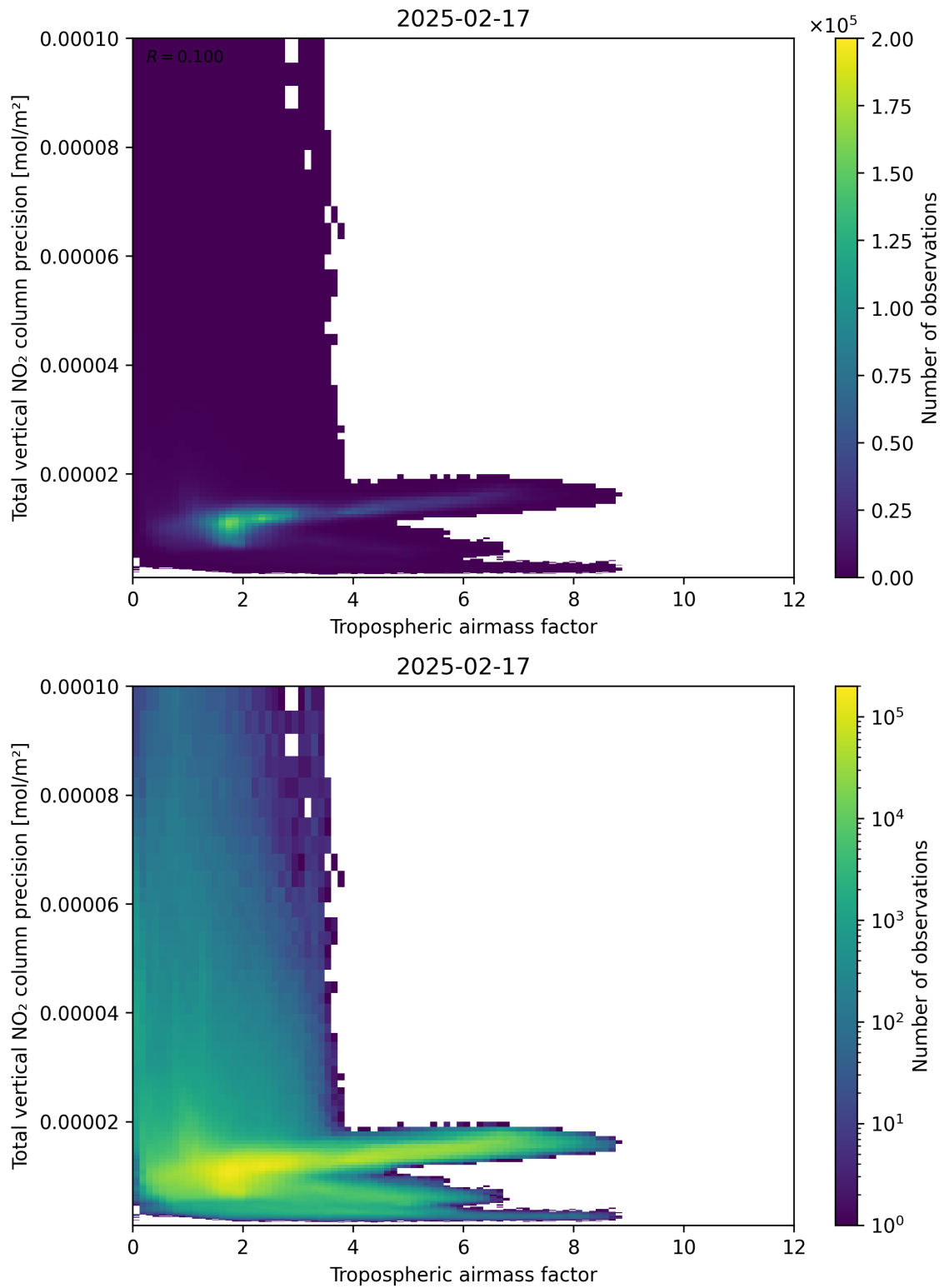
Figure 78: Scatter density plot of “Tropospheric air mass factor” against “Total vertical NO 2 column precision” for 2025-02-16 to 2025-02-18.
