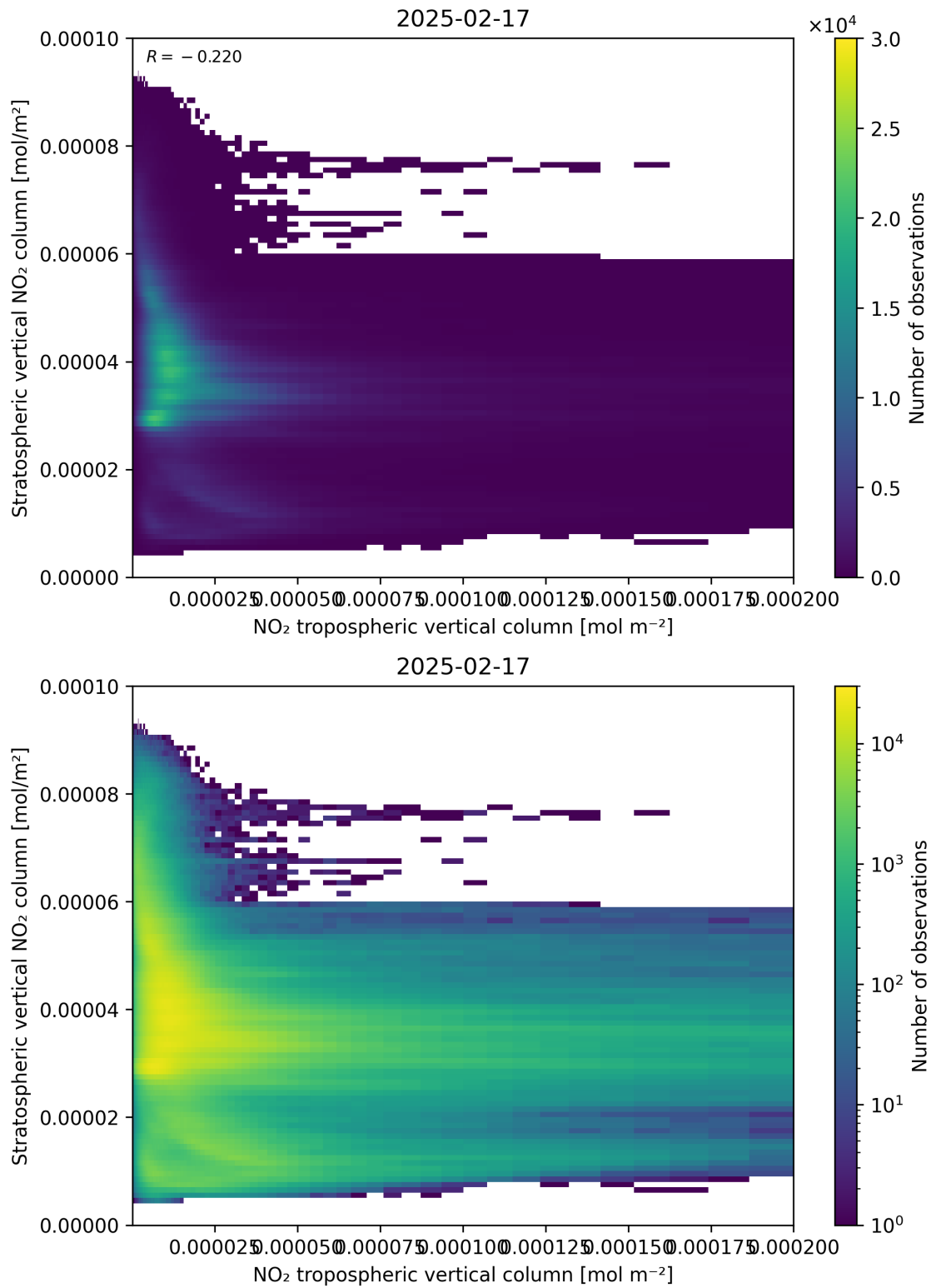
Figure 125: Scatter density plot of “NO 2 tropospheric vertical column” against “Stratospheric vertical NO 2 column” for 2025-02-16 to 2025-02-18.
