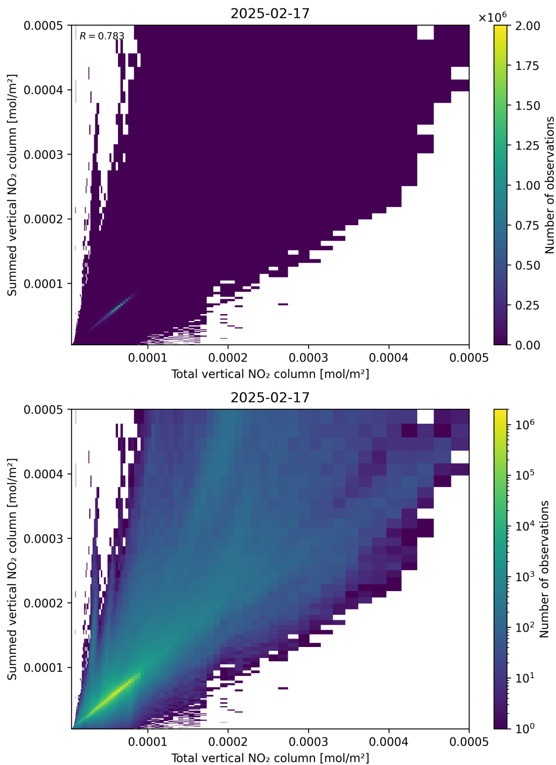
Figure 112: Scatter density plot of “Total vertical NO 2 column” against “Summed vertical NO 2 column” for 2025-02-16 to 2025-02-18.
