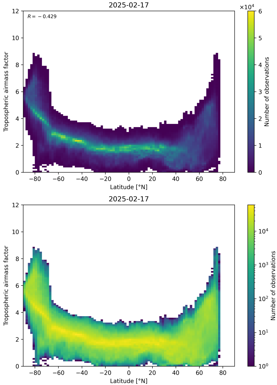
Figure 85: Scatter density plot of “Latitude” against “Tropospheric airmass factor” for 2025-02-16 to 2025-02-18.
