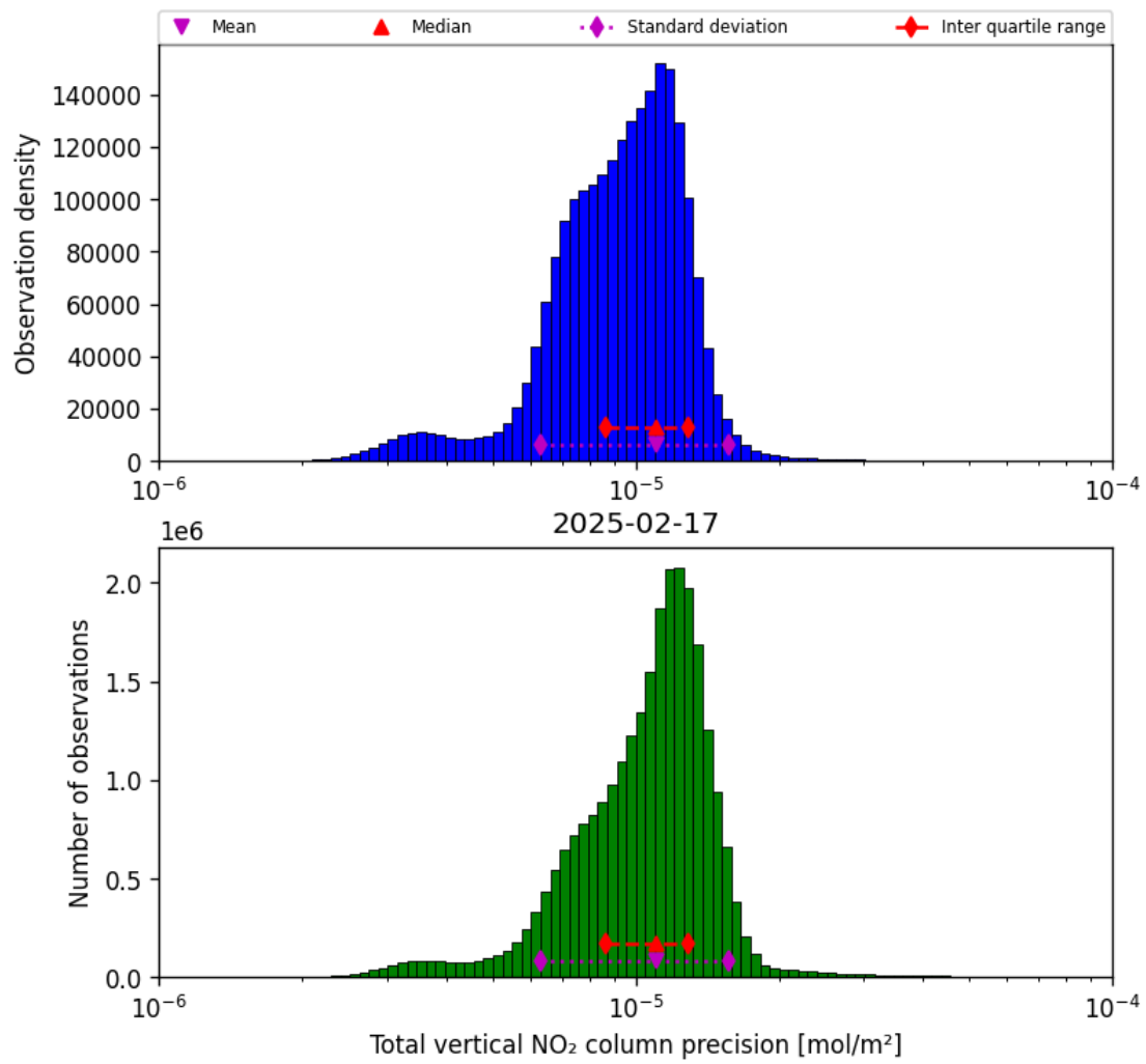
Figure 39: Histogram of “Total vertical NO 2 column precision” for 2025-02-16 to 2025-02-18
