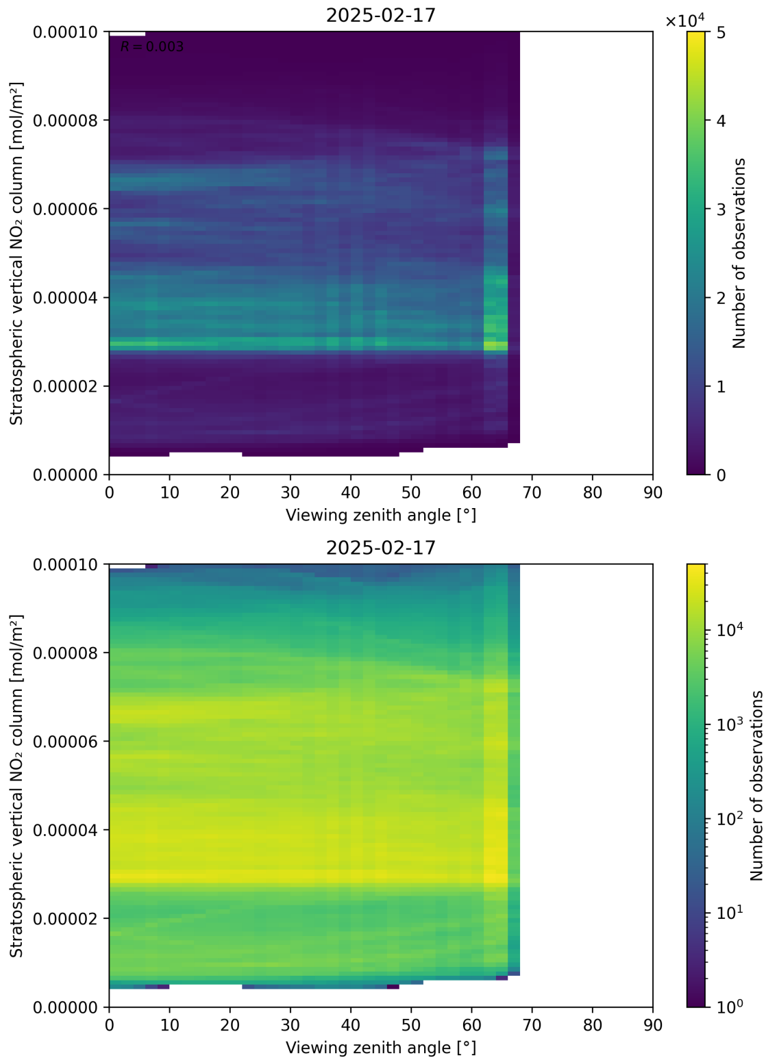
Figure 164: Scatter density plot of “Viewing zenith angle” against “Stratospheric vertical NO 2 column” for 2025-02-16 to 2025-02-18.
