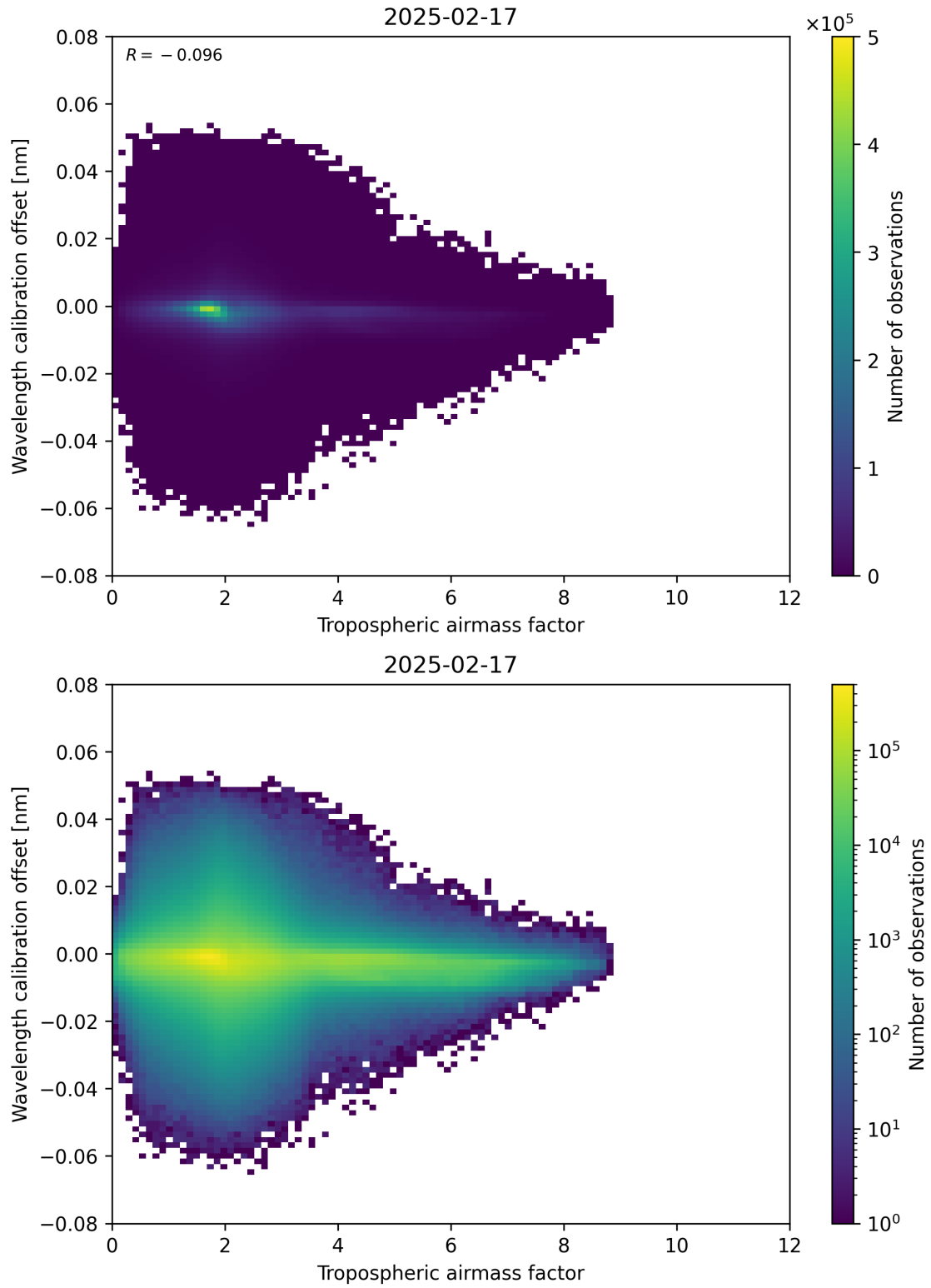
Figure 80: Scatter density plot of “Tropospheric air mass factor” against “Wavelength calibration offset” for 2025-02-16 to 2025-02-18.
