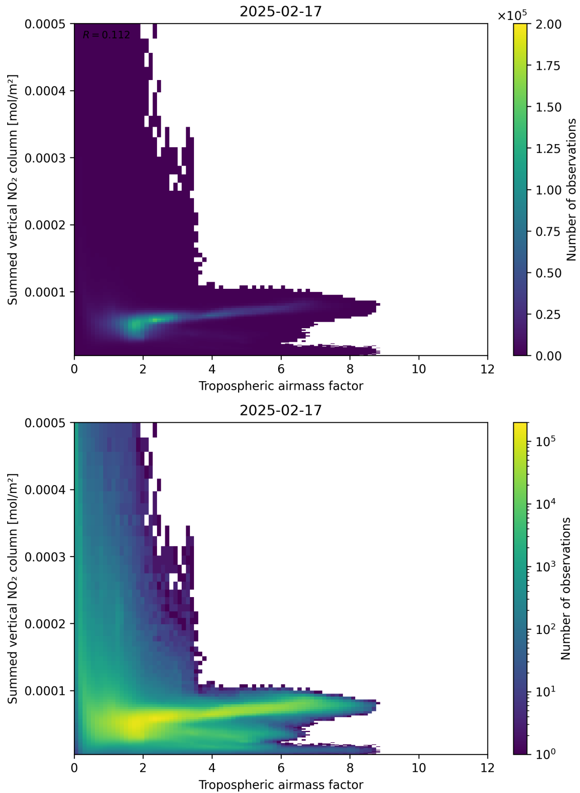
Figure 75: Scatter density plot of “Tropospheric air mass factor” against “Summed vertical NO 2 column” for 2025-02-16 to 2025-02-18.
