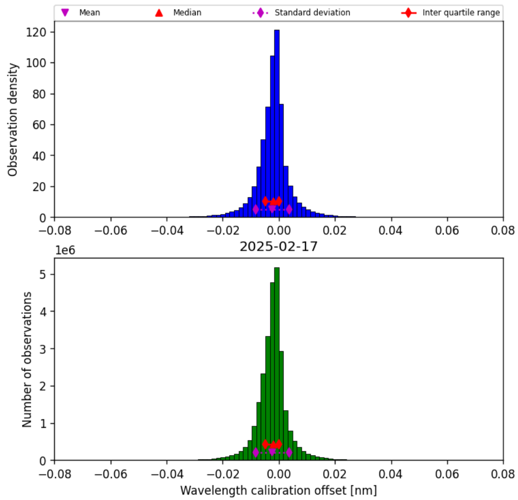
Figure 35: Histogram of “Wavelength calibration offset” for 2025-02-16 to 2025-02-18
