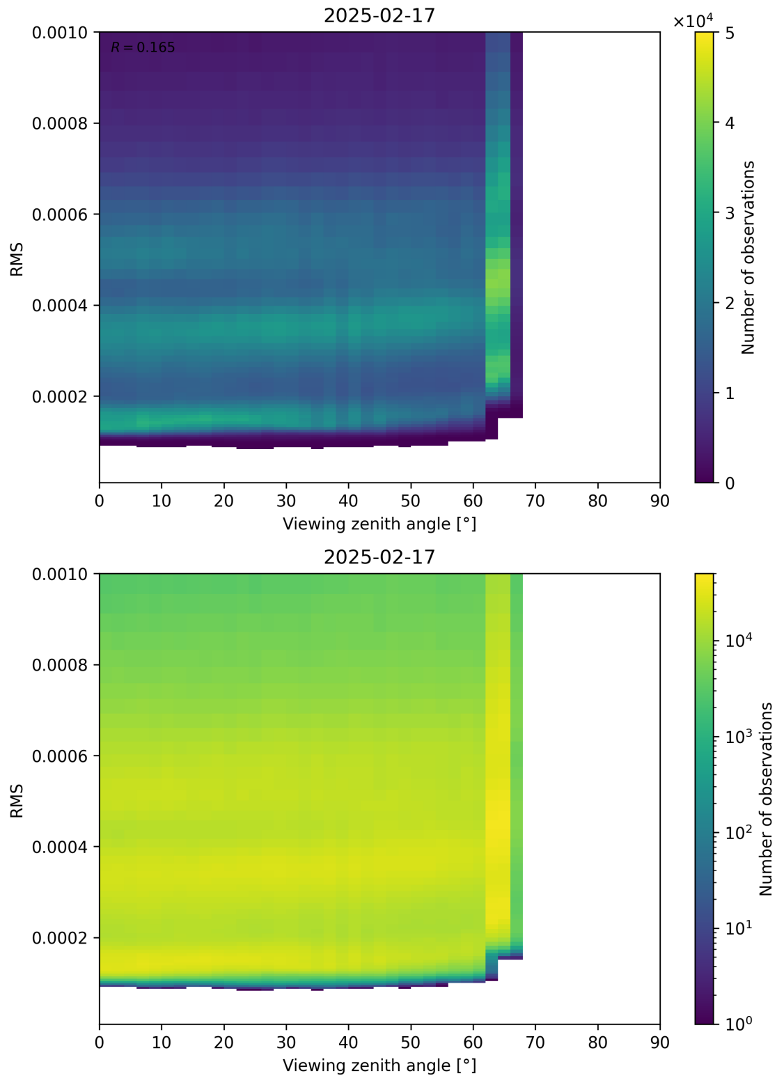
Figure 171: Scatter density plot of “Viewing zenith angle” against “RMS” for 2025-02-16 to 2025-02-18.
