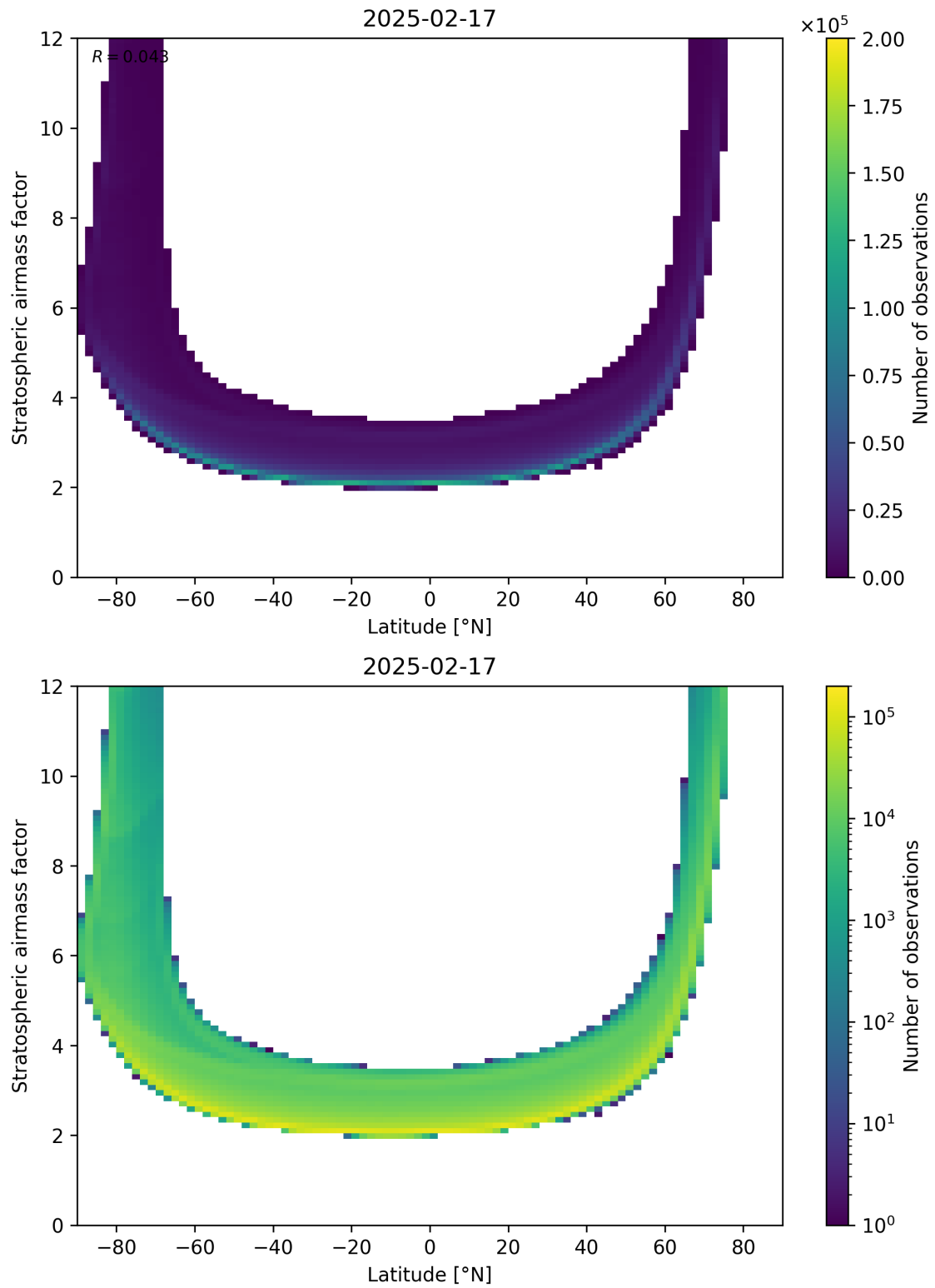
Figure 83: Scatter density plot of “Latitude” against “Stratospheric air mass factor” for 2025-02-16 to 2025-02-18.
