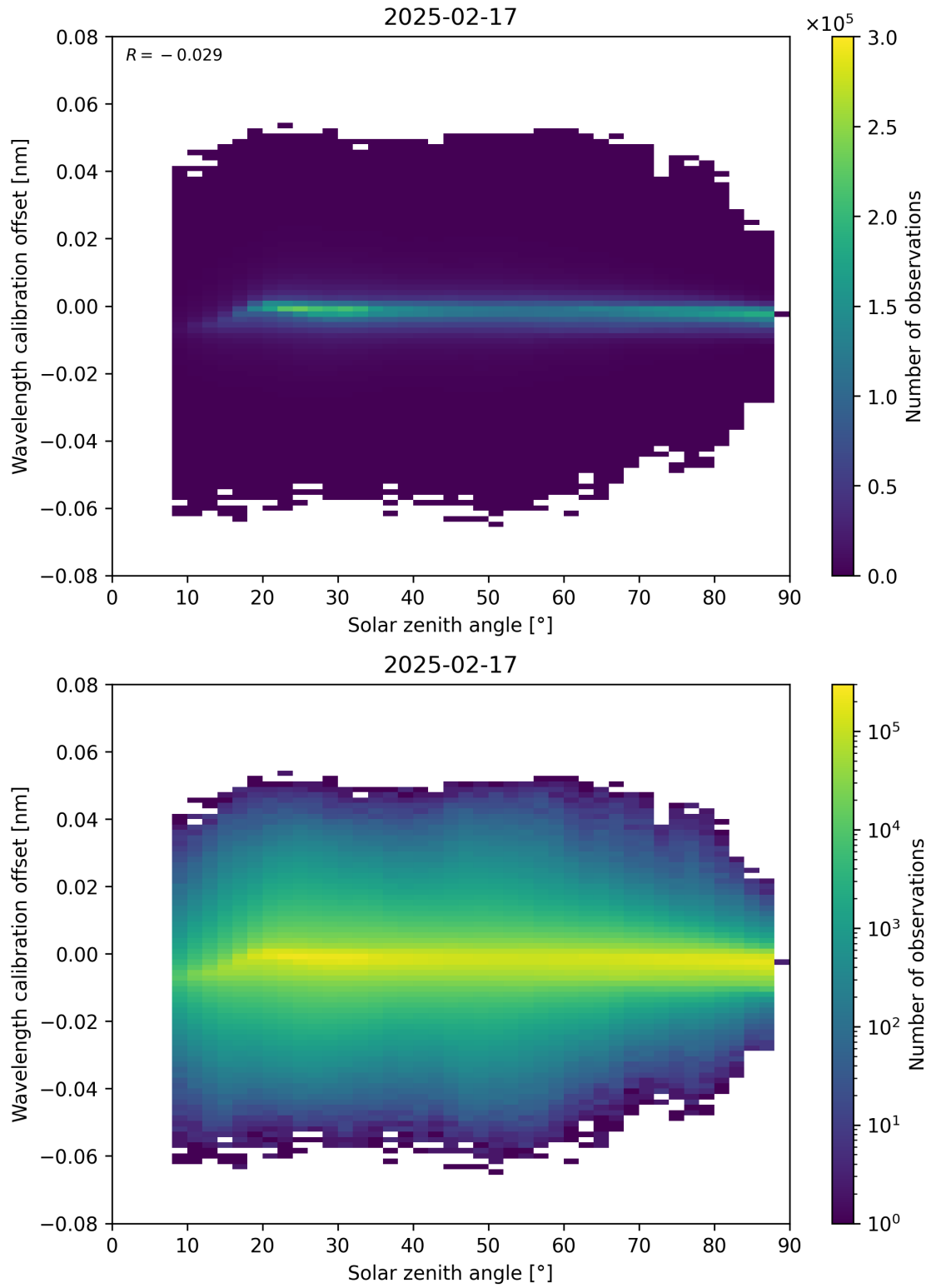
Figure 158: Scatter density plot of “Solar zenith angle” against “Wavelength calibration offset” for 2025-02-16 to 2025-02-18.
