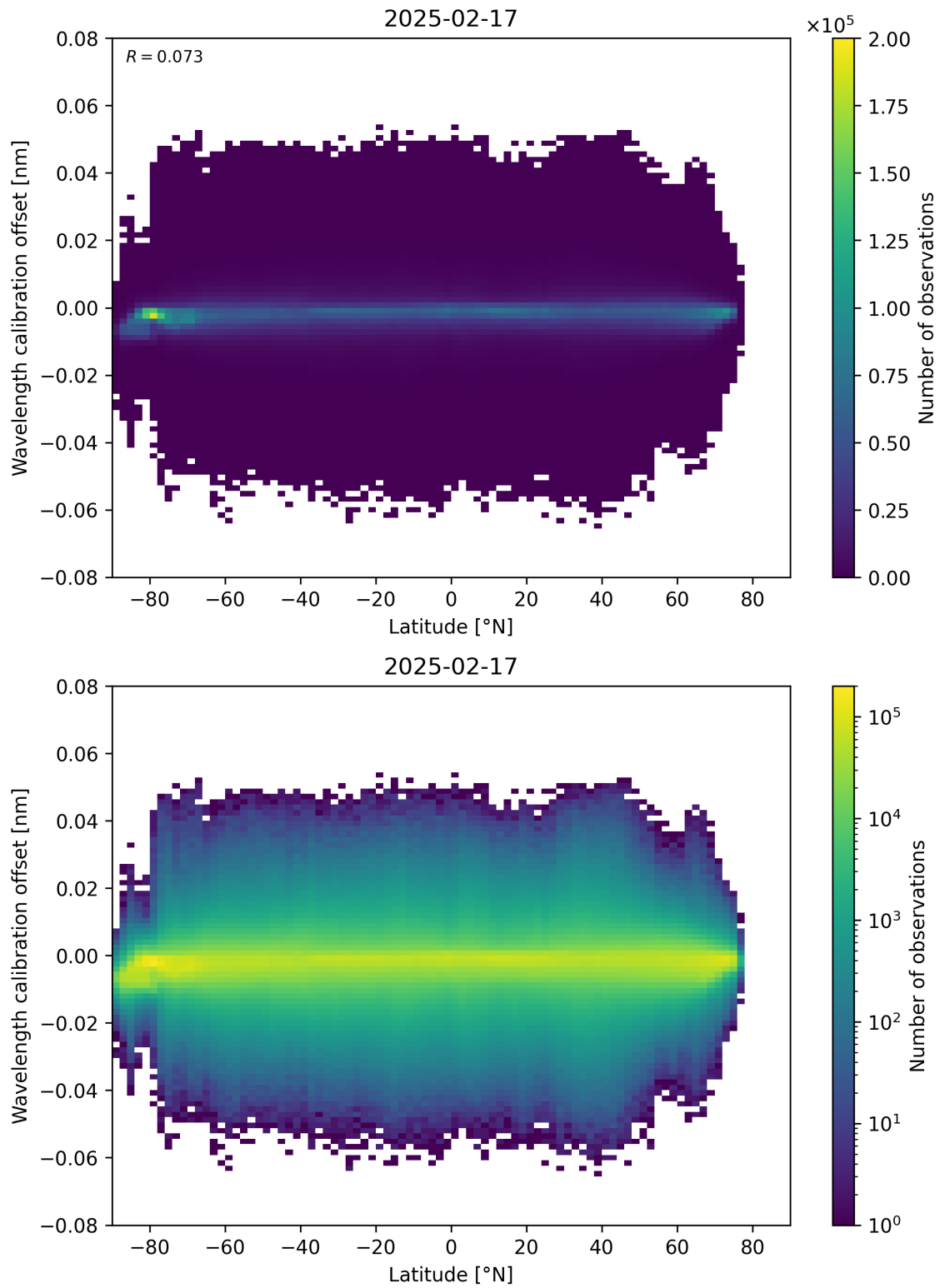
Figure 95: Scatter density plot of “Latitude” against “Wavelength calibration offset” for 2025-02-16 to 2025-02-18.
