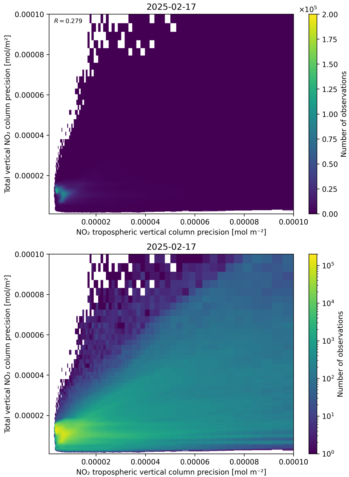
Figure 139: Scatter density plot of “NO 2 tropospheric vertical column precision” against “Total vertical NO 2 column precision” for 2025-02-16 to 2025-02-18.
