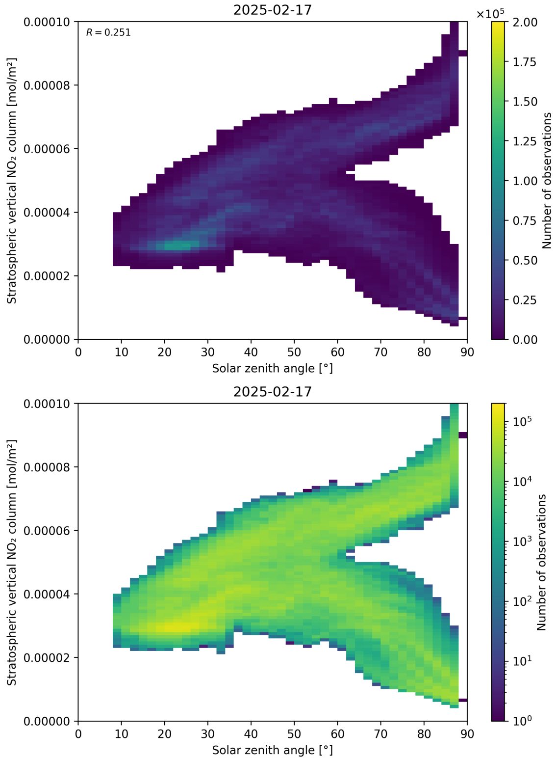
Figure 150: Scatter density plot of “Solar zenith angle” against “Stratospheric vertical NO 2 column” for 2025-02-16 to 2025-02-18.
