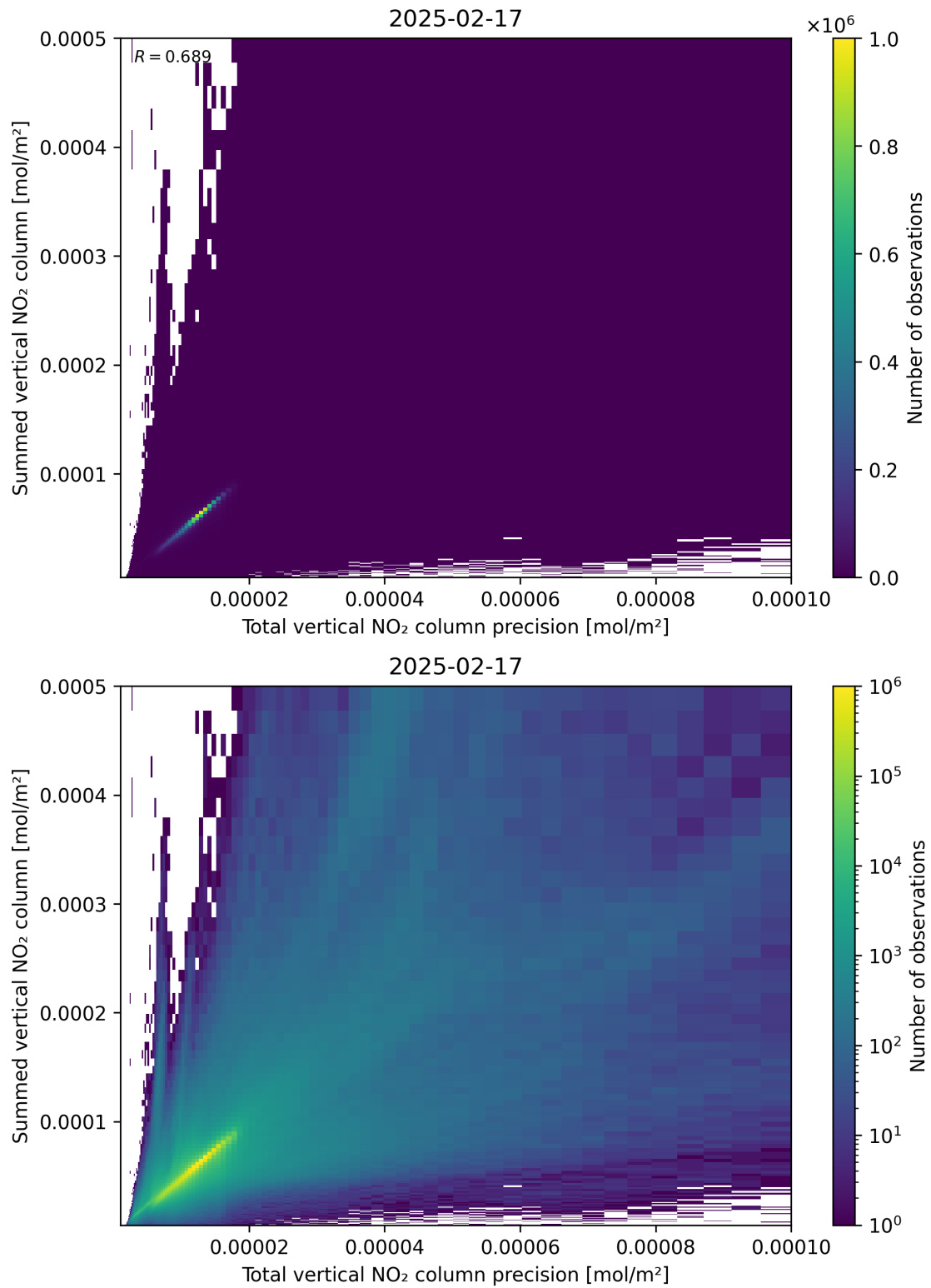
Figure 117: Scatter density plot of “Total vertical NO 2 column precision” against “Summed vertical NO 2 column” for 2025-02-16 to 2025-02-18.
