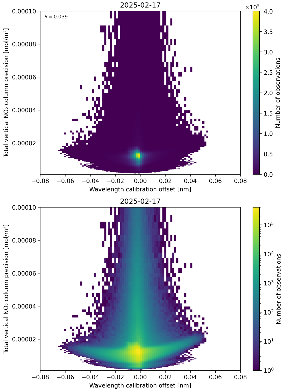
Figure 180: Scatter density plot of “Wavelength calibration offset” against “Total vertical NO 2 column precision” for 2025-02-16 to 2025-02-18.
