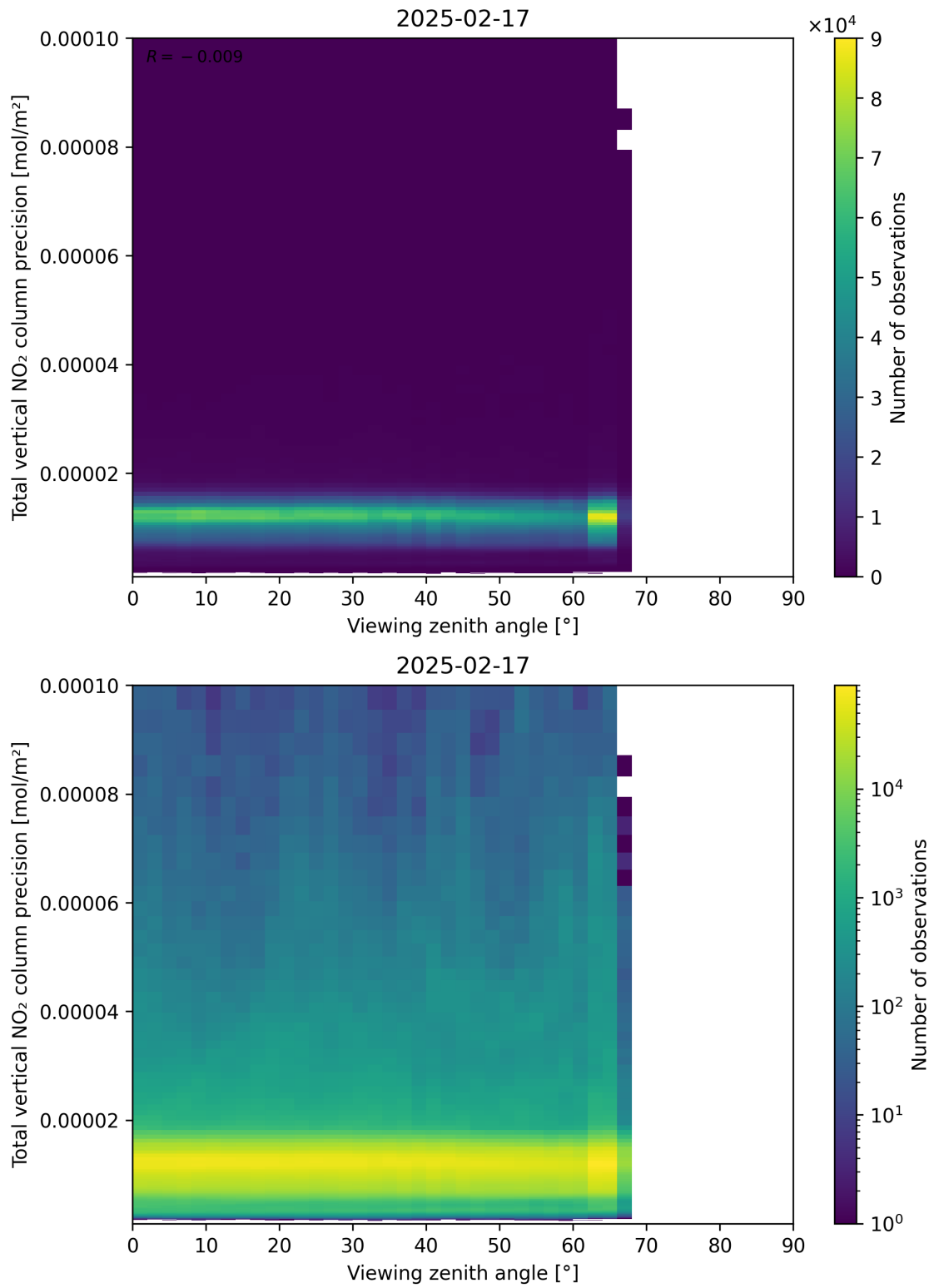
Figure 168: Scatter density plot of “Viewing zenith angle” against “Total vertical NO 2 column precision” for 2025-02-16 to 2025-02-18.
