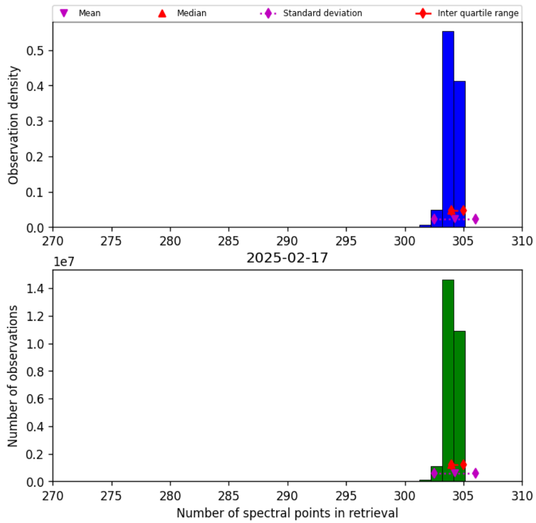
Figure 33: Histogram of “Number of spectral points in retrieval” for 2025-02-16 to 2025-02-18
