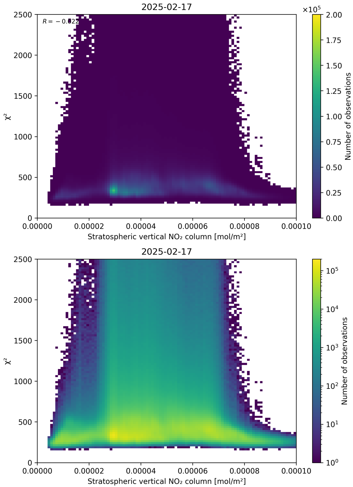
Figure 97: Scatter density plot of “Stratospheric vertical NO 2 column” against “ \chi^2 ” for 2025-02-16 to 2025-02-18.
