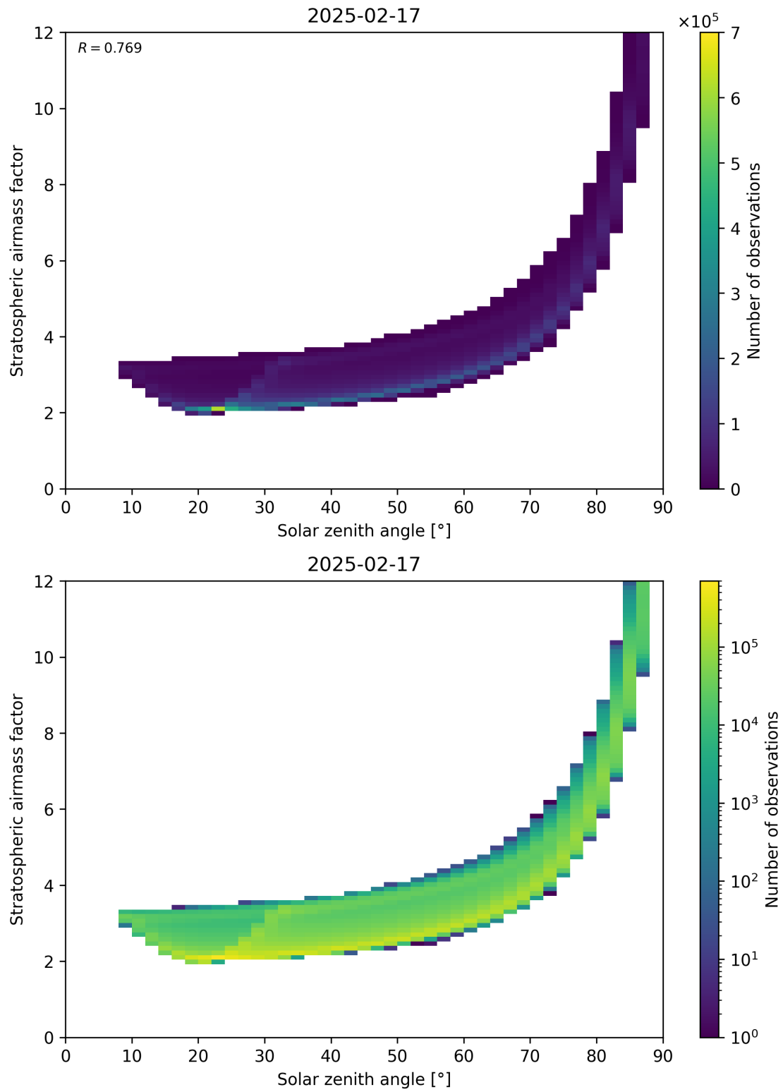
Figure 145: Scatter density plot of “Solar zenith angle” against “Stratospheric airmass factor” for 2025-02-16 to 2025-02-18.
