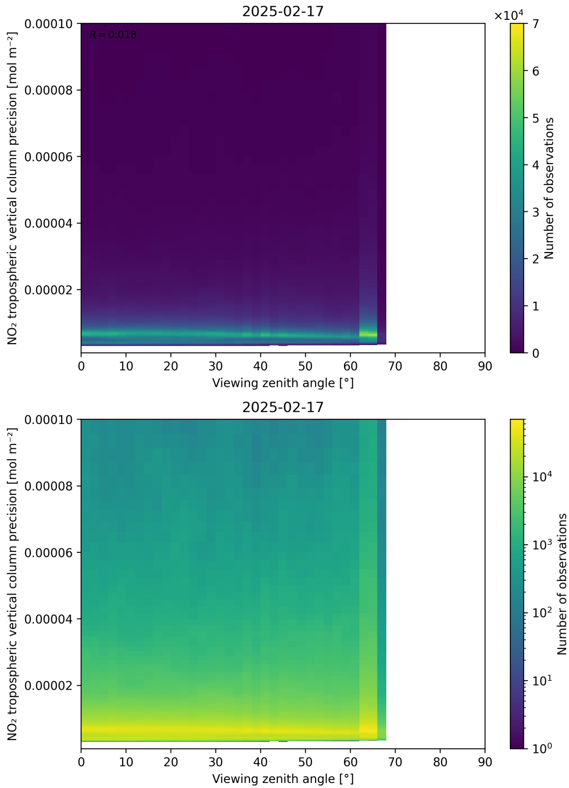
Figure 170: Scatter density plot of “Viewing zenith angle” against “NO 2 tropospheric vertical column precision” for 2025-02-16 to 2025-02-18.
