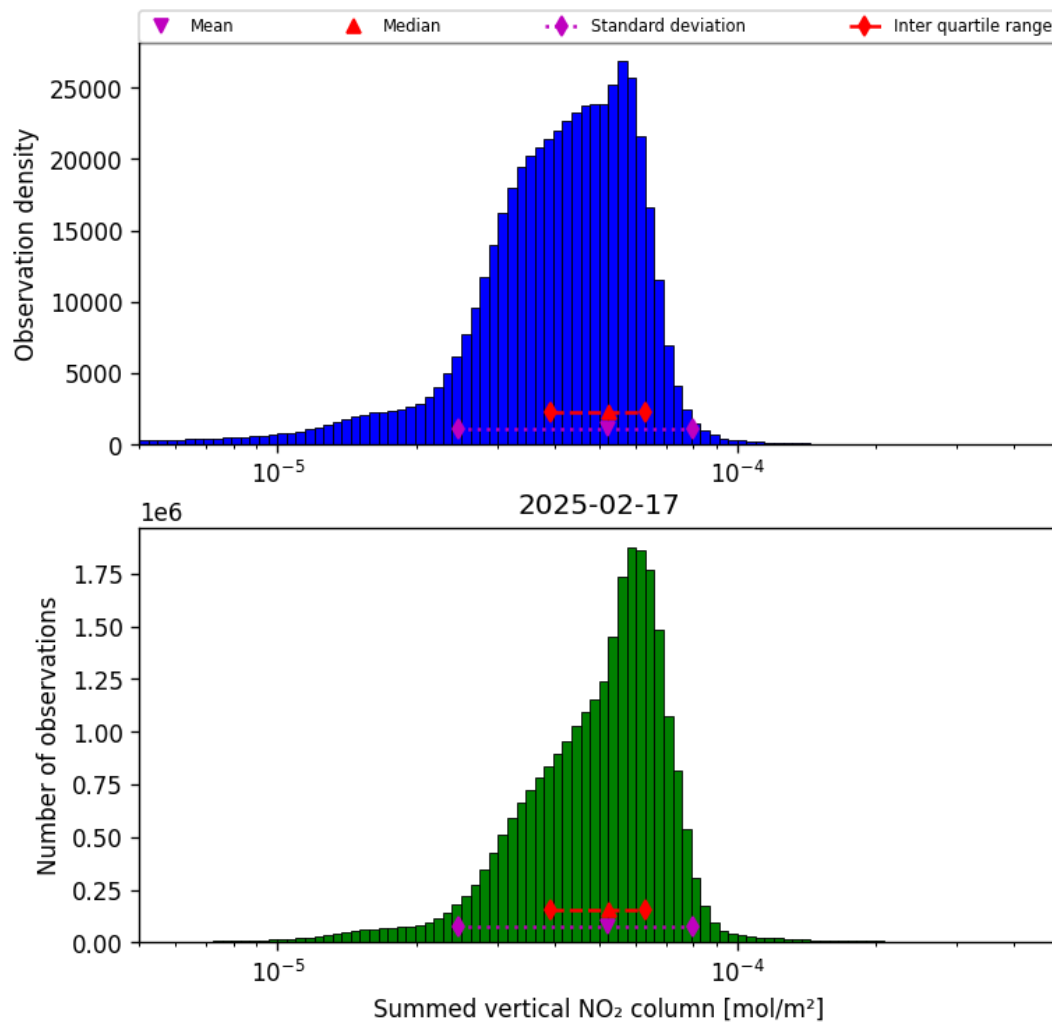
Figure 40: Histogram of “Summed vertical NO 2 column” for 2025-02-16 to 2025-02-18
