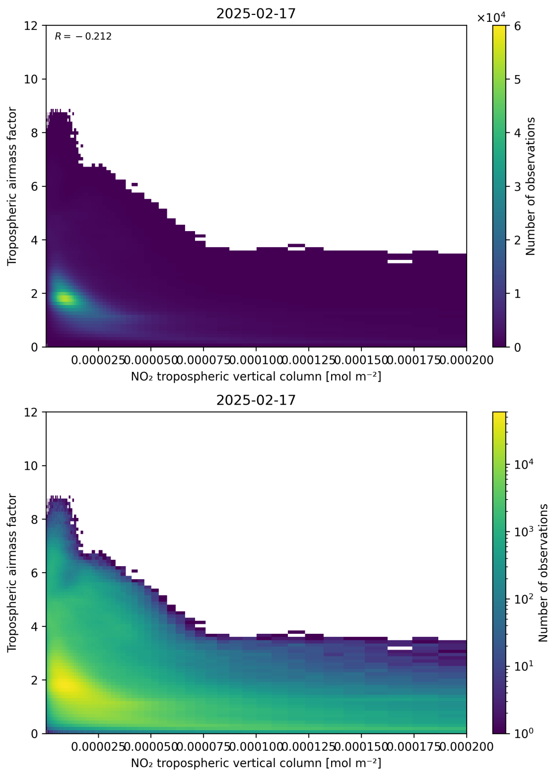
Figure 123: Scatter density plot of “NO 2 tropospheric vertical column” against “Tropospheric air mass factor” for 2025-02-16 to 2025-02-18.
