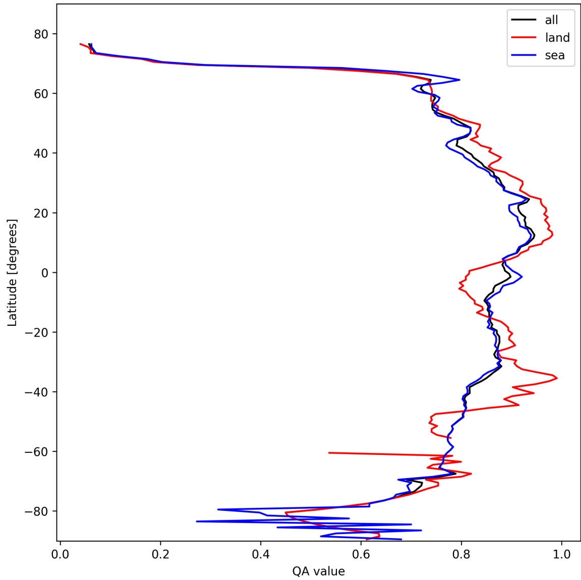
Figure 11: Zonal average of “QA value” for 2025-02-16 to 2025-02-18.
