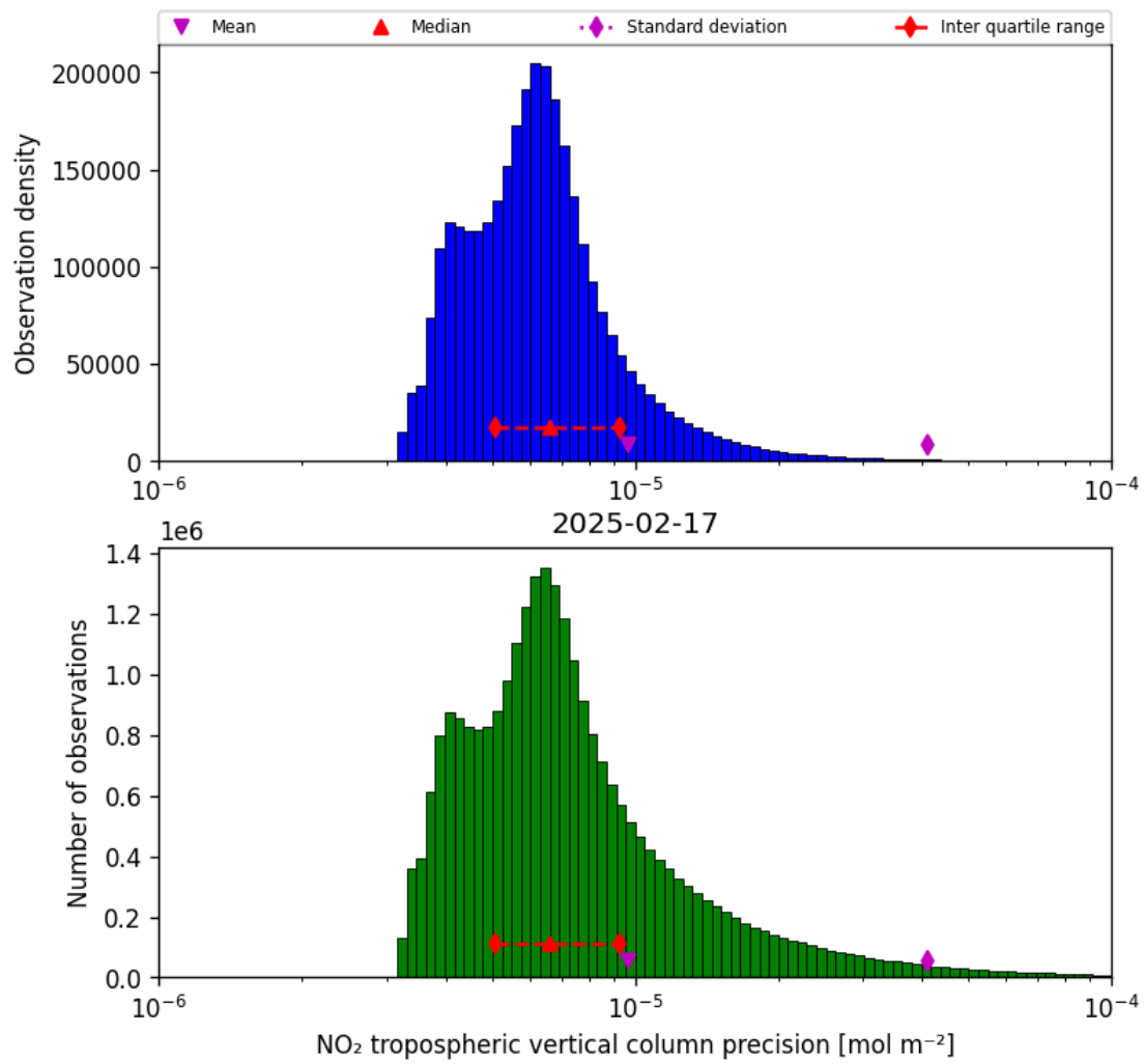
Figure 30: Histogram of "NO 2 tropospheric vertical column precision" for 2025-02-16 to 2025-02-18
