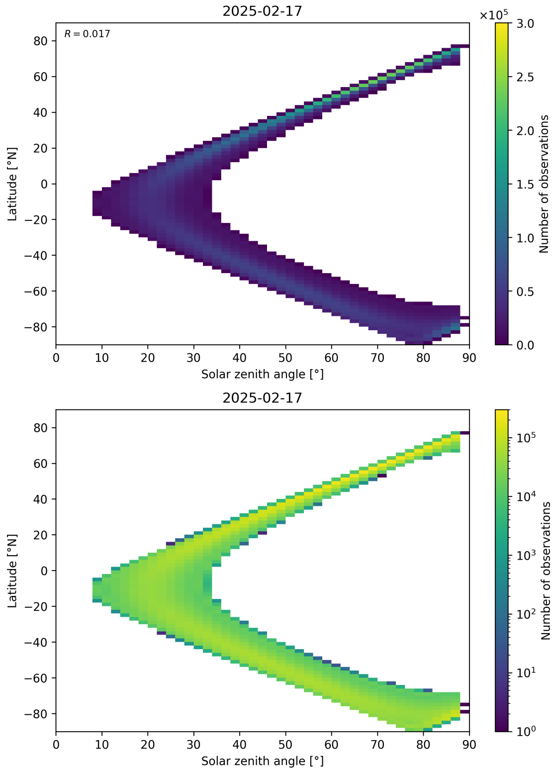
Figure 149: Scatter density plot of “Solar zenith angle” against “Latitude” for 2025-02-16 to 2025-02-18.
