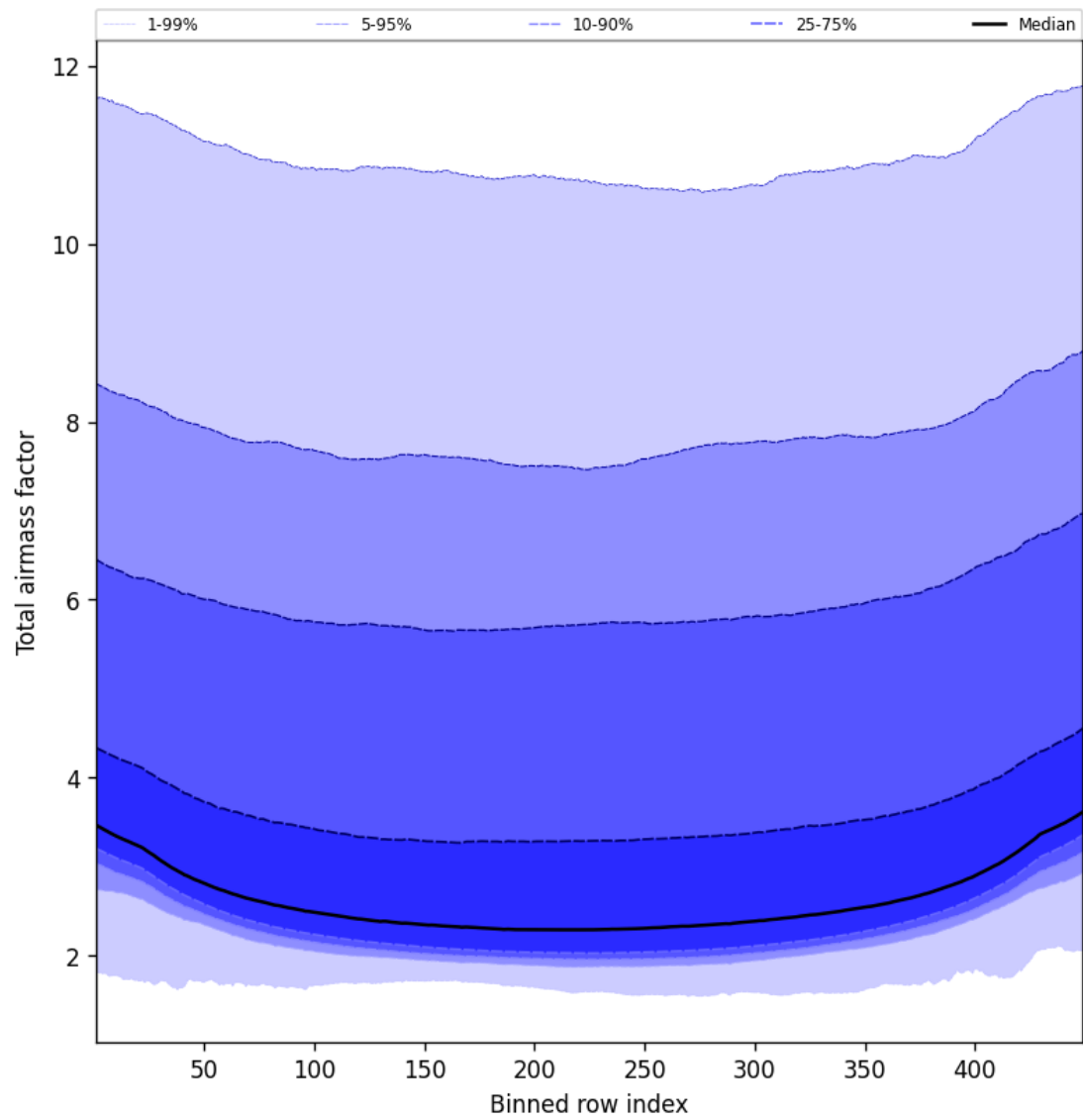
Figure 49: Along track statistics of “Total airmass factor” for 2025-02-16 to 2025-02-18
