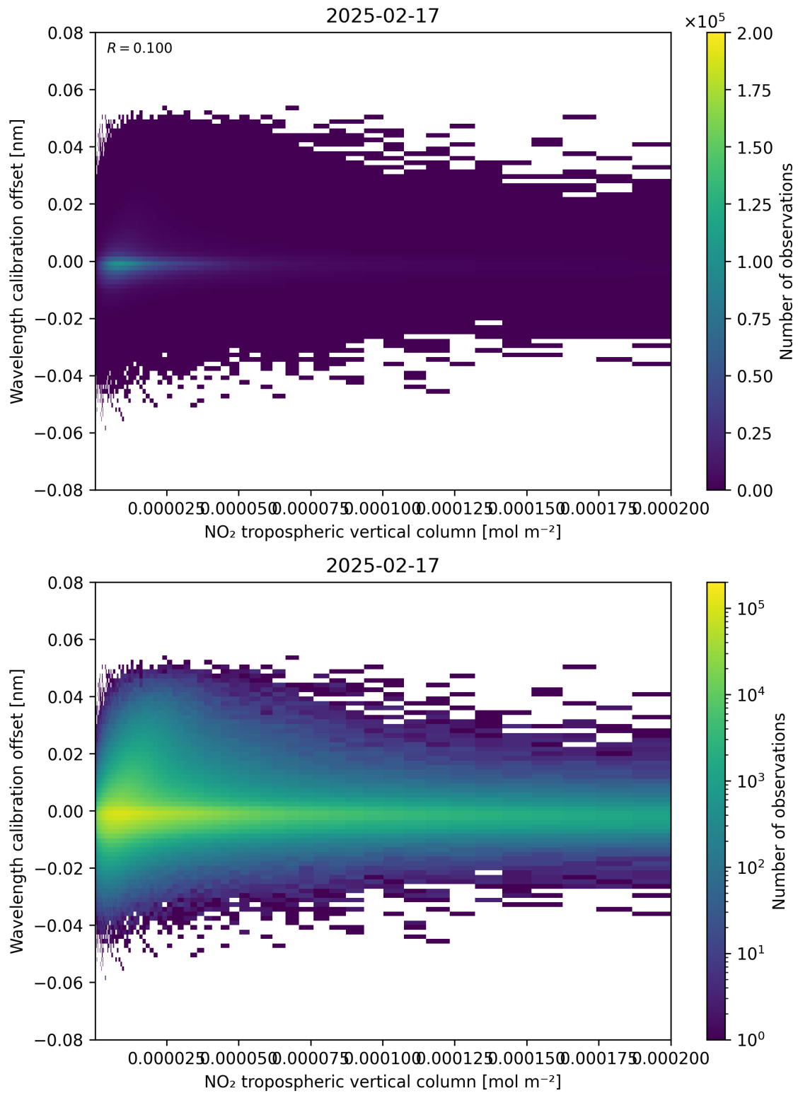
Figure 143: Scatter density plot of “NO 2 tropospheric vertical column” against “Wavelength calibration offset” for 2025-02-16 to 2025-02-18.
