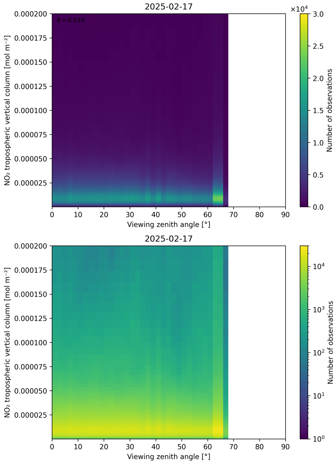
Figure 169: Scatter density plot of “Viewing zenith angle” against “NO 2 tropospheric vertical column” for 2025-02-16 to 2025-02-18.
