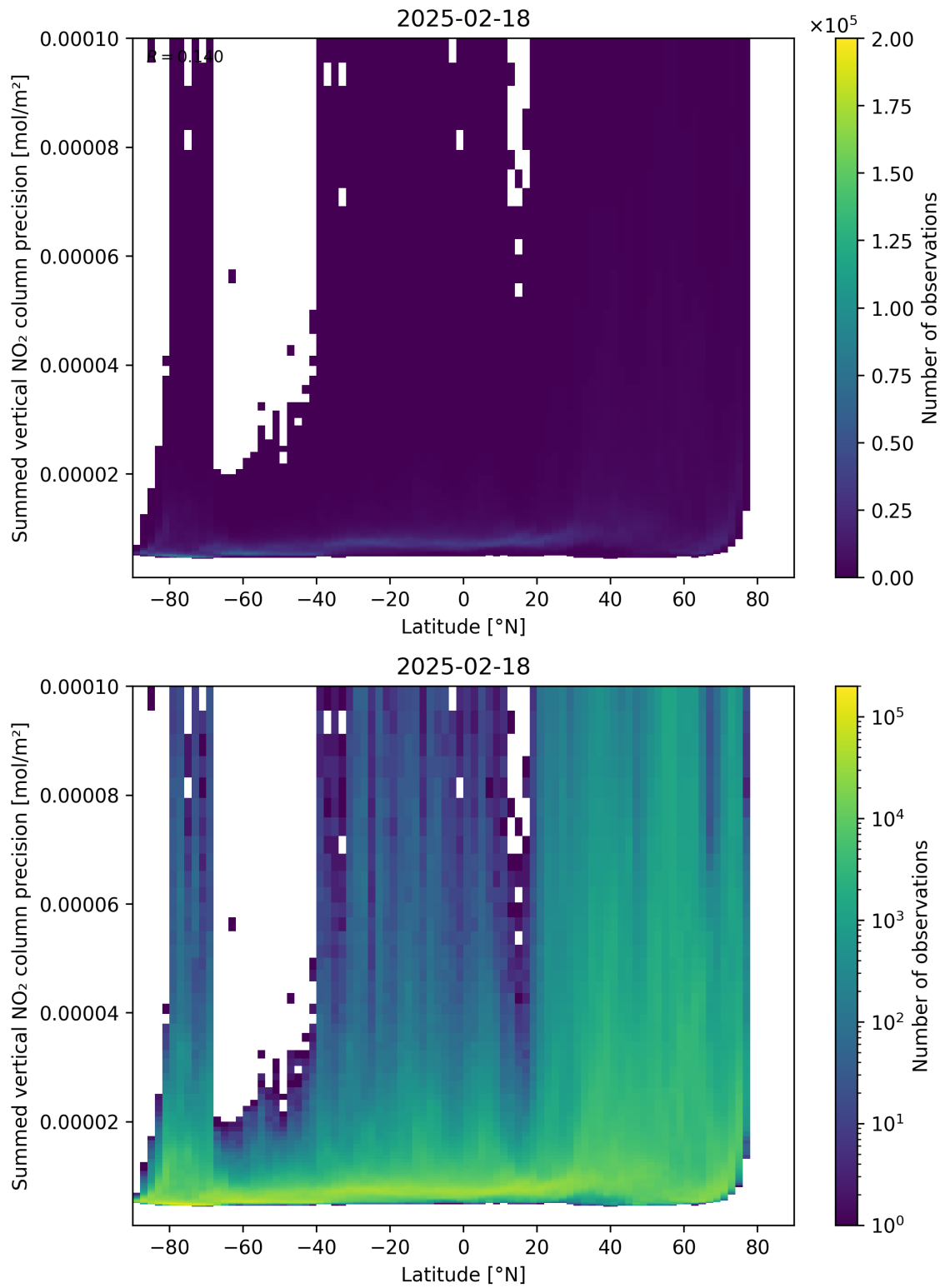
Figure 89: Scatter density plot of “Latitude” against “Summed vertical NO 2 column precision” for 2025-02-18 to 2025-02-19.
