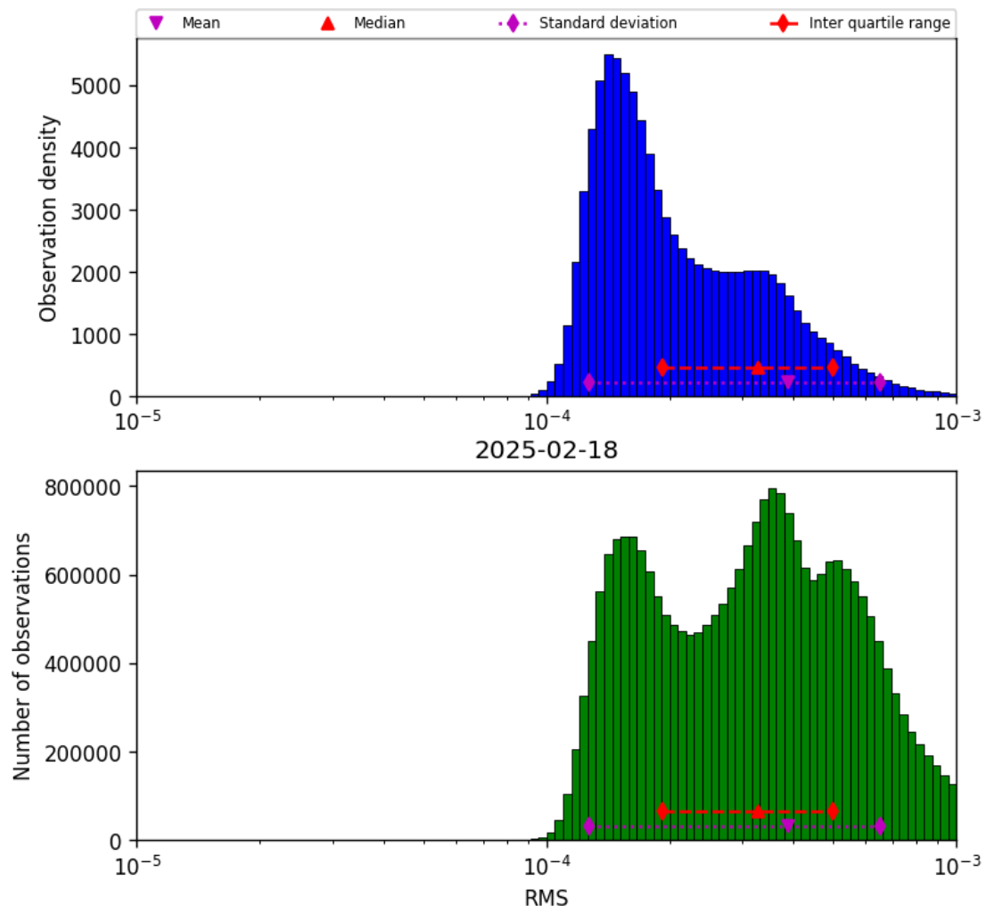
Figure 43: Histogram of “RMS” for 2025-02-18 to 2025-02-19
