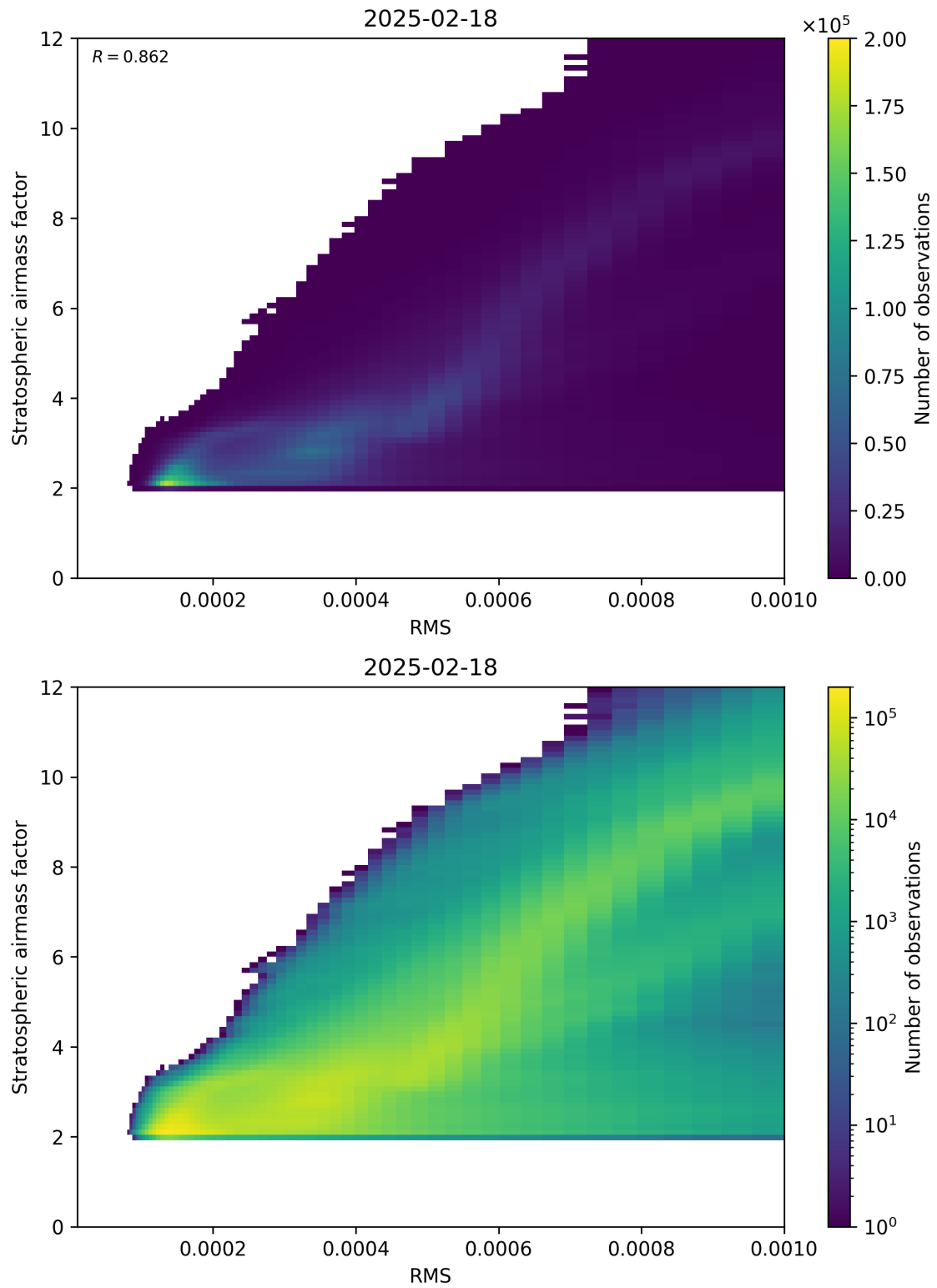
Figure 144: Scatter density plot of “RMS” against “Stratospheric airmass factor” for 2025-02-18 to 2025-02-19.
