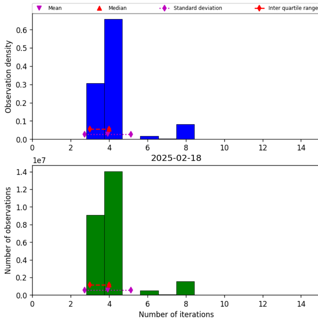
Figure 34: Histogram of “Number of iterations” for 2025-02-18 to 2025-02-19
