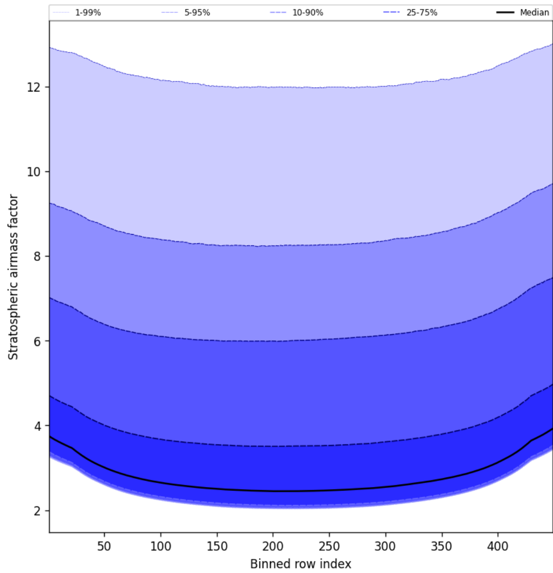
Figure 61: Along track statistics of “Stratospheric airmass factor” for 2025-02-18 to 2025-02-19
