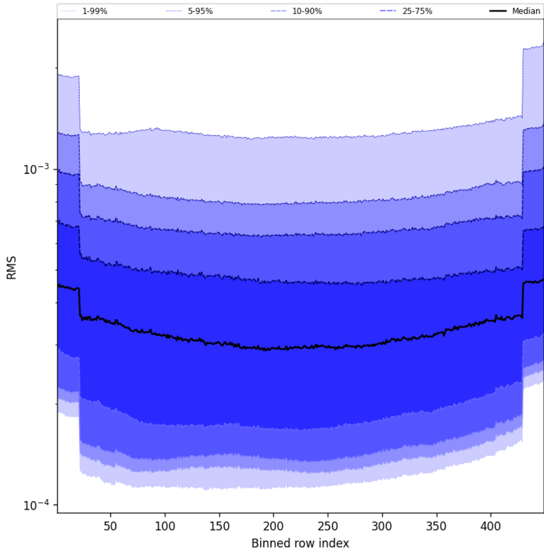
Figure 60: Along track statistics of “RMS” for 2025-02-18 to 2025-02-19
