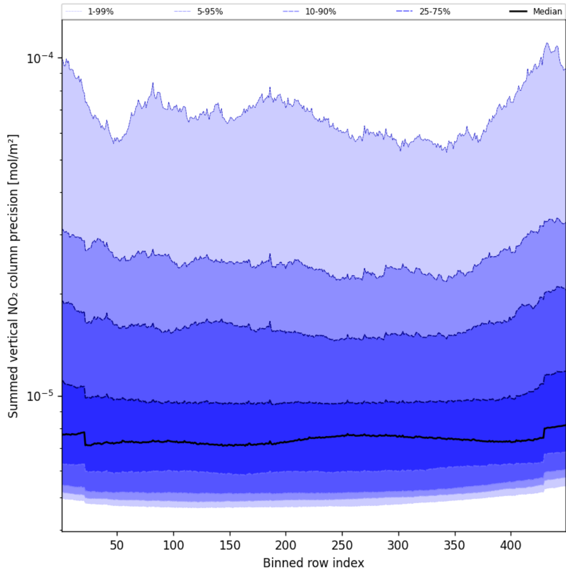
Figure 58: Along track statistics of “Summed vertical NO 2 column precision” for 2025-02-18 to 2025-02-19
