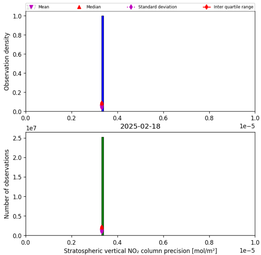
Figure 37: Histogram of “Stratospheric vertical NO 2 column precision” for 2025-02-18 to 2025-02-19
