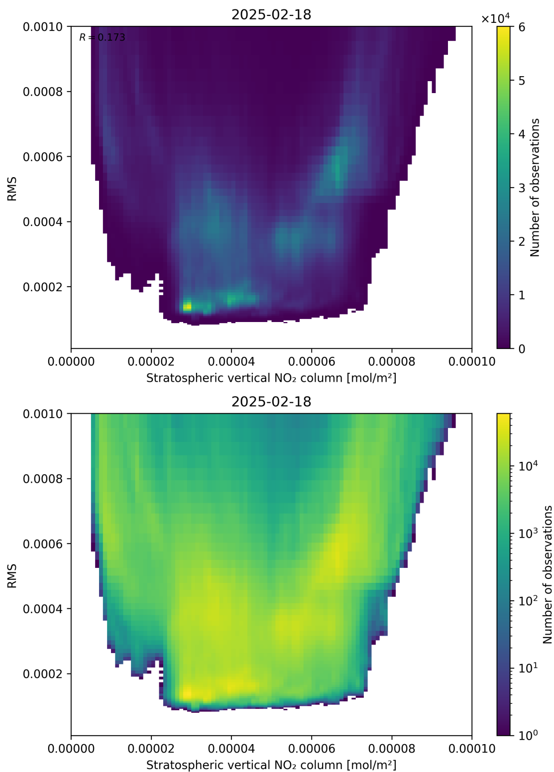
Figure 102: Scatter density plot of “Stratospheric vertical NO 2 column” against “RMS” for 2025-02-18 to 2025-02-19.
