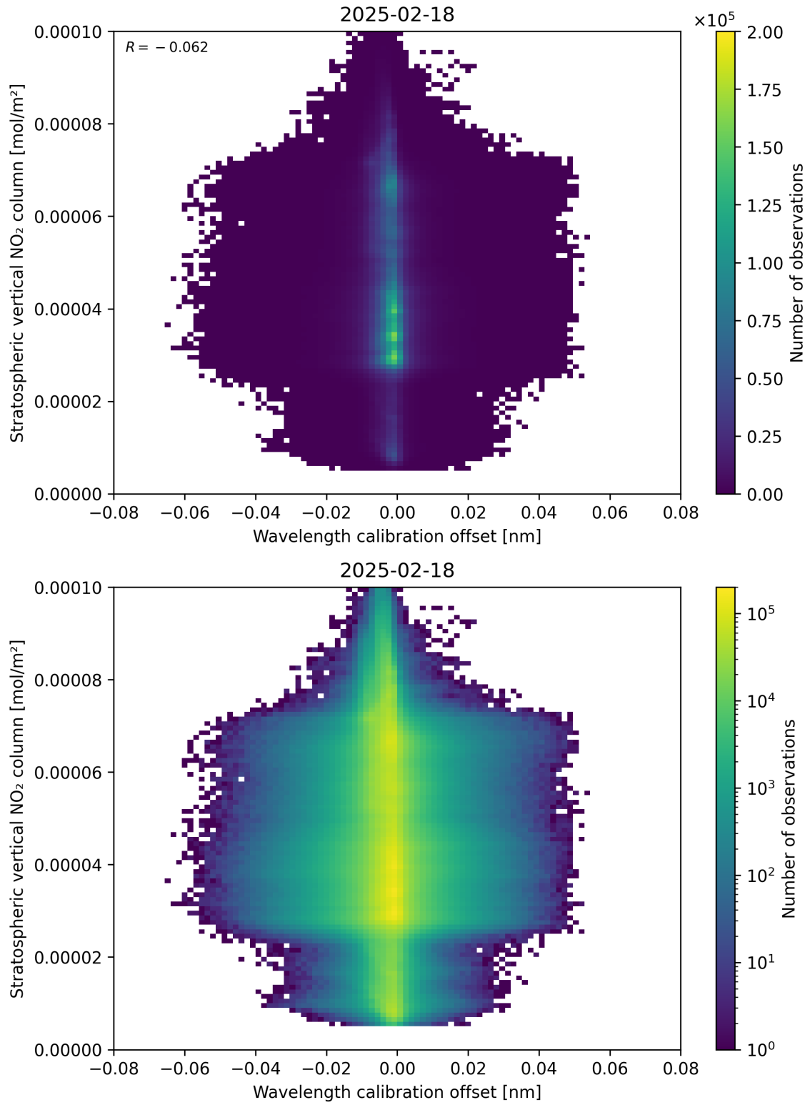
Figure 176: Scatter density plot of “Wavelength calibration offset” against “Stratospheric vertical NO 2 column” for 2025-02-18 to 2025-02-19.
