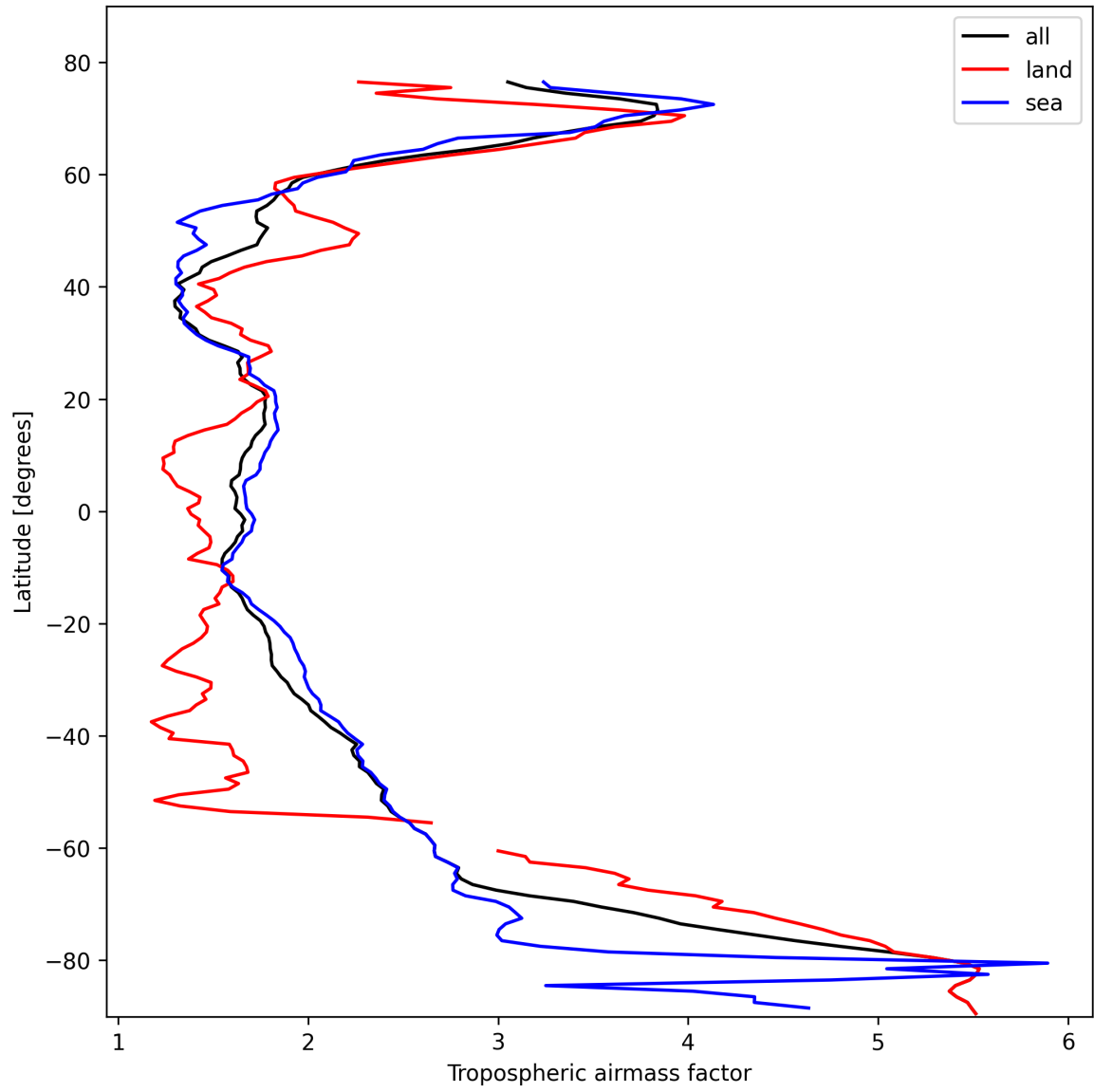
Figure 14: Zonal average of “Tropospheric airmass factor” for 2025-02-18 to 2025-02-19.
