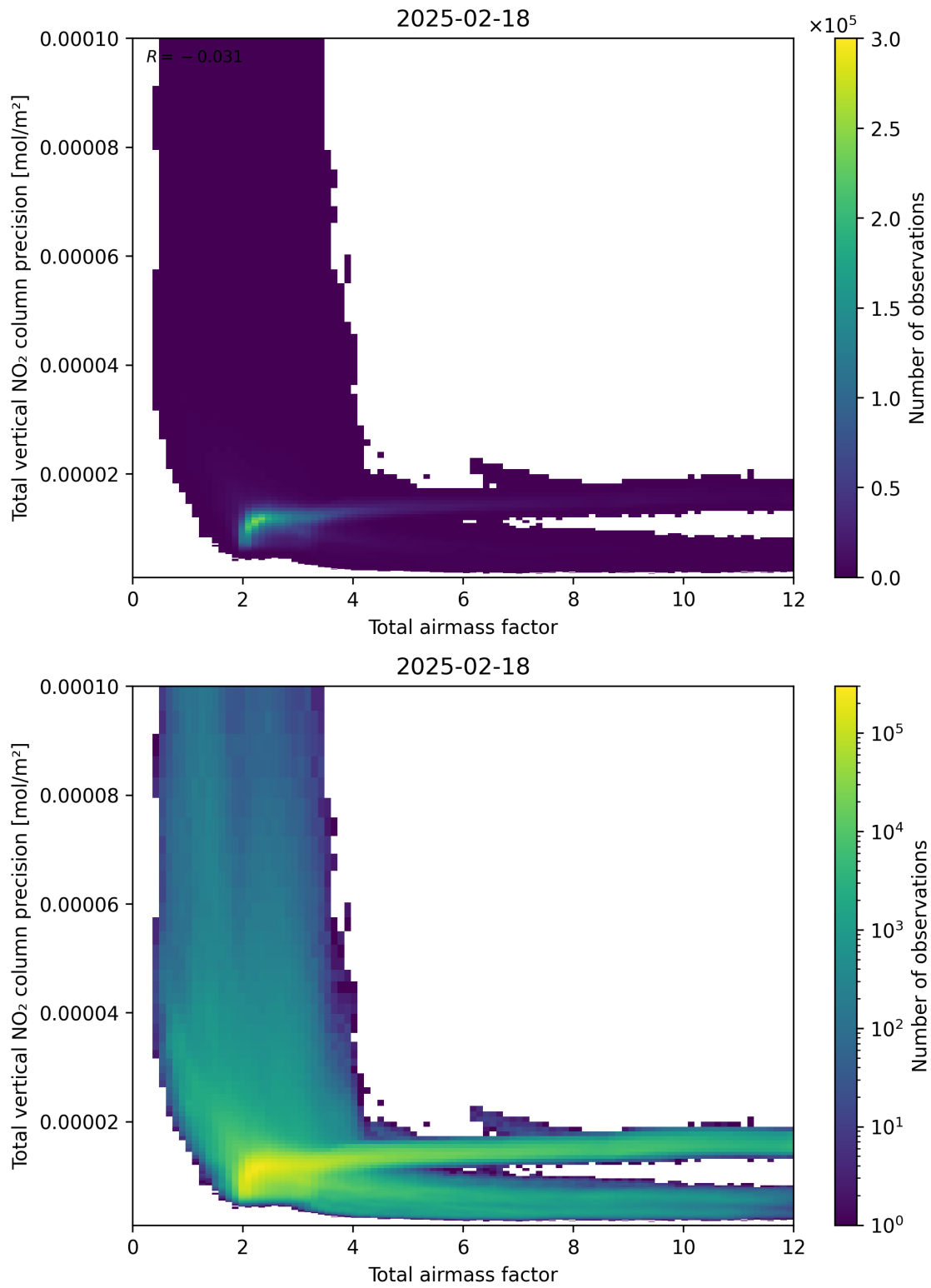
Figure 68: Scatter density plot of “Total airmass factor” against “Total vertical NO 2 column precision” for 2025-02-18 to 2025-02-19.
