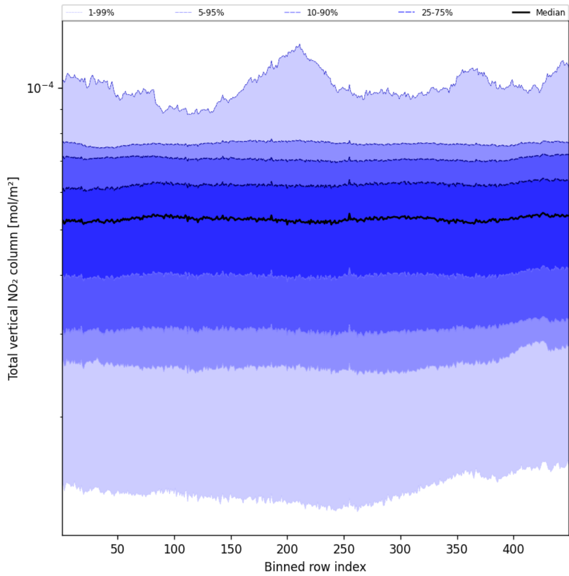
Figure 55: Along track statistics of “Total vertical NO 2 column” for 2025-02-18 to 2025-02-19
