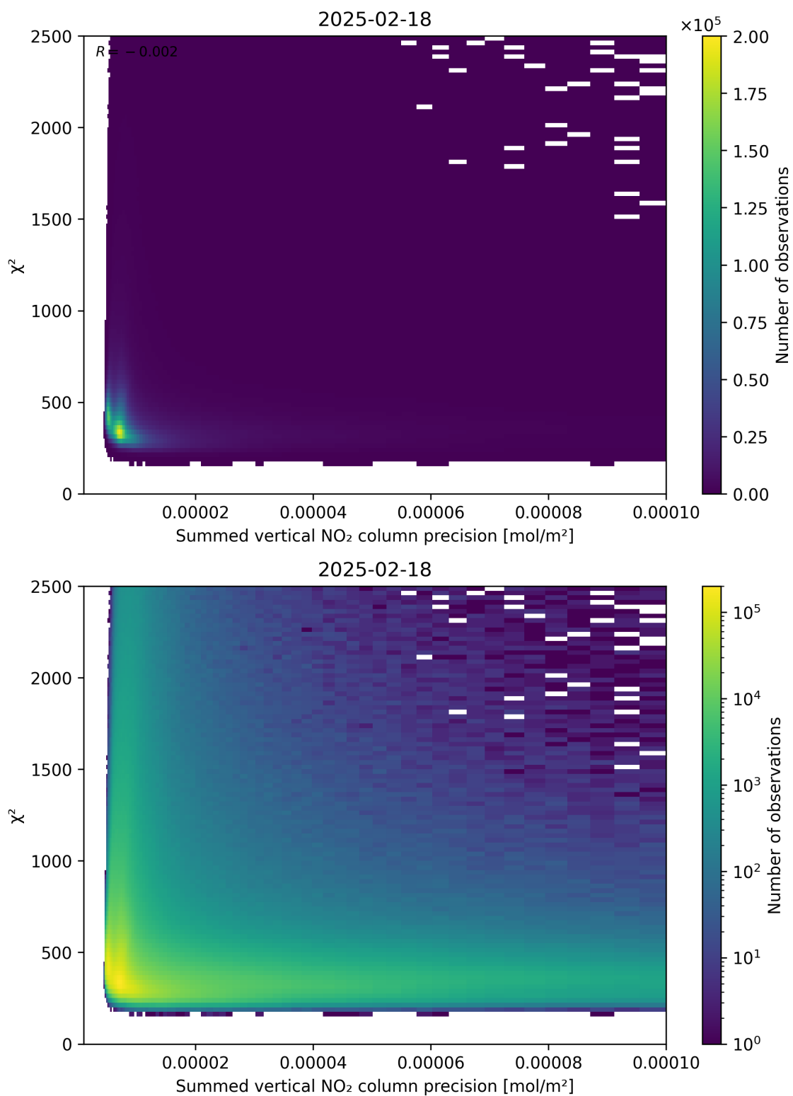
Figure 107: Scatter density plot of “Summed vertical NO 2 column precision” against “ \chi^2 ” for 2025-02-18 to 2025-02-19.
