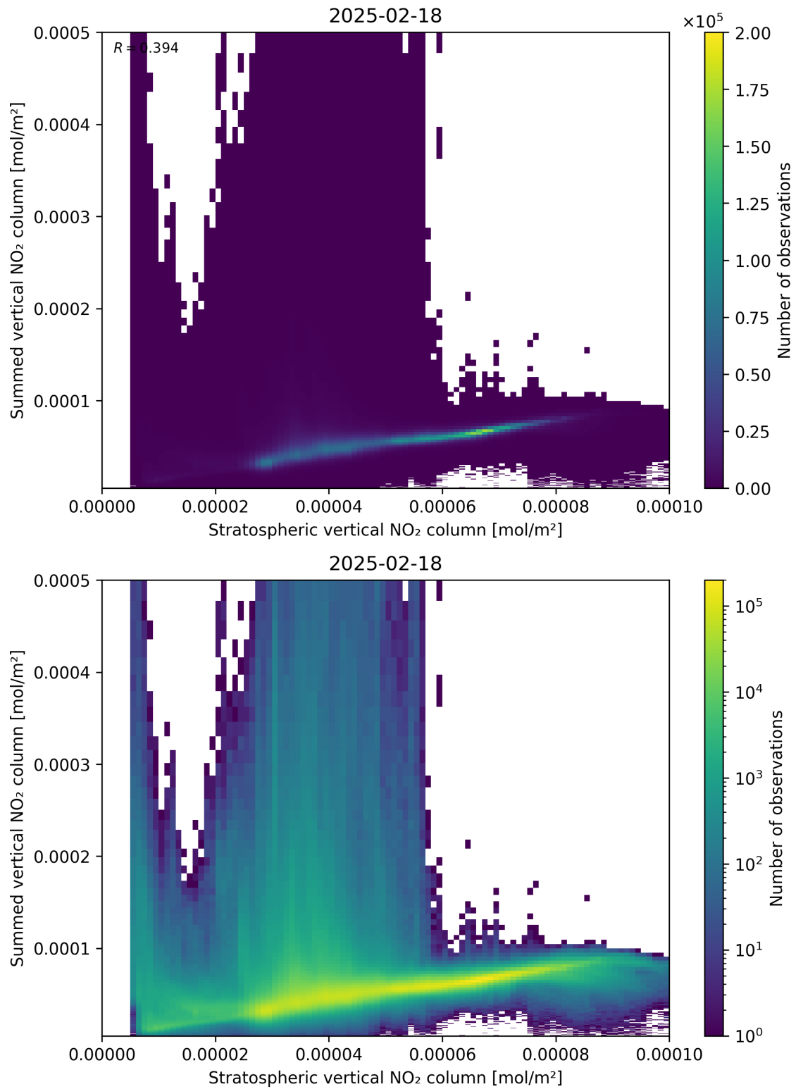
Figure 98: Scatter density plot of “Stratospheric vertical NO 2 column” against “Summed vertical NO 2 column” for 2025-02-18 to 2025-02-19.
