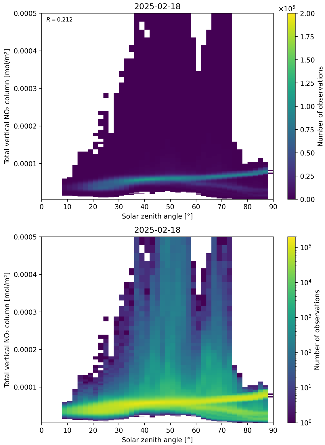
Figure 153: Scatter density plot of “Solar zenith angle” against “Total vertical NO 2 column” for 2025-02-18 to 2025-02-19.
