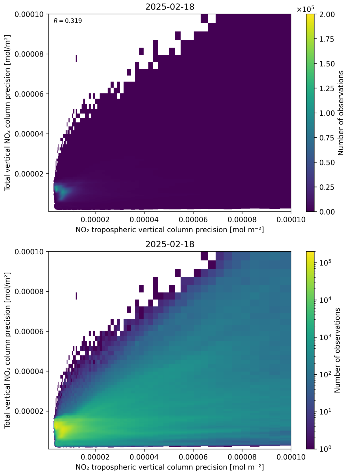
Figure 139: Scatter density plot of “NO 2 tropospheric vertical column precision” against “Total vertical NO 2 column precision” for 2025-02-18 to 2025-02-19.
