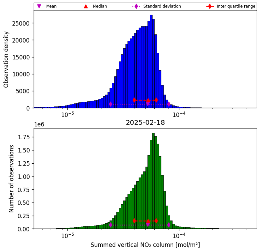
Figure 40: Histogram of “Summed vertical NO 2 column” for 2025-02-18 to 2025-02-19
