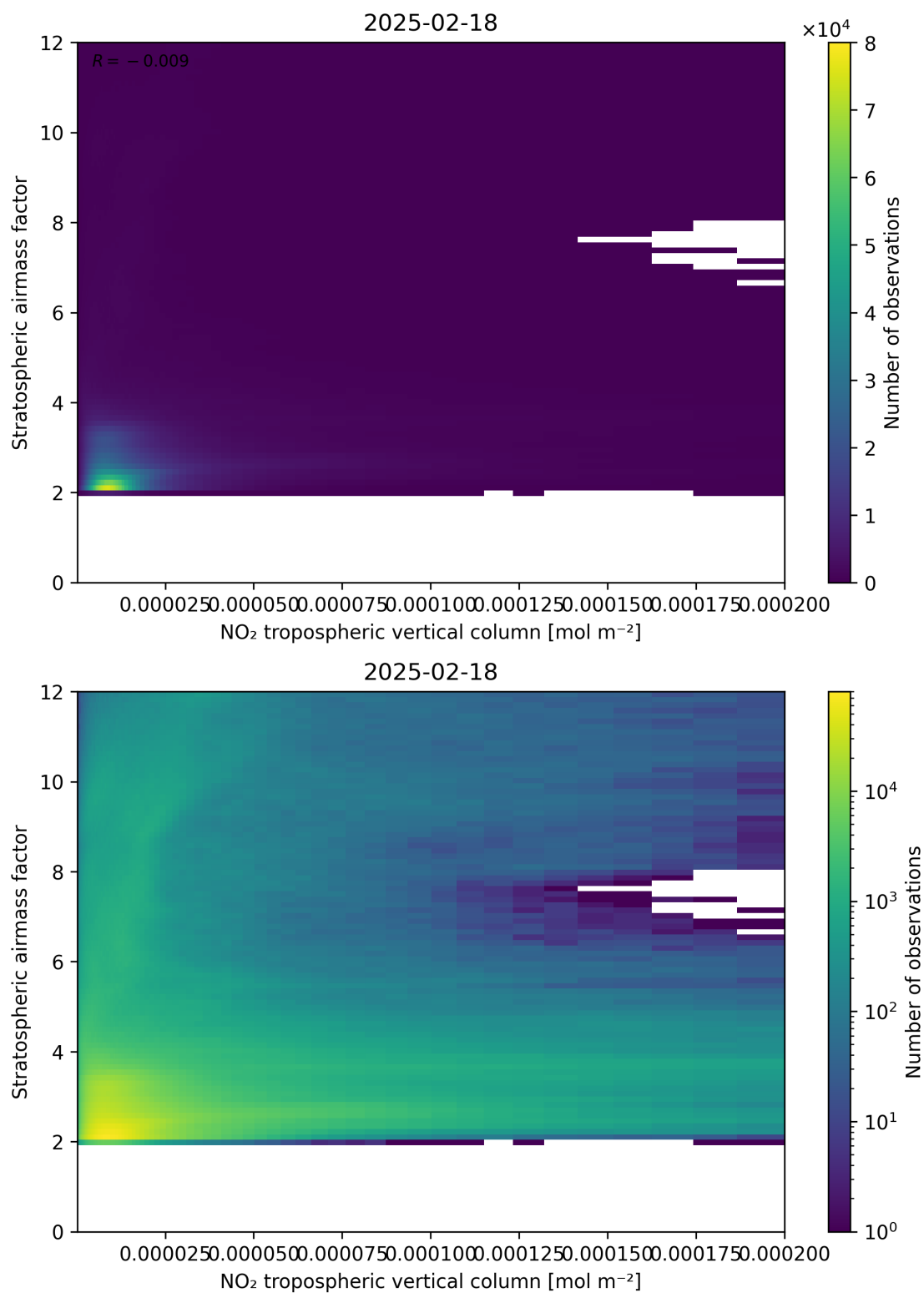
Figure 121: Scatter density plot of “NO 2 tropospheric vertical column” against “Stratospheric air mass factor” for 2025-02-18 to 2025-02-19.
