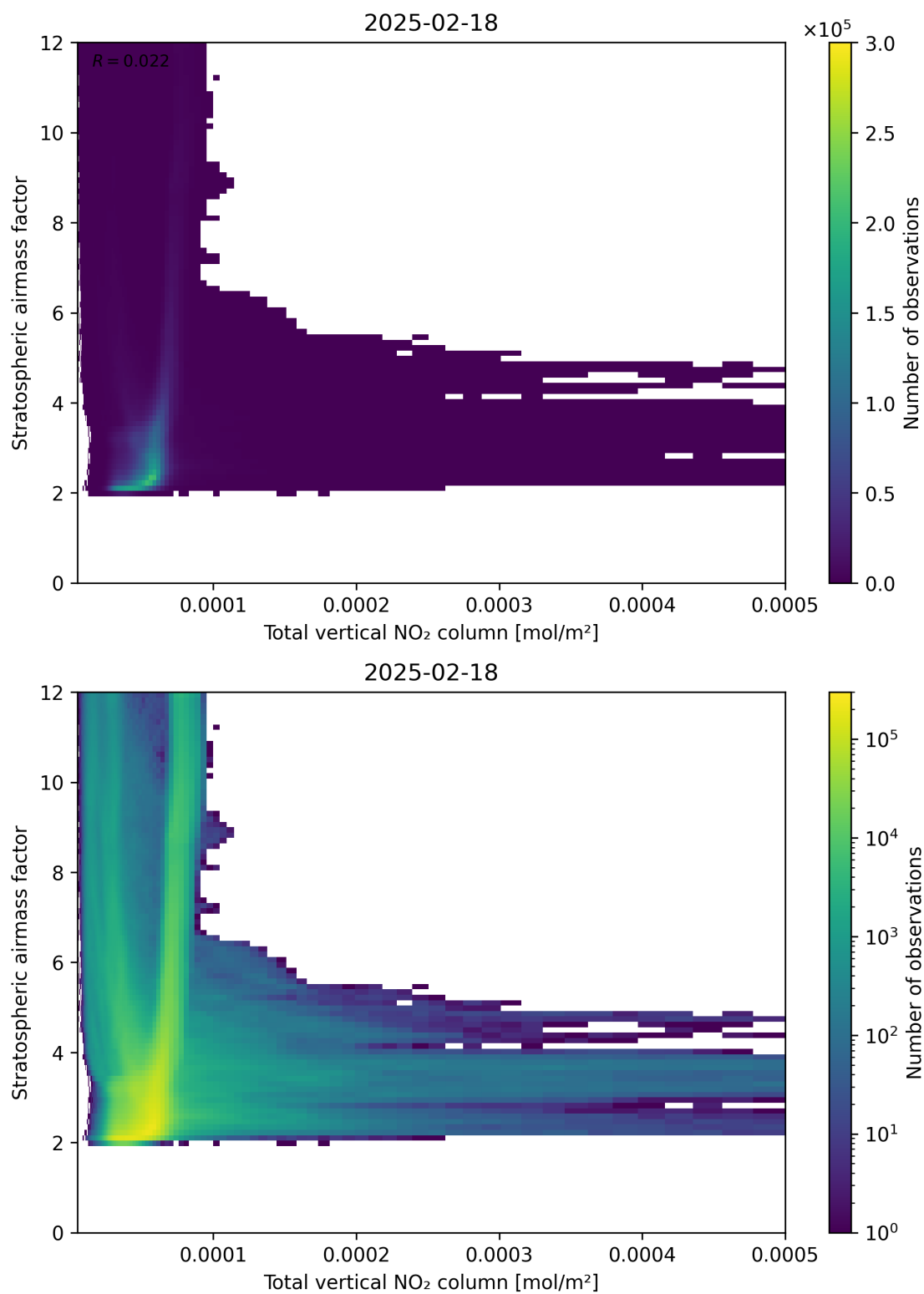
Figure 110: Scatter density plot of “Total vertical NO 2 column” against “Stratospheric airmass factor” for 2025-02-18 to 2025-02-19.
