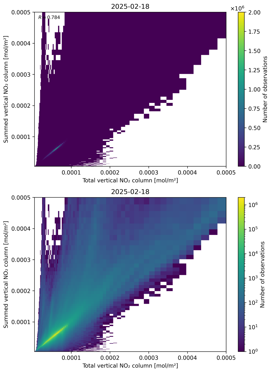
Figure 112: Scatter density plot of “Total vertical NO 2 column” against “Summed vertical NO 2 column” for 2025-02-18 to 2025-02-19.
