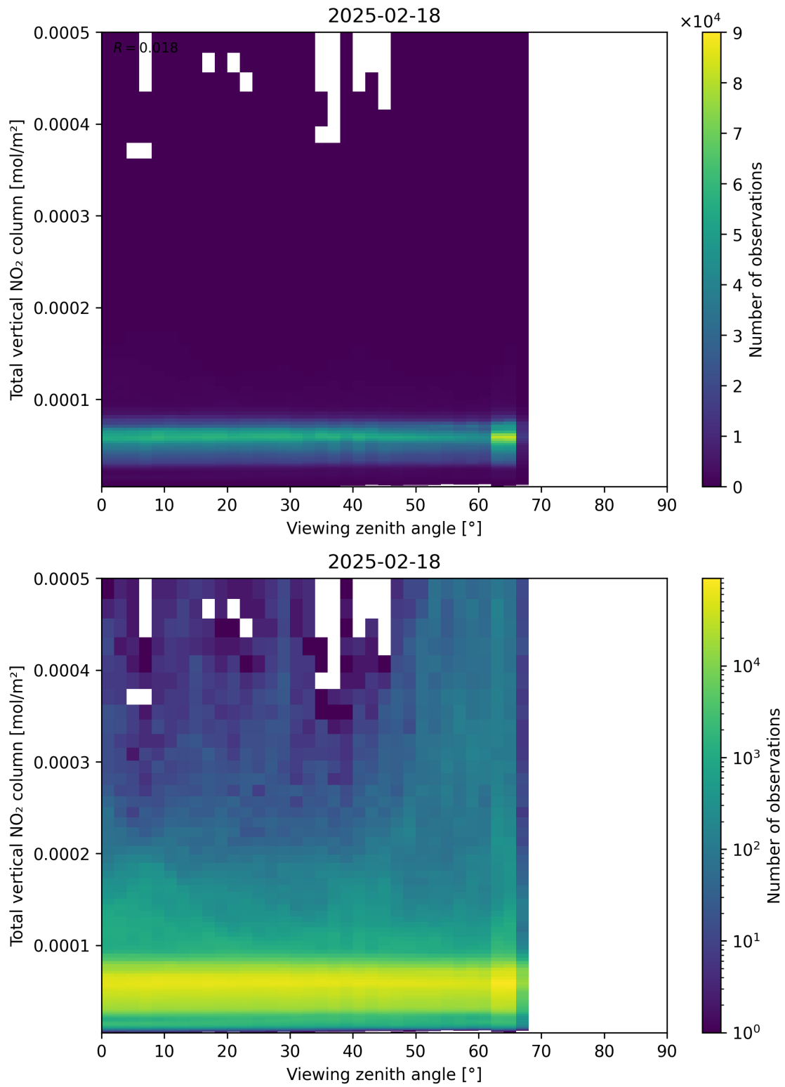
Figure 167: Scatter density plot of “Viewing zenith angle” against “Total vertical NO 2 column” for 2025-02-18 to 2025-02-19.
