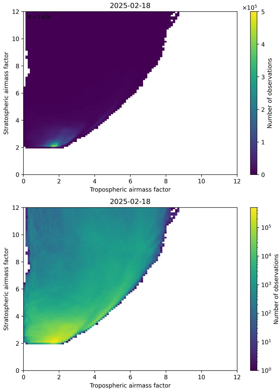
Figure 71: Scatter density plot of “Tropospheric airmass factor” against “Stratospheric airmass factor” for 2025-02-18 to 2025-02-19.
