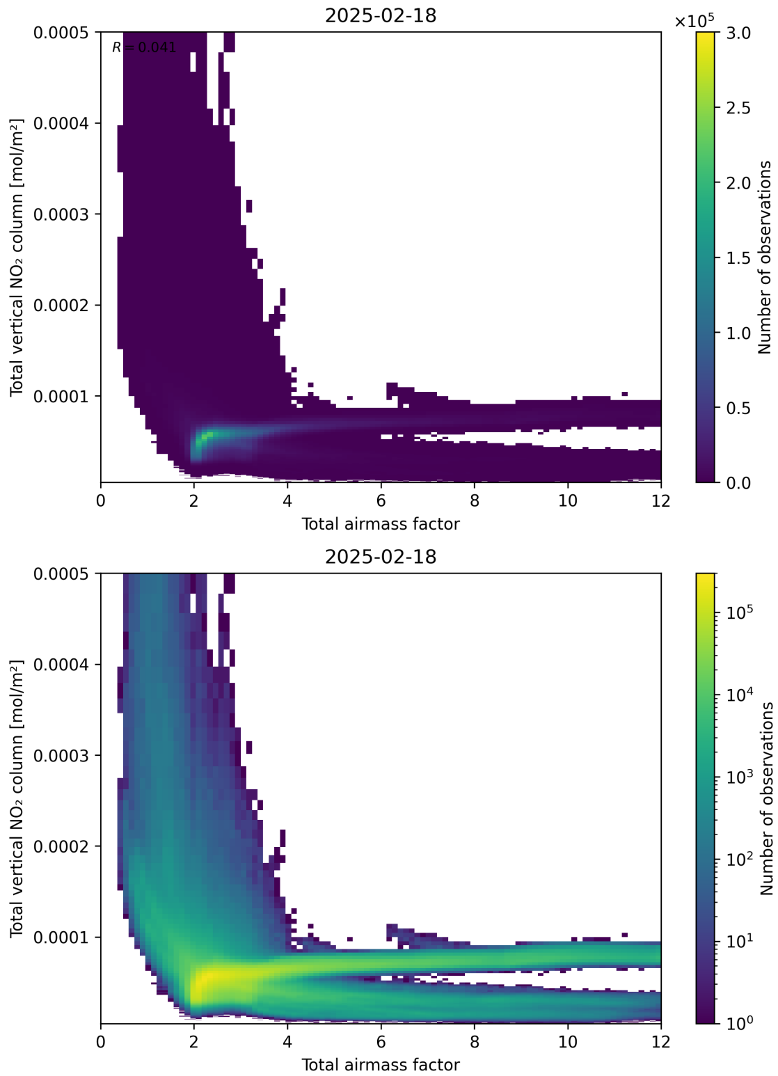
Figure 67: Scatter density plot of “Total airmass factor” against “Total vertical NO 2 column” for 2025-02-18 to 2025-02-19.
