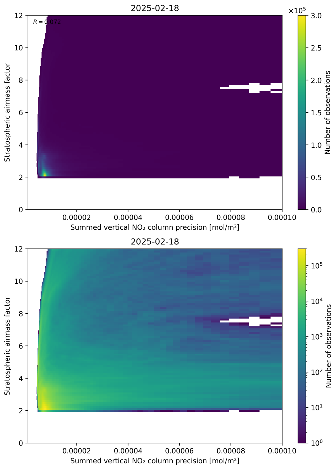
Figure 106: Scatter density plot of “Summed vertical NO 2 column precision” against “Stratospheric airmass factor” for 2025-02-18 to 2025-02-19.
