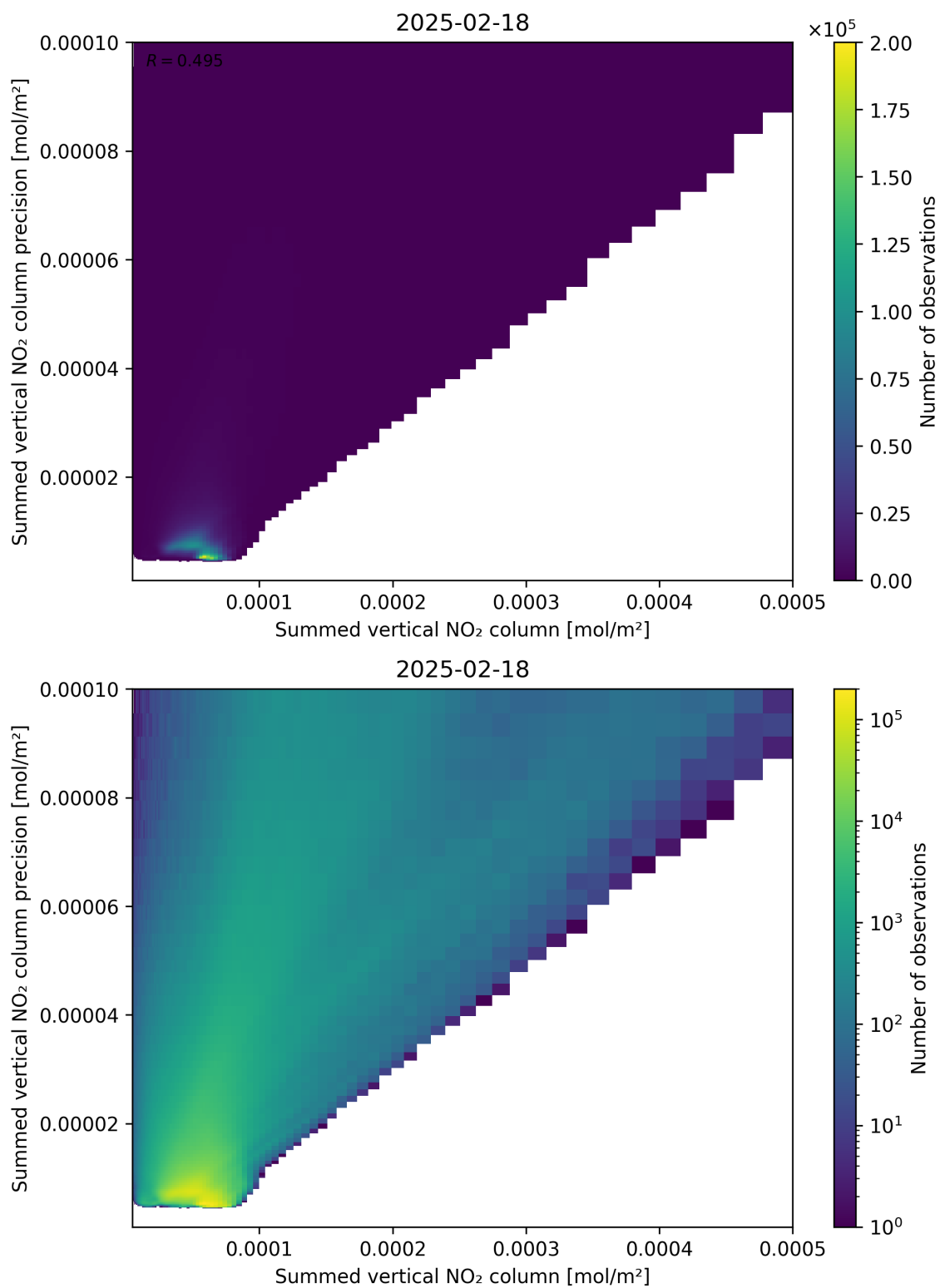
Figure 105: Scatter density plot of “Summed vertical NO 2 column” against “Summed vertical NO 2 column precision” for 2025-02-18 to 2025-02-19.
