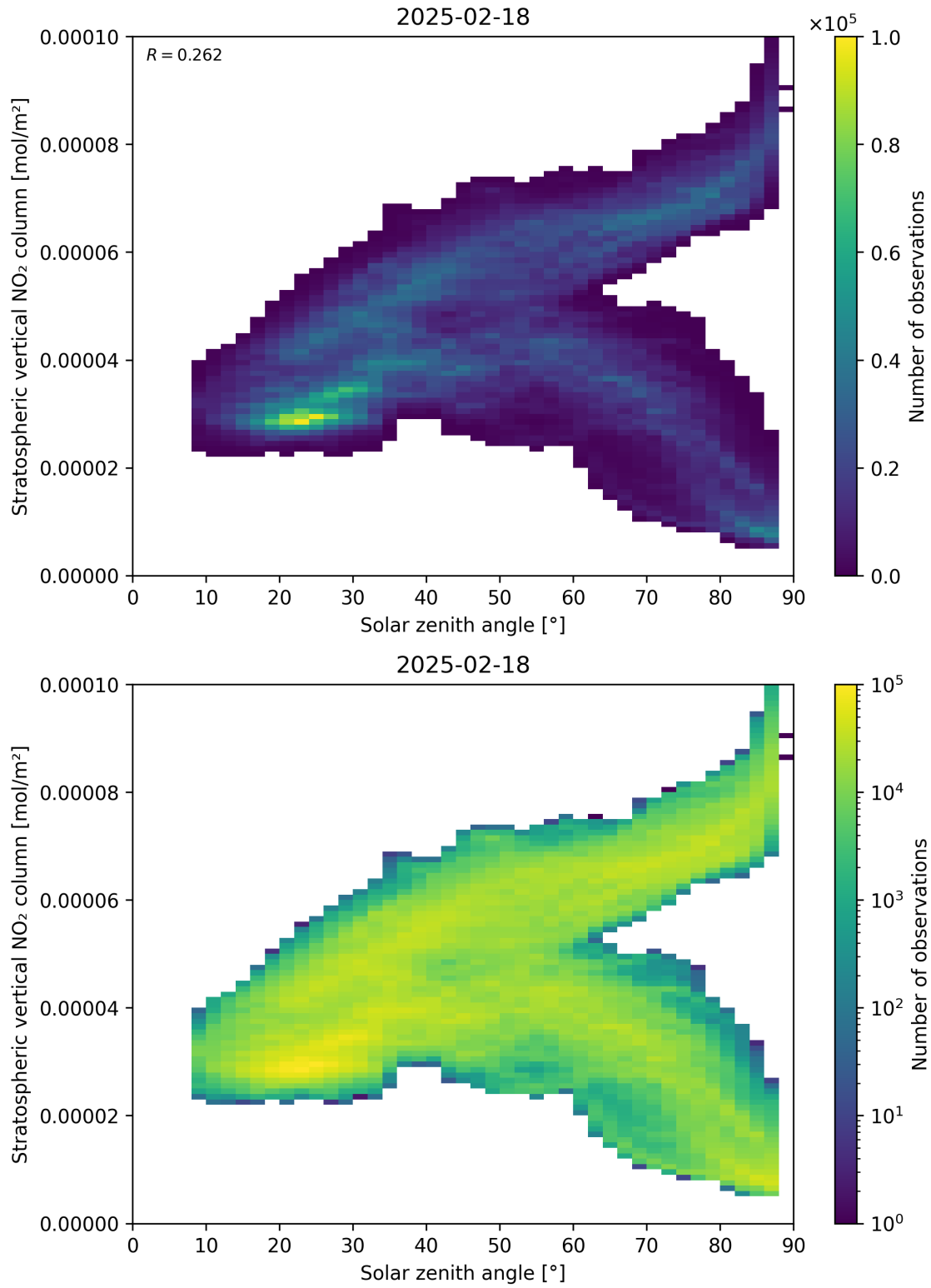
Figure 150: Scatter density plot of “Solar zenith angle” against “Stratospheric vertical NO 2 column” for 2025-02-18 to 2025-02-19.
