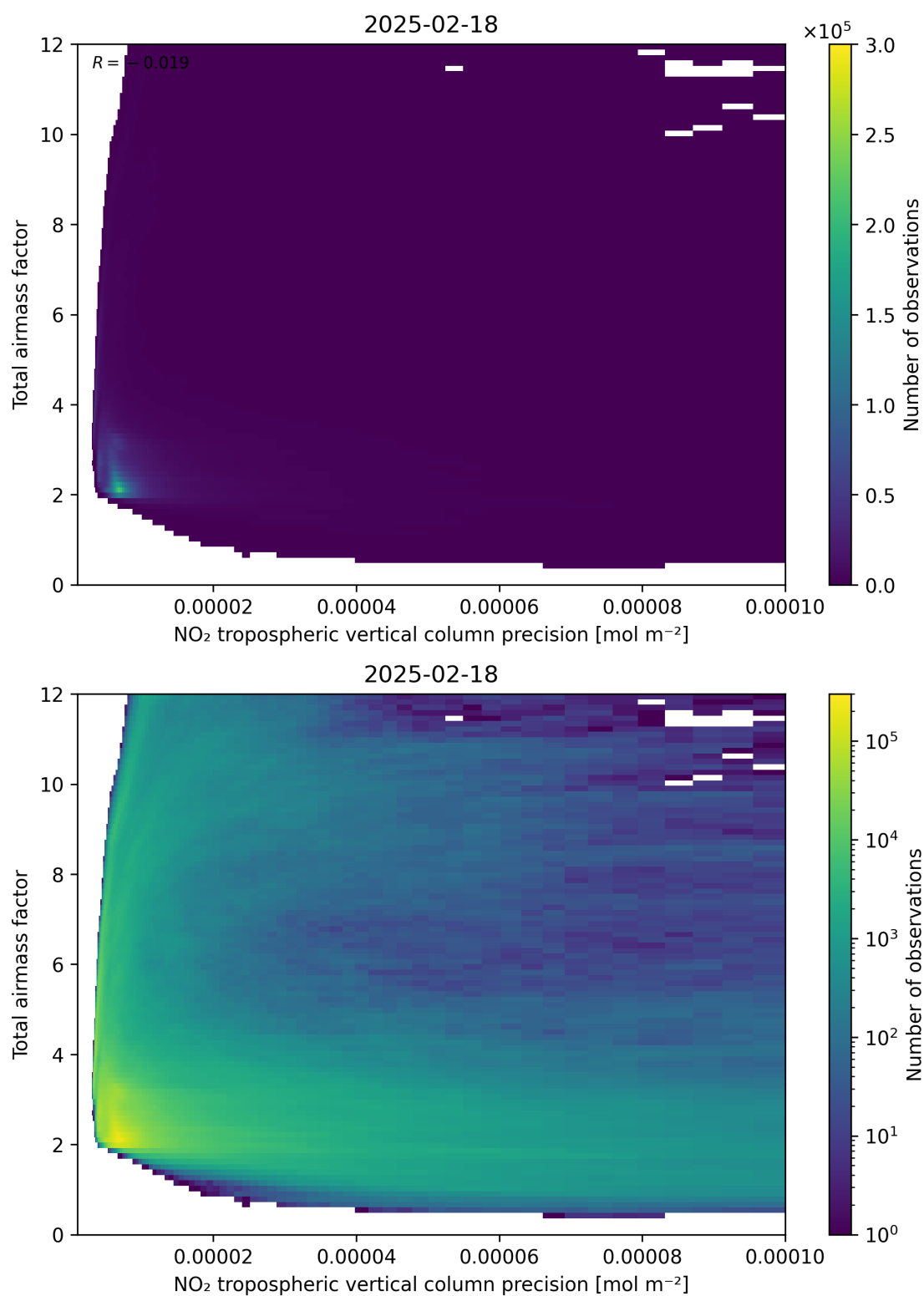
Figure 132: Scatter density plot of “NO 2 tropospheric vertical column precision” against “Total air mass factor” for 2025-02-18 to 2025-02-19.
