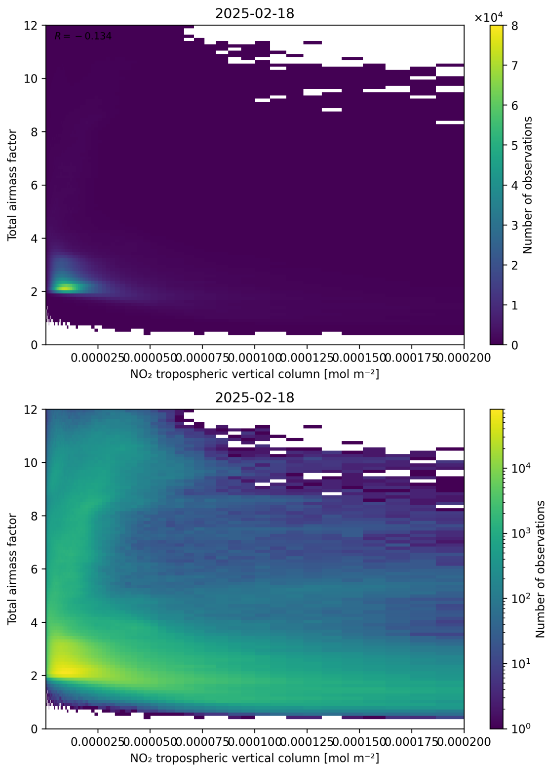
Figure 122: Scatter density plot of “NO 2 tropospheric vertical column” against “Total air mass factor” for 2025-02-18 to 2025-02-19.
