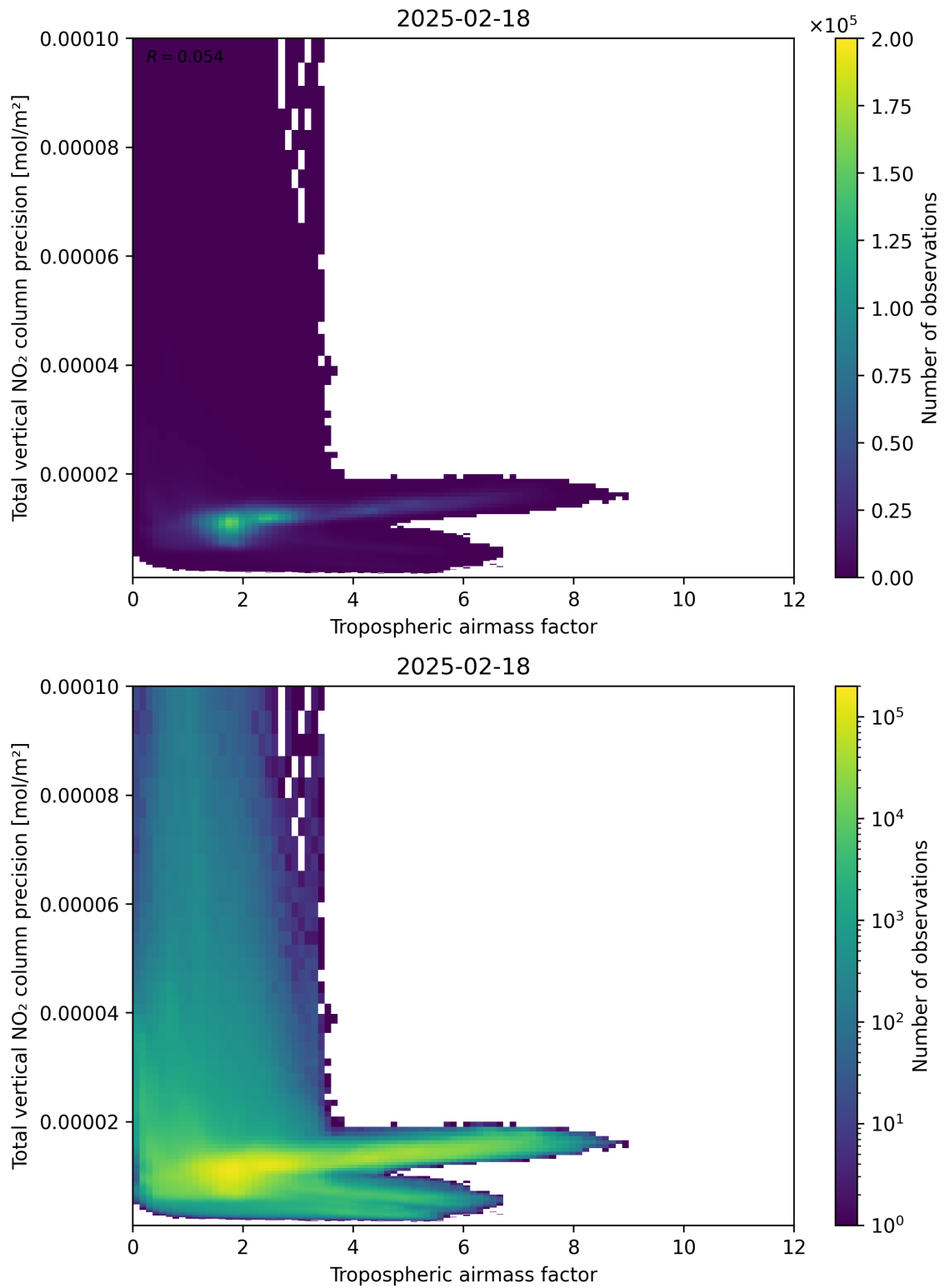
Figure 78: Scatter density plot of “Tropospheric air mass factor” against “Total vertical NO 2 column precision” for 2025-02-18 to 2025-02-19.
