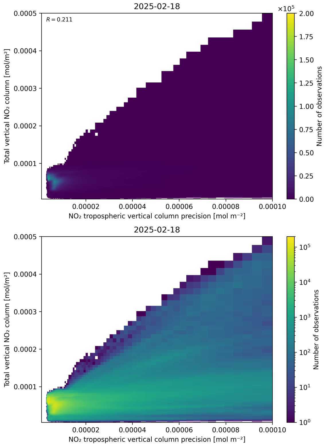
Figure 138: Scatter density plot of “NO 2 tropospheric vertical column precision” against “Total vertical NO 2 column” for 2025-02-18 to 2025-02-19.
