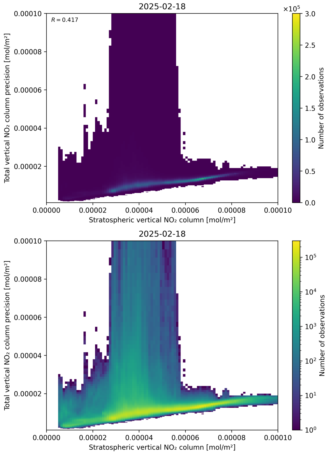
Figure 101: Scatter density plot of “Stratospheric vertical NO 2 column” against “Total vertical NO 2 column precision” for 2025-02-18 to 2025-02-19.
