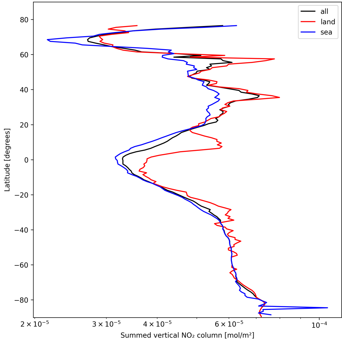
Figure 23: Zonal average of “Summed vertical NO 2 column” for 2025-02-18 to 2025-02-19.
