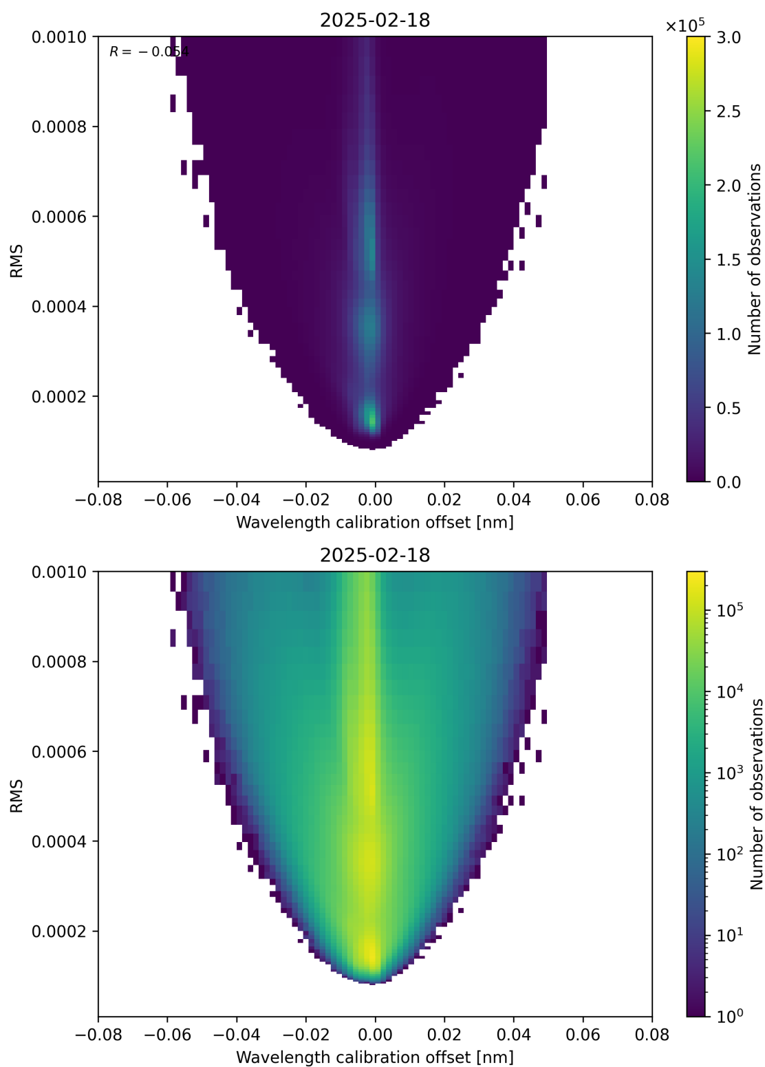
Figure 181: Scatter density plot of “Wavelength calibration offset” against “RMS” for 2025-02-18 to 2025-02-19.
