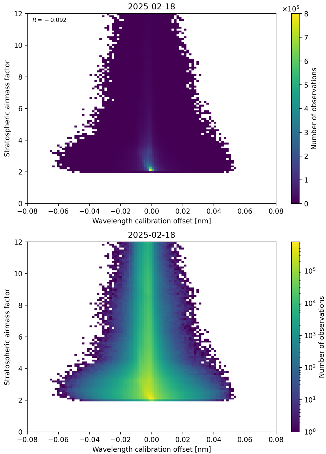
Figure 174: Scatter density plot of “Wavelength calibration offset” against “Stratospheric airmass factor” for 2025-02-18 to 2025-02-19.
