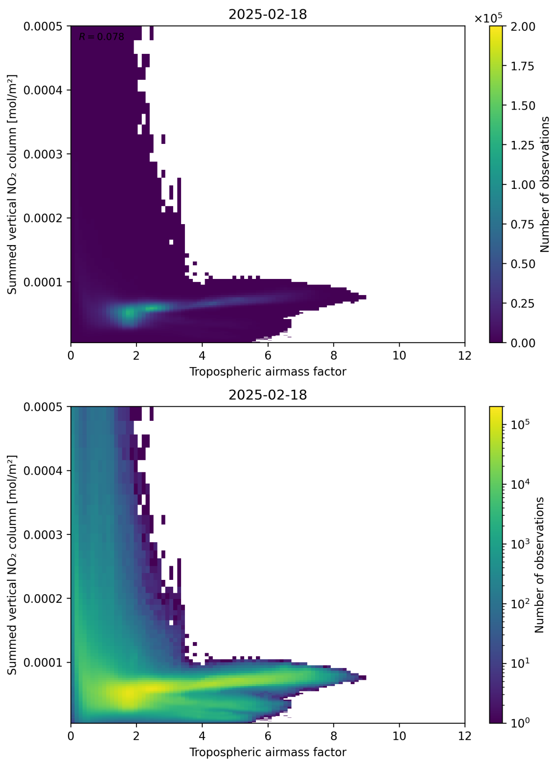
Figure 75: Scatter density plot of “Tropospheric air mass factor” against “Summed vertical NO 2 column” for 2025-02-18 to 2025-02-19.
