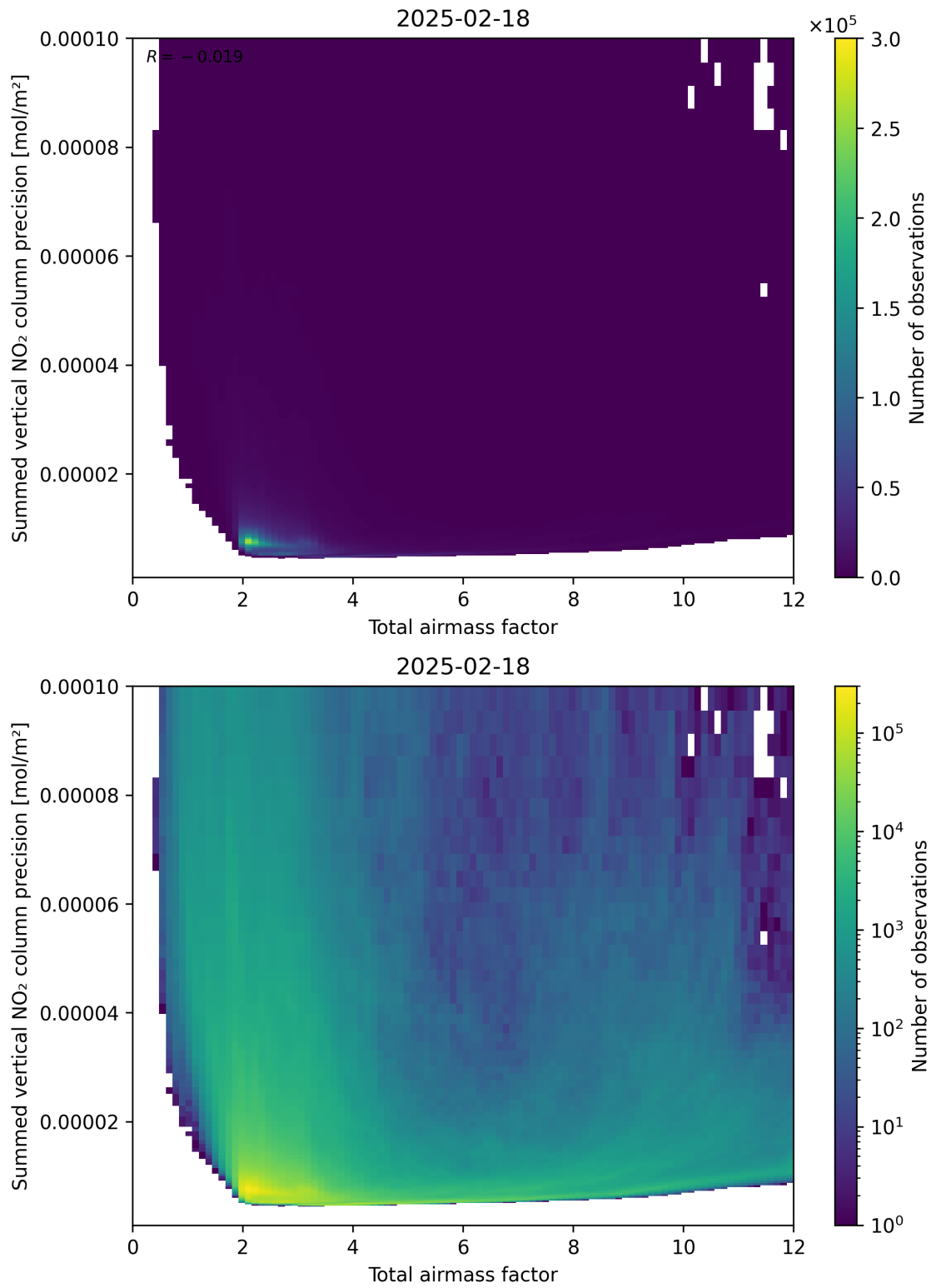
Figure 66: Scatter density plot of “Total airmass factor” against “Summed vertical NO 2 column precision” for 2025-02-18 to 2025-02-19.
