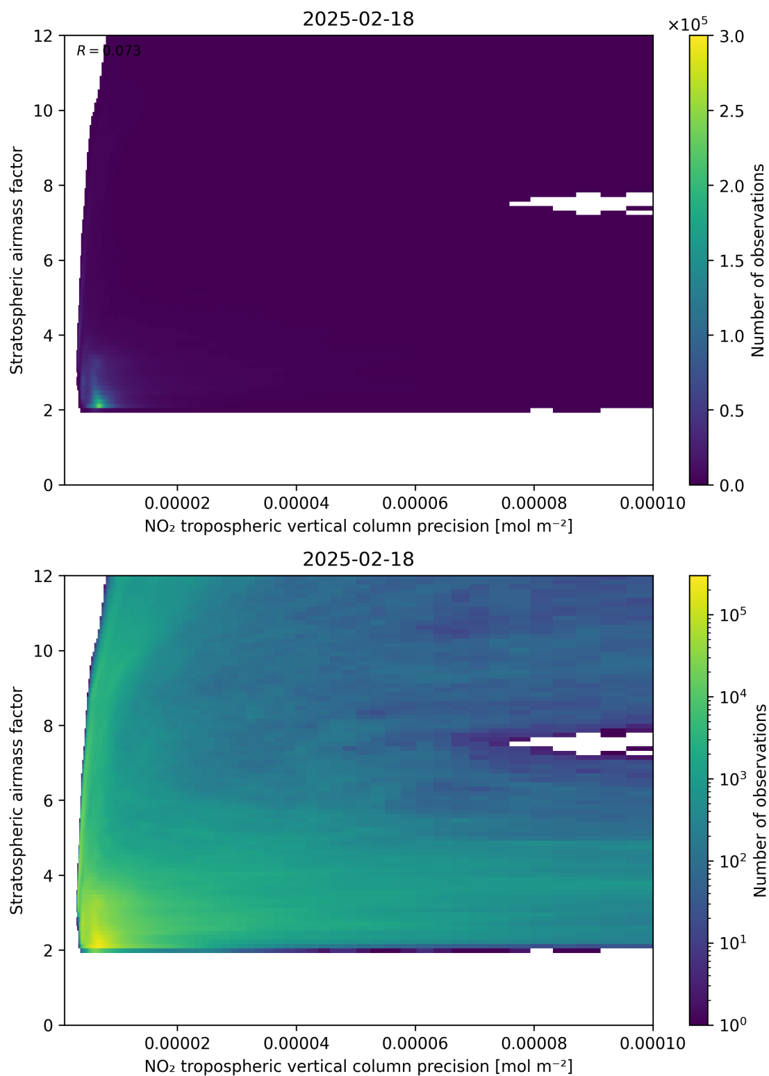
Figure 131: Scatter density plot of “NO 2 tropospheric vertical column precision” against “Stratospheric airmass factor” for 2025-02-18 to 2025-02-19.
