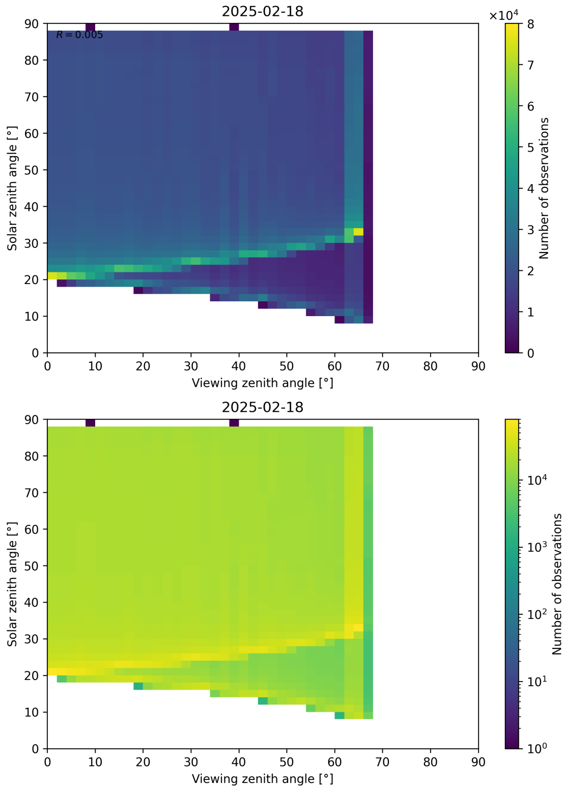
Figure 172: Scatter density plot of “Viewing zenith angle” against “Solar zenith angle” for 2025-02-18 to 2025-02-19.
