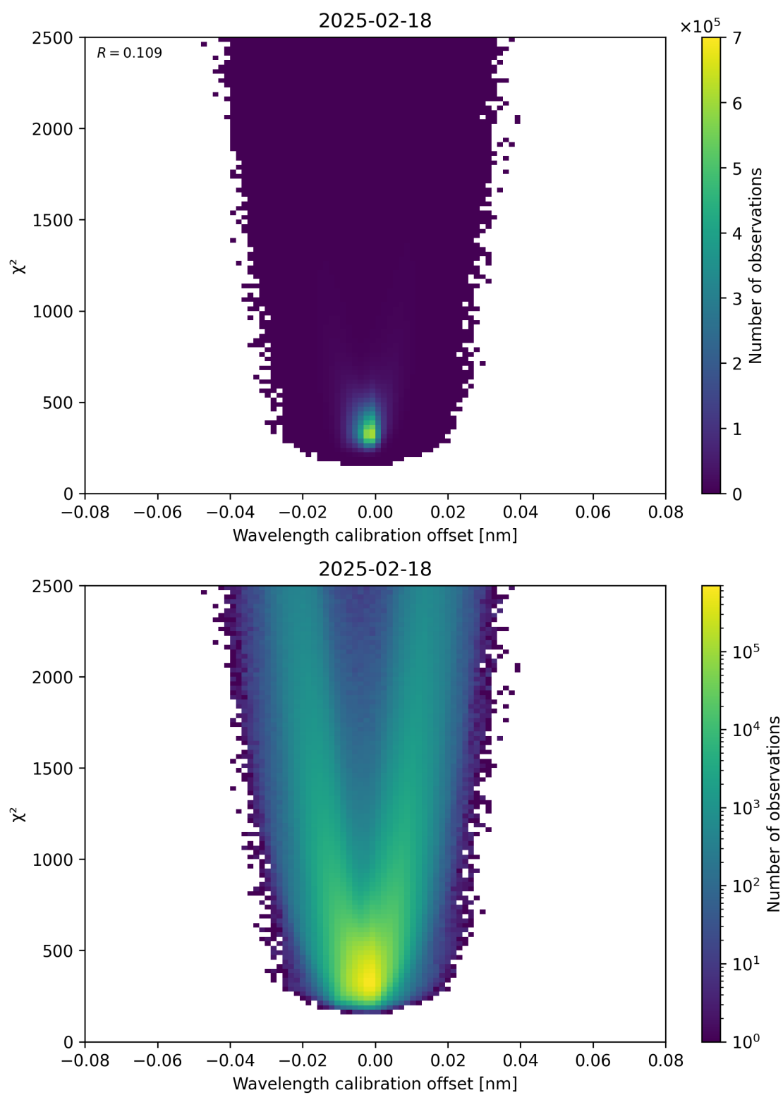
Figure 175: Scatter density plot of “Wavelength calibration offset” against “ \chi^2 ” for 2025-02-18 to 2025-02-19.
