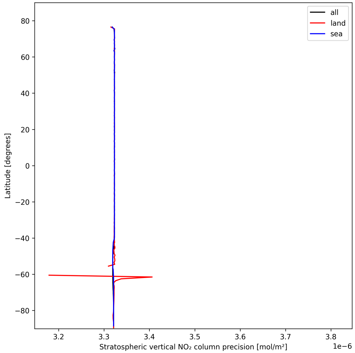
Figure 20: Zonal average of “Stratospheric vertical NO 2 column precision” for 2025-02-18 to 2025-02-19.
