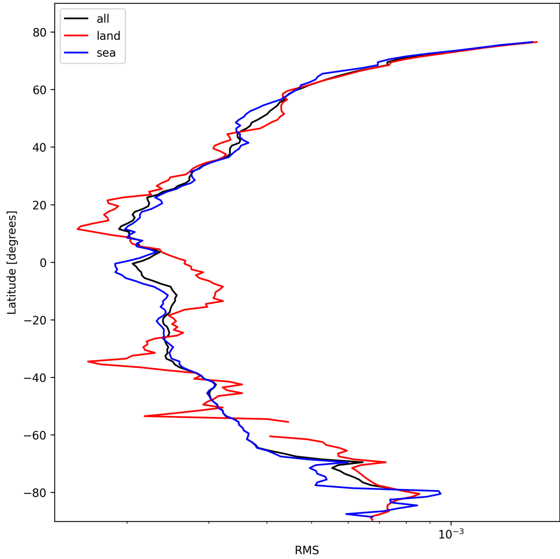
Figure 26: Zonal average of “RMS” for 2025-02-18 to 2025-02-19.
