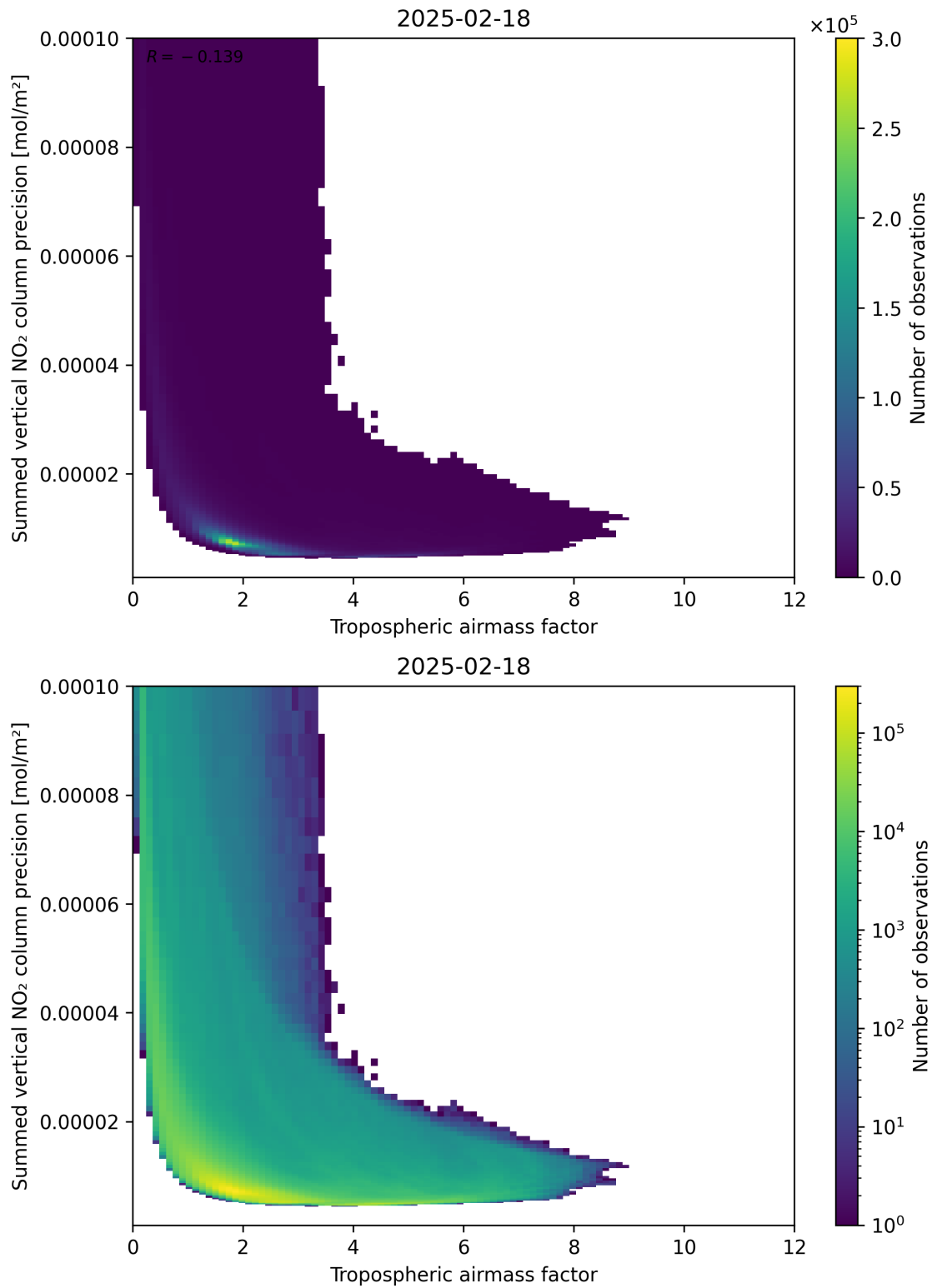
Figure 76: Scatter density plot of “Tropospheric air mass factor” against “Summed vertical NO 2 column precision” for 2025-02-18 to 2025-02-19.
