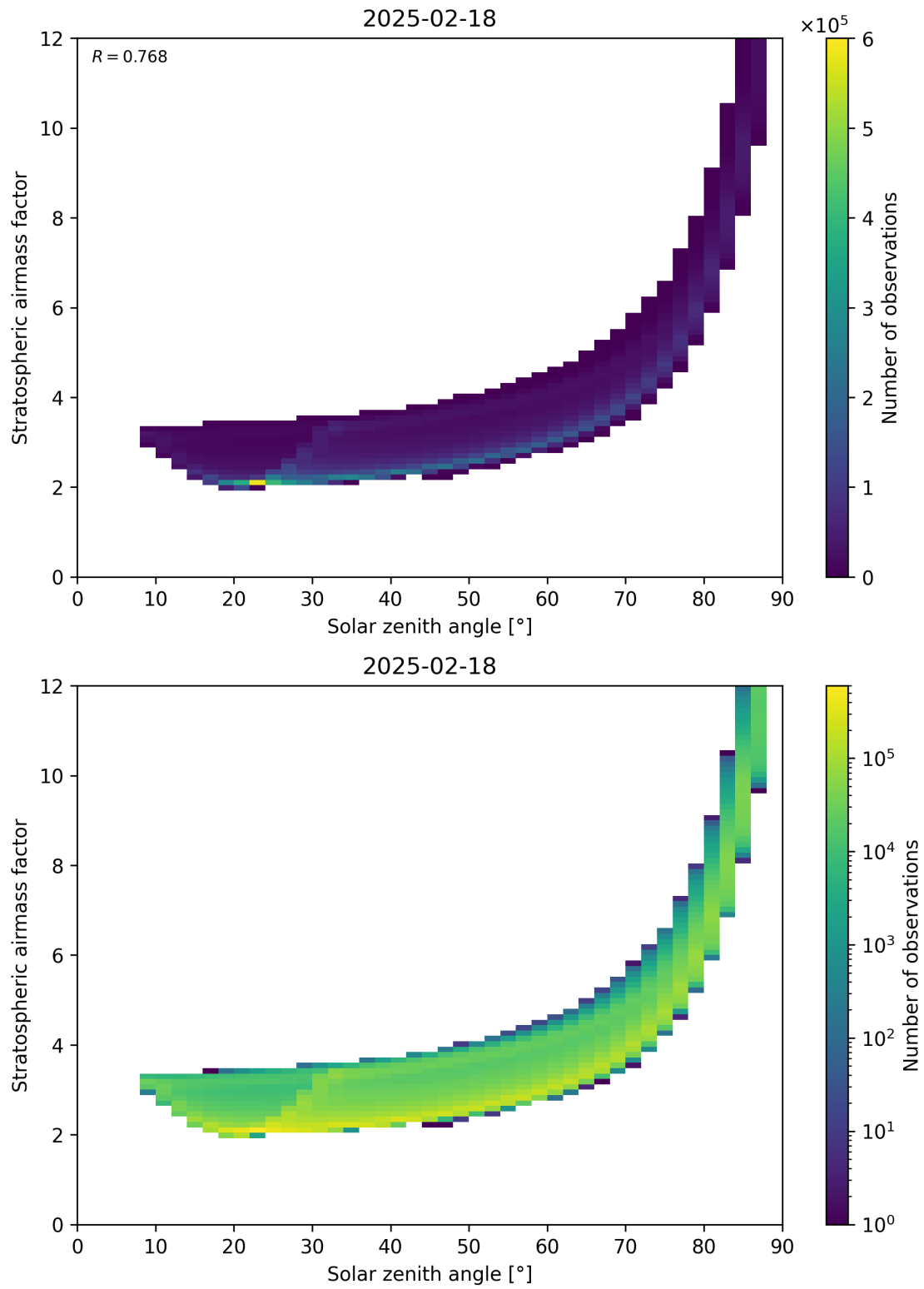
Figure 145: Scatter density plot of “Solar zenith angle” against “Stratospheric airmass factor” for 2025-02-18 to 2025-02-19.
