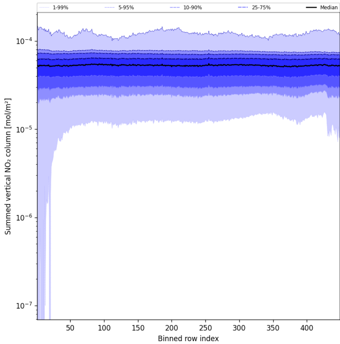
Figure 57: Along track statistics of “Summed vertical NO 2 column” for 2025-02-18 to 2025-02-19
