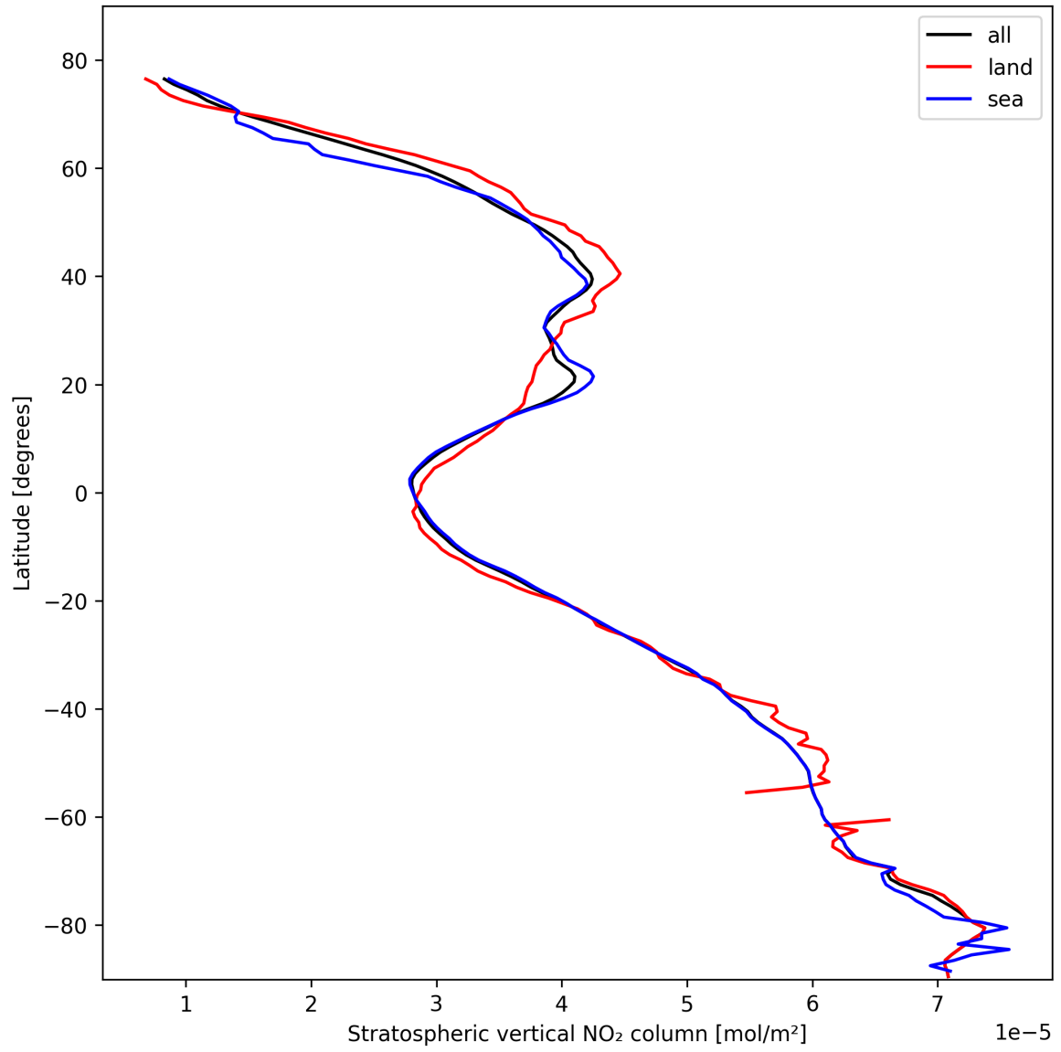
Figure 19: Zonal average of “Stratospheric vertical NO 2 column” for 2025-02-18 to 2025-02-19.
