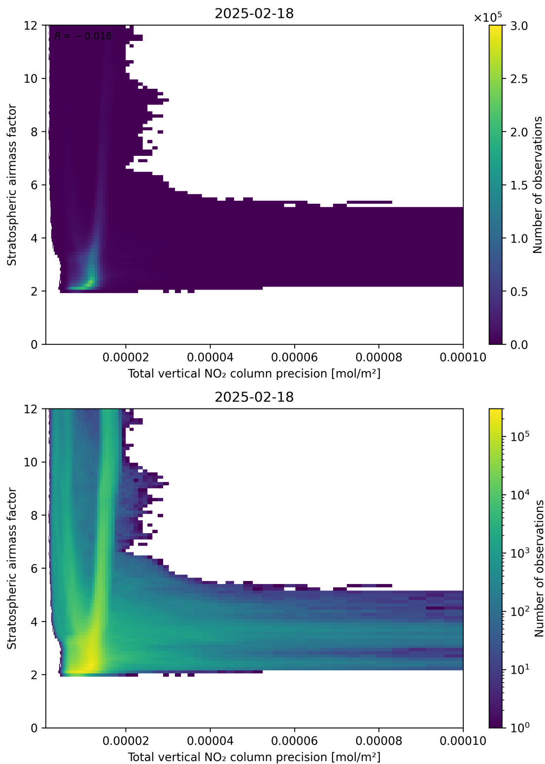
Figure 115: Scatter density plot of “Total vertical NO 2 column precision” against “Stratospheric airmass factor” for 2025-02-18 to 2025-02-19.
