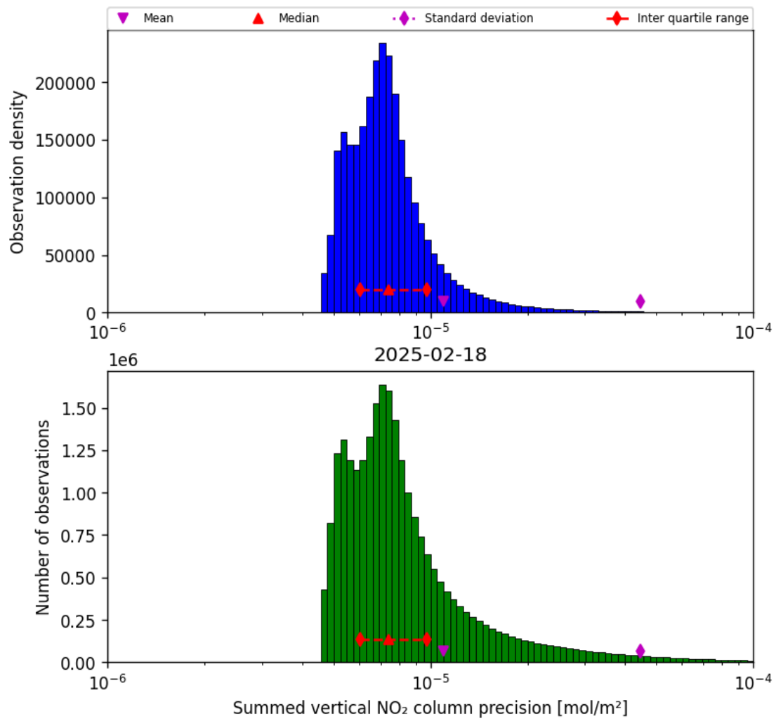
Figure 41: Histogram of "Summed vertical NO 2 column precision" for 2025-02-18 to 2025-02-19
