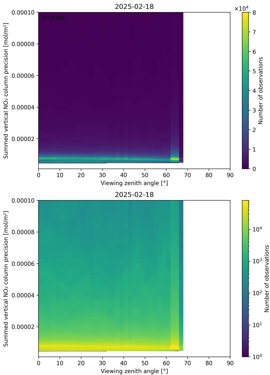
Figure 166: Scatter density plot of “Viewing zenith angle” against “Summed vertical NO 2 column precision” for 2025-02-18 to 2025-02-19.
