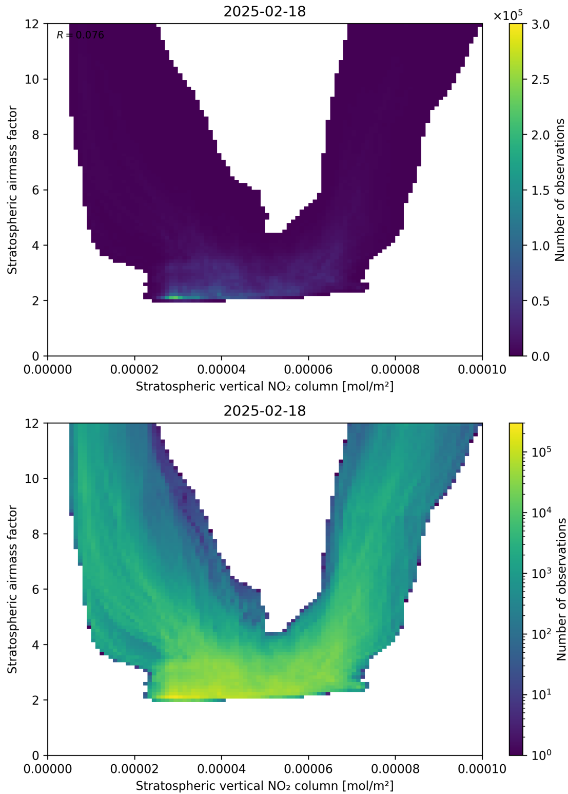
Figure 96: Scatter density plot of “Stratospheric vertical NO 2 column” against “Stratospheric airmass factor” for 2025-02-18 to 2025-02-19.
