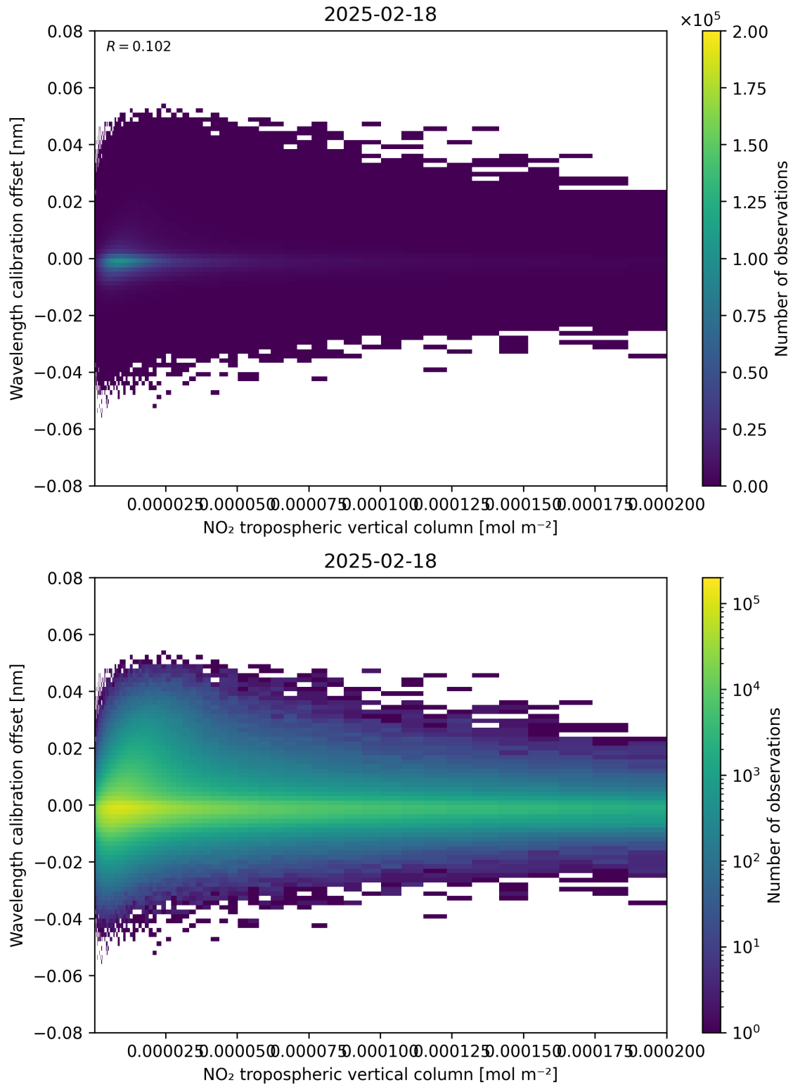
Figure 143: Scatter density plot of “NO 2 tropospheric vertical column” against “Wavelength calibration offset” for 2025-02-18 to 2025-02-19.
