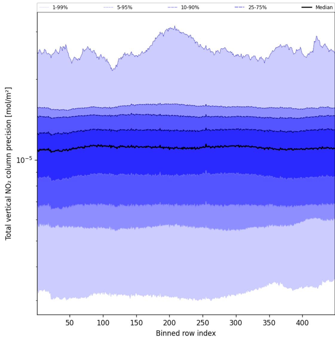
Figure 56: Along track statistics of “Total vertical NO 2 column precision” for 2025-02-18 to 2025-02-19
