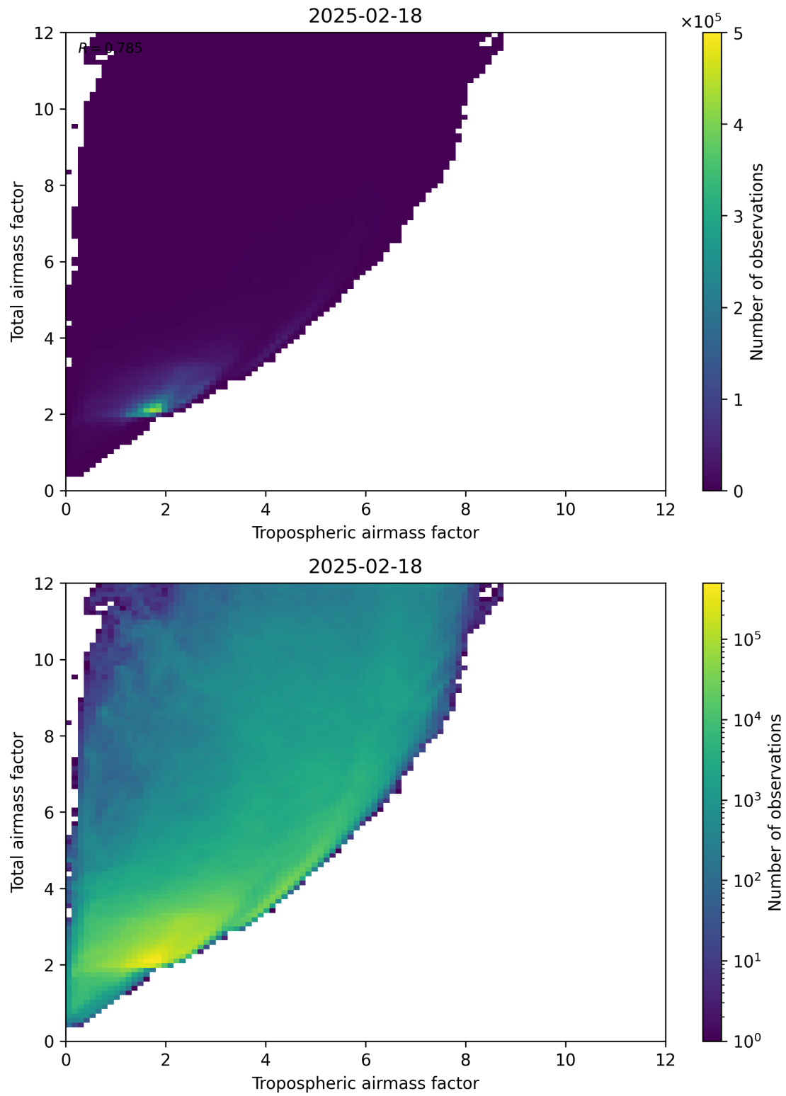
Figure 72: Scatter density plot of “Tropospheric airmass factor” against “Total airmass factor” for 2025-02-18 to 2025-02-19.
