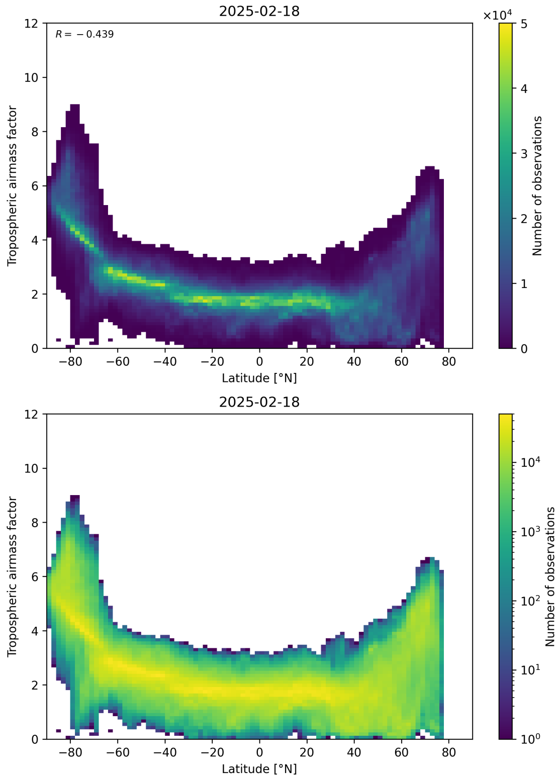
Figure 85: Scatter density plot of “Latitude” against “Tropospheric air mass factor” for 2025-02-18 to 2025-02-19.
