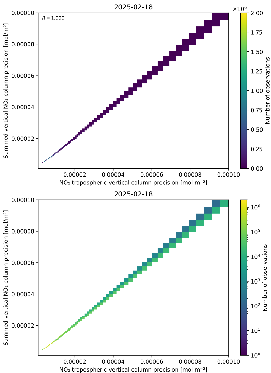
Figure 137: Scatter density plot of “NO 2 tropospheric vertical column precision” against “Summed vertical NO 2 column precision” for 2025-02-18 to 2025-02-19.
