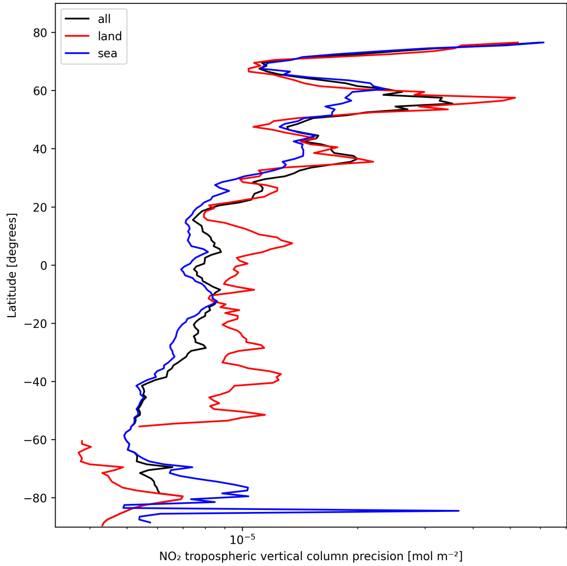
Figure 13: Zonal average of “NO 2 tropospheric vertical column precision” for 2025-02-18 to 2025-02-19.
