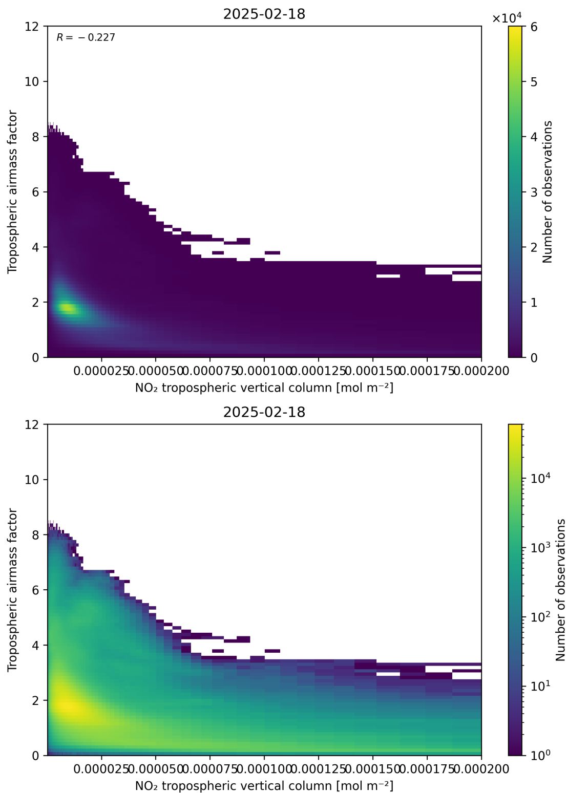
Figure 123: Scatter density plot of “NO 2 tropospheric vertical column” against “Tropospheric air mass factor” for 2025-02-18 to 2025-02-19.
