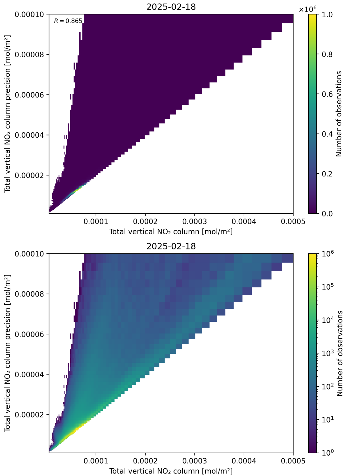
Figure 114: Scatter density plot of “Total vertical NO 2 column” against “Total vertical NO 2 column precision” for 2025-02-18 to 2025-02-19.
