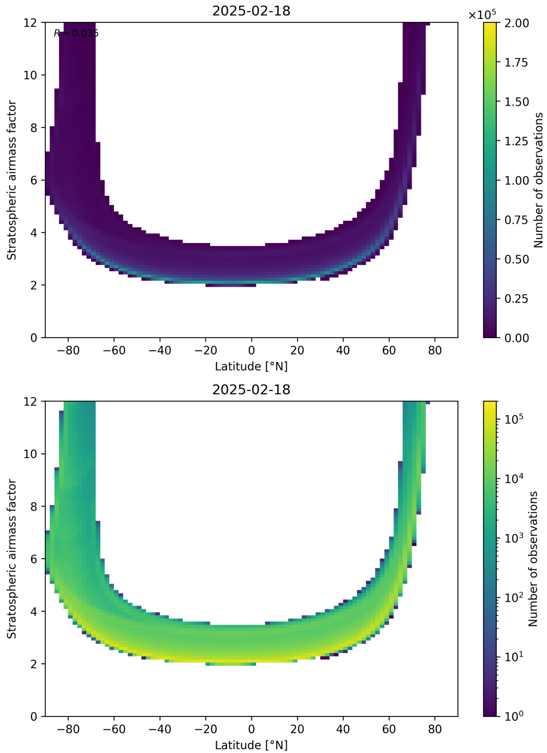
Figure 83: Scatter density plot of “Latitude” against “Stratospheric air mass factor” for 2025-02-18 to 2025-02-19.
