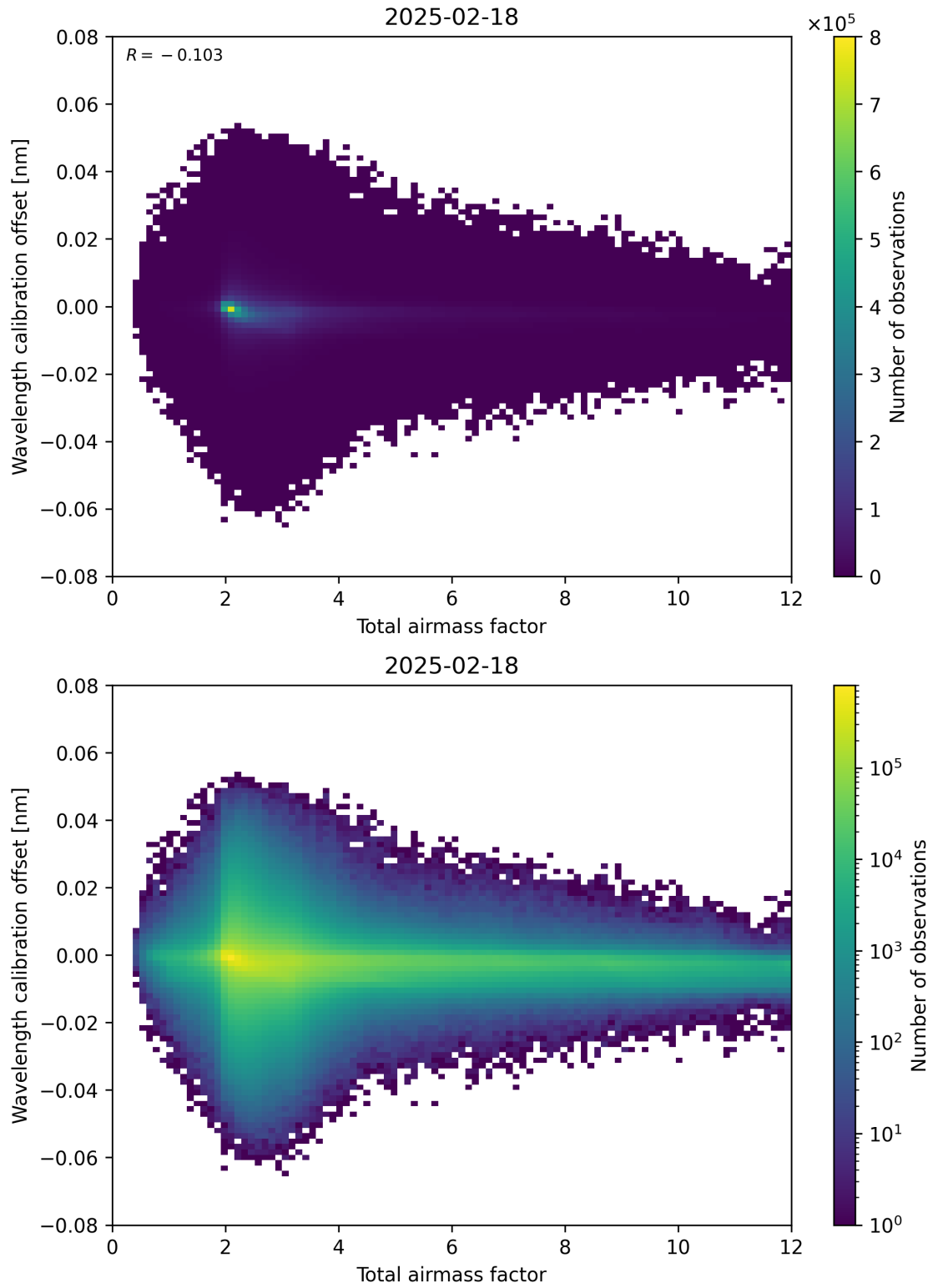
Figure 70: Scatter density plot of “Total airmass factor” against “Wavelength calibration offset” for 2025-02-18 to 2025-02-19.
