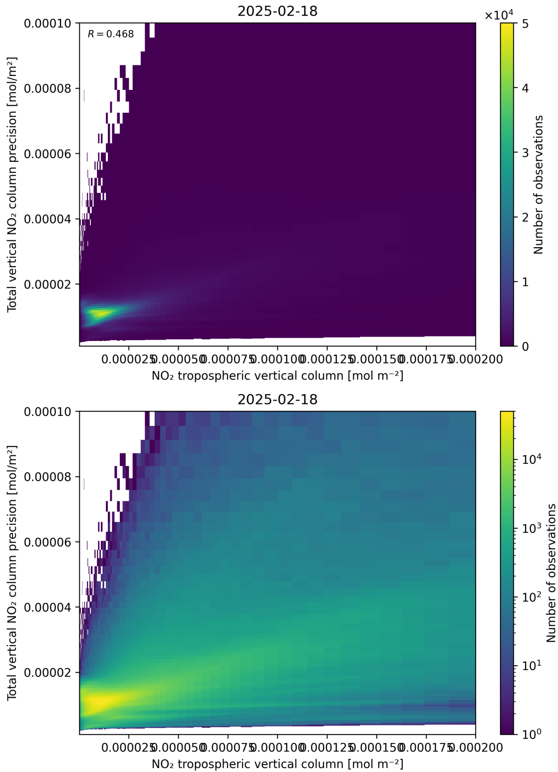
Figure 129: Scatter density plot of “NO 2 tropospheric vertical column” against “Total vertical NO 2 column precision” for 2025-02-18 to 2025-02-19.
