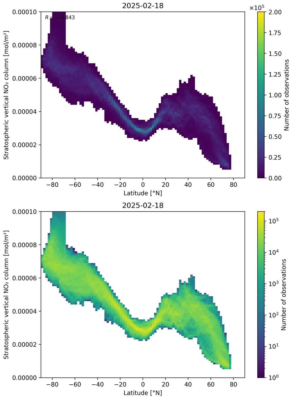
Figure 87: Scatter density plot of “Latitude” against “Stratospheric vertical NO 2 column” for 2025-02-18 to 2025-02-19.
