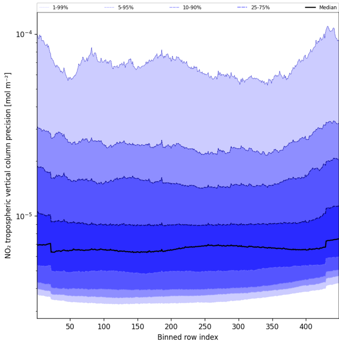
Figure 47: Along track statistics of “NO 2 tropospheric vertical column precision” for 2025-02-18 to 2025-02-19
