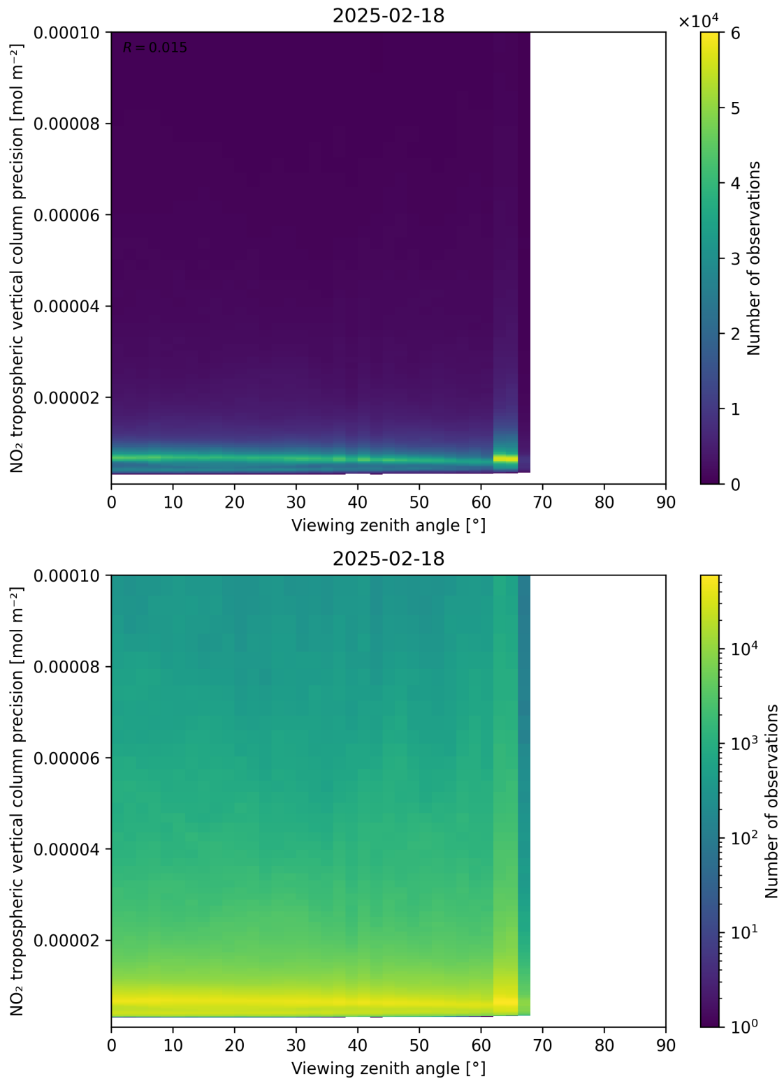
Figure 170: Scatter density plot of “Viewing zenith angle” against “NO 2 tropospheric vertical column precision” for 2025-02-18 to 2025-02-19.
