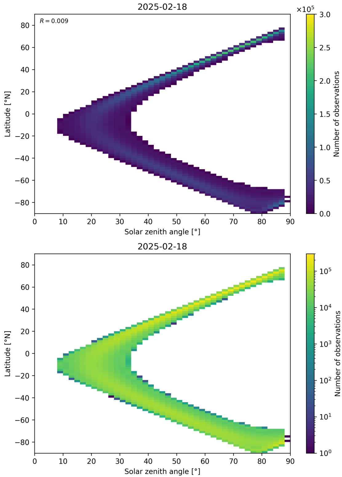
Figure 149: Scatter density plot of “Solar zenith angle” against “Latitude” for 2025-02-18 to 2025-02-19.
