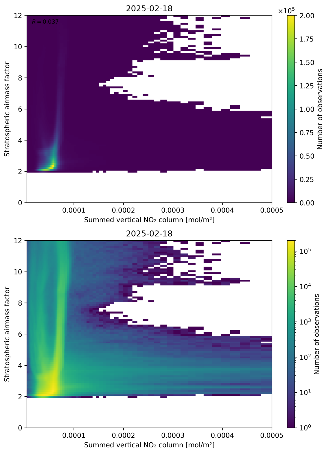
Figure 103: Scatter density plot of “Summed vertical NO 2 column” against “Stratospheric airmass factor” for 2025-02-18 to 2025-02-19.
