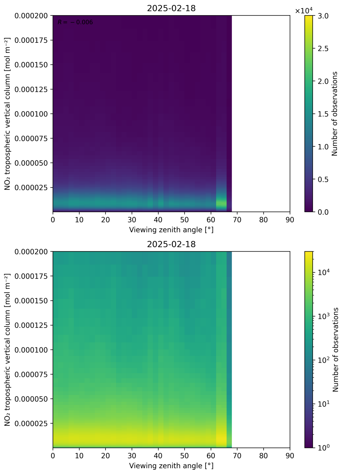
Figure 169: Scatter density plot of “Viewing zenith angle” against “NO 2 tropospheric vertical column” for 2025-02-18 to 2025-02-19.
