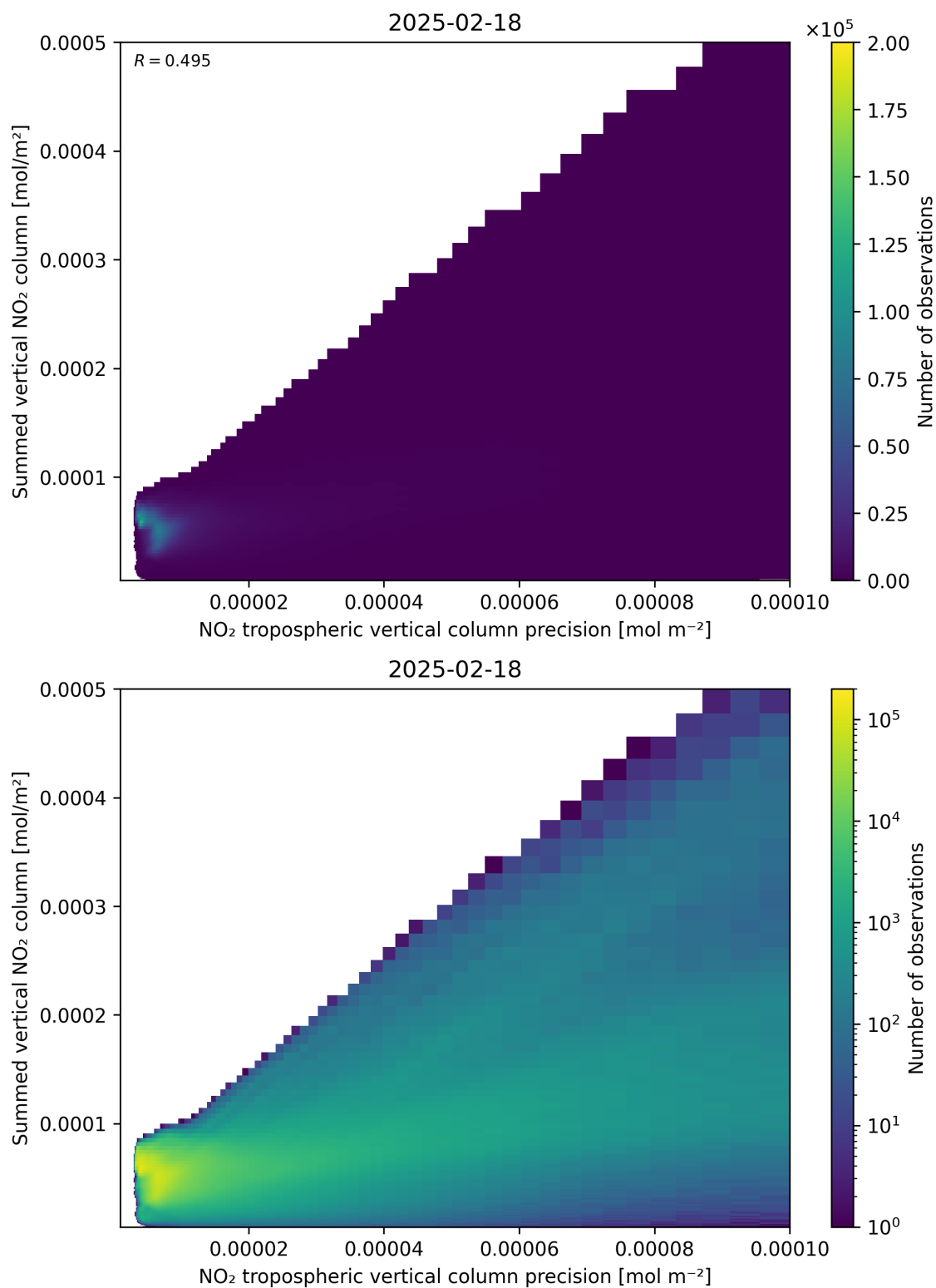
Figure 136: Scatter density plot of “NO 2 tropospheric vertical column precision” against “Summed vertical NO 2 column” for 2025-02-18 to 2025-02-19.
