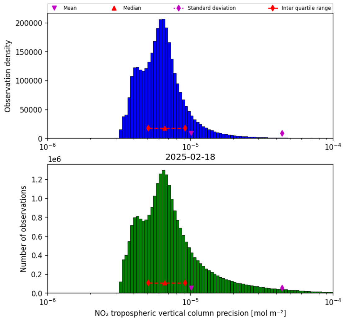
Figure 30: Histogram of “NO 2 tropospheric vertical column precision” for 2025-02-18 to 2025-02-19
