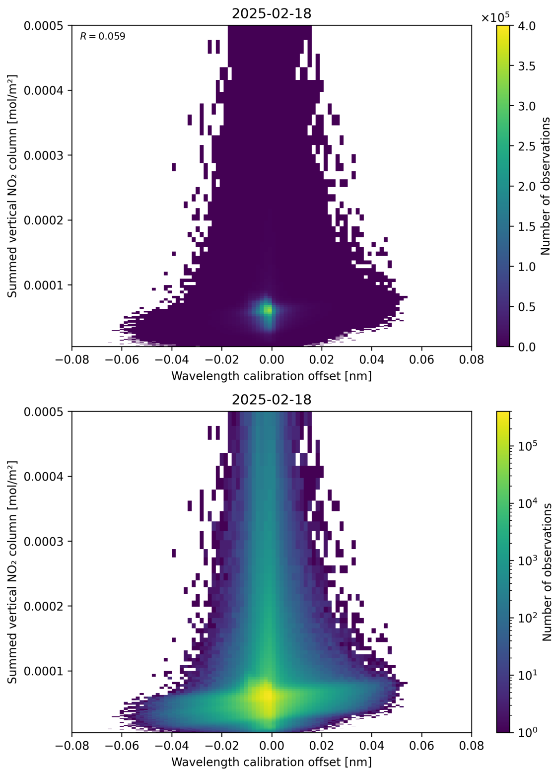
Figure 177: Scatter density plot of “Wavelength calibration offset” against “Summed vertical NO 2 column” for 2025-02-18 to 2025-02-19.
