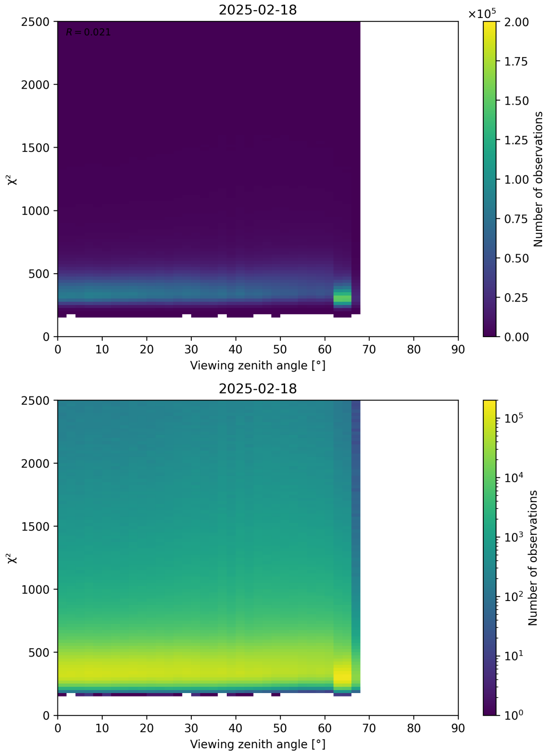
Figure 162: Scatter density plot of “Viewing zenith angle” against “ \chi^2 ” for 2025-02-18 to 2025-02-19.
