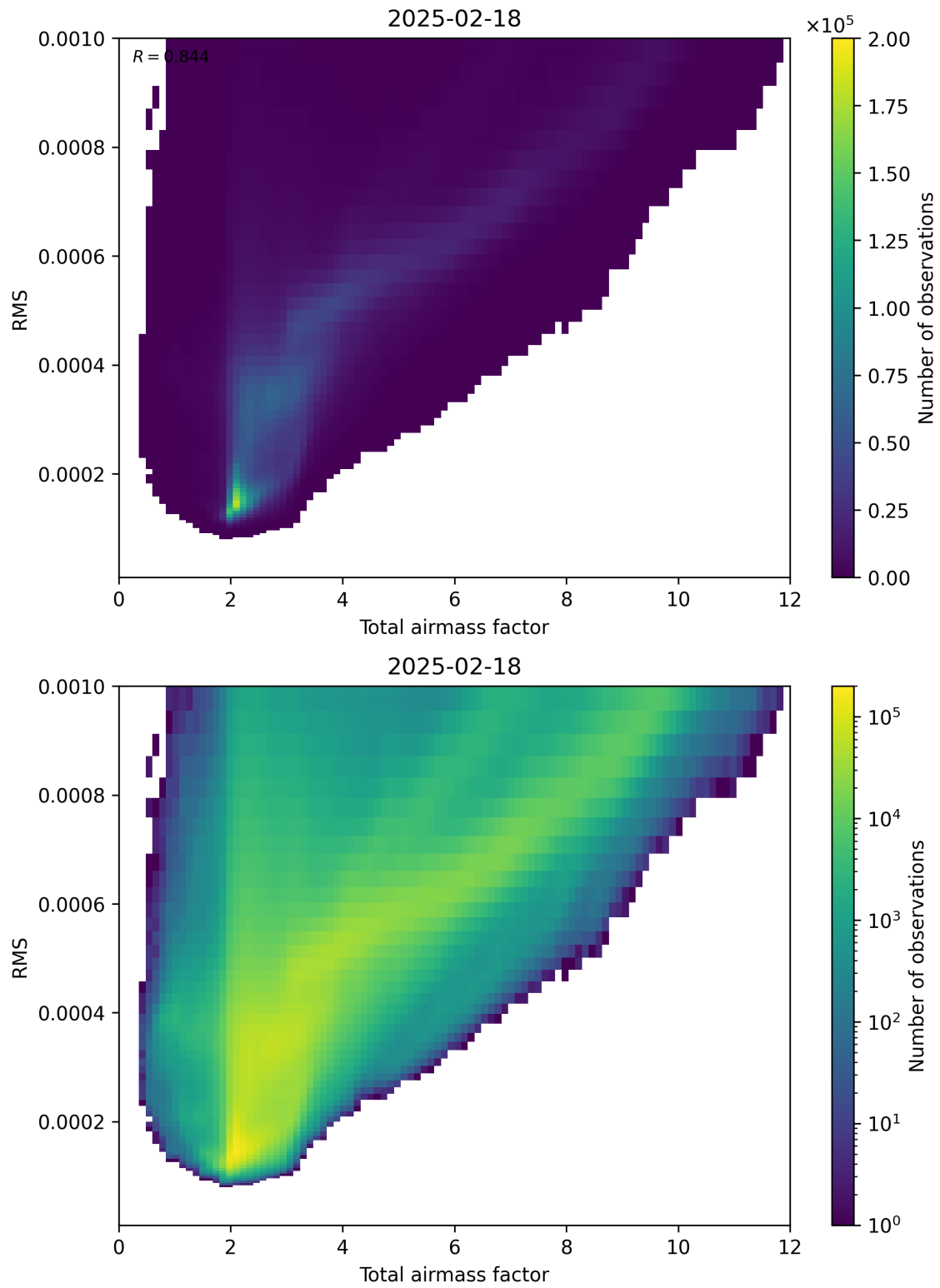
Figure 69: Scatter density plot of “Total airmass factor” against “RMS” for 2025-02-18 to 2025-02-19.
