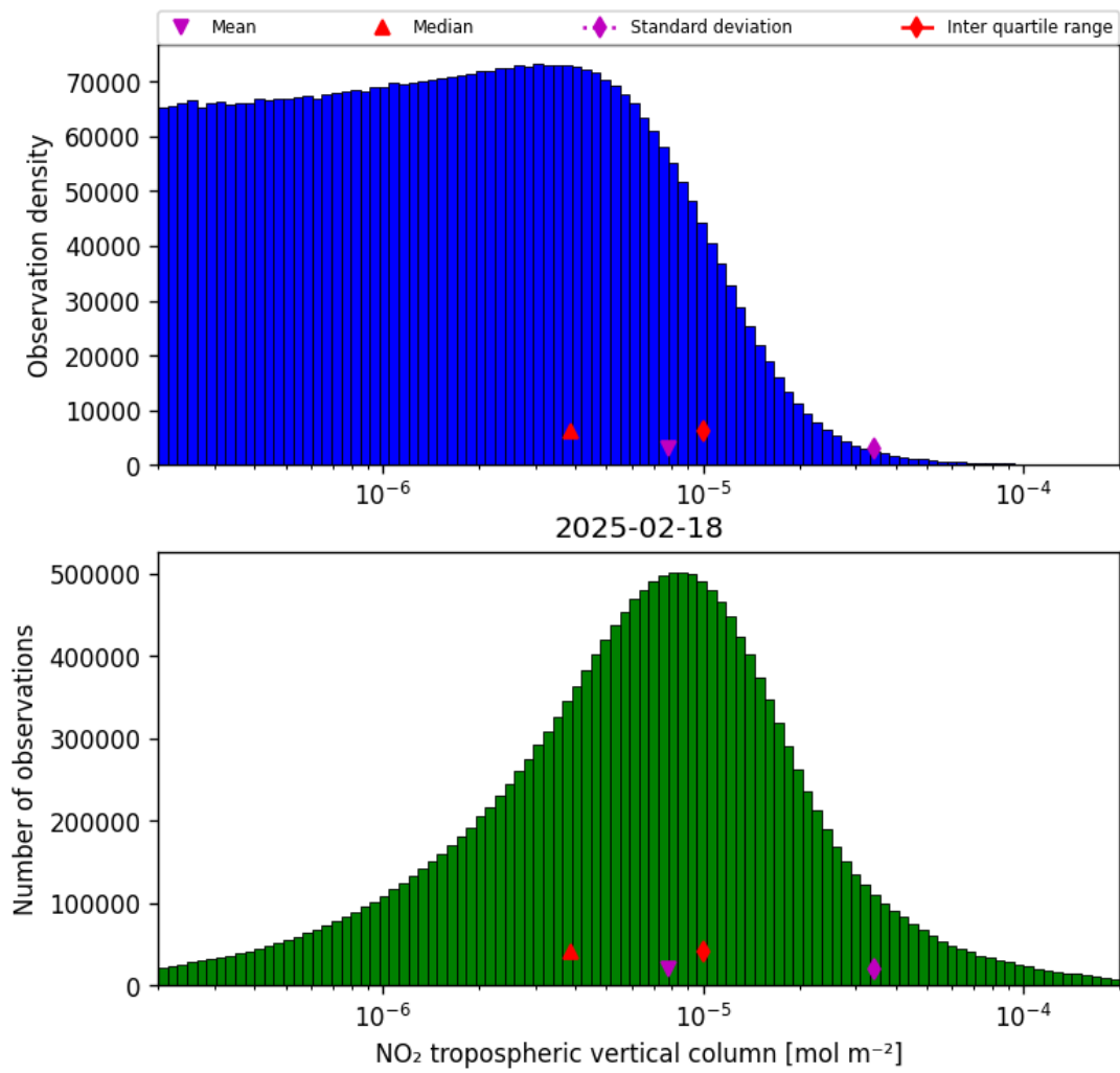
Figure 29: Histogram of “NO 2 tropospheric vertical column” for 2025-02-18 to 2025-02-19
