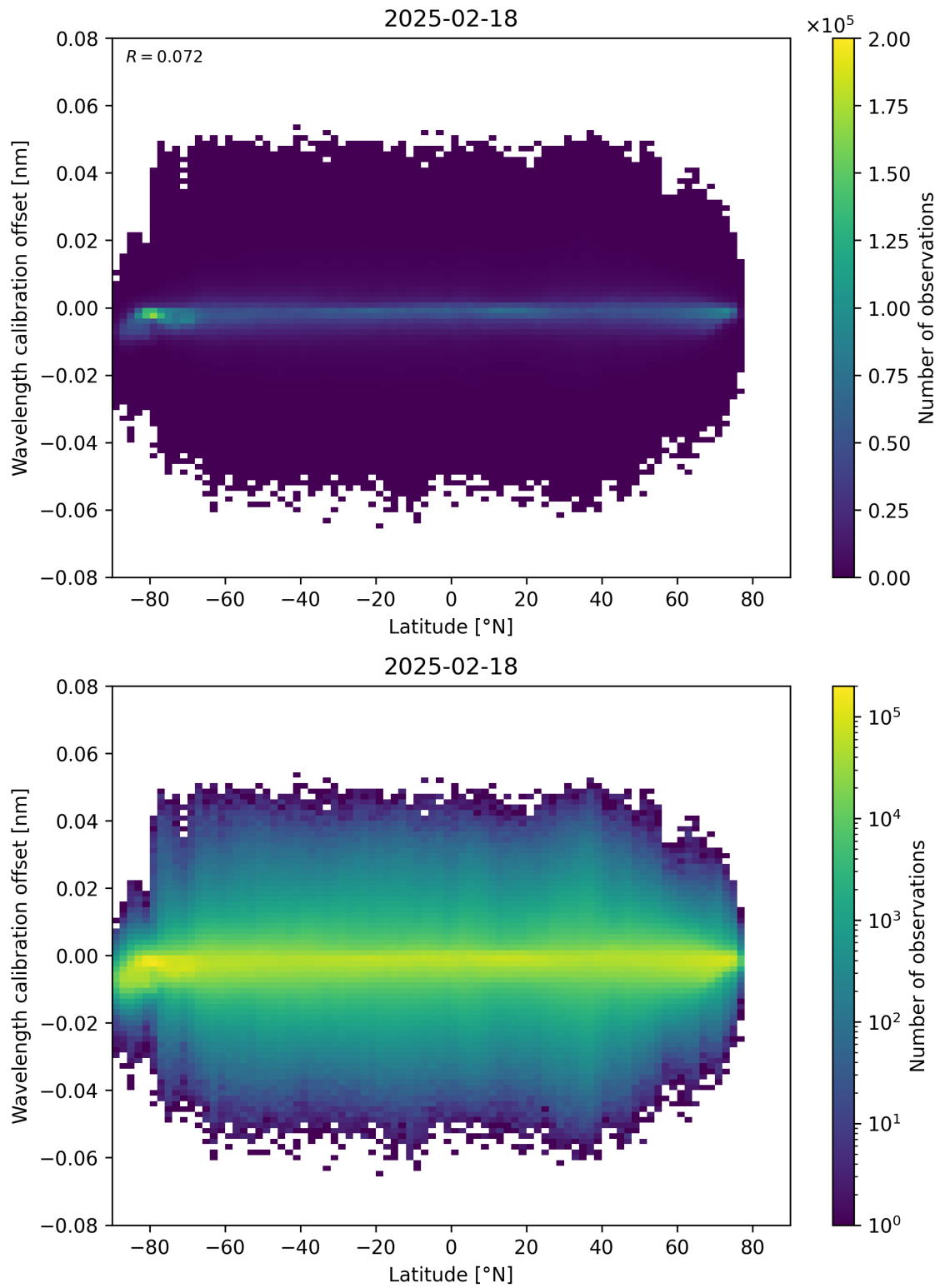
Figure 95: Scatter density plot of “Latitude” against “Wavelength calibration offset” for 2025-02-18 to 2025-02-19.
