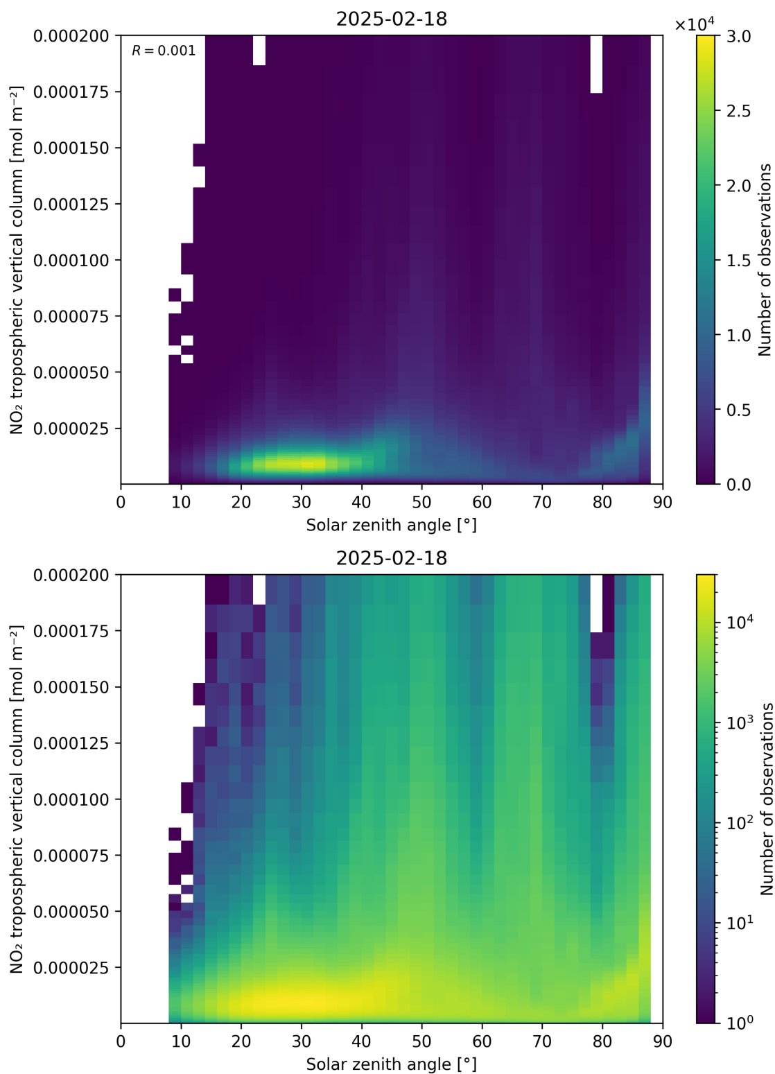
Figure 155: Scatter density plot of “Solar zenith angle” against “NO 2 tropospheric vertical column” for 2025-02-18 to 2025-02-19.
