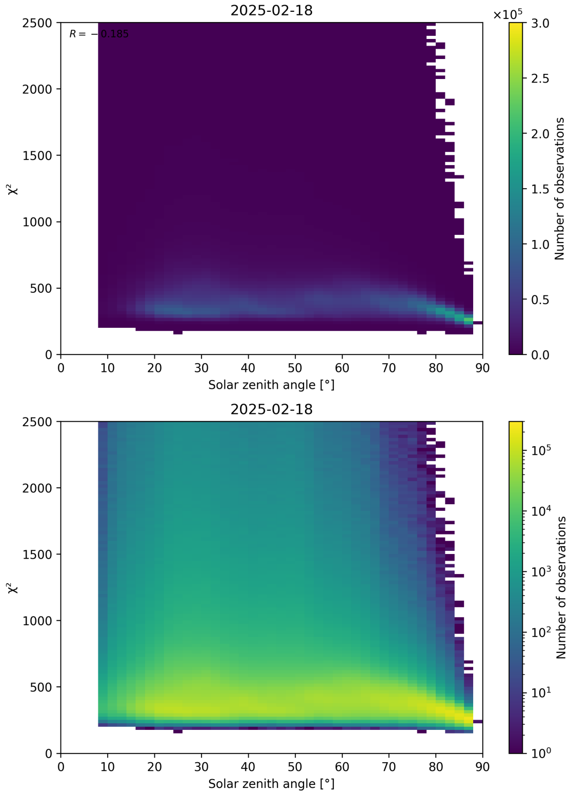
Figure 148: Scatter density plot of “Solar zenith angle” against “ \chi^2 ” for 2025-02-18 to 2025-02-19.
