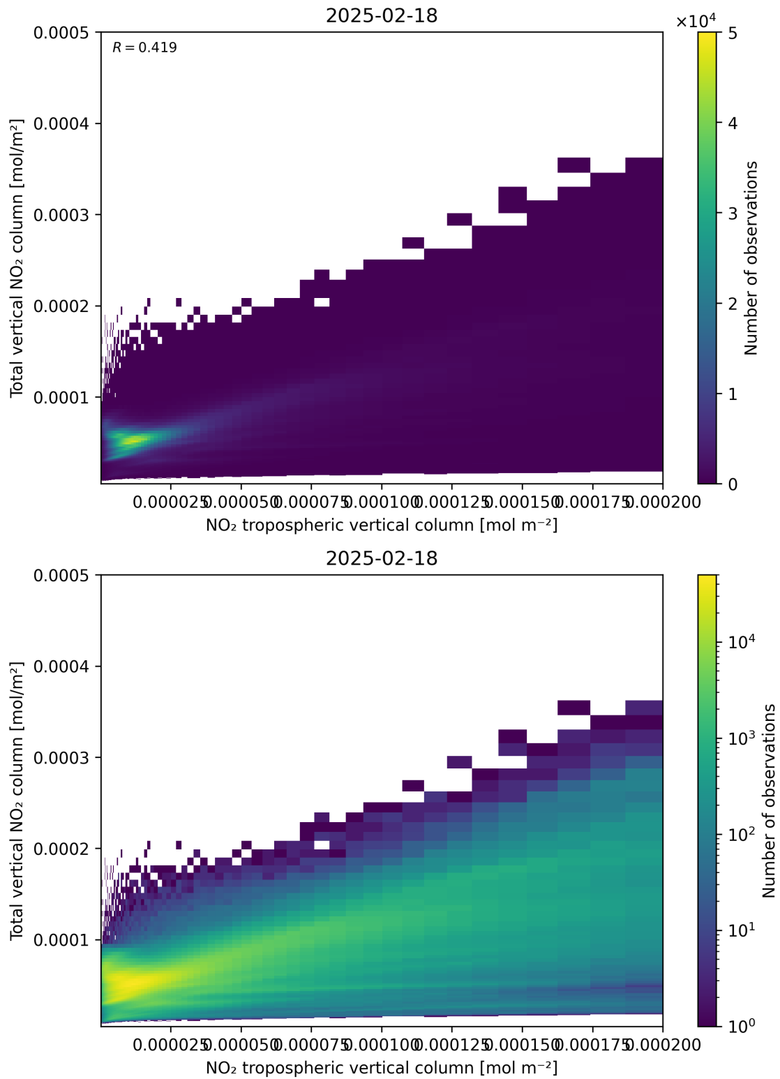
Figure 128: Scatter density plot of “NO 2 tropospheric vertical column” against “Total vertical NO 2 column” for 2025-02-18 to 2025-02-19.
