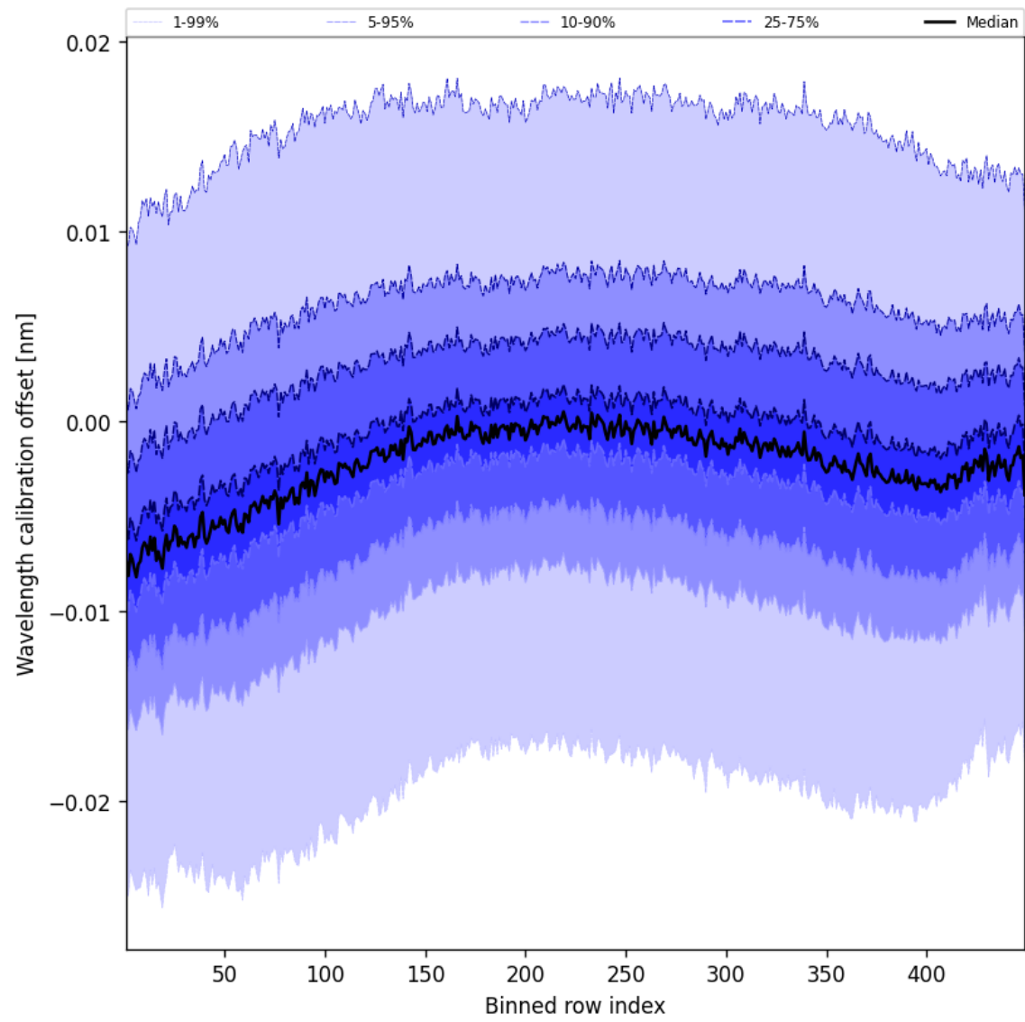
Figure 52: Along track statistics of “Wavelength calibration offset” for 2025-02-18 to 2025-02-19
