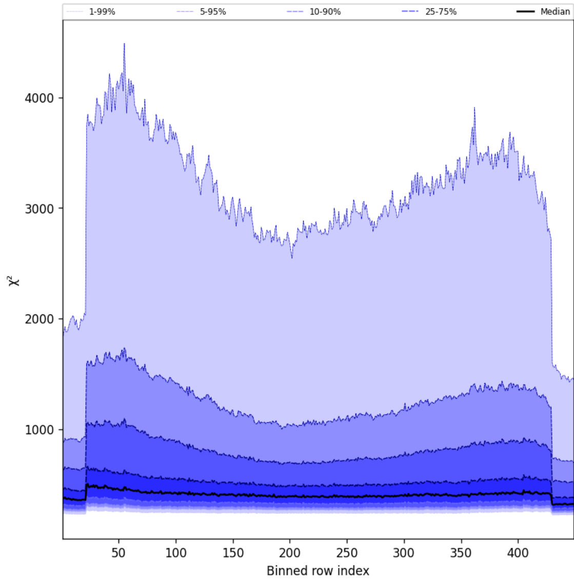
Figure 59: Along track statistics of “ \chi^2 ” for 2025-02-18 to 2025-02-19
