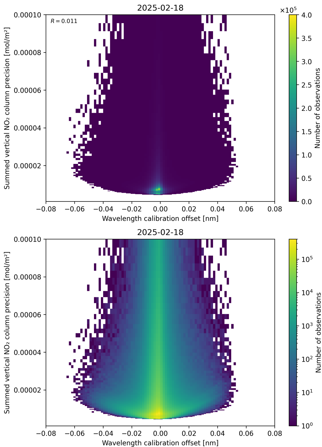
Figure 178: Scatter density plot of “Wavelength calibration offset” against “Summed vertical NO 2 column precision” for 2025-02-18 to 2025-02-19.
