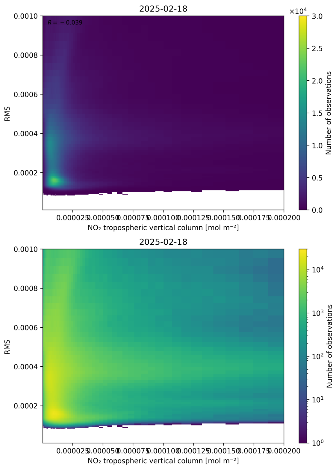
Figure 142: Scatter density plot of “NO 2 tropospheric vertical column” against “RMS” for 2025-02-18 to 2025-02-19.
