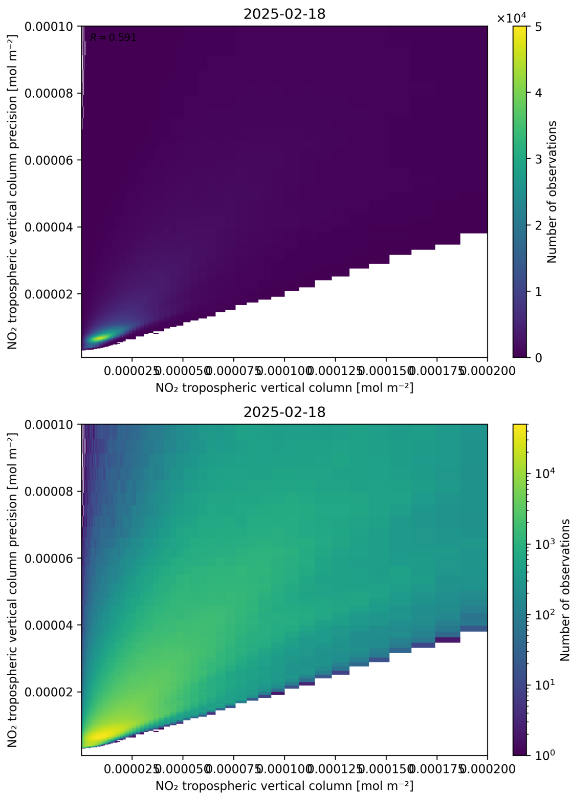
Figure 130: Scatter density plot of “NO 2 tropospheric vertical column” against “NO 2 tropospheric vertical column precision” for 2025-02-18 to 2025-02-19.
