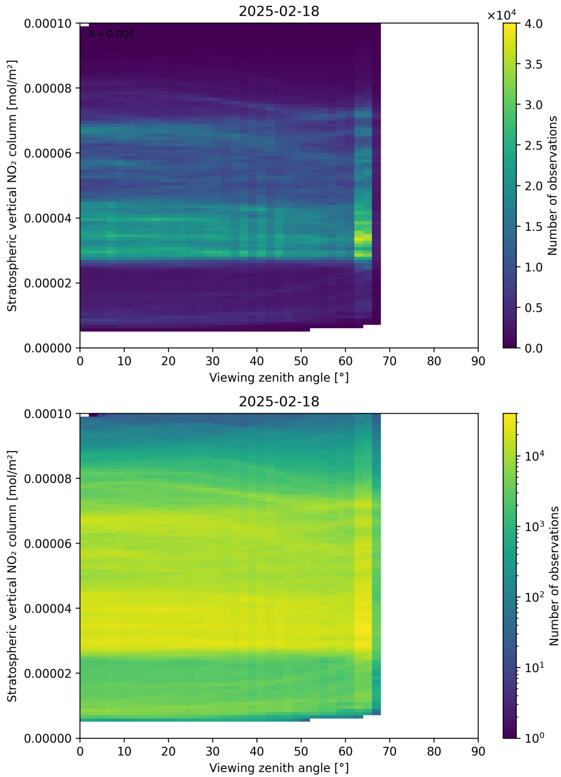
Figure 164: Scatter density plot of “Viewing zenith angle” against “Stratospheric vertical NO 2 column” for 2025-02-18 to 2025-02-19.
