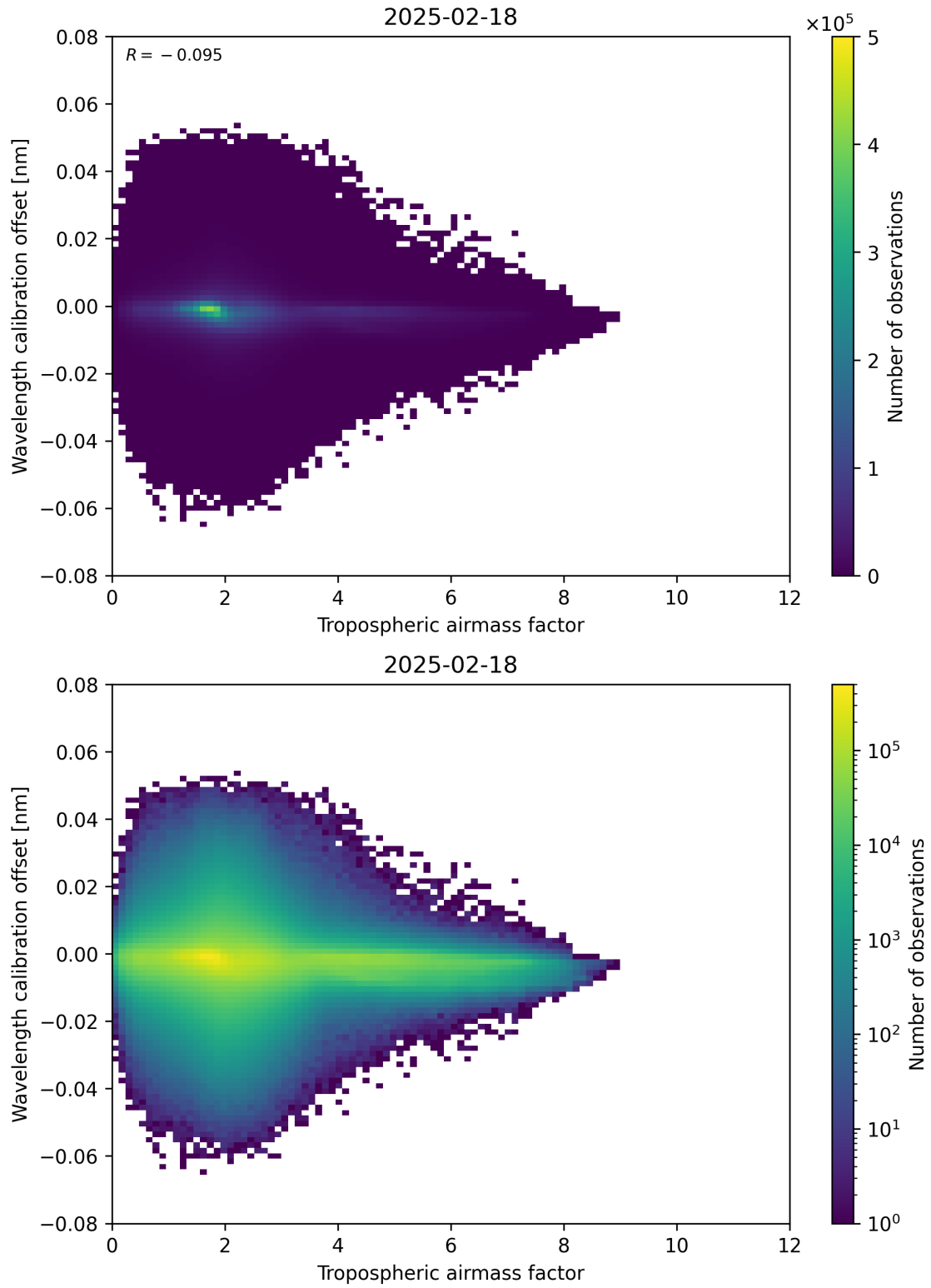
Figure 80: Scatter density plot of “Tropospheric airmass factor” against “Wavelength calibration offset” for 2025-02-18 to 2025-02-19.
