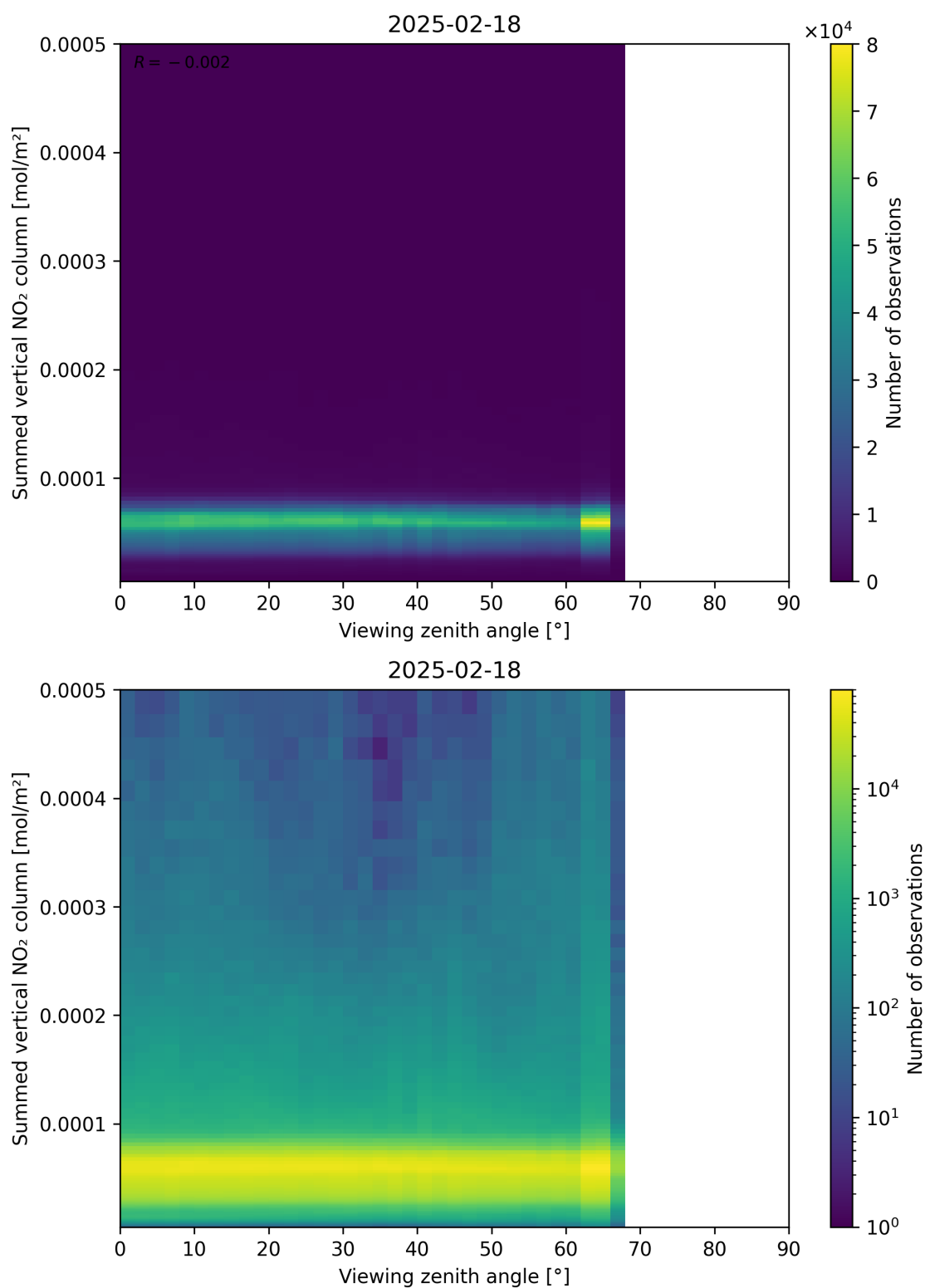
Figure 165: Scatter density plot of “Viewing zenith angle” against “Summed vertical NO 2 column” for 2025-02-18 to 2025-02-19.
