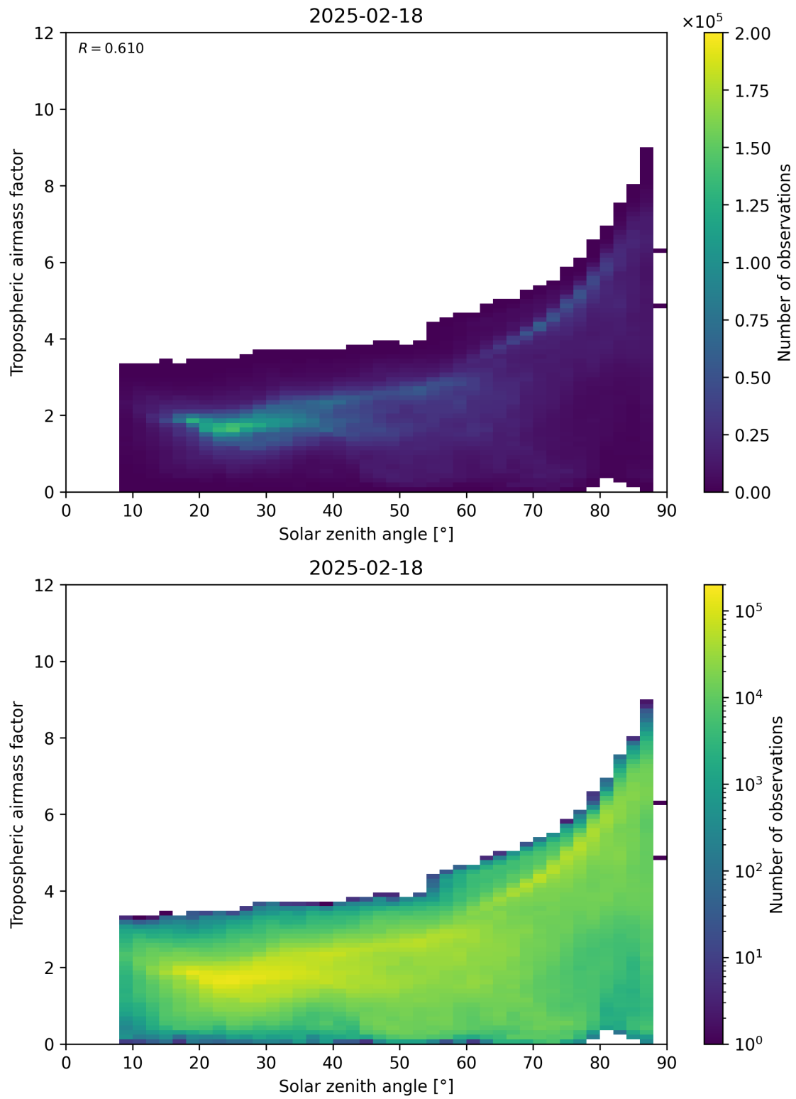
Figure 147: Scatter density plot of “Solar zenith angle” against “Tropospheric airmass factor” for 2025-02-18 to 2025-02-19.
