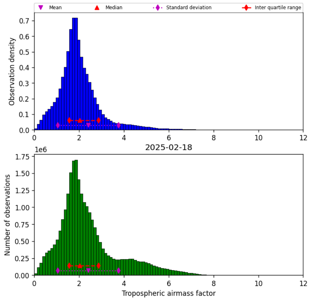
Figure 31: Histogram of “Tropospheric airmass factor” for 2025-02-18 to 2025-02-19
