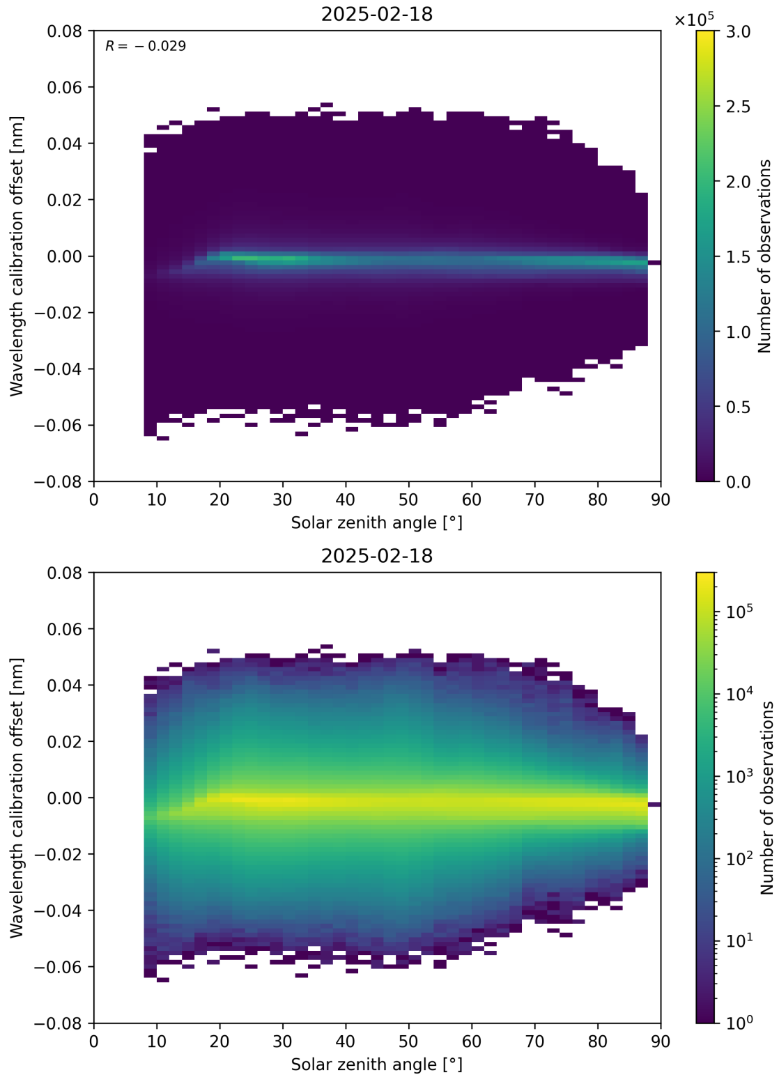
Figure 158: Scatter density plot of “Solar zenith angle” against “Wavelength calibration offset” for 2025-02-18 to 2025-02-19.
