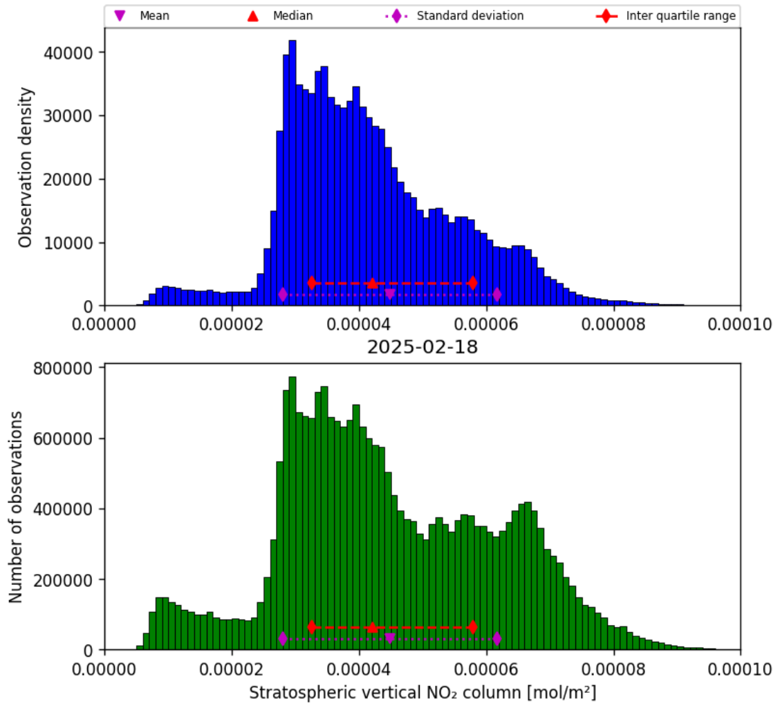
Figure 36: Histogram of “Stratospheric vertical NO 2 column” for 2025-02-18 to 2025-02-19
