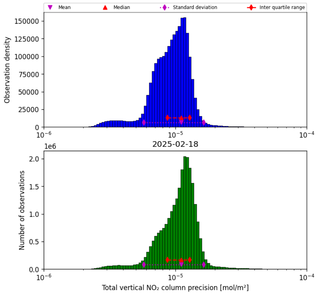
Figure 39: Histogram of “Total vertical NO 2 column precision” for 2025-02-18 to 2025-02-19
