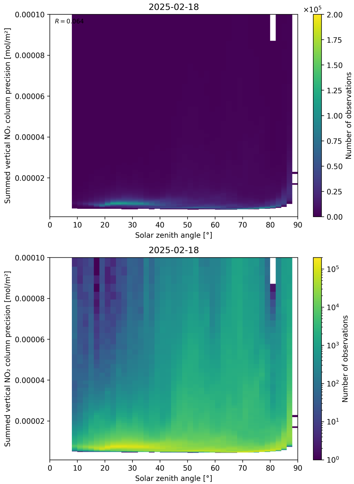
Figure 152: Scatter density plot of “Solar zenith angle” against “Summed vertical NO 2 column precision” for 2025-02-18 to 2025-02-19.
