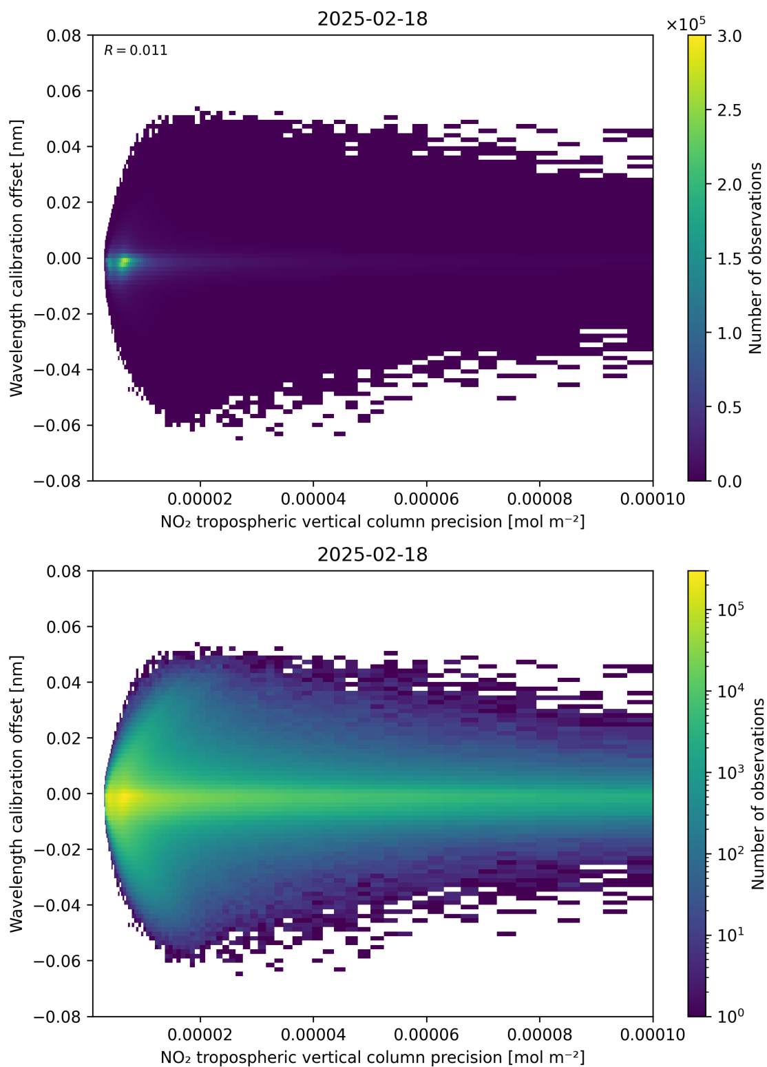
Figure 141: Scatter density plot of “NO 2 tropospheric vertical column precision” against “Wavelength calibration offset” for 2025-02-18 to 2025-02-19.
