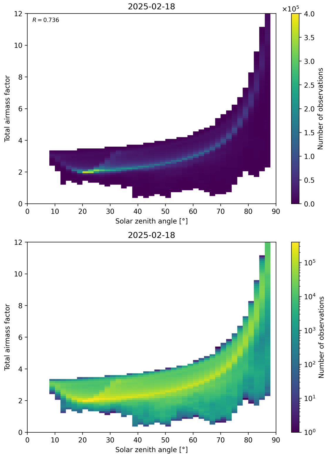
Figure 146: Scatter density plot of “Solar zenith angle” against “Total air mass factor” for 2025-02-18 to 2025-02-19.
