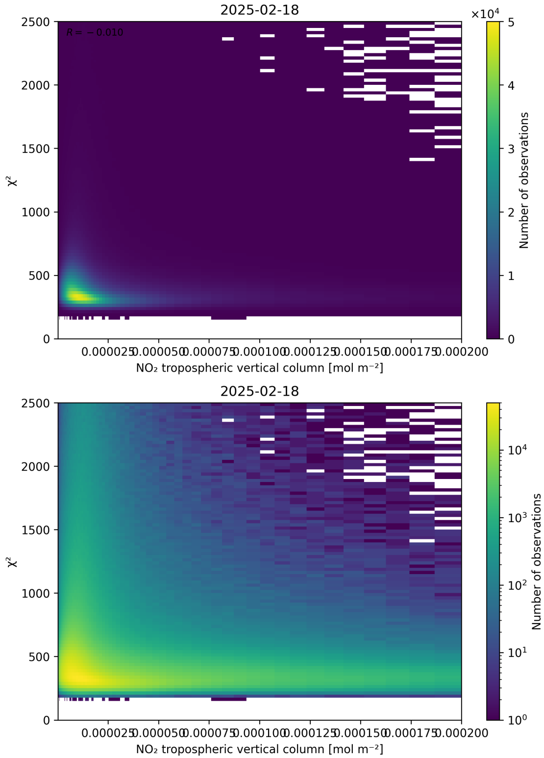
Figure 124: Scatter density plot of “NO 2 tropospheric vertical column” against “ \chi^2 ” for 2025-02-18 to 2025-02-19.
