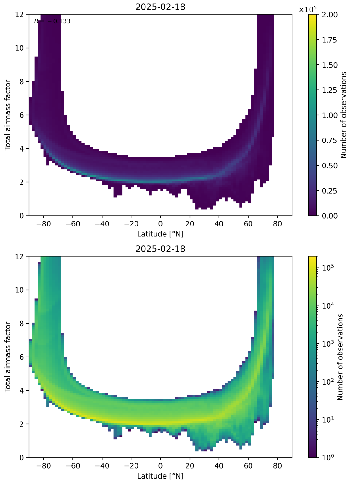
Figure 84: Scatter density plot of “Latitude” against “Total airmass factor” for 2025-02-18 to 2025-02-19.
