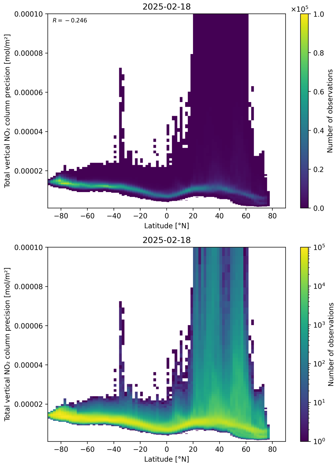
Figure 91: Scatter density plot of “Latitude” against “Total vertical NO 2 column precision” for 2025-02-18 to 2025-02-19.
