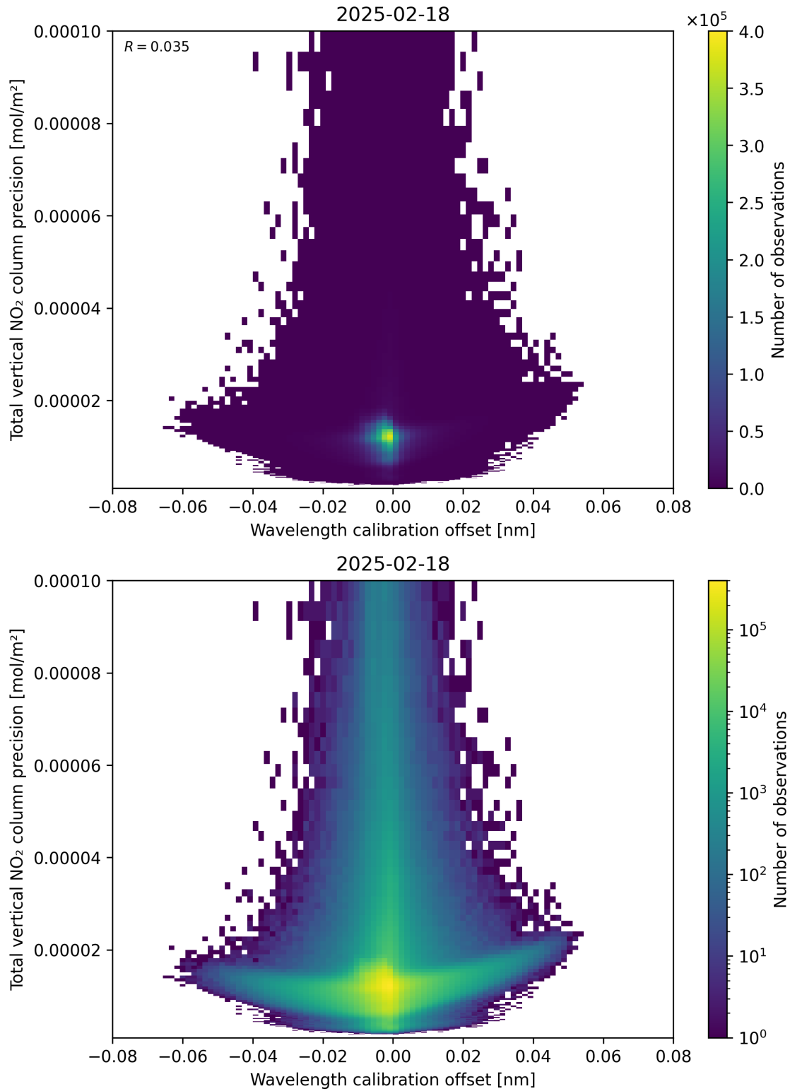
Figure 180: Scatter density plot of “Wavelength calibration offset” against “Total vertical NO 2 column precision” for 2025-02-18 to 2025-02-19.
