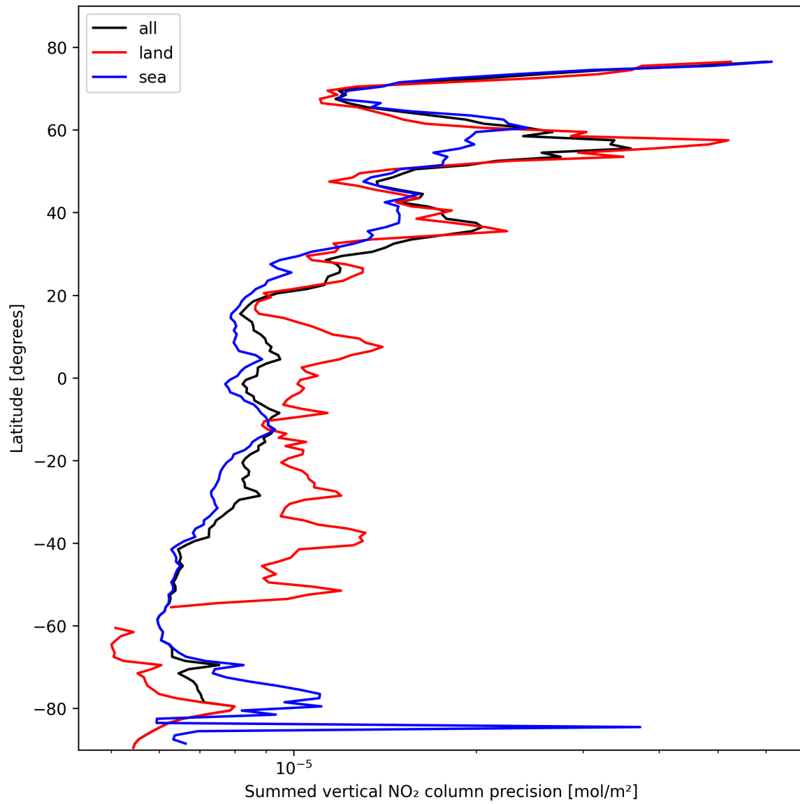
Figure 24: Zonal average of “Summed vertical NO 2 column precision” for 2025-02-18 to 2025-02-19.
