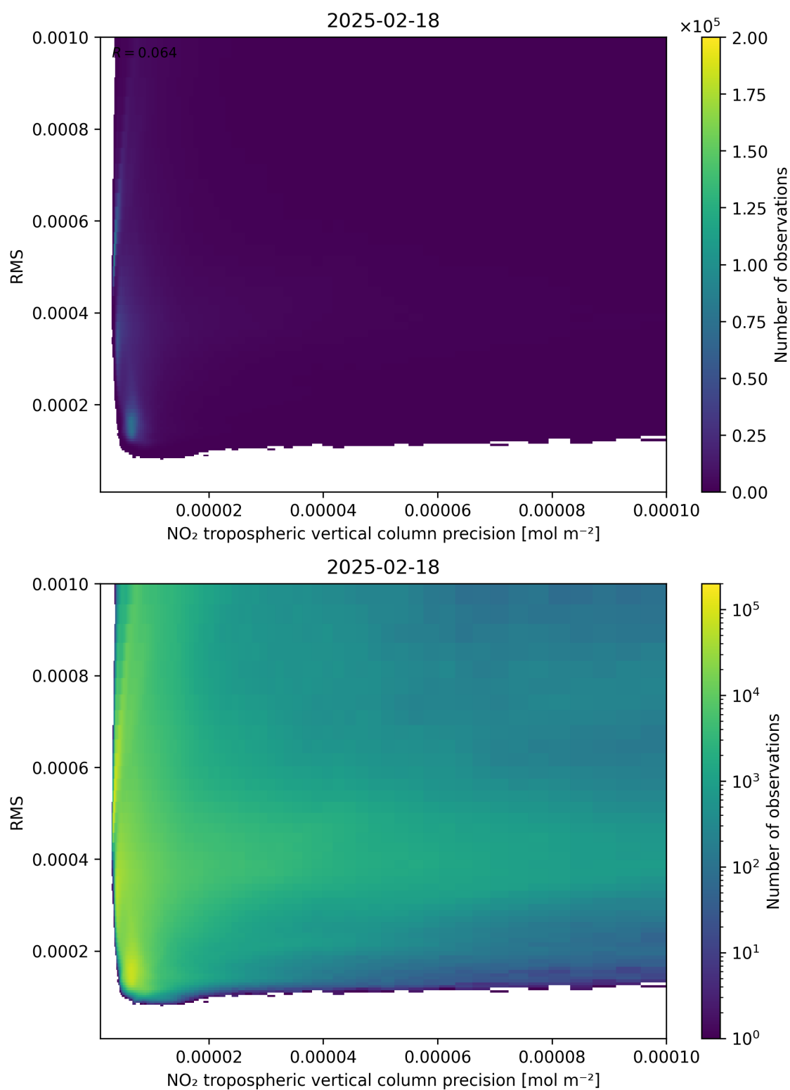
Figure 140: Scatter density plot of “NO 2 tropospheric vertical column precision” against “RMS” for 2025-02-18 to 2025-02-19.
