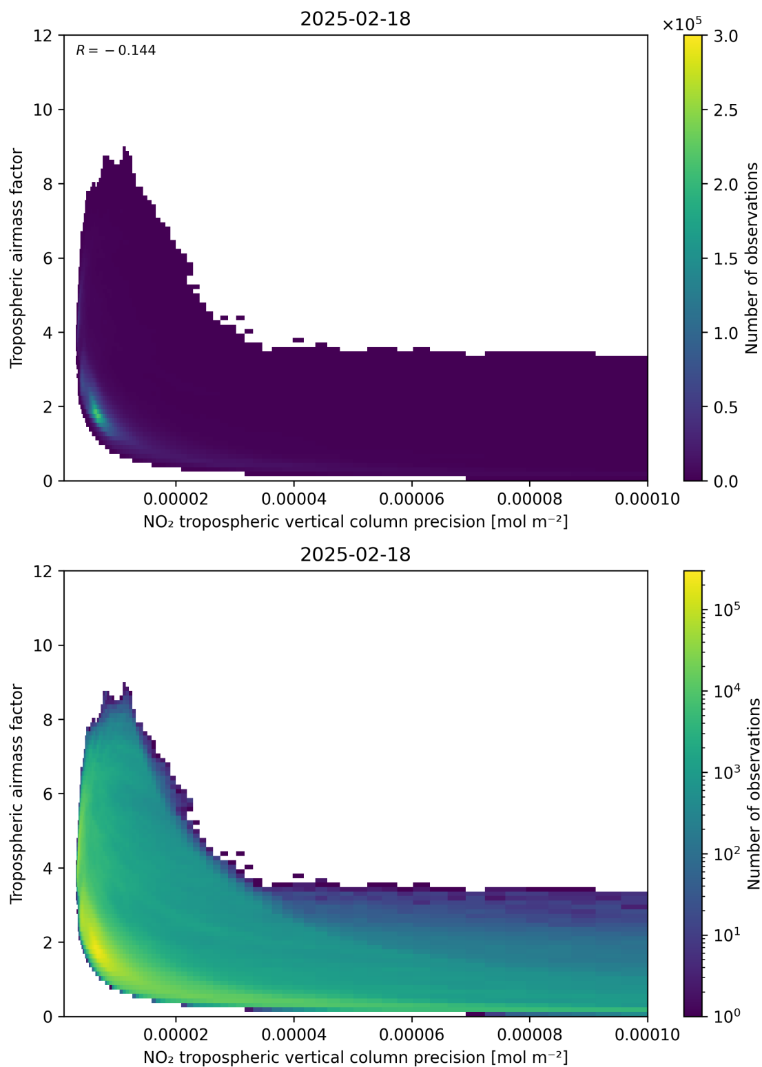
Figure 133: Scatter density plot of “NO 2 tropospheric vertical column precision” against “Tropospheric airmass factor” for 2025-02-18 to 2025-02-19.
