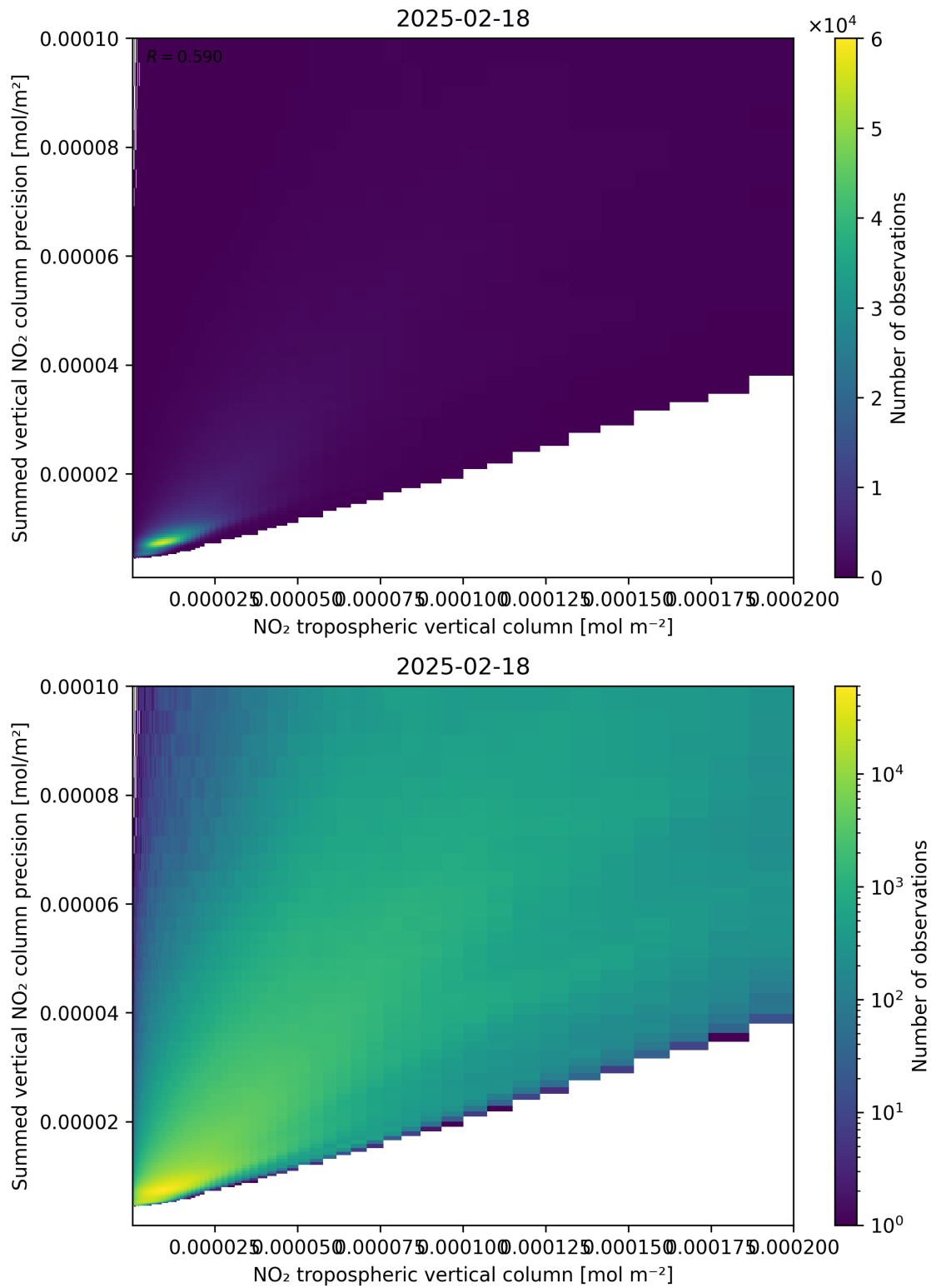
Figure 127: Scatter density plot of “NO 2 tropospheric vertical column” against “Summed vertical NO 2 column precision” for 2025-02-18 to 2025-02-19.
