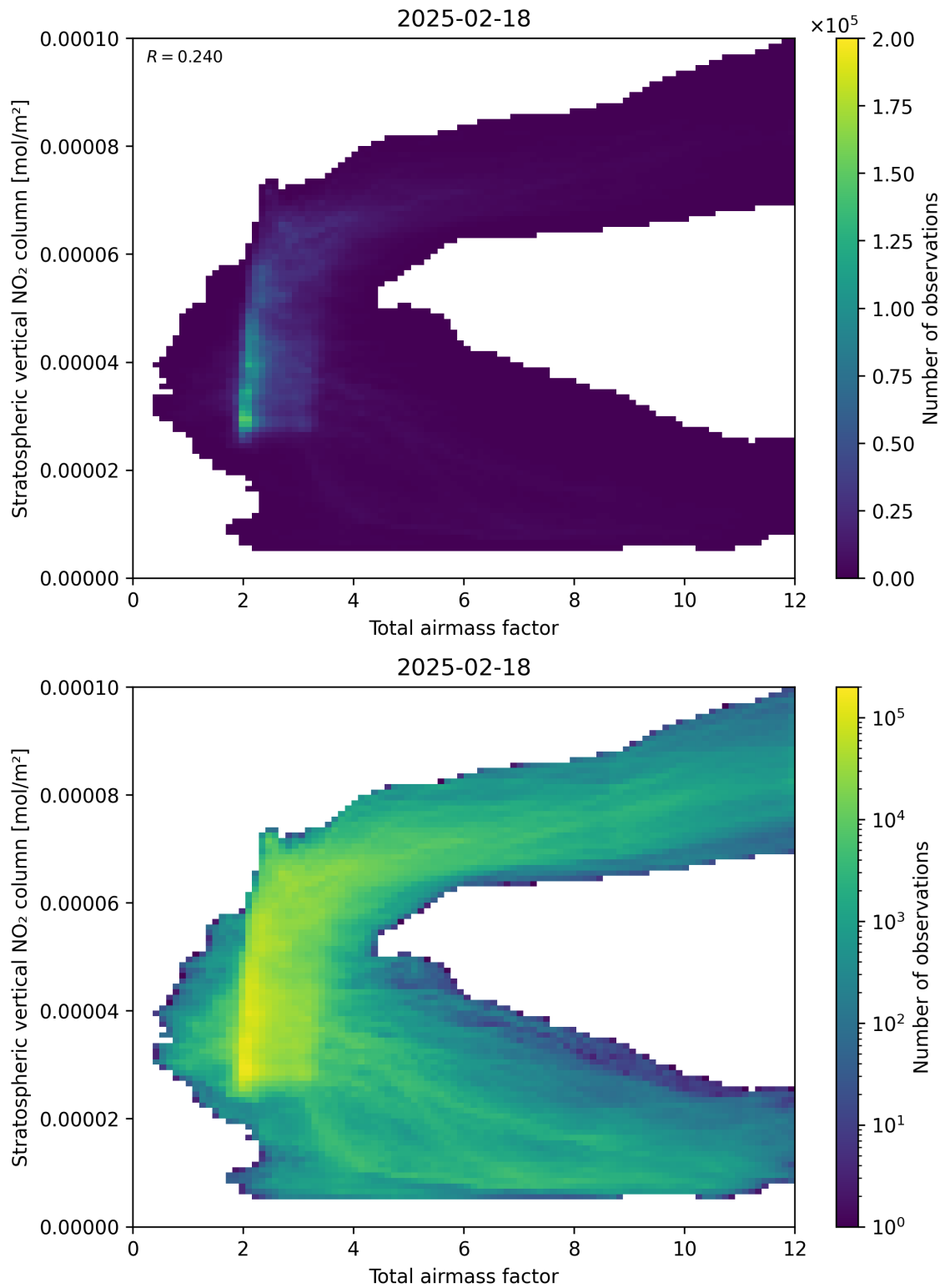
Figure 64: Scatter density plot of “Total airmass factor” against “Stratospheric vertical \text{NO}_2 column” for 2025-02-18 to 2025-02-19.
