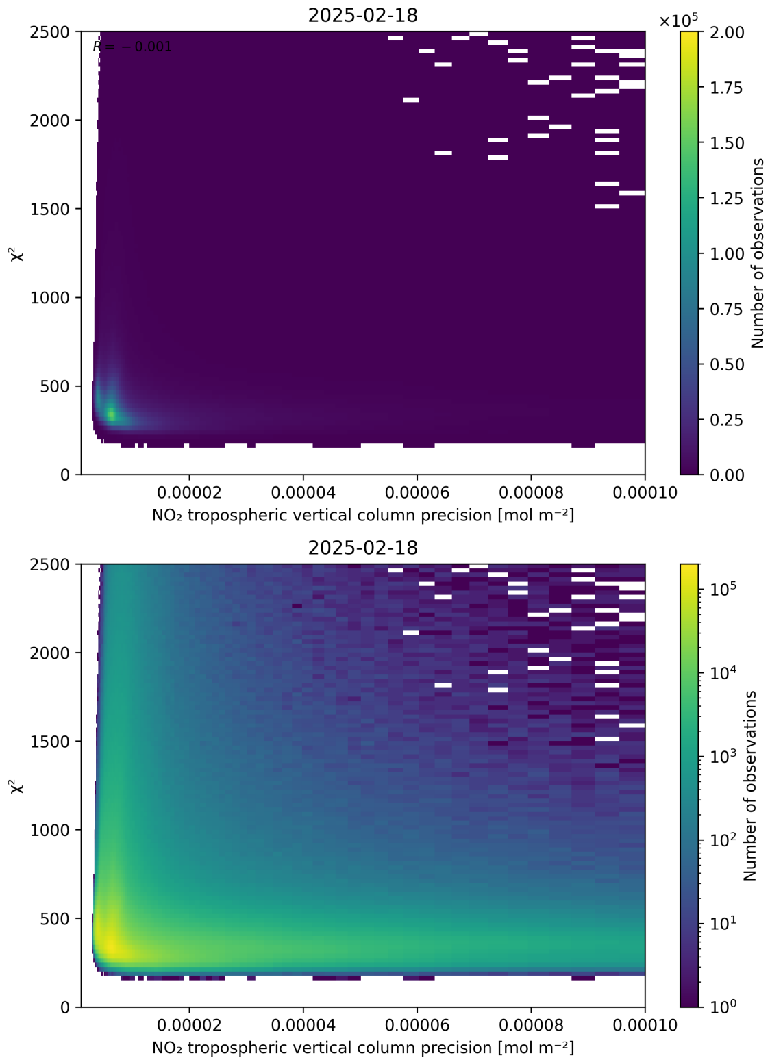
Figure 134: Scatter density plot of “NO 2 tropospheric vertical column precision” against “ \chi^2 ” for 2025-02-18 to 2025-02-19.
