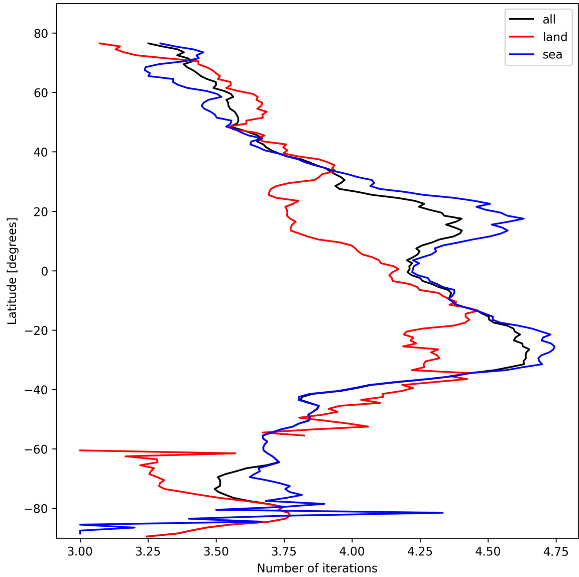
Figure 17: Zonal average of “Number of iterations” for 2025-02-18 to 2025-02-19.
