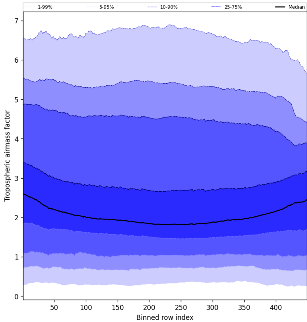
Figure 48: Along track statistics of “Tropospheric airmass factor” for 2025-02-18 to 2025-02-19
