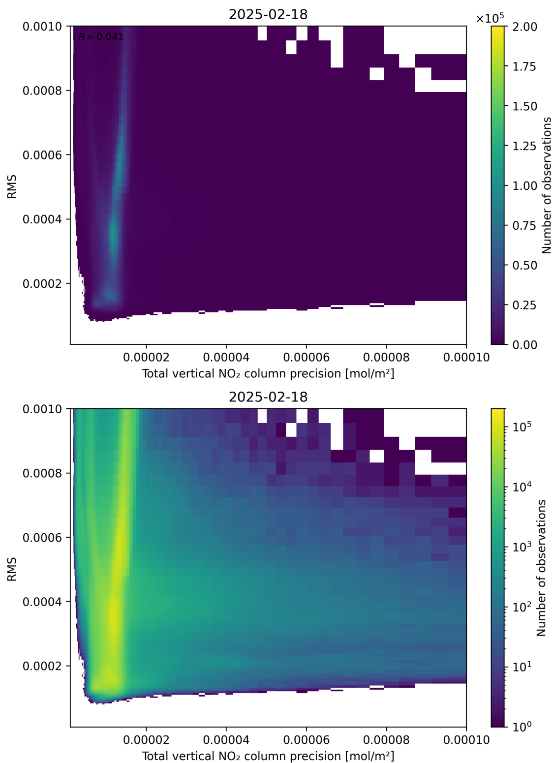
Figure 119: Scatter density plot of “Total vertical NO 2 column precision” against “RMS” for 2025-02-18 to 2025-02-19.
