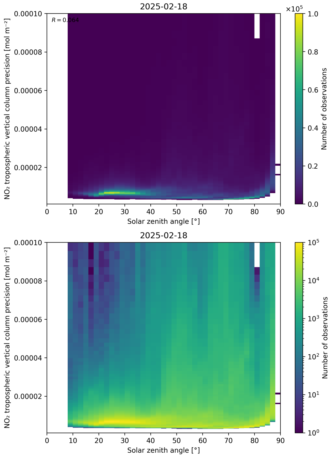
Figure 156: Scatter density plot of “Solar zenith angle” against “NO 2 tropospheric vertical column precision” for 2025-02-18 to 2025-02-19.
