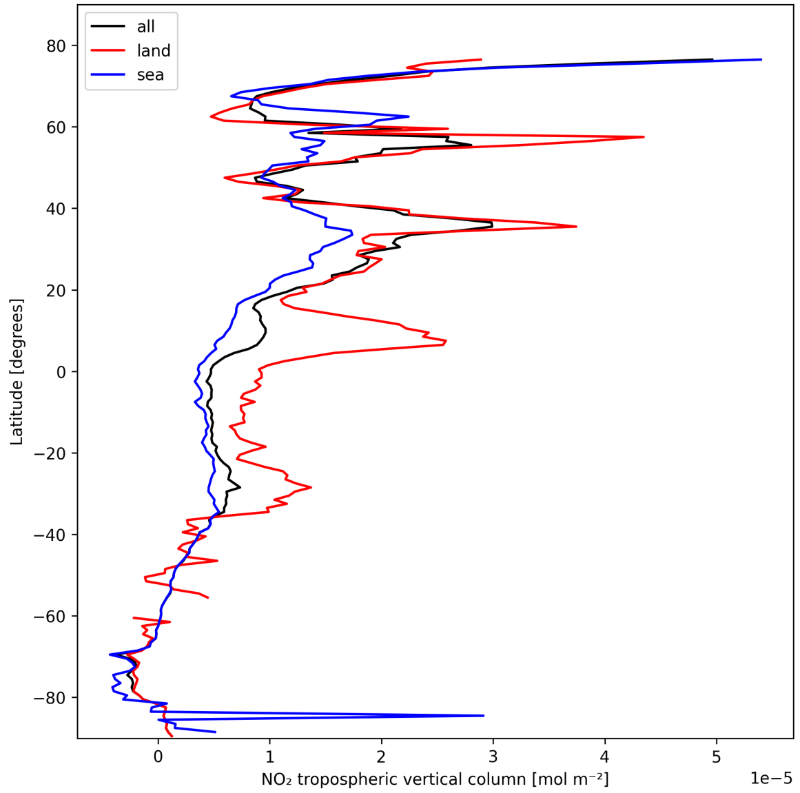
Figure 12: Zonal average of “NO 2 tropospheric vertical column” for 2025-02-18 to 2025-02-19.
