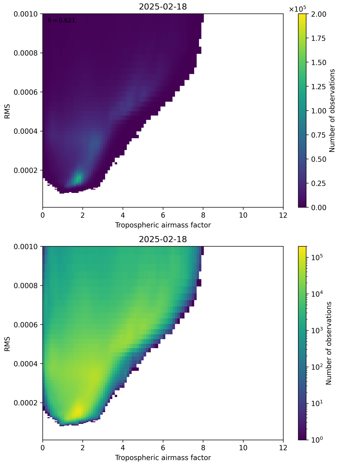
Figure 79: Scatter density plot of “Tropospheric airmass factor” against “RMS” for 2025-02-18 to 2025-02-19.
