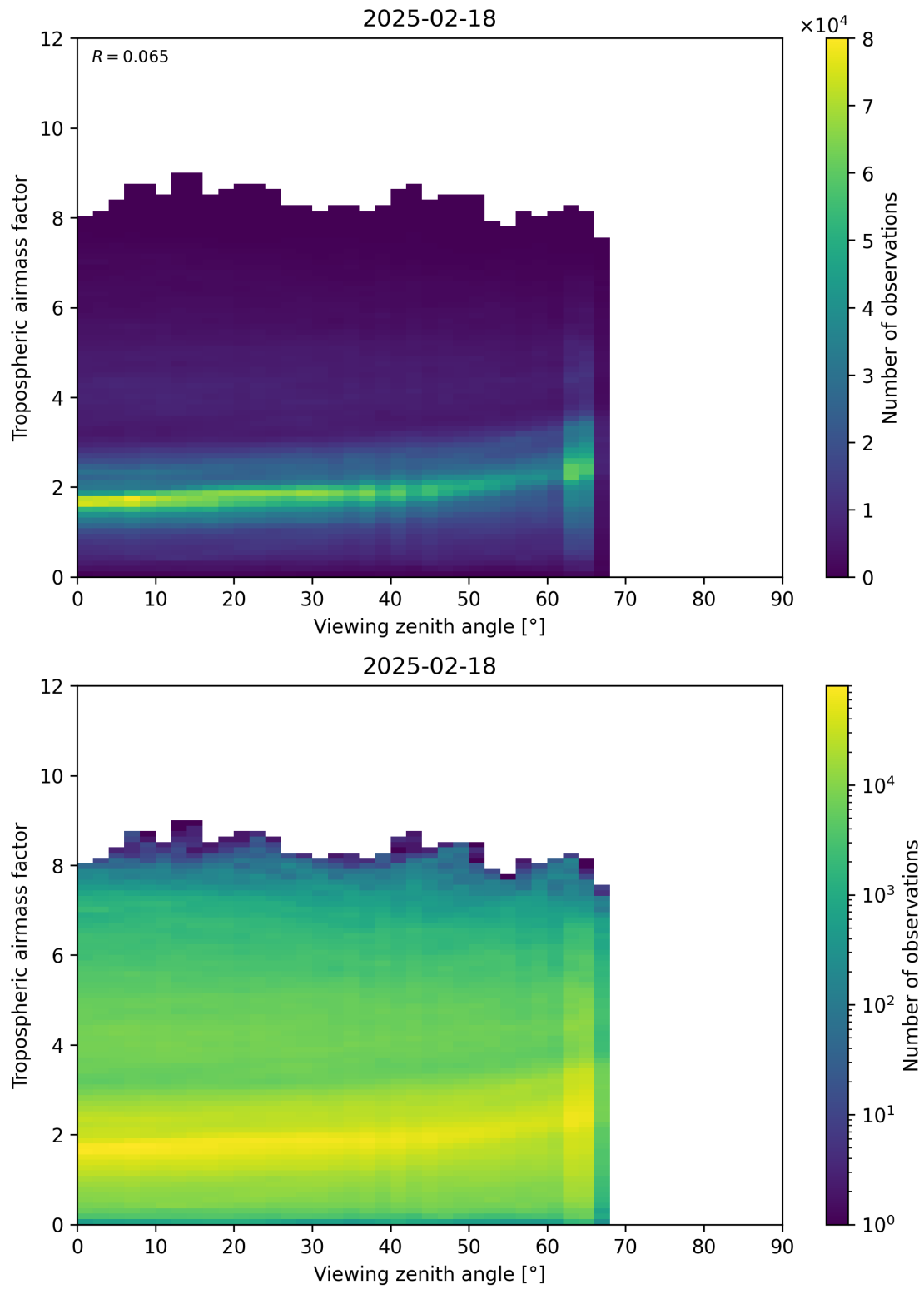
Figure 161: Scatter density plot of “Viewing zenith angle” against “Tropospheric airmass factor” for 2025-02-18 to 2025-02-19.
