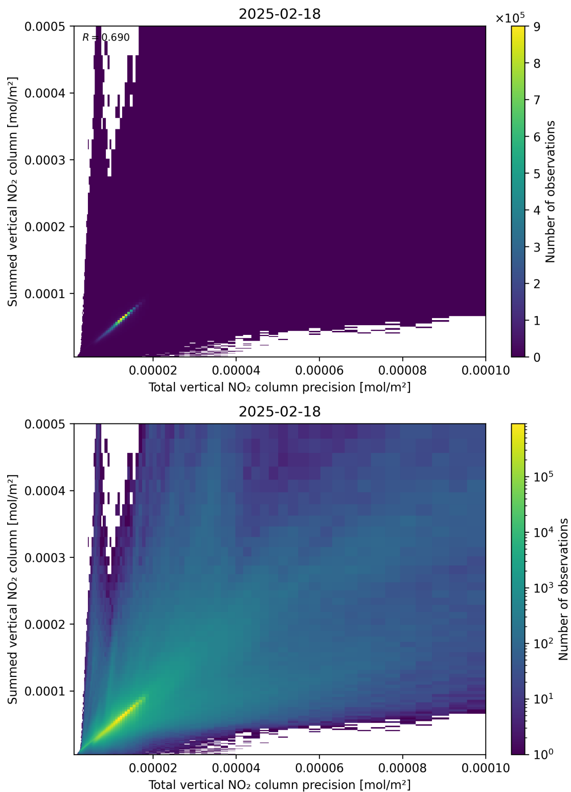
Figure 117: Scatter density plot of “Total vertical NO 2 column precision” against “Summed vertical NO 2 column” for 2025-02-18 to 2025-02-19.
