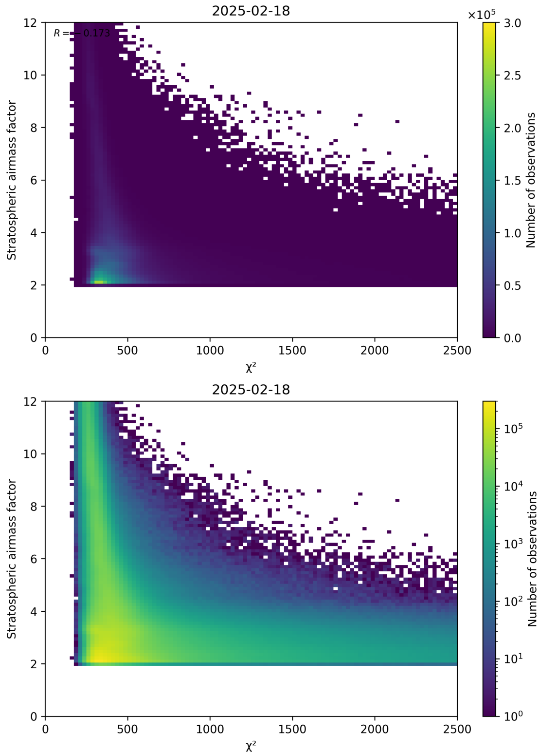
Figure 81: Scatter density plot of “ \chi^2 ” against “Stratospheric airmass factor” for 2025-02-18 to 2025-02-19.
