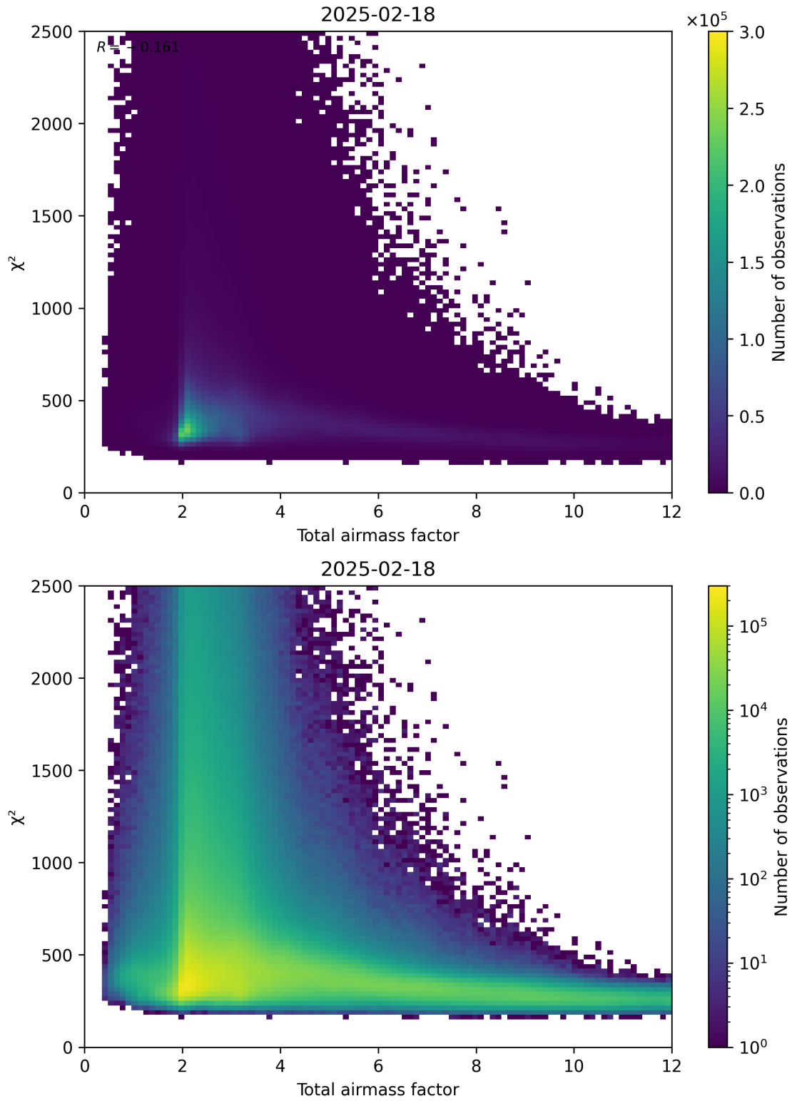
Figure 63: Scatter density plot of “Total airmass factor” against “ \chi^2 ” for 2025-02-18 to 2025-02-19.
