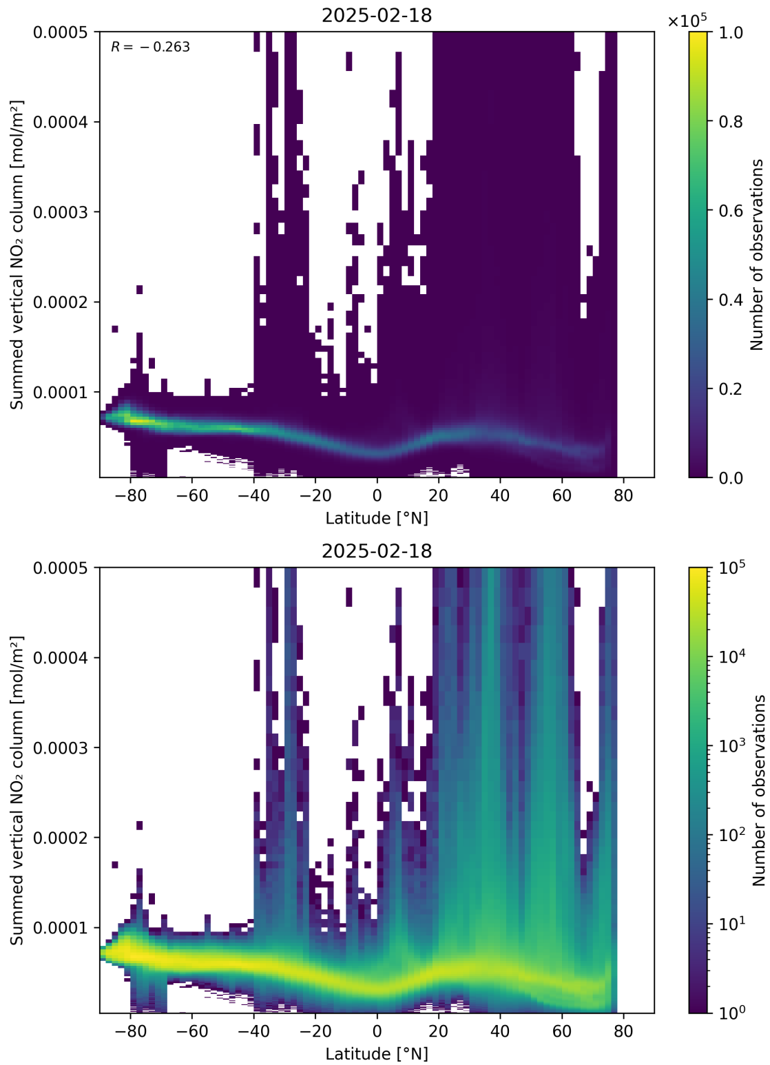
Figure 88: Scatter density plot of “Latitude” against “Summed vertical NO 2 column” for 2025-02-18 to 2025-02-19.
