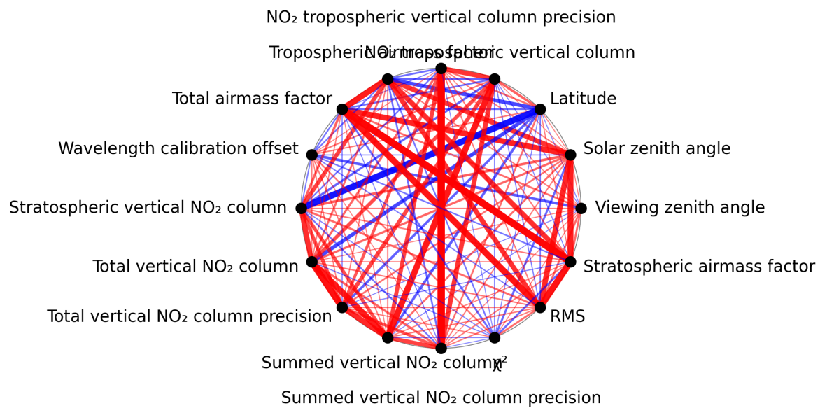
Figure 1: Map of correlation graph for 2025-02-18 to 2025-02-19.
