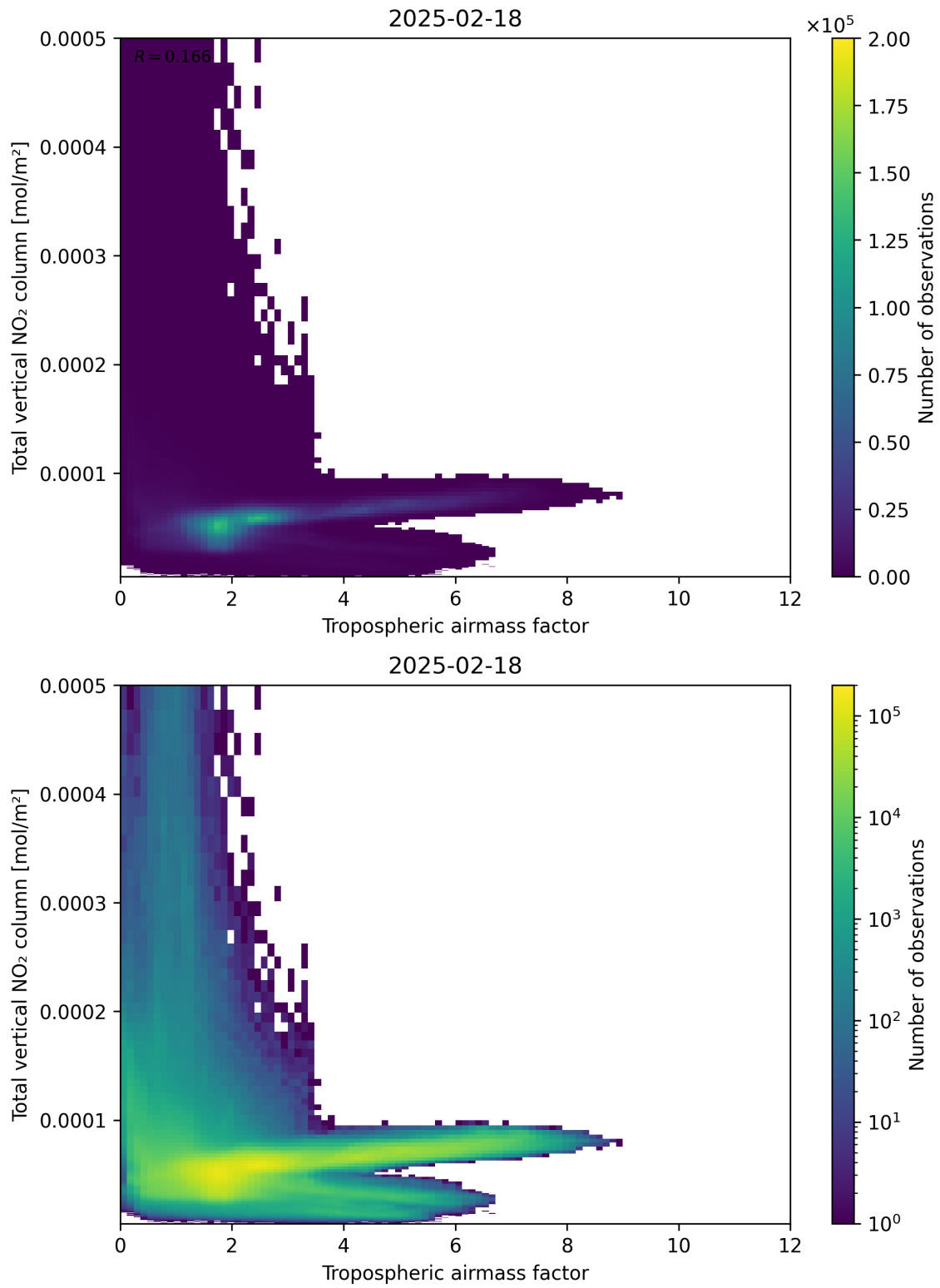
Figure 77: Scatter density plot of “Tropospheric airmass factor” against “Total vertical NO 2 column” for 2025-02-18 to 2025-02-19.
