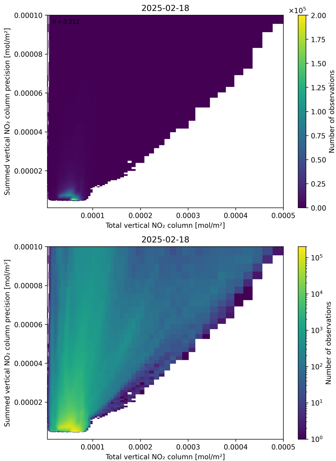
Figure 113: Scatter density plot of “Total vertical NO 2 column” against “Summed vertical NO 2 column precision” for 2025-02-18 to 2025-02-19.
