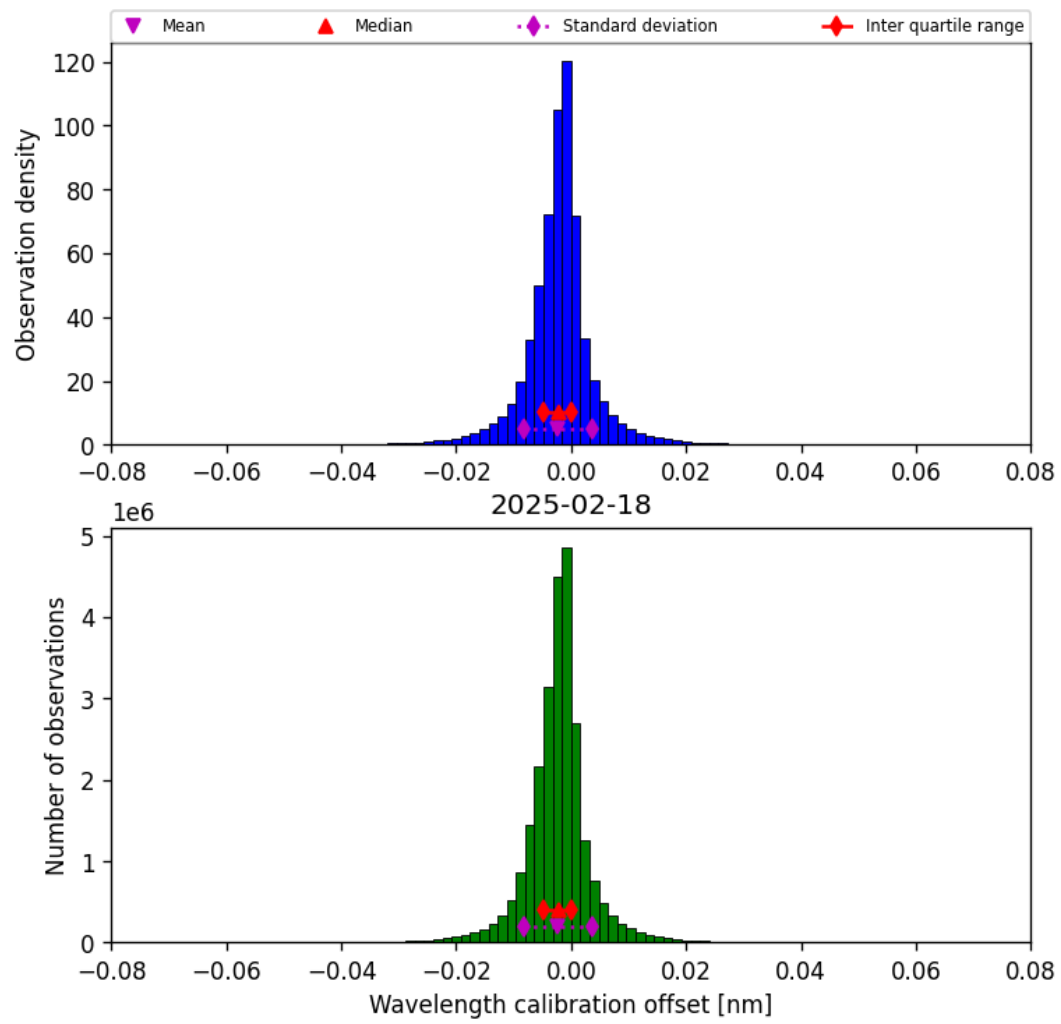
Figure 35: Histogram of “Wavelength calibration offset” for 2025-02-18 to 2025-02-19
