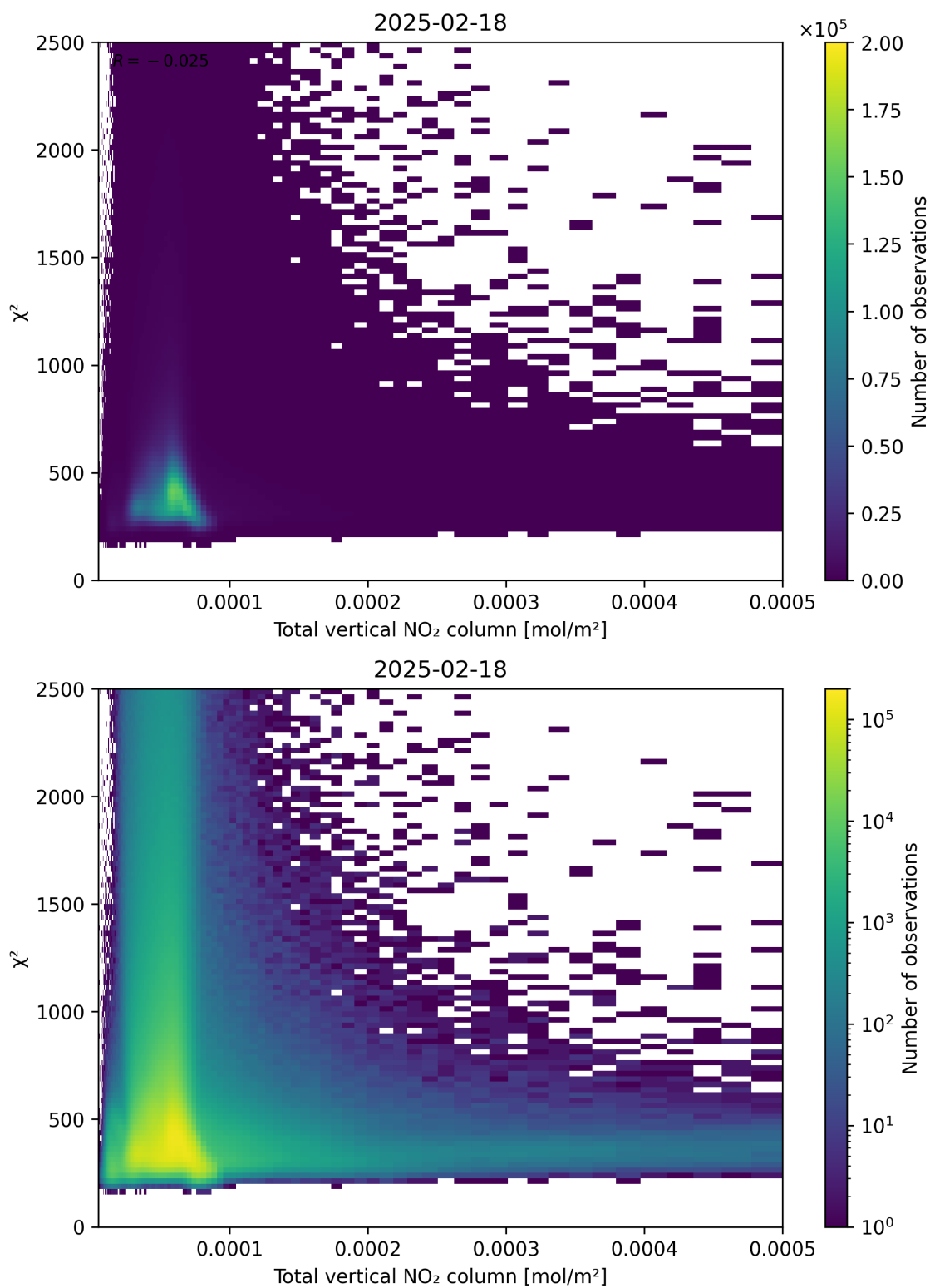
Figure 111: Scatter density plot of “Total vertical NO 2 column” against “ \chi^2 ” for 2025-02-18 to 2025-02-19.
