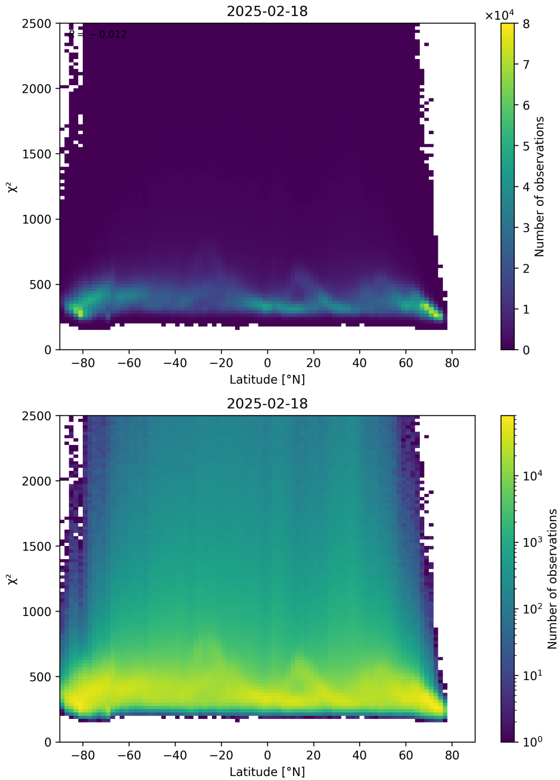
Figure 86: Scatter density plot of “Latitude” against “ \chi^2 ” for 2025-02-18 to 2025-02-19.
