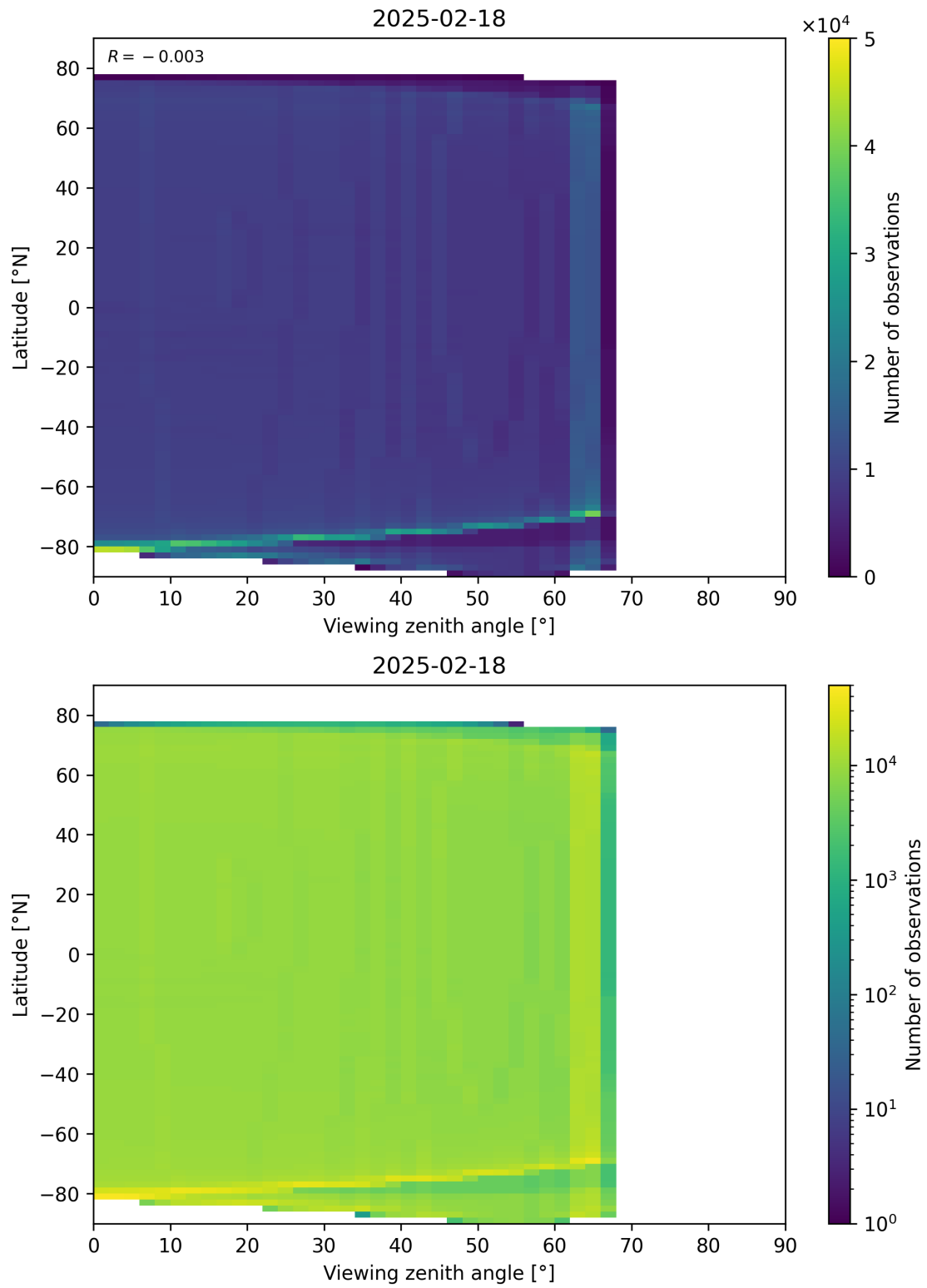
Figure 163: Scatter density plot of “Viewing zenith angle” against “Latitude” for 2025-02-18 to 2025-02-19.
