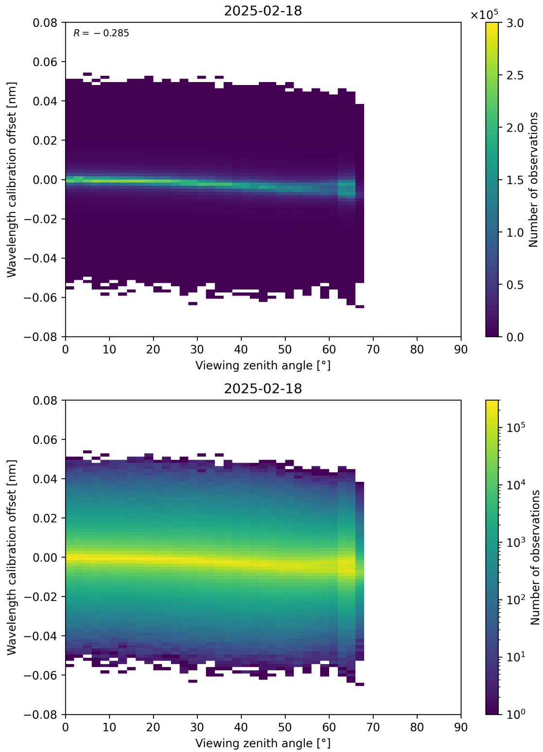
Figure 173: Scatter density plot of “Viewing zenith angle” against “Wavelength calibration offset” for 2025-02-18 to 2025-02-19.
