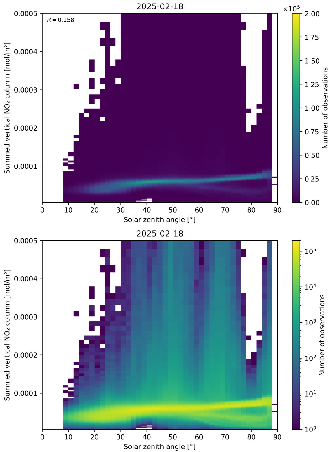
Figure 151: Scatter density plot of “Solar zenith angle” against “Summed vertical NO 2 column” for 2025-02-18 to 2025-02-19.
