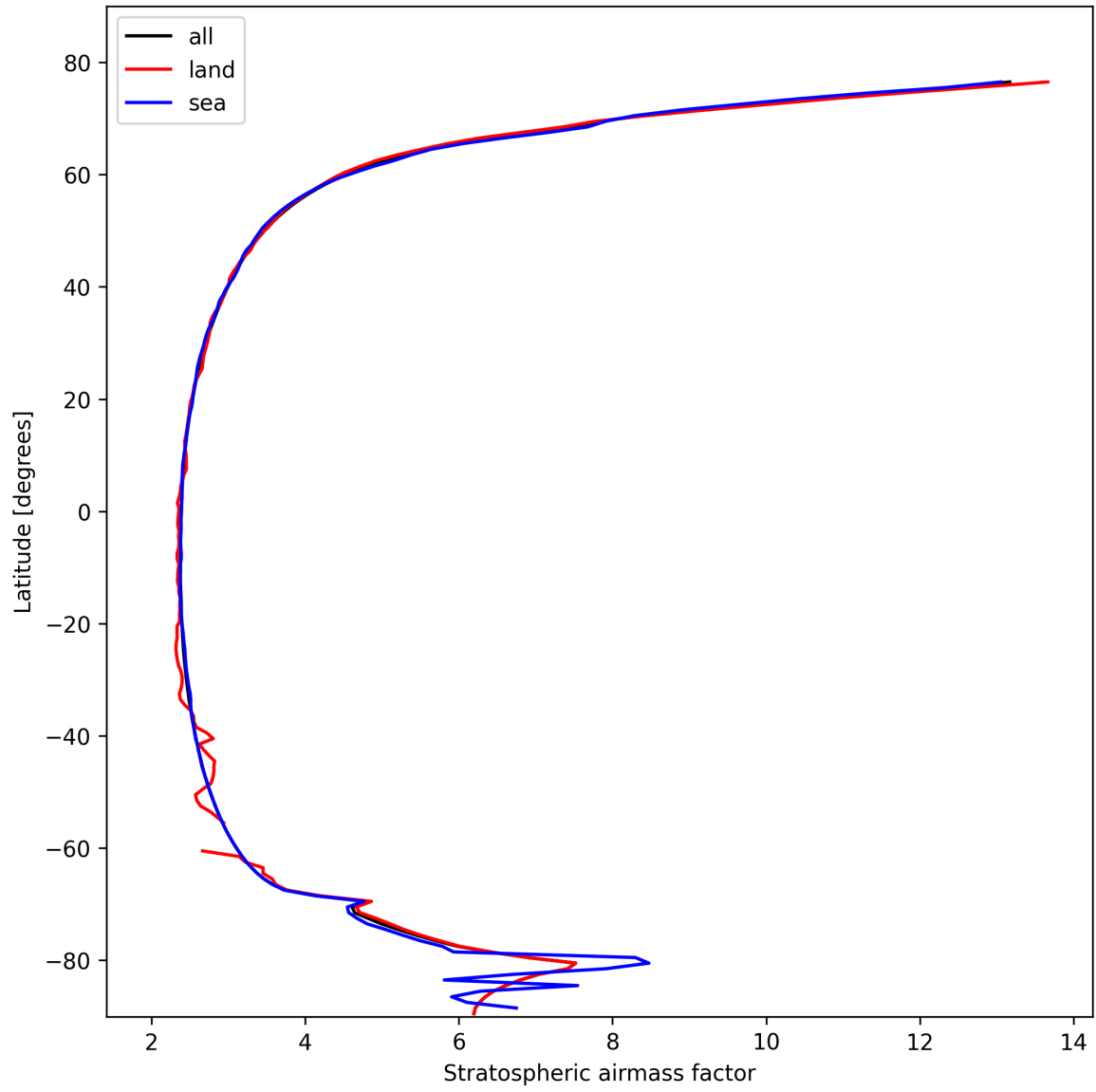
Figure 27: Zonal average of “Stratospheric airmass factor” for 2025-02-18 to 2025-02-19.
