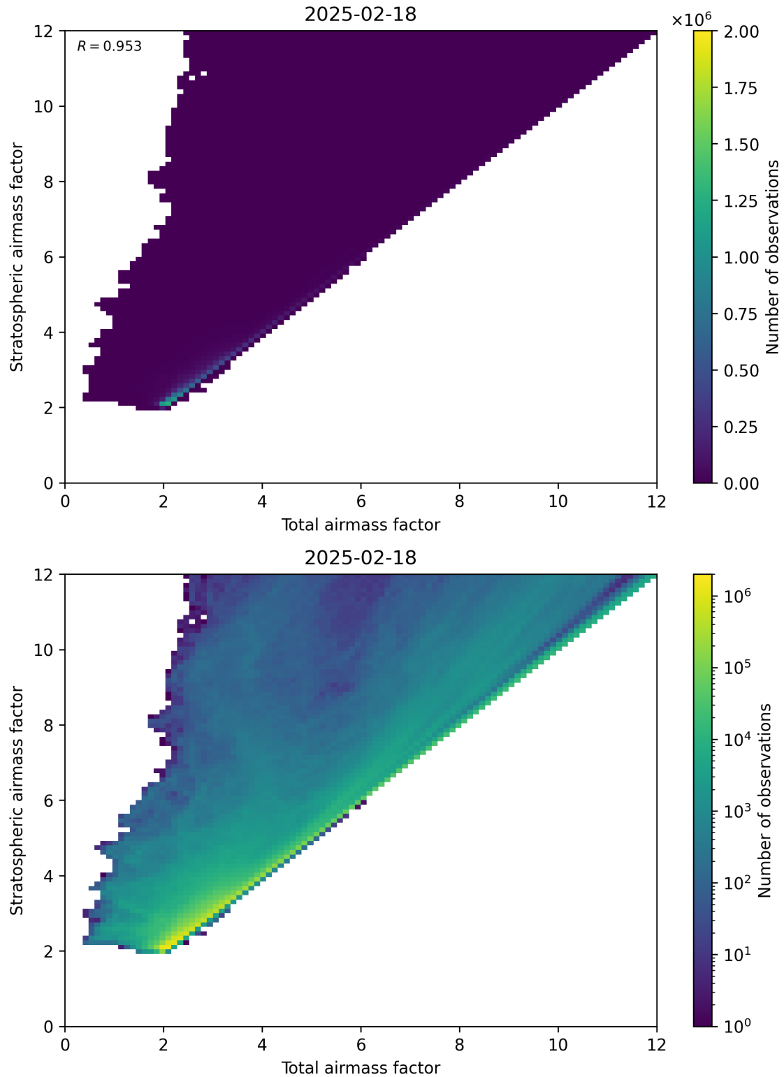
Figure 62: Scatter density plot of “Total airmass factor” against “Stratospheric airmass factor” for 2025-02-18 to 2025-02-19.
