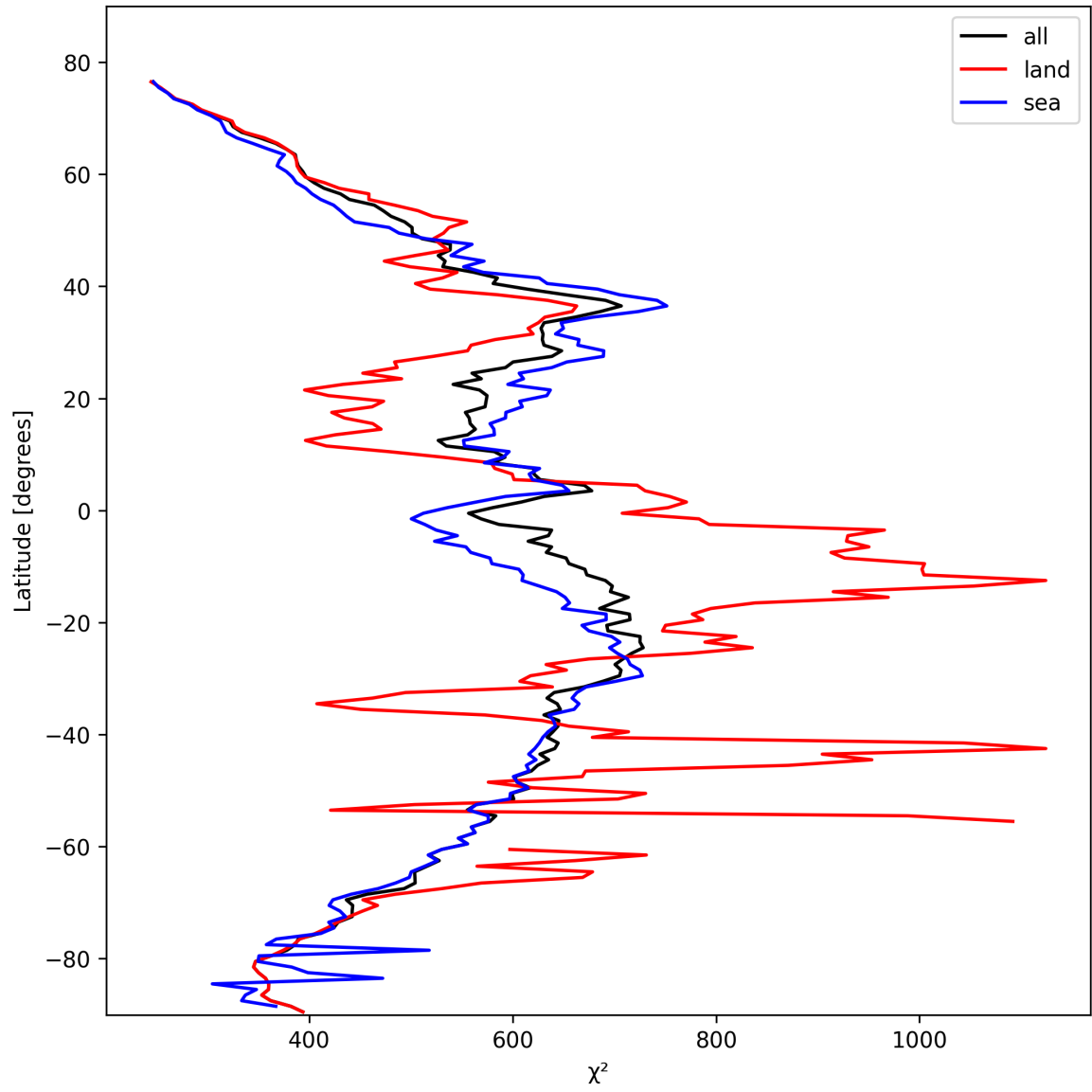
Figure 25: Zonal average of “ \chi^2 ” for 2025-02-18 to 2025-02-19.
