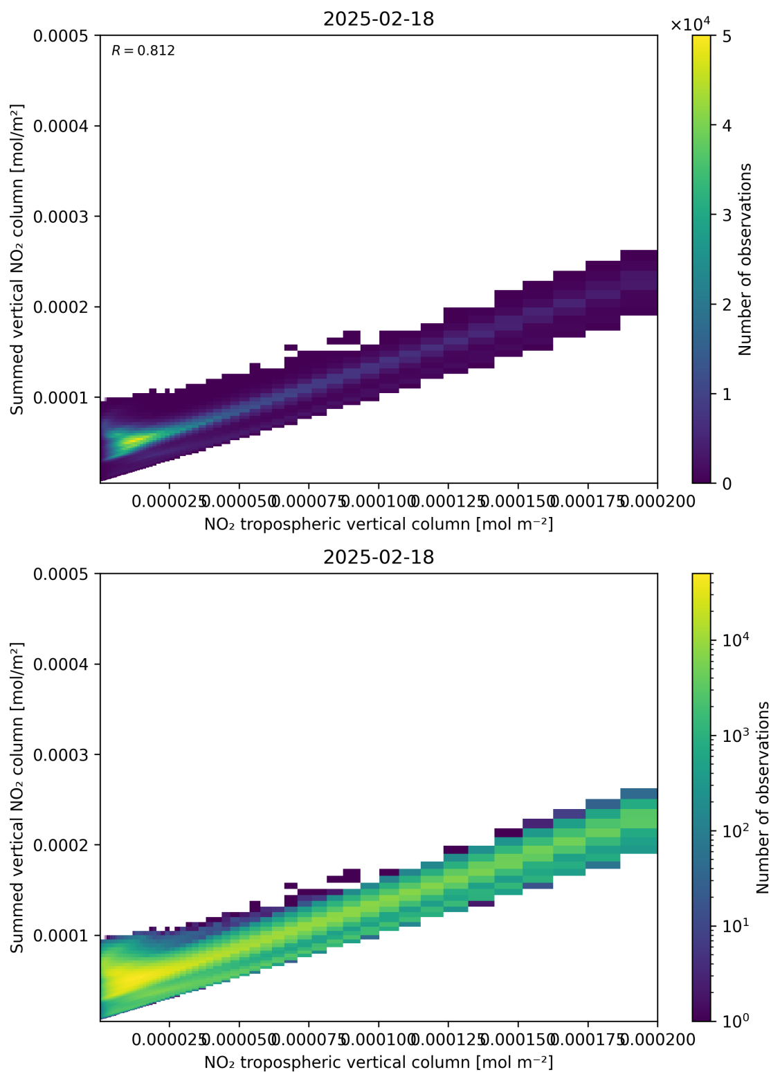
Figure 126: Scatter density plot of “NO 2 tropospheric vertical column” against “Summed vertical NO 2 column” for 2025-02-18 to 2025-02-19.
