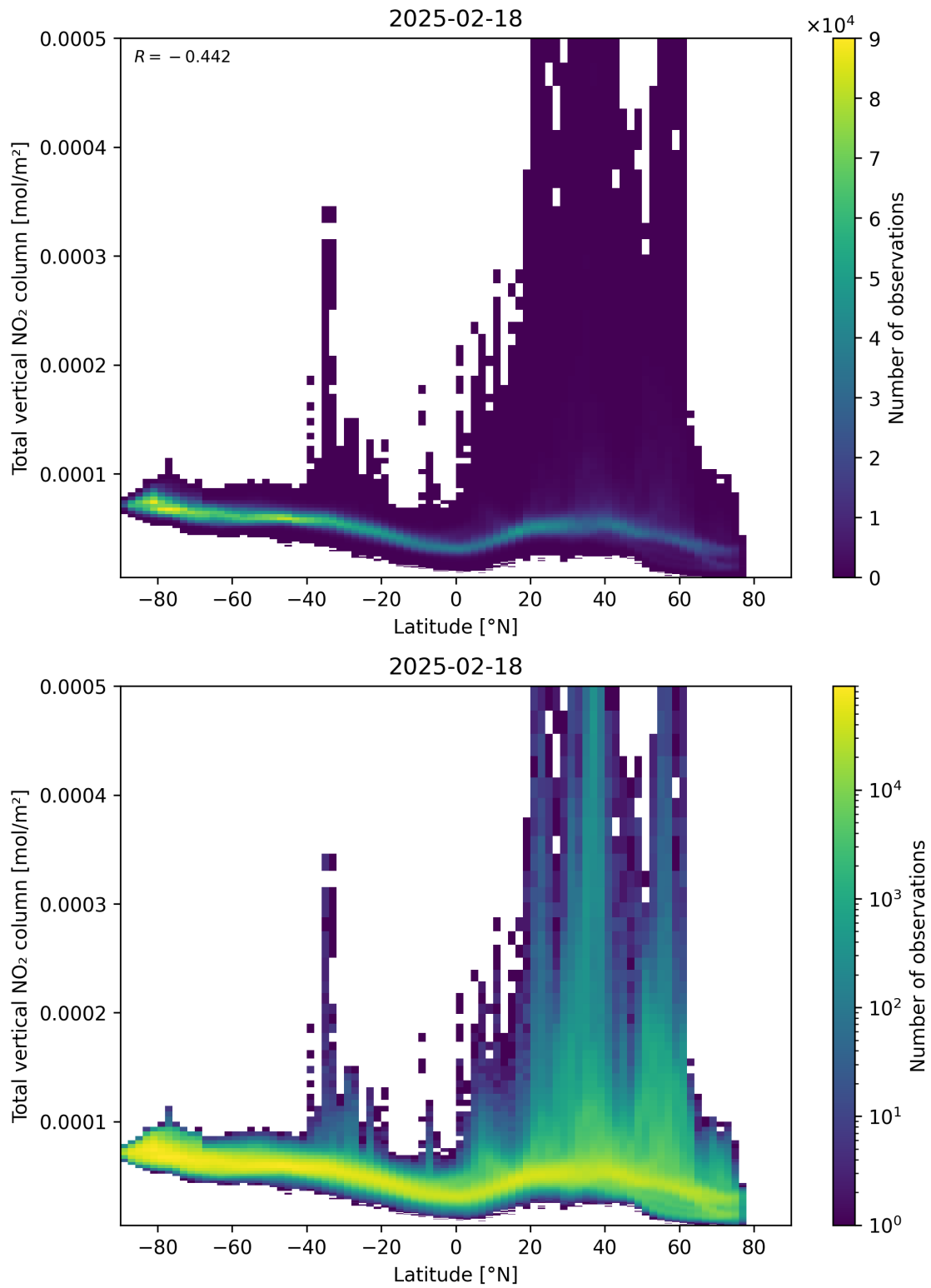
Figure 90: Scatter density plot of “Latitude” against “Total vertical NO 2 column” for 2025-02-18 to 2025-02-19.
