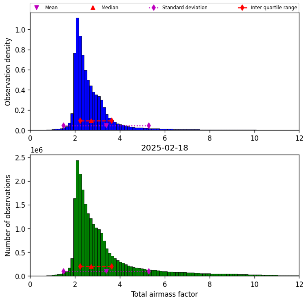
Figure 32: Histogram of “Total airmass factor” for 2025-02-18 to 2025-02-19
