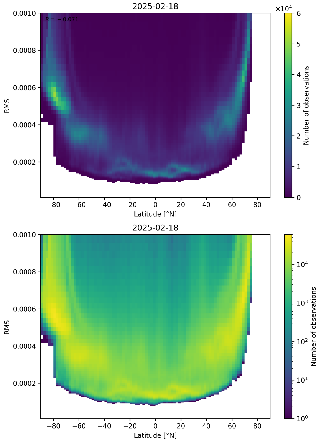
Figure 94: Scatter density plot of “Latitude” against “RMS” for 2025-02-18 to 2025-02-19.
