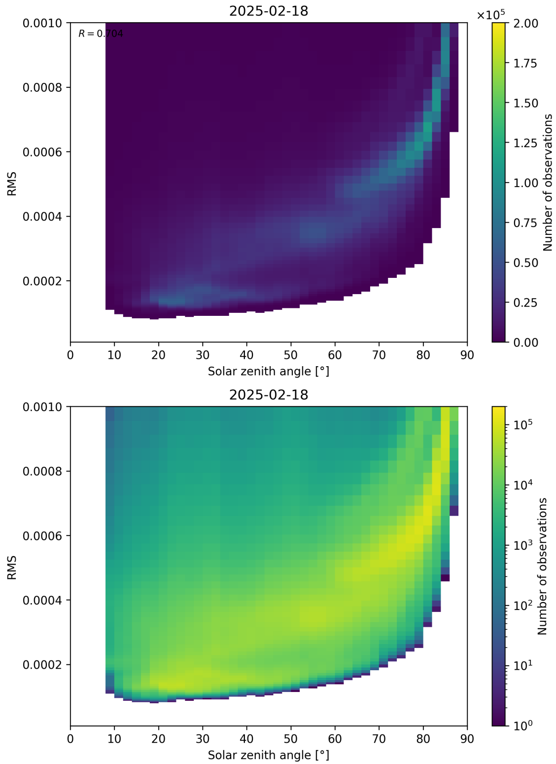
Figure 157: Scatter density plot of “Solar zenith angle” against “RMS” for 2025-02-18 to 2025-02-19.
