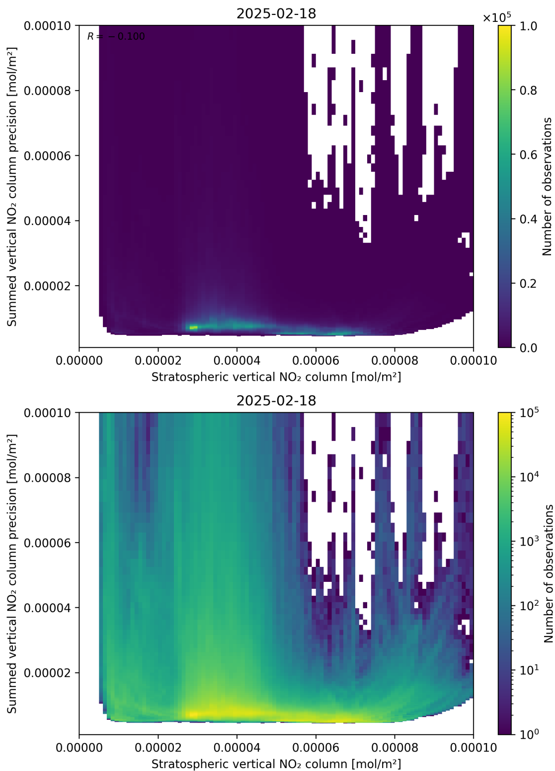
Figure 99: Scatter density plot of “Stratospheric vertical NO 2 column” against “Summed vertical NO 2 column precision” for 2025-02-18 to 2025-02-19.
