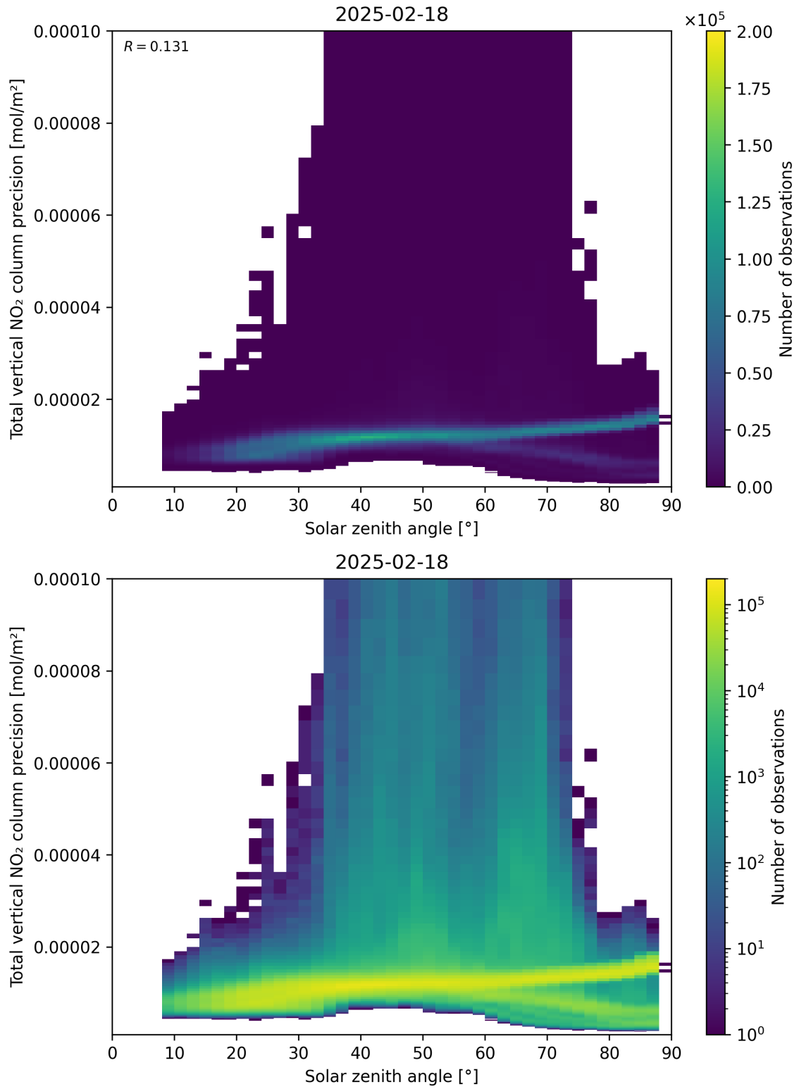
Figure 154: Scatter density plot of “Solar zenith angle” against “Total vertical NO 2 column precision” for 2025-02-18 to 2025-02-19.
