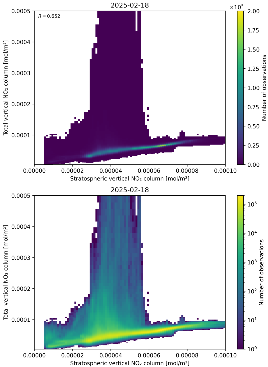
Figure 100: Scatter density plot of “Stratospheric vertical NO 2 column” against “Total vertical NO 2 column” for 2025-02-18 to 2025-02-19.
