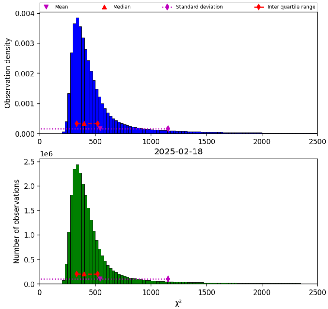
Figure 42: Histogram of “ \chi^2 ” for 2025-02-18 to 2025-02-19
