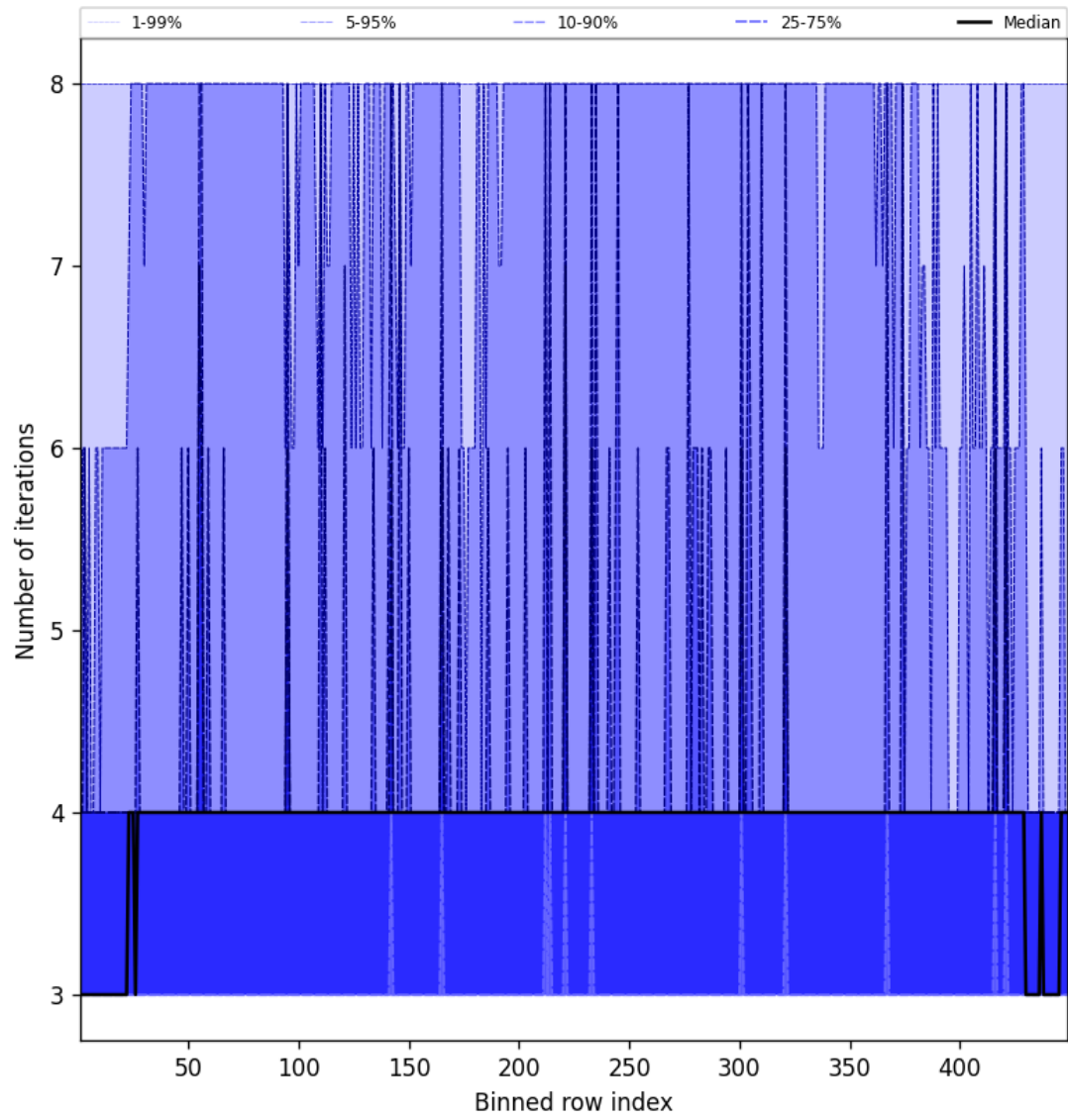
Figure 51: Along track statistics of "Number of iterations" for 2025-02-18 to 2025-02-19
