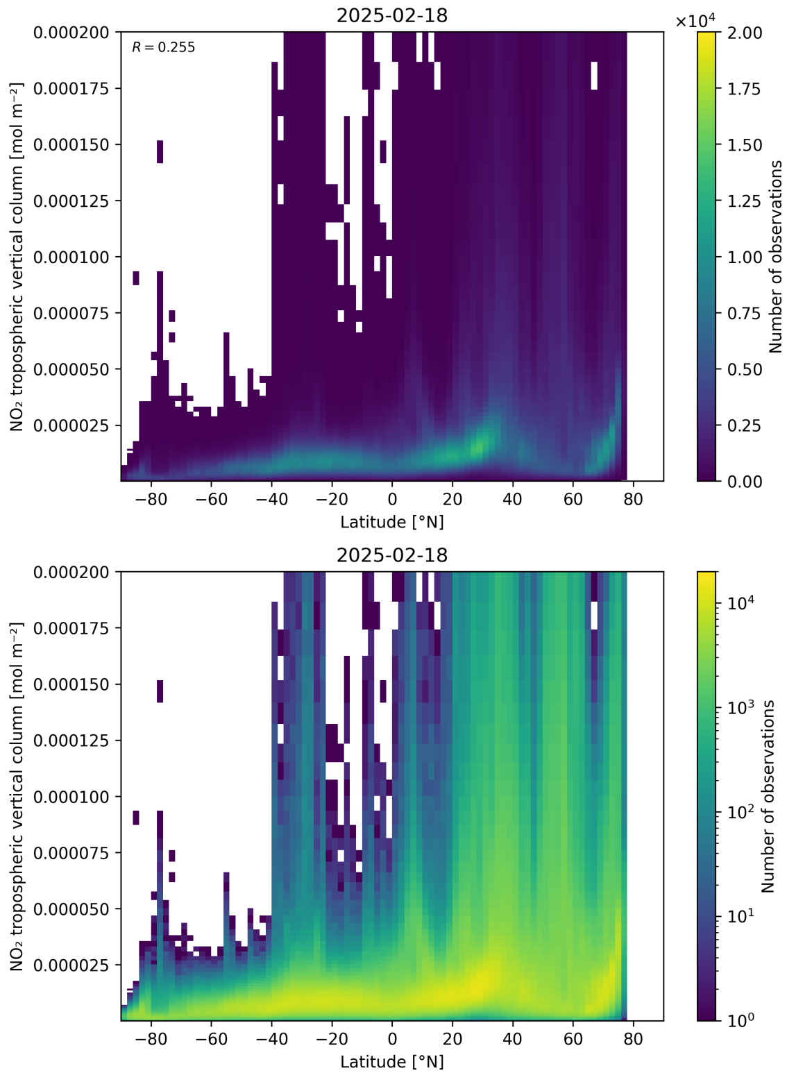
Figure 92: Scatter density plot of “Latitude” against “NO 2 tropospheric vertical column” for 2025-02-18 to 2025-02-19.
