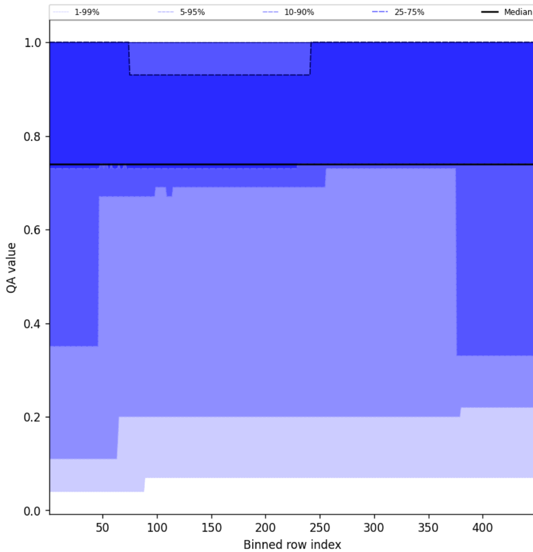
Figure 45: Along track statistics of “QA value” for 2025-02-18 to 2025-02-19
