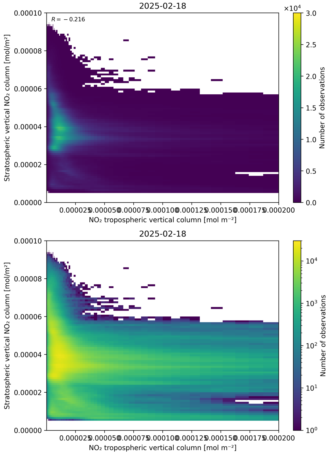
Figure 125: Scatter density plot of “NO 2 tropospheric vertical column” against “Stratospheric vertical NO 2 column” for 2025-02-18 to 2025-02-19.
