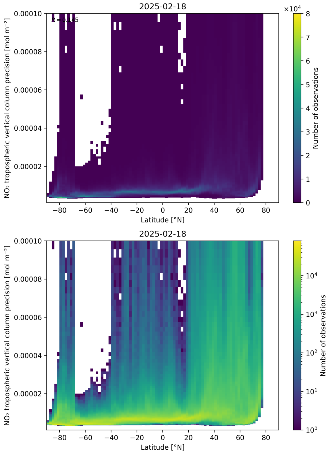
Figure 93: Scatter density plot of “Latitude” against “NO 2 tropospheric vertical column precision” for 2025-02-18 to 2025-02-19.
