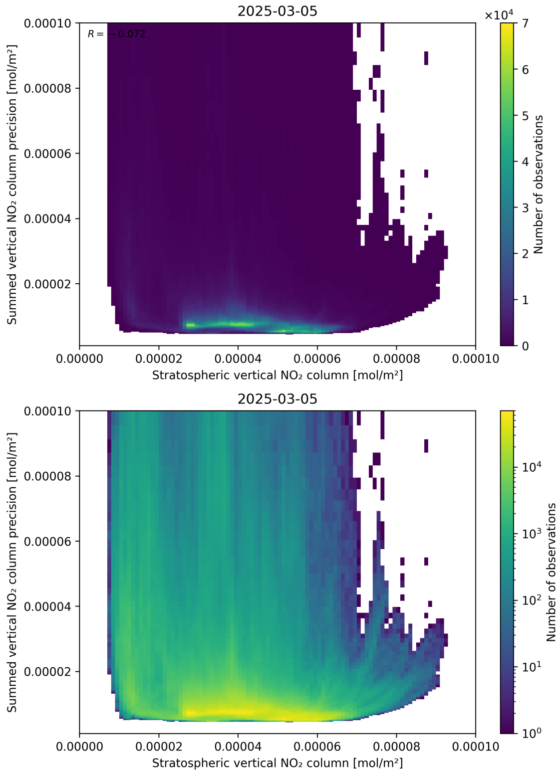
Figure 99: Scatter density plot of “Stratospheric vertical NO 2 column” against “Summed vertical NO 2 column precision” for 2025-03-05 to 2025-03-05.
