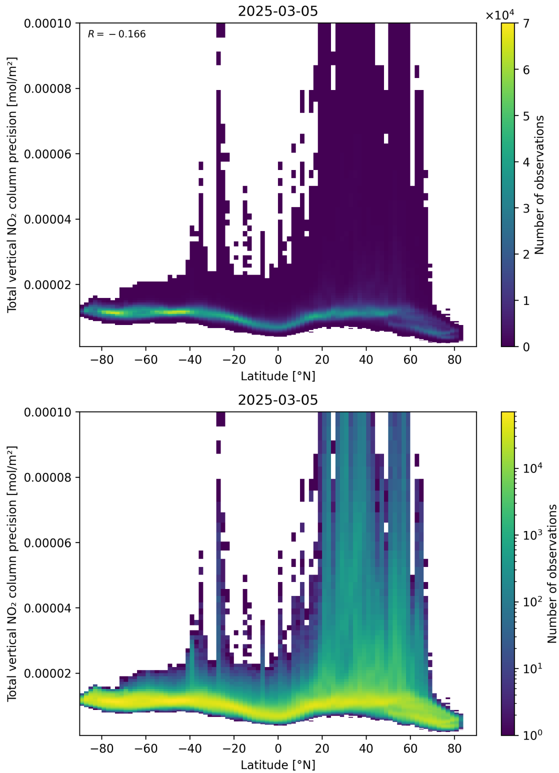
Figure 91: Scatter density plot of “Latitude” against “Total vertical NO 2 column precision” for 2025-03-05 to 2025-03-05.
