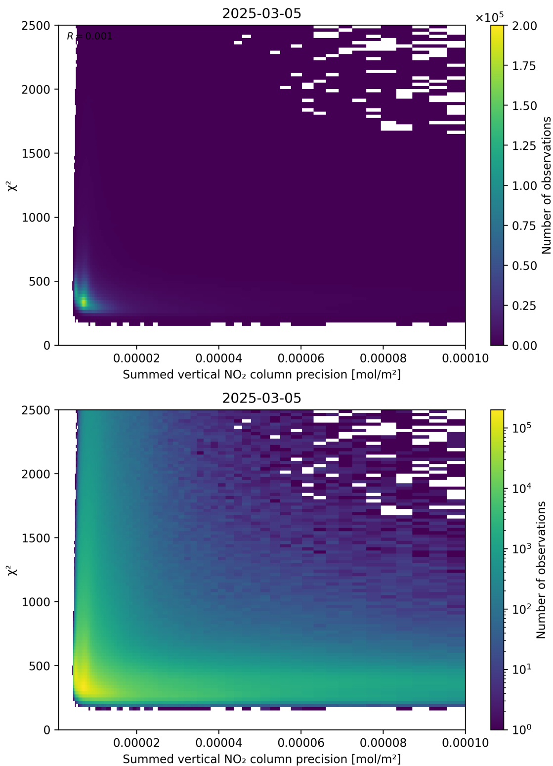
Figure 107: Scatter density plot of “Summed vertical NO 2 column precision” against “ \chi^2 ” for 2025-03-05 to 2025-03-05.
