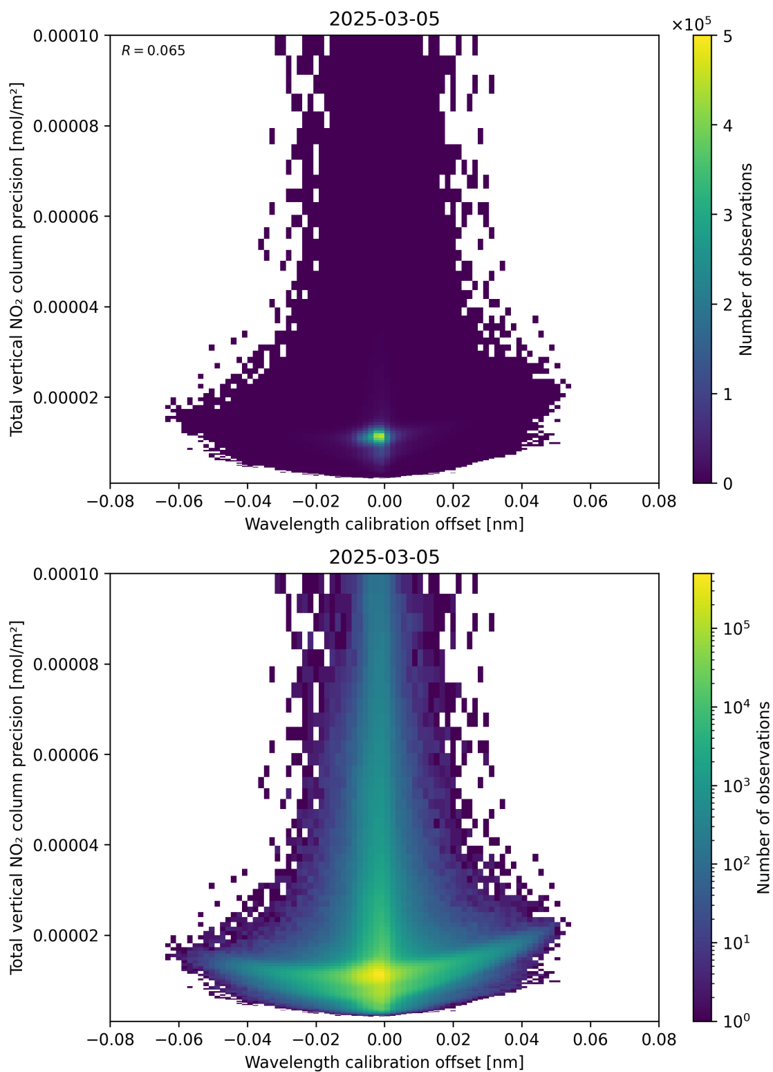
Figure 180: Scatter density plot of “Wavelength calibration offset” against “Total vertical NO 2 column precision” for 2025-03-05 to 2025-03-05.
