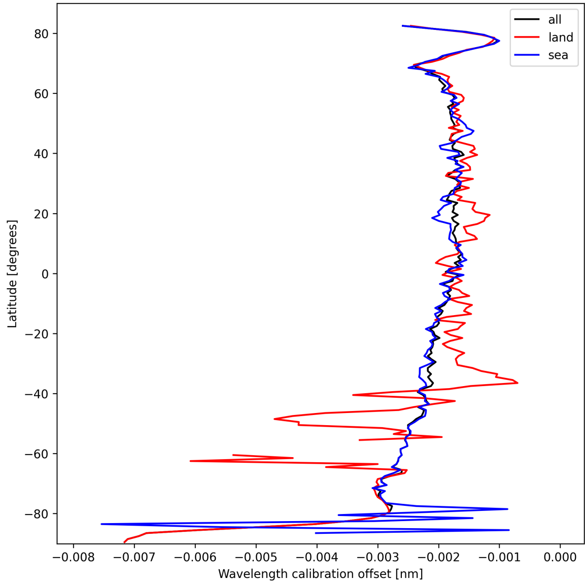
Figure 18: Zonal average of “Wavelength calibration offset” for 2025-03-05 to 2025-03-05.
