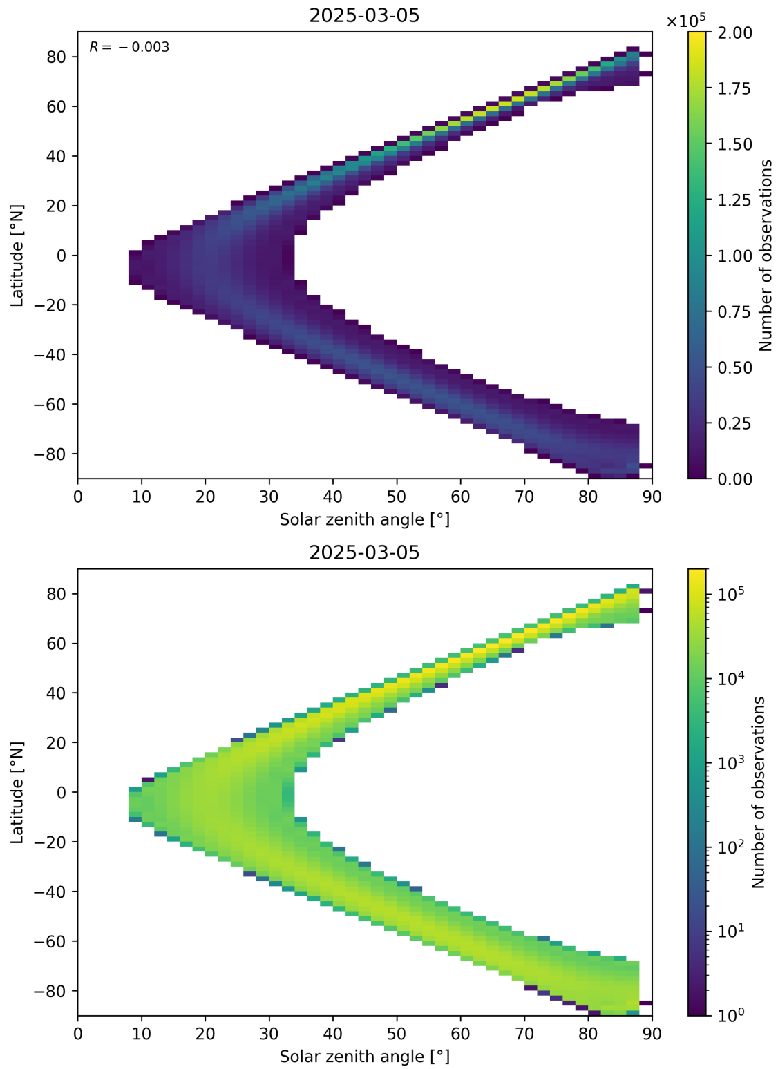
Figure 149: Scatter density plot of “Solar zenith angle” against “Latitude” for 2025-03-05 to 2025-03-05.
