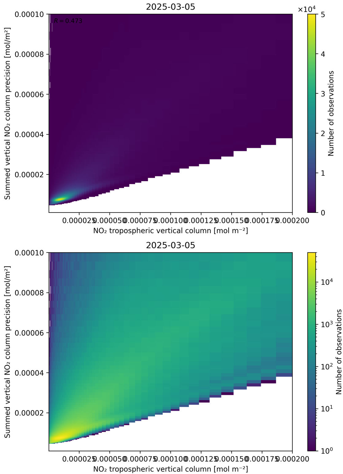
Figure 127: Scatter density plot of “NO 2 tropospheric vertical column” against “Summed vertical NO 2 column precision” for 2025-03-05 to 2025-03-05.
