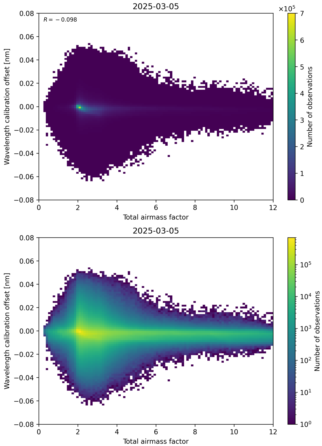
Figure 70: Scatter density plot of “Total airmass factor” against “Wavelength calibration offset” for 2025-03-05 to 2025-03-05.
