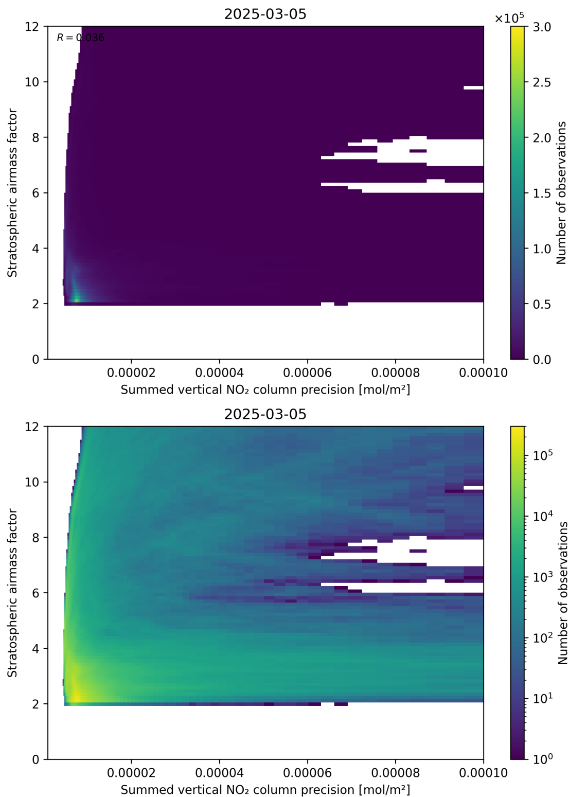
Figure 106: Scatter density plot of “Summed vertical NO 2 column precision” against “Stratospheric airmass factor” for 2025-03-05 to 2025-03-05.
