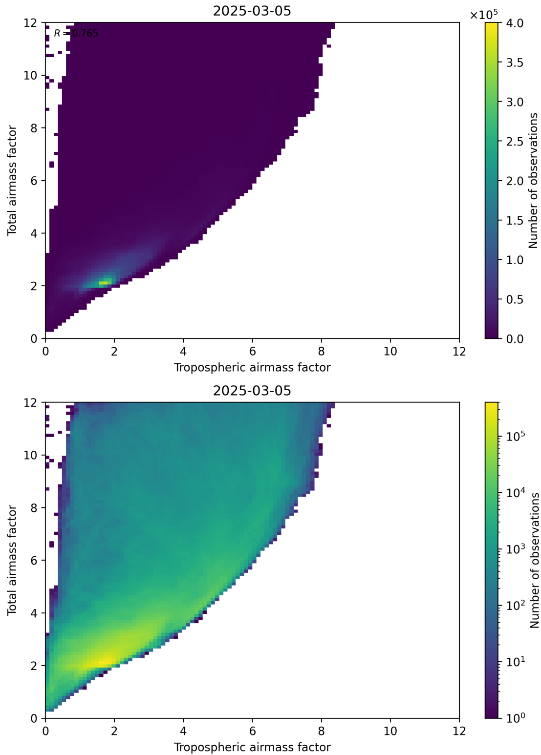
Figure 72: Scatter density plot of “Tropospheric airmass factor” against “Total airmass factor” for 2025-03-05 to 2025-03-05.
