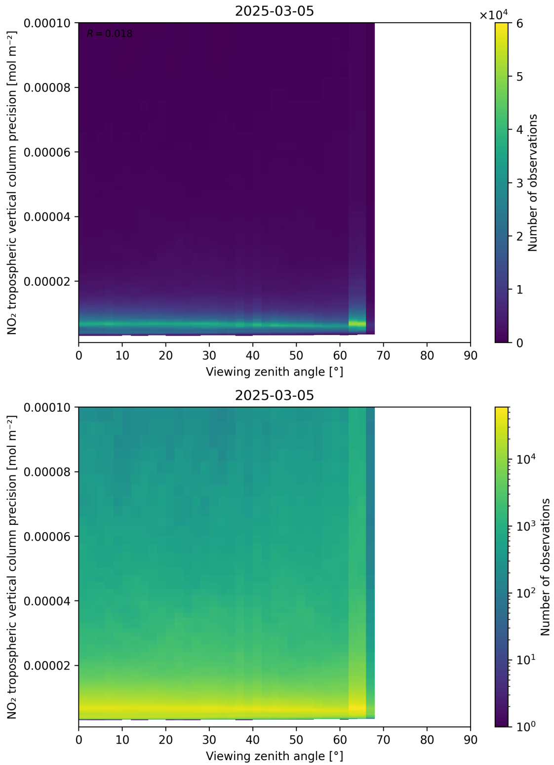
Figure 170: Scatter density plot of “Viewing zenith angle” against “NO 2 tropospheric vertical column precision” for 2025-03-05 to 2025-03-05.
