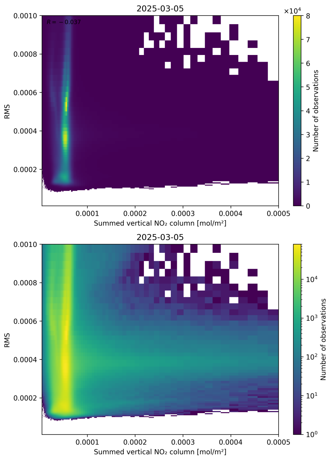
Figure 109: Scatter density plot of “Summed vertical NO 2 column” against “RMS” for 2025-03-05 to 2025-03-05.
