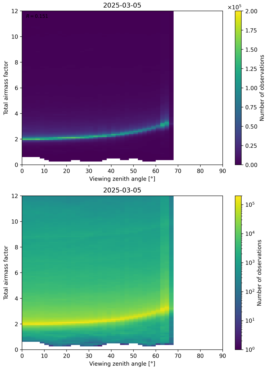
Figure 160: Scatter density plot of “Viewing zenith angle” against “Total airmass factor” for 2025-03-05 to 2025-03-05.
