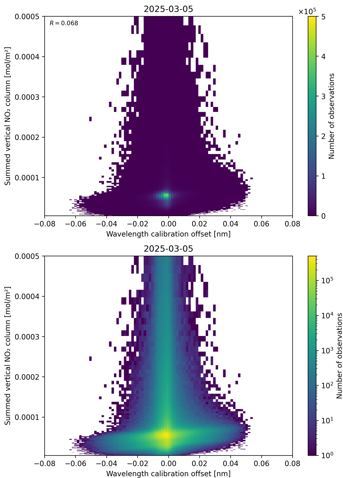
Figure 177: Scatter density plot of “Wavelength calibration offset” against “Summed vertical NO 2 column” for 2025-03-05 to 2025-03-05.
