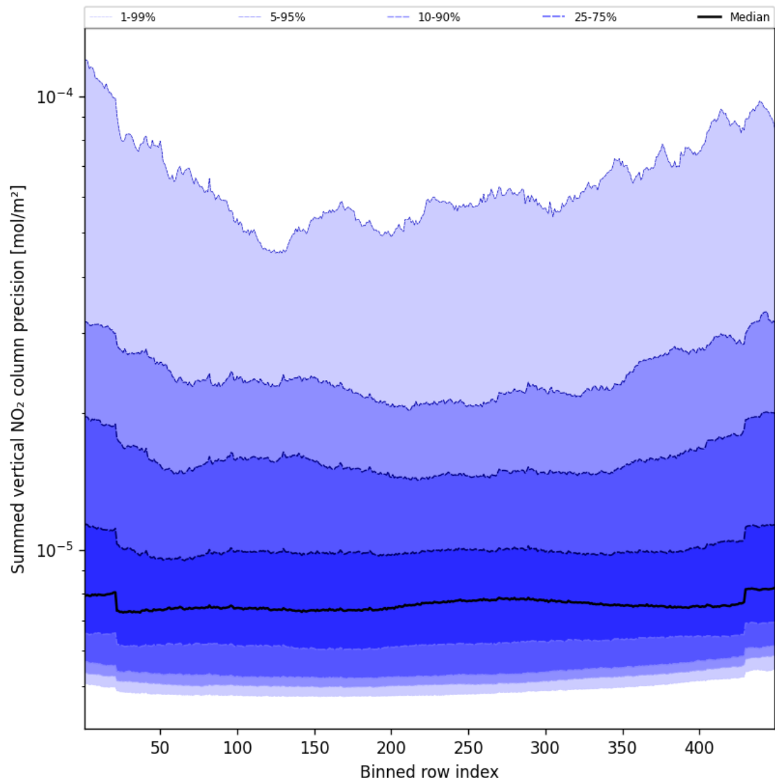
Figure 58: Along track statistics of “Summed vertical NO 2 column precision” for 2025-03-05 to 2025-03-05
