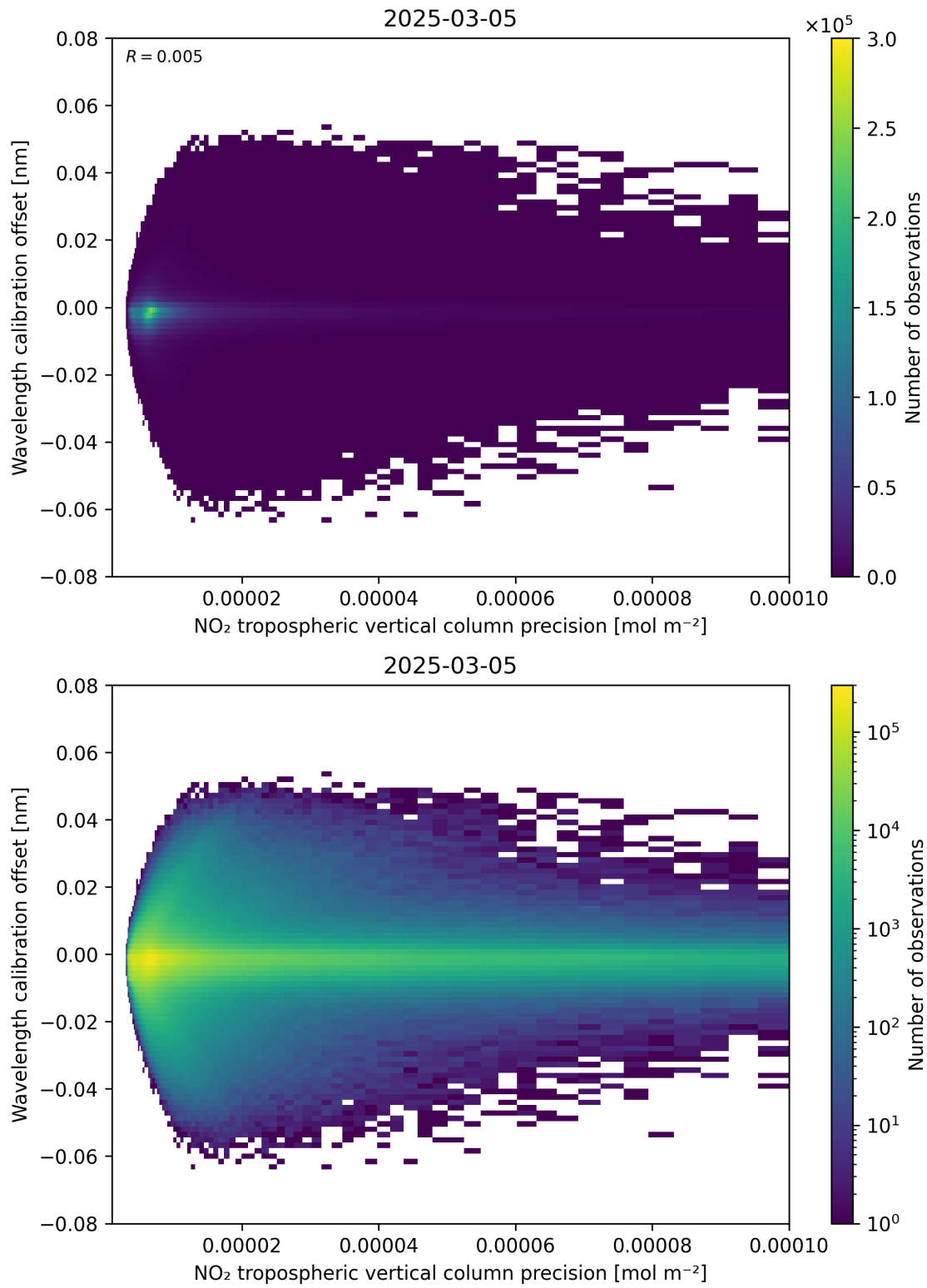
Figure 141: Scatter density plot of “NO 2 tropospheric vertical column precision” against “Wavelength calibration offset” for 2025-03-05 to 2025-03-05.
