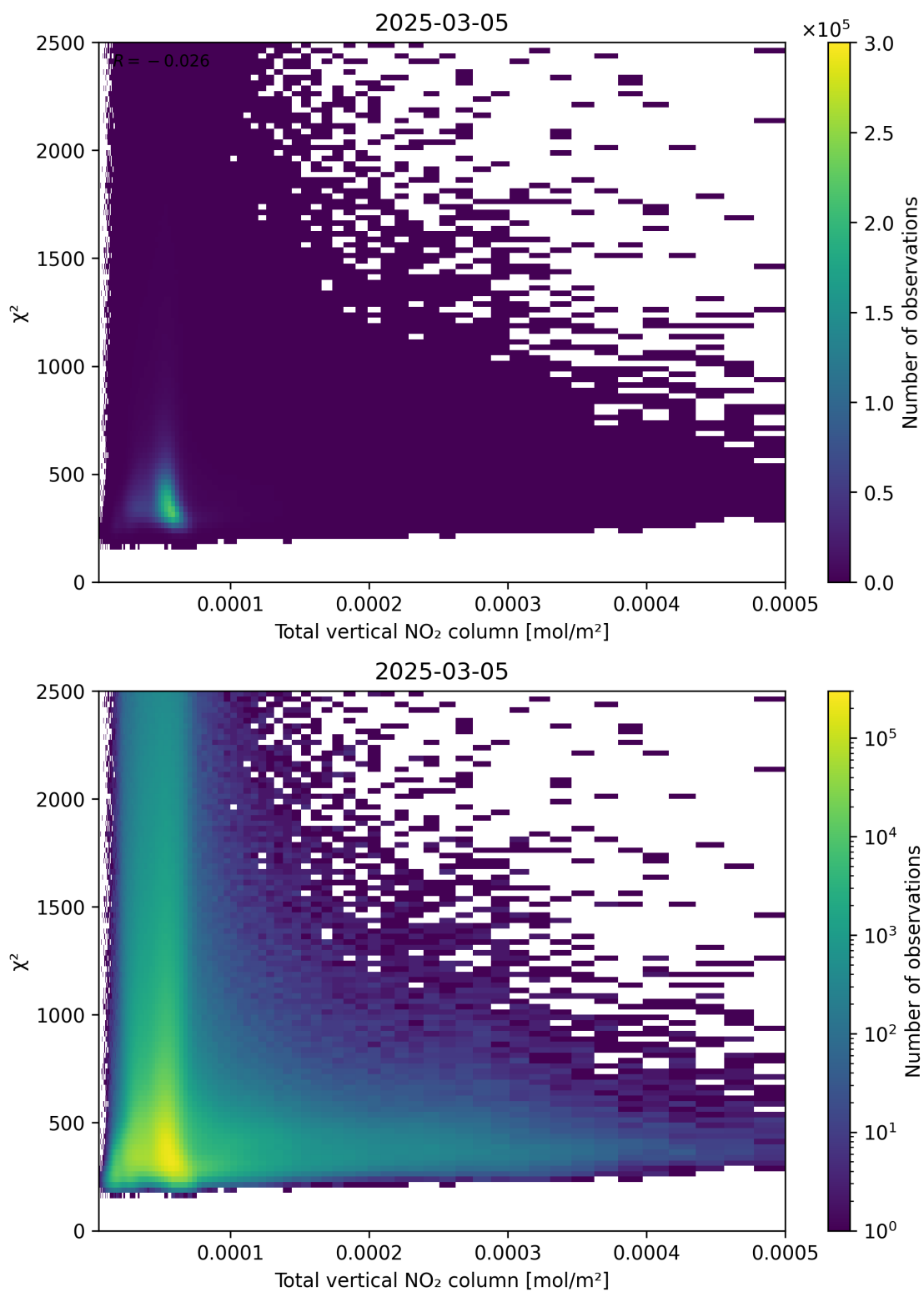
Figure 111: Scatter density plot of "Total vertical NO 2 column" against " \chi^2 " for 2025-03-05 to 2025-03-05.
