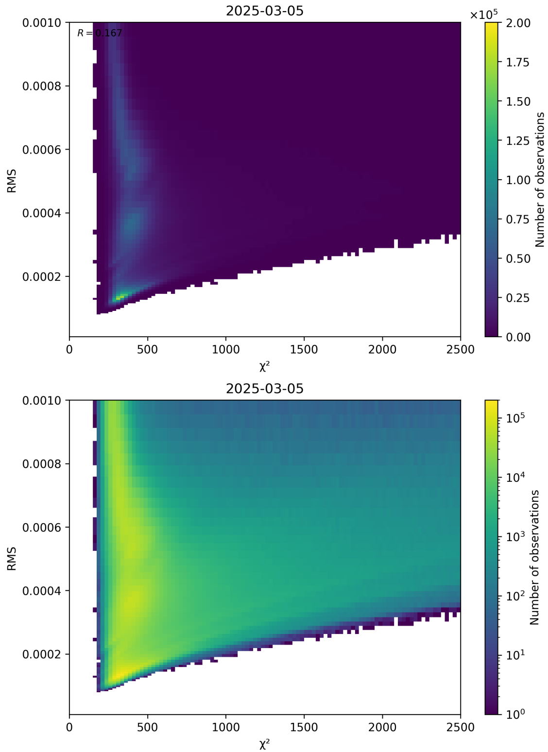
Figure 82: Scatter density plot of “ \chi^2 ” against “RMS” for 2025-03-05 to 2025-03-05.
