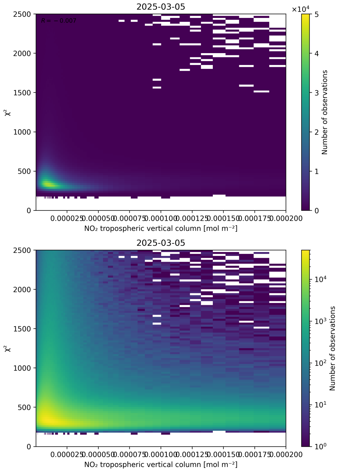
Figure 124: Scatter density plot of “NO 2 tropospheric vertical column” against “ \chi^2 ” for 2025-03-05 to 2025-03-05.
