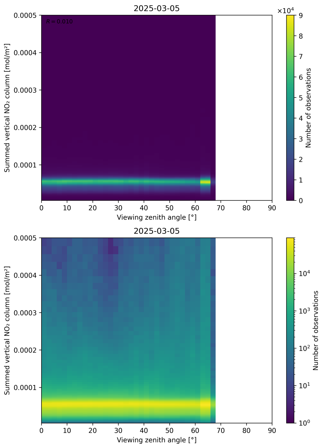
Figure 165: Scatter density plot of “Viewing zenith angle” against “Summed vertical NO 2 column” for 2025-03-05 to 2025-03-05.
