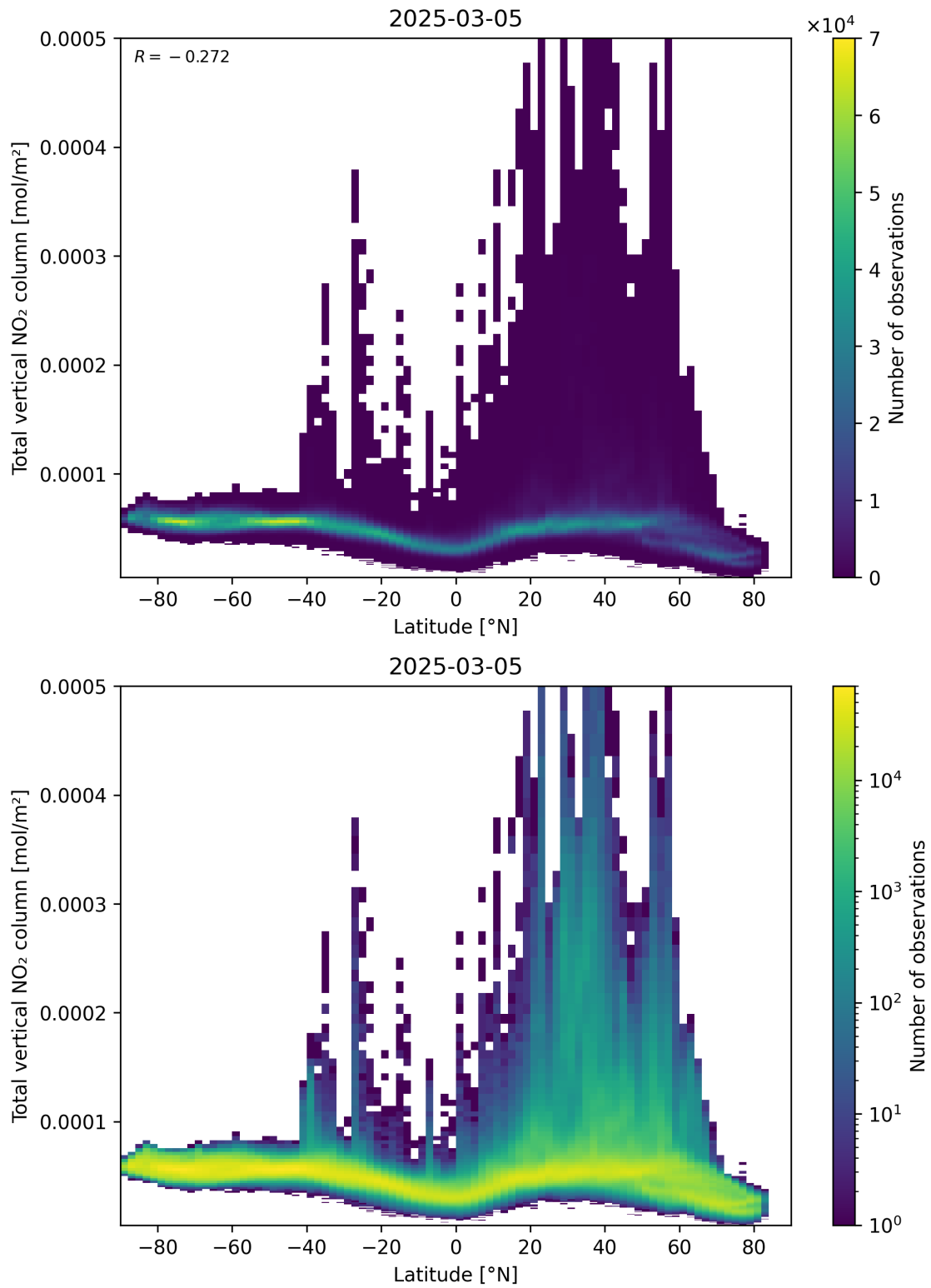
Figure 90: Scatter density plot of “Latitude” against “Total vertical NO 2 column” for 2025-03-05 to 2025-03-05.
