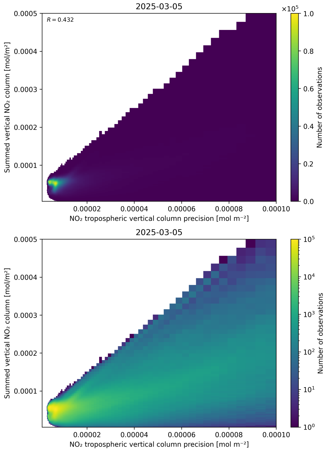
Figure 136: Scatter density plot of “NO 2 tropospheric vertical column precision” against “Summed vertical NO 2 column” for 2025-03-05 to 2025-03-05.
