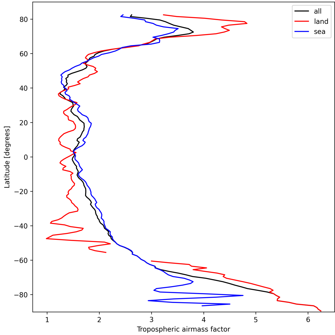
Figure 14: Zonal average of “Tropospheric airmass factor” for 2025-03-05 to 2025-03-05.
