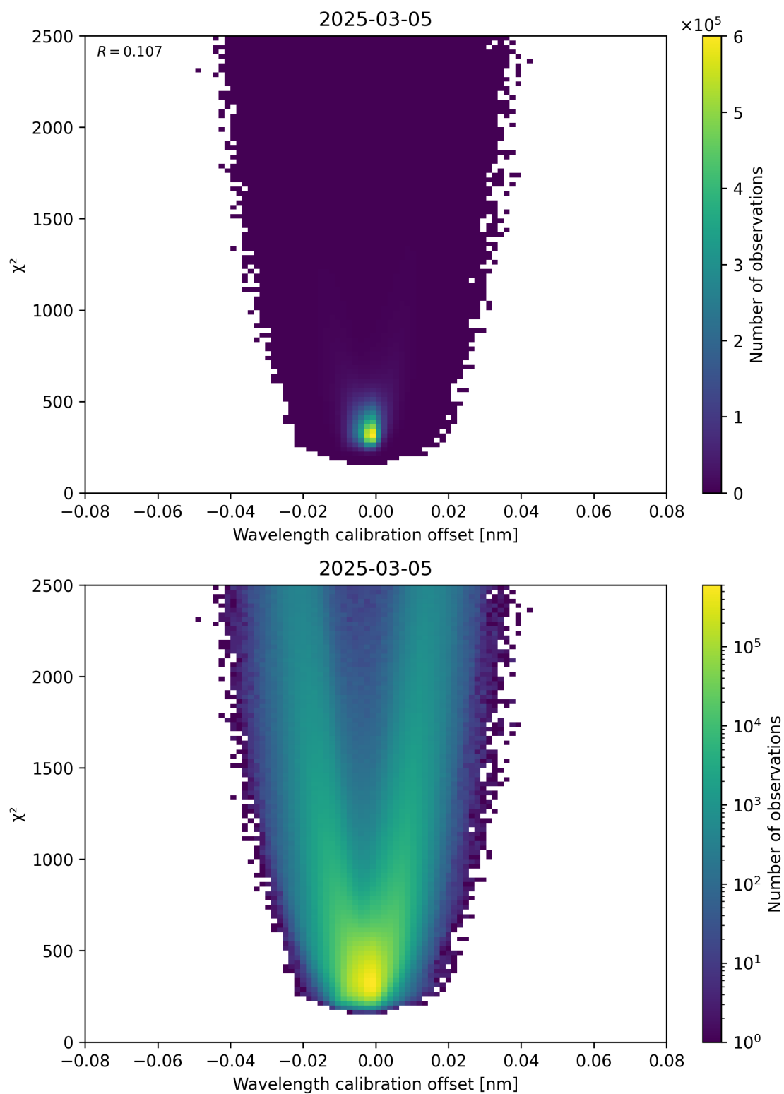
Figure 175: Scatter density plot of “Wavelength calibration offset” against “ \chi^2 ” for 2025-03-05 to 2025-03-05.
