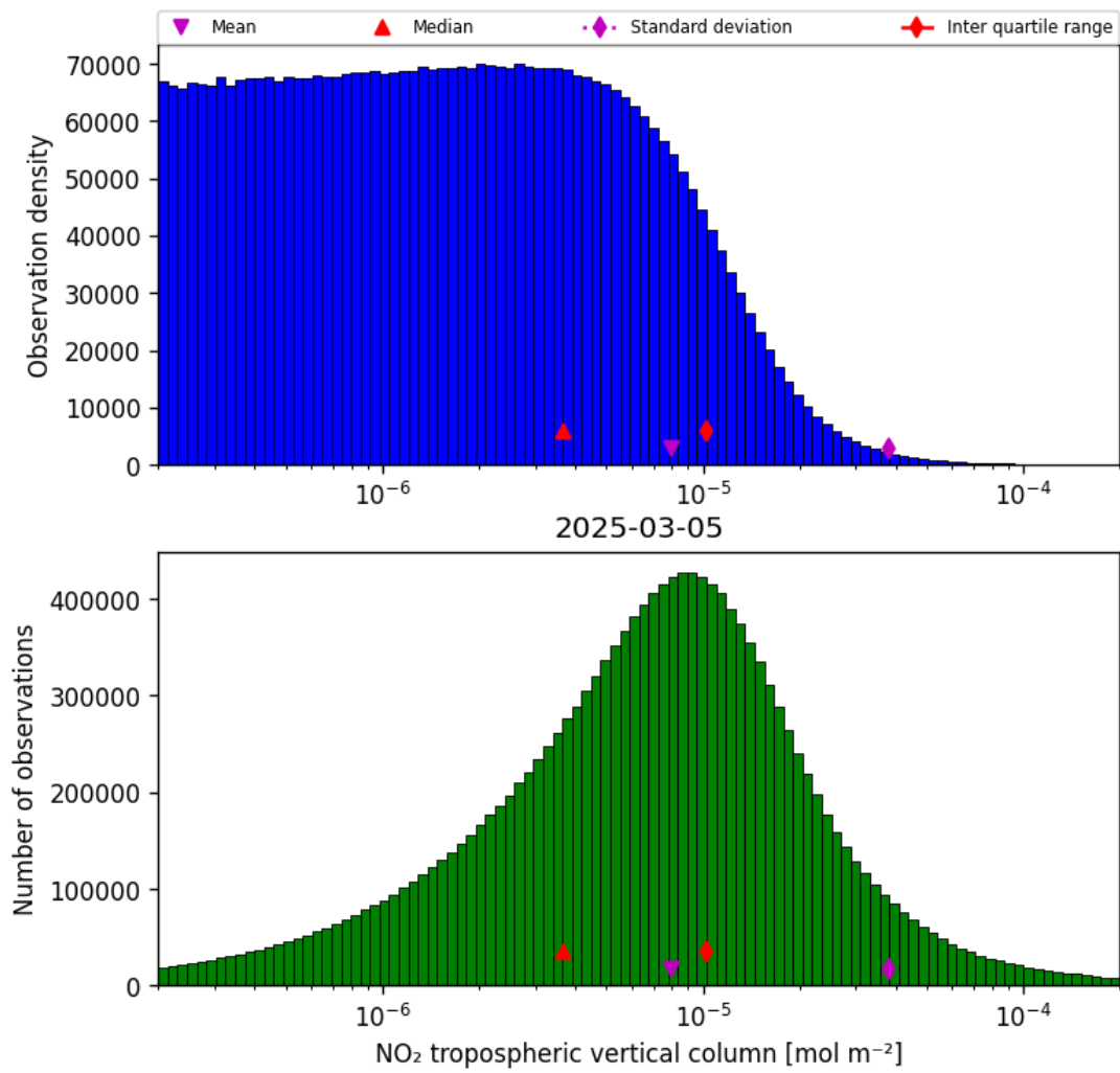
Figure 29: Histogram of “NO 2 tropospheric vertical column” for 2025-03-05 to 2025-03-05
