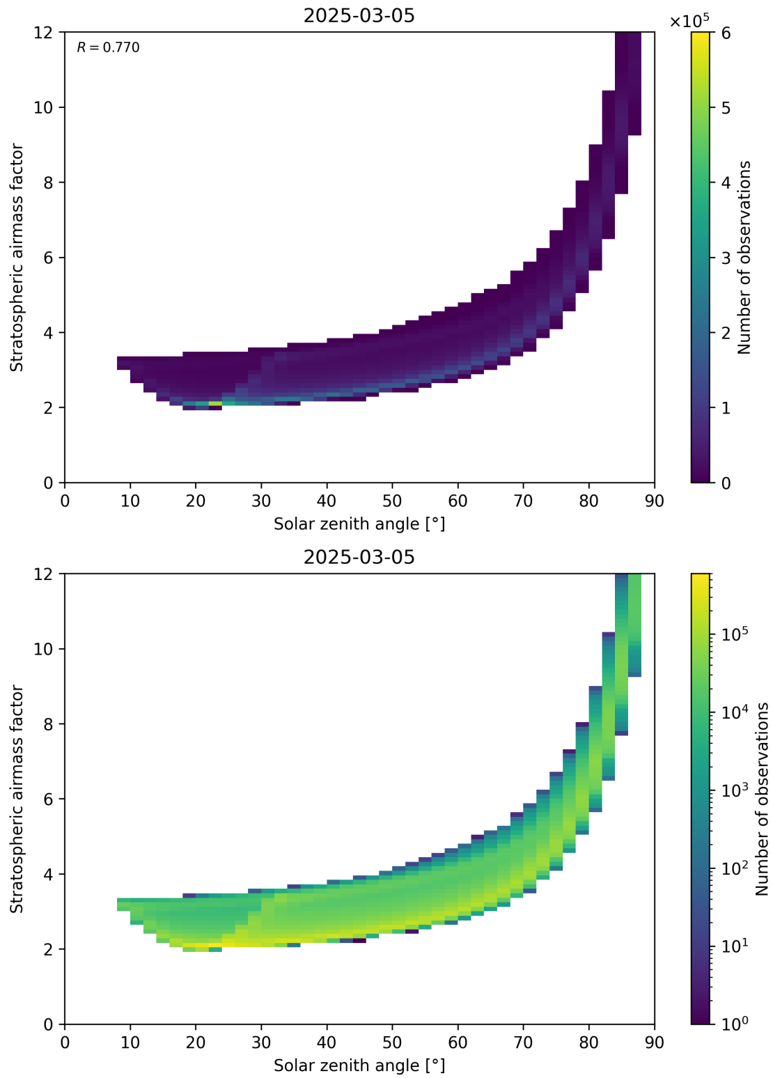
Figure 145: Scatter density plot of “Solar zenith angle” against “Stratospheric airmass factor” for 2025-03-05 to 2025-03-05.
