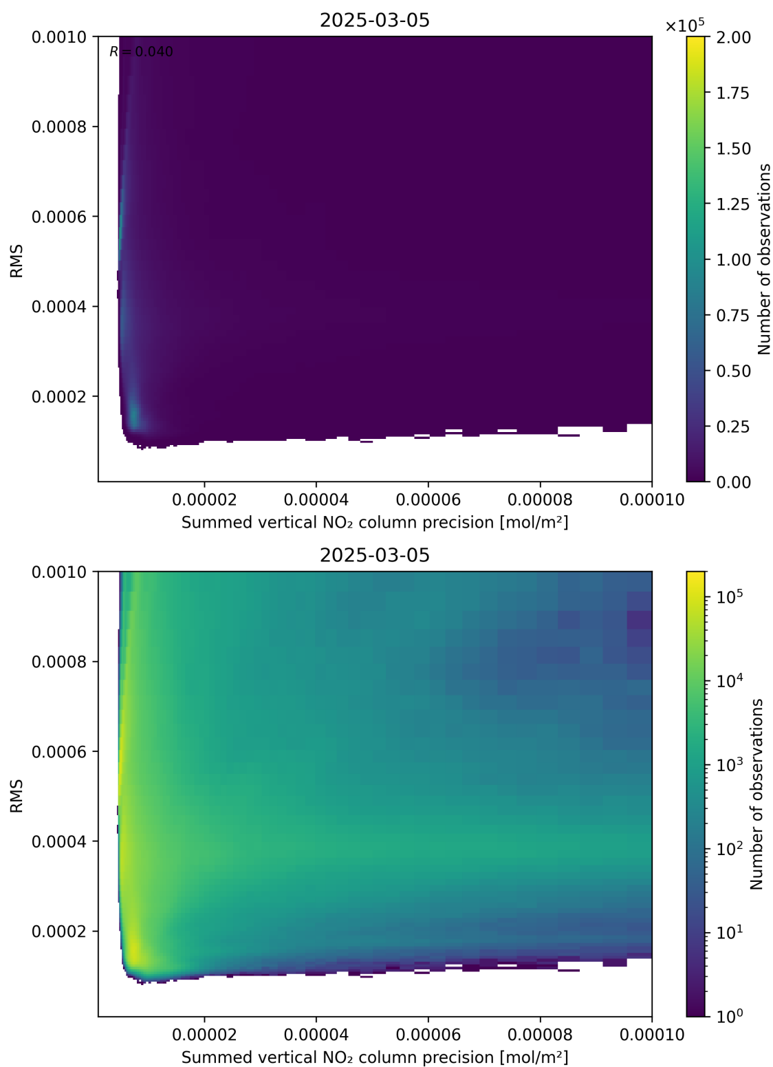
Figure 108: Scatter density plot of “Summed vertical NO 2 column precision” against “RMS” for 2025-03-05 to 2025-03-05.
