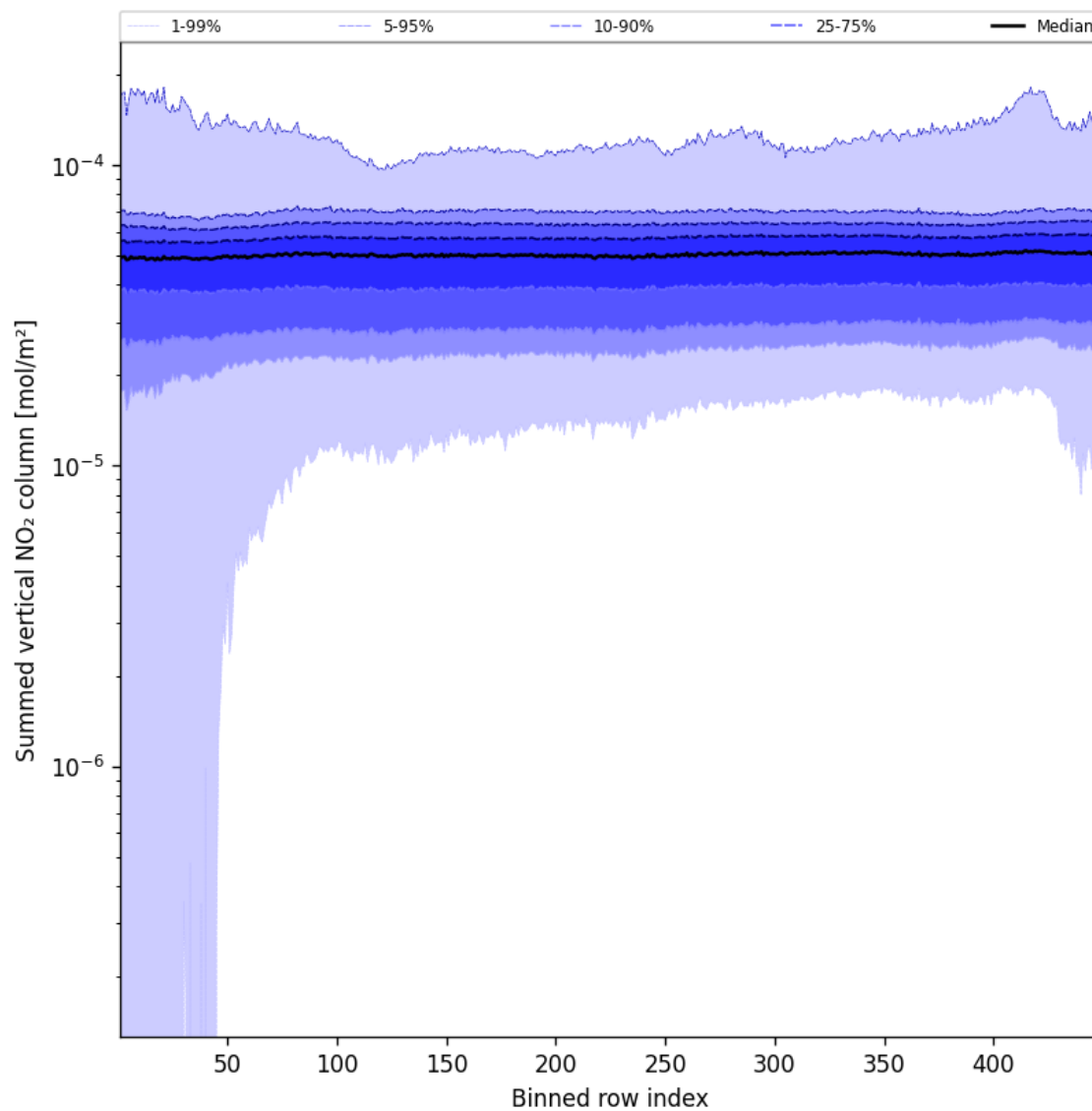
Figure 57: Along track statistics of “Summed vertical NO 2 column” for 2025-03-05 to 2025-03-05
