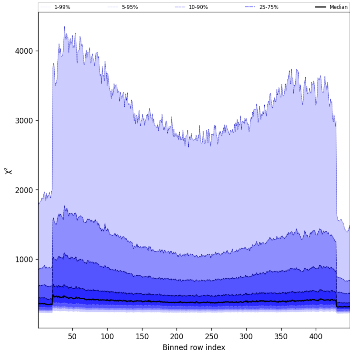
Figure 59: Along track statistics of “ \chi^2 ” for 2025-03-05 to 2025-03-05
