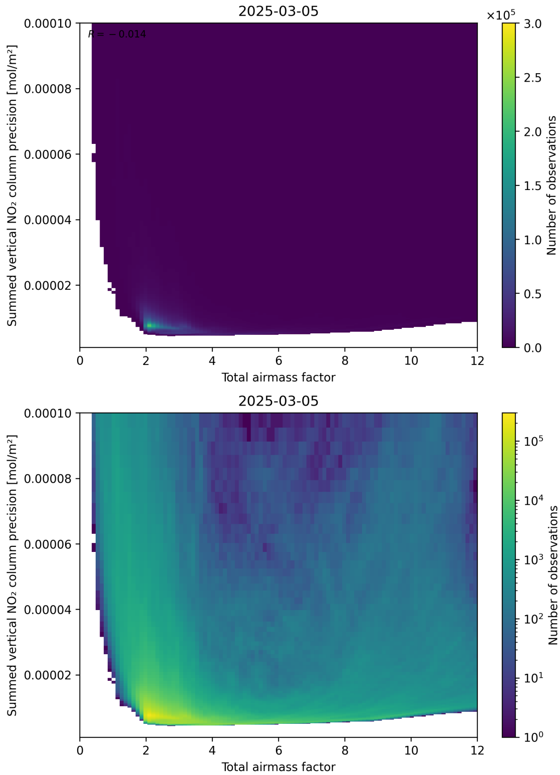
Figure 66: Scatter density plot of “Total airmass factor” against “Summed vertical NO 2 column precision” for 2025-03-05 to 2025-03-05.
