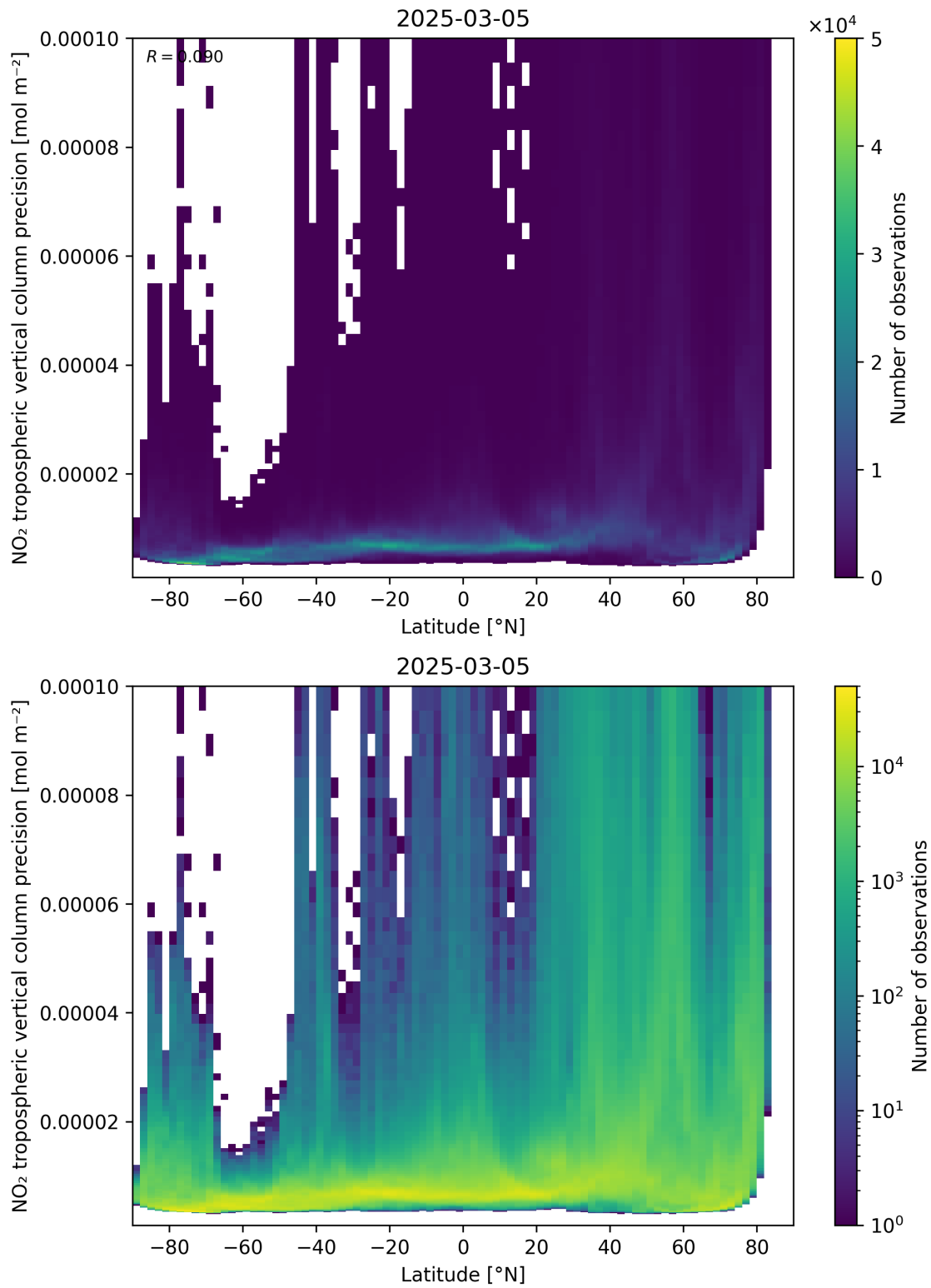
Figure 93: Scatter density plot of “Latitude” against “NO 2 tropospheric vertical column precision” for 2025-03-05 to 2025-03-05.
