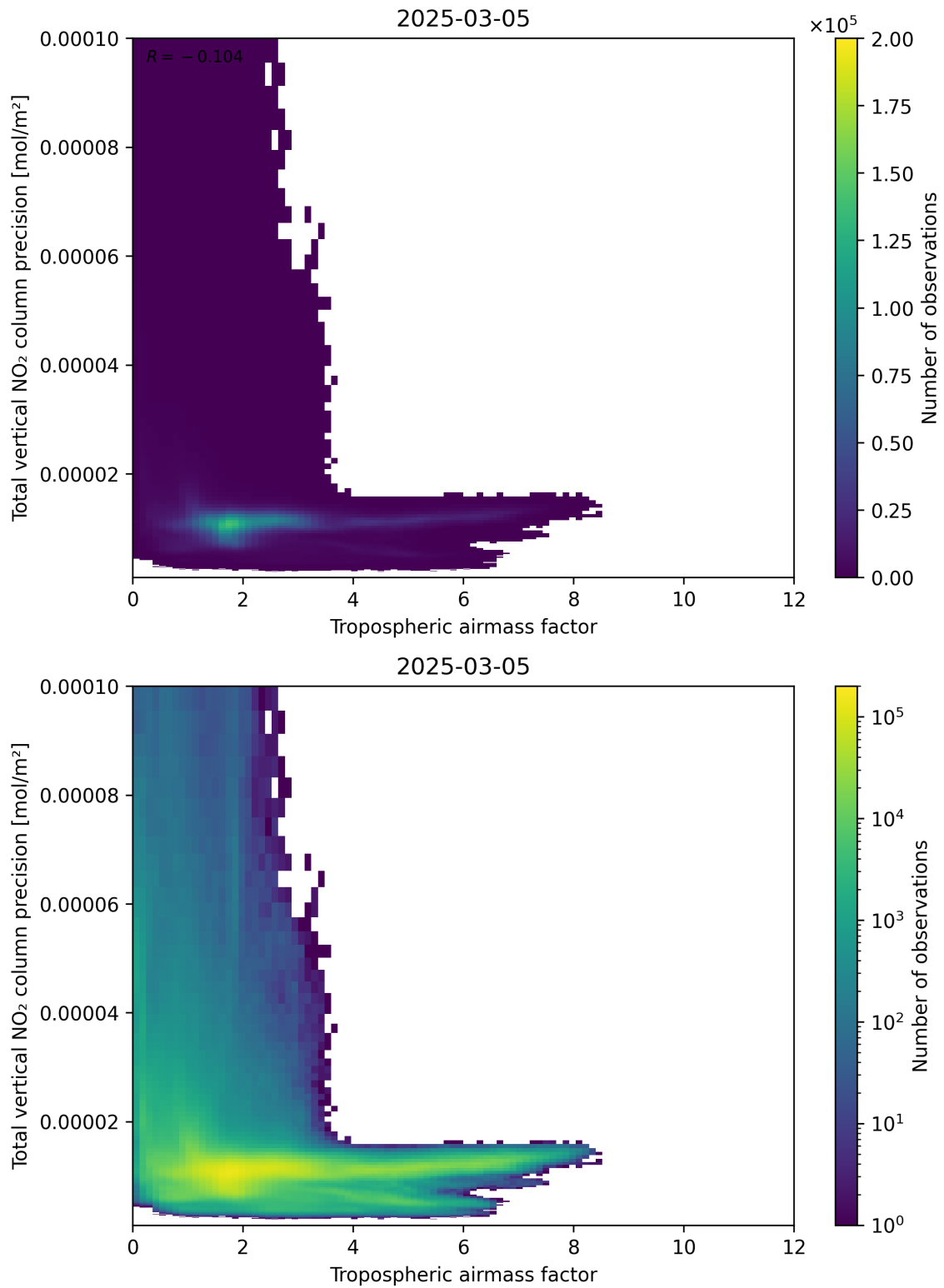
Figure 78: Scatter density plot of “Tropospheric air mass factor” against “Total vertical NO 2 column precision” for 2025-03-05 to 2025-03-05.
