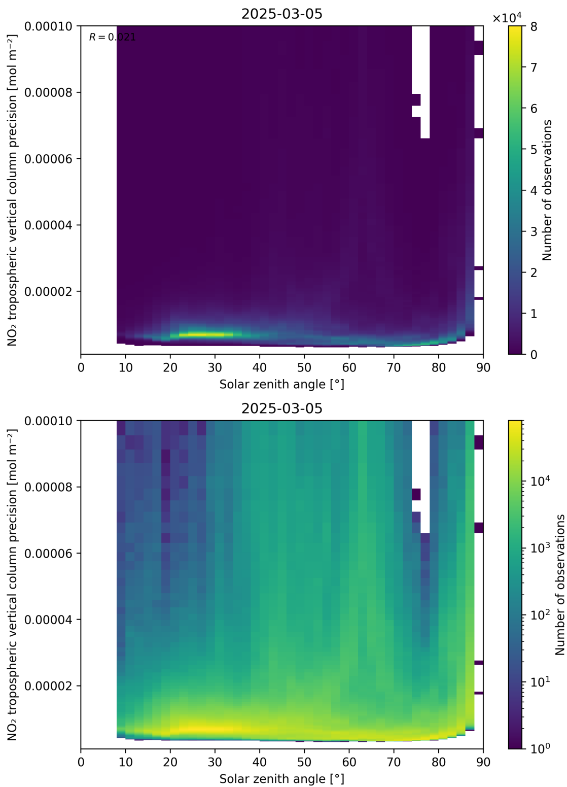
Figure 156: Scatter density plot of “Solar zenith angle” against “NO 2 tropospheric vertical column precision” for 2025-03-05 to 2025-03-05.
