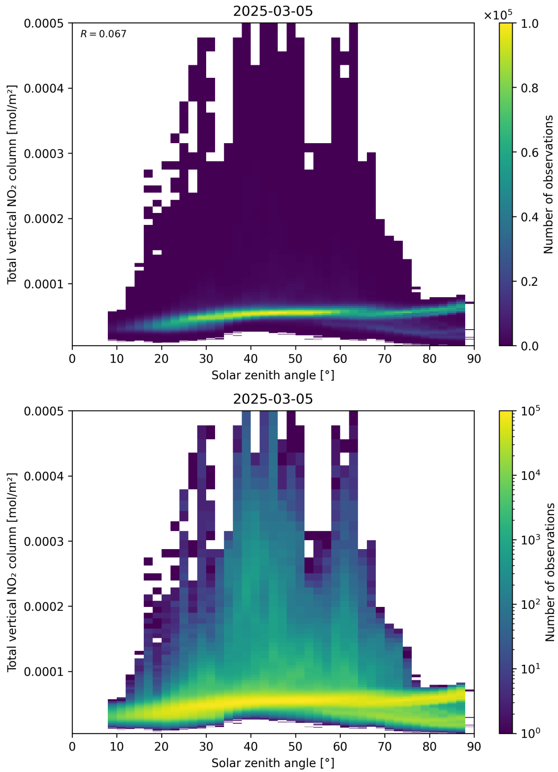
Figure 153: Scatter density plot of “Solar zenith angle” against “Total vertical NO 2 column” for 2025-03-05 to 2025-03-05.
