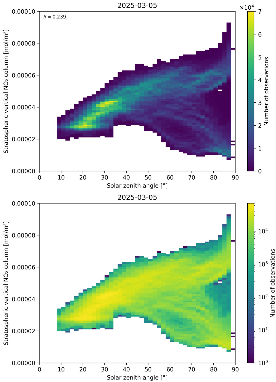
Figure 150: Scatter density plot of “Solar zenith angle” against “Stratospheric vertical NO 2 column” for 2025-03-05 to 2025-03-05.
