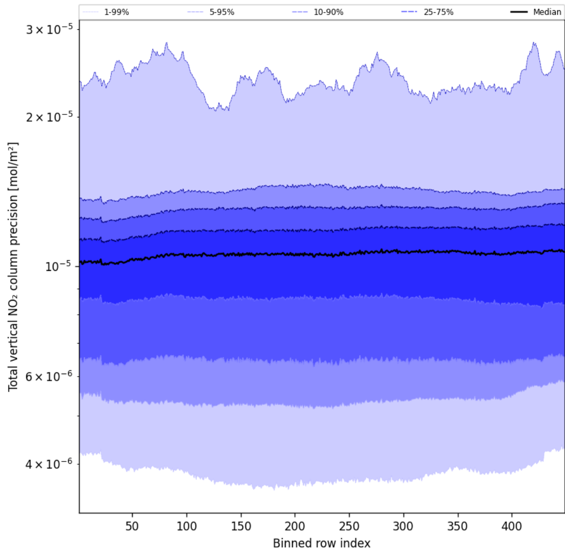
Figure 56: Along track statistics of “Total vertical NO 2 column precision” for 2025-03-05 to 2025-03-05
