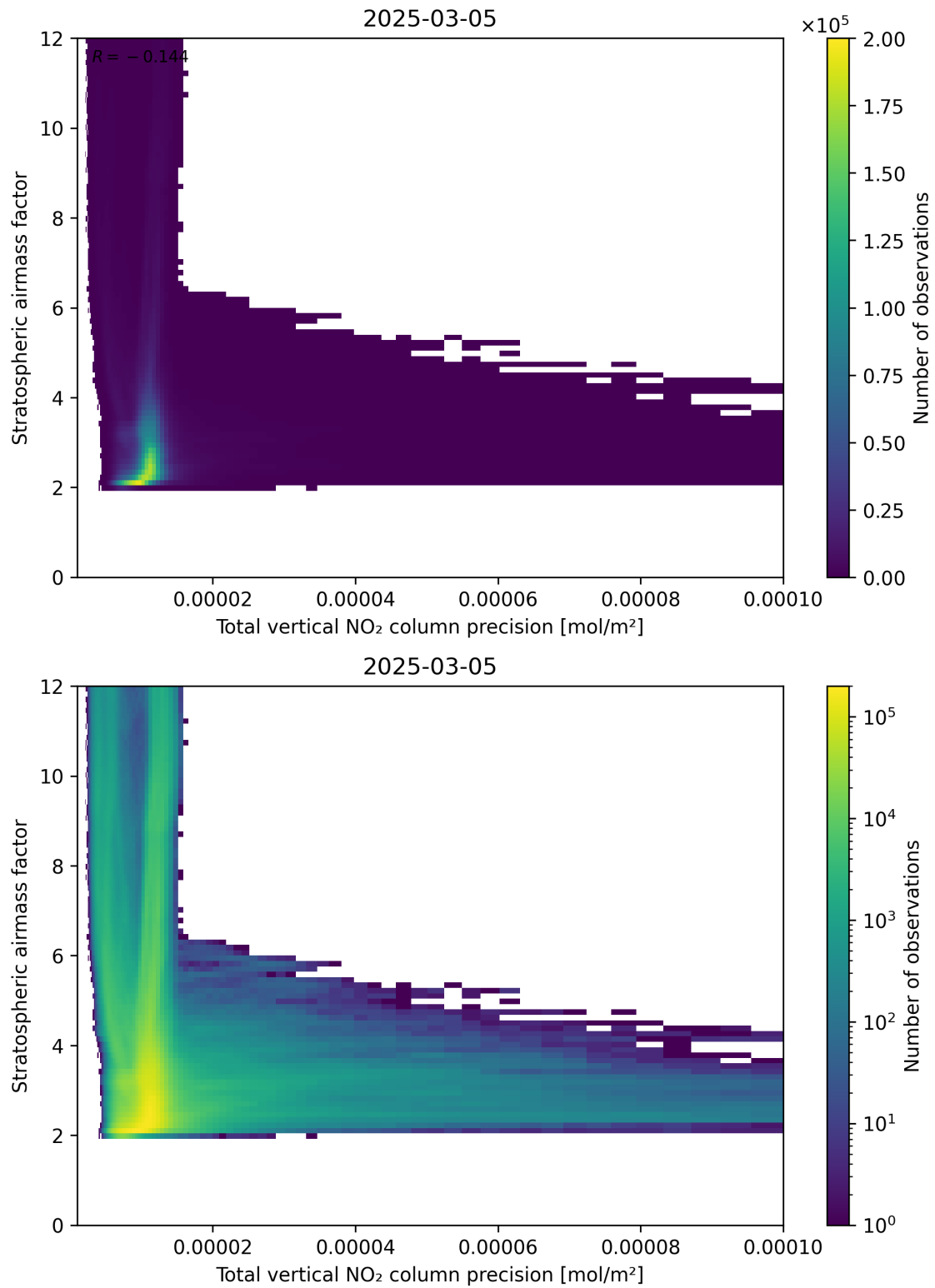
Figure 115: Scatter density plot of “Total vertical NO 2 column precision” against “Stratospheric air mass factor” for 2025-03-05 to 2025-03-05.
