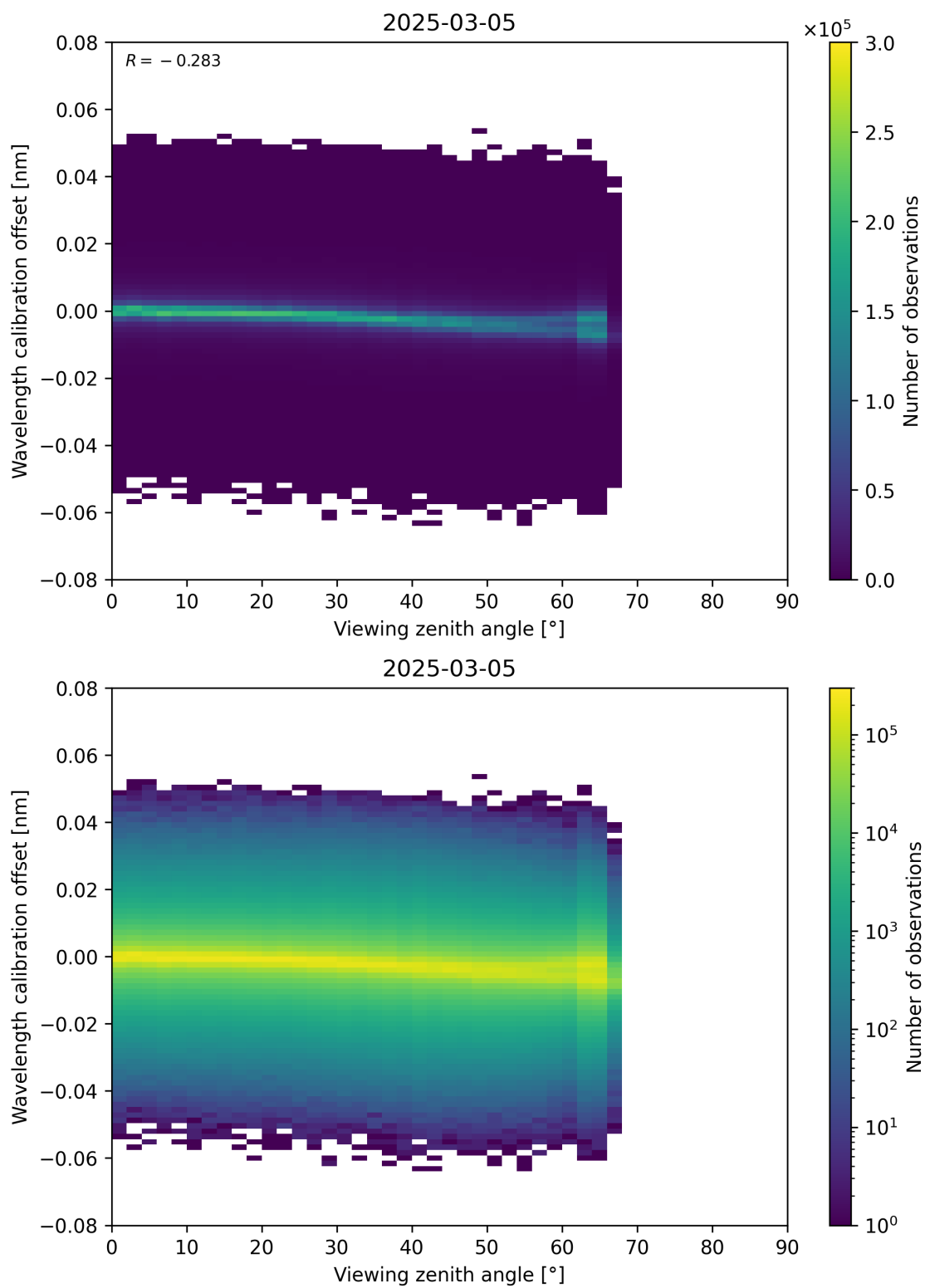
Figure 173: Scatter density plot of “Viewing zenith angle” against “Wavelength calibration offset” for 2025-03-05 to 2025-03-05.
