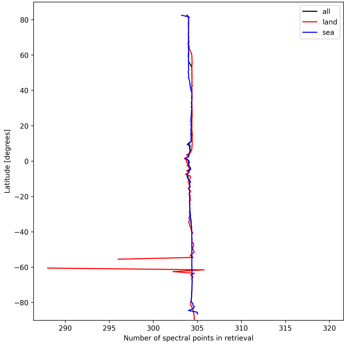
Figure 16: Zonal average of “Number of spectral points in retrieval” for 2025-03-05 to 2025-03-05.
