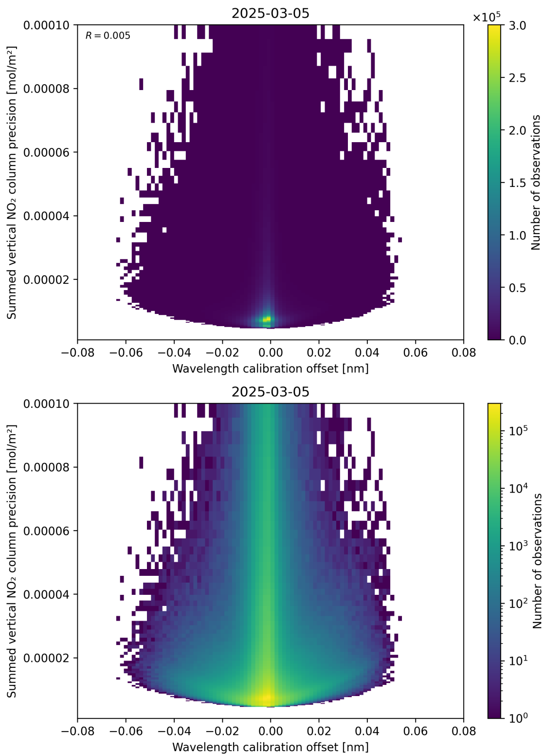
Figure 178: Scatter density plot of “Wavelength calibration offset” against “Summed vertical NO 2 column precision” for 2025-03-05 to 2025-03-05.
