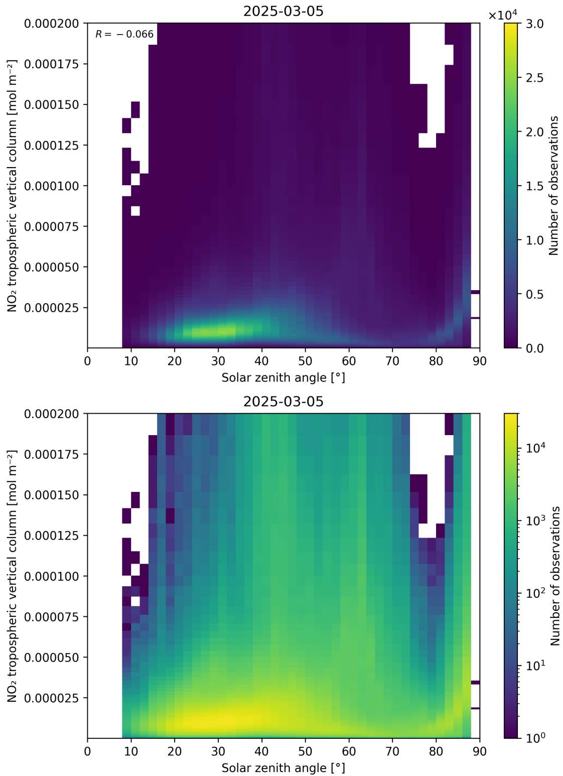
Figure 155: Scatter density plot of “Solar zenith angle” against “NO 2 tropospheric vertical column” for 2025-03-05 to 2025-03-05.
