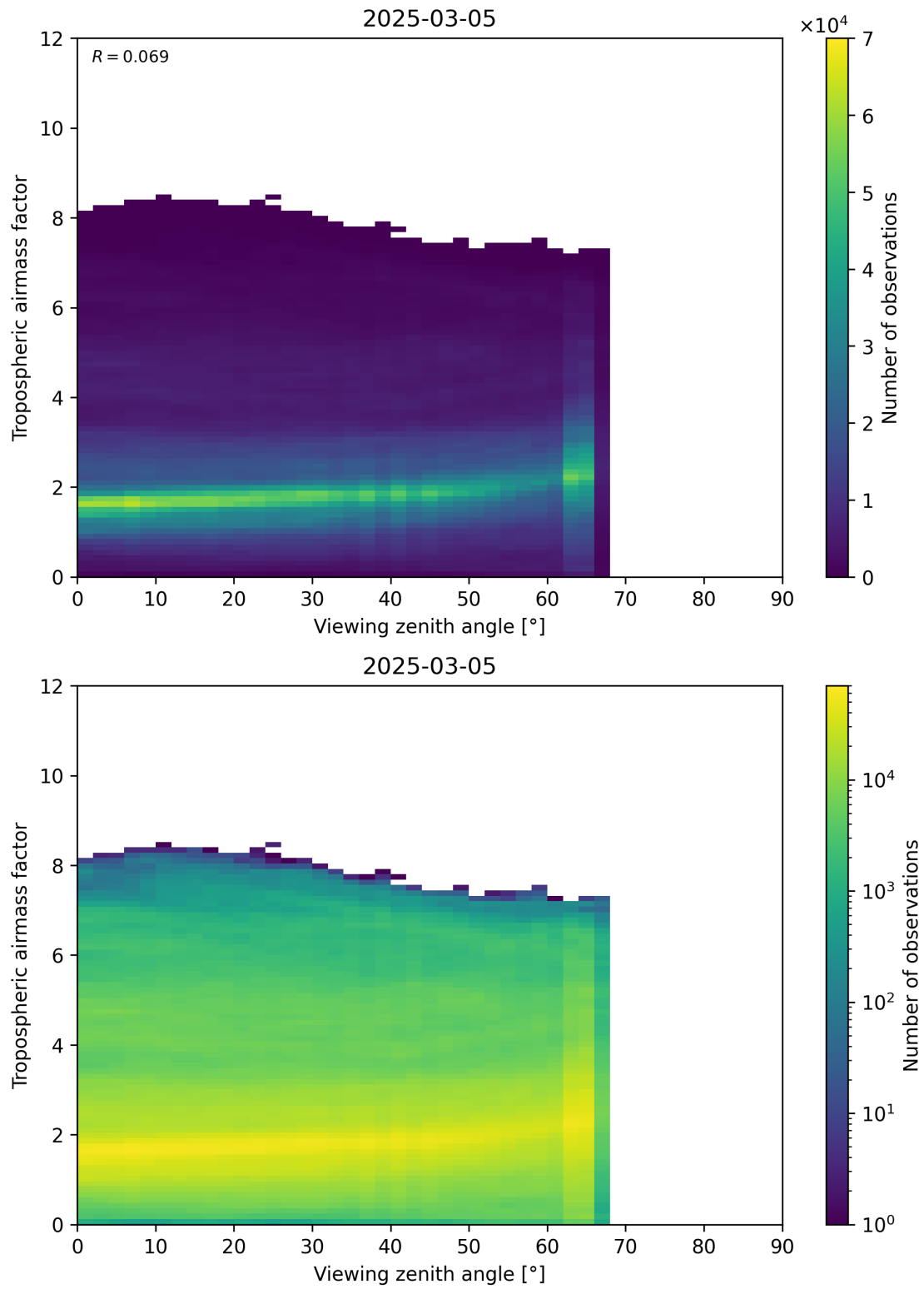
Figure 161: Scatter density plot of “Viewing zenith angle” against “Tropospheric airmass factor” for 2025-03-05 to 2025-03-05.
