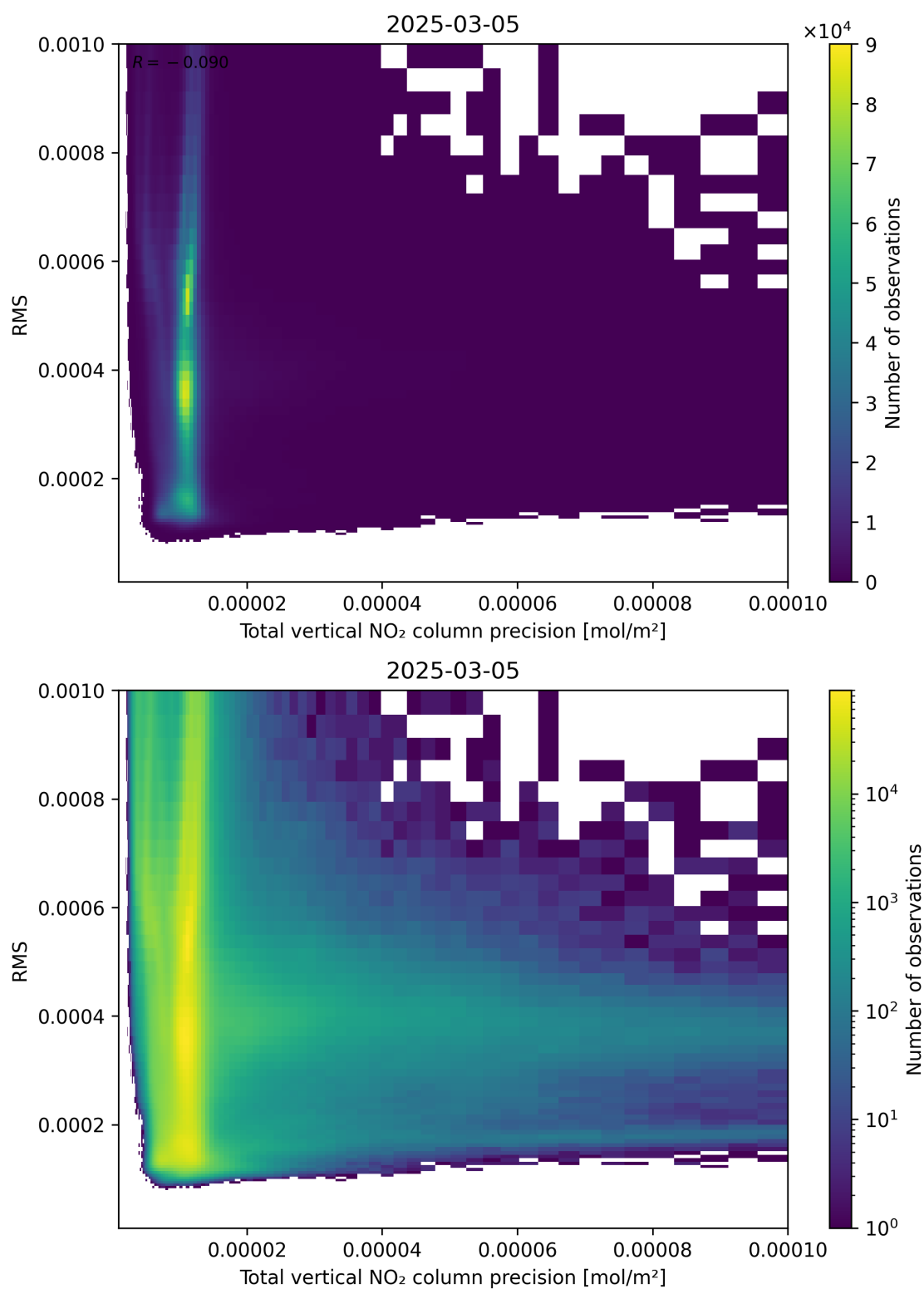
Figure 119: Scatter density plot of “Total vertical NO 2 column precision” against “RMS” for 2025-03-05 to 2025-03-05.
