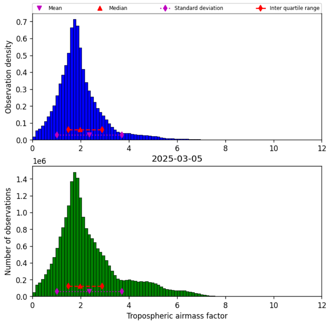
Figure 31: Histogram of “Tropospheric airmass factor” for 2025-03-05 to 2025-03-05
