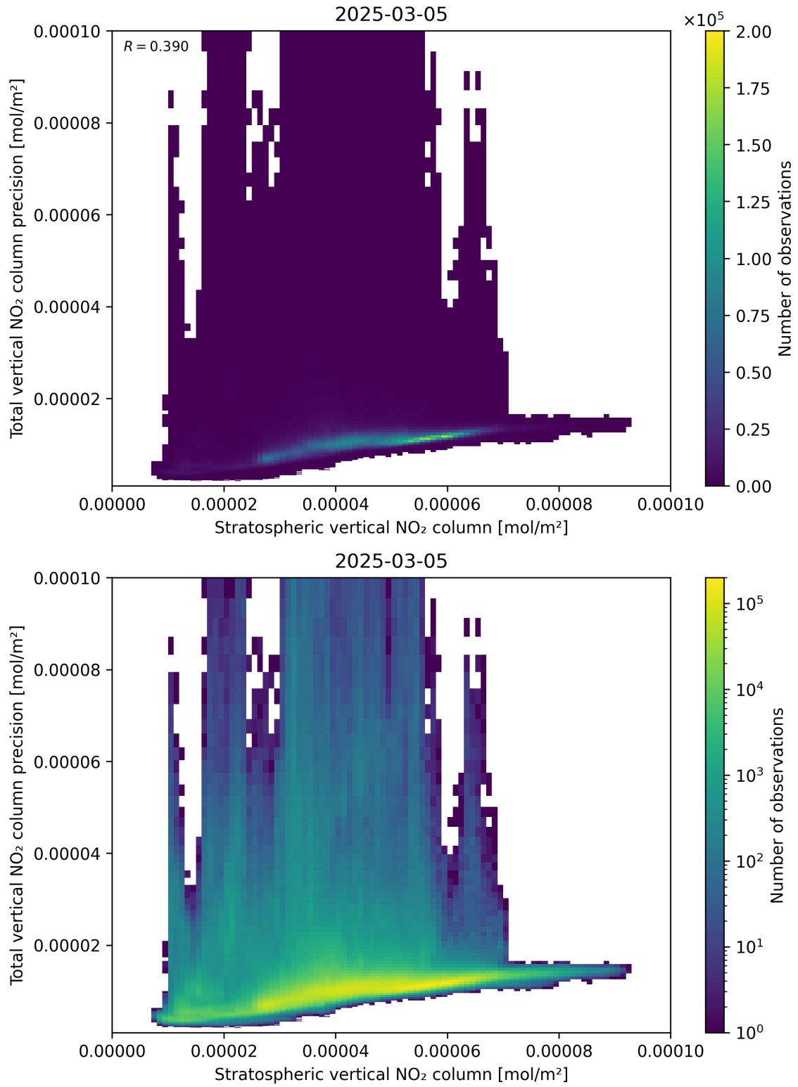
Figure 101: Scatter density plot of “Stratospheric vertical NO 2 column” against “Total vertical NO 2 column precision” for 2025-03-05 to 2025-03-05.
