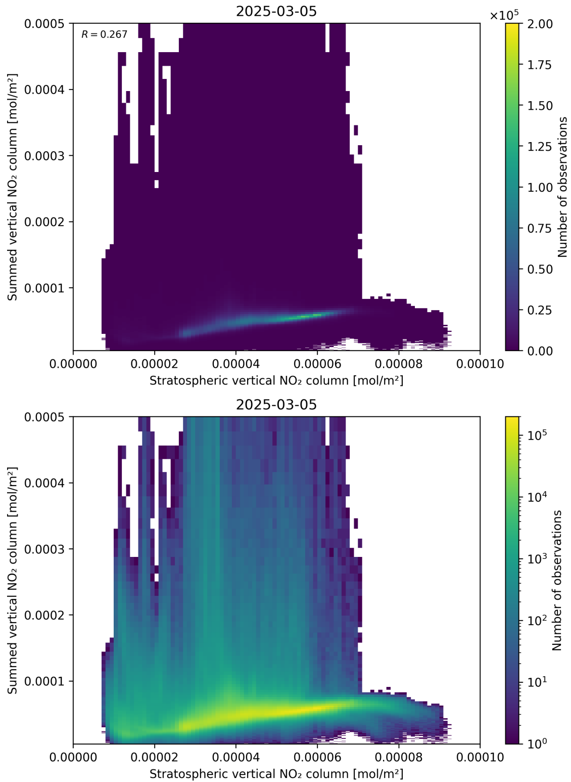
Figure 98: Scatter density plot of “Stratospheric vertical NO 2 column” against “Summed vertical NO 2 column” for 2025-03-05 to 2025-03-05.
