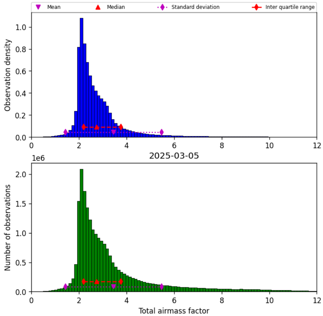
Figure 32: Histogram of “Total airmass factor” for 2025-03-05 to 2025-03-05
