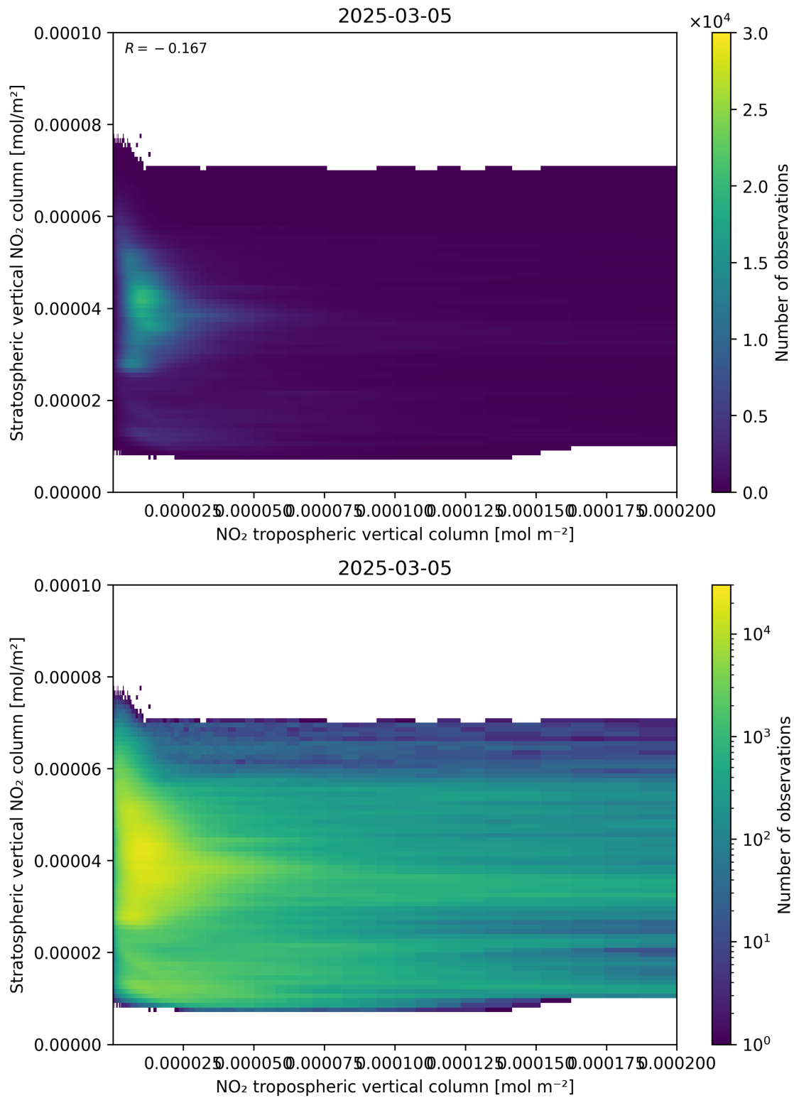
Figure 125: Scatter density plot of “NO 2 tropospheric vertical column” against “Stratospheric vertical NO 2 column” for 2025-03-05 to 2025-03-05.
