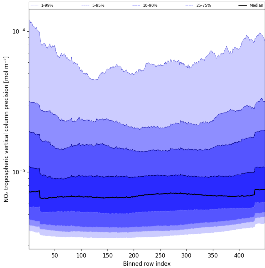
Figure 47: Along track statistics of “NO 2 tropospheric vertical column precision” for 2025-03-05 to 2025-03-05
