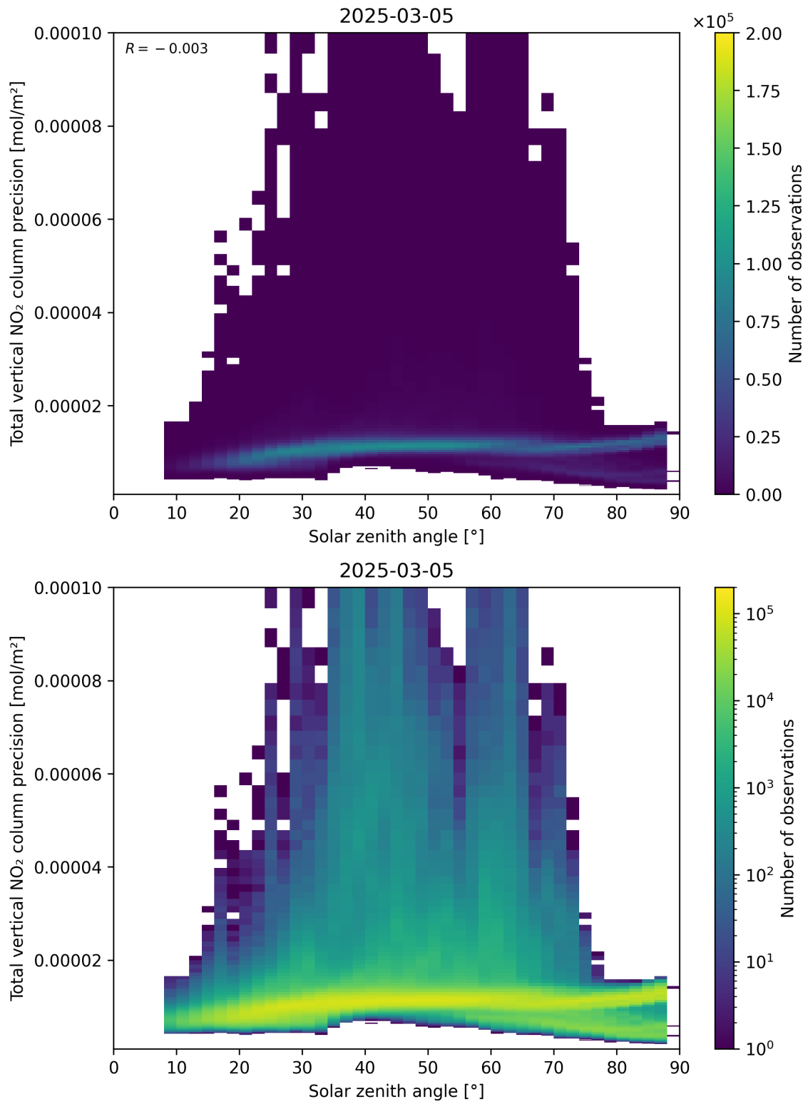
Figure 154: Scatter density plot of “Solar zenith angle” against “Total vertical NO 2 column precision” for 2025-03-05 to 2025-03-05.
