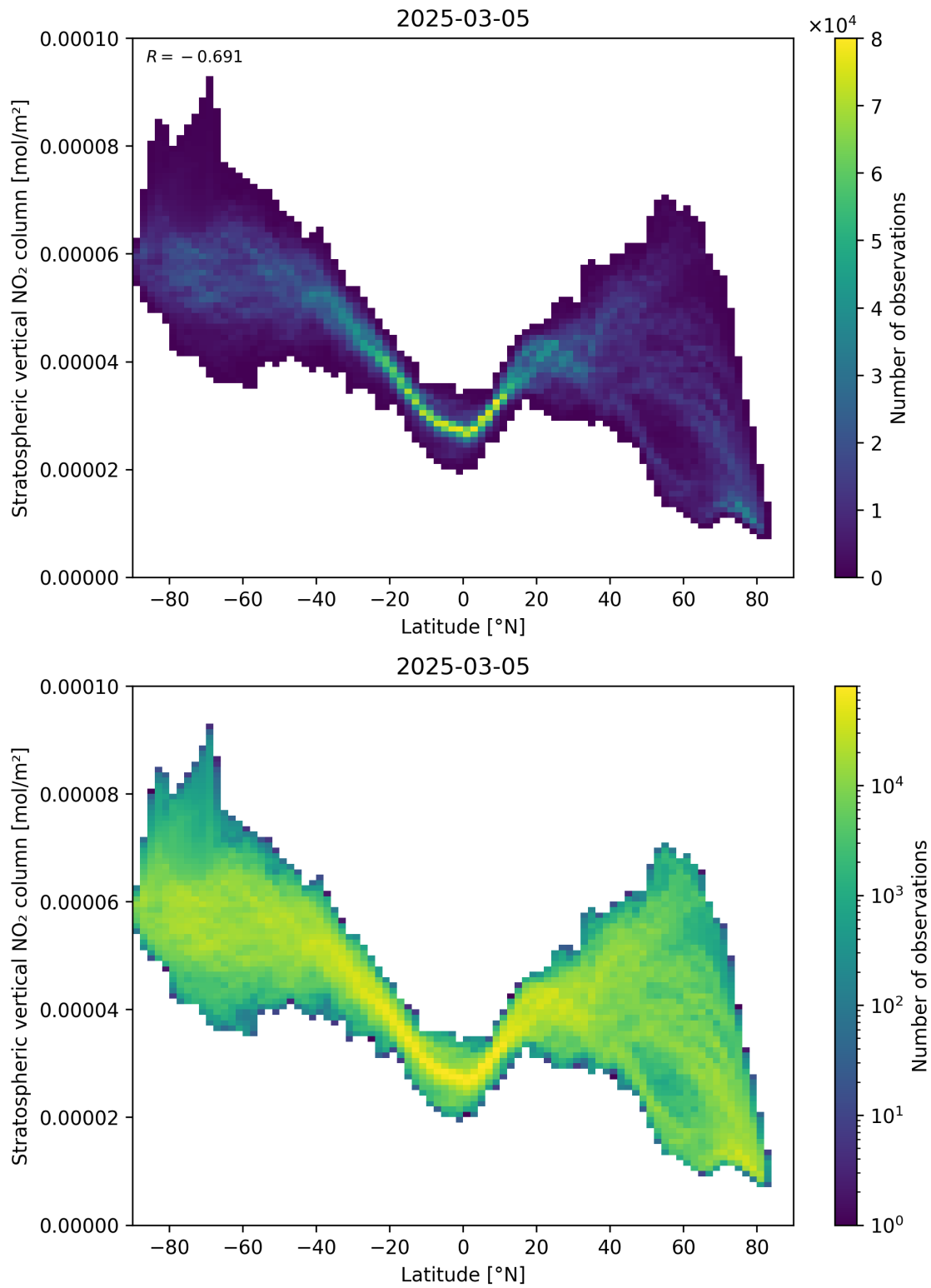
Figure 87: Scatter density plot of “Latitude” against “Stratospheric vertical NO 2 column” for 2025-03-05 to 2025-03-05.
