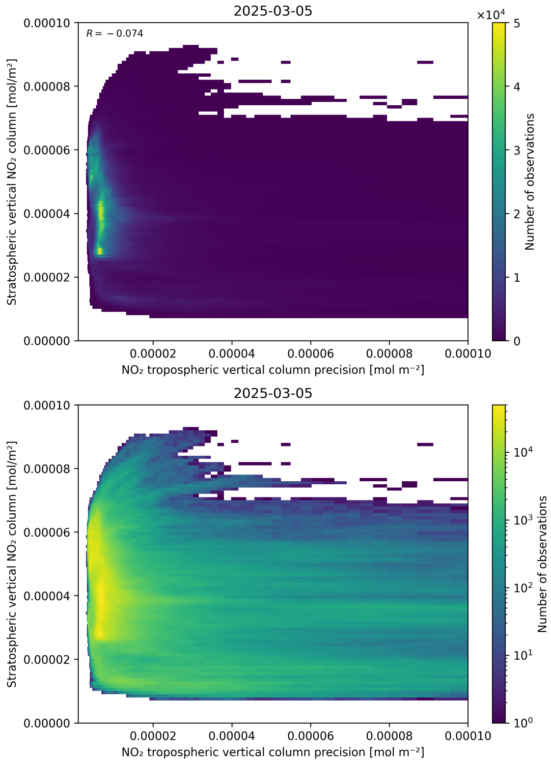
Figure 135: Scatter density plot of “NO 2 tropospheric vertical column precision” against “Stratospheric vertical NO 2 column” for 2025-03-05 to 2025-03-05.
