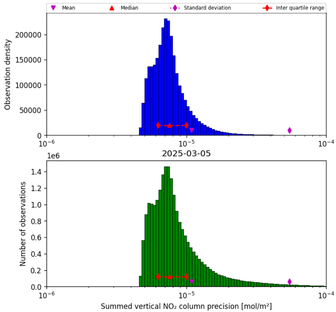
Figure 41: Histogram of "Summed vertical NO 2 column precision" for 2025-03-05 to 2025-03-05
