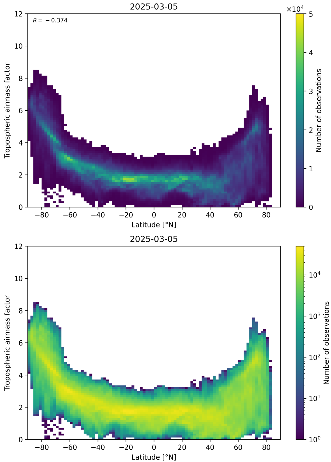
Figure 85: Scatter density plot of “Latitude” against “Tropospheric airmass factor” for 2025-03-05 to 2025-03-05.
