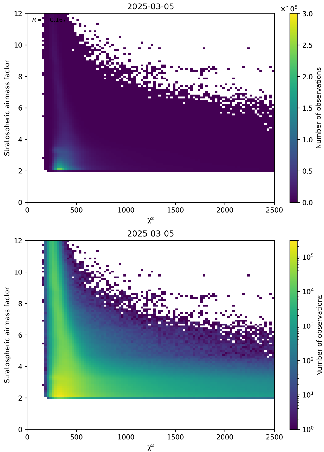
Figure 81: Scatter density plot of " \chi^2 " against "Stratospheric airmass factor" for 2025-03-05 to 2025-03-05.
