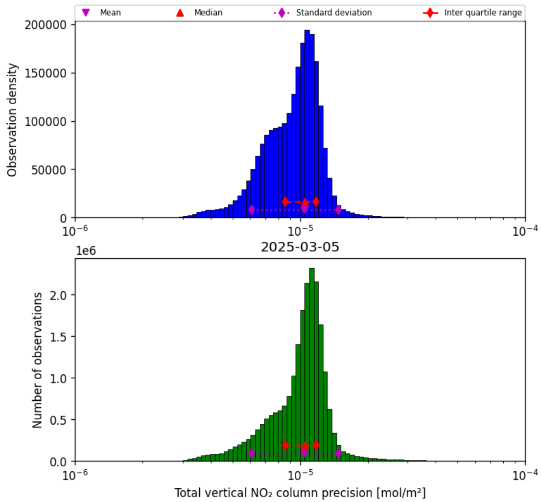
Figure 39: Histogram of “Total vertical NO 2 column precision” for 2025-03-05 to 2025-03-05
