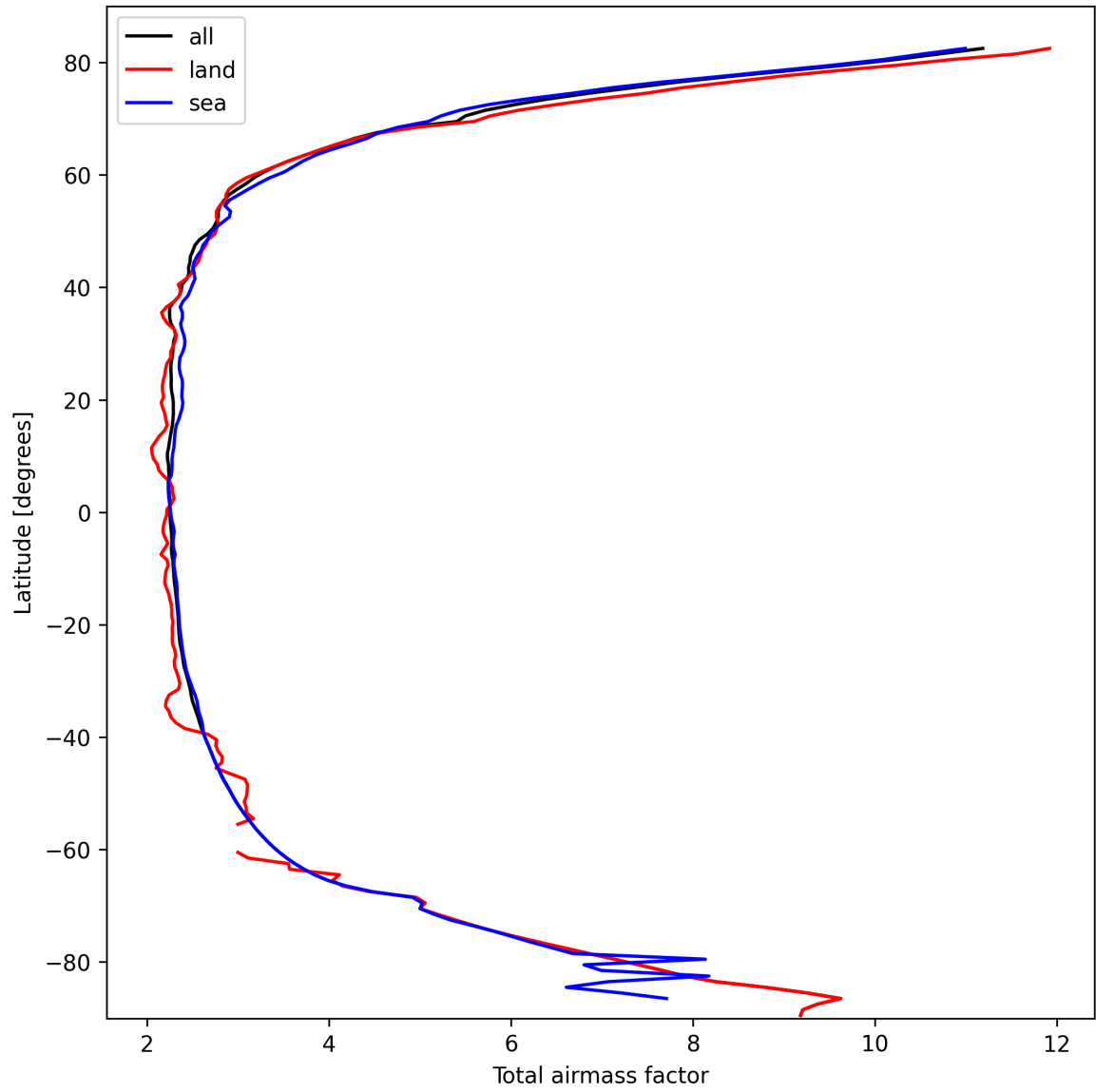
Figure 15: Zonal average of “Total airmass factor” for 2025-03-05 to 2025-03-05.
