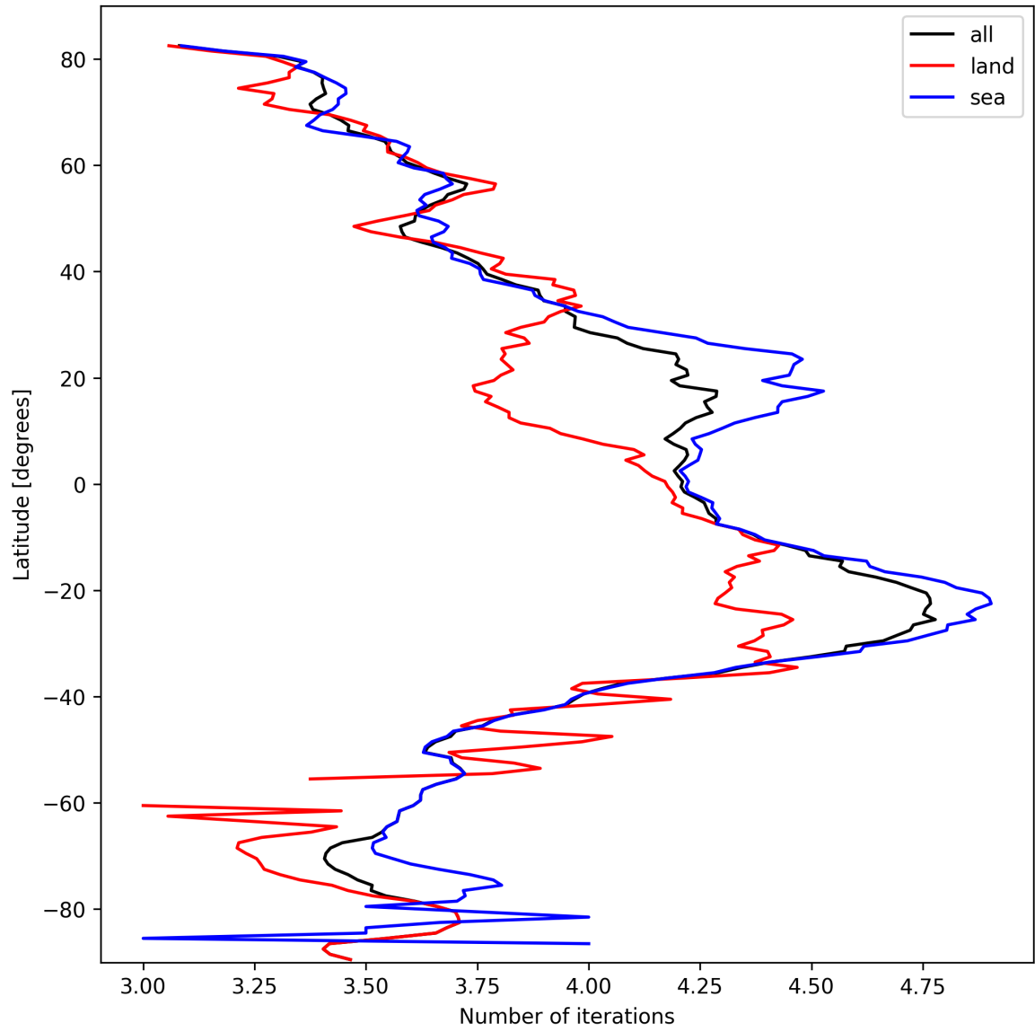
Figure 17: Zonal average of “Number of iterations” for 2025-03-05 to 2025-03-05.
