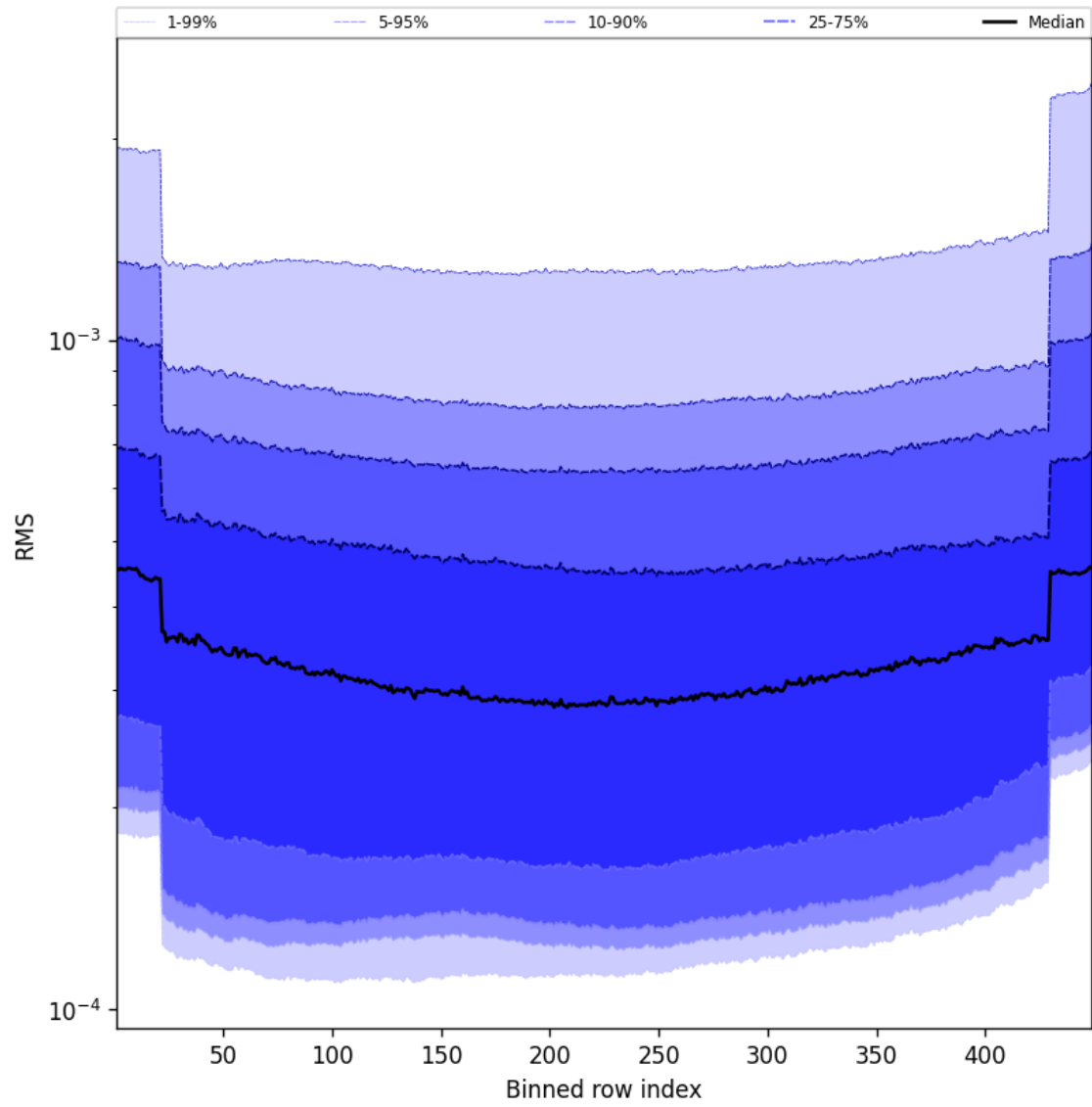
Figure 60: Along track statistics of “RMS” for 2025-03-05 to 2025-03-05
