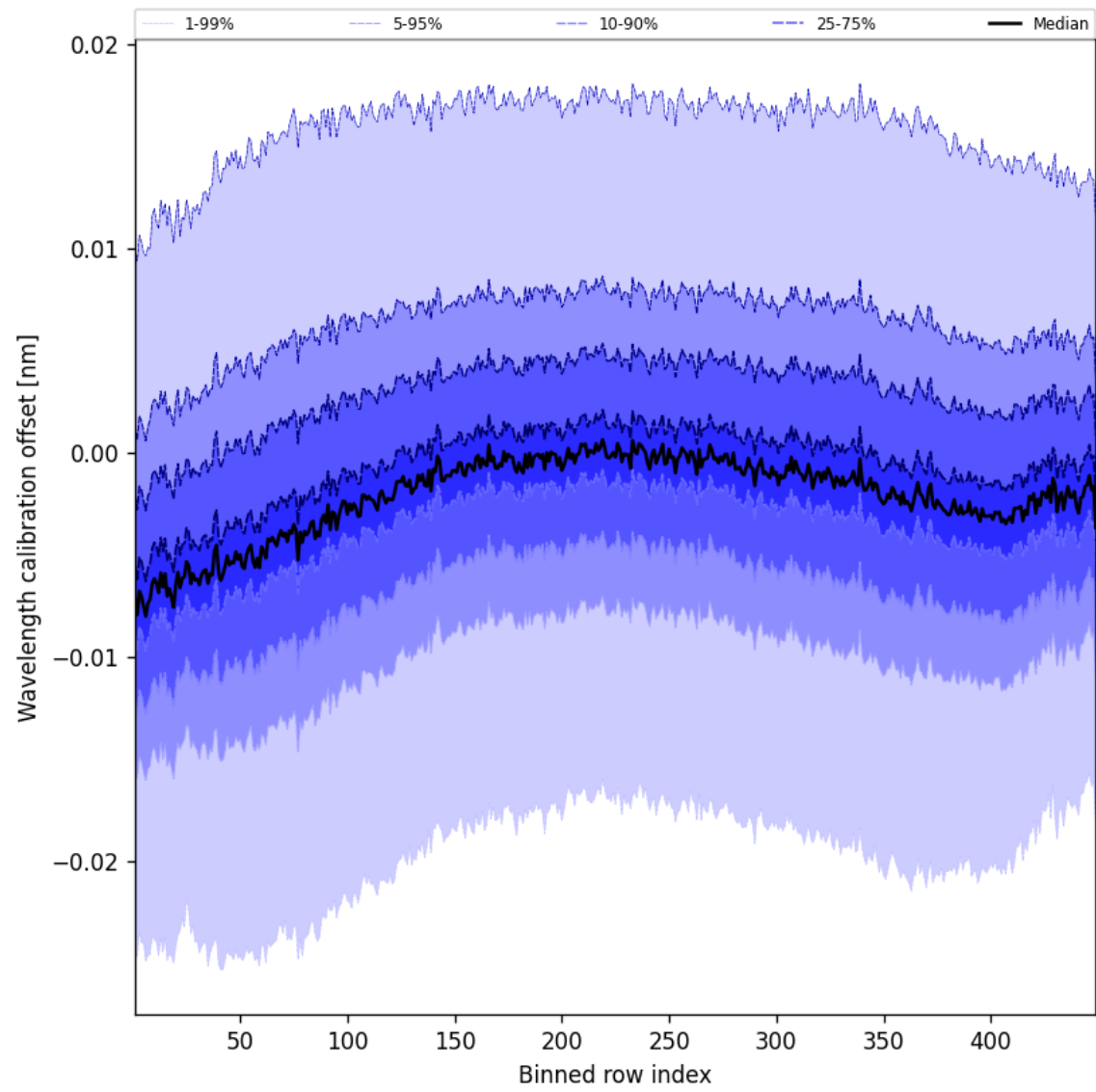
Figure 52: Along track statistics of “Wavelength calibration offset” for 2025-03-05 to 2025-03-05
