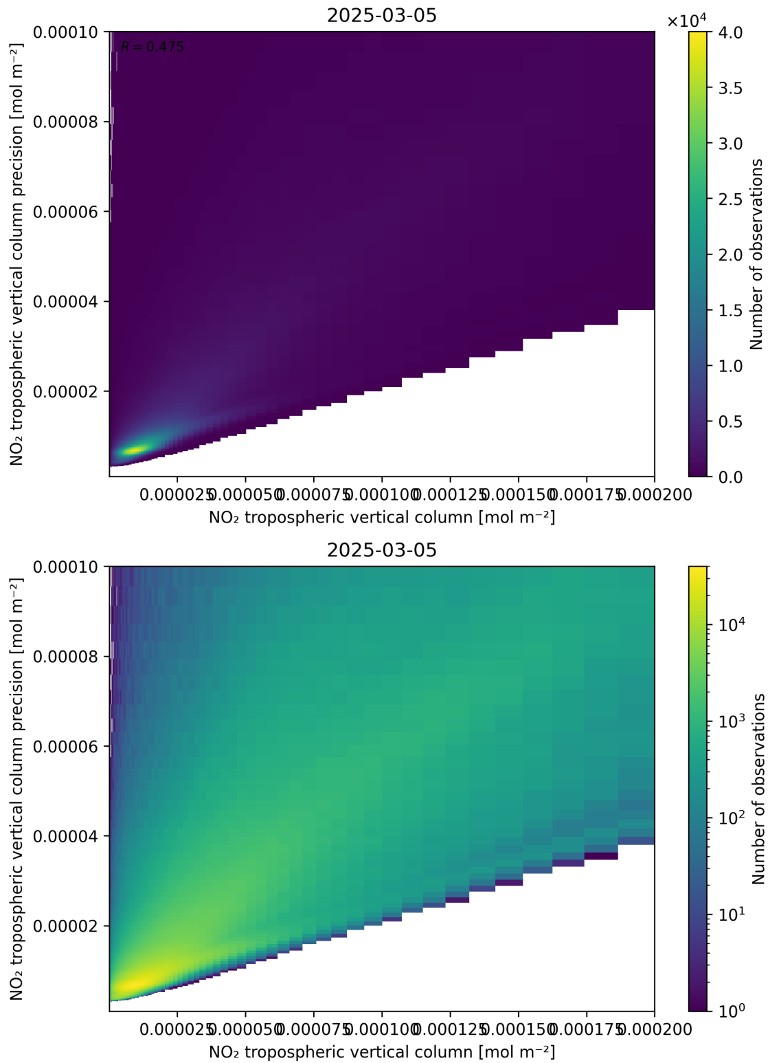
Figure 130: Scatter density plot of “NO 2 tropospheric vertical column” against “NO 2 tropospheric vertical column precision” for 2025-03-05 to 2025-03-05.
