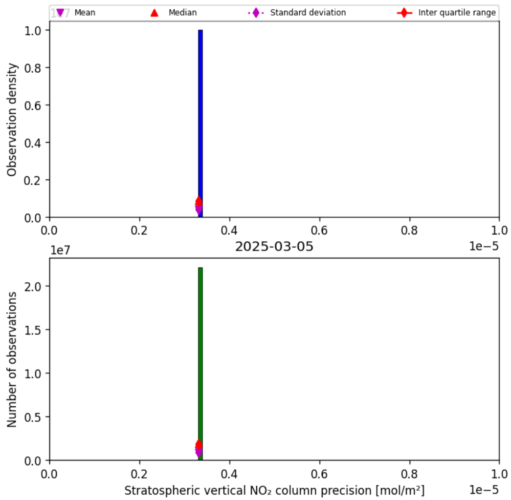
Figure 37: Histogram of “Stratospheric vertical NO 2 column precision” for 2025-03-05 to 2025-03-05
