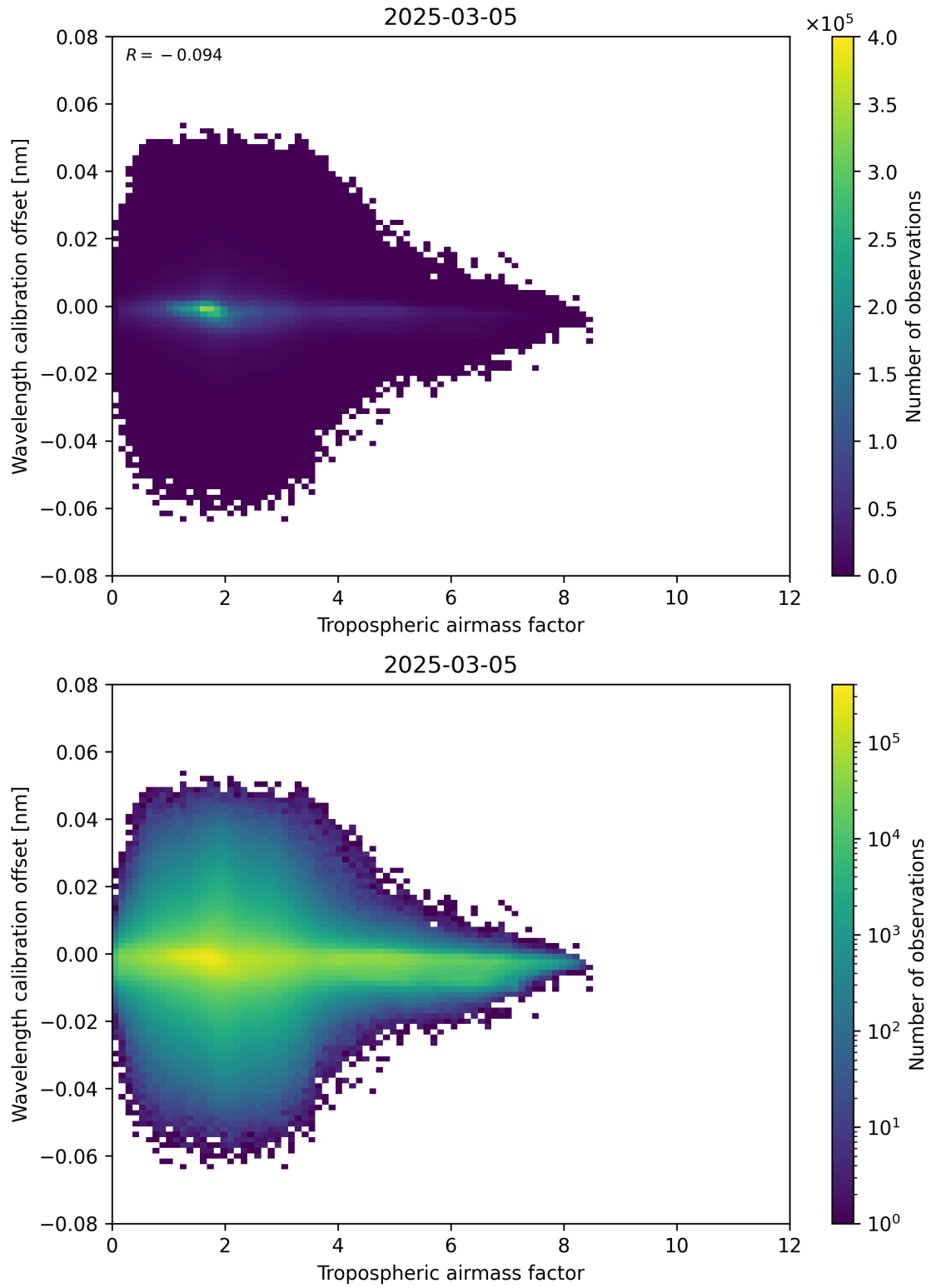
Figure 80: Scatter density plot of “Tropospheric airmass factor” against “Wavelength calibration offset” for 2025-03-05 to 2025-03-05.
