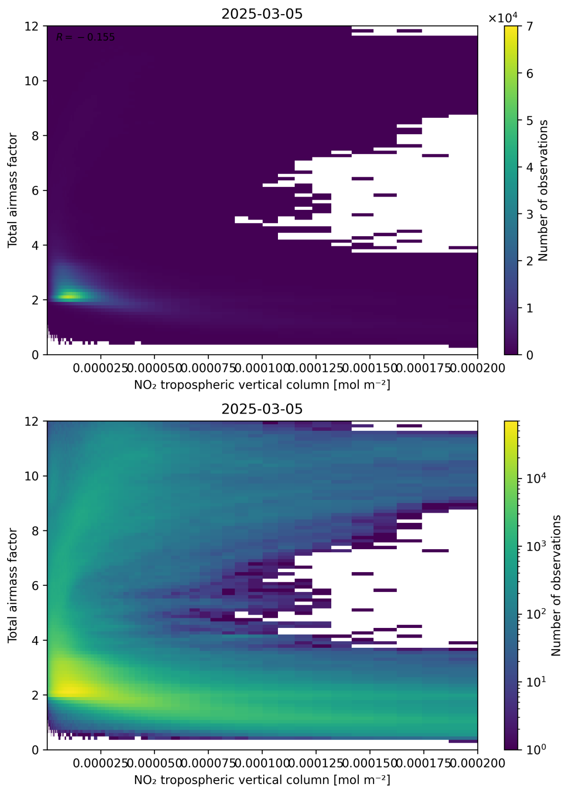
Figure 122: Scatter density plot of “NO 2 tropospheric vertical column” against “Total air mass factor” for 2025-03-05 to 2025-03-05.
