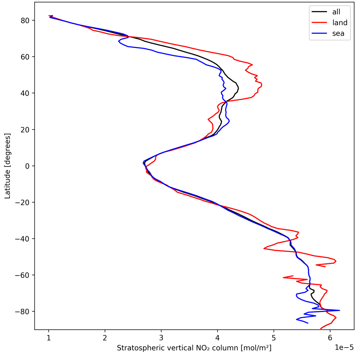
Figure 19: Zonal average of “Stratospheric vertical NO 2 column” for 2025-03-05 to 2025-03-05.
