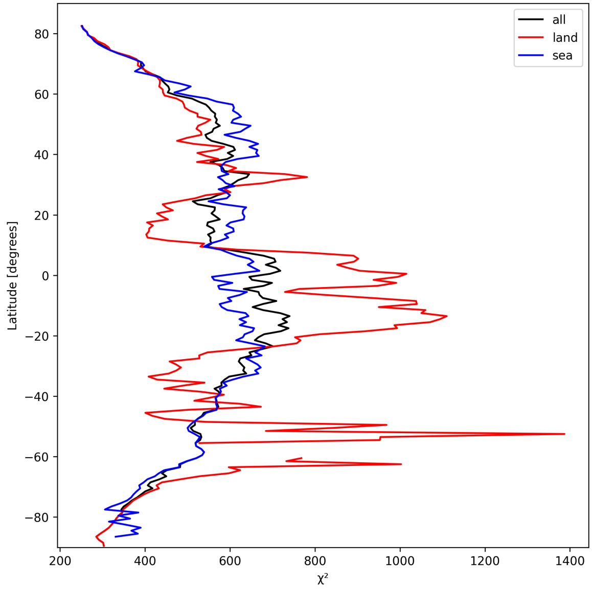
Figure 25: Zonal average of “ \chi^2 ” for 2025-03-05 to 2025-03-05.
