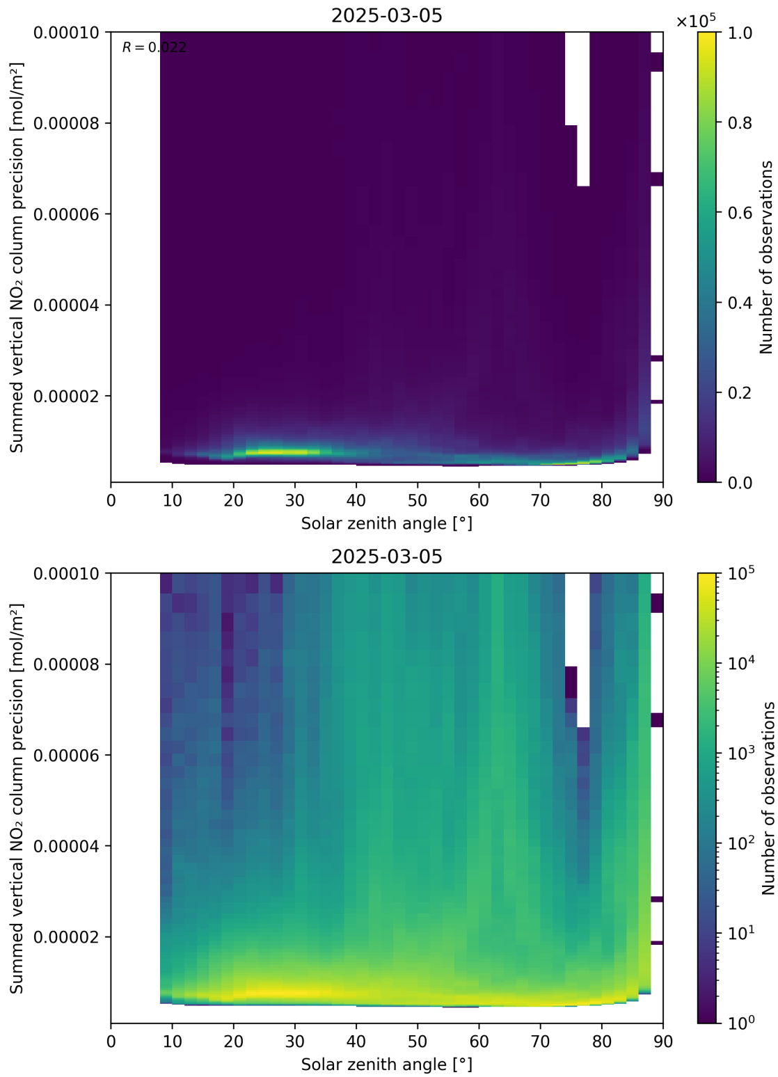
Figure 152: Scatter density plot of “Solar zenith angle” against “Summed vertical NO 2 column precision” for 2025-03-05 to 2025-03-05.
