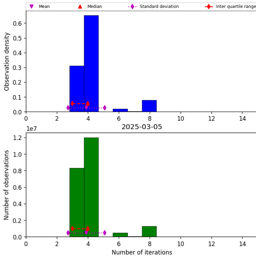
Figure 34: Histogram of "Number of iterations" for 2025-03-05 to 2025-03-05
