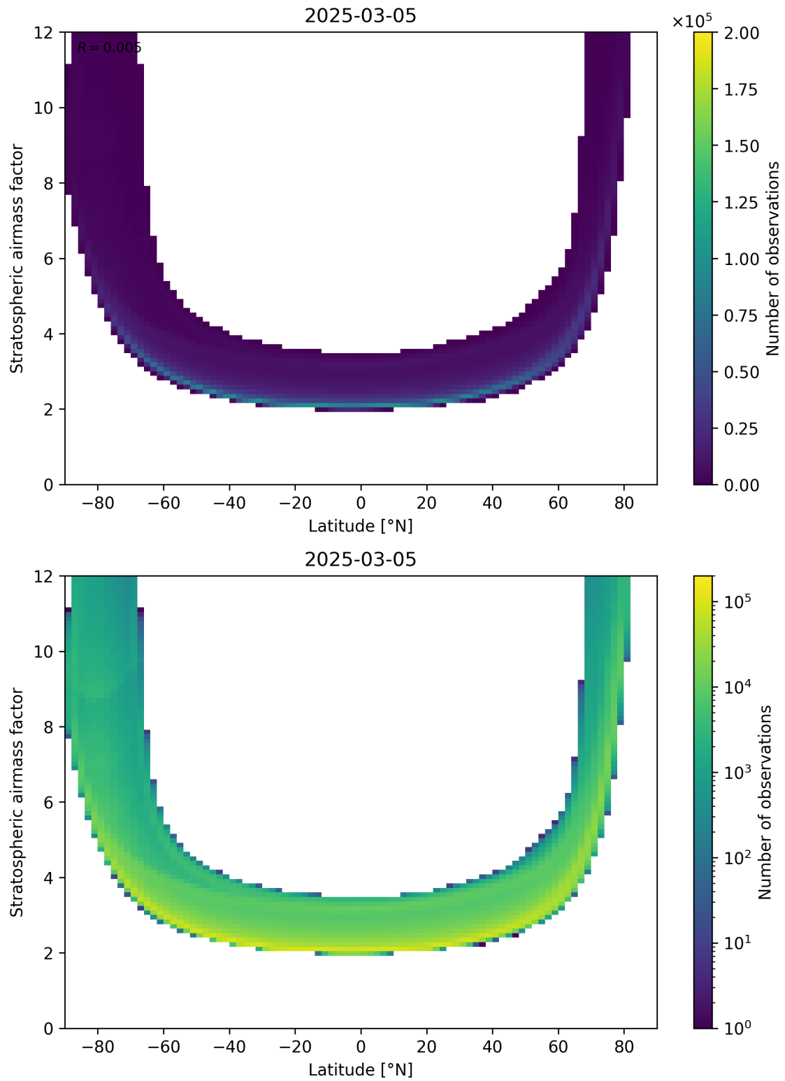
Figure 83: Scatter density plot of “Latitude” against “Stratospheric airmass factor” for 2025-03-05 to 2025-03-05.
