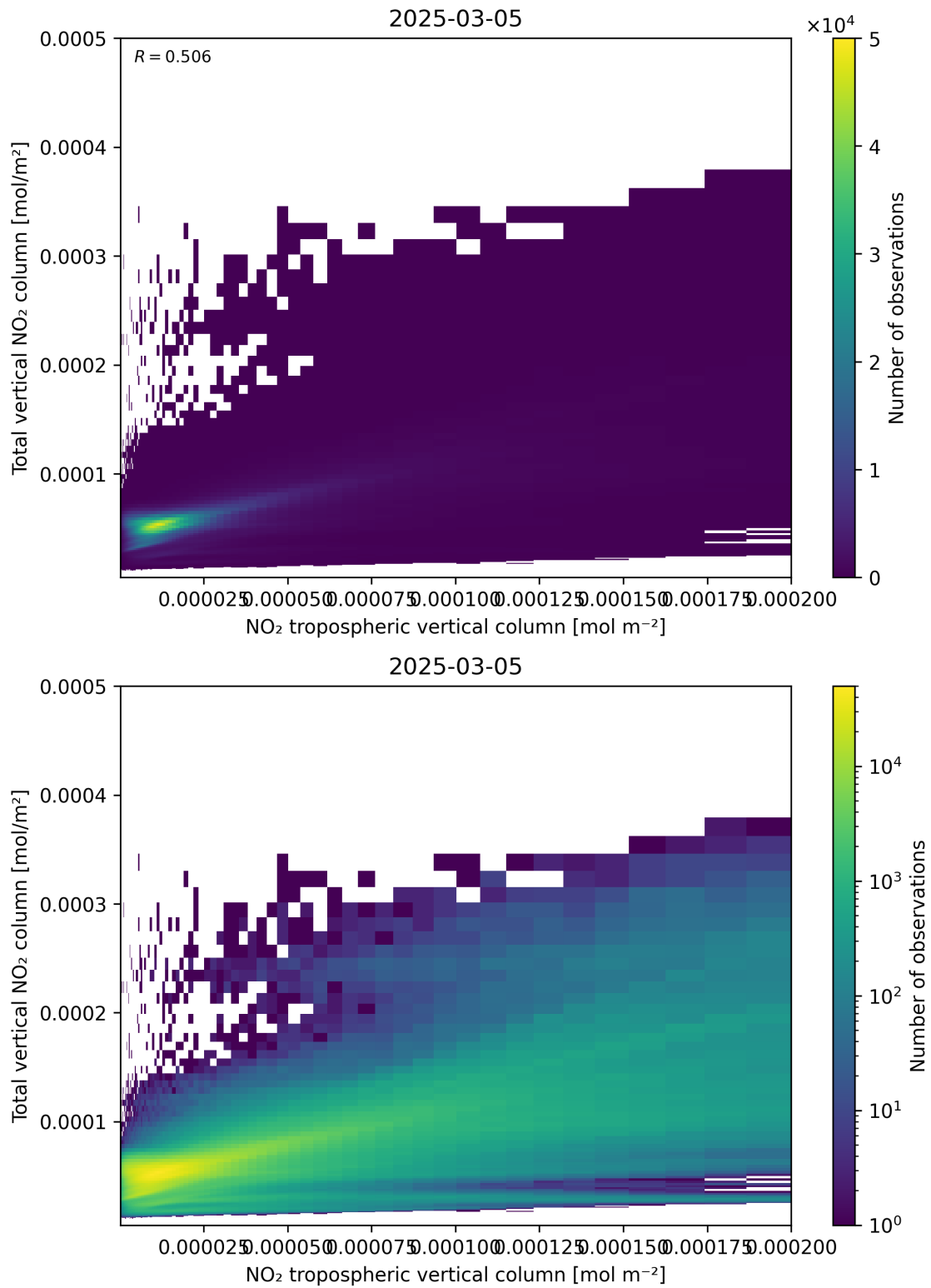
Figure 128: Scatter density plot of “NO 2 tropospheric vertical column” against “Total vertical NO 2 column” for 2025-03-05 to 2025-03-05.
