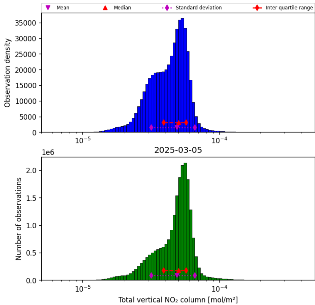
Figure 38: Histogram of “Total vertical NO 2 column” for 2025-03-05 to 2025-03-05
