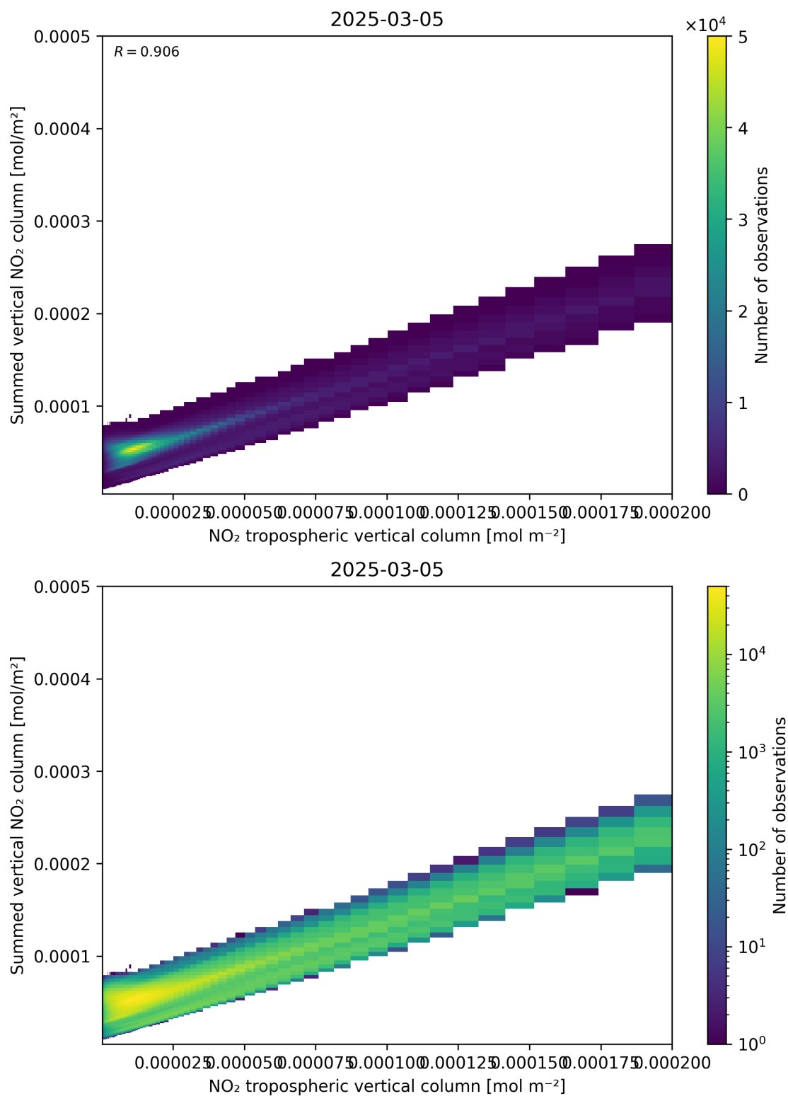
Figure 126: Scatter density plot of “NO 2 tropospheric vertical column” against “Summed vertical NO 2 column” for 2025-03-05 to 2025-03-05.
