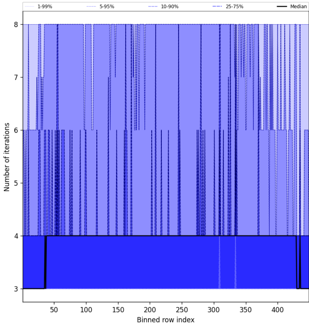
Figure 51: Along track statistics of “Number of iterations” for 2025-03-05 to 2025-03-05
