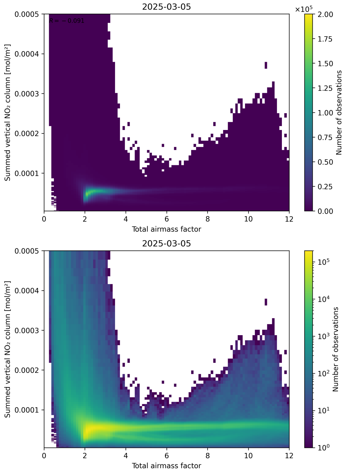
Figure 65: Scatter density plot of “Total airmass factor” against “Summed vertical NO 2 column” for 2025-03-05 to 2025-03-05.
