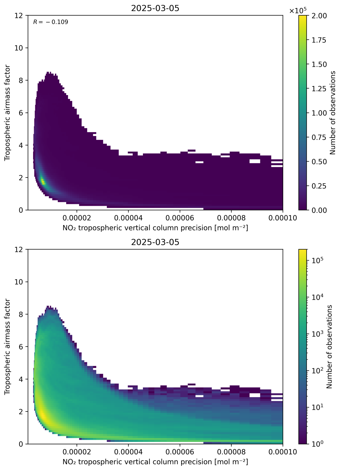
Figure 133: Scatter density plot of “NO 2 tropospheric vertical column precision” against “Tropospheric air mass factor” for 2025-03-05 to 2025-03-05.
