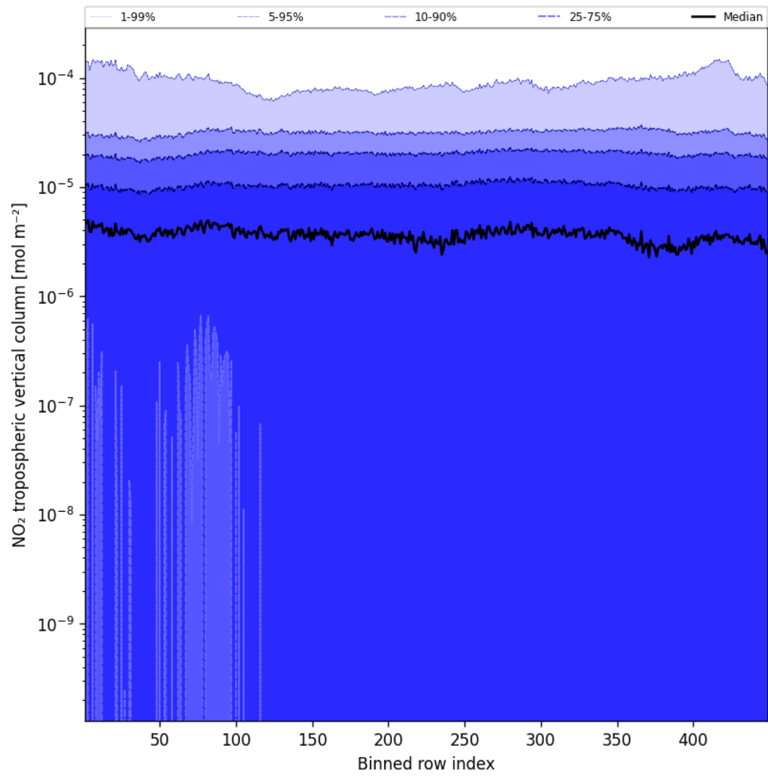
Figure 46: Along track statistics of “ \text{NO}_2 tropospheric vertical column” for 2025-03-05 to 2025-03-05
