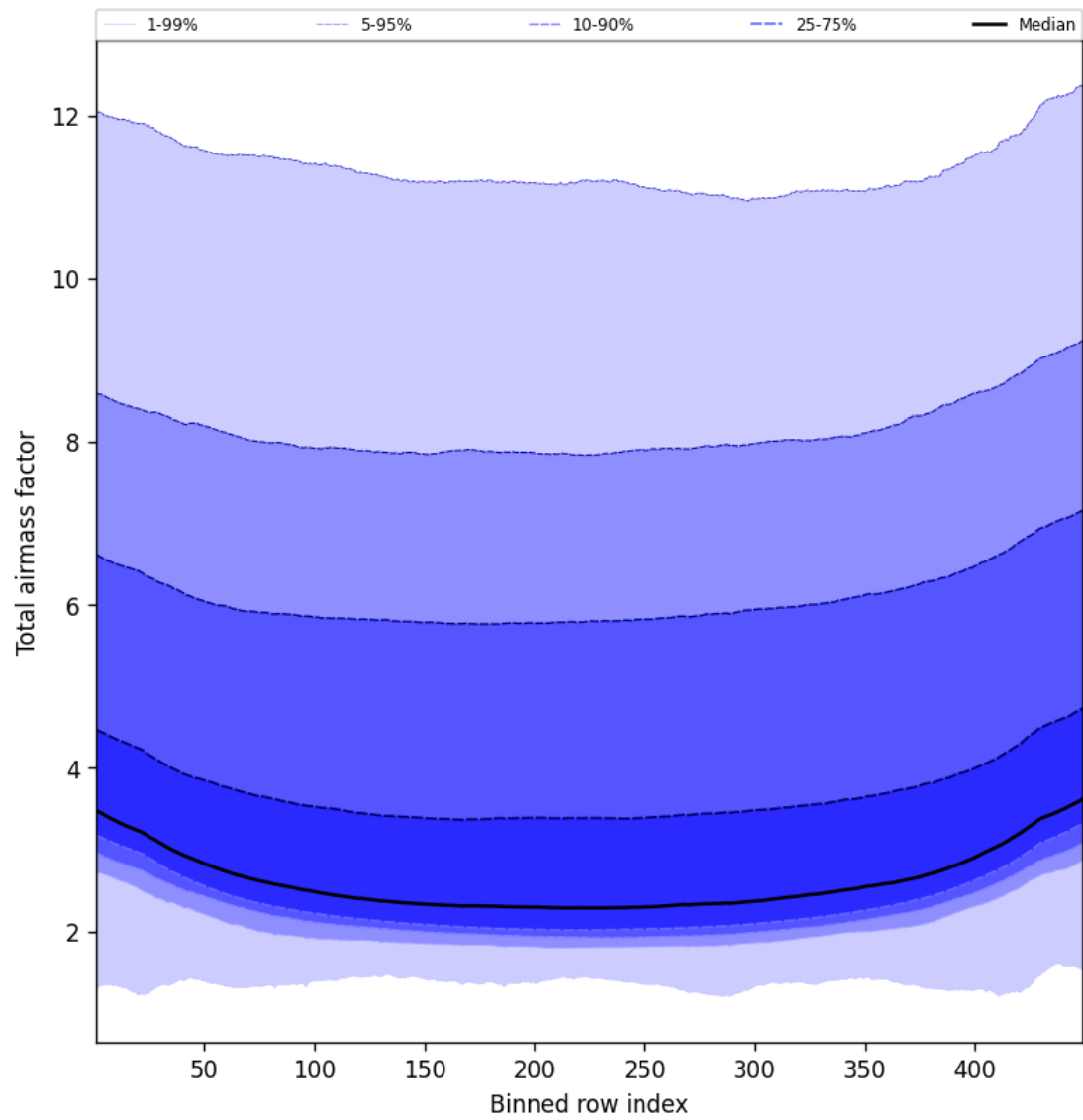
Figure 49: Along track statistics of “Total airmass factor” for 2025-03-05 to 2025-03-05
