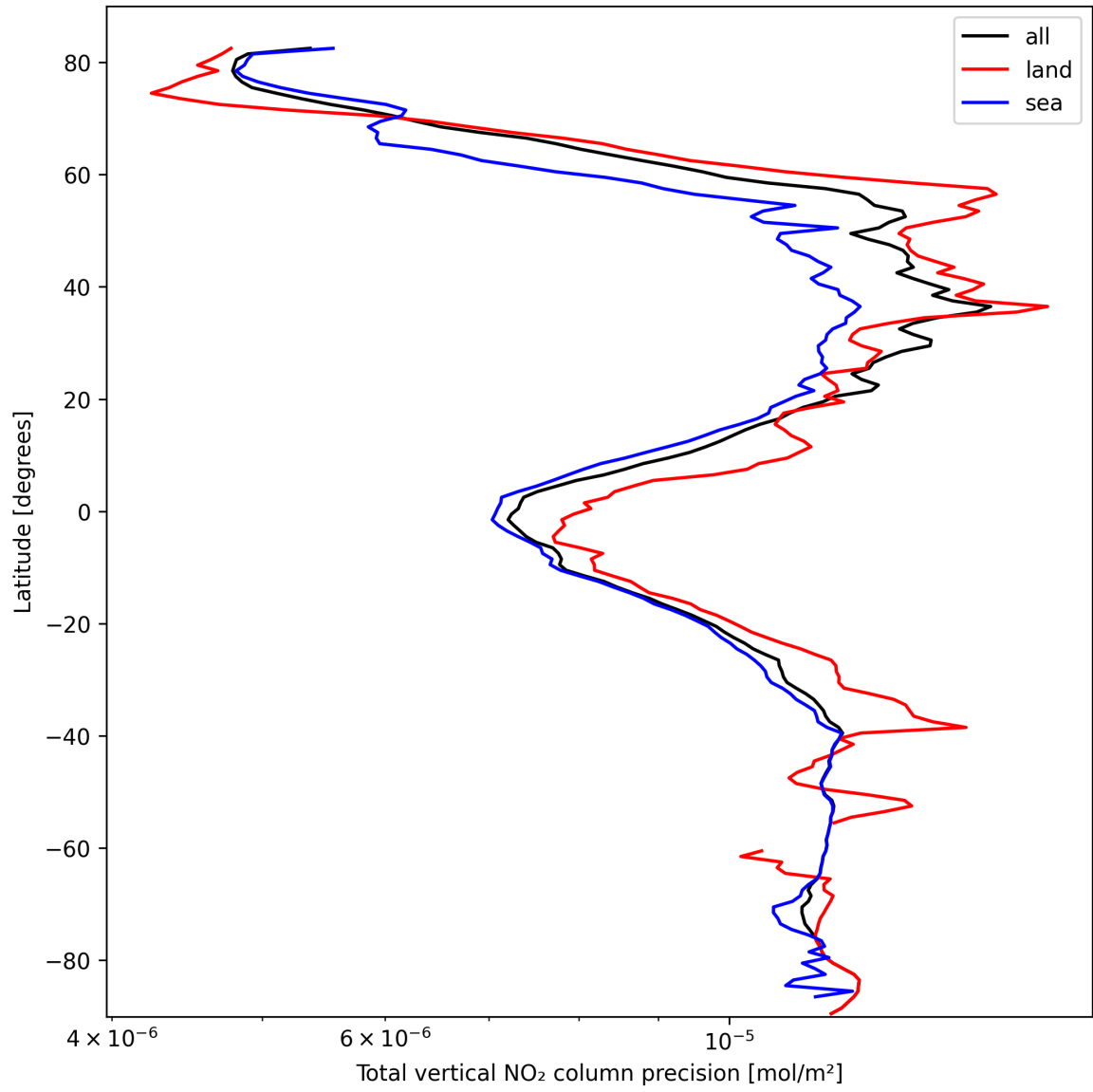
Figure 22: Zonal average of “Total vertical NO 2 column precision” for 2025-03-05 to 2025-03-05.
