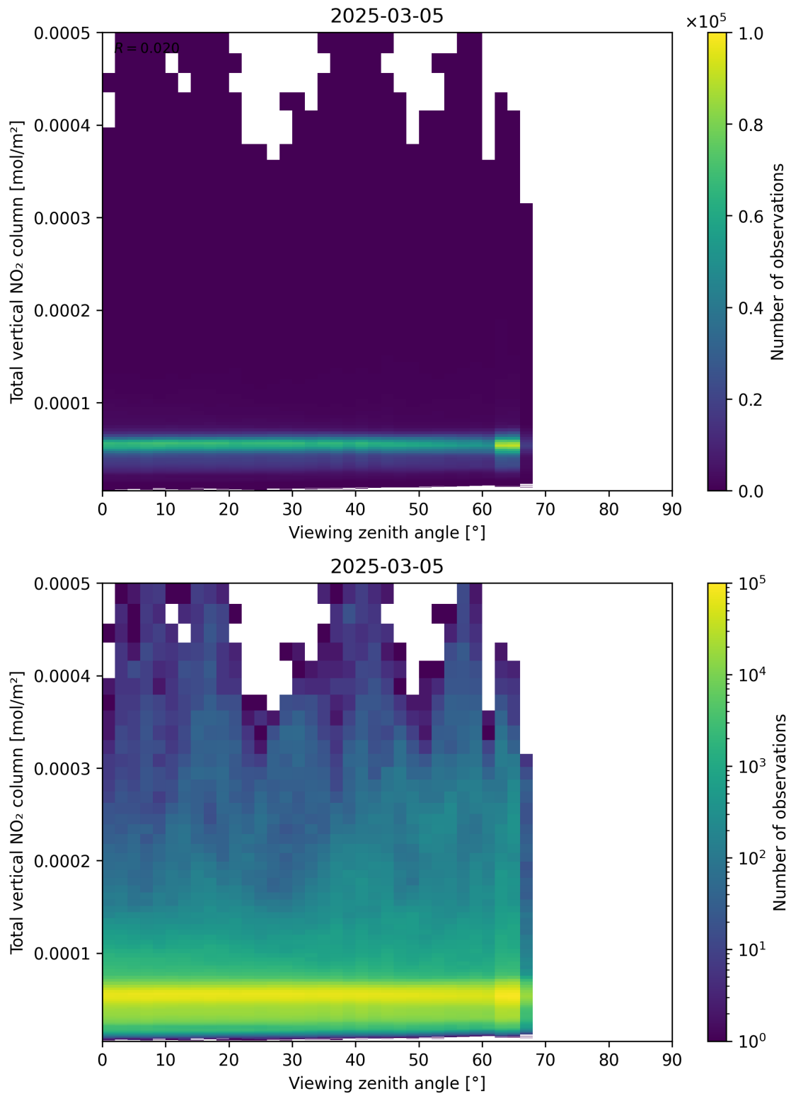
Figure 167: Scatter density plot of “Viewing zenith angle” against “Total vertical NO 2 column” for 2025-03-05 to 2025-03-05.
