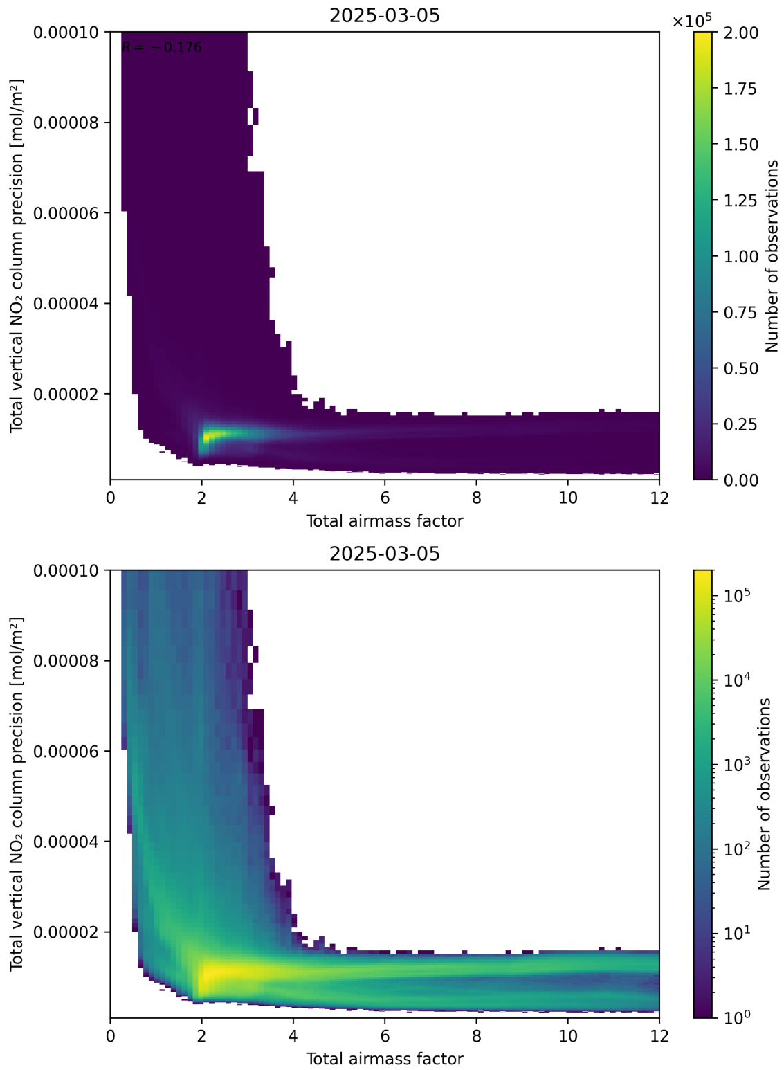
Figure 68: Scatter density plot of “Total airmass factor” against “Total vertical NO 2 column precision” for 2025-03-05 to 2025-03-05.
