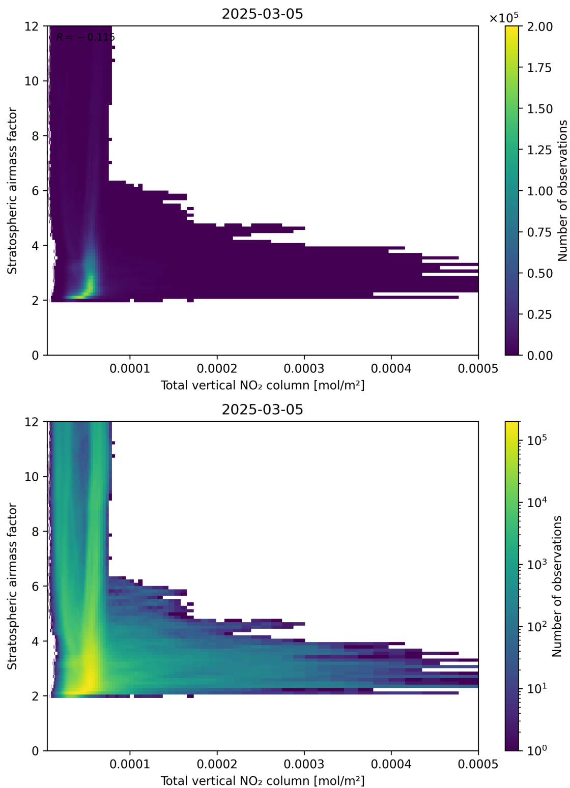
Figure 110: Scatter density plot of “Total vertical NO 2 column” against “Stratospheric airmass factor” for 2025-03-05 to 2025-03-05.
