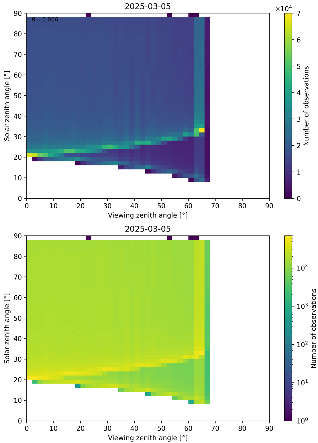
Figure 172: Scatter density plot of “Viewing zenith angle” against “Solar zenith angle” for 2025-03-05 to 2025-03-05.
