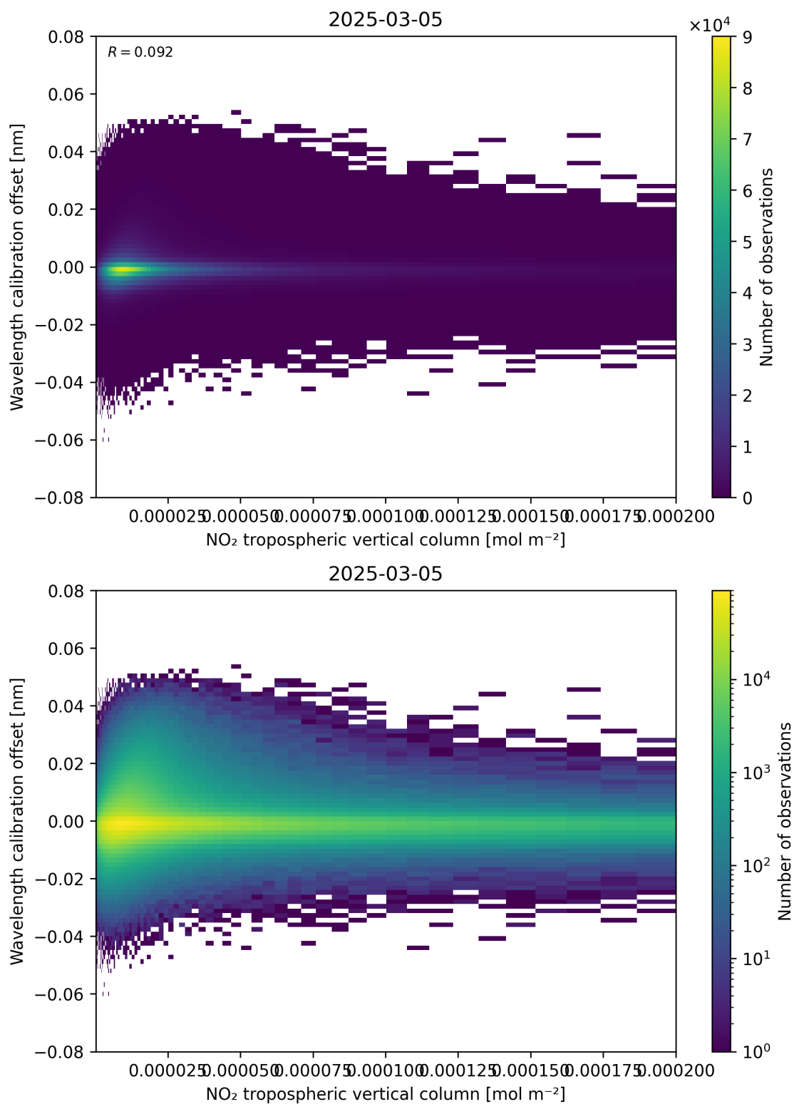
Figure 143: Scatter density plot of “NO 2 tropospheric vertical column” against “Wavelength calibration offset” for 2025-03-05 to 2025-03-05.
