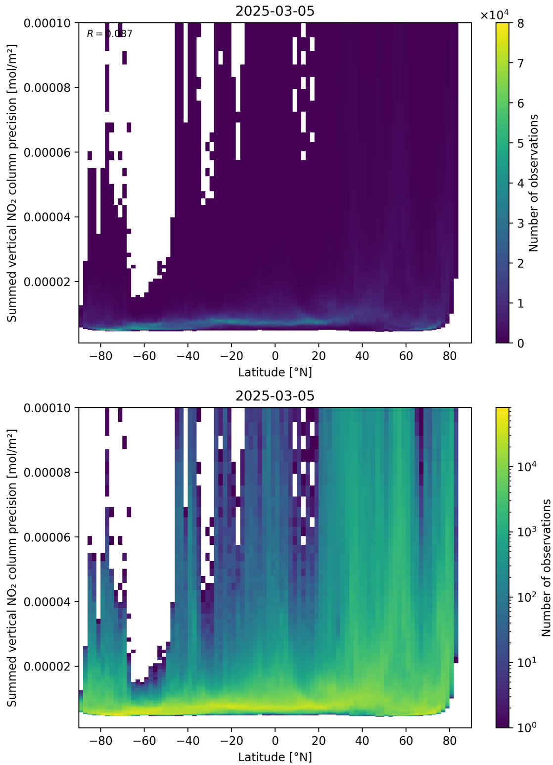
Figure 89: Scatter density plot of “Latitude” against “Summed vertical NO 2 column precision” for 2025-03-05 to 2025-03-05.
