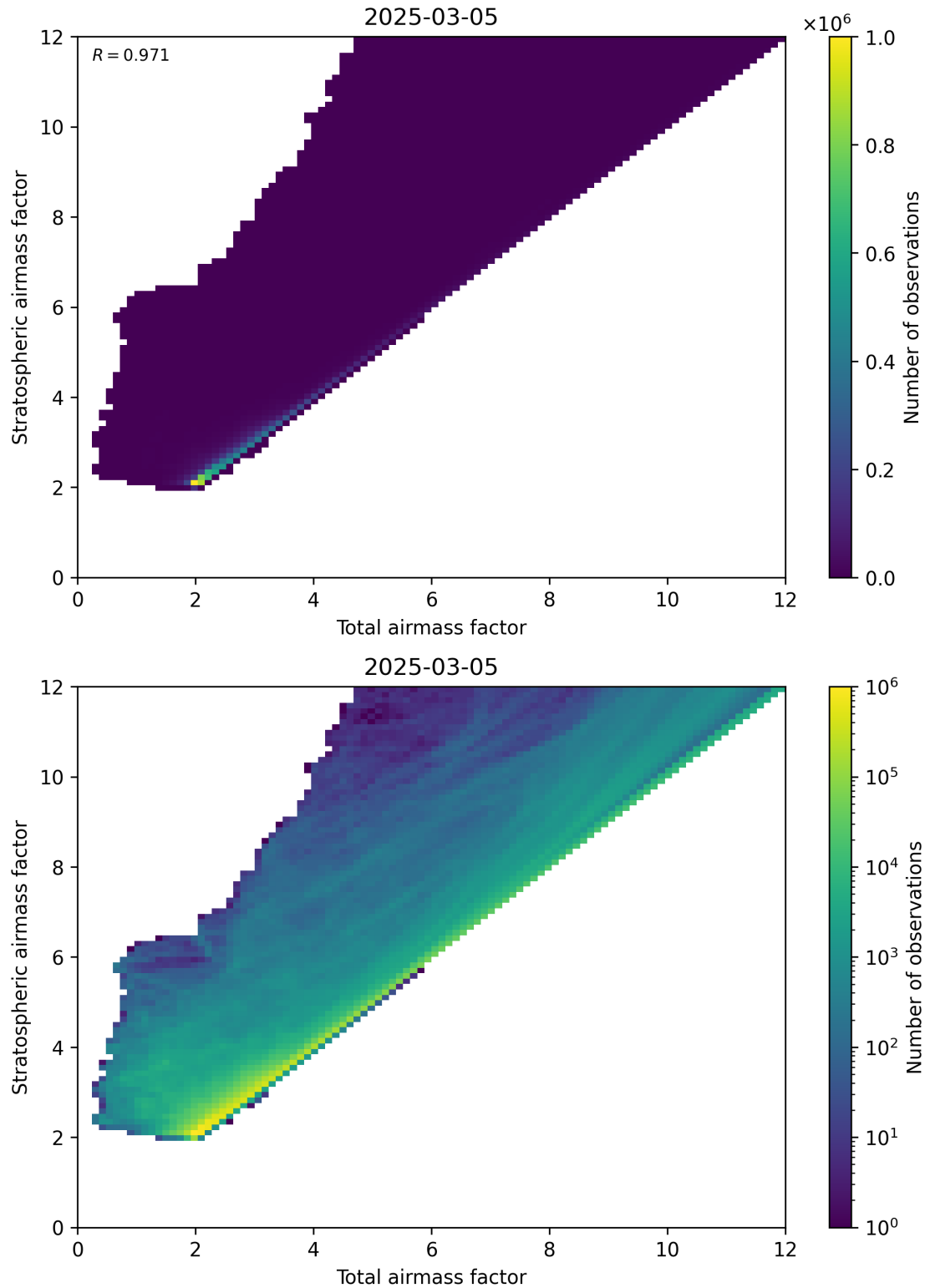
Figure 62: Scatter density plot of “Total airmass factor” against “Stratospheric airmass factor” for 2025-03-05 to 2025-03-05.
