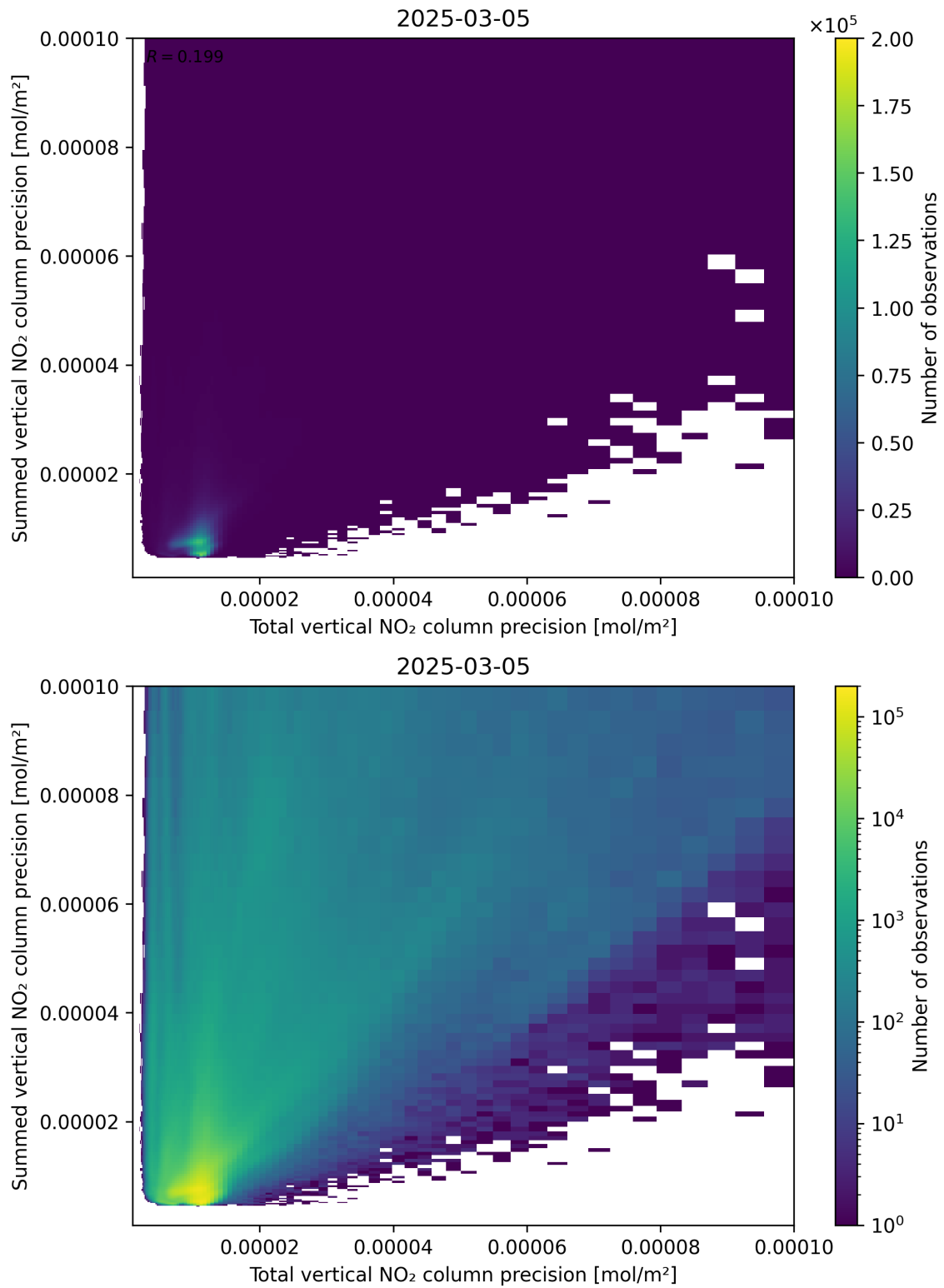
Figure 118: Scatter density plot of “Total vertical NO 2 column precision” against “Summed vertical NO 2 column precision” for 2025-03-05 to 2025-03-05.
