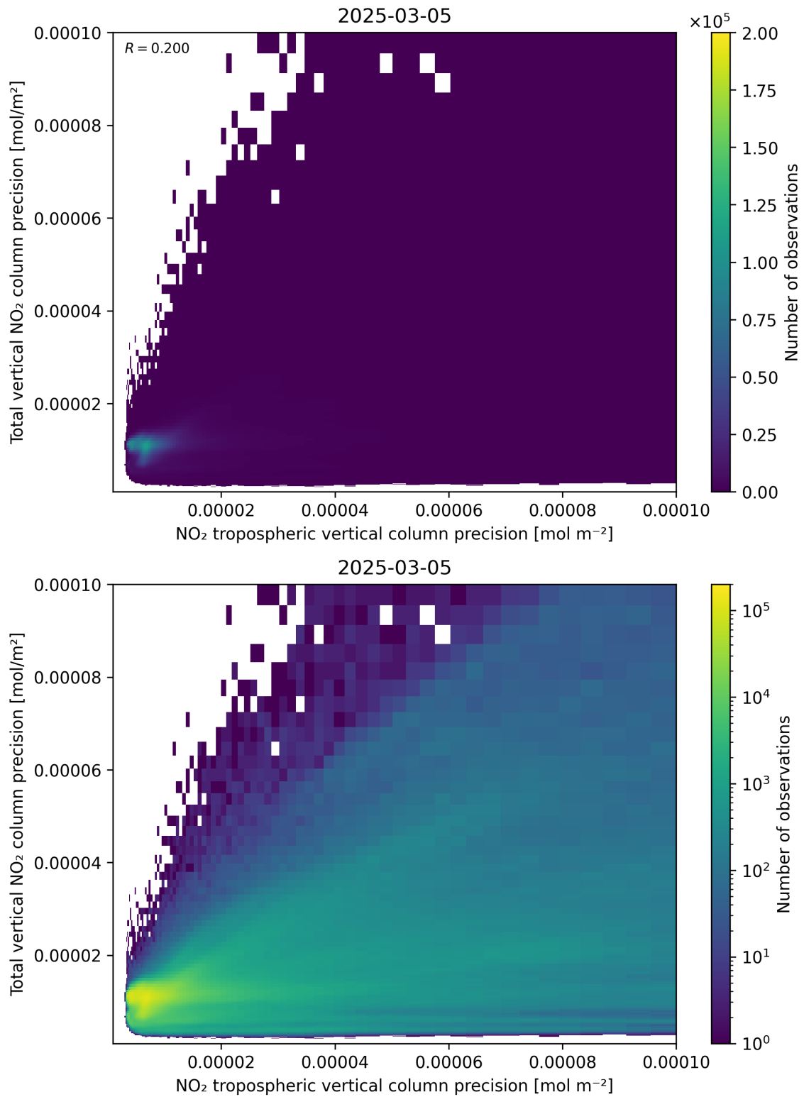
Figure 139: Scatter density plot of “NO 2 tropospheric vertical column precision” against “Total vertical NO 2 column precision” for 2025-03-05 to 2025-03-05.
