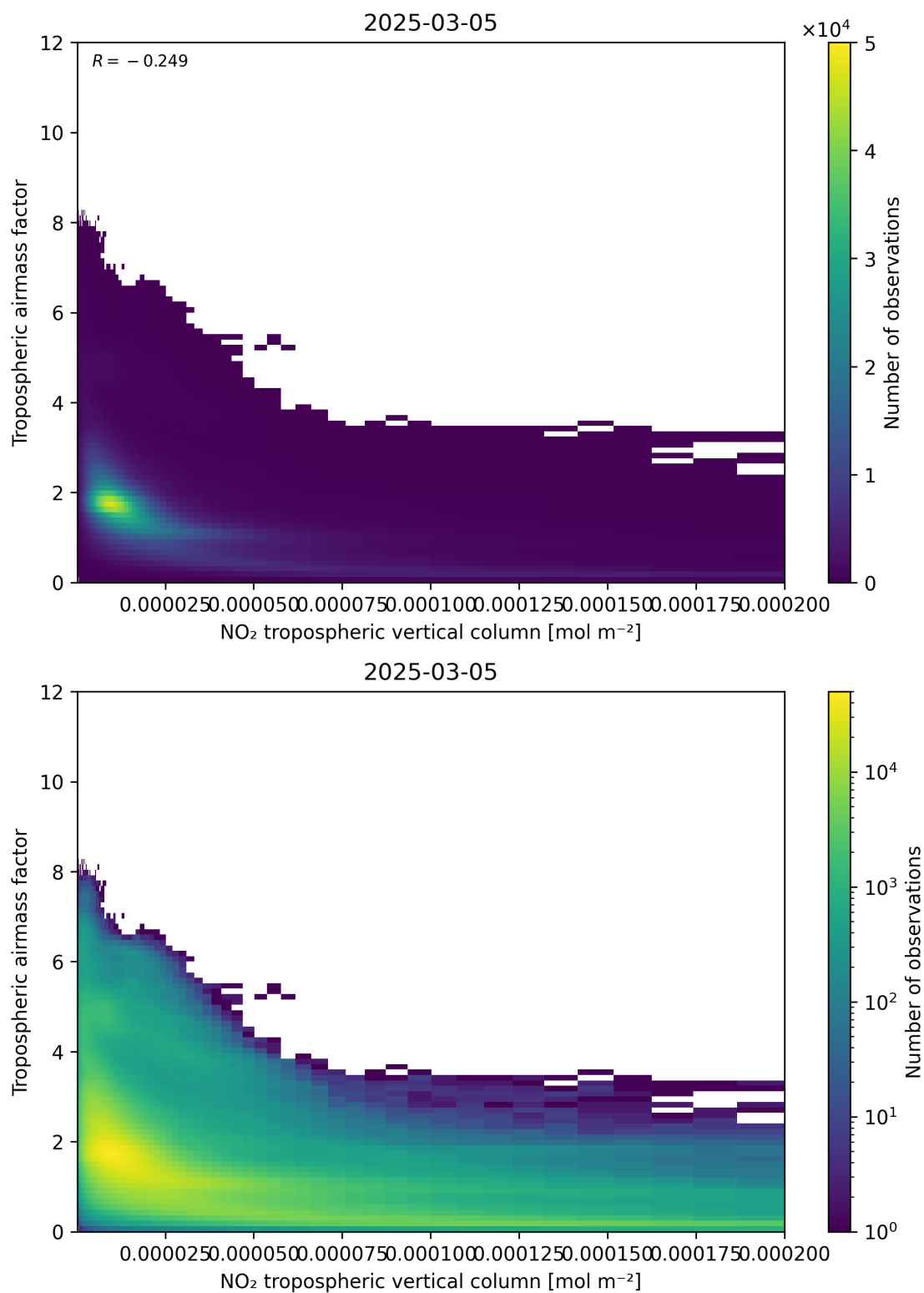
Figure 123: Scatter density plot of “NO 2 tropospheric vertical column” against “Tropospheric air mass factor” for 2025-03-05 to 2025-03-05.
