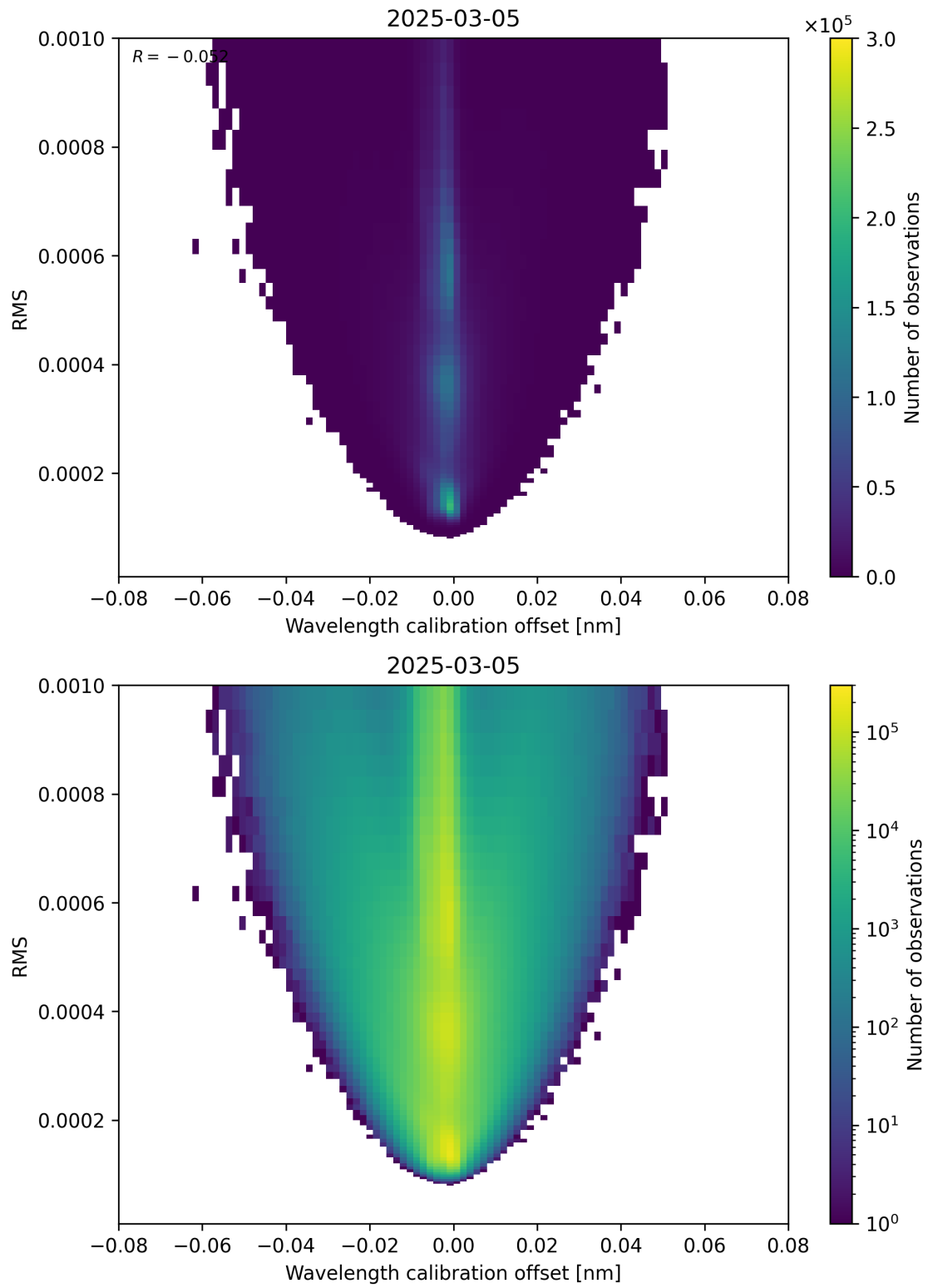
Figure 181: Scatter density plot of “Wavelength calibration offset” against “RMS” for 2025-03-05 to 2025-03-05.
