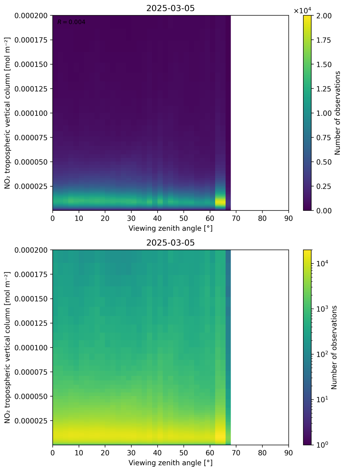
Figure 169: Scatter density plot of “Viewing zenith angle” against “NO 2 tropospheric vertical column” for 2025-03-05 to 2025-03-05.
