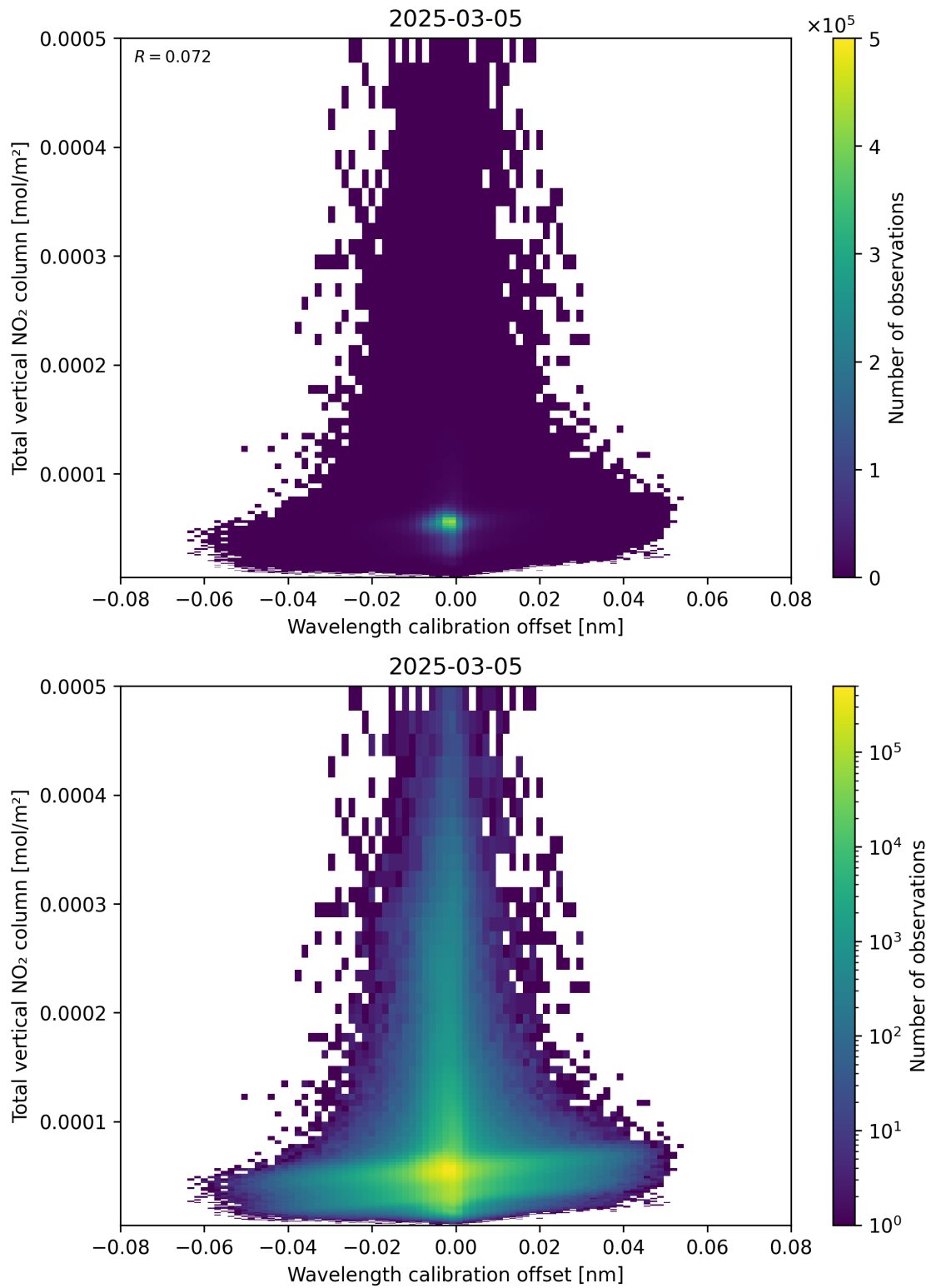
Figure 179: Scatter density plot of “Wavelength calibration offset” against “Total vertical NO 2 column” for 2025-03-05 to 2025-03-05.
