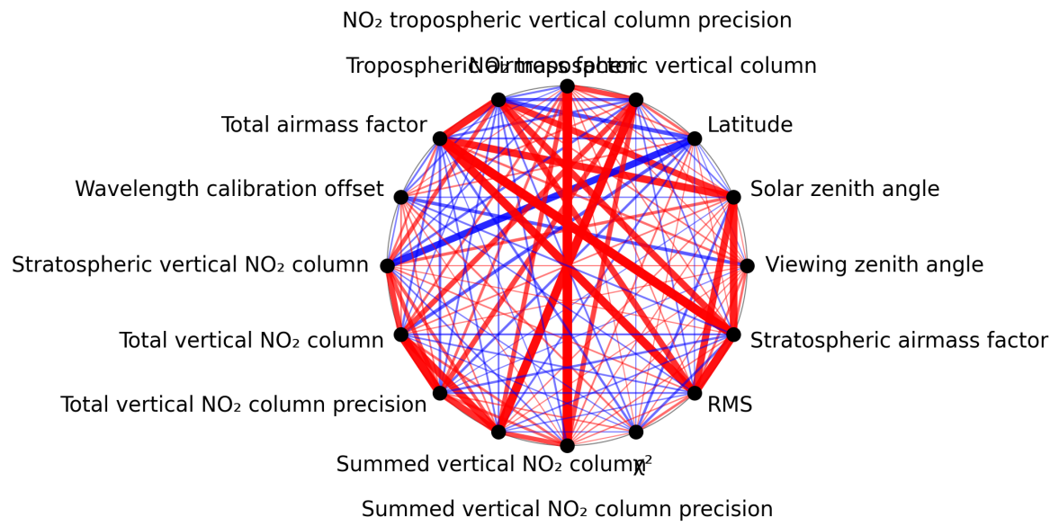
Figure 1: Map of correlation graph for 2025-03-05 to 2025-03-05.
