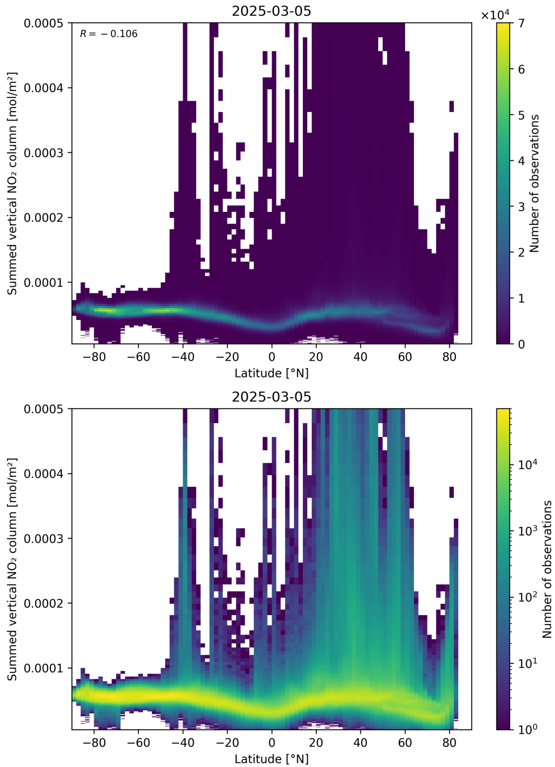
Figure 88: Scatter density plot of “Latitude” against “Summed vertical NO 2 column” for 2025-03-05 to 2025-03-05.
