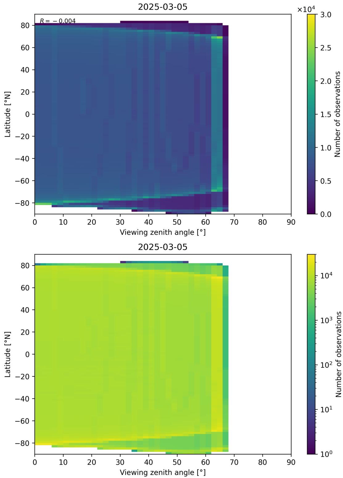
Figure 163: Scatter density plot of “Viewing zenith angle” against “Latitude” for 2025-03-05 to 2025-03-05.
