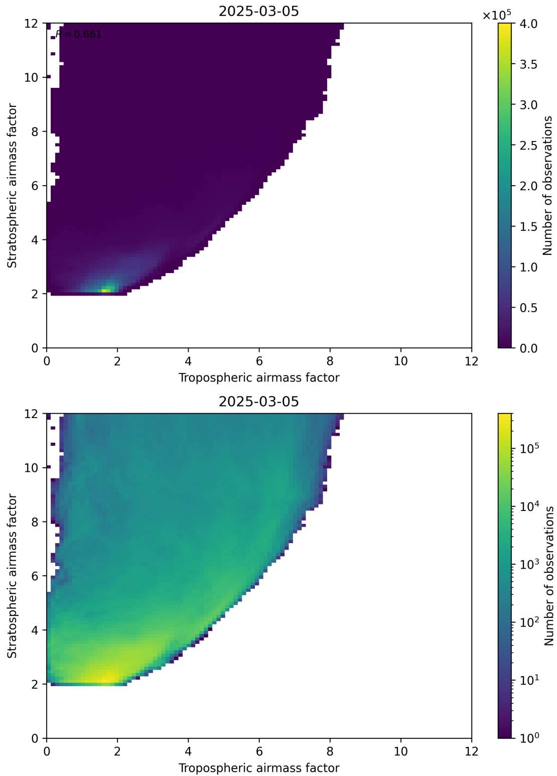
Figure 71: Scatter density plot of “Tropospheric airmass factor” against “Stratospheric airmass factor” for 2025-03-05 to 2025-03-05.
