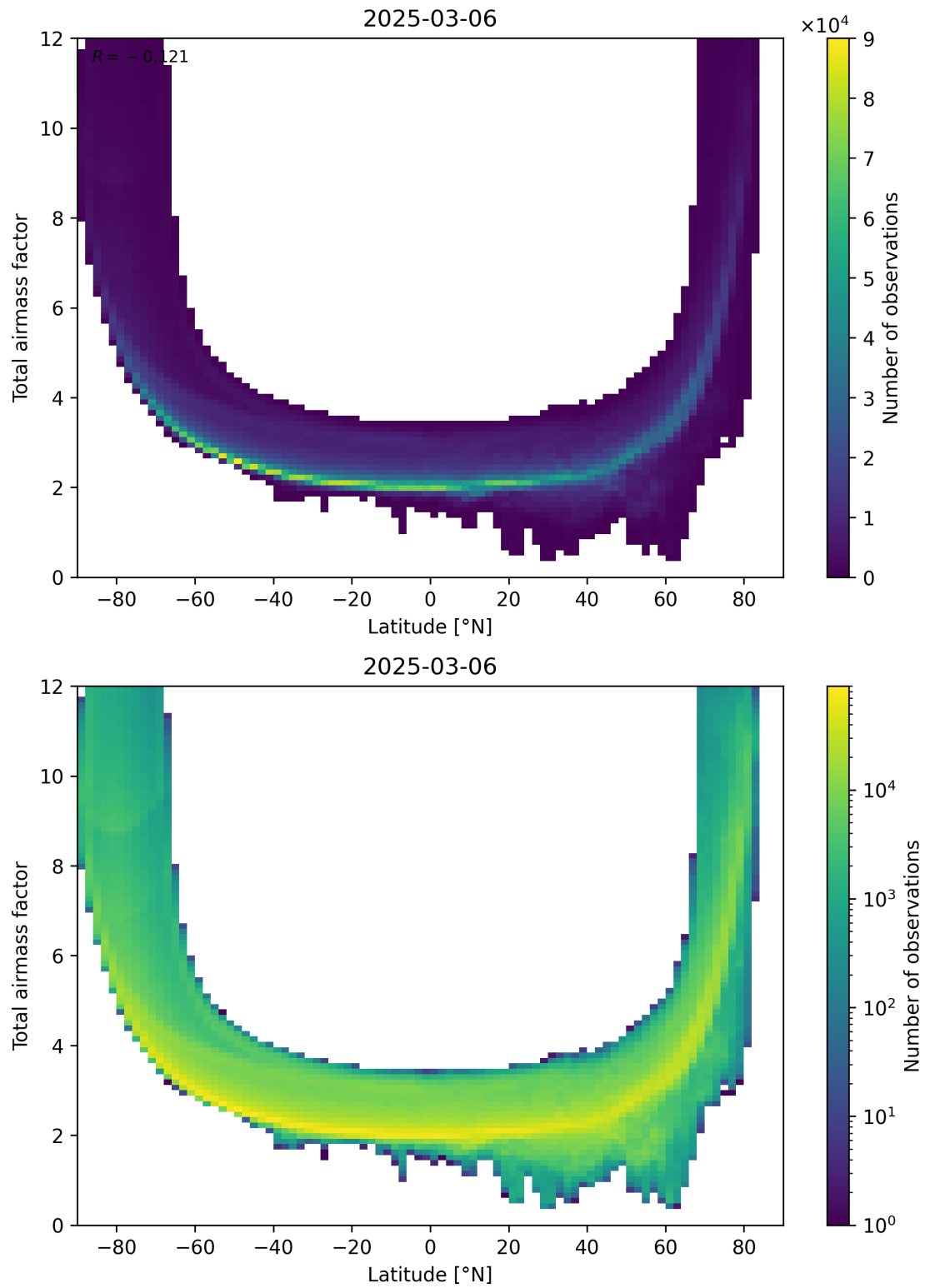
Figure 84: Scatter density plot of “Latitude” against “Total airmass factor” for 2025-03-06 to 2025-03-07.
