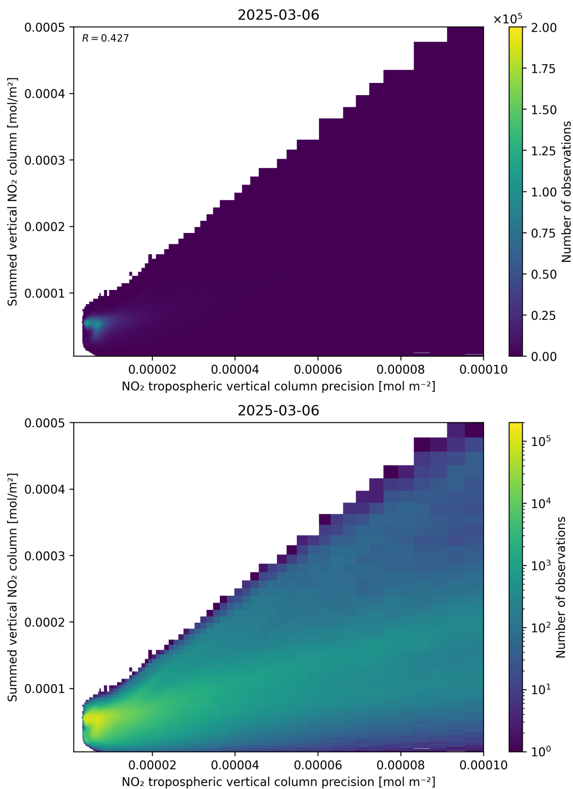
Figure 136: Scatter density plot of “NO 2 tropospheric vertical column precision” against “Summed vertical NO 2 column” for 2025-03-06 to 2025-03-07.
