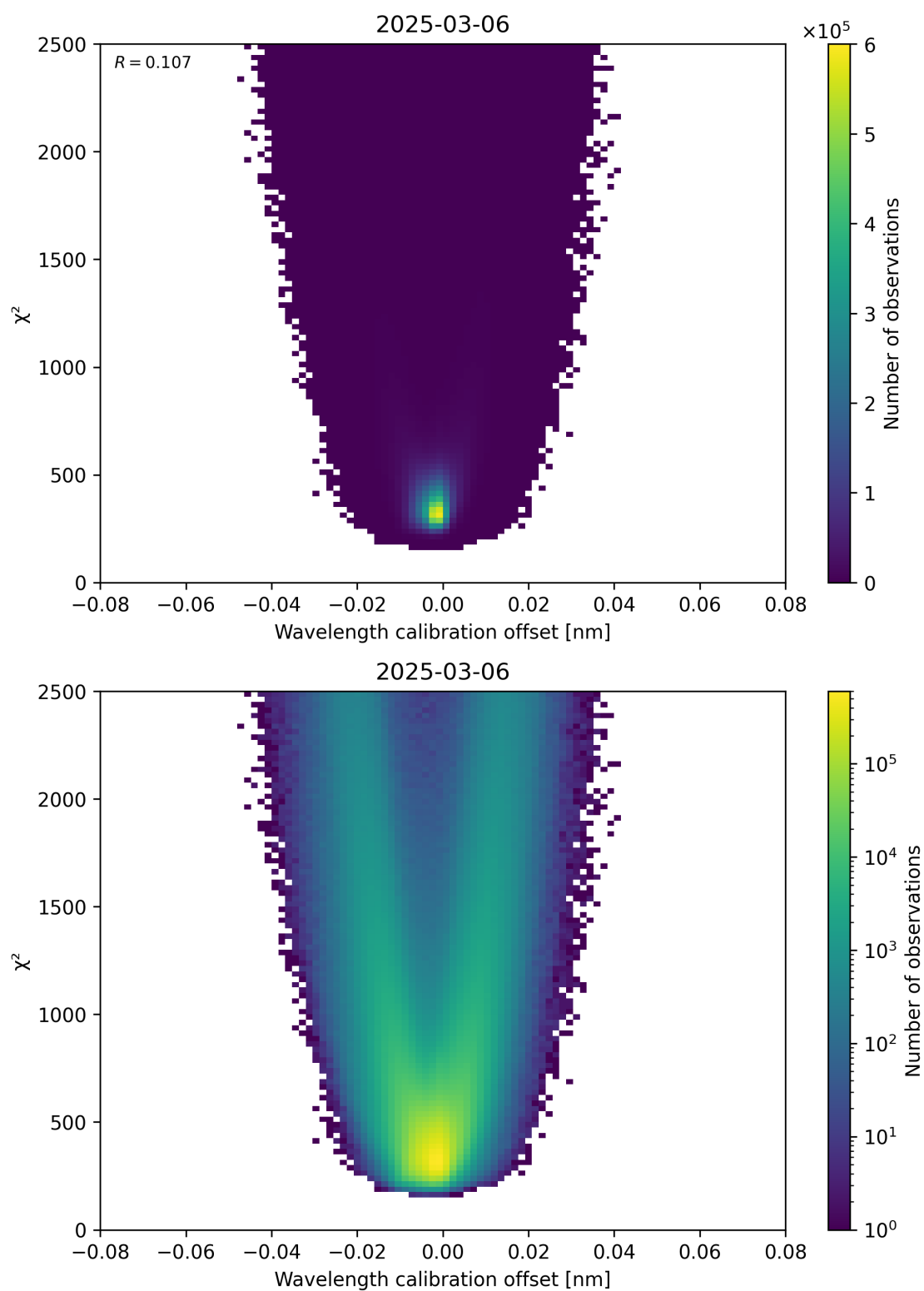
Figure 175: Scatter density plot of “Wavelength calibration offset” against “ \chi^2 ” for 2025-03-06 to 2025-03-07.
