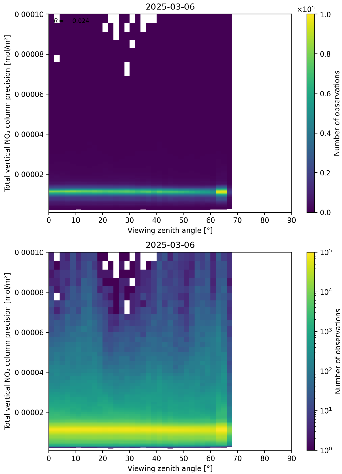
Figure 168: Scatter density plot of “Viewing zenith angle” against “Total vertical NO 2 column precision” for 2025-03-06 to 2025-03-07.
