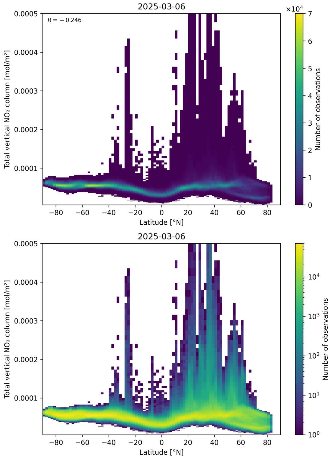
Figure 90: Scatter density plot of “Latitude” against “Total vertical NO 2 column” for 2025-03-06 to 2025-03-07.
