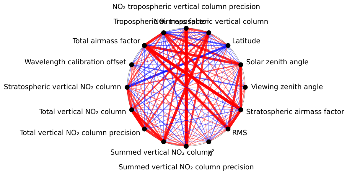
Figure 1: Map of correlation graph for 2025-03-06 to 2025-03-07.
