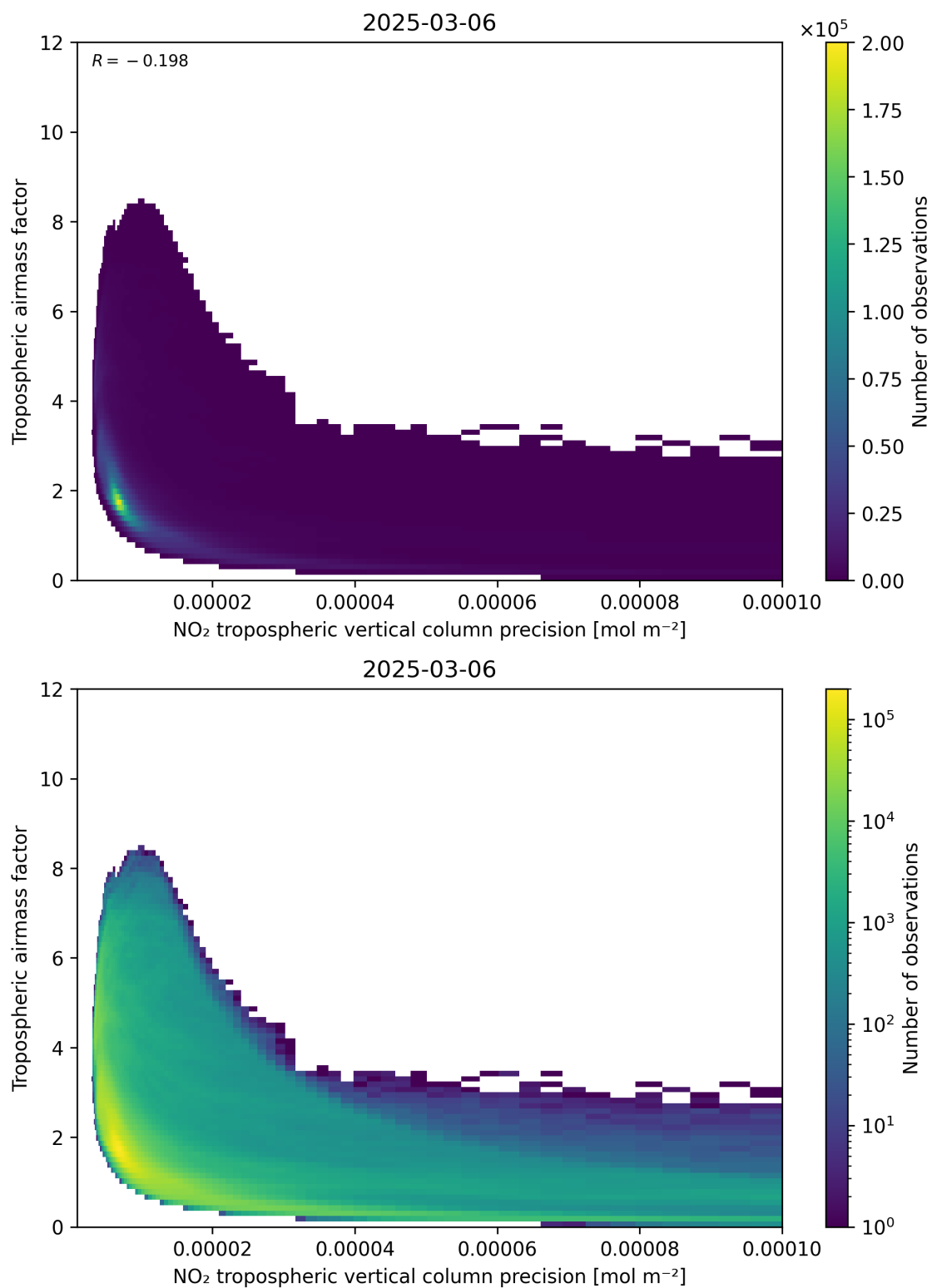
Figure 133: Scatter density plot of “NO 2 tropospheric vertical column precision” against “Tropospheric air mass factor” for 2025-03-06 to 2025-03-07.
