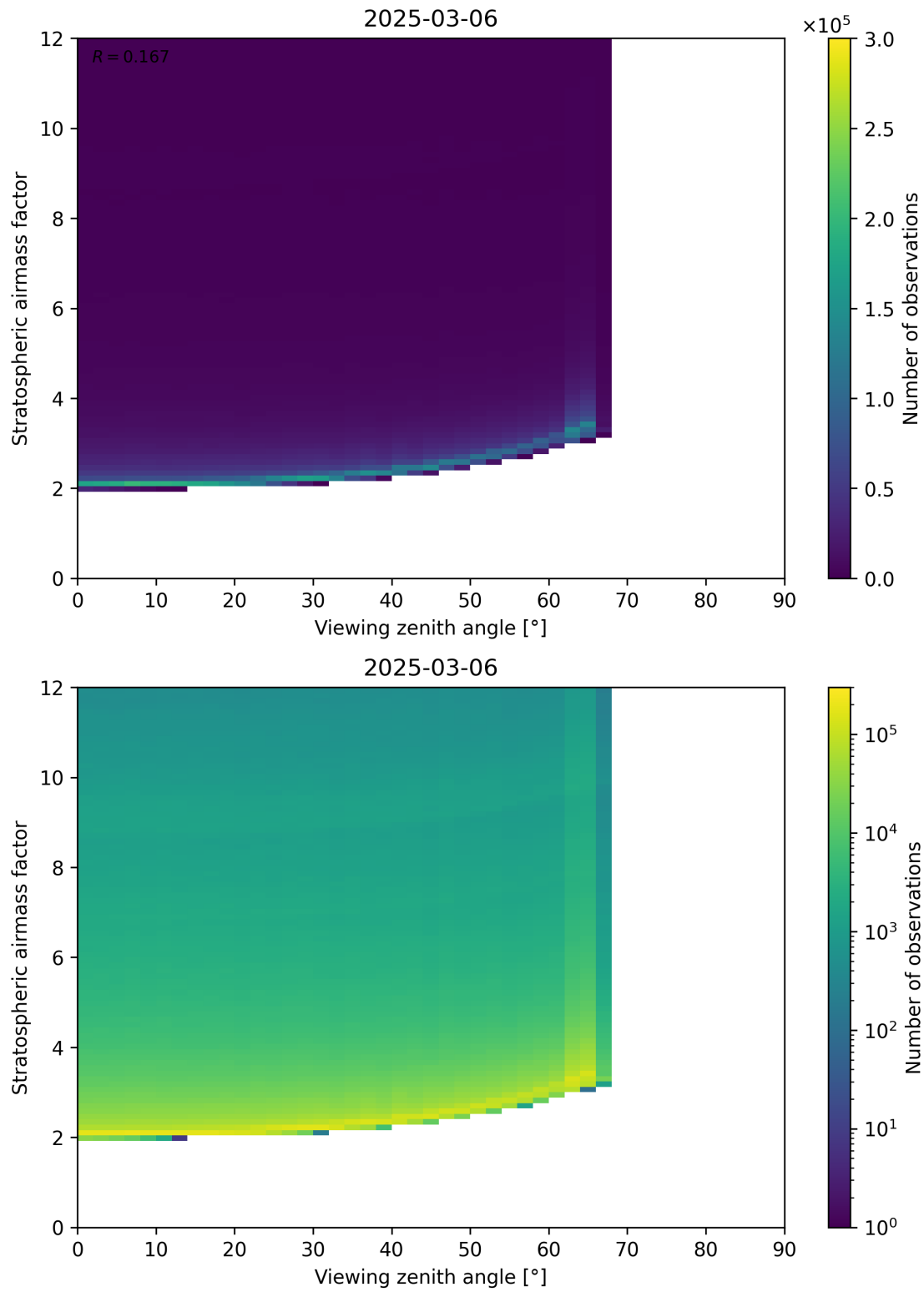
Figure 159: Scatter density plot of “Viewing zenith angle” against “Stratospheric airmass factor” for 2025-03-06 to 2025-03-07.
