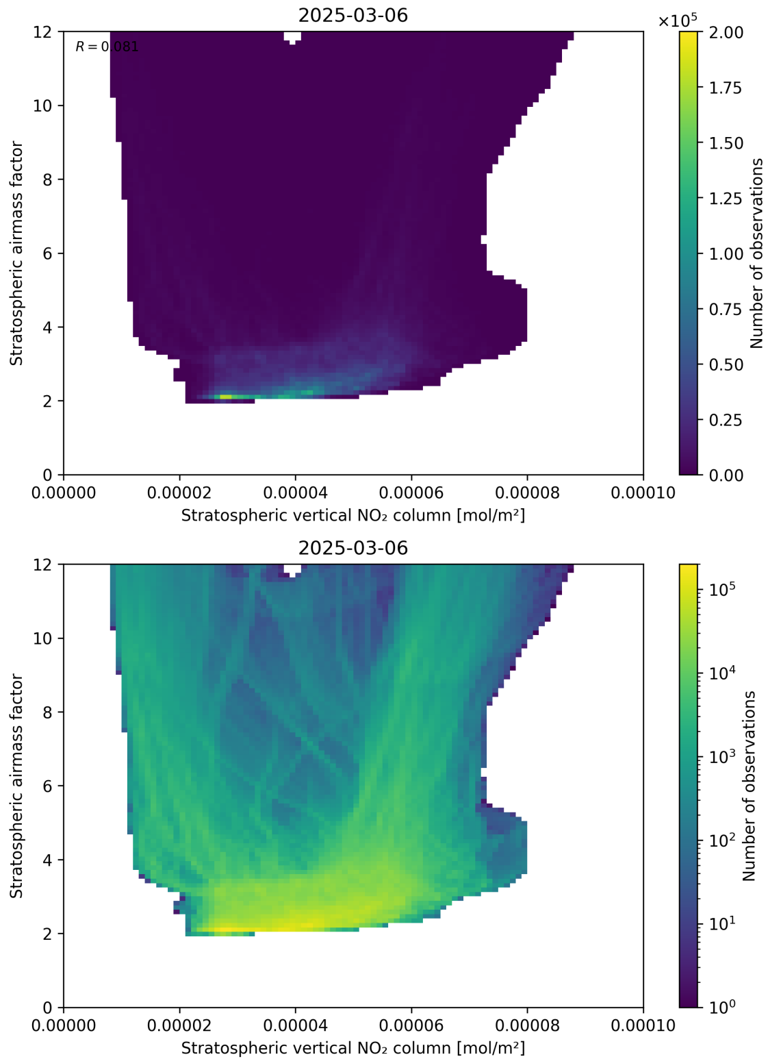
Figure 96: Scatter density plot of “Stratospheric vertical NO 2 column” against “Stratospheric airmass factor” for 2025-03-06 to 2025-03-07.
