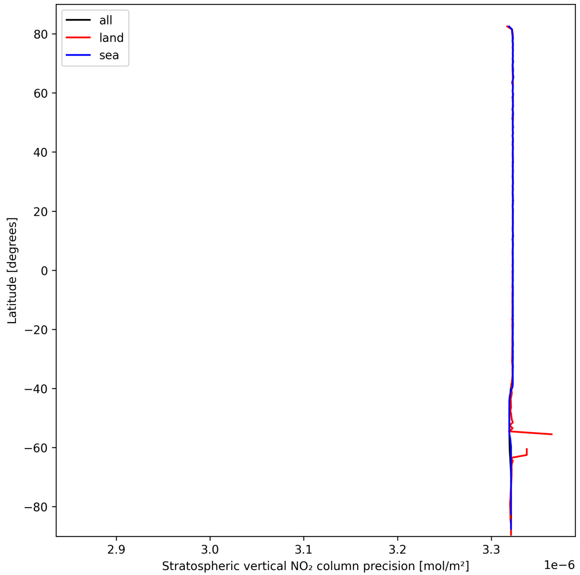
Figure 20: Zonal average of “Stratospheric vertical NO 2 column precision” for 2025-03-06 to 2025-03-07.
