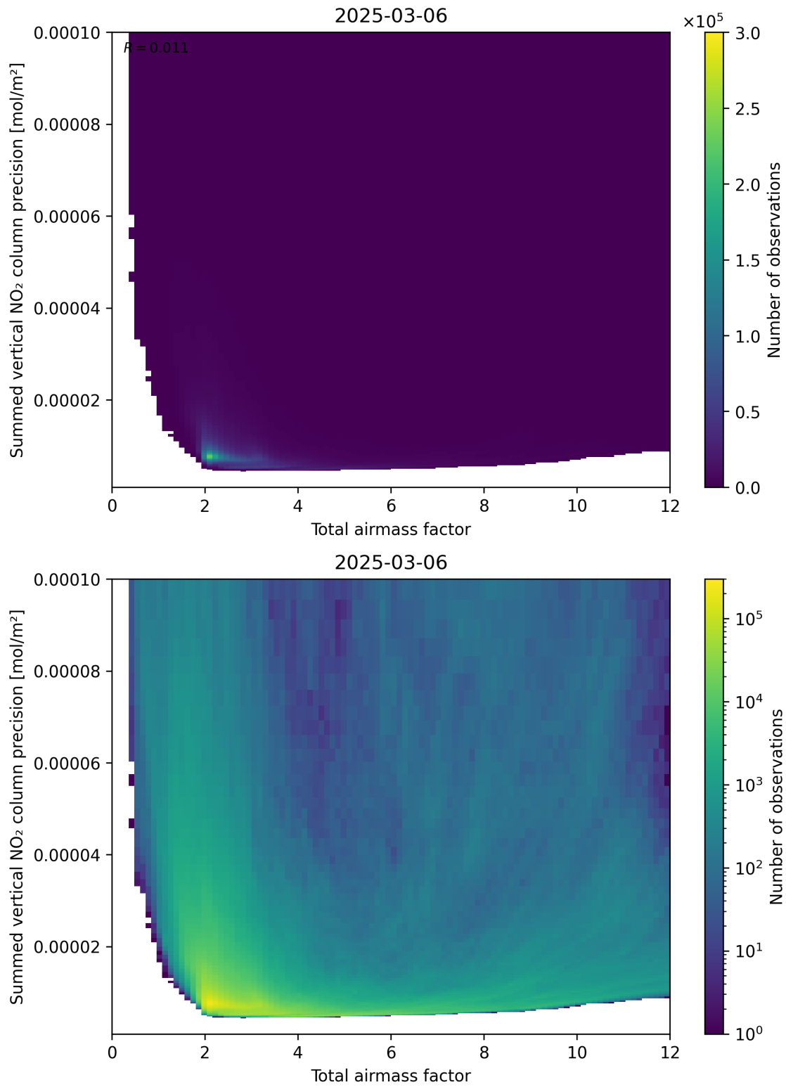
Figure 66: Scatter density plot of “Total airmass factor” against “Summed vertical NO 2 column precision” for 2025-03-06 to 2025-03-07.
