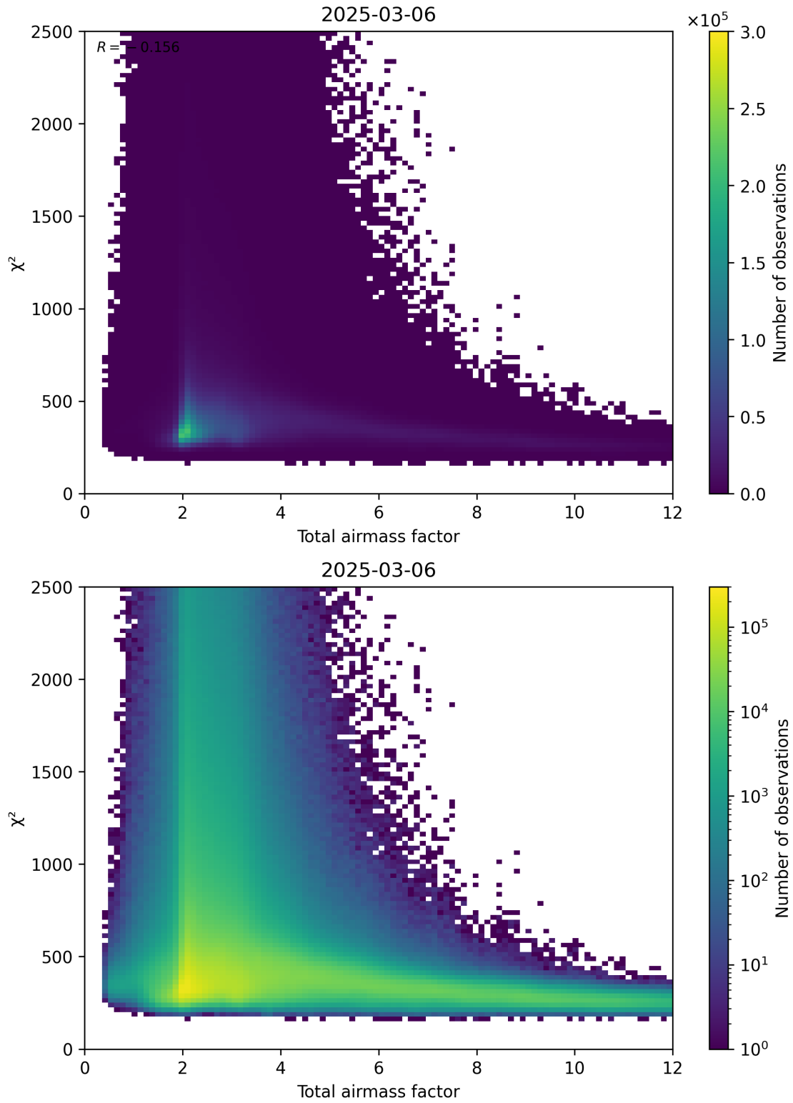
Figure 63: Scatter density plot of “Total airmass factor” against “ \chi^2 ” for 2025-03-06 to 2025-03-07.
