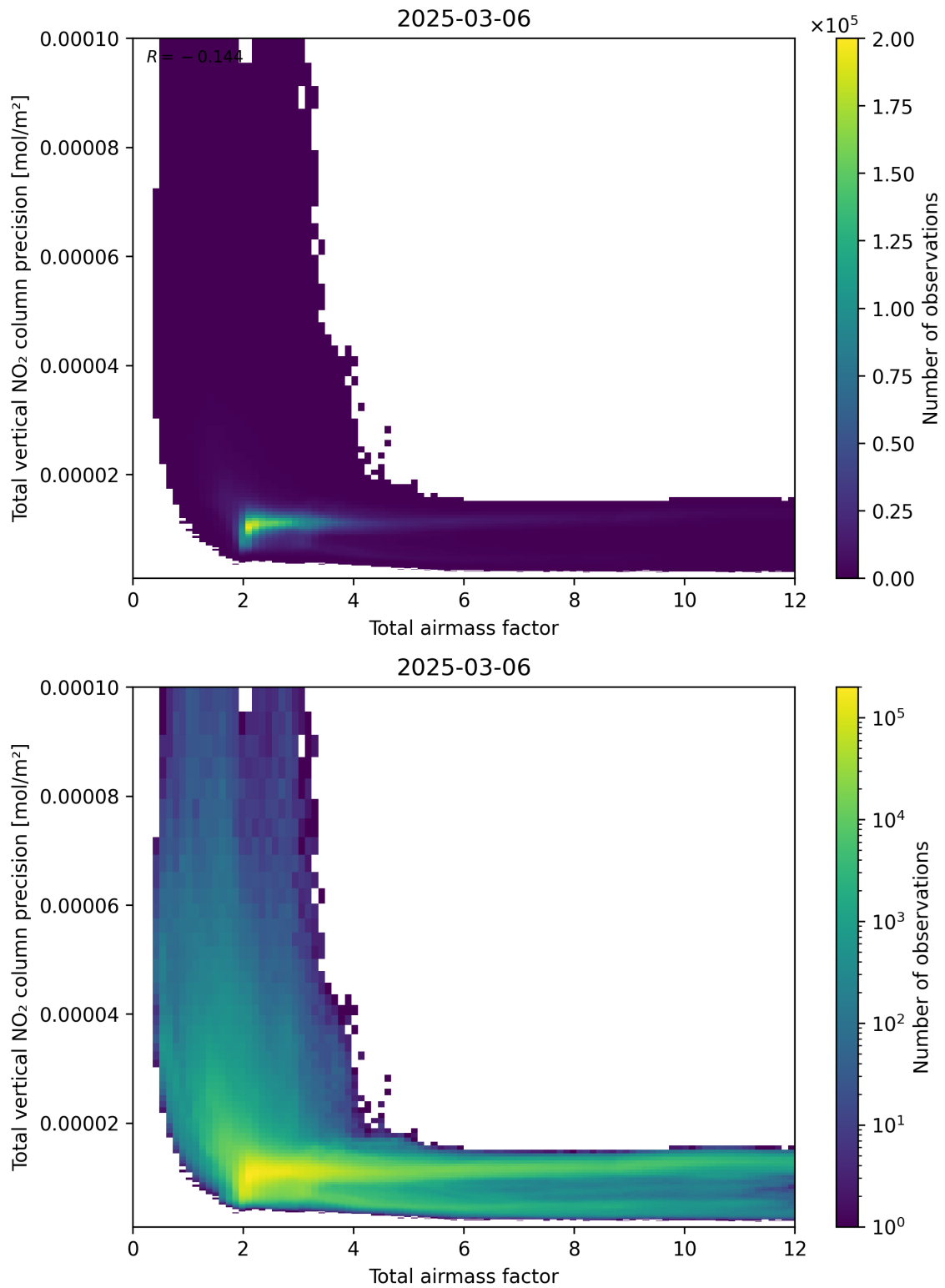
Figure 68: Scatter density plot of “Total airmass factor” against “Total vertical NO 2 column precision” for 2025-03-06 to 2025-03-07.
