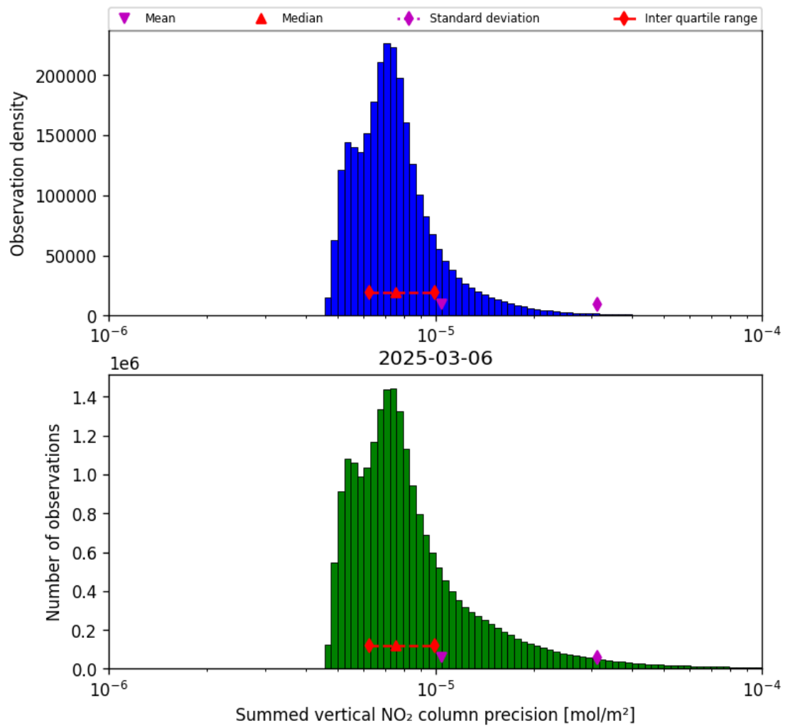
Figure 41: Histogram of "Summed vertical NO 2 column precision" for 2025-03-06 to 2025-03-07
