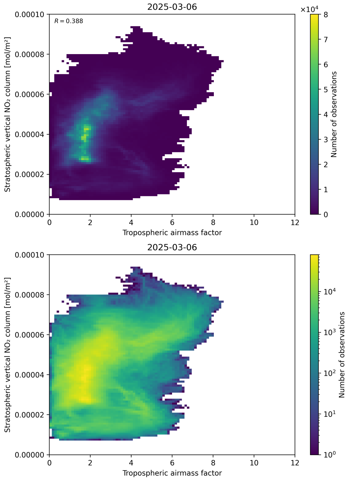
Figure 74: Scatter density plot of “Tropospheric airmass factor” against “Stratospheric vertical NO 2 column” for 2025-03-06 to 2025-03-07.
