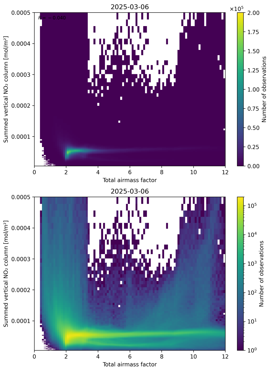
Figure 65: Scatter density plot of “Total airmass factor” against “Summed vertical NO 2 column” for 2025-03-06 to 2025-03-07.
