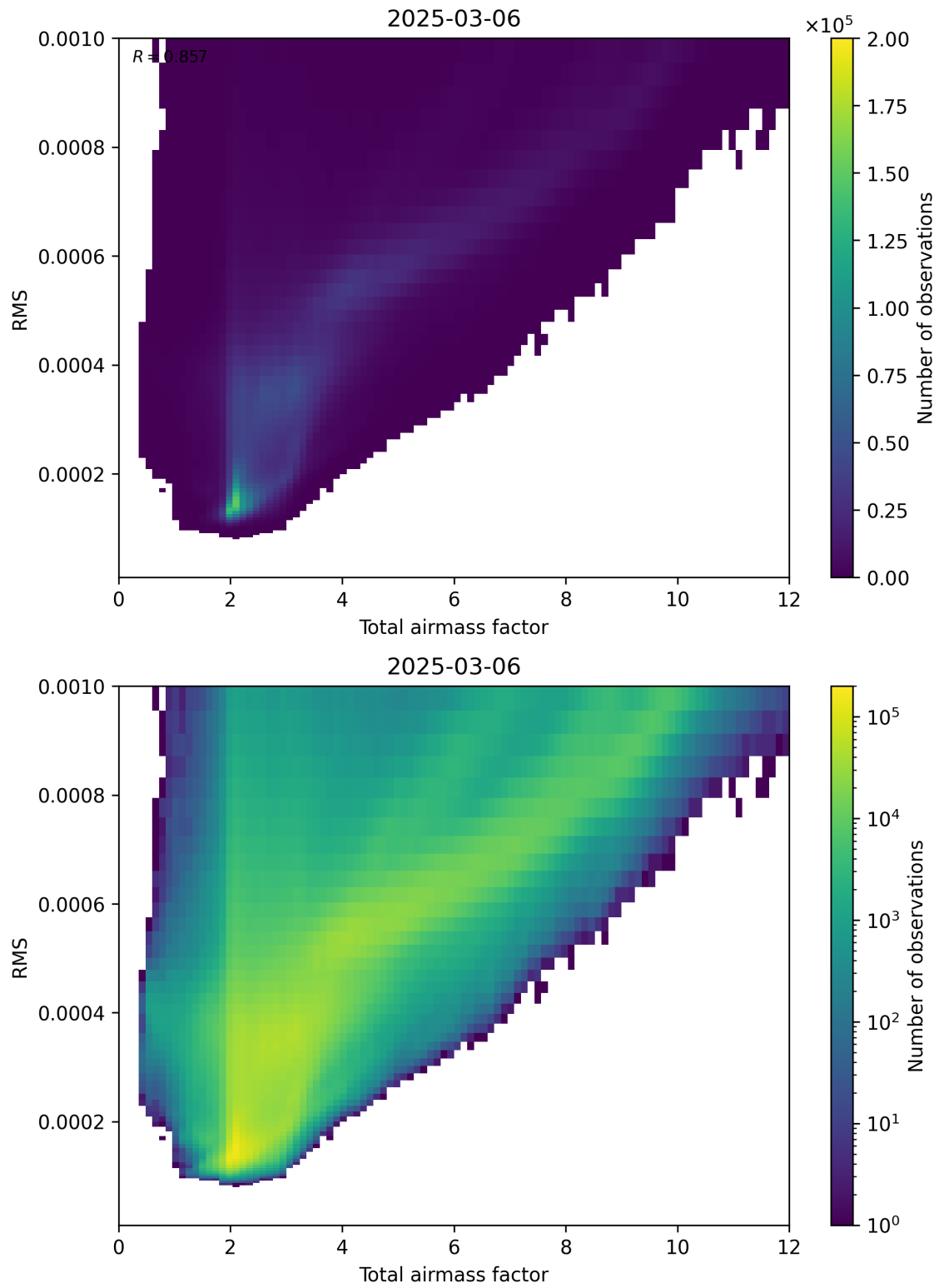
Figure 69: Scatter density plot of “Total airmass factor” against “RMS” for 2025-03-06 to 2025-03-07.
