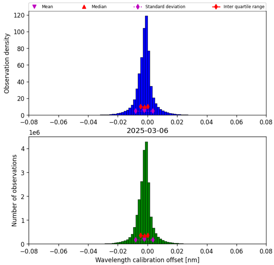
Figure 35: Histogram of “Wavelength calibration offset” for 2025-03-06 to 2025-03-07
