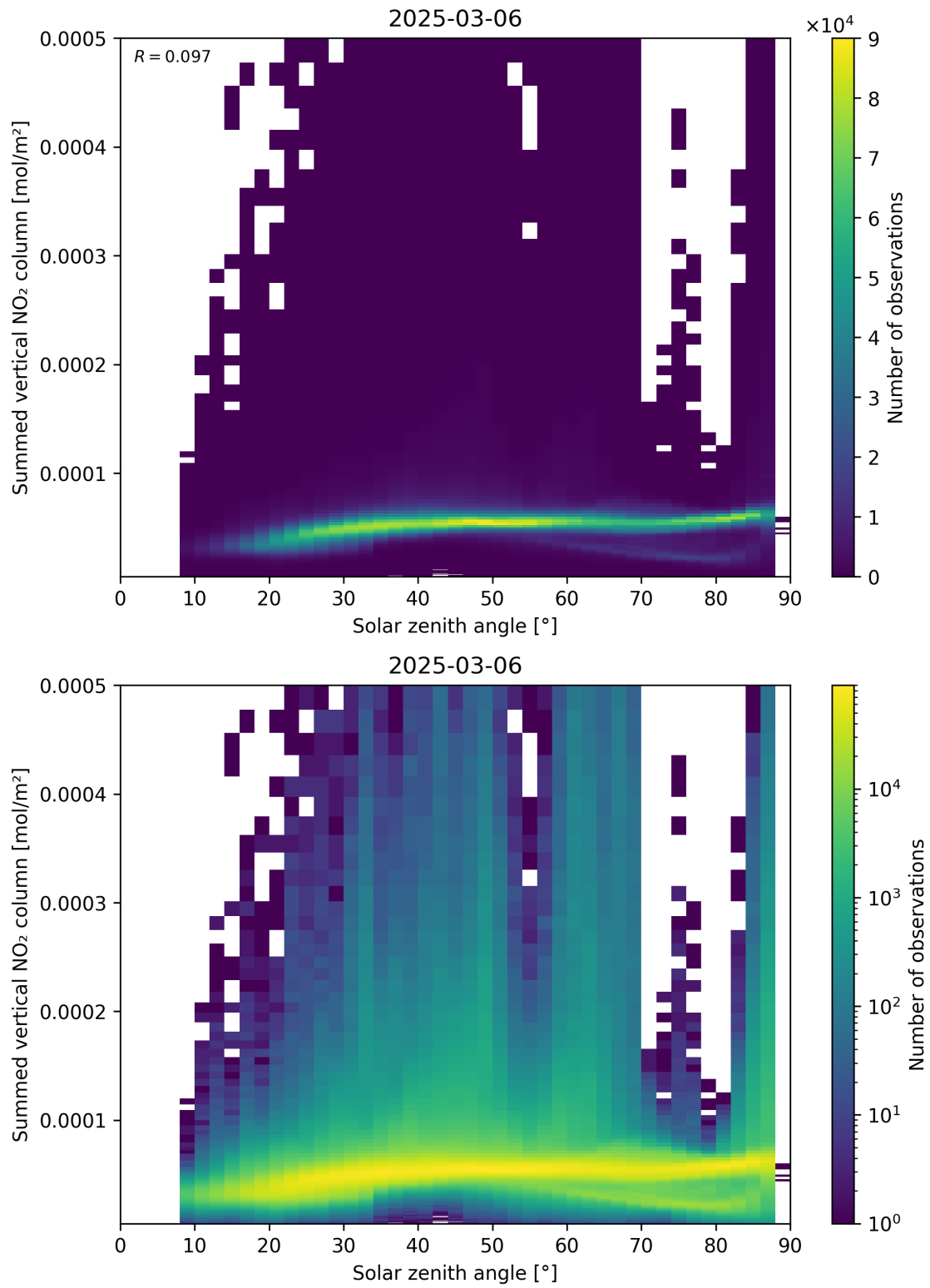
Figure 151: Scatter density plot of “Solar zenith angle” against “Summed vertical NO 2 column” for 2025-03-06 to 2025-03-07.
