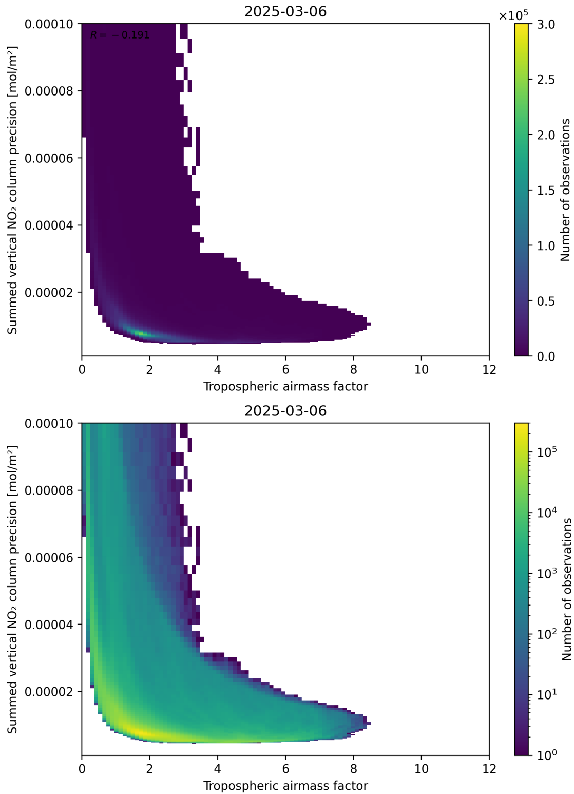
Figure 76: Scatter density plot of “Tropospheric air mass factor” against “Summed vertical NO 2 column precision” for 2025-03-06 to 2025-03-07.
