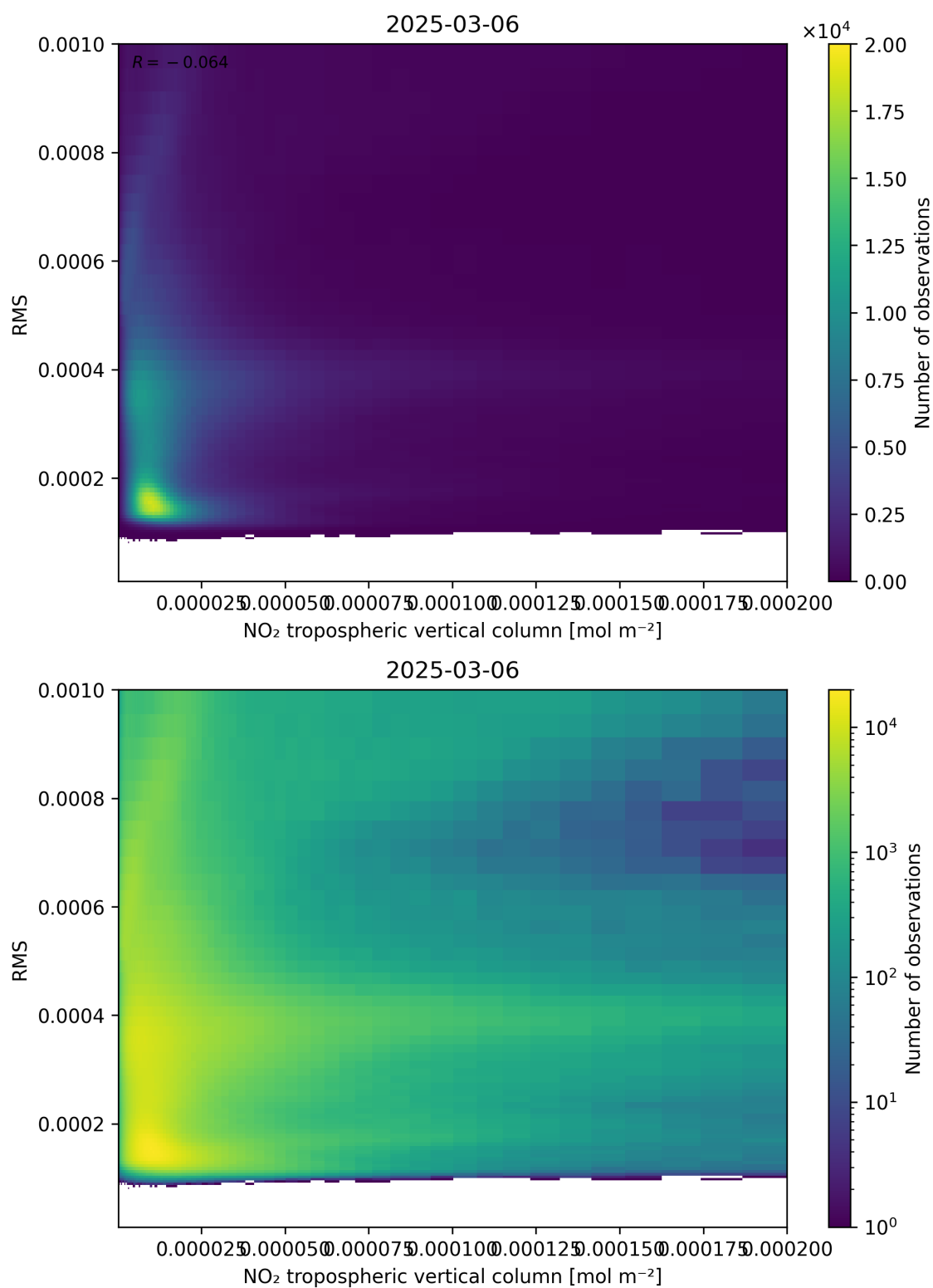
Figure 142: Scatter density plot of “NO 2 tropospheric vertical column” against “RMS” for 2025-03-06 to 2025-03-07.
