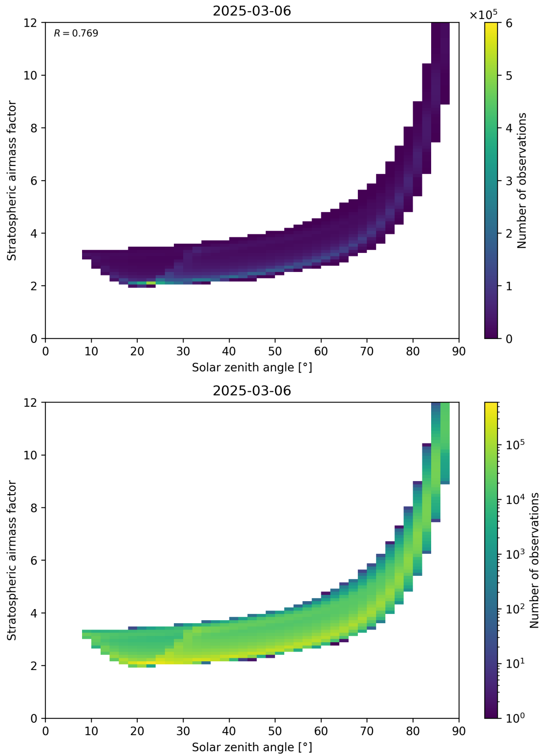
Figure 145: Scatter density plot of “Solar zenith angle” against “Stratospheric airmass factor” for 2025-03-06 to 2025-03-07.
