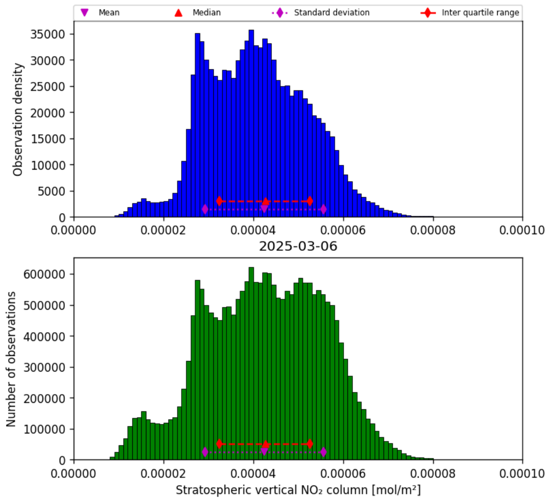
Figure 36: Histogram of “Stratospheric vertical NO 2 column” for 2025-03-06 to 2025-03-07
