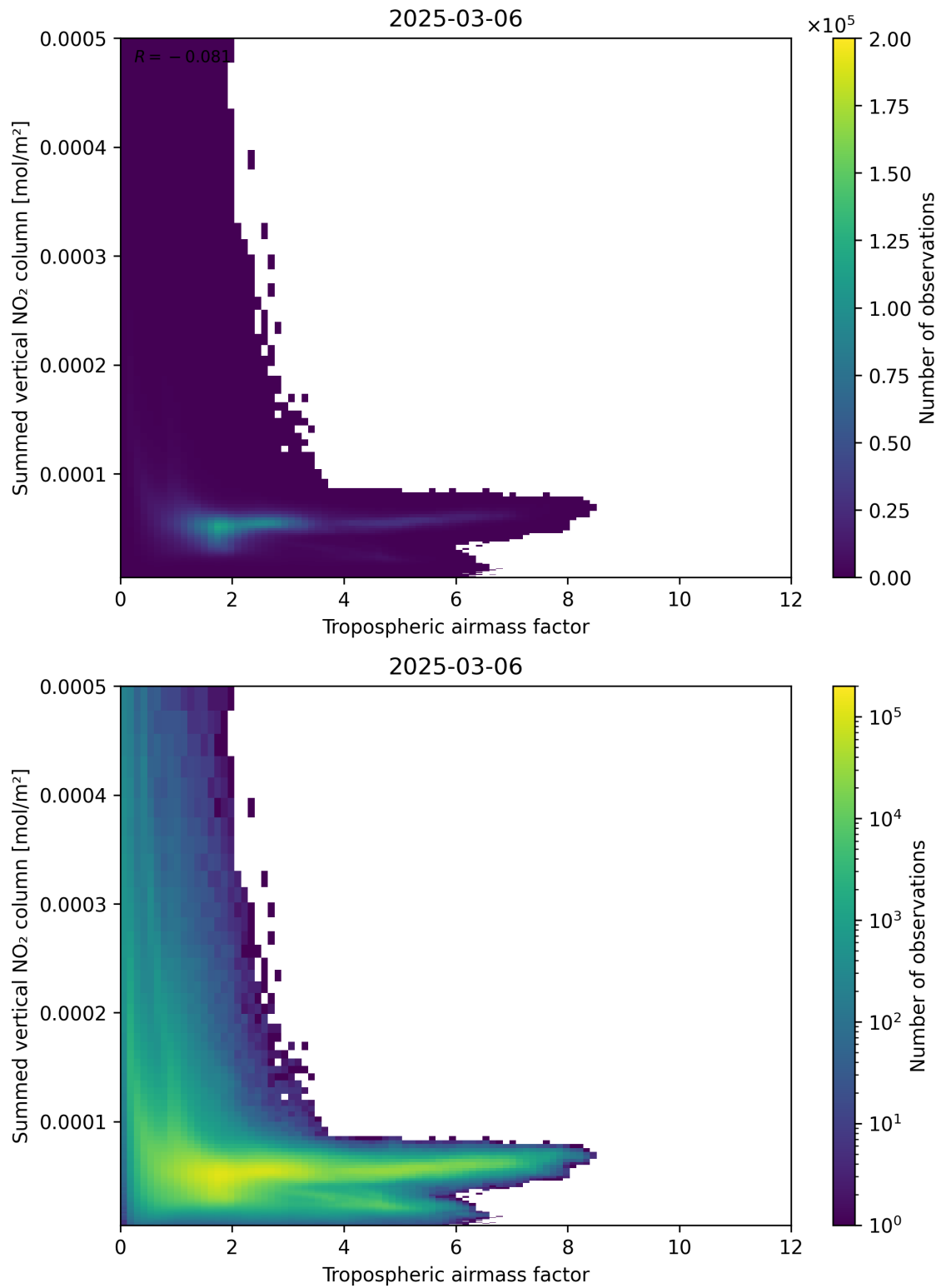
Figure 75: Scatter density plot of “Tropospheric air mass factor” against “Summed vertical NO 2 column” for 2025-03-06 to 2025-03-07.
