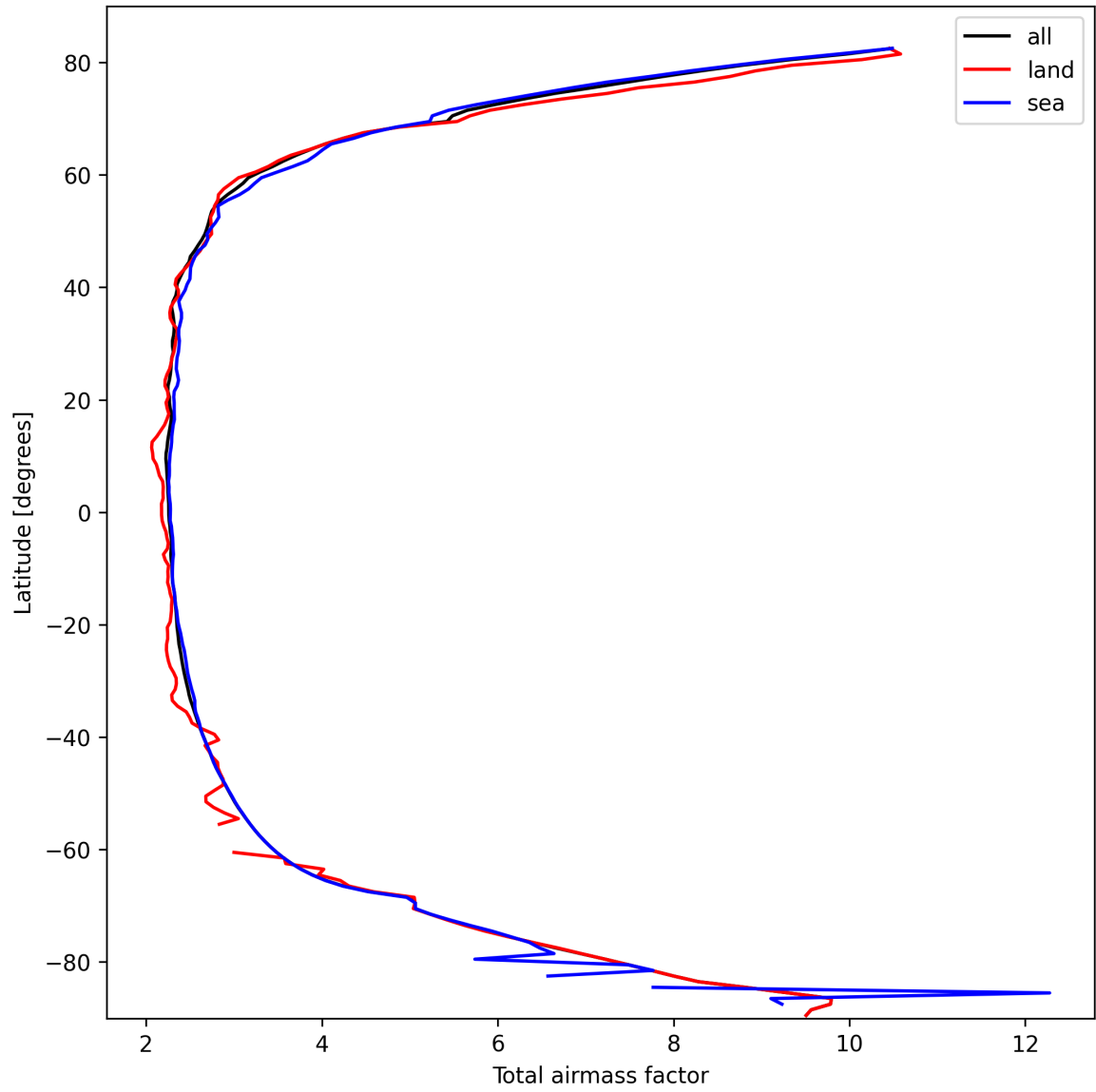
Figure 15: Zonal average of “Total airmass factor” for 2025-03-06 to 2025-03-07.
