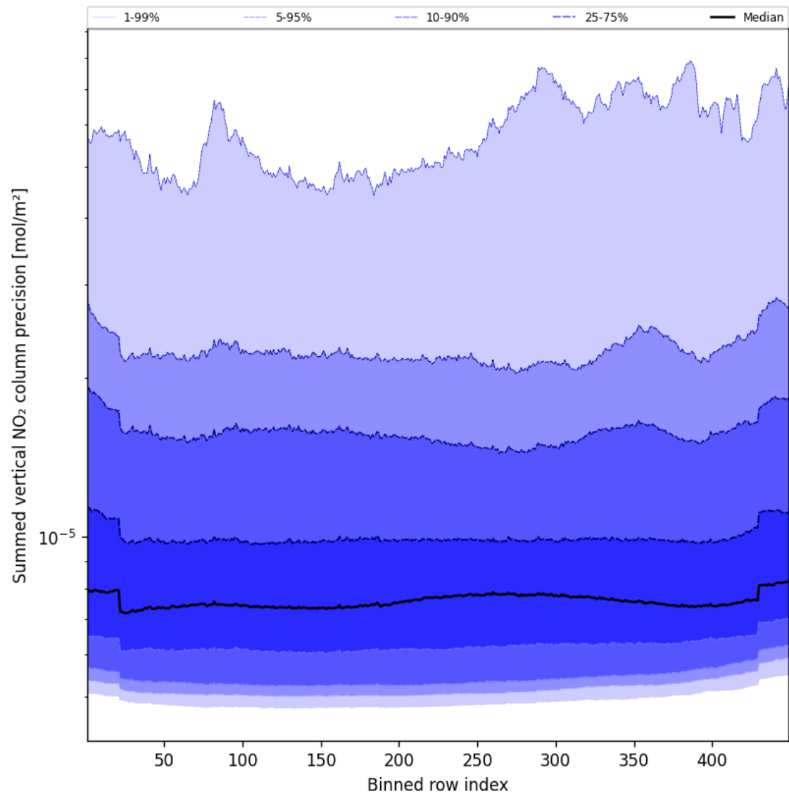
Figure 58: Along track statistics of “Summed vertical NO 2 column precision” for 2025-03-06 to 2025-03-07
