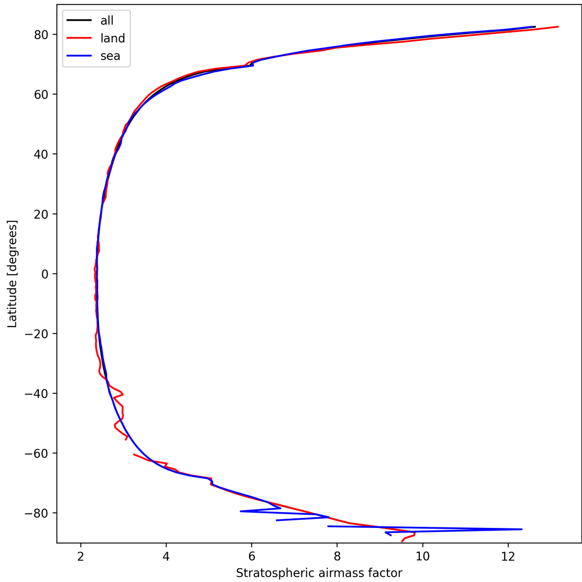
Figure 27: Zonal average of “Stratospheric airmass factor” for 2025-03-06 to 2025-03-07.
