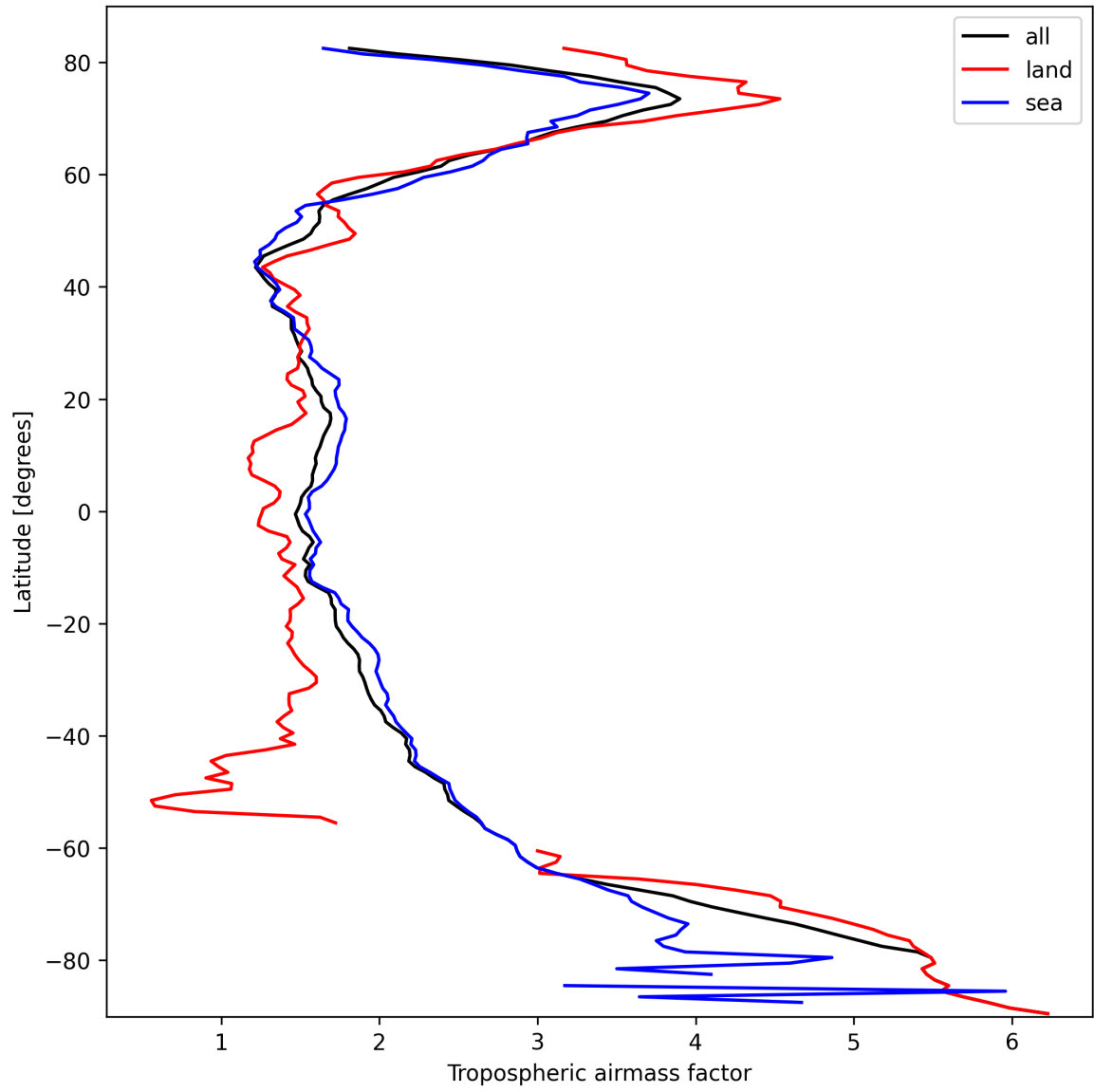
Figure 14: Zonal average of “Tropospheric air mass factor” for 2025-03-06 to 2025-03-07.
