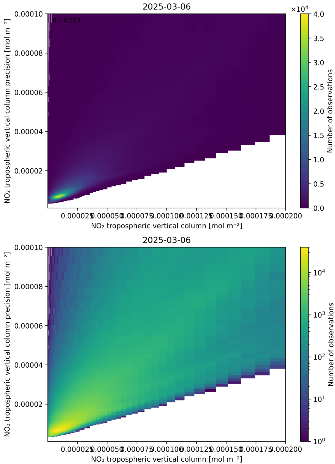
Figure 130: Scatter density plot of “NO 2 tropospheric vertical column” against “NO 2 tropospheric vertical column precision” for 2025-03-06 to 2025-03-07.
