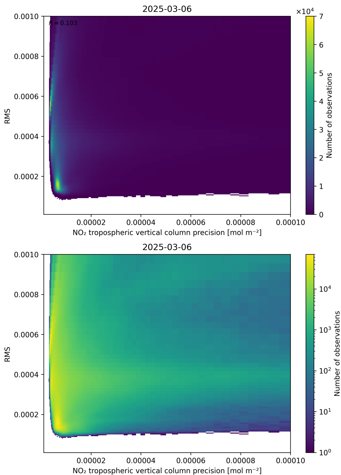
Figure 140: Scatter density plot of “NO 2 tropospheric vertical column precision” against “RMS” for 2025-03-06 to 2025-03-07.
