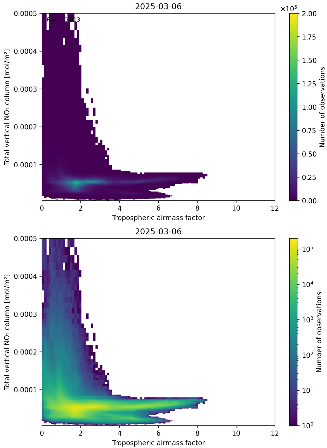
Figure 77: Scatter density plot of “Tropospheric airmass factor” against “Total vertical NO 2 column” for 2025-03-06 to 2025-03-07.
