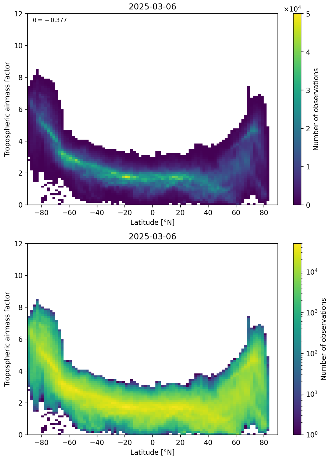
Figure 85: Scatter density plot of “Latitude” against “Tropospheric airmass factor” for 2025-03-06 to 2025-03-07.
