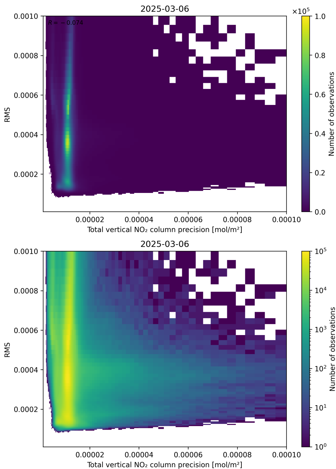
Figure 119: Scatter density plot of “Total vertical NO 2 column precision” against “RMS” for 2025-03-06 to 2025-03-07.
