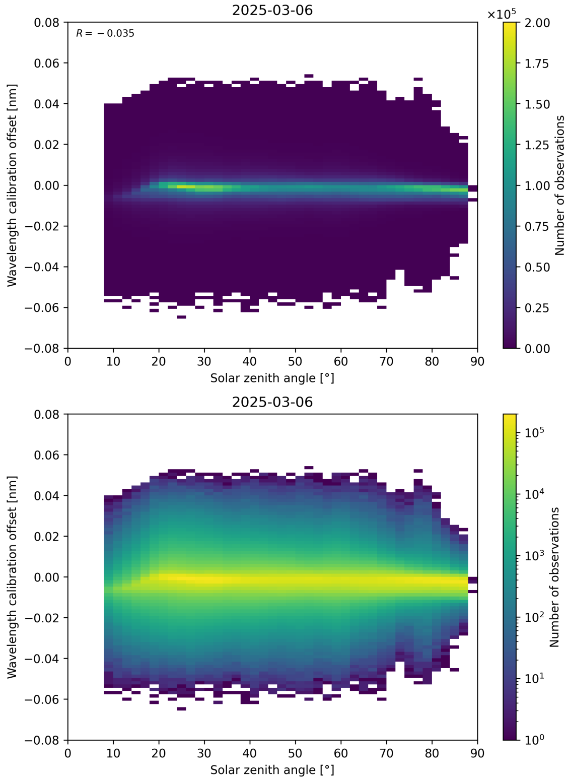
Figure 158: Scatter density plot of “Solar zenith angle” against “Wavelength calibration offset” for 2025-03-06 to 2025-03-07.
