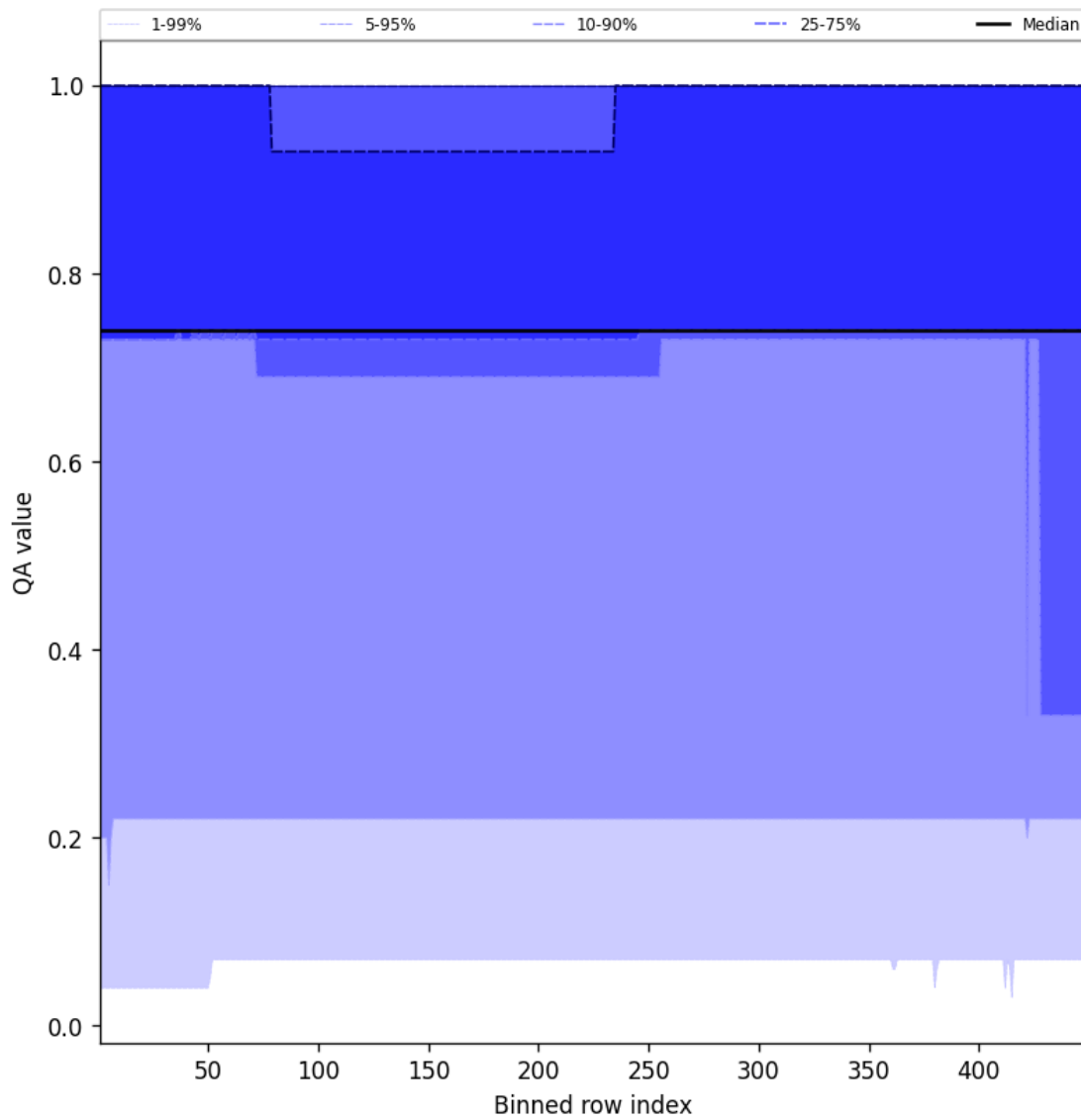
Figure 45: Along track statistics of “QA value” for 2025-03-06 to 2025-03-07
