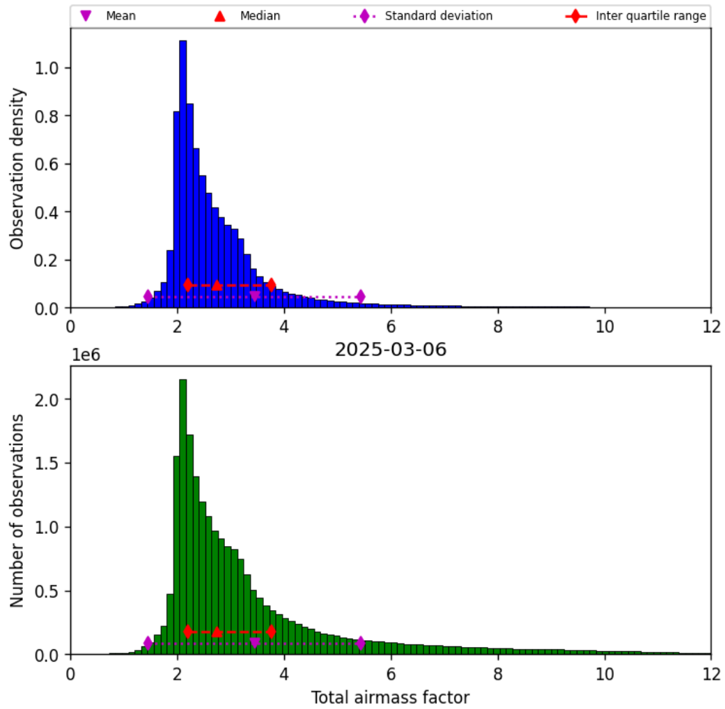
Figure 32: Histogram of “Total airmass factor” for 2025-03-06 to 2025-03-07
