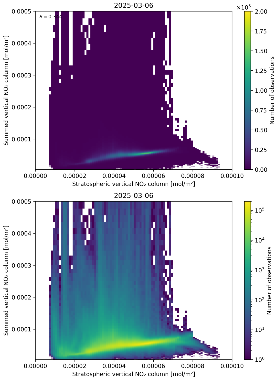
Figure 98: Scatter density plot of “Stratospheric vertical NO 2 column” against “Summed vertical NO 2 column” for 2025-03-06 to 2025-03-07.
