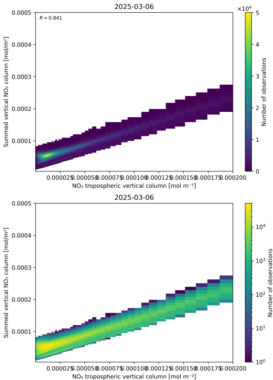
Figure 126: Scatter density plot of “NO 2 tropospheric vertical column” against “Summed vertical NO 2 column” for 2025-03-06 to 2025-03-07.
