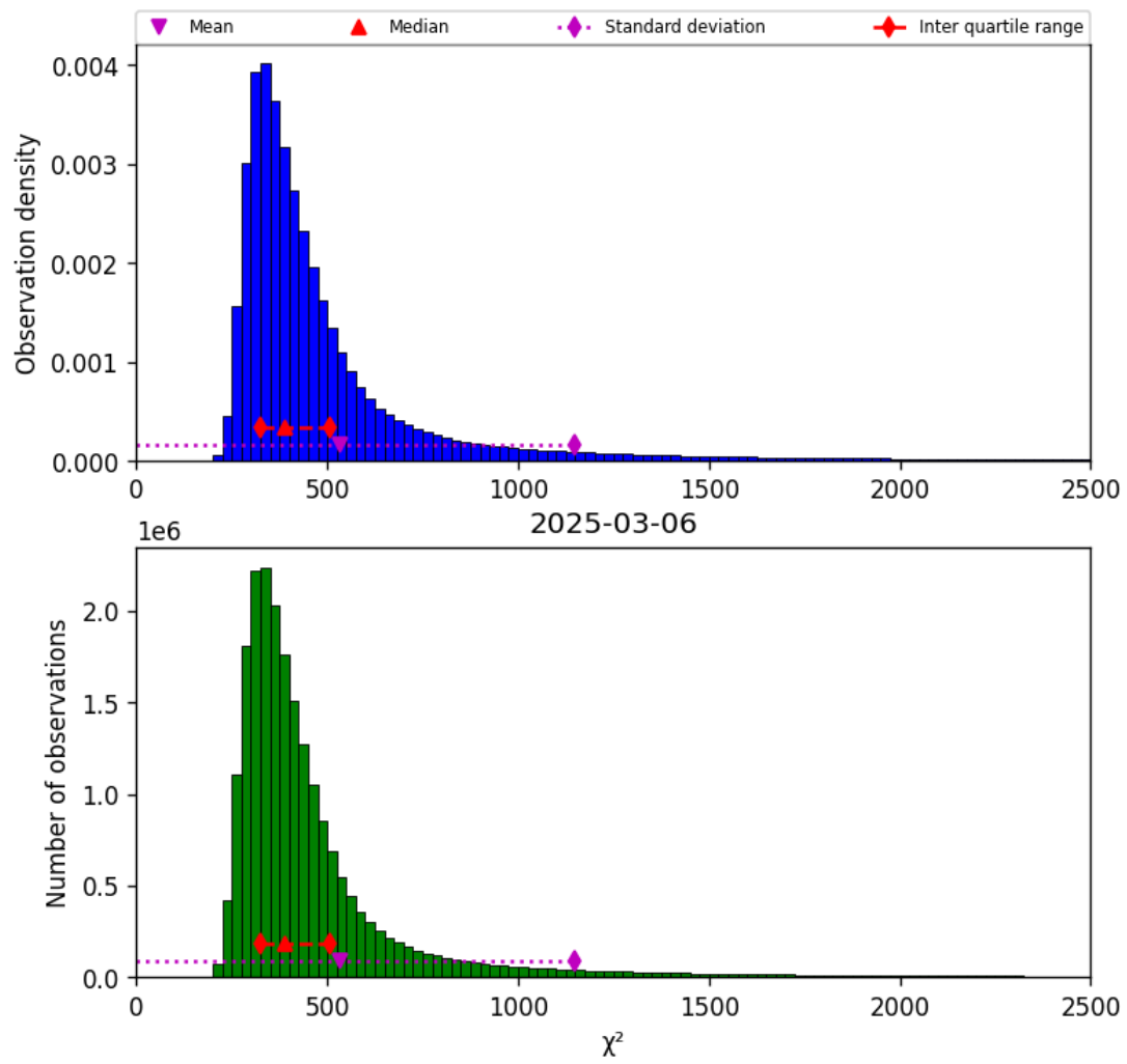
Figure 42: Histogram of " \chi^2 " for 2025-03-06 to 2025-03-07
