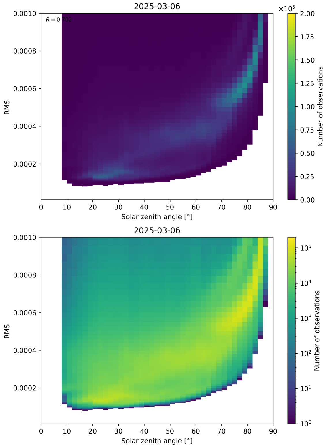
Figure 157: Scatter density plot of “Solar zenith angle” against “RMS” for 2025-03-06 to 2025-03-07.
