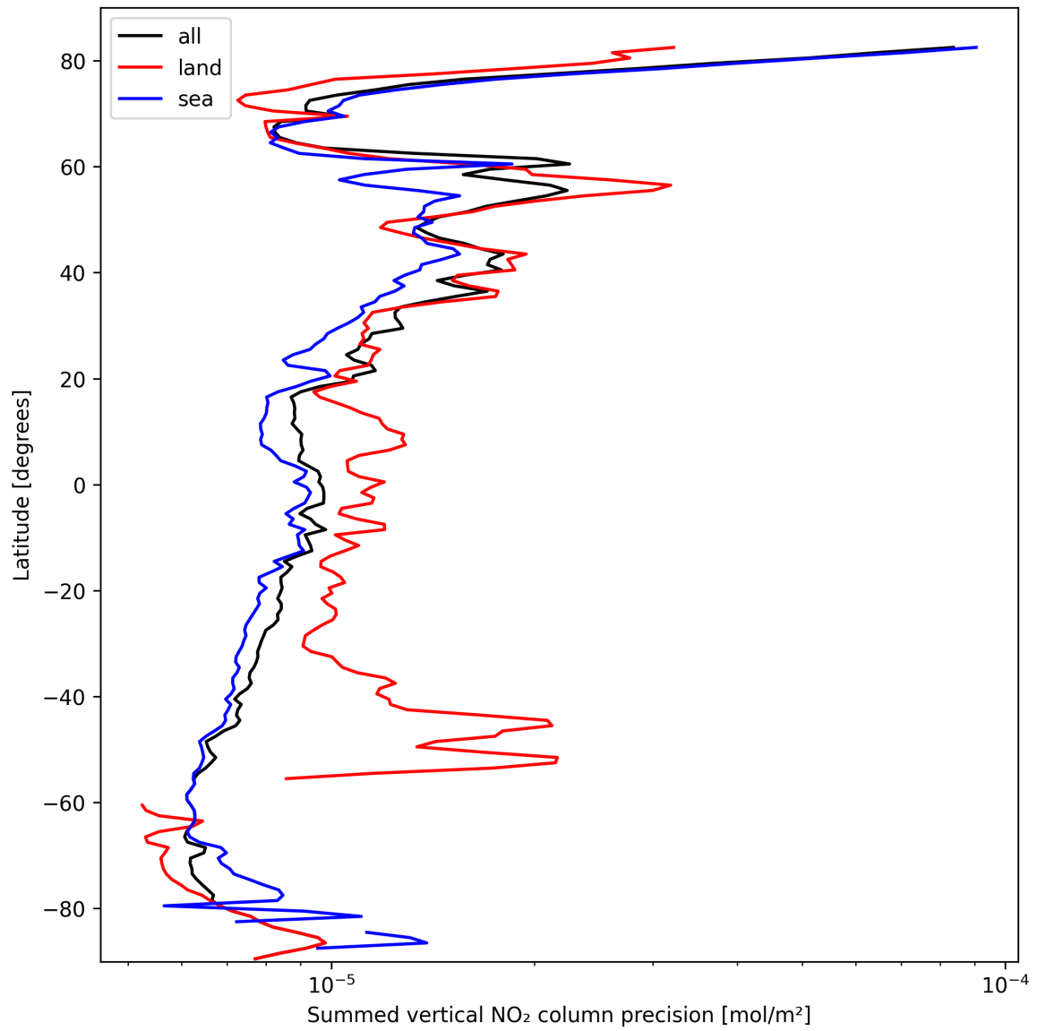
Figure 24: Zonal average of “Summed vertical NO 2 column precision” for 2025-03-06 to 2025-03-07.
