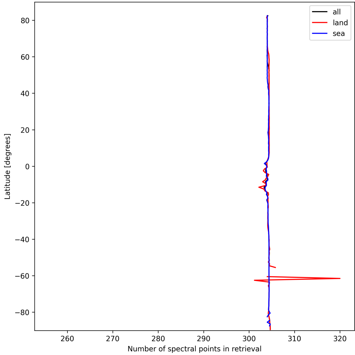
Figure 16: Zonal average of “Number of spectral points in retrieval” for 2025-03-06 to 2025-03-07.
