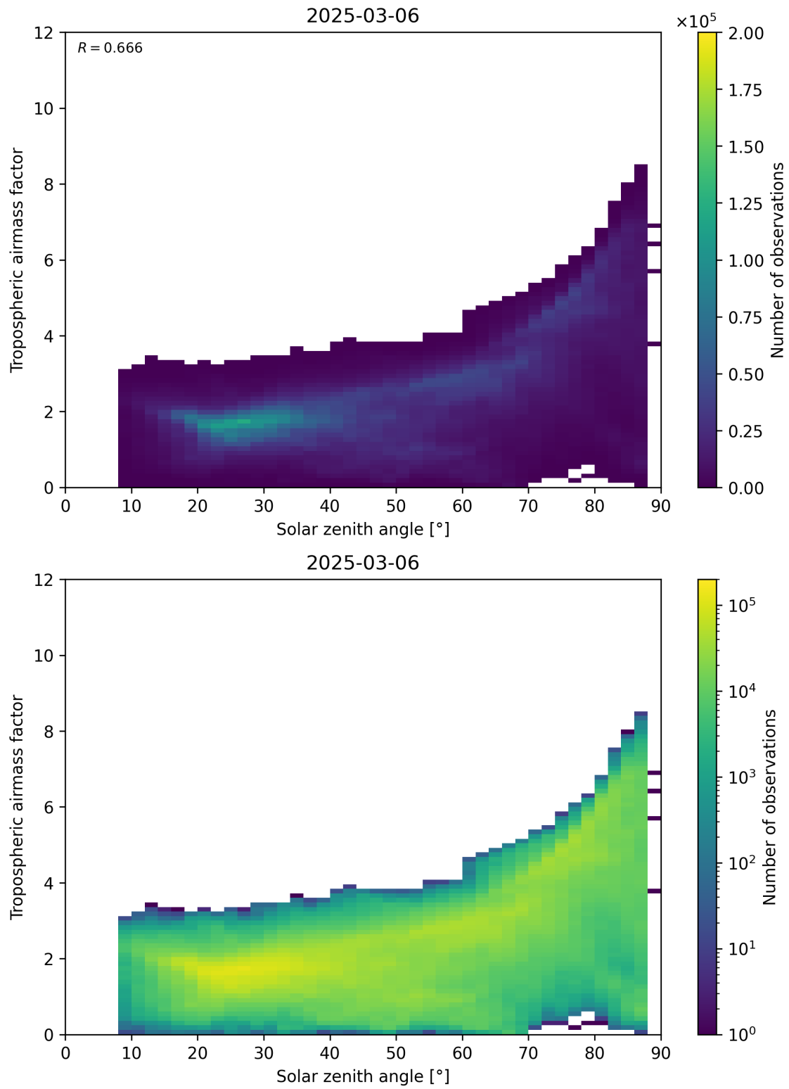
Figure 147: Scatter density plot of “Solar zenith angle” against “Tropospheric airmass factor” for 2025-03-06 to 2025-03-07.
