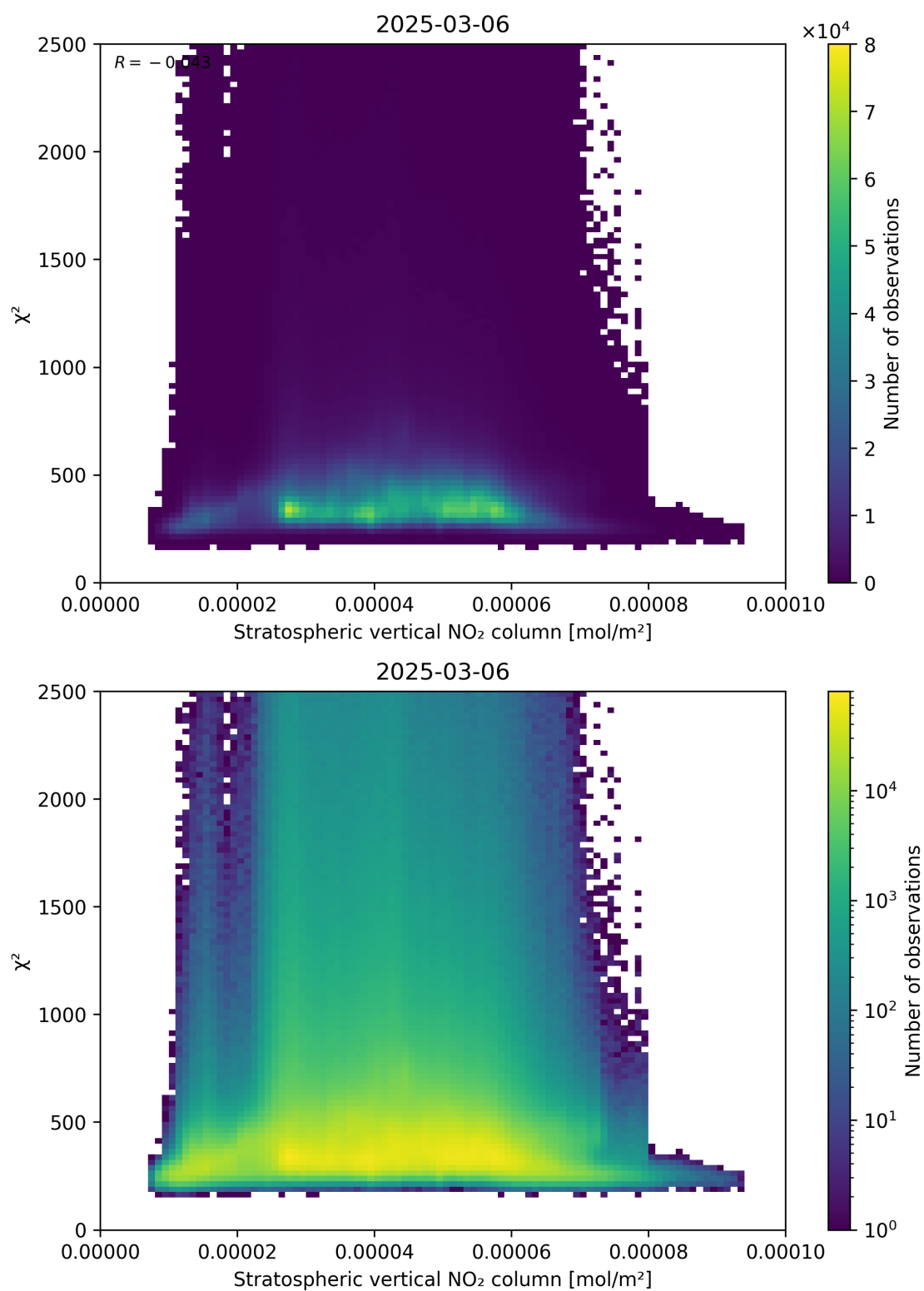
Figure 97: Scatter density plot of “Stratospheric vertical NO 2 column” against “ \chi^2 ” for 2025-03-06 to 2025-03-07.
