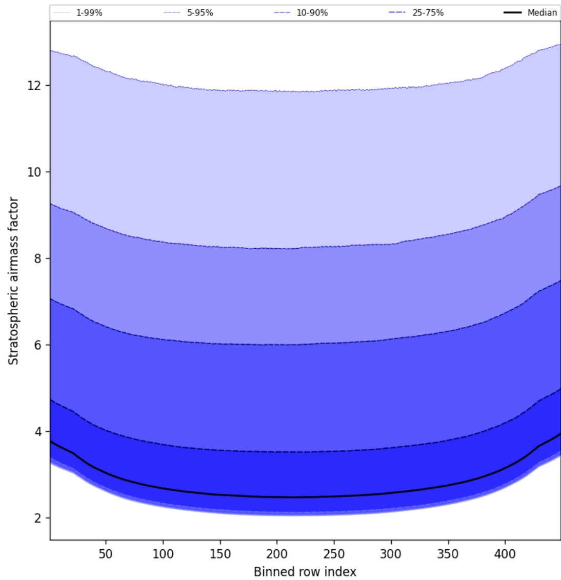
Figure 61: Along track statistics of “Stratospheric airmass factor” for 2025-03-06 to 2025-03-07
