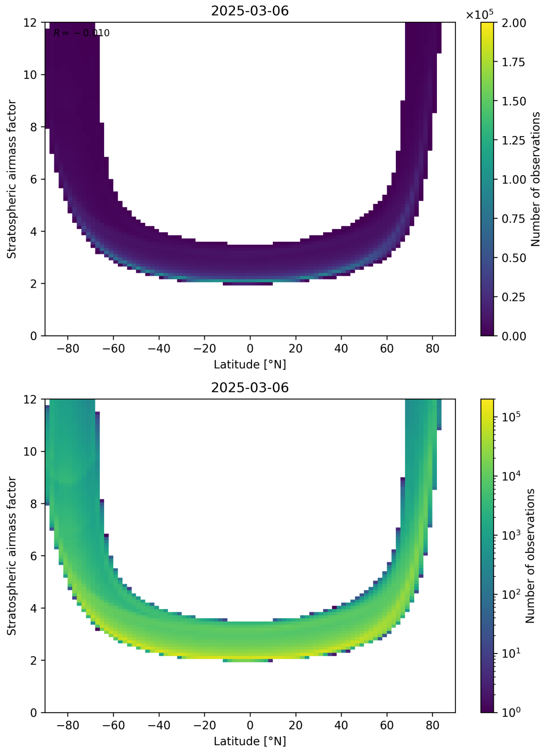
Figure 83: Scatter density plot of “Latitude” against “Stratospheric airmass factor” for 2025-03-06 to 2025-03-07.
