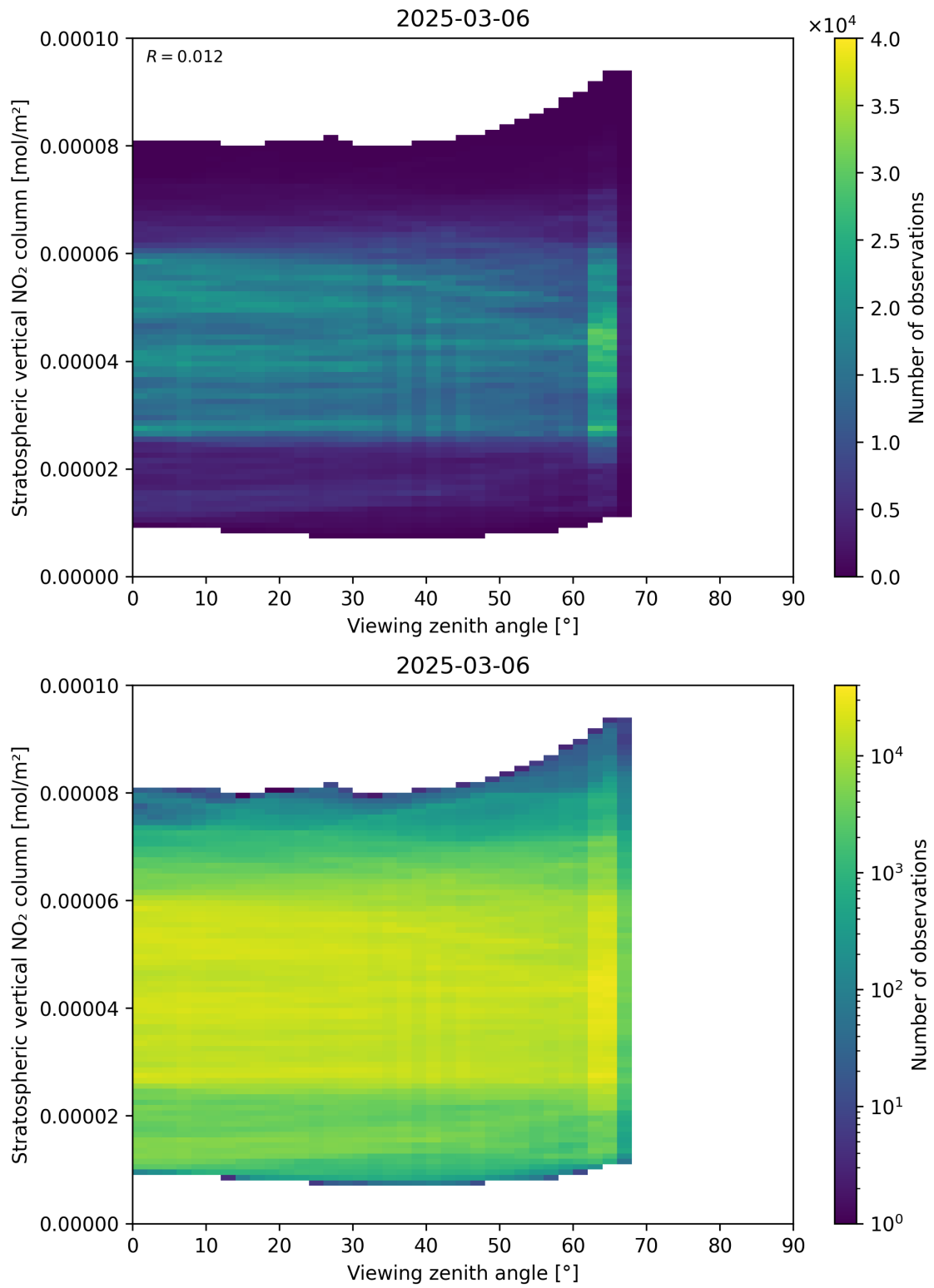
Figure 164: Scatter density plot of “Viewing zenith angle” against “Stratospheric vertical NO 2 column” for 2025-03-06 to 2025-03-07.
