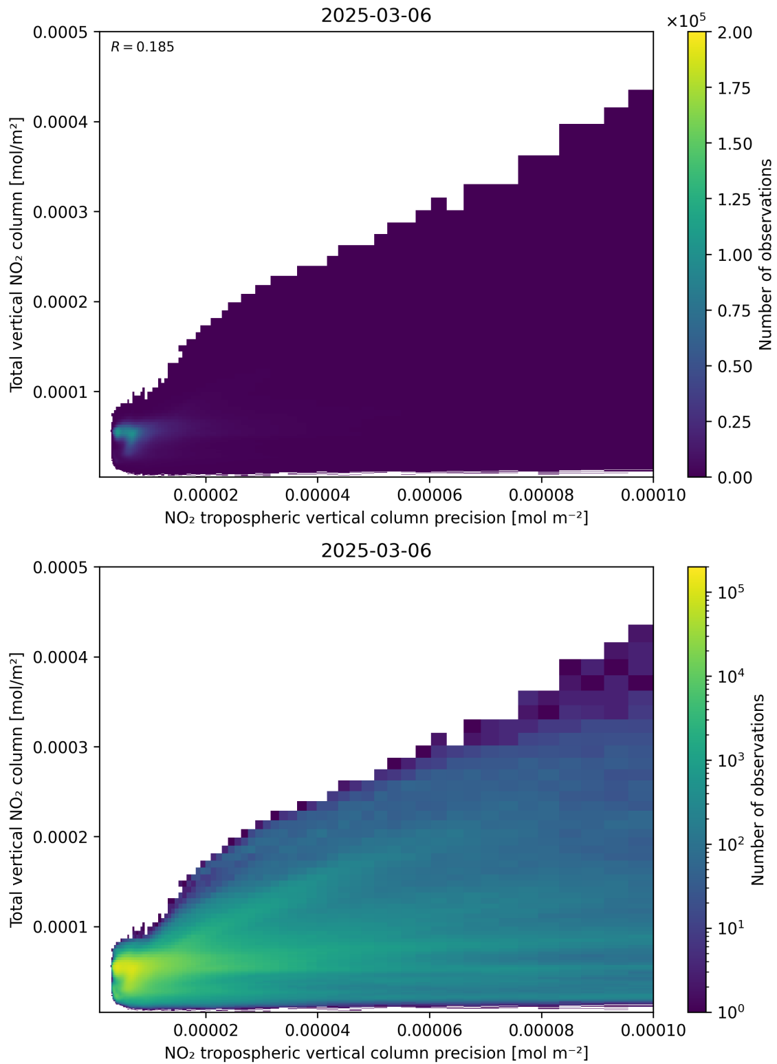
Figure 138: Scatter density plot of “NO 2 tropospheric vertical column precision” against “Total vertical NO 2 column” for 2025-03-06 to 2025-03-07.
