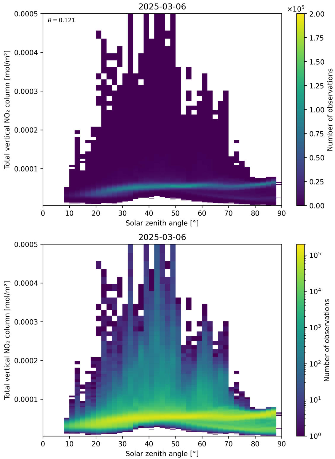
Figure 153: Scatter density plot of “Solar zenith angle” against “Total vertical NO 2 column” for 2025-03-06 to 2025-03-07.
