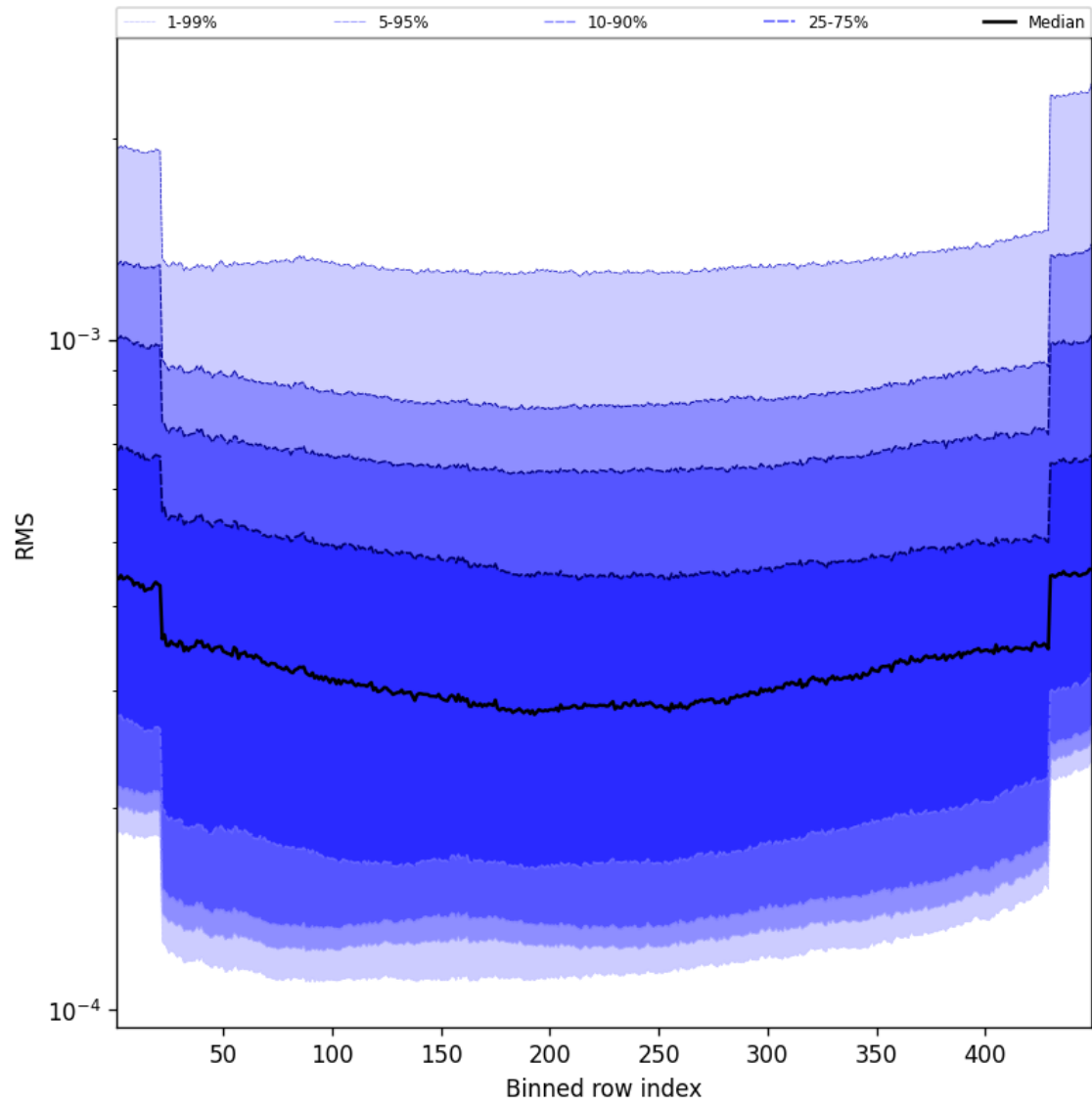
Figure 60: Along track statistics of “RMS” for 2025-03-06 to 2025-03-07
