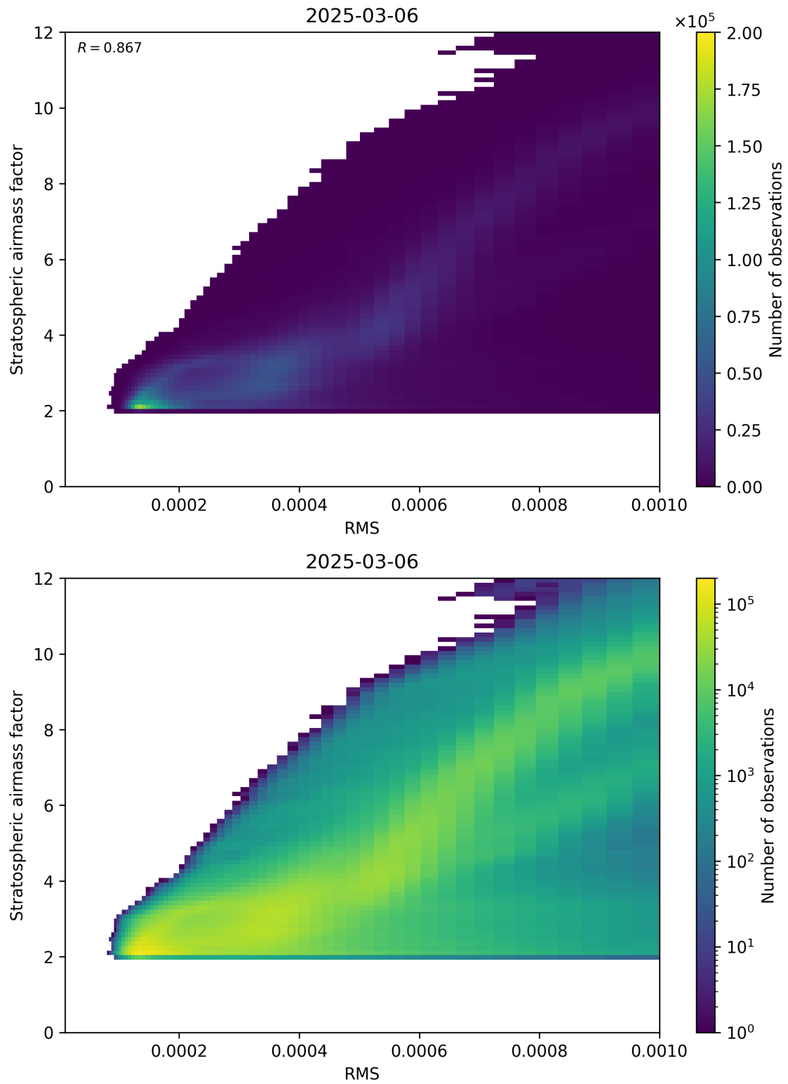
Figure 144: Scatter density plot of “RMS” against “Stratospheric airmass factor” for 2025-03-06 to 2025-03-07.
