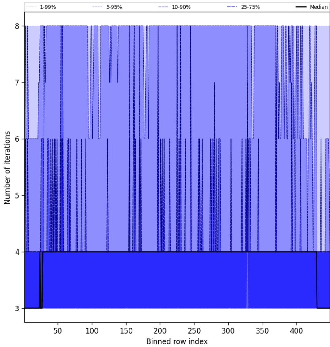
Figure 51: Along track statistics of “Number of iterations” for 2025-03-06 to 2025-03-07
