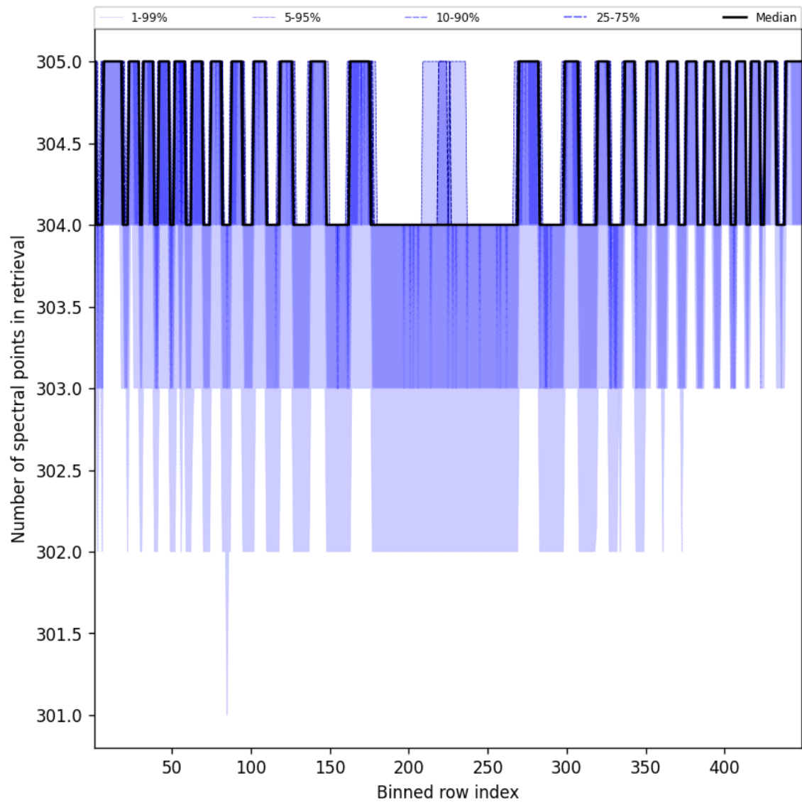
Figure 50: Along track statistics of “Number of spectral points in retrieval” for 2025-03-06 to 2025-03-07
