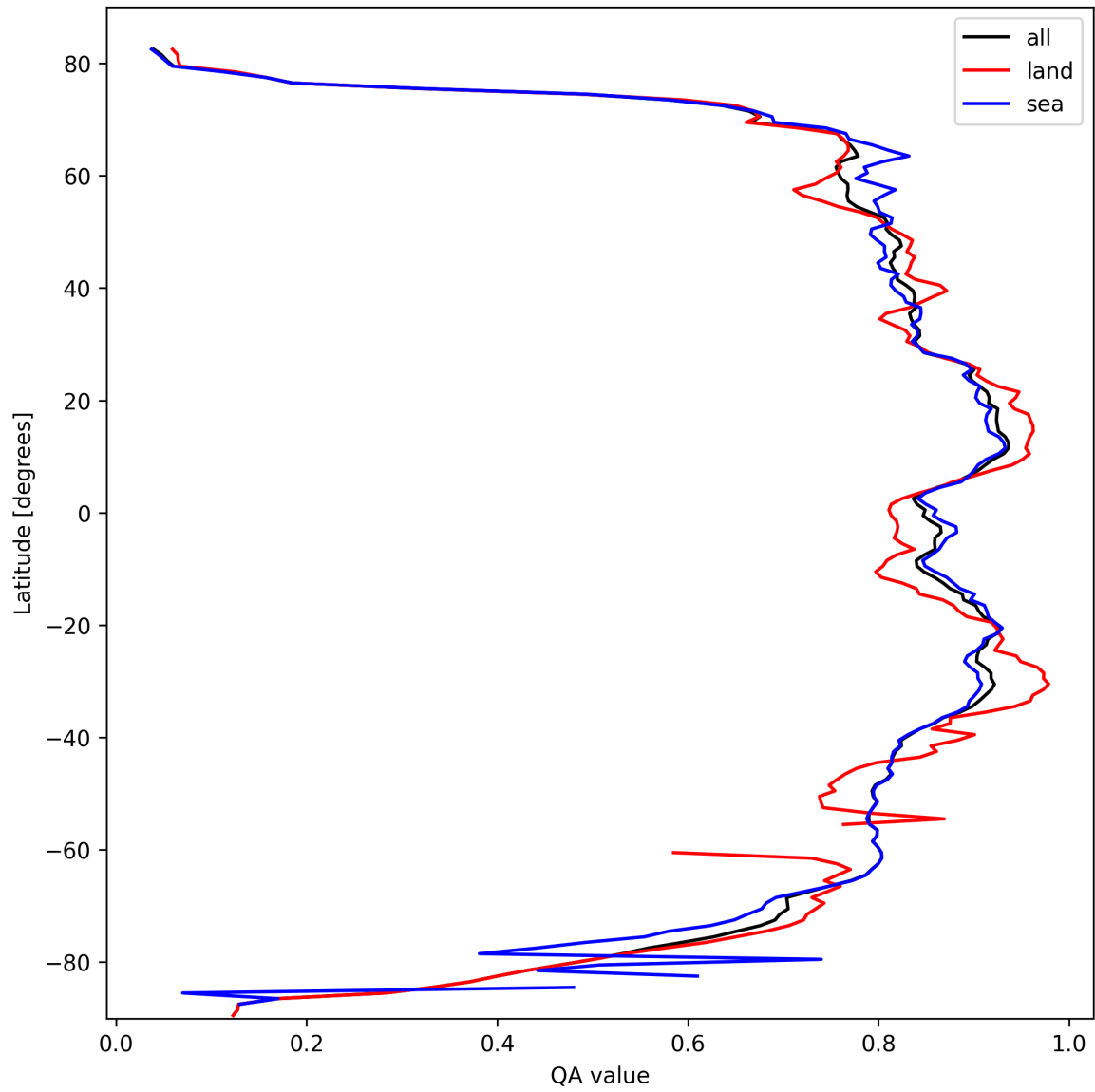
Figure 11: Zonal average of “QA value” for 2025-03-06 to 2025-03-07.
