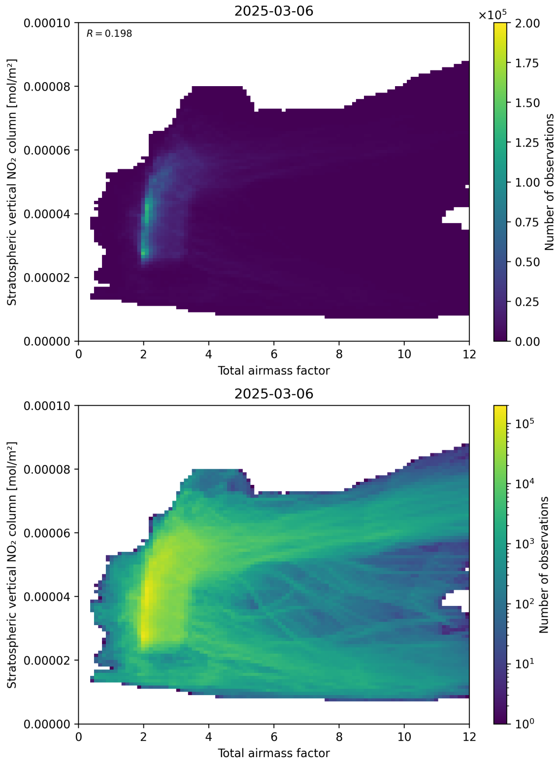
Figure 64: Scatter density plot of “Total airmass factor” against “Stratospheric vertical \text{NO}_2 column” for 2025-03-06 to 2025-03-07.
