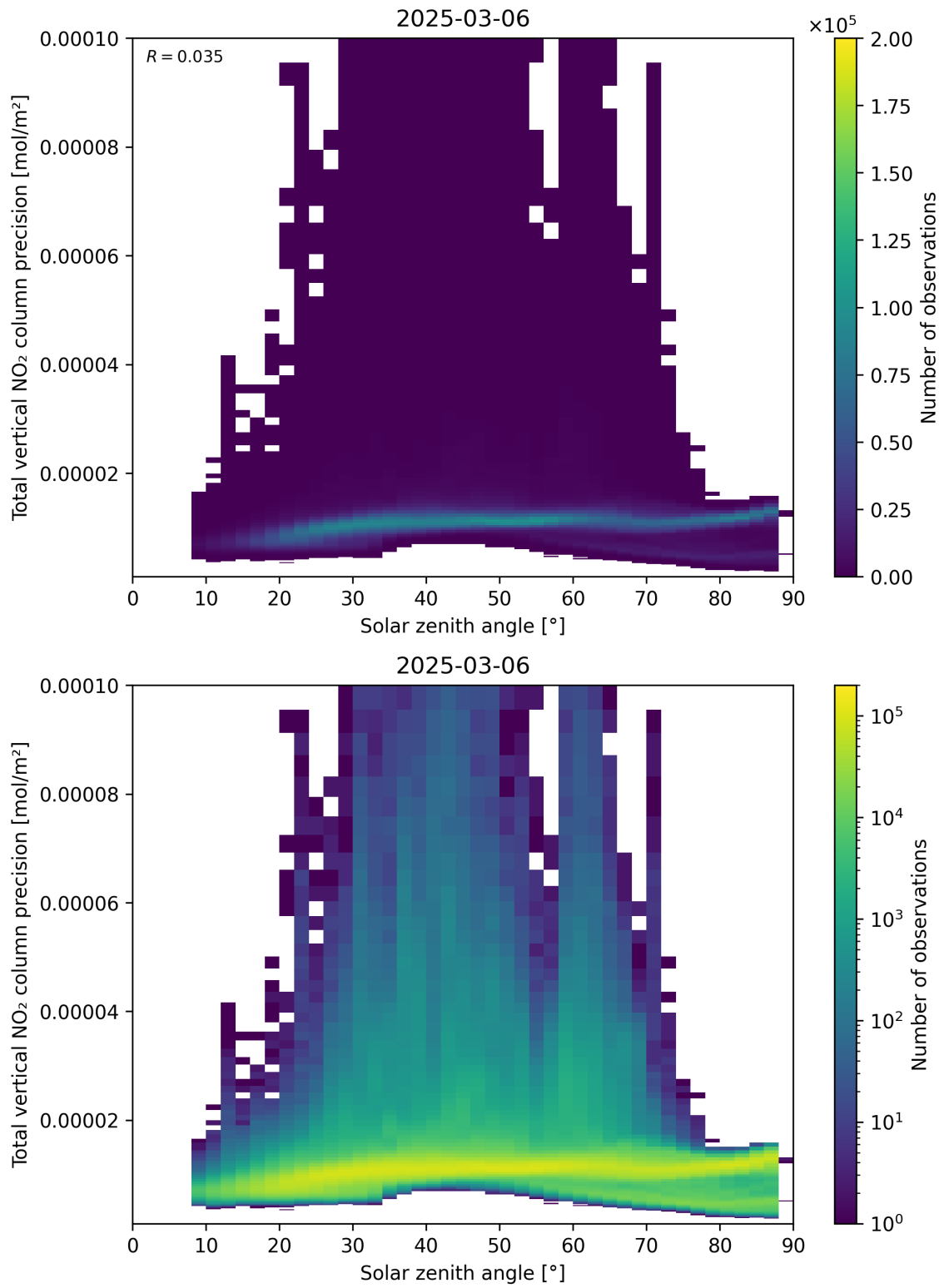
Figure 154: Scatter density plot of “Solar zenith angle” against “Total vertical NO 2 column precision” for 2025-03-06 to 2025-03-07.
