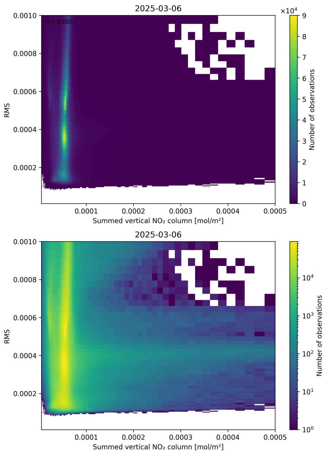
Figure 109: Scatter density plot of “Summed vertical NO 2 column” against “RMS” for 2025-03-06 to 2025-03-07.
