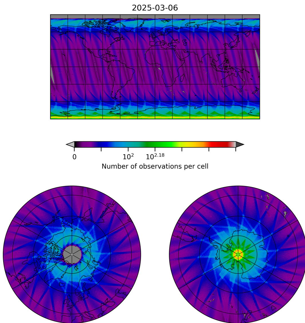
Figure 10: Map of the number of observations for 2025-03-06 to 2025-03-07
