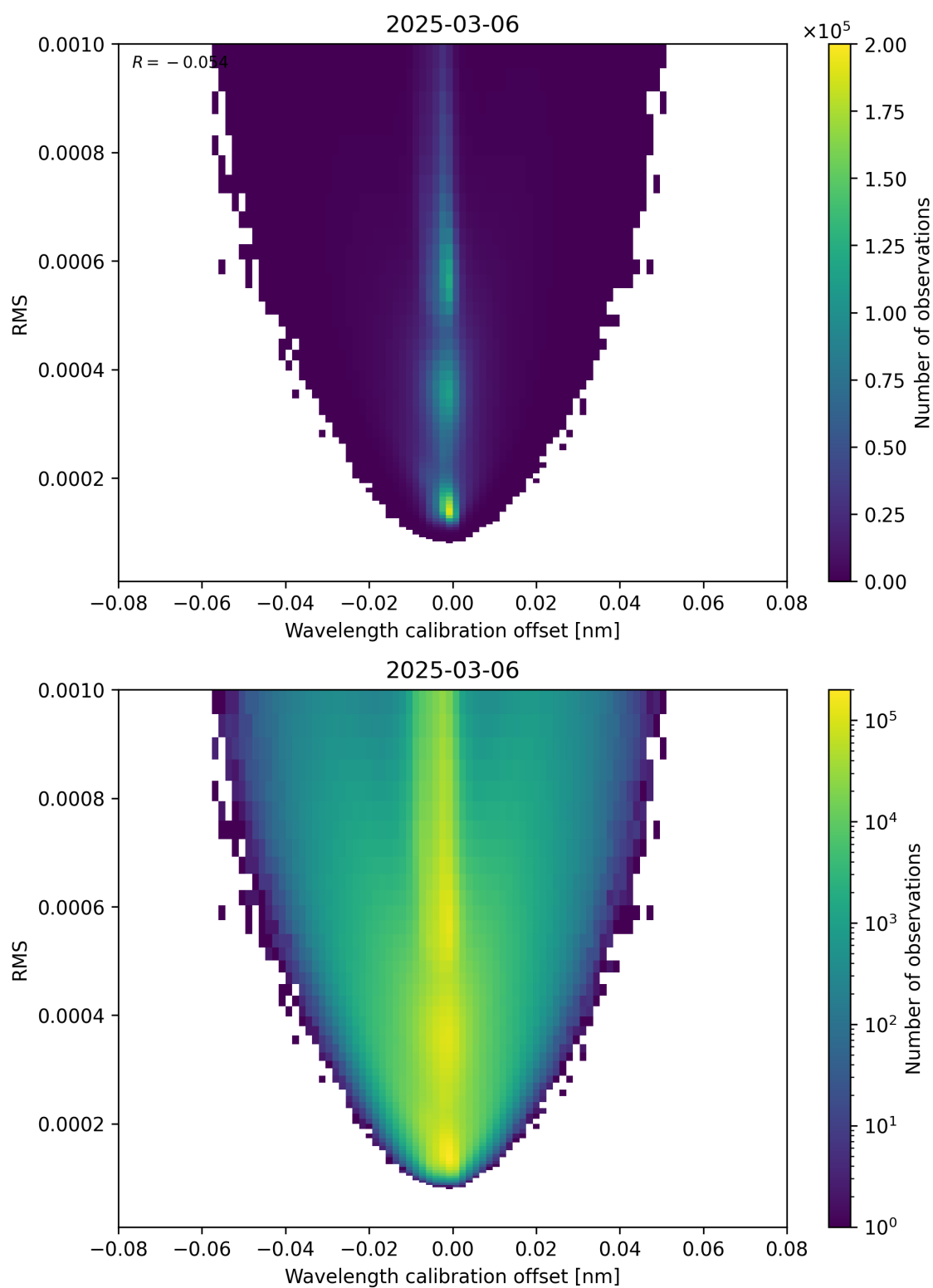
Figure 181: Scatter density plot of “Wavelength calibration offset” against “RMS” for 2025-03-06 to 2025-03-07.
