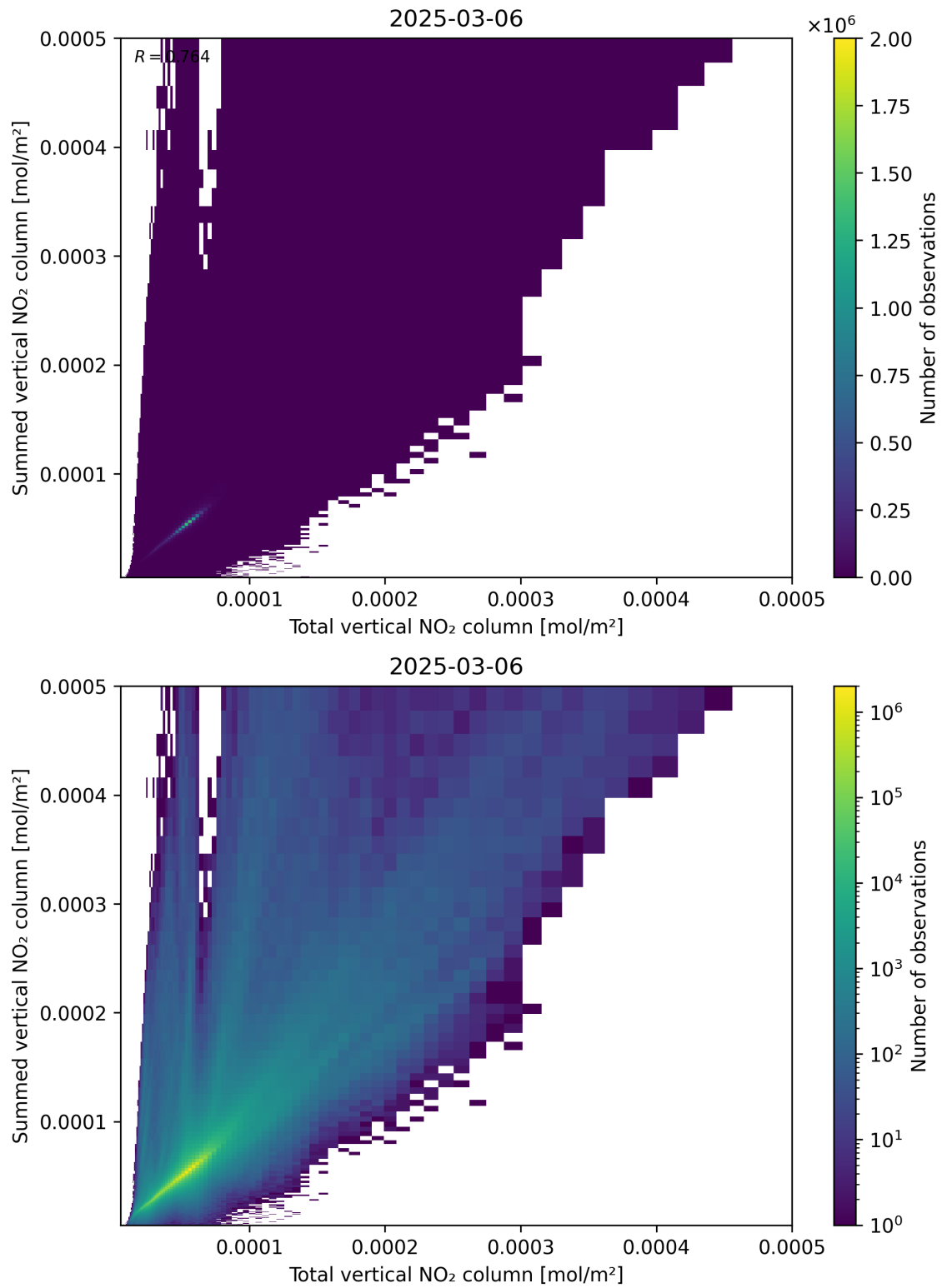
Figure 112: Scatter density plot of “Total vertical NO 2 column” against “Summed vertical NO 2 column” for 2025-03-06 to 2025-03-07.
