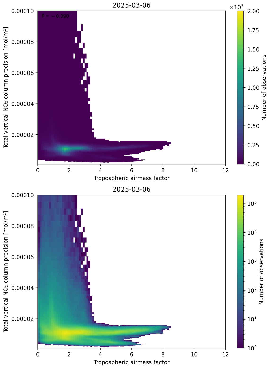
Figure 78: Scatter density plot of “Tropospheric air mass factor” against “Total vertical NO 2 column precision” for 2025-03-06 to 2025-03-07.
