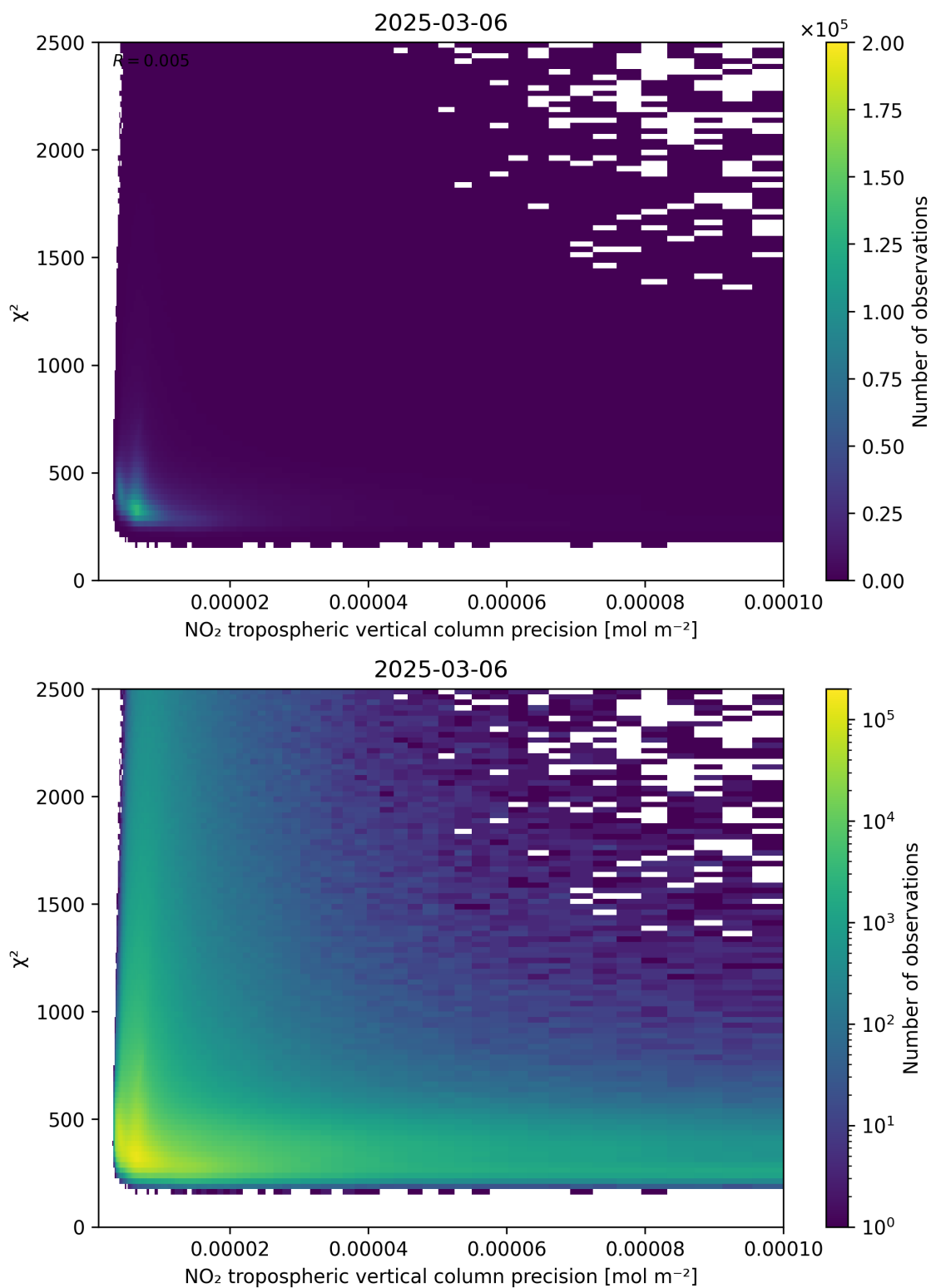
Figure 134: Scatter density plot of “NO 2 tropospheric vertical column precision” against “ \chi^2 ” for 2025-03-06 to 2025-03-07.
