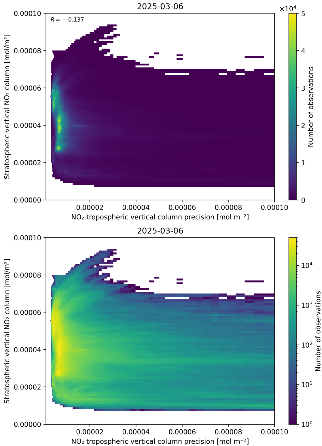
Figure 135: Scatter density plot of “NO 2 tropospheric vertical column precision” against “Stratospheric vertical NO 2 column” for 2025-03-06 to 2025-03-07.
