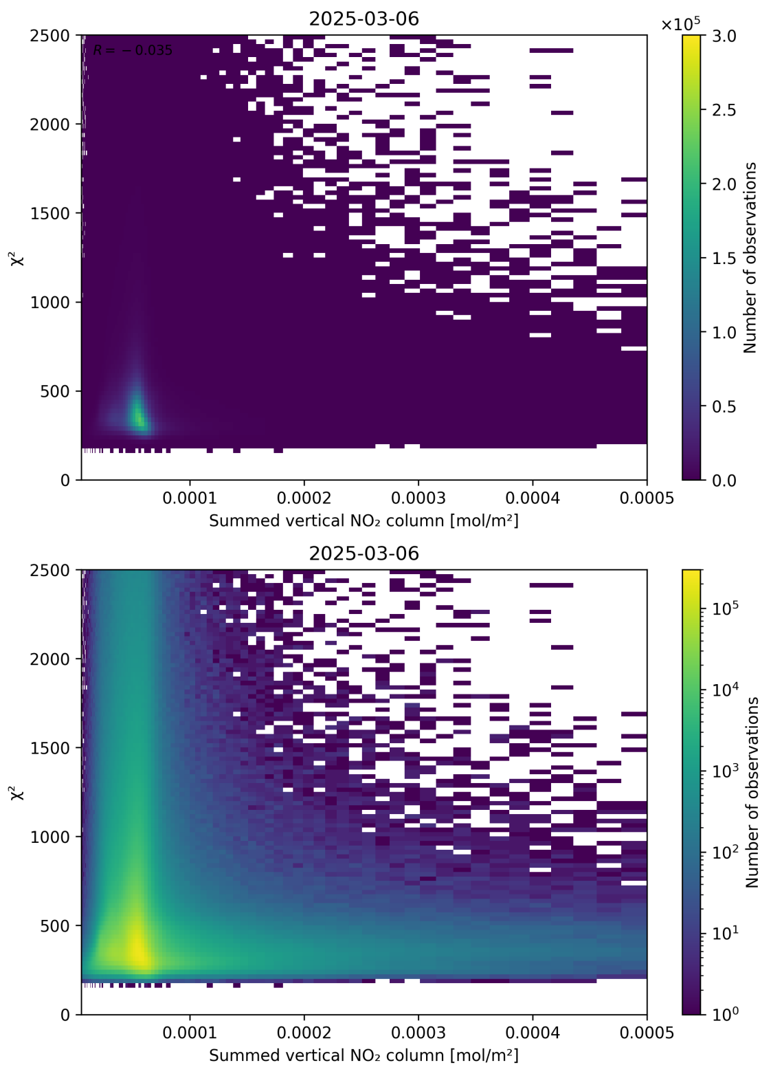
Figure 104: Scatter density plot of “Summed vertical NO 2 column” against “ \chi^2 ” for 2025-03-06 to 2025-03-07.
