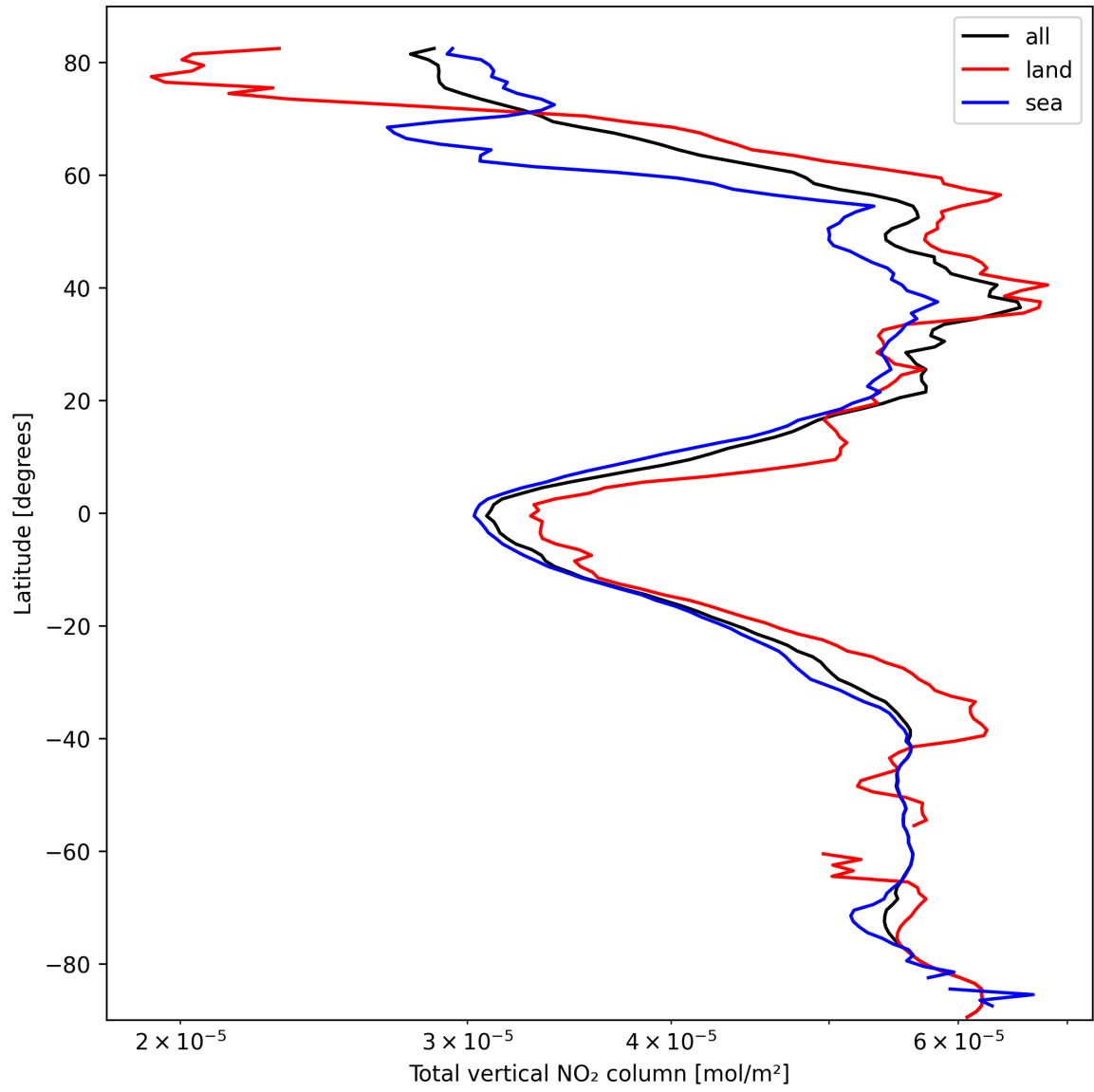
Figure 21: Zonal average of “Total vertical NO 2 column” for 2025-03-06 to 2025-03-07.
