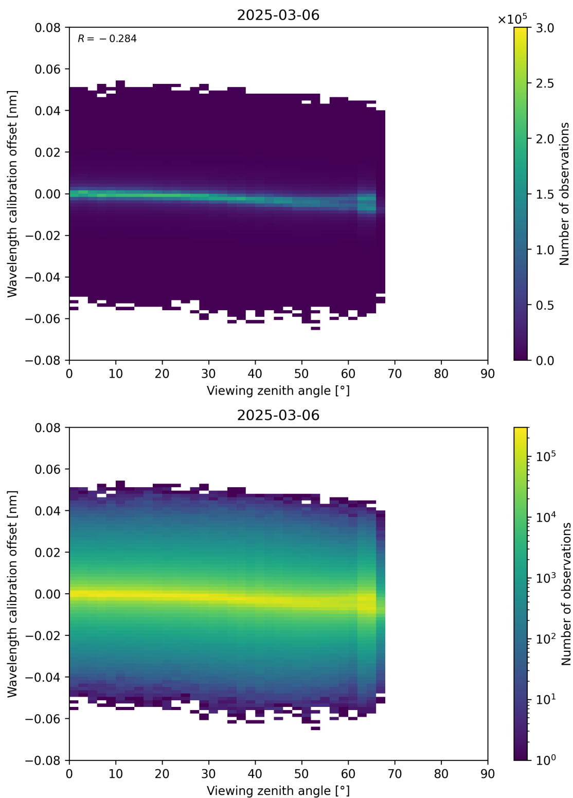
Figure 173: Scatter density plot of “Viewing zenith angle” against “Wavelength calibration offset” for 2025-03-06 to 2025-03-07.
