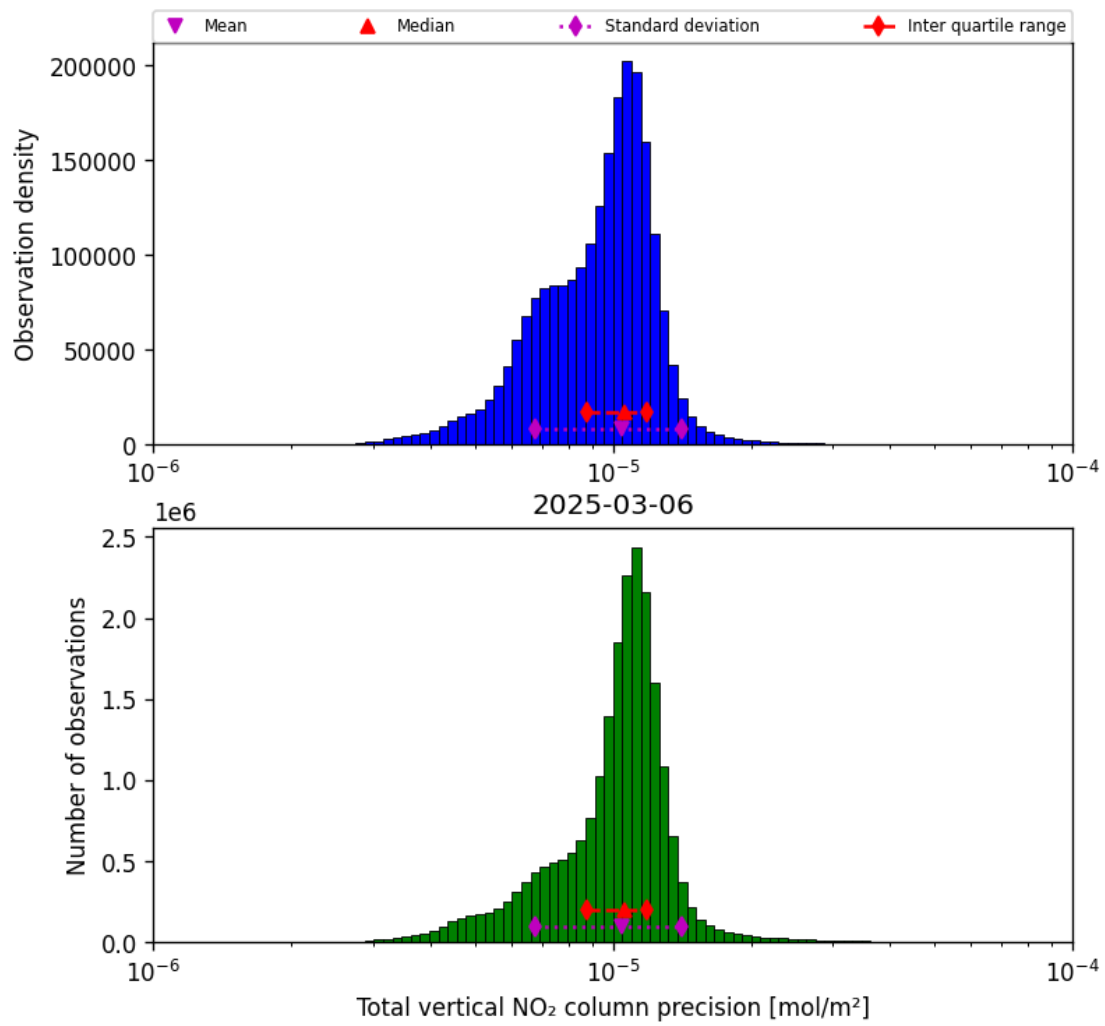
Figure 39: Histogram of "Total vertical NO 2 column precision" for 2025-03-06 to 2025-03-07
