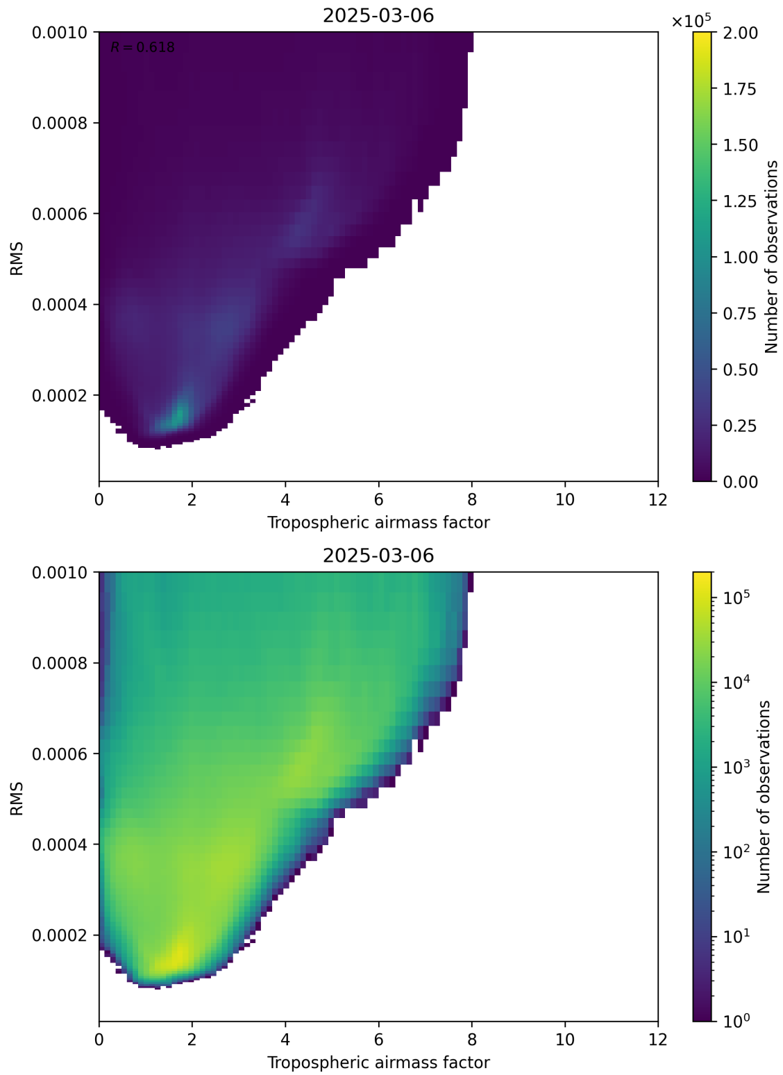
Figure 79: Scatter density plot of “Tropospheric airmass factor” against “RMS” for 2025-03-06 to 2025-03-07.
