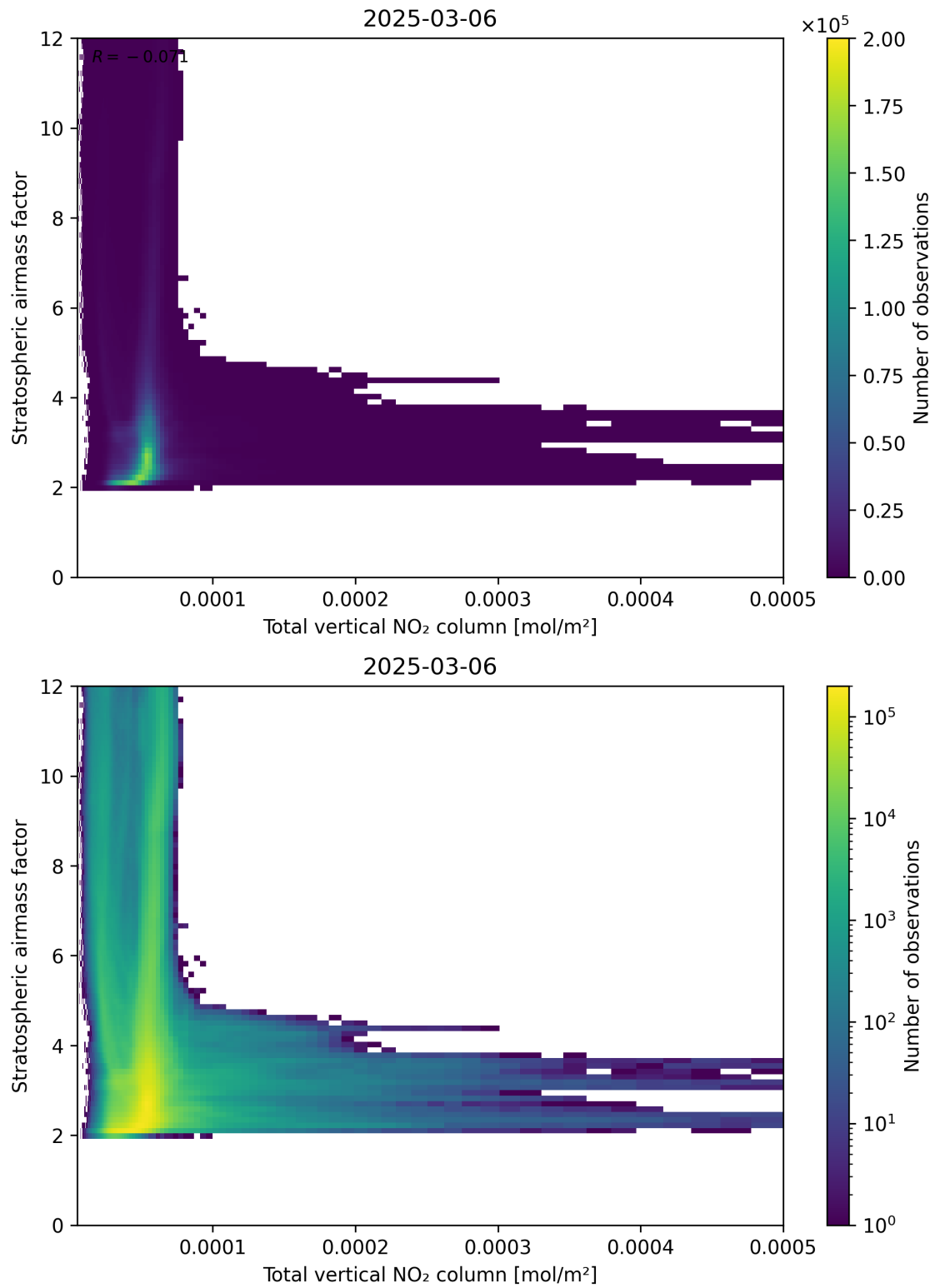
Figure 110: Scatter density plot of “Total vertical NO 2 column” against “Stratospheric airmass factor” for 2025-03-06 to 2025-03-07.
