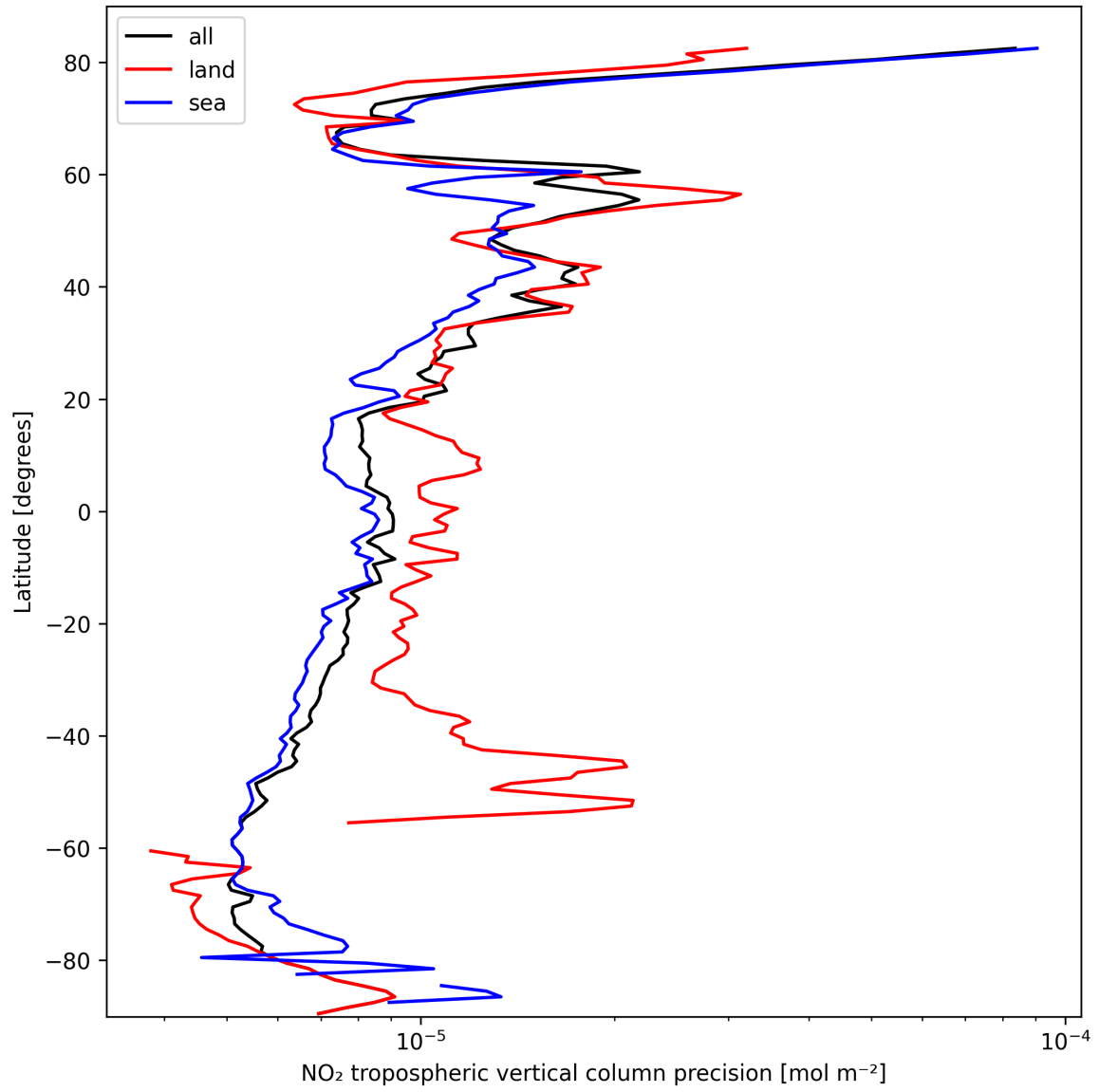
Figure 13: Zonal average of “NO 2 tropospheric vertical column precision” for 2025-03-06 to 2025-03-07.
