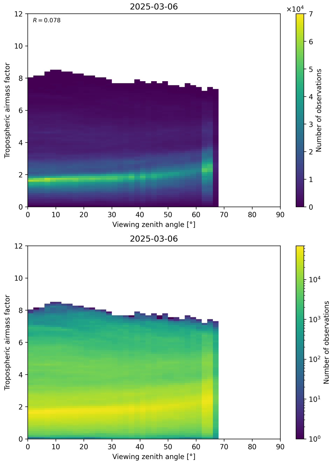
Figure 161: Scatter density plot of “Viewing zenith angle” against “Tropospheric airmass factor” for 2025-03-06 to 2025-03-07.
