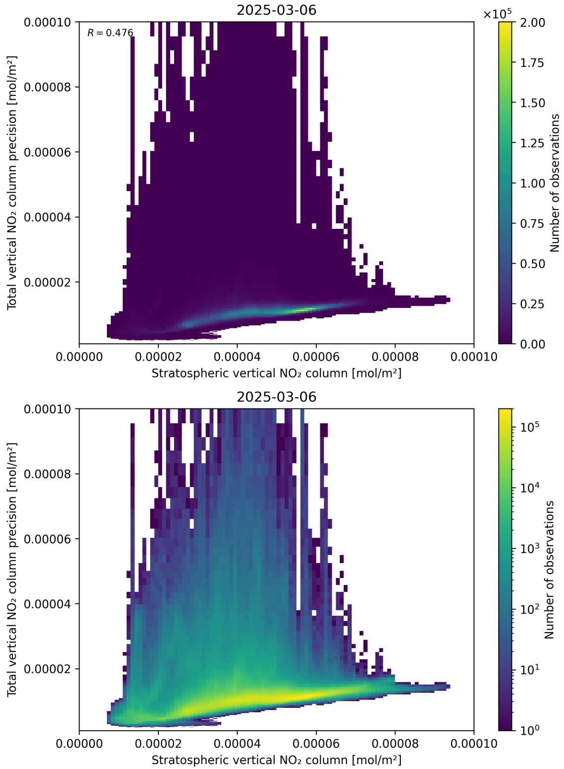
Figure 101: Scatter density plot of “Stratospheric vertical NO 2 column” against “Total vertical NO 2 column precision” for 2025-03-06 to 2025-03-07.
