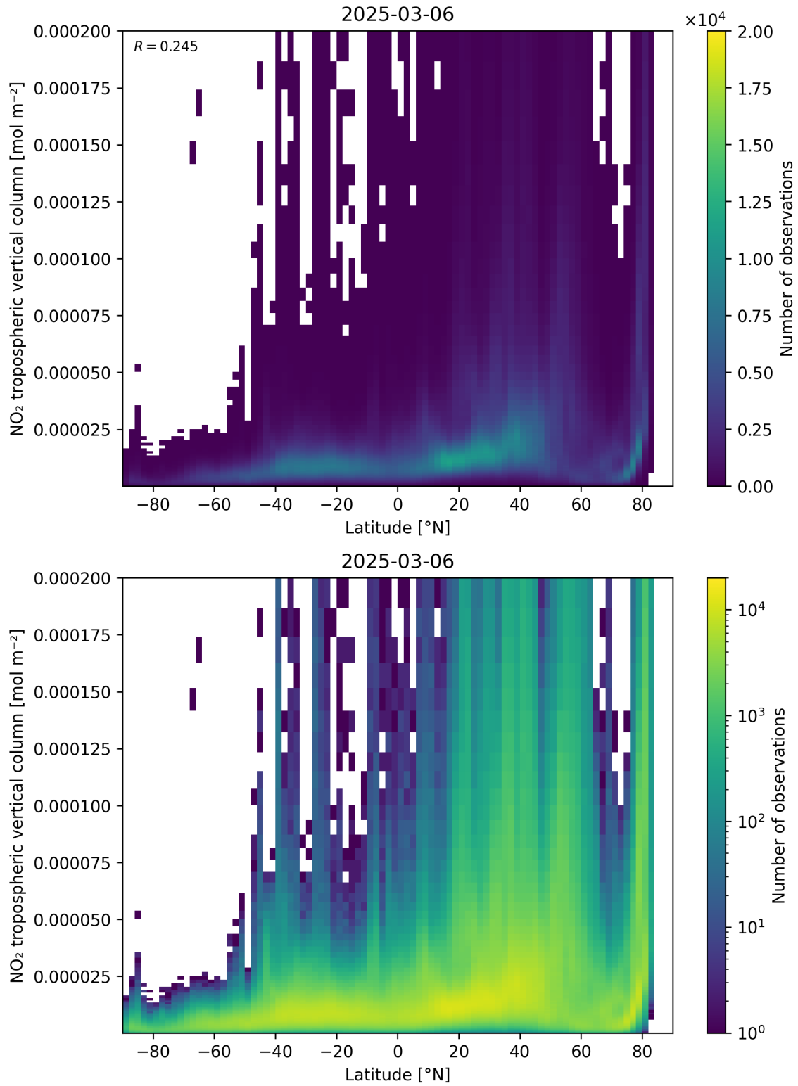
Figure 92: Scatter density plot of “Latitude” against “NO 2 tropospheric vertical column” for 2025-03-06 to 2025-03-07.
