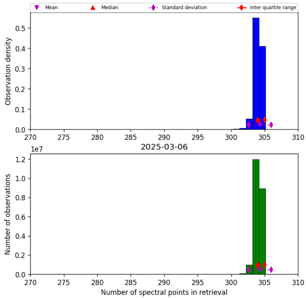
Figure 33: Histogram of “Number of spectral points in retrieval” for 2025-03-06 to 2025-03-07
