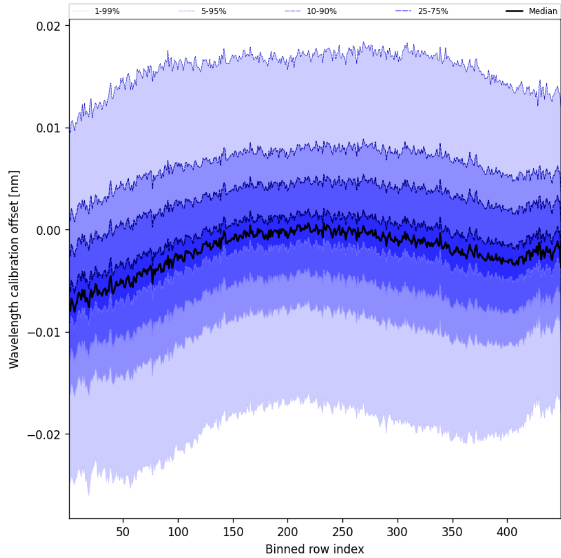
Figure 52: Along track statistics of “Wavelength calibration offset” for 2025-03-06 to 2025-03-07
