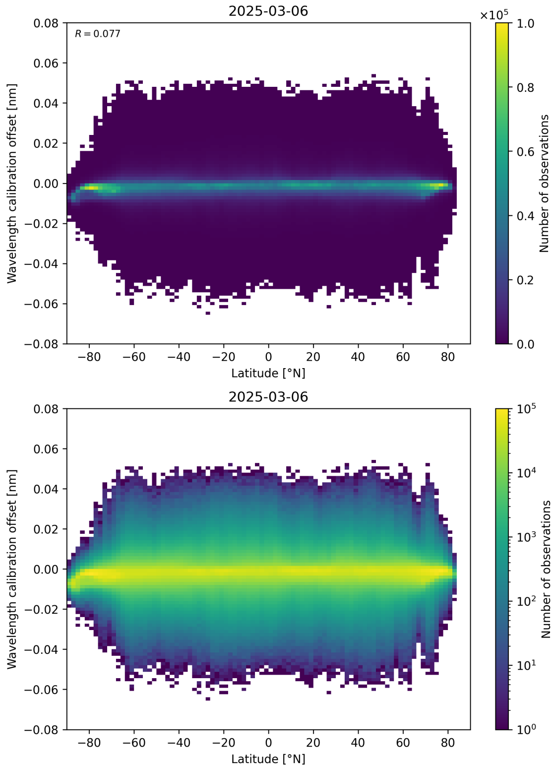
Figure 95: Scatter density plot of “Latitude” against “Wavelength calibration offset” for 2025-03-06 to 2025-03-07.
