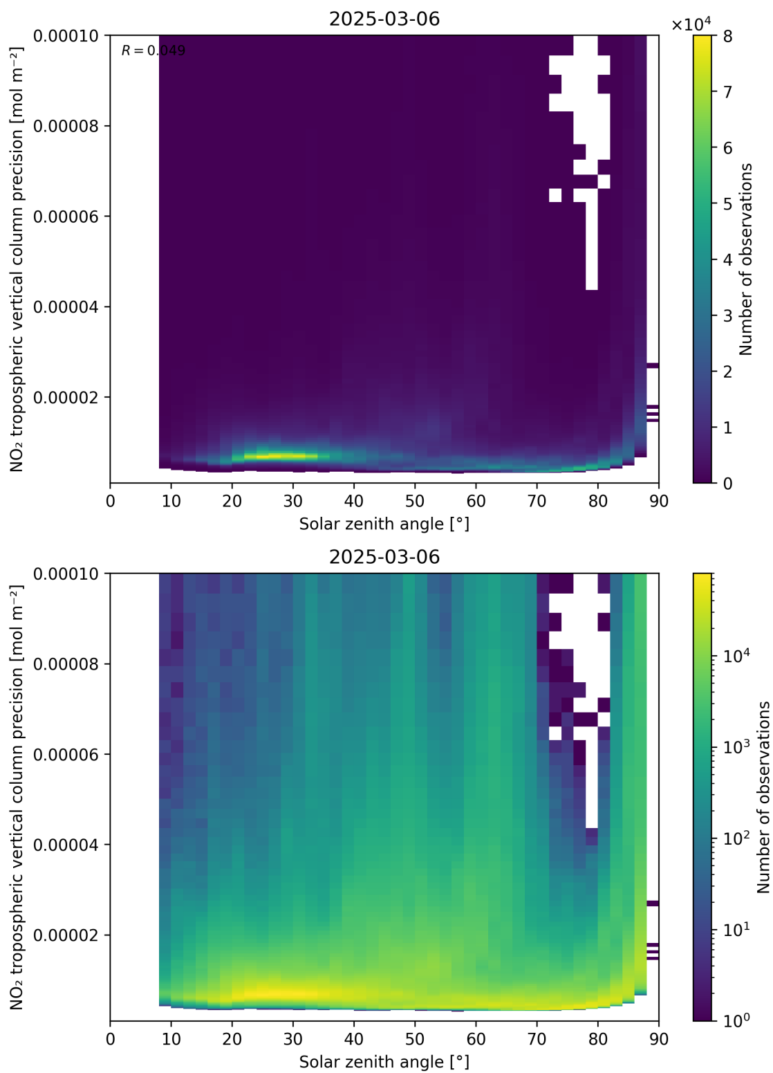
Figure 156: Scatter density plot of “Solar zenith angle” against “NO 2 tropospheric vertical column precision” for 2025-03-06 to 2025-03-07.
