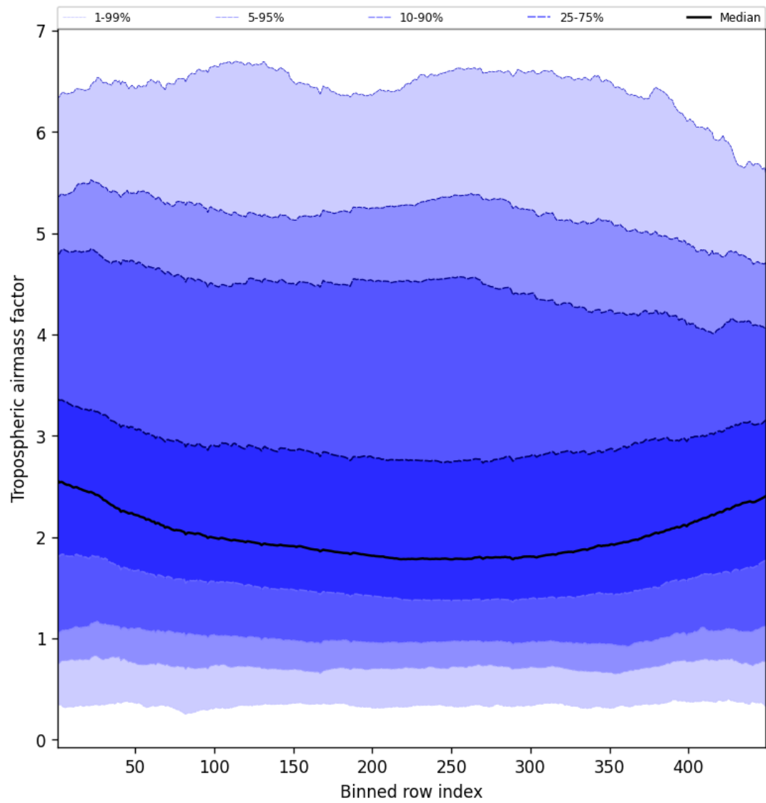
Figure 48: Along track statistics of "Tropospheric air mass factor" for 2025-03-06 to 2025-03-07
