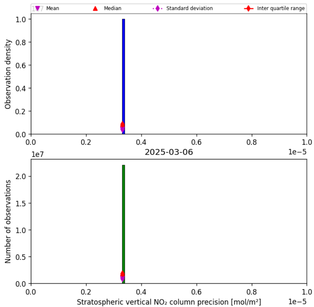
Figure 37: Histogram of “Stratospheric vertical NO 2 column precision” for 2025-03-06 to 2025-03-07
