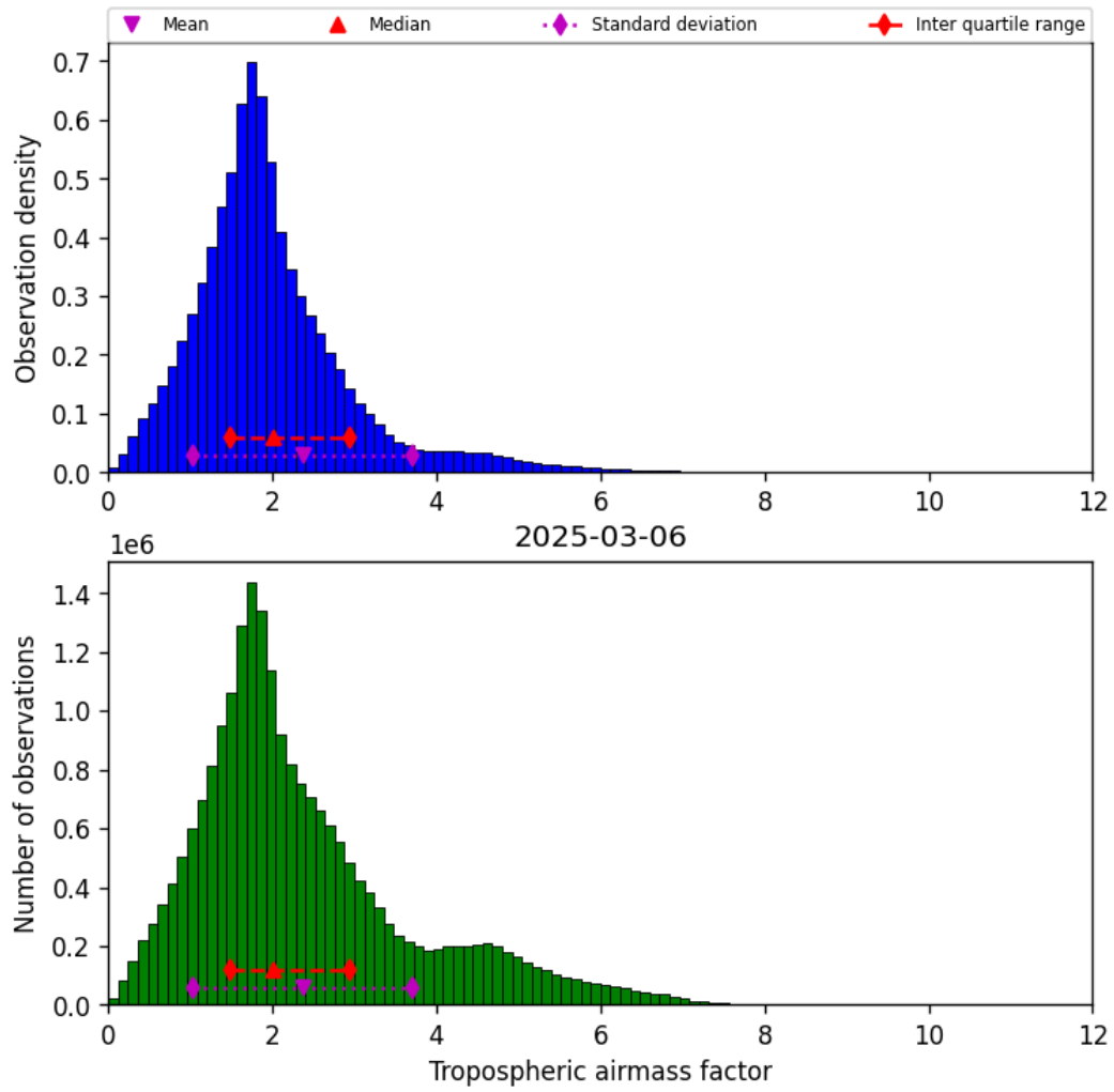
Figure 31: Histogram of “Tropospheric airmass factor” for 2025-03-06 to 2025-03-07
