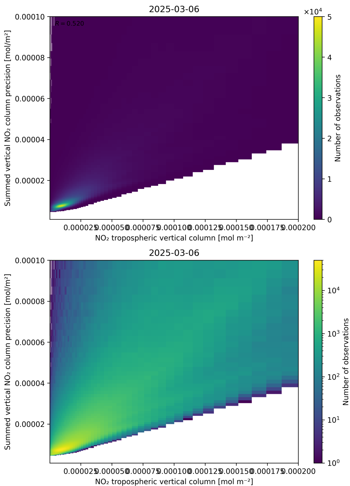
Figure 127: Scatter density plot of “NO 2 tropospheric vertical column” against “Summed vertical NO 2 column precision” for 2025-03-06 to 2025-03-07.
