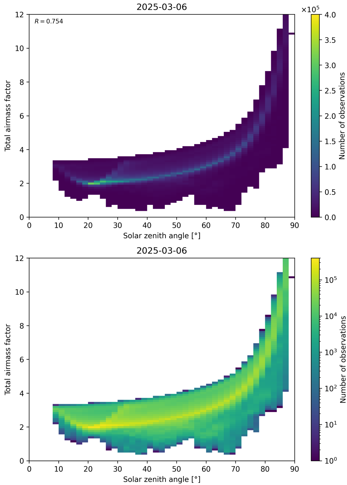
Figure 146: Scatter density plot of “Solar zenith angle” against “Total air mass factor” for 2025-03-06 to 2025-03-07.
