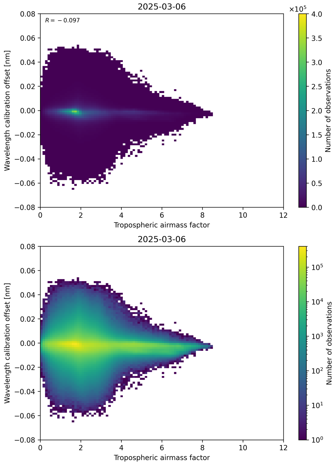
Figure 80: Scatter density plot of “Tropospheric airmass factor” against “Wavelength calibration offset” for 2025-03-06 to 2025-03-07.
