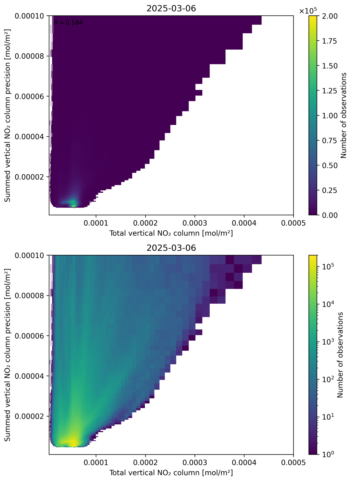
Figure 113: Scatter density plot of “Total vertical NO 2 column” against “Summed vertical NO 2 column precision” for 2025-03-06 to 2025-03-07.
