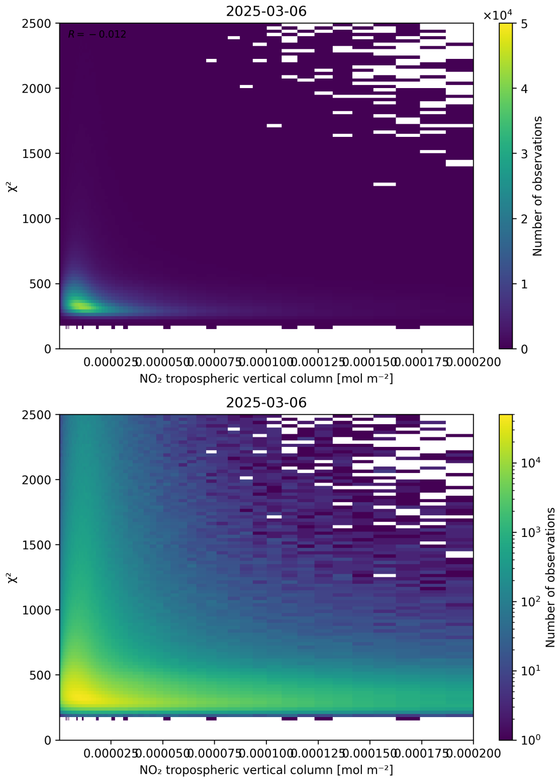
Figure 124: Scatter density plot of “NO 2 tropospheric vertical column” against “ \chi^2 ” for 2025-03-06 to 2025-03-07.
