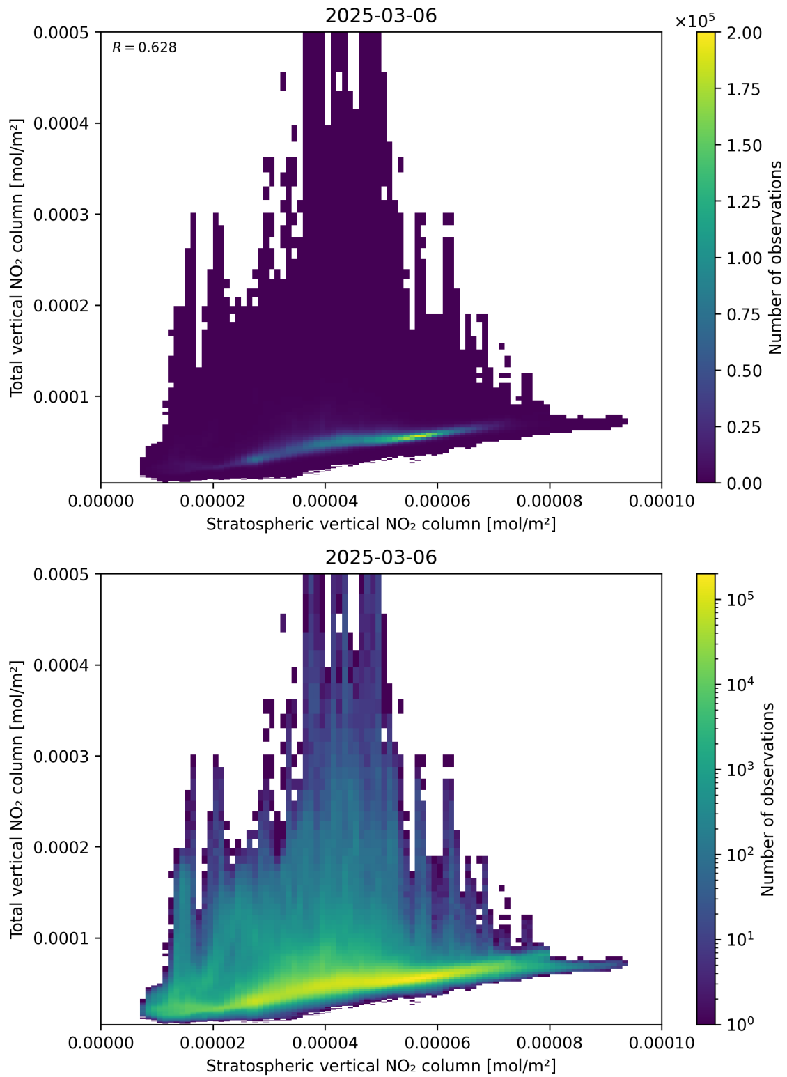
Figure 100: Scatter density plot of “Stratospheric vertical NO 2 column” against “Total vertical NO 2 column” for 2025-03-06 to 2025-03-07.
