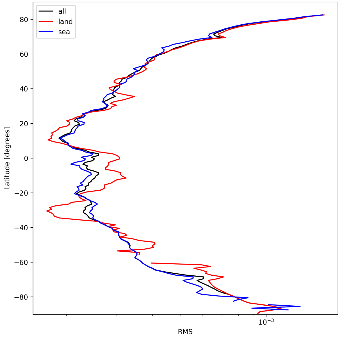
Figure 26: Zonal average of “RMS” for 2025-03-06 to 2025-03-07.
