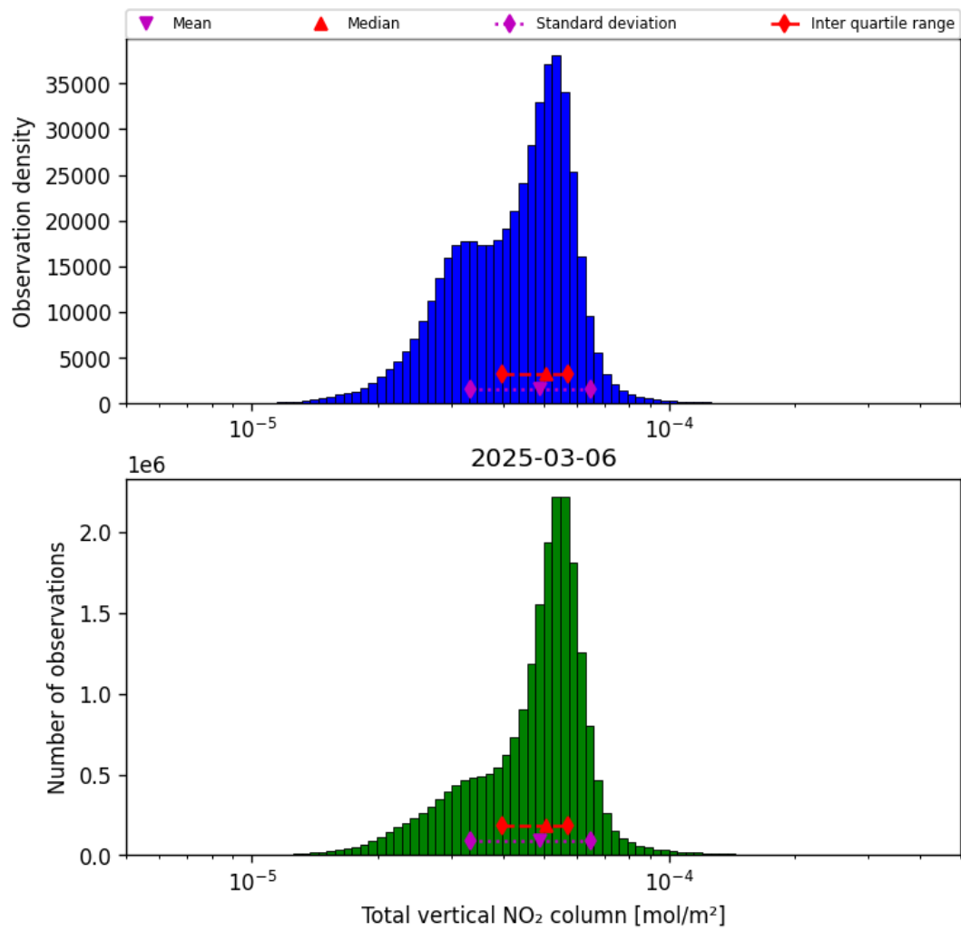
Figure 38: Histogram of “Total vertical NO 2 column” for 2025-03-06 to 2025-03-07
