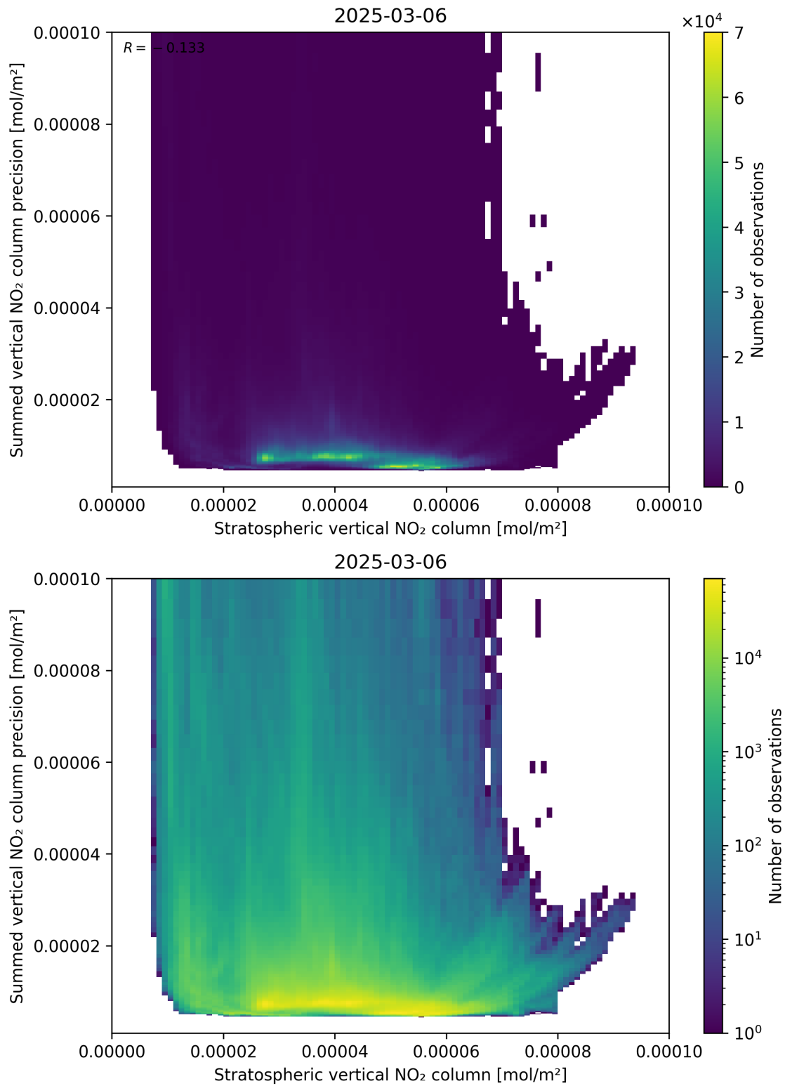
Figure 99: Scatter density plot of “Stratospheric vertical NO 2 column” against “Summed vertical NO 2 column precision” for 2025-03-06 to 2025-03-07.
