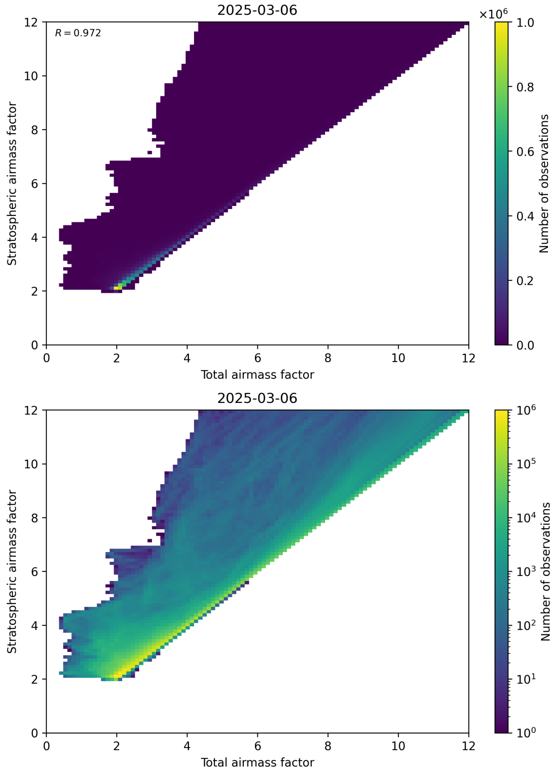
Figure 62: Scatter density plot of “Total airmass factor” against “Stratospheric airmass factor” for 2025-03-06 to 2025-03-07.
