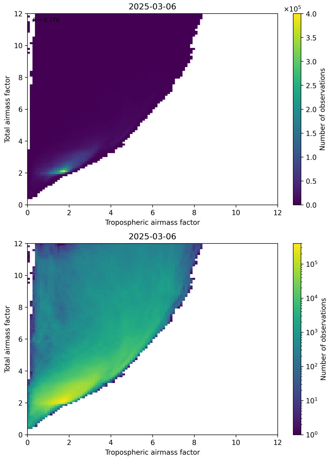
Figure 72: Scatter density plot of “Tropospheric airmass factor” against “Total airmass factor” for 2025-03-06 to 2025-03-07.
