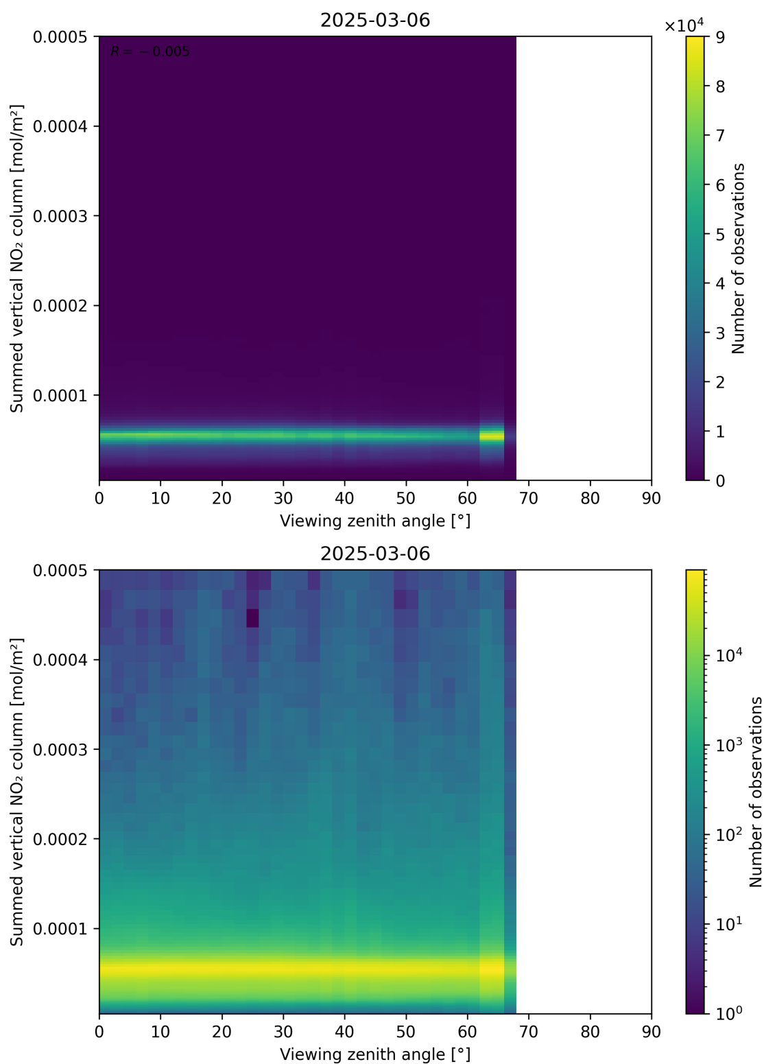
Figure 165: Scatter density plot of “Viewing zenith angle” against “Summed vertical NO 2 column” for 2025-03-06 to 2025-03-07.
