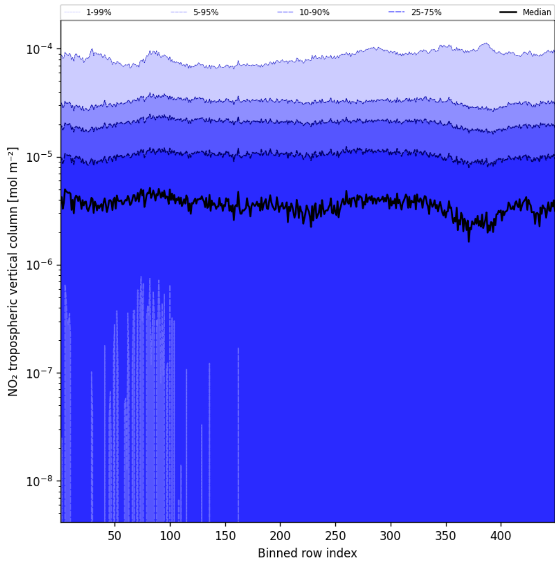
Figure 46: Along track statistics of “NO 2 tropospheric vertical column” for 2025-03-06 to 2025-03-07
