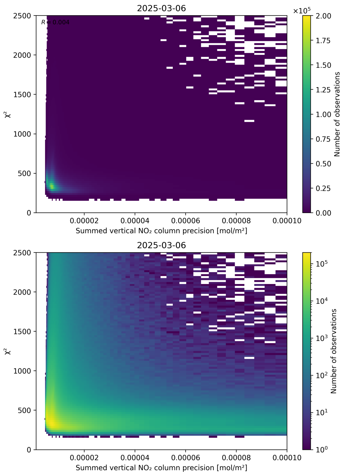
Figure 107: Scatter density plot of “Summed vertical NO 2 column precision” against “ \chi^2 ” for 2025-03-06 to 2025-03-07.
