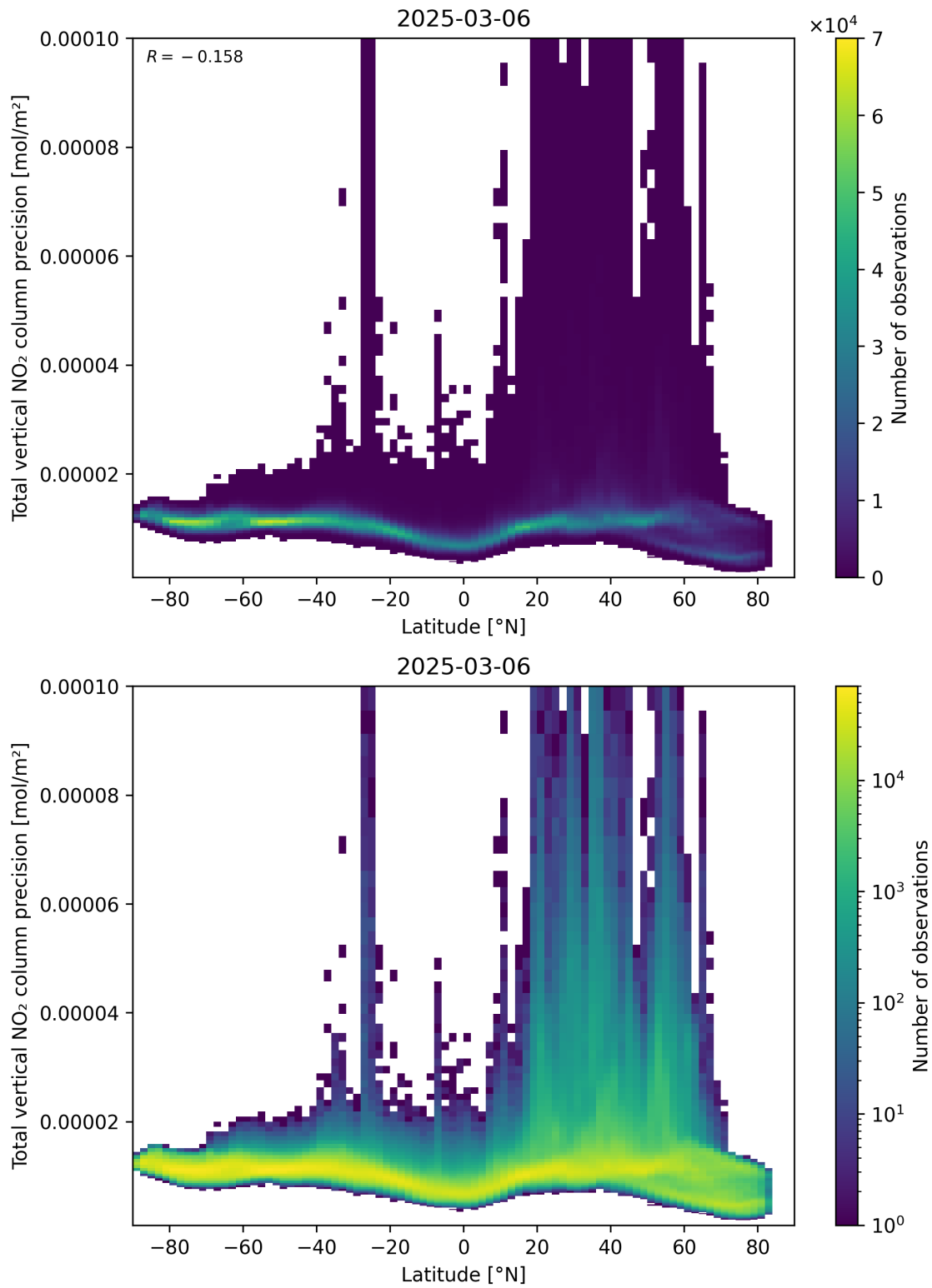
Figure 91: Scatter density plot of “Latitude” against “Total vertical NO 2 column precision” for 2025-03-06 to 2025-03-07.
