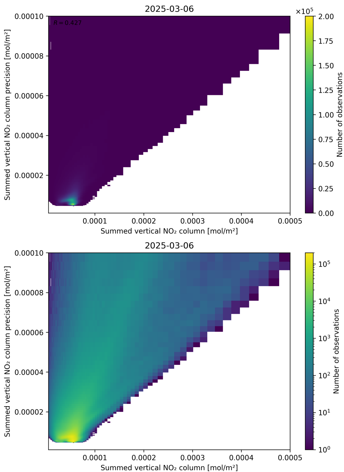
Figure 105: Scatter density plot of “Summed vertical NO 2 column” against “Summed vertical NO 2 column precision” for 2025-03-06 to 2025-03-07.
