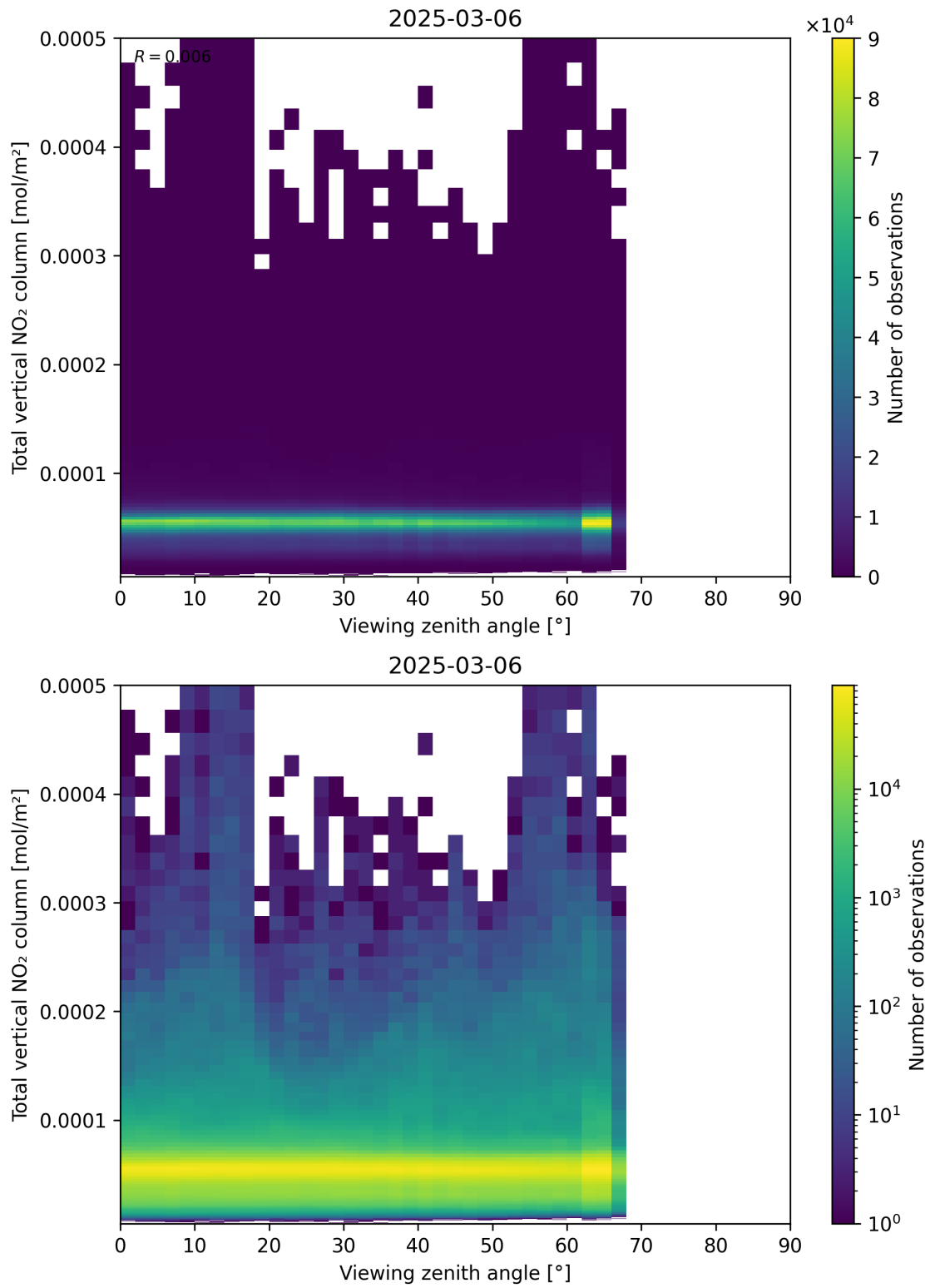
Figure 167: Scatter density plot of “Viewing zenith angle” against “Total vertical NO 2 column” for 2025-03-06 to 2025-03-07.
