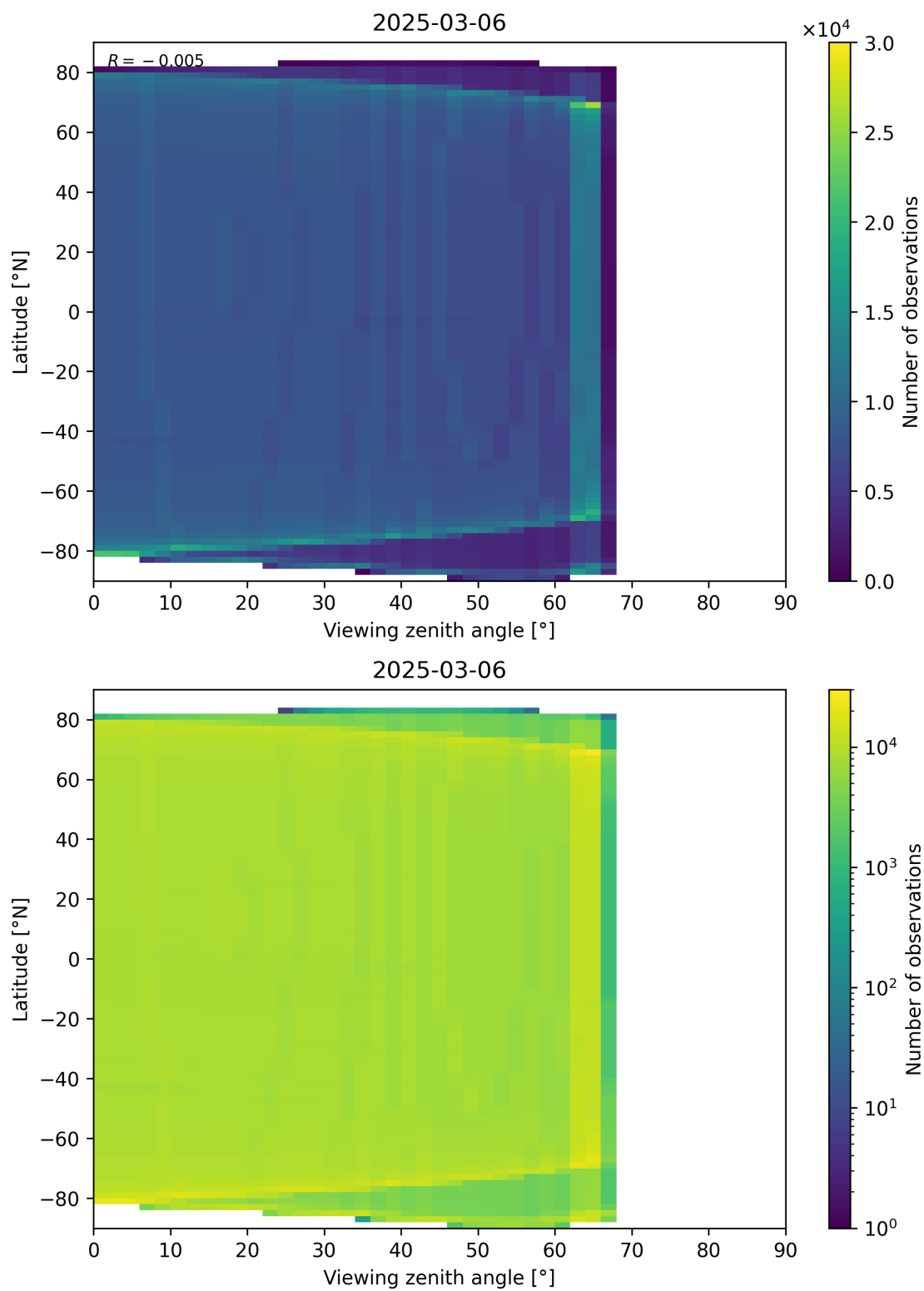
Figure 163: Scatter density plot of “Viewing zenith angle” against “Latitude” for 2025-03-06 to 2025-03-07.
