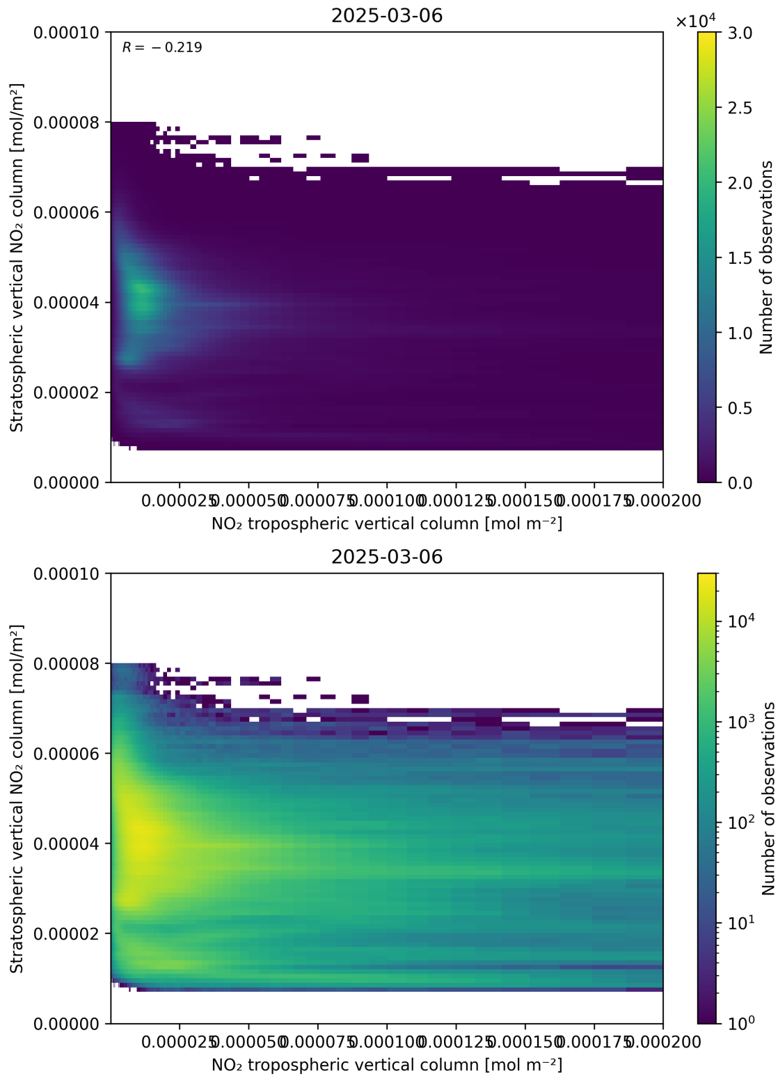
Figure 125: Scatter density plot of “NO 2 tropospheric vertical column” against “Stratospheric vertical NO 2 column” for 2025-03-06 to 2025-03-07.
