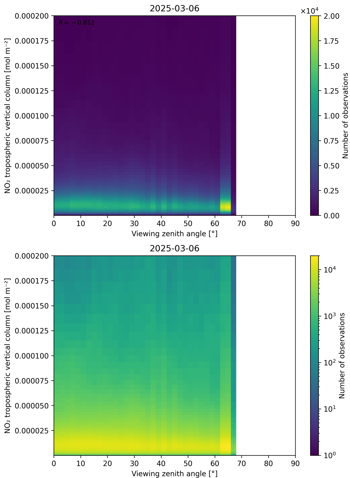
Figure 169: Scatter density plot of “Viewing zenith angle” against “NO 2 tropospheric vertical column” for 2025-03-06 to 2025-03-07.
