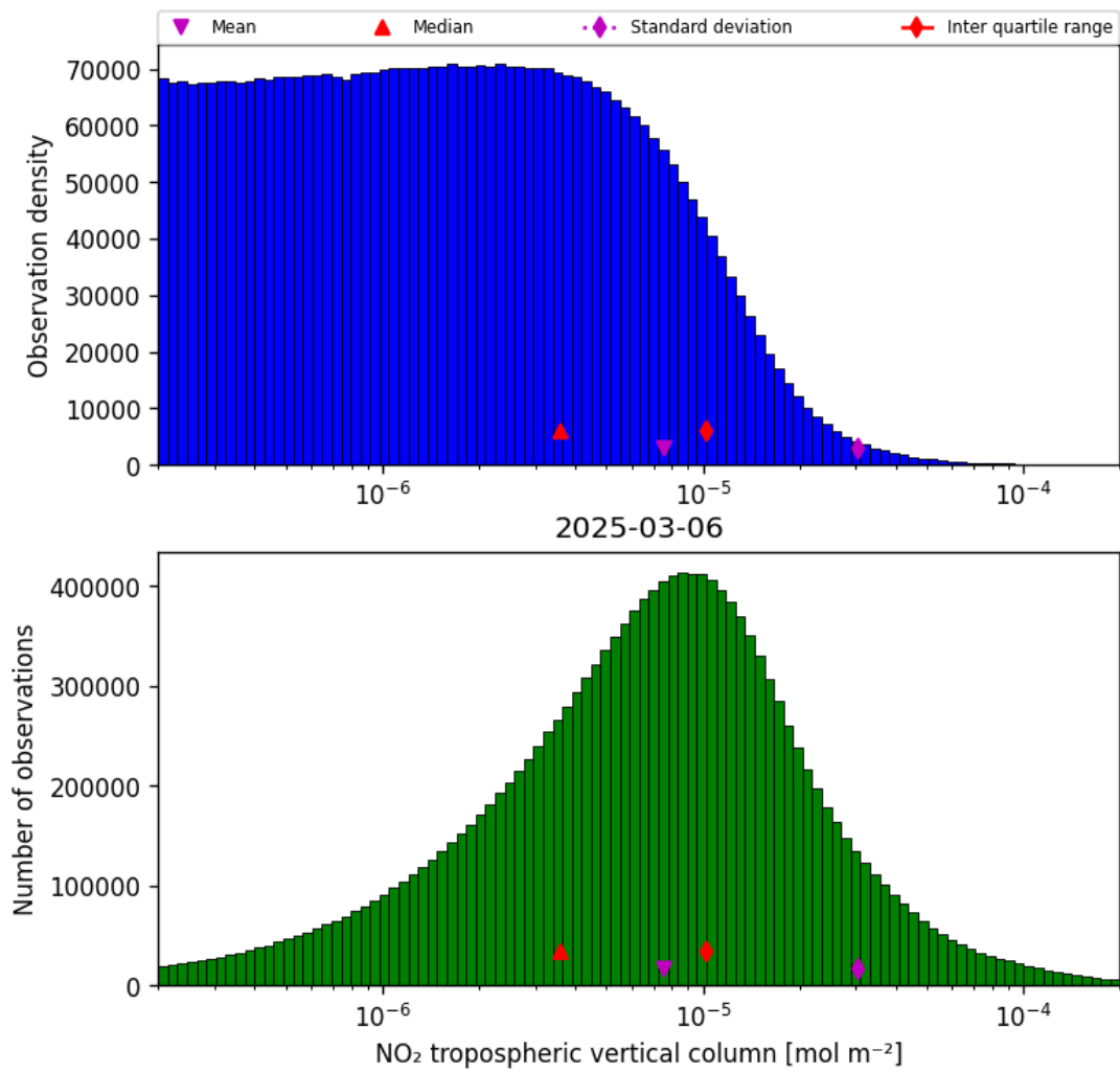
Figure 29: Histogram of “NO 2 tropospheric vertical column” for 2025-03-06 to 2025-03-07
