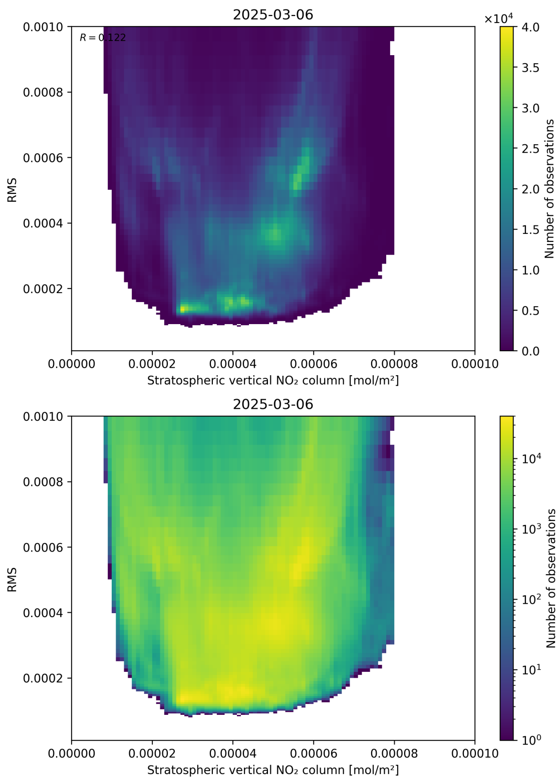
Figure 102: Scatter density plot of “Stratospheric vertical NO 2 column” against “RMS” for 2025-03-06 to 2025-03-07.
