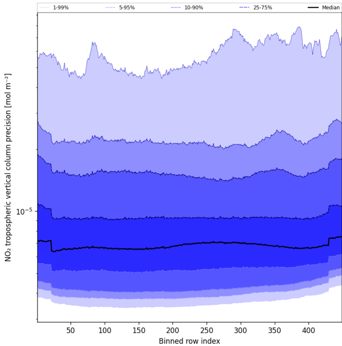
Figure 47: Along track statistics of “NO 2 tropospheric vertical column precision” for 2025-03-06 to 2025-03-07
