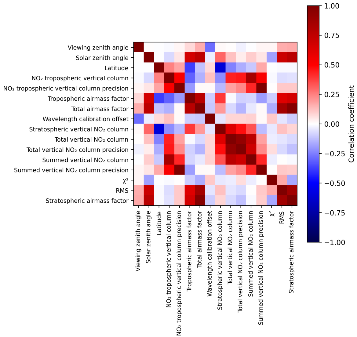
Figure 2: Map of correlation matrix for 2025-03-06 to 2025-03-07.
