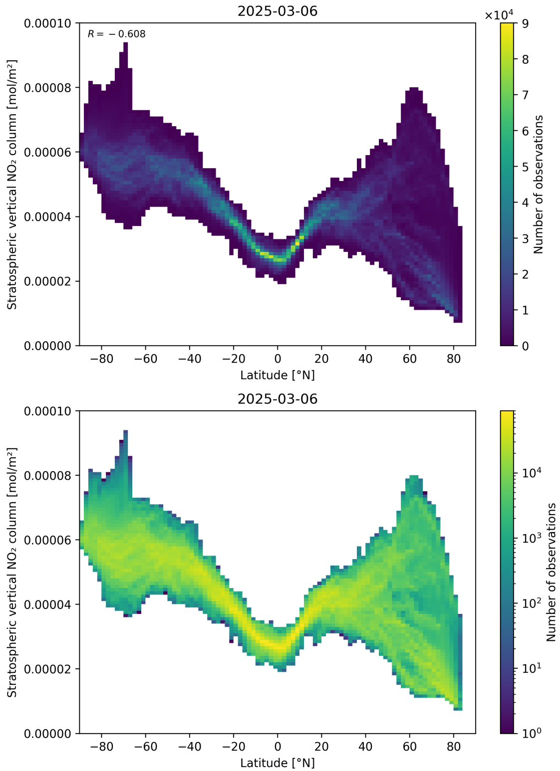
Figure 87: Scatter density plot of “Latitude” against “Stratospheric vertical NO 2 column” for 2025-03-06 to 2025-03-07.
