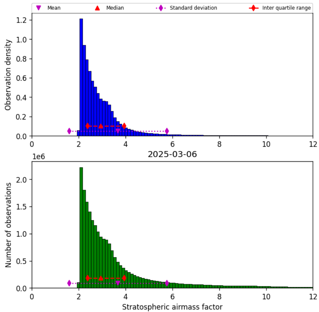
Figure 44: Histogram of “Stratospheric airmass factor” for 2025-03-06 to 2025-03-07
