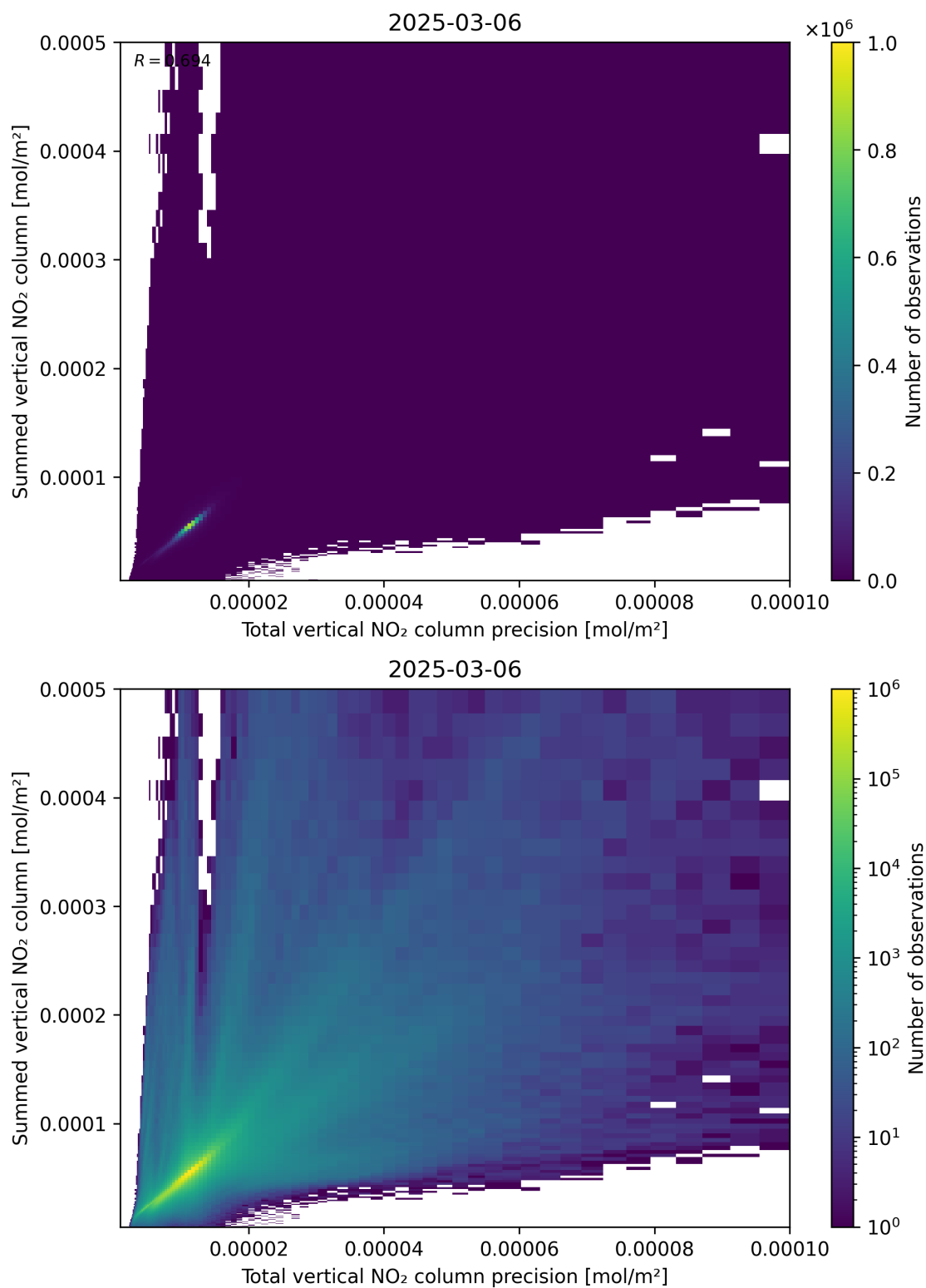
Figure 117: Scatter density plot of “Total vertical NO 2 column precision” against “Summed vertical NO 2 column” for 2025-03-06 to 2025-03-07.
