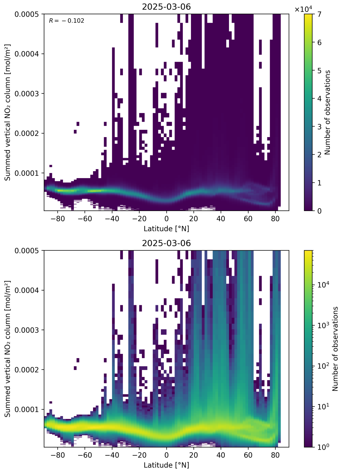
Figure 88: Scatter density plot of “Latitude” against “Summed vertical NO 2 column” for 2025-03-06 to 2025-03-07.
