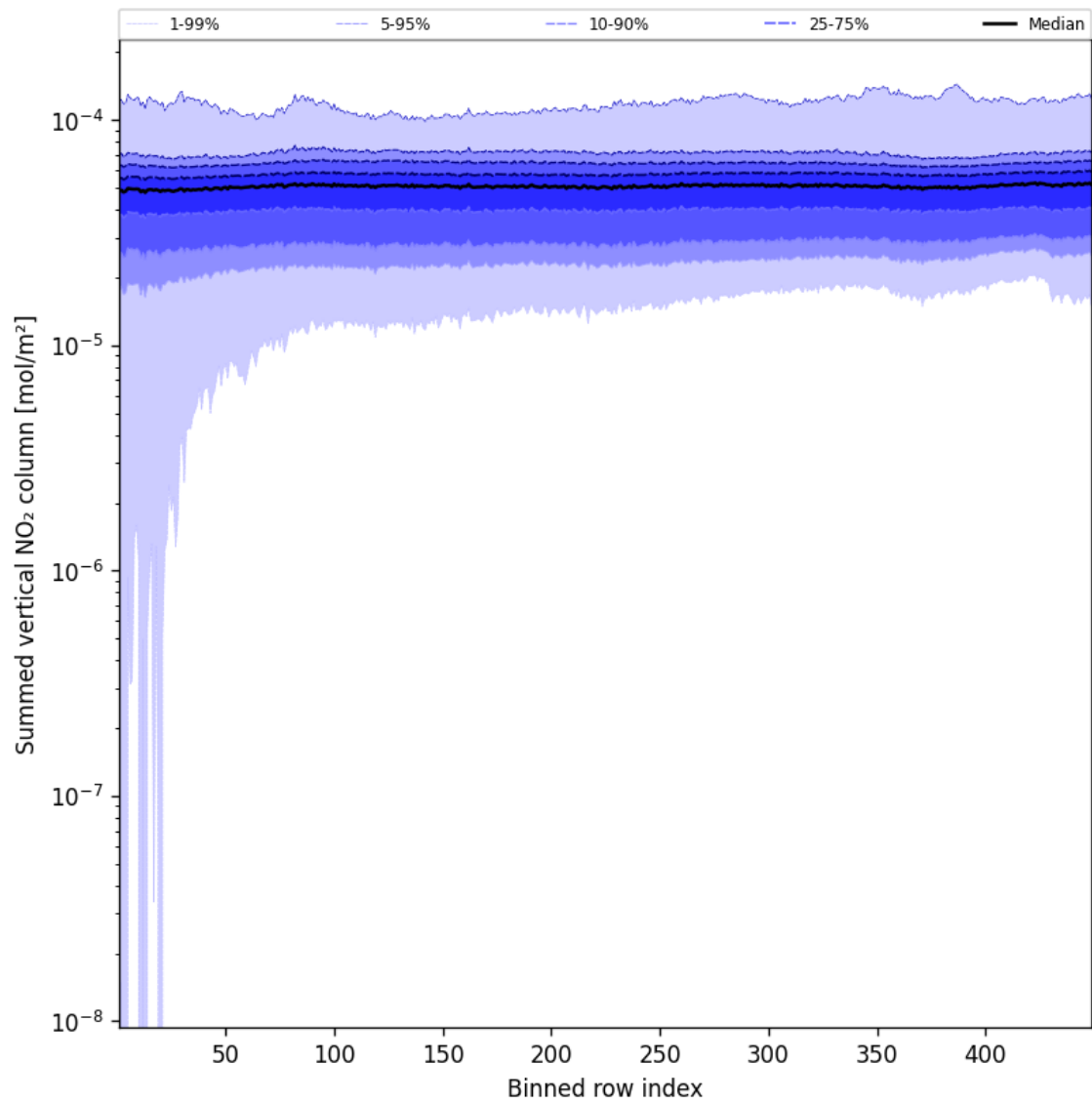
Figure 57: Along track statistics of “Summed vertical NO 2 column” for 2025-03-06 to 2025-03-07
