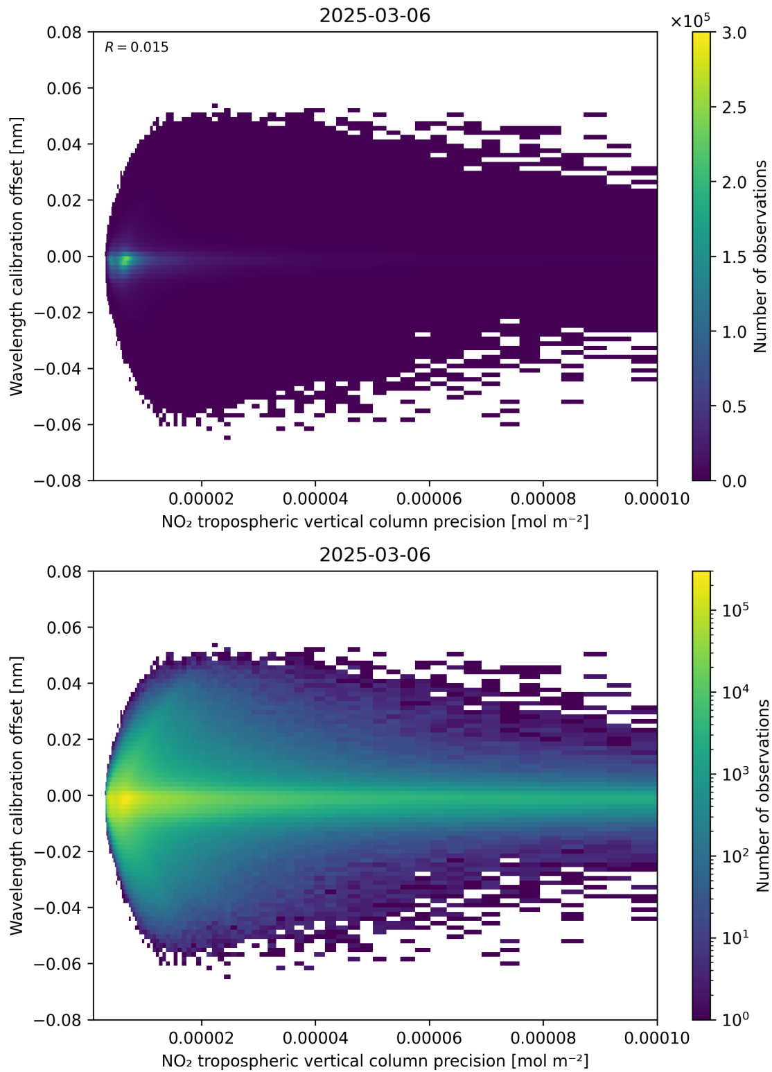
Figure 141: Scatter density plot of “NO 2 tropospheric vertical column precision” against “Wavelength calibration offset” for 2025-03-06 to 2025-03-07.
