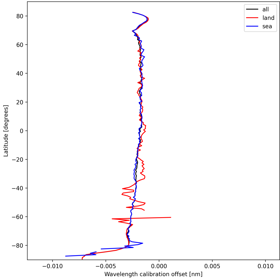
Figure 18: Zonal average of “Wavelength calibration offset” for 2025-03-06 to 2025-03-07.
