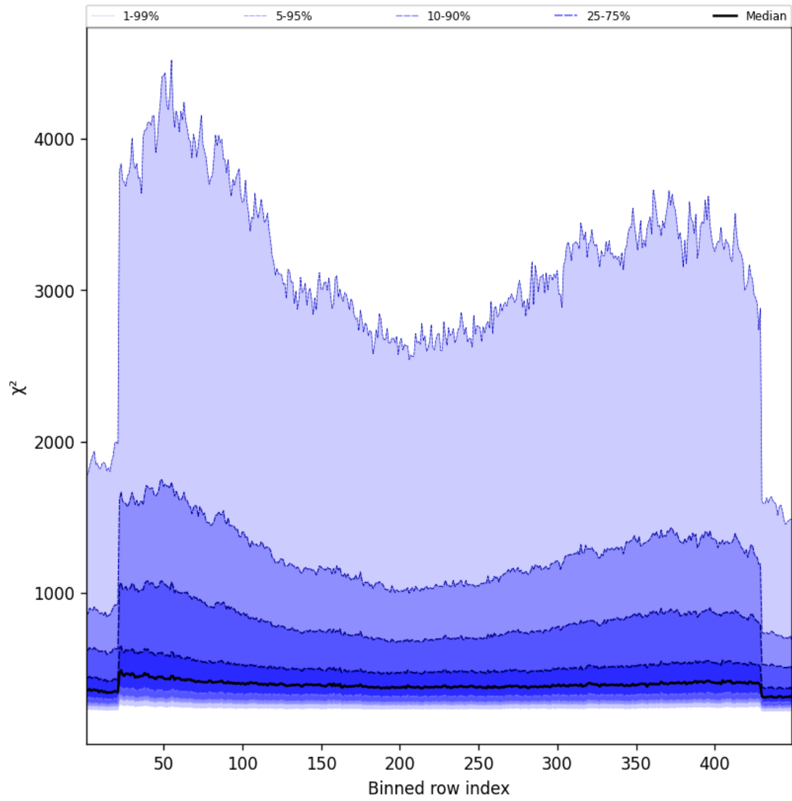
Figure 59: Along track statistics of “ \chi^2 ” for 2025-03-06 to 2025-03-07
