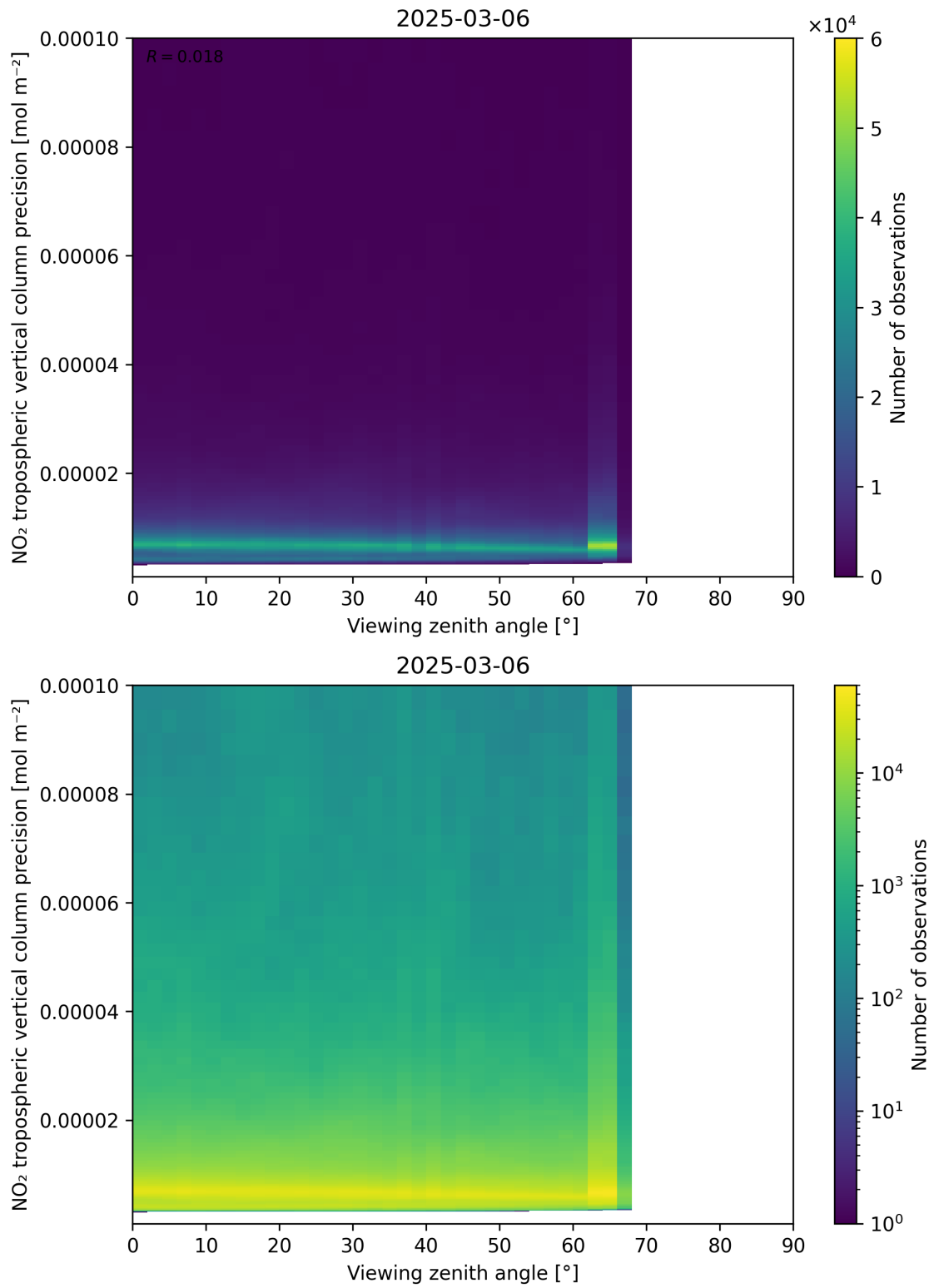
Figure 170: Scatter density plot of “Viewing zenith angle” against “NO 2 tropospheric vertical column precision” for 2025-03-06 to 2025-03-07.
