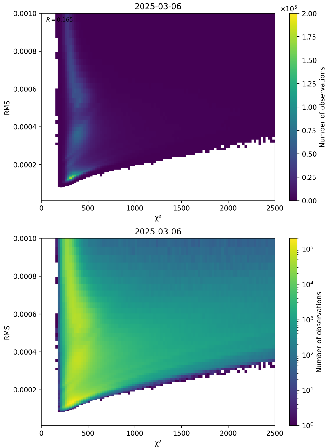
Figure 82: Scatter density plot of “ \chi^2 ” against “RMS” for 2025-03-06 to 2025-03-07.
