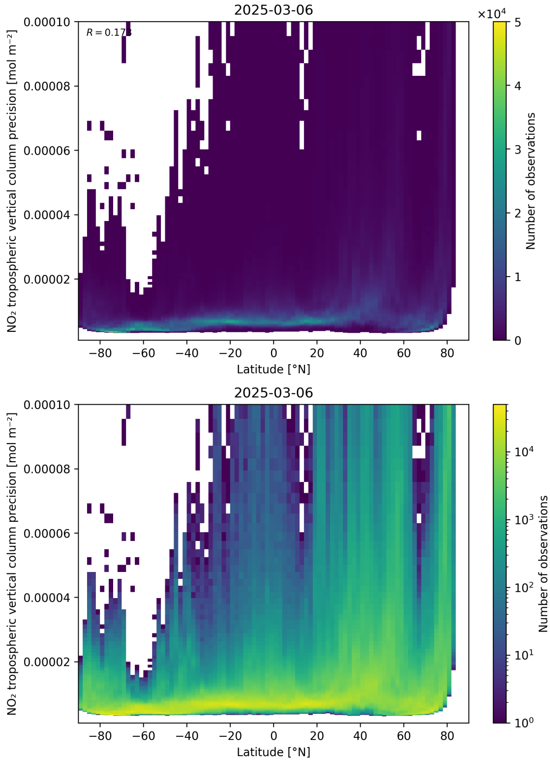
Figure 93: Scatter density plot of “Latitude” against “NO 2 tropospheric vertical column precision” for 2025-03-06 to 2025-03-07.
