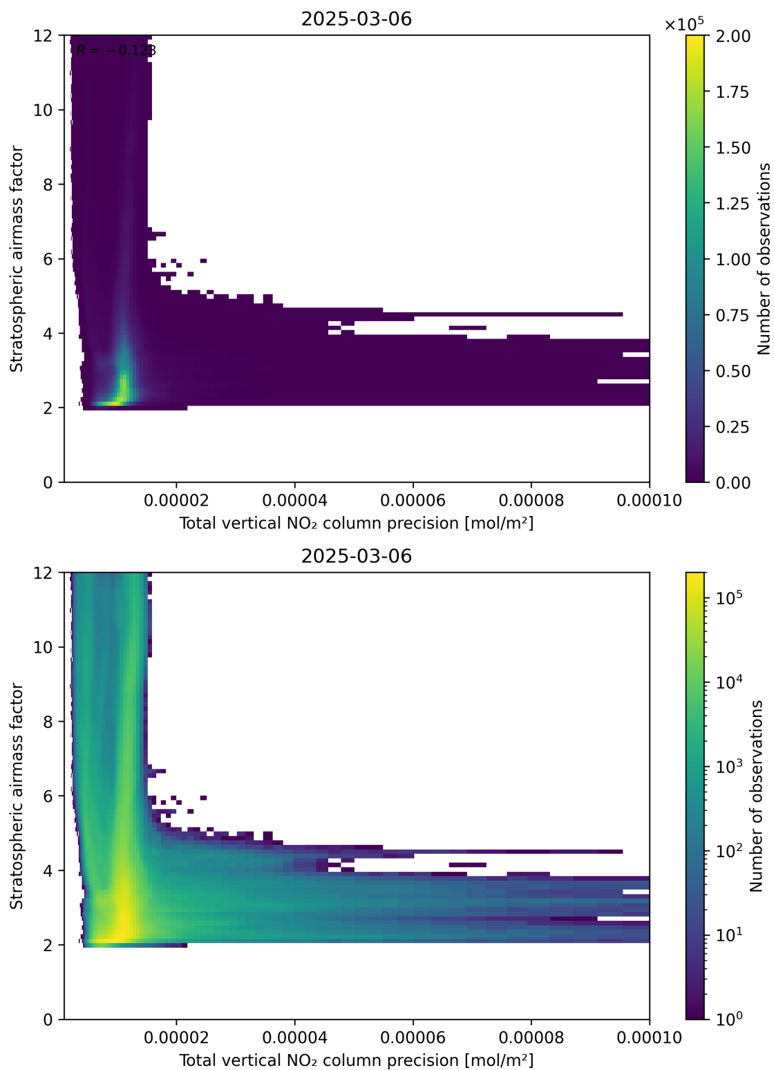
Figure 115: Scatter density plot of “Total vertical NO 2 column precision” against “Stratospheric air mass factor” for 2025-03-06 to 2025-03-07.
