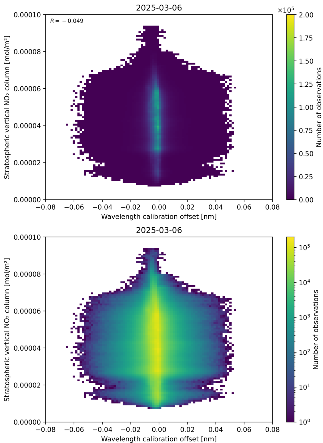
Figure 176: Scatter density plot of “Wavelength calibration offset” against “Stratospheric vertical NO 2 column” for 2025-03-06 to 2025-03-07.
