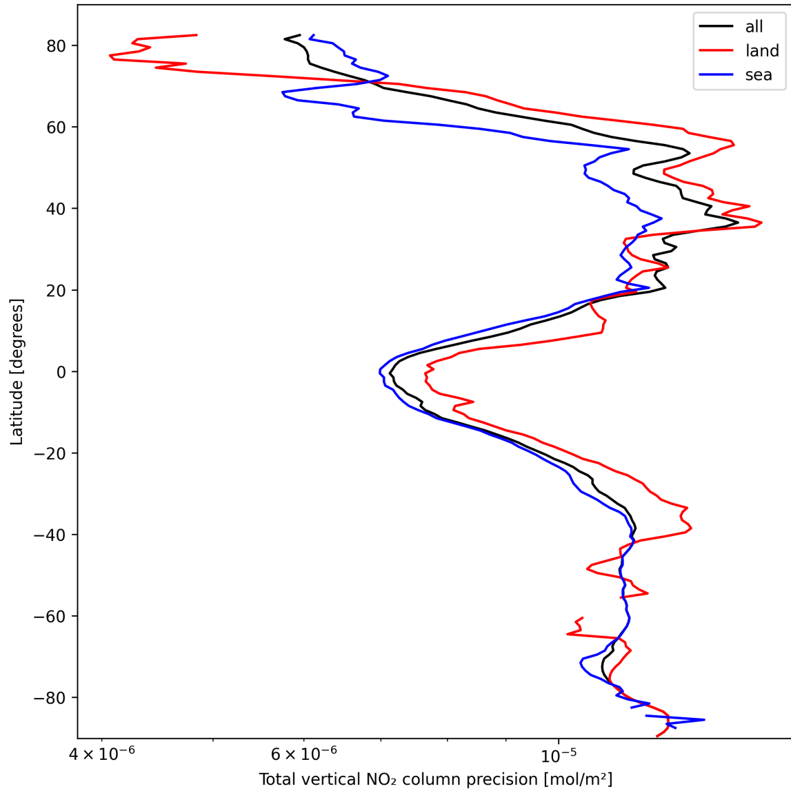
Figure 22: Zonal average of “Total vertical NO 2 column precision” for 2025-03-06 to 2025-03-07.
