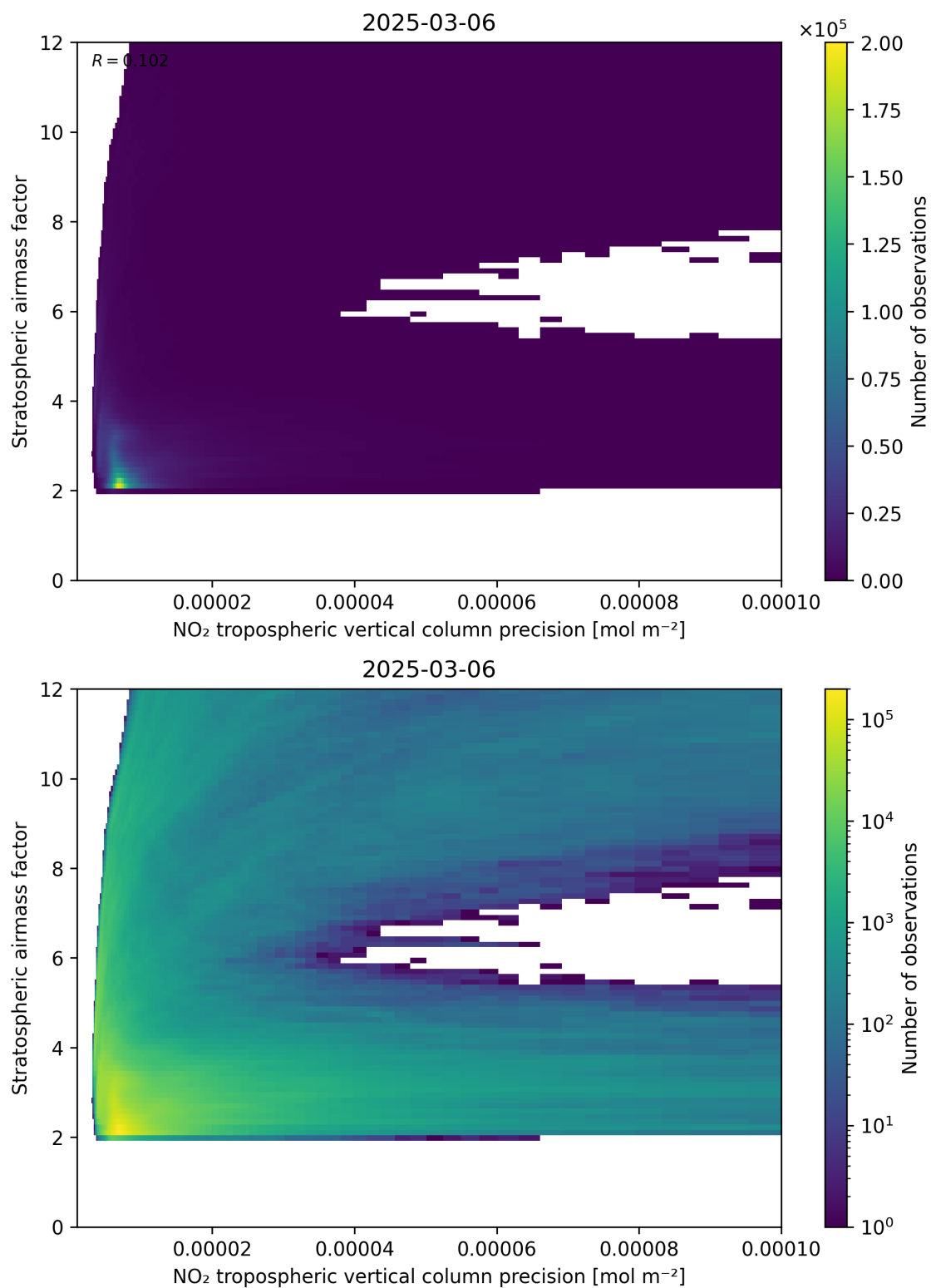
Figure 131: Scatter density plot of “NO 2 tropospheric vertical column precision” against “Stratospheric airmass factor” for 2025-03-06 to 2025-03-07.
