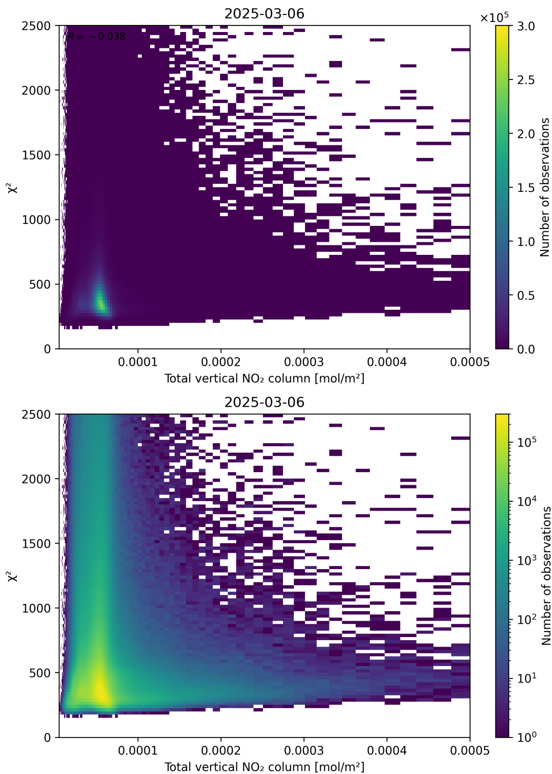
Figure 111: Scatter density plot of “Total vertical NO 2 column” against “ \chi^2 ” for 2025-03-06 to 2025-03-07.
