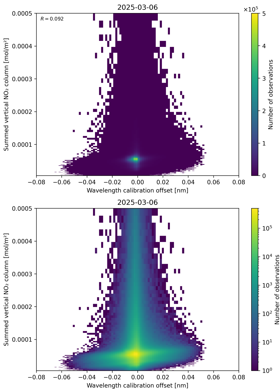
Figure 177: Scatter density plot of “Wavelength calibration offset” against “Summed vertical NO 2 column” for 2025-03-06 to 2025-03-07.
