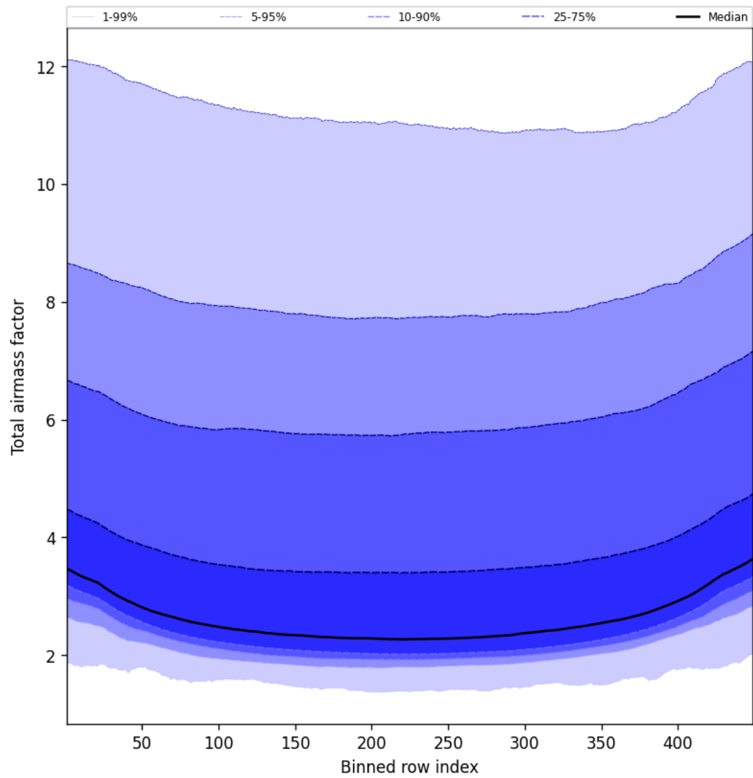
Figure 49: Along track statistics of “Total airmass factor” for 2025-03-06 to 2025-03-07
