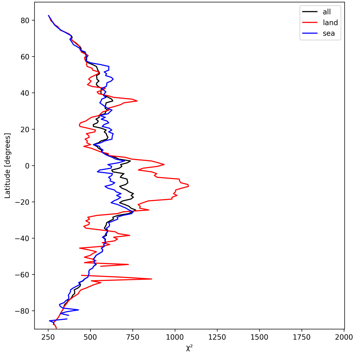
Figure 25: Zonal average of “ \chi^2 ” for 2025-03-06 to 2025-03-07.
