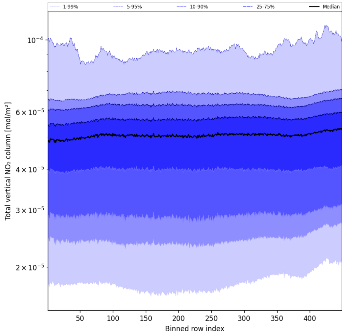
Figure 55: Along track statistics of “Total vertical NO 2 column” for 2025-03-06 to 2025-03-07
