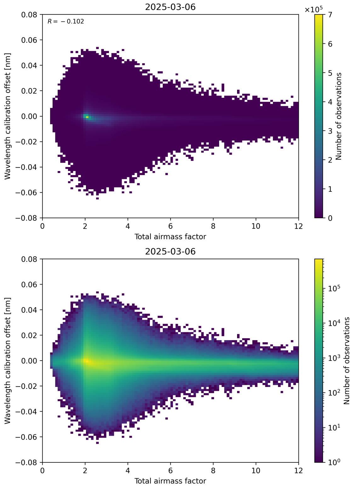
Figure 70: Scatter density plot of “Total airmass factor” against “Wavelength calibration offset” for 2025-03-06 to 2025-03-07.
