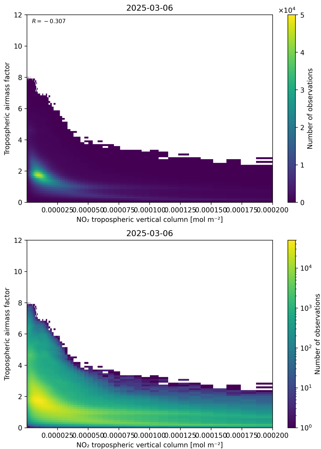
Figure 123: Scatter density plot of “NO 2 tropospheric vertical column” against “Tropospheric air mass factor” for 2025-03-06 to 2025-03-07.
