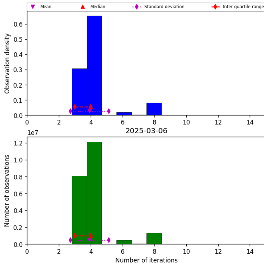
Figure 34: Histogram of “Number of iterations” for 2025-03-06 to 2025-03-07
