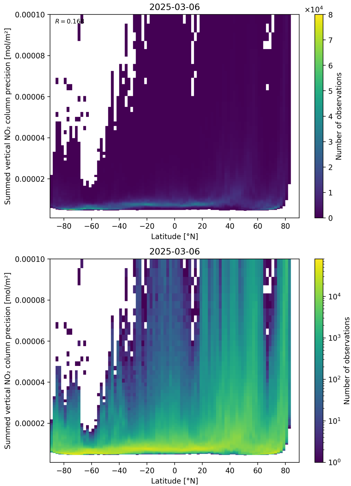
Figure 89: Scatter density plot of “Latitude” against “Summed vertical NO 2 column precision” for 2025-03-06 to 2025-03-07.
