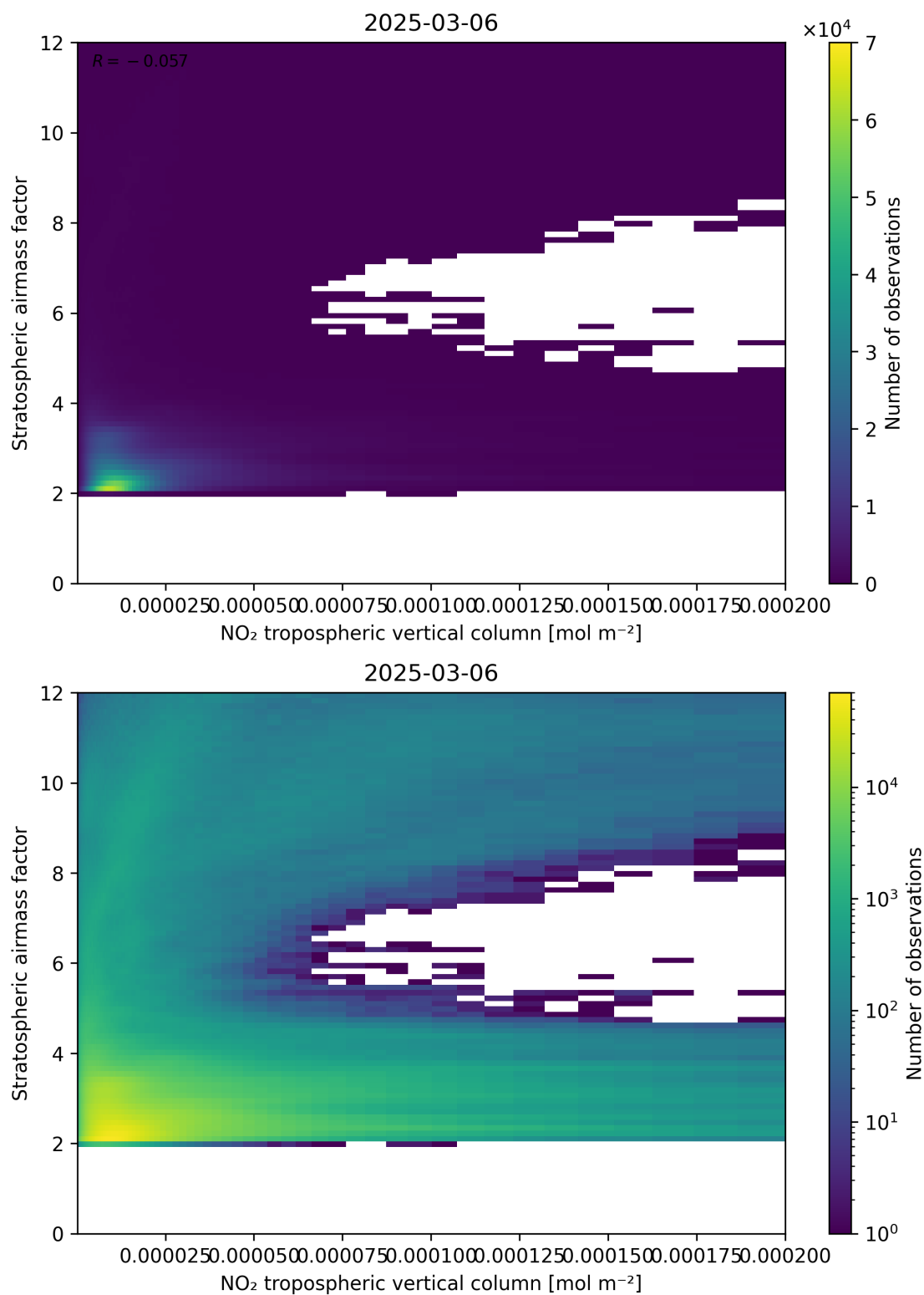
Figure 121: Scatter density plot of “NO 2 tropospheric vertical column” against “Stratospheric air mass factor” for 2025-03-06 to 2025-03-07.
