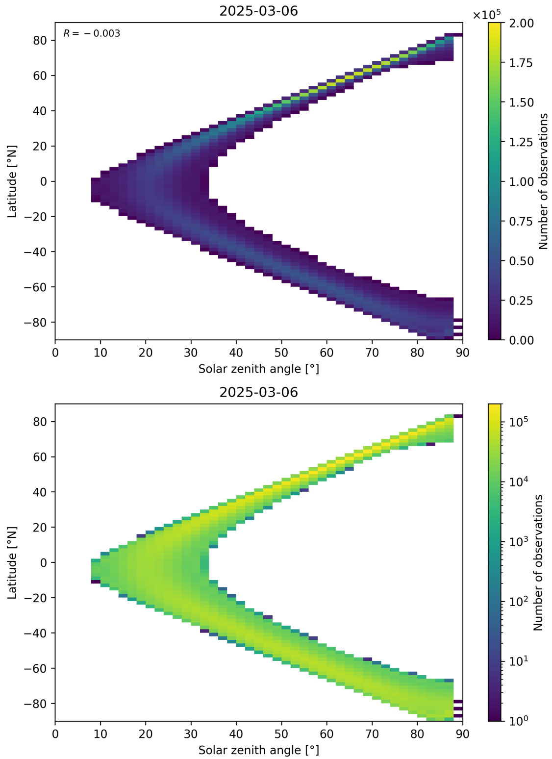
Figure 149: Scatter density plot of “Solar zenith angle” against “Latitude” for 2025-03-06 to 2025-03-07.
