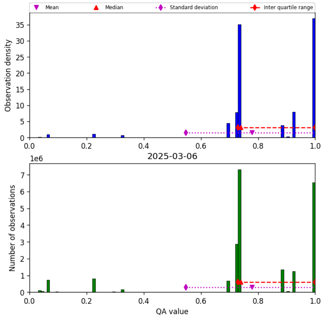
Figure 28: Histogram of “QA value” for 2025-03-06 to 2025-03-07
