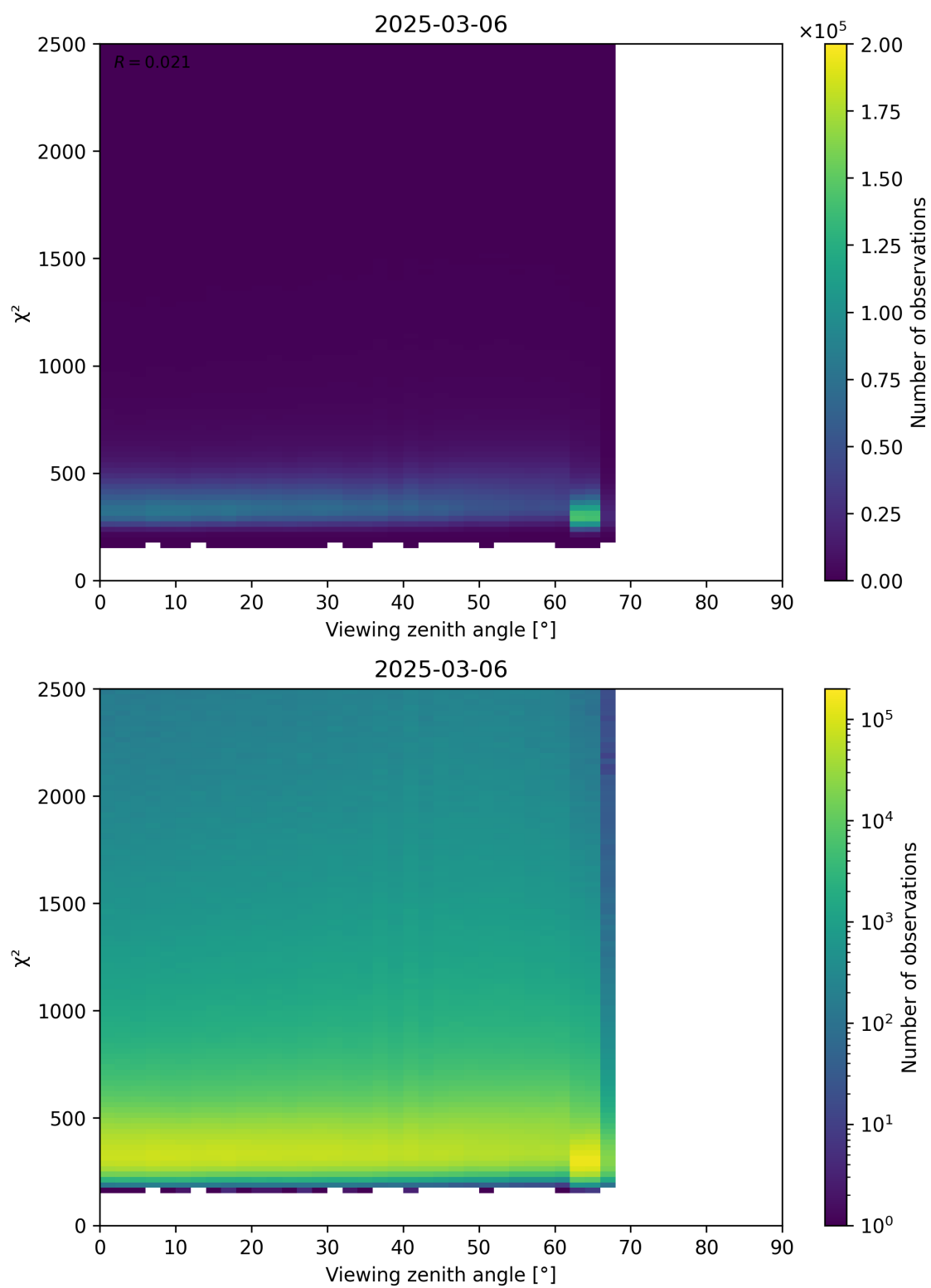
Figure 162: Scatter density plot of “Viewing zenith angle” against “ \chi^2 ” for 2025-03-06 to 2025-03-07.
