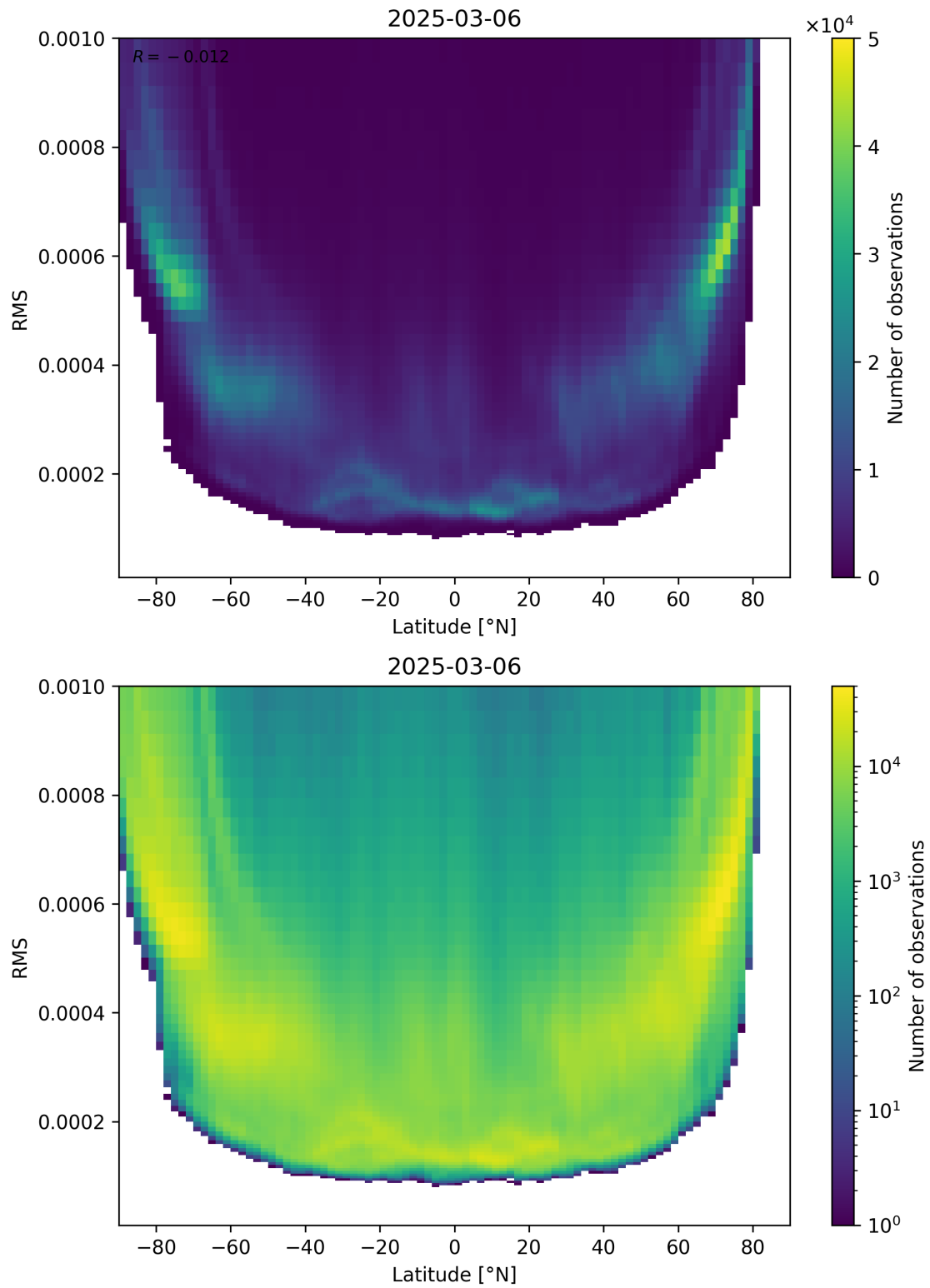
Figure 94: Scatter density plot of “Latitude” against “RMS” for 2025-03-06 to 2025-03-07.
