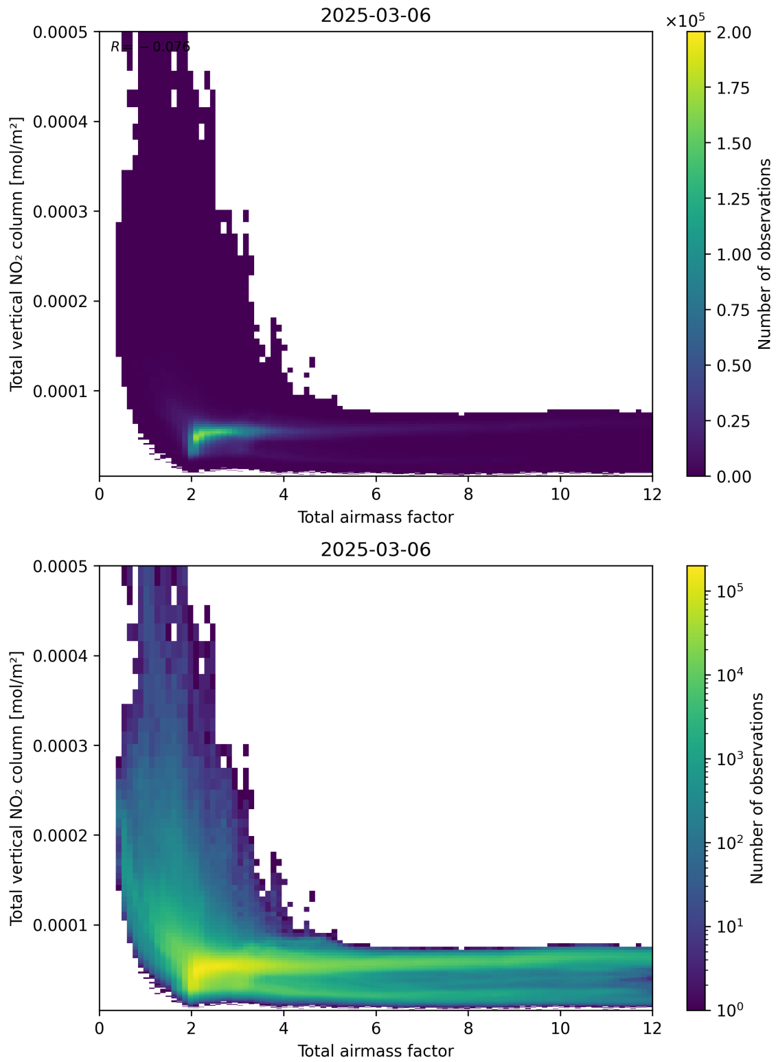
Figure 67: Scatter density plot of “Total airmass factor” against “Total vertical NO 2 column” for 2025-03-06 to 2025-03-07.
