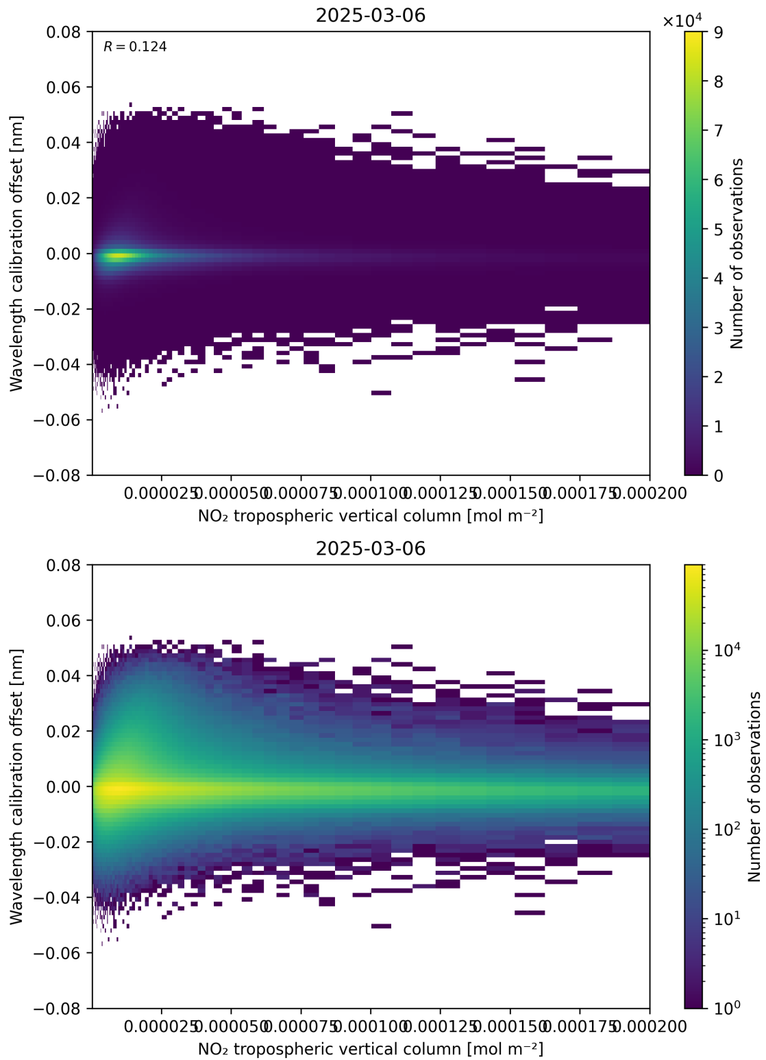
Figure 143: Scatter density plot of “NO 2 tropospheric vertical column” against “Wavelength calibration offset” for 2025-03-06 to 2025-03-07.
