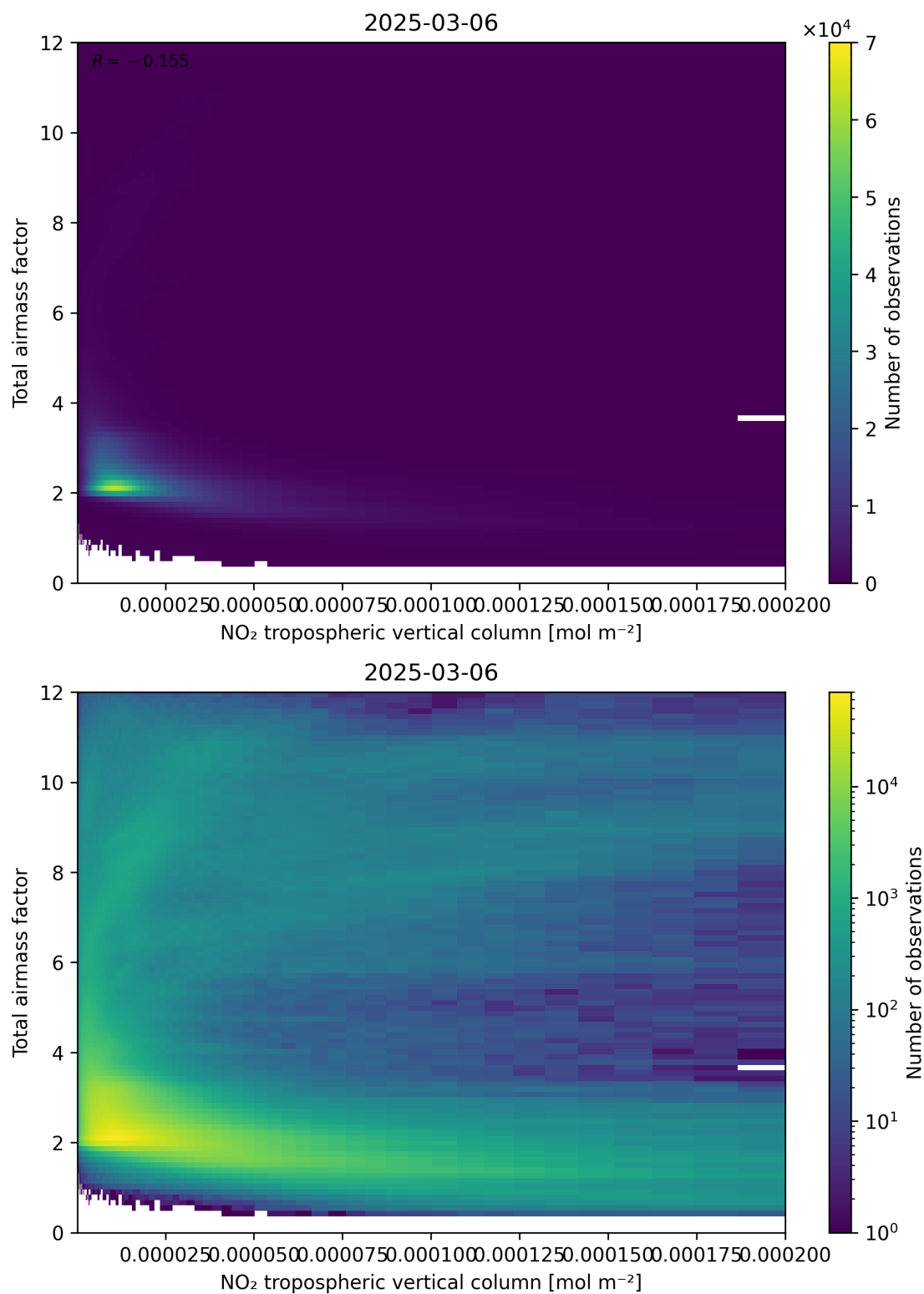
Figure 122: Scatter density plot of “NO 2 tropospheric vertical column” against “Total air mass factor” for 2025-03-06 to 2025-03-07.
