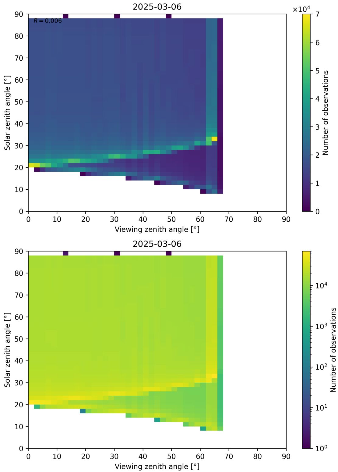
Figure 172: Scatter density plot of “Viewing zenith angle” against “Solar zenith angle” for 2025-03-06 to 2025-03-07.
