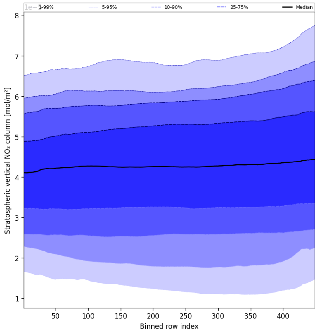
Figure 53: Along track statistics of “Stratospheric vertical NO 2 column” for 2025-03-06 to 2025-03-07
