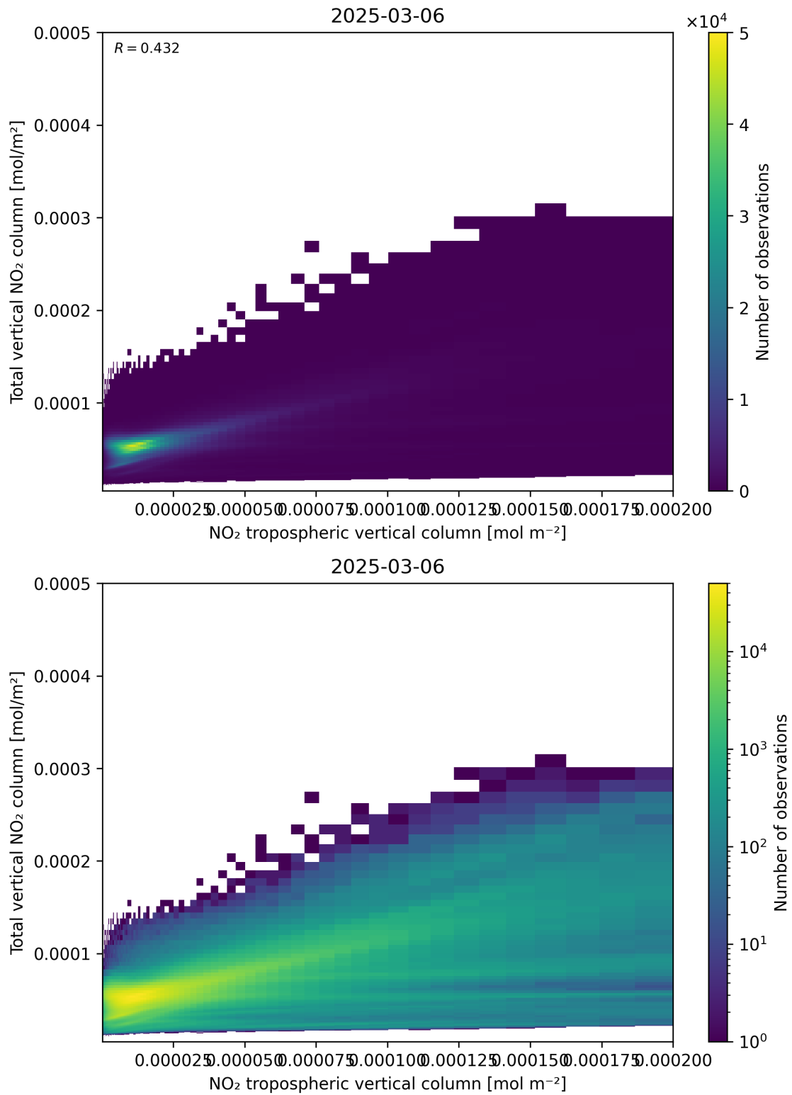
Figure 128: Scatter density plot of “NO 2 tropospheric vertical column” against “Total vertical NO 2 column” for 2025-03-06 to 2025-03-07.
