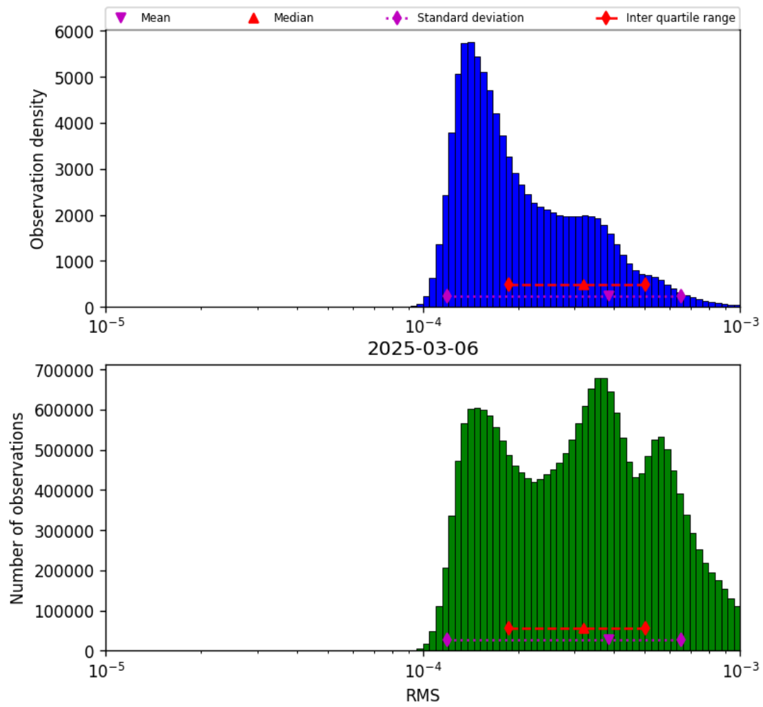
Figure 43: Histogram of “RMS” for 2025-03-06 to 2025-03-07
