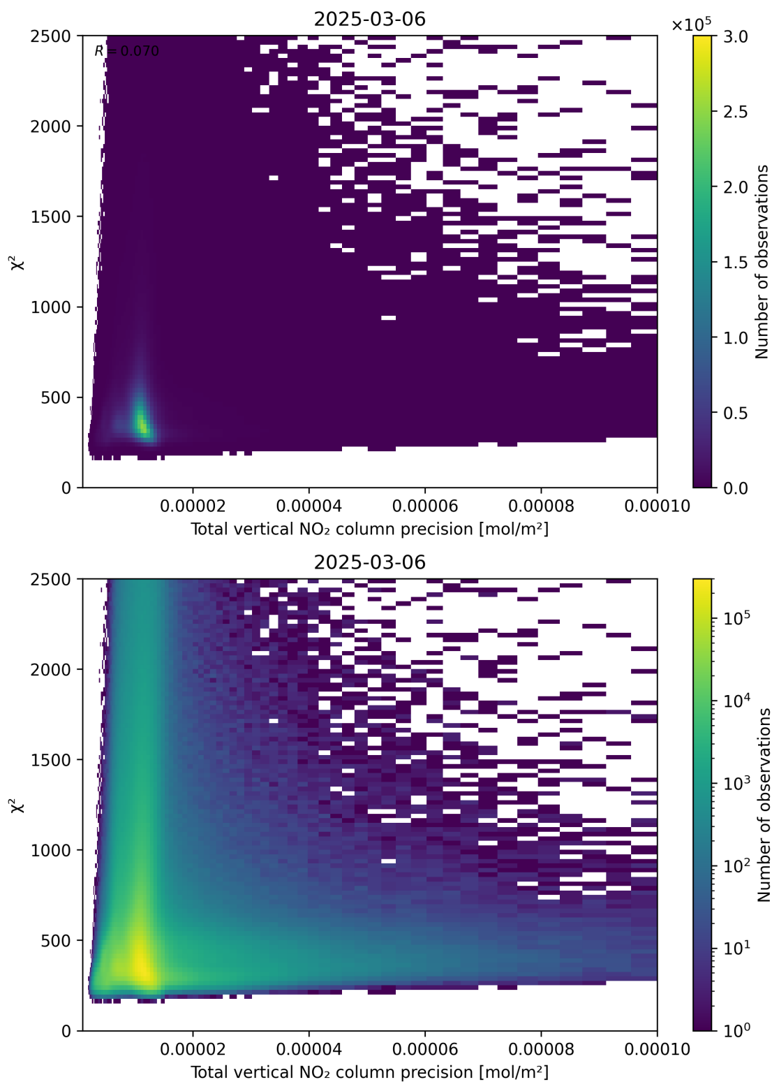
Figure 116: Scatter density plot of “Total vertical NO 2 column precision” against “ \chi^2 ” for 2025-03-06 to 2025-03-07.
