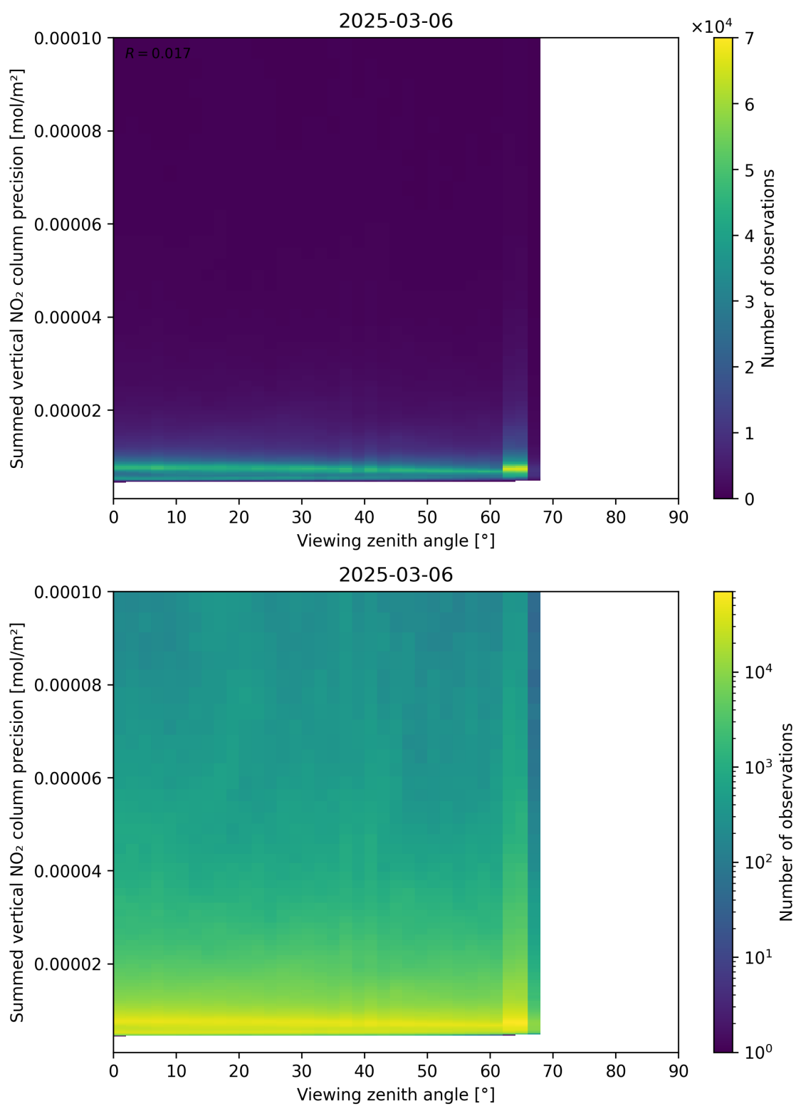
Figure 166: Scatter density plot of “Viewing zenith angle” against “Summed vertical NO 2 column precision” for 2025-03-06 to 2025-03-07.
