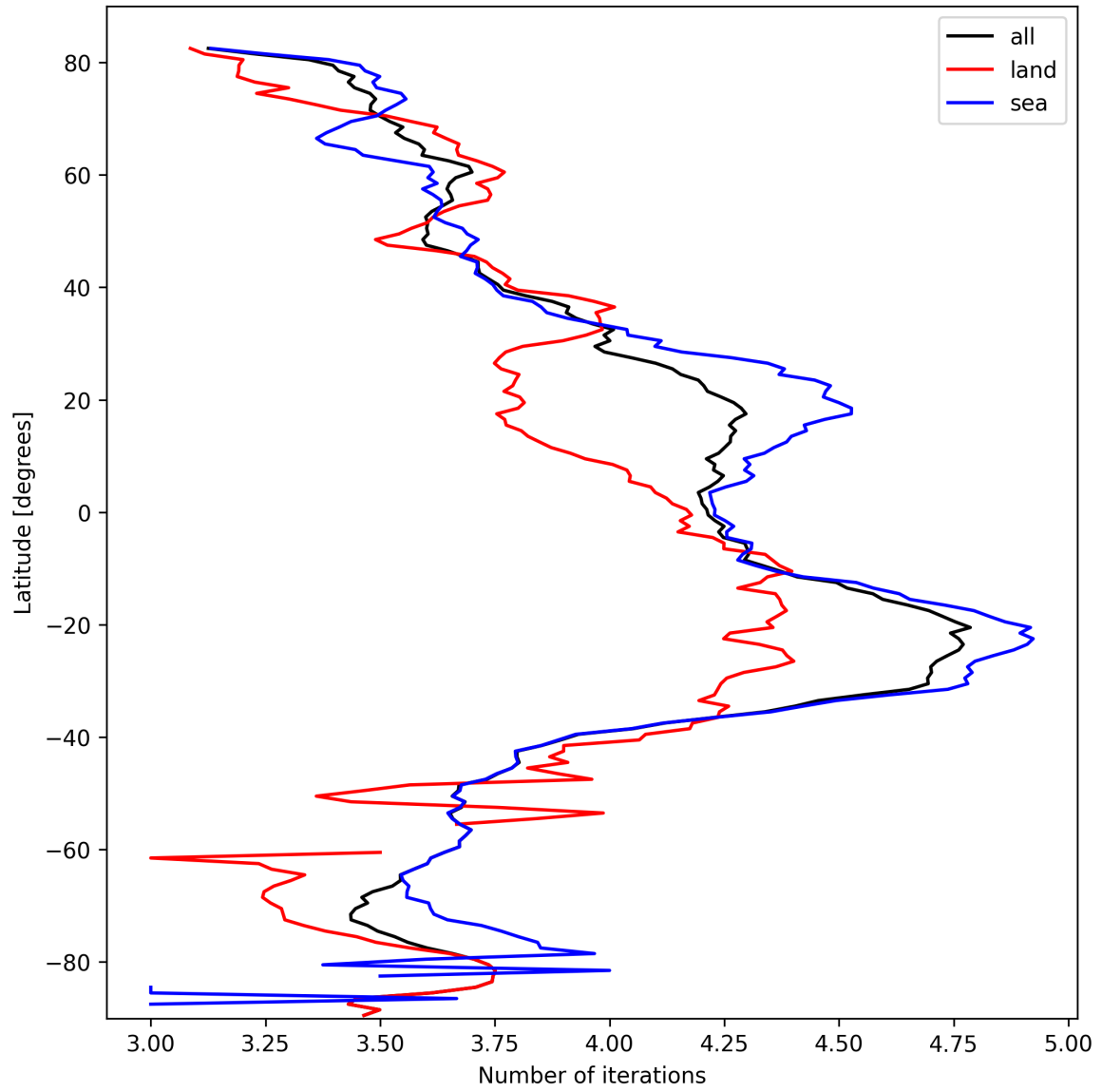
Figure 17: Zonal average of “Number of iterations” for 2025-03-06 to 2025-03-07.
