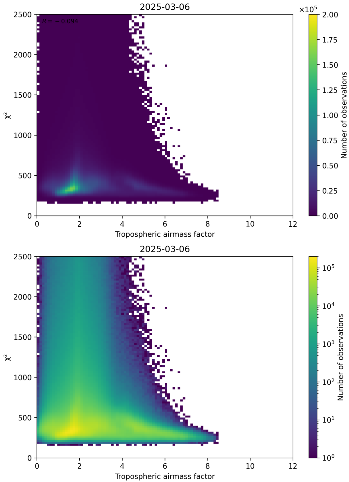
Figure 73: Scatter density plot of “Tropospheric airmass factor” against “ \chi^2 ” for 2025-03-06 to 2025-03-07.
