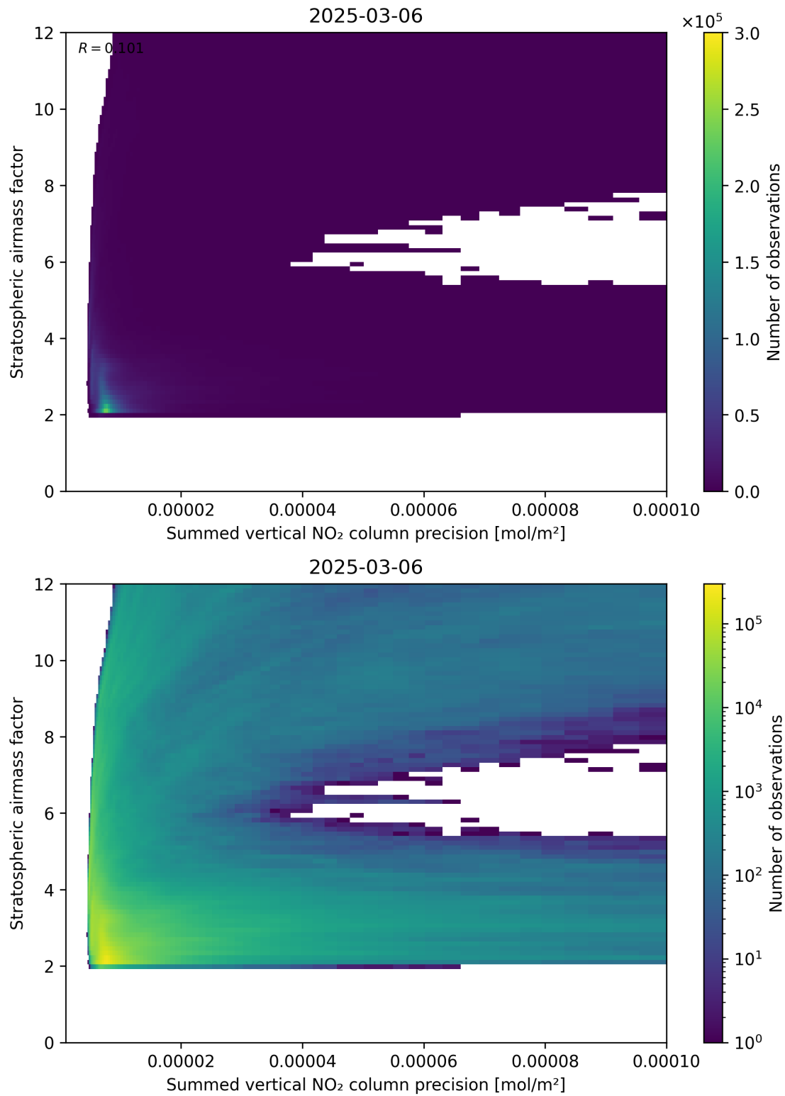
Figure 106: Scatter density plot of “Summed vertical NO 2 column precision” against “Stratospheric airmass factor” for 2025-03-06 to 2025-03-07.
