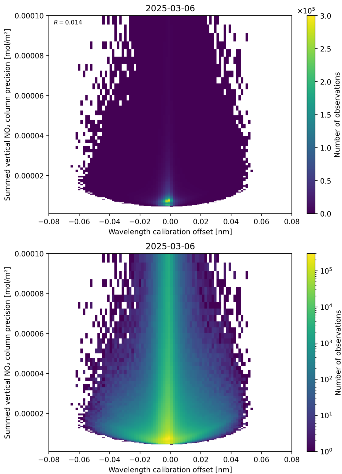
Figure 178: Scatter density plot of “Wavelength calibration offset” against “Summed vertical NO 2 column precision” for 2025-03-06 to 2025-03-07.
