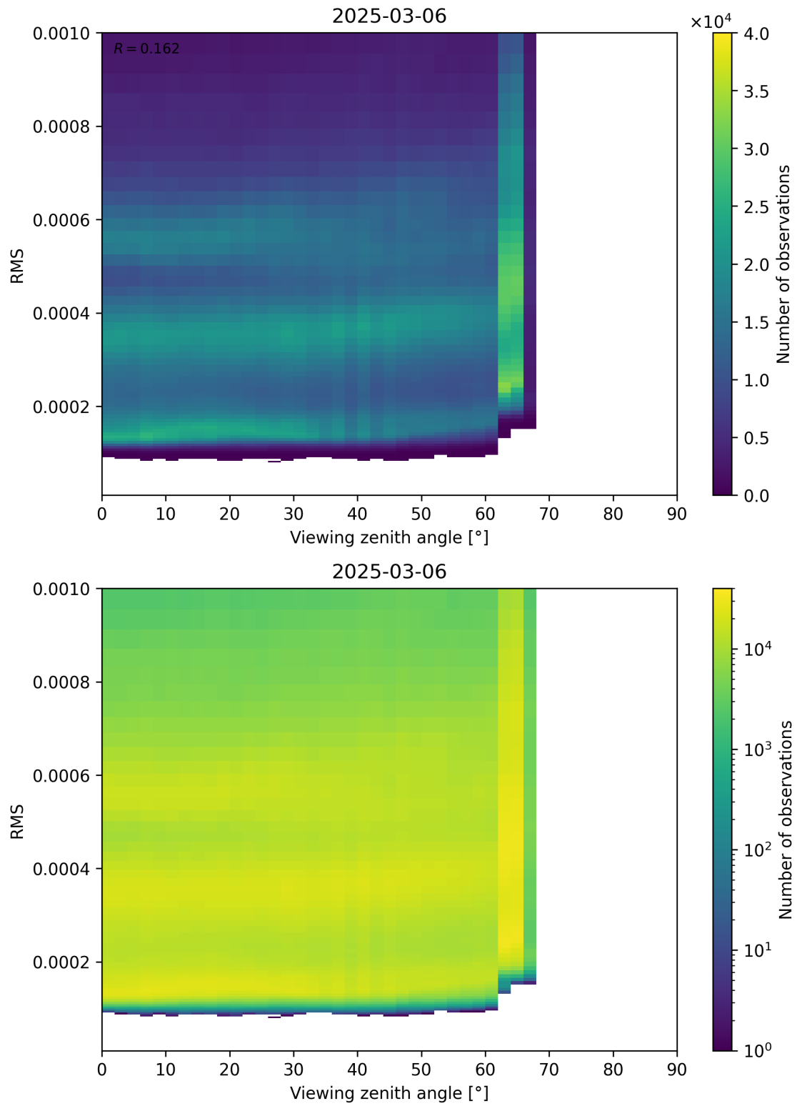
Figure 171: Scatter density plot of “Viewing zenith angle” against “RMS” for 2025-03-06 to 2025-03-07.
