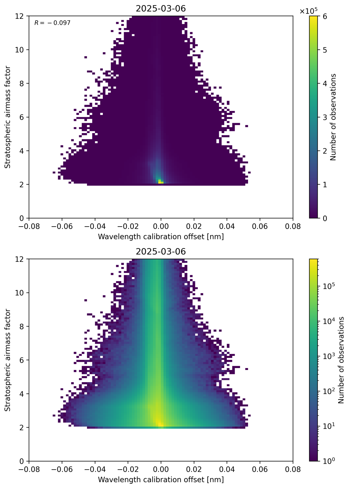
Figure 174: Scatter density plot of “Wavelength calibration offset” against “Stratospheric airmass factor” for 2025-03-06 to 2025-03-07.
