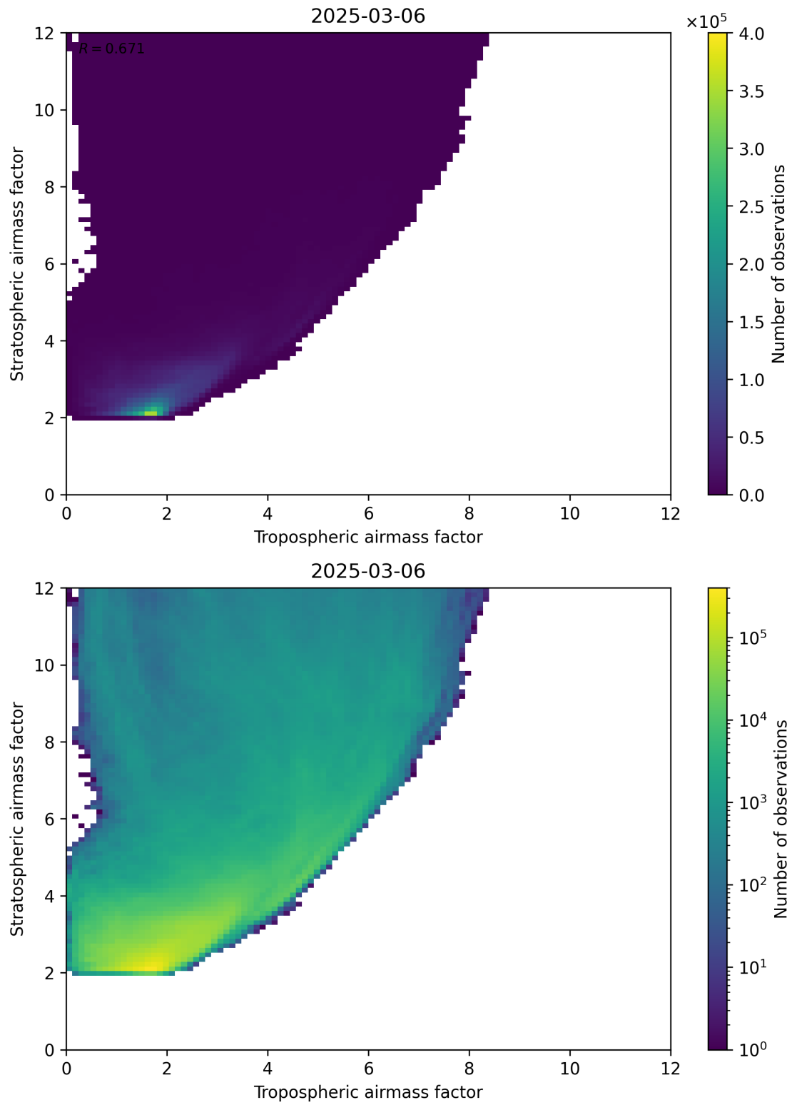
Figure 71: Scatter density plot of “Tropospheric airmass factor” against “Stratospheric airmass factor” for 2025-03-06 to 2025-03-07.
