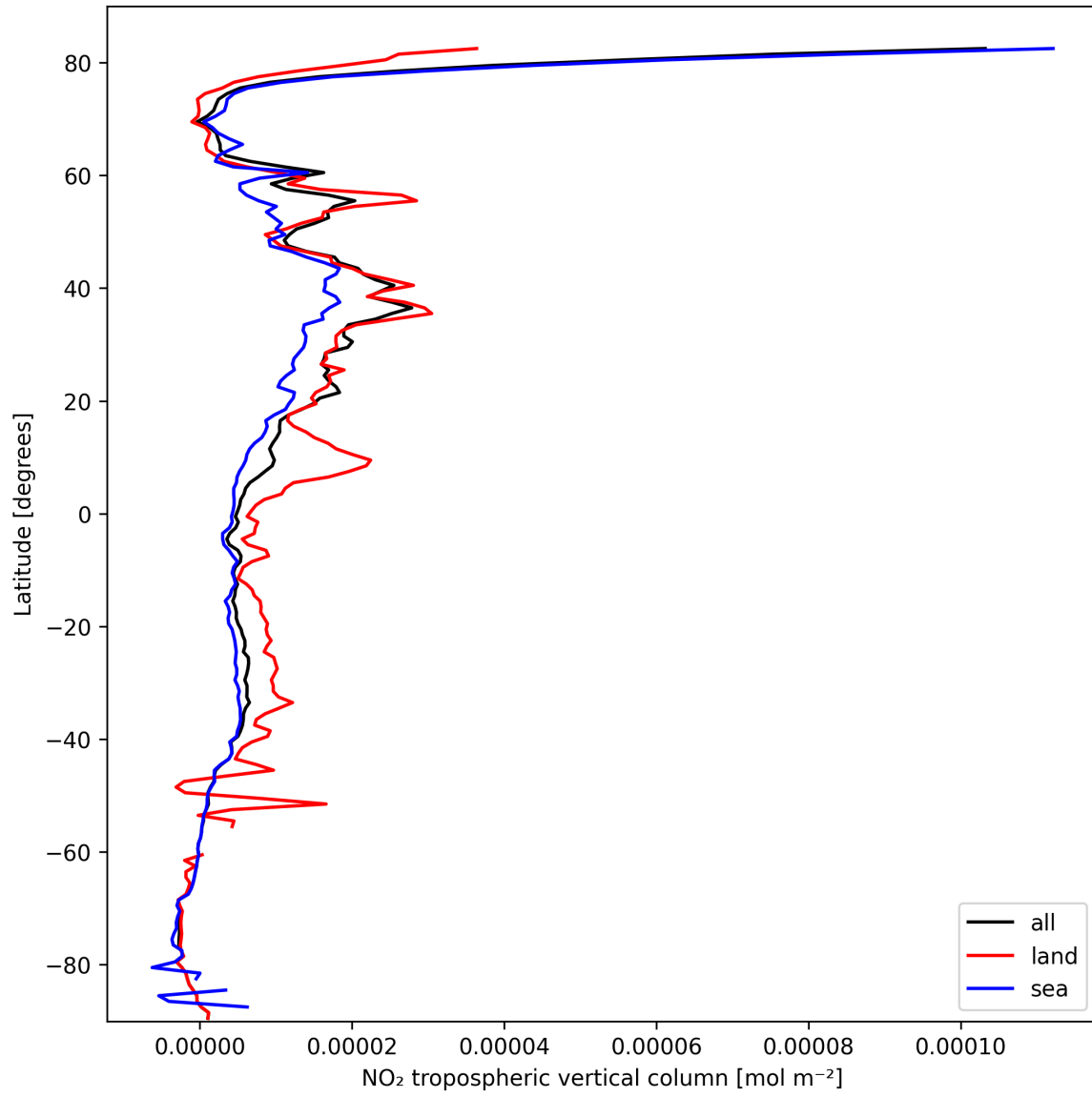
Figure 12: Zonal average of “NO 2 tropospheric vertical column” for 2025-03-06 to 2025-03-07.
