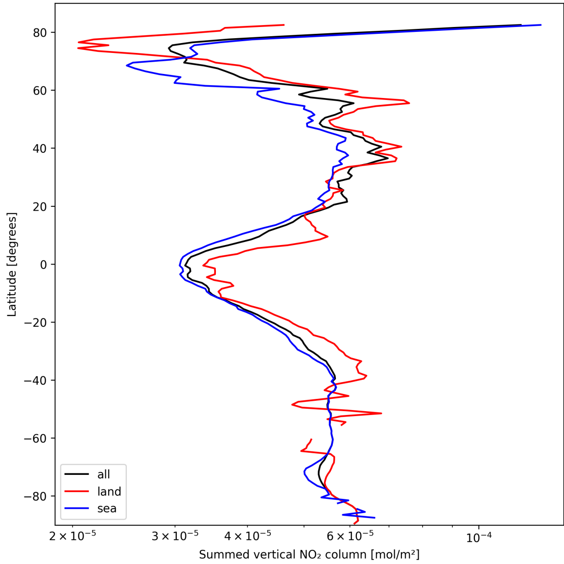
Figure 23: Zonal average of “Summed vertical NO 2 column” for 2025-03-06 to 2025-03-07.
