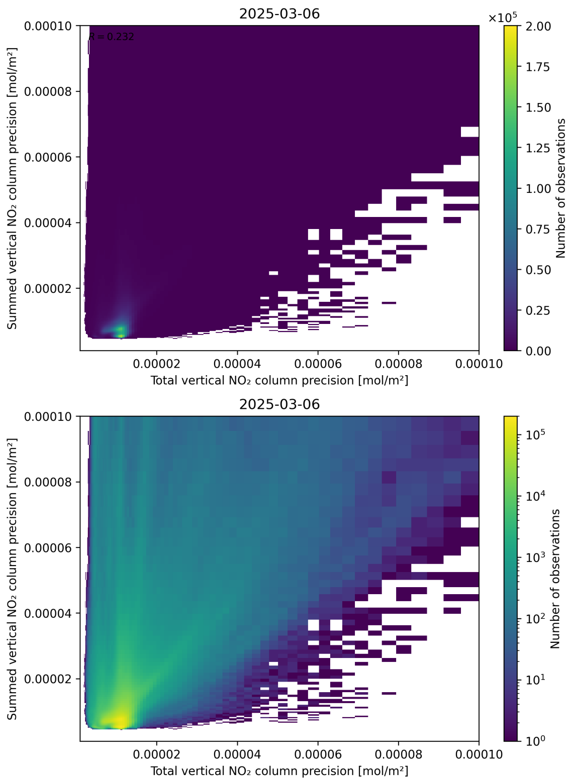
Figure 118: Scatter density plot of “Total vertical NO 2 column precision” against “Summed vertical NO 2 column precision” for 2025-03-06 to 2025-03-07.
