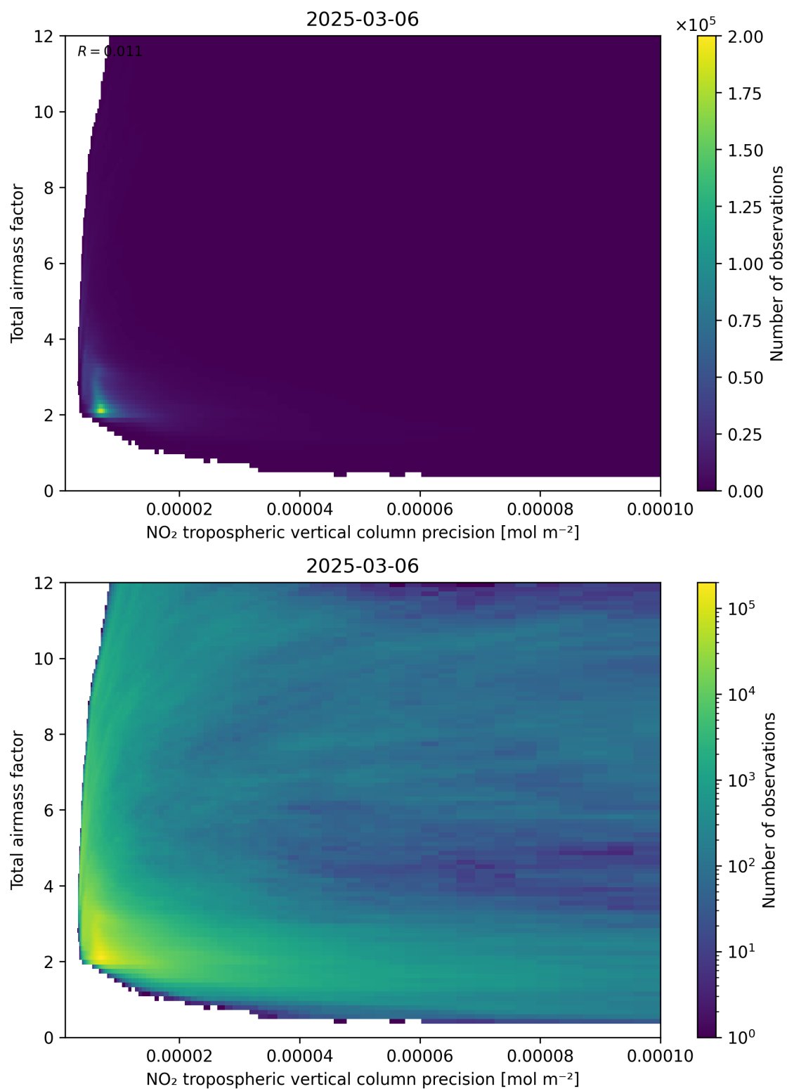
Figure 132: Scatter density plot of “NO 2 tropospheric vertical column precision” against “Total air mass factor” for 2025-03-06 to 2025-03-07.
