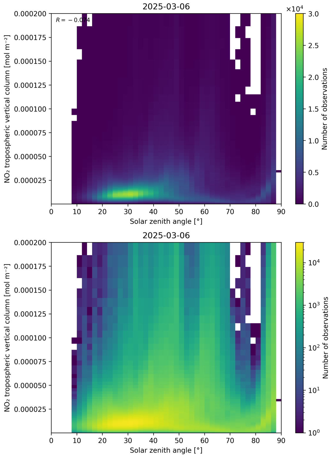
Figure 155: Scatter density plot of “Solar zenith angle” against “NO 2 tropospheric vertical column” for 2025-03-06 to 2025-03-07.
