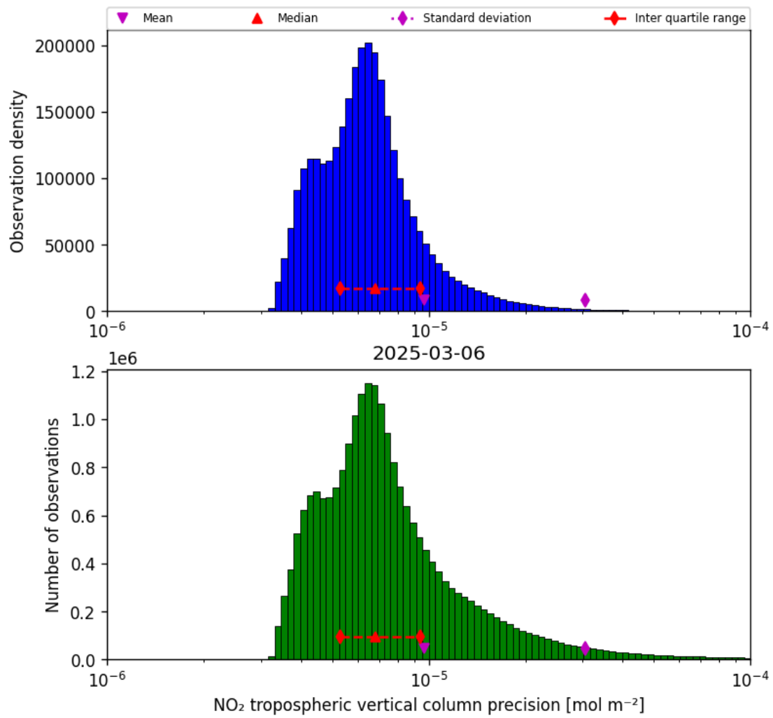
Figure 30: Histogram of “NO 2 tropospheric vertical column precision” for 2025-03-06 to 2025-03-07
