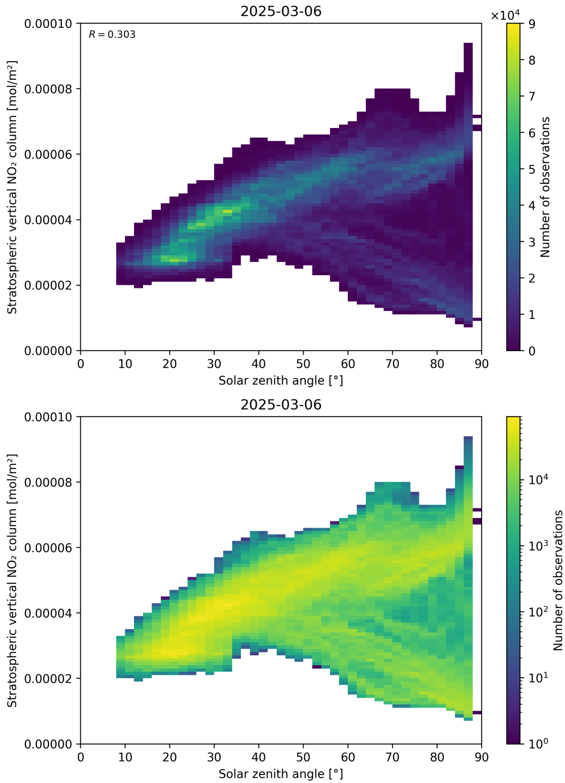
Figure 150: Scatter density plot of “Solar zenith angle” against “Stratospheric vertical NO 2 column” for 2025-03-06 to 2025-03-07.
