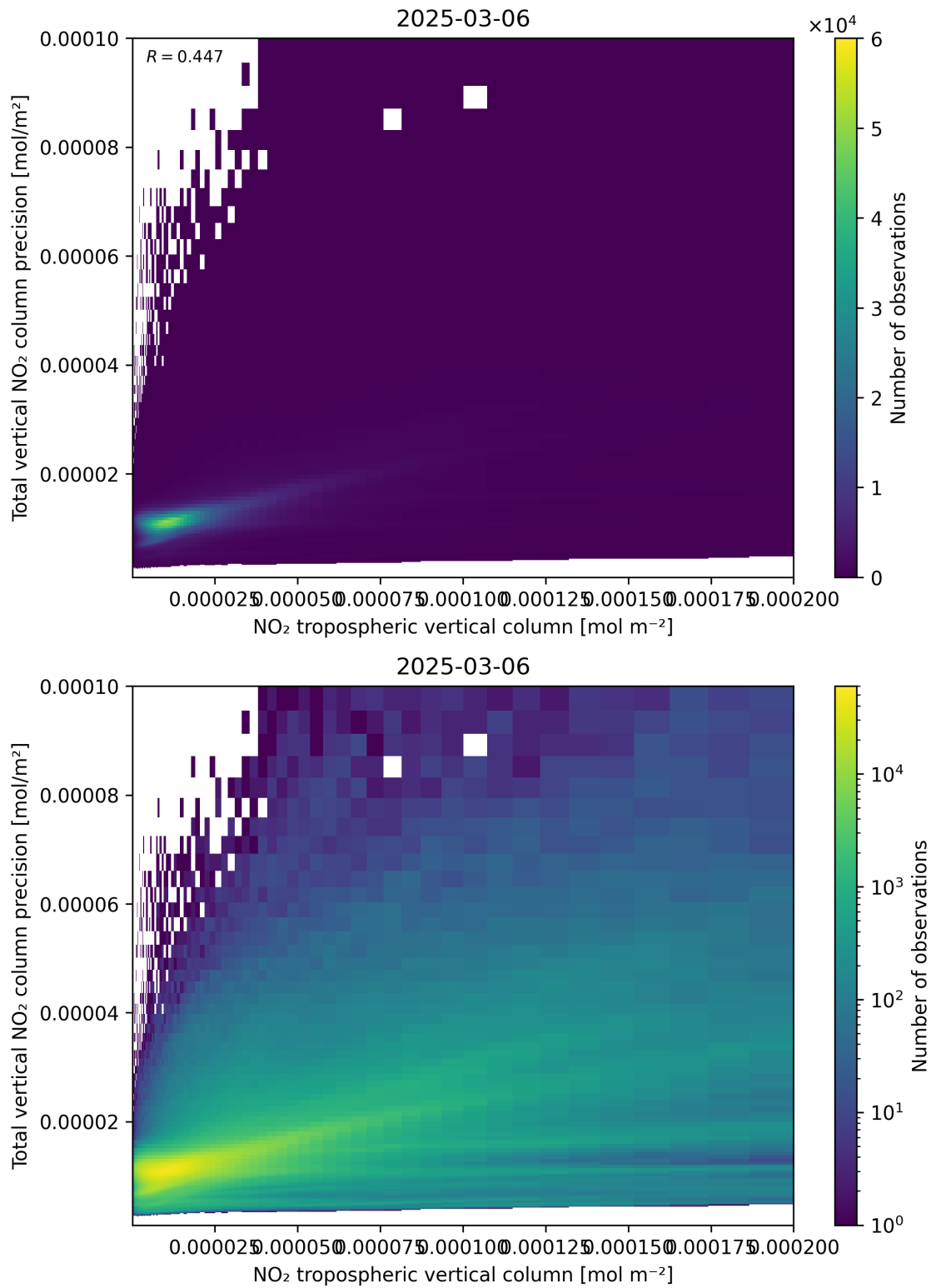
Figure 129: Scatter density plot of “NO 2 tropospheric vertical column” against “Total vertical NO 2 column precision” for 2025-03-06 to 2025-03-07.
