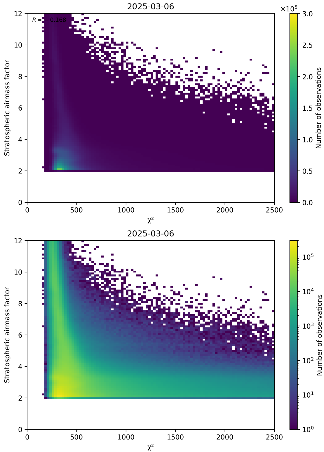
Figure 81: Scatter density plot of “ \chi^2 ” against “Stratospheric airmass factor” for 2025-03-06 to 2025-03-07.
