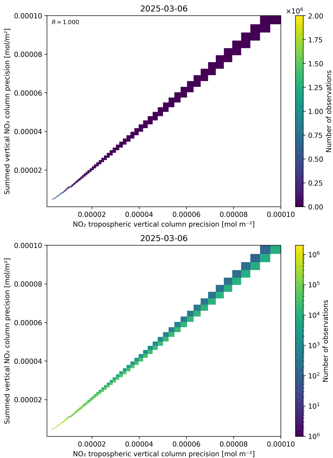
Figure 137: Scatter density plot of “NO 2 tropospheric vertical column precision” against “Summed vertical NO 2 column precision” for 2025-03-06 to 2025-03-07.
