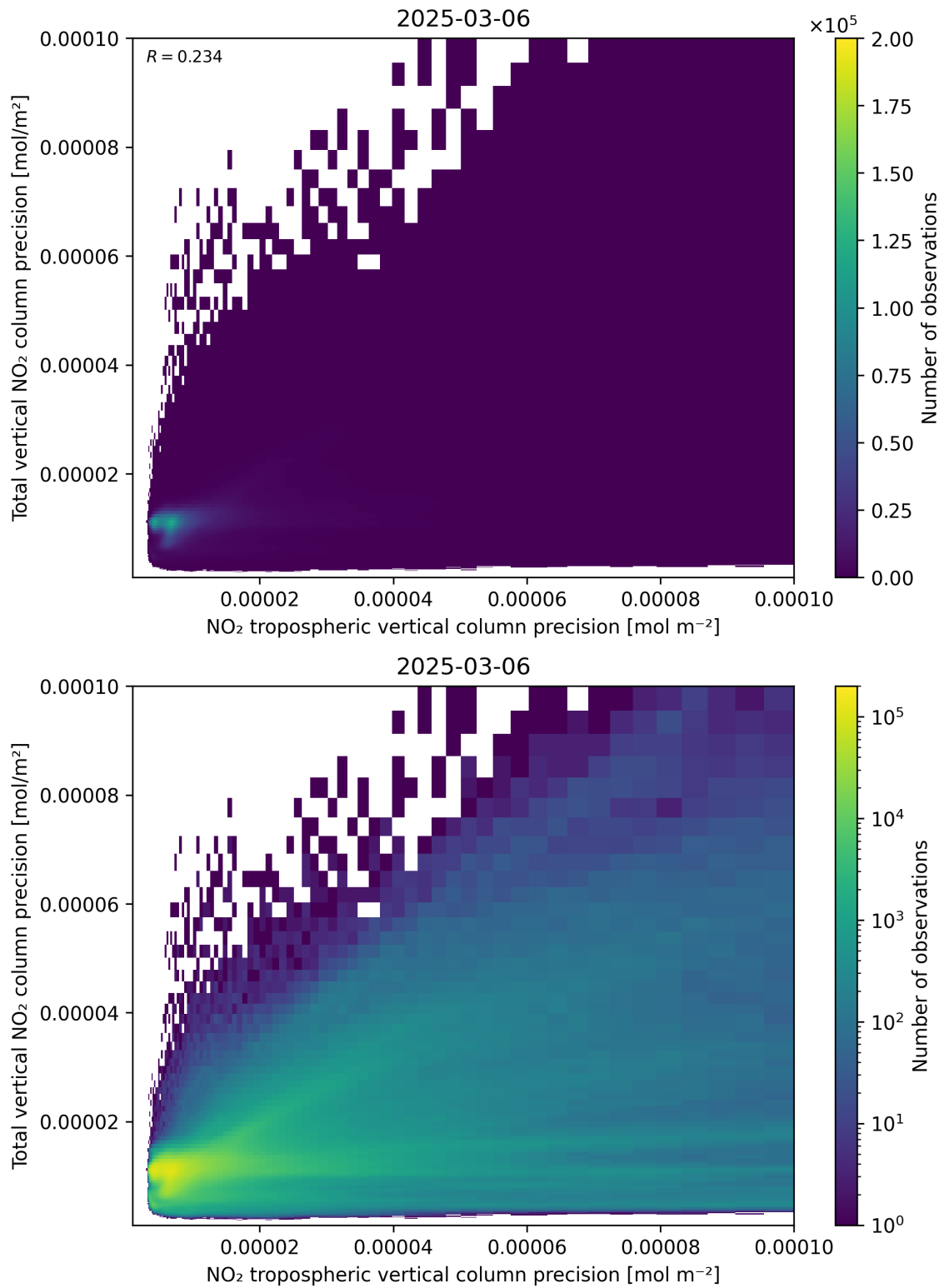
Figure 139: Scatter density plot of “NO 2 tropospheric vertical column precision” against “Total vertical NO 2 column precision” for 2025-03-06 to 2025-03-07.
