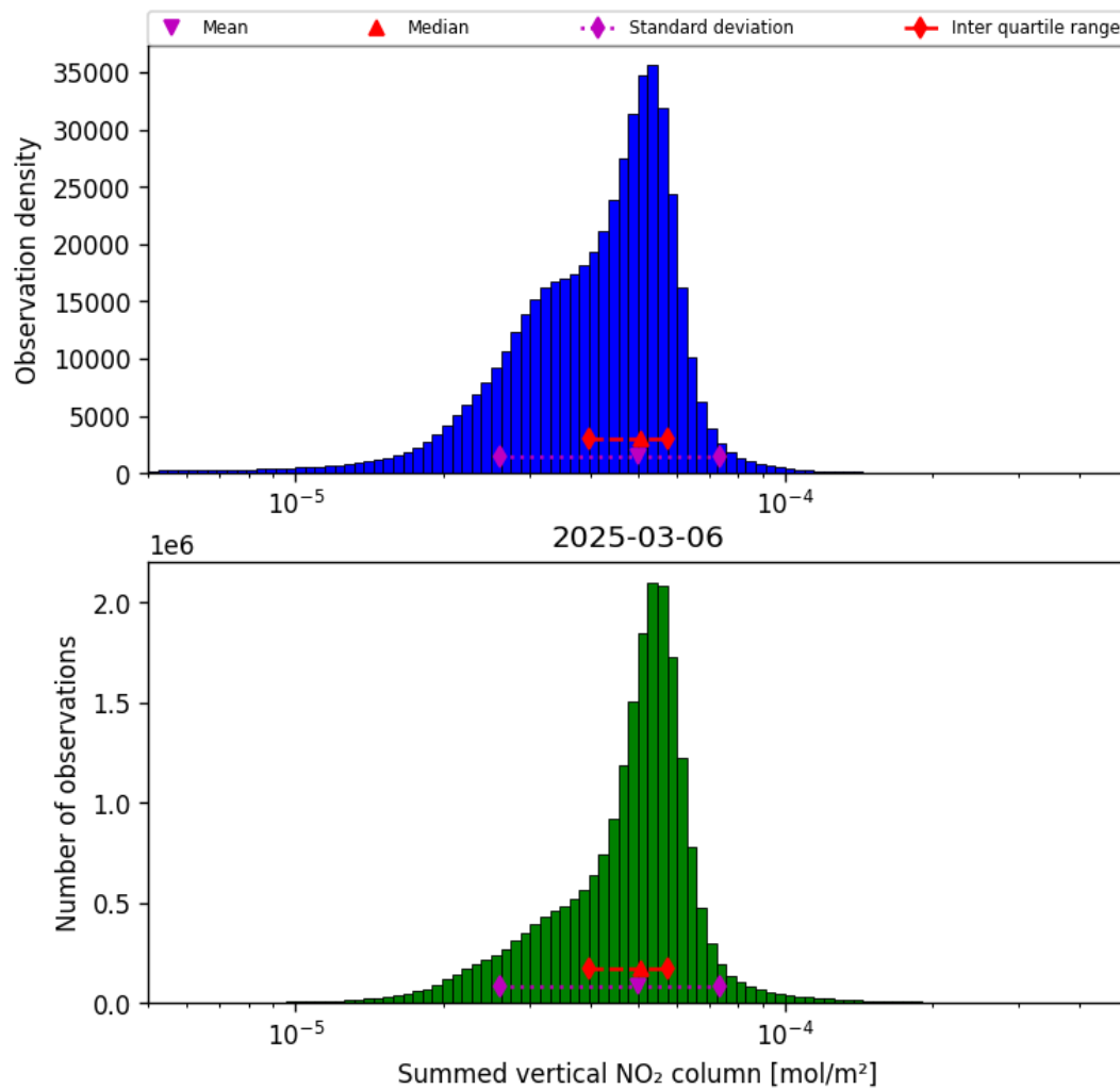
Figure 40: Histogram of “Summed vertical NO 2 column” for 2025-03-06 to 2025-03-07
