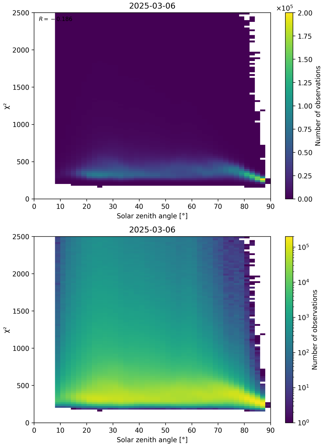
Figure 148: Scatter density plot of “Solar zenith angle” against “ \chi^2 ” for 2025-03-06 to 2025-03-07.
