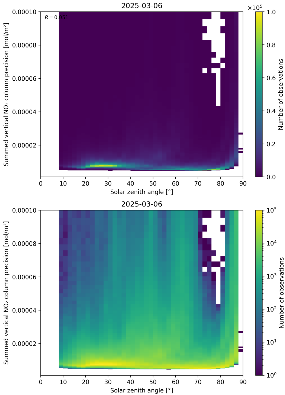
Figure 152: Scatter density plot of “Solar zenith angle” against “Summed vertical NO 2 column precision” for 2025-03-06 to 2025-03-07.
