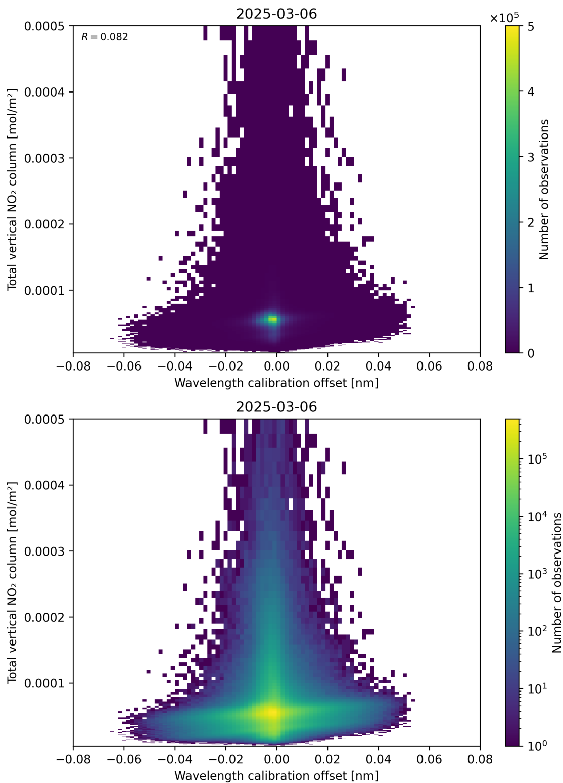
Figure 179: Scatter density plot of “Wavelength calibration offset” against “Total vertical NO 2 column” for 2025-03-06 to 2025-03-07.
