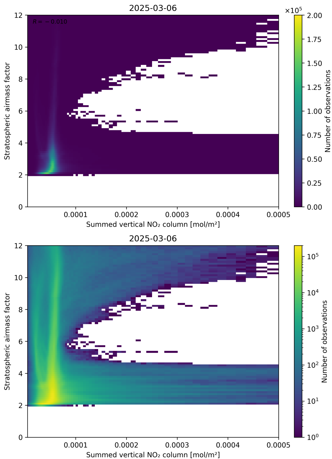
Figure 103: Scatter density plot of “Summed vertical NO 2 column” against “Stratospheric airmass factor” for 2025-03-06 to 2025-03-07.
