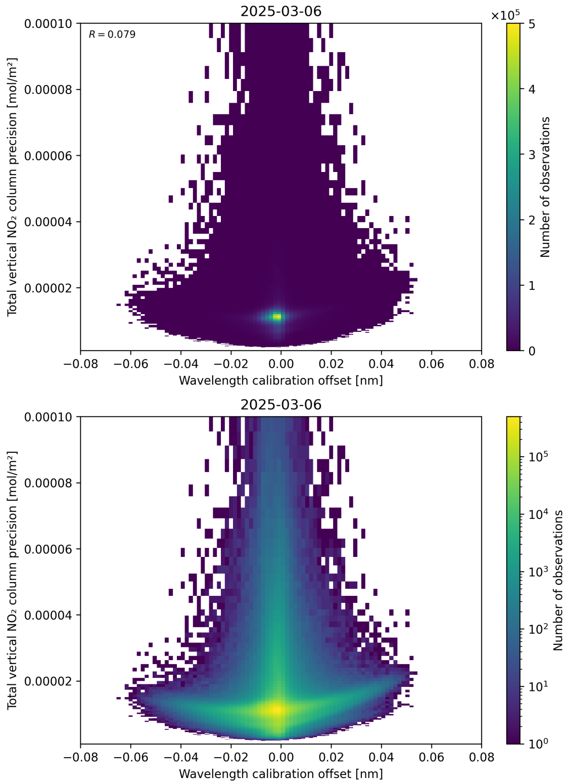
Figure 180: Scatter density plot of “Wavelength calibration offset” against “Total vertical NO 2 column precision” for 2025-03-06 to 2025-03-07.
