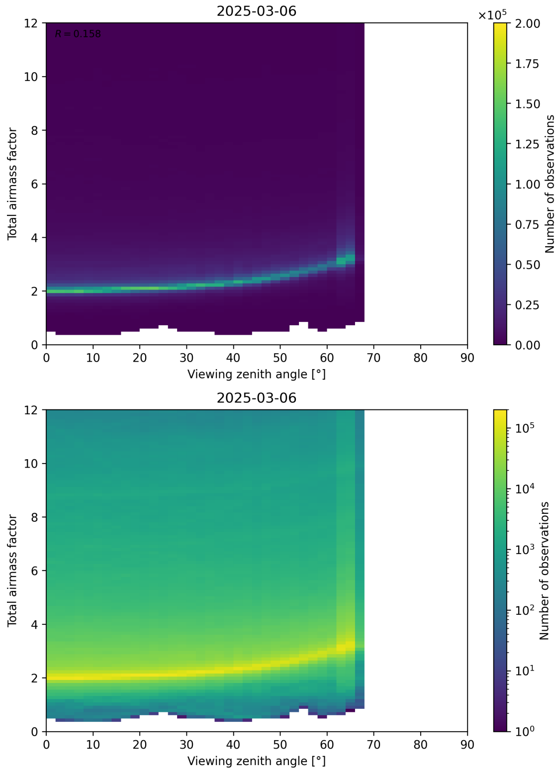
Figure 160: Scatter density plot of “Viewing zenith angle” against “Total airmass factor” for 2025-03-06 to 2025-03-07.
