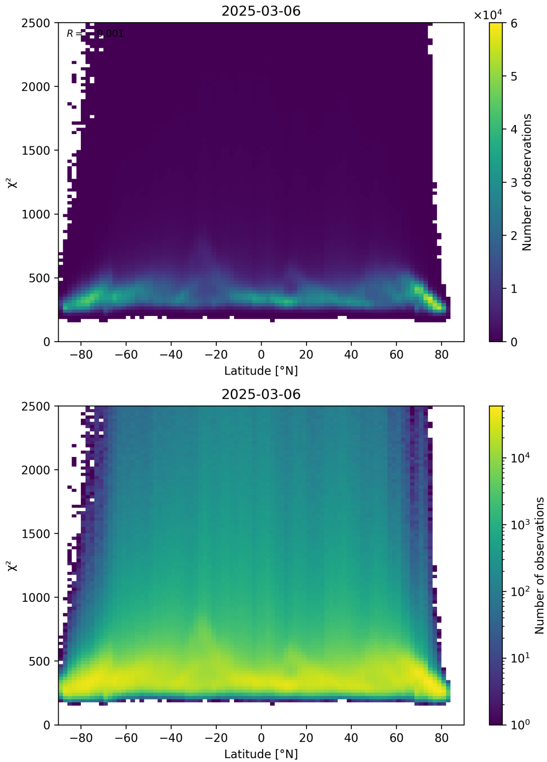
Figure 86: Scatter density plot of “Latitude” against “ \chi^2 ” for 2025-03-06 to 2025-03-07.
