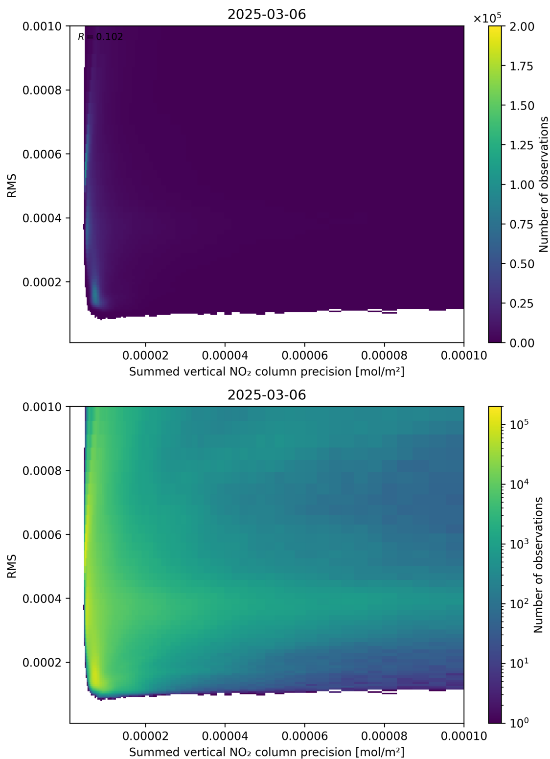
Figure 108: Scatter density plot of “Summed vertical NO 2 column precision” against “RMS” for 2025-03-06 to 2025-03-07.
