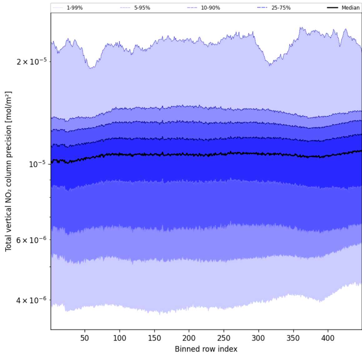
Figure 56: Along track statistics of “Total vertical NO 2 column precision” for 2025-03-06 to 2025-03-07
