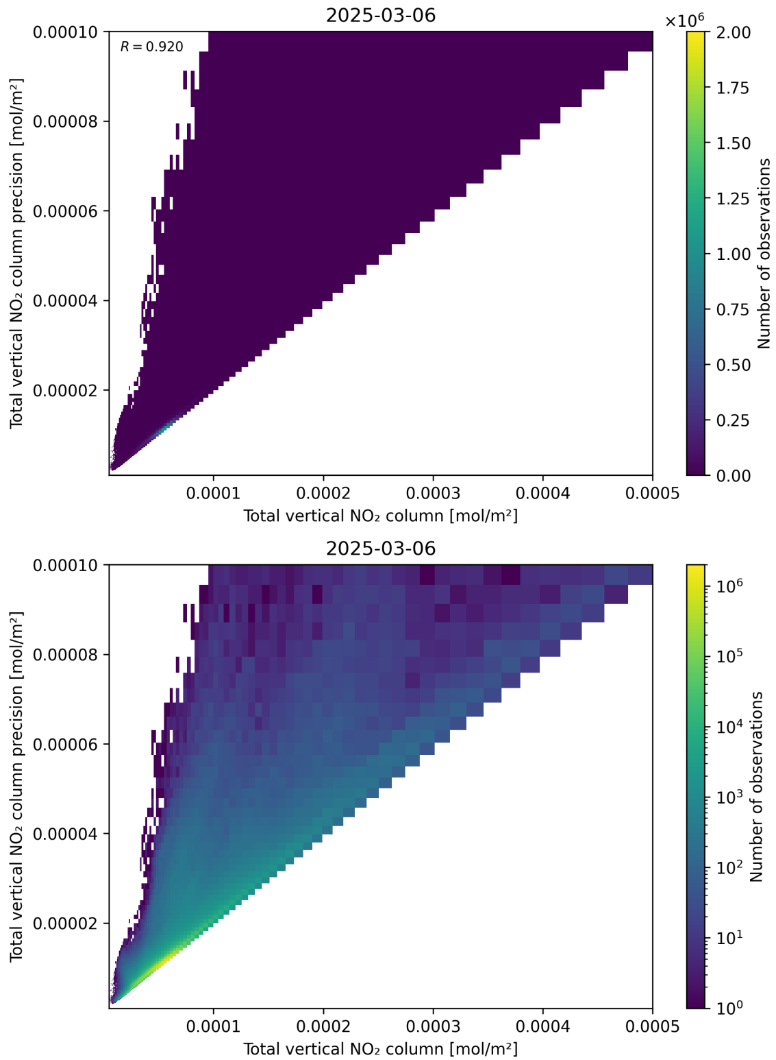
Figure 114: Scatter density plot of “Total vertical NO 2 column” against “Total vertical NO 2 column precision” for 2025-03-06 to 2025-03-07.
