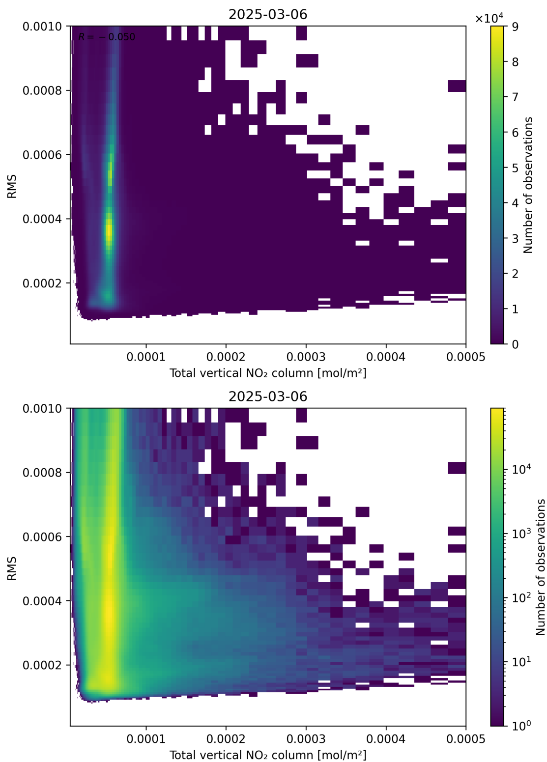
Figure 120: Scatter density plot of “Total vertical NO 2 column” against “RMS” for 2025-03-06 to 2025-03-07.
