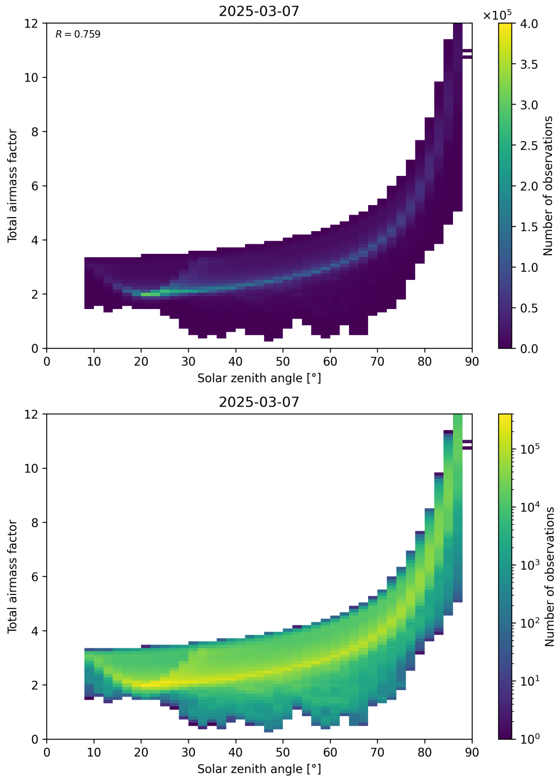
Figure 146: Scatter density plot of “Solar zenith angle” against “Total air mass factor” for 2025-03-07 to 2025-03-08.
