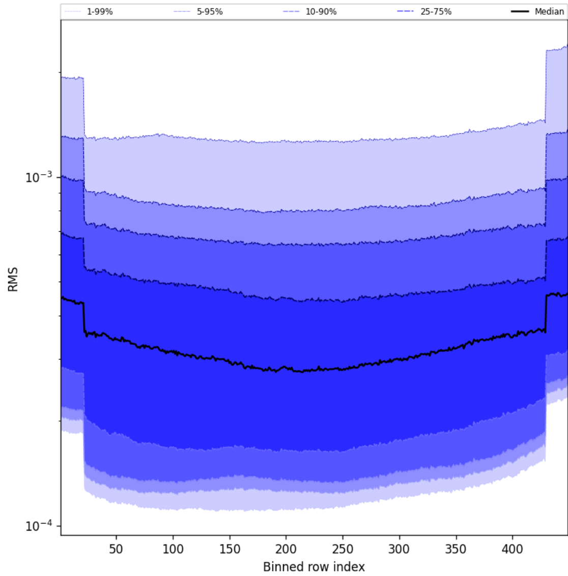
Figure 60: Along track statistics of “RMS” for 2025-03-07 to 2025-03-08
