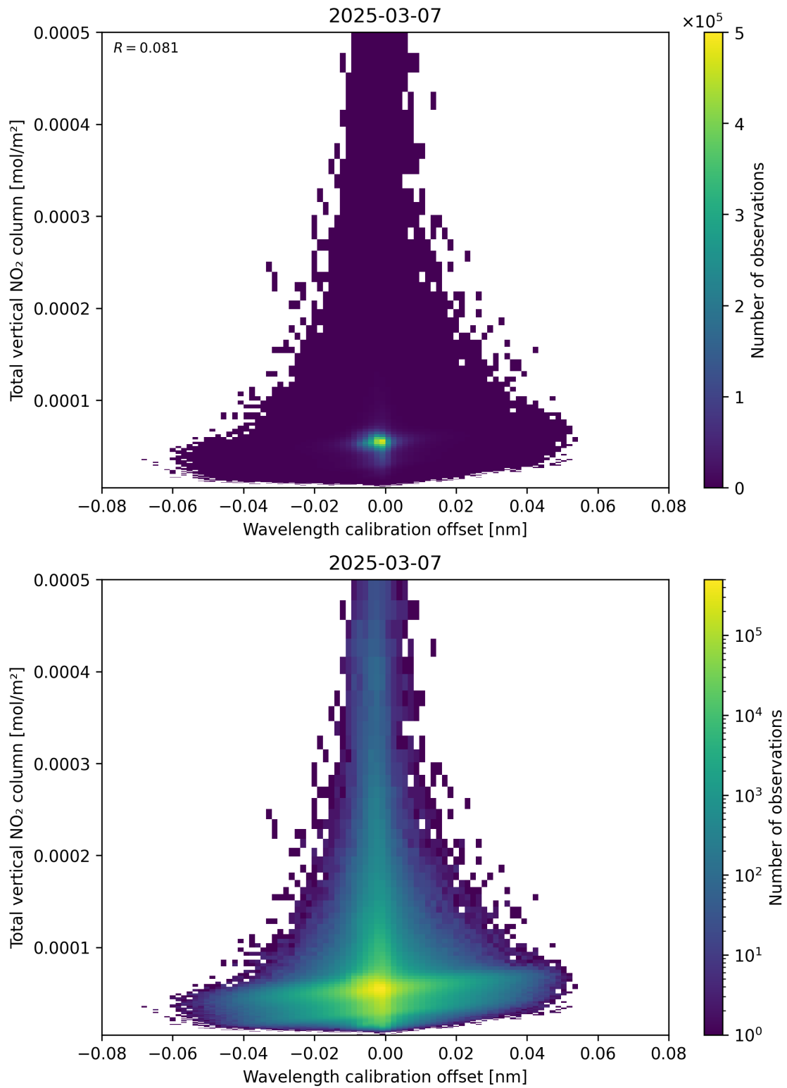
Figure 179: Scatter density plot of “Wavelength calibration offset” against “Total vertical NO 2 column” for 2025-03-07 to 2025-03-08.
