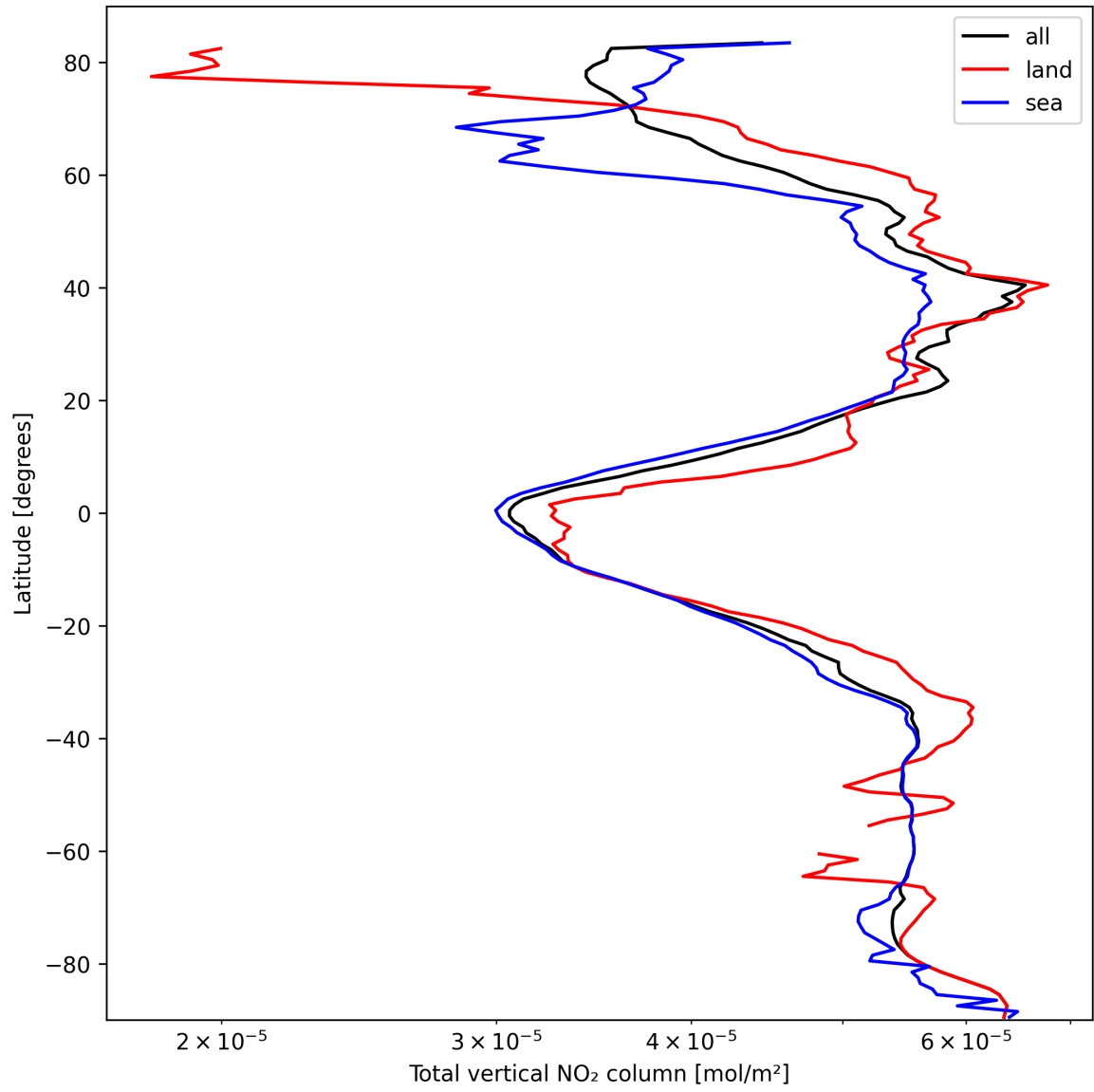
Figure 21: Zonal average of “Total vertical NO 2 column” for 2025-03-07 to 2025-03-08.
