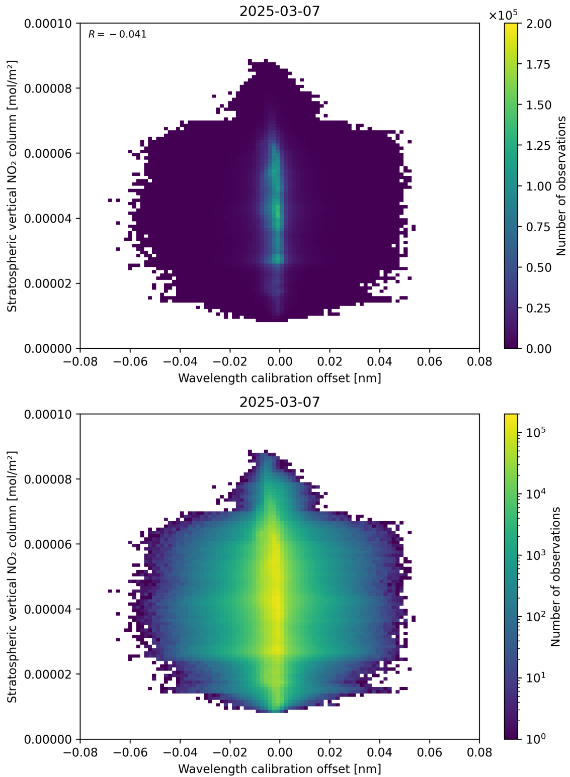
Figure 176: Scatter density plot of “Wavelength calibration offset” against “Stratospheric vertical NO 2 column” for 2025-03-07 to 2025-03-08.
