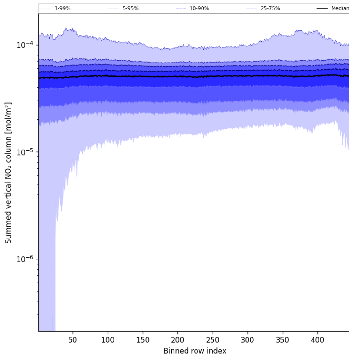
Figure 57: Along track statistics of “Summed vertical NO 2 column” for 2025-03-07 to 2025-03-08
