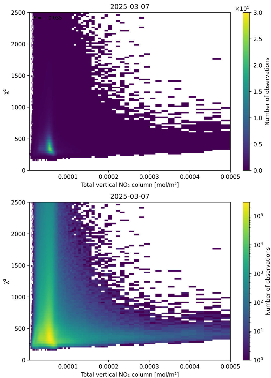
Figure 111: Scatter density plot of “Total vertical NO 2 column” against “ \chi^2 ” for 2025-03-07 to 2025-03-08.
