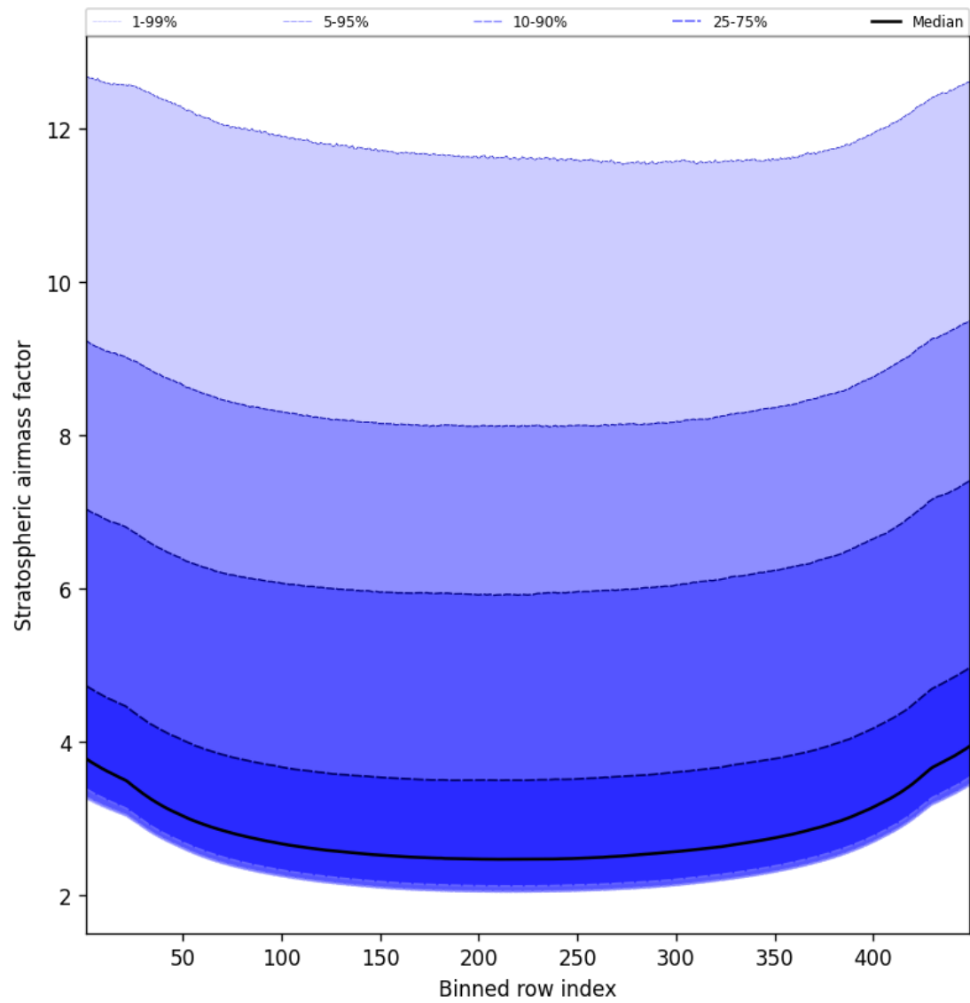
Figure 61: Along track statistics of “Stratospheric airmass factor” for 2025-03-07 to 2025-03-08
