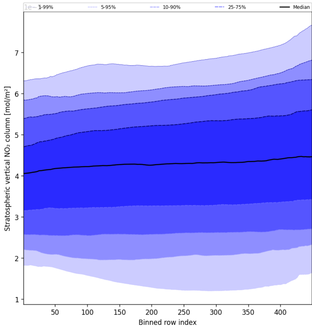
Figure 53: Along track statistics of “Stratospheric vertical NO 2 column” for 2025-03-07 to 2025-03-08
