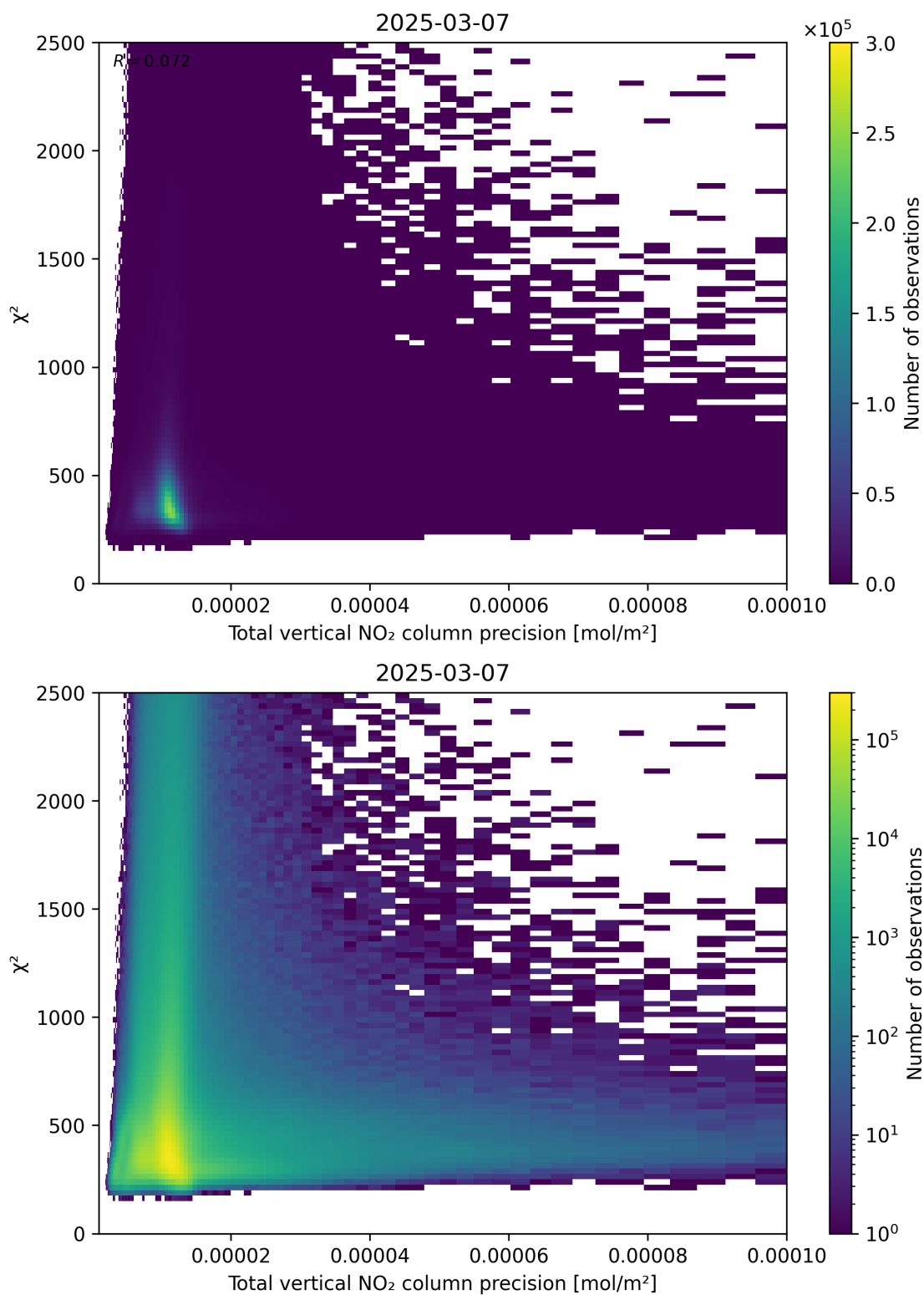
Figure 116: Scatter density plot of “Total vertical NO 2 column precision” against “ \chi^2 ” for 2025-03-07 to 2025-03-08.
