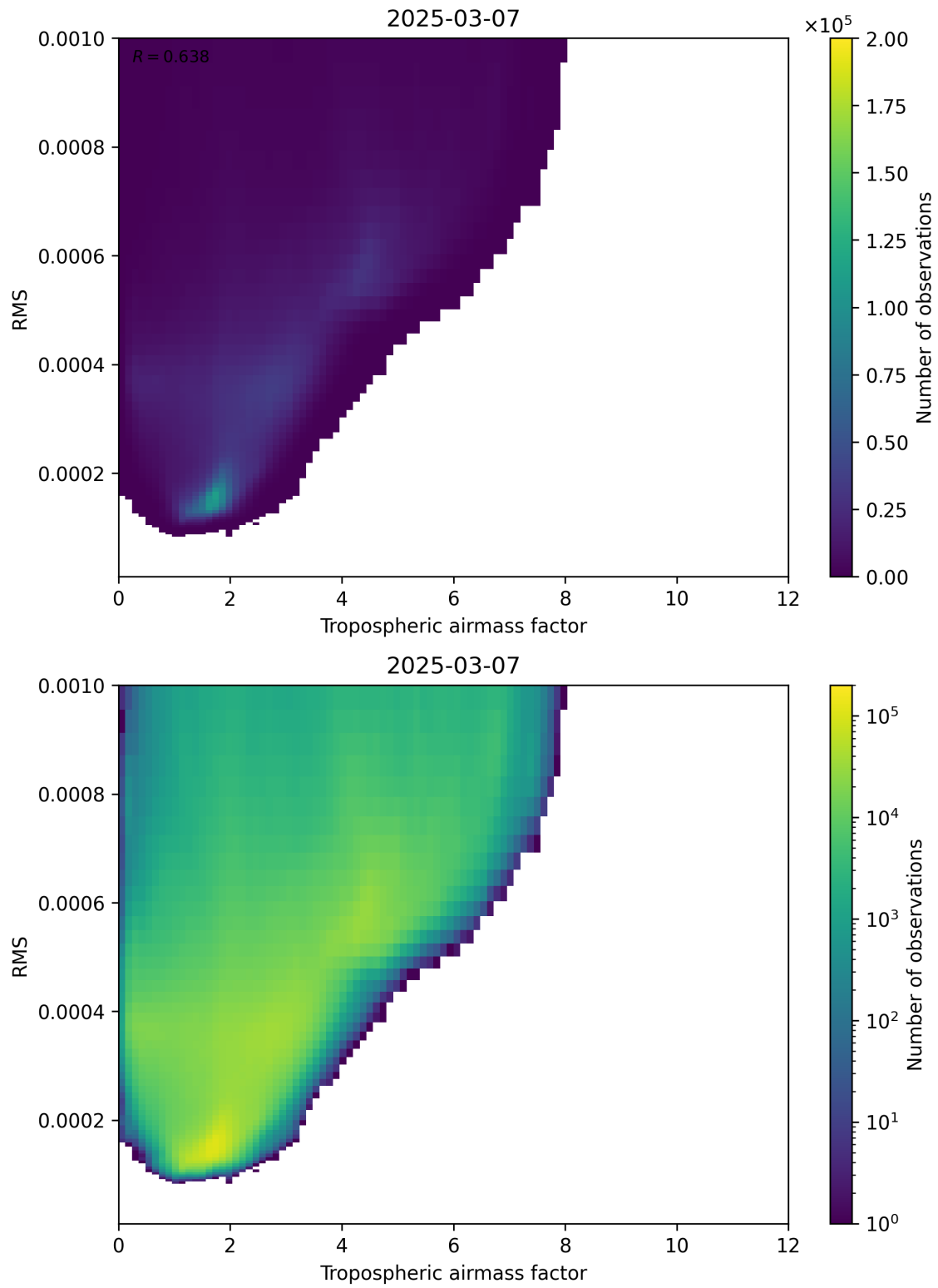
Figure 79: Scatter density plot of “Tropospheric airmass factor” against “RMS” for 2025-03-07 to 2025-03-08.
