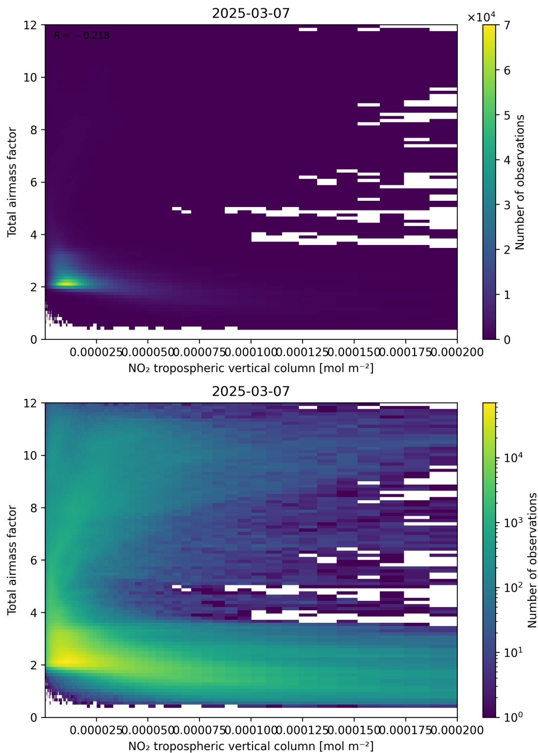
Figure 122: Scatter density plot of “NO 2 tropospheric vertical column” against “Total air mass factor” for 2025-03-07 to 2025-03-08.
