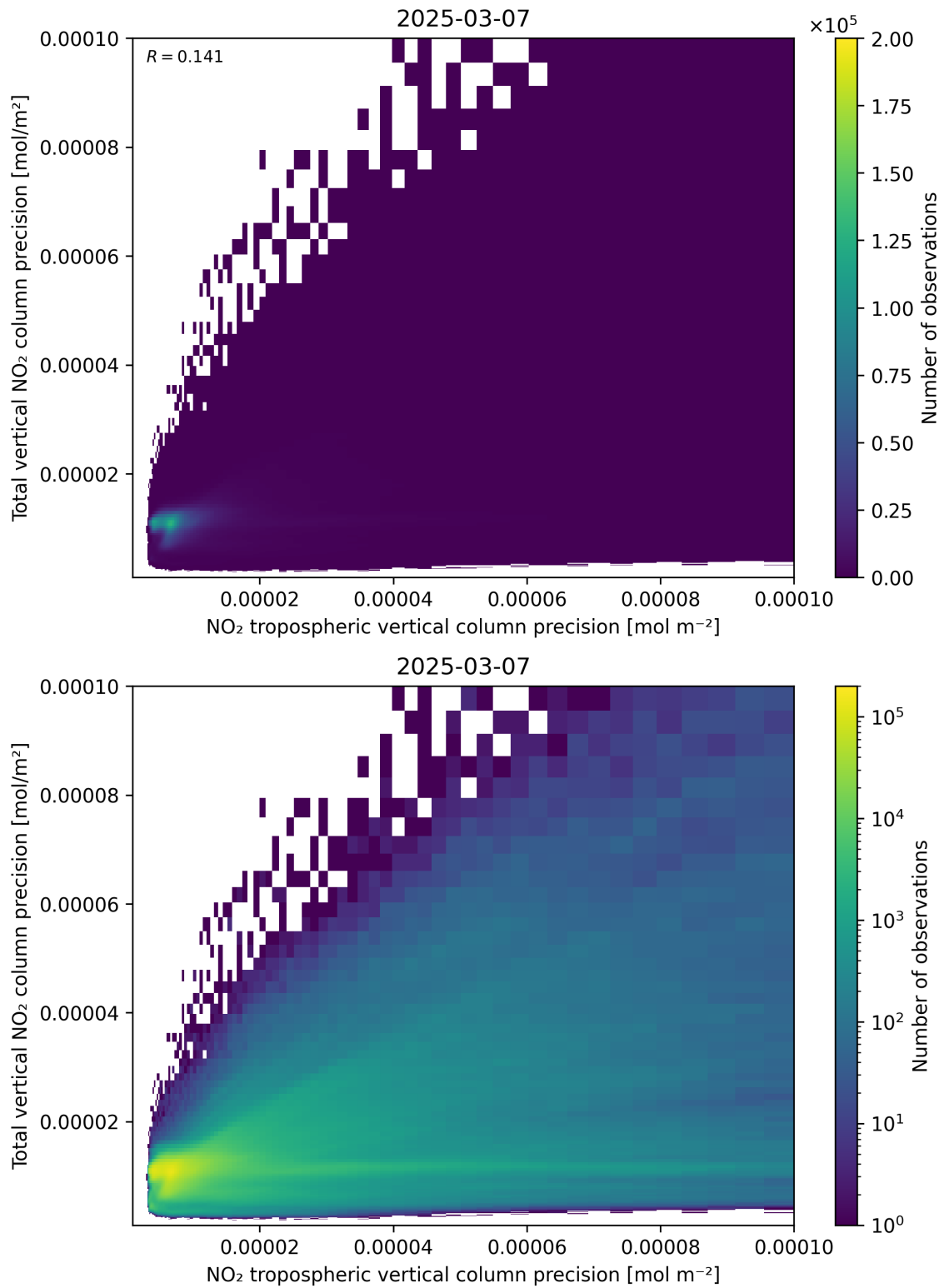
Figure 139: Scatter density plot of “NO 2 tropospheric vertical column precision” against “Total vertical NO 2 column precision” for 2025-03-07 to 2025-03-08.
