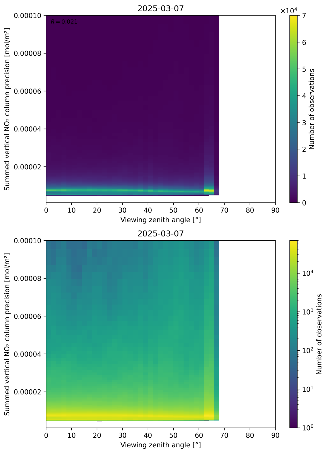
Figure 166: Scatter density plot of “Viewing zenith angle” against “Summed vertical NO 2 column precision” for 2025-03-07 to 2025-03-08.
