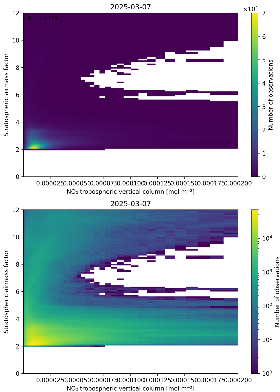
Figure 121: Scatter density plot of “NO 2 tropospheric vertical column” against “Stratospheric air mass factor” for 2025-03-07 to 2025-03-08.
