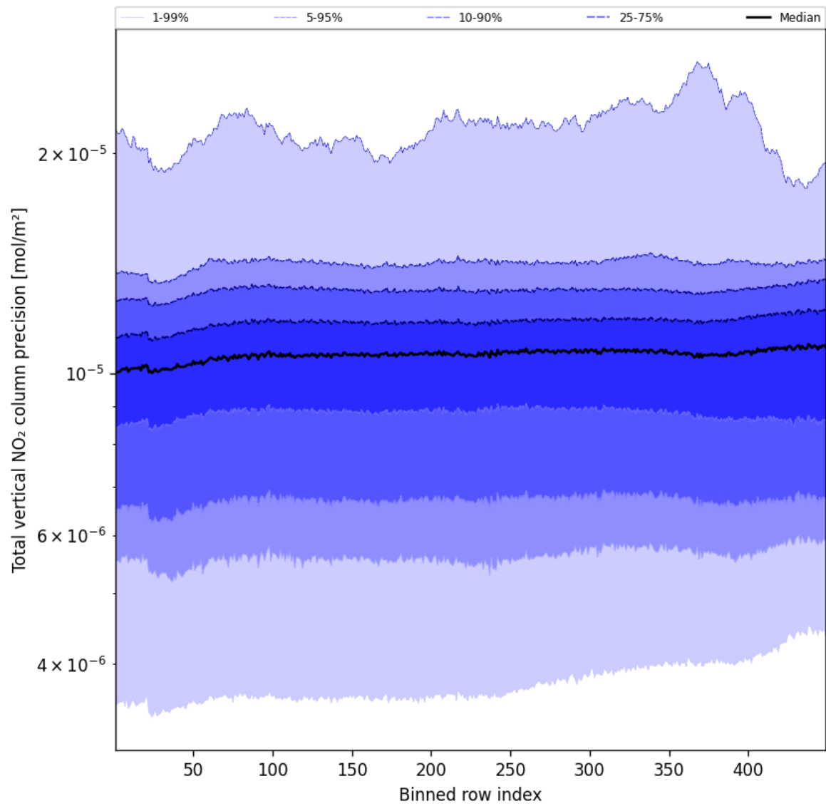
Figure 56: Along track statistics of “Total vertical NO 2 column precision” for 2025-03-07 to 2025-03-08
