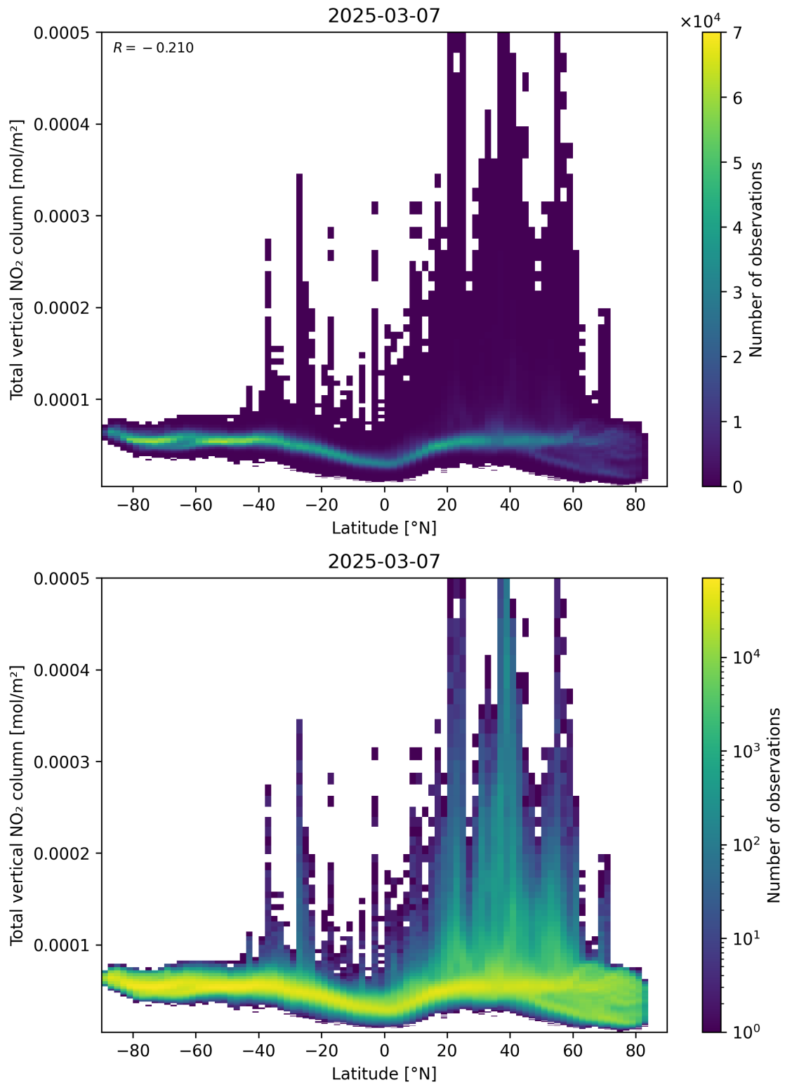
Figure 90: Scatter density plot of “Latitude” against “Total vertical NO 2 column” for 2025-03-07 to 2025-03-08.
