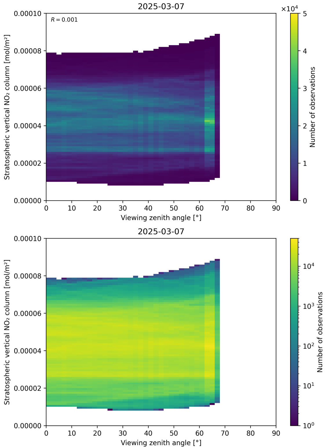
Figure 164: Scatter density plot of “Viewing zenith angle” against “Stratospheric vertical NO 2 column” for 2025-03-07 to 2025-03-08.
