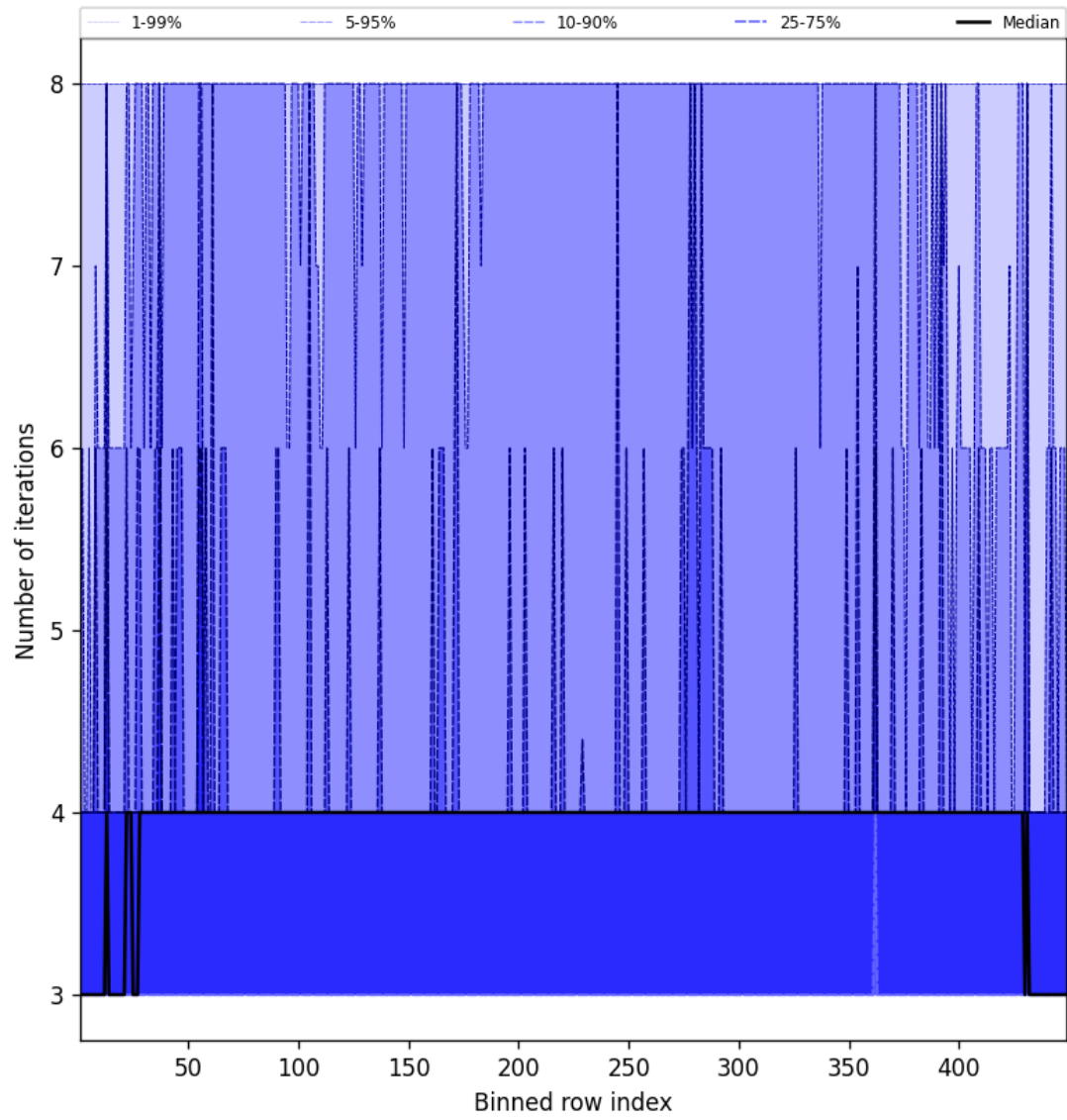
Figure 51: Along track statistics of “Number of iterations” for 2025-03-07 to 2025-03-08
