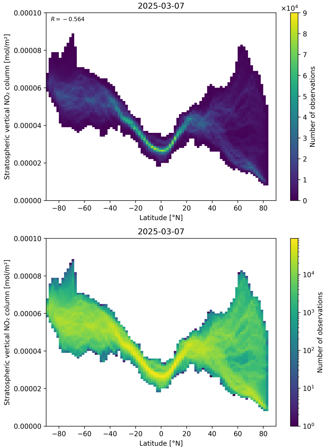
Figure 87: Scatter density plot of “Latitude” against “Stratospheric vertical NO 2 column” for 2025-03-07 to 2025-03-08.
