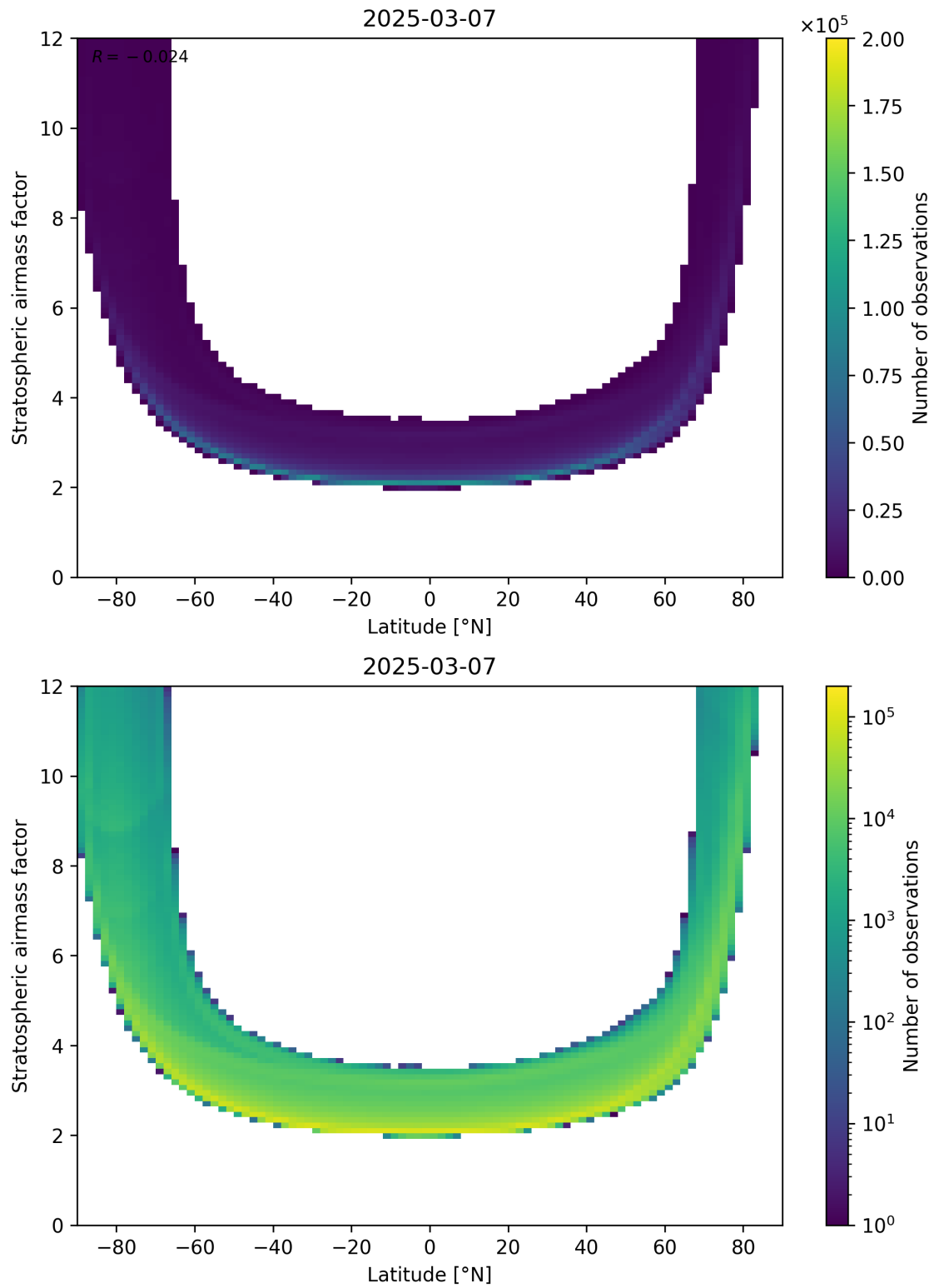
Figure 83: Scatter density plot of “Latitude” against “Stratospheric airmass factor” for 2025-03-07 to 2025-03-08.
