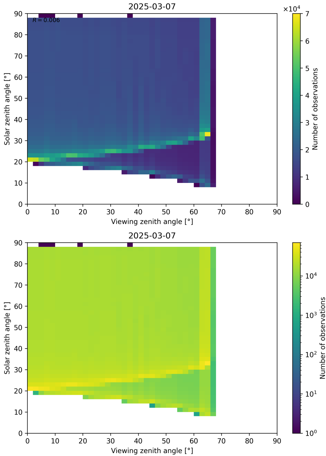
Figure 172: Scatter density plot of “Viewing zenith angle” against “Solar zenith angle” for 2025-03-07 to 2025-03-08.
