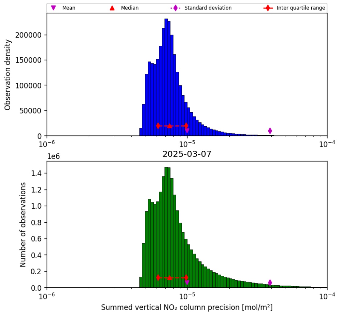
Figure 41: Histogram of “Summed vertical NO 2 column precision” for 2025-03-07 to 2025-03-08
