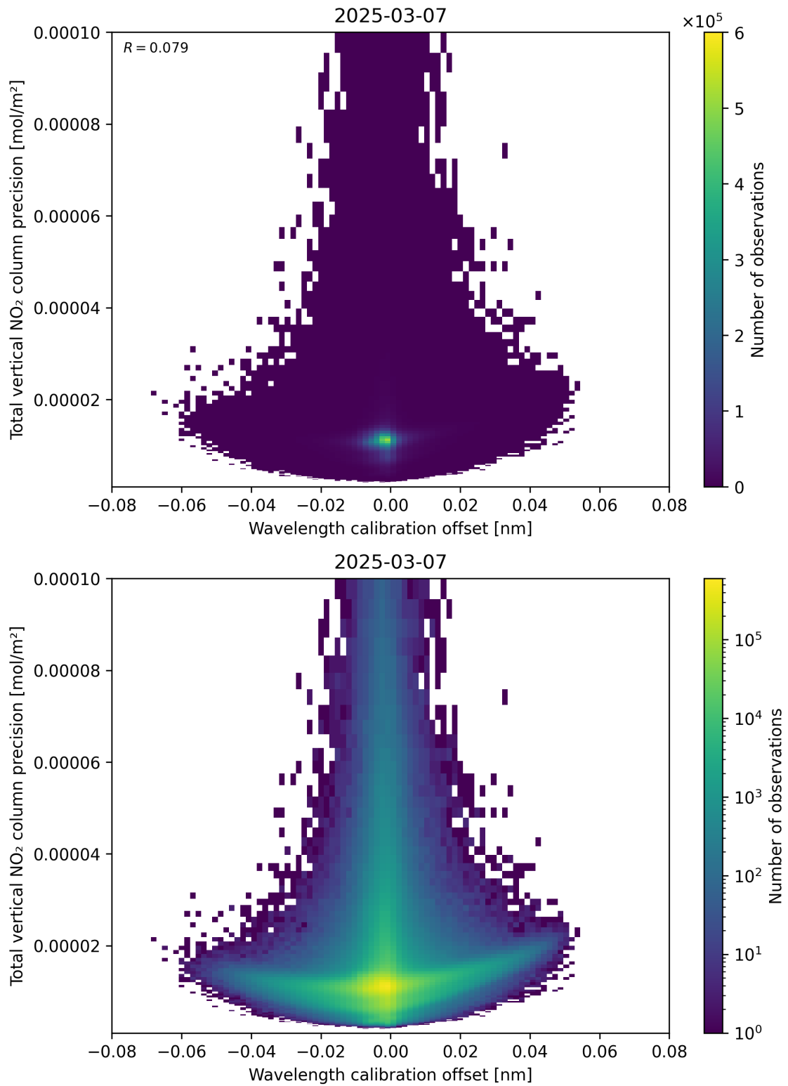
Figure 180: Scatter density plot of “Wavelength calibration offset” against “Total vertical NO 2 column precision” for 2025-03-07 to 2025-03-08.
