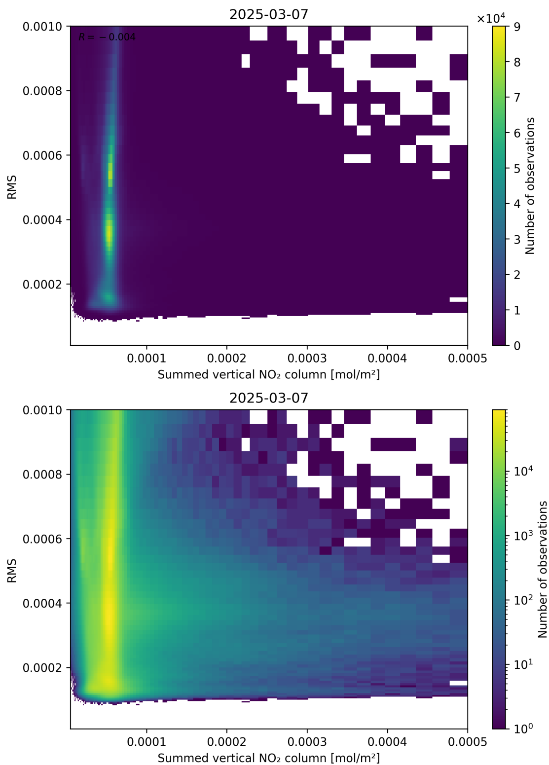
Figure 109: Scatter density plot of “Summed vertical NO 2 column” against “RMS” for 2025-03-07 to 2025-03-08.
