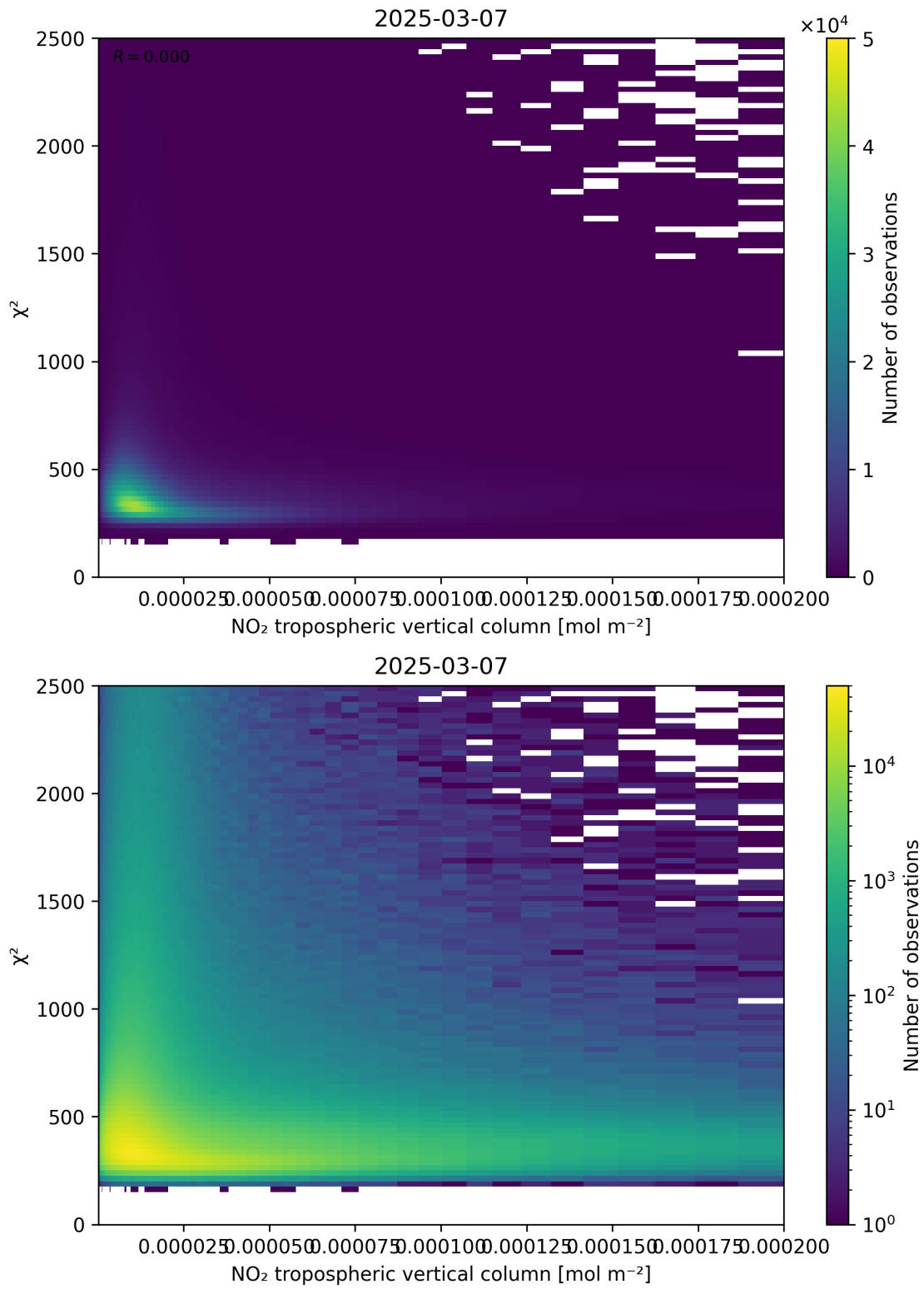
Figure 124: Scatter density plot of “NO 2 tropospheric vertical column” against “ \chi^2 ” for 2025-03-07 to 2025-03-08.
