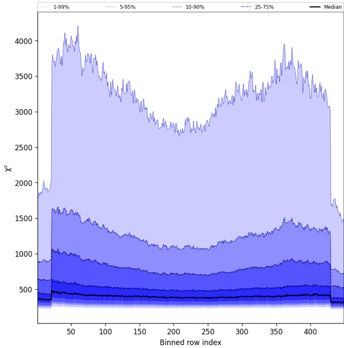
Figure 59: Along track statistics of “ \chi^2 ” for 2025-03-07 to 2025-03-08
