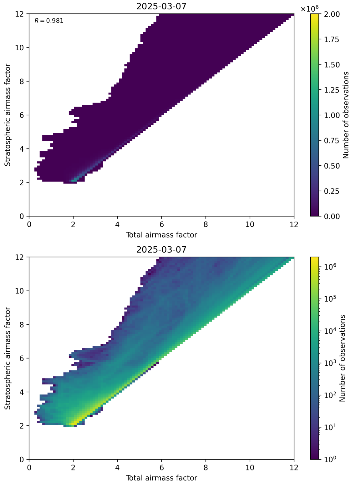
Figure 62: Scatter density plot of “Total airmass factor” against “Stratospheric airmass factor” for 2025-03-07 to 2025-03-08.
