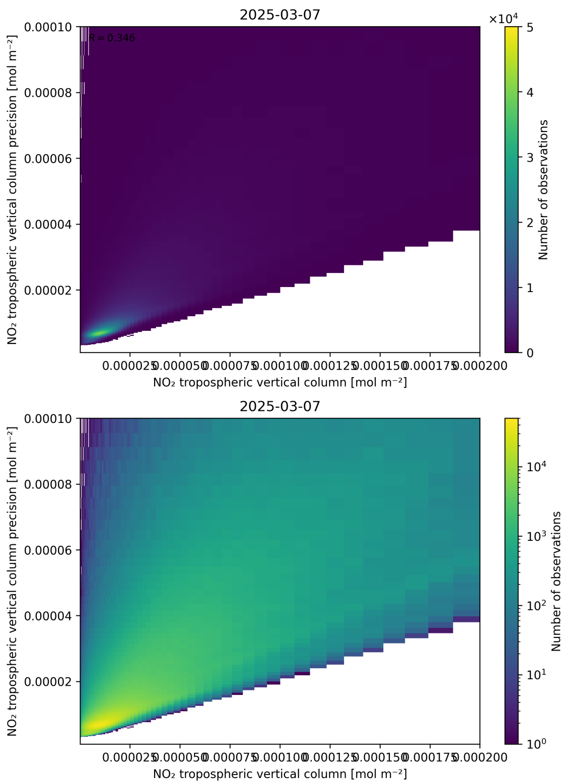
Figure 130: Scatter density plot of “NO 2 tropospheric vertical column” against “NO 2 tropospheric vertical column precision” for 2025-03-07 to 2025-03-08.
