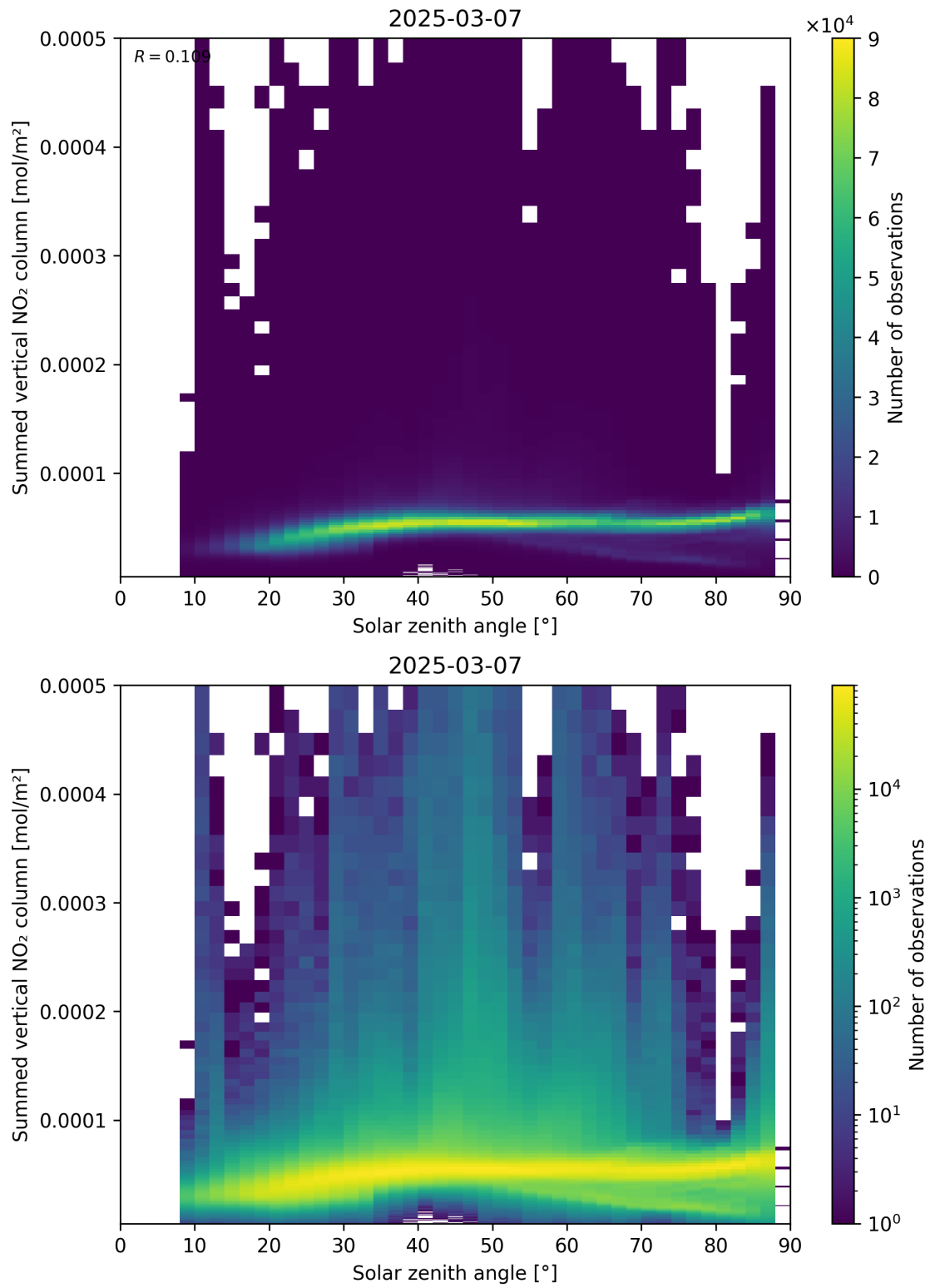
Figure 151: Scatter density plot of “Solar zenith angle” against “Summed vertical NO 2 column” for 2025-03-07 to 2025-03-08.
