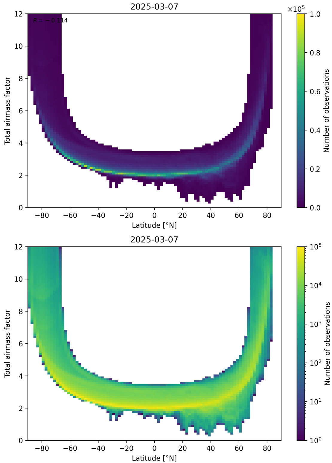
Figure 84: Scatter density plot of “Latitude” against “Total airmass factor” for 2025-03-07 to 2025-03-08.
