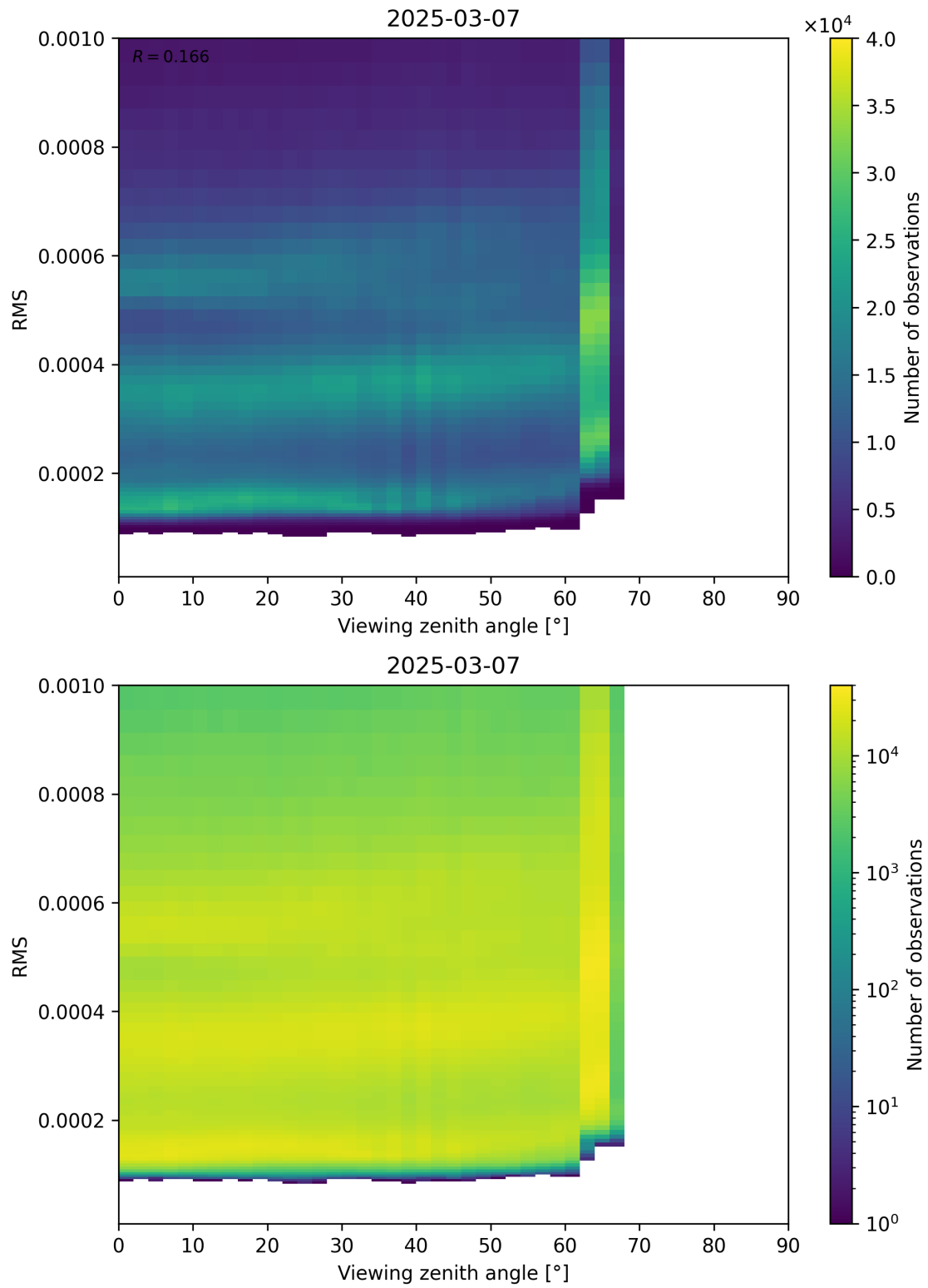
Figure 171: Scatter density plot of “Viewing zenith angle” against “RMS” for 2025-03-07 to 2025-03-08.
