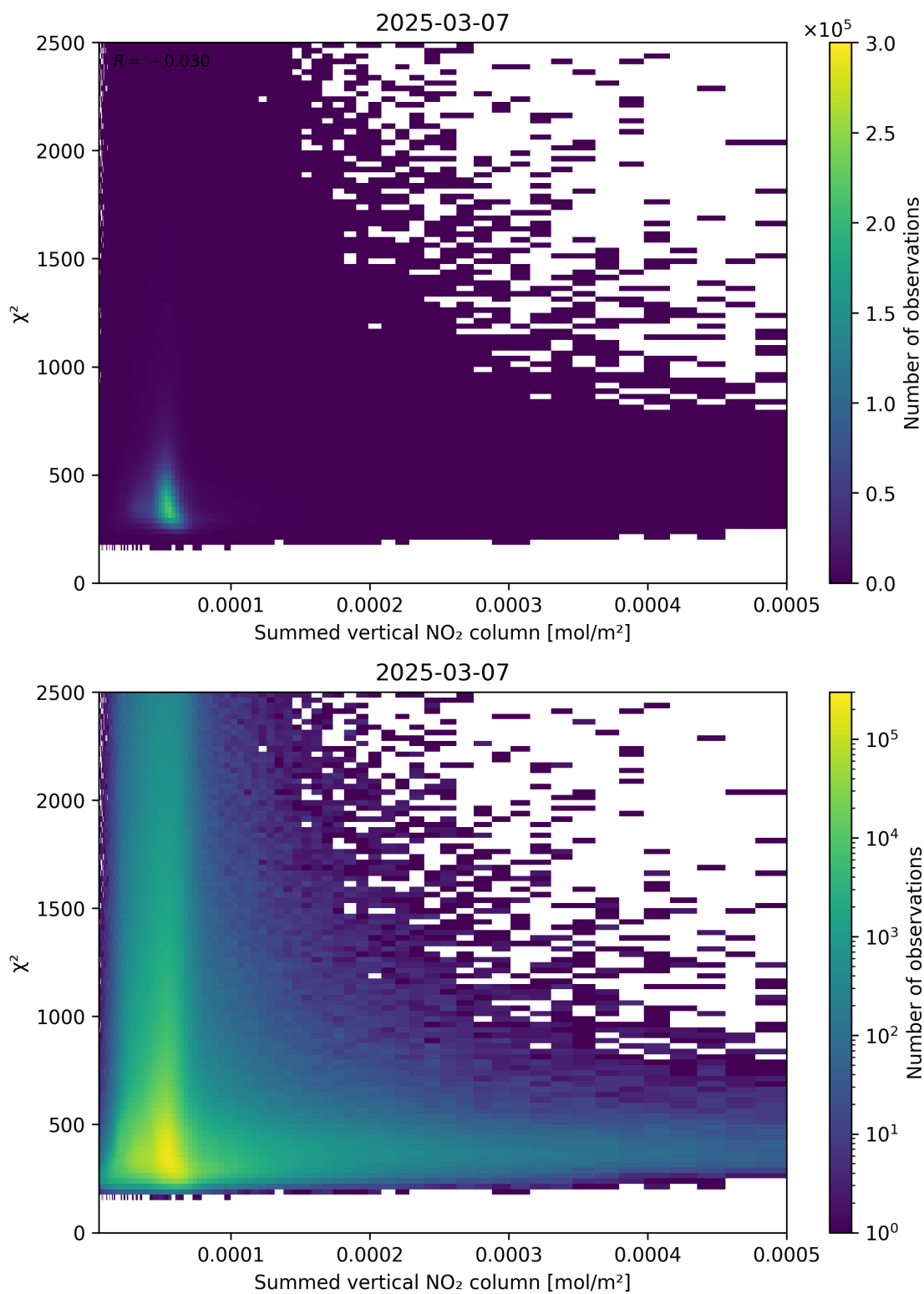
Figure 104: Scatter density plot of “Summed vertical NO 2 column” against “ \chi^2 ” for 2025-03-07 to 2025-03-08.
