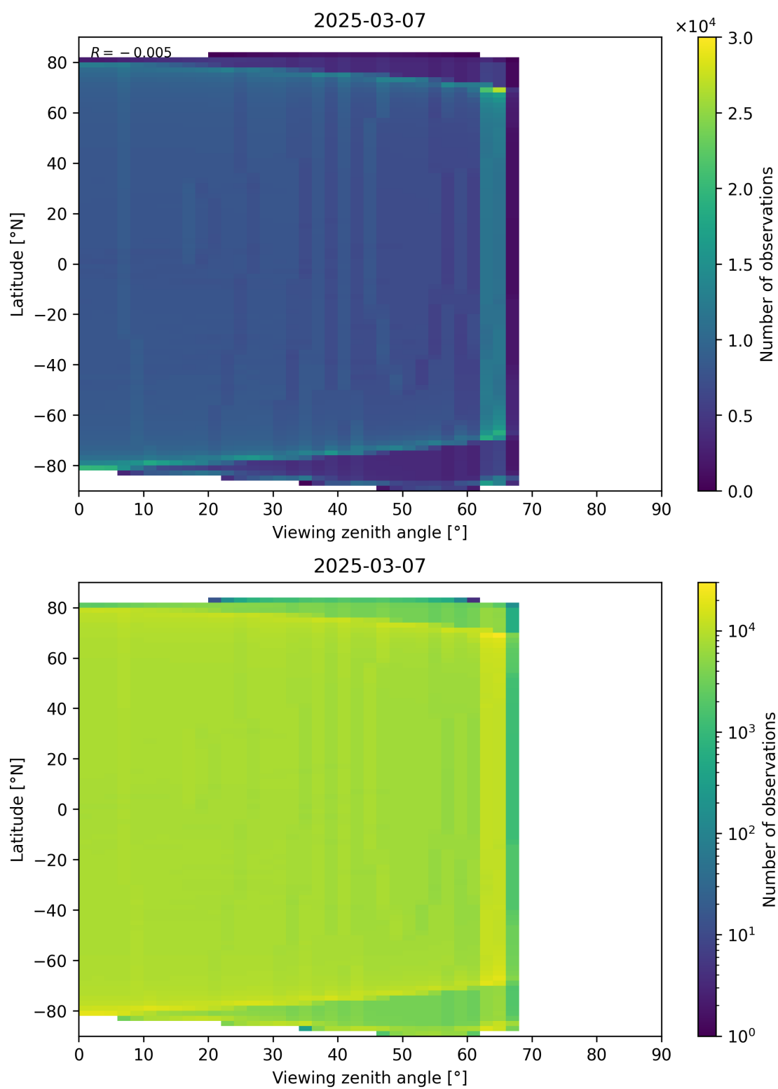
Figure 163: Scatter density plot of “Viewing zenith angle” against “Latitude” for 2025-03-07 to 2025-03-08.
