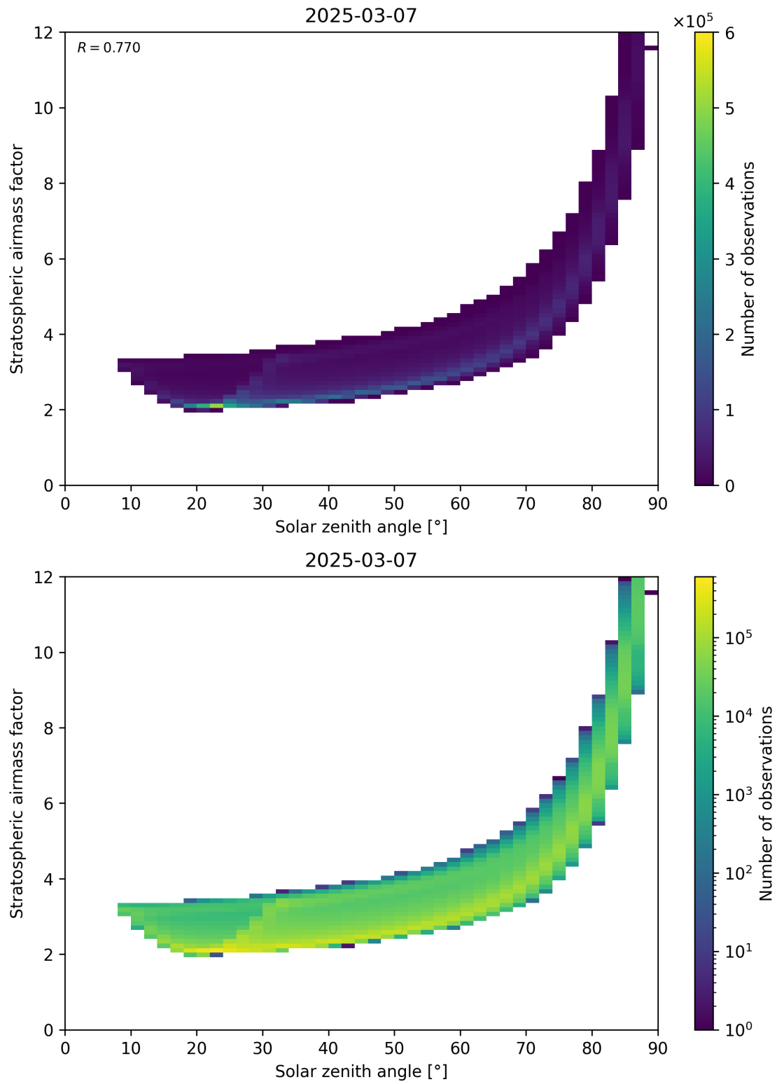
Figure 145: Scatter density plot of “Solar zenith angle” against “Stratospheric airmass factor” for 2025-03-07 to 2025-03-08.
