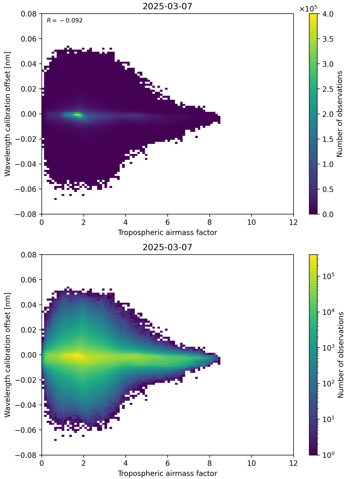
Figure 80: Scatter density plot of “Tropospheric airmass factor” against “Wavelength calibration offset” for 2025-03-07 to 2025-03-08.
