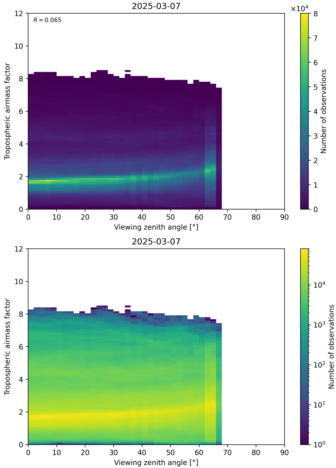
Figure 161: Scatter density plot of “Viewing zenith angle” against “Tropospheric airmass factor” for 2025-03-07 to 2025-03-08.
