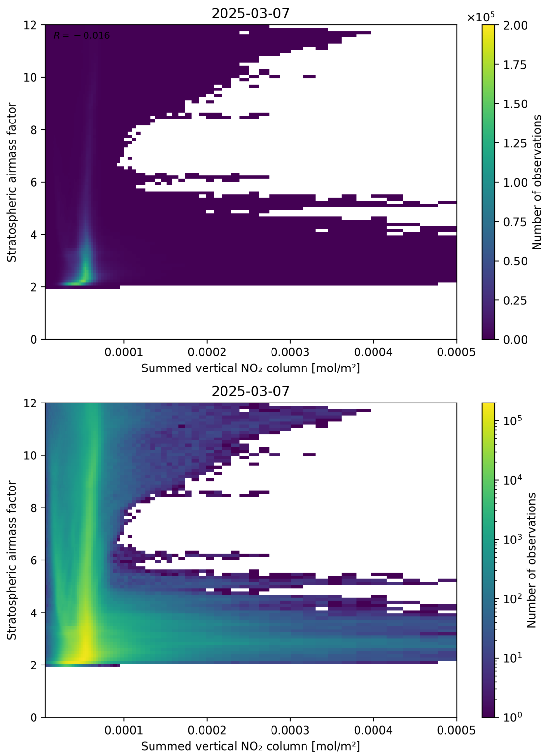
Figure 103: Scatter density plot of “Summed vertical NO 2 column” against “Stratospheric air mass factor” for 2025-03-07 to 2025-03-08.
