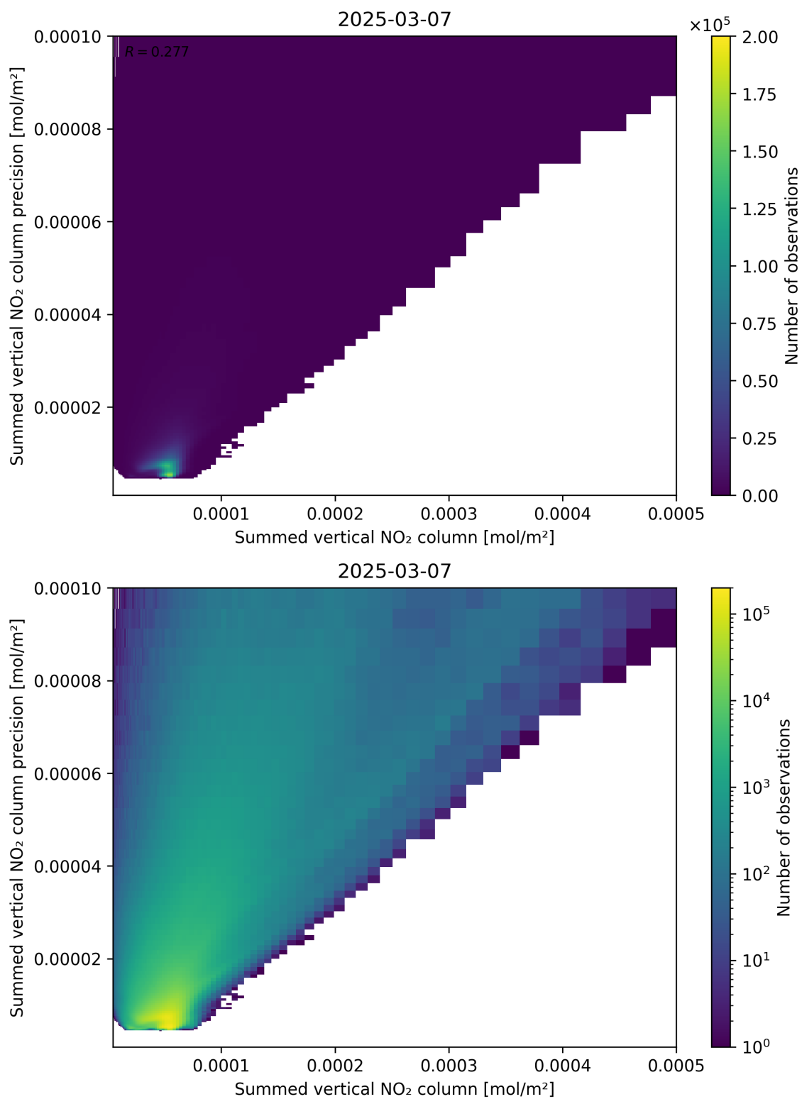
Figure 105: Scatter density plot of “Summed vertical NO 2 column” against “Summed vertical NO 2 column precision” for 2025-03-07 to 2025-03-08.
