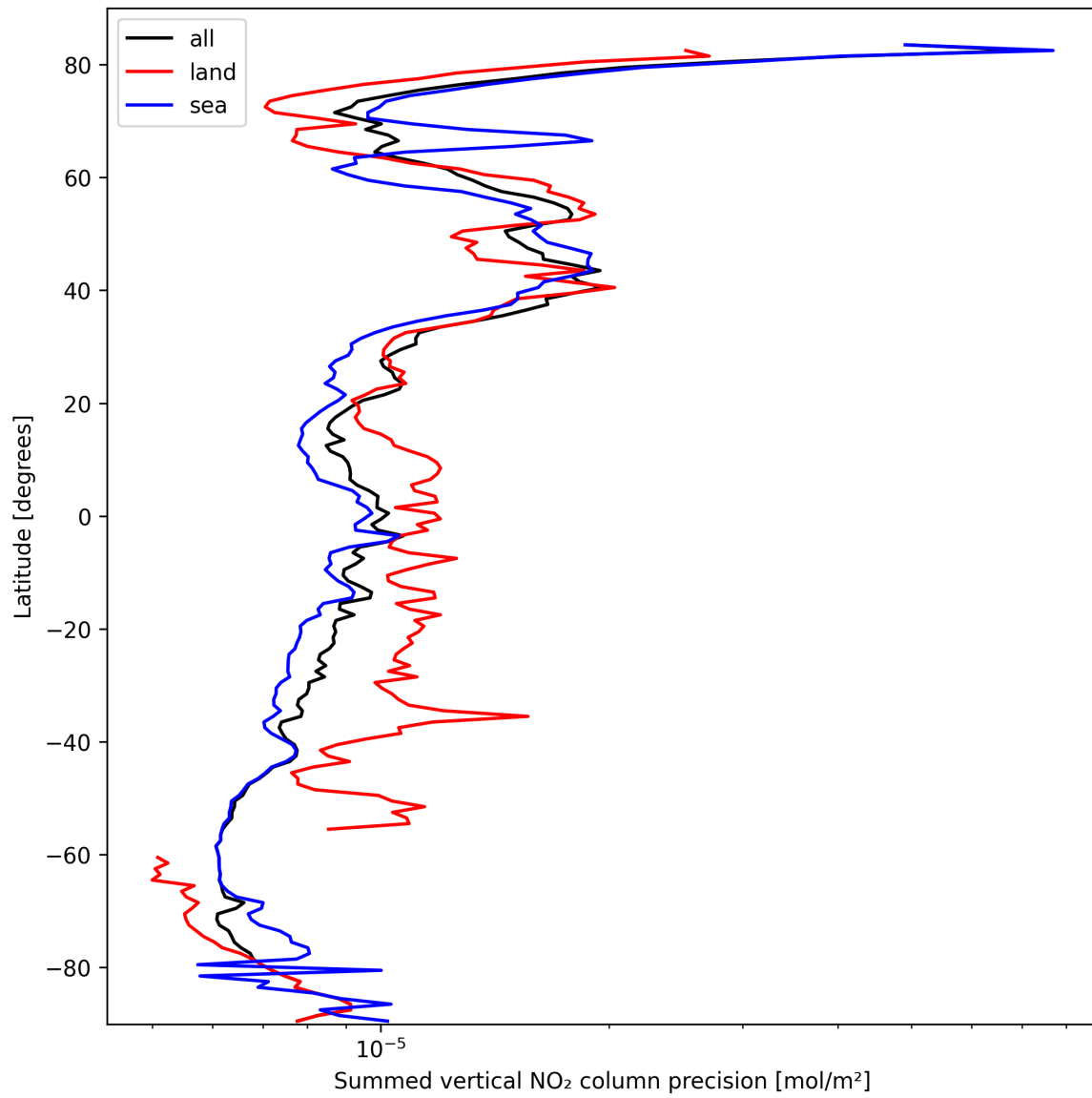
Figure 24: Zonal average of “Summed vertical NO 2 column precision” for 2025-03-07 to 2025-03-08.
