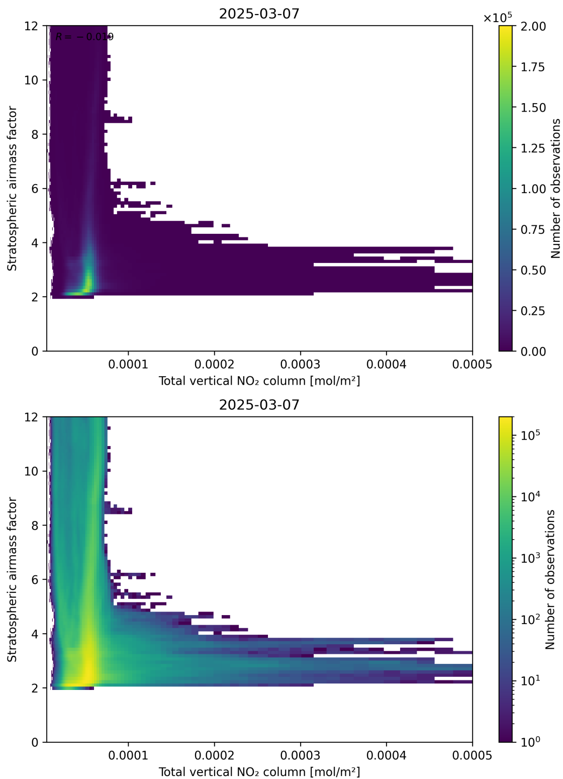
Figure 110: Scatter density plot of “Total vertical NO 2 column” against “Stratospheric air mass factor” for 2025-03-07 to 2025-03-08.
