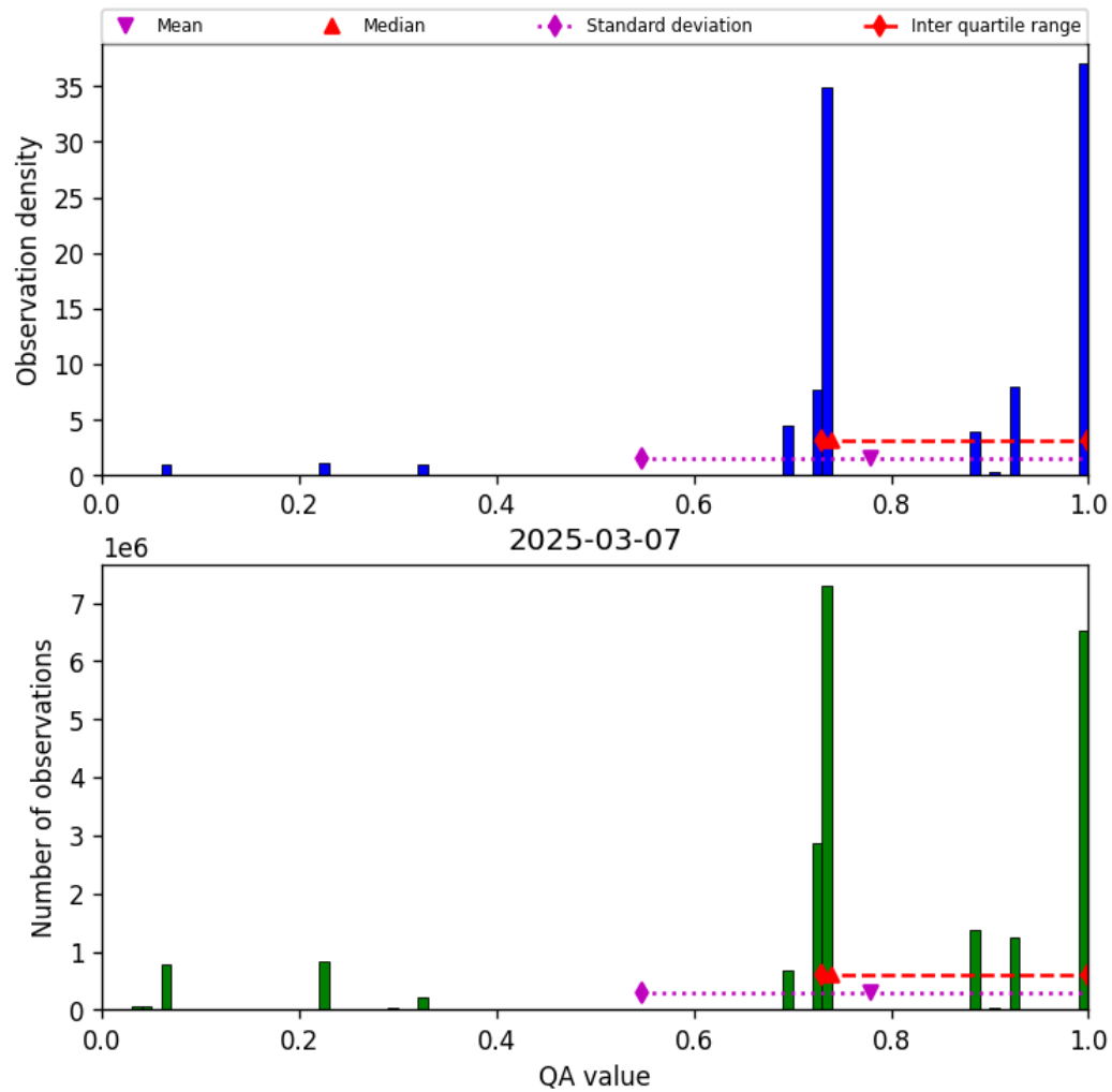
Figure 28: Histogram of “QA value” for 2025-03-07 to 2025-03-08
