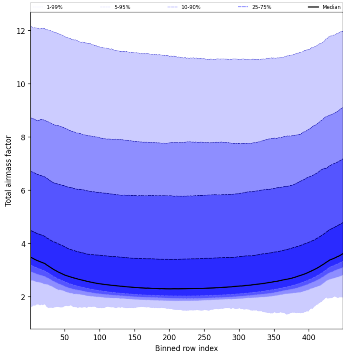
Figure 49: Along track statistics of “Total airmass factor” for 2025-03-07 to 2025-03-08
