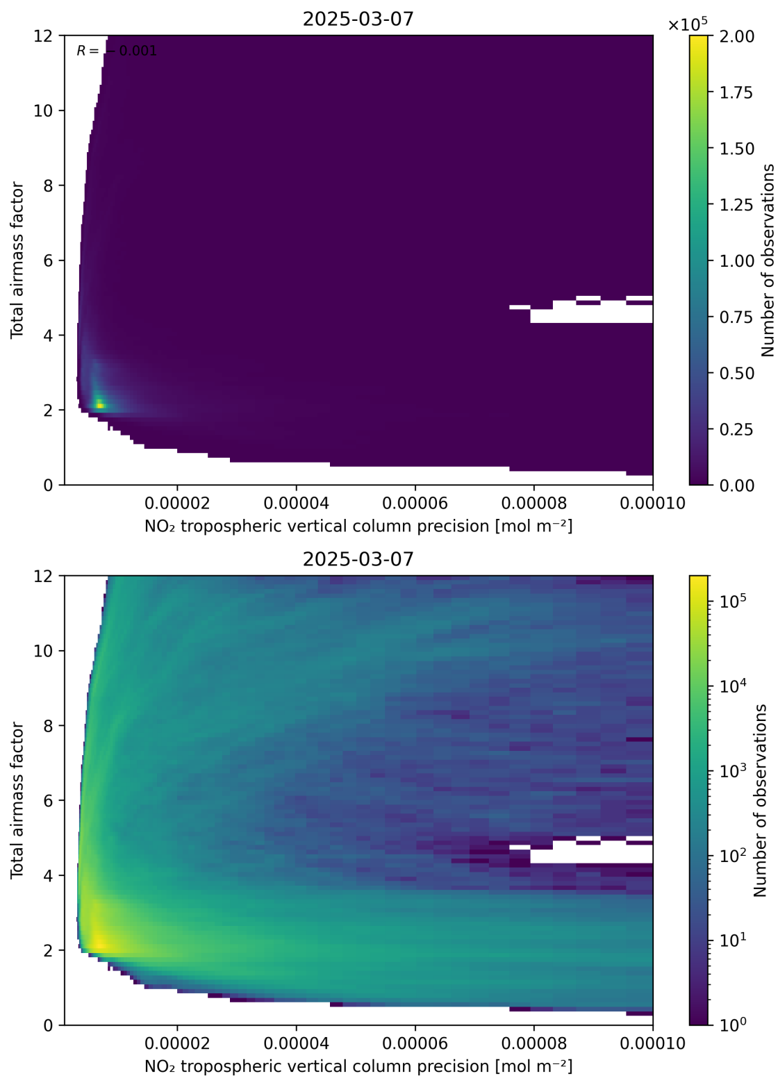
Figure 132: Scatter density plot of “NO 2 tropospheric vertical column precision” against “Total air mass factor” for 2025-03-07 to 2025-03-08.
