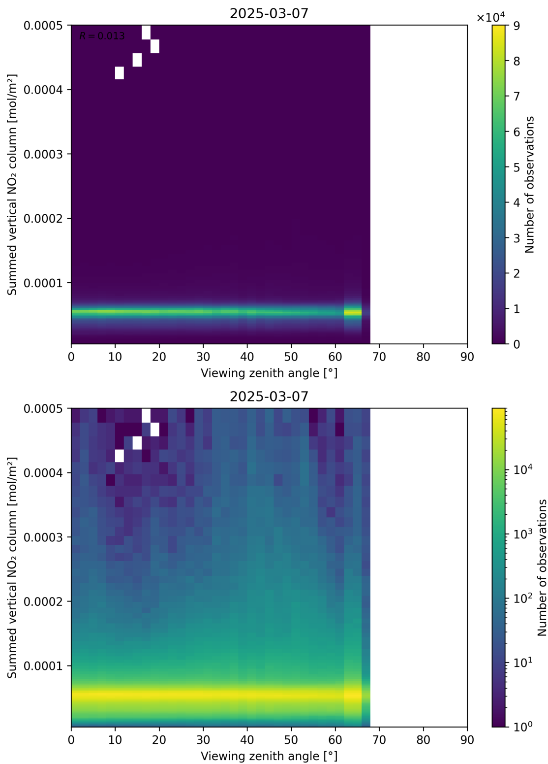
Figure 165: Scatter density plot of “Viewing zenith angle” against “Summed vertical NO 2 column” for 2025-03-07 to 2025-03-08.
