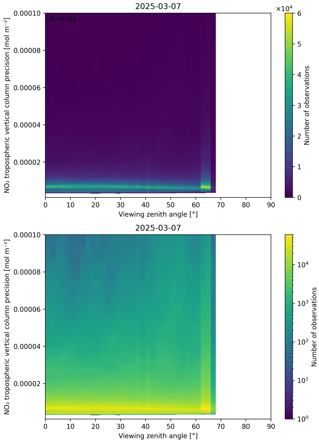
Figure 170: Scatter density plot of “Viewing zenith angle” against “NO 2 tropospheric vertical column precision” for 2025-03-07 to 2025-03-08.
