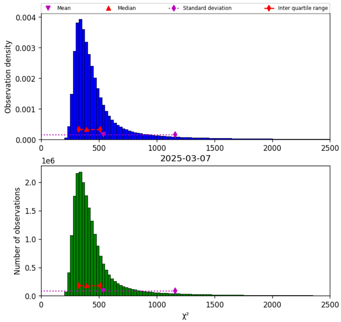
Figure 42: Histogram of " \chi^2 " for 2025-03-07 to 2025-03-08
