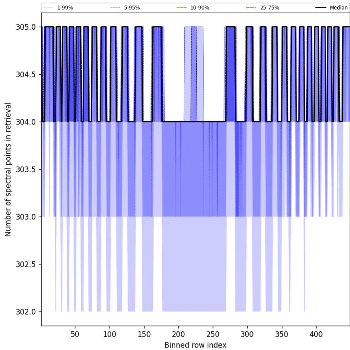
Figure 50: Along track statistics of “Number of spectral points in retrieval” for 2025-03-07 to 2025-03-08
