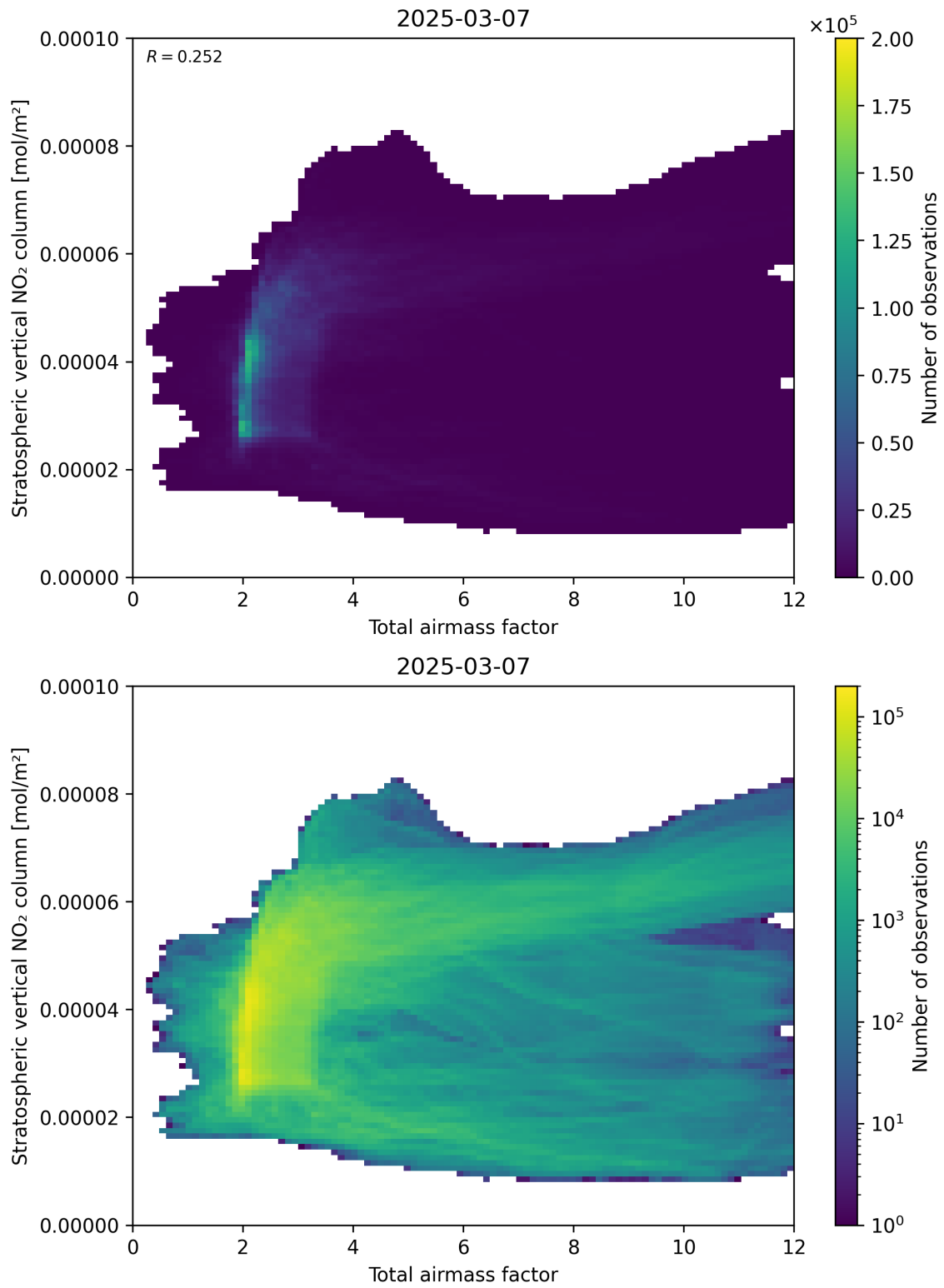
Figure 64: Scatter density plot of “Total airmass factor” against “Stratospheric vertical \text{NO}_2 column” for 2025-03-07 to 2025-03-08.
