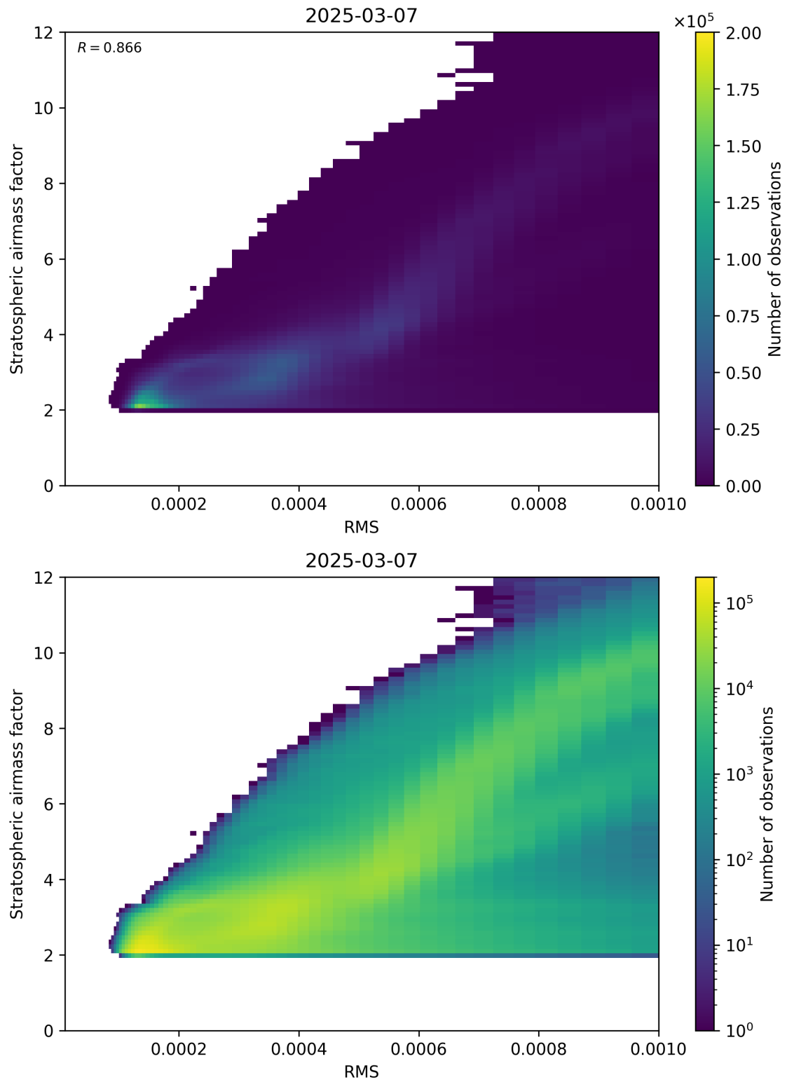
Figure 144: Scatter density plot of “RMS” against “Stratospheric airmass factor” for 2025-03-07 to 2025-03-08.
