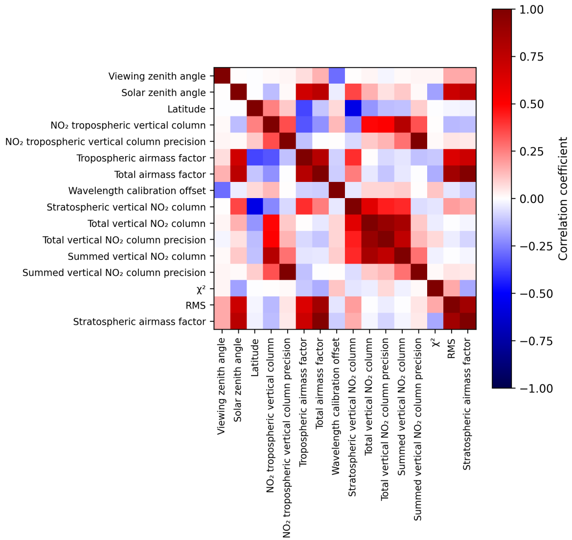
Figure 2: Map of correlation matrix for 2025-03-07 to 2025-03-08.
