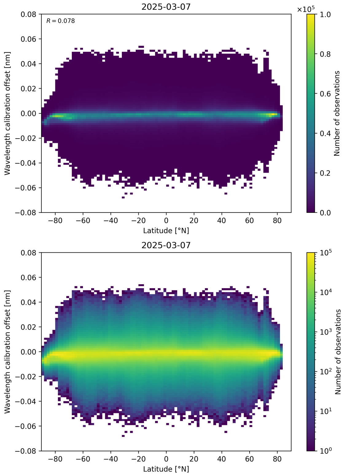
Figure 95: Scatter density plot of “Latitude” against “Wavelength calibration offset” for 2025-03-07 to 2025-03-08.
