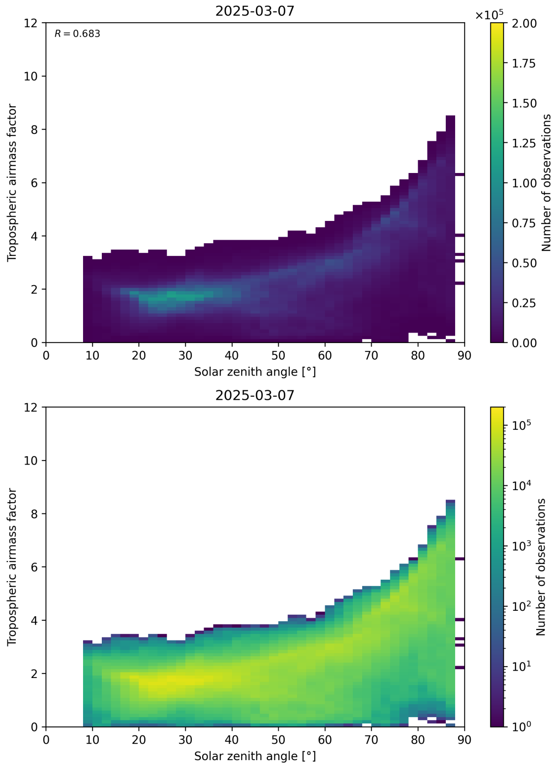
Figure 147: Scatter density plot of “Solar zenith angle” against “Tropospheric airmass factor” for 2025-03-07 to 2025-03-08.
