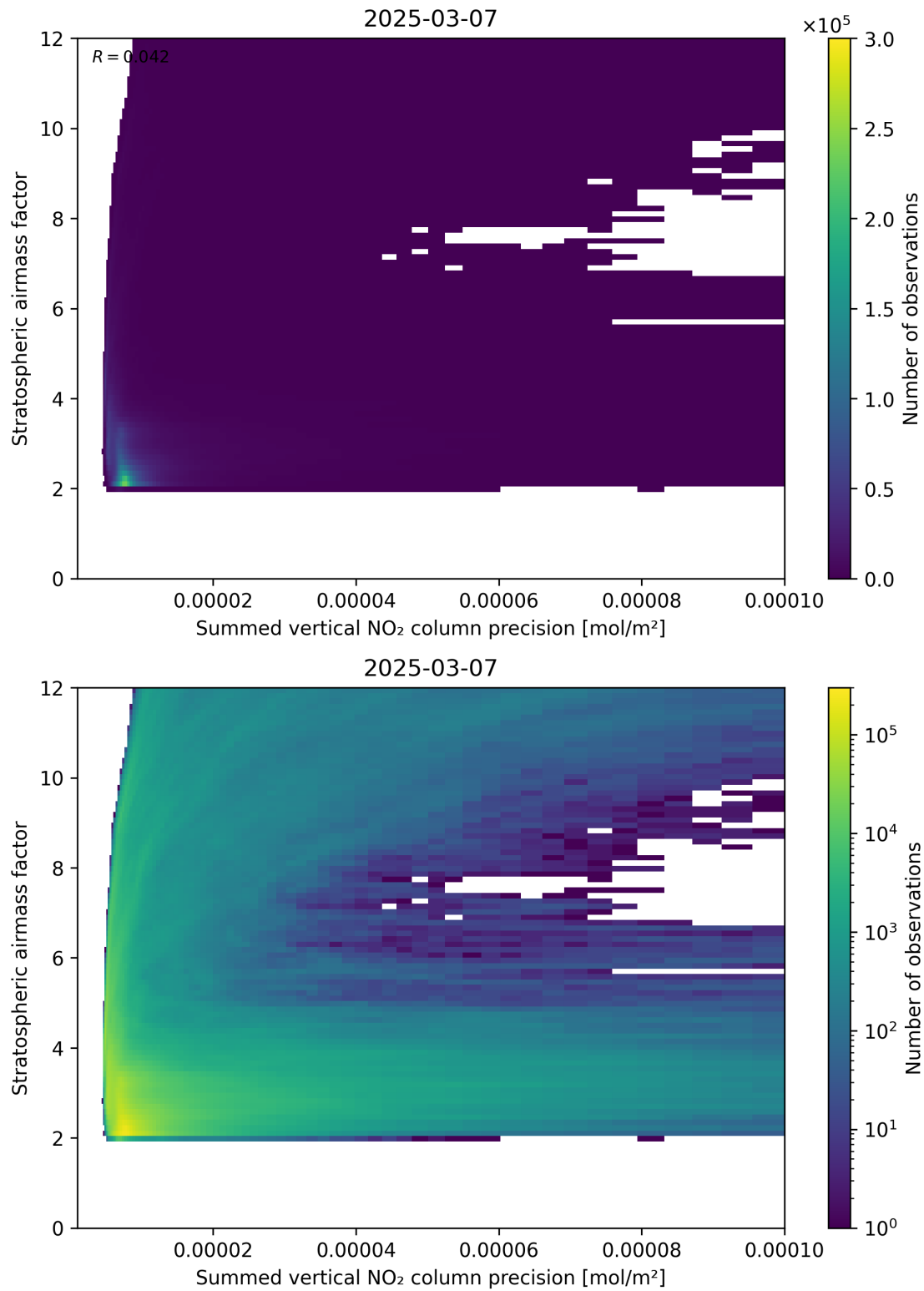
Figure 106: Scatter density plot of “Summed vertical NO 2 column precision” against “Stratospheric airmass factor” for 2025-03-07 to 2025-03-08.
