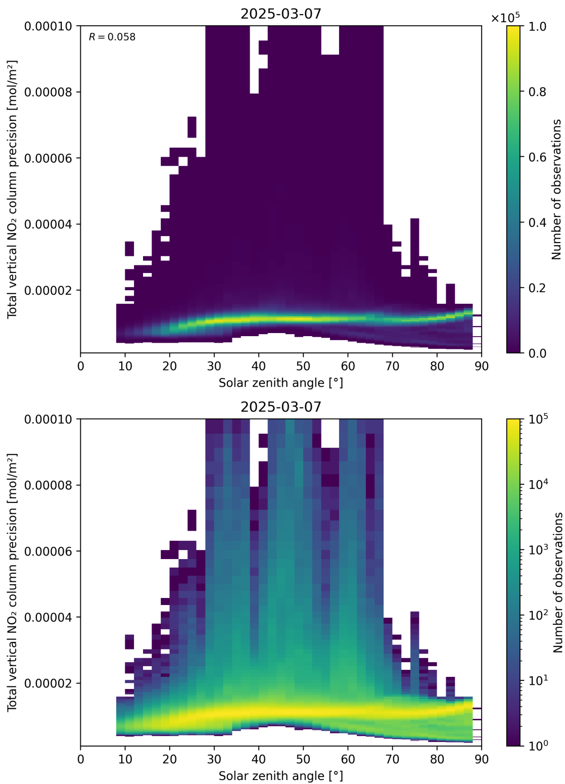
Figure 154: Scatter density plot of “Solar zenith angle” against “Total vertical NO 2 column precision” for 2025-03-07 to 2025-03-08.
