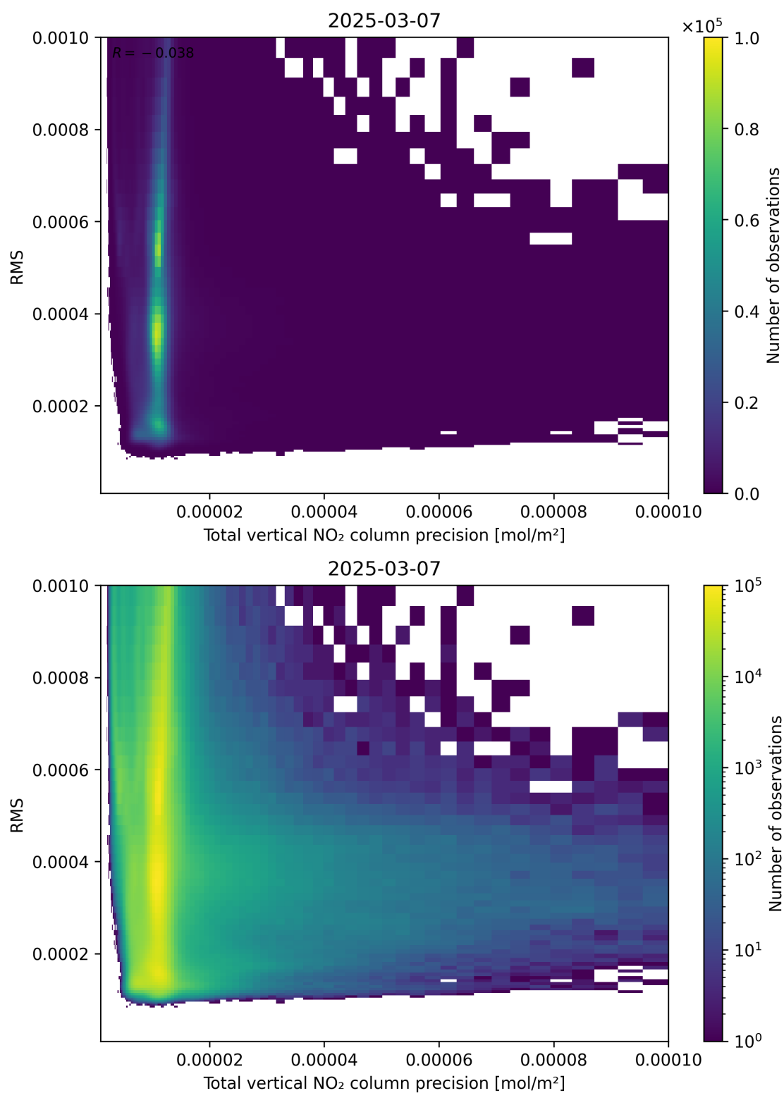
Figure 119: Scatter density plot of “Total vertical NO 2 column precision” against “RMS” for 2025-03-07 to 2025-03-08.
