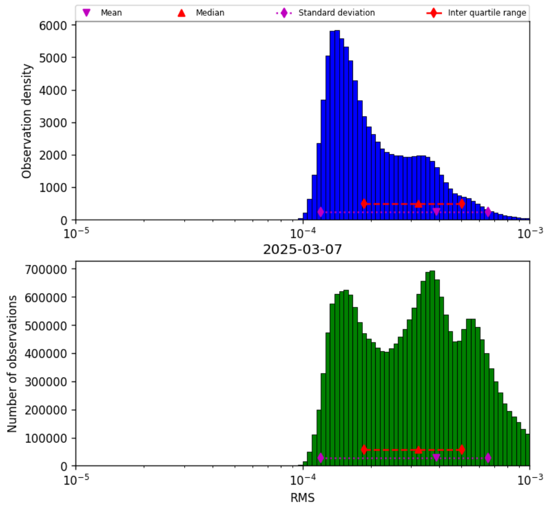
Figure 43: Histogram of “RMS” for 2025-03-07 to 2025-03-08
