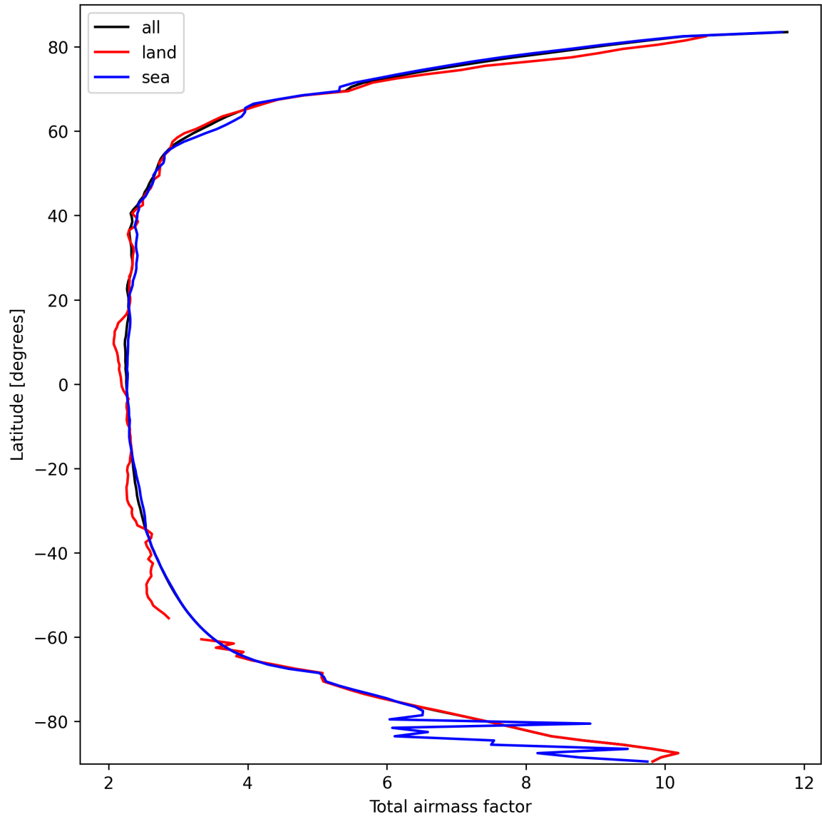
Figure 15: Zonal average of “Total airmass factor” for 2025-03-07 to 2025-03-08.
