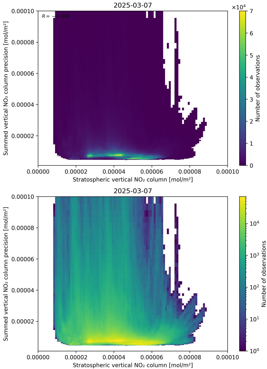
Figure 99: Scatter density plot of “Stratospheric vertical NO 2 column” against “Summed vertical NO 2 column precision” for 2025-03-07 to 2025-03-08.
