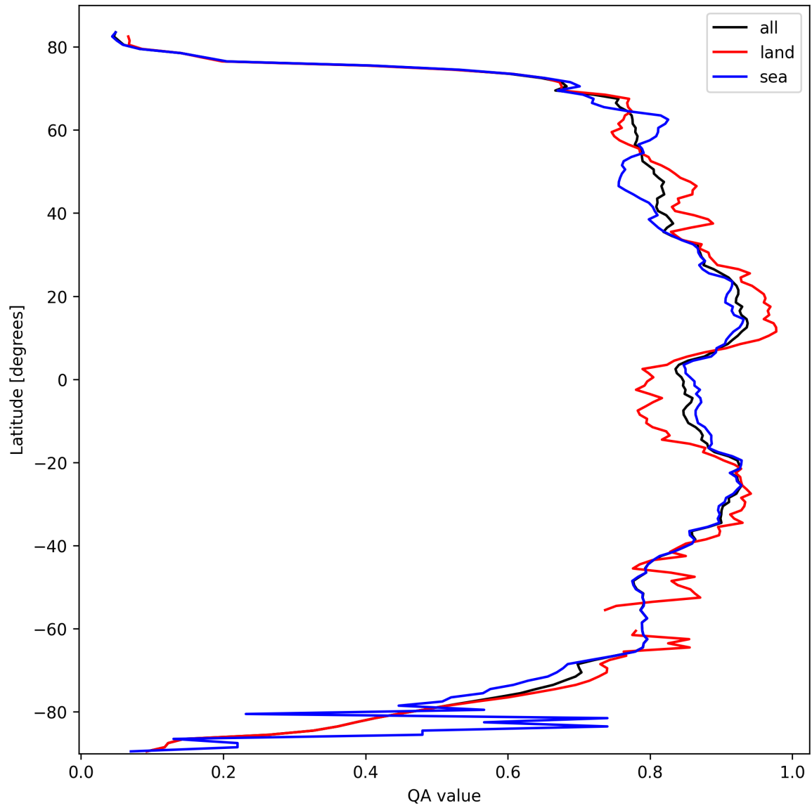
Figure 11: Zonal average of “QA value” for 2025-03-07 to 2025-03-08.
