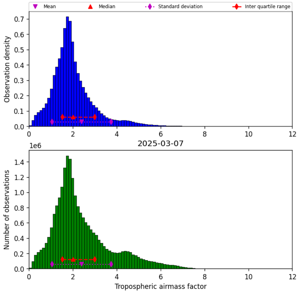
Figure 31: Histogram of “Tropospheric airmass factor” for 2025-03-07 to 2025-03-08
