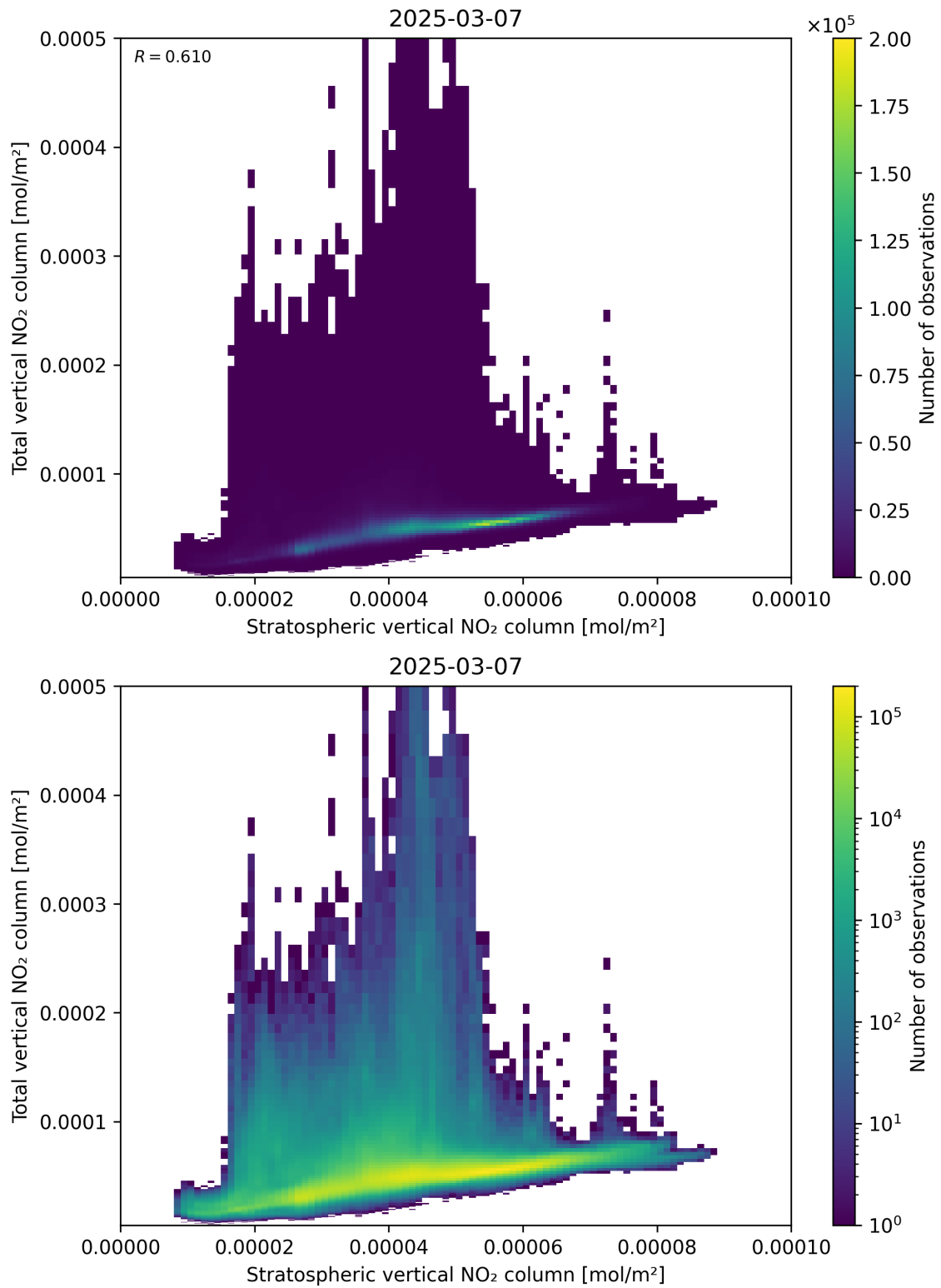
Figure 100: Scatter density plot of “Stratospheric vertical NO 2 column” against “Total vertical NO 2 column” for 2025-03-07 to 2025-03-08.
