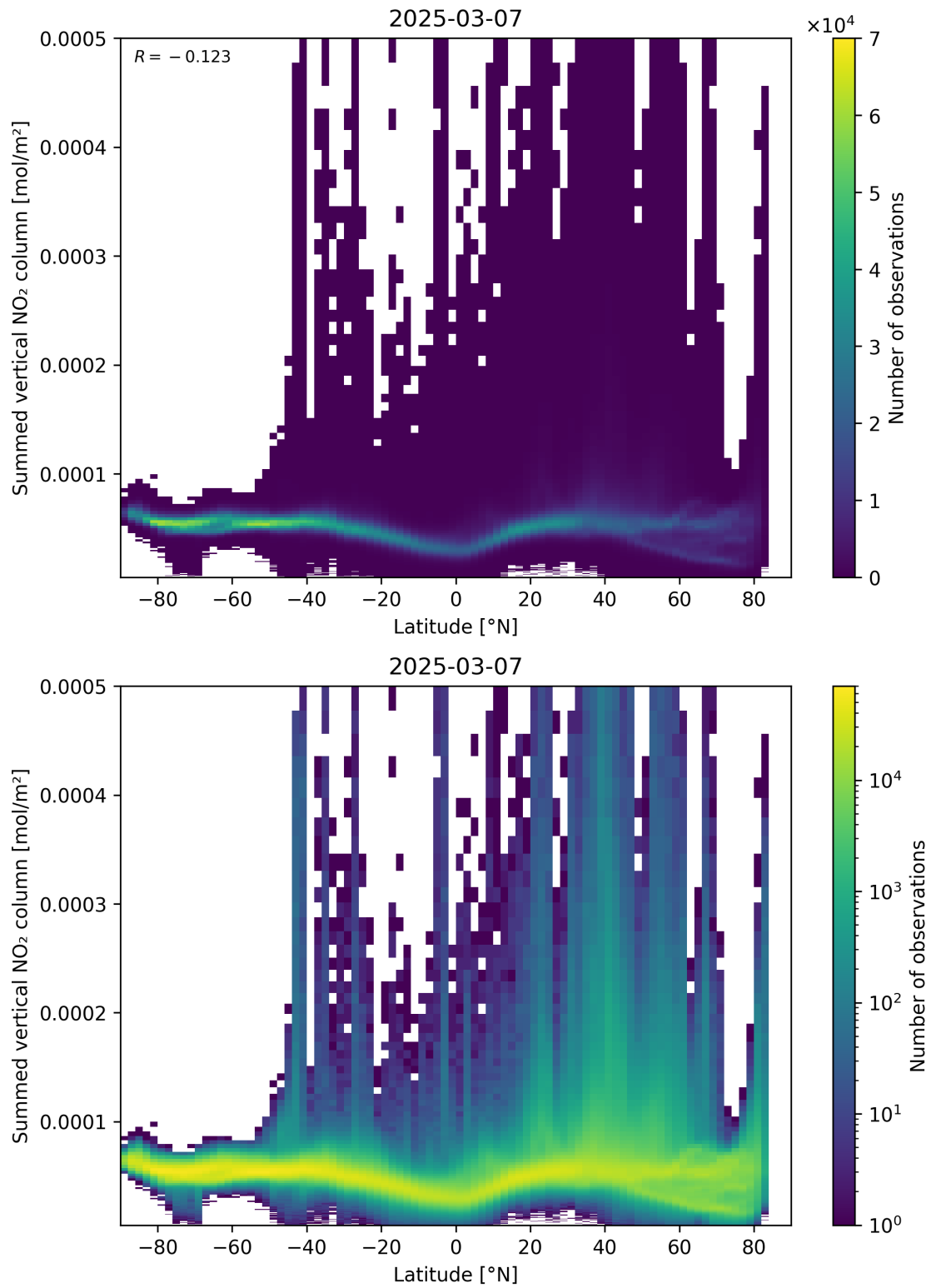
Figure 88: Scatter density plot of “Latitude” against “Summed vertical NO 2 column” for 2025-03-07 to 2025-03-08.
