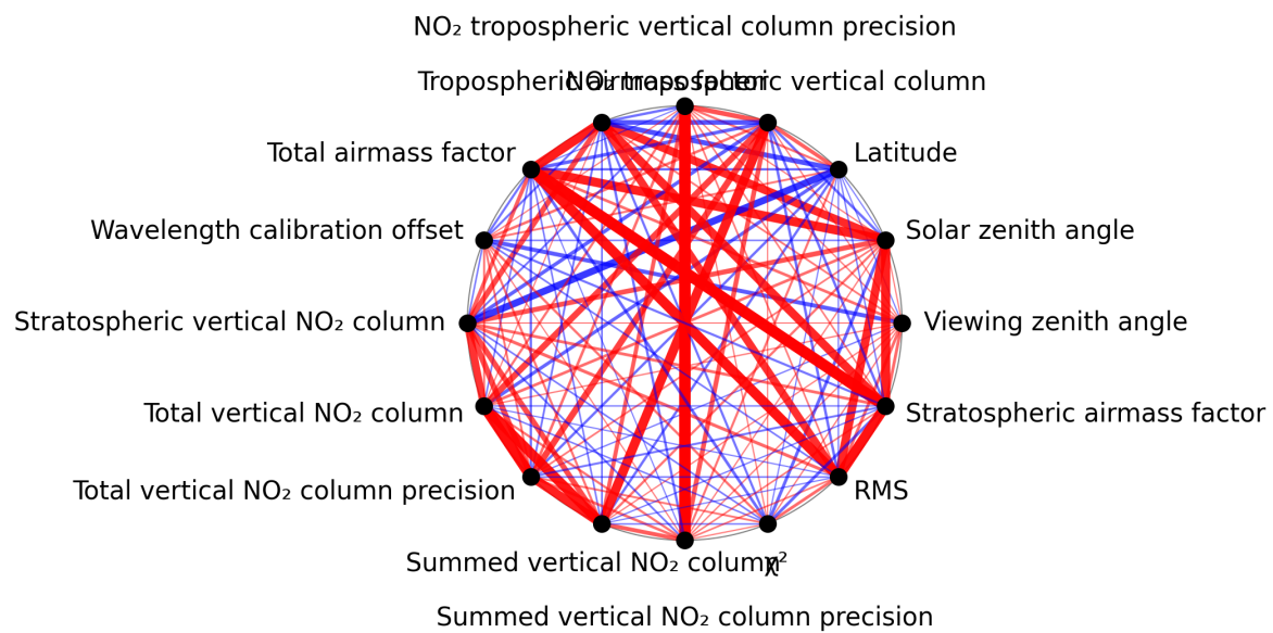
Figure 1: Map of correlation graph for 2025-03-07 to 2025-03-08.
