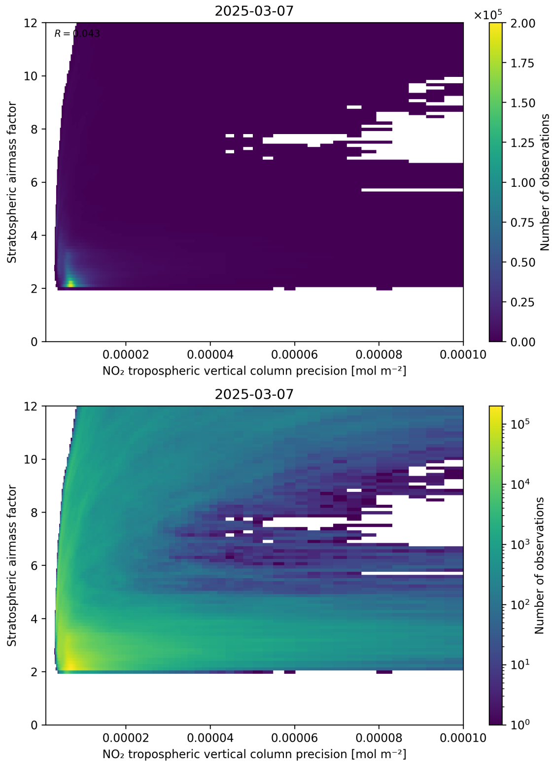
Figure 131: Scatter density plot of “NO 2 tropospheric vertical column precision” against “Stratospheric airmass factor” for 2025-03-07 to 2025-03-08.
