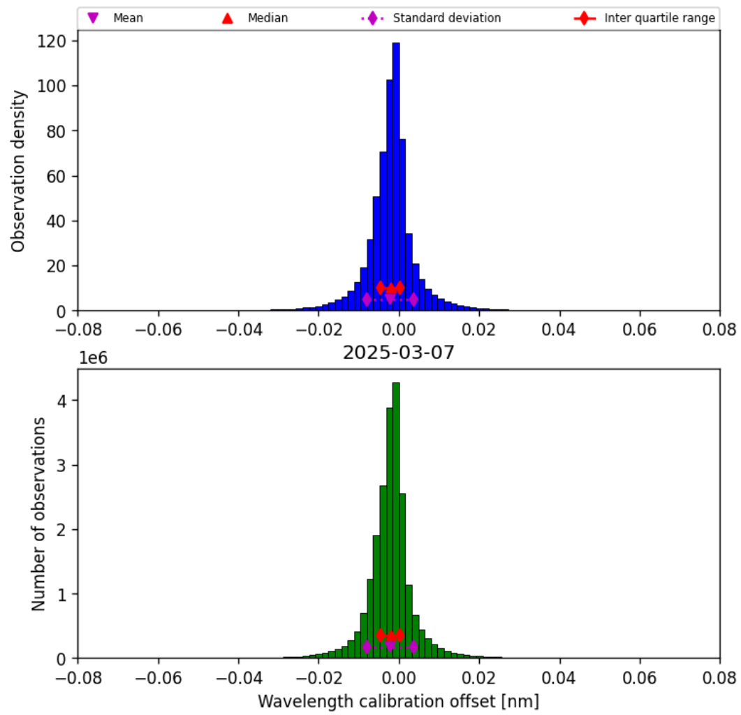
Figure 35: Histogram of “Wavelength calibration offset” for 2025-03-07 to 2025-03-08
