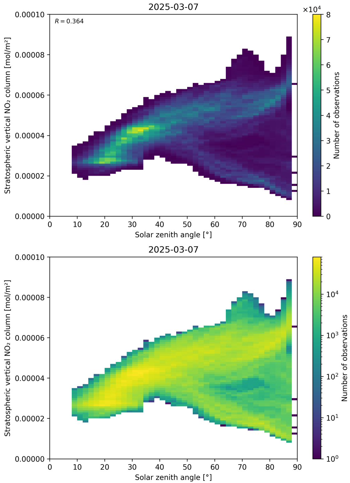
Figure 150: Scatter density plot of “Solar zenith angle” against “Stratospheric vertical NO 2 column” for 2025-03-07 to 2025-03-08.
