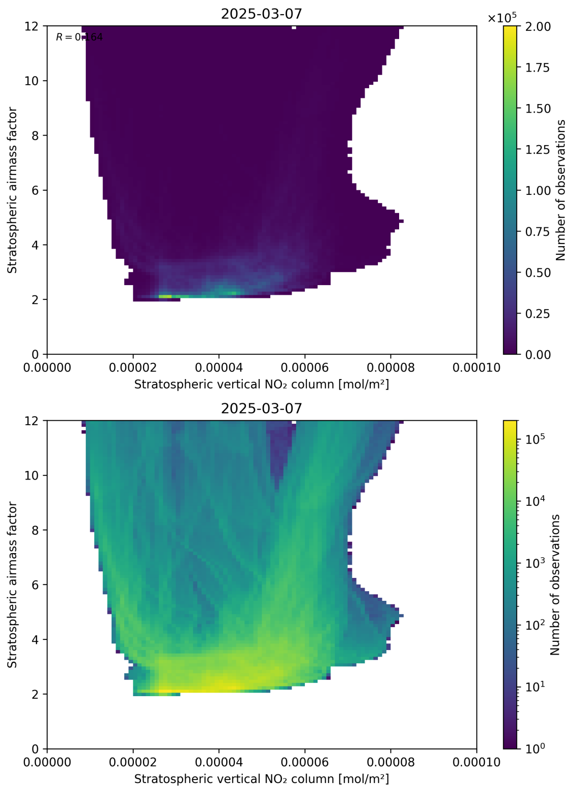
Figure 96: Scatter density plot of “Stratospheric vertical NO 2 column” against “Stratospheric airmass factor” for 2025-03-07 to 2025-03-08.
