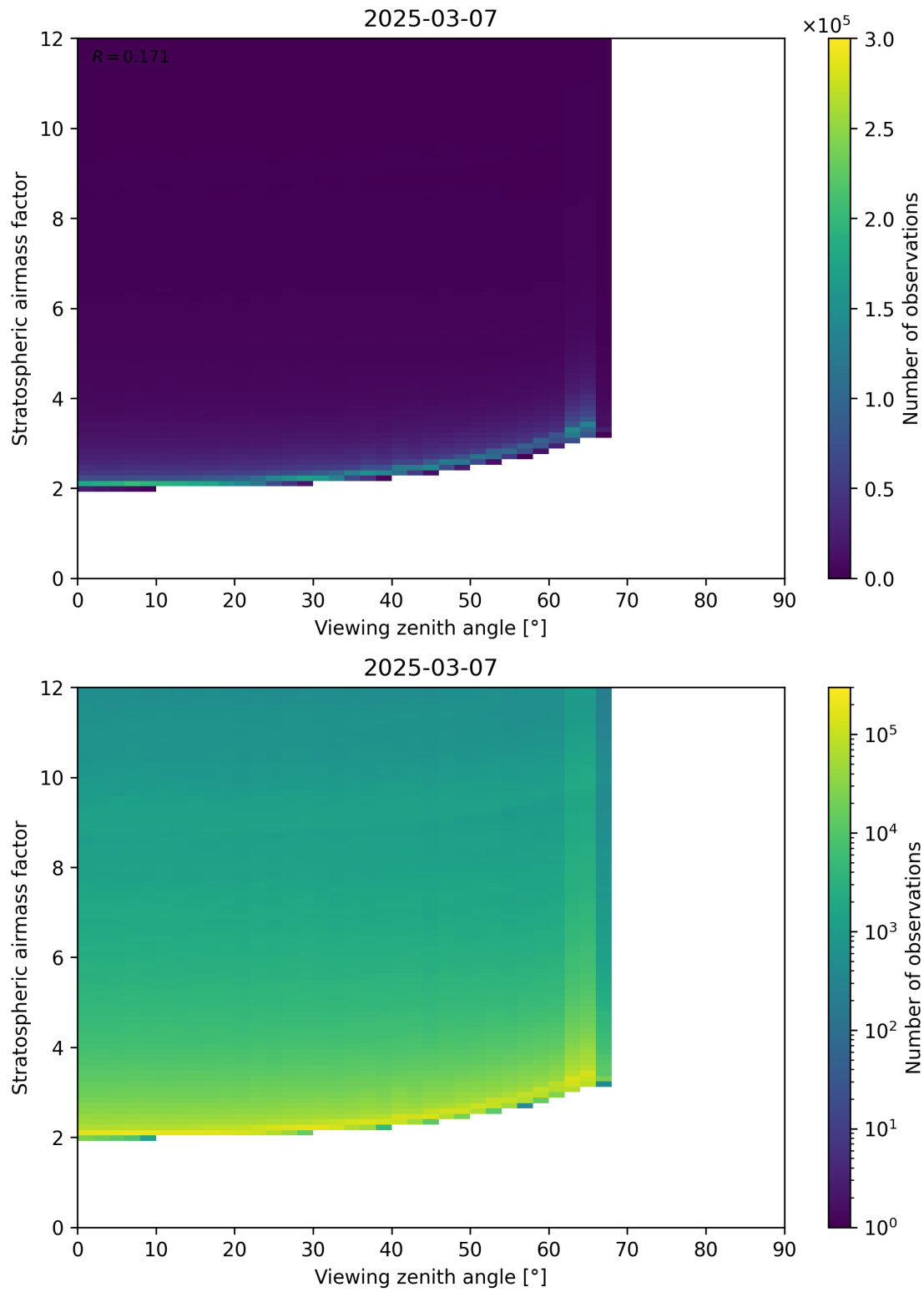
Figure 159: Scatter density plot of “Viewing zenith angle” against “Stratospheric airmass factor” for 2025-03-07 to 2025-03-08.
