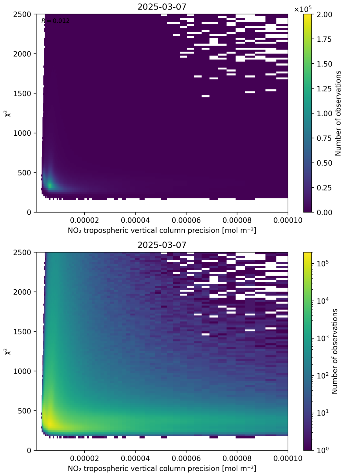
Figure 134: Scatter density plot of “NO 2 tropospheric vertical column precision” against “ \chi^2 ” for 2025-03-07 to 2025-03-08.
