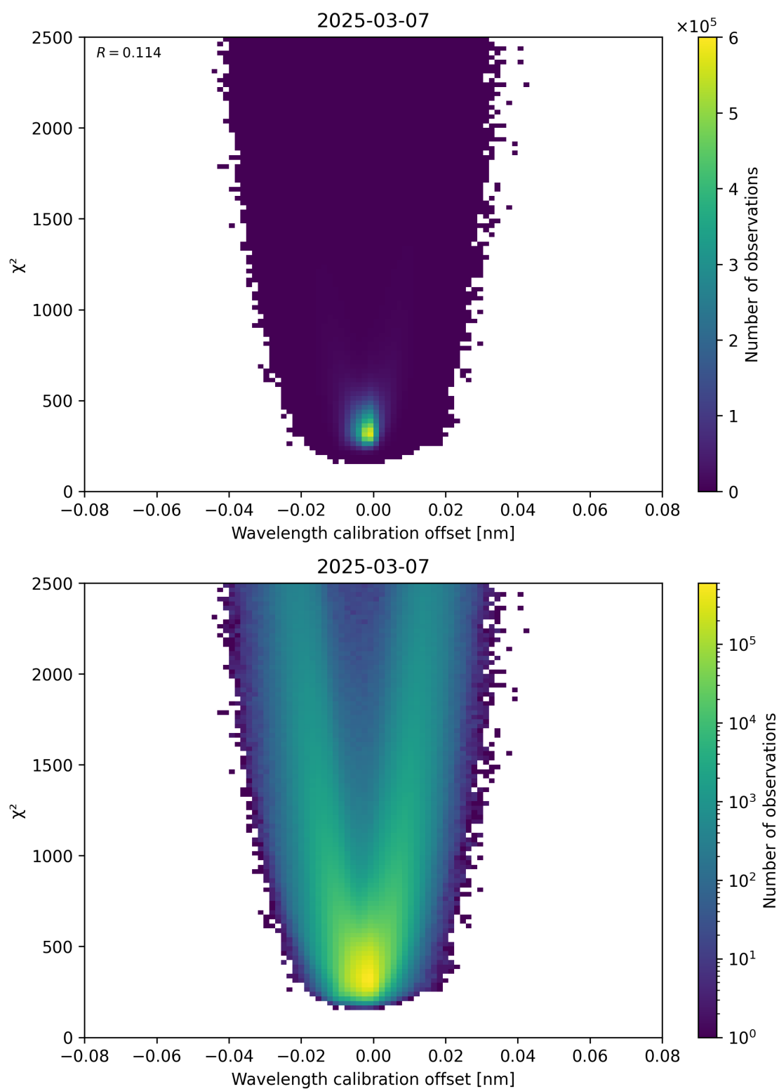
Figure 175: Scatter density plot of “Wavelength calibration offset” against “ \chi^2 ” for 2025-03-07 to 2025-03-08.
