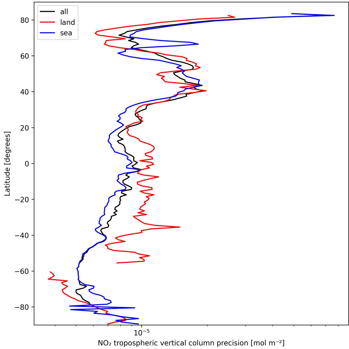
Figure 13: Zonal average of “NO 2 tropospheric vertical column precision” for 2025-03-07 to 2025-03-08.
