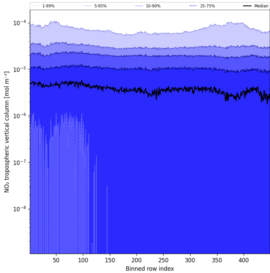
Figure 46: Along track statistics of “NO 2 tropospheric vertical column” for 2025-03-07 to 2025-03-08
