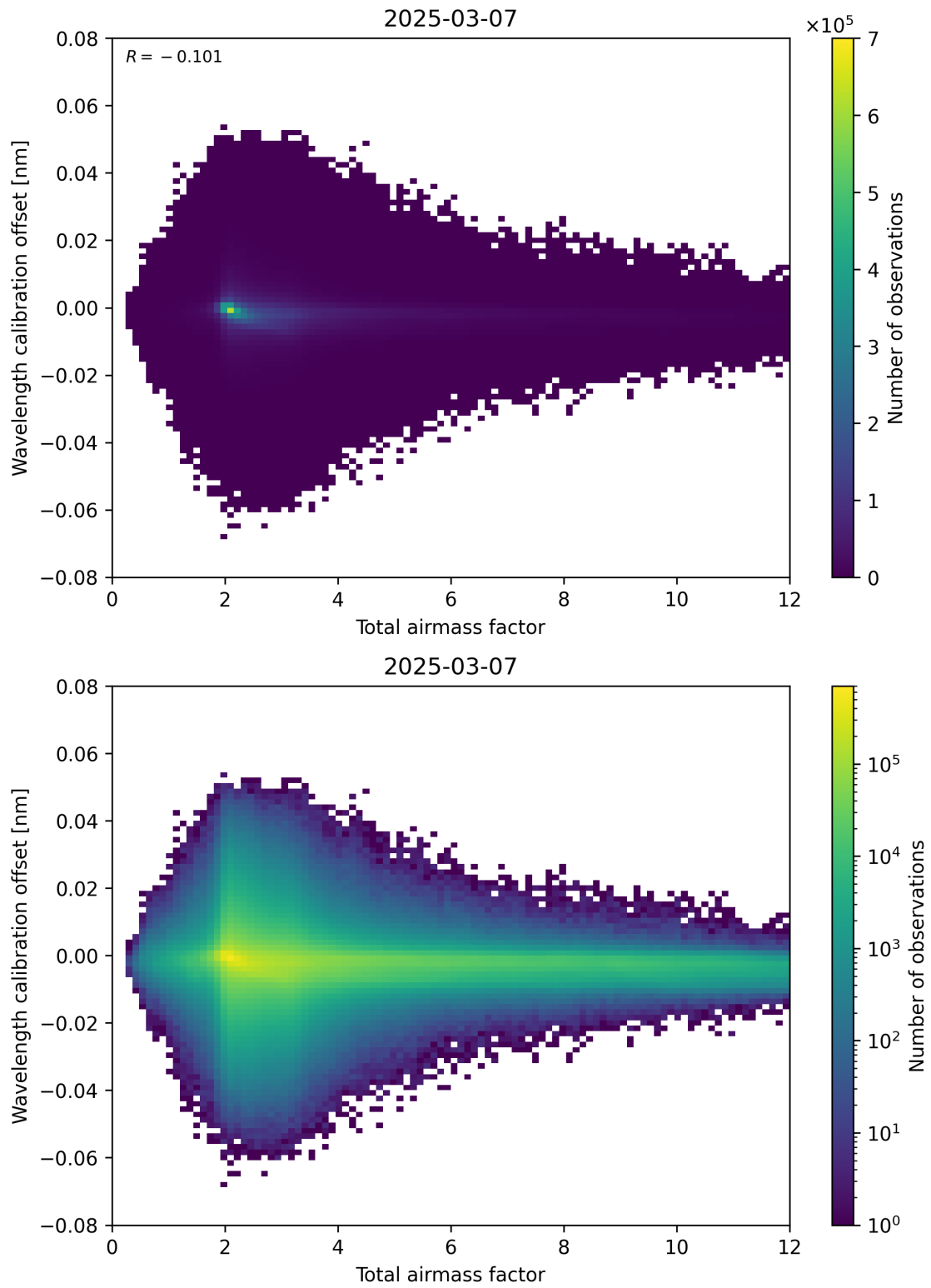
Figure 70: Scatter density plot of “Total airmass factor” against “Wavelength calibration offset” for 2025-03-07 to 2025-03-08.
