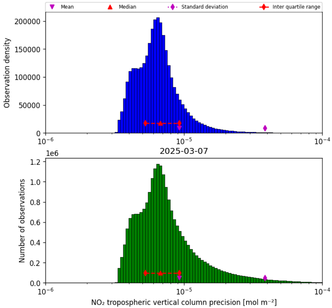
Figure 30: Histogram of “NO 2 tropospheric vertical column precision” for 2025-03-07 to 2025-03-08
