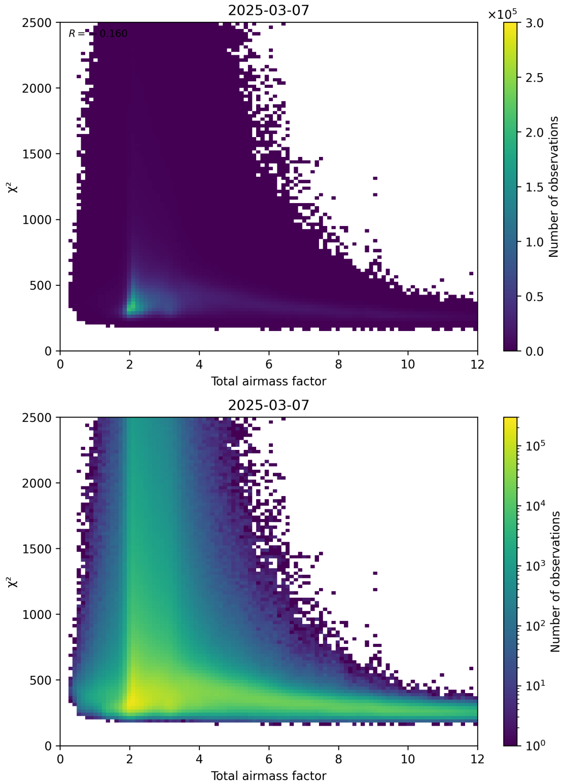
Figure 63: Scatter density plot of “Total airmass factor” against “ \chi^2 ” for 2025-03-07 to 2025-03-08.
