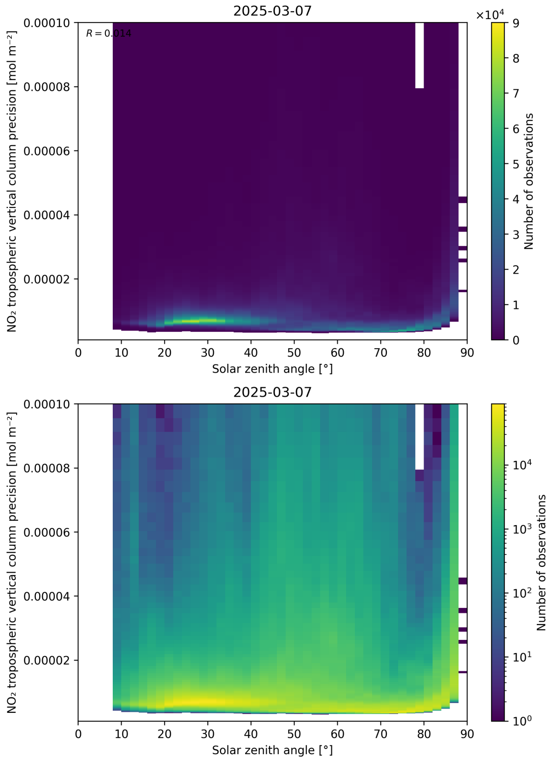
Figure 156: Scatter density plot of “Solar zenith angle” against “NO 2 tropospheric vertical column precision” for 2025-03-07 to 2025-03-08.
