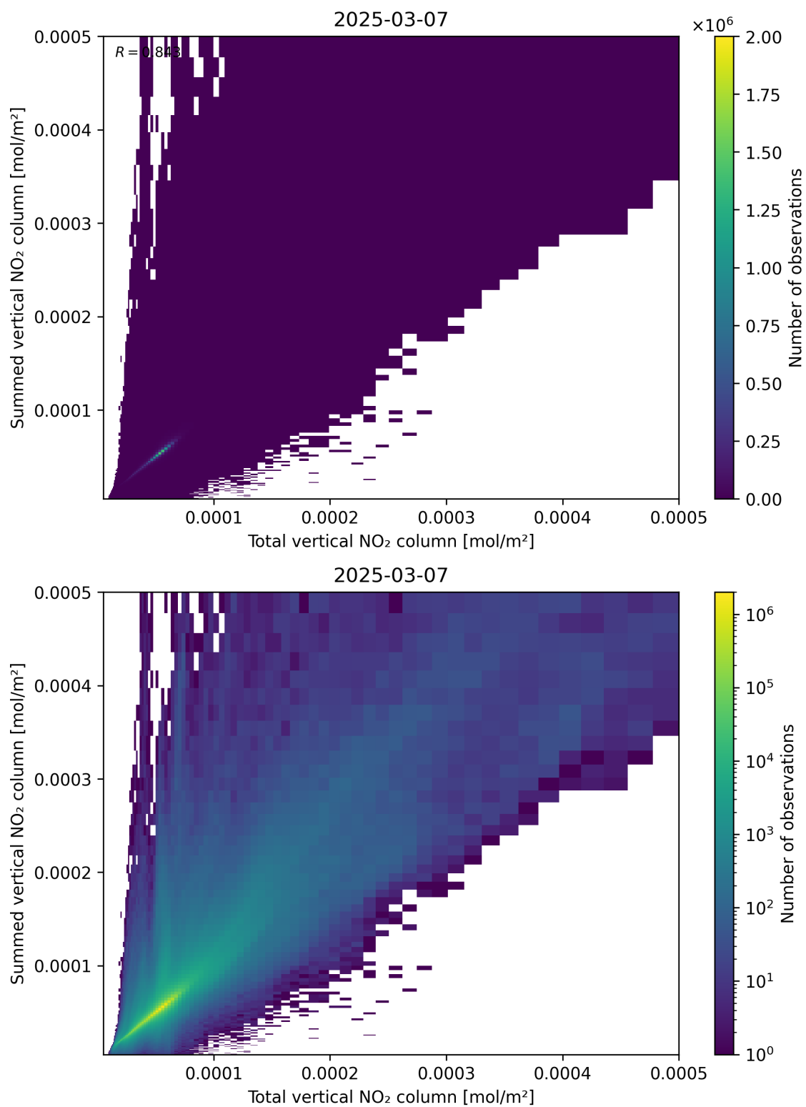
Figure 112: Scatter density plot of “Total vertical NO 2 column” against “Summed vertical NO 2 column” for 2025-03-07 to 2025-03-08.
