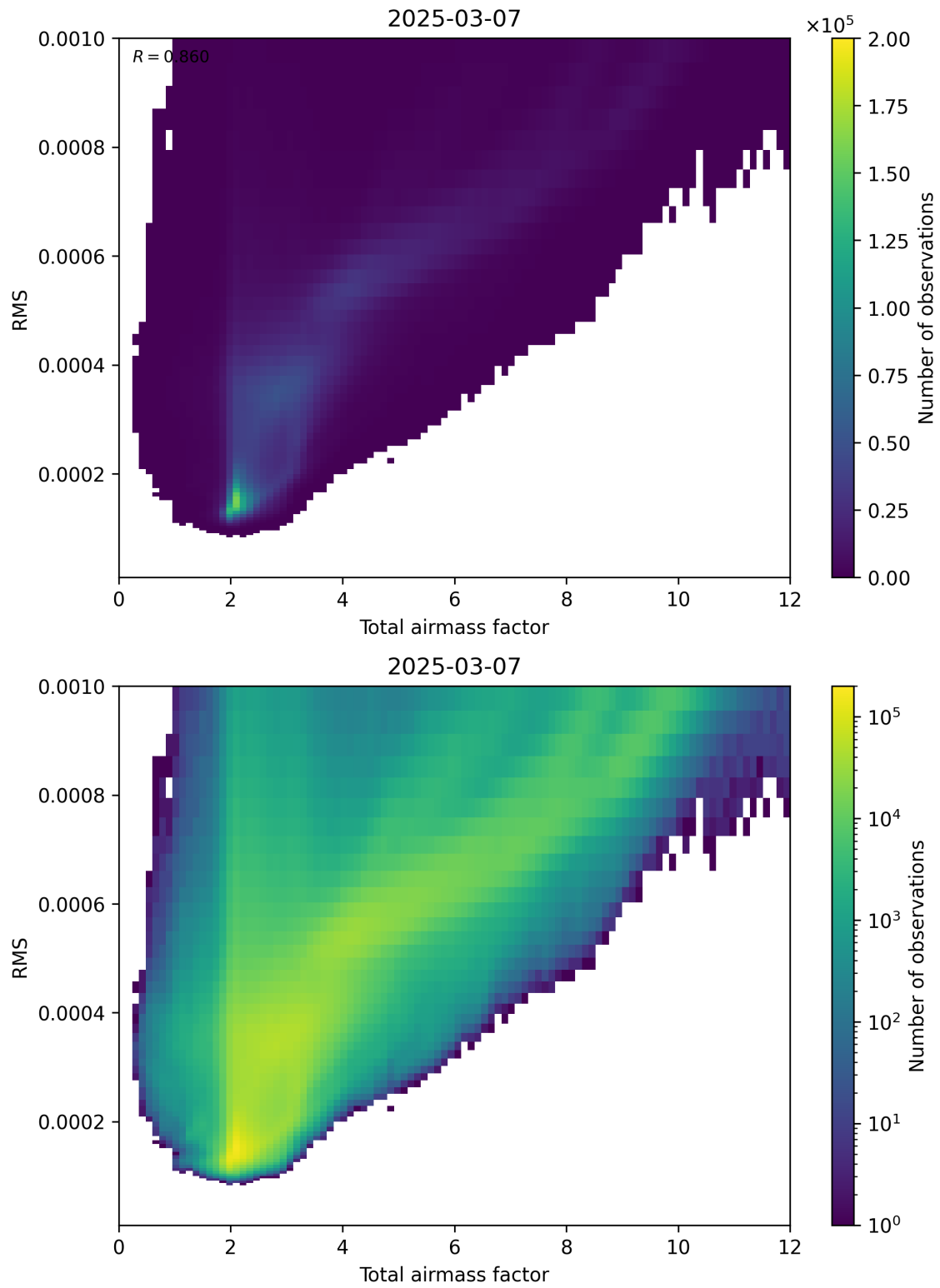
Figure 69: Scatter density plot of “Total airmass factor” against “RMS” for 2025-03-07 to 2025-03-08.
