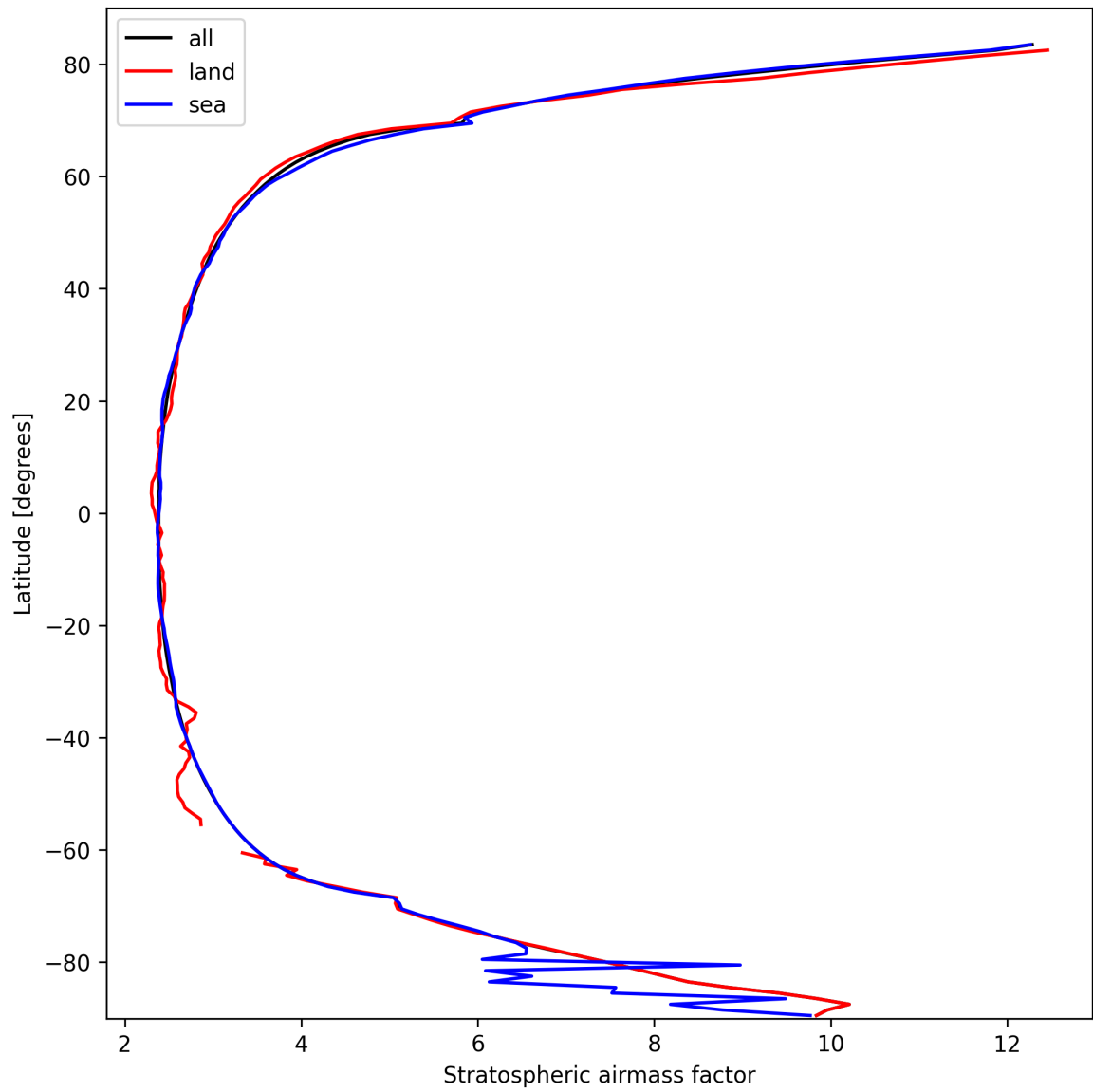
Figure 27: Zonal average of “Stratospheric airmass factor” for 2025-03-07 to 2025-03-08.
