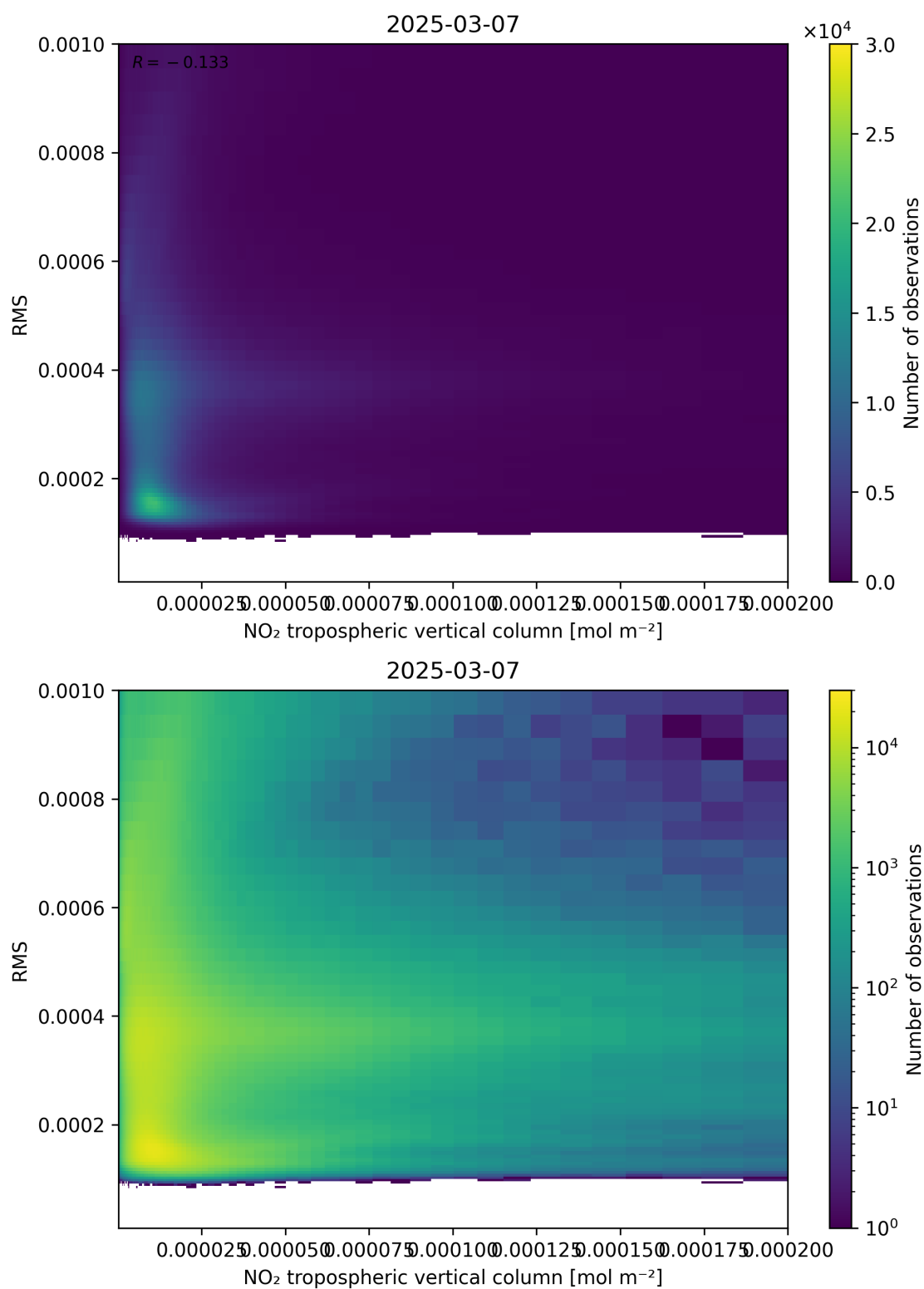
Figure 142: Scatter density plot of “NO 2 tropospheric vertical column” against “RMS” for 2025-03-07 to 2025-03-08.
