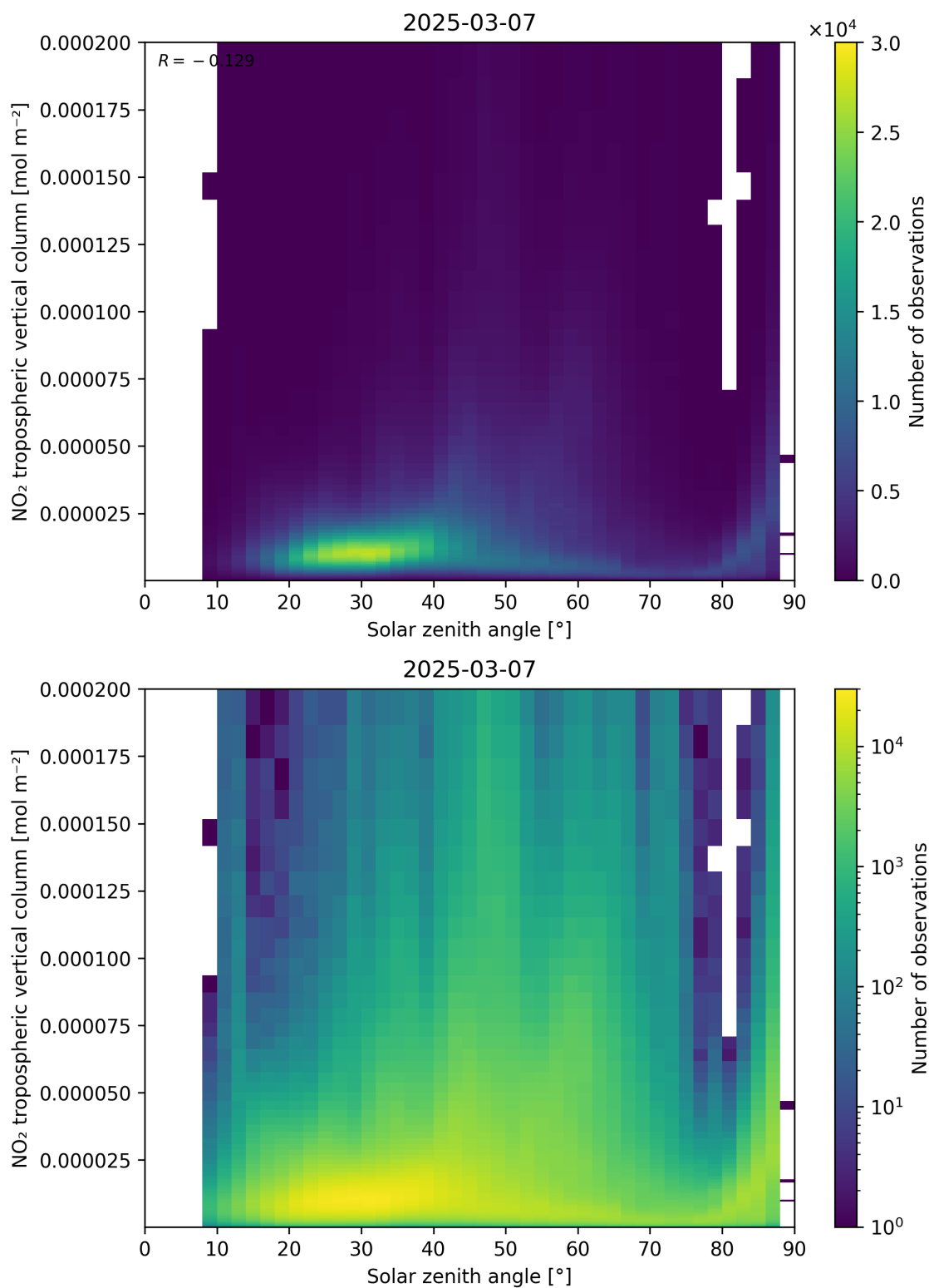
Figure 155: Scatter density plot of “Solar zenith angle” against “NO 2 tropospheric vertical column” for 2025-03-07 to 2025-03-08.
