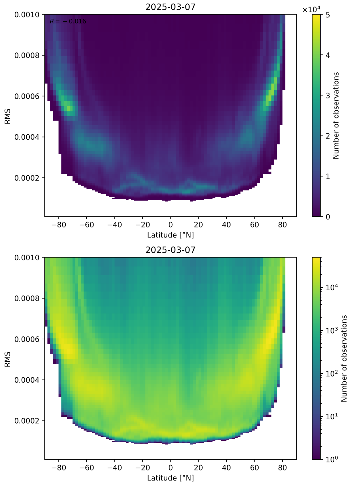
Figure 94: Scatter density plot of “Latitude” against “RMS” for 2025-03-07 to 2025-03-08.
