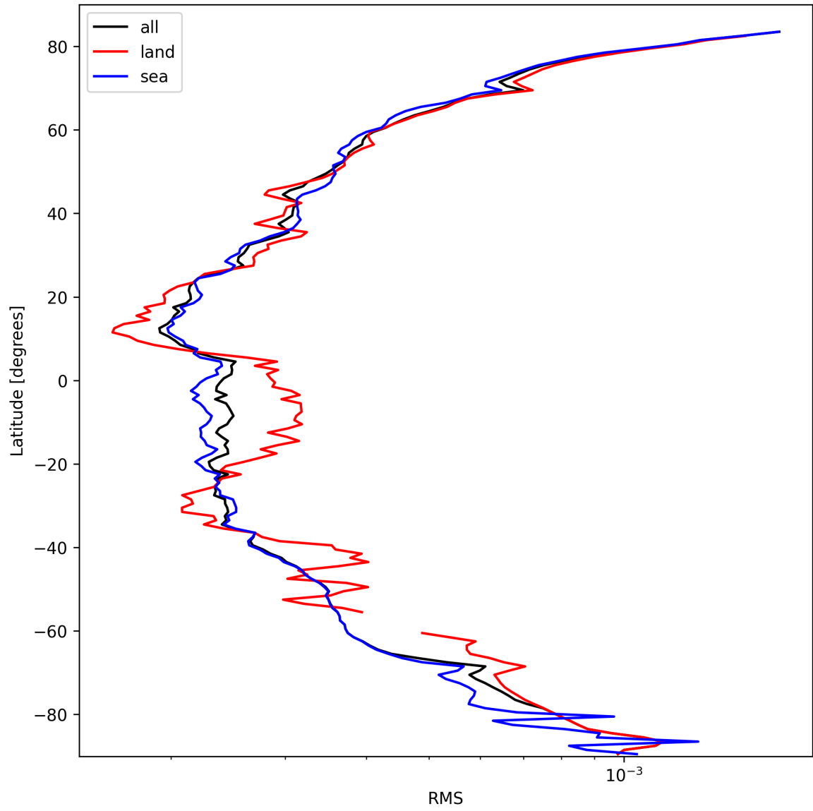
Figure 26: Zonal average of “RMS” for 2025-03-07 to 2025-03-08.
