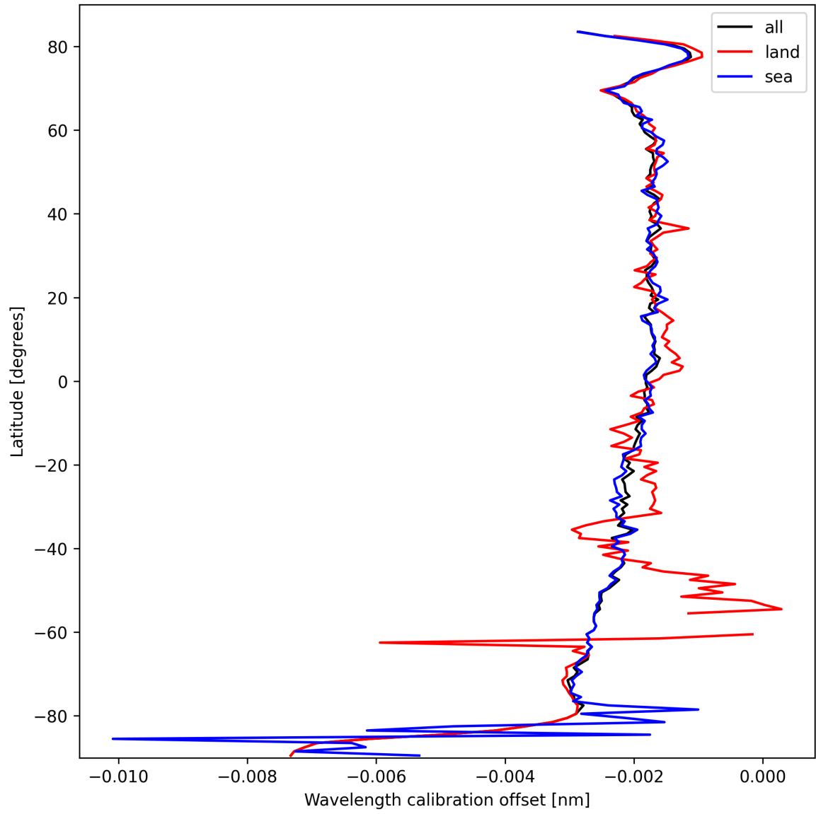
Figure 18: Zonal average of “Wavelength calibration offset” for 2025-03-07 to 2025-03-08.
