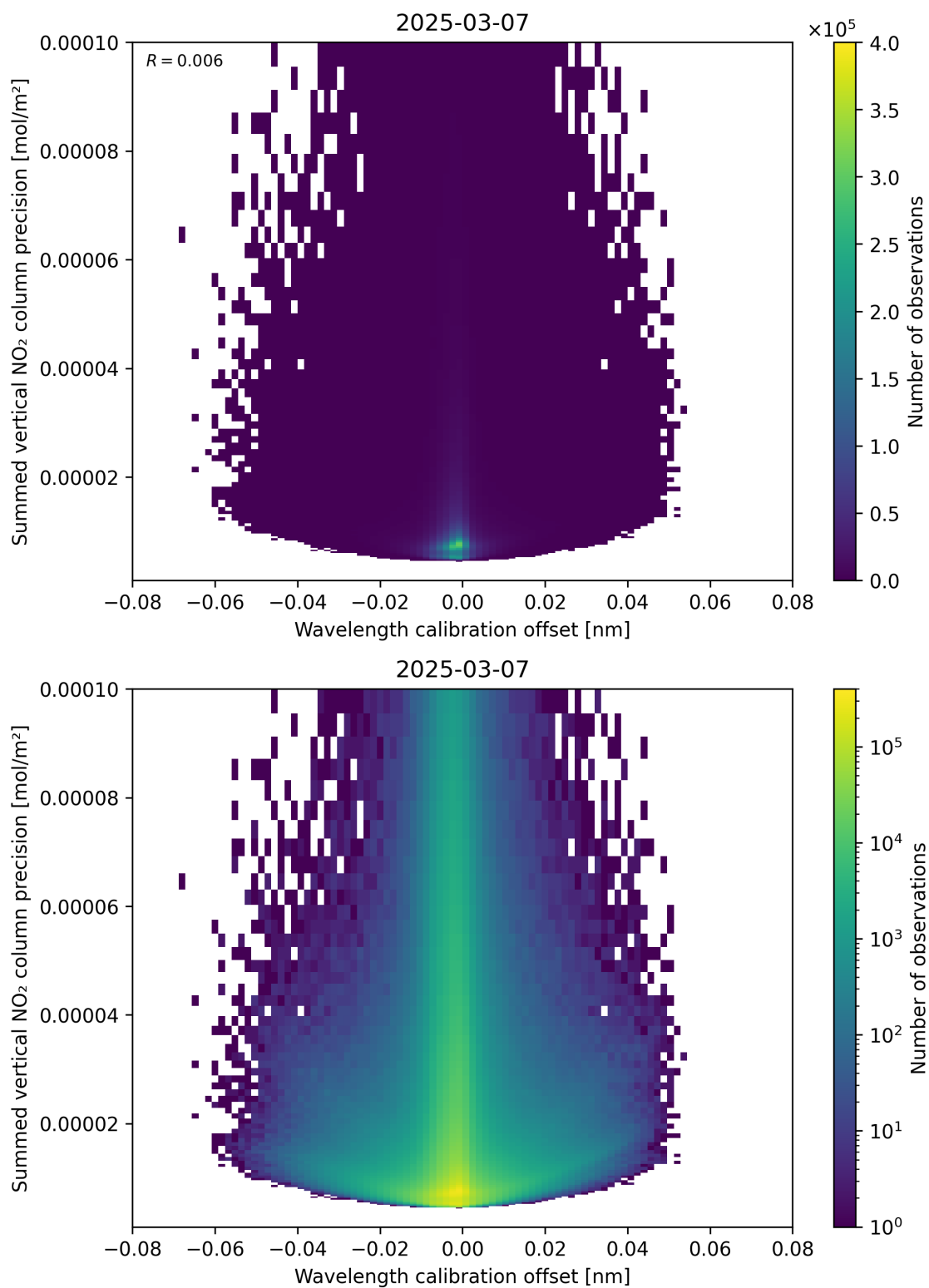
Figure 178: Scatter density plot of “Wavelength calibration offset” against “Summed vertical NO 2 column precision” for 2025-03-07 to 2025-03-08.
