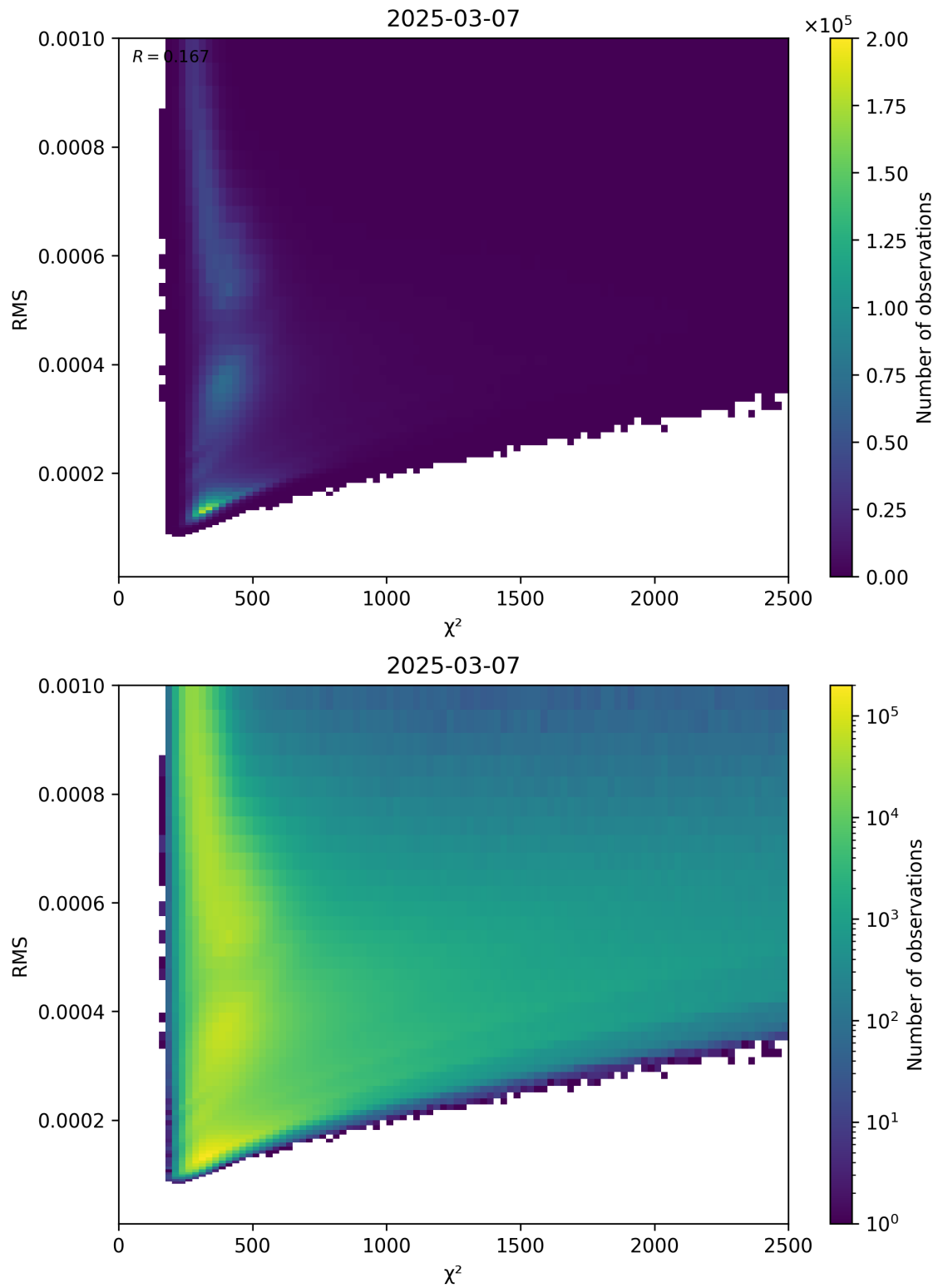
Figure 82: Scatter density plot of “ \chi^2 ” against “RMS” for 2025-03-07 to 2025-03-08.
