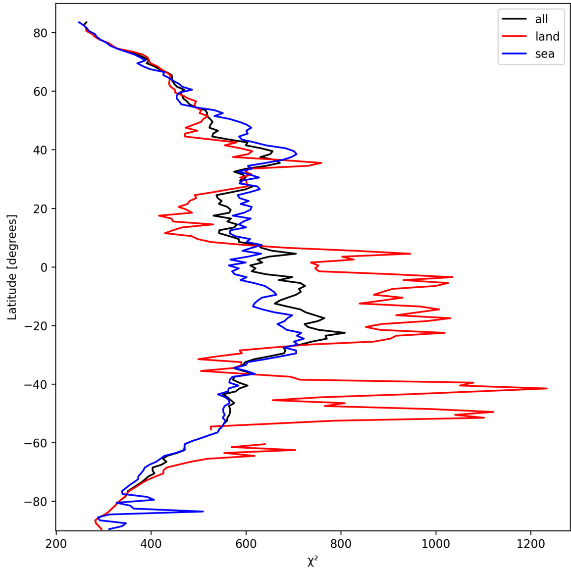
Figure 25: Zonal average of “ \chi^2 ” for 2025-03-07 to 2025-03-08.
