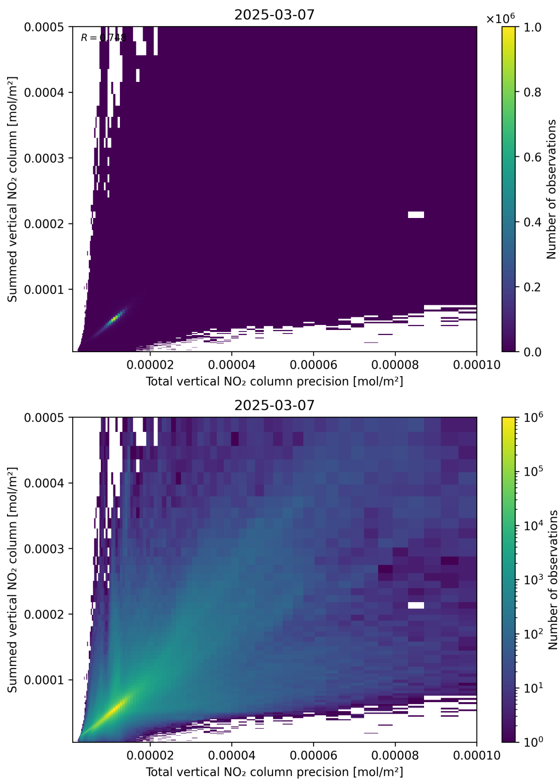
Figure 117: Scatter density plot of “Total vertical NO 2 column precision” against “Summed vertical NO 2 column” for 2025-03-07 to 2025-03-08.
