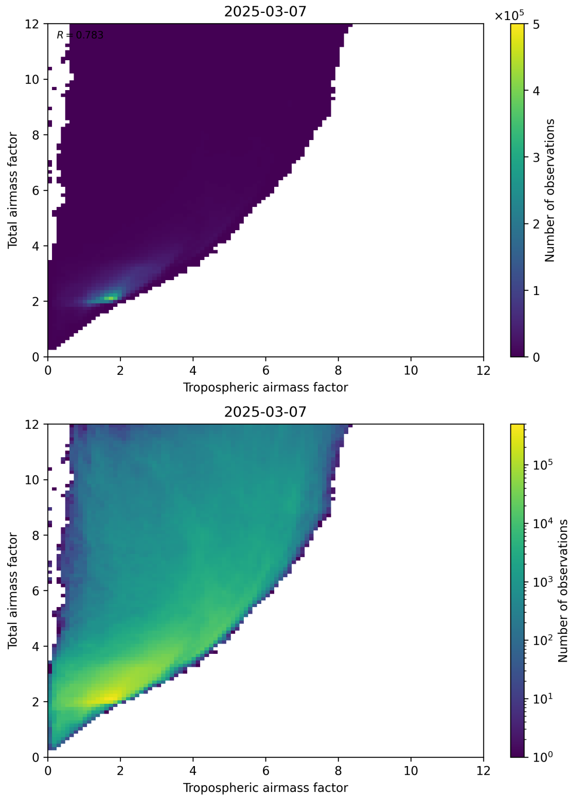
Figure 72: Scatter density plot of “Tropospheric airmass factor” against “Total airmass factor” for 2025-03-07 to 2025-03-08.
