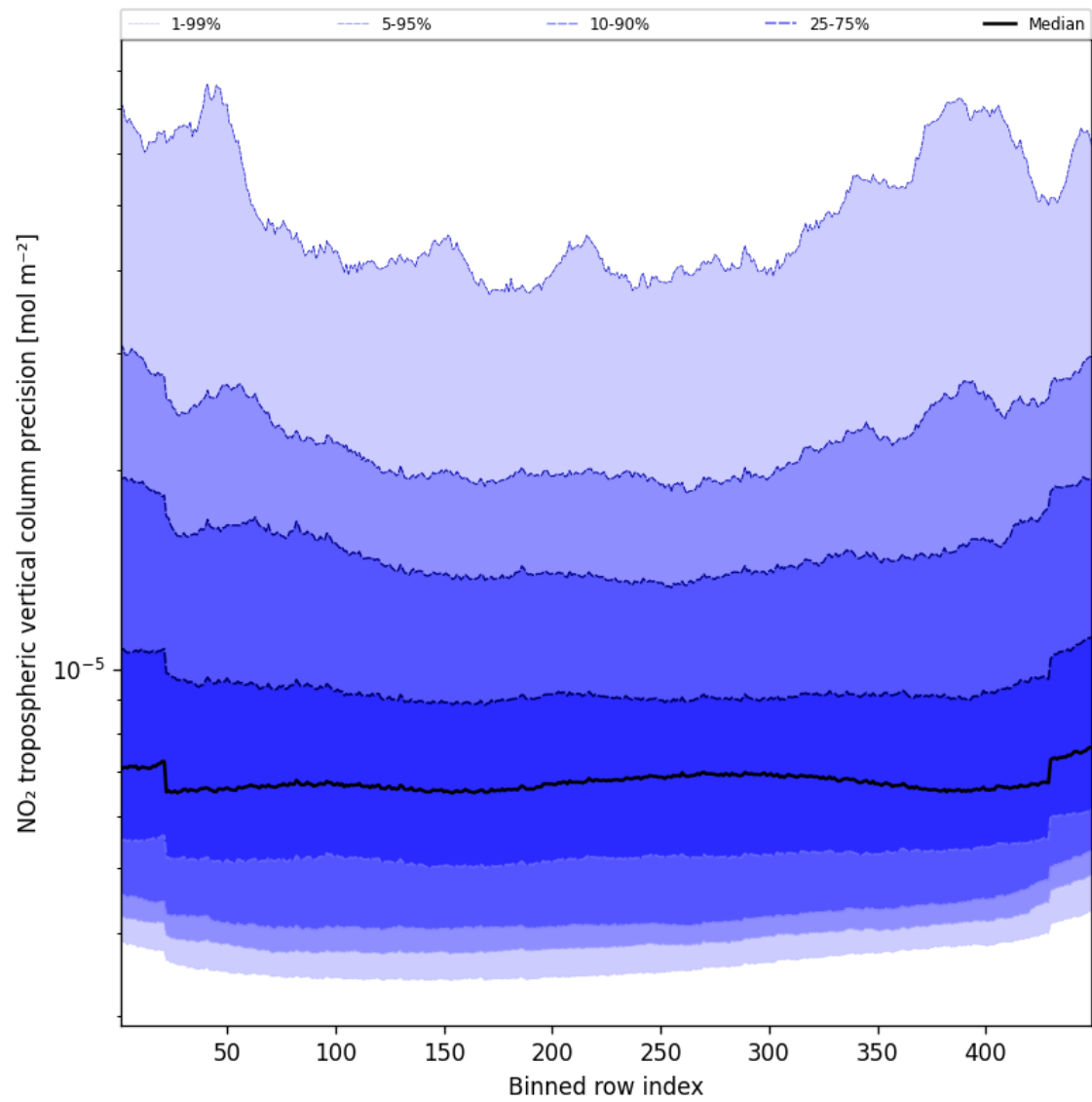
Figure 47: Along track statistics of “NO 2 tropospheric vertical column precision” for 2025-03-07 to 2025-03-08
