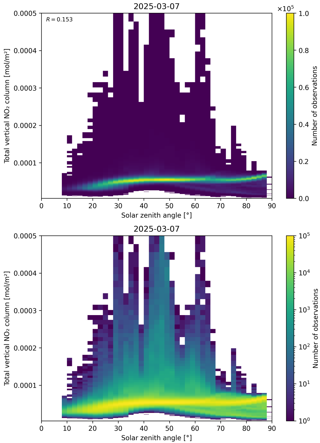
Figure 153: Scatter density plot of “Solar zenith angle” against “Total vertical NO 2 column” for 2025-03-07 to 2025-03-08.
