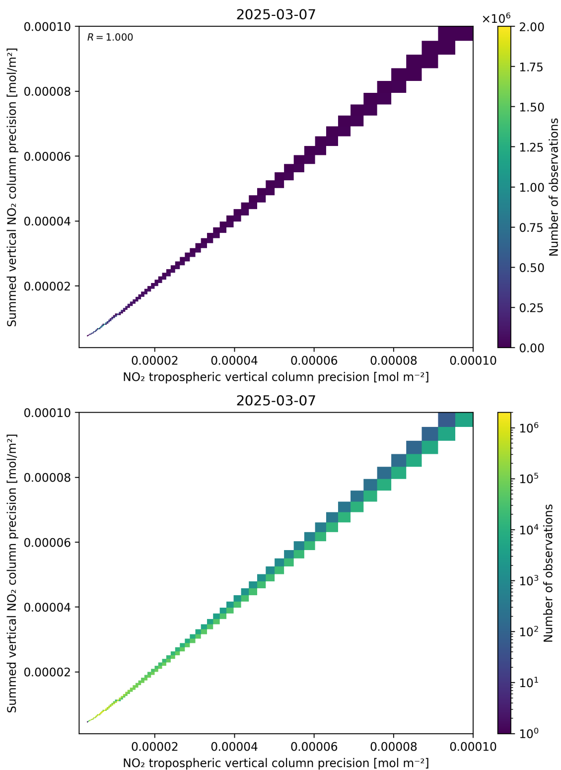
Figure 137: Scatter density plot of “NO 2 tropospheric vertical column precision” against “Summed vertical NO 2 column precision” for 2025-03-07 to 2025-03-08.
