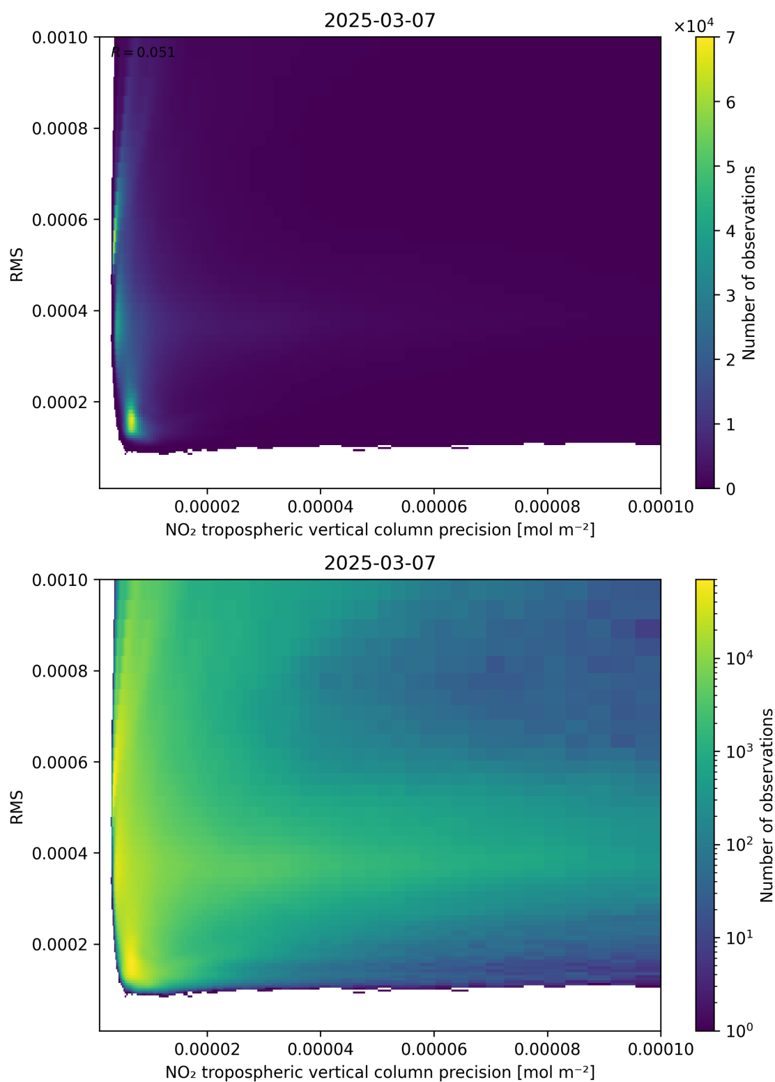
Figure 140: Scatter density plot of “NO 2 tropospheric vertical column precision” against “RMS” for 2025-03-07 to 2025-03-08.
