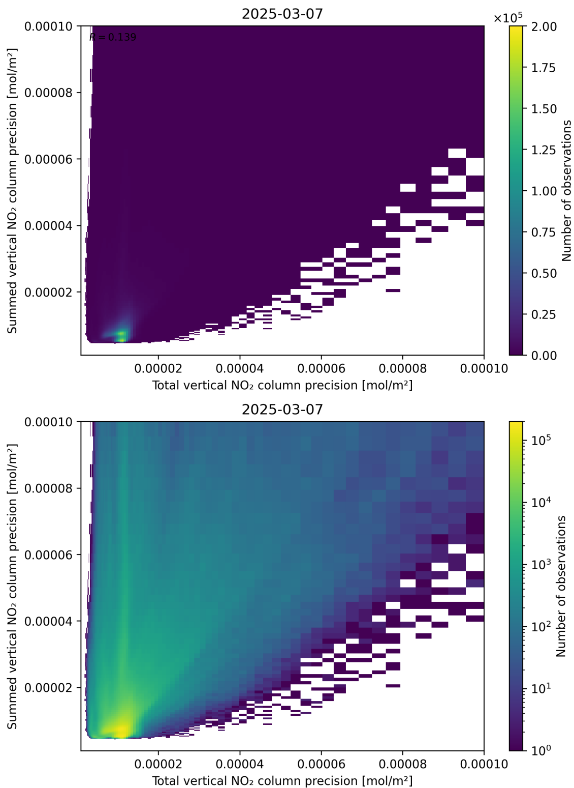
Figure 118: Scatter density plot of “Total vertical NO 2 column precision” against “Summed vertical NO 2 column precision” for 2025-03-07 to 2025-03-08.
