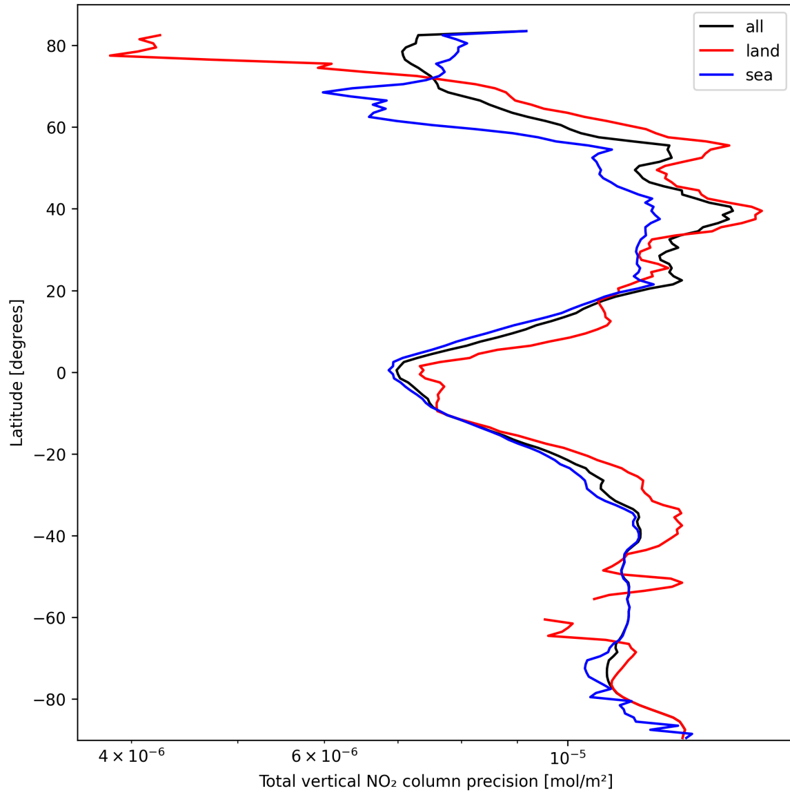
Figure 22: Zonal average of “Total vertical NO 2 column precision” for 2025-03-07 to 2025-03-08.
