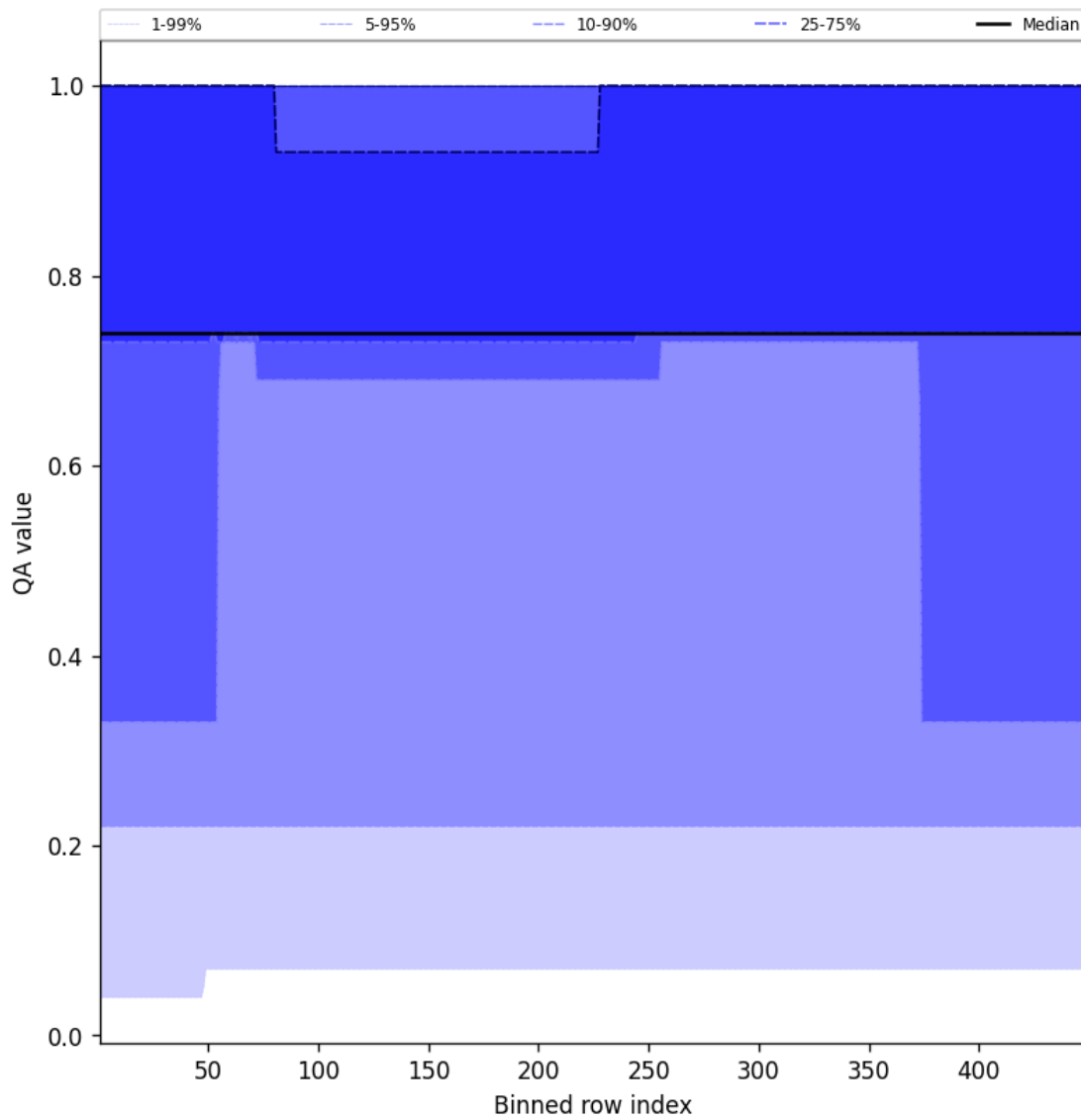
Figure 45: Along track statistics of “QA value” for 2025-03-07 to 2025-03-08
