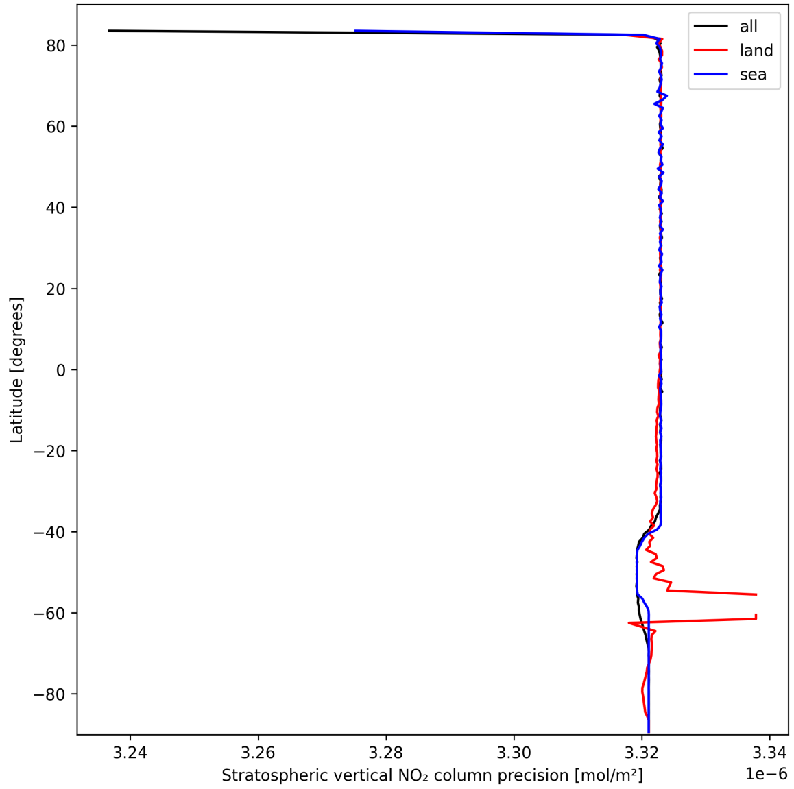
Figure 20: Zonal average of “Stratospheric vertical NO 2 column precision” for 2025-03-07 to 2025-03-08.
