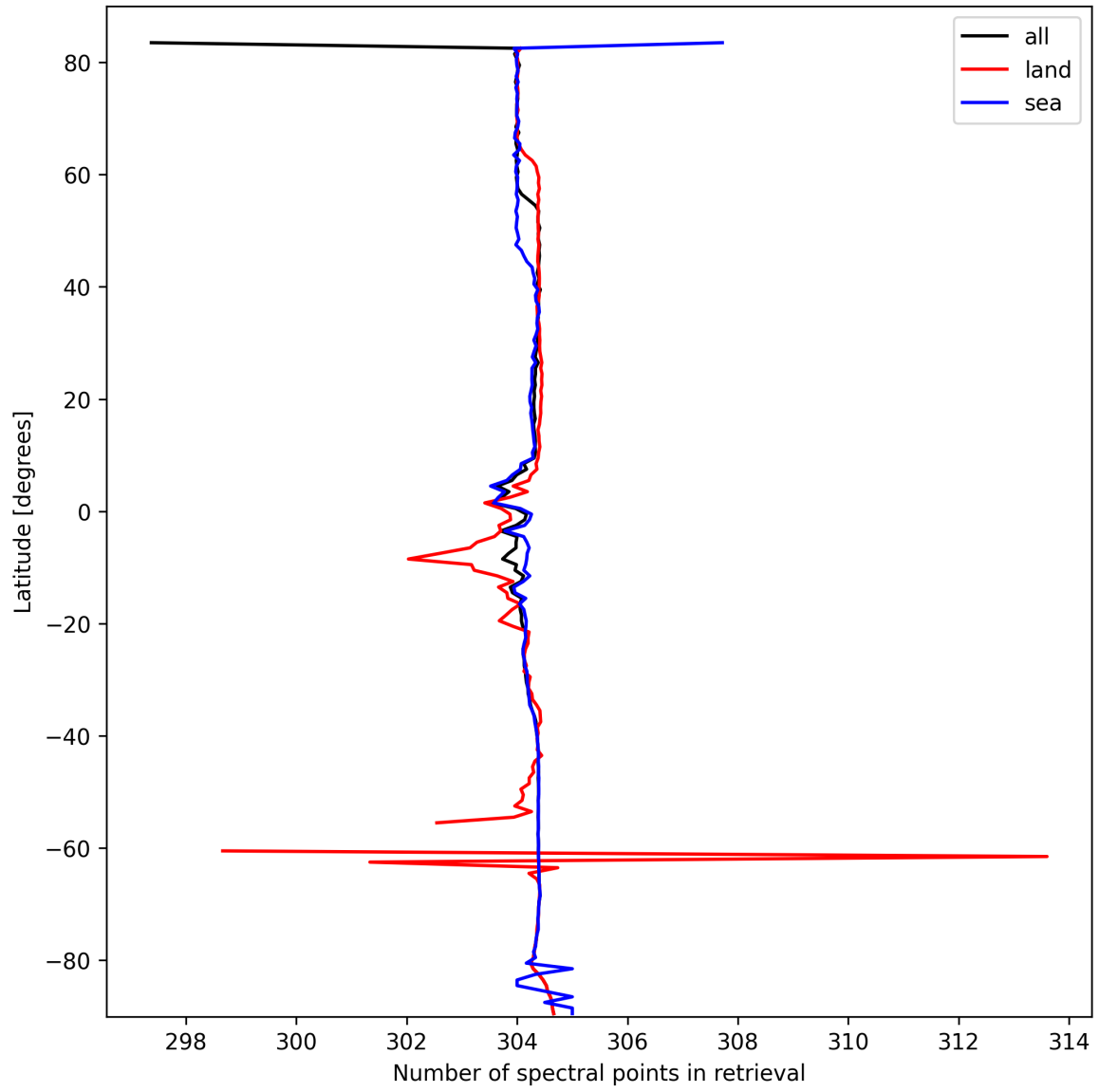
Figure 16: Zonal average of “Number of spectral points in retrieval” for 2025-03-07 to 2025-03-08.
