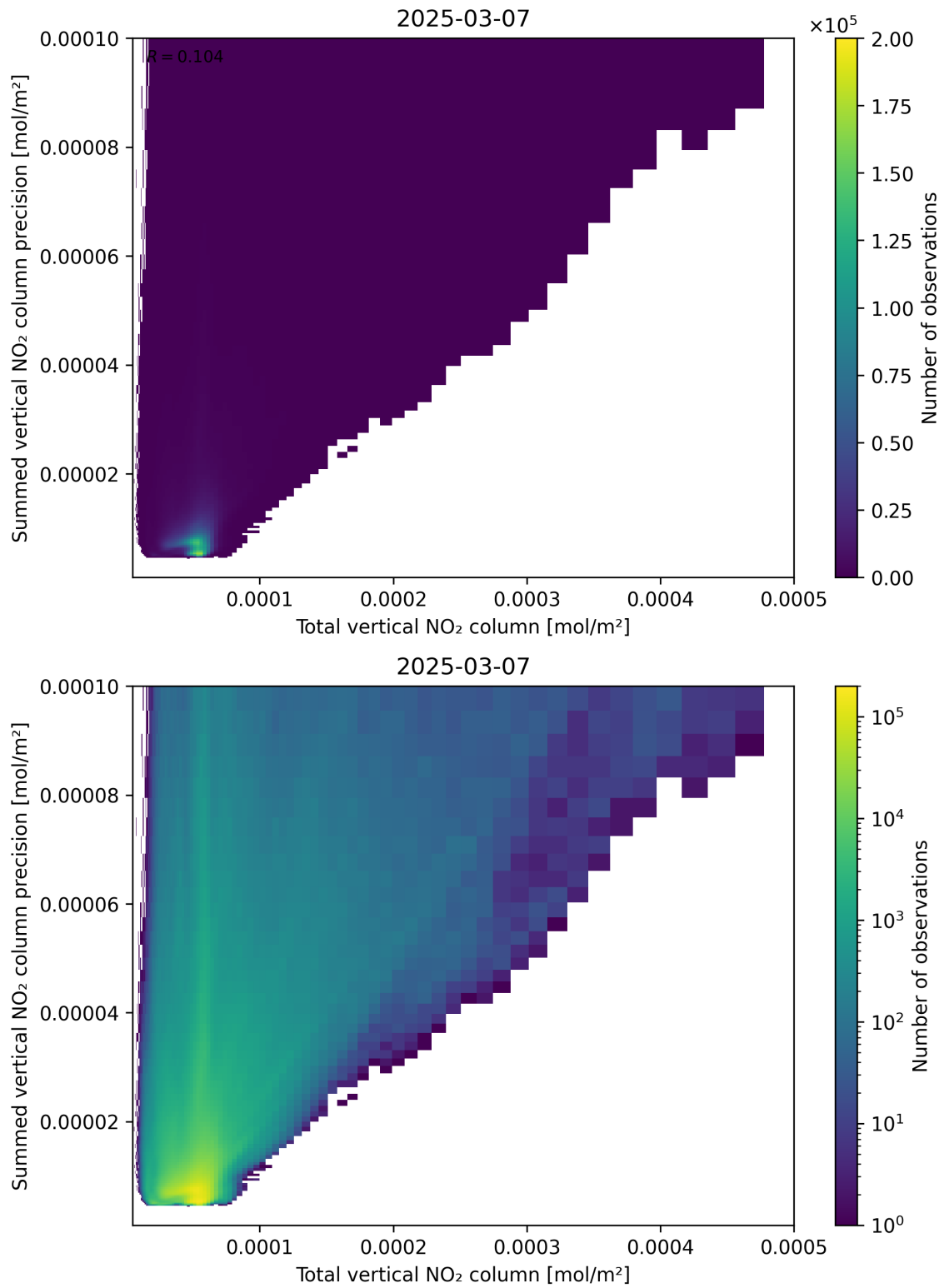
Figure 113: Scatter density plot of “Total vertical NO 2 column” against “Summed vertical NO 2 column precision” for 2025-03-07 to 2025-03-08.
