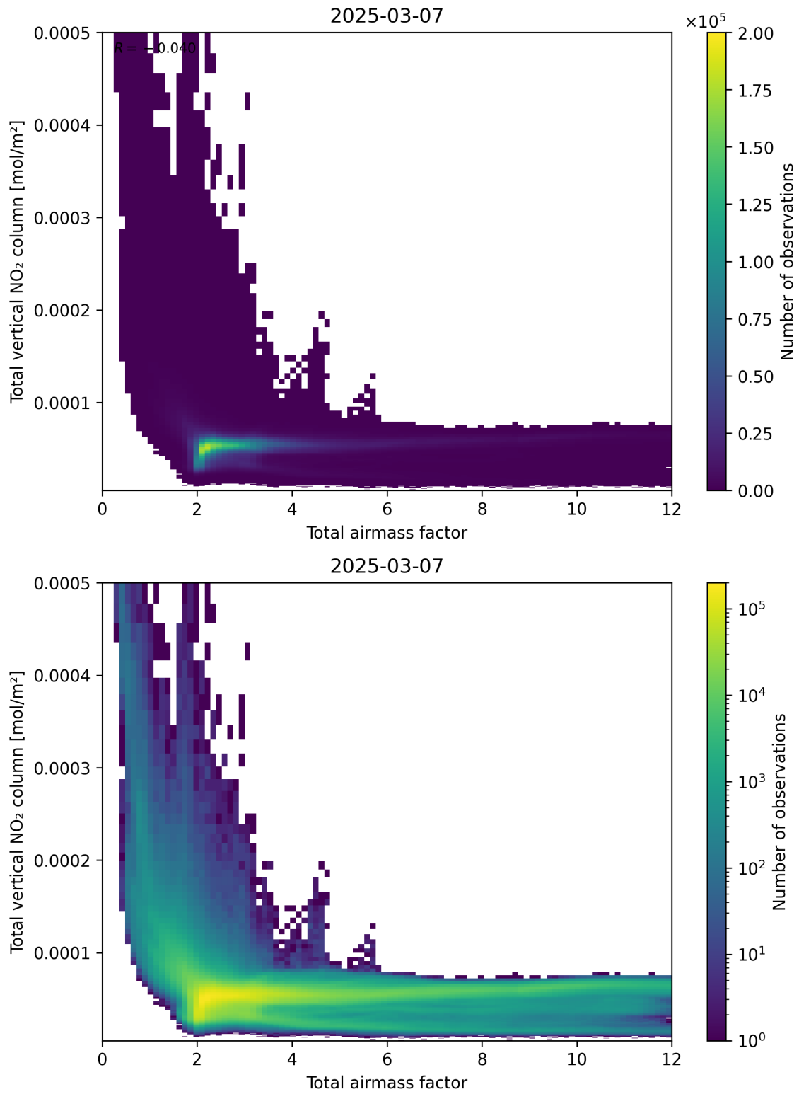
Figure 67: Scatter density plot of “Total airmass factor” against “Total vertical NO 2 column” for 2025-03-07 to 2025-03-08.
