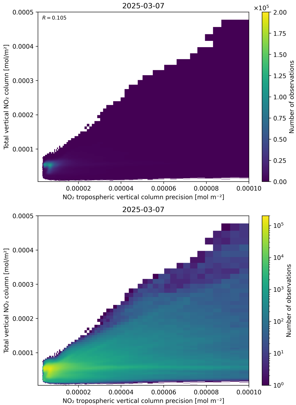
Figure 138: Scatter density plot of “NO 2 tropospheric vertical column precision” against “Total vertical NO 2 column” for 2025-03-07 to 2025-03-08.
