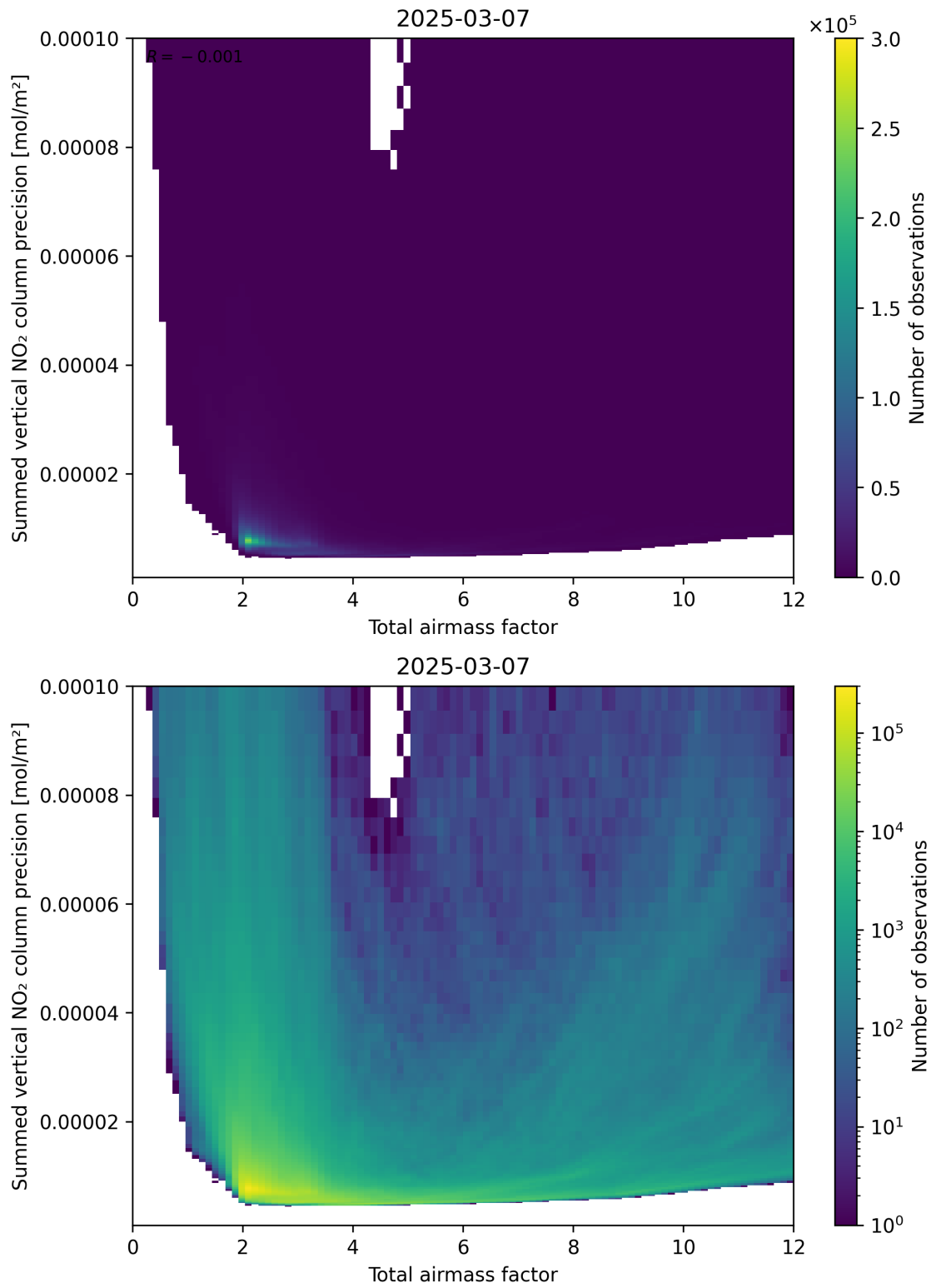
Figure 66: Scatter density plot of “Total airmass factor” against “Summed vertical NO 2 column precision” for 2025-03-07 to 2025-03-08.
