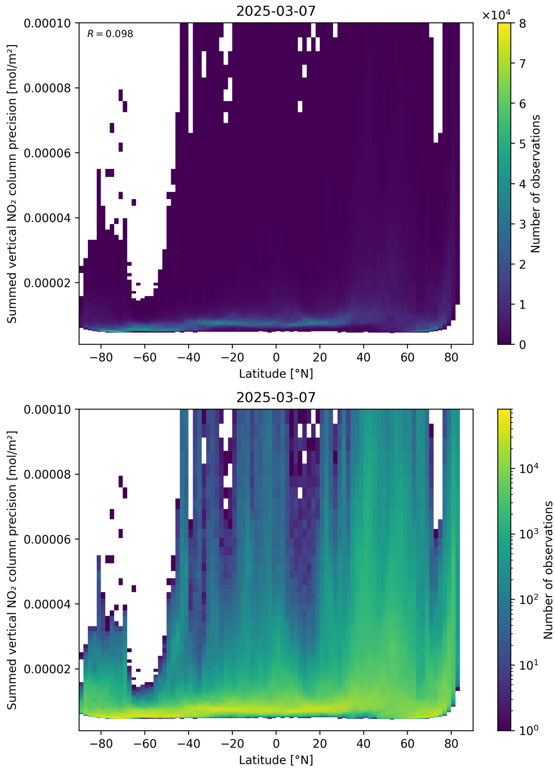
Figure 89: Scatter density plot of “Latitude” against “Summed vertical NO 2 column precision” for 2025-03-07 to 2025-03-08.
