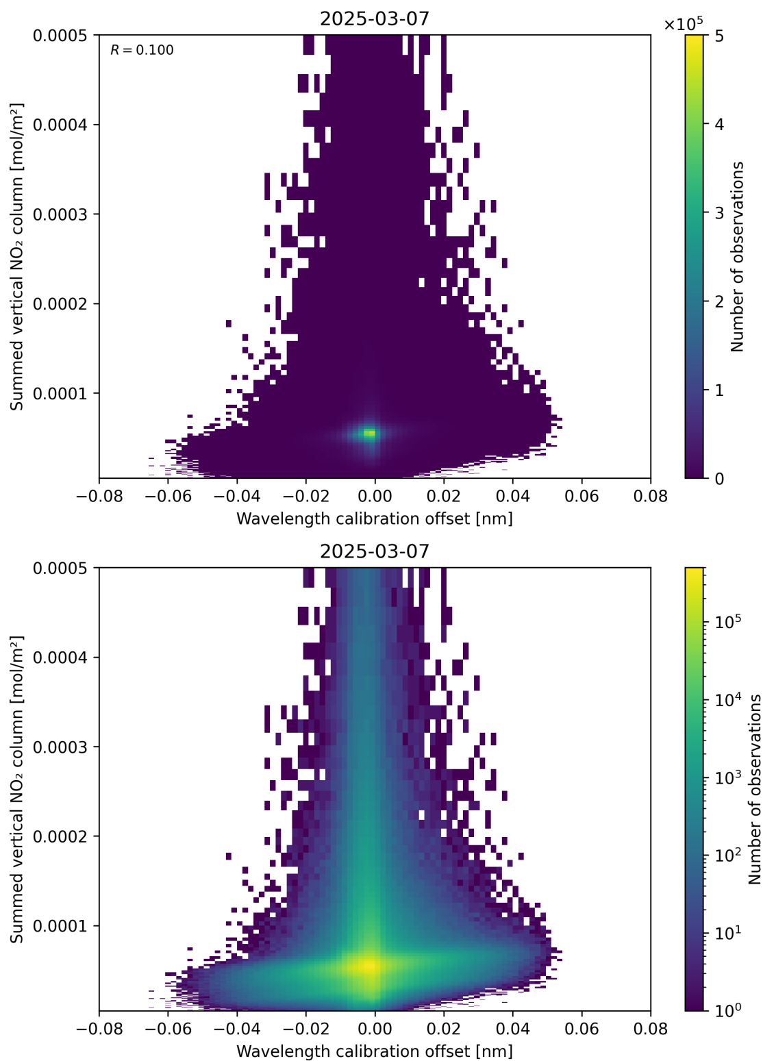
Figure 177: Scatter density plot of “Wavelength calibration offset” against “Summed vertical NO 2 column” for 2025-03-07 to 2025-03-08.
