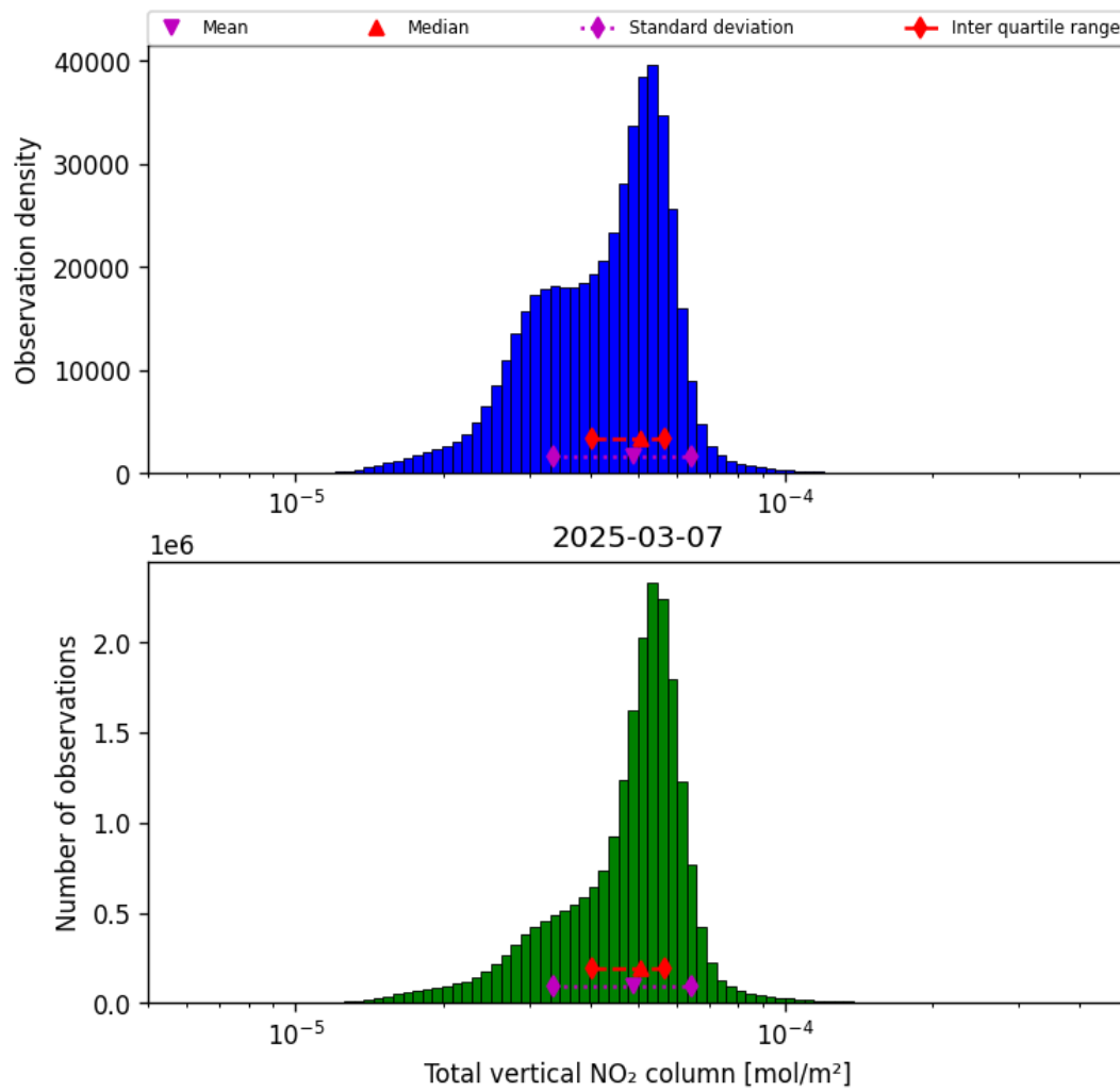
Figure 38: Histogram of “Total vertical NO 2 column” for 2025-03-07 to 2025-03-08
