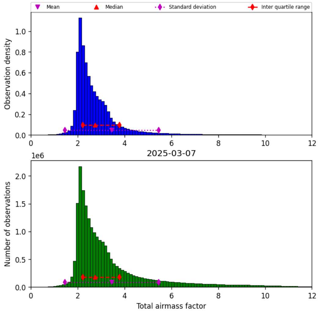
Figure 32: Histogram of “Total airmass factor” for 2025-03-07 to 2025-03-08
