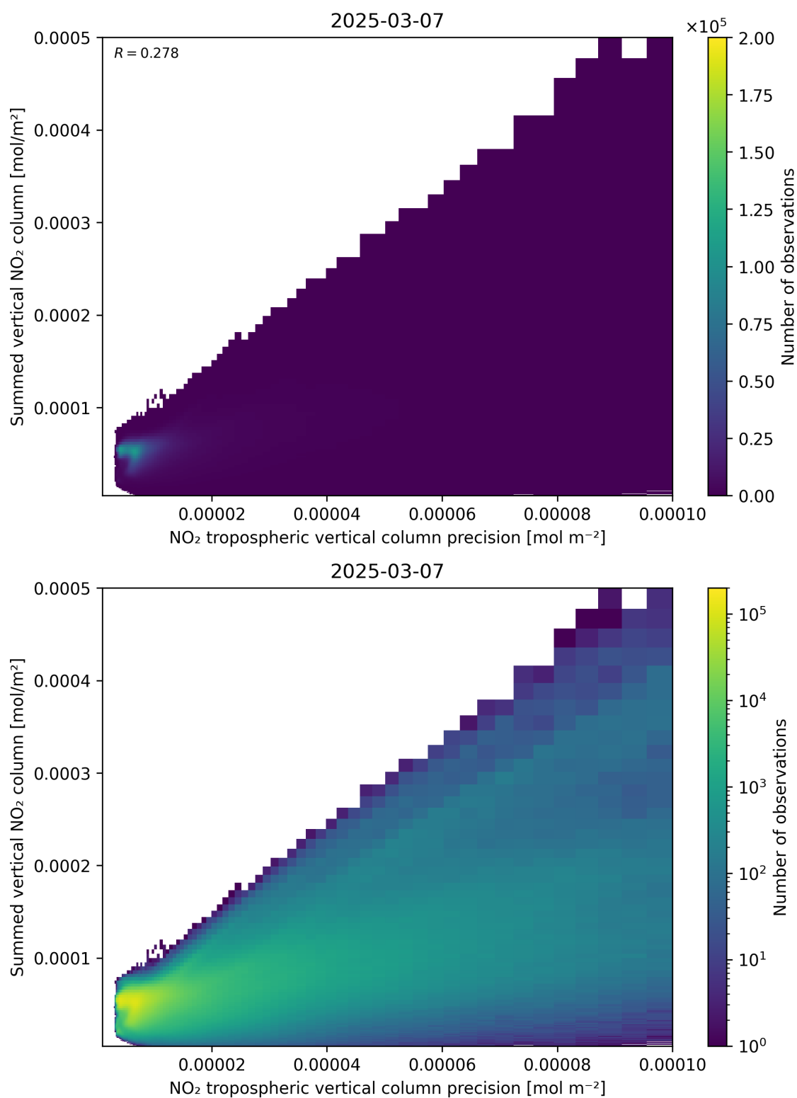
Figure 136: Scatter density plot of “NO 2 tropospheric vertical column precision” against “Summed vertical NO 2 column” for 2025-03-07 to 2025-03-08.
