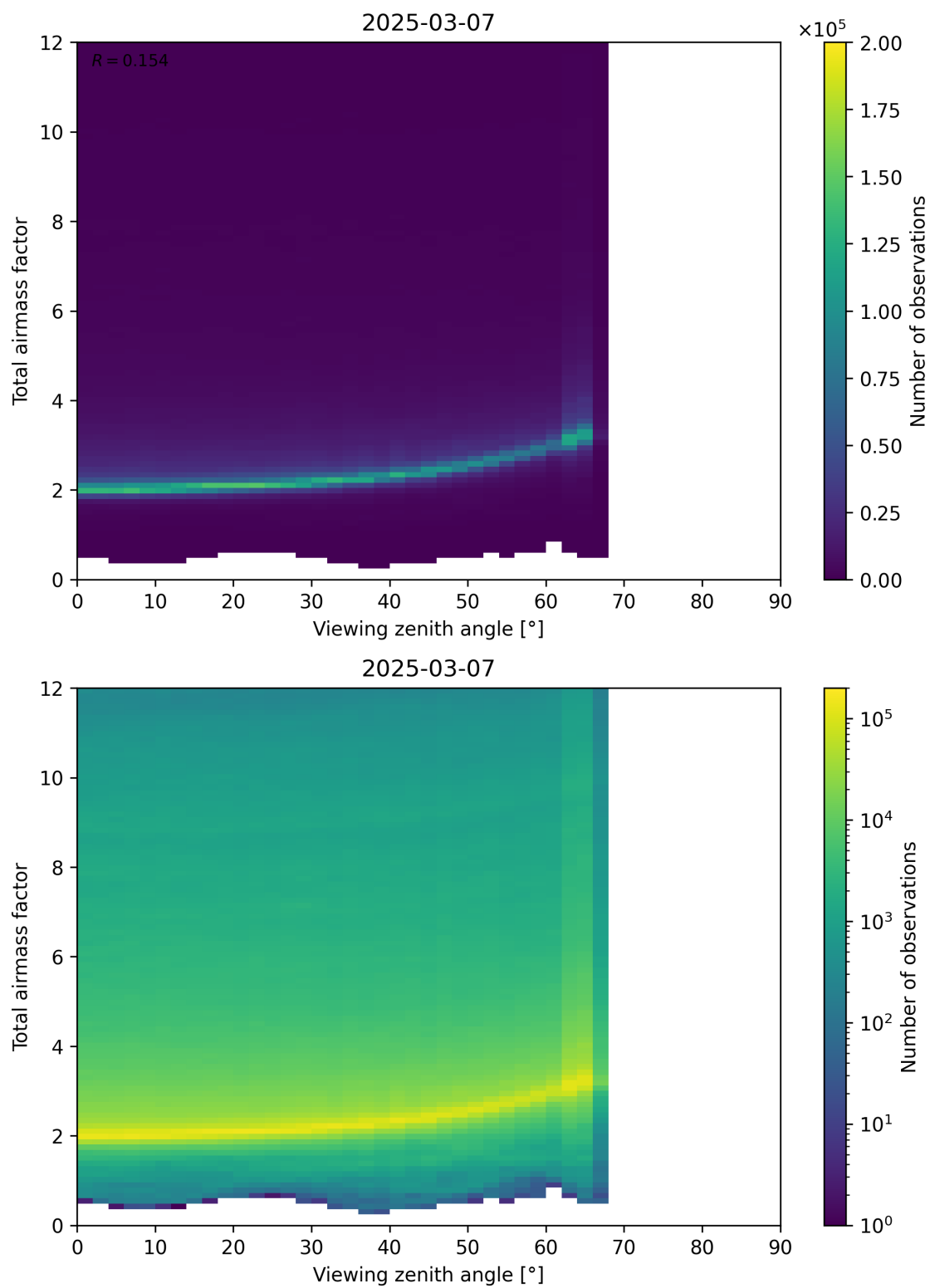
Figure 160: Scatter density plot of “Viewing zenith angle” against “Total airmass factor” for 2025-03-07 to 2025-03-08.
