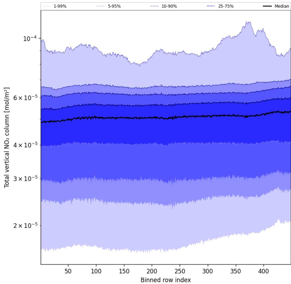
Figure 55: Along track statistics of “Total vertical NO 2 column” for 2025-03-07 to 2025-03-08
