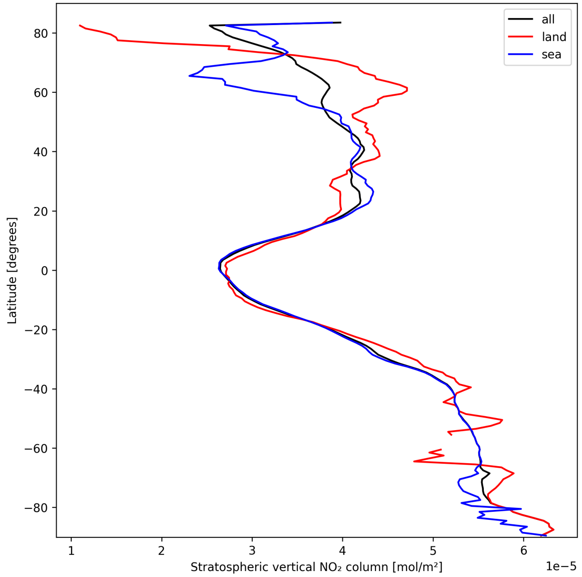
Figure 19: Zonal average of “Stratospheric vertical NO 2 column” for 2025-03-07 to 2025-03-08.
