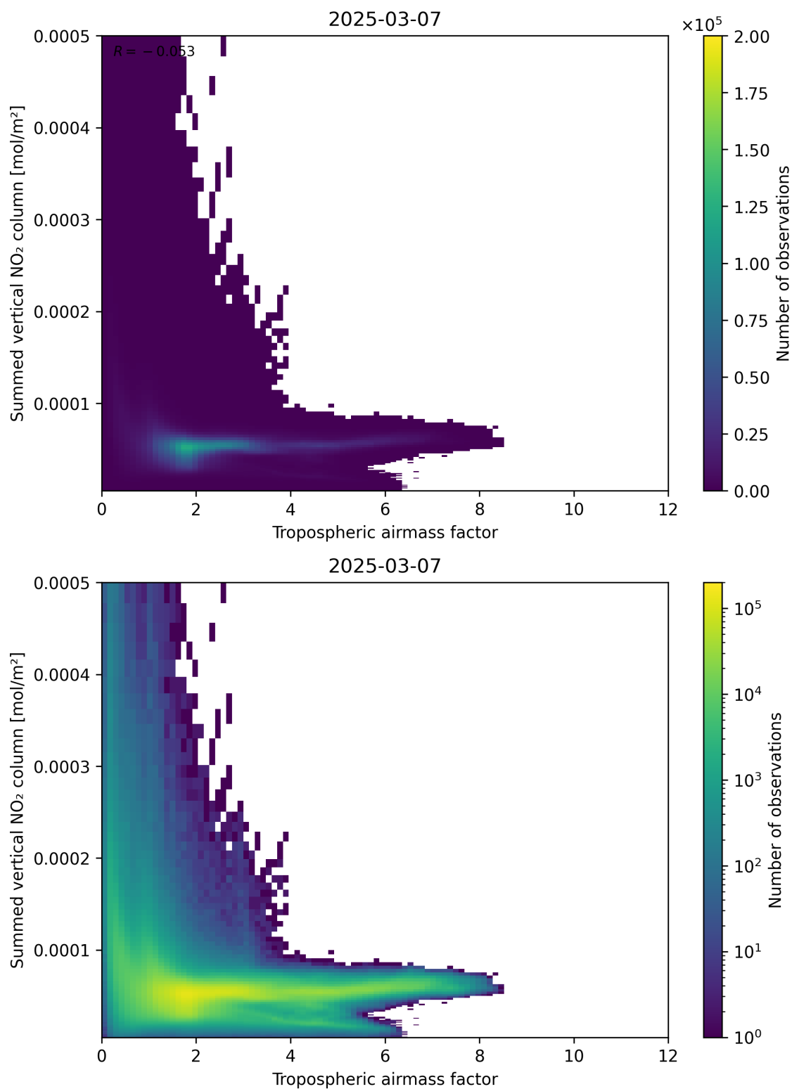
Figure 75: Scatter density plot of “Tropospheric airmass factor” against “Summed vertical NO 2 column” for 2025-03-07 to 2025-03-08.
