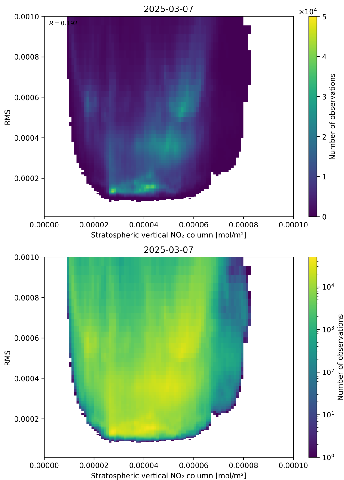
Figure 102: Scatter density plot of “Stratospheric vertical NO 2 column” against “RMS” for 2025-03-07 to 2025-03-08.
