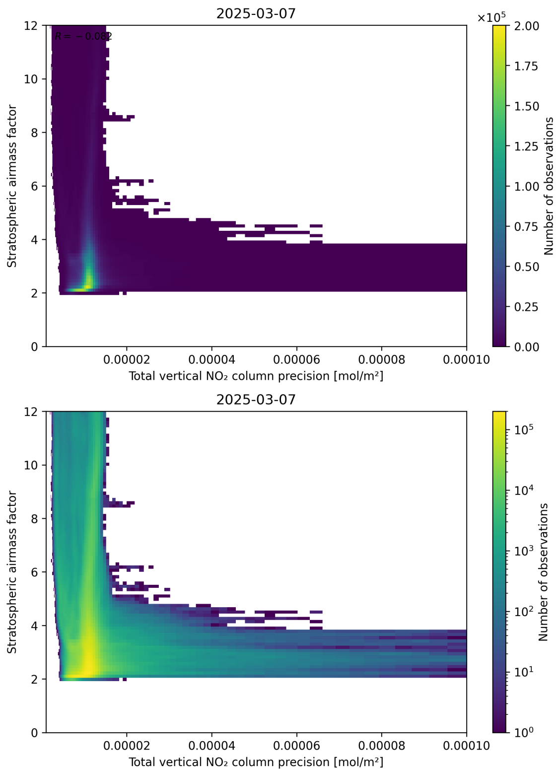
Figure 115: Scatter density plot of “Total vertical NO 2 column precision” against “Stratospheric air mass factor” for 2025-03-07 to 2025-03-08.
