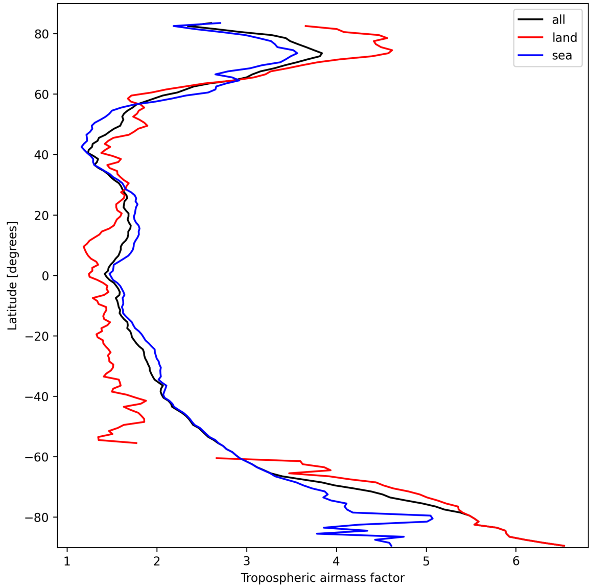
Figure 14: Zonal average of “Tropospheric airmass factor” for 2025-03-07 to 2025-03-08.
