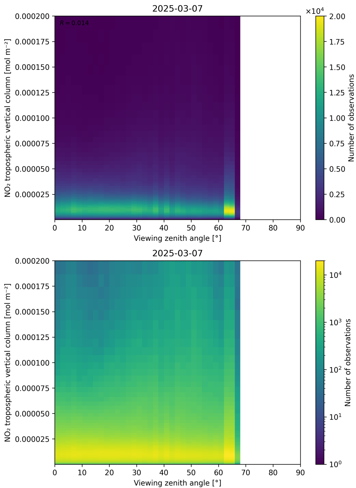
Figure 169: Scatter density plot of “Viewing zenith angle” against “NO 2 tropospheric vertical column” for 2025-03-07 to 2025-03-08.
