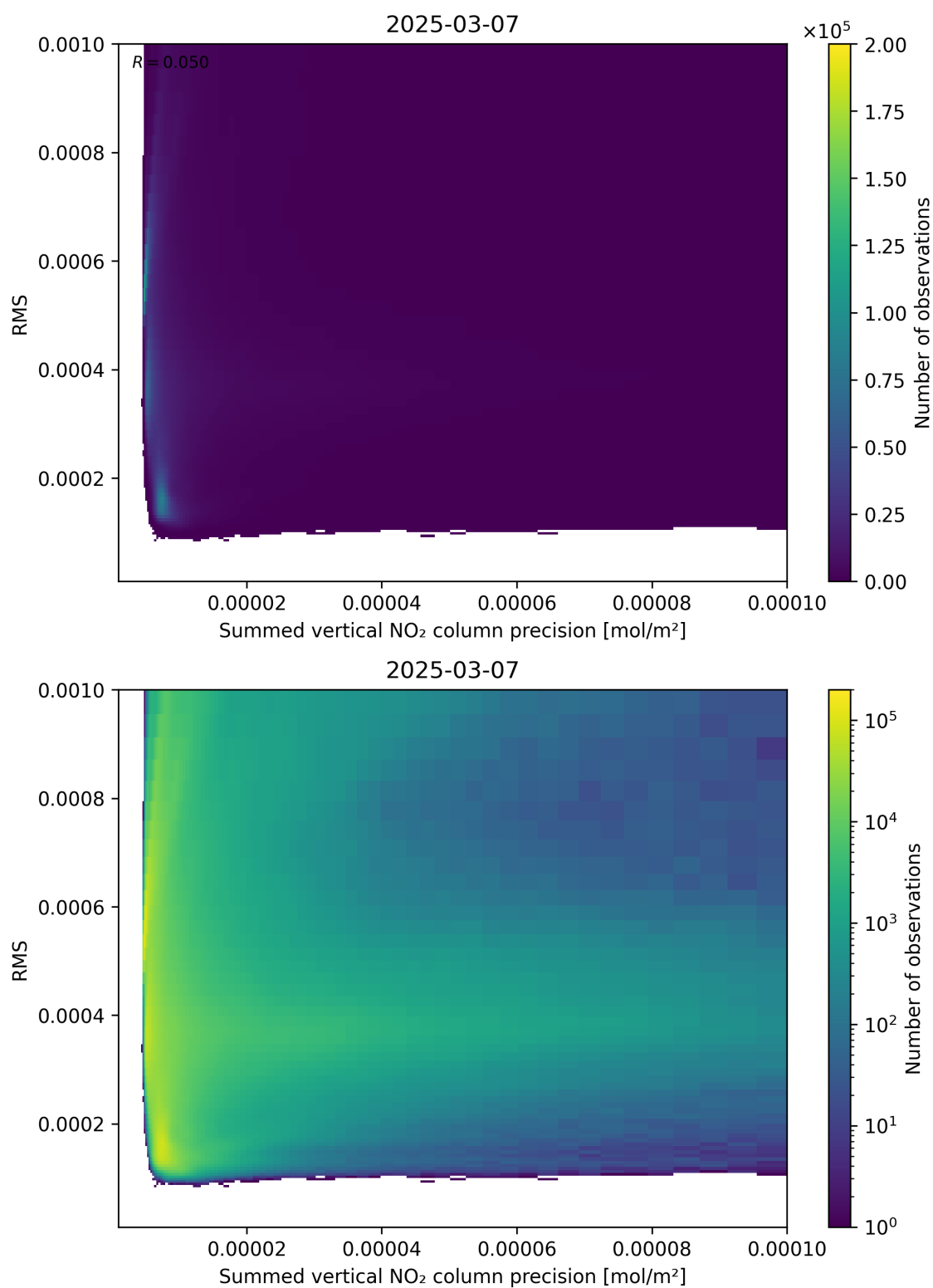
Figure 108: Scatter density plot of “Summed vertical NO 2 column precision” against “RMS” for 2025-03-07 to 2025-03-08.
