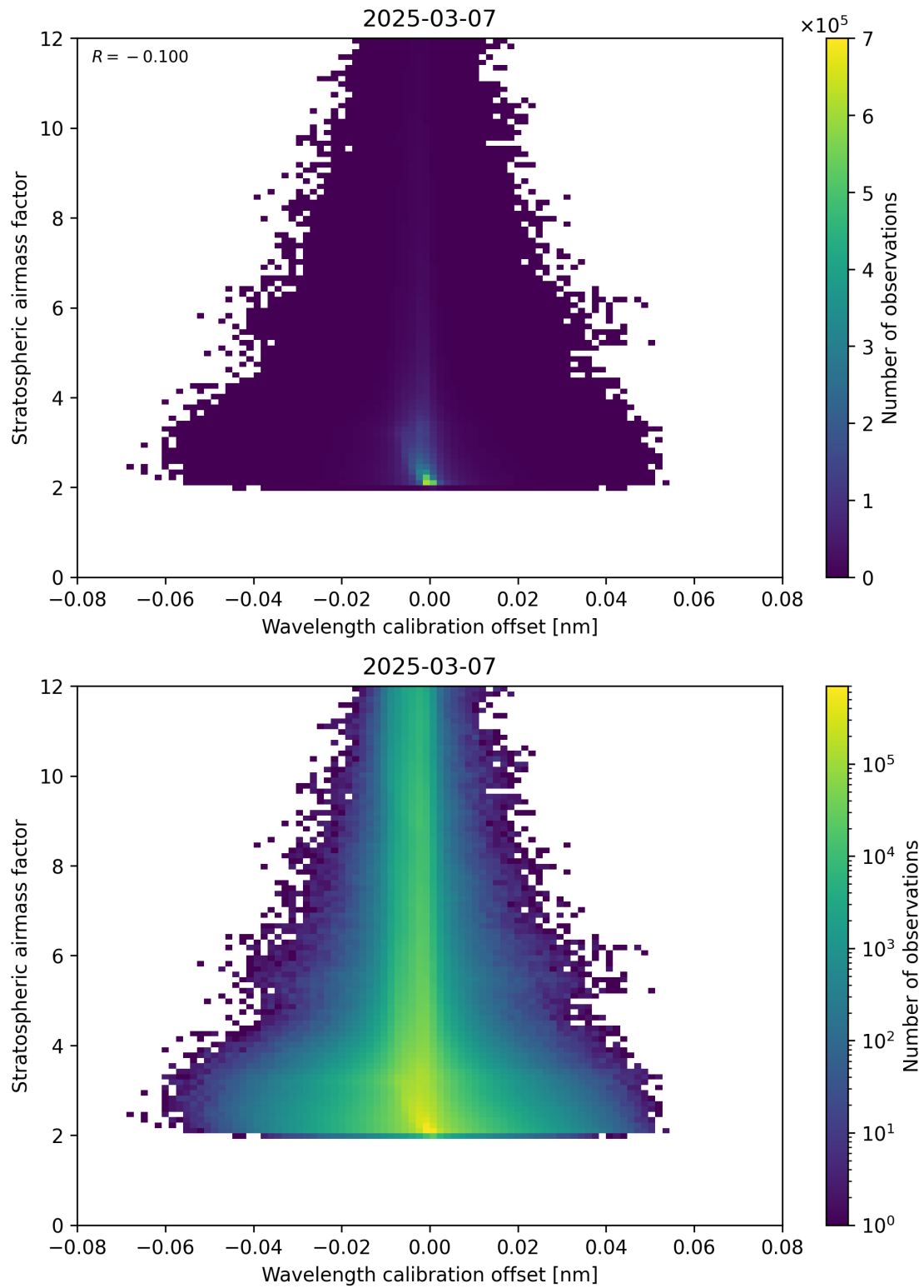
Figure 174: Scatter density plot of “Wavelength calibration offset” against “Stratospheric airmass factor” for 2025-03-07 to 2025-03-08.
