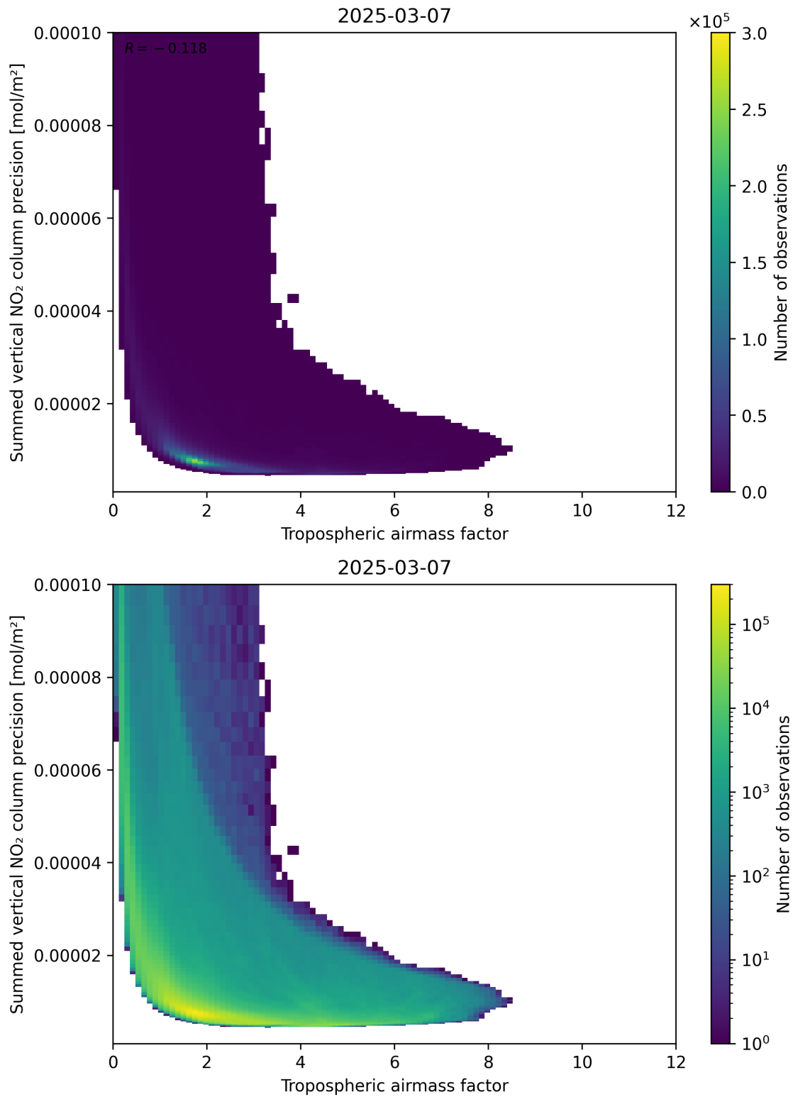
Figure 76: Scatter density plot of “Tropospheric air mass factor” against “Summed vertical NO 2 column precision” for 2025-03-07 to 2025-03-08.
