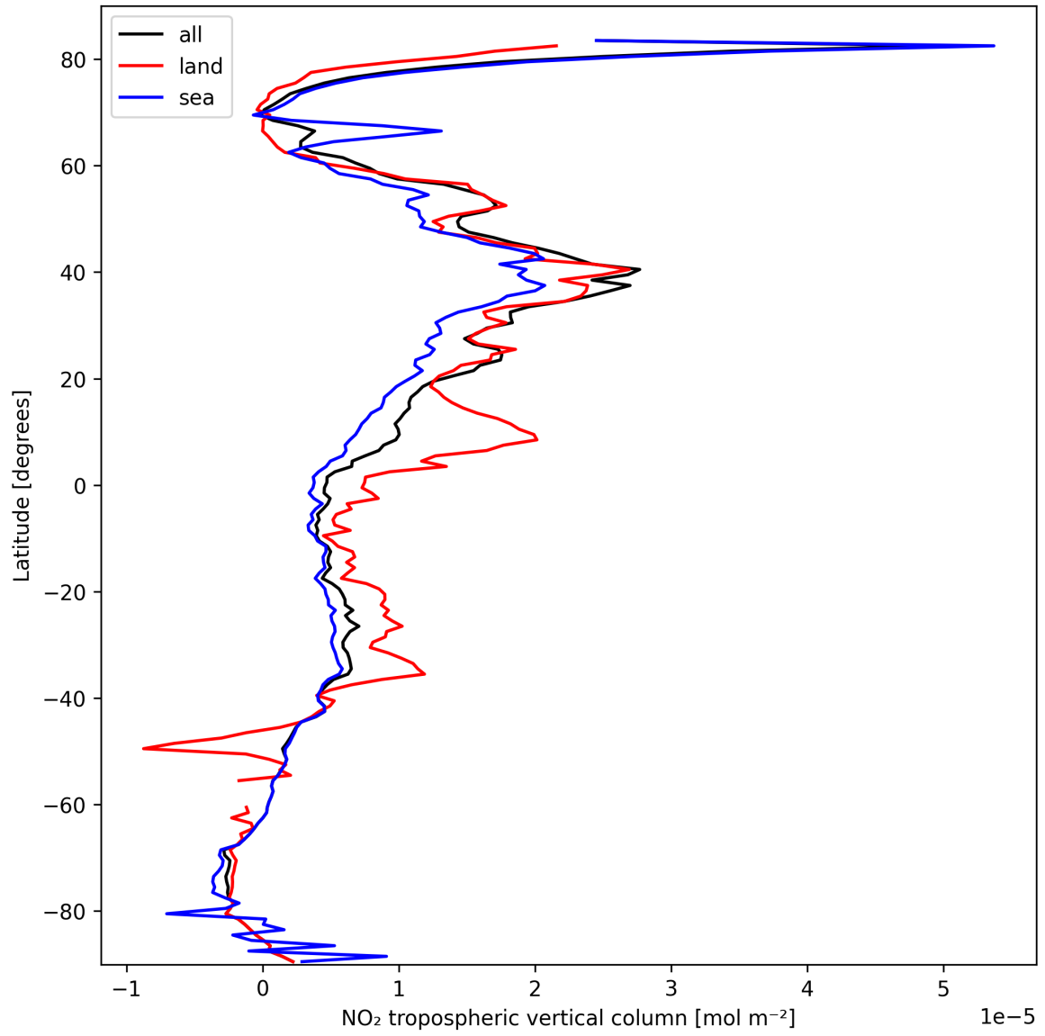
Figure 12: Zonal average of “NO 2 tropospheric vertical column” for 2025-03-07 to 2025-03-08.
