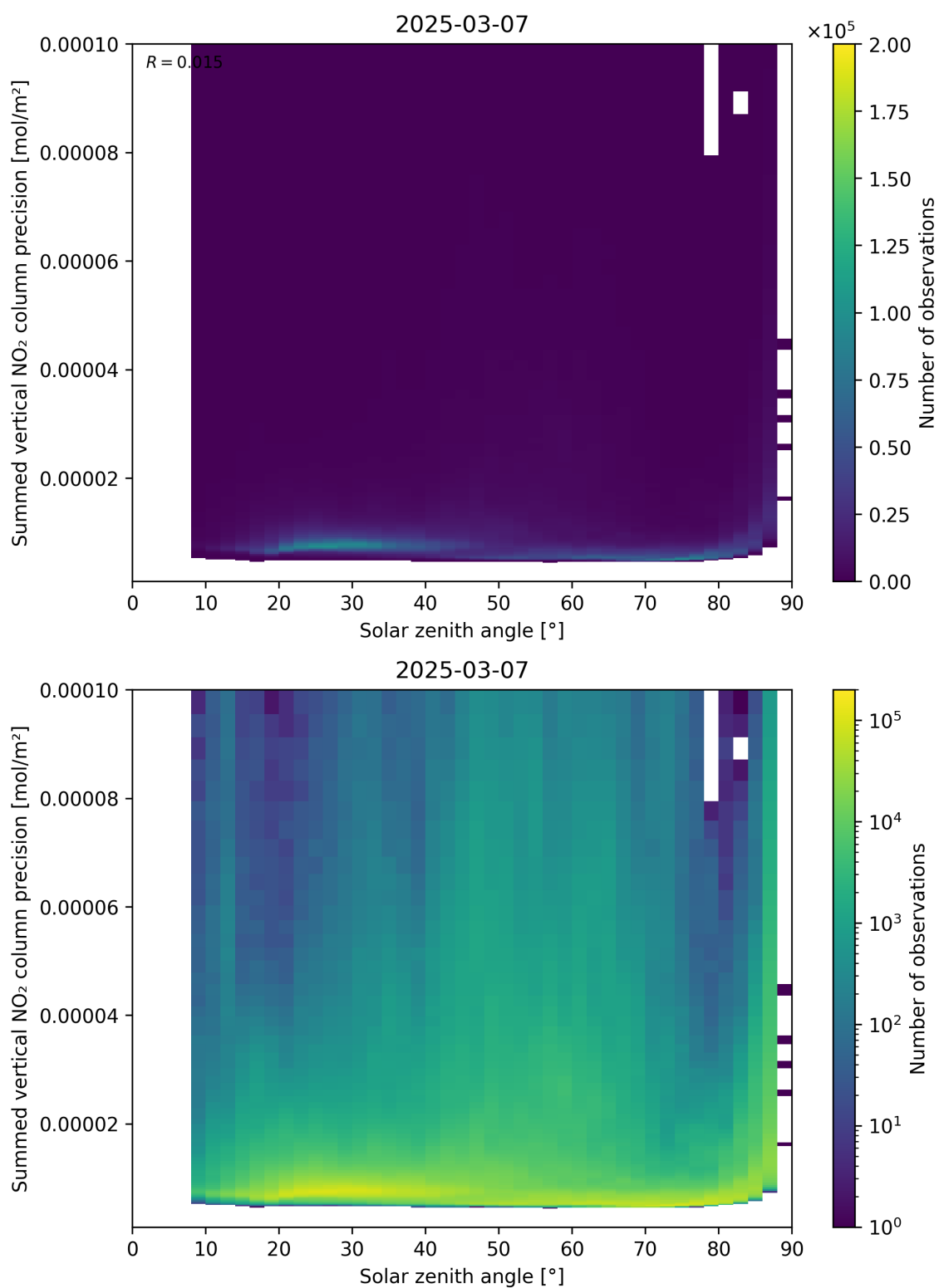
Figure 152: Scatter density plot of “Solar zenith angle” against “Summed vertical NO 2 column precision” for 2025-03-07 to 2025-03-08.
