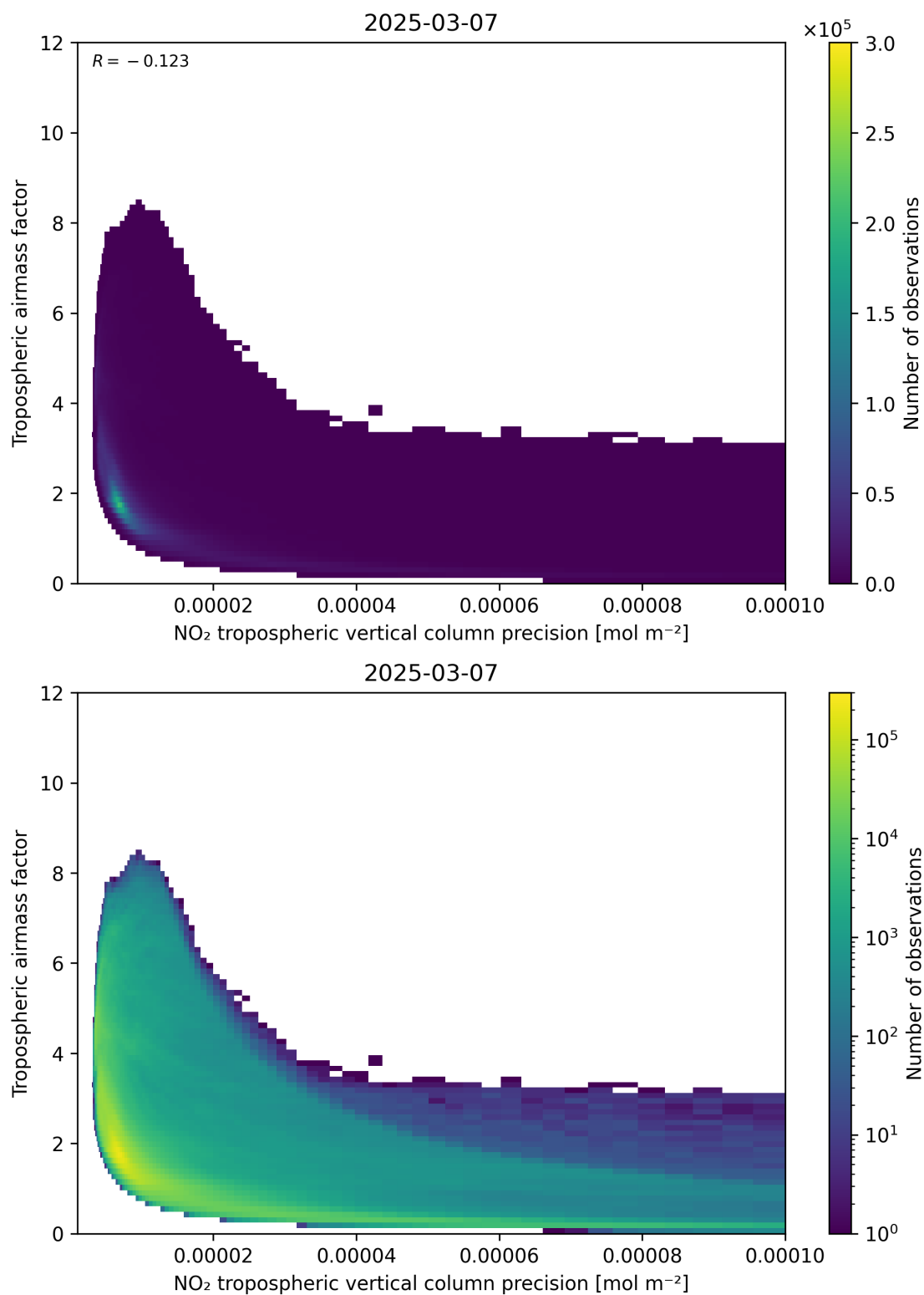
Figure 133: Scatter density plot of “NO 2 tropospheric vertical column precision” against “Tropospheric airmass factor” for 2025-03-07 to 2025-03-08.
