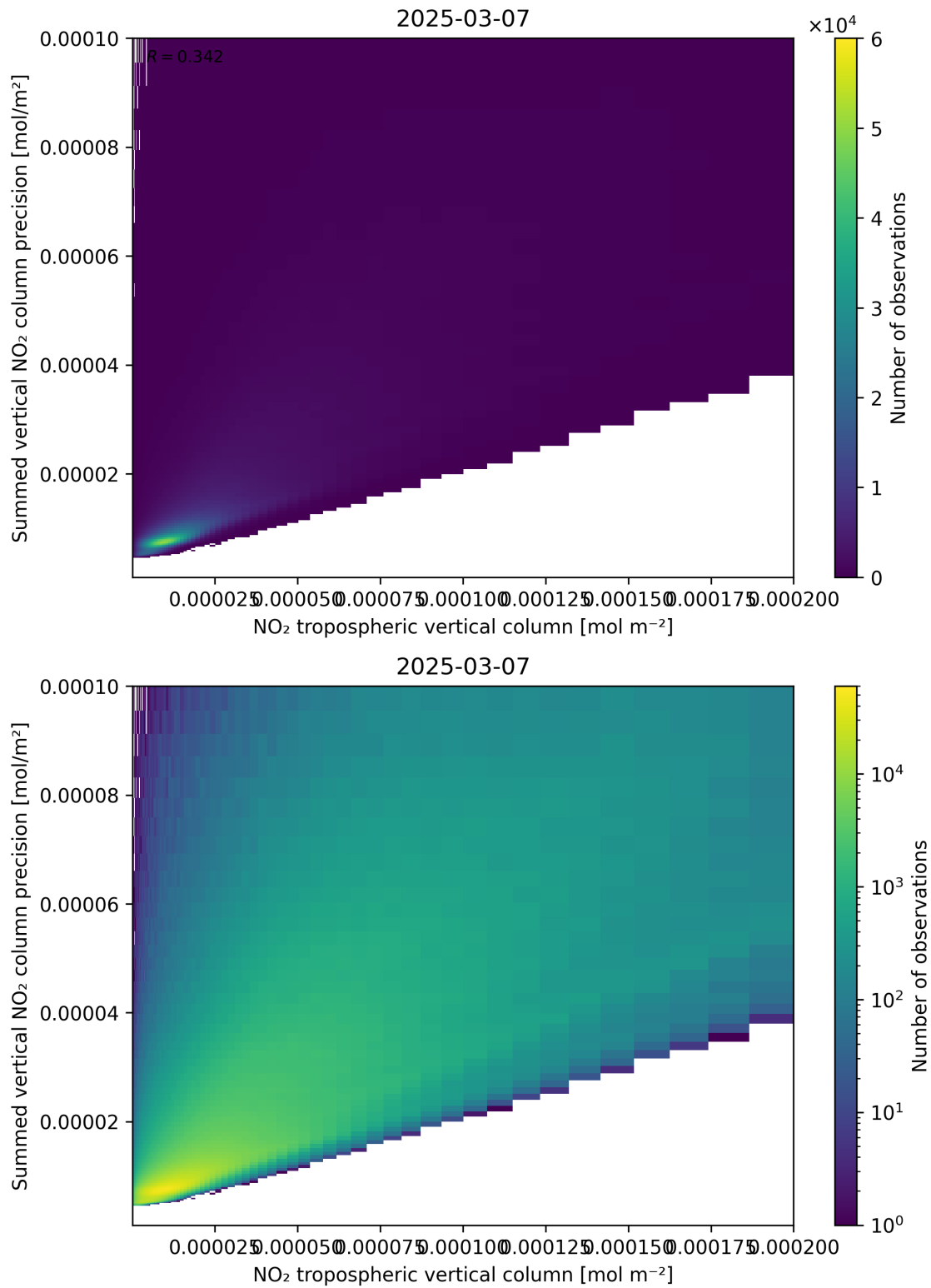
Figure 127: Scatter density plot of “NO 2 tropospheric vertical column” against “Summed vertical NO 2 column precision” for 2025-03-07 to 2025-03-08.
