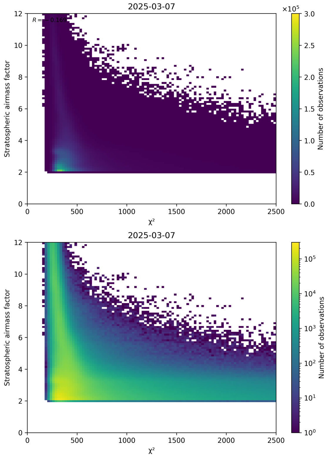
Figure 81: Scatter density plot of “ \chi^2 ” against “Stratospheric airmass factor” for 2025-03-07 to 2025-03-08.
