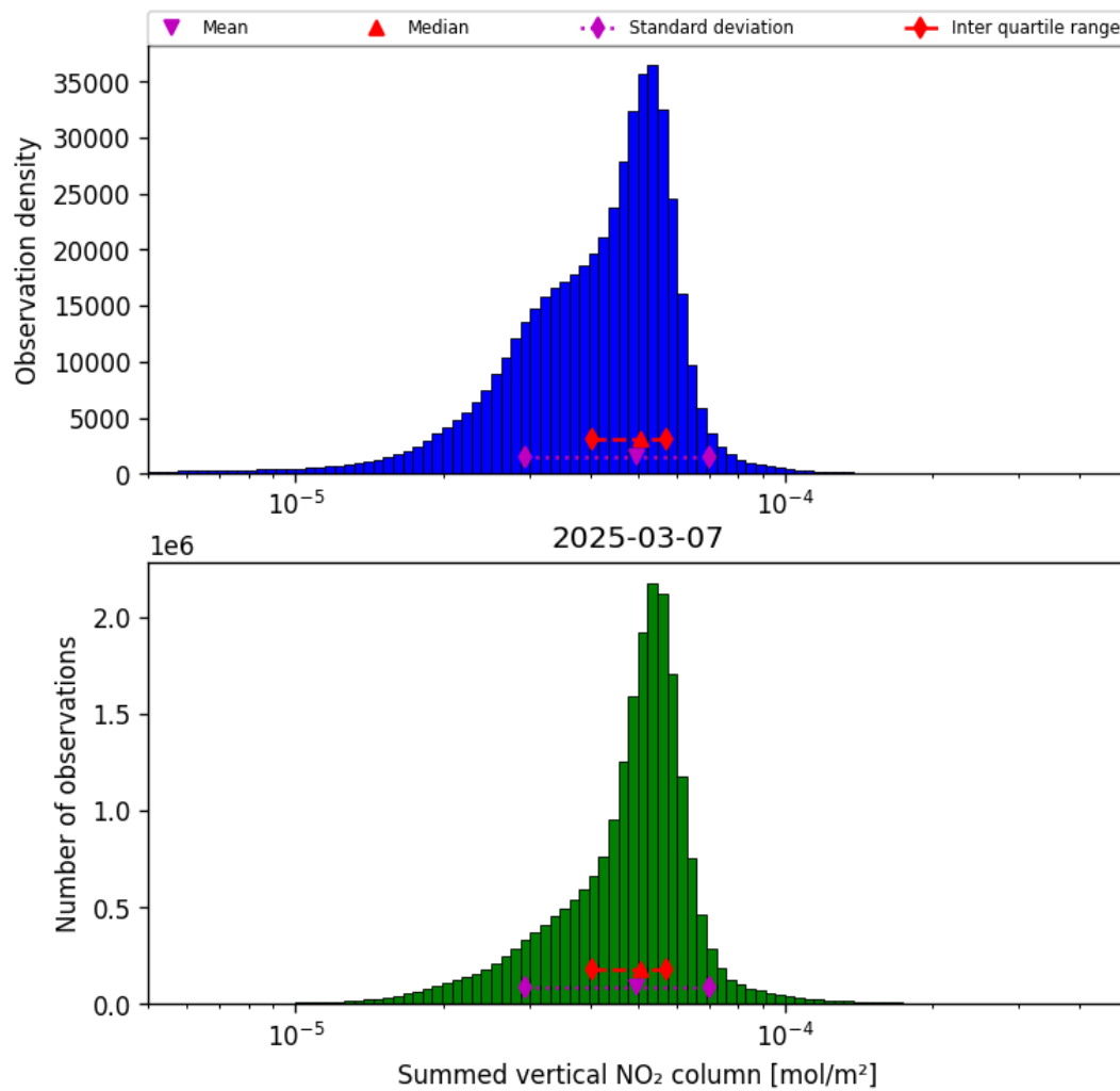
Figure 40: Histogram of “Summed vertical NO 2 column” for 2025-03-07 to 2025-03-08
