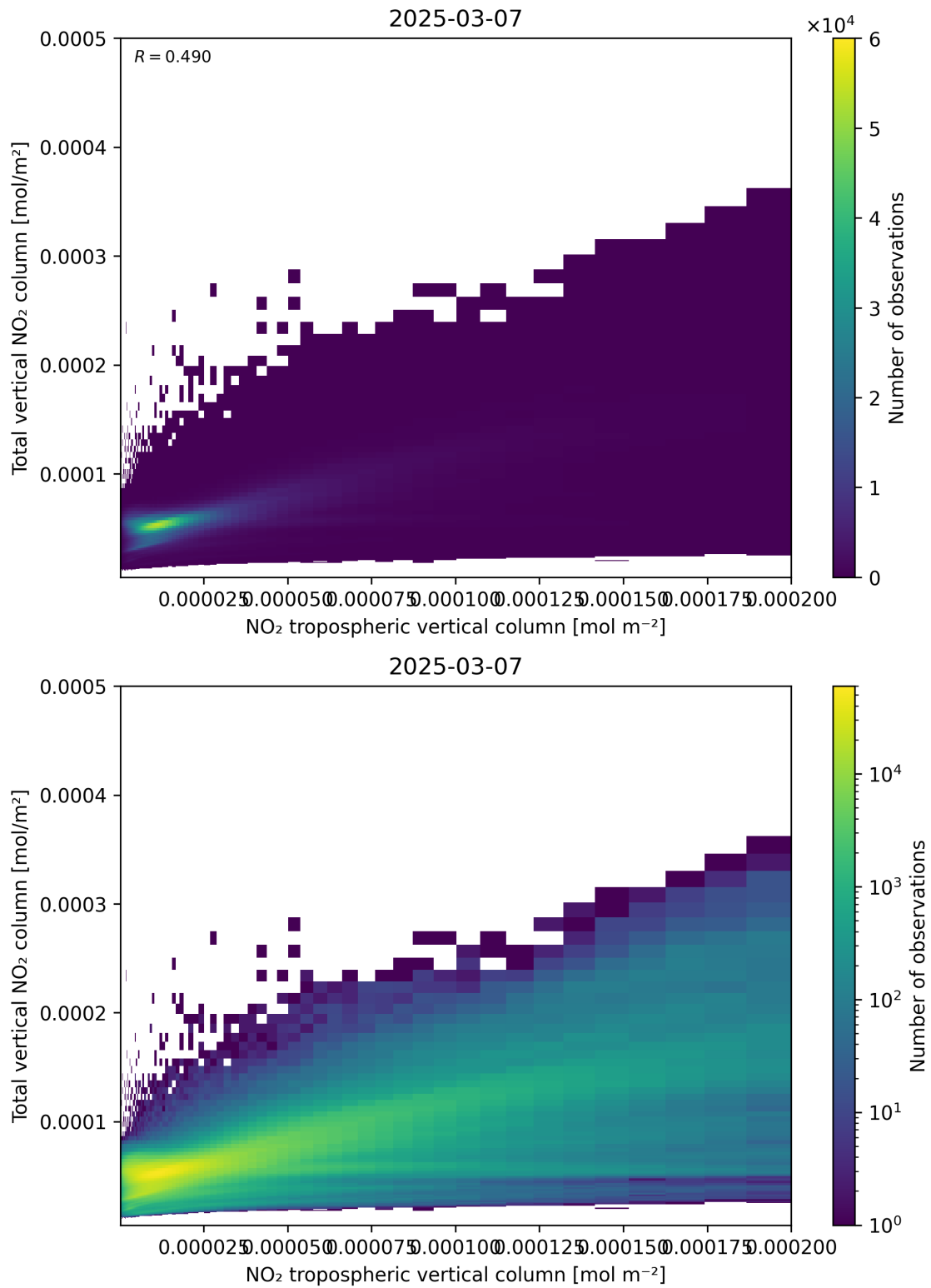
Figure 128: Scatter density plot of “NO 2 tropospheric vertical column” against “Total vertical NO 2 column” for 2025-03-07 to 2025-03-08.
