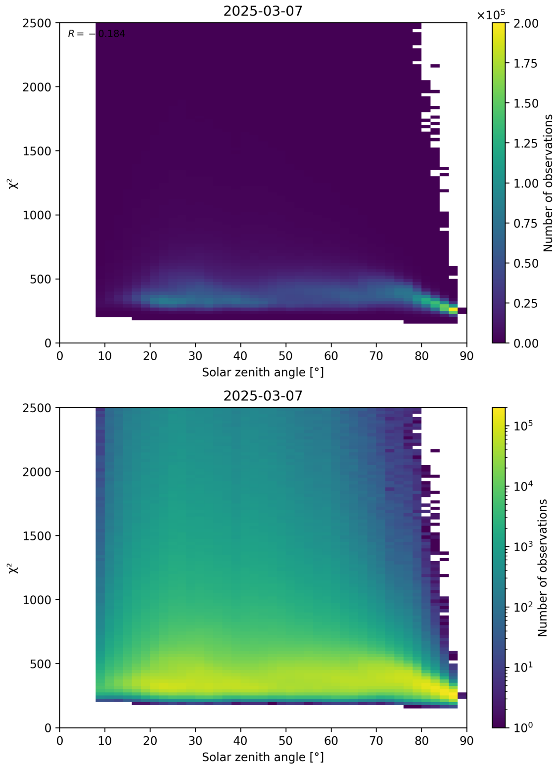
Figure 148: Scatter density plot of “Solar zenith angle” against “ \chi^2 ” for 2025-03-07 to 2025-03-08.
