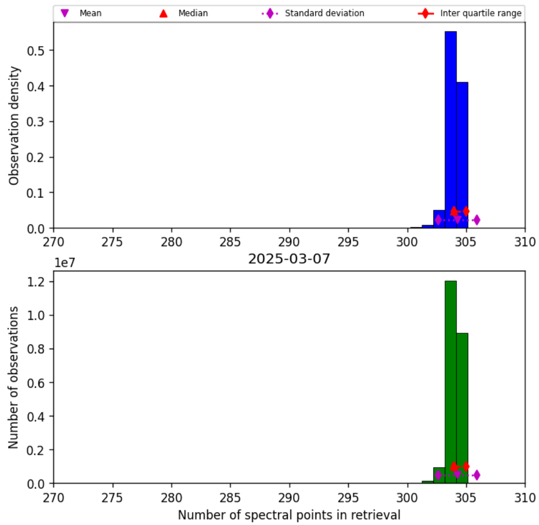
Figure 33: Histogram of “Number of spectral points in retrieval” for 2025-03-07 to 2025-03-08
