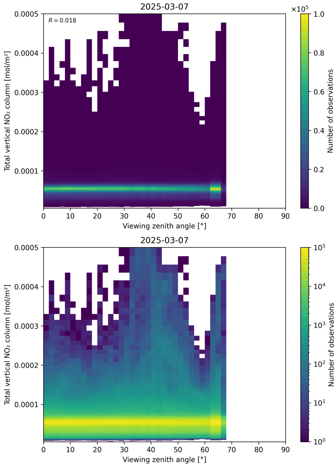
Figure 167: Scatter density plot of “Viewing zenith angle” against “Total vertical NO 2 column” for 2025-03-07 to 2025-03-08.
