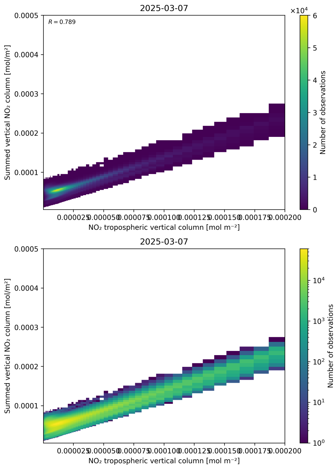
Figure 126: Scatter density plot of “NO 2 tropospheric vertical column” against “Summed vertical NO 2 column” for 2025-03-07 to 2025-03-08.
