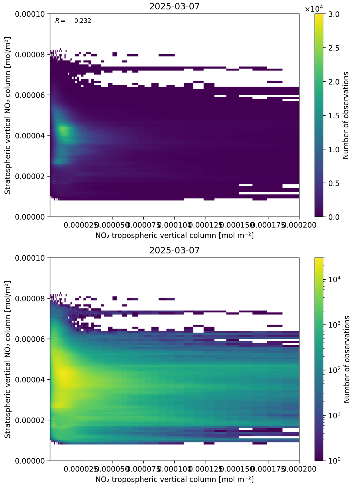
Figure 125: Scatter density plot of “NO 2 tropospheric vertical column” against “Stratospheric vertical NO 2 column” for 2025-03-07 to 2025-03-08.
