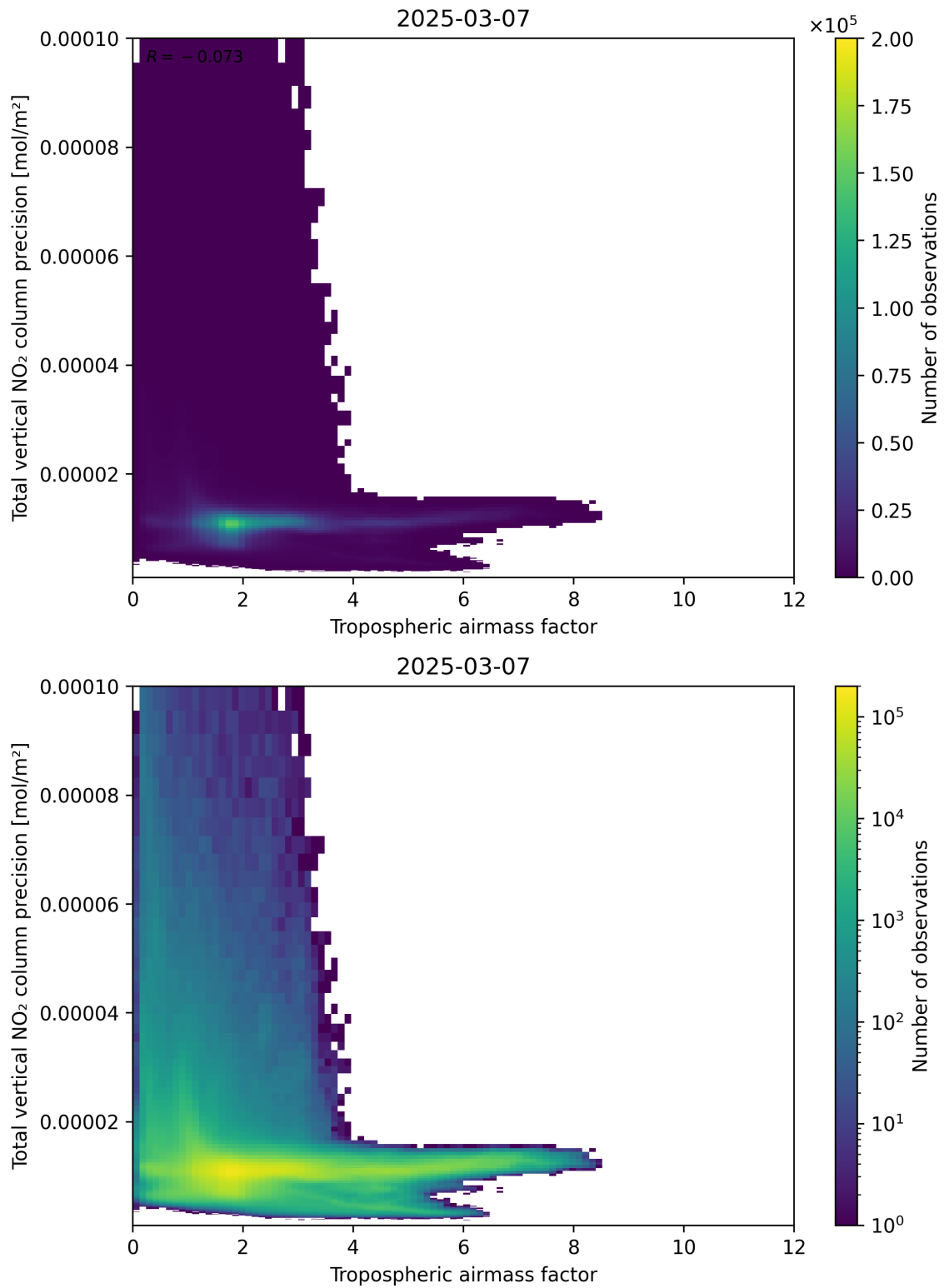
Figure 78: Scatter density plot of “Tropospheric air mass factor” against “Total vertical NO 2 column precision” for 2025-03-07 to 2025-03-08.
