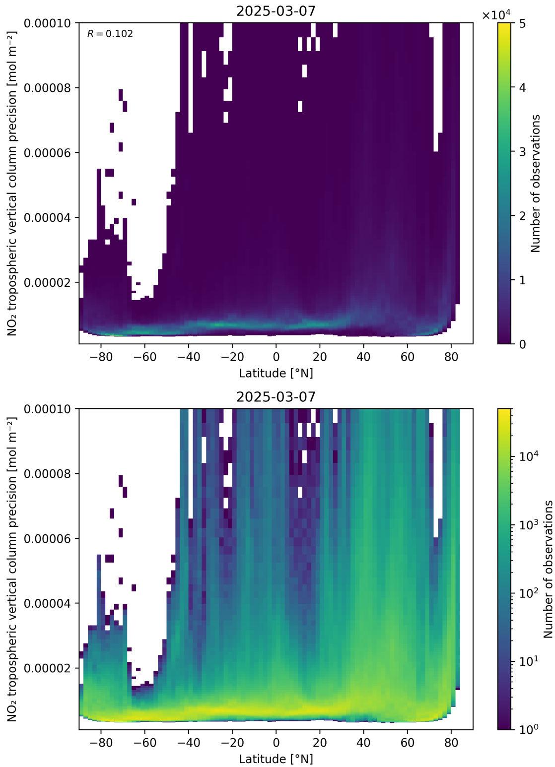
Figure 93: Scatter density plot of “Latitude” against “NO 2 tropospheric vertical column precision” for 2025-03-07 to 2025-03-08.
