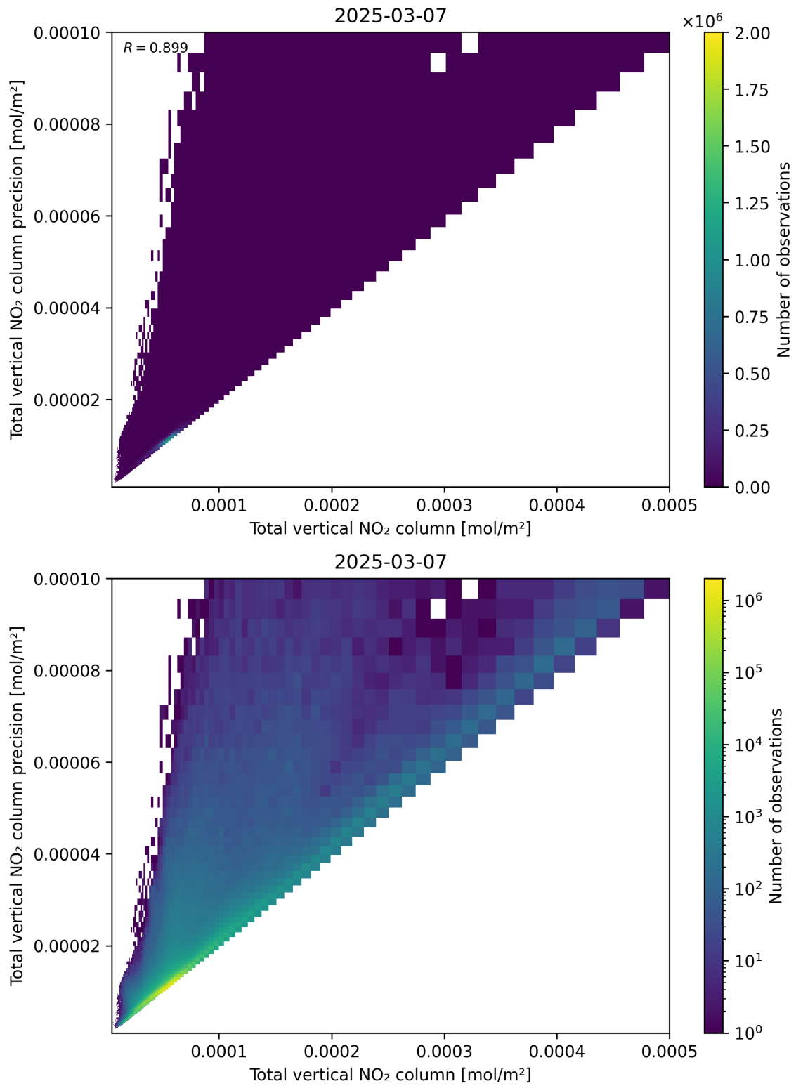
Figure 114: Scatter density plot of “Total vertical NO 2 column” against “Total vertical NO 2 column precision” for 2025-03-07 to 2025-03-08.
