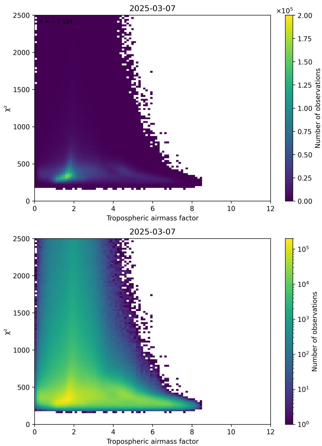
Figure 73: Scatter density plot of “Tropospheric airmass factor” against “ \chi^2 ” for 2025-03-07 to 2025-03-08.
