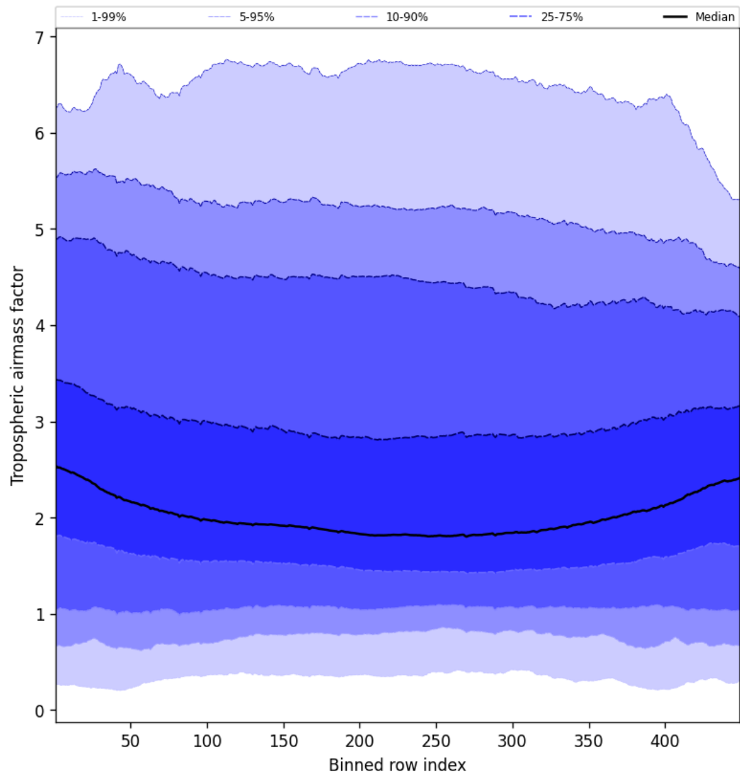
Figure 48: Along track statistics of “Tropospheric air mass factor” for 2025-03-07 to 2025-03-08
