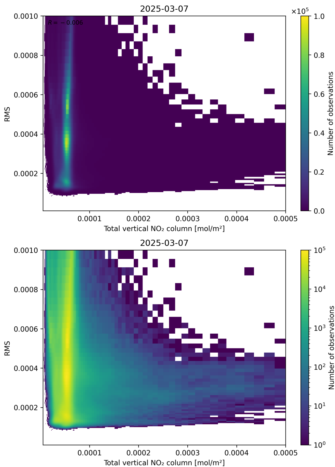
Figure 120: Scatter density plot of “Total vertical NO 2 column” against “RMS” for 2025-03-07 to 2025-03-08.
