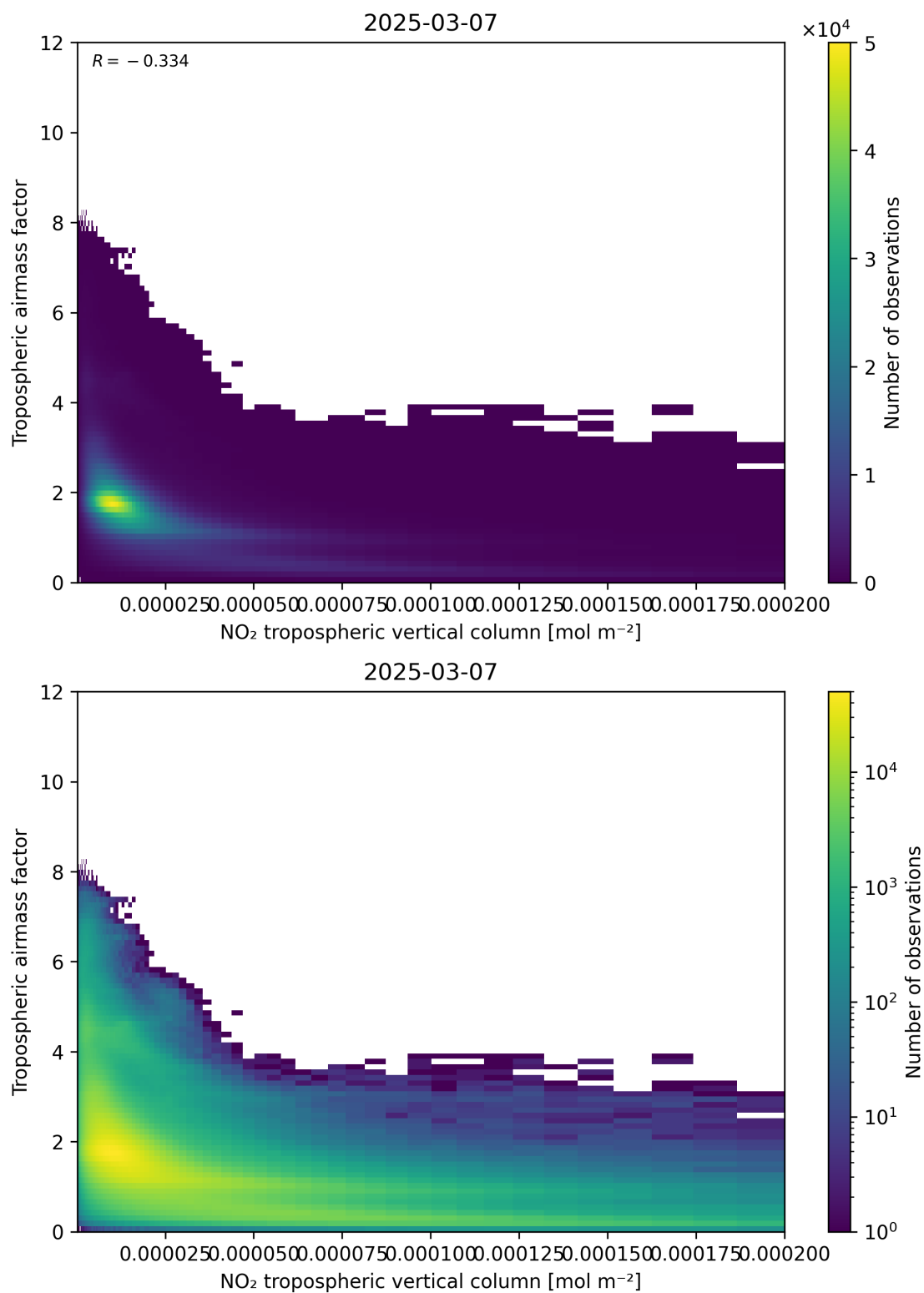
Figure 123: Scatter density plot of “NO 2 tropospheric vertical column” against “Tropospheric air mass factor” for 2025-03-07 to 2025-03-08.
