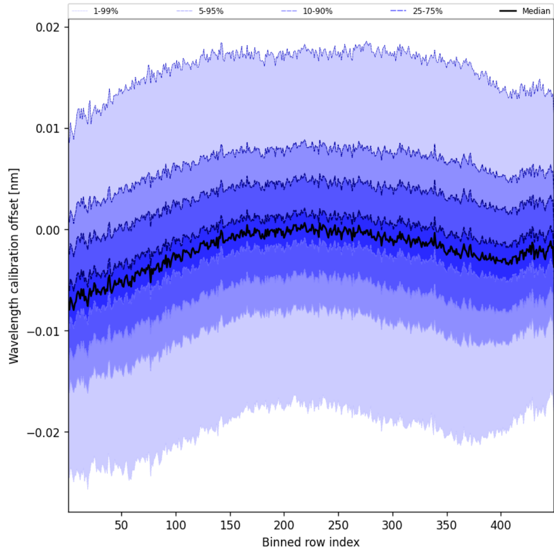
Figure 52: Along track statistics of “Wavelength calibration offset” for 2025-03-07 to 2025-03-08
