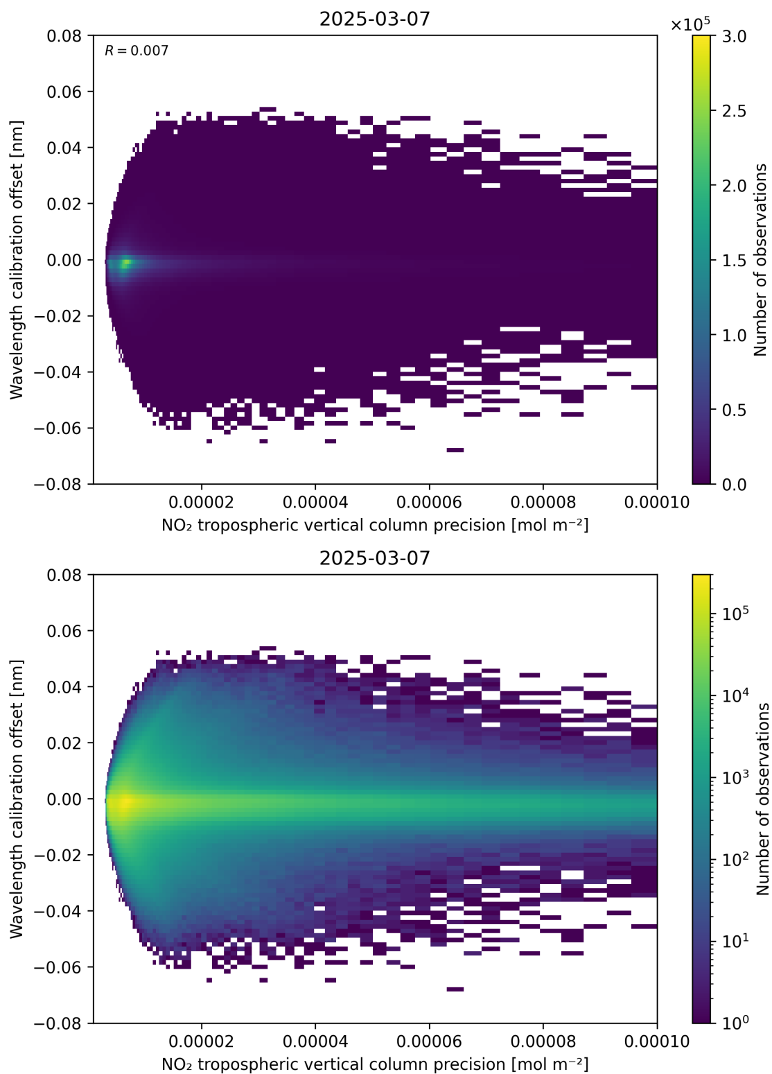
Figure 141: Scatter density plot of “NO 2 tropospheric vertical column precision” against “Wavelength calibration offset” for 2025-03-07 to 2025-03-08.
