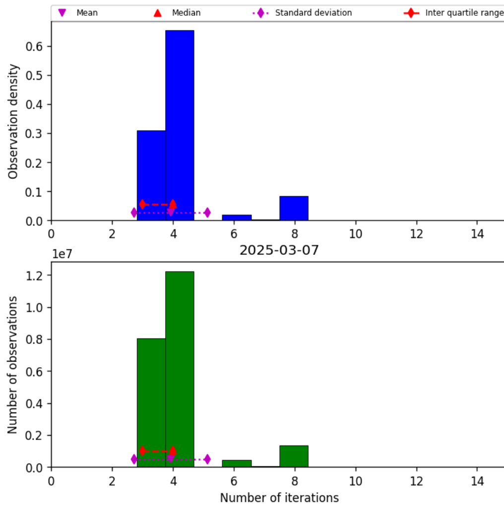
Figure 34: Histogram of “Number of iterations” for 2025-03-07 to 2025-03-08
