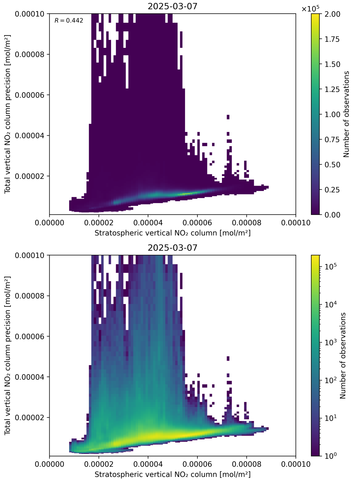
Figure 101: Scatter density plot of “Stratospheric vertical NO 2 column” against “Total vertical NO 2 column precision” for 2025-03-07 to 2025-03-08.
