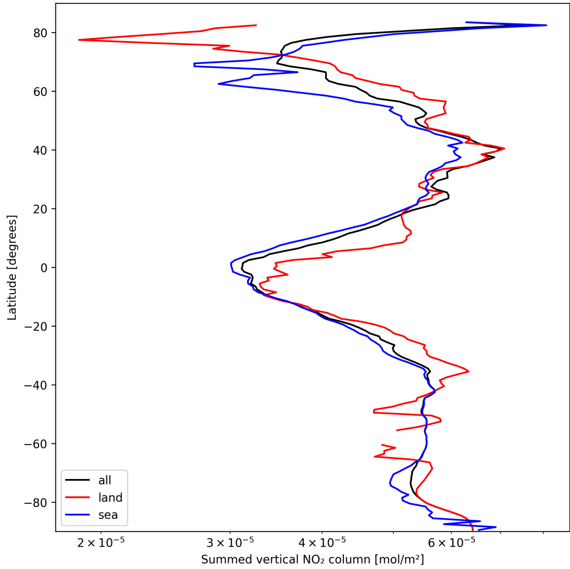
Figure 23: Zonal average of “Summed vertical NO 2 column” for 2025-03-07 to 2025-03-08.
