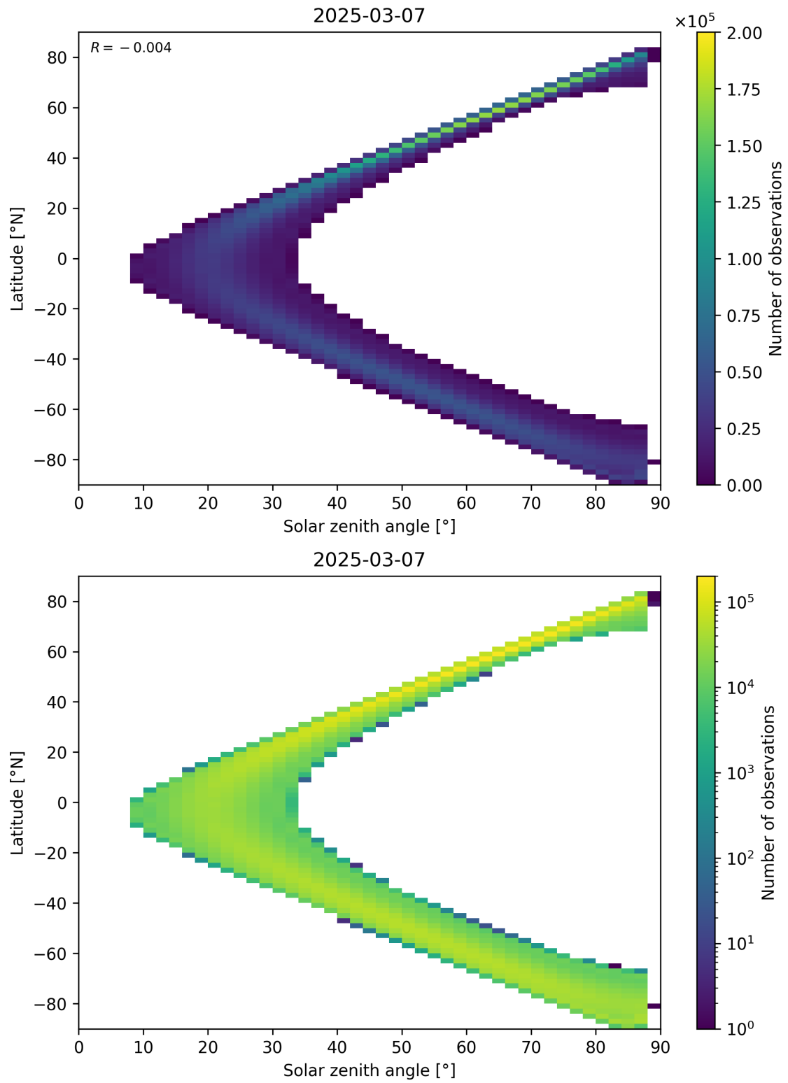
Figure 149: Scatter density plot of “Solar zenith angle” against “Latitude” for 2025-03-07 to 2025-03-08.
