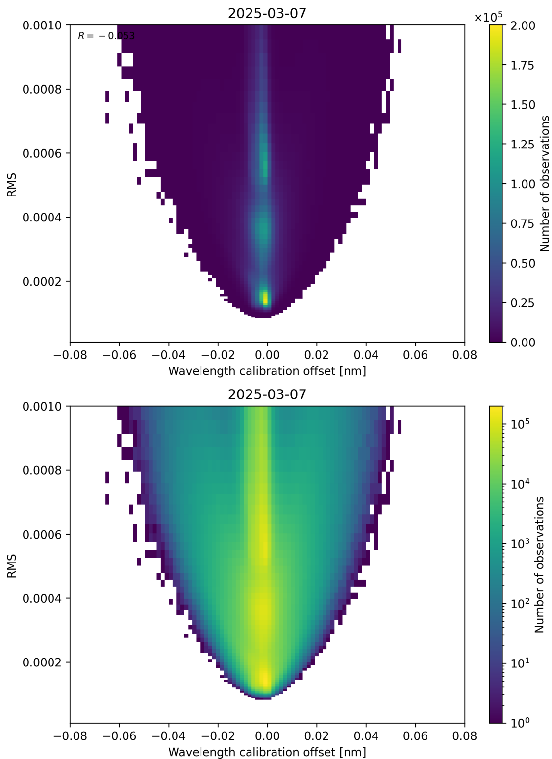
Figure 181: Scatter density plot of “Wavelength calibration offset” against “RMS” for 2025-03-07 to 2025-03-08.
