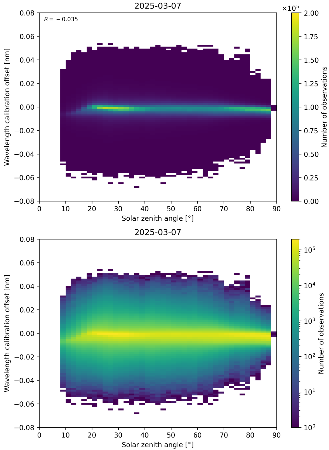
Figure 158: Scatter density plot of “Solar zenith angle” against “Wavelength calibration offset” for 2025-03-07 to 2025-03-08.
