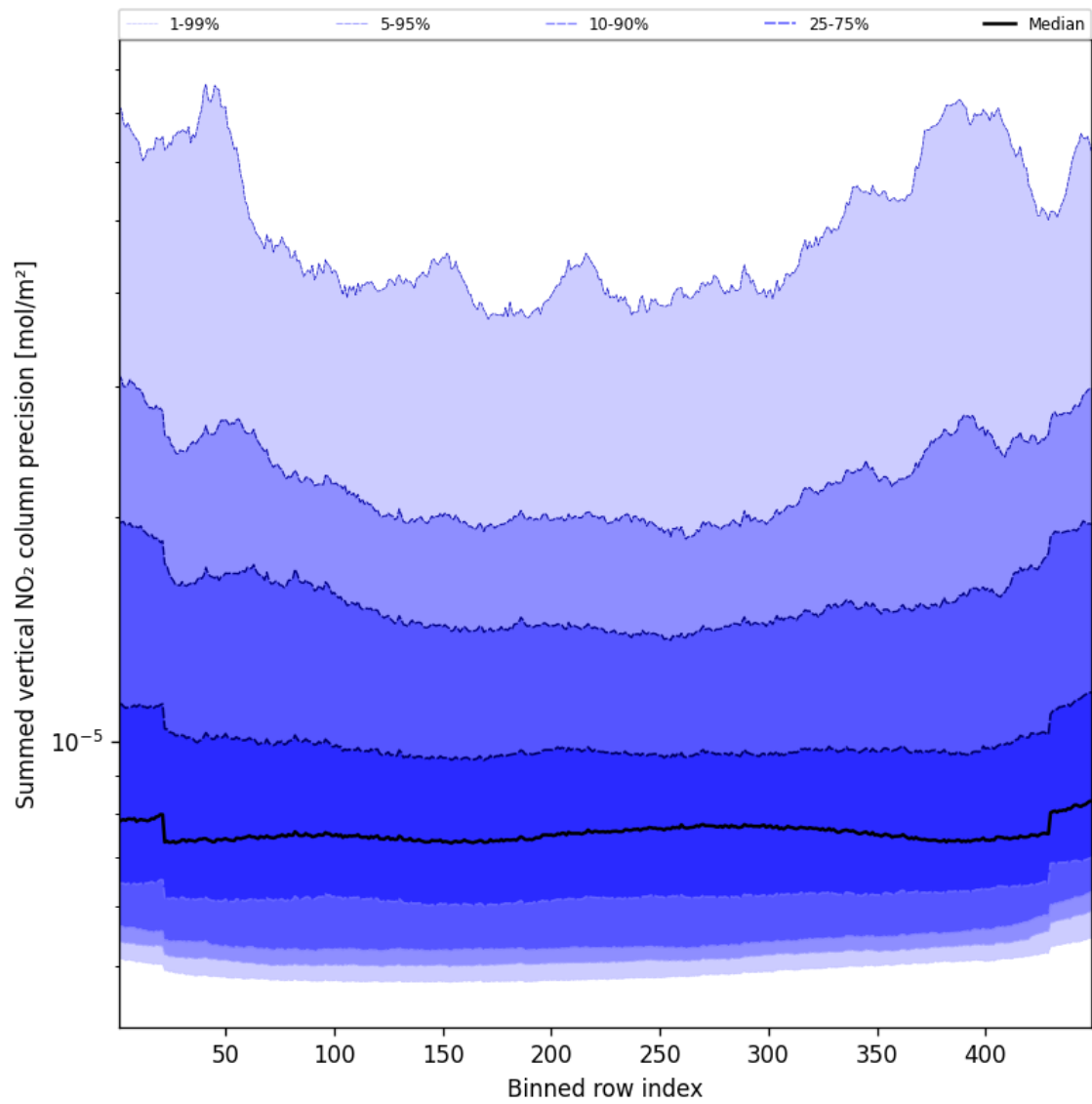
Figure 58: Along track statistics of “Summed vertical NO 2 column precision” for 2025-03-07 to 2025-03-08
