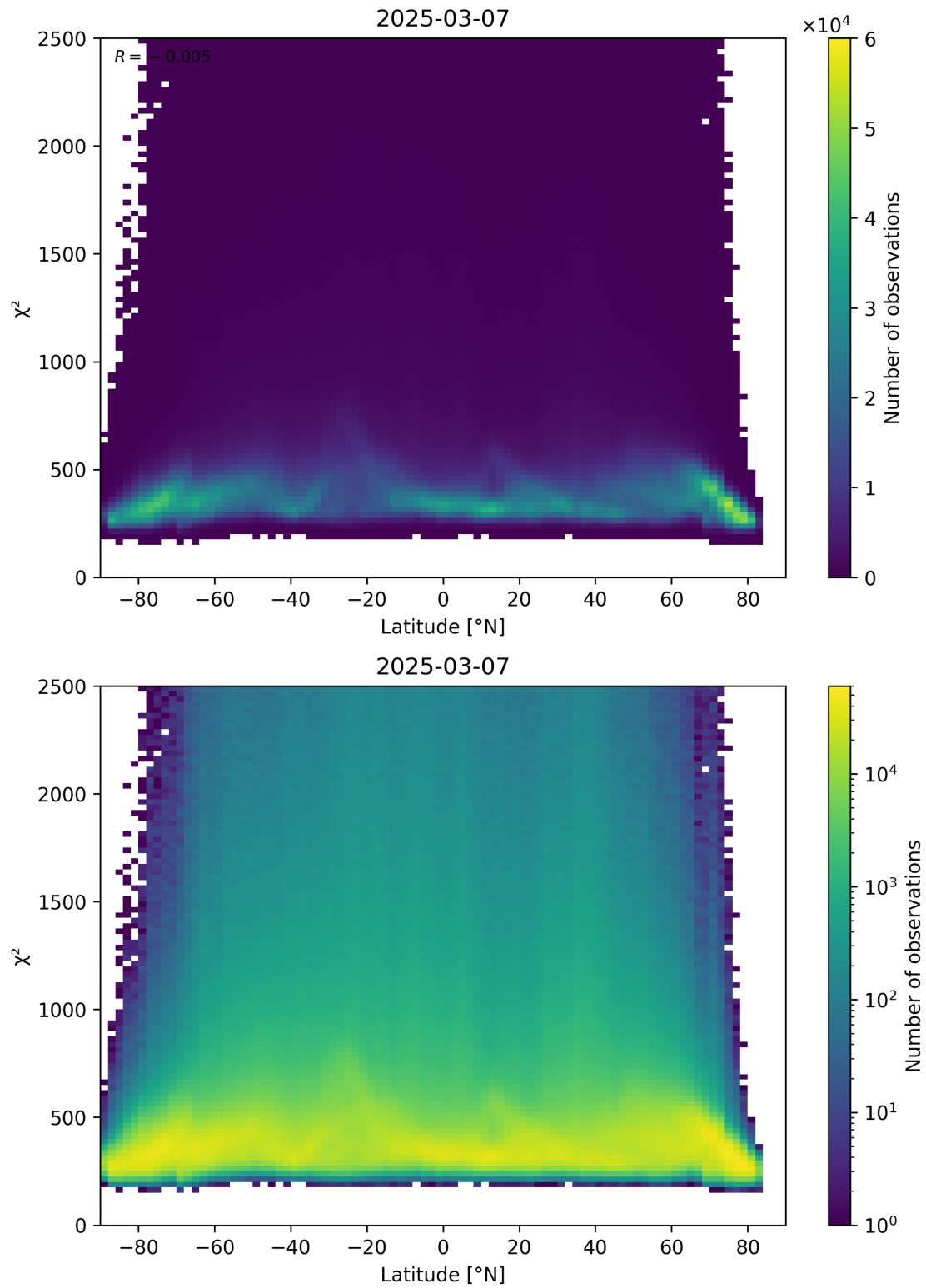
Figure 86: Scatter density plot of “Latitude” against “ \chi^2 ” for 2025-03-07 to 2025-03-08.
