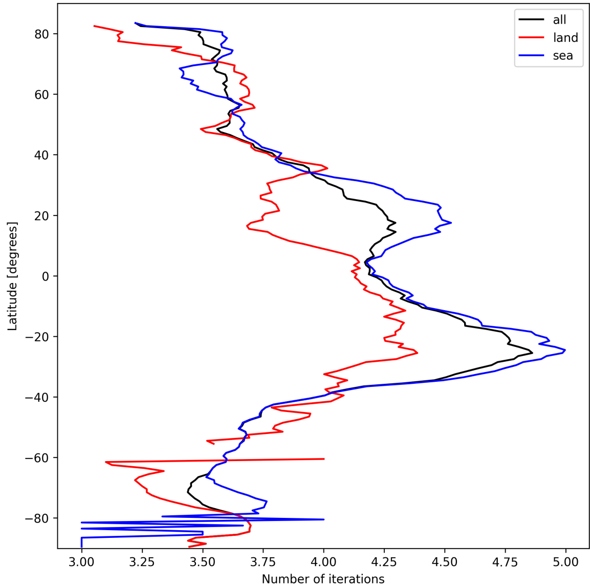
Figure 17: Zonal average of “Number of iterations” for 2025-03-07 to 2025-03-08.
