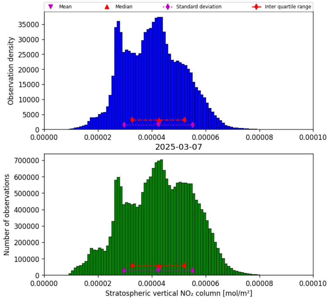
Figure 36: Histogram of “Stratospheric vertical NO 2 column” for 2025-03-07 to 2025-03-08
