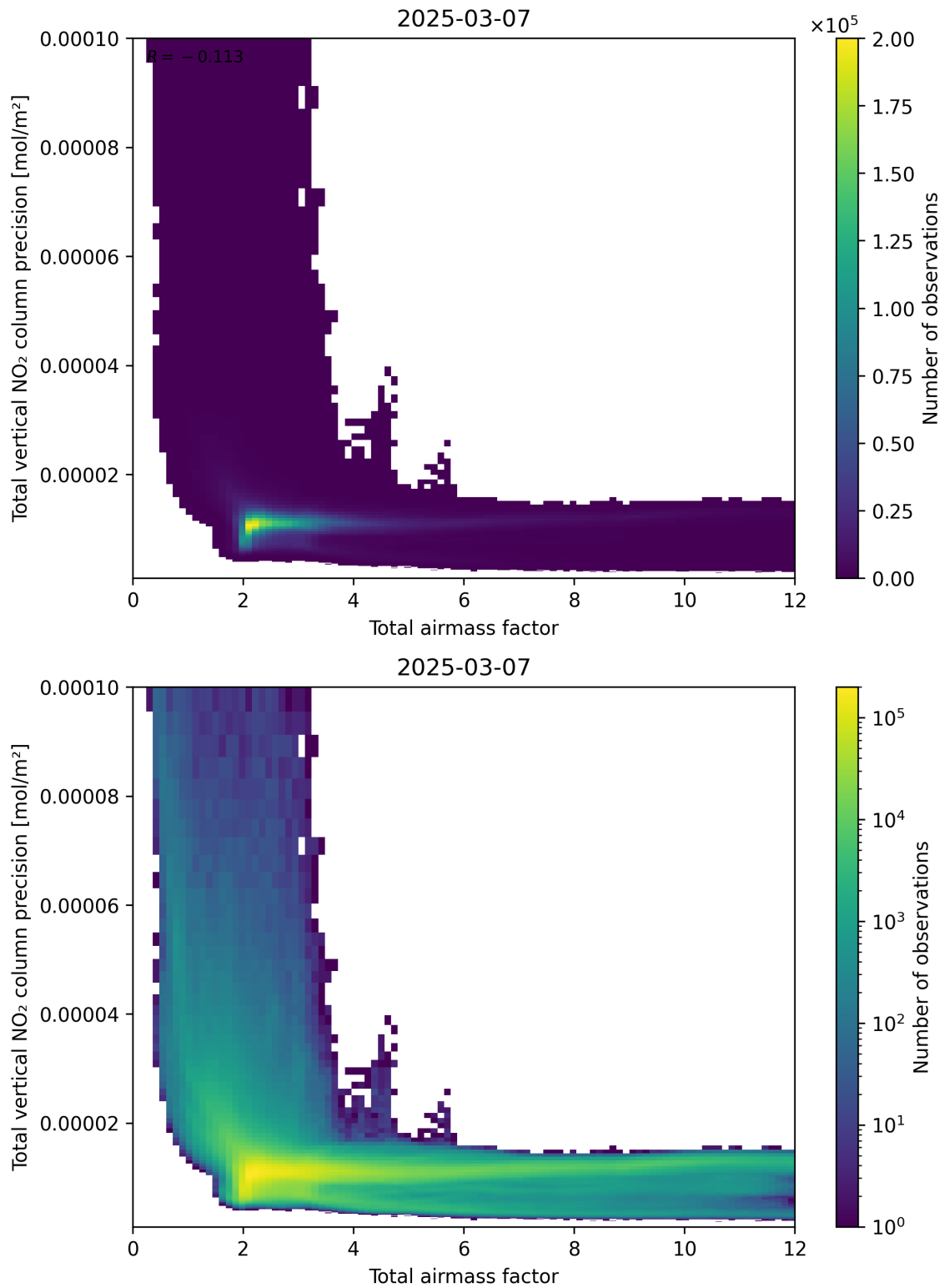
Figure 68: Scatter density plot of “Total airmass factor” against “Total vertical NO 2 column precision” for 2025-03-07 to 2025-03-08.
