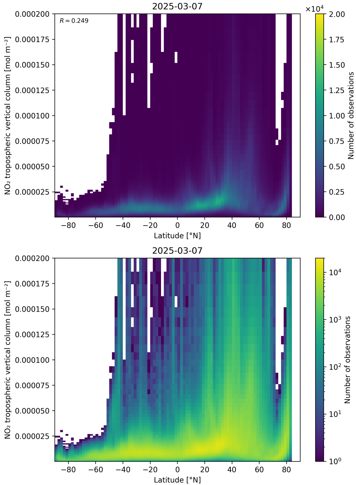
Figure 92: Scatter density plot of “Latitude” against “NO 2 tropospheric vertical column” for 2025-03-07 to 2025-03-08.
