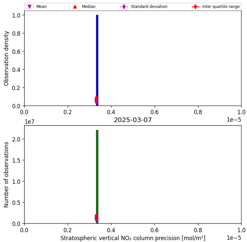
Figure 37: Histogram of “Stratospheric vertical NO 2 column precision” for 2025-03-07 to 2025-03-08
