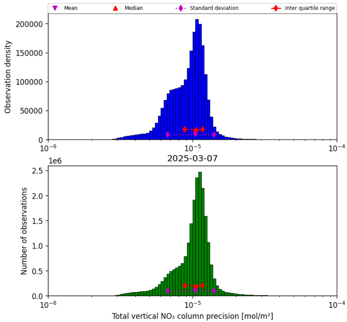
Figure 39: Histogram of “Total vertical NO 2 column precision” for 2025-03-07 to 2025-03-08
