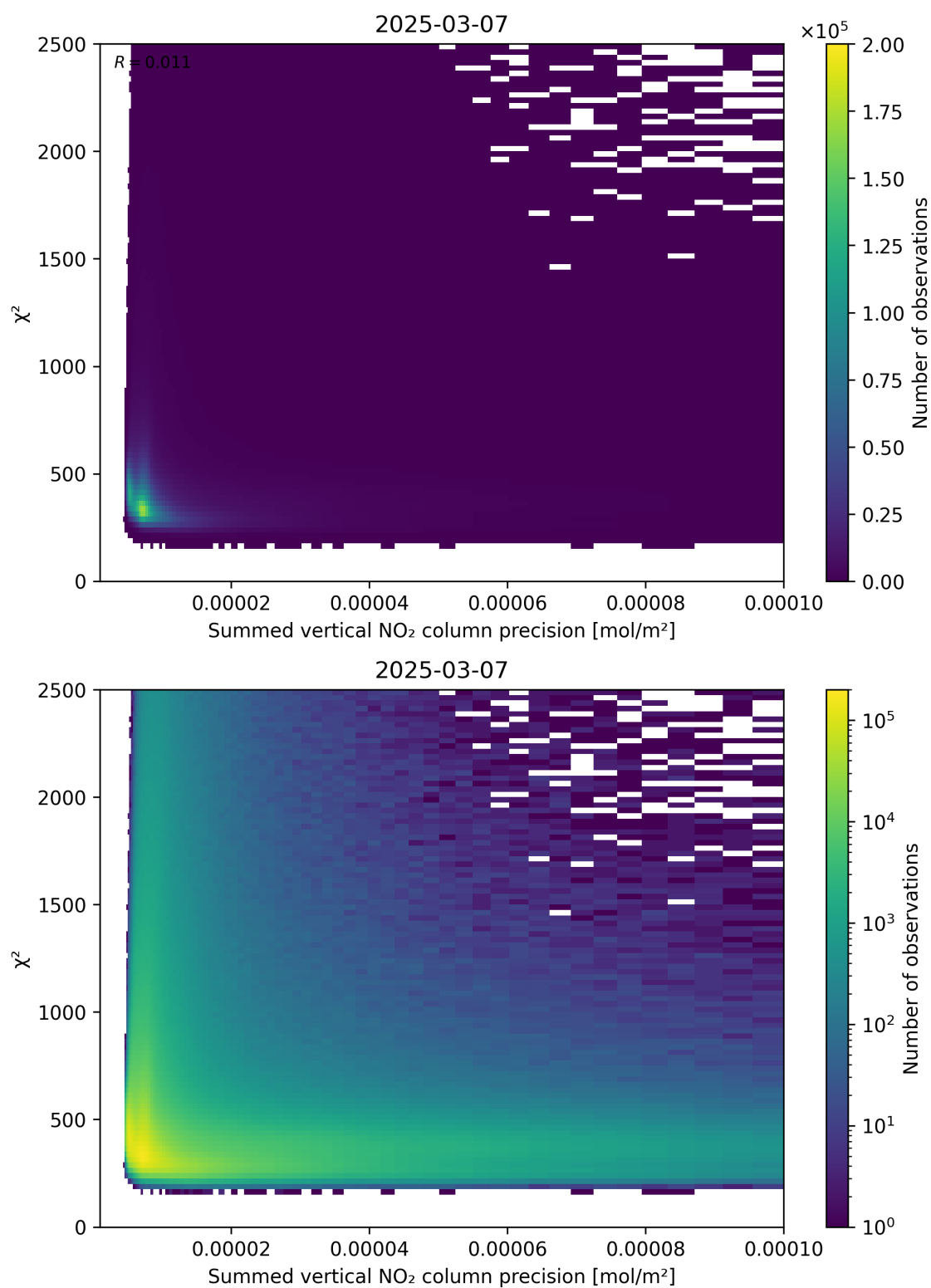
Figure 107: Scatter density plot of “Summed vertical NO 2 column precision” against “ \chi^2 ” for 2025-03-07 to 2025-03-08.
