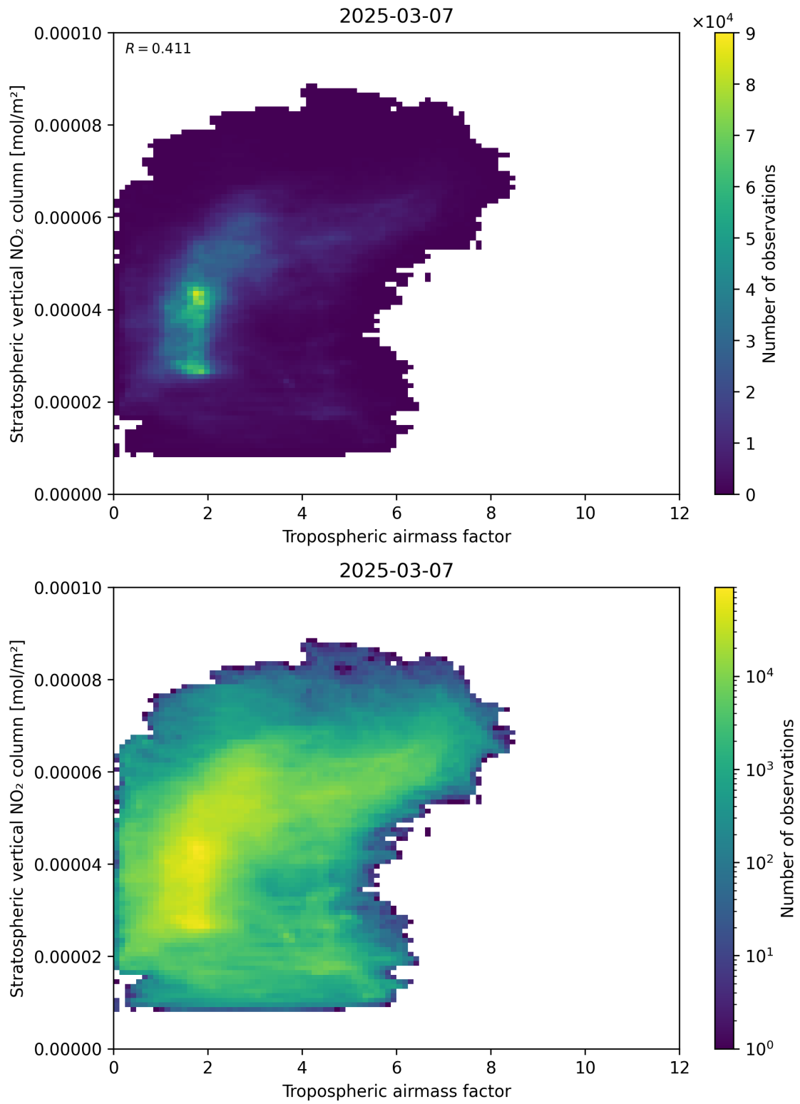
Figure 74: Scatter density plot of “Tropospheric air mass factor” against “Stratospheric vertical NO 2 column” for 2025-03-07 to 2025-03-08.
