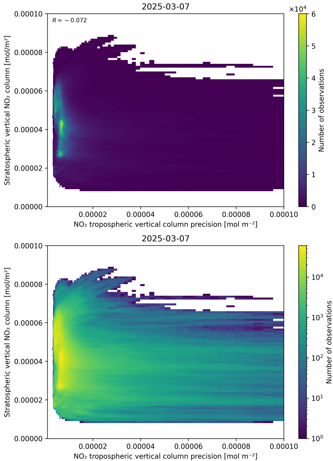
Figure 135: Scatter density plot of “NO 2 tropospheric vertical column precision” against “Stratospheric vertical NO 2 column” for 2025-03-07 to 2025-03-08.
