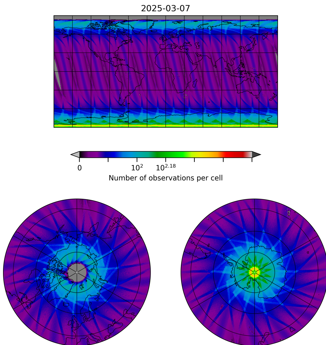
Figure 10: Map of the number of observations for 2025-03-07 to 2025-03-08
