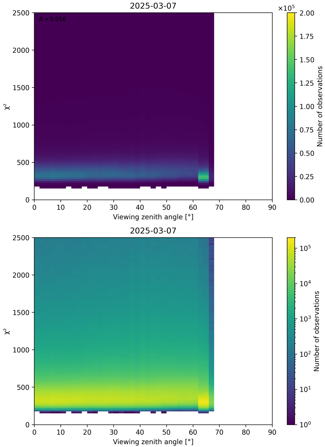
Figure 162: Scatter density plot of “Viewing zenith angle” against “ \chi^2 ” for 2025-03-07 to 2025-03-08.
