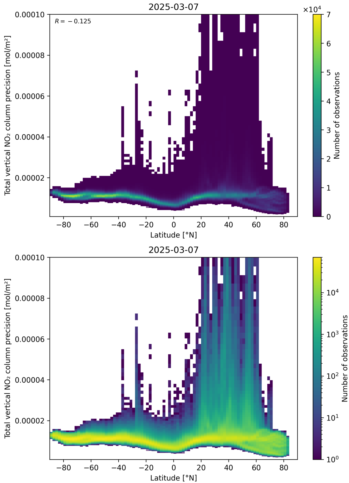
Figure 91: Scatter density plot of “Latitude” against “Total vertical NO 2 column precision” for 2025-03-07 to 2025-03-08.
