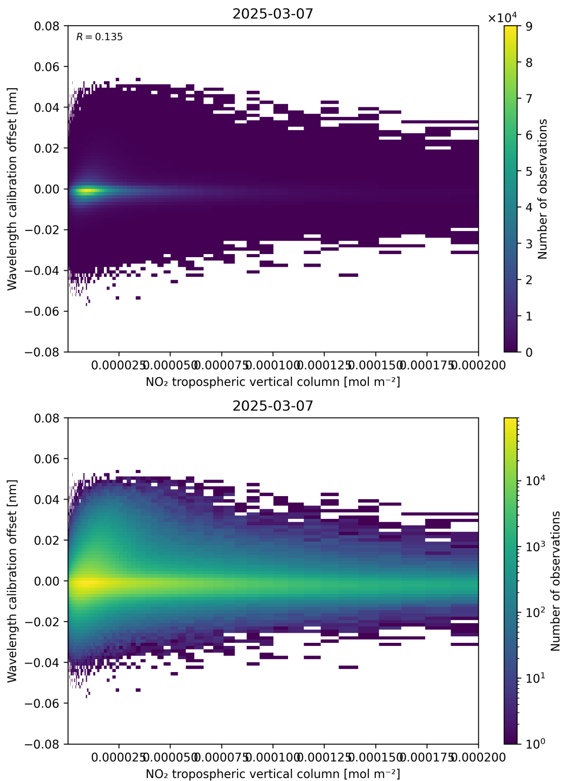
Figure 143: Scatter density plot of “NO 2 tropospheric vertical column” against “Wavelength calibration offset” for 2025-03-07 to 2025-03-08.
