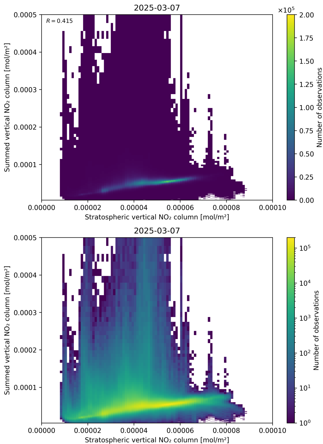
Figure 98: Scatter density plot of “Stratospheric vertical NO 2 column” against “Summed vertical NO 2 column” for 2025-03-07 to 2025-03-08.
