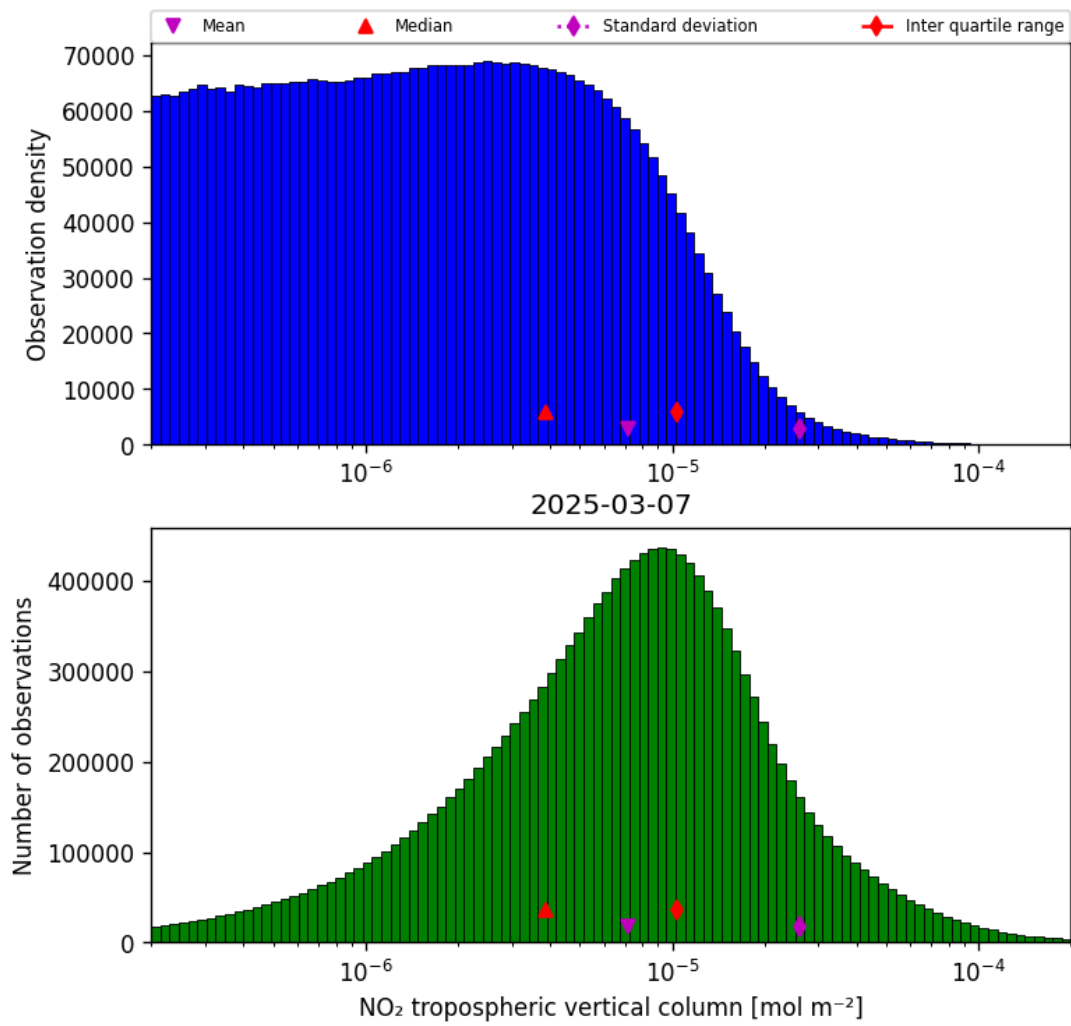
Figure 29: Histogram of “NO 2 tropospheric vertical column” for 2025-03-07 to 2025-03-08
