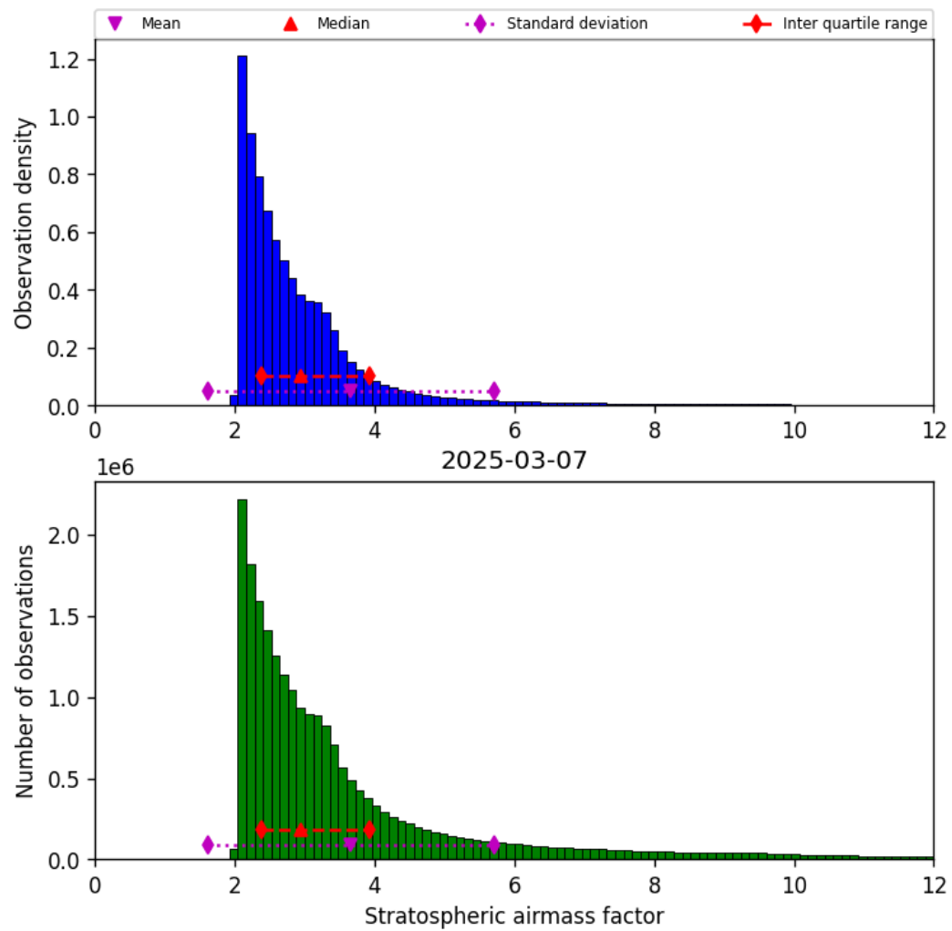
Figure 44: Histogram of “Stratospheric airmass factor” for 2025-03-07 to 2025-03-08
