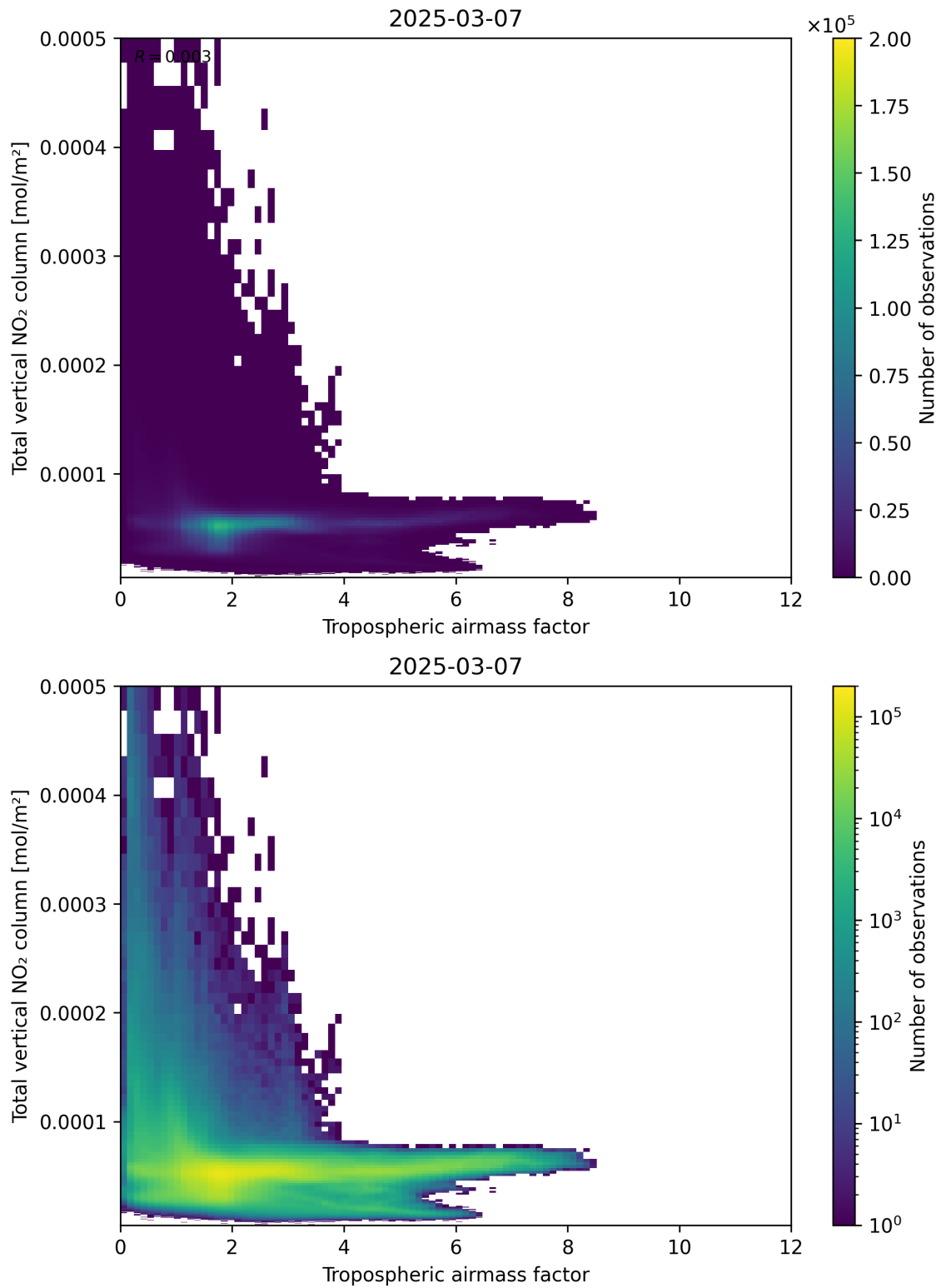
Figure 77: Scatter density plot of “Tropospheric airmass factor” against “Total vertical NO 2 column” for 2025-03-07 to 2025-03-08.
