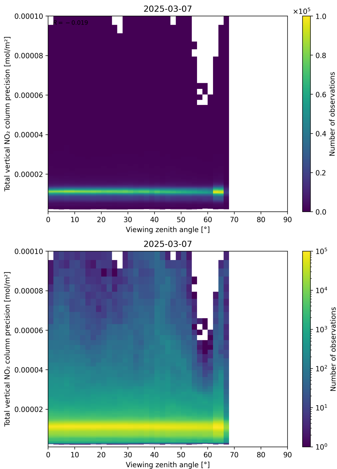
Figure 168: Scatter density plot of “Viewing zenith angle” against “Total vertical NO 2 column precision” for 2025-03-07 to 2025-03-08.
