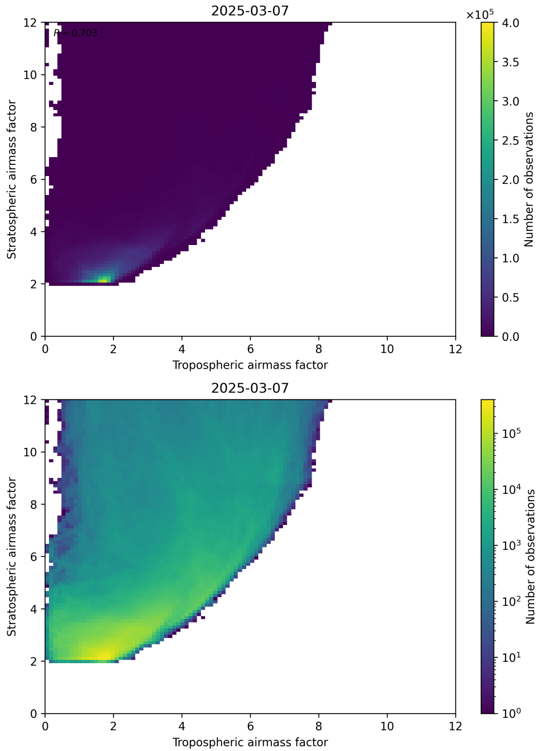
Figure 71: Scatter density plot of “Tropospheric airmass factor” against “Stratospheric airmass factor” for 2025-03-07 to 2025-03-08.
