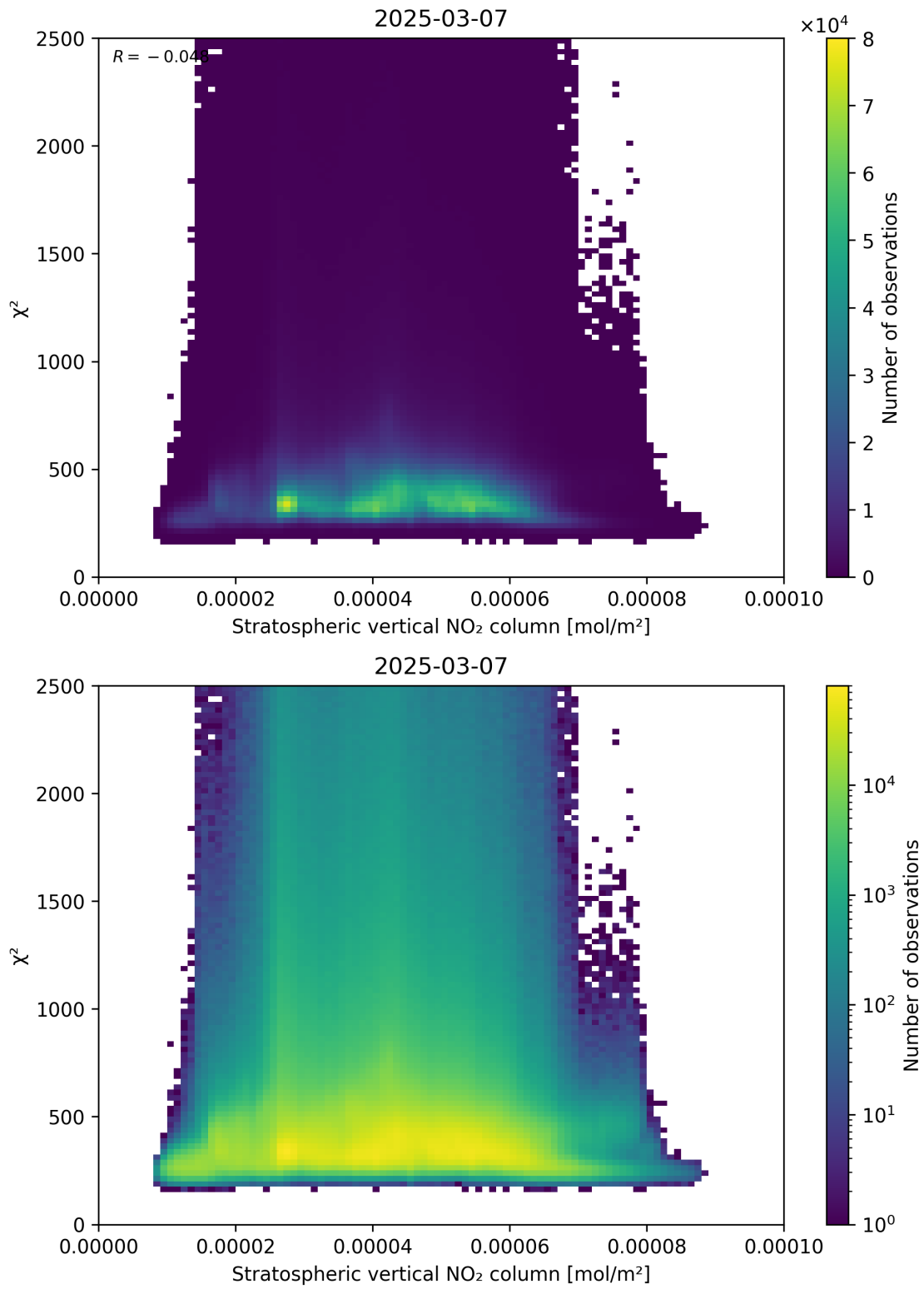
Figure 97: Scatter density plot of “Stratospheric vertical NO 2 column” against “ \chi^2 ” for 2025-03-07 to 2025-03-08.
