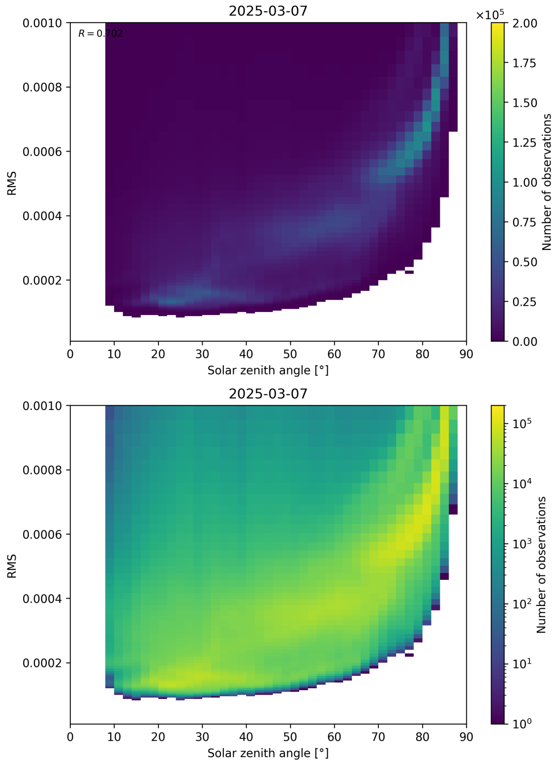
Figure 157: Scatter density plot of “Solar zenith angle” against “RMS” for 2025-03-07 to 2025-03-08.
