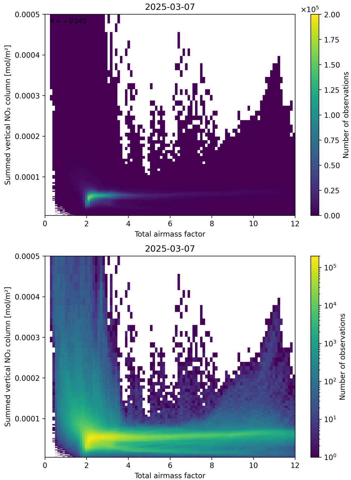
Figure 65: Scatter density plot of “Total airmass factor” against “Summed vertical NO 2 column” for 2025-03-07 to 2025-03-08.
