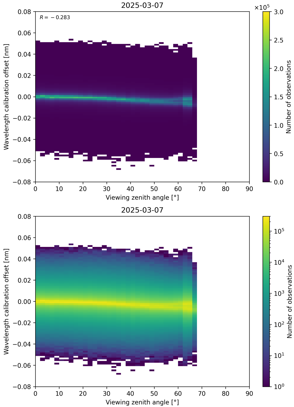
Figure 173: Scatter density plot of “Viewing zenith angle” against “Wavelength calibration offset” for 2025-03-07 to 2025-03-08.
