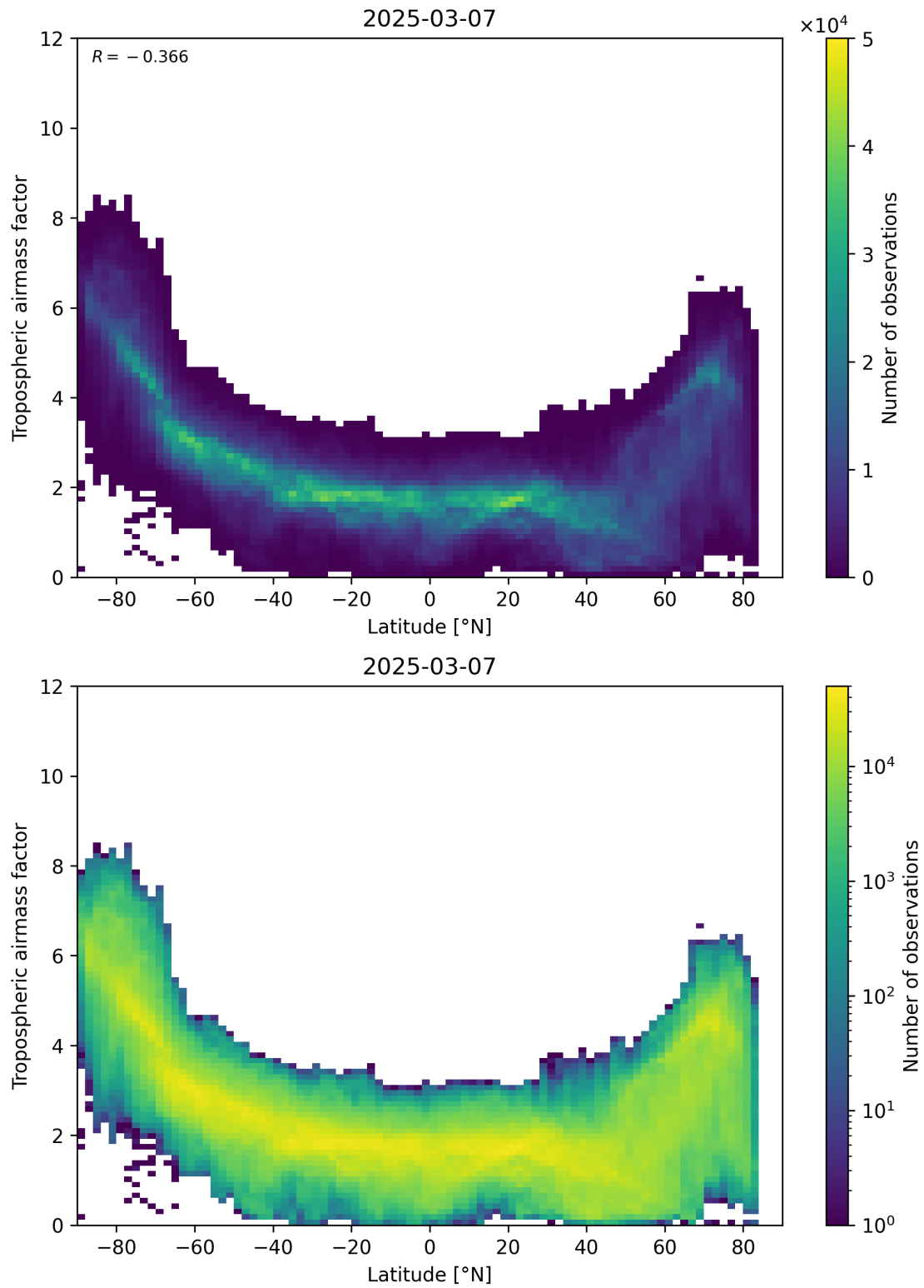
Figure 85: Scatter density plot of “Latitude” against “Tropospheric airmass factor” for 2025-03-07 to 2025-03-08.
