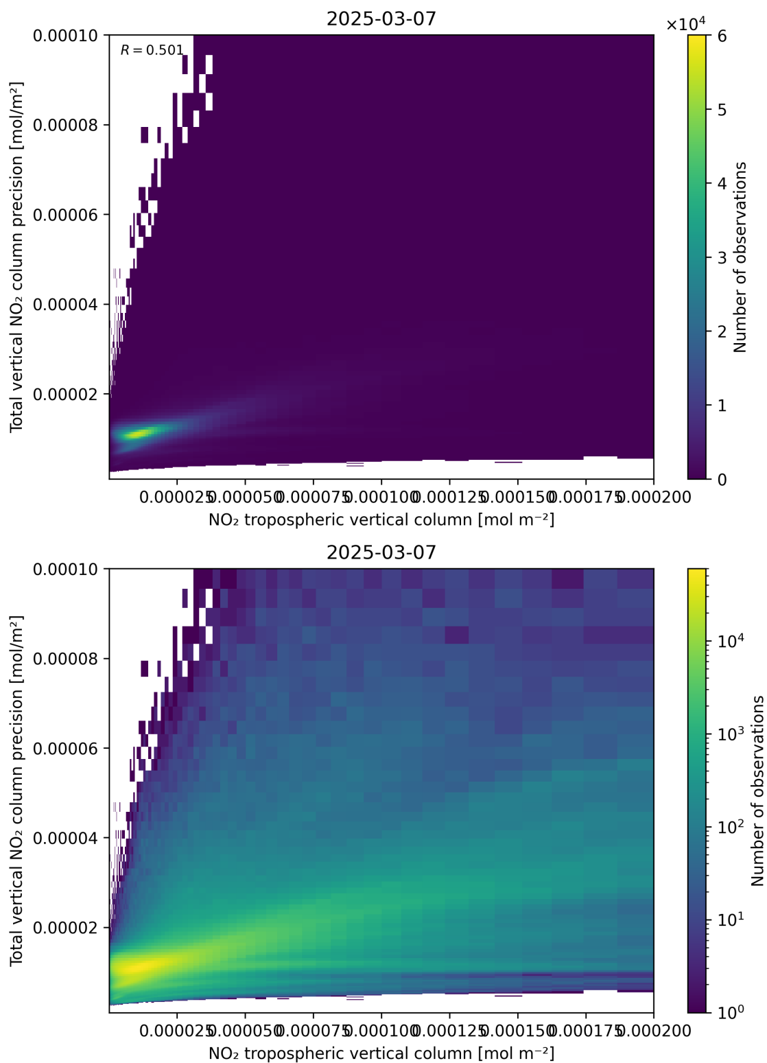
Figure 129: Scatter density plot of “NO 2 tropospheric vertical column” against “Total vertical NO 2 column precision” for 2025-03-07 to 2025-03-08.
