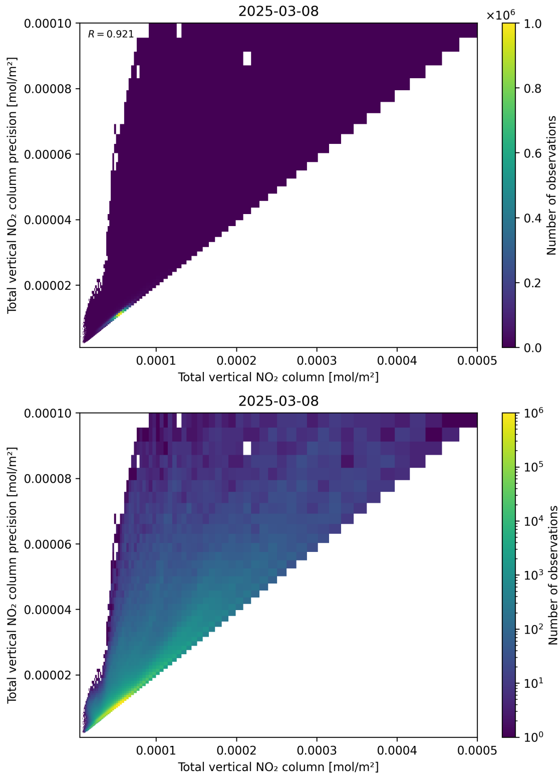
Figure 114: Scatter density plot of “Total vertical NO 2 column” against “Total vertical NO 2 column precision” for 2025-03-08 to 2025-03-09.
