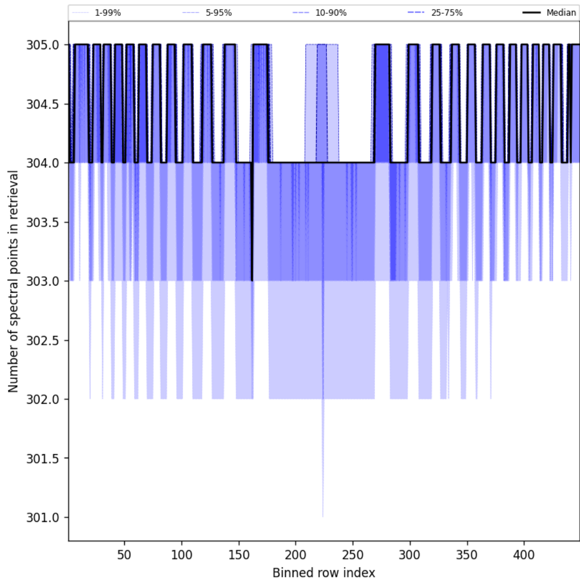
Figure 50: Along track statistics of “Number of spectral points in retrieval” for 2025-03-08 to 2025-03-09
