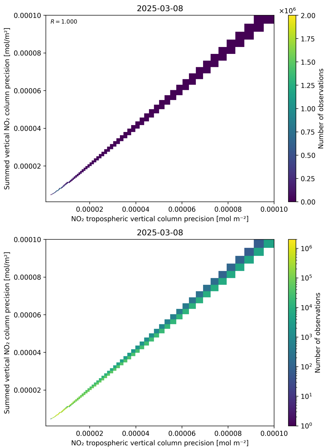
Figure 137: Scatter density plot of “NO 2 tropospheric vertical column precision” against “Summed vertical NO 2 column precision” for 2025-03-08 to 2025-03-09.
