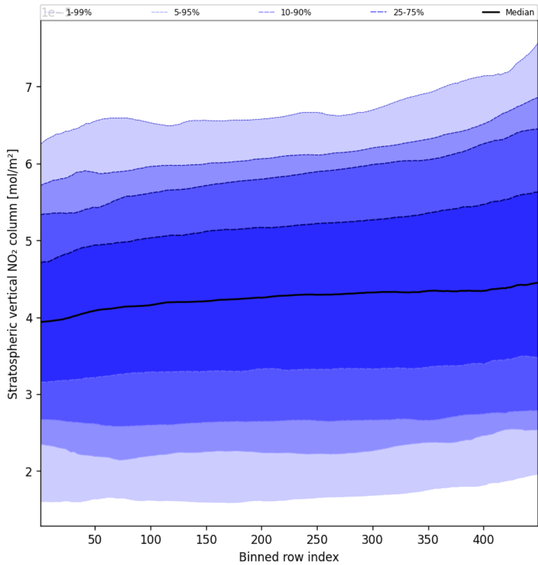
Figure 53: Along track statistics of “Stratospheric vertical NO 2 column” for 2025-03-08 to 2025-03-09
