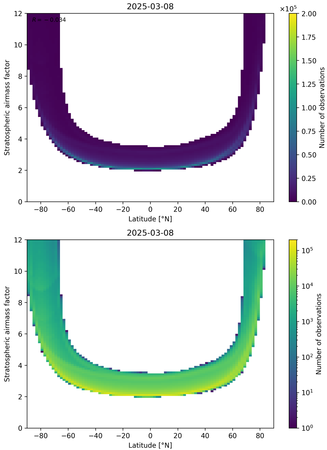
Figure 83: Scatter density plot of “Latitude” against “Stratospheric air mass factor” for 2025-03-08 to 2025-03-09.
