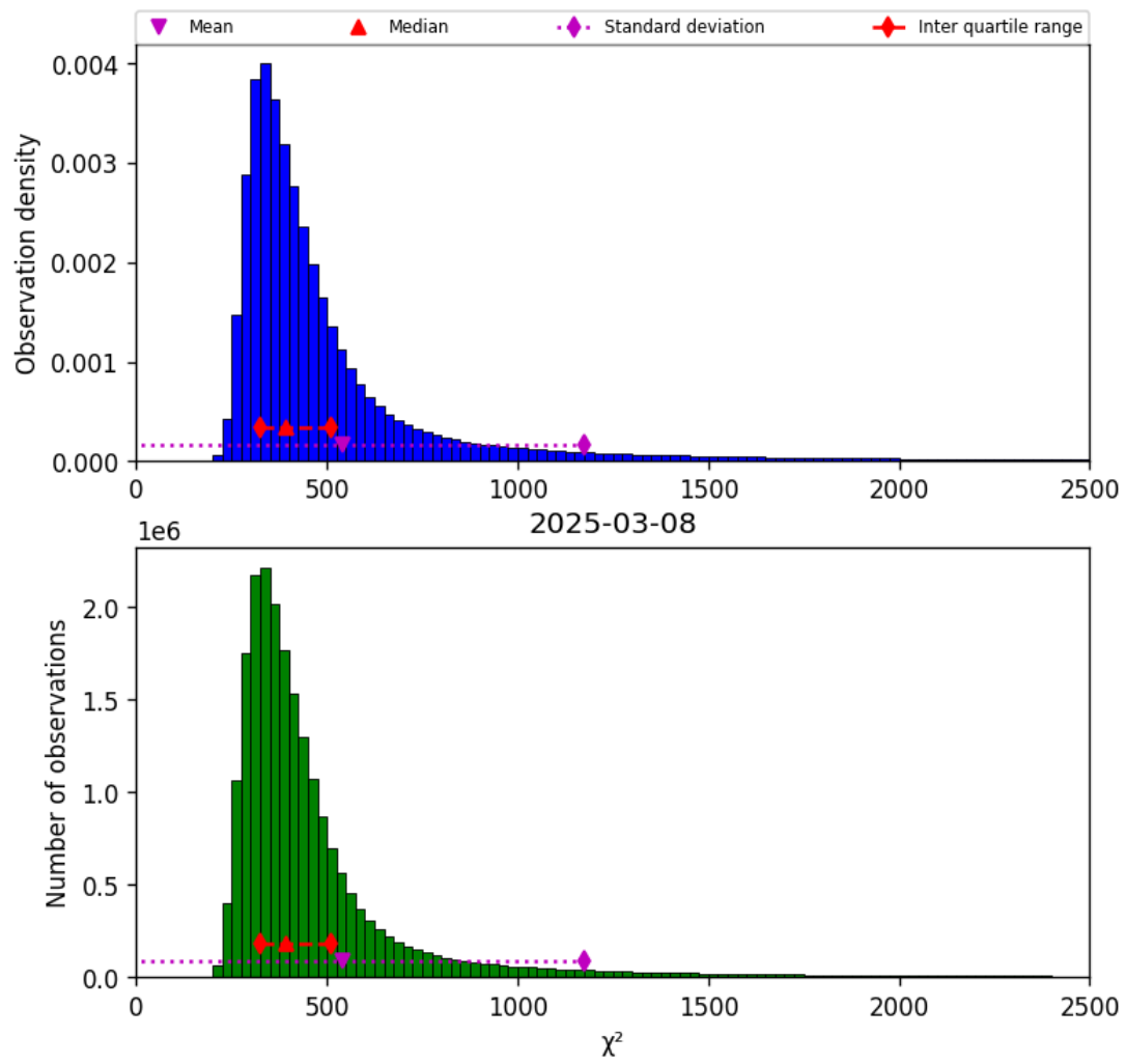
Figure 42: Histogram of “ \chi^2 ” for 2025-03-08 to 2025-03-09
