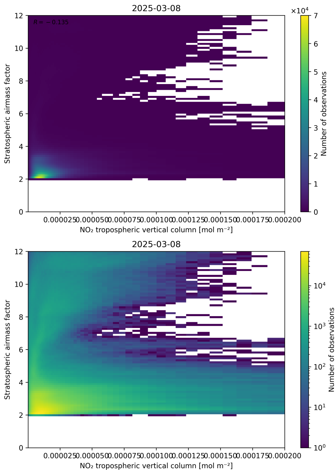
Figure 121: Scatter density plot of “NO 2 tropospheric vertical column” against “Stratospheric air mass factor” for 2025-03-08 to 2025-03-09.
