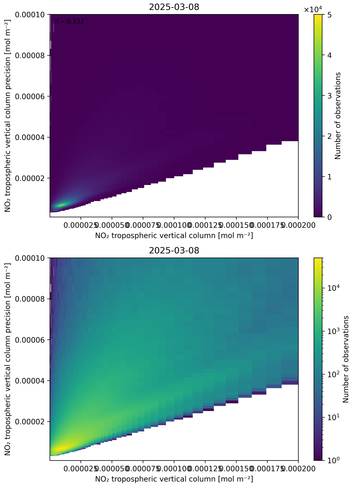
Figure 130: Scatter density plot of “NO 2 tropospheric vertical column” against “NO 2 tropospheric vertical column precision” for 2025-03-08 to 2025-03-09.
