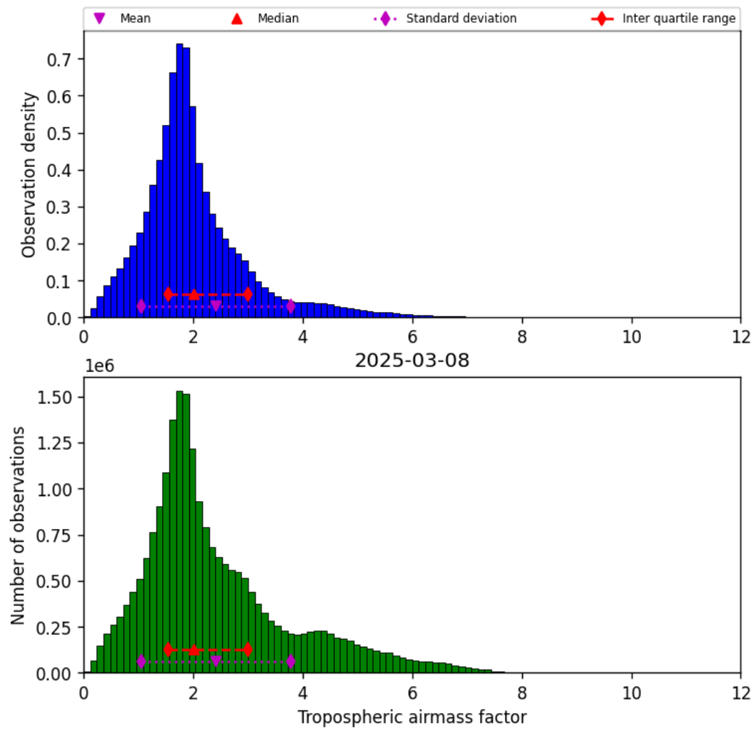
Figure 31: Histogram of “Tropospheric airmass factor” for 2025-03-08 to 2025-03-09
