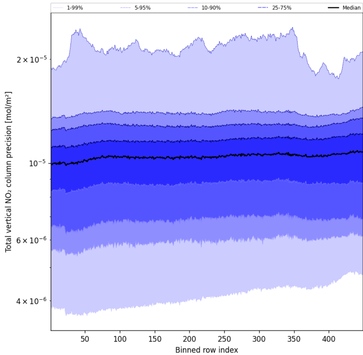
Figure 56: Along track statistics of “Total vertical NO 2 column precision” for 2025-03-08 to 2025-03-09
