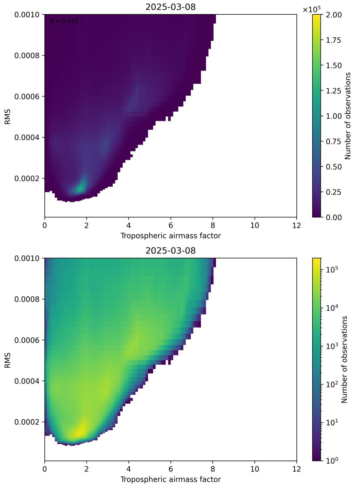
Figure 79: Scatter density plot of “Tropospheric airmass factor” against “RMS” for 2025-03-08 to 2025-03-09.
