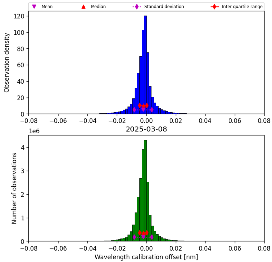
Figure 35: Histogram of “Wavelength calibration offset” for 2025-03-08 to 2025-03-09
