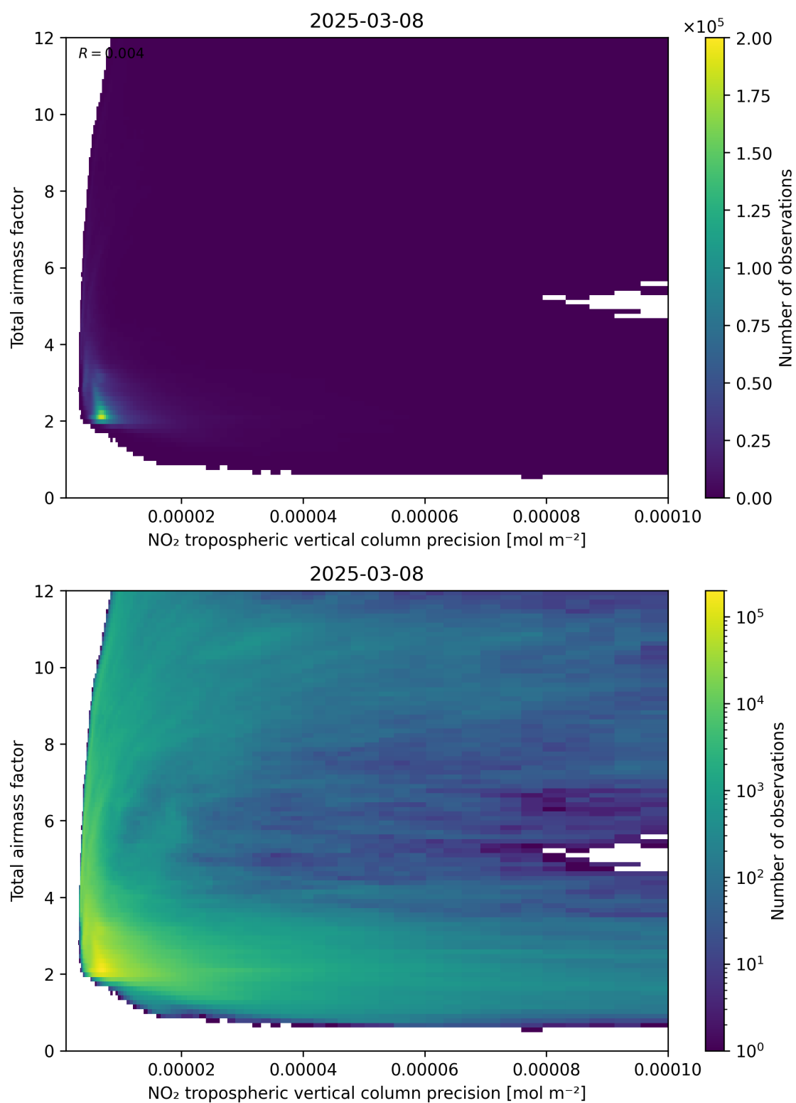
Figure 132: Scatter density plot of “NO 2 tropospheric vertical column precision” against “Total air mass factor” for 2025-03-08 to 2025-03-09.
