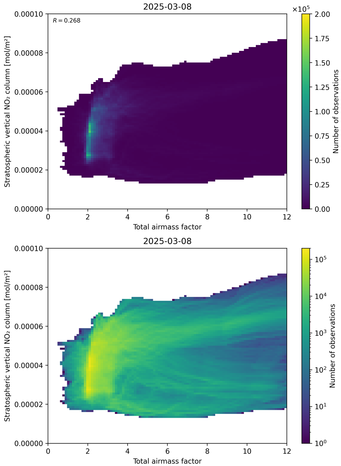
Figure 64: Scatter density plot of “Total airmass factor” against “Stratospheric vertical \text{NO}_2 column” for 2025-03-08 to 2025-03-09.
