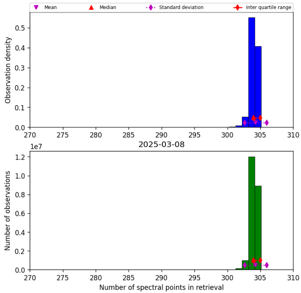
Figure 33: Histogram of “Number of spectral points in retrieval” for 2025-03-08 to 2025-03-09
