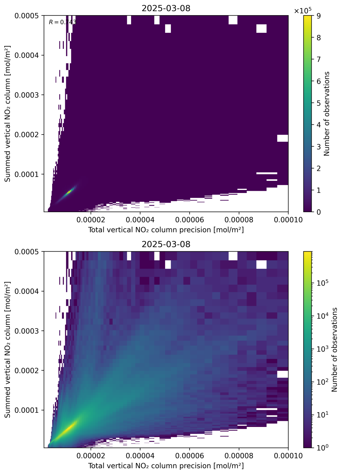
Figure 117: Scatter density plot of “Total vertical NO 2 column precision” against “Summed vertical NO 2 column” for 2025-03-08 to 2025-03-09.
