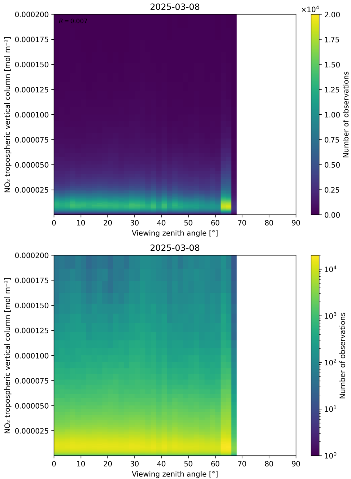
Figure 169: Scatter density plot of “Viewing zenith angle” against “NO 2 tropospheric vertical column” for 2025-03-08 to 2025-03-09.
