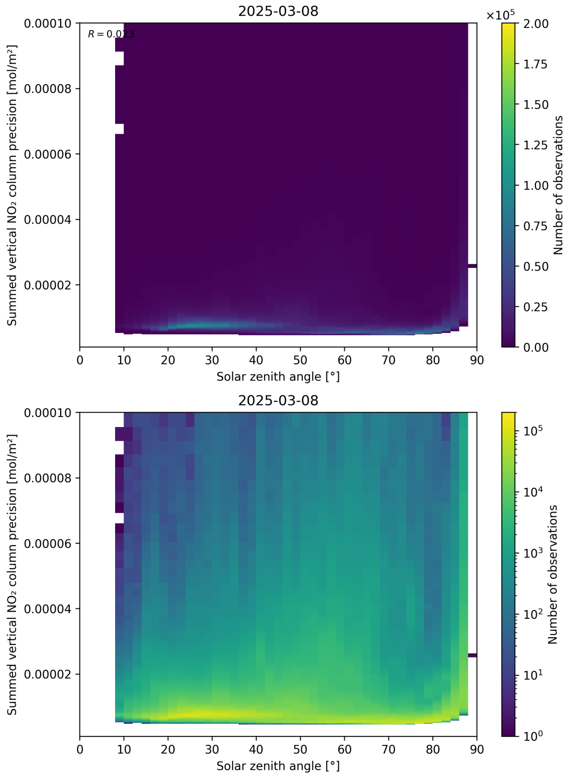
Figure 152: Scatter density plot of “Solar zenith angle” against “Summed vertical NO 2 column precision” for 2025-03-08 to 2025-03-09.
