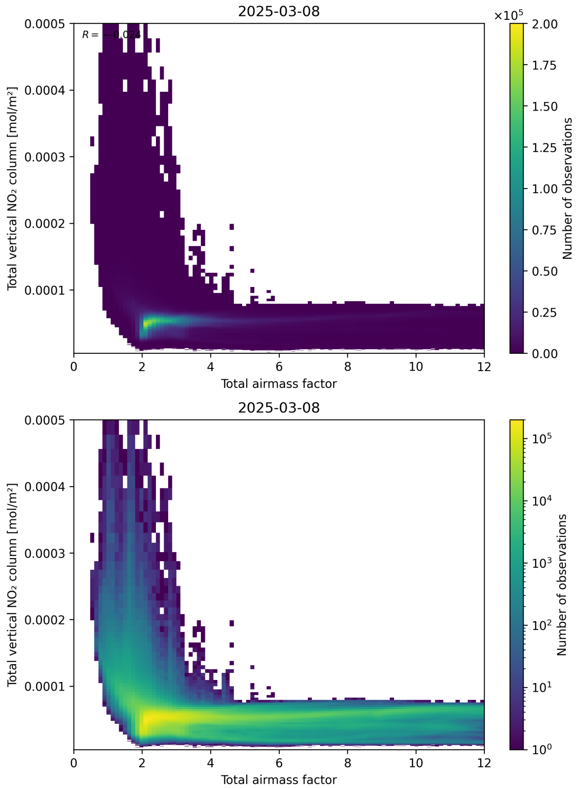
Figure 67: Scatter density plot of “Total airmass factor” against “Total vertical NO 2 column” for 2025-03-08 to 2025-03-09.
