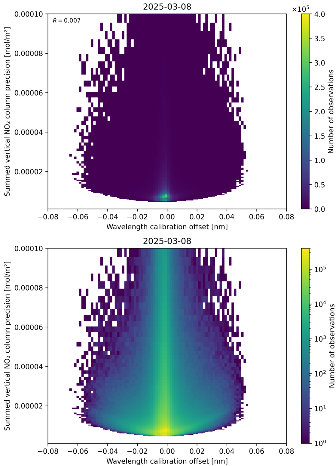
Figure 178: Scatter density plot of “Wavelength calibration offset” against “Summed vertical NO 2 column precision” for 2025-03-08 to 2025-03-09.
