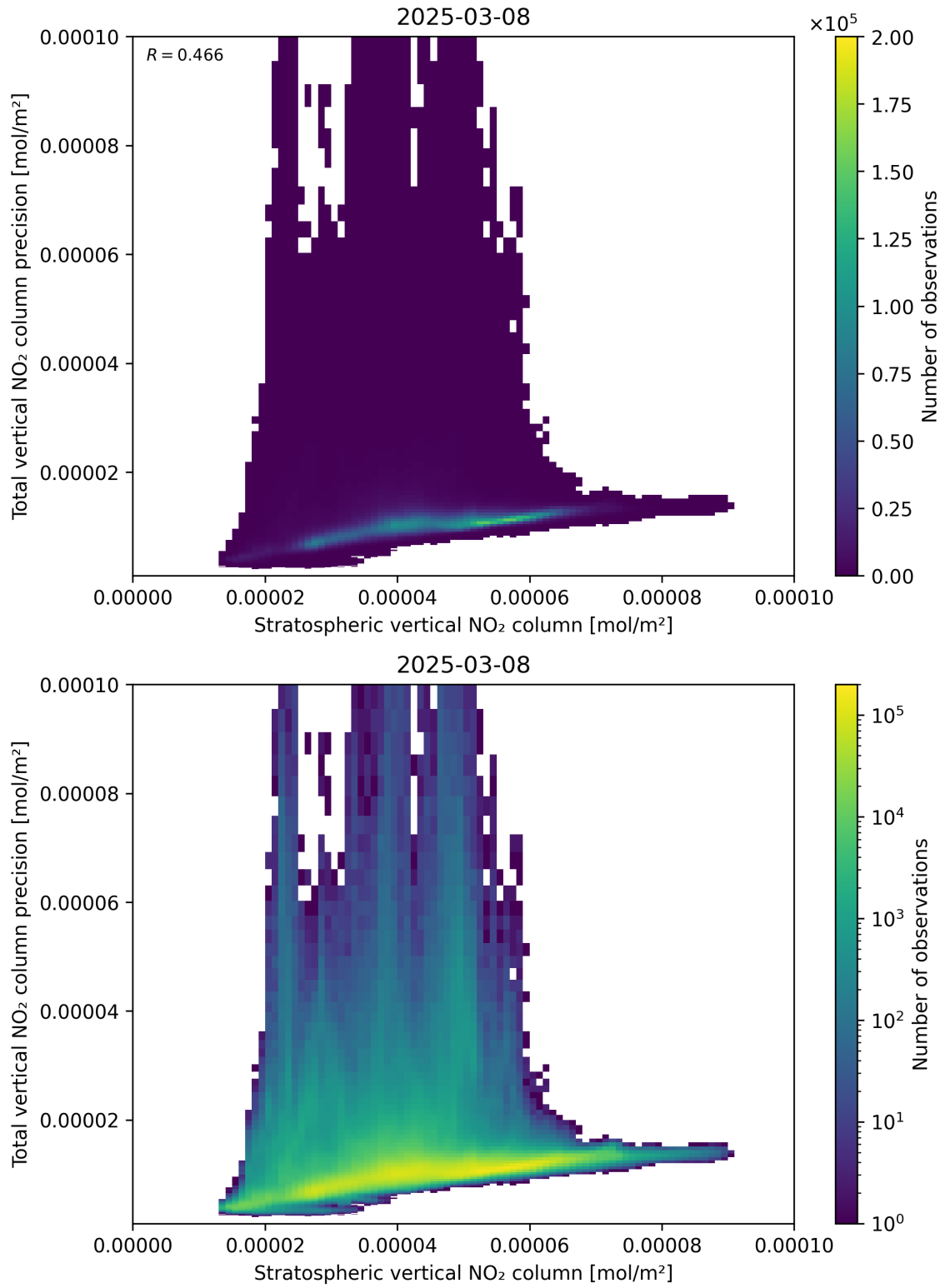
Figure 101: Scatter density plot of “Stratospheric vertical NO 2 column” against “Total vertical NO 2 column precision” for 2025-03-08 to 2025-03-09.
