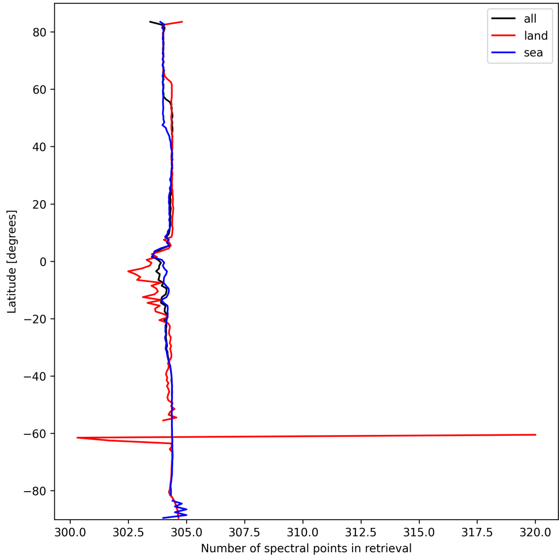
Figure 16: Zonal average of “Number of spectral points in retrieval” for 2025-03-08 to 2025-03-09.
