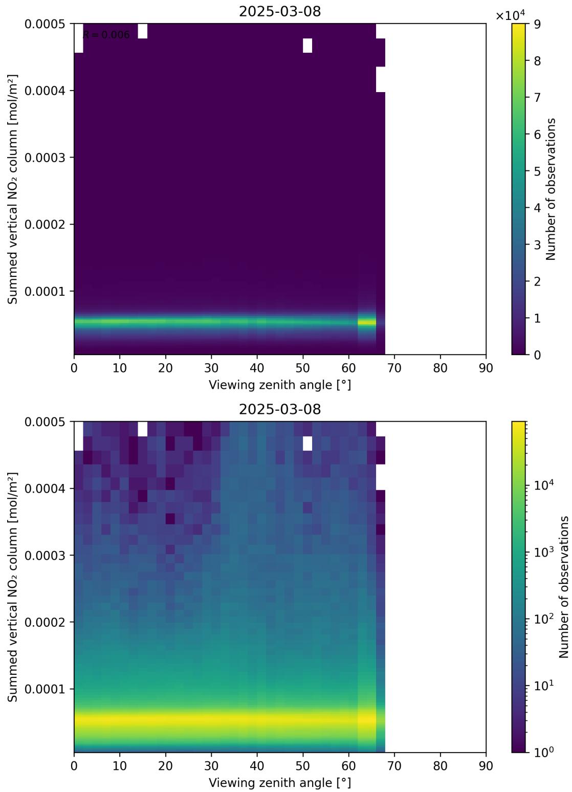
Figure 165: Scatter density plot of “Viewing zenith angle” against “Summed vertical NO 2 column” for 2025-03-08 to 2025-03-09.
