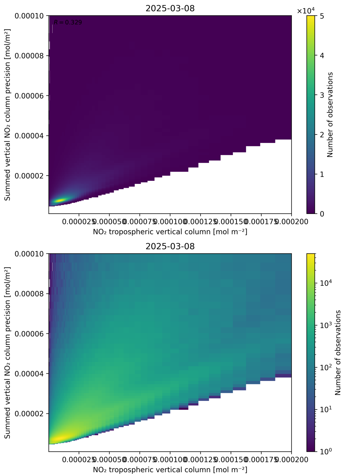
Figure 127: Scatter density plot of “NO 2 tropospheric vertical column” against “Summed vertical NO 2 column precision” for 2025-03-08 to 2025-03-09.
