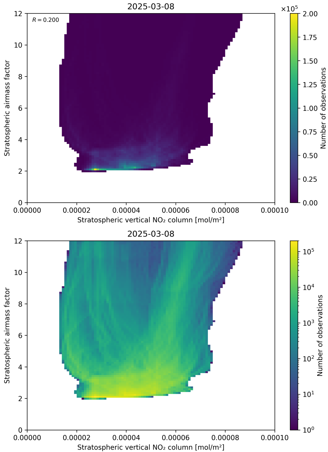
Figure 96: Scatter density plot of “Stratospheric vertical NO 2 column” against “Stratospheric airmass factor” for 2025-03-08 to 2025-03-09.
