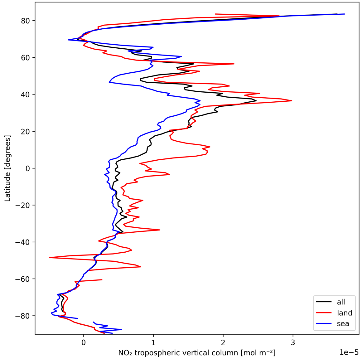
Figure 12: Zonal average of “NO 2 tropospheric vertical column” for 2025-03-08 to 2025-03-09.
