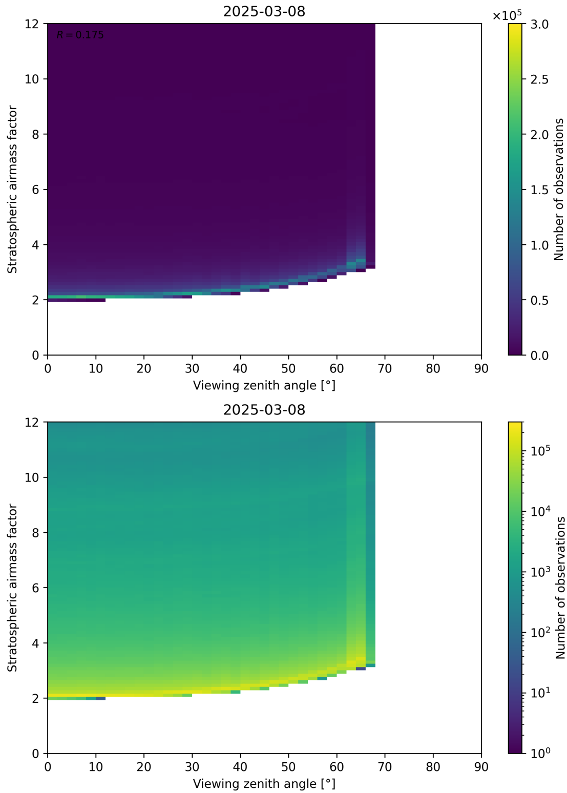
Figure 159: Scatter density plot of “Viewing zenith angle” against “Stratospheric airmass factor” for 2025-03-08 to 2025-03-09.
