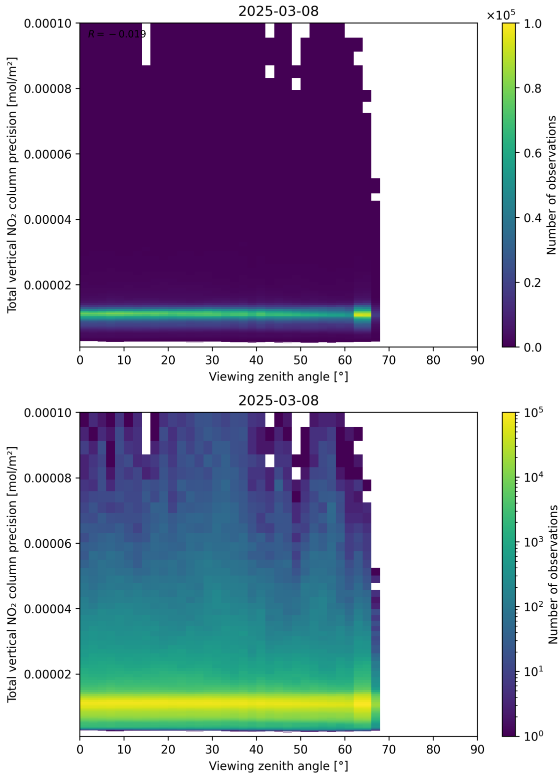
Figure 168: Scatter density plot of “Viewing zenith angle” against “Total vertical NO 2 column precision” for 2025-03-08 to 2025-03-09.
