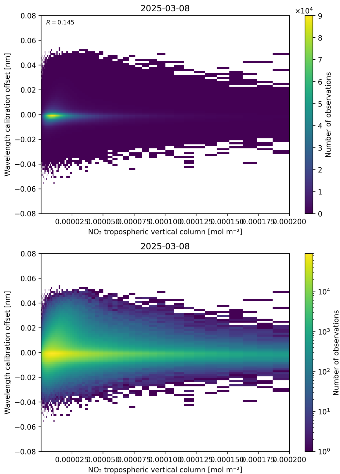
Figure 143: Scatter density plot of “NO 2 tropospheric vertical column” against “Wavelength calibration offset” for 2025-03-08 to 2025-03-09.
