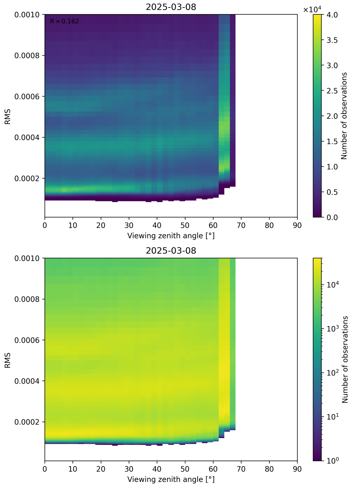
Figure 171: Scatter density plot of “Viewing zenith angle” against “RMS” for 2025-03-08 to 2025-03-09.
