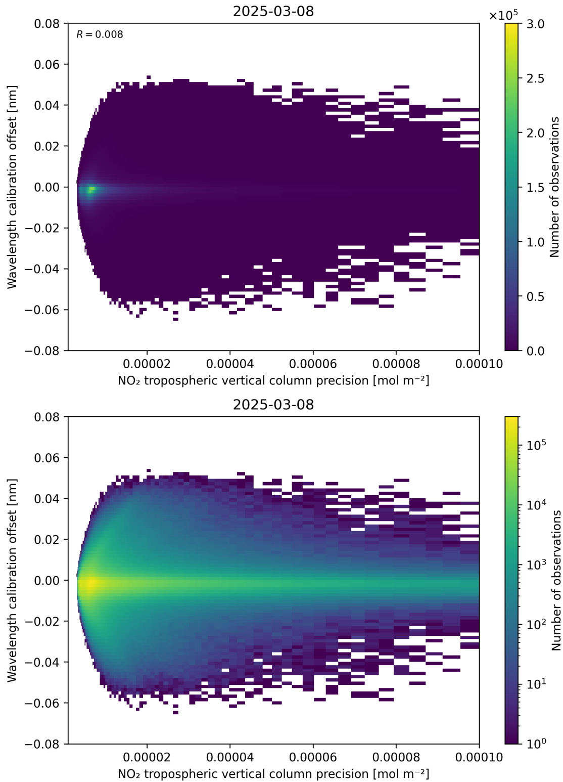
Figure 141: Scatter density plot of “NO 2 tropospheric vertical column precision” against “Wavelength calibration offset” for 2025-03-08 to 2025-03-09.
