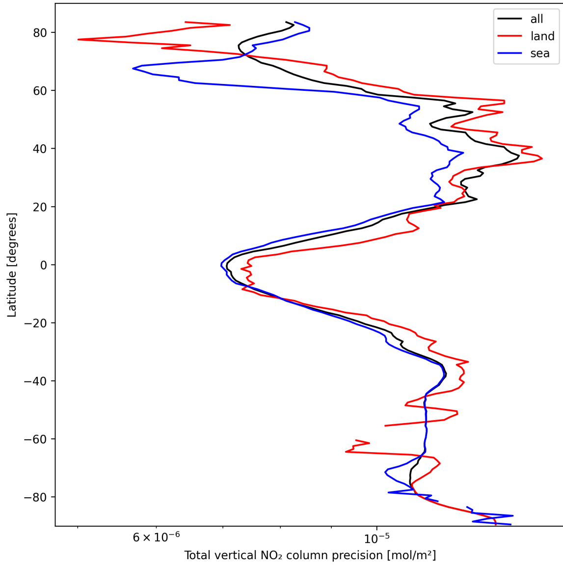
Figure 22: Zonal average of “Total vertical NO 2 column precision” for 2025-03-08 to 2025-03-09.
