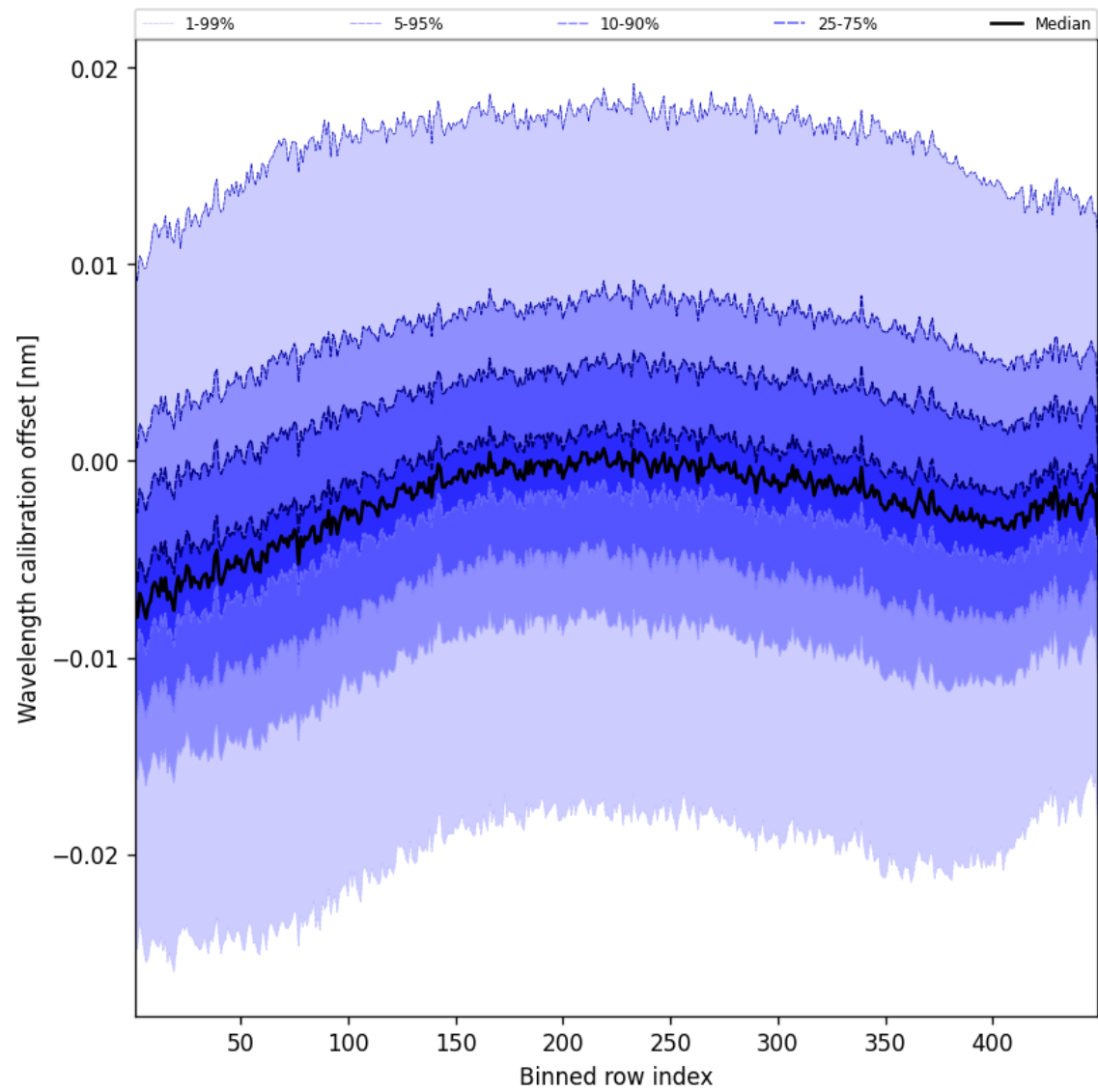
Figure 52: Along track statistics of “Wavelength calibration offset” for 2025-03-08 to 2025-03-09
