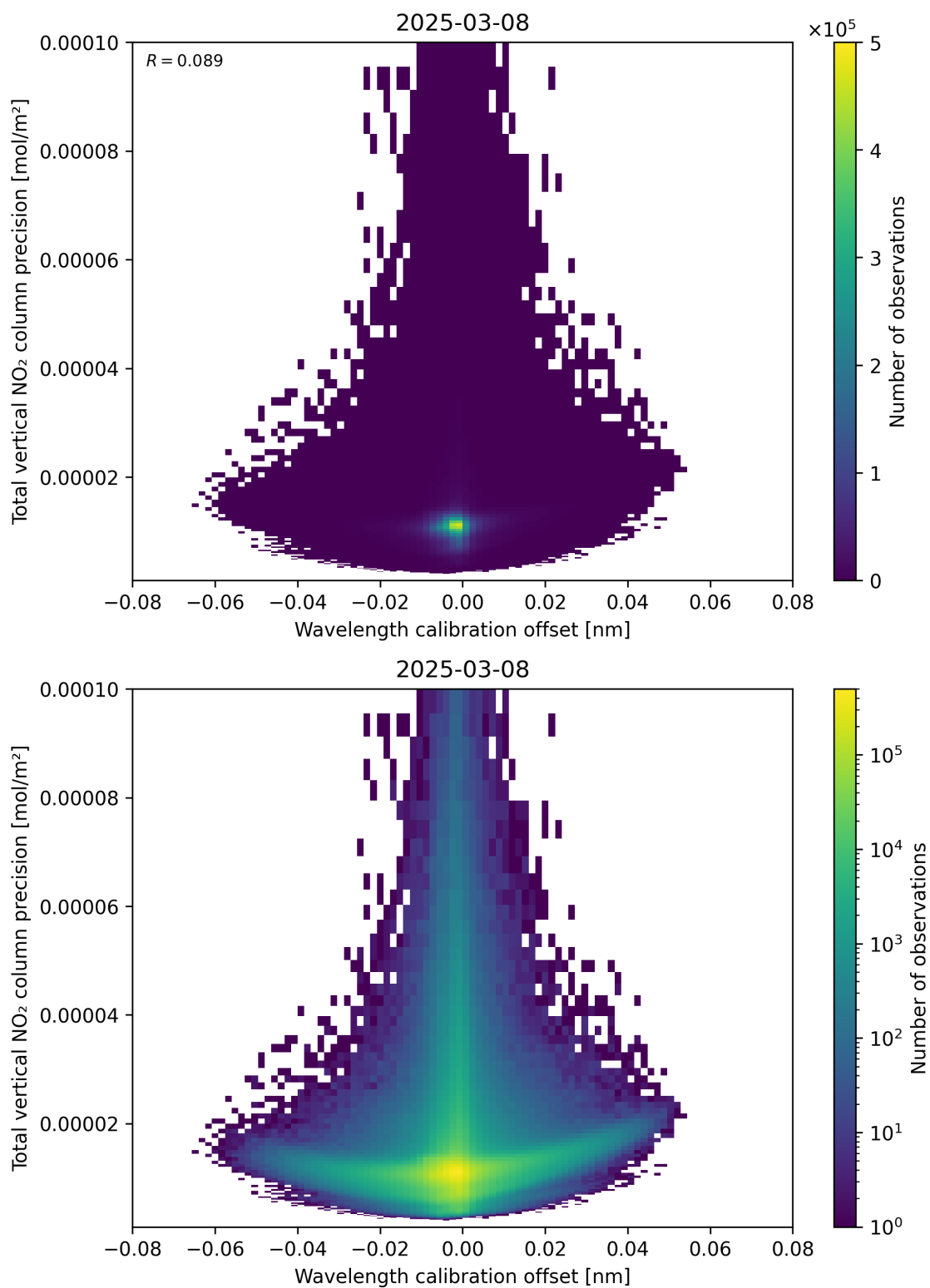
Figure 180: Scatter density plot of “Wavelength calibration offset” against “Total vertical NO 2 column precision” for 2025-03-08 to 2025-03-09.
