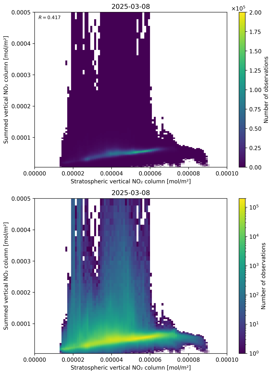
Figure 98: Scatter density plot of “Stratospheric vertical NO 2 column” against “Summed vertical NO 2 column” for 2025-03-08 to 2025-03-09.
