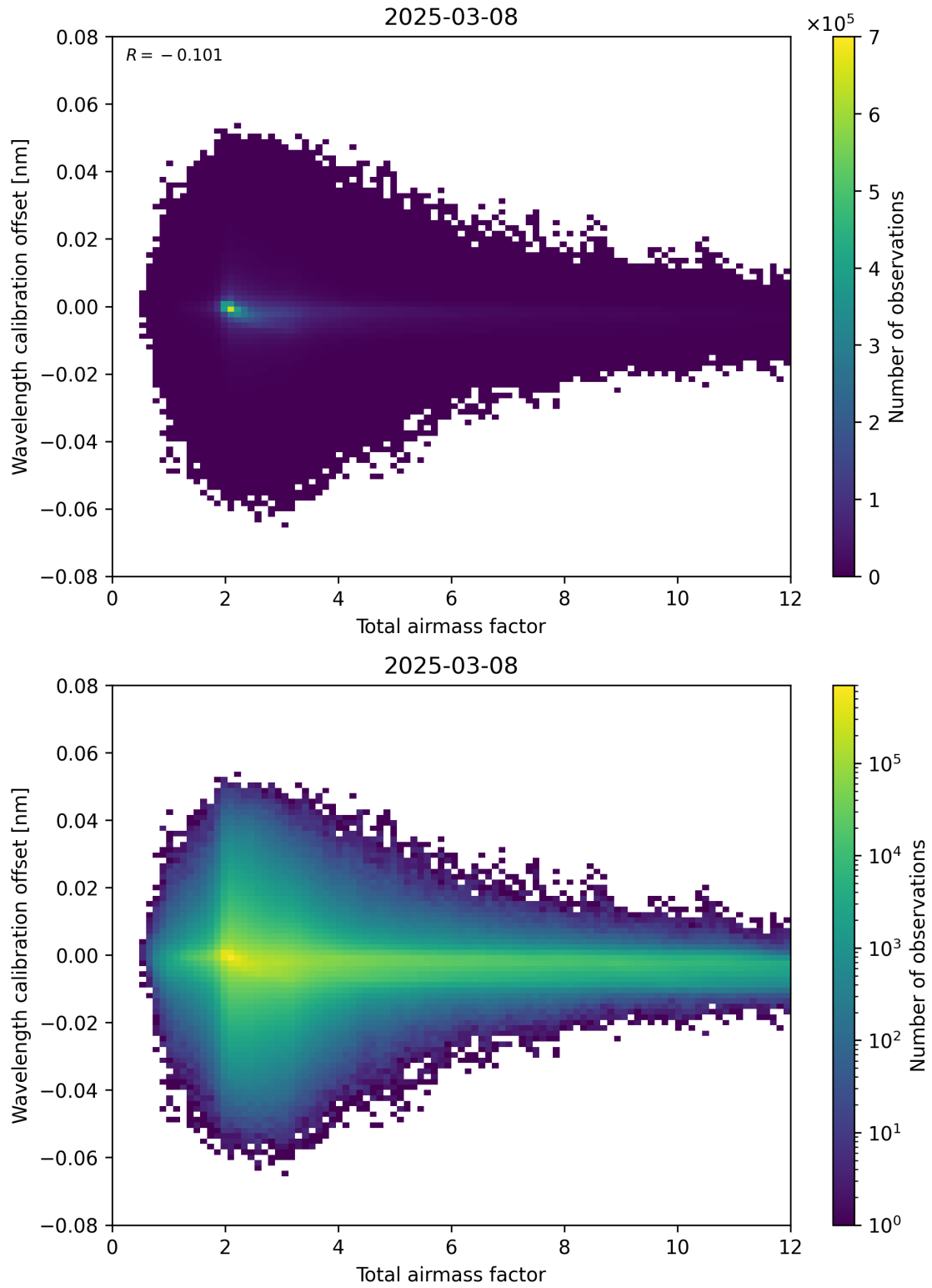
Figure 70: Scatter density plot of “Total airmass factor” against “Wavelength calibration offset” for 2025-03-08 to 2025-03-09.
