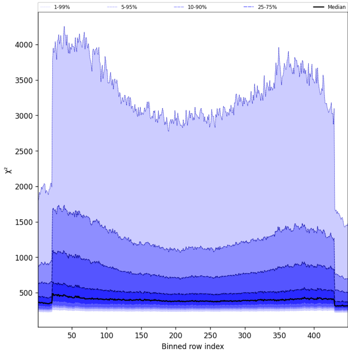
Figure 59: Along track statistics of “ \chi^2 ” for 2025-03-08 to 2025-03-09
