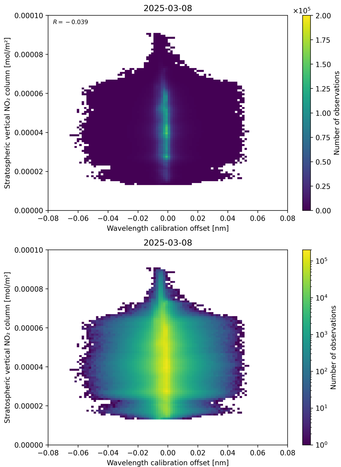
Figure 176: Scatter density plot of “Wavelength calibration offset” against “Stratospheric vertical NO 2 column” for 2025-03-08 to 2025-03-09.
