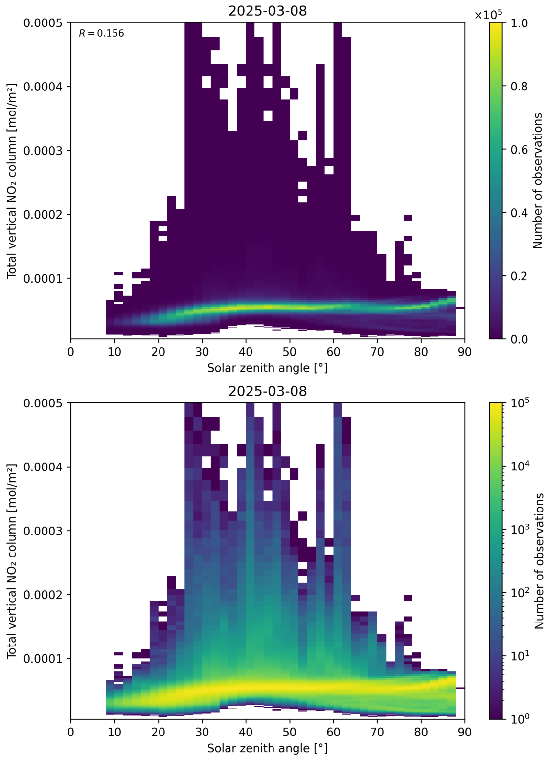
Figure 153: Scatter density plot of “Solar zenith angle” against “Total vertical NO 2 column” for 2025-03-08 to 2025-03-09.
