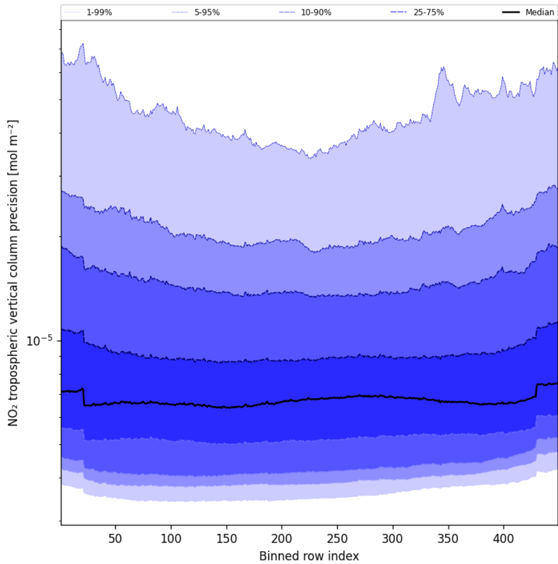
Figure 47: Along track statistics of “NO 2 tropospheric vertical column precision” for 2025-03-08 to 2025-03-09
