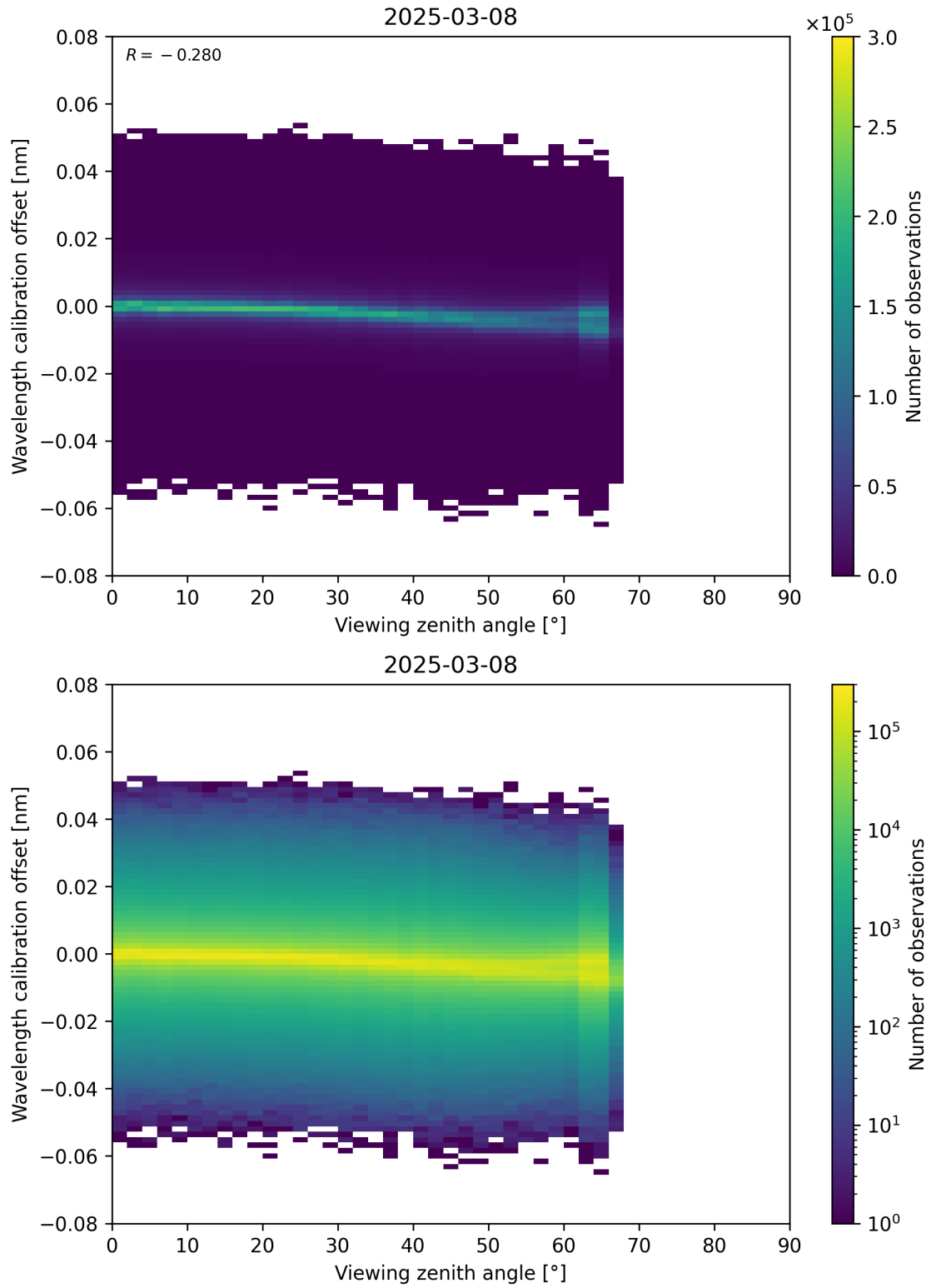
Figure 173: Scatter density plot of “Viewing zenith angle” against “Wavelength calibration offset” for 2025-03-08 to 2025-03-09.
