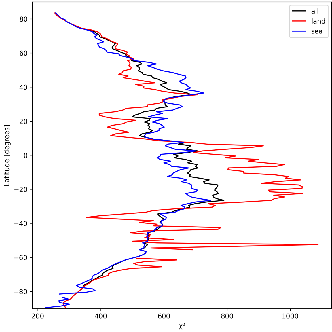
Figure 25: Zonal average of “ \chi^2 ” for 2025-03-08 to 2025-03-09.
