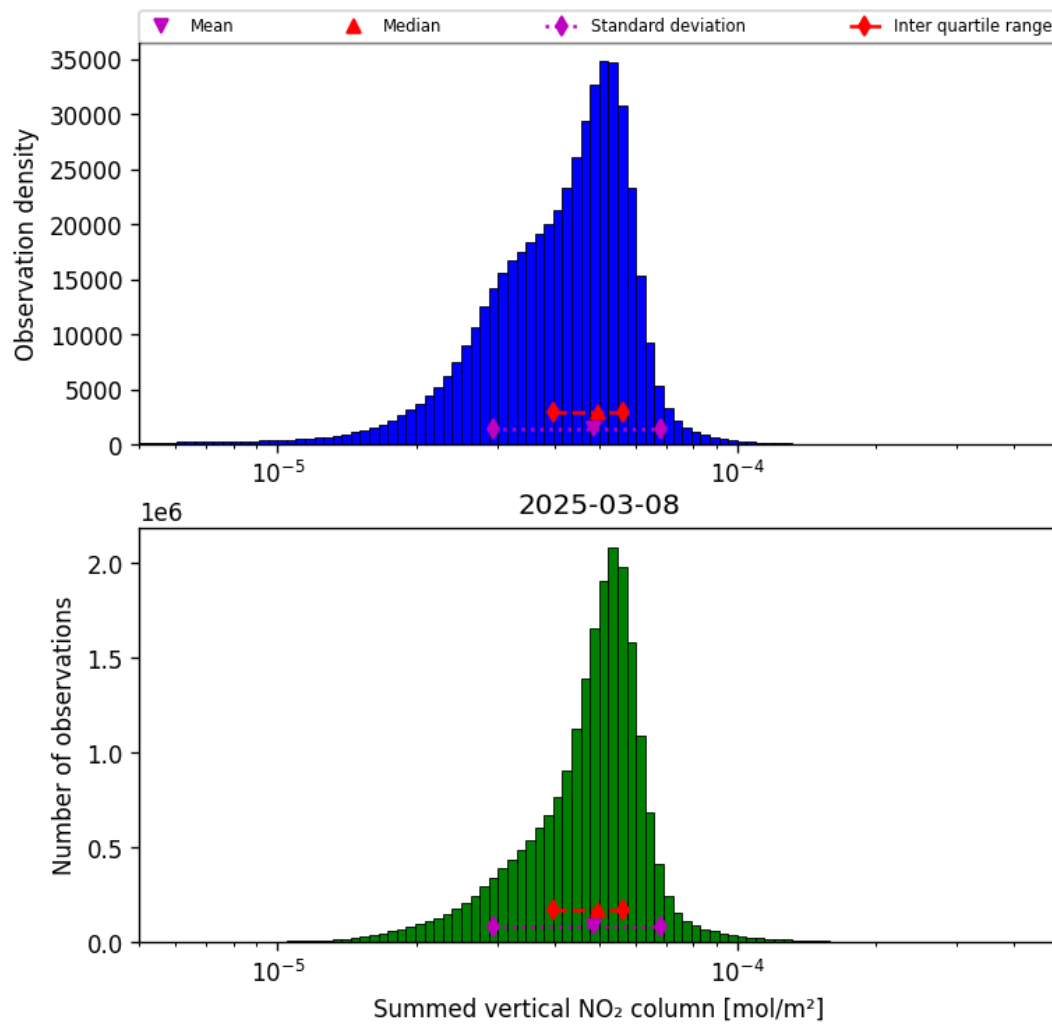
Figure 40: Histogram of “Summed vertical NO 2 column” for 2025-03-08 to 2025-03-09
