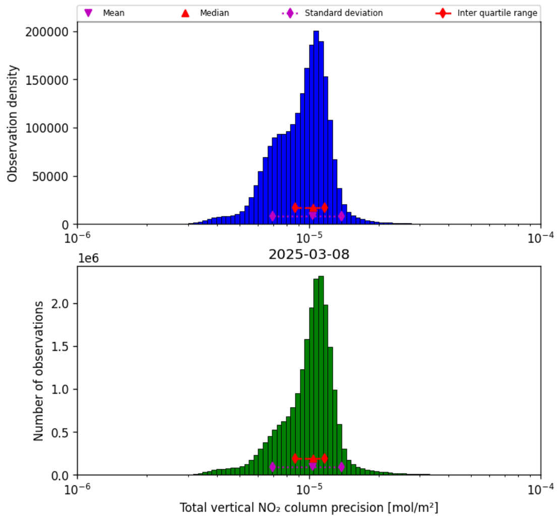
Figure 39: Histogram of “Total vertical NO 2 column precision” for 2025-03-08 to 2025-03-09
