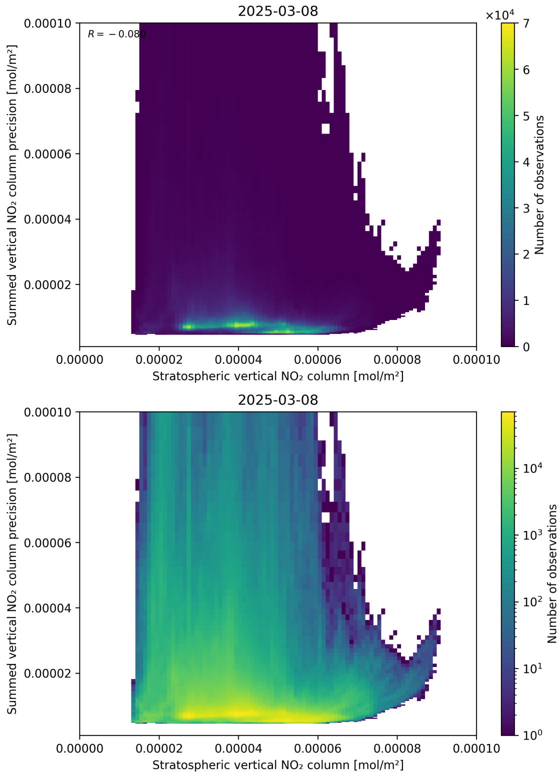
Figure 99: Scatter density plot of “Stratospheric vertical NO 2 column” against “Summed vertical NO 2 column precision” for 2025-03-08 to 2025-03-09.
