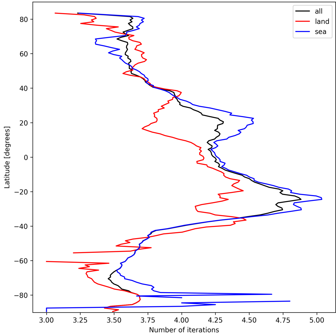
Figure 17: Zonal average of “Number of iterations” for 2025-03-08 to 2025-03-09.
