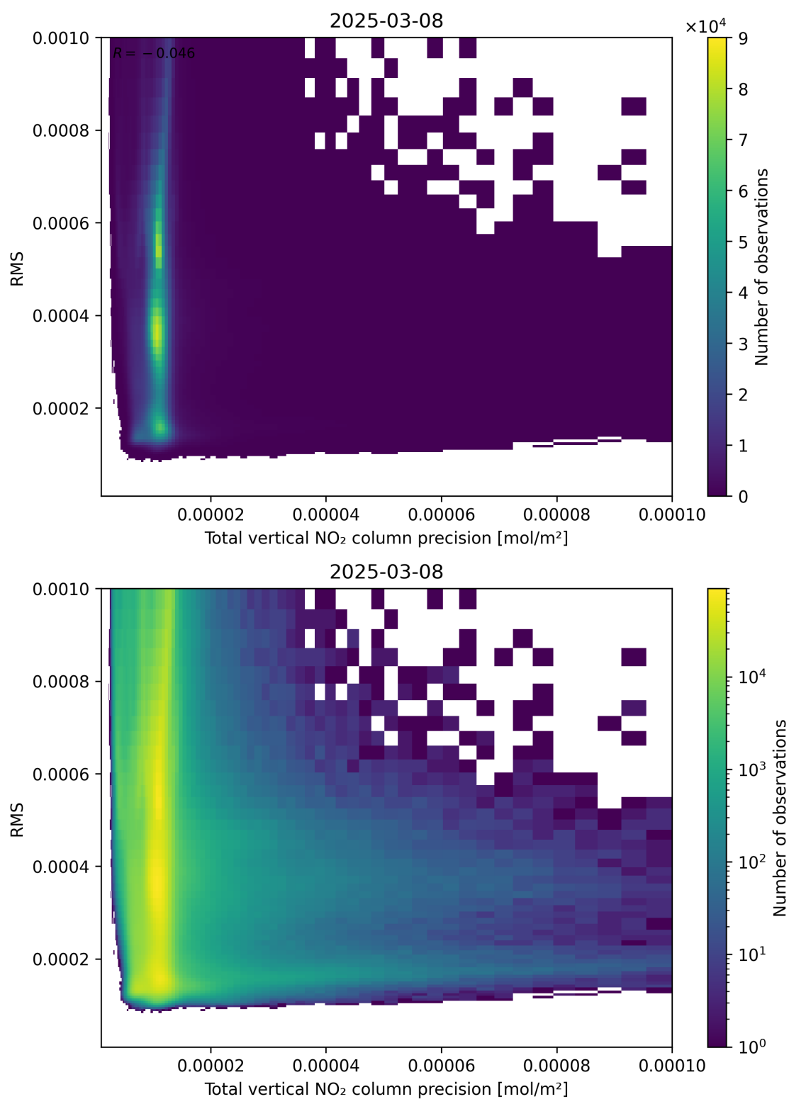
Figure 119: Scatter density plot of “Total vertical NO 2 column precision” against “RMS” for 2025-03-08 to 2025-03-09.
