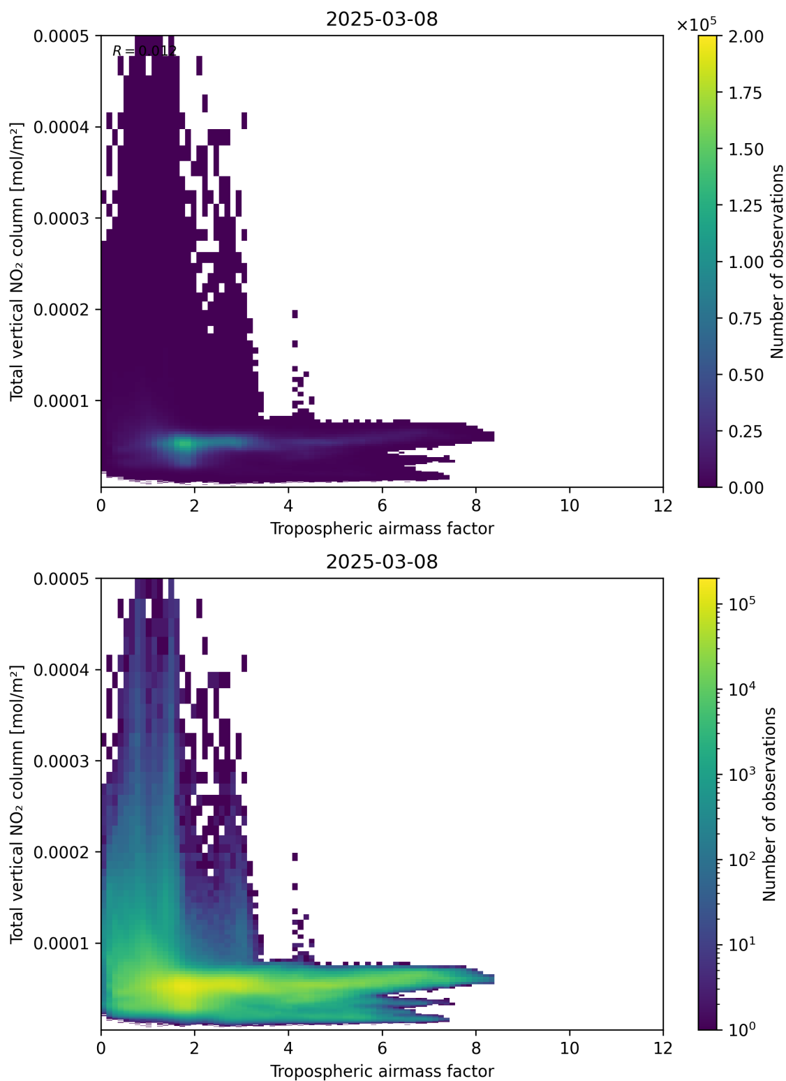
Figure 77: Scatter density plot of “Tropospheric airmass factor” against “Total vertical NO 2 column” for 2025-03-08 to 2025-03-09.
