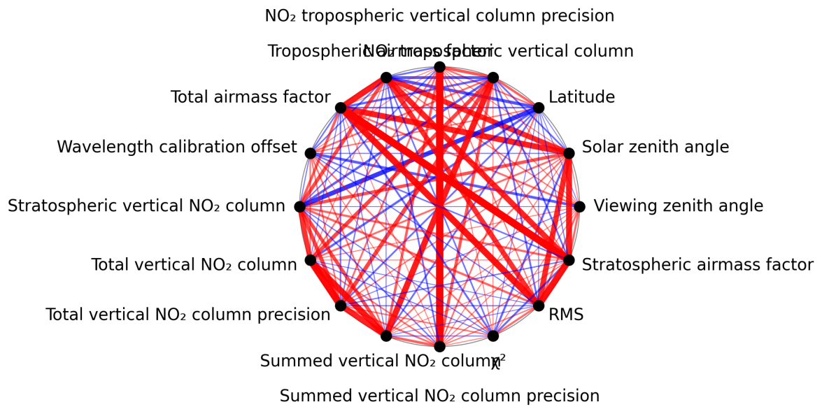
Figure 1: Map of correlation graph for 2025-03-08 to 2025-03-09.
