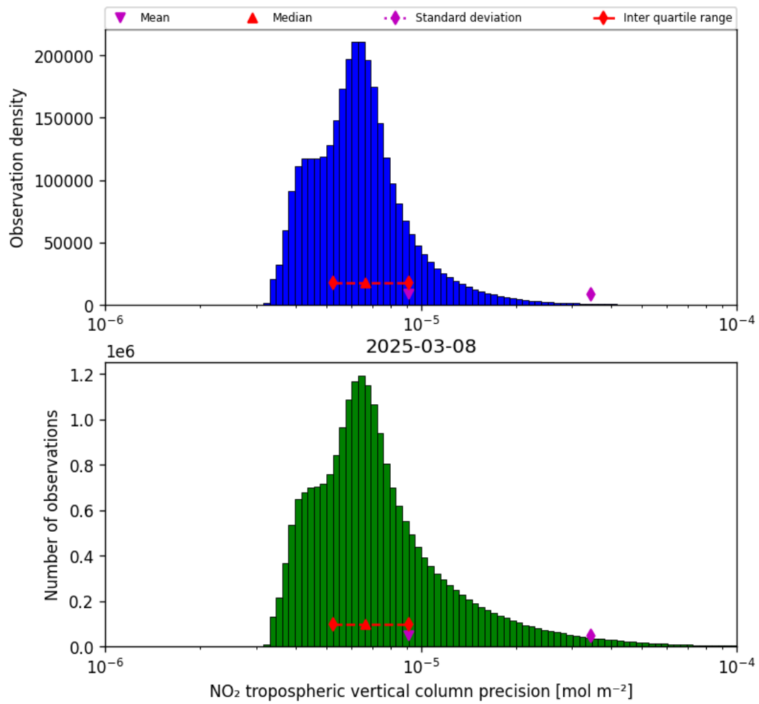
Figure 30: Histogram of “NO 2 tropospheric vertical column precision” for 2025-03-08 to 2025-03-09
