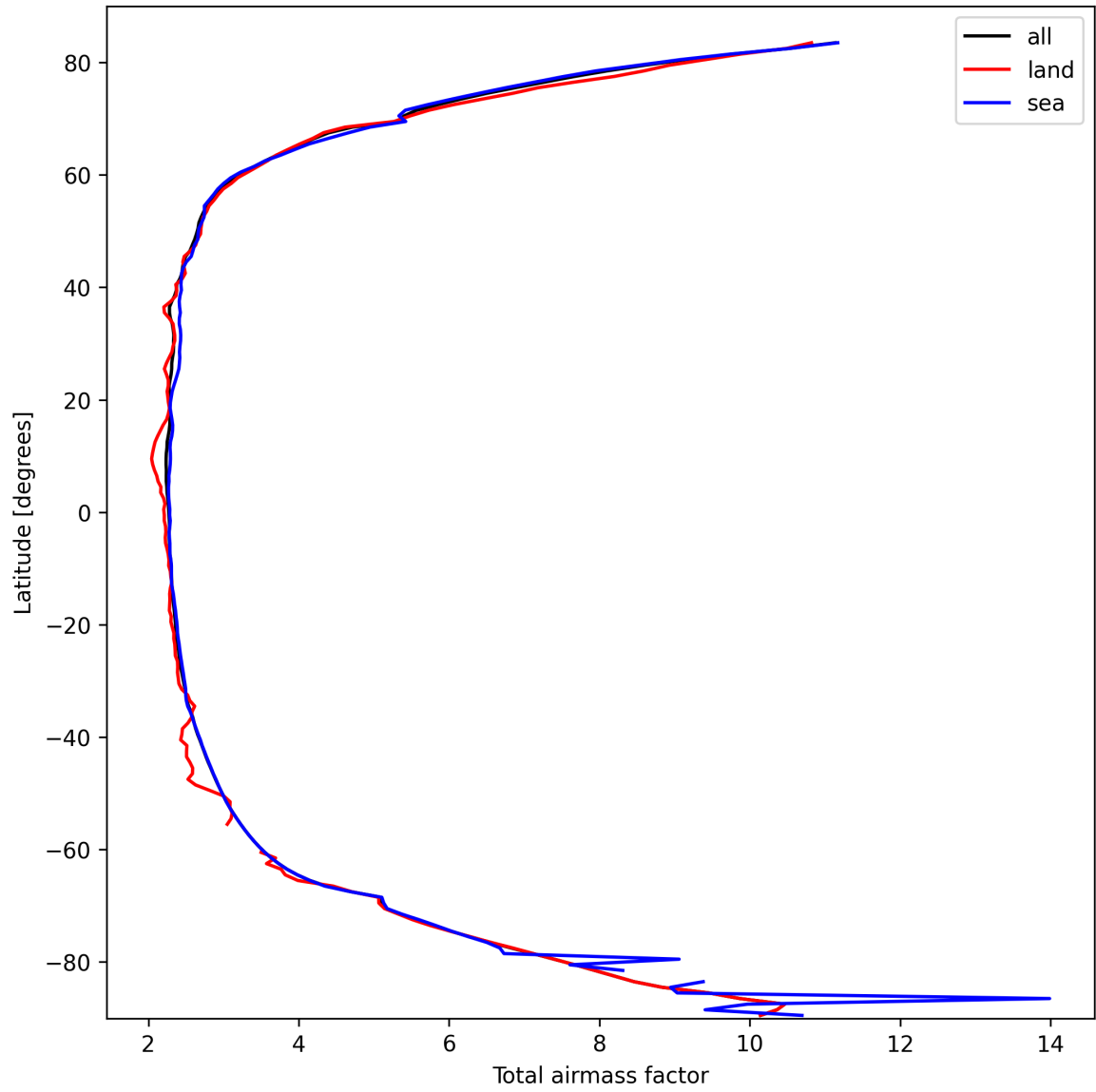
Figure 15: Zonal average of “Total airmass factor” for 2025-03-08 to 2025-03-09.
