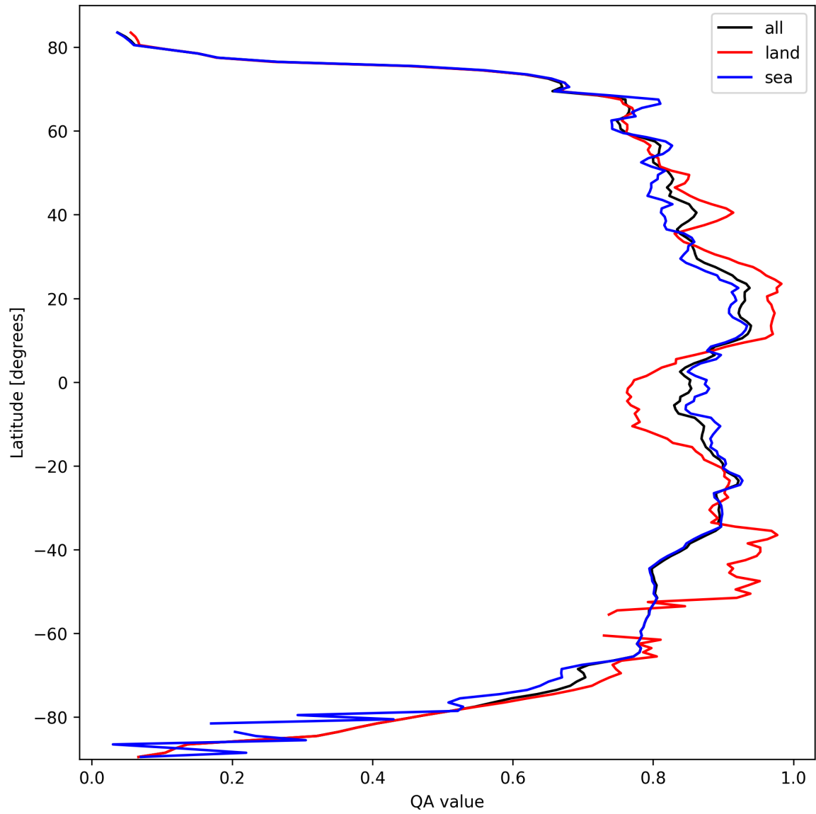
Figure 11: Zonal average of “QA value” for 2025-03-08 to 2025-03-09.
