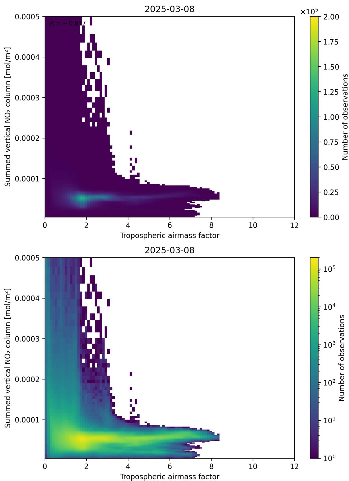
Figure 75: Scatter density plot of “Tropospheric air mass factor” against “Summed vertical NO 2 column” for 2025-03-08 to 2025-03-09.
