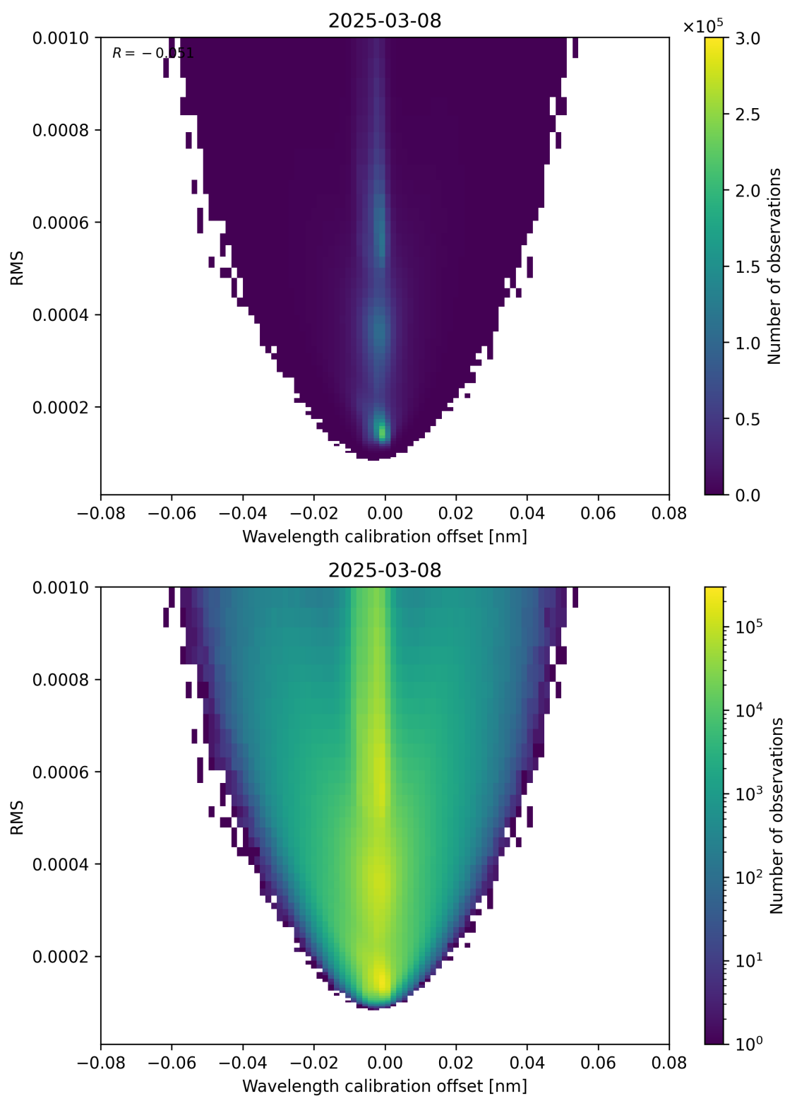
Figure 181: Scatter density plot of “Wavelength calibration offset” against “RMS” for 2025-03-08 to 2025-03-09.
