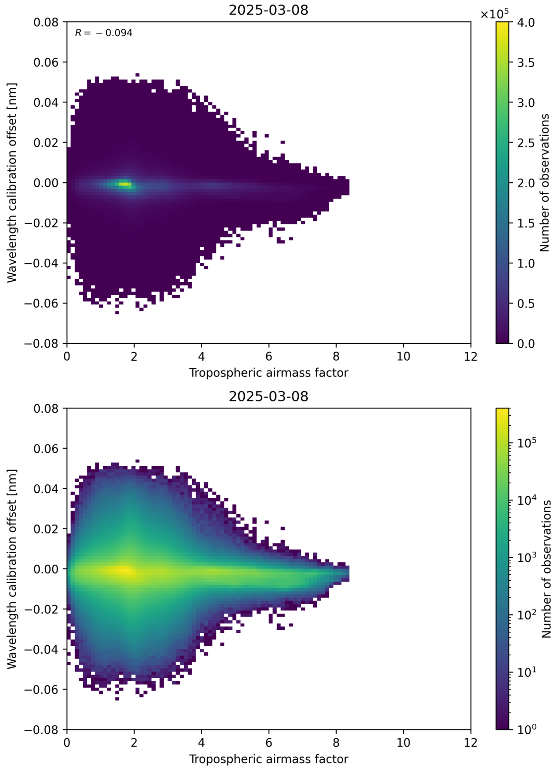
Figure 80: Scatter density plot of “Tropospheric airmass factor” against “Wavelength calibration offset” for 2025-03-08 to 2025-03-09.
