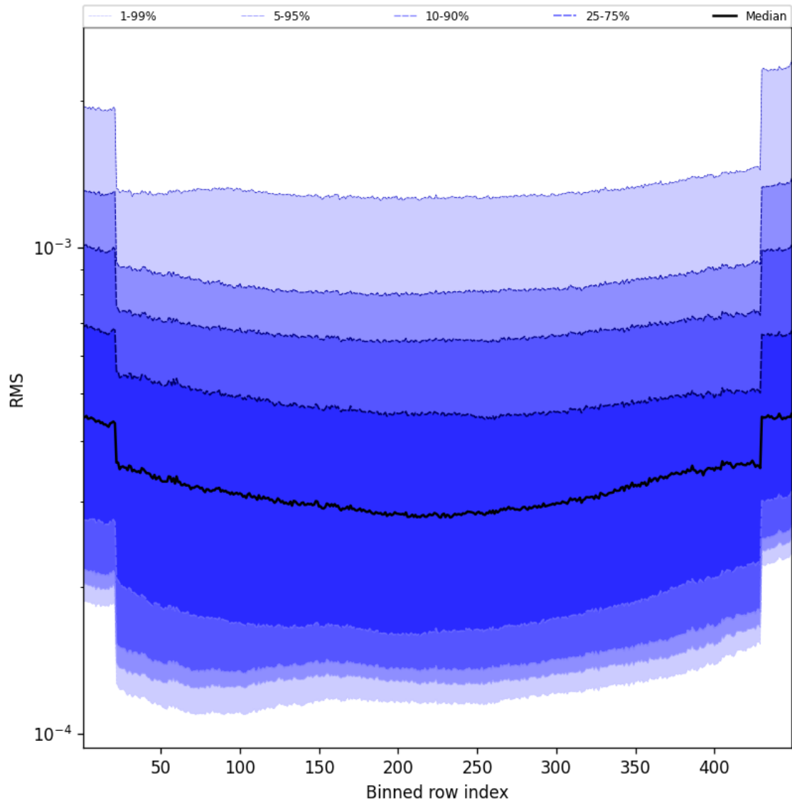
Figure 60: Along track statistics of “RMS” for 2025-03-08 to 2025-03-09
