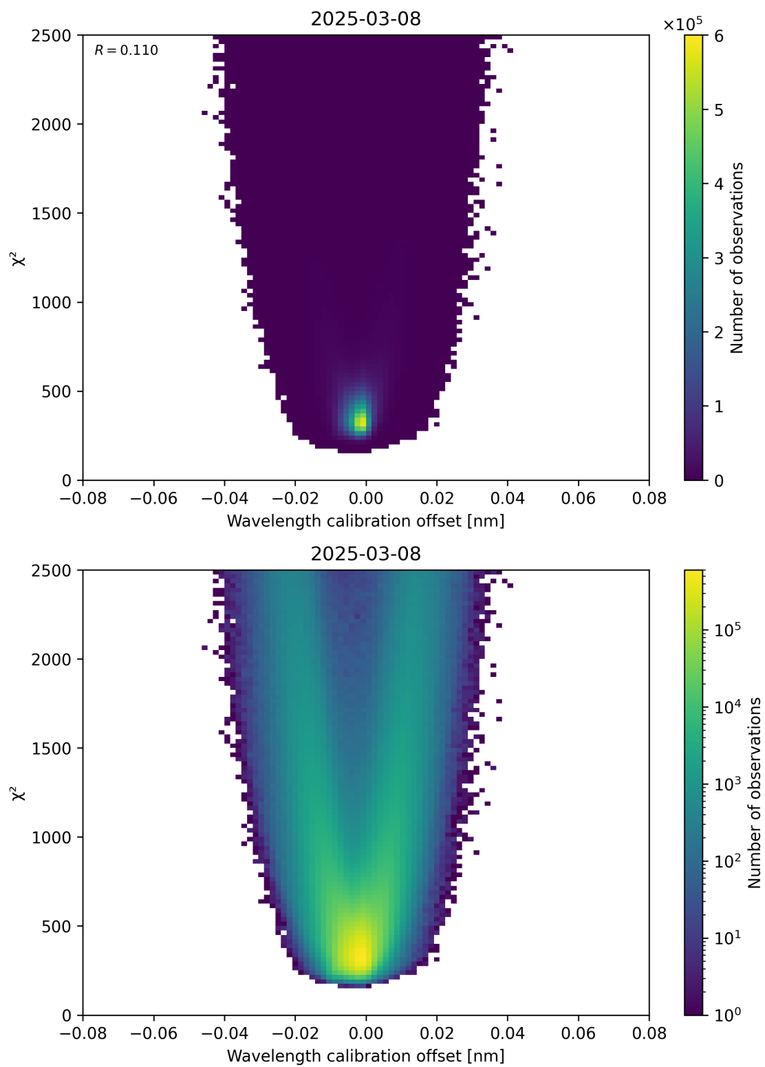
Figure 175: Scatter density plot of “Wavelength calibration offset” against “ \chi^2 ” for 2025-03-08 to 2025-03-09.
