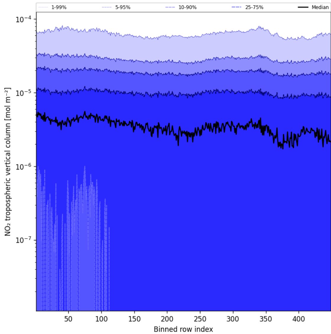
Figure 46: Along track statistics of “NO 2 tropospheric vertical column” for 2025-03-08 to 2025-03-09
