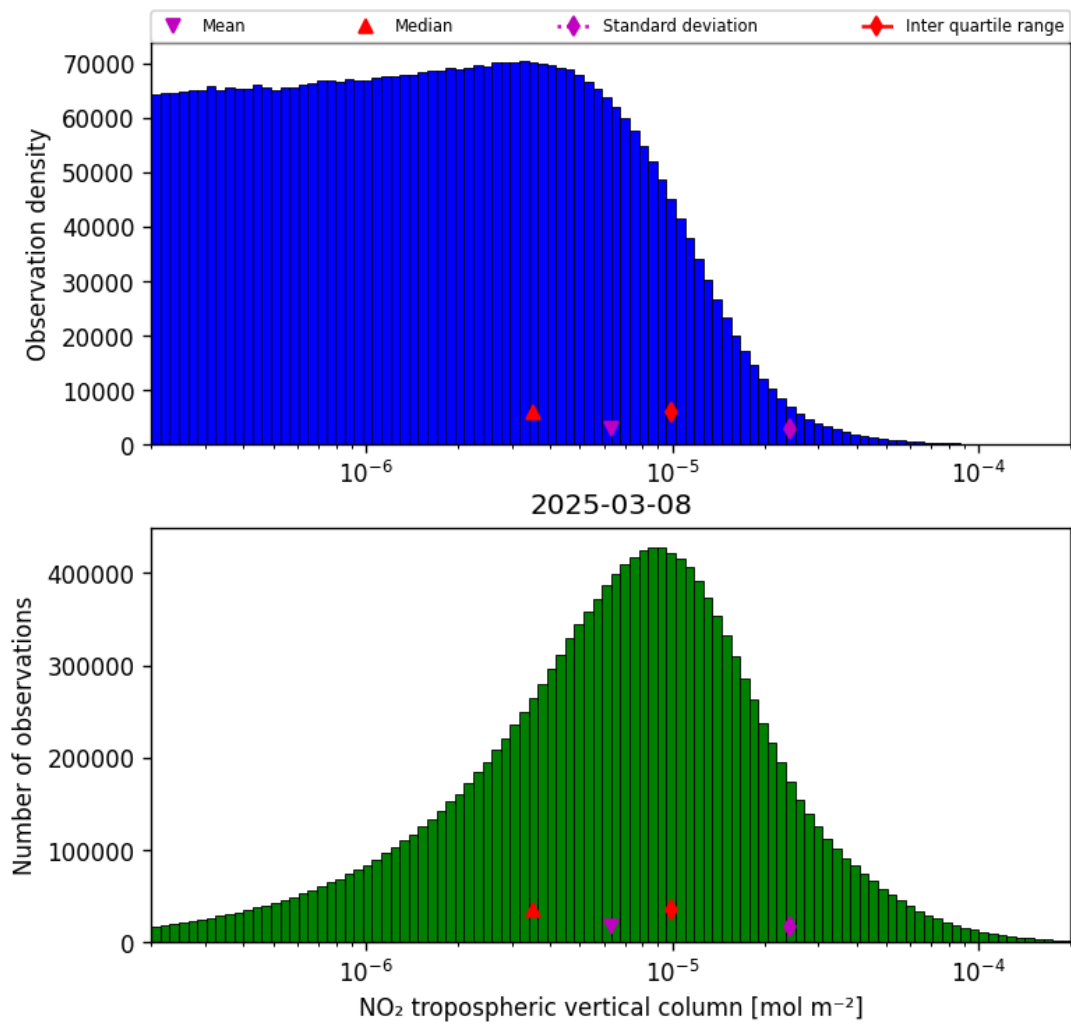
Figure 29: Histogram of “NO 2 tropospheric vertical column” for 2025-03-08 to 2025-03-09
