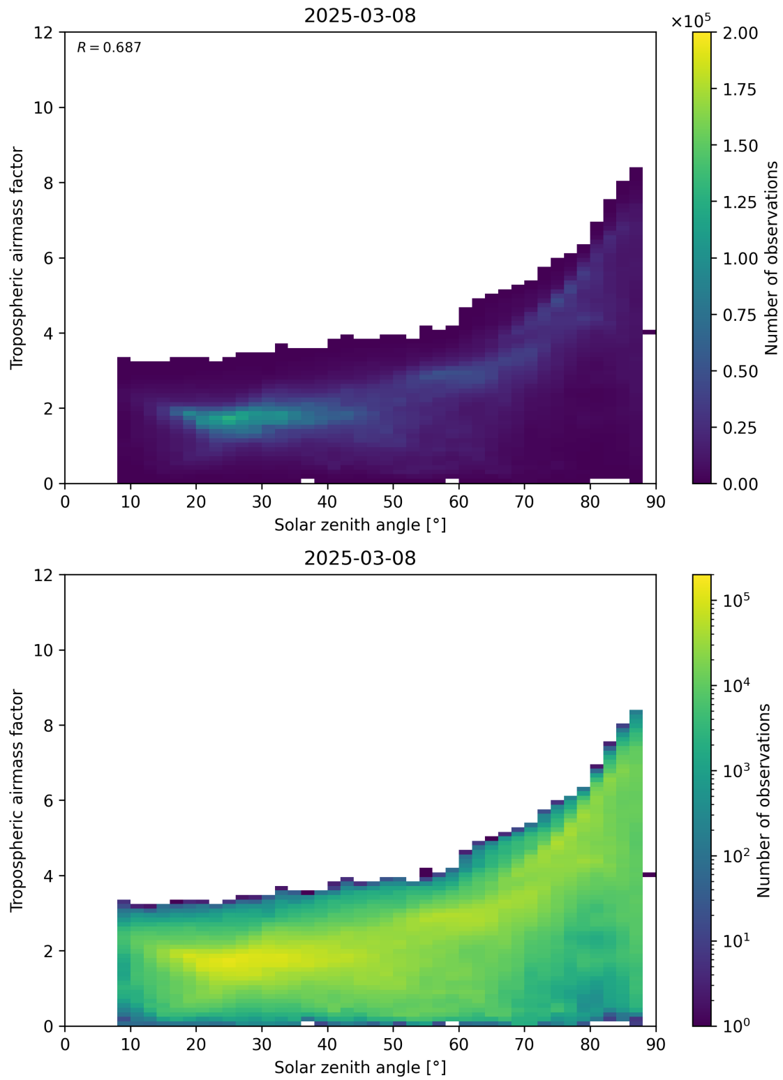
Figure 147: Scatter density plot of “Solar zenith angle” against “Tropospheric airmass factor” for 2025-03-08 to 2025-03-09.
