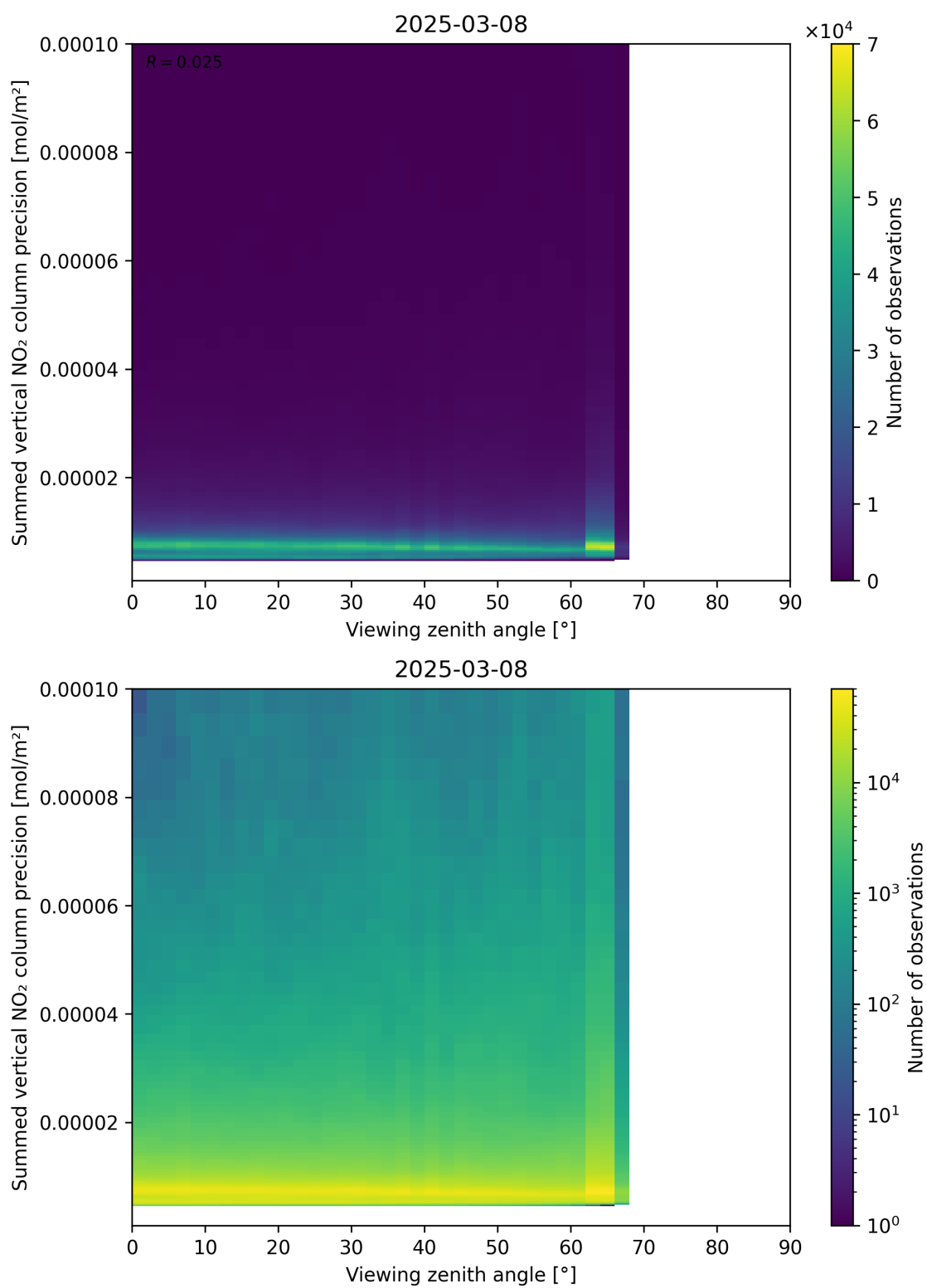
Figure 166: Scatter density plot of “Viewing zenith angle” against “Summed vertical NO 2 column precision” for 2025-03-08 to 2025-03-09.
