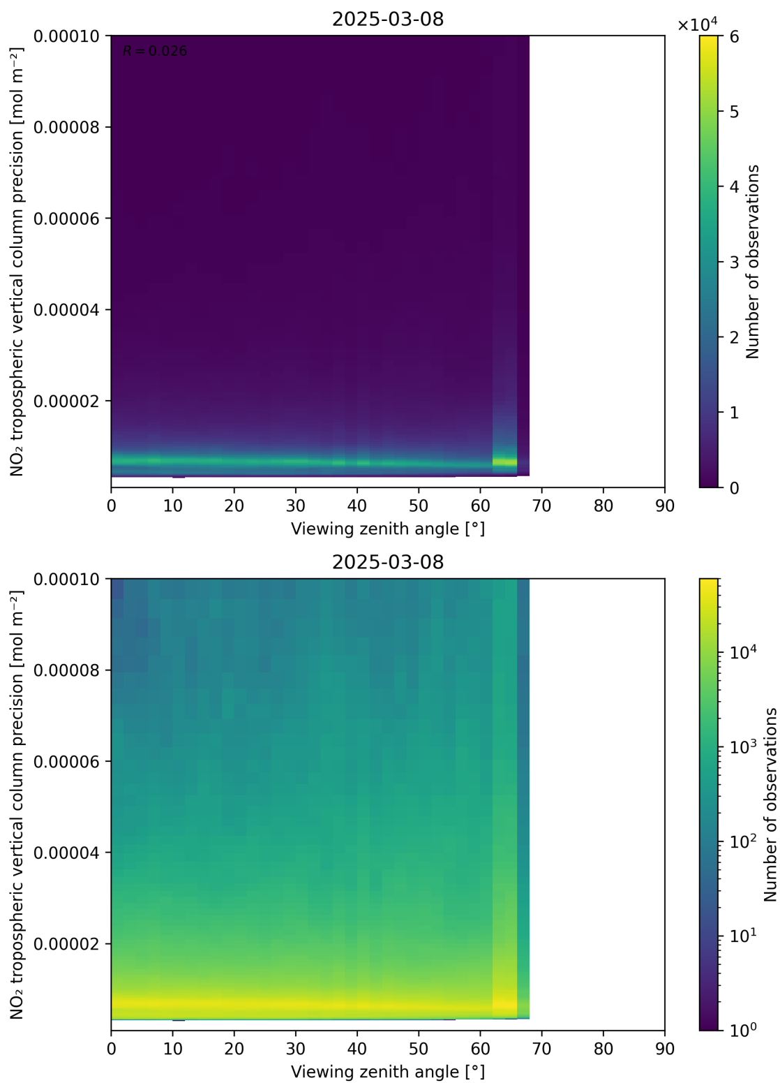
Figure 170: Scatter density plot of “Viewing zenith angle” against “NO 2 tropospheric vertical column precision” for 2025-03-08 to 2025-03-09.
