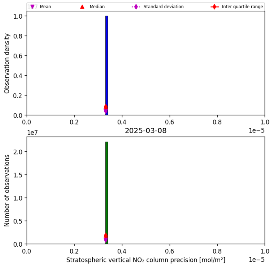
Figure 37: Histogram of “Stratospheric vertical NO 2 column precision” for 2025-03-08 to 2025-03-09
