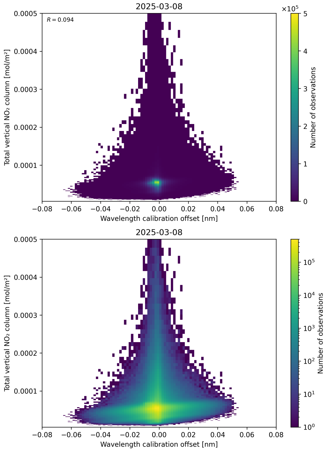
Figure 179: Scatter density plot of “Wavelength calibration offset” against “Total vertical NO 2 column” for 2025-03-08 to 2025-03-09.
