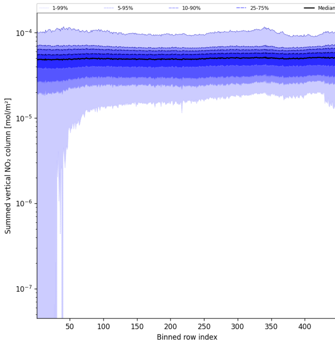
Figure 57: Along track statistics of “Summed vertical NO 2 column” for 2025-03-08 to 2025-03-09
