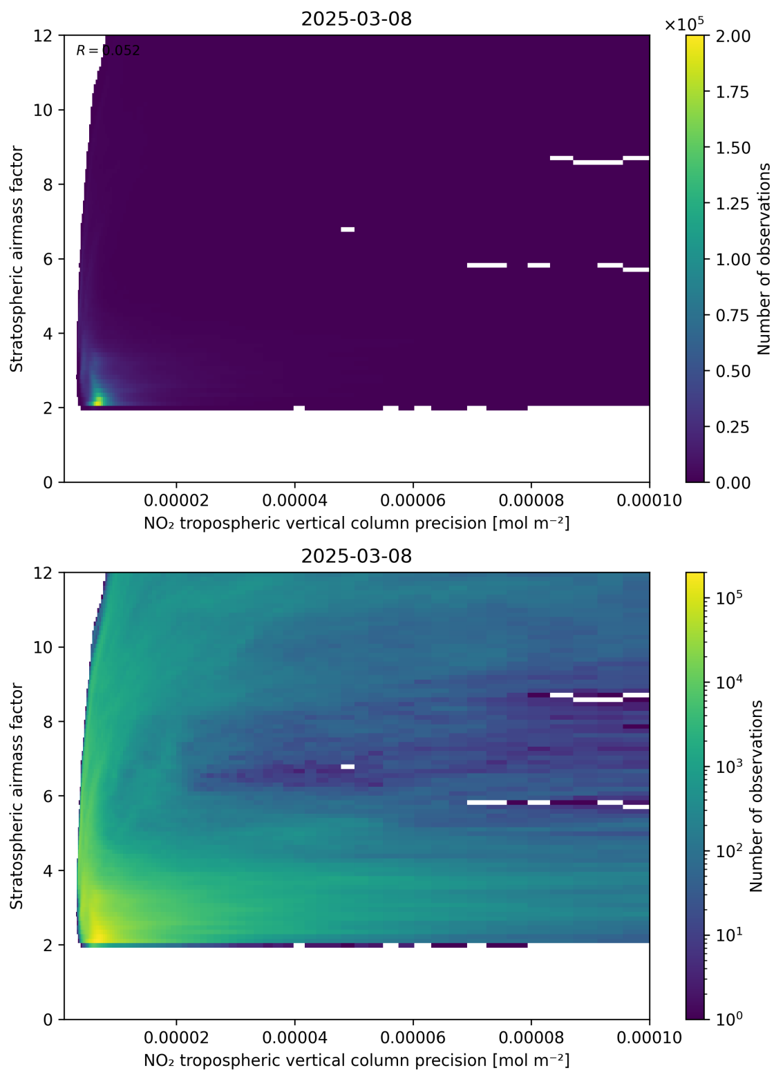
Figure 131: Scatter density plot of “NO 2 tropospheric vertical column precision” against “Stratospheric airmass factor” for 2025-03-08 to 2025-03-09.
