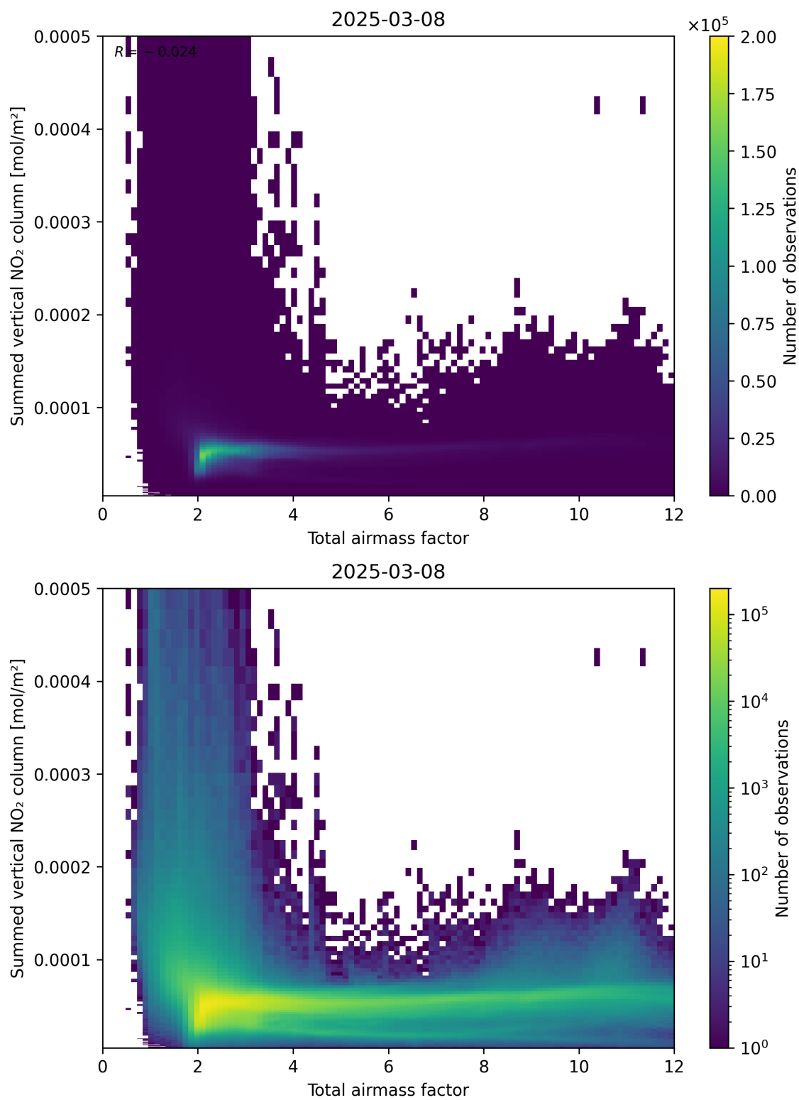
Figure 65: Scatter density plot of “Total airmass factor” against “Summed vertical NO 2 column” for 2025-03-08 to 2025-03-09.
