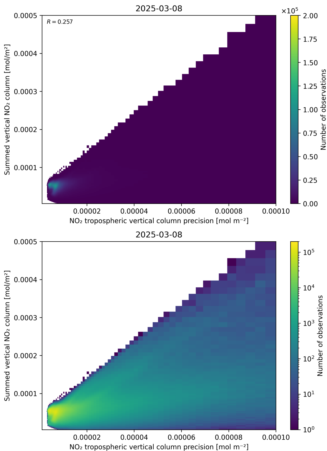
Figure 136: Scatter density plot of “NO 2 tropospheric vertical column precision” against “Summed vertical NO 2 column” for 2025-03-08 to 2025-03-09.
