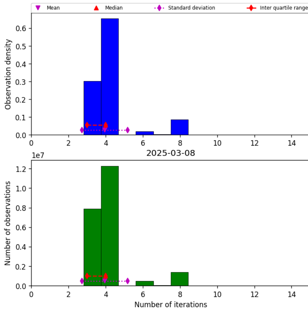
Figure 34: Histogram of “Number of iterations” for 2025-03-08 to 2025-03-09
