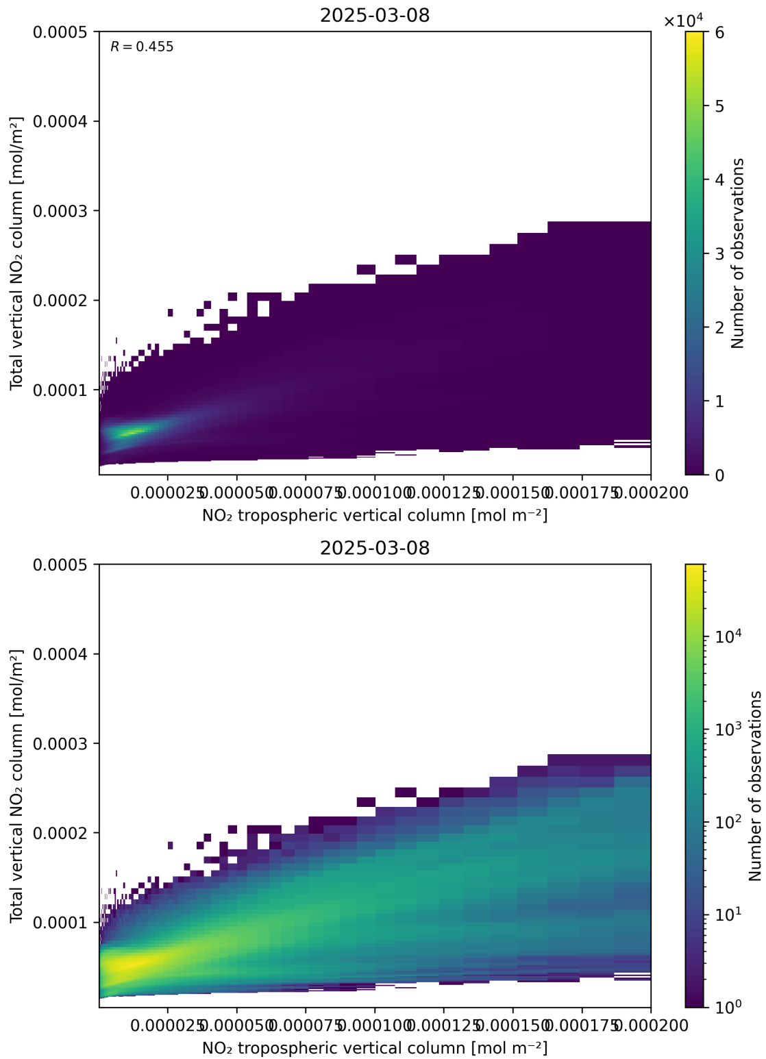
Figure 128: Scatter density plot of “NO 2 tropospheric vertical column” against “Total vertical NO 2 column” for 2025-03-08 to 2025-03-09.
