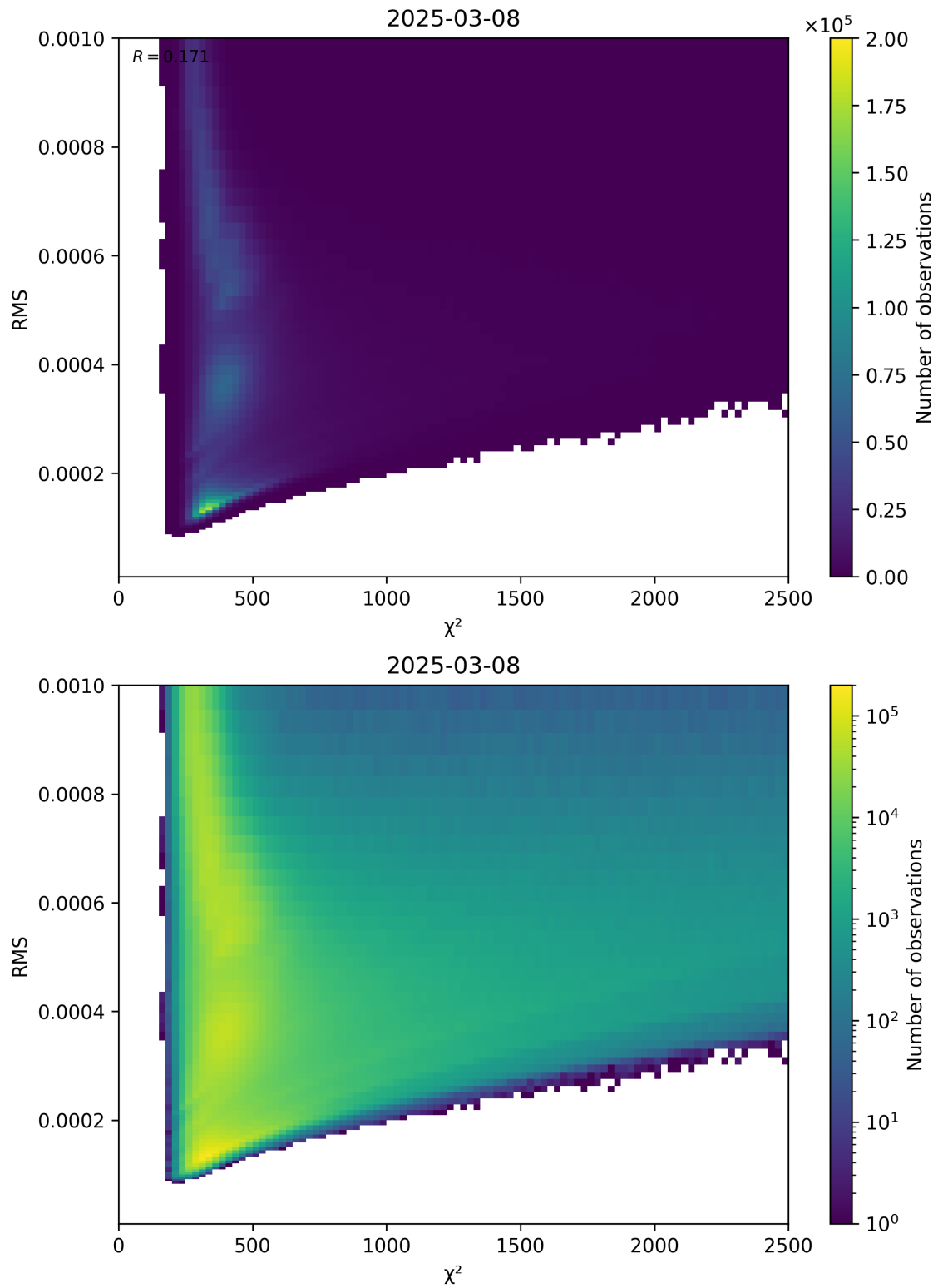
Figure 82: Scatter density plot of “ \chi^2 ” against “RMS” for 2025-03-08 to 2025-03-09.
