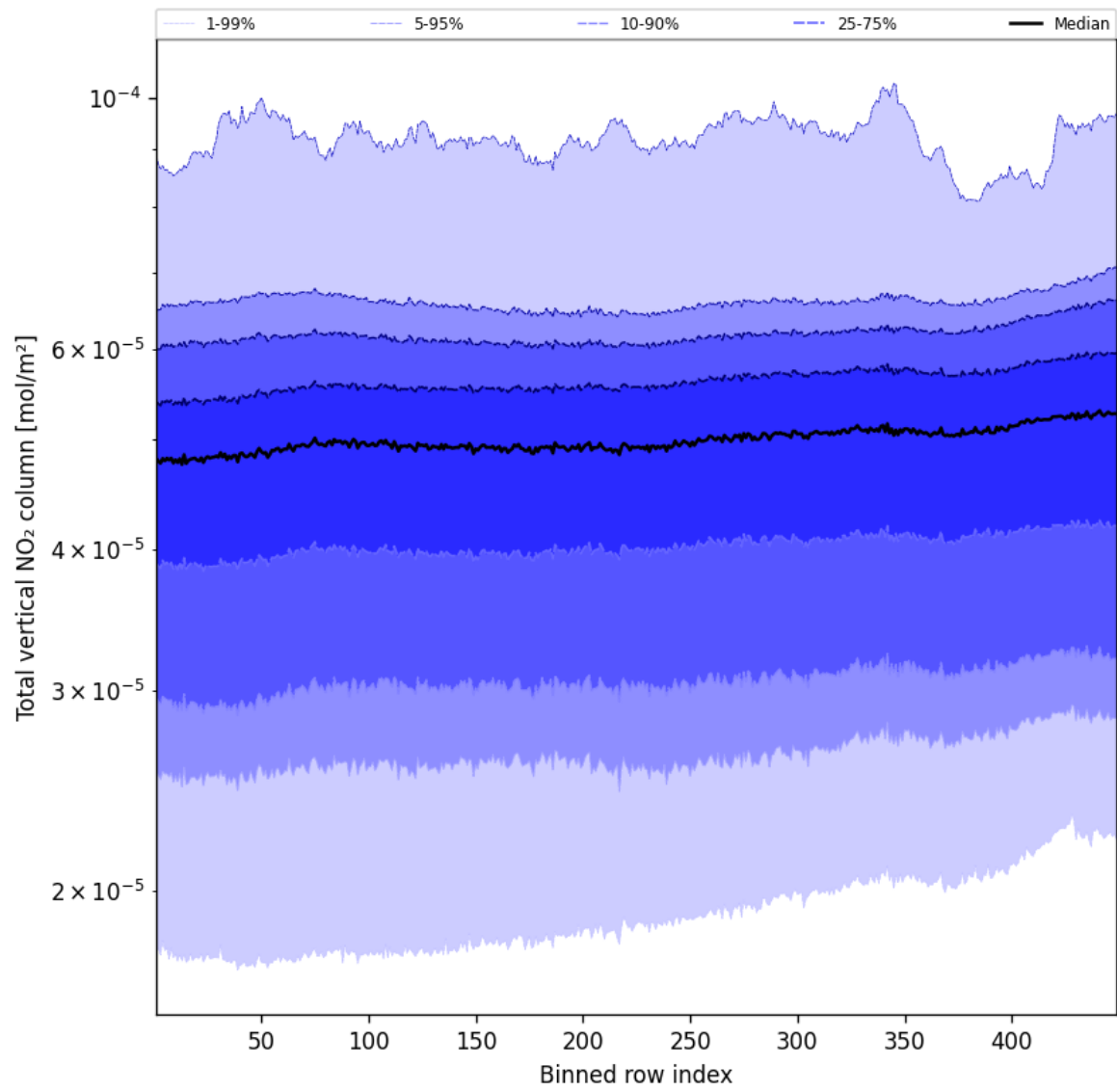
Figure 55: Along track statistics of “Total vertical NO 2 column” for 2025-03-08 to 2025-03-09
