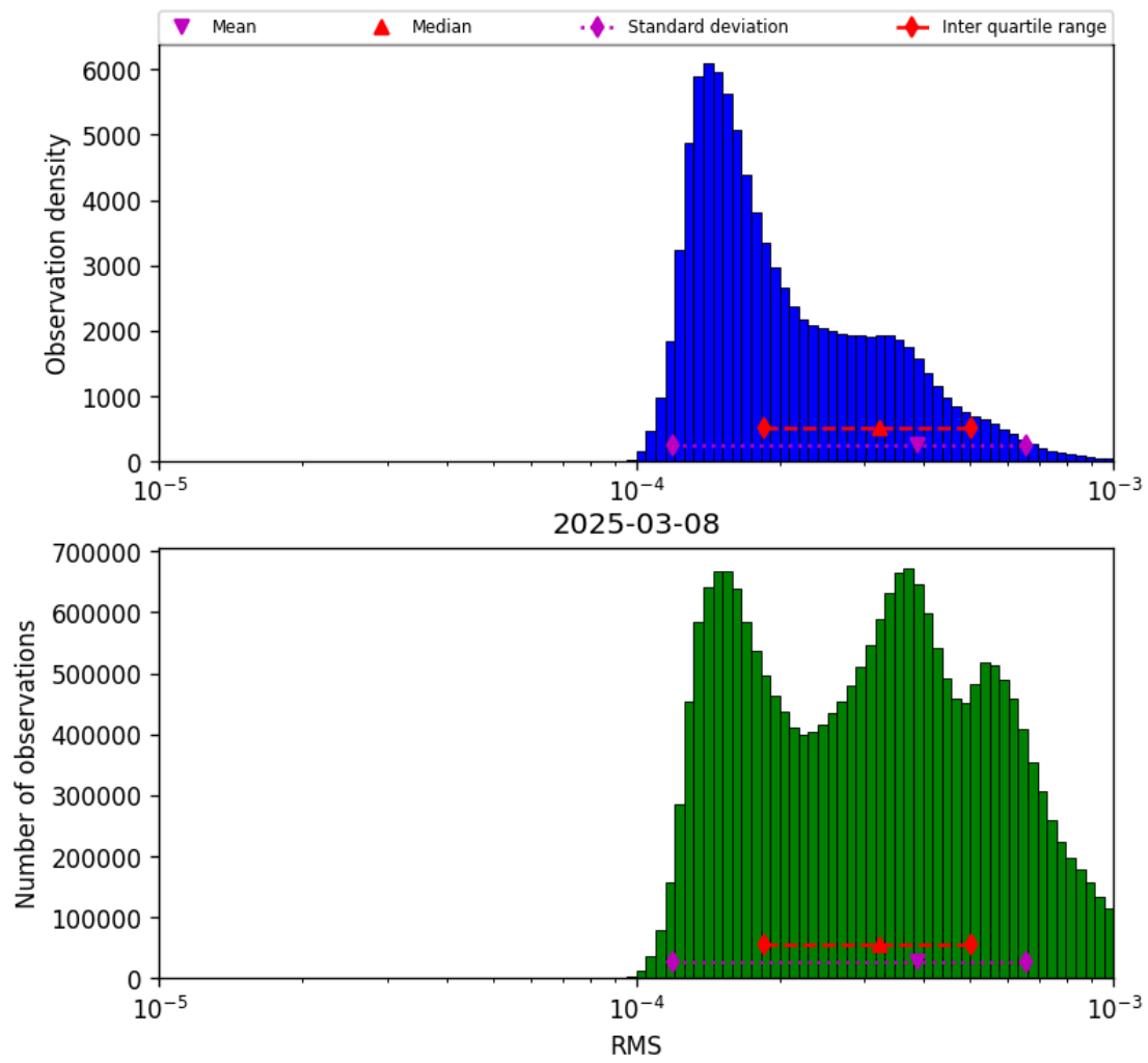
Figure 43: Histogram of “RMS” for 2025-03-08 to 2025-03-09
