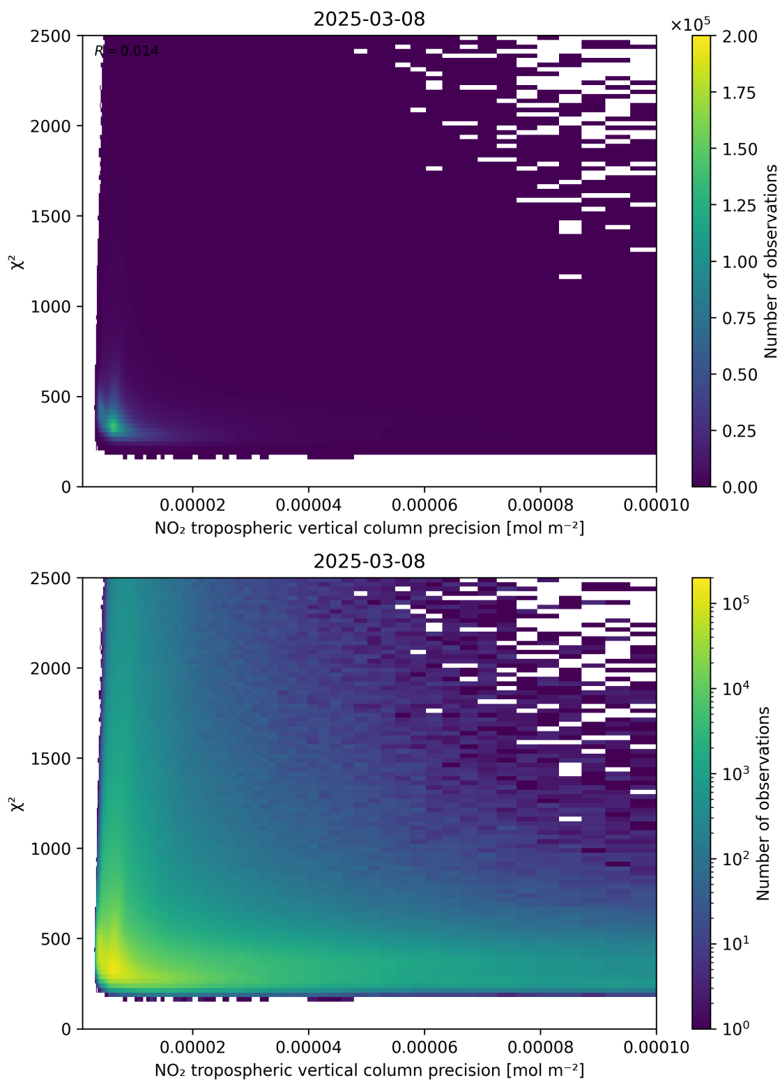
Figure 134: Scatter density plot of “NO 2 tropospheric vertical column precision” against “ \chi^2 ” for 2025-03-08 to 2025-03-09.
