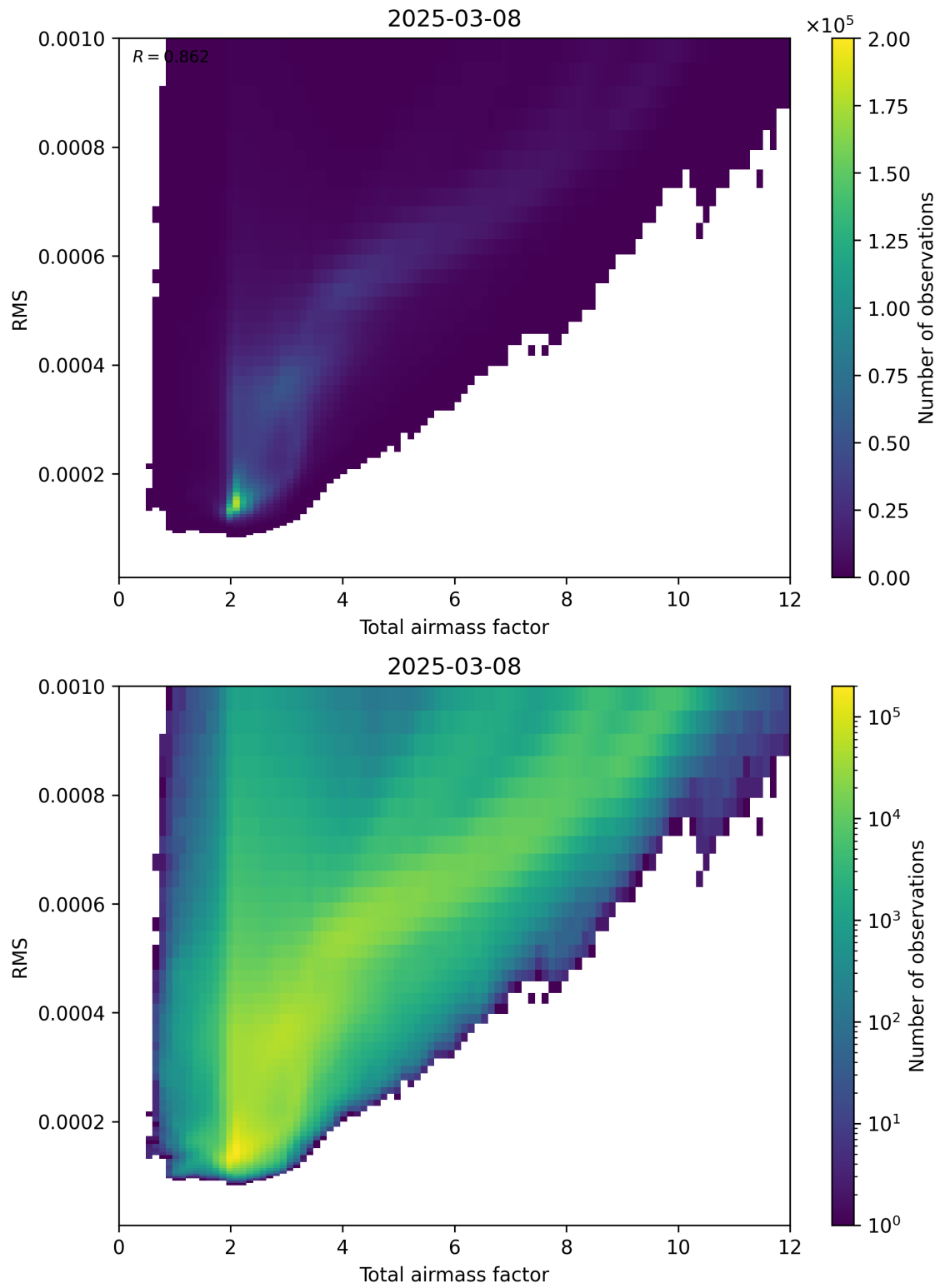
Figure 69: Scatter density plot of “Total airmass factor” against “RMS” for 2025-03-08 to 2025-03-09.
