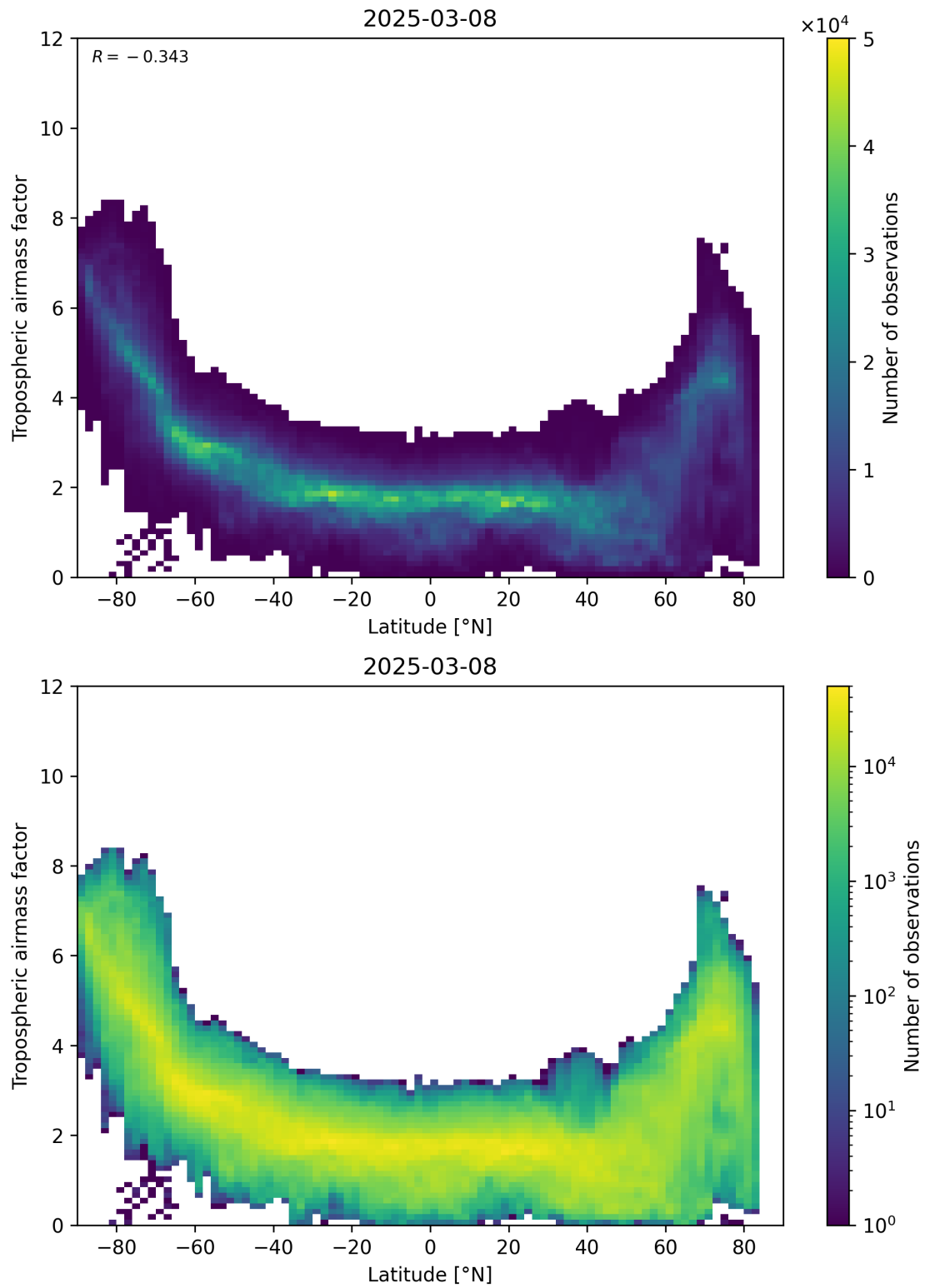
Figure 85: Scatter density plot of “Latitude” against “Tropospheric airmass factor” for 2025-03-08 to 2025-03-09.
