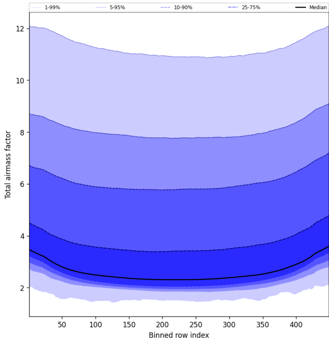
Figure 49: Along track statistics of “Total airmass factor” for 2025-03-08 to 2025-03-09
