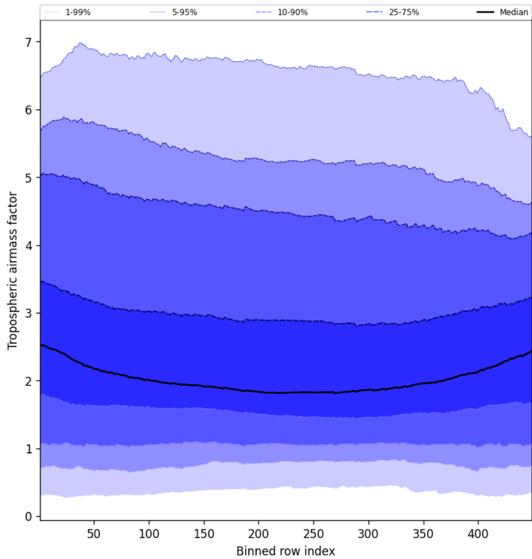
Figure 48: Along track statistics of “Tropospheric airmass factor” for 2025-03-08 to 2025-03-09
