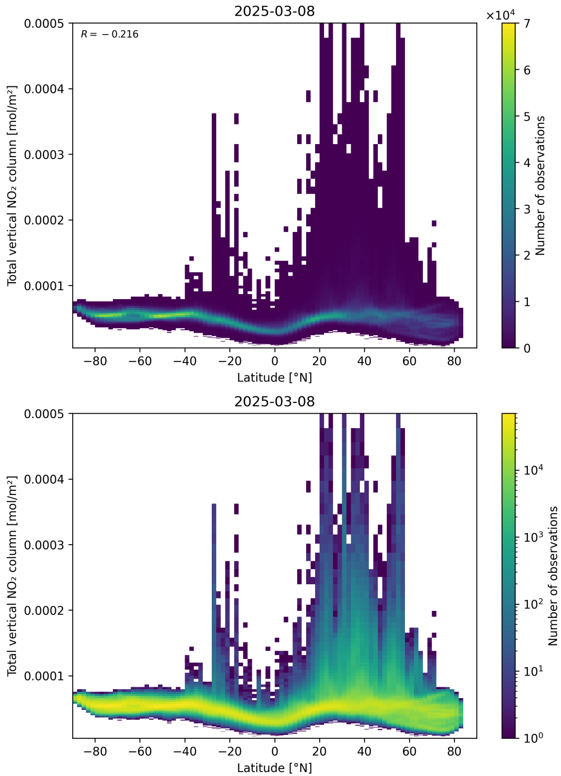
Figure 90: Scatter density plot of “Latitude” against “Total vertical NO 2 column” for 2025-03-08 to 2025-03-09.
