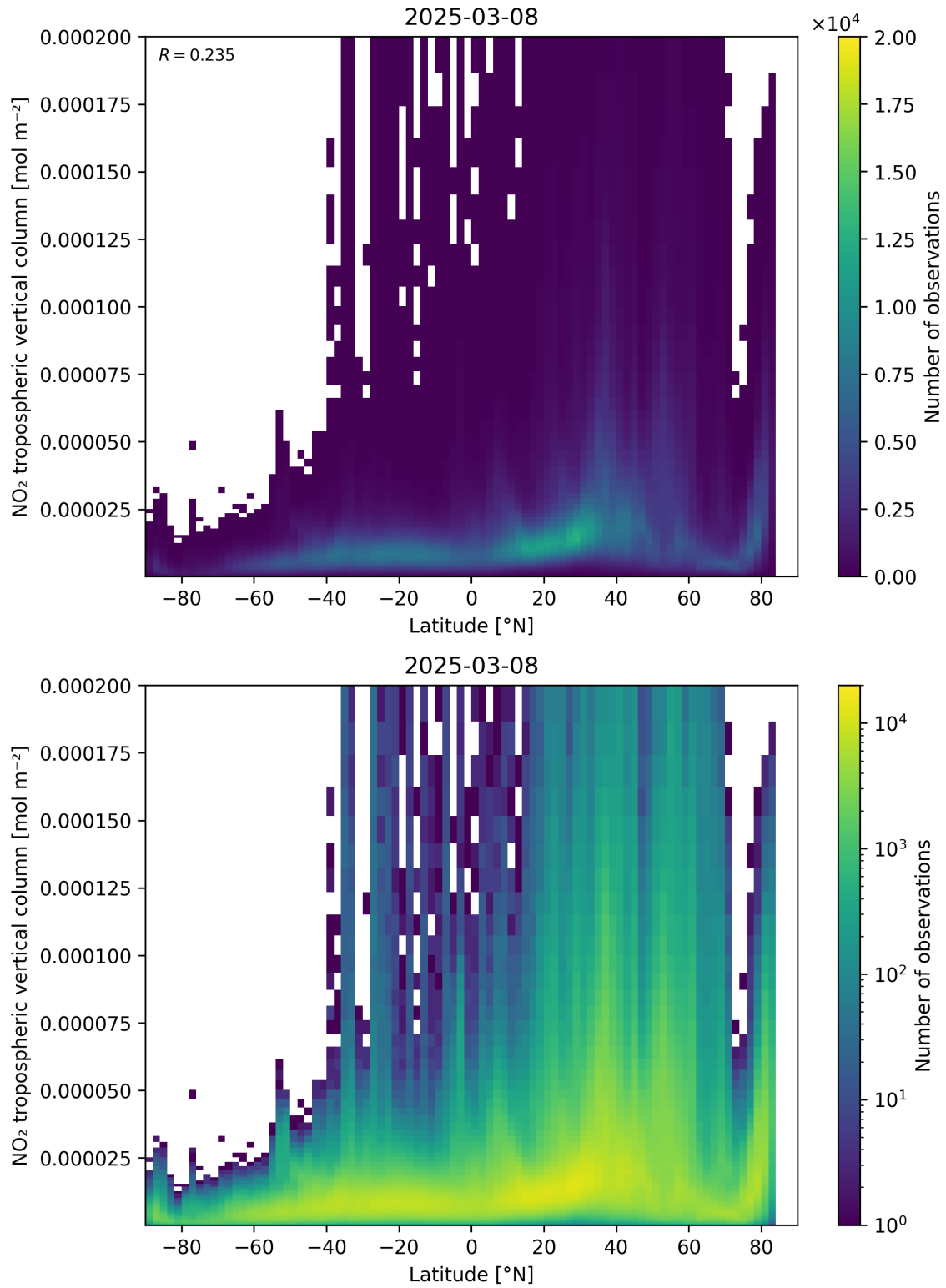
Figure 92: Scatter density plot of “Latitude” against “NO 2 tropospheric vertical column” for 2025-03-08 to 2025-03-09.
