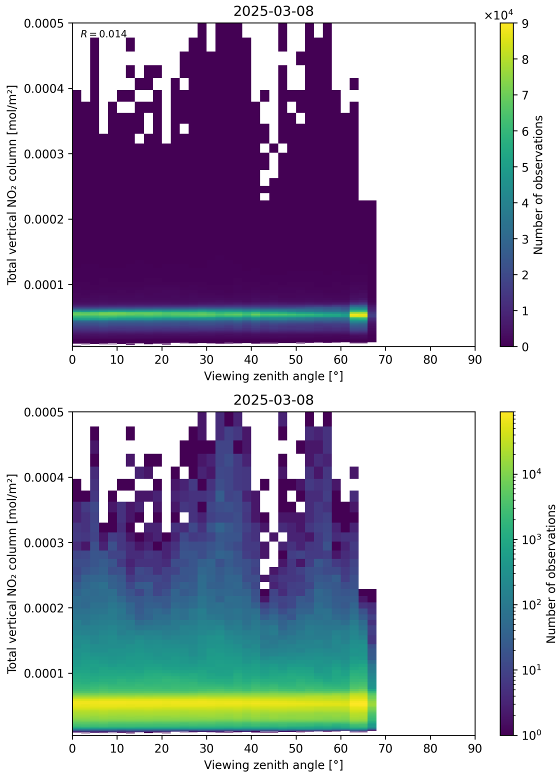
Figure 167: Scatter density plot of “Viewing zenith angle” against “Total vertical NO 2 column” for 2025-03-08 to 2025-03-09.
