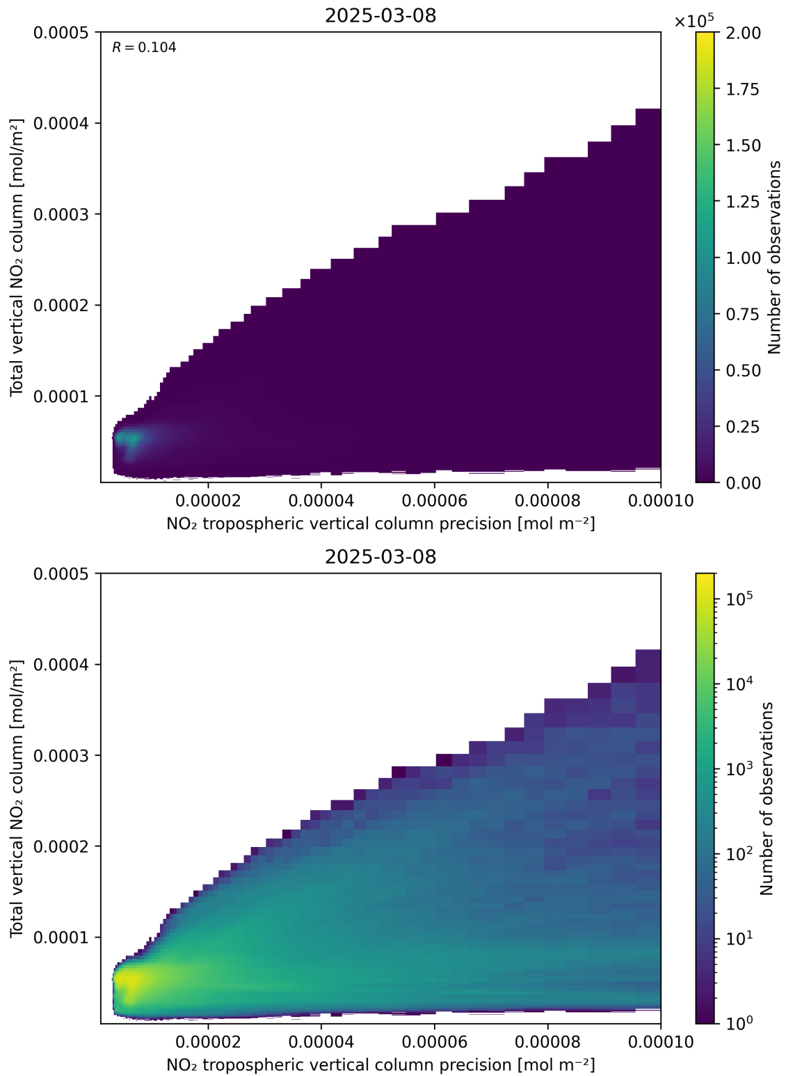
Figure 138: Scatter density plot of “NO 2 tropospheric vertical column precision” against “Total vertical NO 2 column” for 2025-03-08 to 2025-03-09.
