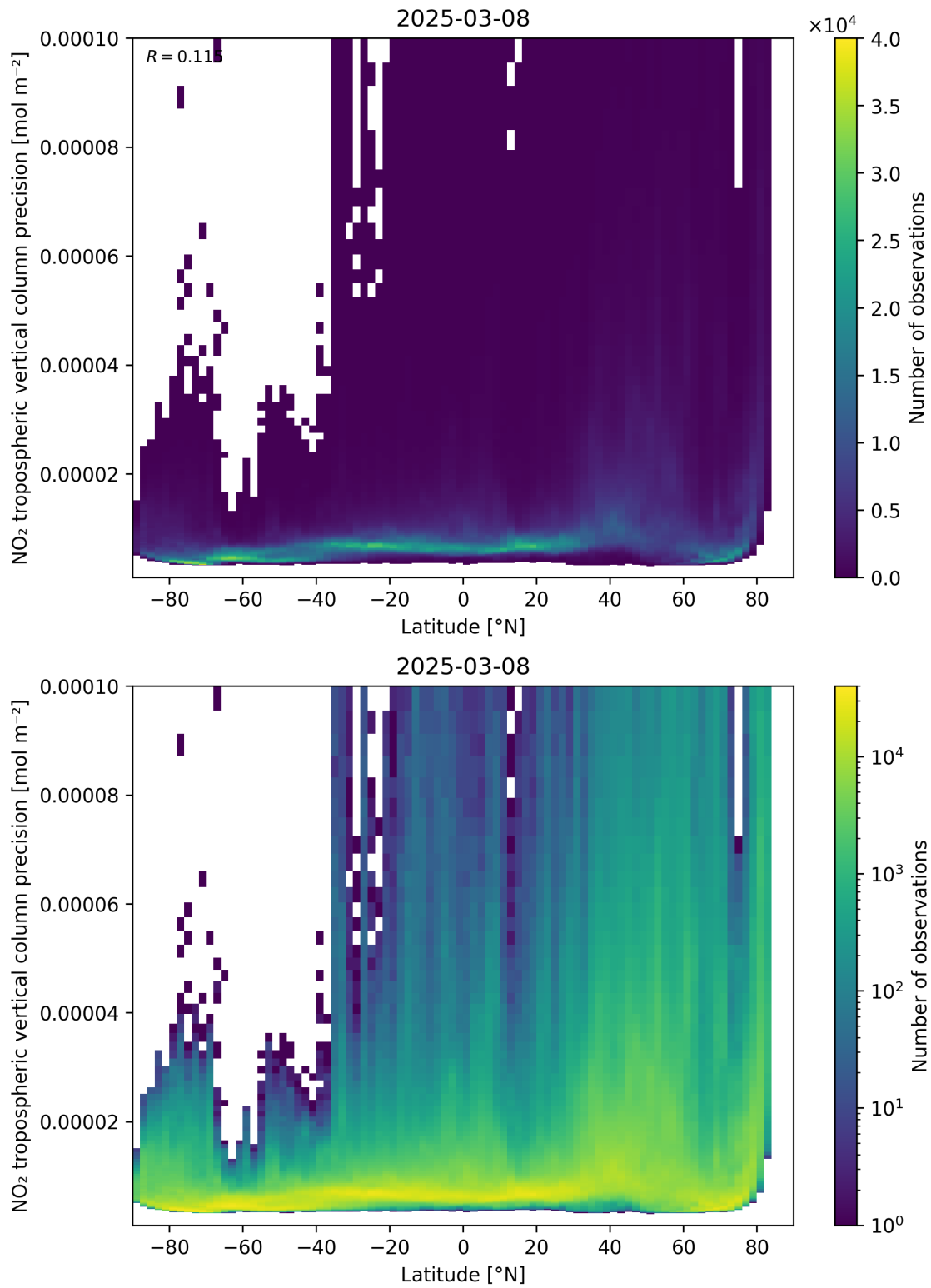
Figure 93: Scatter density plot of “Latitude” against “NO 2 tropospheric vertical column precision” for 2025-03-08 to 2025-03-09.
