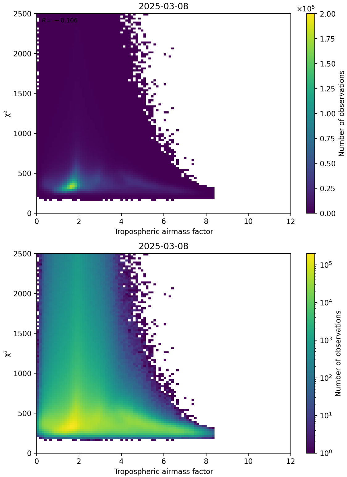
Figure 73: Scatter density plot of “Tropospheric airmass factor” against “ \chi^2 ” for 2025-03-08 to 2025-03-09.
