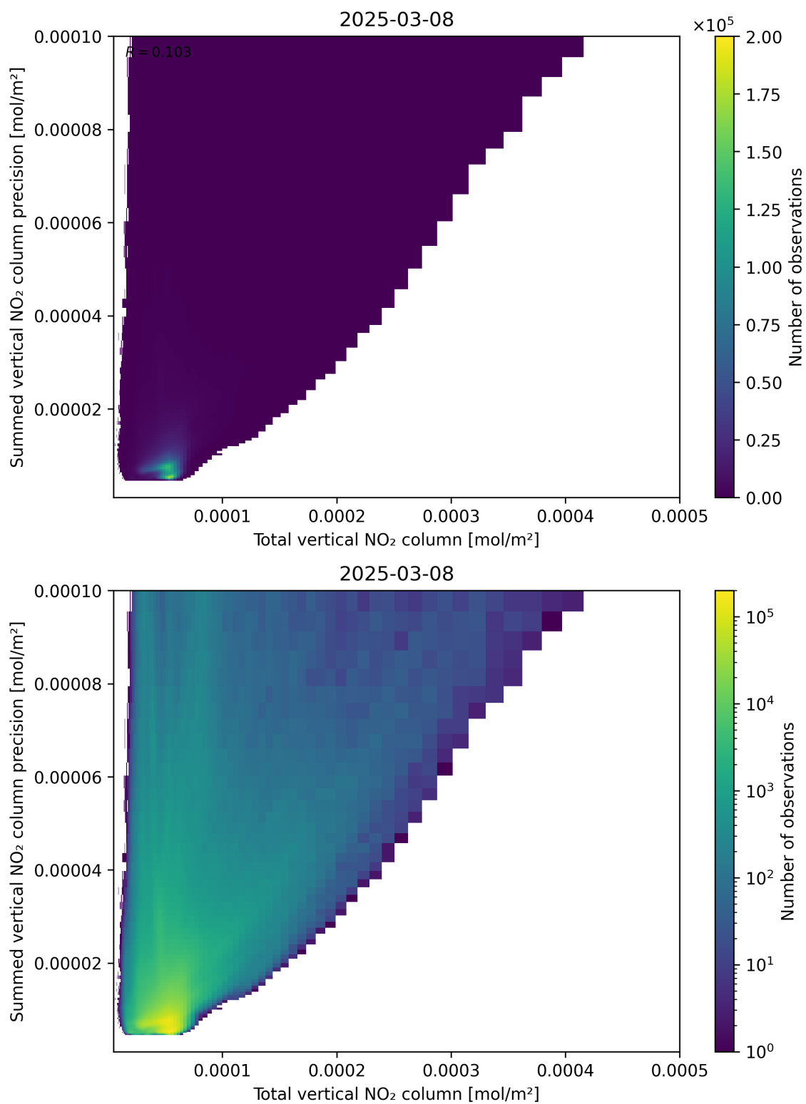
Figure 113: Scatter density plot of “Total vertical NO 2 column” against “Summed vertical NO 2 column precision” for 2025-03-08 to 2025-03-09.
