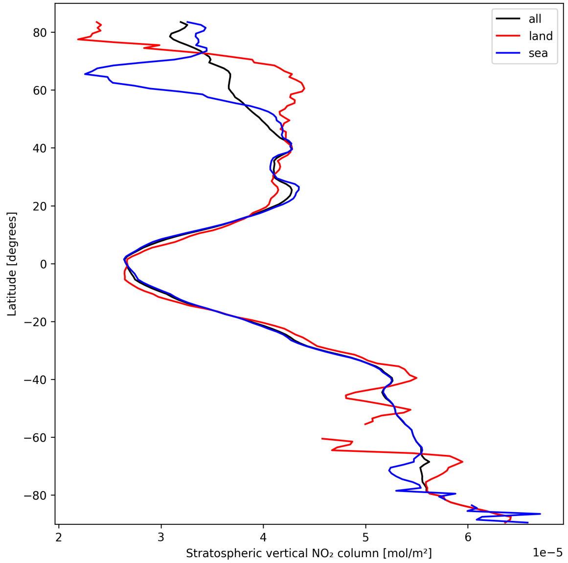
Figure 19: Zonal average of “Stratospheric vertical NO 2 column” for 2025-03-08 to 2025-03-09.
