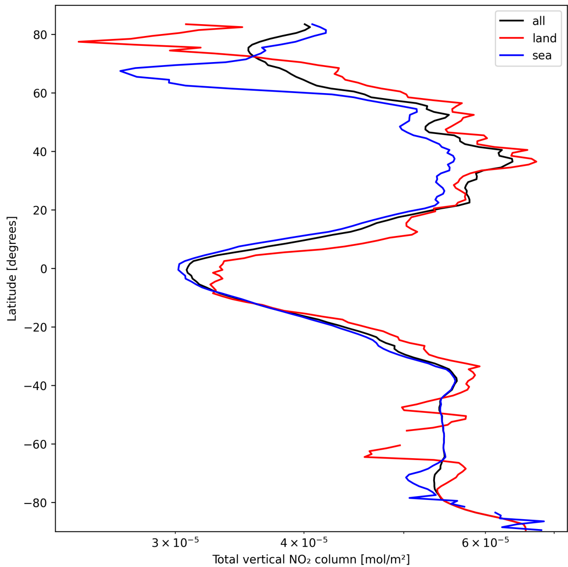
Figure 21: Zonal average of “Total vertical NO 2 column” for 2025-03-08 to 2025-03-09.
