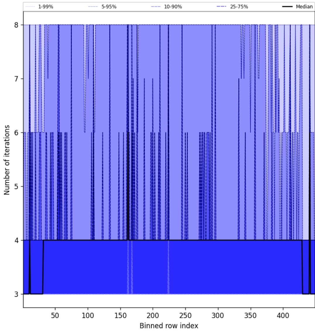
Figure 51: Along track statistics of “Number of iterations” for 2025-03-08 to 2025-03-09
