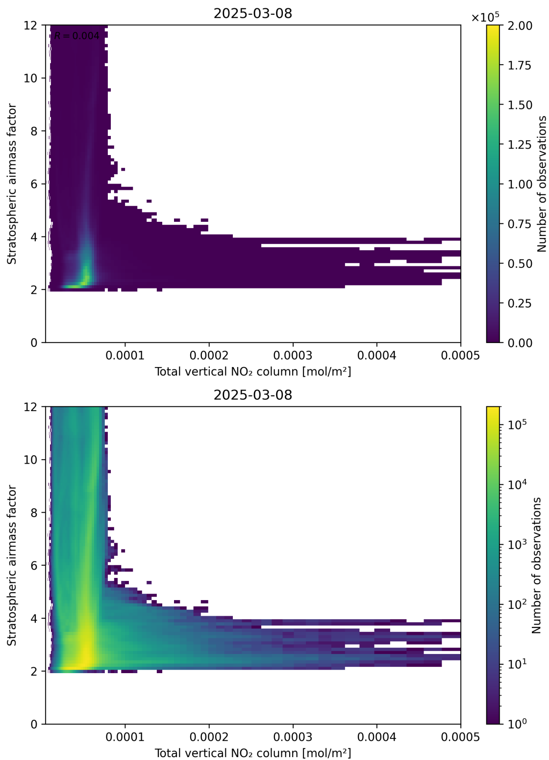
Figure 110: Scatter density plot of “Total vertical NO 2 column” against “Stratospheric airmass factor” for 2025-03-08 to 2025-03-09.
