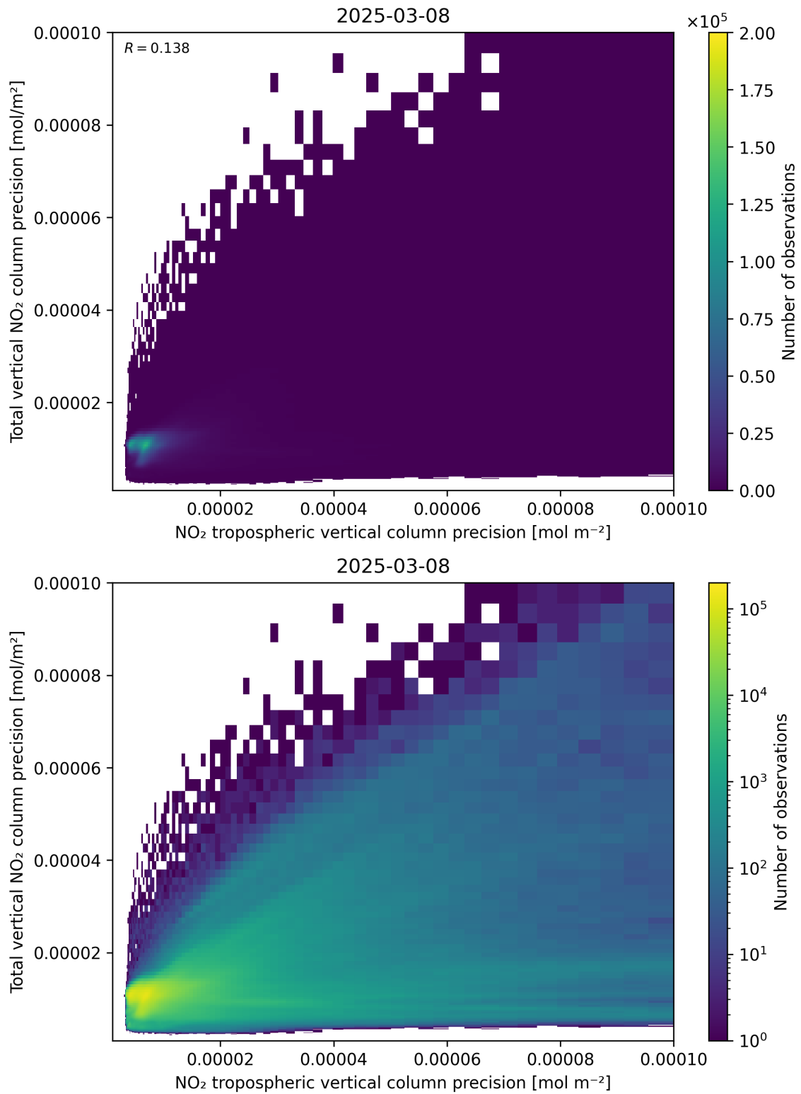
Figure 139: Scatter density plot of “NO 2 tropospheric vertical column precision” against “Total vertical NO 2 column precision” for 2025-03-08 to 2025-03-09.
