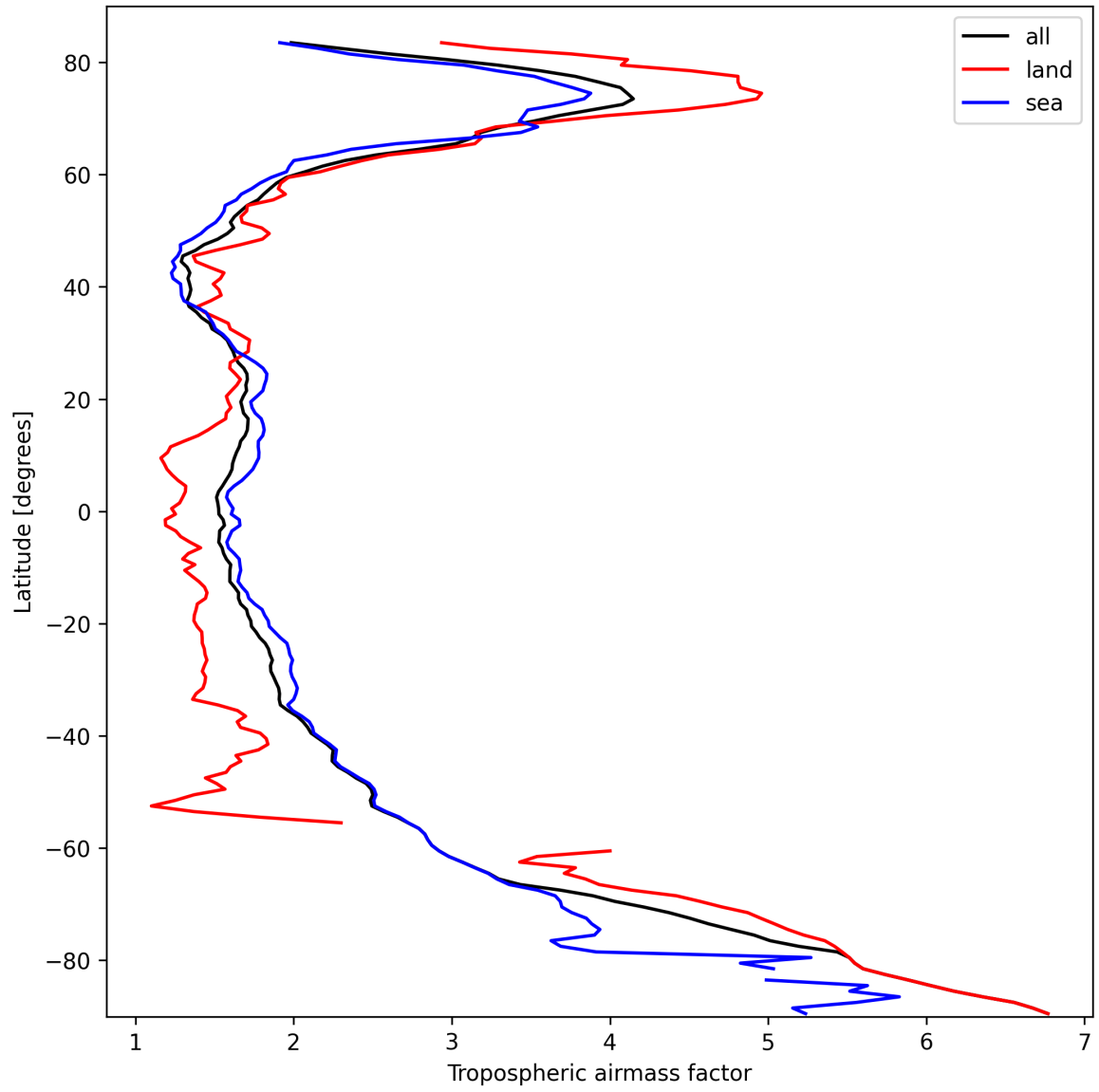
Figure 14: Zonal average of “Tropospheric airmass factor” for 2025-03-08 to 2025-03-09.
