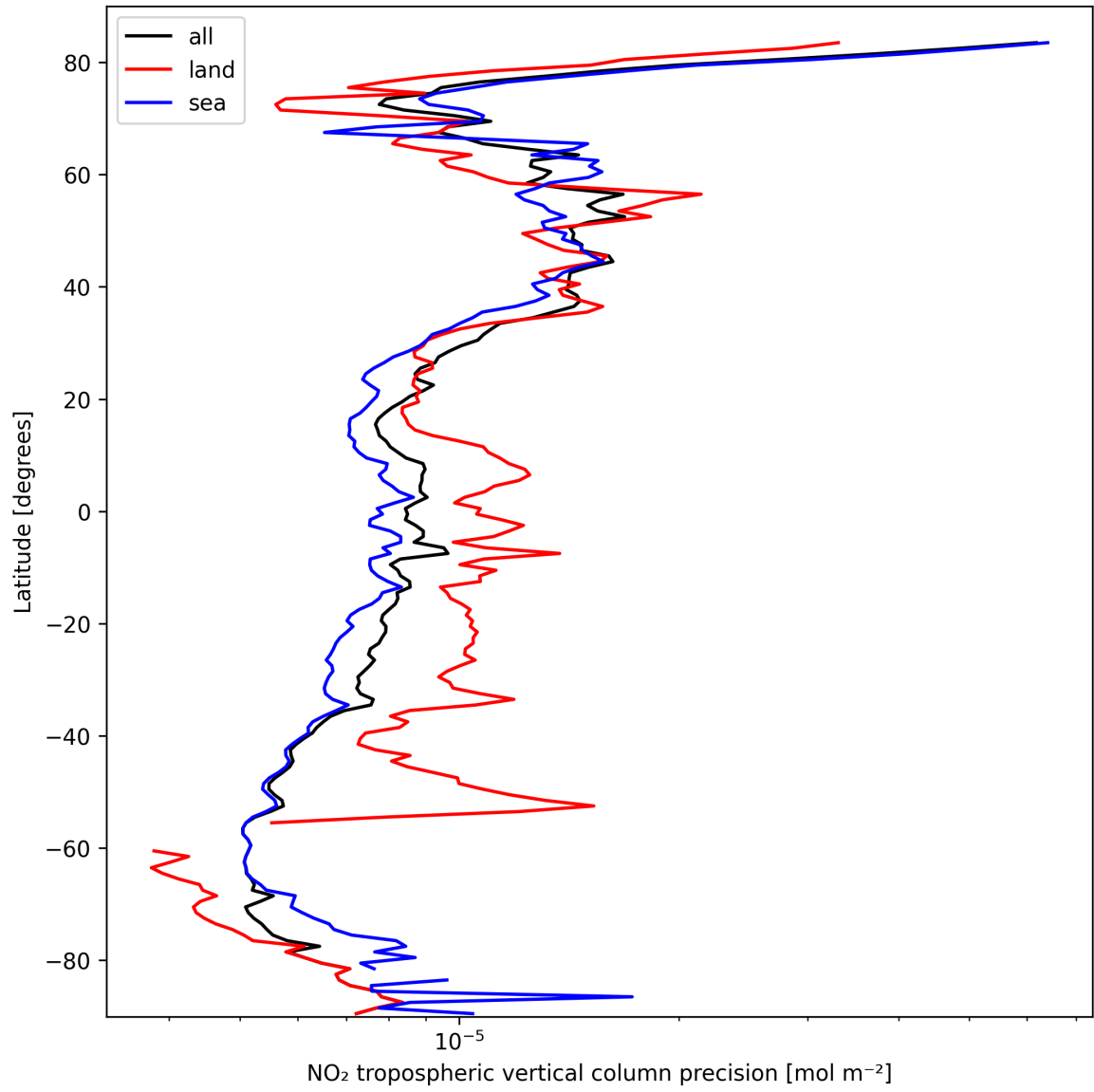
Figure 13: Zonal average of “NO 2 tropospheric vertical column precision” for 2025-03-08 to 2025-03-09.
