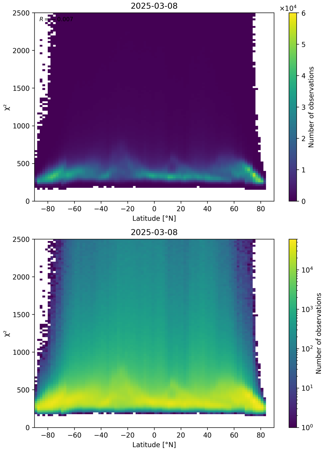
Figure 86: Scatter density plot of “Latitude” against “ \chi^2 ” for 2025-03-08 to 2025-03-09.
