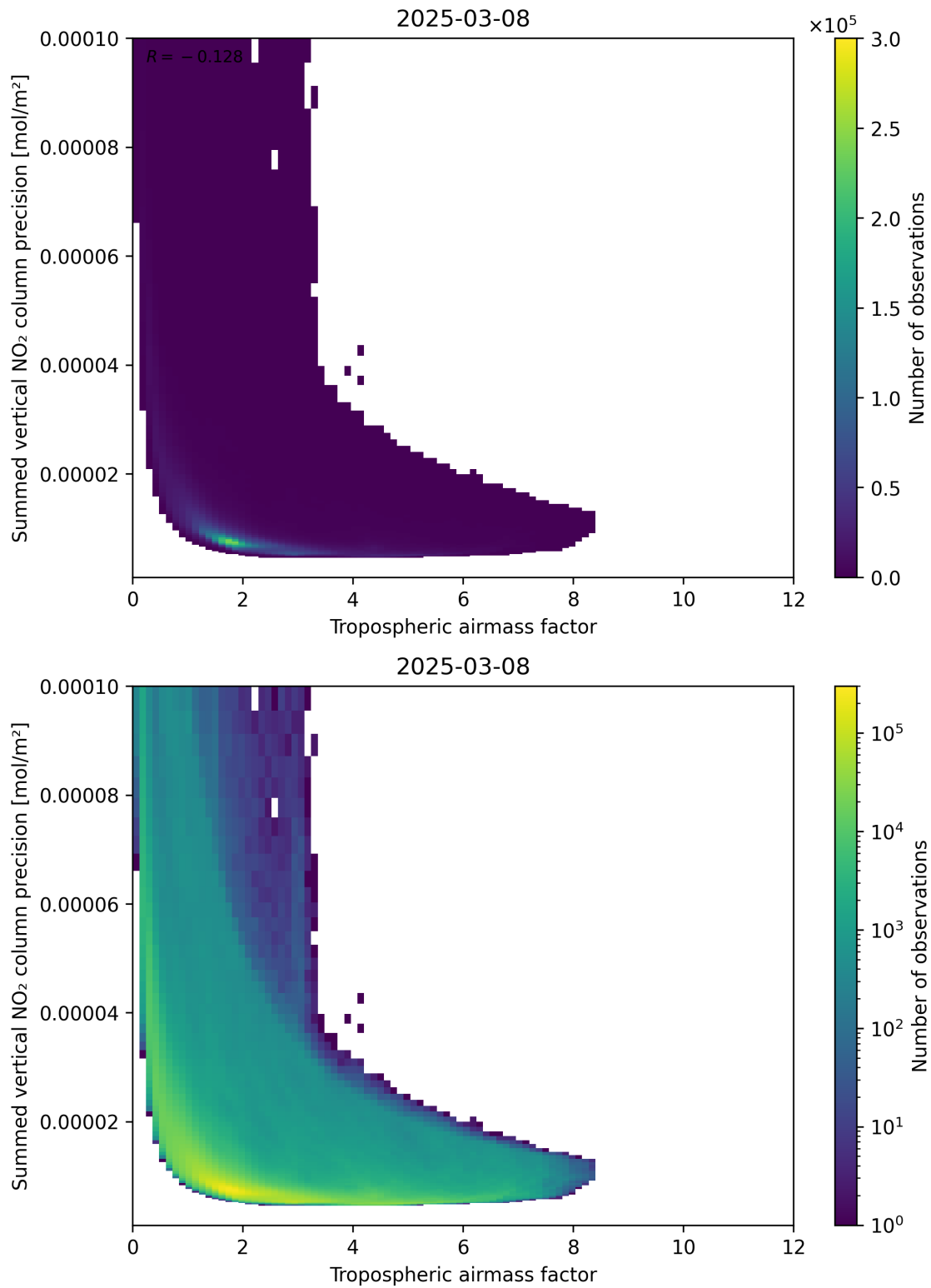
Figure 76: Scatter density plot of “Tropospheric air mass factor” against “Summed vertical NO 2 column precision” for 2025-03-08 to 2025-03-09.
