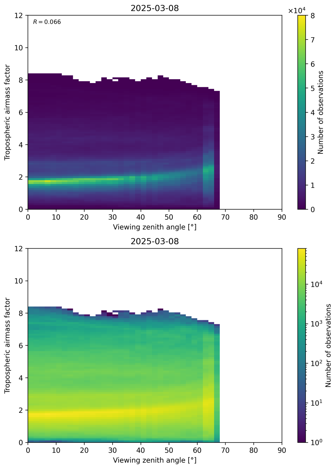
Figure 161: Scatter density plot of “Viewing zenith angle” against “Tropospheric airmass factor” for 2025-03-08 to 2025-03-09.
