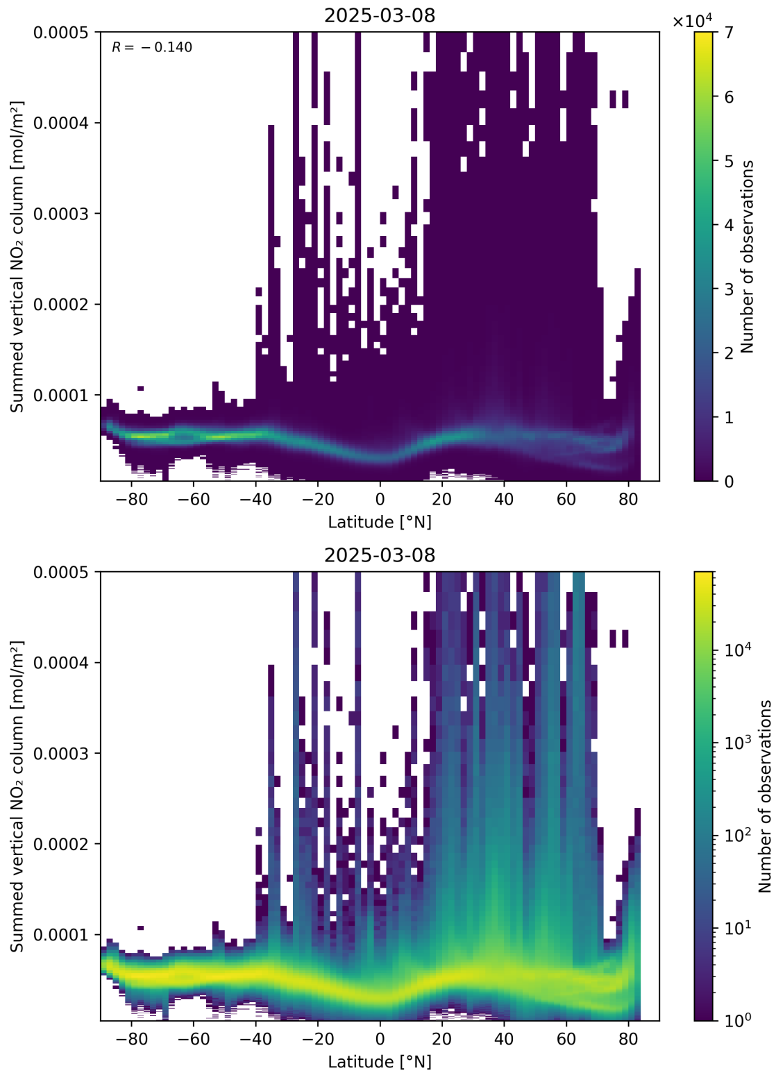
Figure 88: Scatter density plot of “Latitude” against “Summed vertical NO 2 column” for 2025-03-08 to 2025-03-09.
