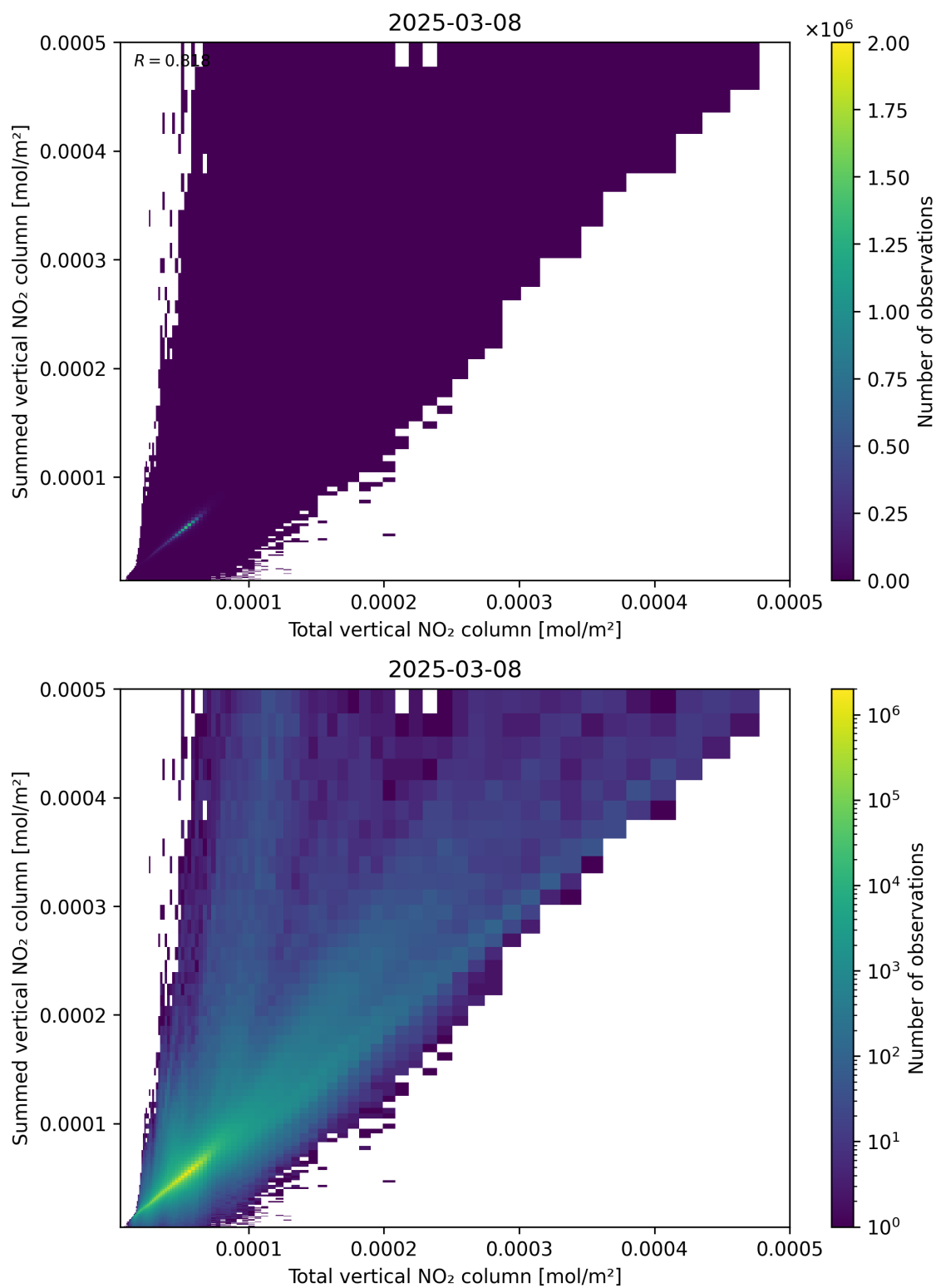
Figure 112: Scatter density plot of “Total vertical NO 2 column” against “Summed vertical NO 2 column” for 2025-03-08 to 2025-03-09.
