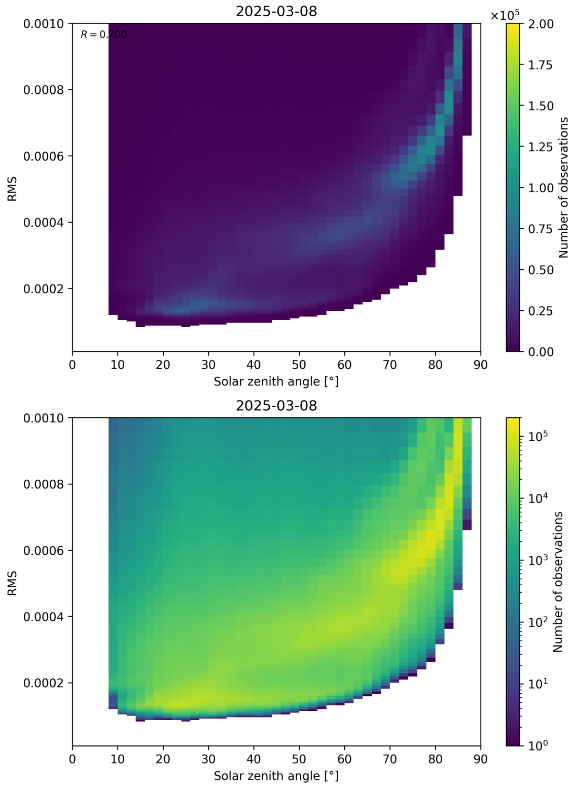
Figure 157: Scatter density plot of “Solar zenith angle” against “RMS” for 2025-03-08 to 2025-03-09.
