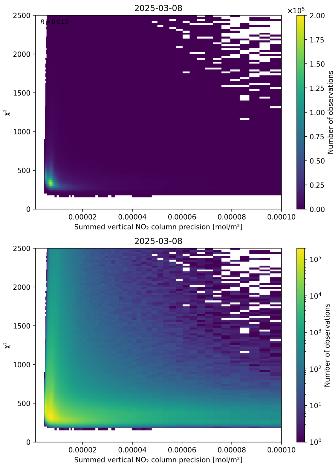
Figure 107: Scatter density plot of “Summed vertical NO 2 column precision” against “ \chi^2 ” for 2025-03-08 to 2025-03-09.
