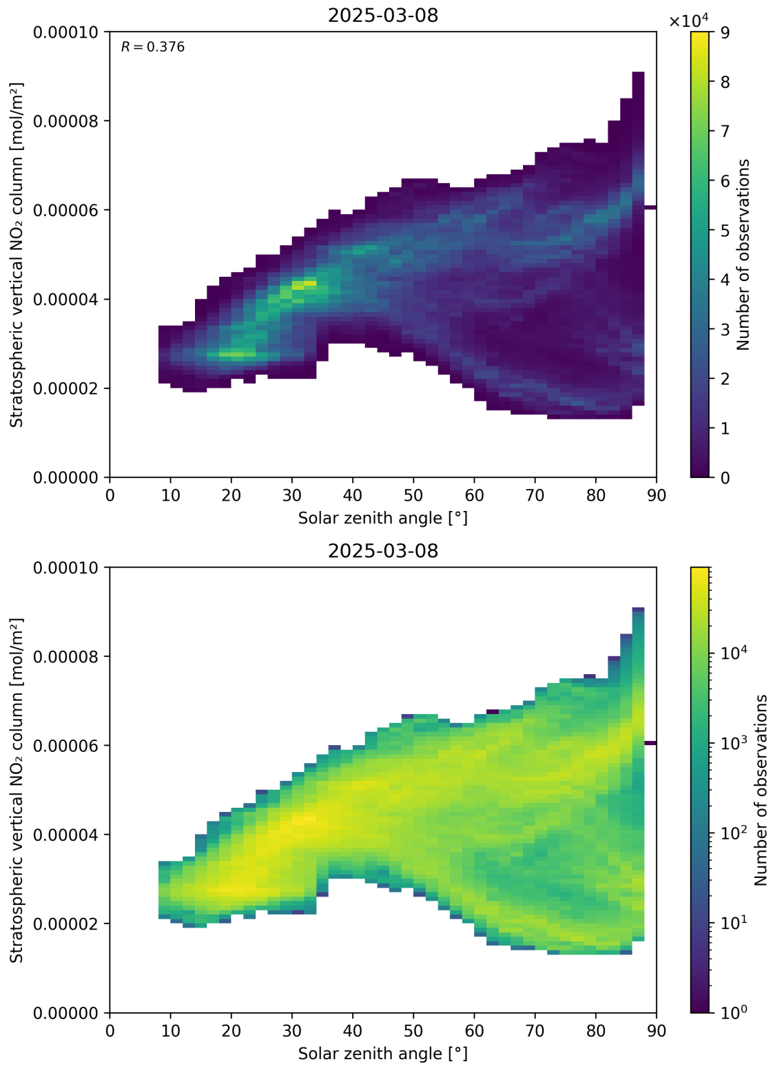
Figure 150: Scatter density plot of “Solar zenith angle” against “Stratospheric vertical NO 2 column” for 2025-03-08 to 2025-03-09.
