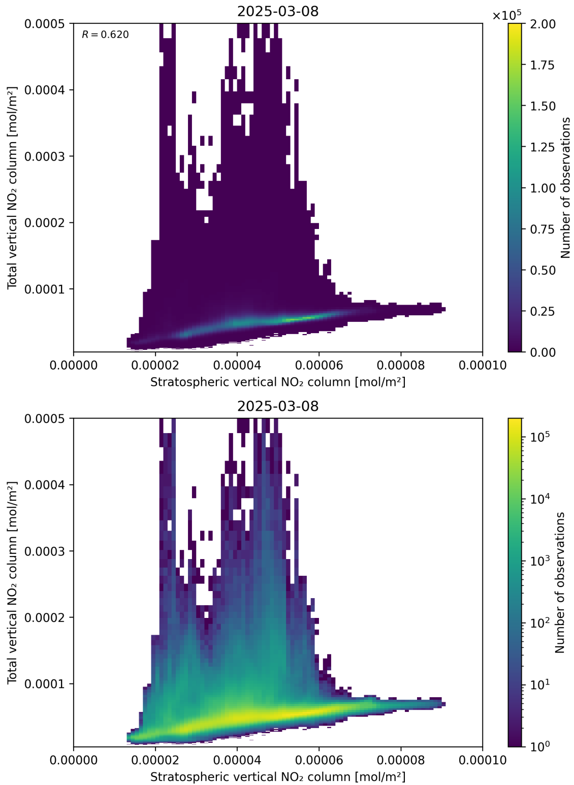
Figure 100: Scatter density plot of “Stratospheric vertical NO 2 column” against “Total vertical NO 2 column” for 2025-03-08 to 2025-03-09.
