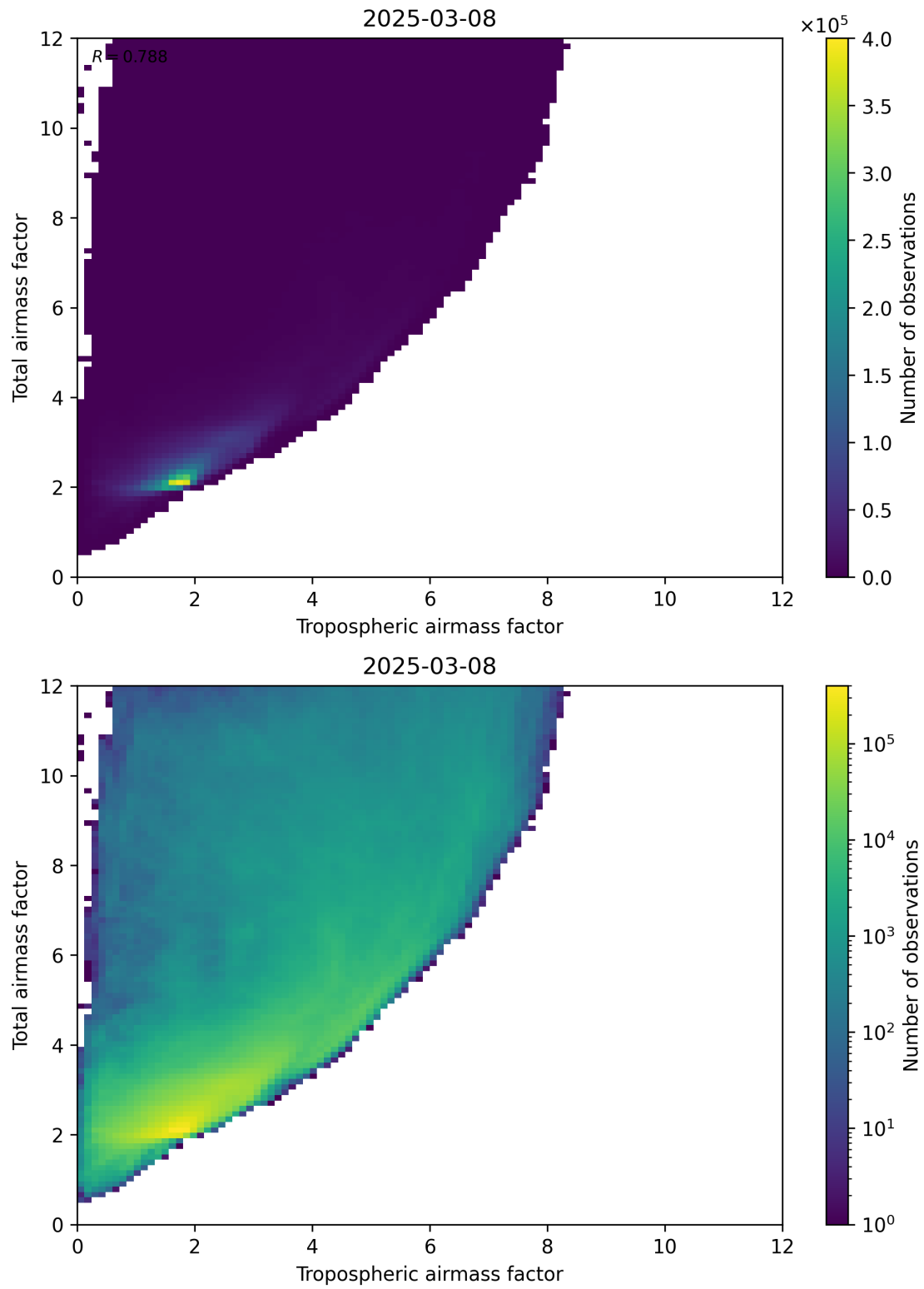
Figure 72: Scatter density plot of “Tropospheric airmass factor” against “Total airmass factor” for 2025-03-08 to 2025-03-09.
