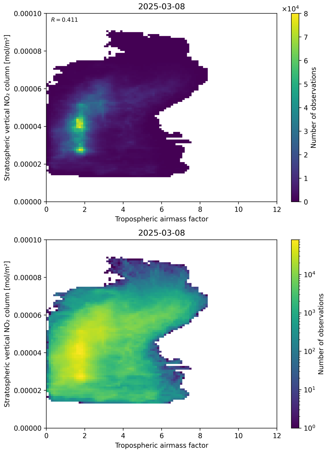
Figure 74: Scatter density plot of “Tropospheric airmass factor” against “Stratospheric vertical NO 2 column” for 2025-03-08 to 2025-03-09.
