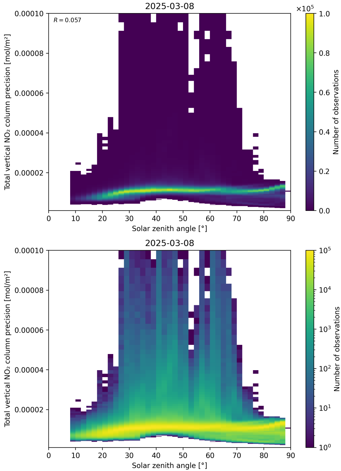
Figure 154: Scatter density plot of “Solar zenith angle” against “Total vertical NO 2 column precision” for 2025-03-08 to 2025-03-09.
