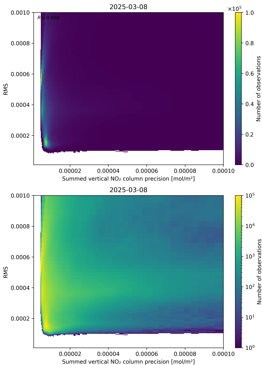
Figure 108: Scatter density plot of “Summed vertical NO 2 column precision” against “RMS” for 2025-03-08 to 2025-03-09.
