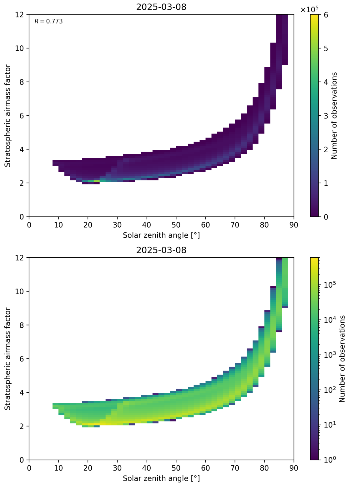
Figure 145: Scatter density plot of “Solar zenith angle” against “Stratospheric airmass factor” for 2025-03-08 to 2025-03-09.
