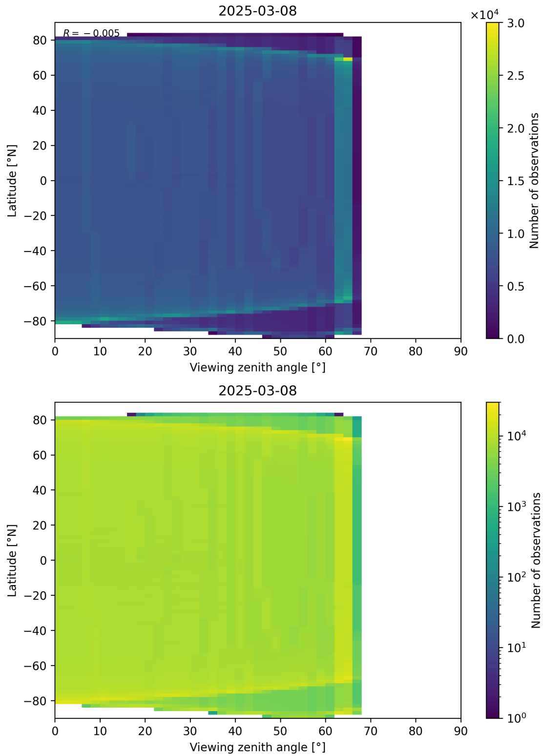
Figure 163: Scatter density plot of “Viewing zenith angle” against “Latitude” for 2025-03-08 to 2025-03-09.
