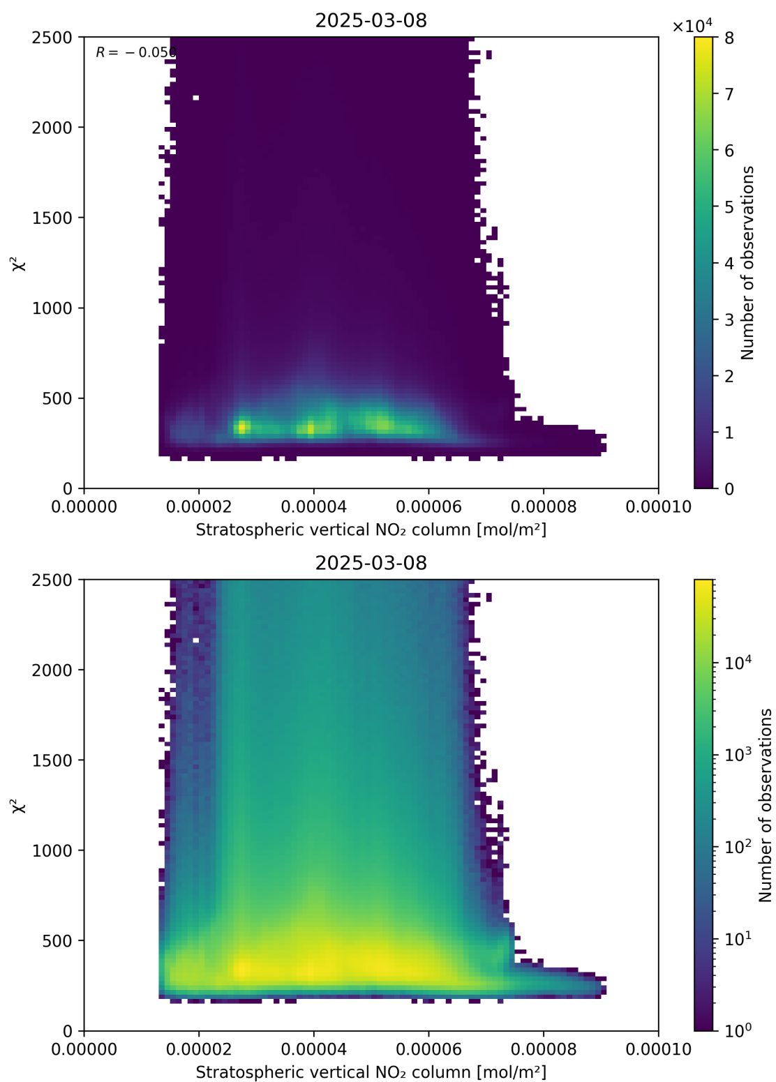
Figure 97: Scatter density plot of “Stratospheric vertical NO 2 column” against “ \chi^2 ” for 2025-03-08 to 2025-03-09.
