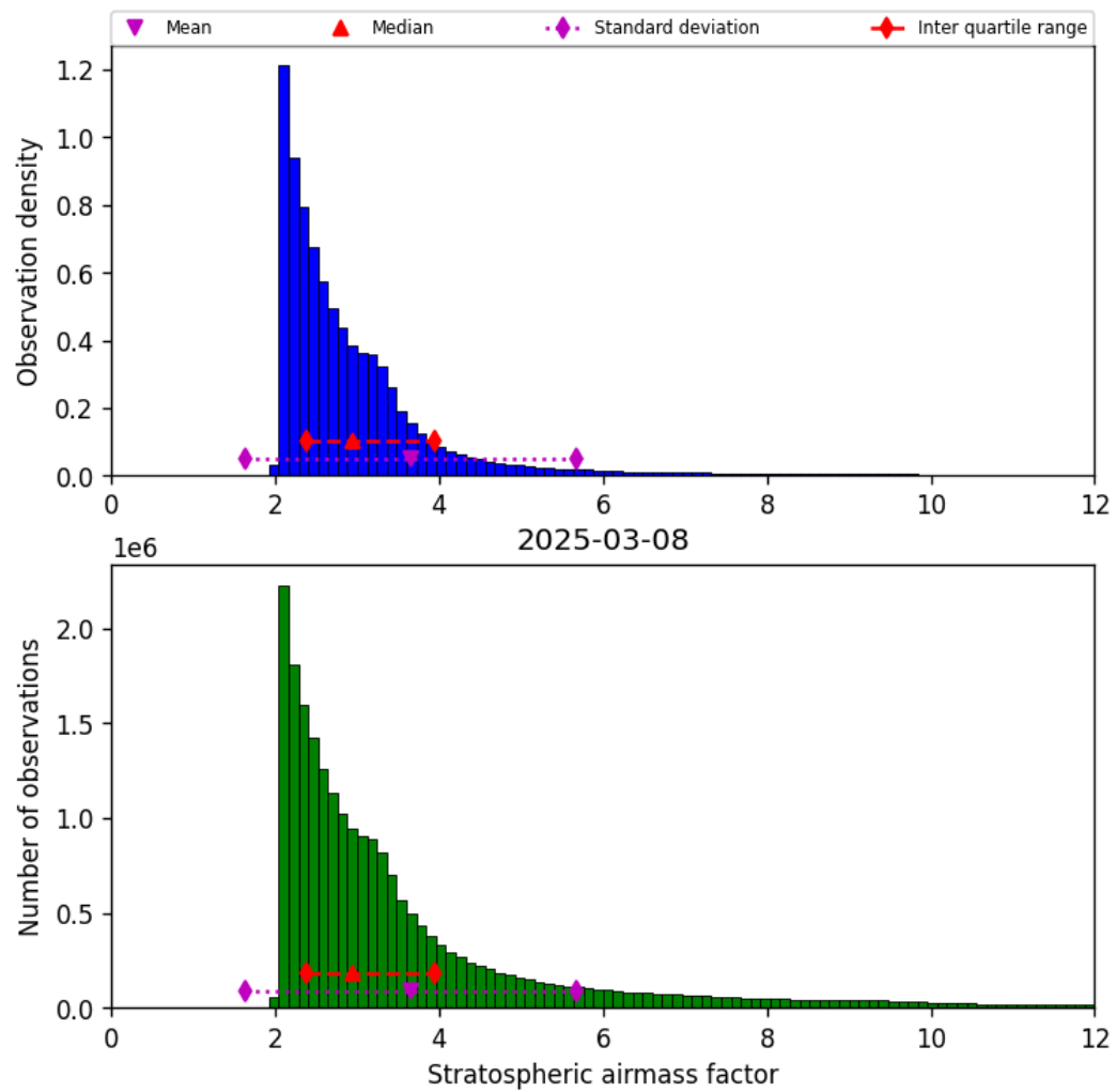
Figure 44: Histogram of “Stratospheric airmass factor” for 2025-03-08 to 2025-03-09
