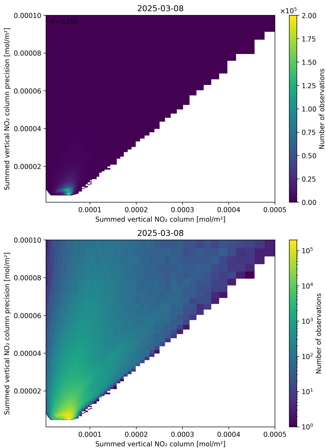
Figure 105: Scatter density plot of “Summed vertical NO 2 column” against “Summed vertical NO 2 column precision” for 2025-03-08 to 2025-03-09.
