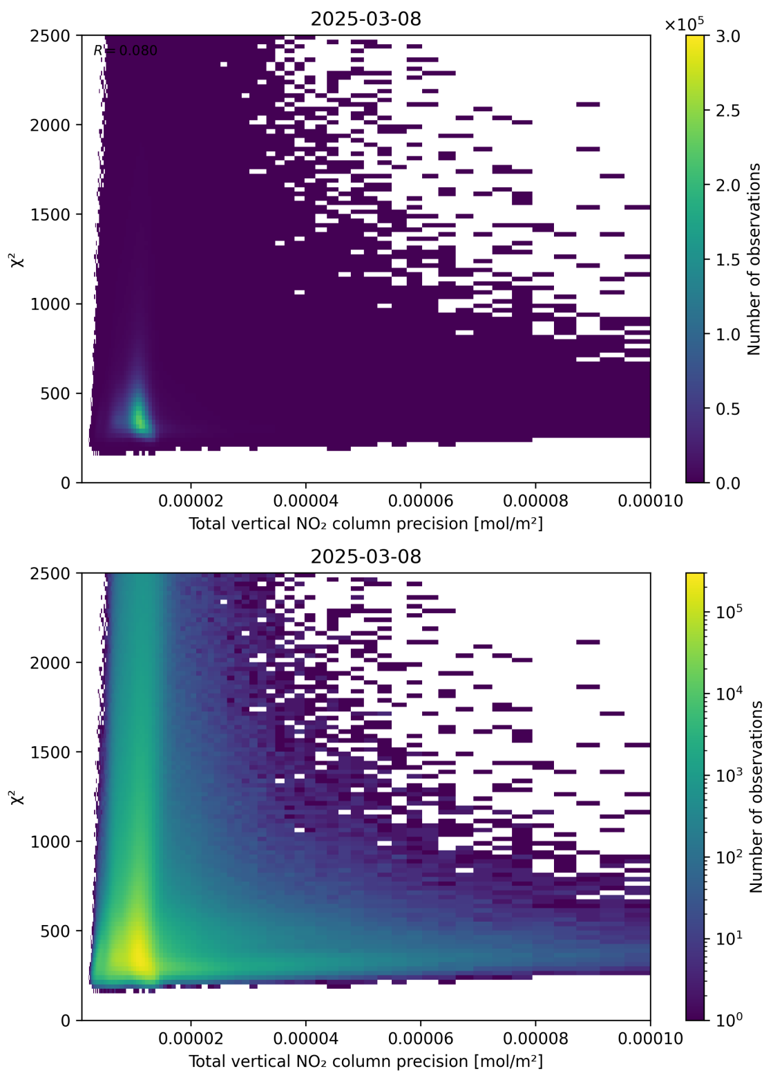
Figure 116: Scatter density plot of “Total vertical NO 2 column precision” against “ \chi^2 ” for 2025-03-08 to 2025-03-09.
