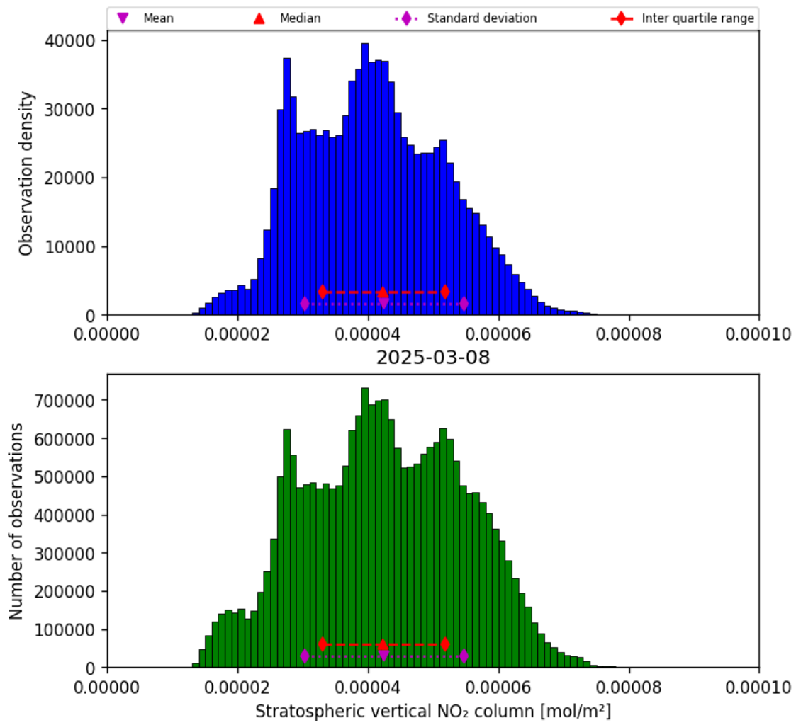
Figure 36: Histogram of “Stratospheric vertical NO 2 column” for 2025-03-08 to 2025-03-09
