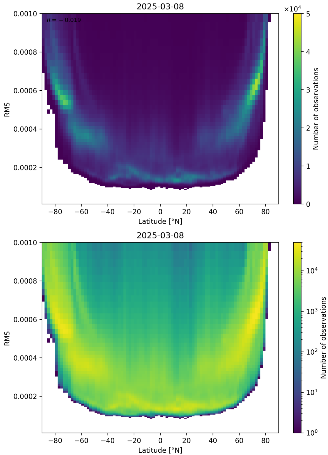
Figure 94: Scatter density plot of “Latitude” against “RMS” for 2025-03-08 to 2025-03-09.
