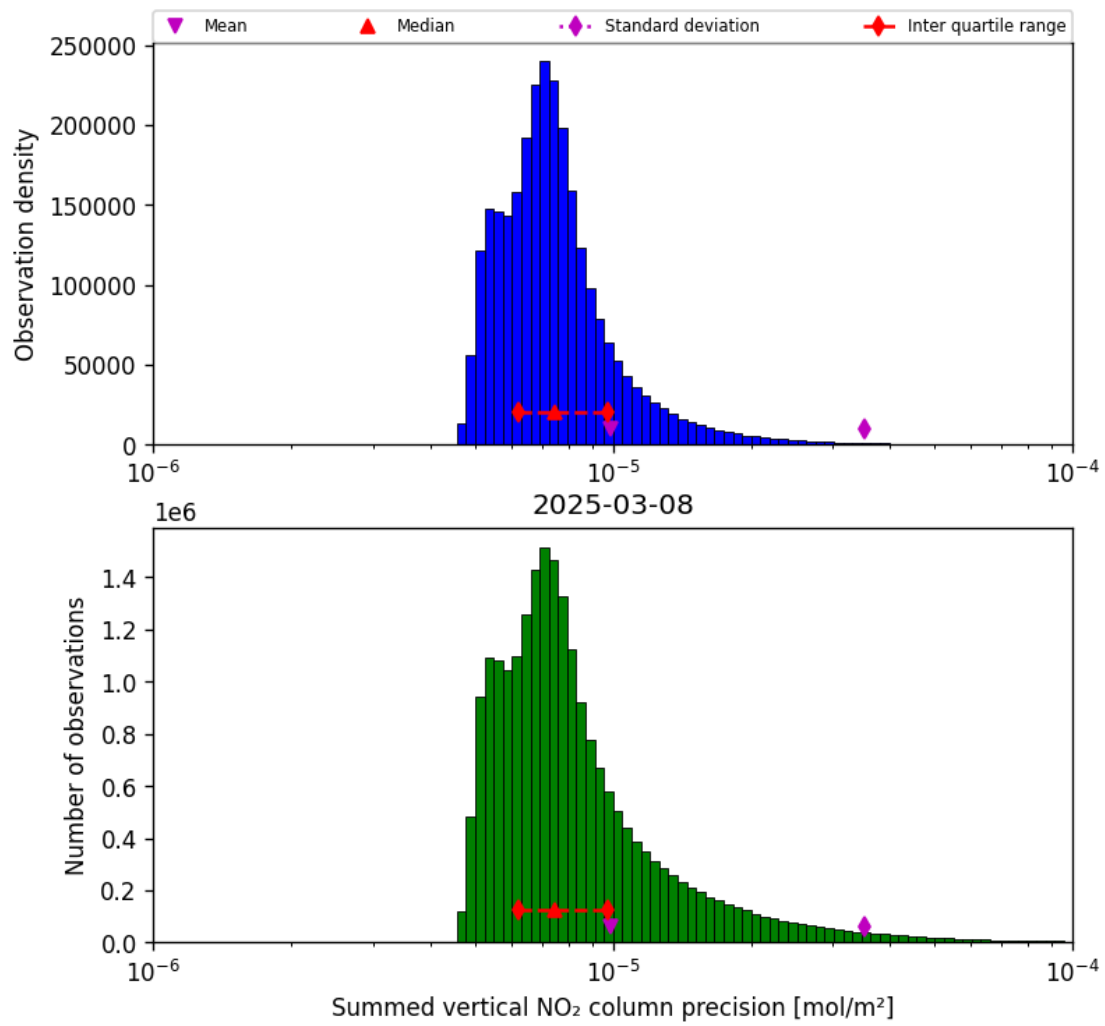
Figure 41: Histogram of "Summed vertical NO 2 column precision" for 2025-03-08 to 2025-03-09
