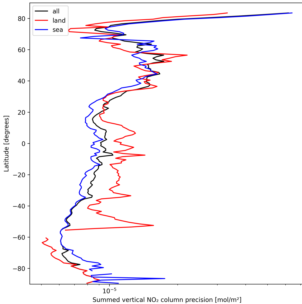
Figure 24: Zonal average of “Summed vertical NO 2 column precision” for 2025-03-08 to 2025-03-09.
