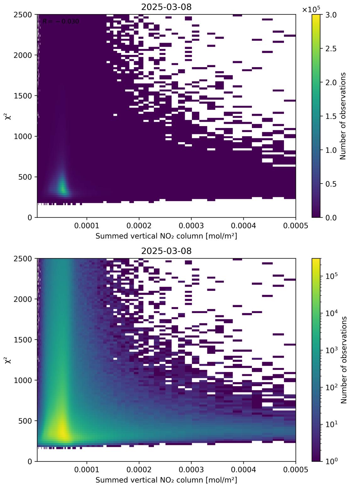
Figure 104: Scatter density plot of “Summed vertical NO 2 column” against “ \chi^2 ” for 2025-03-08 to 2025-03-09.
