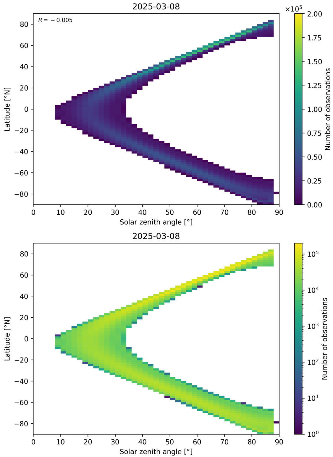
Figure 149: Scatter density plot of “Solar zenith angle” against “Latitude” for 2025-03-08 to 2025-03-09.
