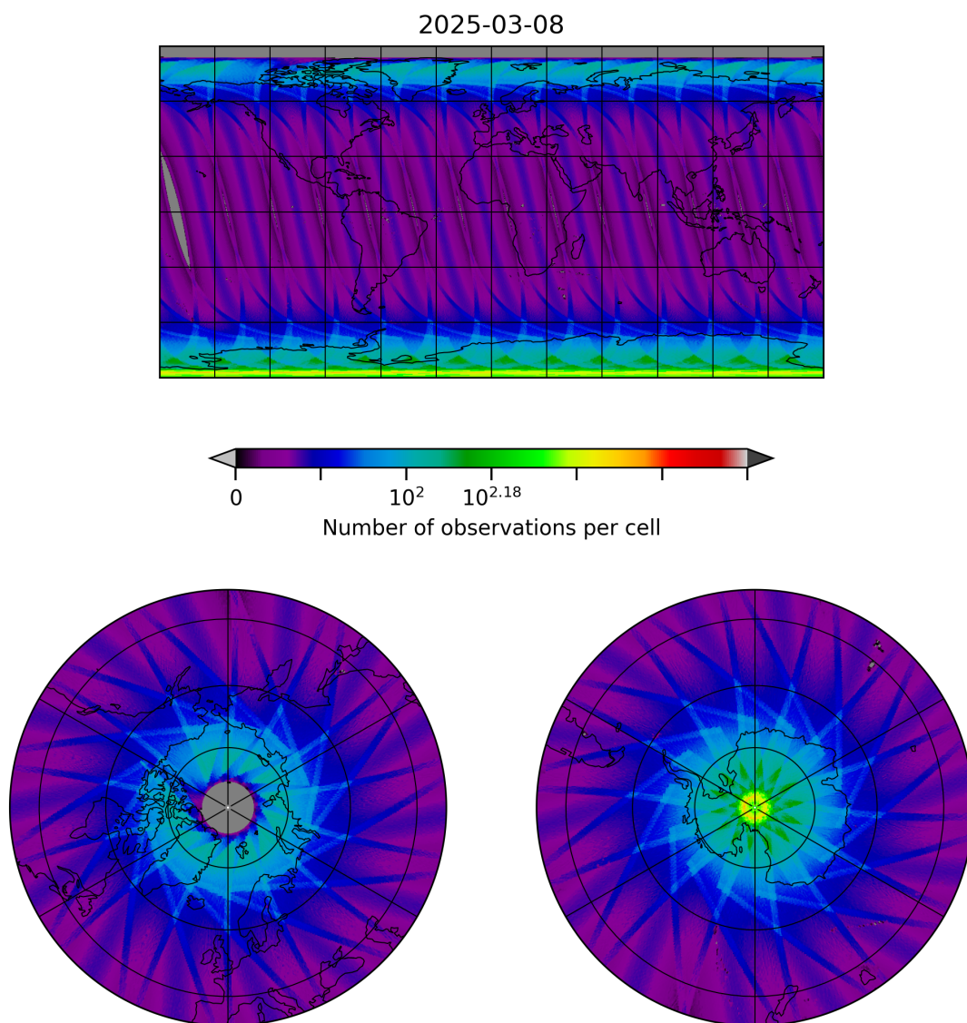
Figure 10: Map of the number of observations for 2025-03-08 to 2025-03-09
