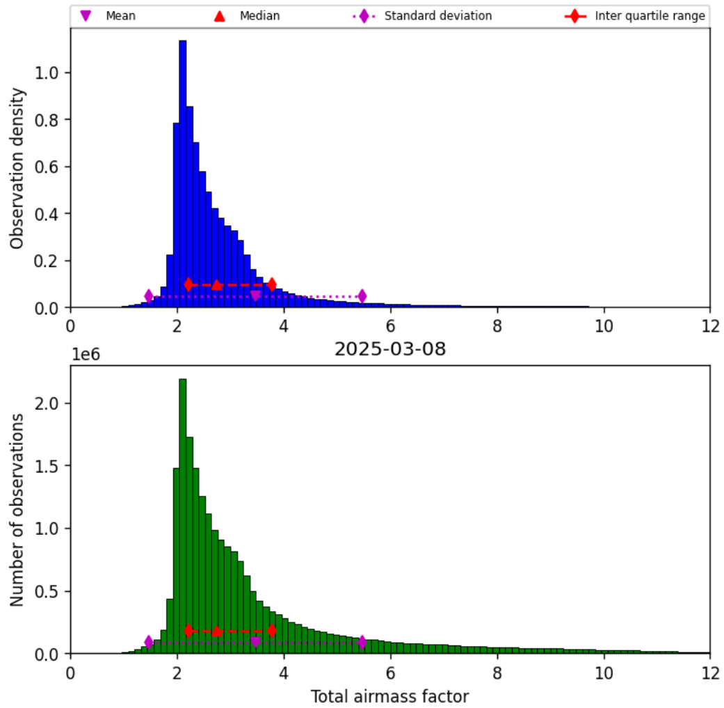
Figure 32: Histogram of “Total airmass factor” for 2025-03-08 to 2025-03-09
