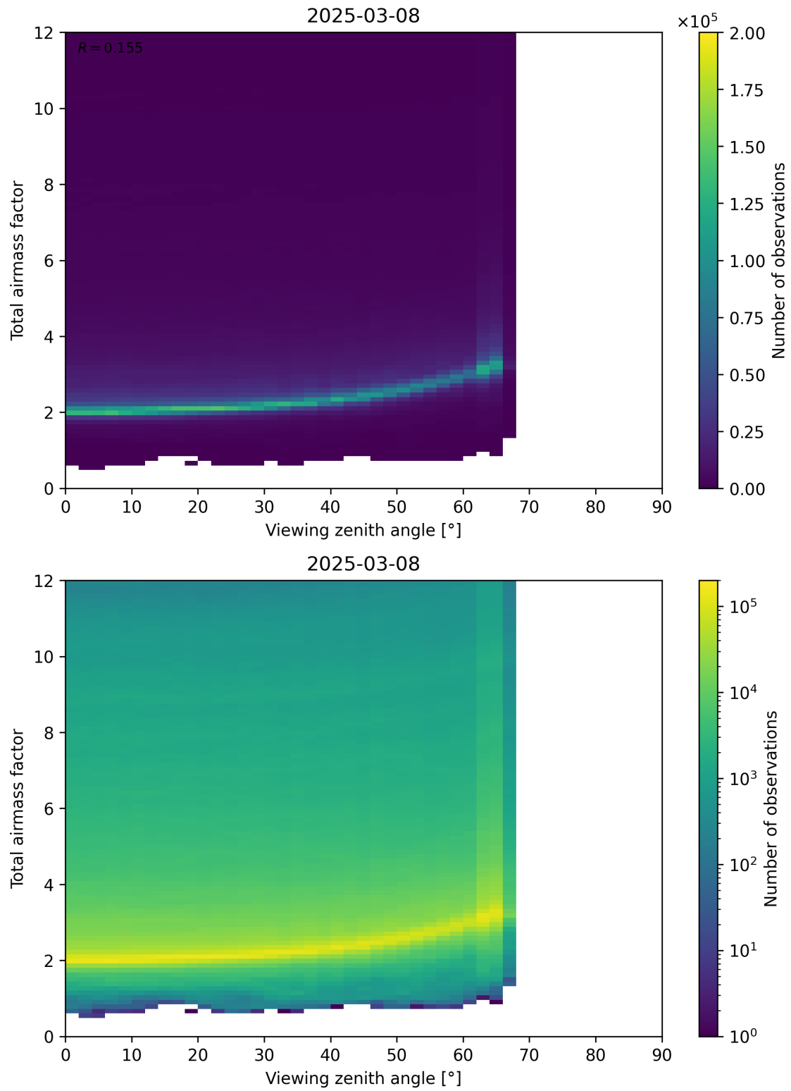
Figure 160: Scatter density plot of “Viewing zenith angle” against “Total airmass factor” for 2025-03-08 to 2025-03-09.
