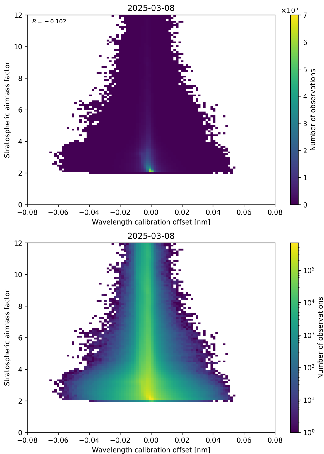
Figure 174: Scatter density plot of “Wavelength calibration offset” against “Stratospheric airmass factor” for 2025-03-08 to 2025-03-09.
