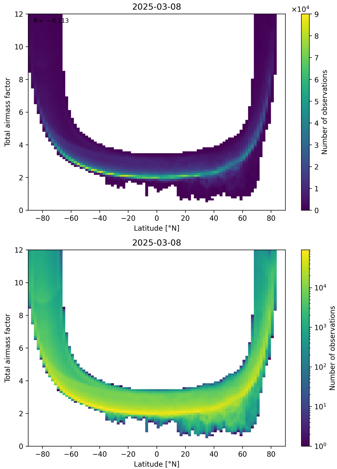
Figure 84: Scatter density plot of “Latitude” against “Total airmass factor” for 2025-03-08 to 2025-03-09.
