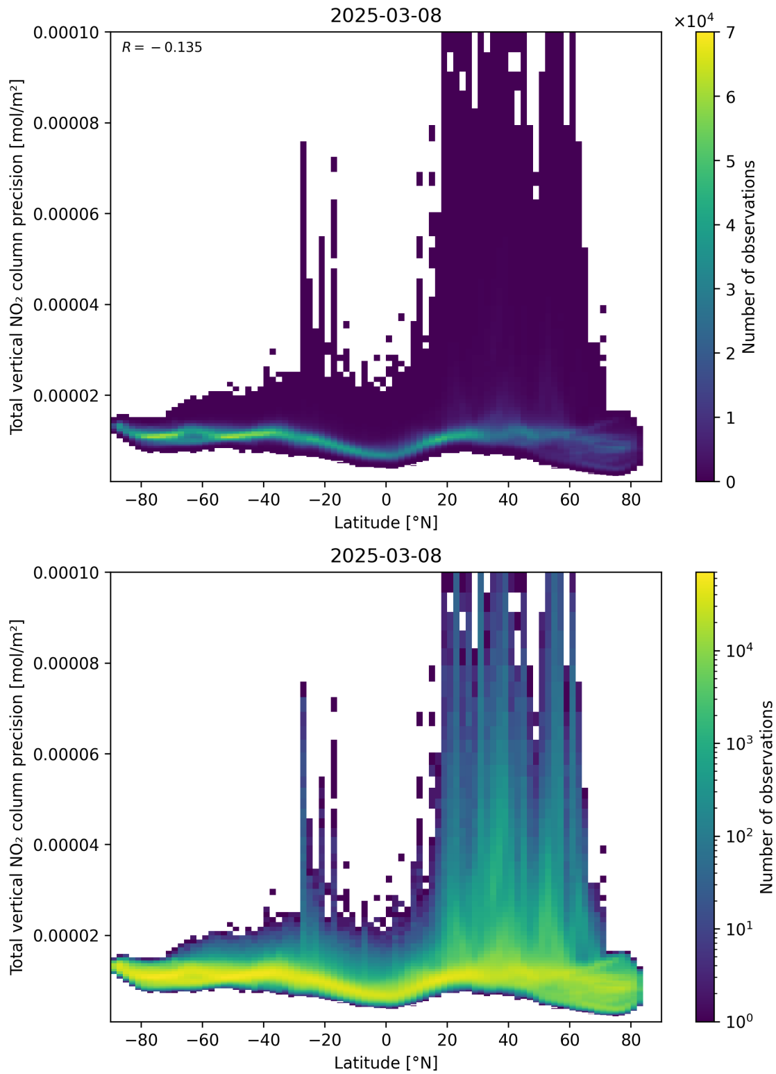
Figure 91: Scatter density plot of “Latitude” against “Total vertical NO 2 column precision” for 2025-03-08 to 2025-03-09.
