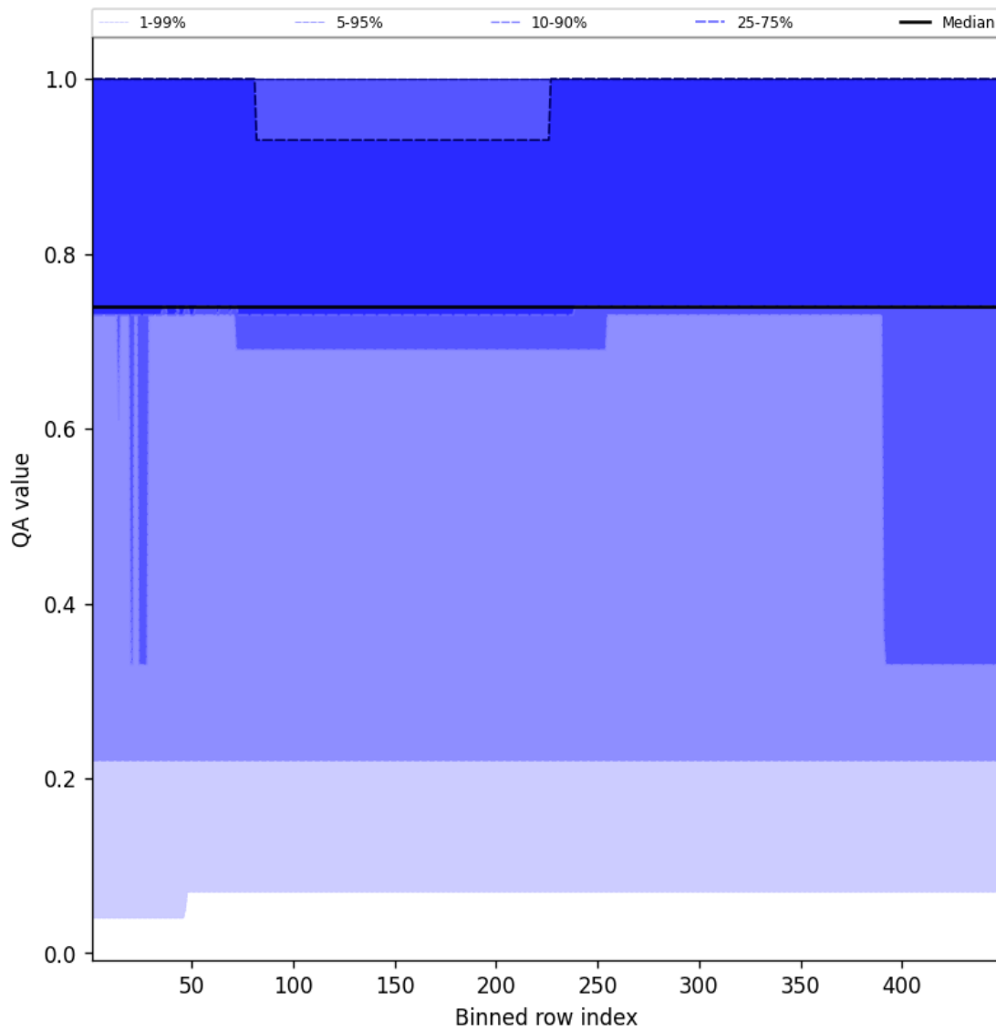
Figure 45: Along track statistics of "QA value" for 2025-03-08 to 2025-03-09
