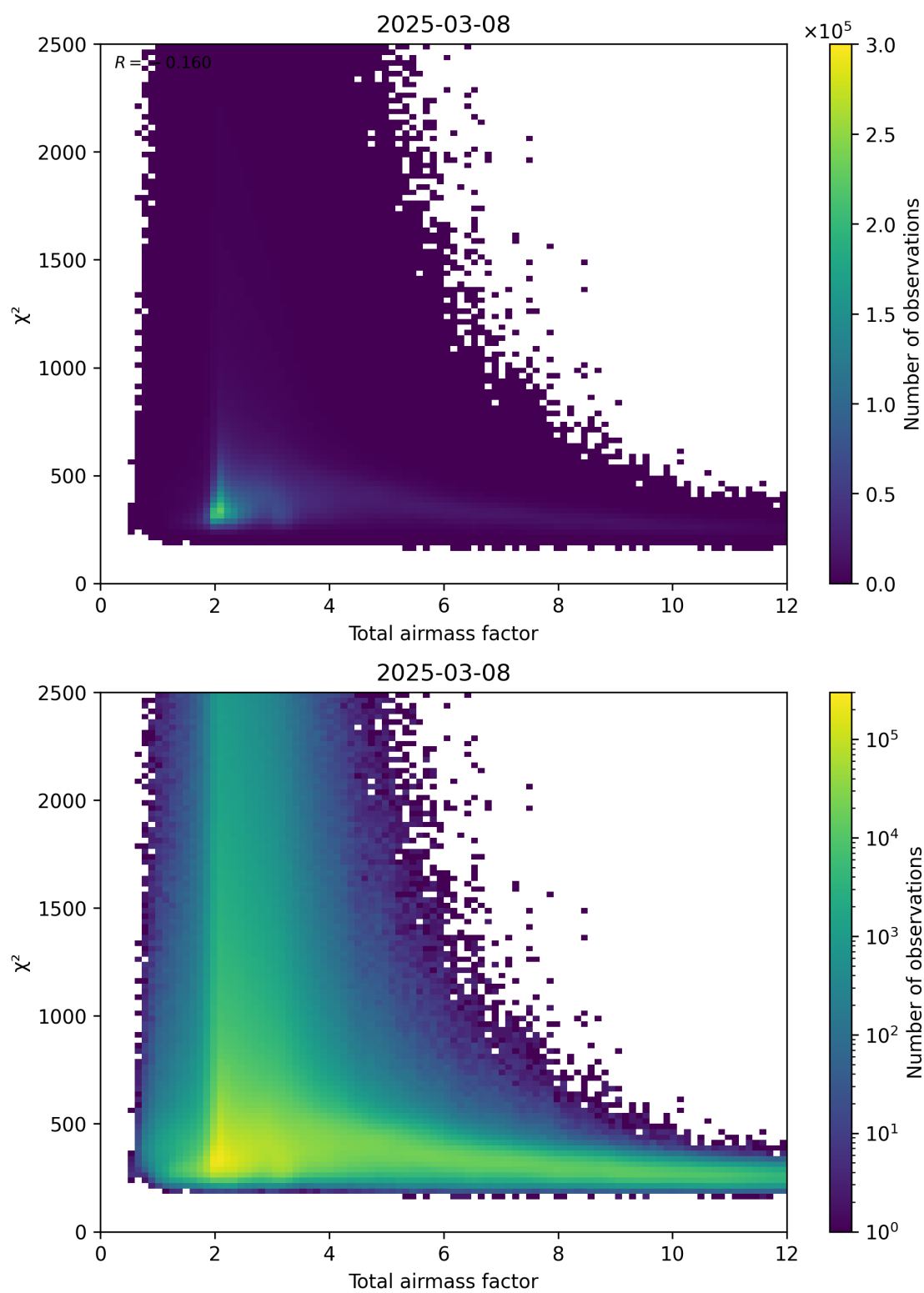
Figure 63: Scatter density plot of “Total airmass factor” against “ \chi^2 ” for 2025-03-08 to 2025-03-09.
