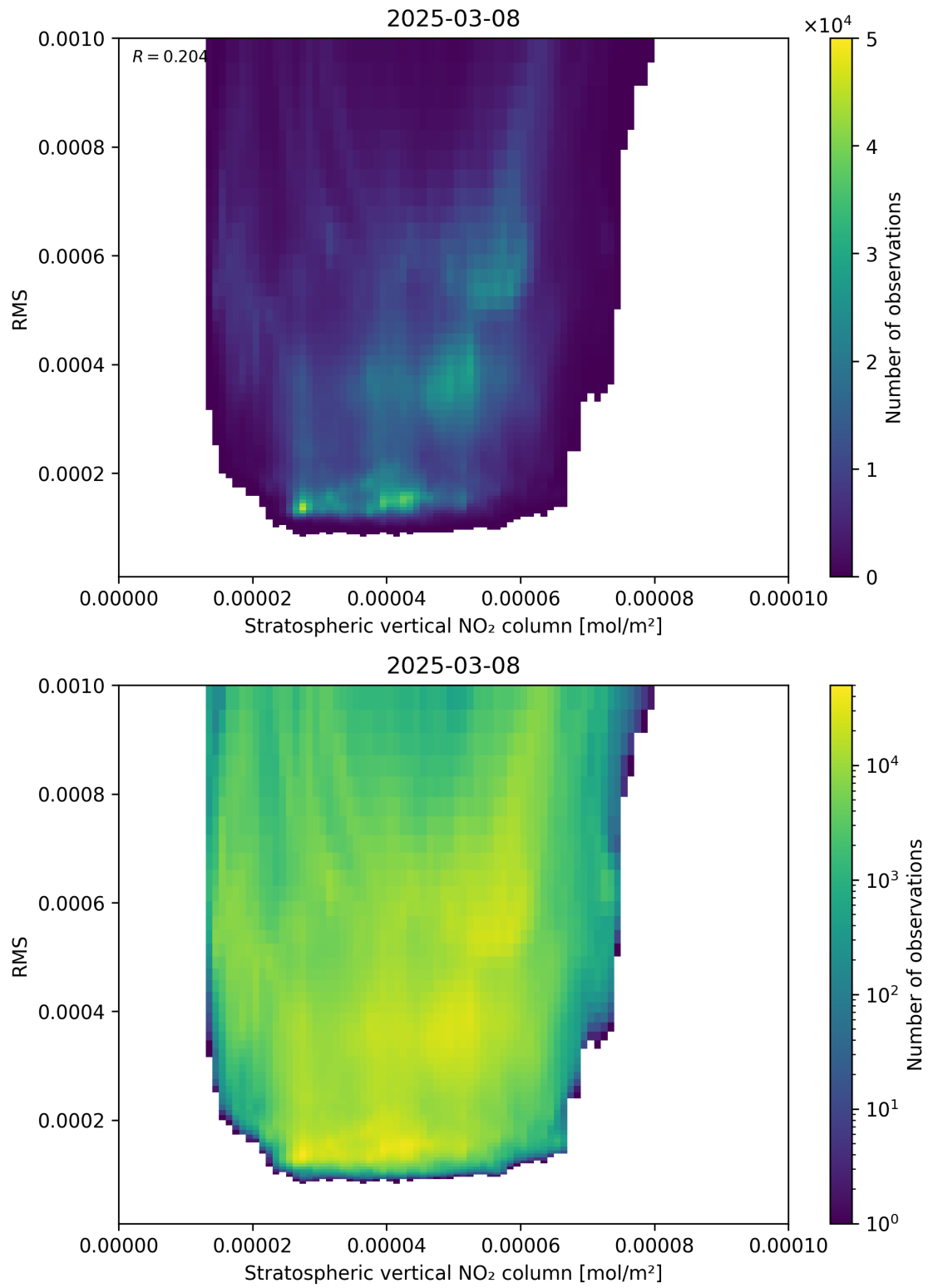
Figure 102: Scatter density plot of “Stratospheric vertical NO 2 column” against “RMS” for 2025-03-08 to 2025-03-09.
