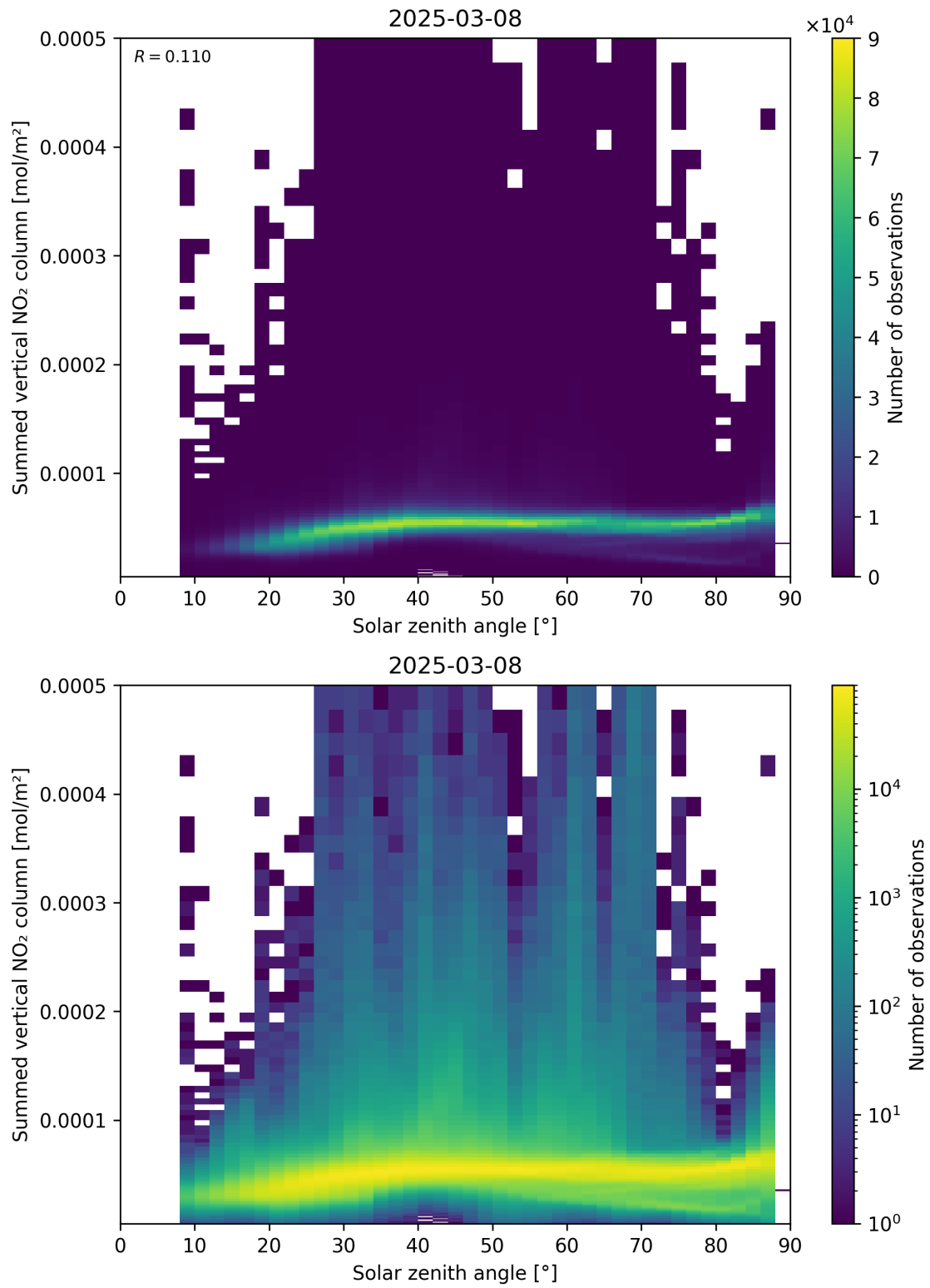
Figure 151: Scatter density plot of “Solar zenith angle” against “Summed vertical NO 2 column” for 2025-03-08 to 2025-03-09.
