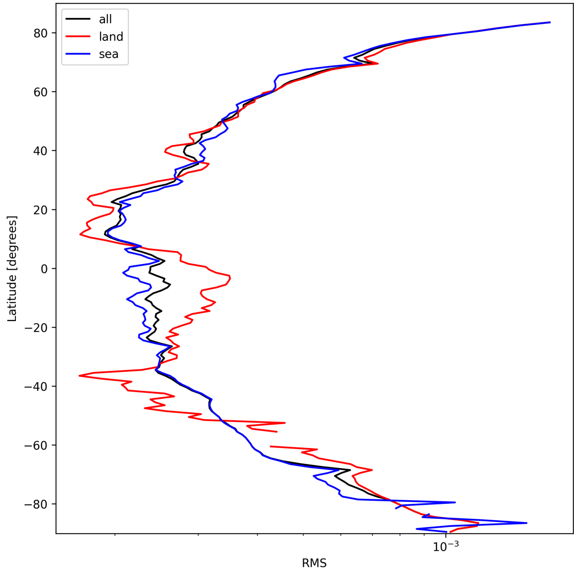
Figure 26: Zonal average of “RMS” for 2025-03-08 to 2025-03-09.
