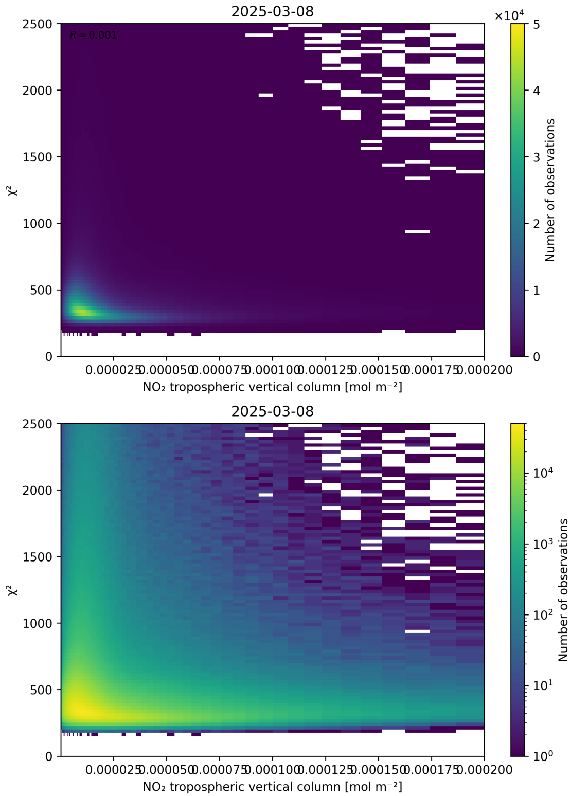
Figure 124: Scatter density plot of “NO 2 tropospheric vertical column” against “ \chi^2 ” for 2025-03-08 to 2025-03-09.
