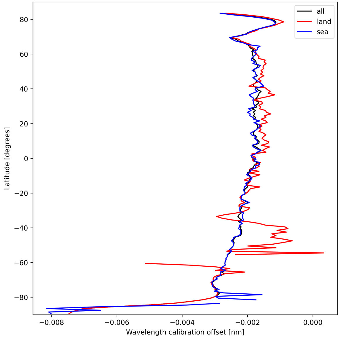
Figure 18: Zonal average of “Wavelength calibration offset” for 2025-03-08 to 2025-03-09.
