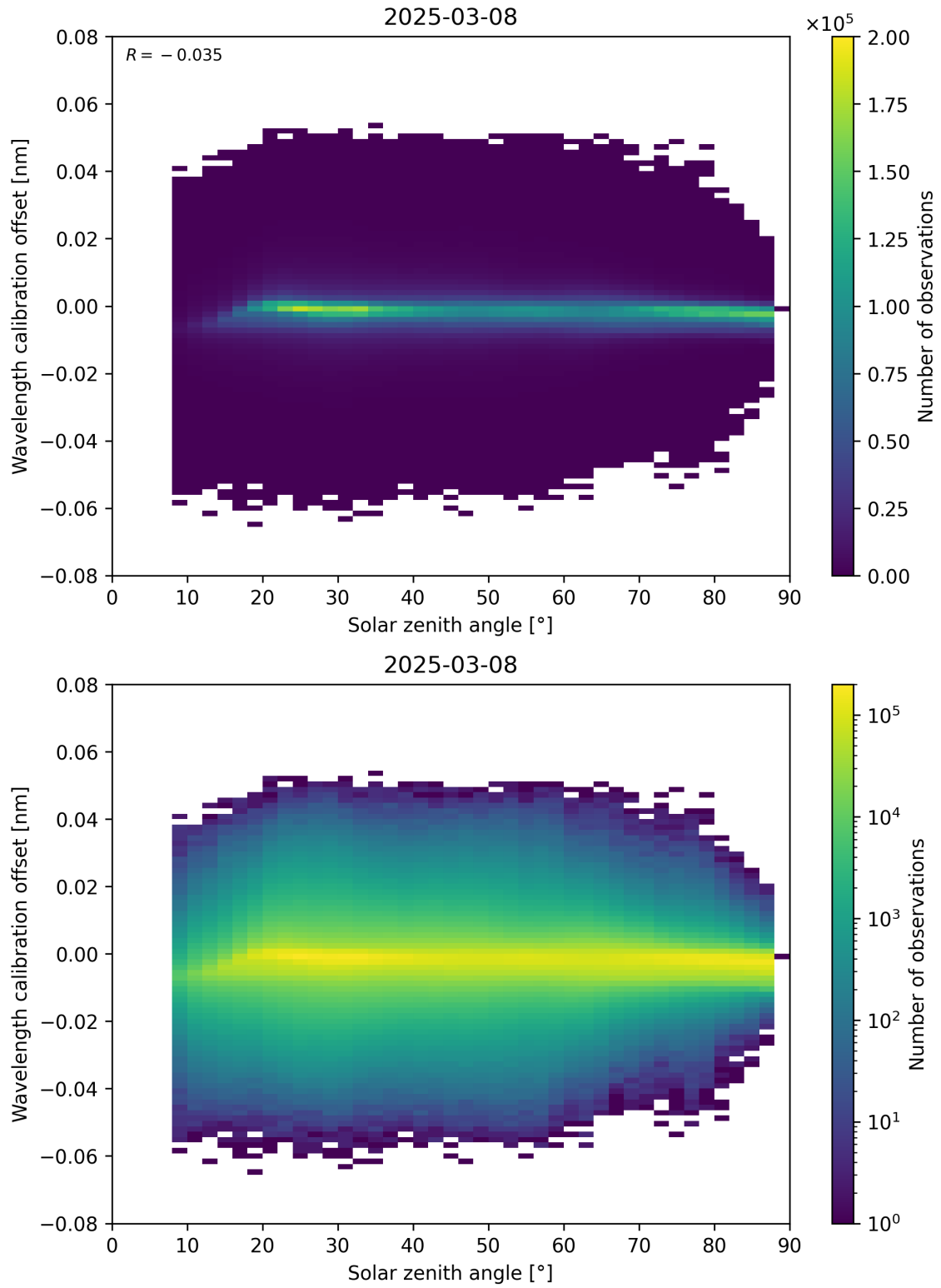
Figure 158: Scatter density plot of “Solar zenith angle” against “Wavelength calibration offset” for 2025-03-08 to 2025-03-09.
