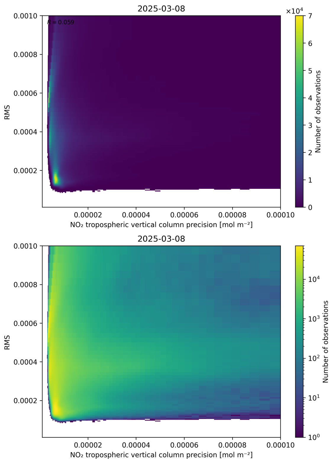
Figure 140: Scatter density plot of “NO 2 tropospheric vertical column precision” against “RMS” for 2025-03-08 to 2025-03-09.
