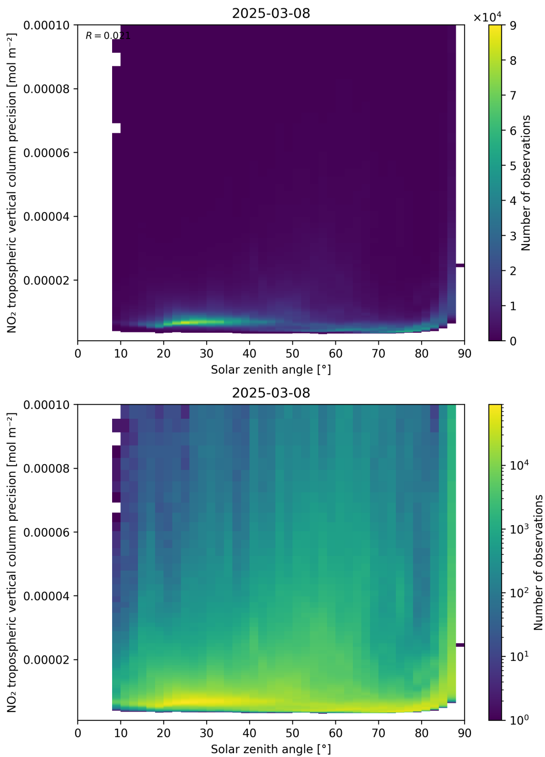
Figure 156: Scatter density plot of “Solar zenith angle” against “NO 2 tropospheric vertical column precision” for 2025-03-08 to 2025-03-09.
