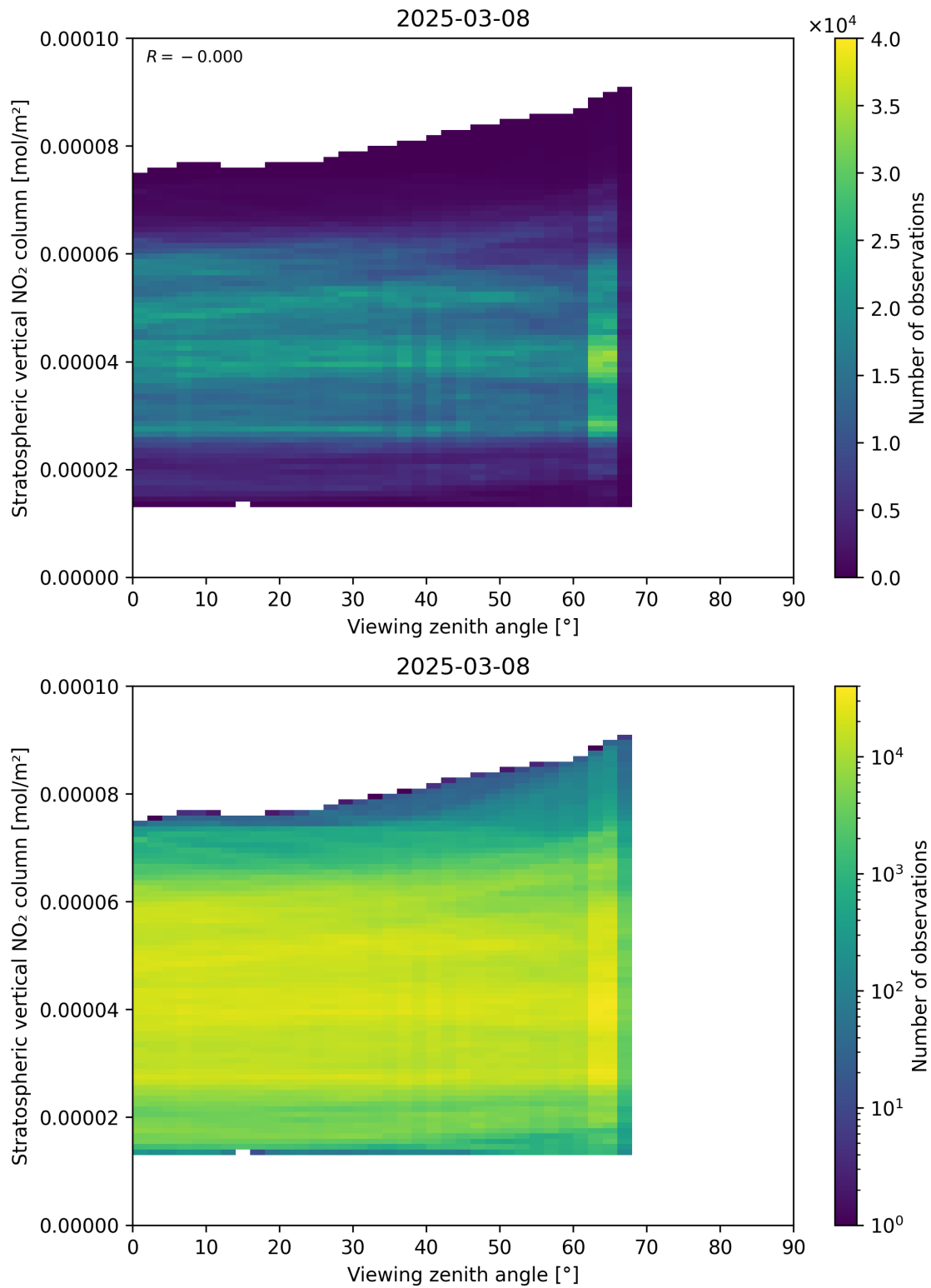
Figure 164: Scatter density plot of “Viewing zenith angle” against “Stratospheric vertical NO 2 column” for 2025-03-08 to 2025-03-09.
