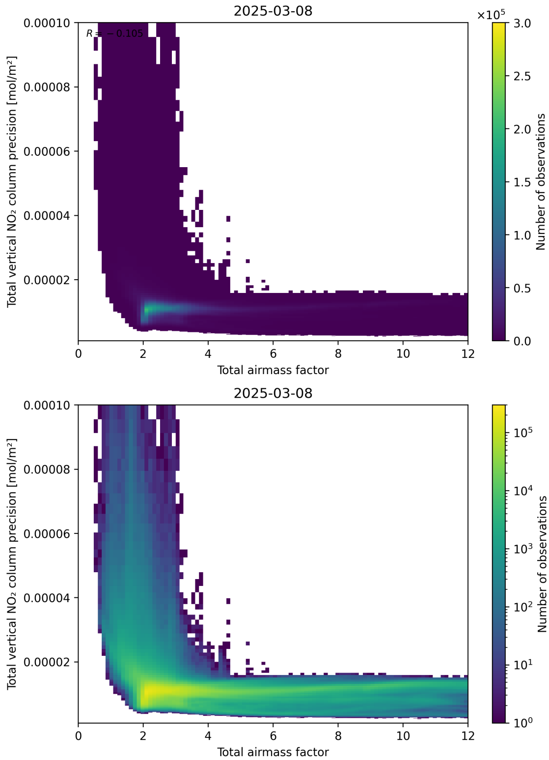
Figure 68: Scatter density plot of “Total airmass factor” against “Total vertical NO 2 column precision” for 2025-03-08 to 2025-03-09.
