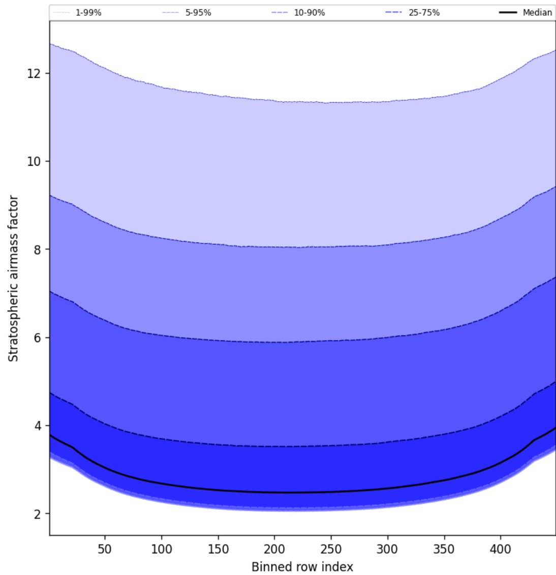
Figure 61: Along track statistics of “Stratospheric airmass factor” for 2025-03-08 to 2025-03-09
