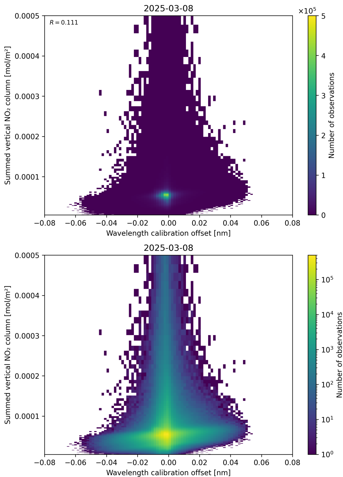
Figure 177: Scatter density plot of “Wavelength calibration offset” against “Summed vertical NO 2 column” for 2025-03-08 to 2025-03-09.
