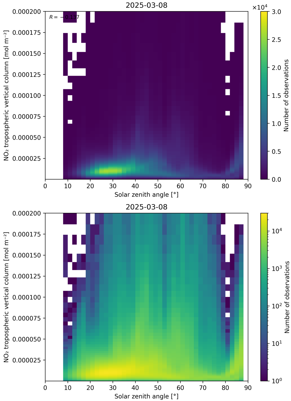
Figure 155: Scatter density plot of “Solar zenith angle” against “NO 2 tropospheric vertical column” for 2025-03-08 to 2025-03-09.
