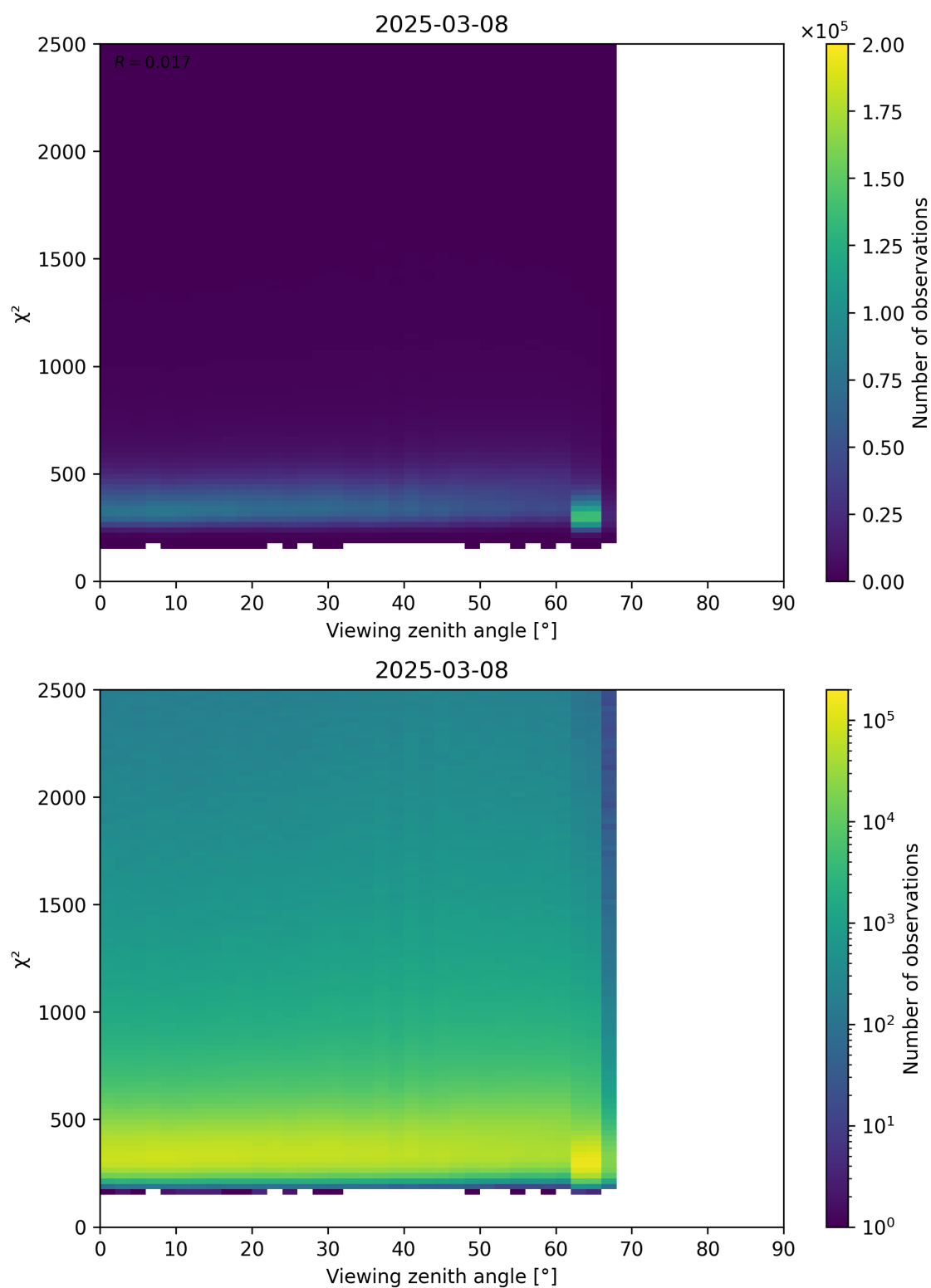
Figure 162: Scatter density plot of “Viewing zenith angle” against “ \chi^2 ” for 2025-03-08 to 2025-03-09.
