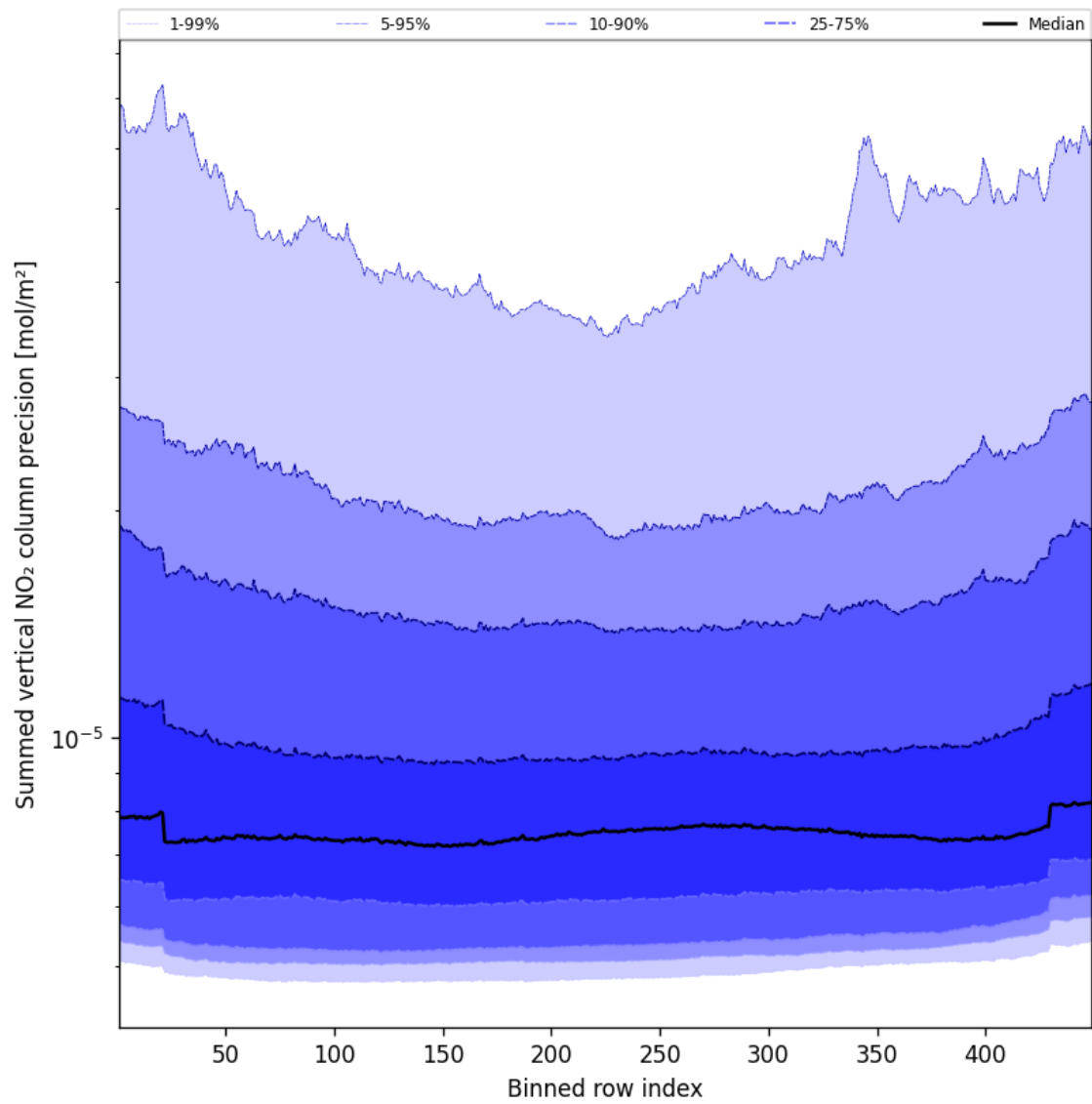
Figure 58: Along track statistics of “Summed vertical NO 2 column precision” for 2025-03-08 to 2025-03-09
