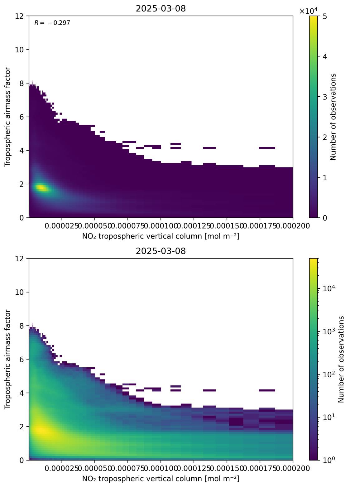
Figure 123: Scatter density plot of “NO 2 tropospheric vertical column” against “Tropospheric air mass factor” for 2025-03-08 to 2025-03-09.
