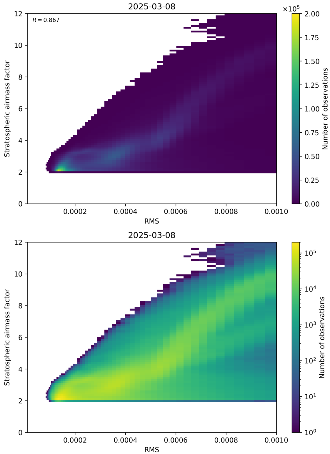
Figure 144: Scatter density plot of “RMS” against “Stratospheric airmass factor” for 2025-03-08 to 2025-03-09.
