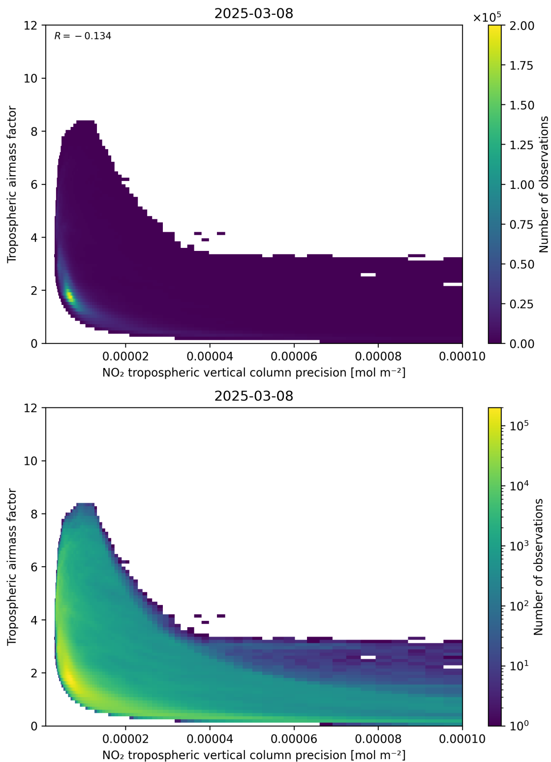
Figure 133: Scatter density plot of “NO 2 tropospheric vertical column precision” against “Tropospheric air mass factor” for 2025-03-08 to 2025-03-09.
