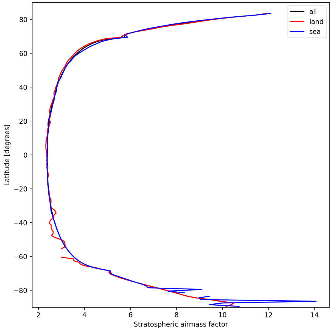
Figure 27: Zonal average of “Stratospheric air mass factor” for 2025-03-08 to 2025-03-09.
