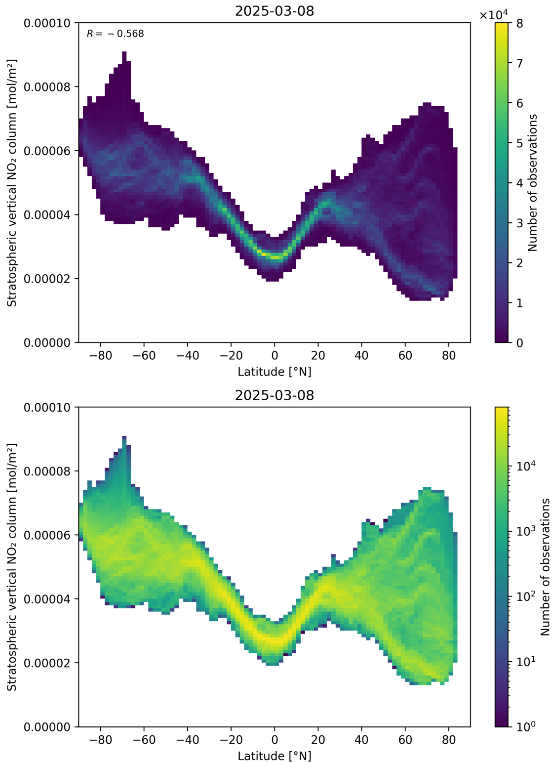
Figure 87: Scatter density plot of “Latitude” against “Stratospheric vertical NO 2 column” for 2025-03-08 to 2025-03-09.
