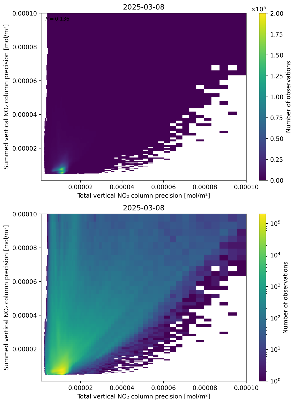
Figure 118: Scatter density plot of “Total vertical NO 2 column precision” against “Summed vertical NO 2 column precision” for 2025-03-08 to 2025-03-09.
