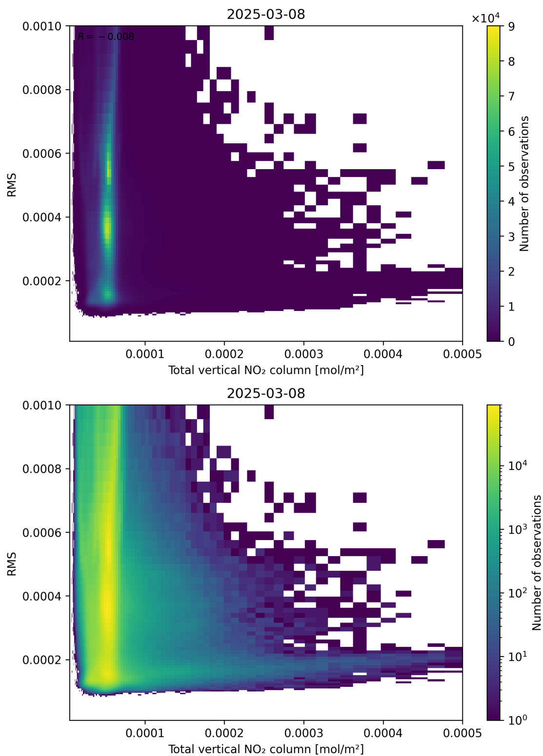
Figure 120: Scatter density plot of “Total vertical NO 2 column” against “RMS” for 2025-03-08 to 2025-03-09.
