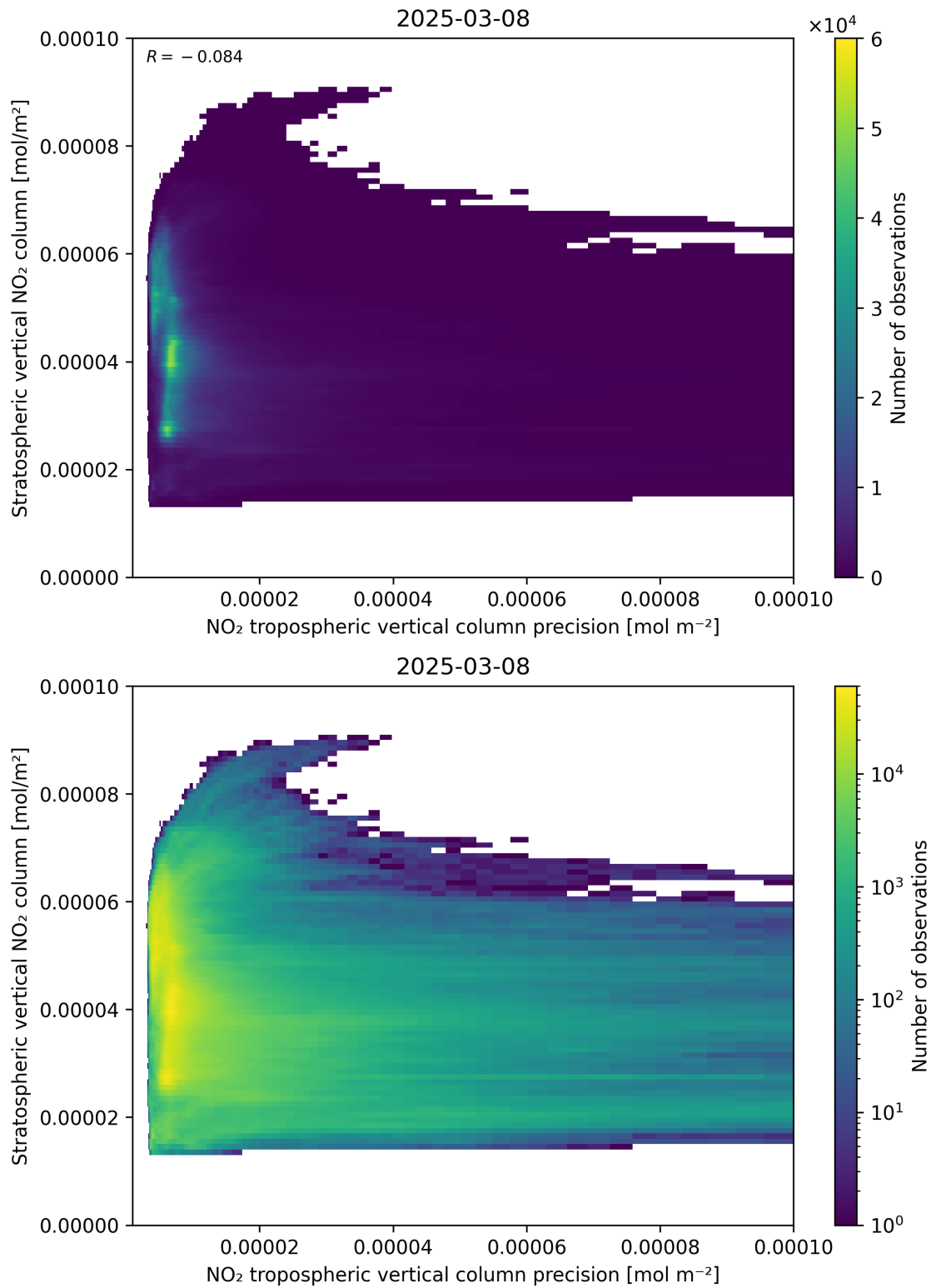
Figure 135: Scatter density plot of “NO 2 tropospheric vertical column precision” against “Stratospheric vertical NO 2 column” for 2025-03-08 to 2025-03-09.
