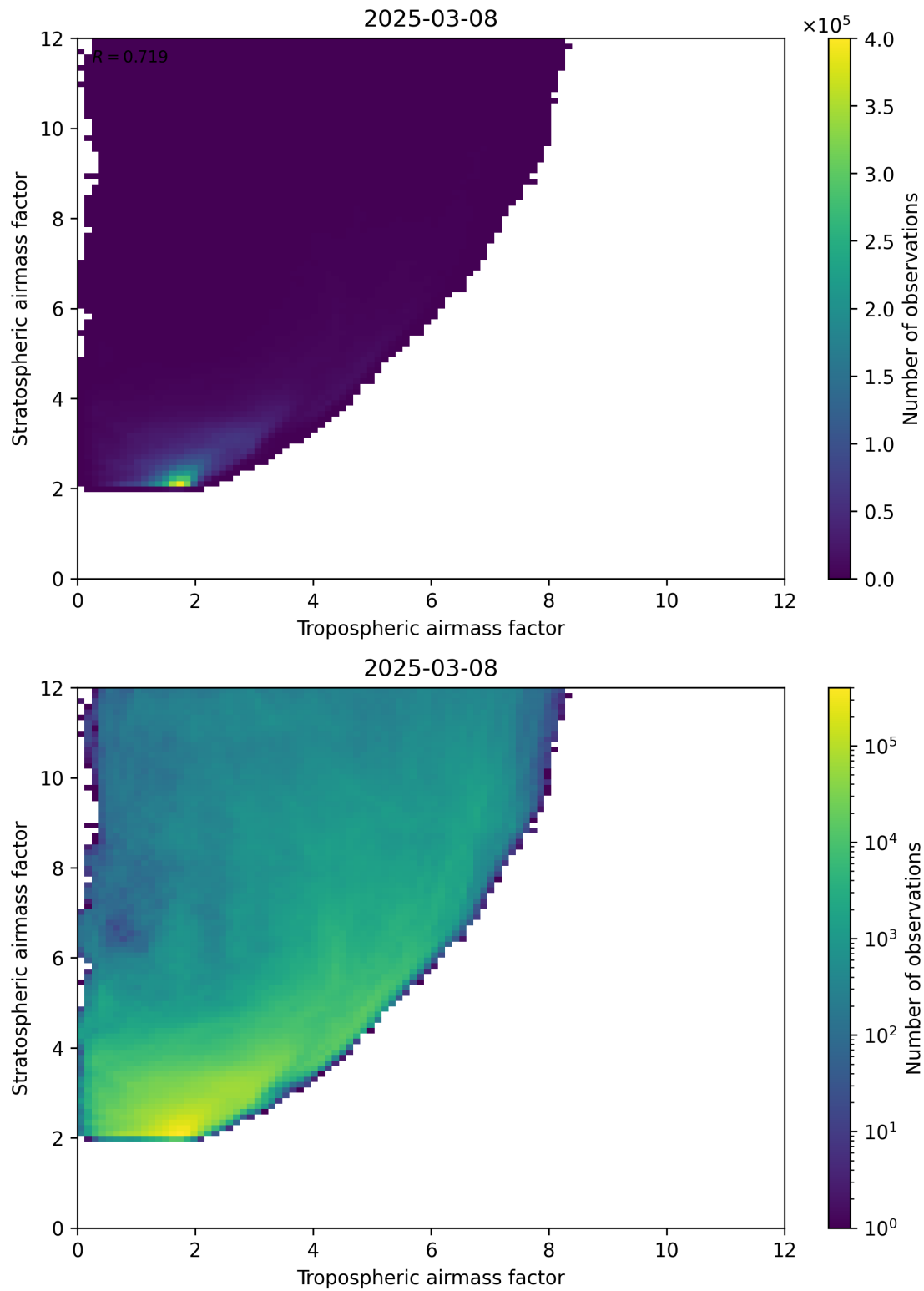
Figure 71: Scatter density plot of “Tropospheric airmass factor” against “Stratospheric airmass factor” for 2025-03-08 to 2025-03-09.
