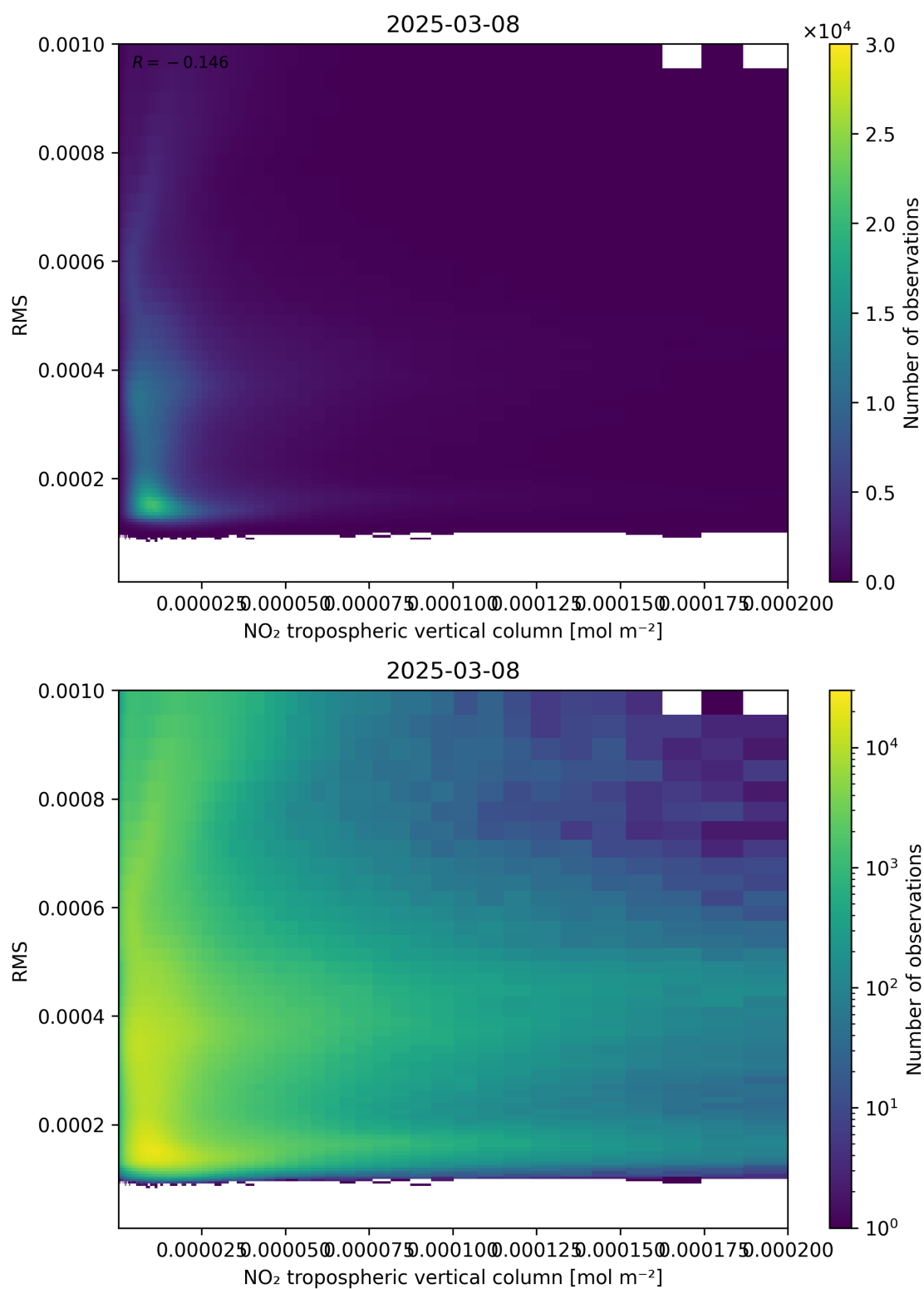
Figure 142: Scatter density plot of “NO 2 tropospheric vertical column” against “RMS” for 2025-03-08 to 2025-03-09.
