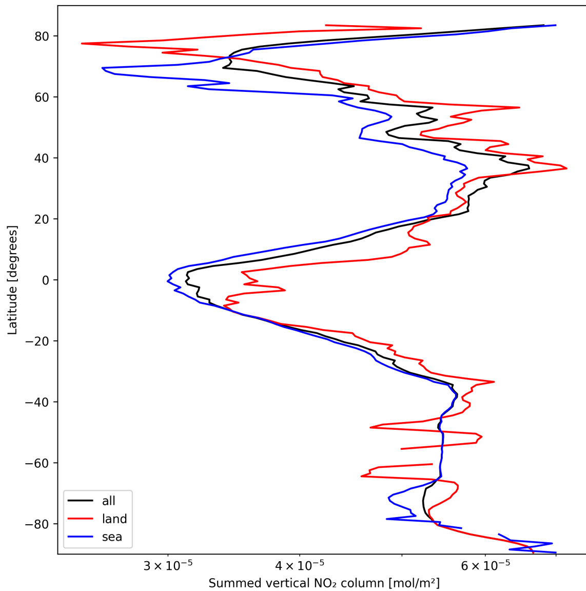
Figure 23: Zonal average of “Summed vertical NO 2 column” for 2025-03-08 to 2025-03-09.
