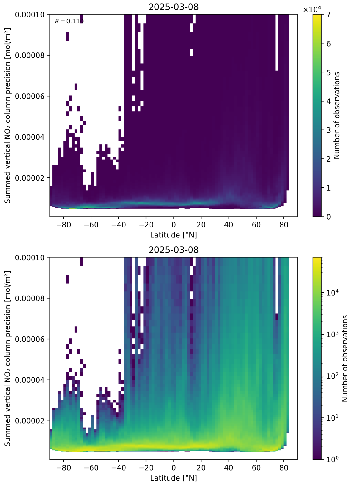
Figure 89: Scatter density plot of “Latitude” against “Summed vertical NO 2 column precision” for 2025-03-08 to 2025-03-09.
