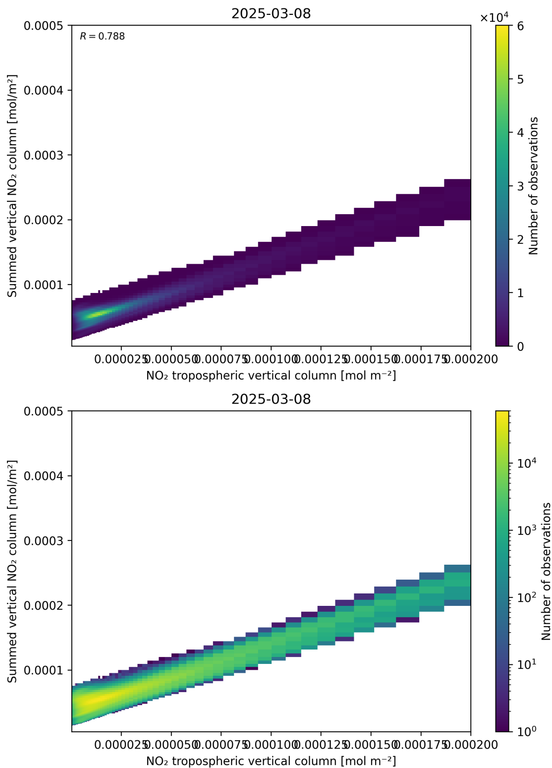
Figure 126: Scatter density plot of “NO 2 tropospheric vertical column” against “Summed vertical NO 2 column” for 2025-03-08 to 2025-03-09.
