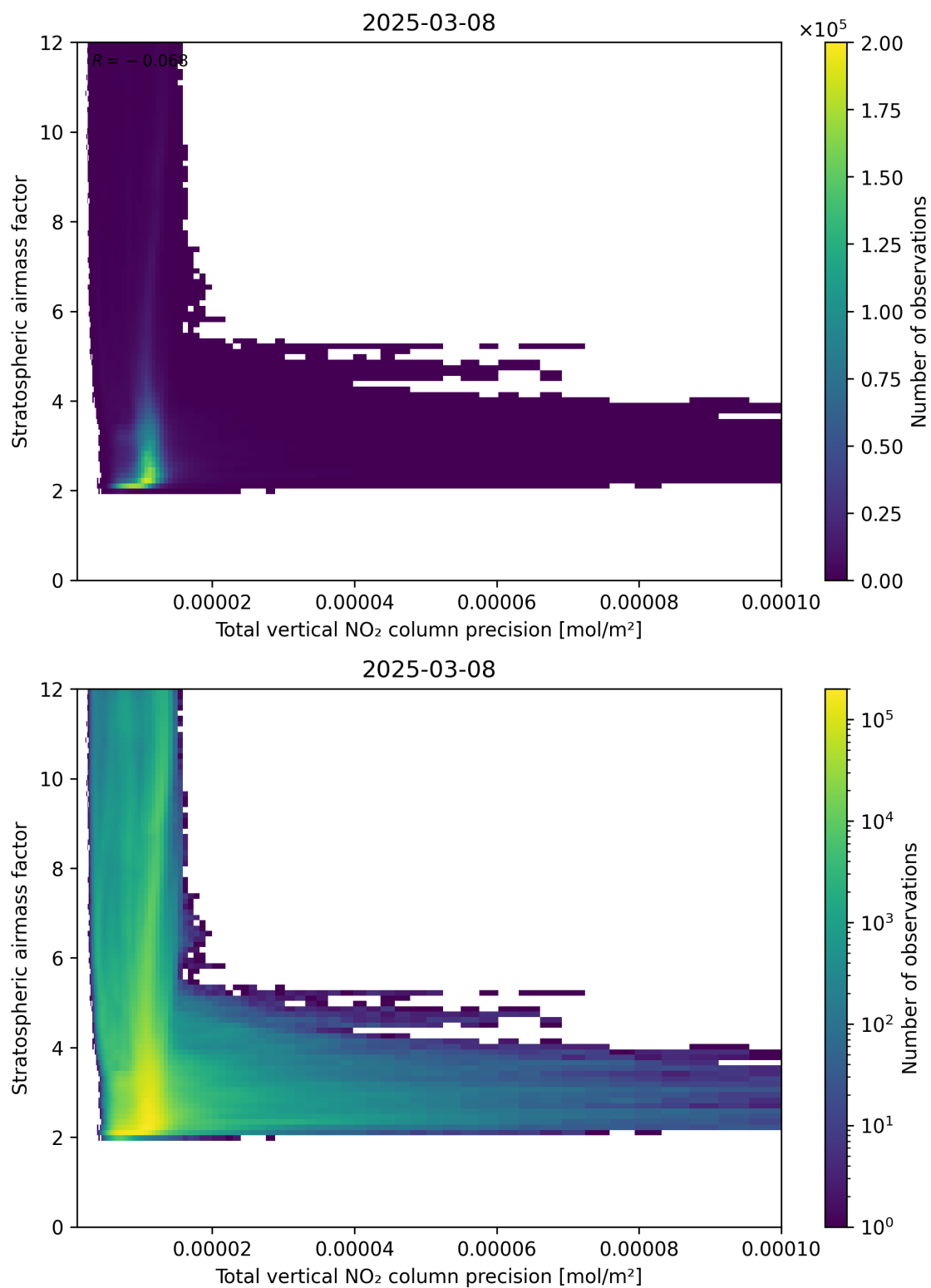
Figure 115: Scatter density plot of “Total vertical NO 2 column precision” against “Stratospheric air mass factor” for 2025-03-08 to 2025-03-09.
