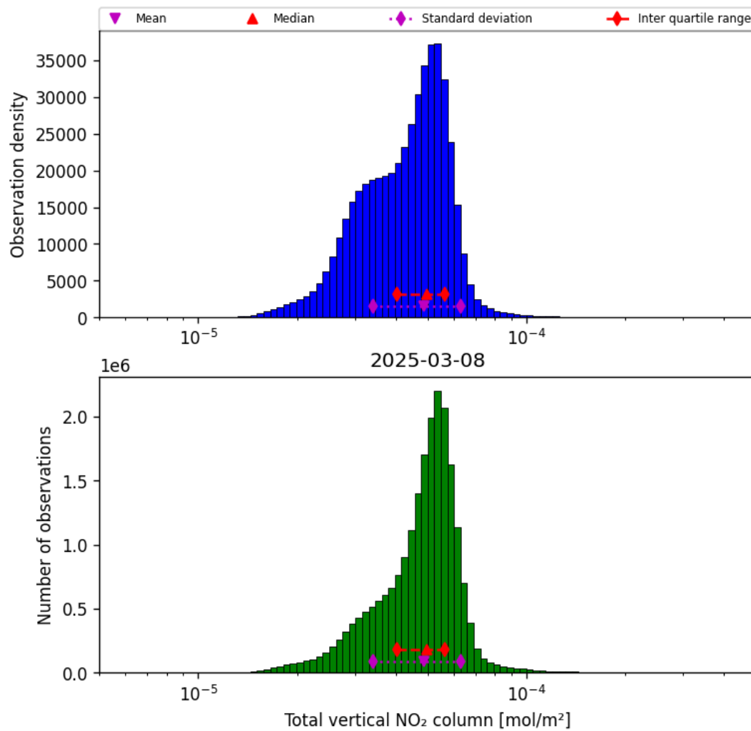
Figure 38: Histogram of “Total vertical NO 2 column” for 2025-03-08 to 2025-03-09
