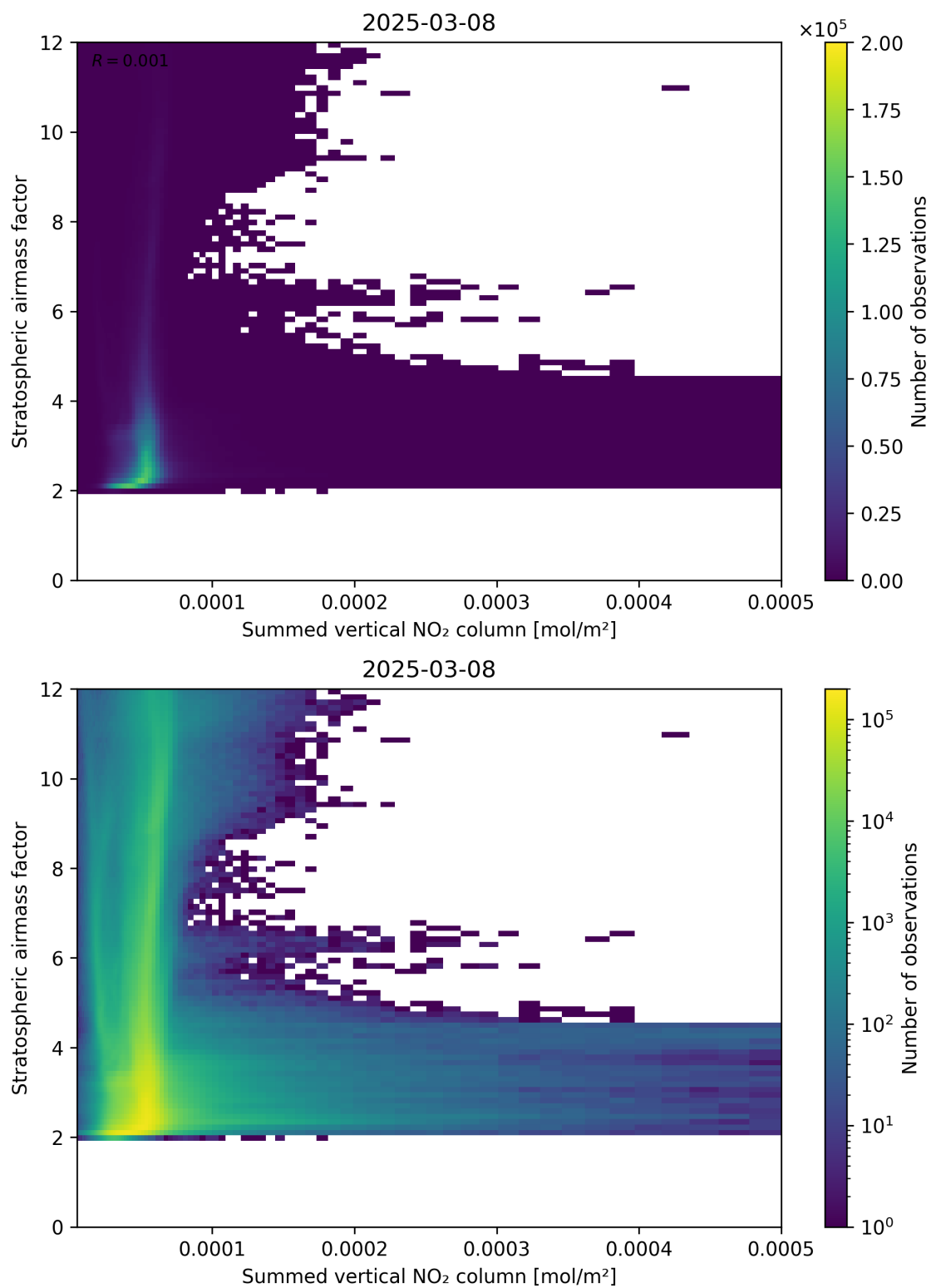
Figure 103: Scatter density plot of “Summed vertical NO 2 column” against “Stratospheric air mass factor” for 2025-03-08 to 2025-03-09.
