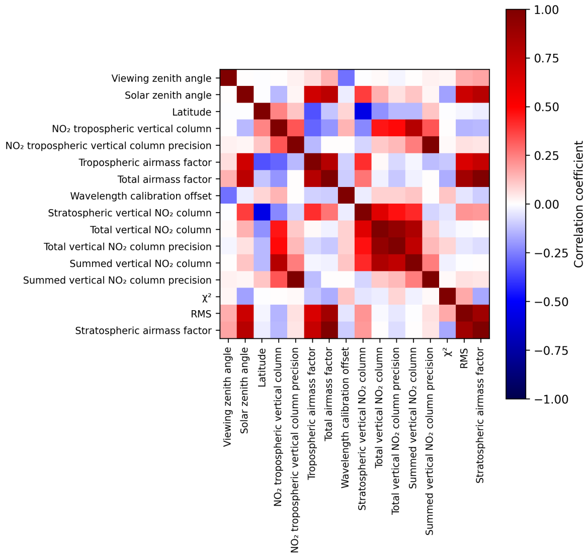
Figure 2: Map of correlation matrix for 2025-03-08 to 2025-03-09.
