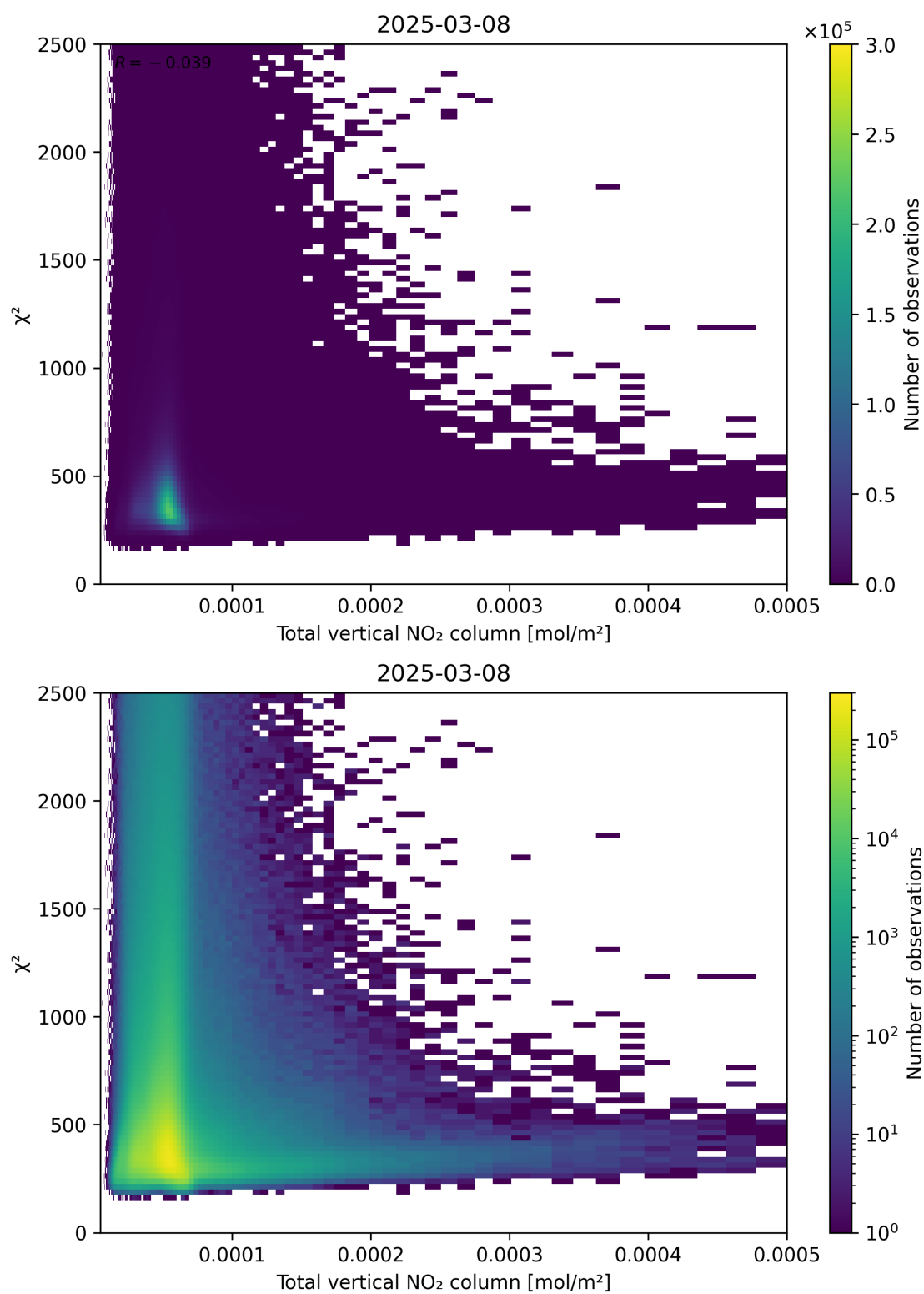
Figure 111: Scatter density plot of “Total vertical NO 2 column” against “ \chi^2 ” for 2025-03-08 to 2025-03-09.
