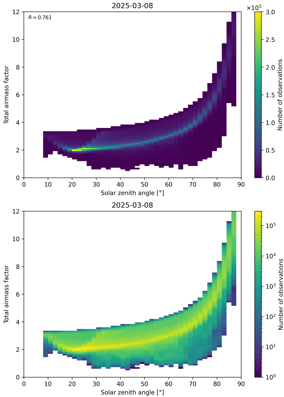
Figure 146: Scatter density plot of “Solar zenith angle” against “Total air mass factor” for 2025-03-08 to 2025-03-09.
