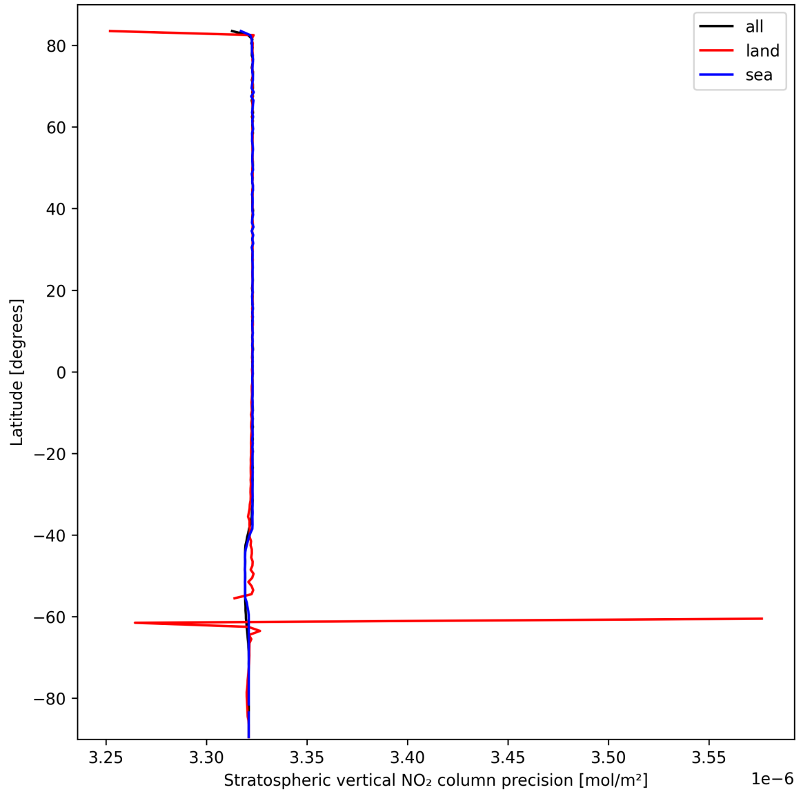
Figure 20: Zonal average of “Stratospheric vertical NO 2 column precision” for 2025-03-08 to 2025-03-09.
