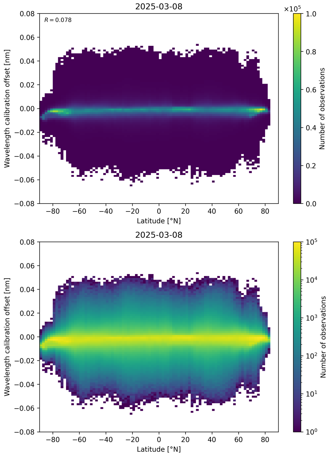
Figure 95: Scatter density plot of “Latitude” against “Wavelength calibration offset” for 2025-03-08 to 2025-03-09.
