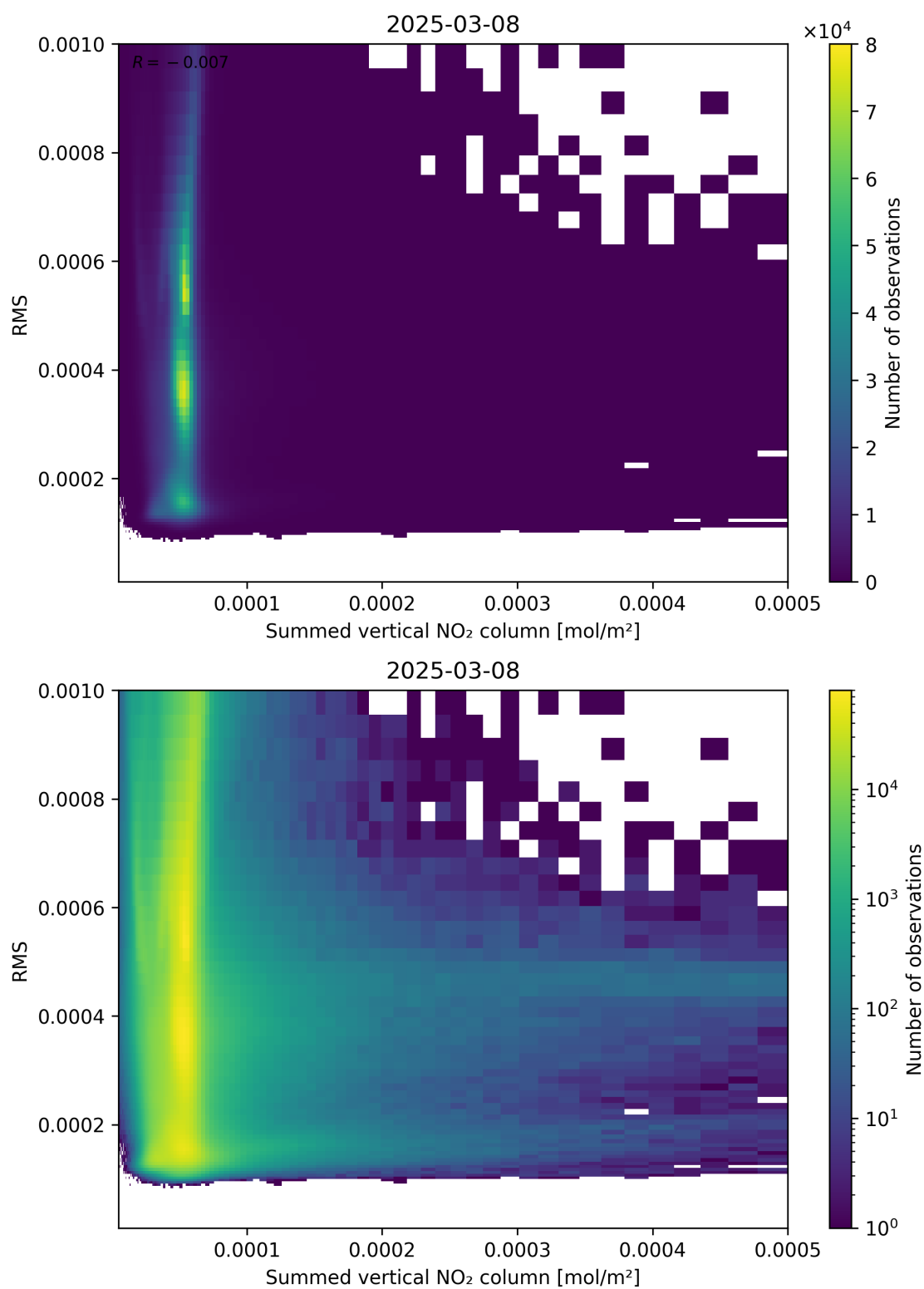
Figure 109: Scatter density plot of “Summed vertical NO 2 column” against “RMS” for 2025-03-08 to 2025-03-09.
