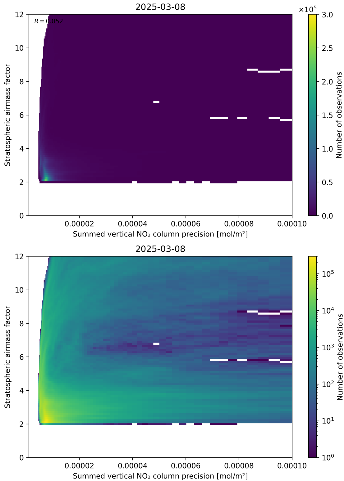
Figure 106: Scatter density plot of “Summed vertical NO 2 column precision” against “Stratospheric airmass factor” for 2025-03-08 to 2025-03-09.
