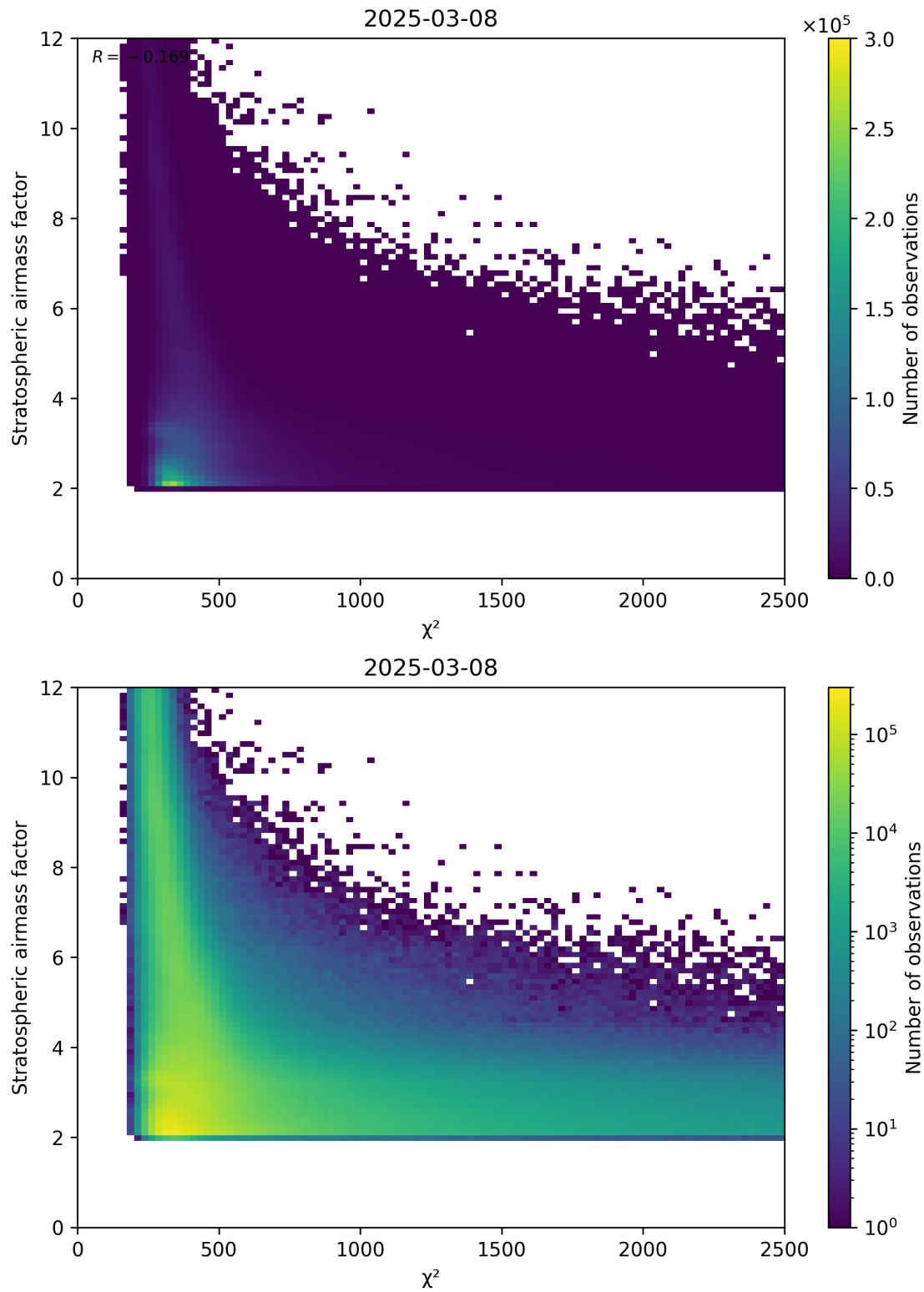
Figure 81: Scatter density plot of “ \chi^2 ” against “Stratospheric airmass factor” for 2025-03-08 to 2025-03-09.
