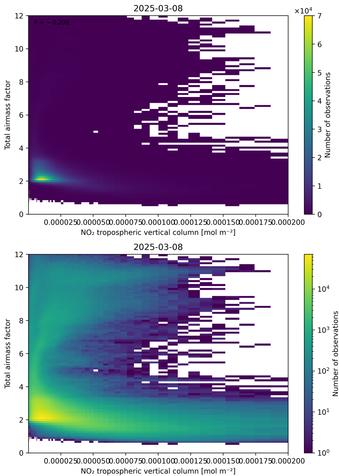
Figure 122: Scatter density plot of “NO 2 tropospheric vertical column” against “Total air mass factor” for 2025-03-08 to 2025-03-09.
