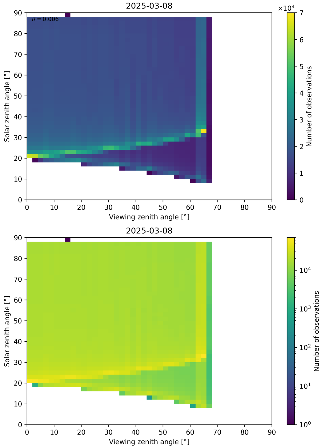
Figure 172: Scatter density plot of “Viewing zenith angle” against “Solar zenith angle” for 2025-03-08 to 2025-03-09.
