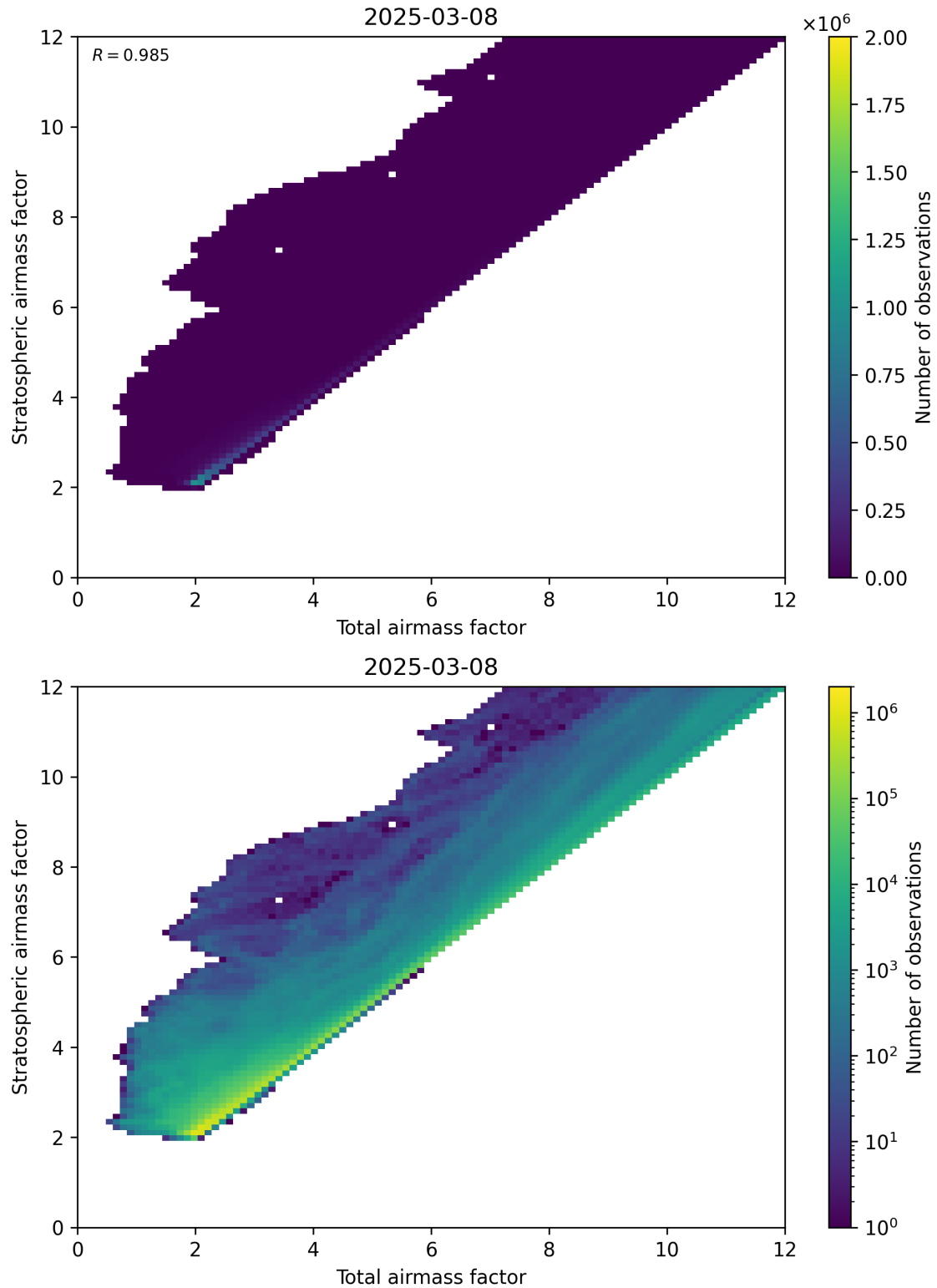
Figure 62: Scatter density plot of “Total airmass factor” against “Stratospheric airmass factor” for 2025-03-08 to 2025-03-09.
