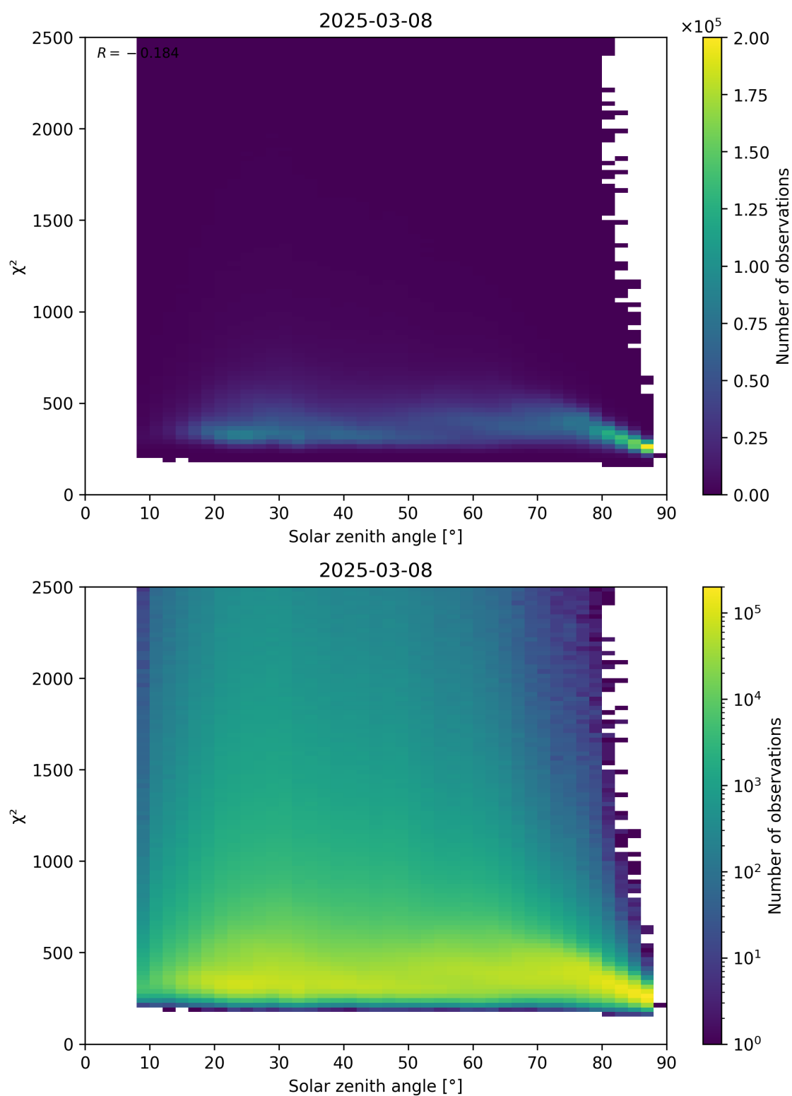
Figure 148: Scatter density plot of “Solar zenith angle” against “ \chi^2 ” for 2025-03-08 to 2025-03-09.
