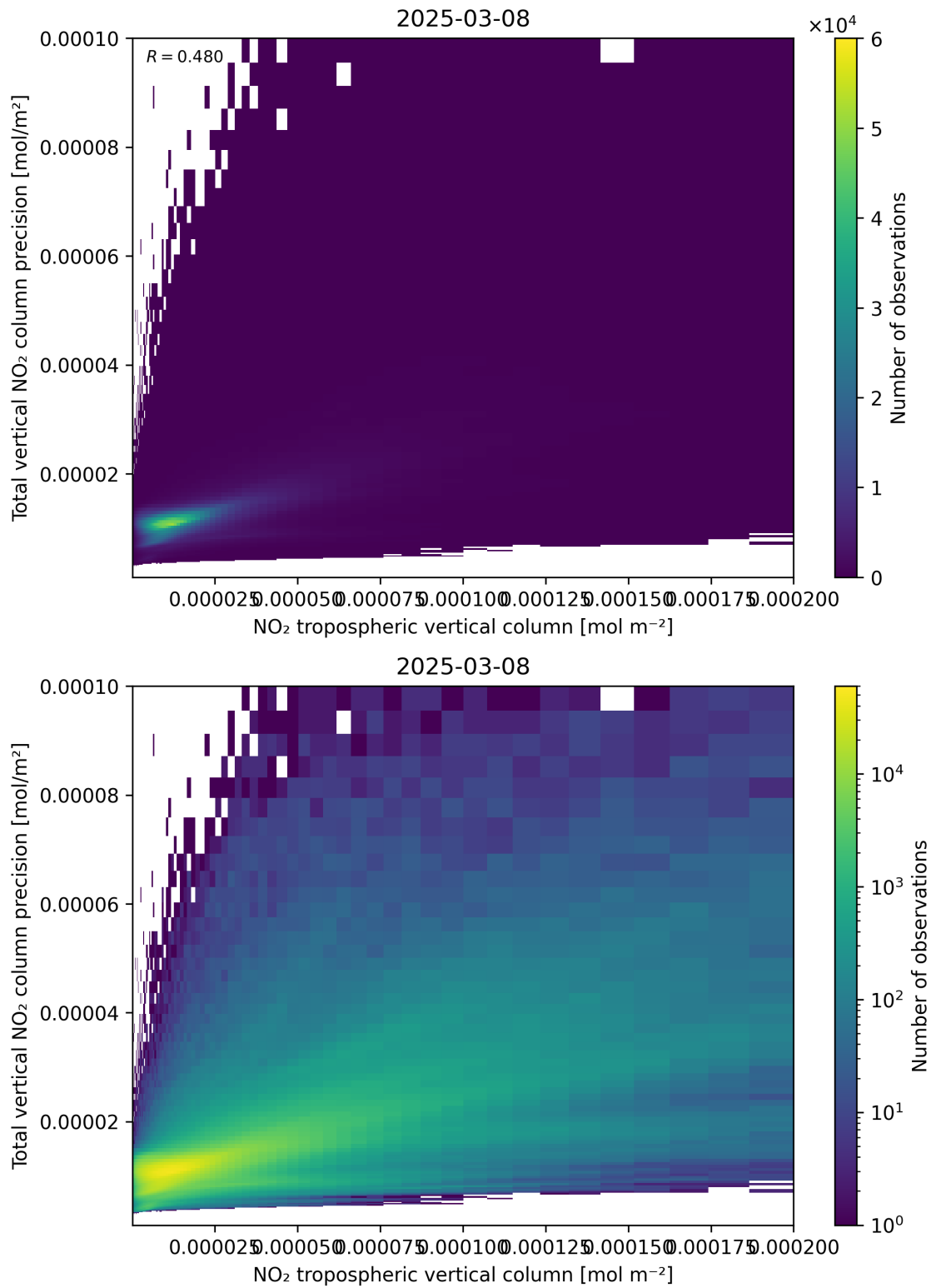
Figure 129: Scatter density plot of “NO 2 tropospheric vertical column” against “Total vertical NO 2 column precision” for 2025-03-08 to 2025-03-09.
