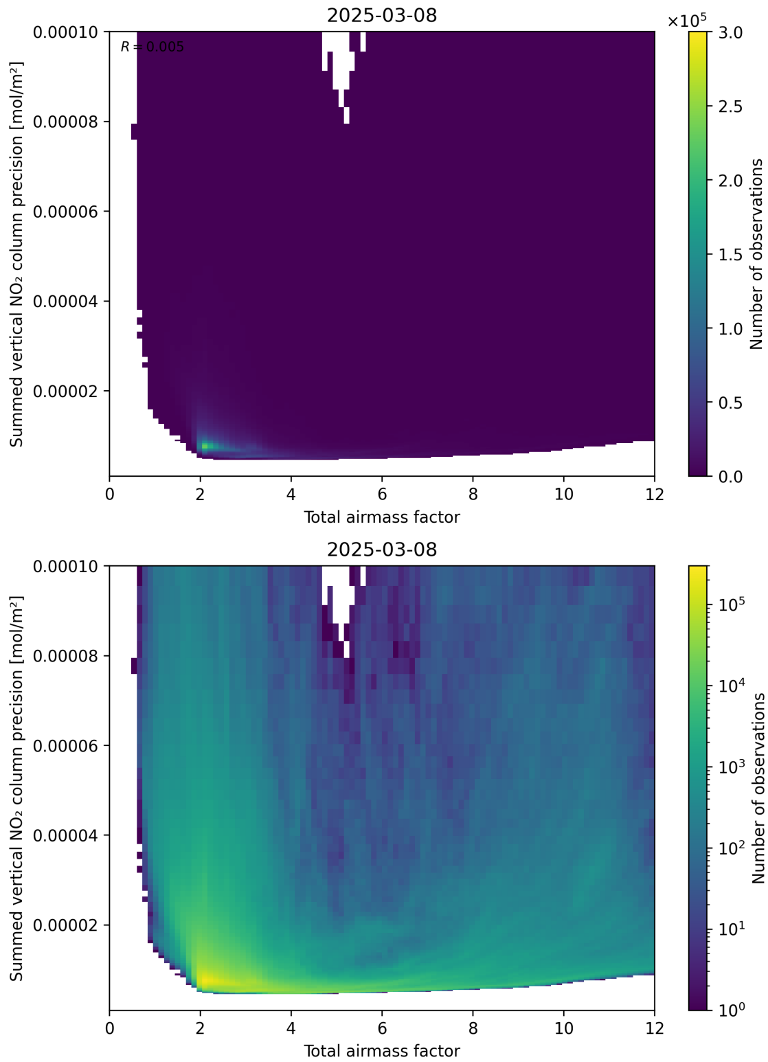
Figure 66: Scatter density plot of “Total airmass factor” against “Summed vertical NO 2 column precision” for 2025-03-08 to 2025-03-09.
