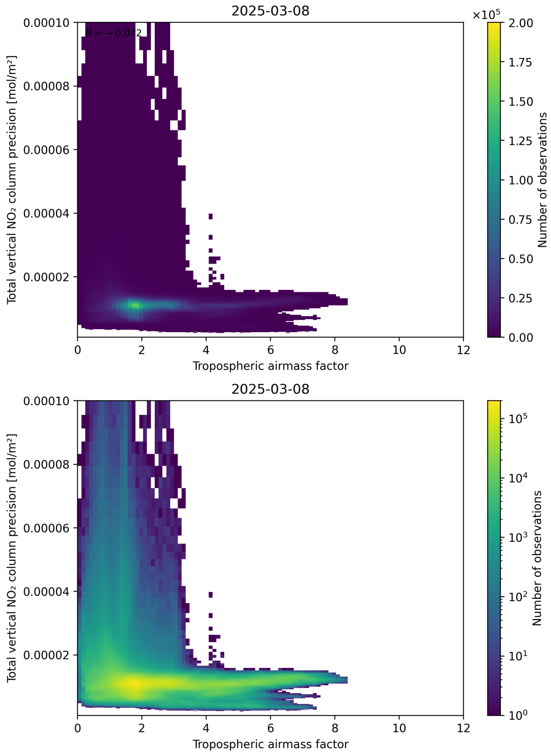
Figure 78: Scatter density plot of “Tropospheric air mass factor” against “Total vertical NO 2 column precision” for 2025-03-08 to 2025-03-09.
