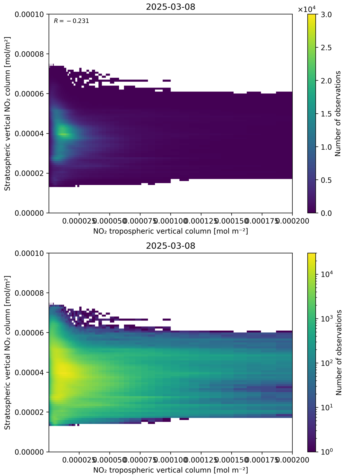
Figure 125: Scatter density plot of “NO 2 tropospheric vertical column” against “Stratospheric vertical NO 2 column” for 2025-03-08 to 2025-03-09.
