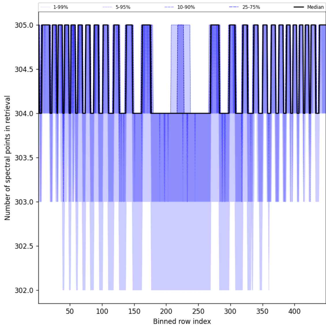
Figure 50: Along track statistics of “Number of spectral points in retrieval” for 2025-03-09 to 2025-03-10
