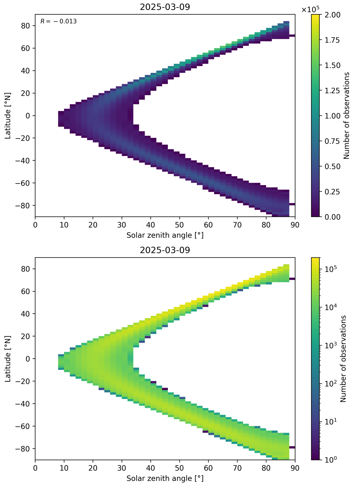
Figure 149: Scatter density plot of “Solar zenith angle” against “Latitude” for 2025-03-09 to 2025-03-10.
