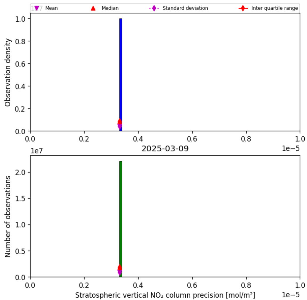
Figure 37: Histogram of “Stratospheric vertical NO 2 column precision” for 2025-03-09 to 2025-03-10
