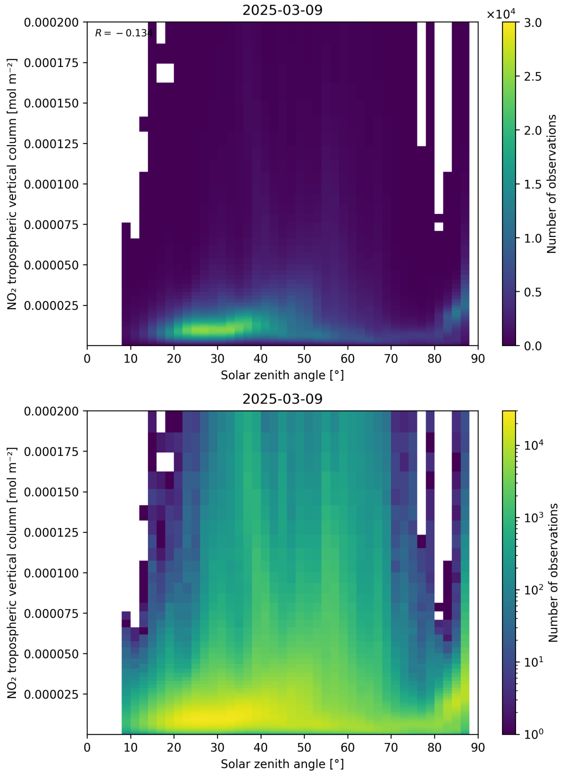
Figure 155: Scatter density plot of “Solar zenith angle” against “NO 2 tropospheric vertical column” for 2025-03-09 to 2025-03-10.
