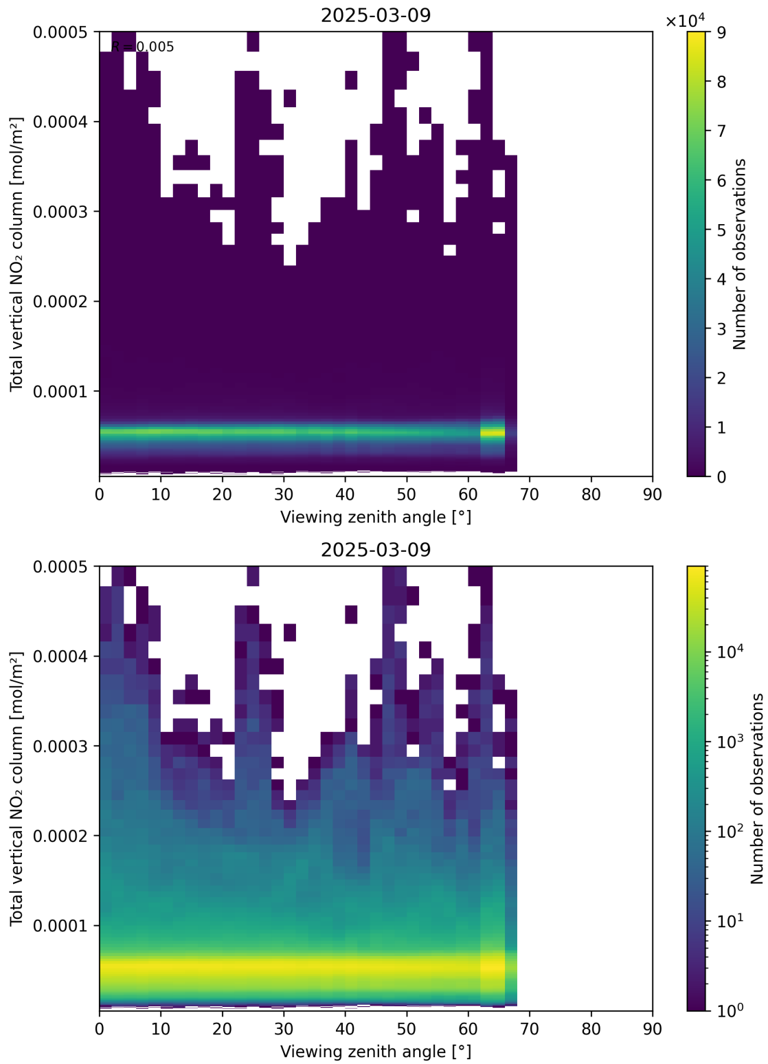
Figure 167: Scatter density plot of “Viewing zenith angle” against “Total vertical NO 2 column” for 2025-03-09 to 2025-03-10.
