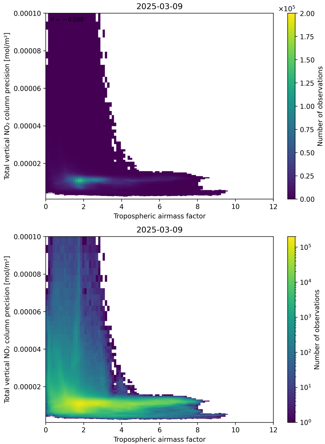
Figure 78: Scatter density plot of “Tropospheric air mass factor” against “Total vertical NO 2 column precision” for 2025-03-09 to 2025-03-10.
