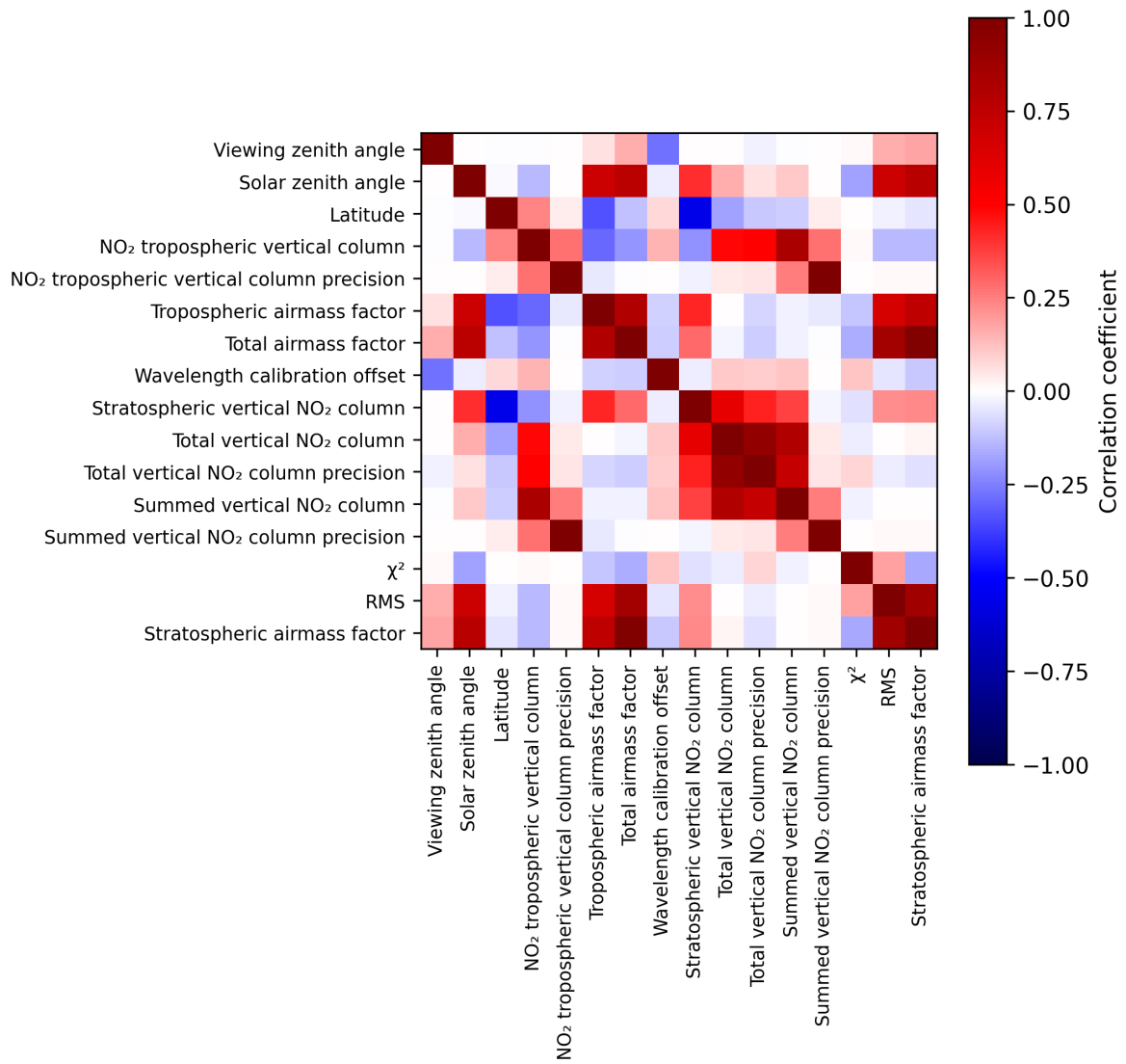
Figure 2: Map of correlation matrix for 2025-03-09 to 2025-03-10.
