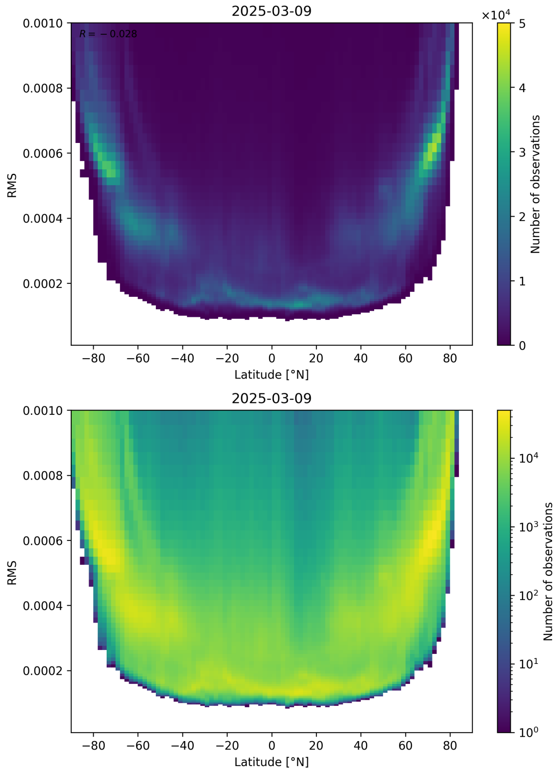
Figure 94: Scatter density plot of “Latitude” against “RMS” for 2025-03-09 to 2025-03-10.
