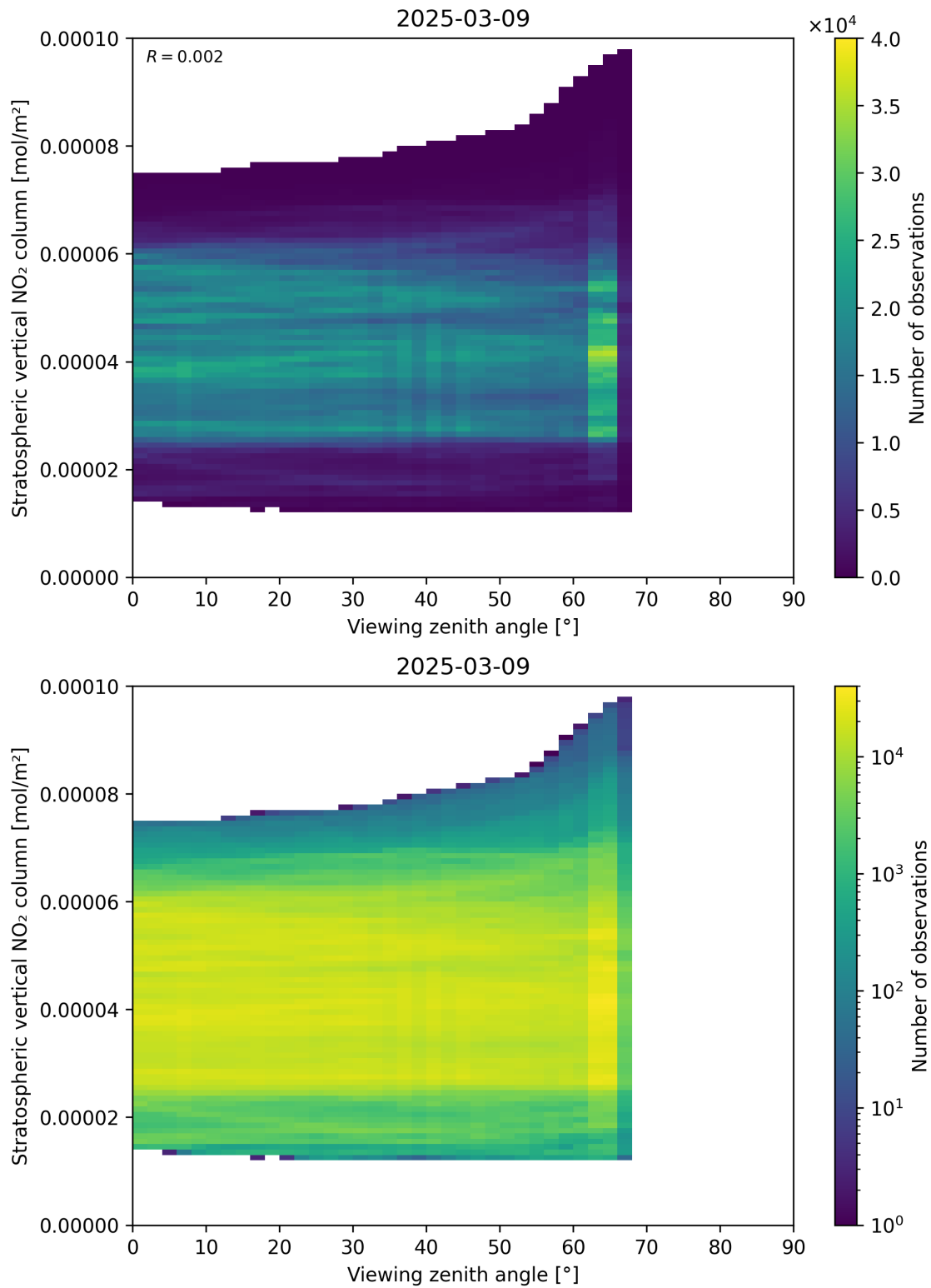
Figure 164: Scatter density plot of “Viewing zenith angle” against “Stratospheric vertical NO 2 column” for 2025-03-09 to 2025-03-10.
