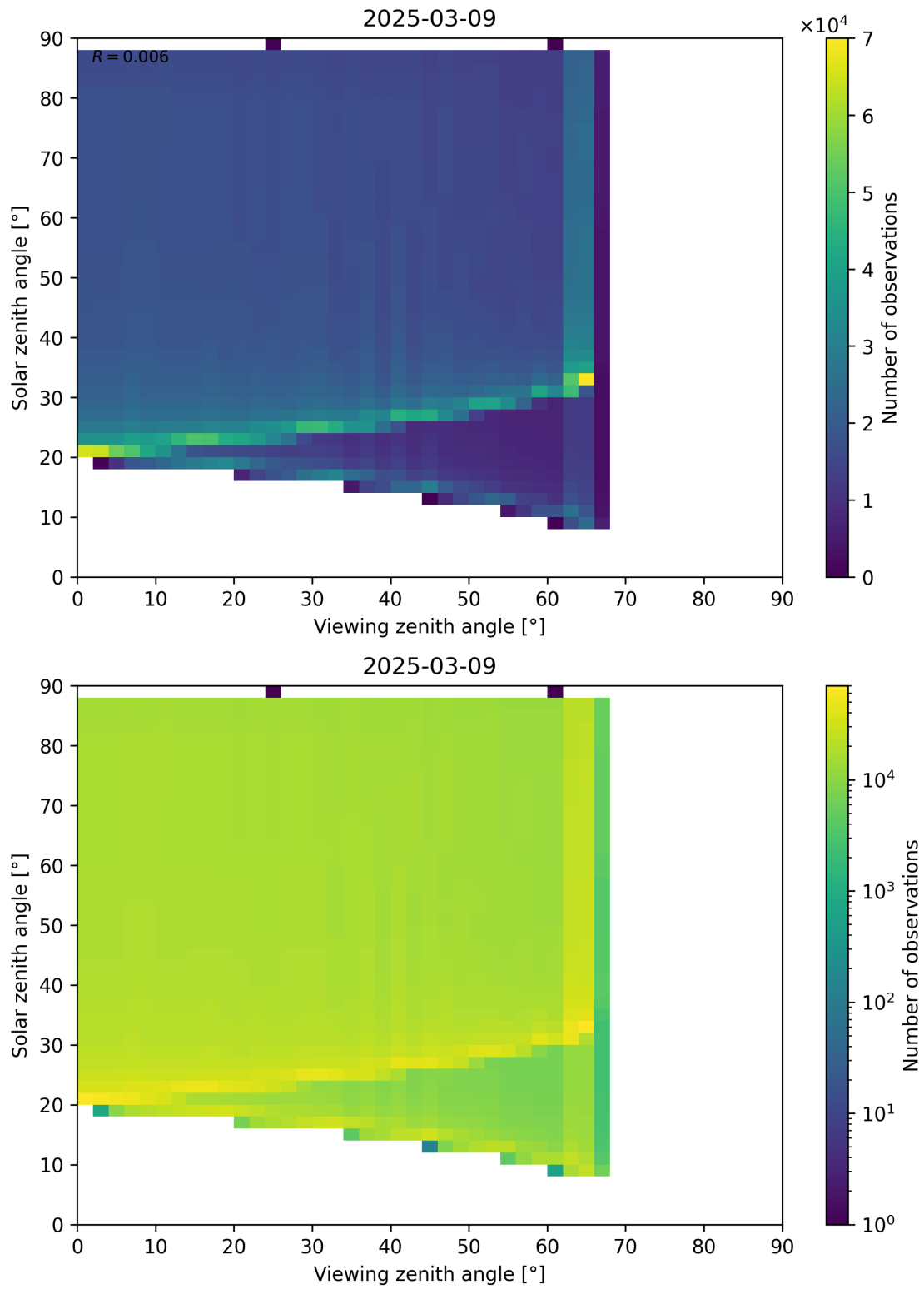
Figure 172: Scatter density plot of “Viewing zenith angle” against “Solar zenith angle” for 2025-03-09 to 2025-03-10.
