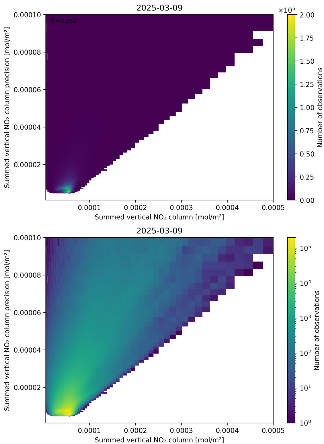
Figure 105: Scatter density plot of “Summed vertical NO 2 column” against “Summed vertical NO 2 column precision” for 2025-03-09 to 2025-03-10.
