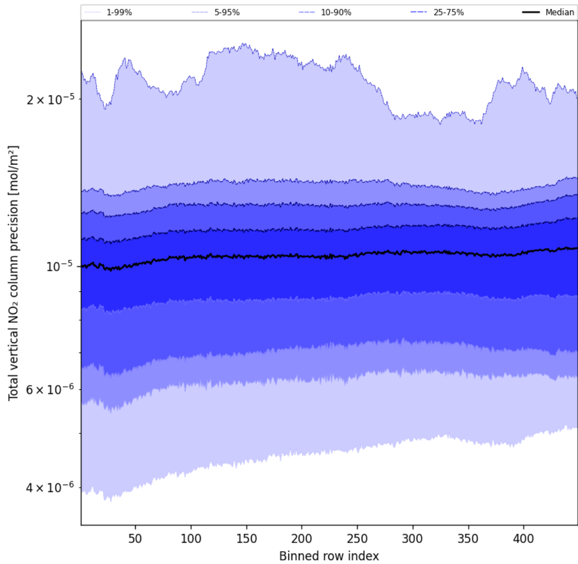
Figure 56: Along track statistics of “Total vertical NO 2 column precision” for 2025-03-09 to 2025-03-10
