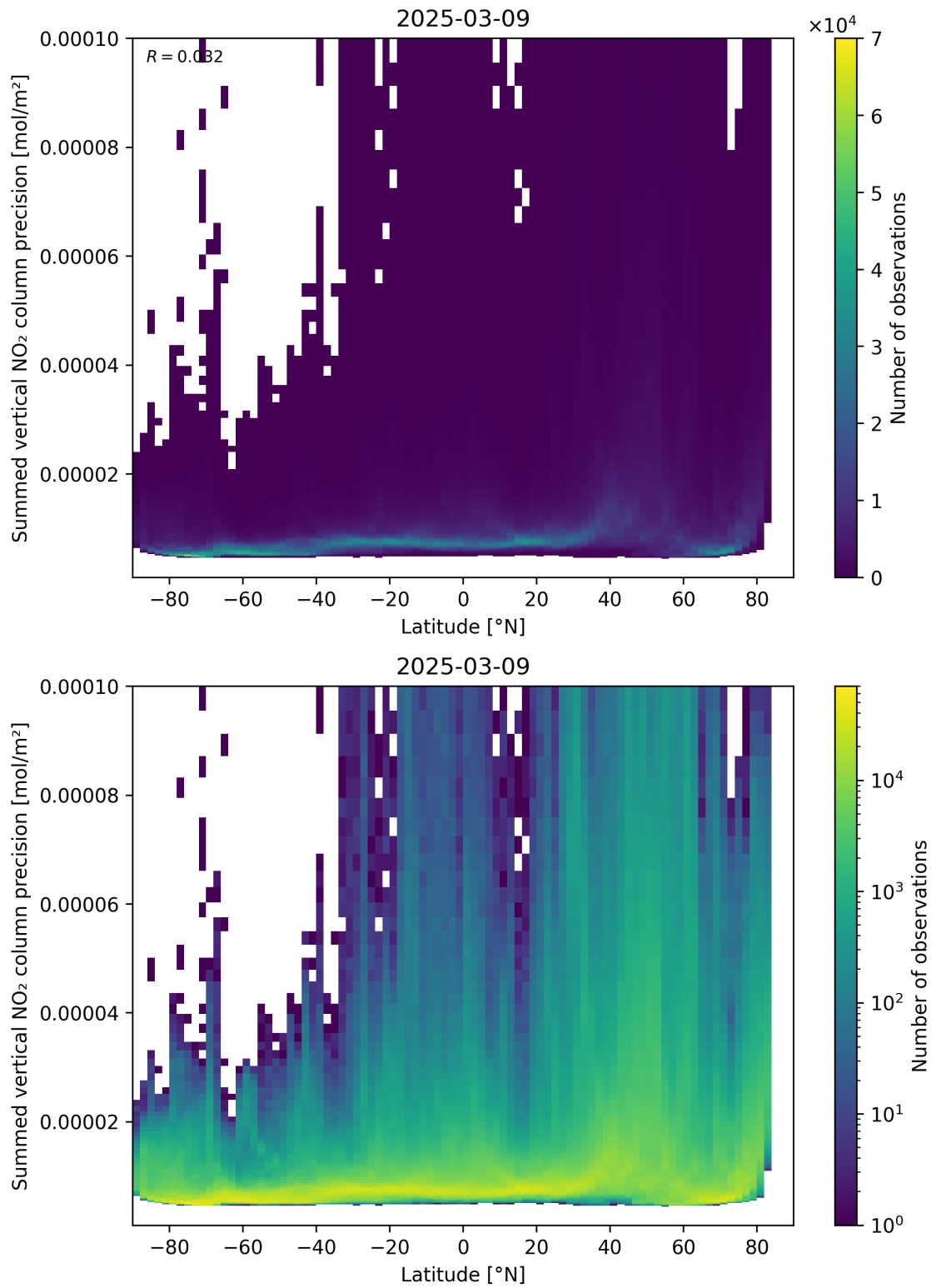
Figure 89: Scatter density plot of “Latitude” against “Summed vertical NO 2 column precision” for 2025-03-09 to 2025-03-10.
