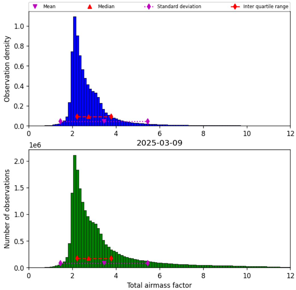
Figure 32: Histogram of “Total airmass factor” for 2025-03-09 to 2025-03-10
