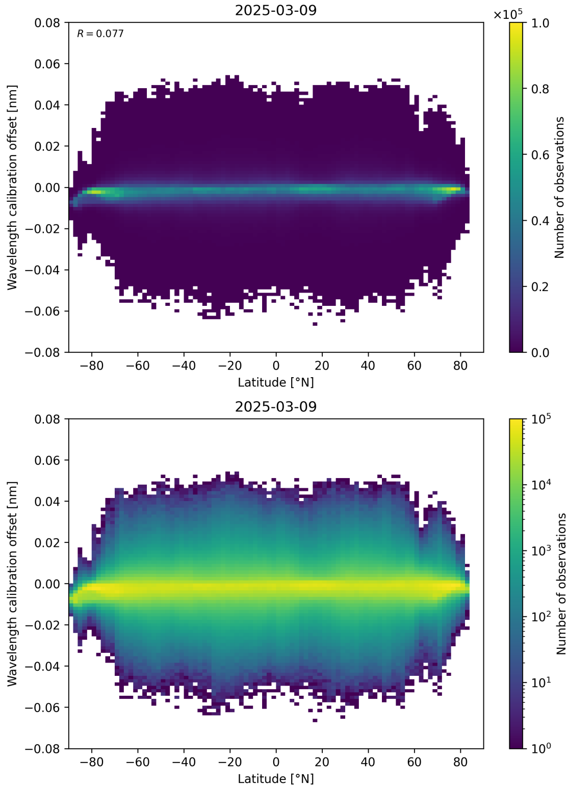
Figure 95: Scatter density plot of “Latitude” against “Wavelength calibration offset” for 2025-03-09 to 2025-03-10.
