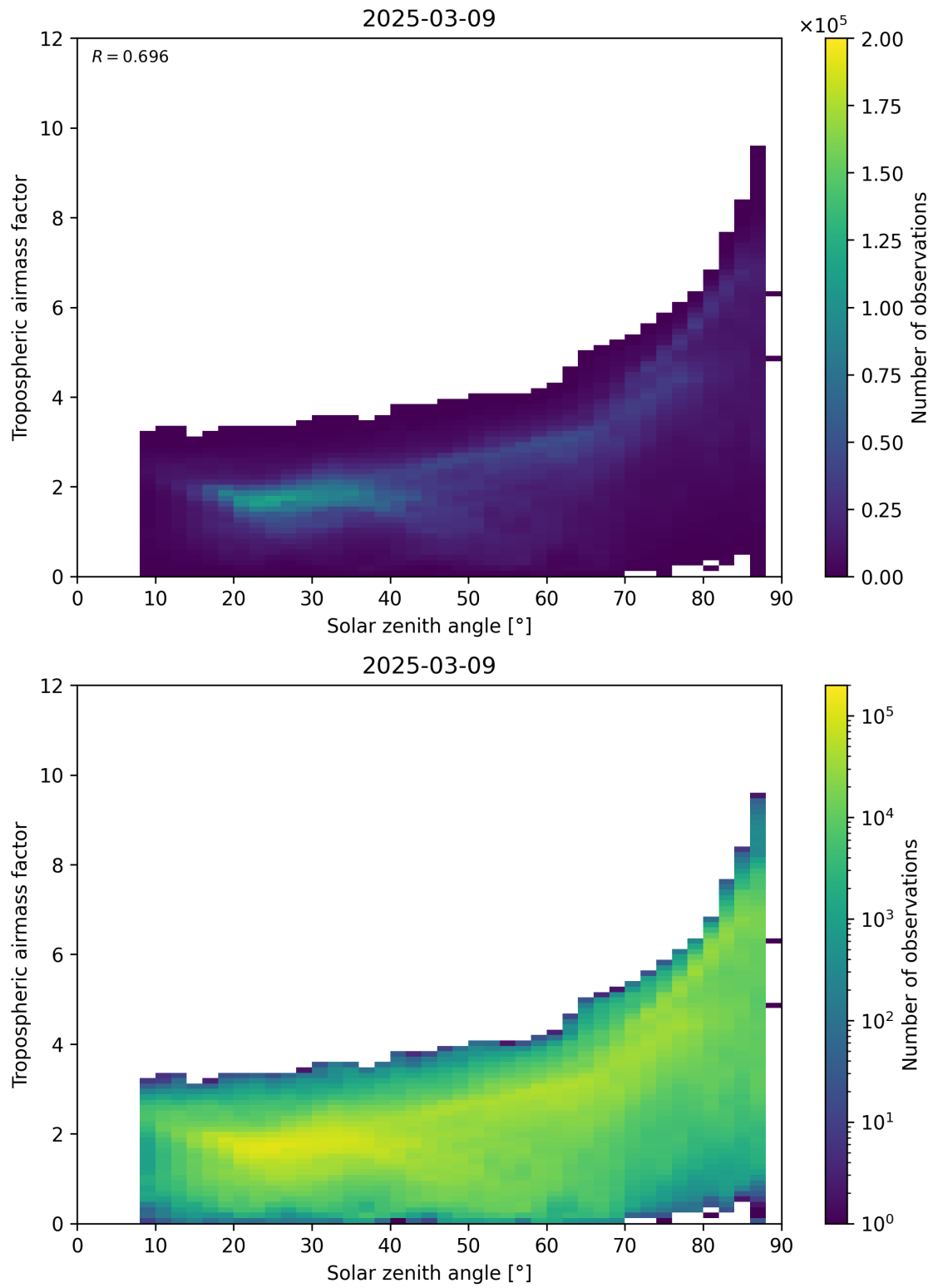
Figure 147: Scatter density plot of “Solar zenith angle” against “Tropospheric airmass factor” for 2025-03-09 to 2025-03-10.
