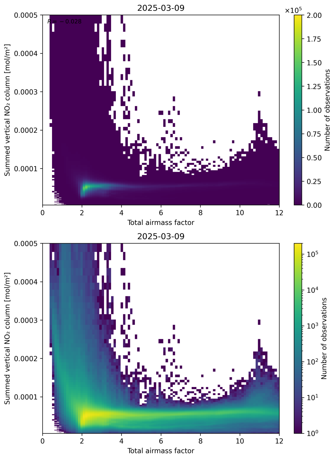
Figure 65: Scatter density plot of “Total airmass factor” against “Summed vertical NO 2 column” for 2025-03-09 to 2025-03-10.
