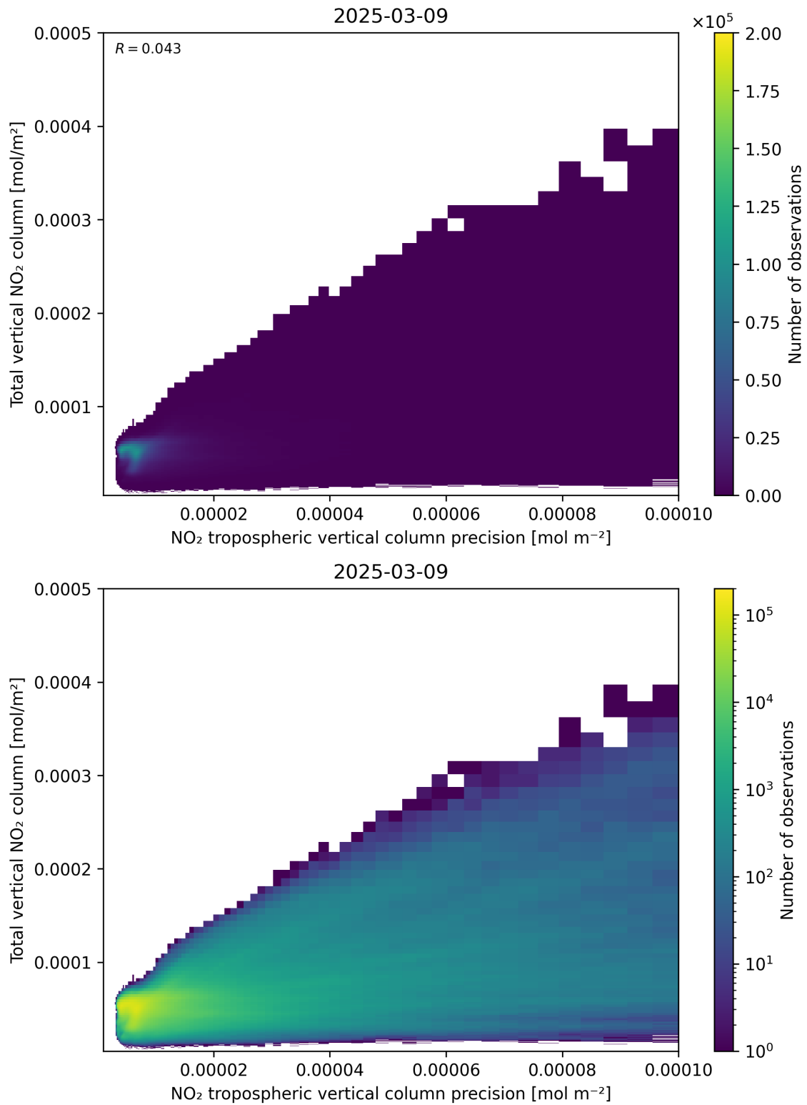
Figure 138: Scatter density plot of “NO 2 tropospheric vertical column precision” against “Total vertical NO 2 column” for 2025-03-09 to 2025-03-10.
