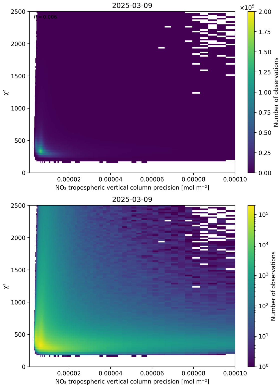
Figure 134: Scatter density plot of “NO 2 tropospheric vertical column precision” against “ \chi^2 ” for 2025-03-09 to 2025-03-10.
