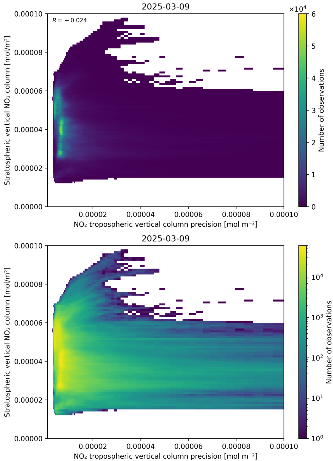
Figure 135: Scatter density plot of “NO 2 tropospheric vertical column precision” against “Stratospheric vertical NO 2 column” for 2025-03-09 to 2025-03-10.
