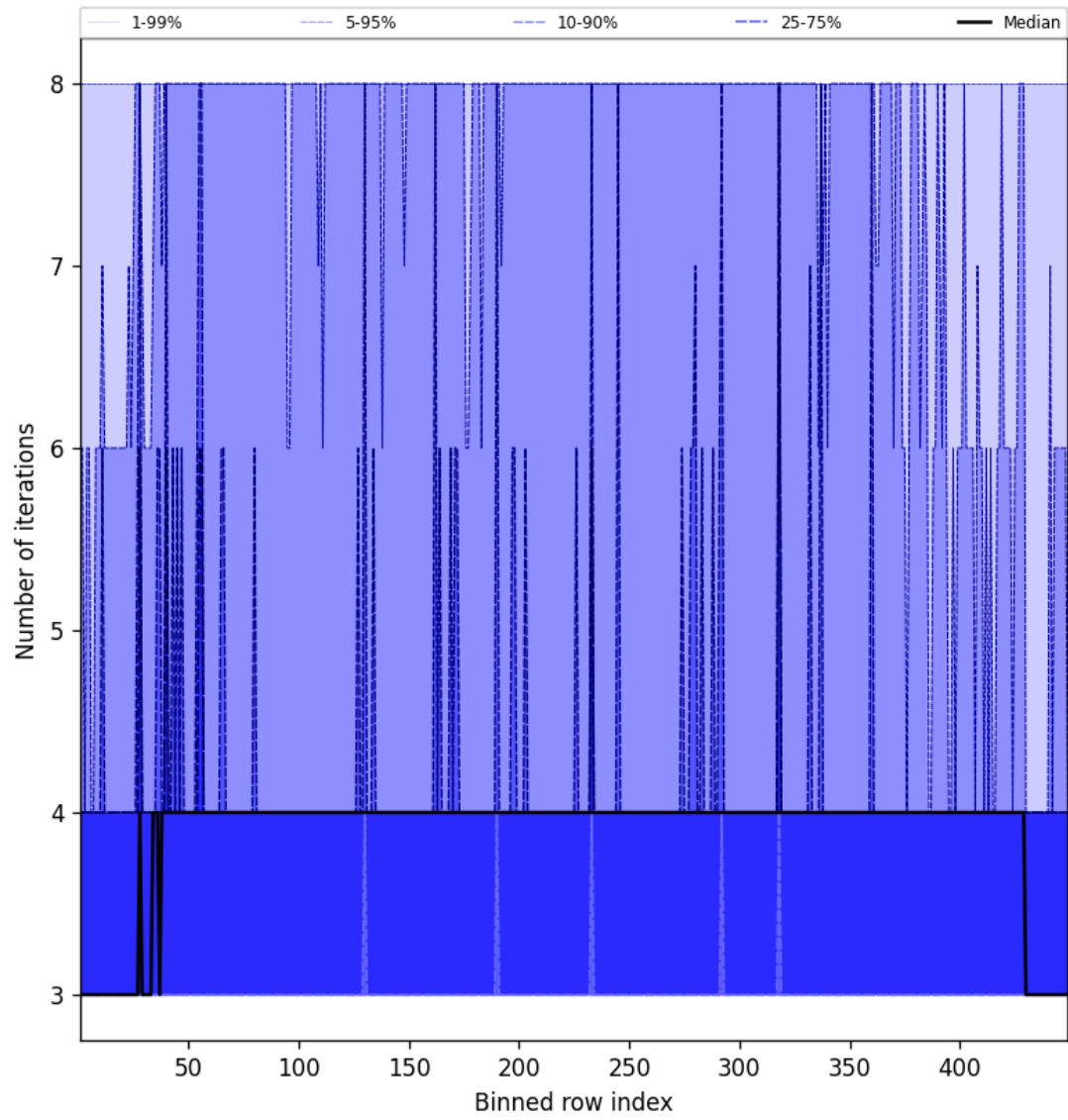
Figure 51: Along track statistics of “Number of iterations” for 2025-03-09 to 2025-03-10
