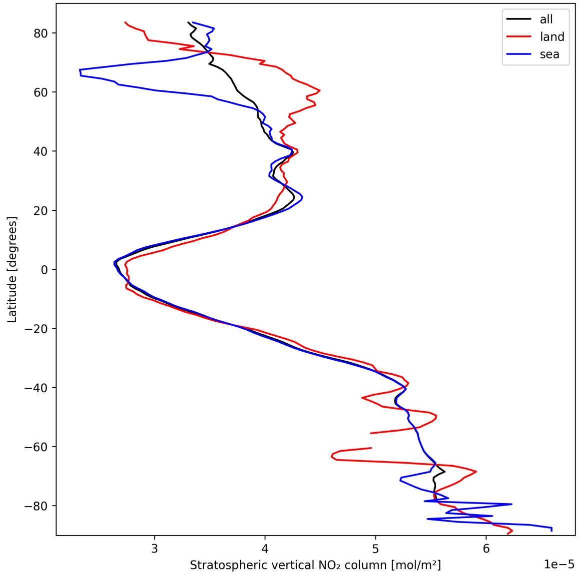
Figure 19: Zonal average of “Stratospheric vertical NO 2 column” for 2025-03-09 to 2025-03-10.
