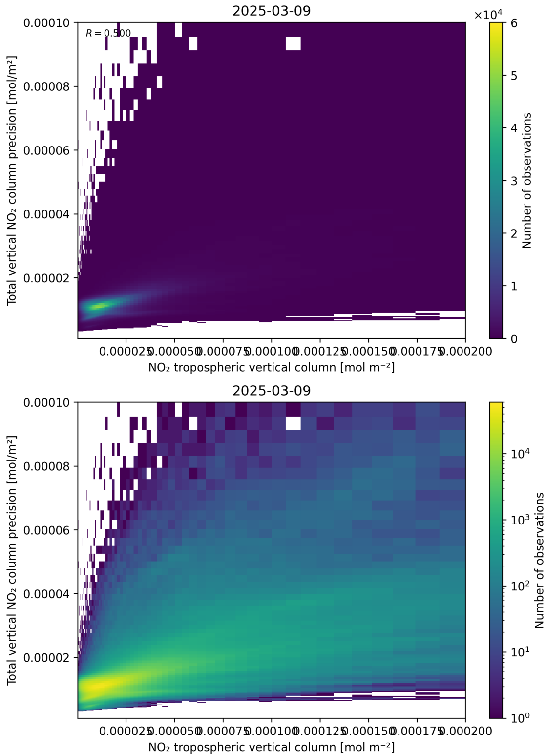
Figure 129: Scatter density plot of “NO 2 tropospheric vertical column” against “Total vertical NO 2 column precision” for 2025-03-09 to 2025-03-10.
