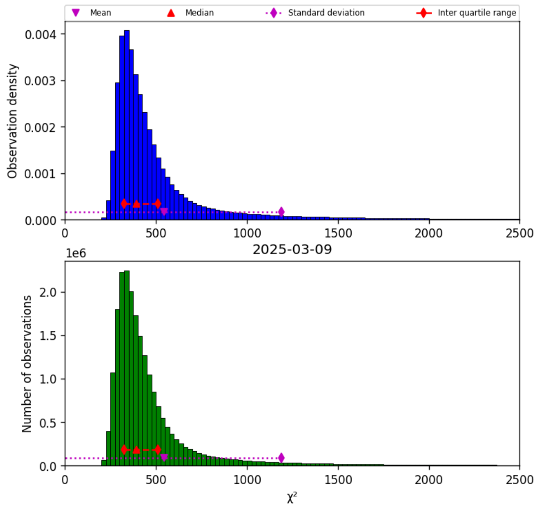
Figure 42: Histogram of “ \chi^2 ” for 2025-03-09 to 2025-03-10
