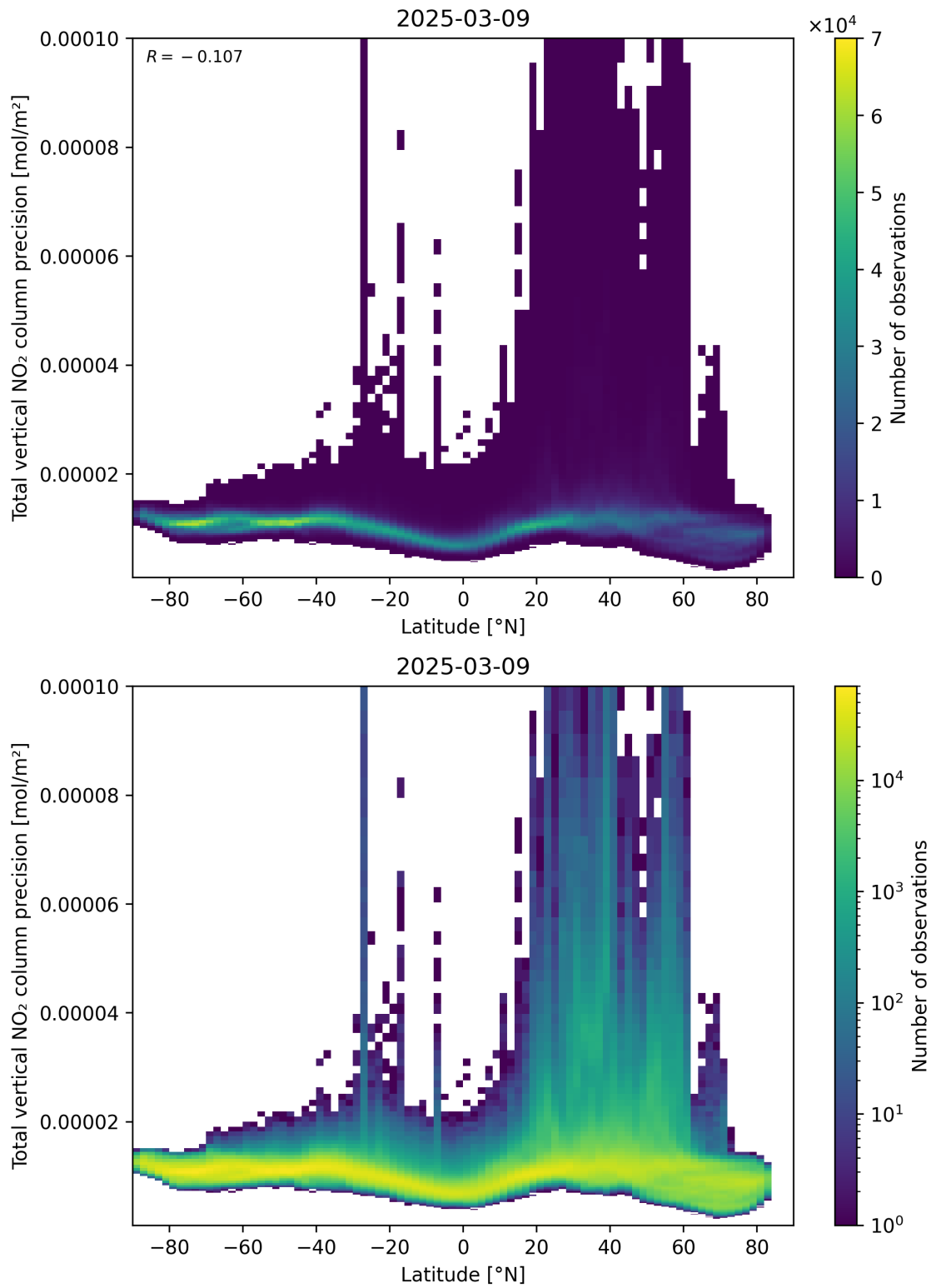
Figure 91: Scatter density plot of “Latitude” against “Total vertical NO 2 column precision” for 2025-03-09 to 2025-03-10.
