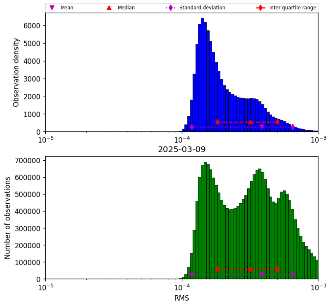
Figure 43: Histogram of “RMS” for 2025-03-09 to 2025-03-10
