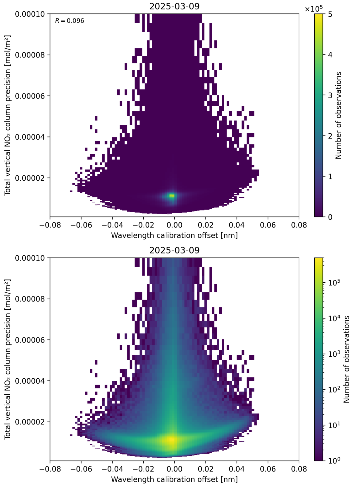
Figure 180: Scatter density plot of “Wavelength calibration offset” against “Total vertical NO 2 column precision” for 2025-03-09 to 2025-03-10.
