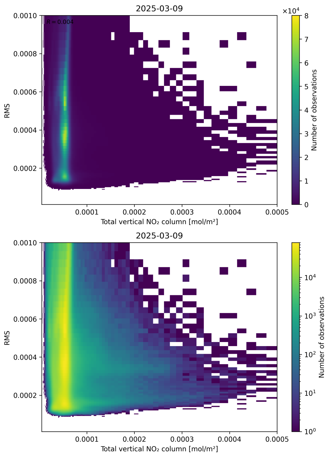
Figure 120: Scatter density plot of “Total vertical NO 2 column” against “RMS” for 2025-03-09 to 2025-03-10.
