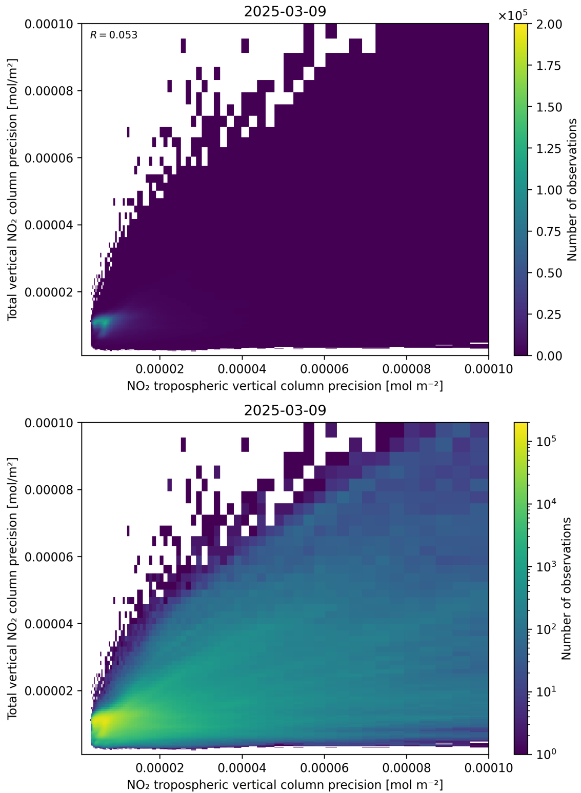
Figure 139: Scatter density plot of “NO 2 tropospheric vertical column precision” against “Total vertical NO 2 column precision” for 2025-03-09 to 2025-03-10.
