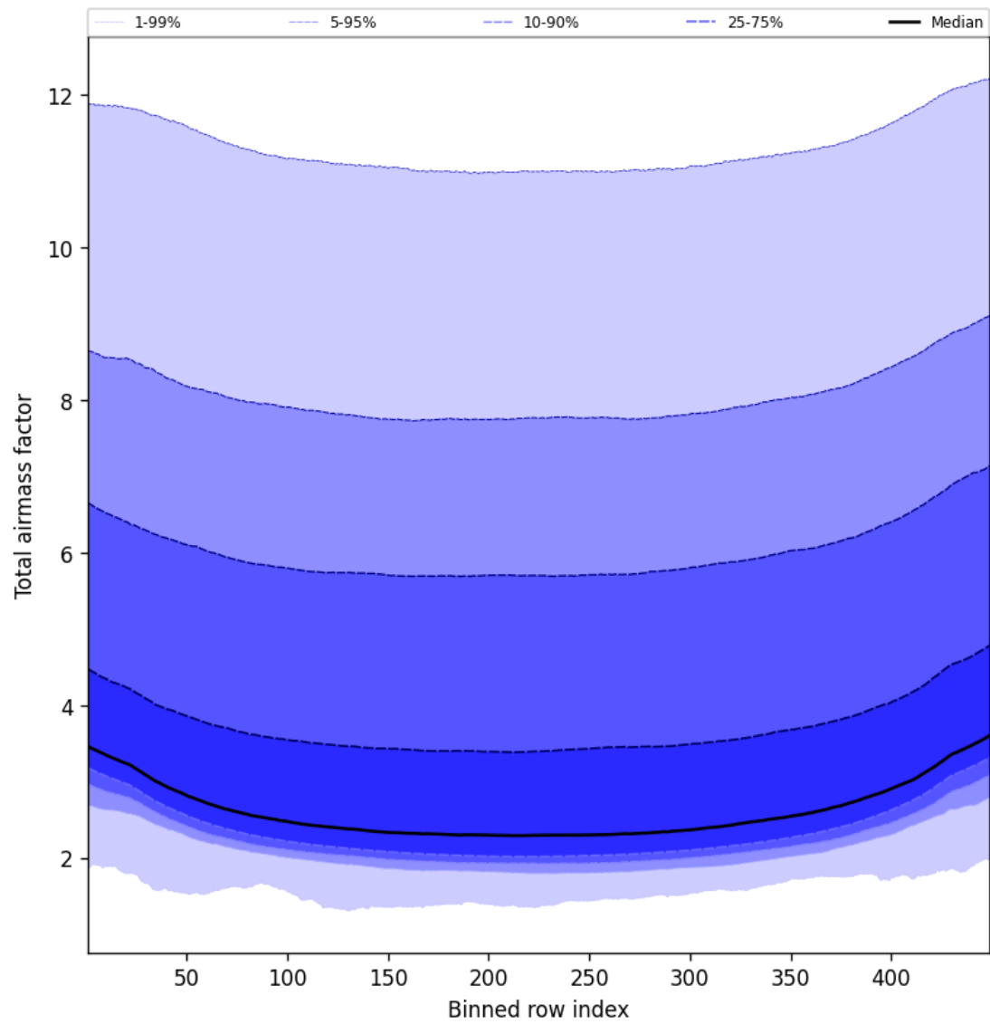
Figure 49: Along track statistics of “Total airmass factor” for 2025-03-09 to 2025-03-10
