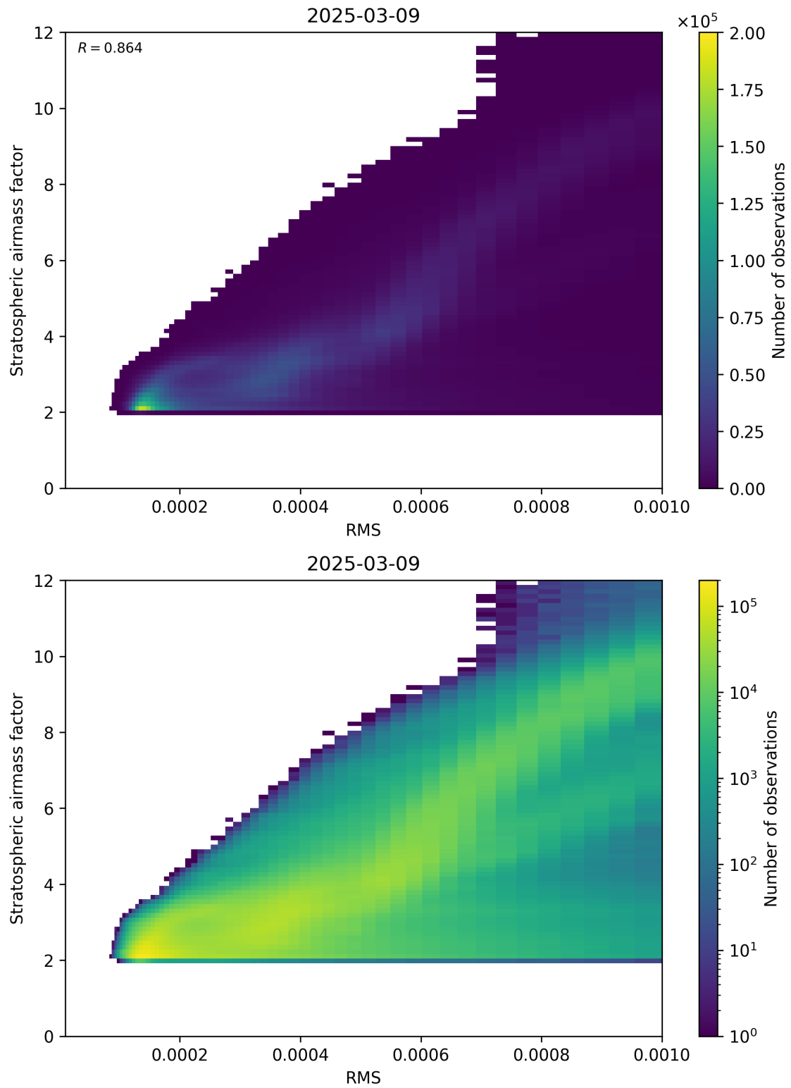
Figure 144: Scatter density plot of “RMS” against “Stratospheric airmass factor” for 2025-03-09 to 2025-03-10.
