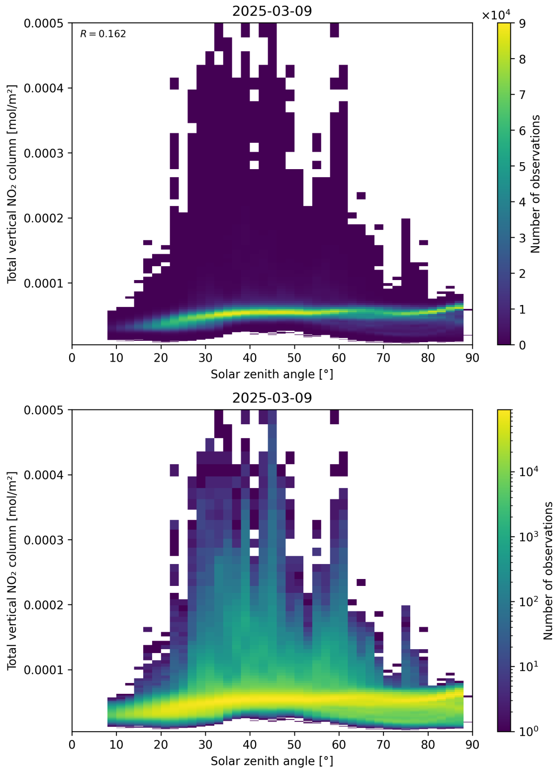
Figure 153: Scatter density plot of “Solar zenith angle” against “Total vertical NO 2 column” for 2025-03-09 to 2025-03-10.
