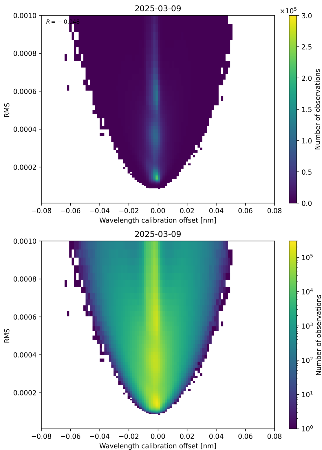
Figure 181: Scatter density plot of “Wavelength calibration offset” against “RMS” for 2025-03-09 to 2025-03-10.
