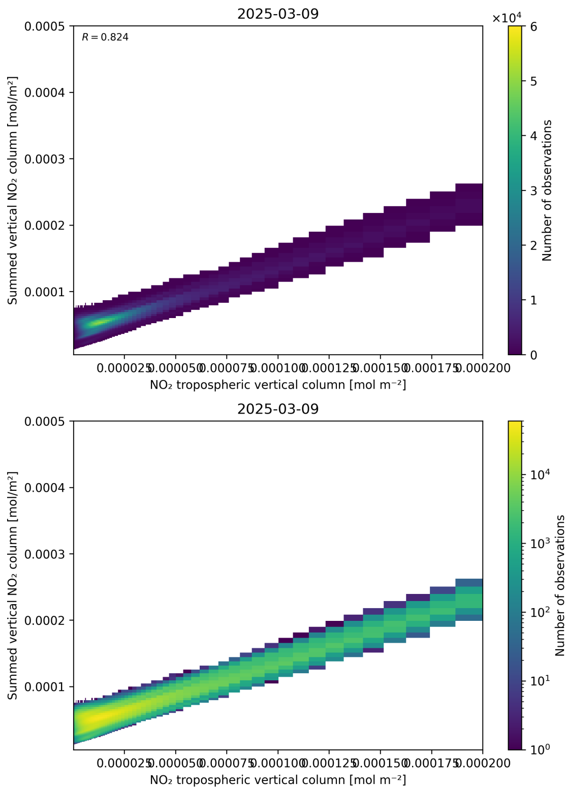
Figure 126: Scatter density plot of “NO 2 tropospheric vertical column” against “Summed vertical NO 2 column” for 2025-03-09 to 2025-03-10.
