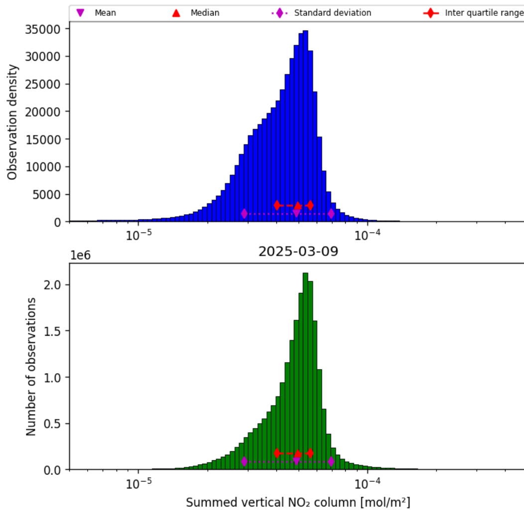
Figure 40: Histogram of “Summed vertical NO 2 column” for 2025-03-09 to 2025-03-10
