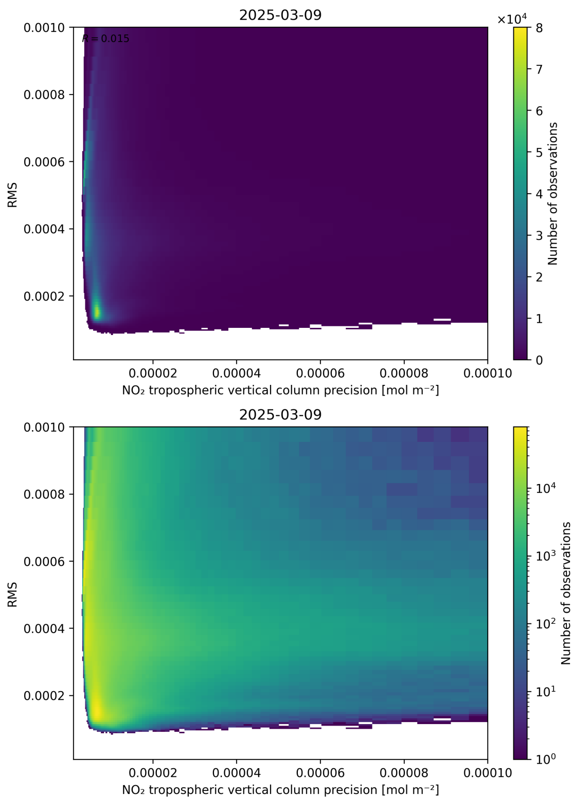
Figure 140: Scatter density plot of “NO 2 tropospheric vertical column precision” against “RMS” for 2025-03-09 to 2025-03-10.
