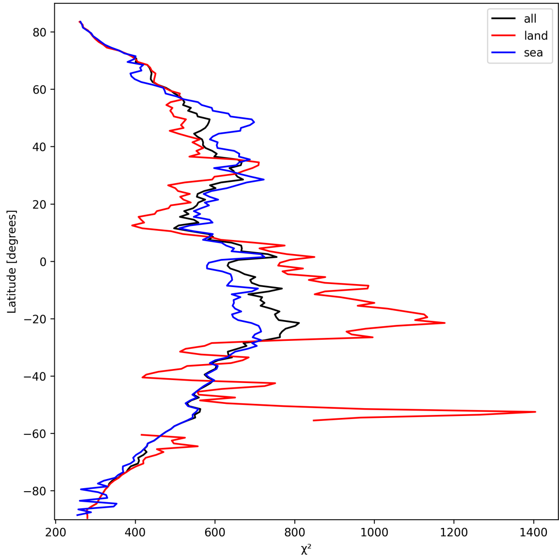
Figure 25: Zonal average of “ \chi^2 ” for 2025-03-09 to 2025-03-10.
