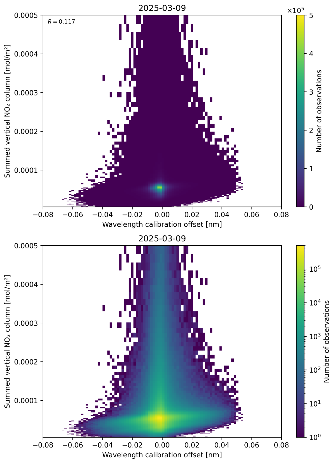
Figure 177: Scatter density plot of “Wavelength calibration offset” against “Summed vertical NO 2 column” for 2025-03-09 to 2025-03-10.
