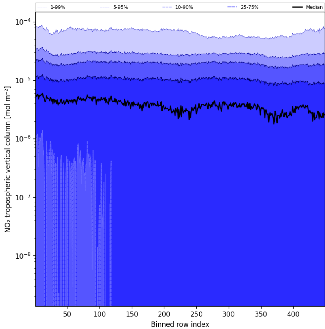
Figure 46: Along track statistics of “NO 2 tropospheric vertical column” for 2025-03-09 to 2025-03-10
