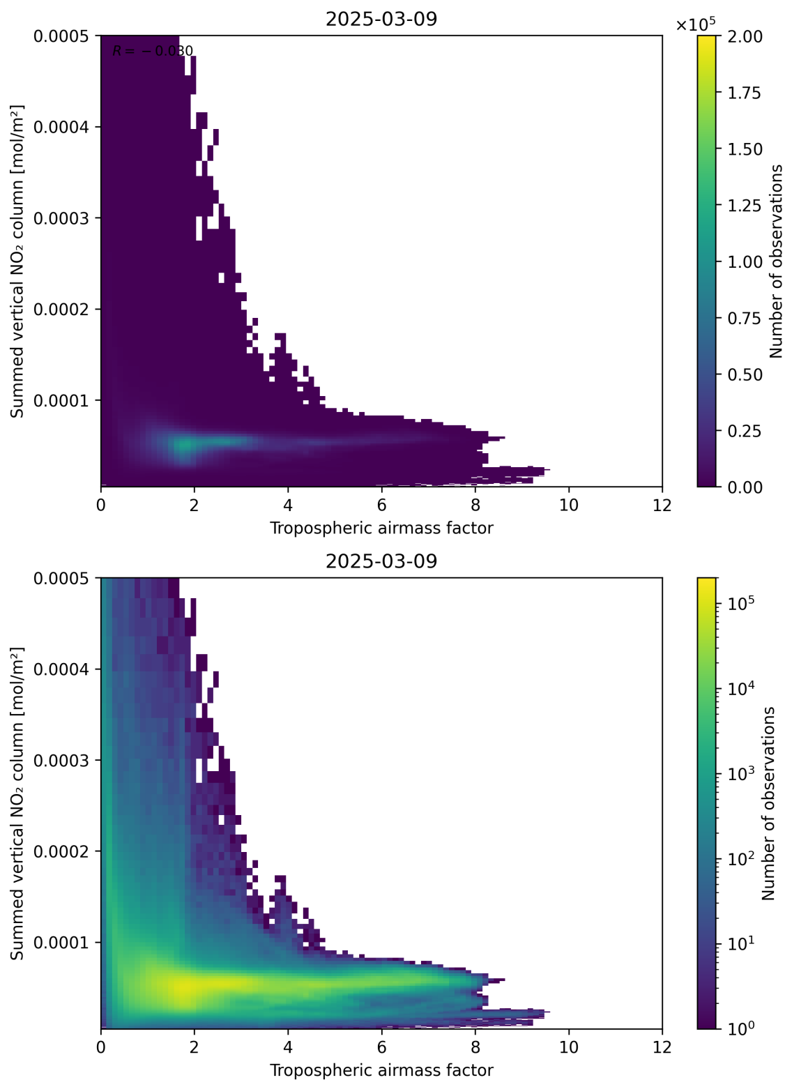
Figure 75: Scatter density plot of “Tropospheric air mass factor” against “Summed vertical NO 2 column” for 2025-03-09 to 2025-03-10.
