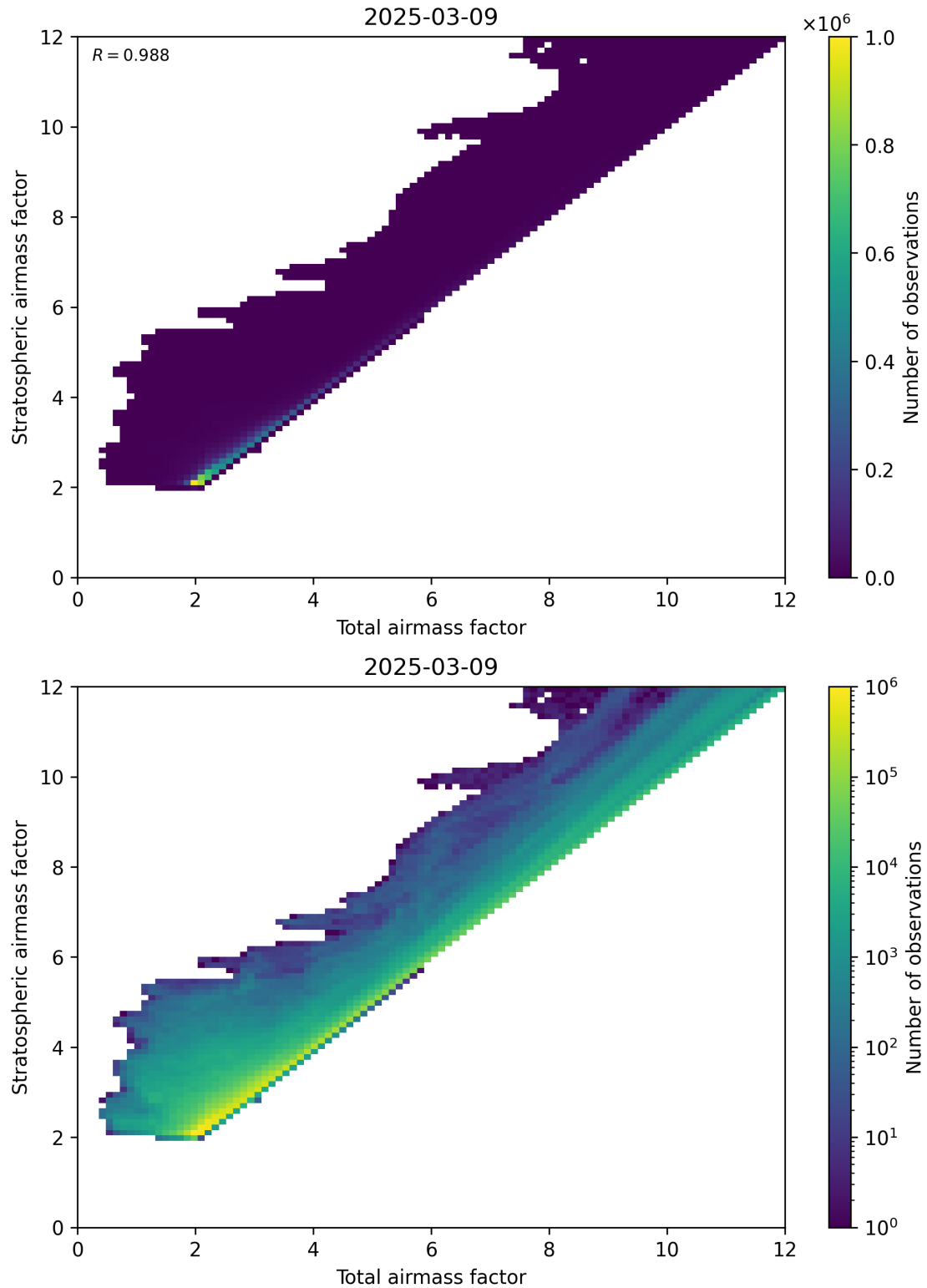
Figure 62: Scatter density plot of “Total airmass factor” against “Stratospheric airmass factor” for 2025-03-09 to 2025-03-10.
