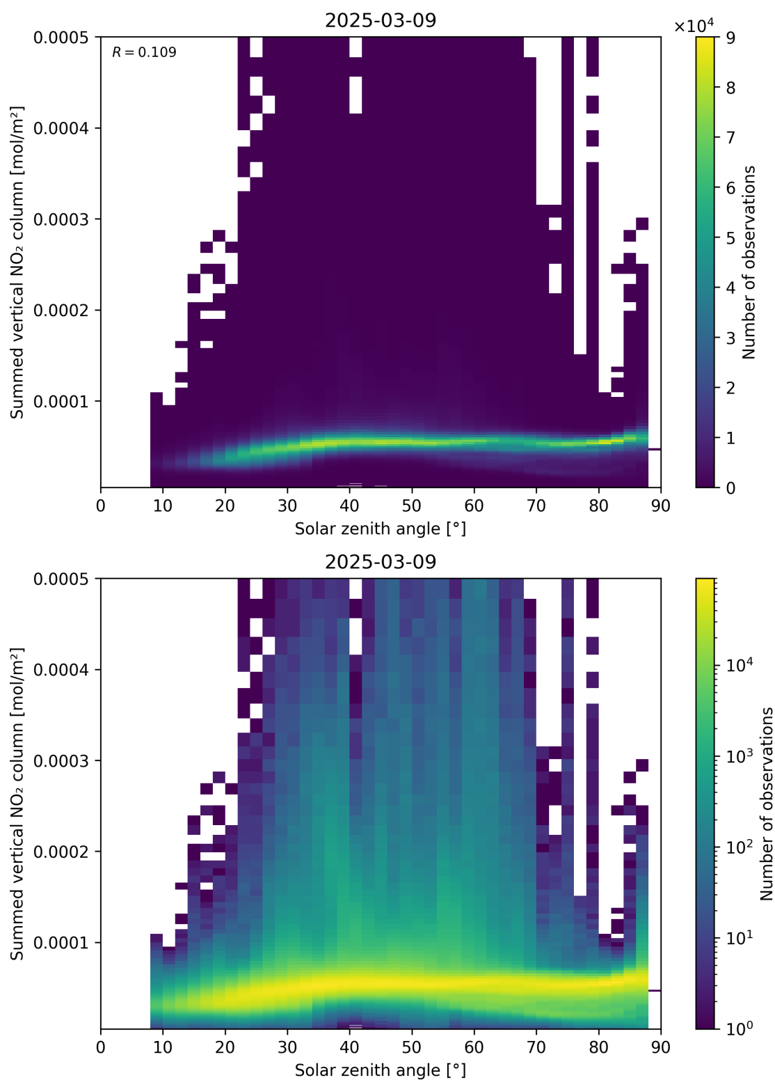
Figure 151: Scatter density plot of “Solar zenith angle” against “Summed vertical NO 2 column” for 2025-03-09 to 2025-03-10.
