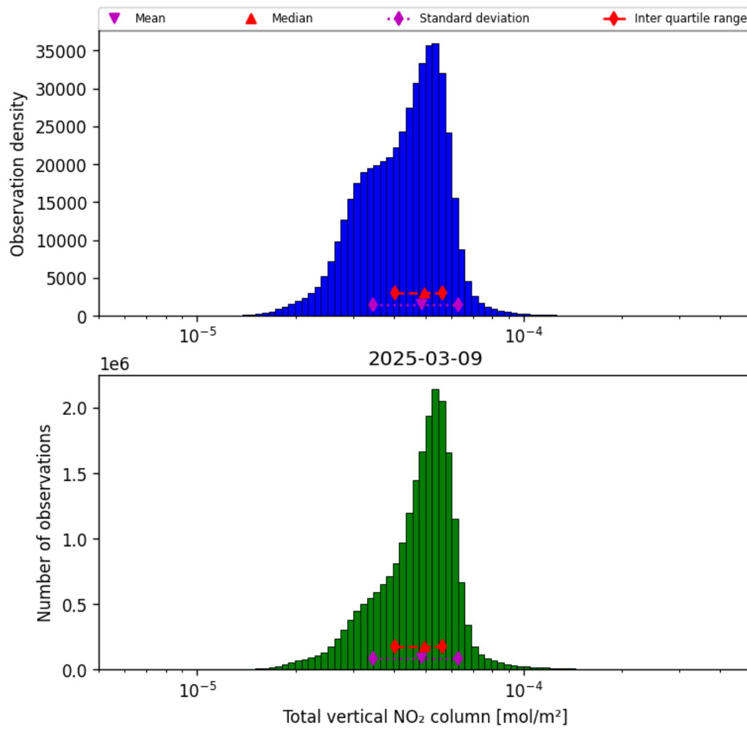
Figure 38: Histogram of “Total vertical NO 2 column” for 2025-03-09 to 2025-03-10
