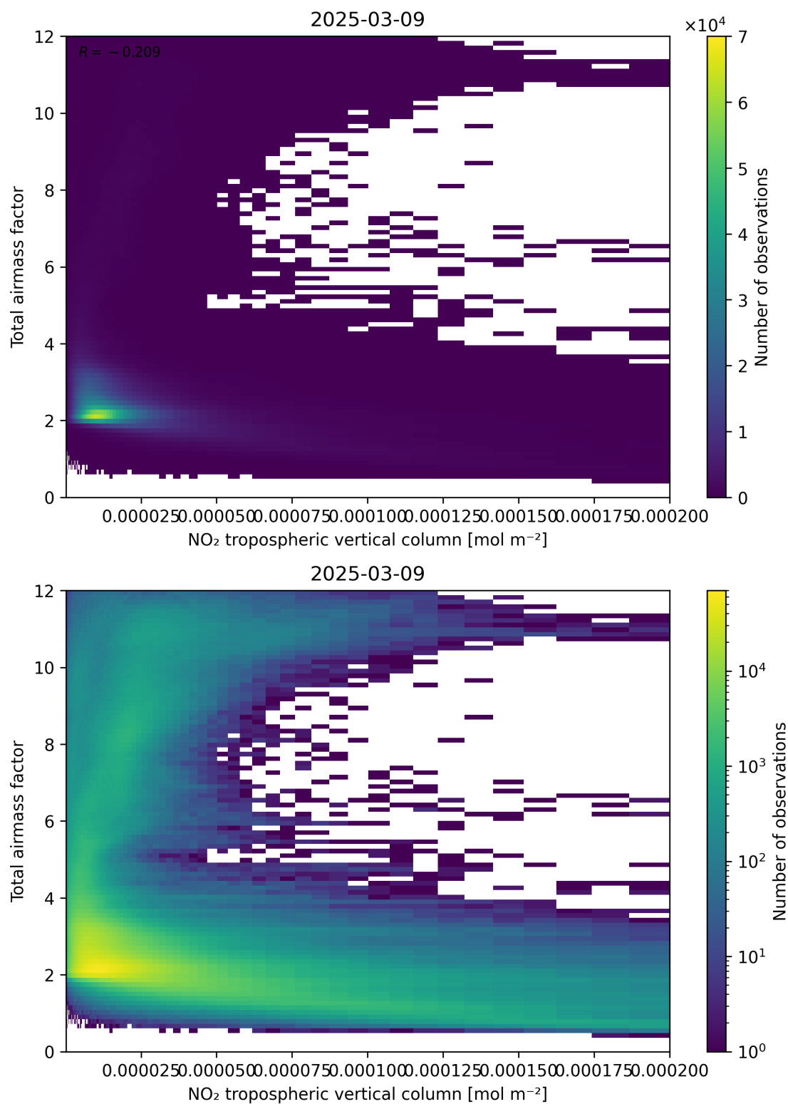
Figure 122: Scatter density plot of “NO 2 tropospheric vertical column” against “Total air mass factor” for 2025-03-09 to 2025-03-10.
