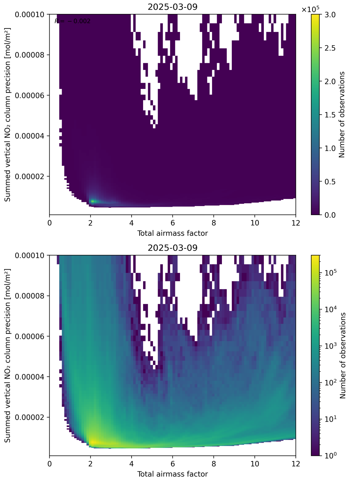
Figure 66: Scatter density plot of “Total airmass factor” against “Summed vertical NO 2 column precision” for 2025-03-09 to 2025-03-10.
