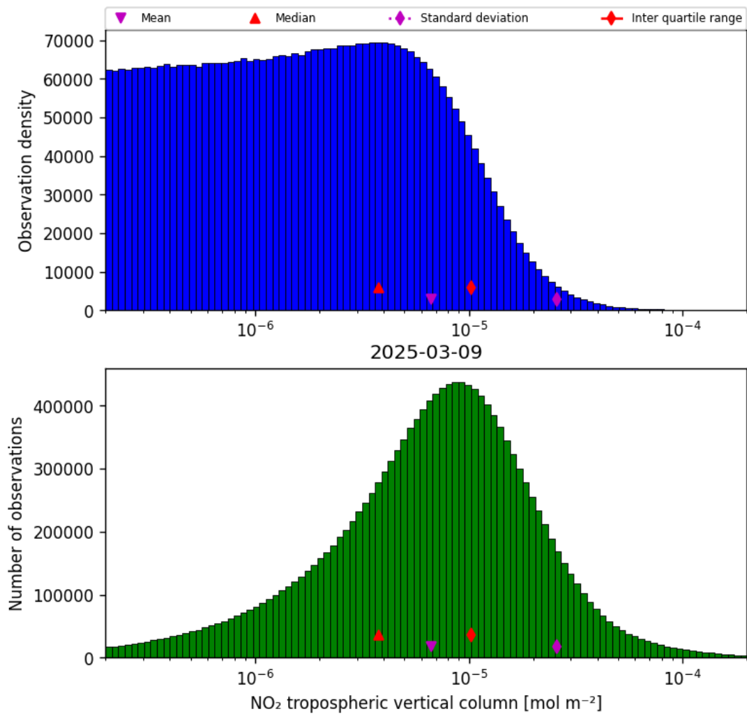
Figure 29: Histogram of “NO 2 tropospheric vertical column” for 2025-03-09 to 2025-03-10
