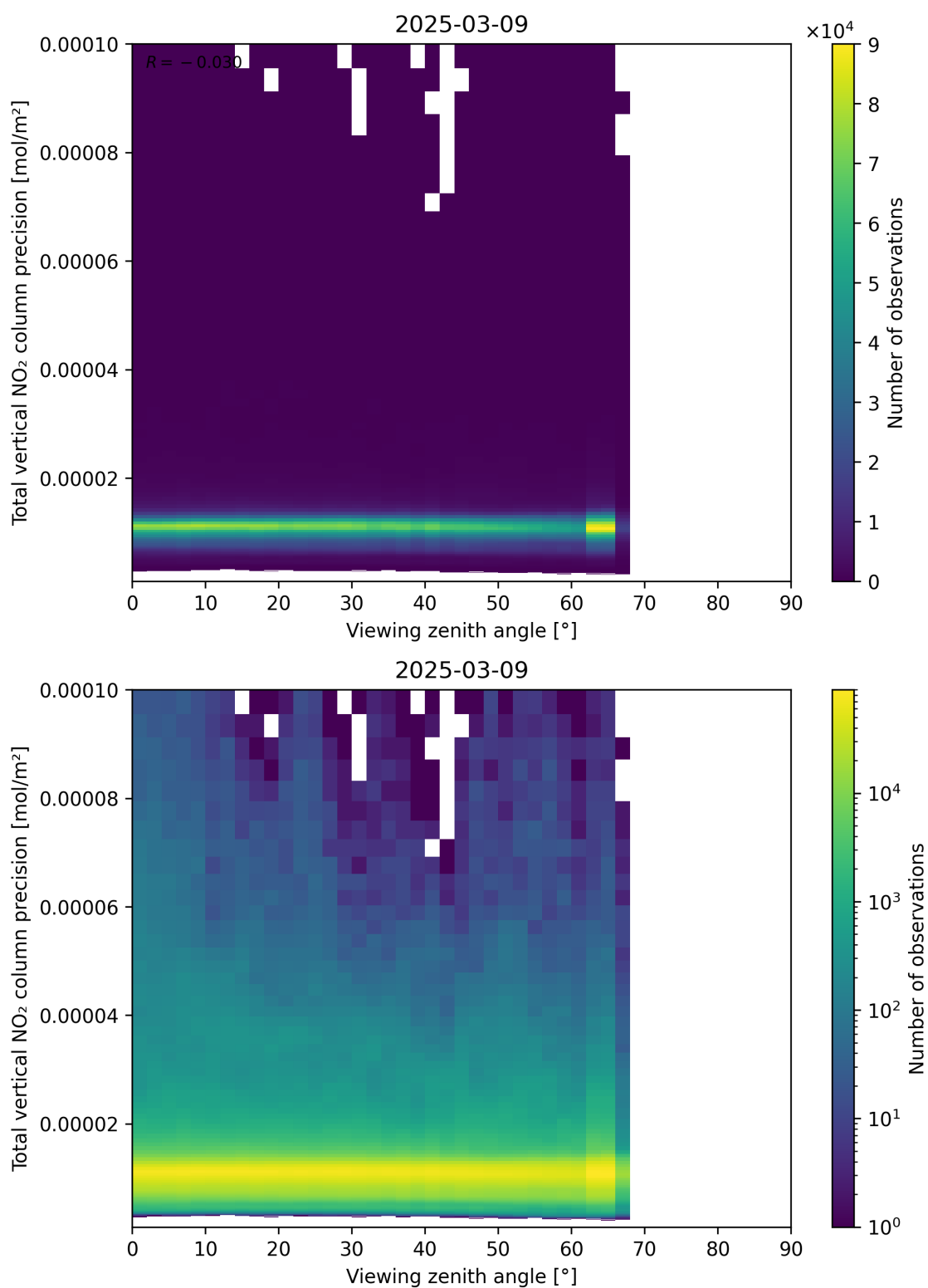
Figure 168: Scatter density plot of “Viewing zenith angle” against “Total vertical NO 2 column precision” for 2025-03-09 to 2025-03-10.
