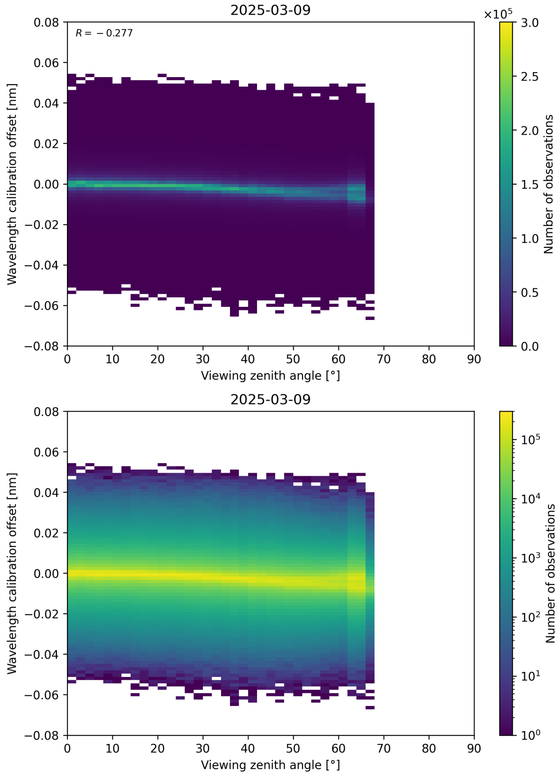
Figure 173: Scatter density plot of “Viewing zenith angle” against “Wavelength calibration offset” for 2025-03-09 to 2025-03-10.
