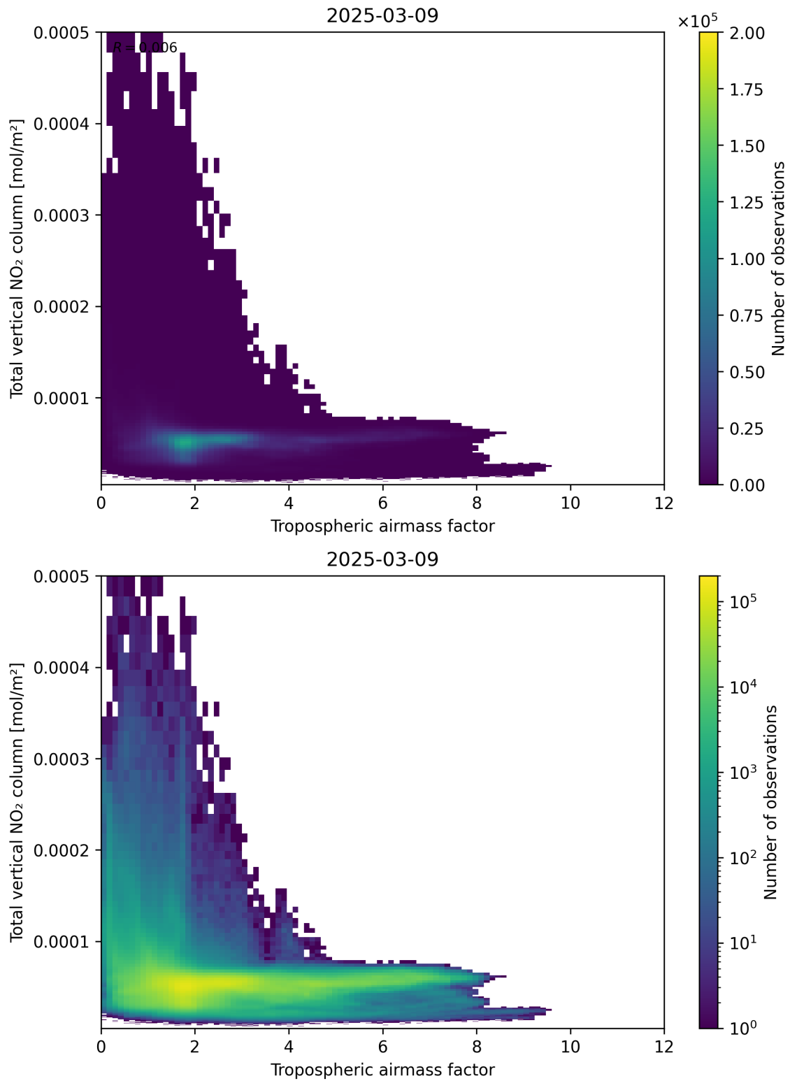
Figure 77: Scatter density plot of “Tropospheric airmass factor” against “Total vertical NO 2 column” for 2025-03-09 to 2025-03-10.
