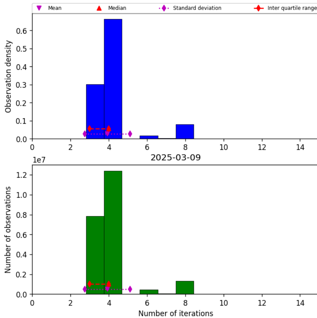
Figure 34: Histogram of “Number of iterations” for 2025-03-09 to 2025-03-10
