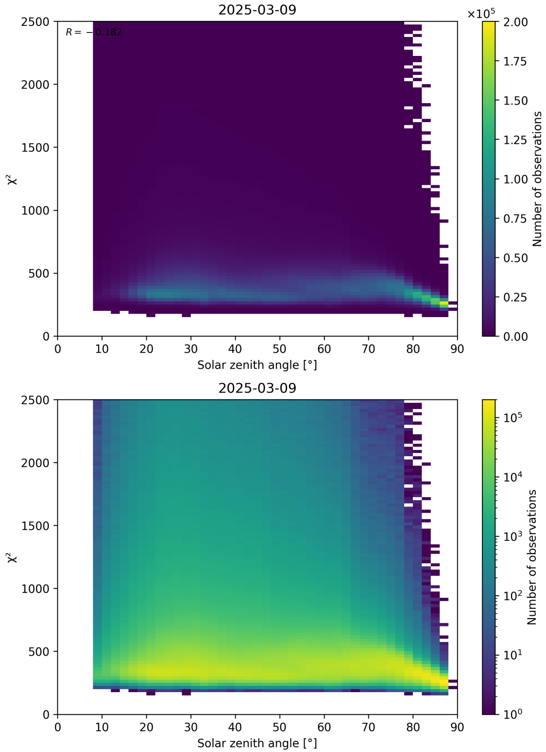
Figure 148: Scatter density plot of “Solar zenith angle” against “ \chi^2 ” for 2025-03-09 to 2025-03-10.
