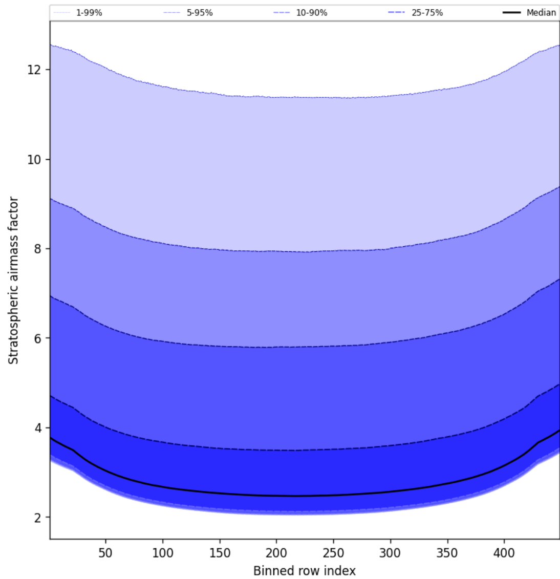
Figure 61: Along track statistics of “Stratospheric airmass factor” for 2025-03-09 to 2025-03-10
