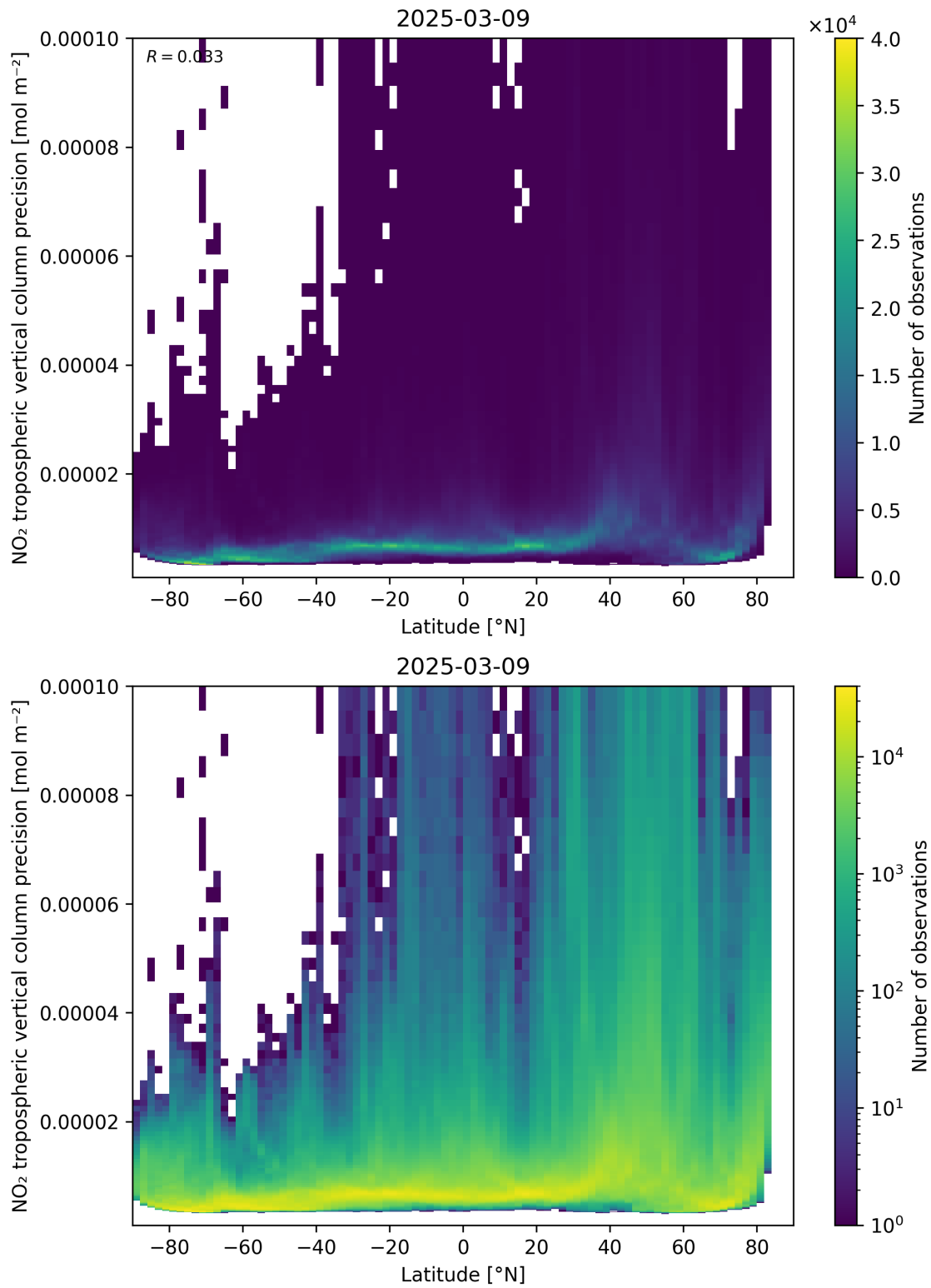
Figure 93: Scatter density plot of “Latitude” against “NO 2 tropospheric vertical column precision” for 2025-03-09 to 2025-03-10.
