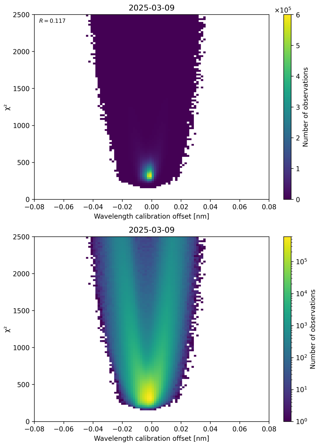
Figure 175: Scatter density plot of “Wavelength calibration offset” against “ \chi^2 ” for 2025-03-09 to 2025-03-10.
