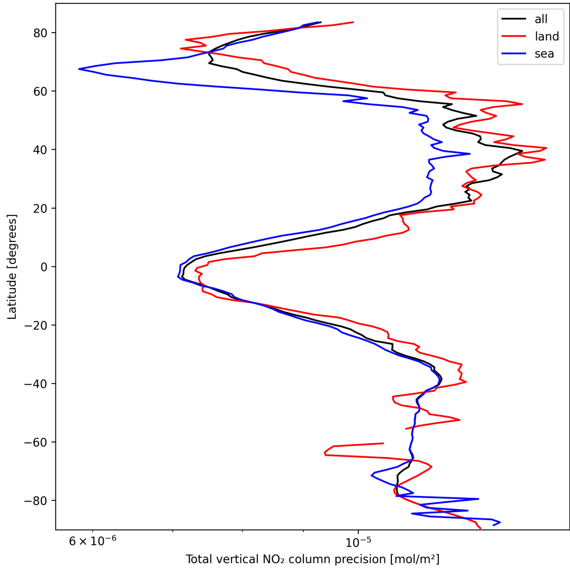
Figure 22: Zonal average of “Total vertical NO 2 column precision” for 2025-03-09 to 2025-03-10.
