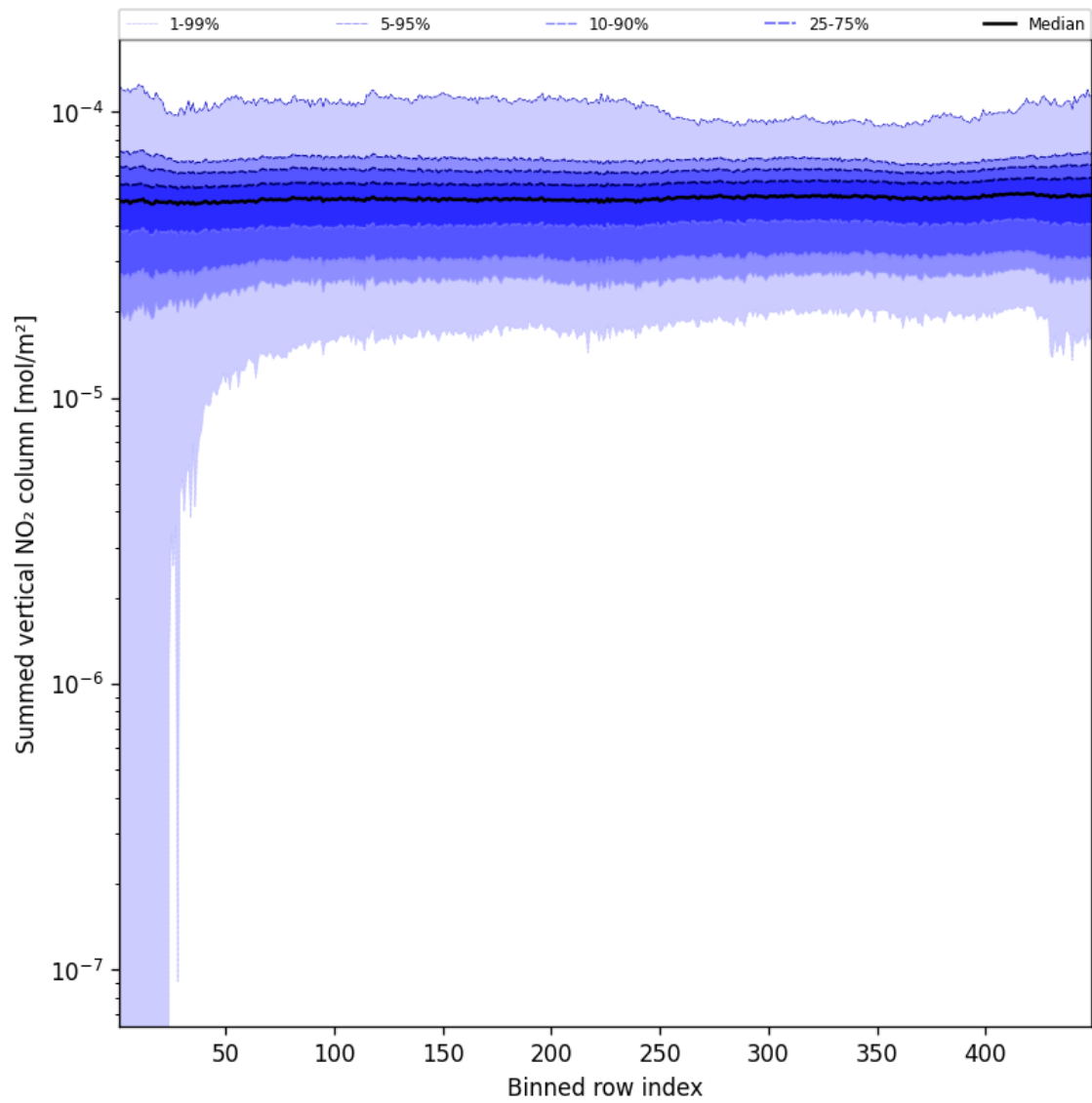
Figure 57: Along track statistics of “Summed vertical NO 2 column” for 2025-03-09 to 2025-03-10
