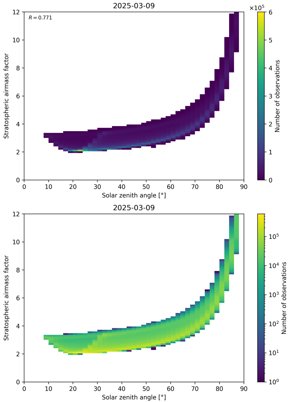
Figure 145: Scatter density plot of “Solar zenith angle” against “Stratospheric airmass factor” for 2025-03-09 to 2025-03-10.
