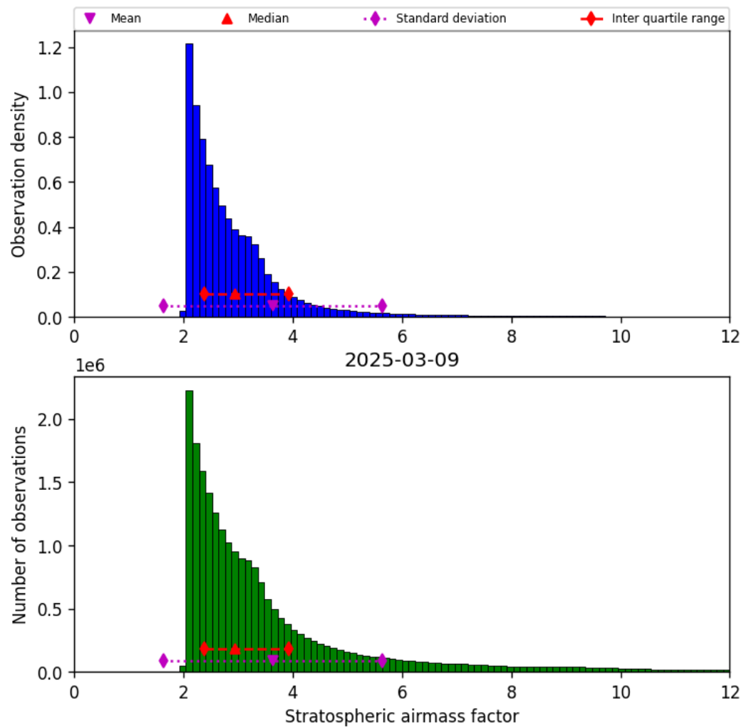
Figure 44: Histogram of “Stratospheric airmass factor” for 2025-03-09 to 2025-03-10
