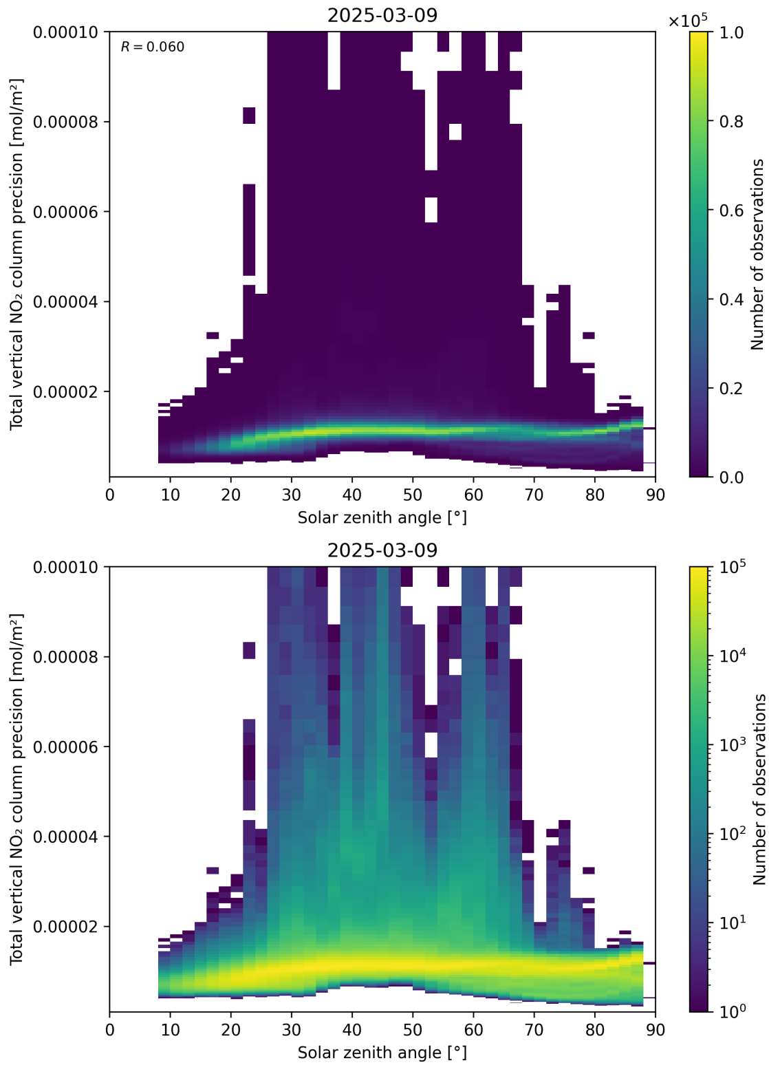
Figure 154: Scatter density plot of “Solar zenith angle” against “Total vertical NO 2 column precision” for 2025-03-09 to 2025-03-10.
