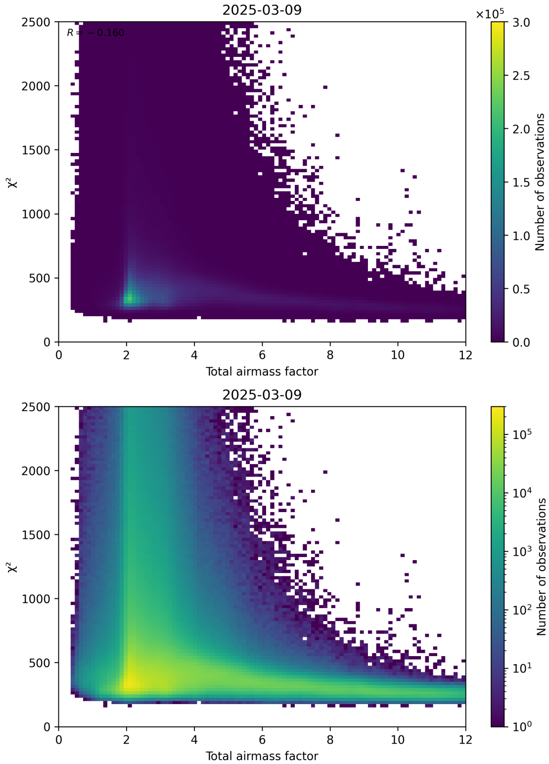
Figure 63: Scatter density plot of “Total airmass factor” against “ \chi^2 ” for 2025-03-09 to 2025-03-10.
