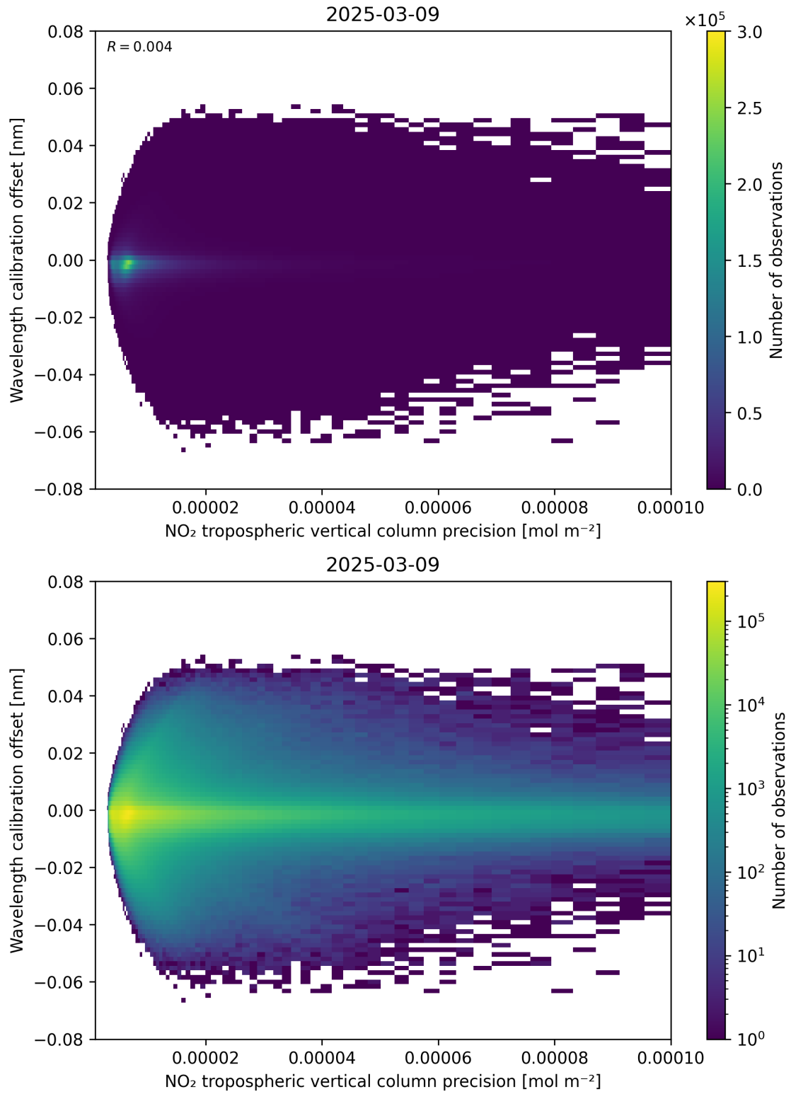
Figure 141: Scatter density plot of “NO 2 tropospheric vertical column precision” against “Wavelength calibration offset” for 2025-03-09 to 2025-03-10.
