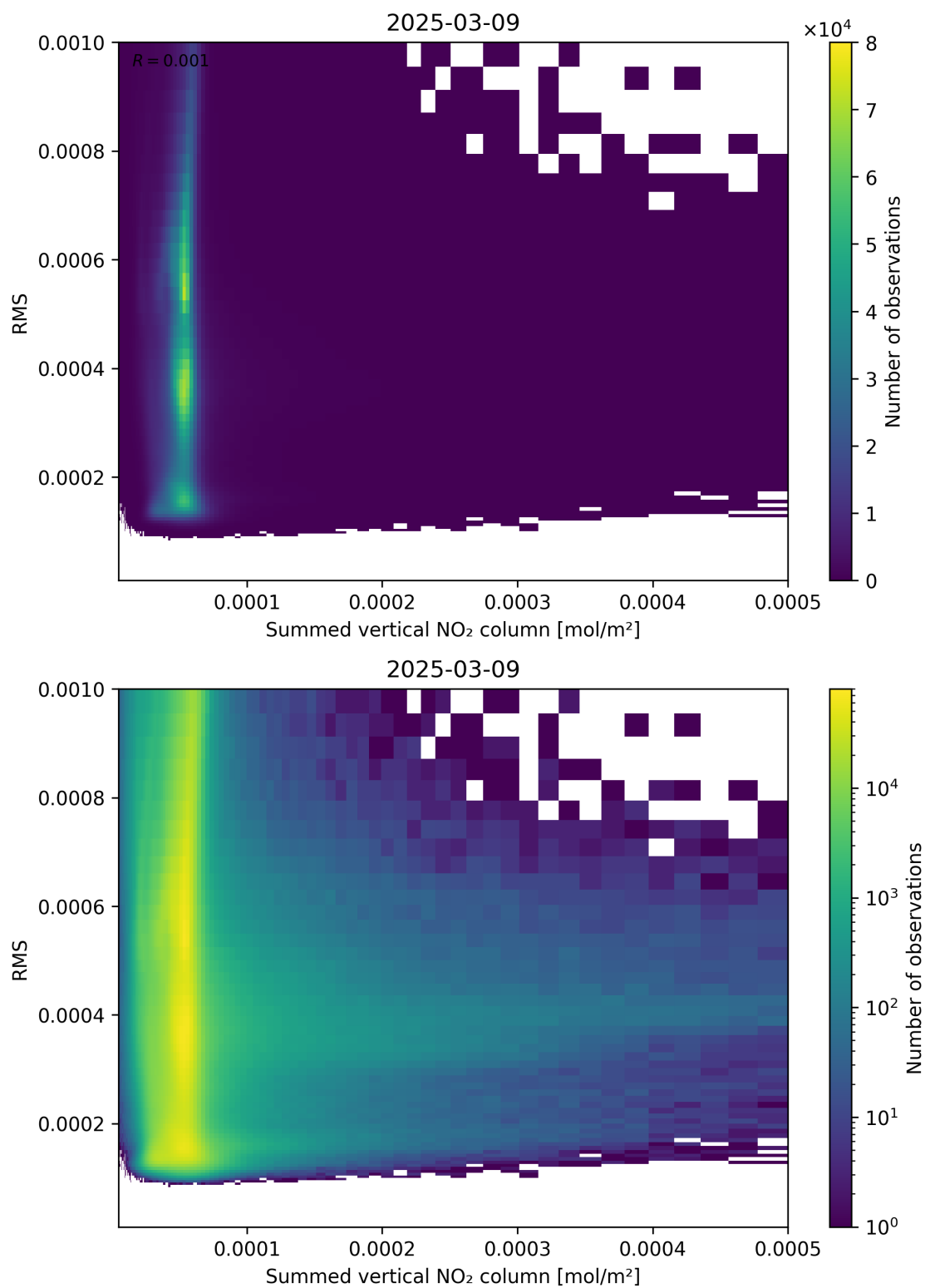
Figure 109: Scatter density plot of “Summed vertical NO 2 column” against “RMS” for 2025-03-09 to 2025-03-10.
