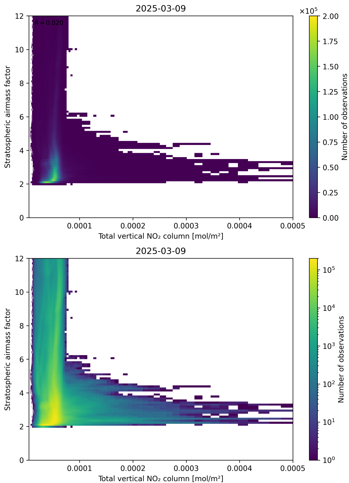
Figure 110: Scatter density plot of “Total vertical NO 2 column” against “Stratospheric airmass factor” for 2025-03-09 to 2025-03-10.
