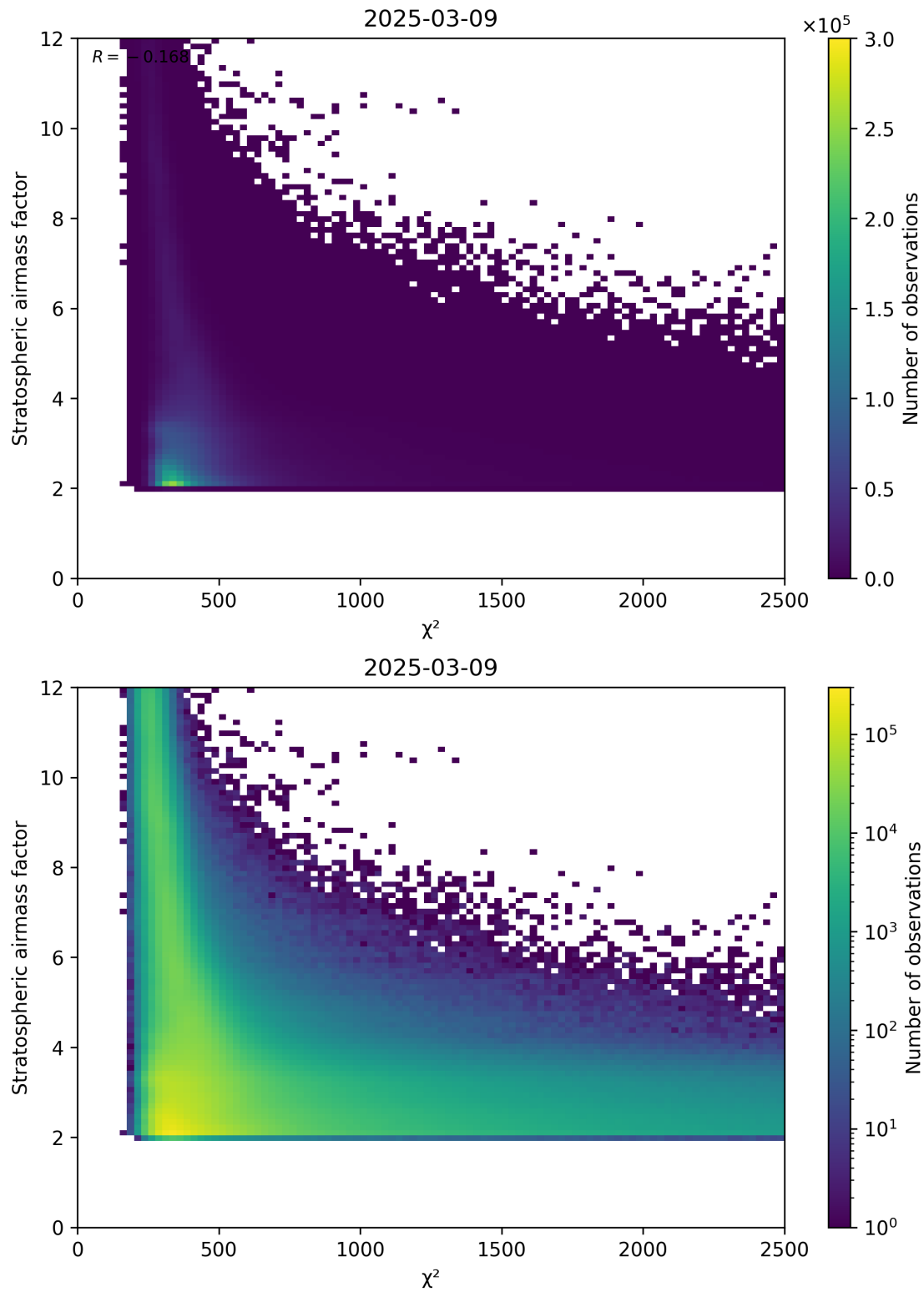
Figure 81: Scatter density plot of “ \chi^2 ” against “Stratospheric airmass factor” for 2025-03-09 to 2025-03-10.
