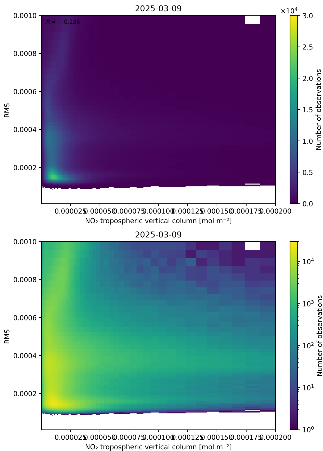
Figure 142: Scatter density plot of “NO 2 tropospheric vertical column” against “RMS” for 2025-03-09 to 2025-03-10.
