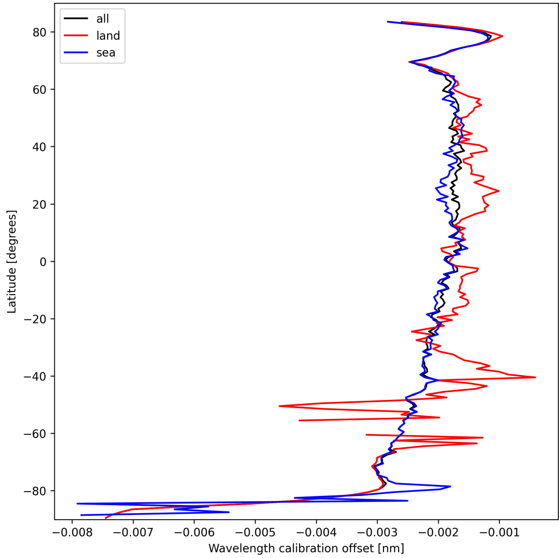
Figure 18: Zonal average of “Wavelength calibration offset” for 2025-03-09 to 2025-03-10.
