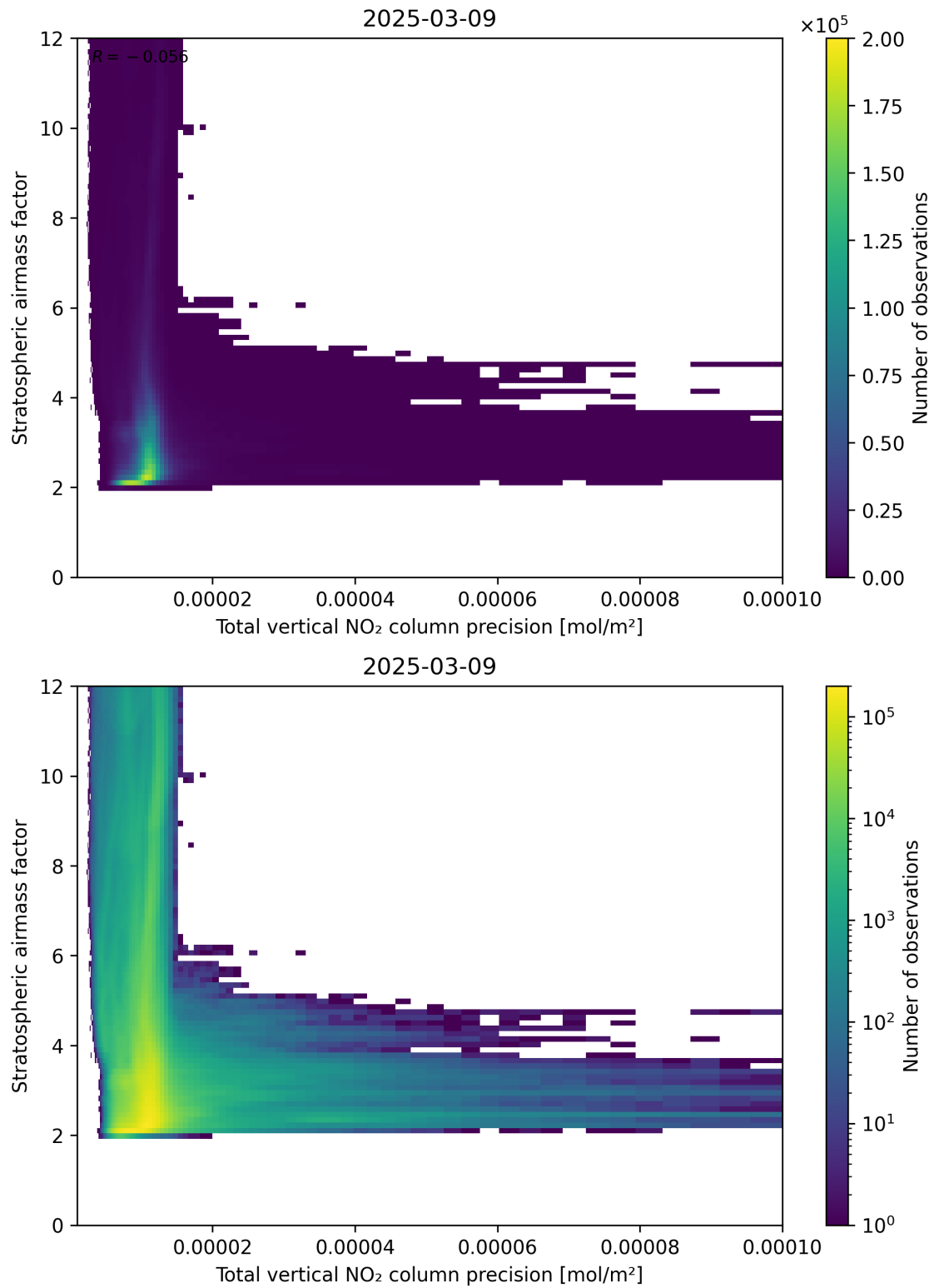
Figure 115: Scatter density plot of “Total vertical NO 2 column precision” against “Stratospheric air mass factor” for 2025-03-09 to 2025-03-10.
