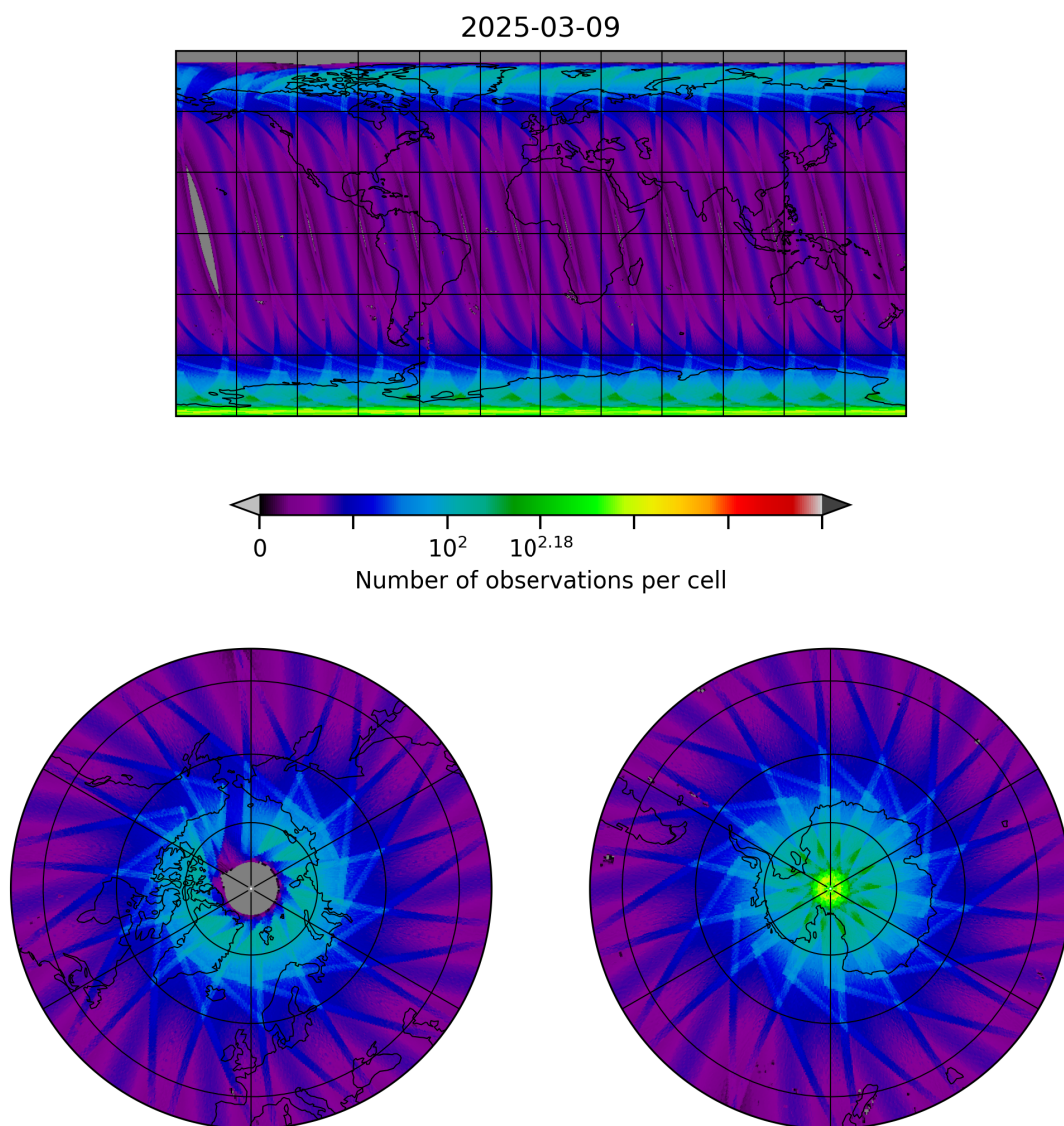
Figure 10: Map of the number of observations for 2025-03-09 to 2025-03-10
