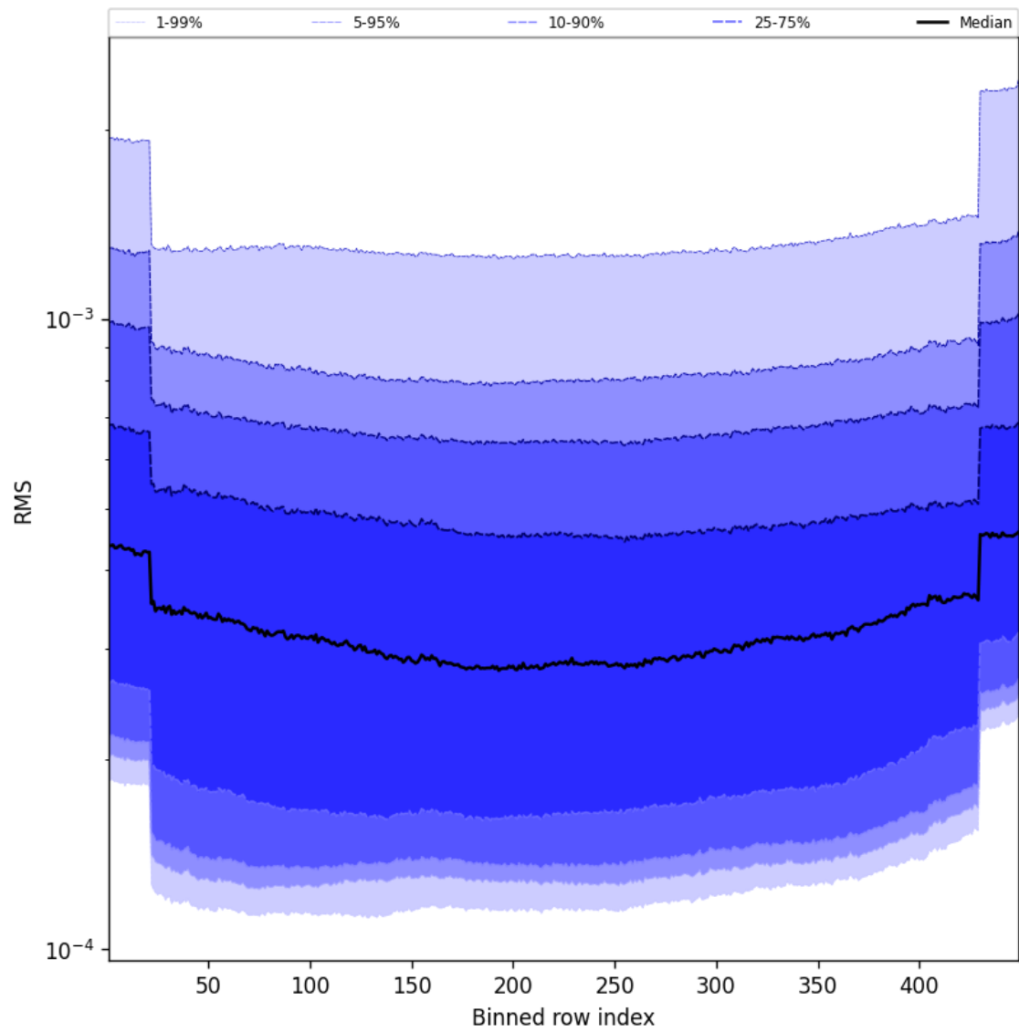
Figure 60: Along track statistics of “RMS” for 2025-03-09 to 2025-03-10
