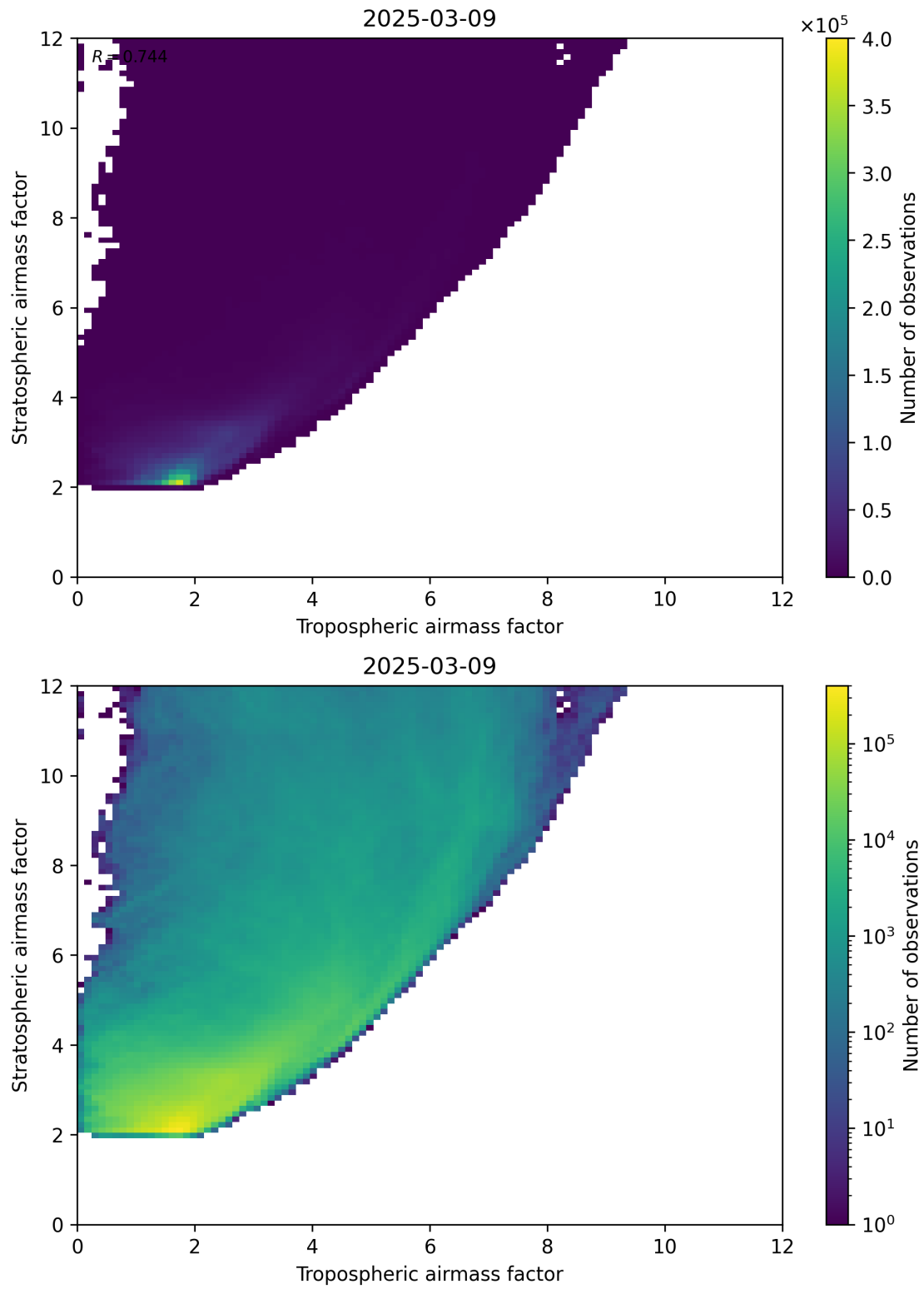
Figure 71: Scatter density plot of “Tropospheric airmass factor” against “Stratospheric airmass factor” for 2025-03-09 to 2025-03-10.
