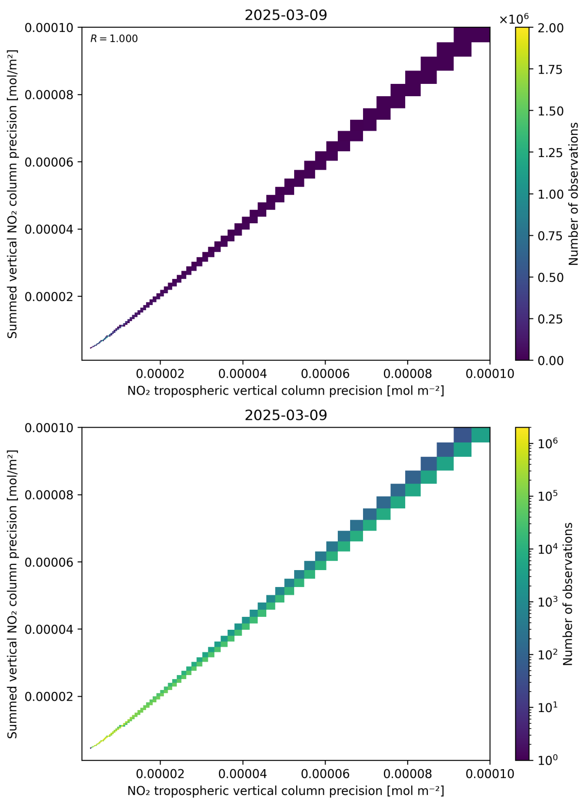
Figure 137: Scatter density plot of “NO 2 tropospheric vertical column precision” against “Summed vertical NO 2 column precision” for 2025-03-09 to 2025-03-10.
