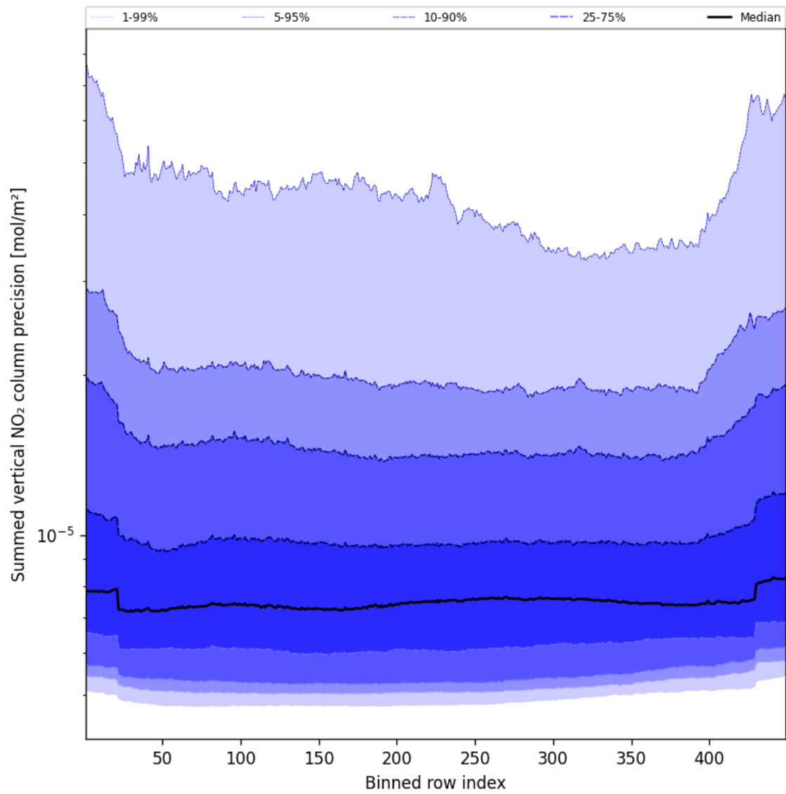
Figure 58: Along track statistics of “Summed vertical NO 2 column precision” for 2025-03-09 to 2025-03-10
