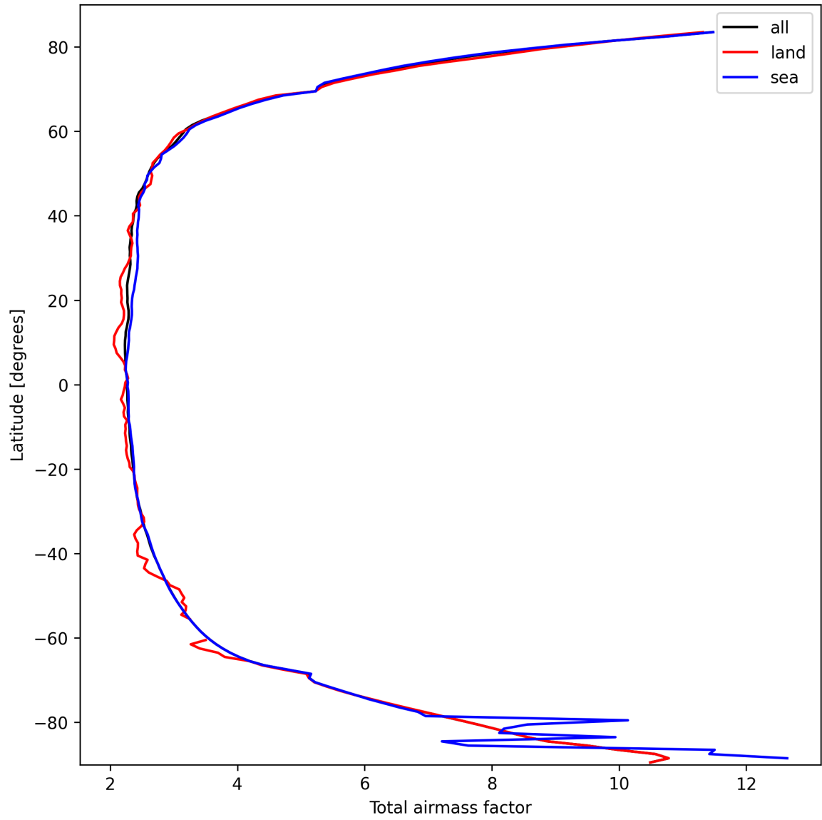
Figure 15: Zonal average of “Total airmass factor” for 2025-03-09 to 2025-03-10.
