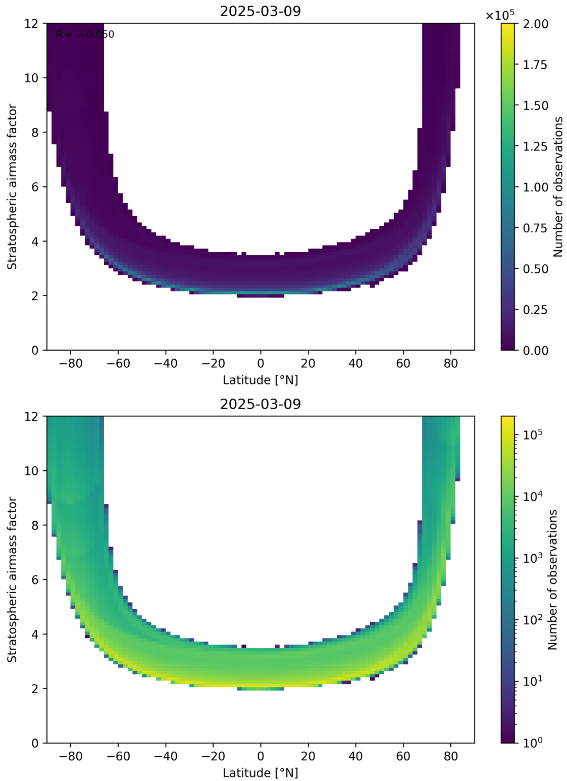
Figure 83: Scatter density plot of “Latitude” against “Stratospheric airmass factor” for 2025-03-09 to 2025-03-10.
