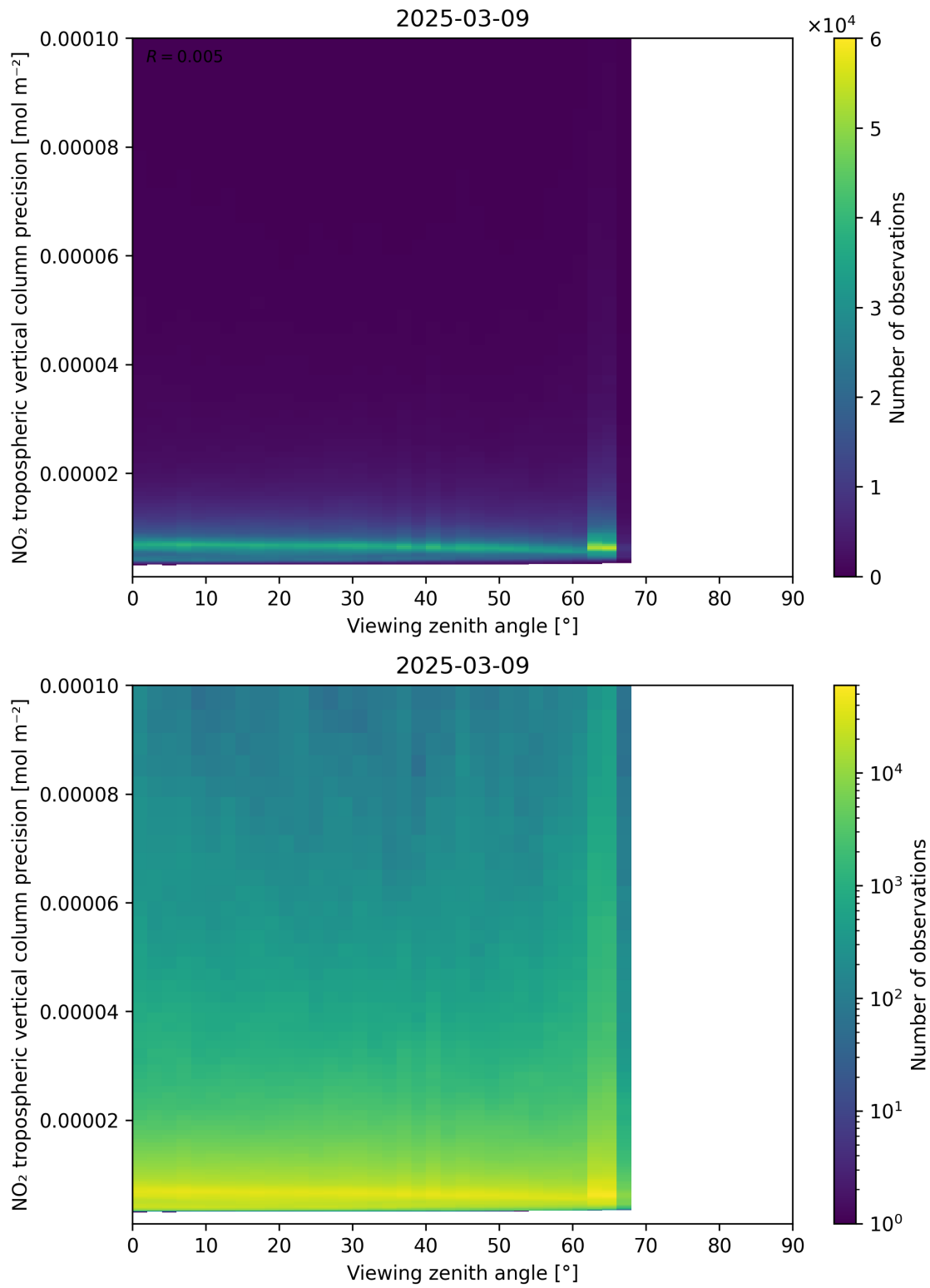
Figure 170: Scatter density plot of “Viewing zenith angle” against “NO 2 tropospheric vertical column precision” for 2025-03-09 to 2025-03-10.
