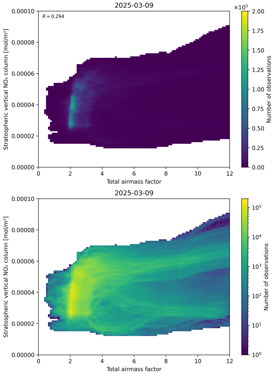
Figure 64: Scatter density plot of “Total airmass factor” against “Stratospheric vertical \text{NO}_2 column” for 2025-03-09 to 2025-03-10.
