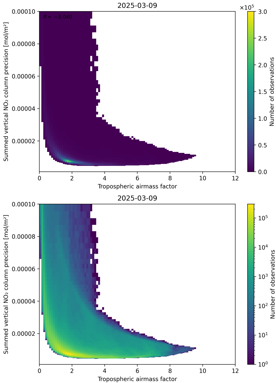
Figure 76: Scatter density plot of “Tropospheric air mass factor” against “Summed vertical NO 2 column precision” for 2025-03-09 to 2025-03-10.
