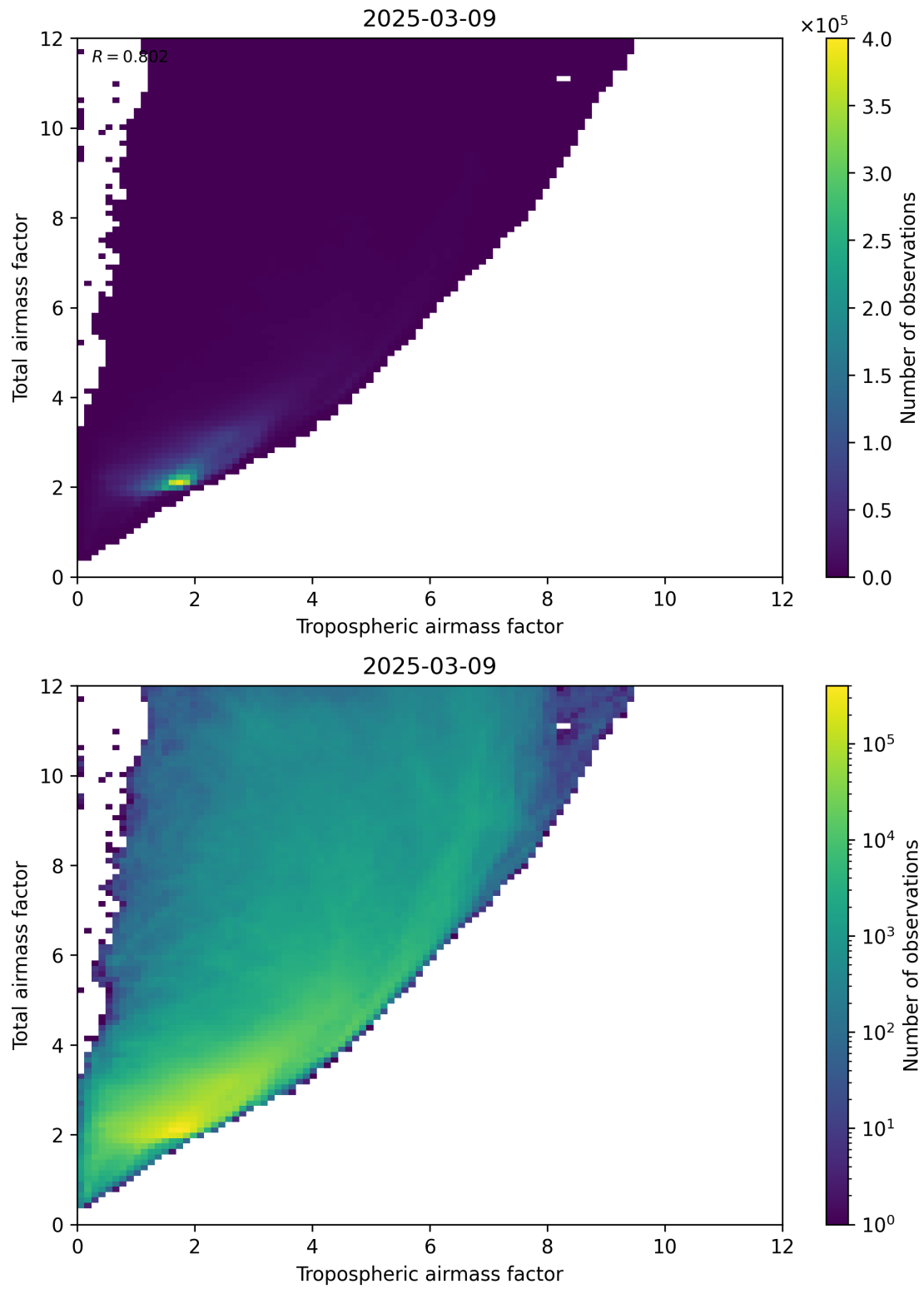
Figure 72: Scatter density plot of “Tropospheric airmass factor” against “Total airmass factor” for 2025-03-09 to 2025-03-10.
