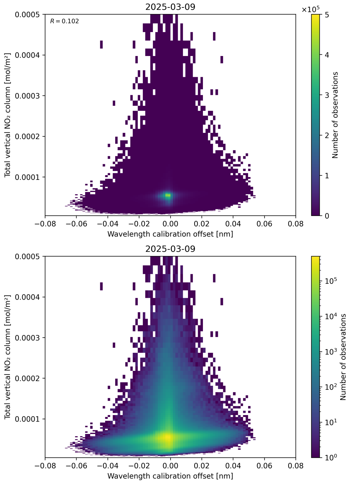
Figure 179: Scatter density plot of “Wavelength calibration offset” against “Total vertical NO 2 column” for 2025-03-09 to 2025-03-10.
