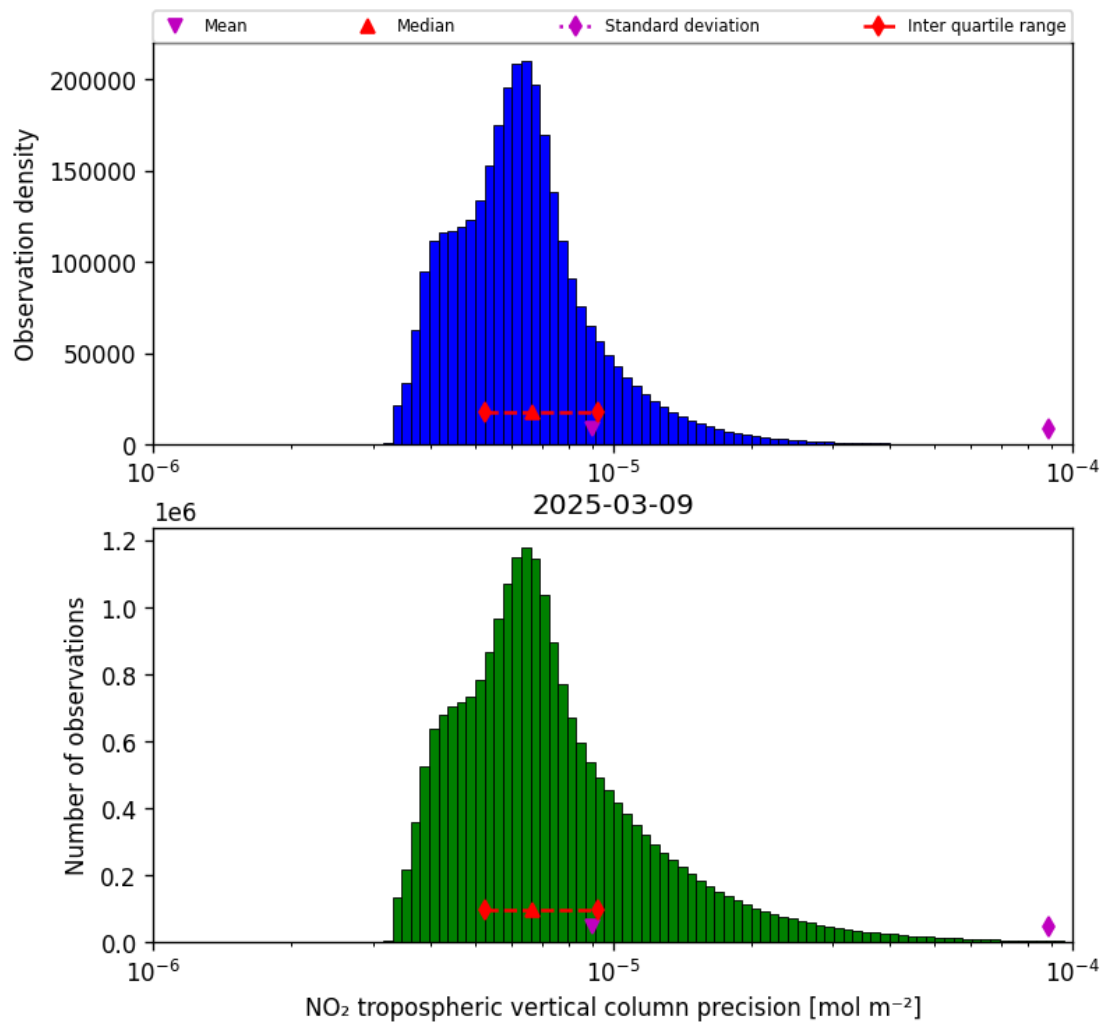
Figure 30: Histogram of “NO 2 tropospheric vertical column precision” for 2025-03-09 to 2025-03-10
