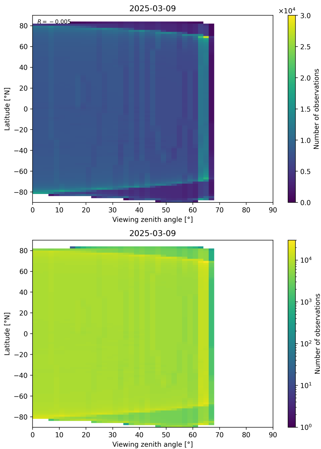
Figure 163: Scatter density plot of “Viewing zenith angle” against “Latitude” for 2025-03-09 to 2025-03-10.
