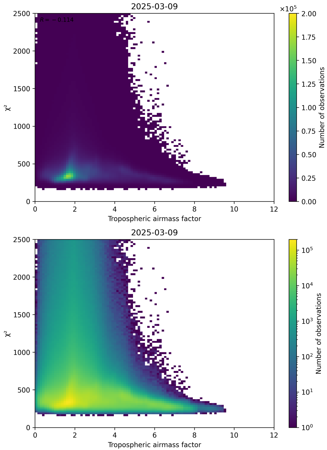
Figure 73: Scatter density plot of “Tropospheric airmass factor” against “ \chi^2 ” for 2025-03-09 to 2025-03-10.
