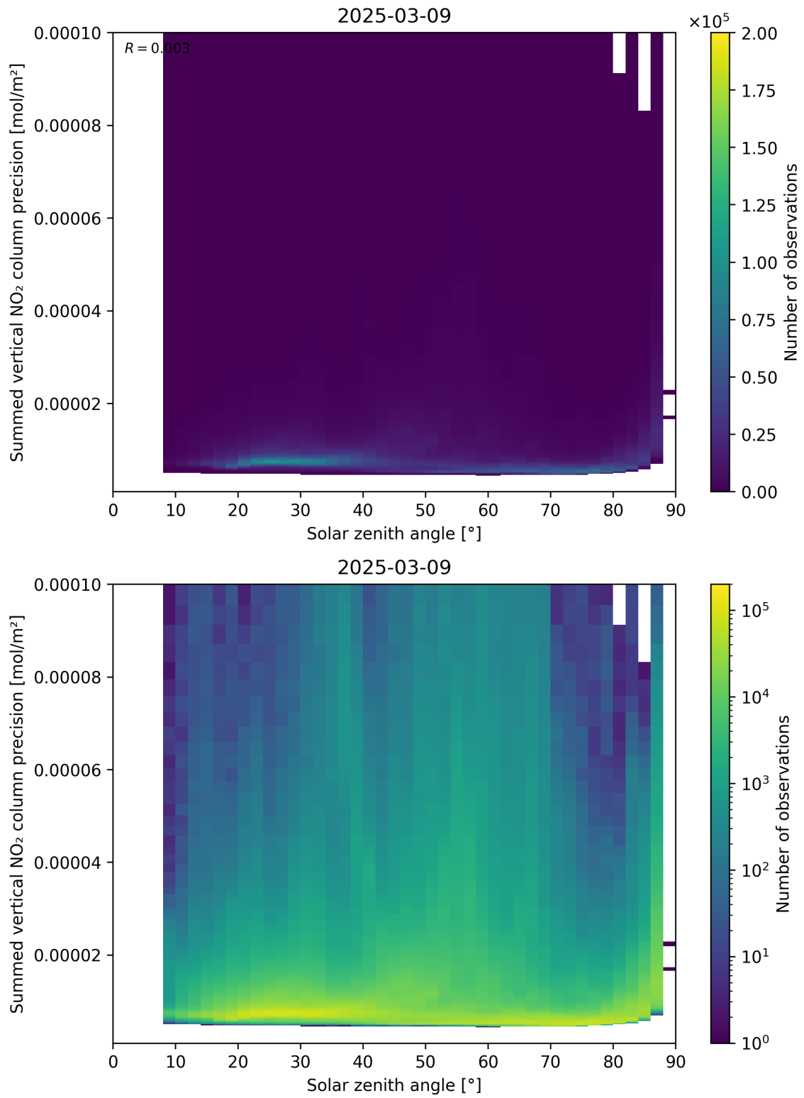
Figure 152: Scatter density plot of “Solar zenith angle” against “Summed vertical NO 2 column precision” for 2025-03-09 to 2025-03-10.
