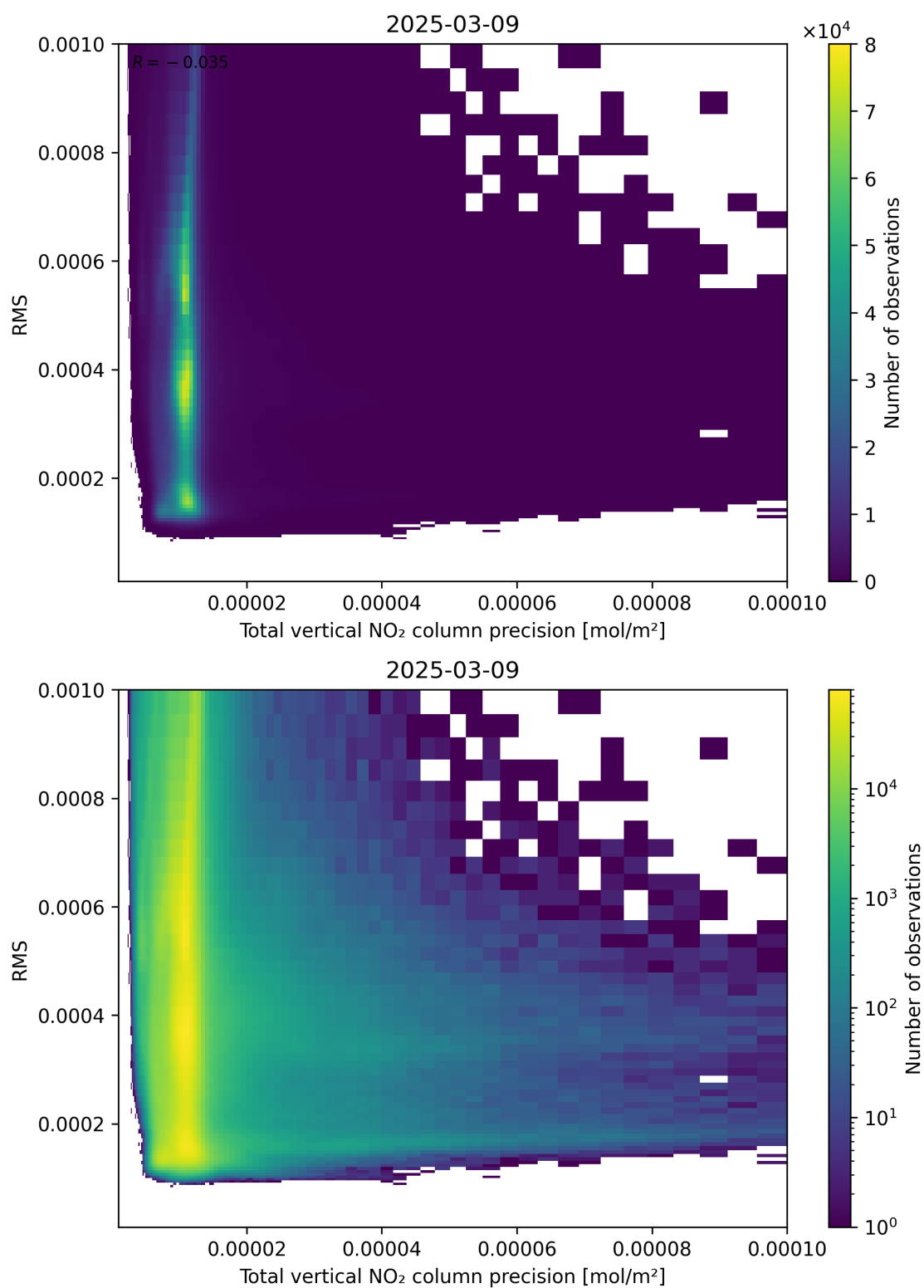
Figure 119: Scatter density plot of “Total vertical NO 2 column precision” against “RMS” for 2025-03-09 to 2025-03-10.
