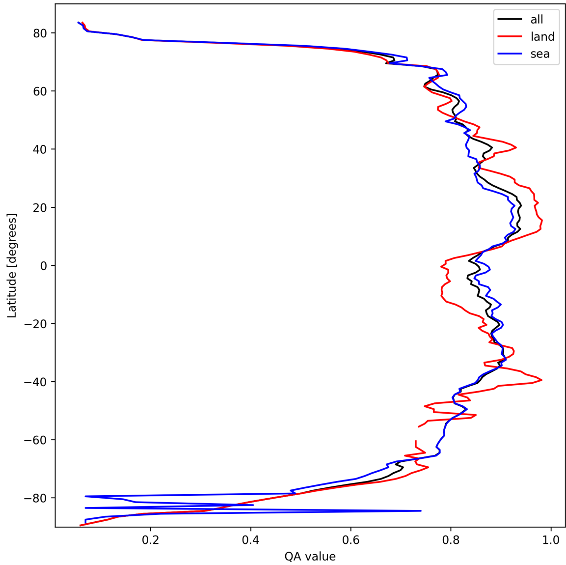
Figure 11: Zonal average of “QA value” for 2025-03-09 to 2025-03-10.
