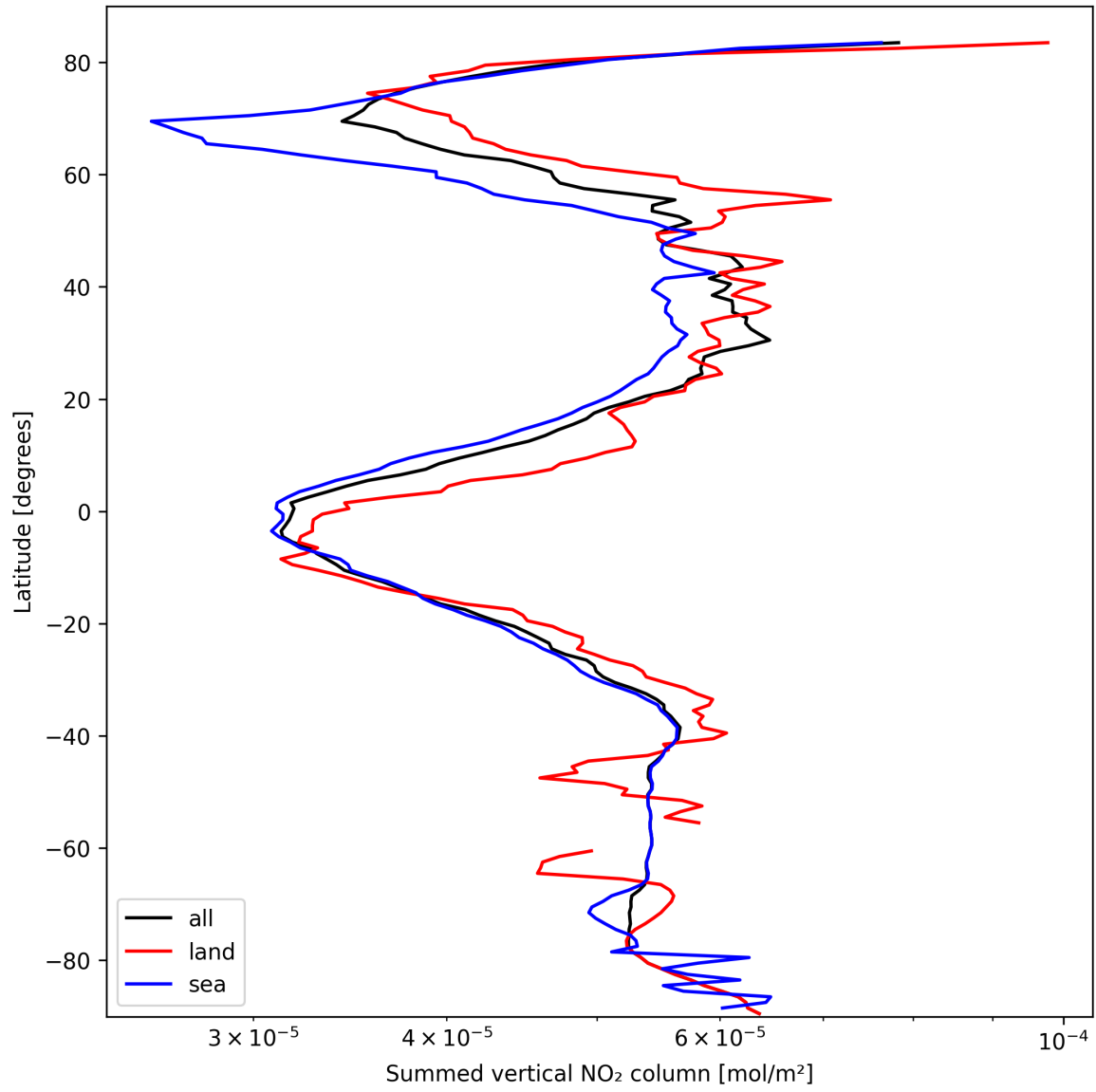
Figure 23: Zonal average of “Summed vertical NO 2 column” for 2025-03-09 to 2025-03-10.
