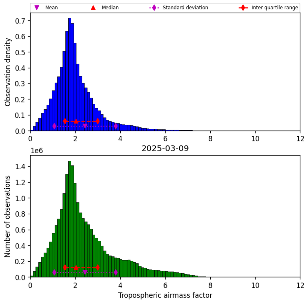
Figure 31: Histogram of “Tropospheric airmass factor” for 2025-03-09 to 2025-03-10
