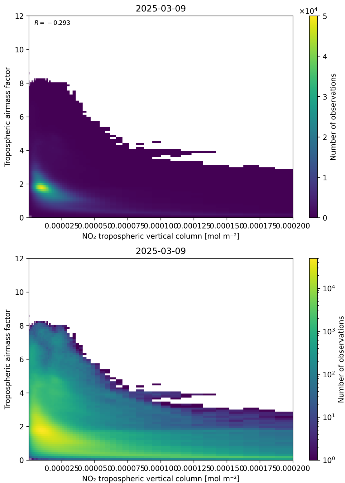
Figure 123: Scatter density plot of “NO 2 tropospheric vertical column” against “Tropospheric air mass factor” for 2025-03-09 to 2025-03-10.
