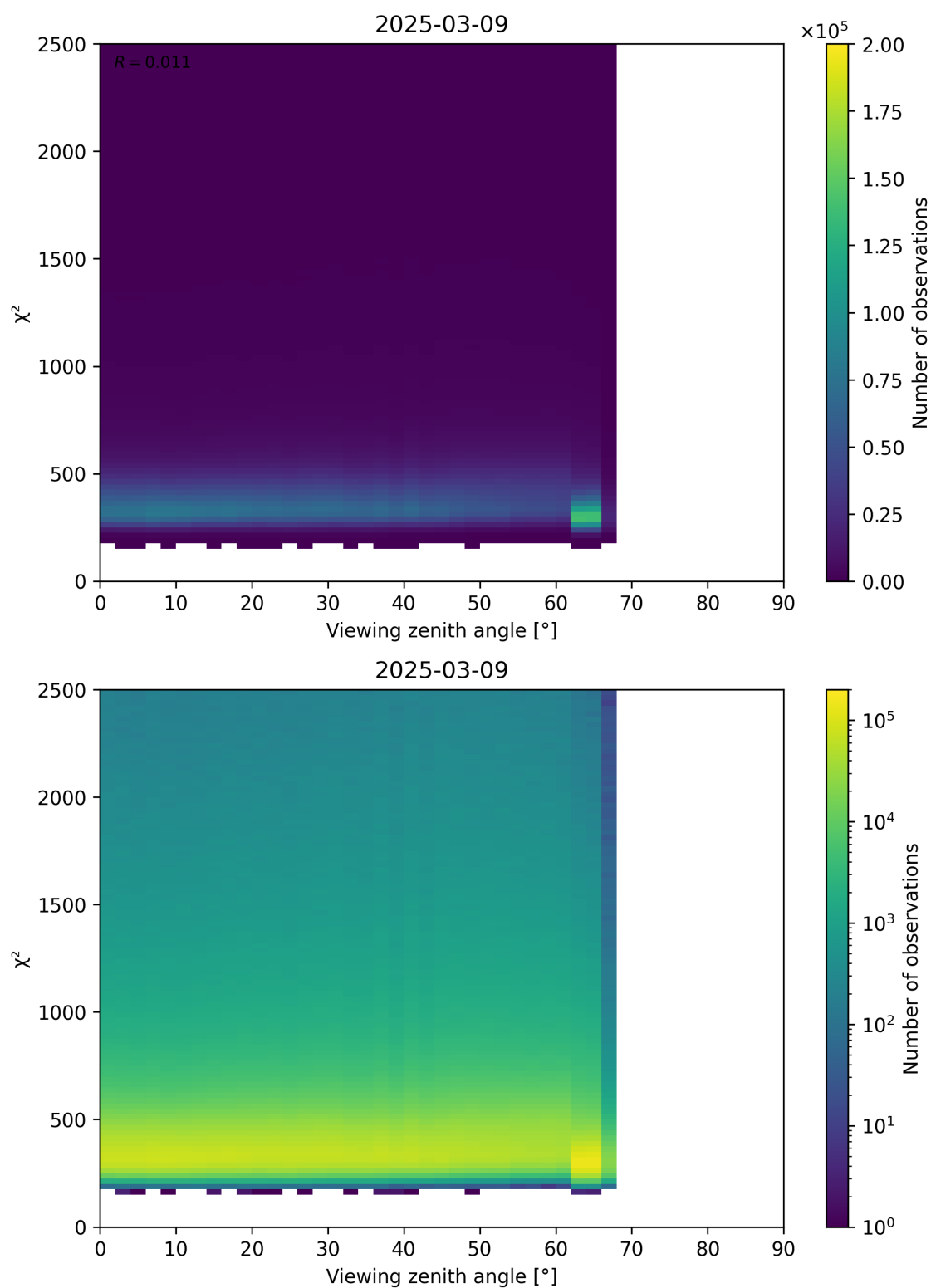
Figure 162: Scatter density plot of “Viewing zenith angle” against “ \chi^2 ” for 2025-03-09 to 2025-03-10.
