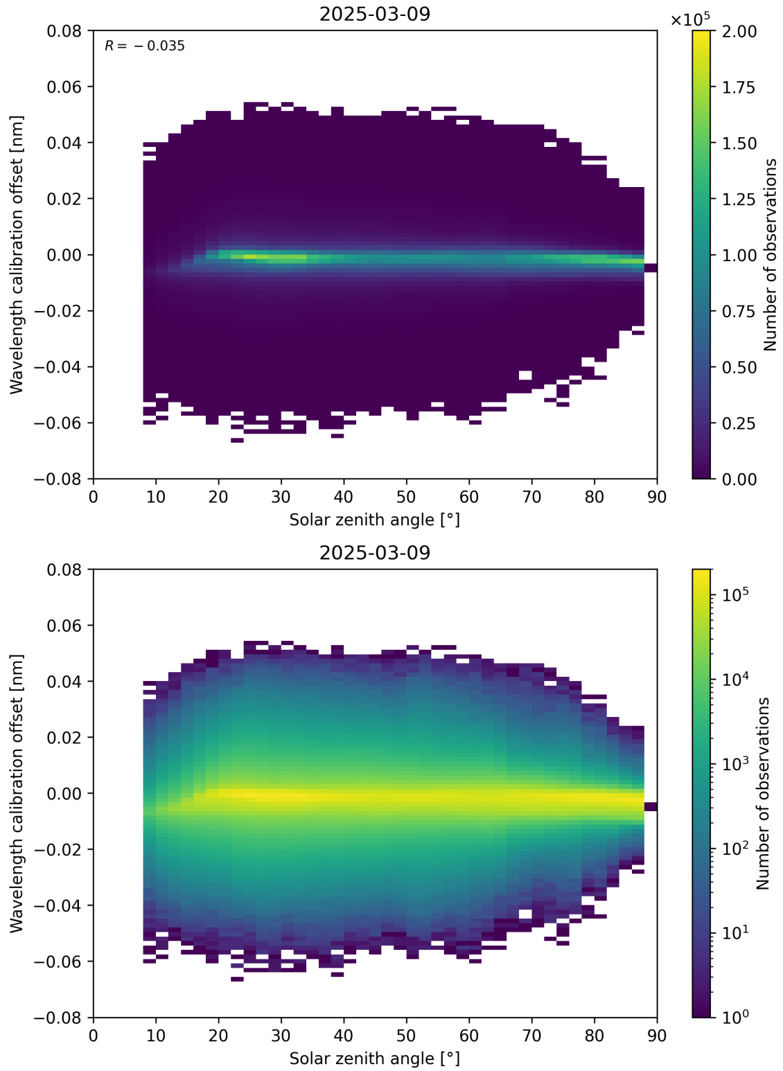
Figure 158: Scatter density plot of “Solar zenith angle” against “Wavelength calibration offset” for 2025-03-09 to 2025-03-10.
