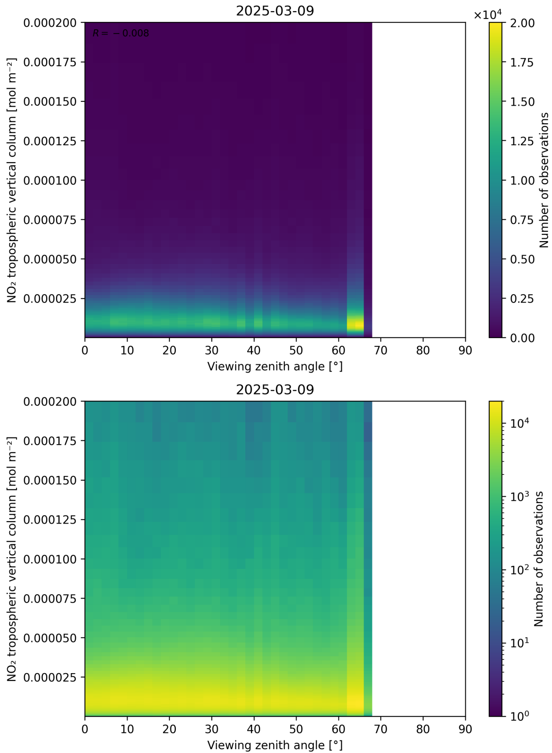
Figure 169: Scatter density plot of “Viewing zenith angle” against “NO 2 tropospheric vertical column” for 2025-03-09 to 2025-03-10.
