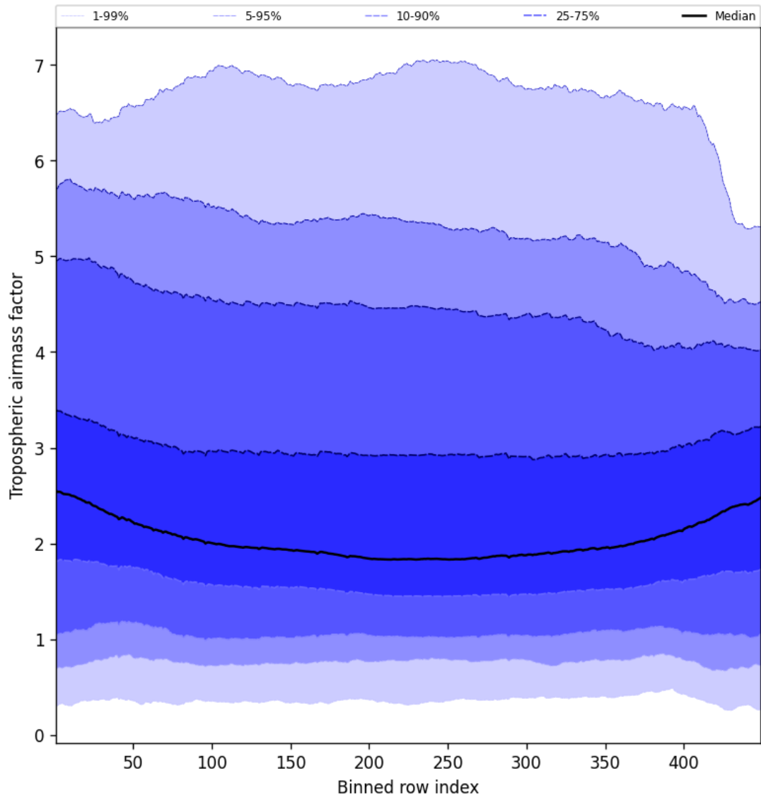
Figure 48: Along track statistics of “Tropospheric air mass factor” for 2025-03-09 to 2025-03-10
