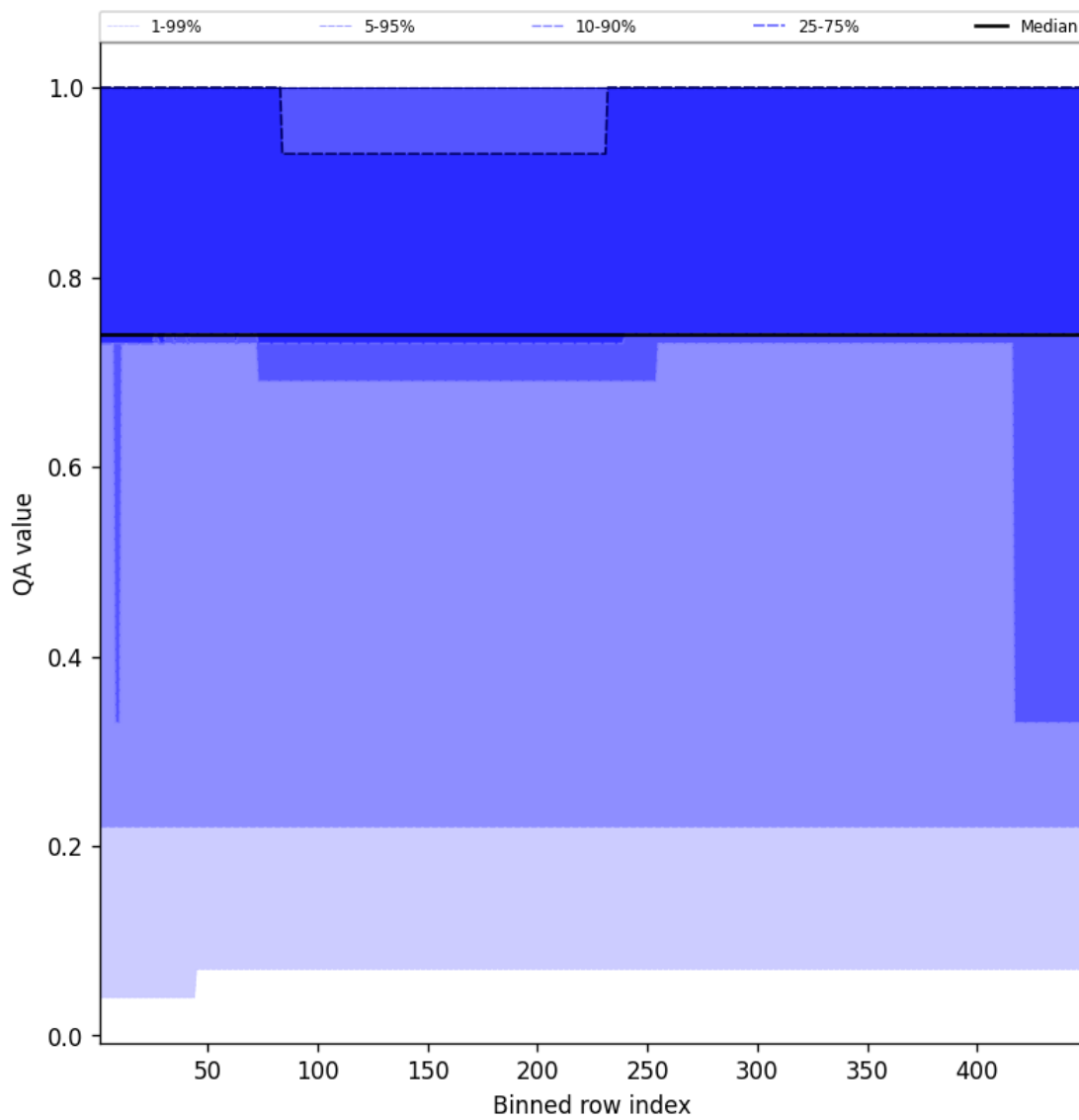
Figure 45: Along track statistics of “QA value” for 2025-03-09 to 2025-03-10
