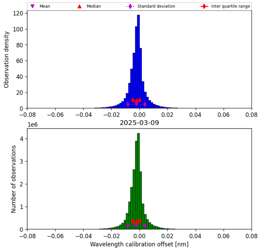
Figure 35: Histogram of “Wavelength calibration offset” for 2025-03-09 to 2025-03-10
