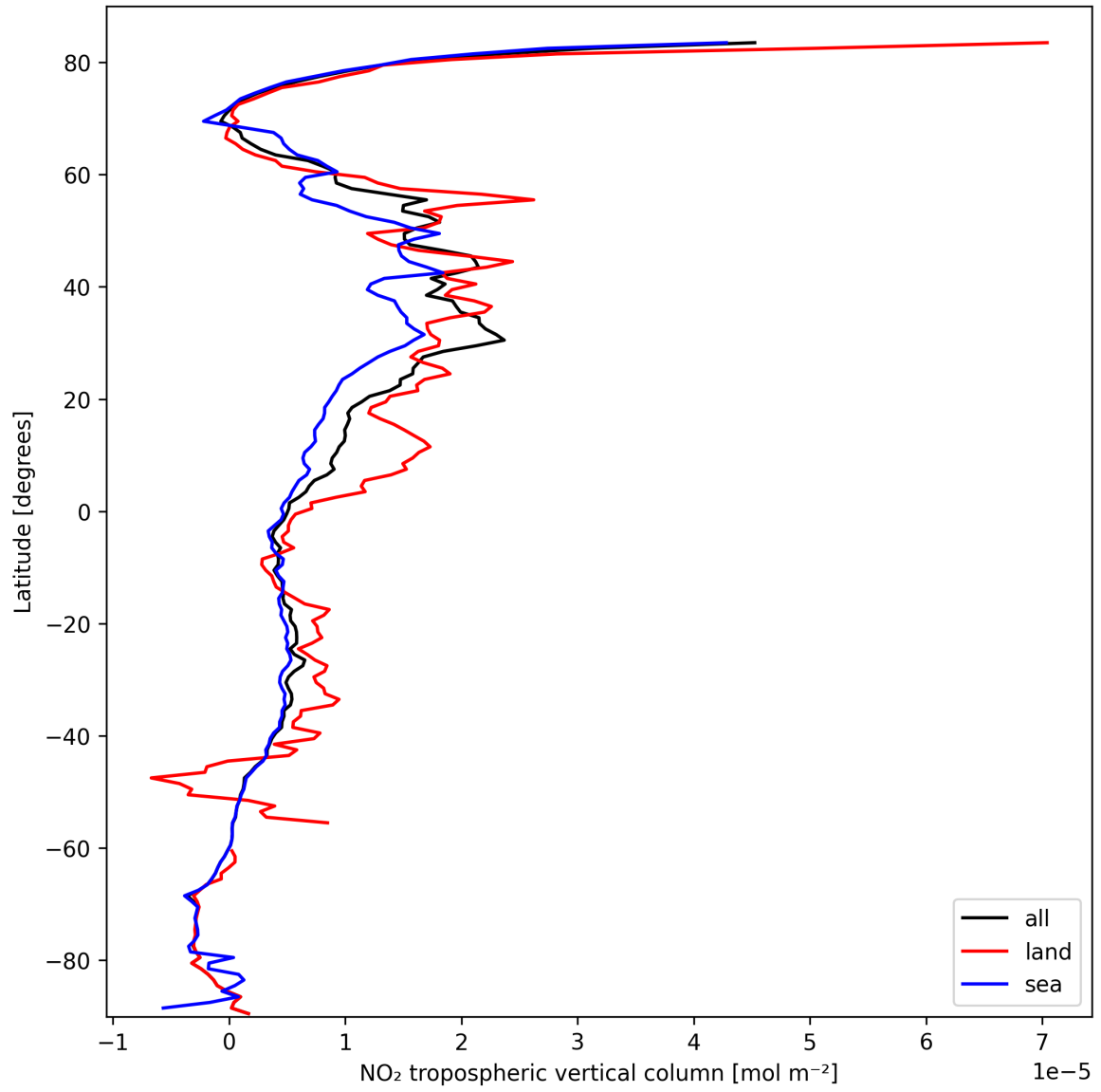
Figure 12: Zonal average of “NO 2 tropospheric vertical column” for 2025-03-09 to 2025-03-10.
