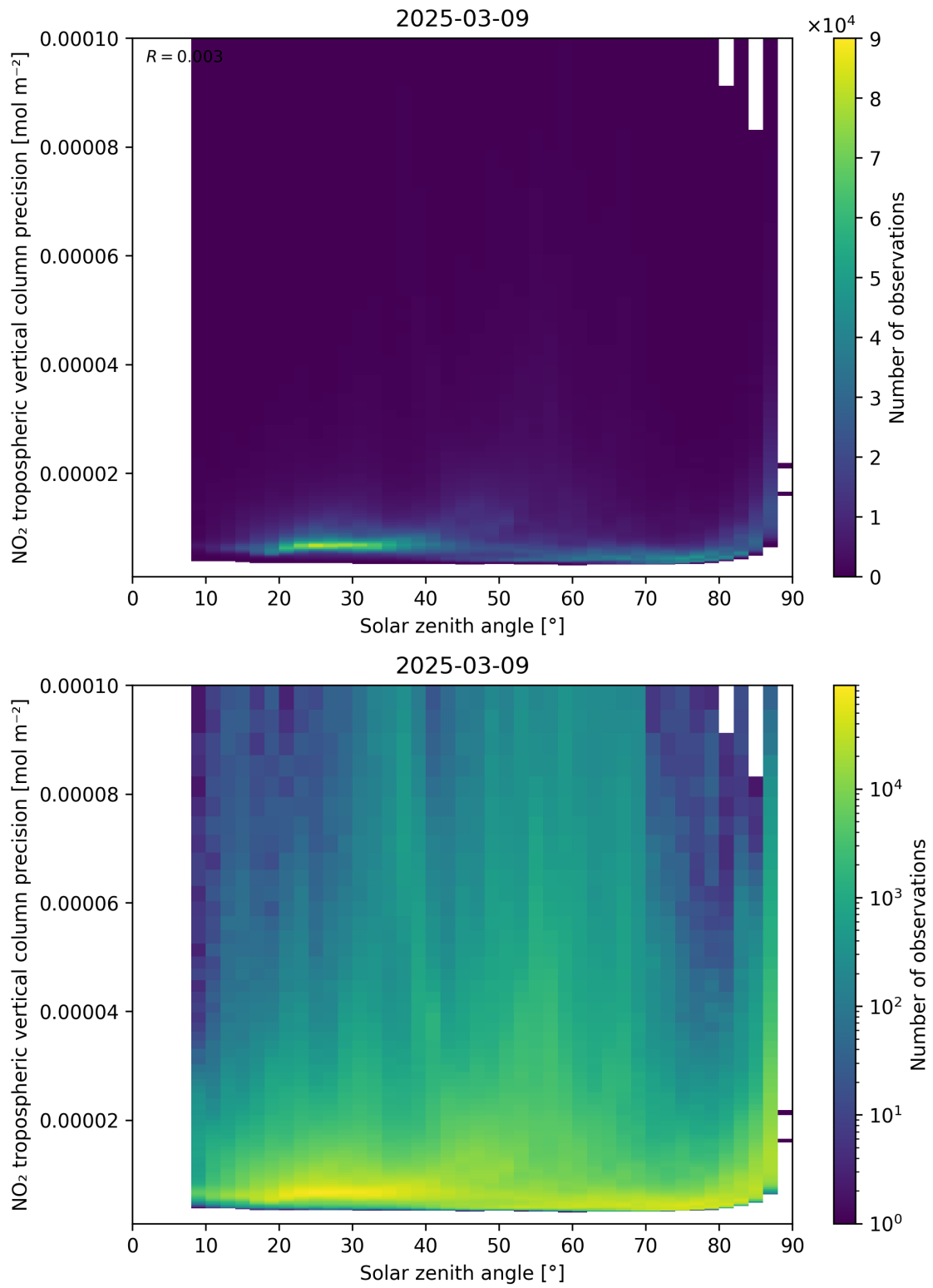
Figure 156: Scatter density plot of “Solar zenith angle” against “NO 2 tropospheric vertical column precision” for 2025-03-09 to 2025-03-10.
