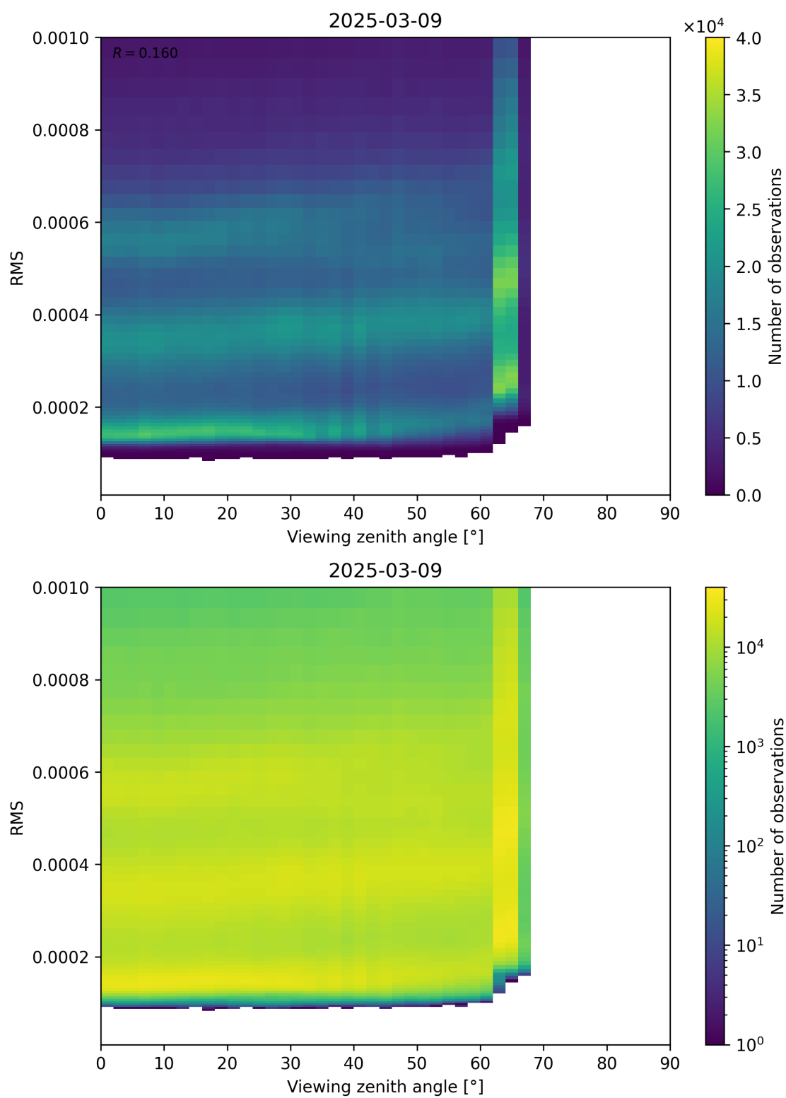
Figure 171: Scatter density plot of “Viewing zenith angle” against “RMS” for 2025-03-09 to 2025-03-10.
