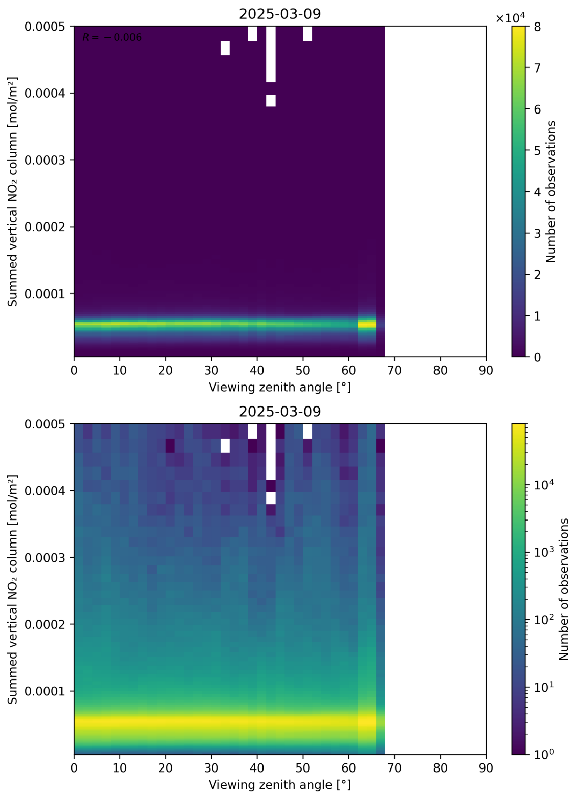
Figure 165: Scatter density plot of “Viewing zenith angle” against “Summed vertical NO 2 column” for 2025-03-09 to 2025-03-10.
