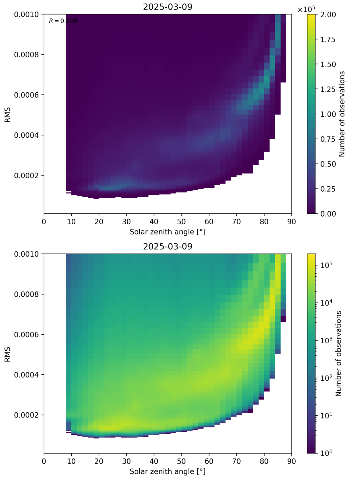
Figure 157: Scatter density plot of “Solar zenith angle” against “RMS” for 2025-03-09 to 2025-03-10.
