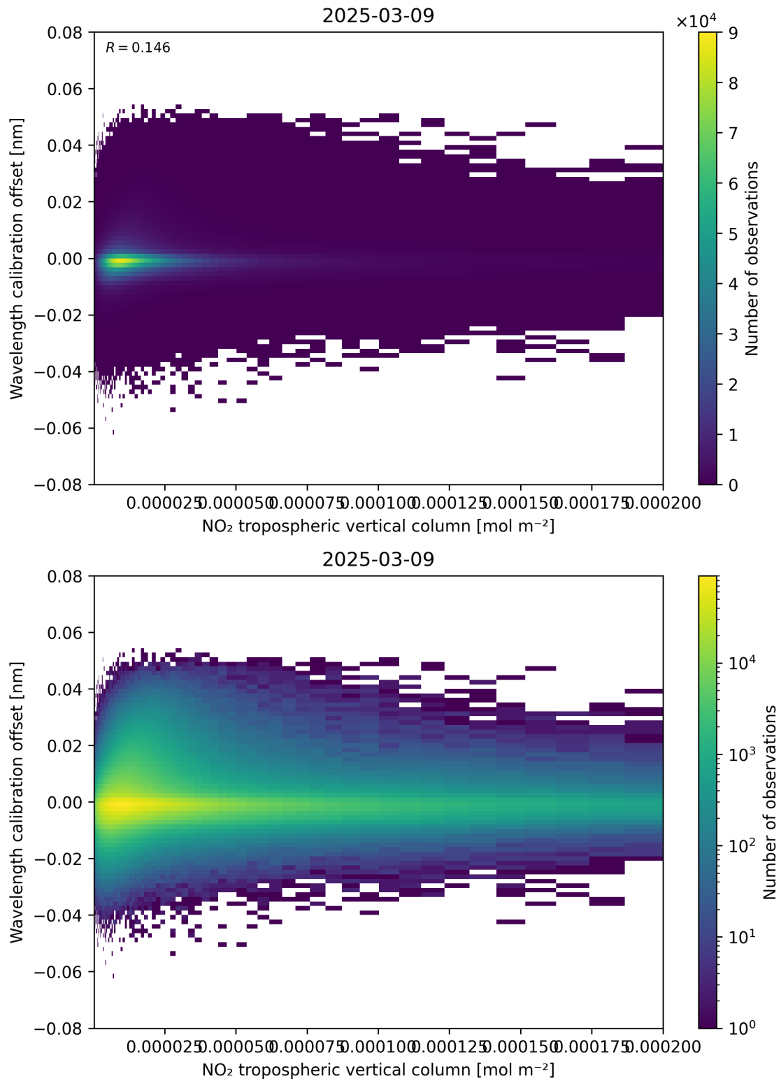
Figure 143: Scatter density plot of “NO 2 tropospheric vertical column” against “Wavelength calibration offset” for 2025-03-09 to 2025-03-10.
