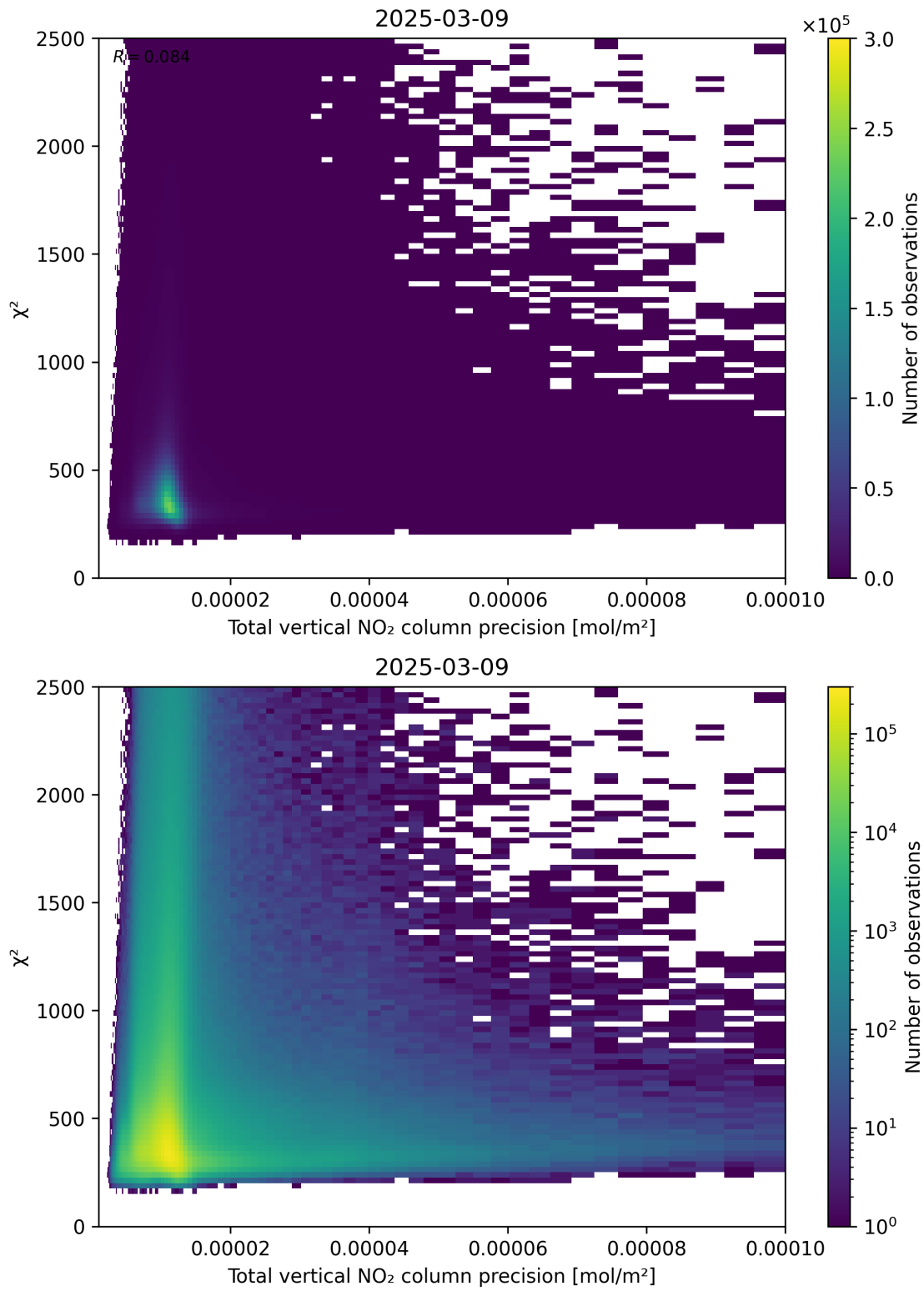
Figure 116: Scatter density plot of “Total vertical NO 2 column precision” against “ \chi^2 ” for 2025-03-09 to 2025-03-10.
