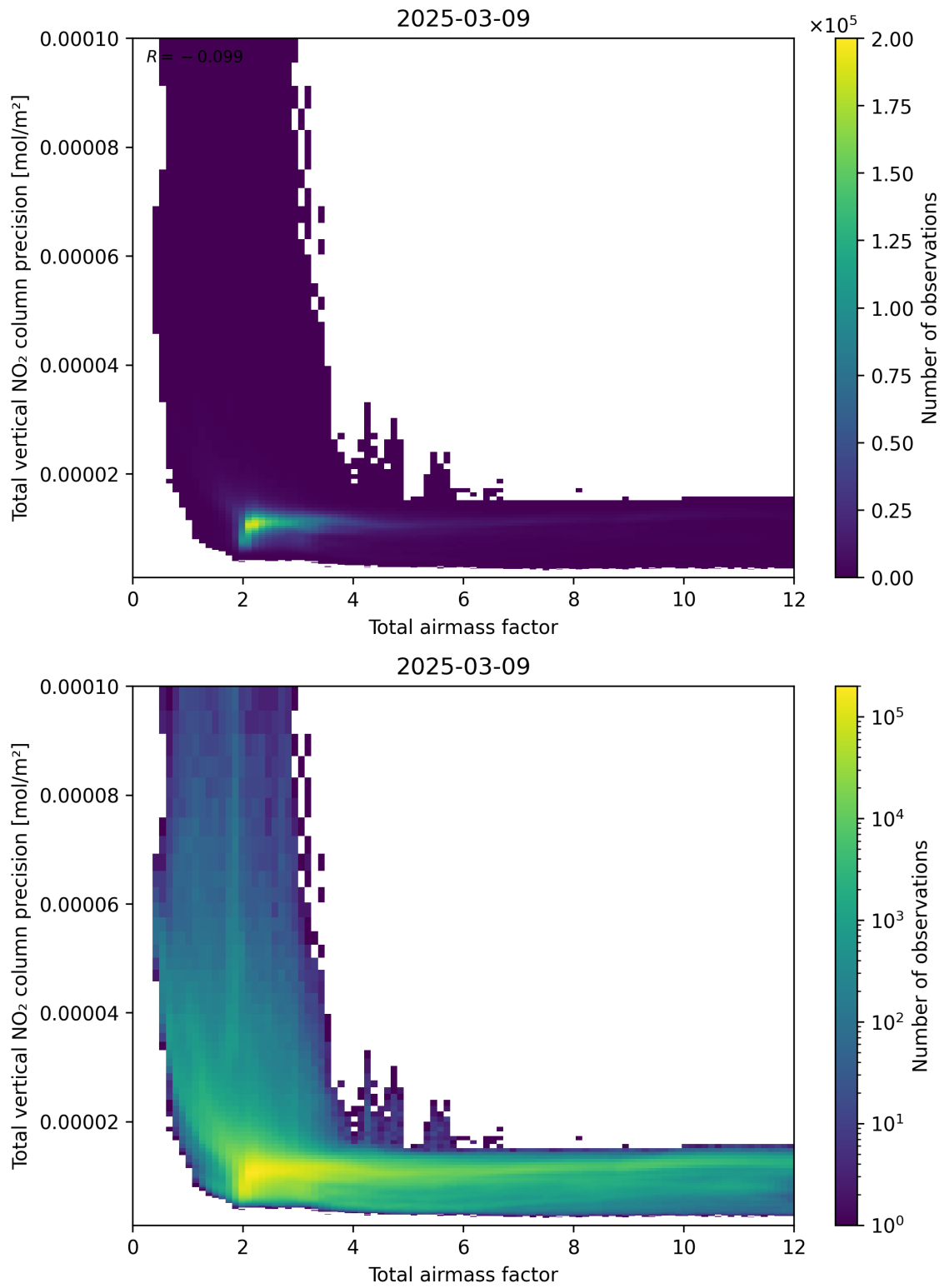
Figure 68: Scatter density plot of “Total airmass factor” against “Total vertical NO 2 column precision” for 2025-03-09 to 2025-03-10.
