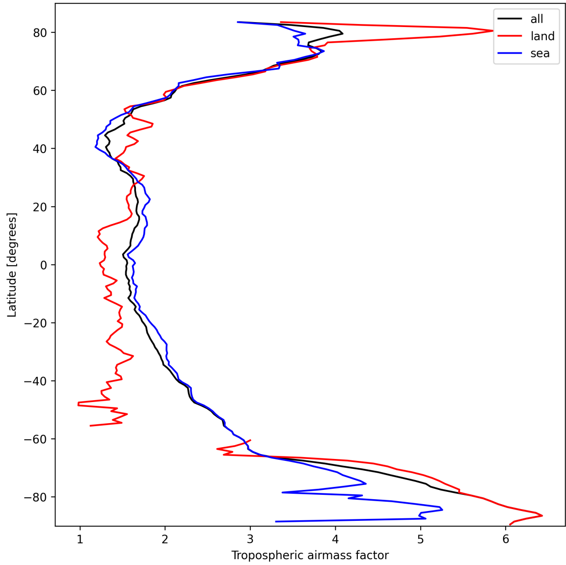
Figure 14: Zonal average of “Tropospheric airmass factor” for 2025-03-09 to 2025-03-10.
