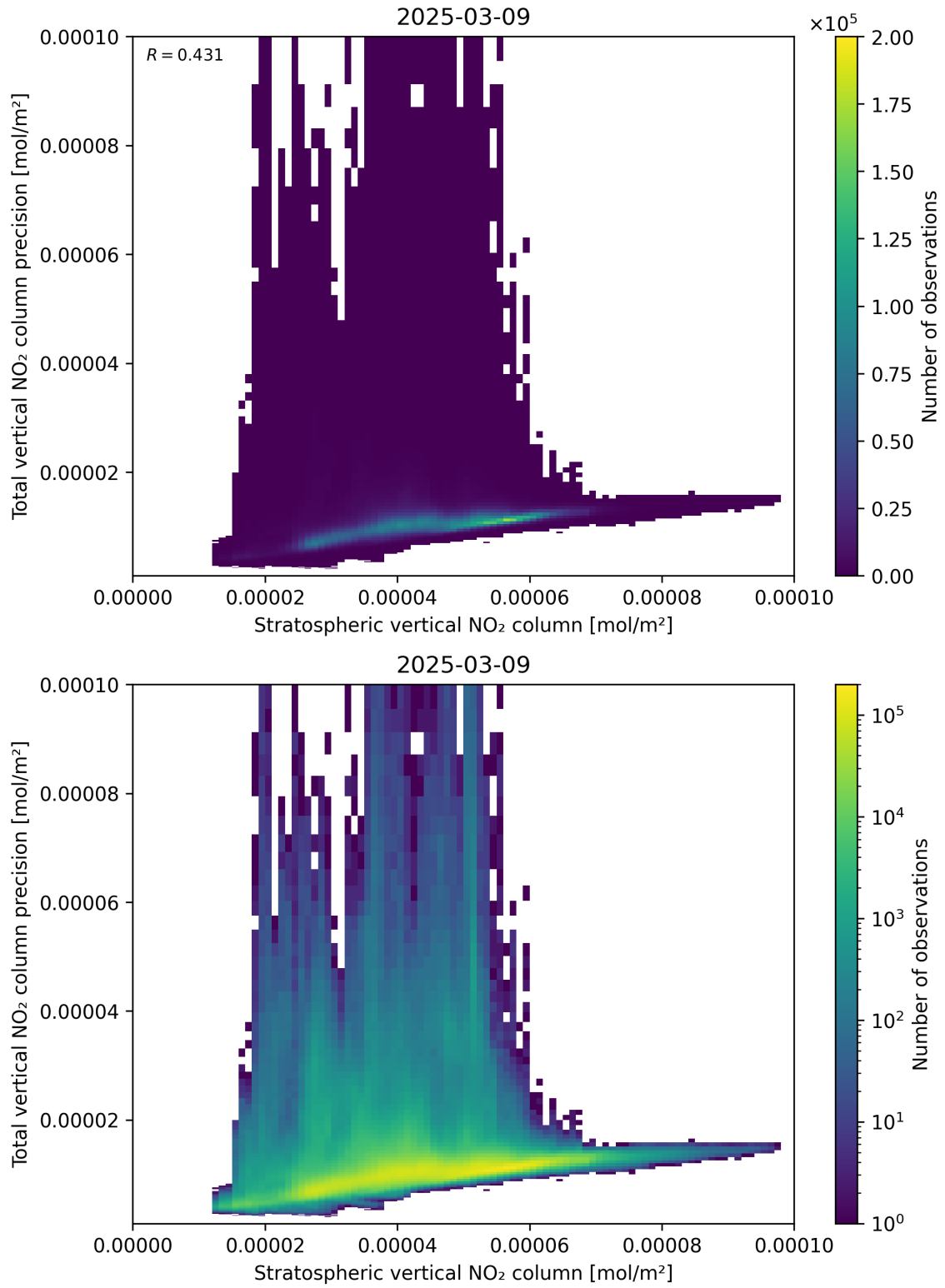
Figure 101: Scatter density plot of “Stratospheric vertical NO 2 column” against “Total vertical NO 2 column precision” for 2025-03-09 to 2025-03-10.
