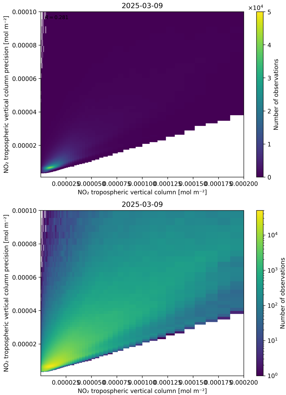
Figure 130: Scatter density plot of “NO 2 tropospheric vertical column” against “NO 2 tropospheric vertical column precision” for 2025-03-09 to 2025-03-10.
