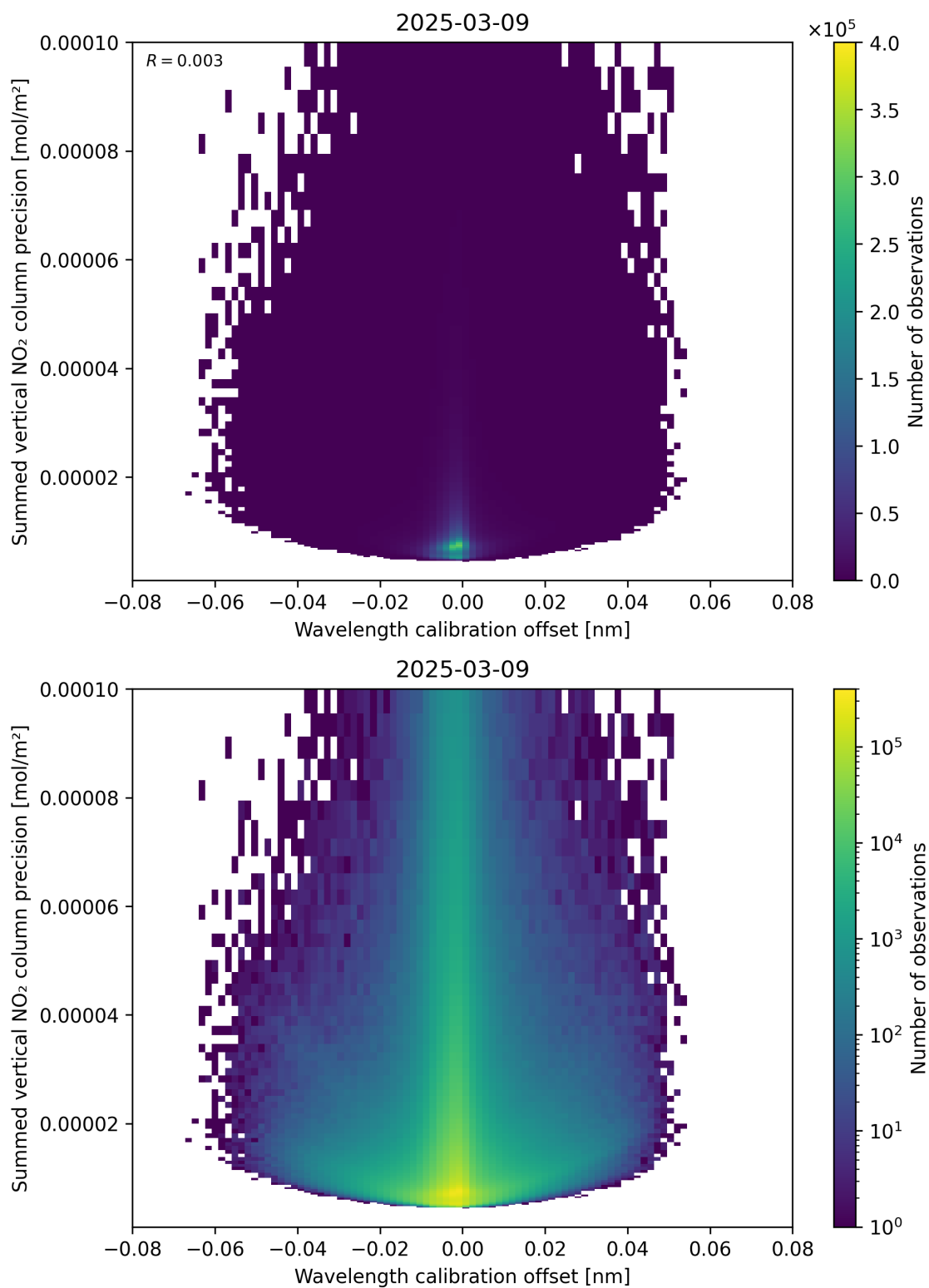
Figure 178: Scatter density plot of “Wavelength calibration offset” against “Summed vertical NO 2 column precision” for 2025-03-09 to 2025-03-10.
