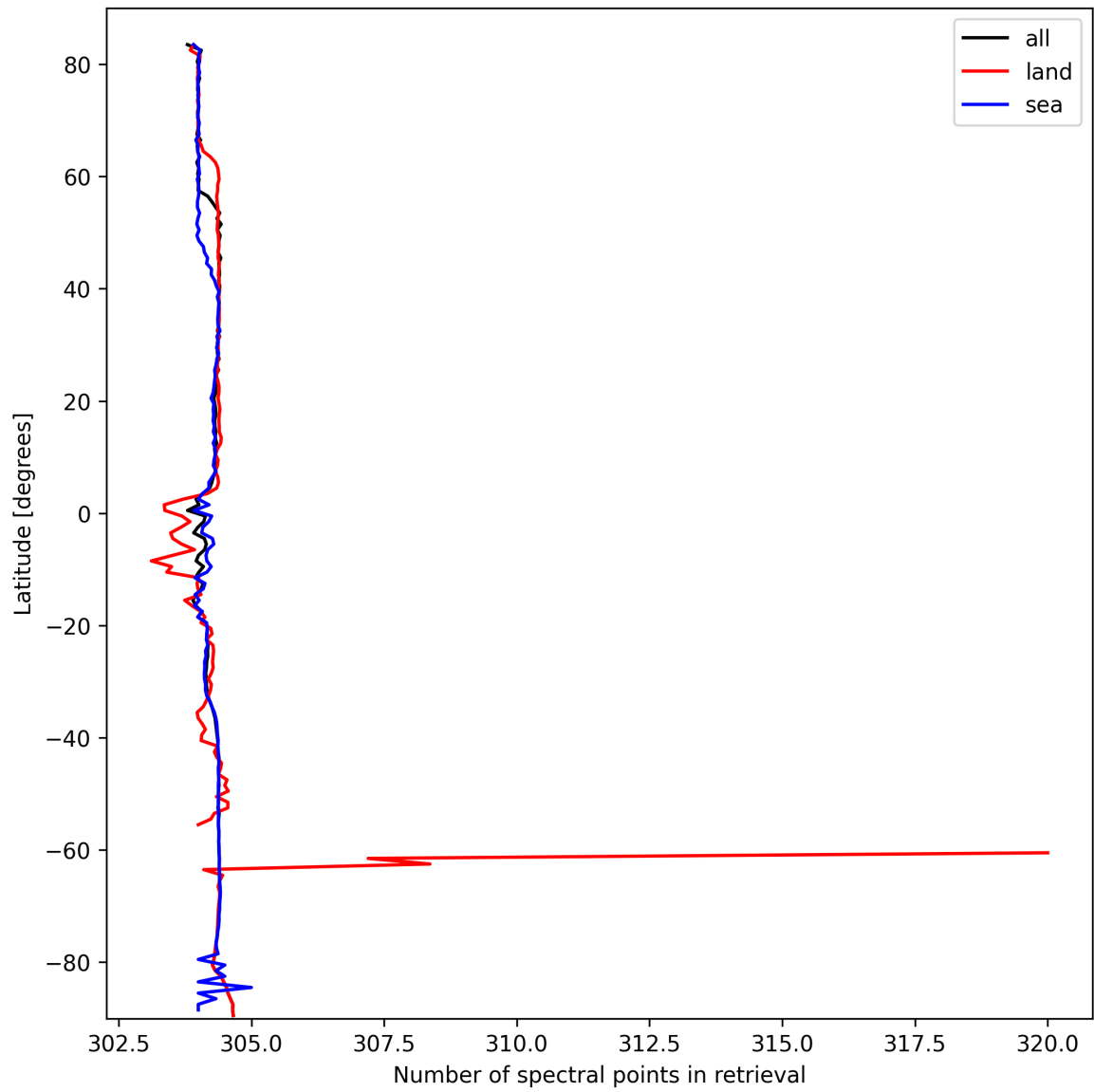
Figure 16: Zonal average of “Number of spectral points in retrieval” for 2025-03-09 to 2025-03-10.
