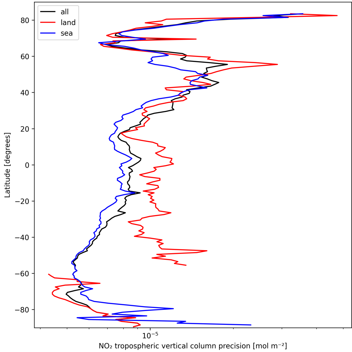
Figure 13: Zonal average of “NO 2 tropospheric vertical column precision” for 2025-03-09 to 2025-03-10.
