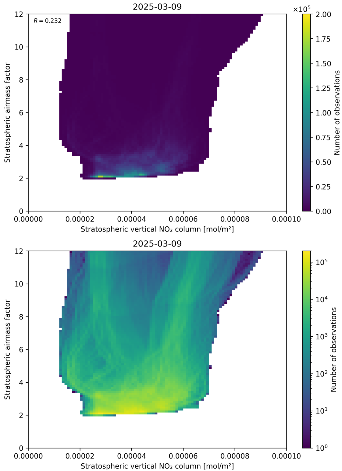
Figure 96: Scatter density plot of “Stratospheric vertical NO 2 column” against “Stratospheric airmass factor” for 2025-03-09 to 2025-03-10.
