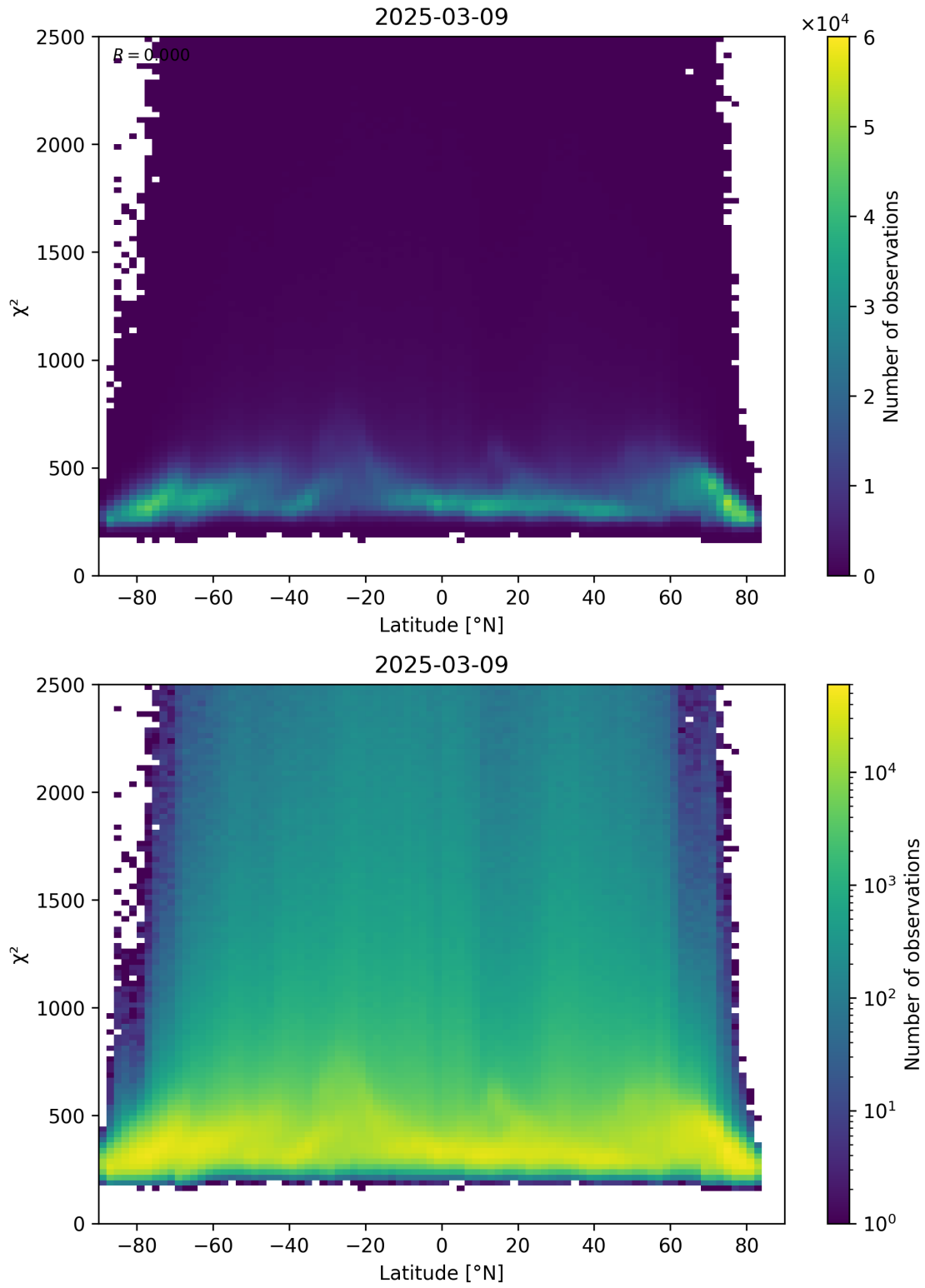
Figure 86: Scatter density plot of “Latitude” against “ \chi^2 ” for 2025-03-09 to 2025-03-10.
