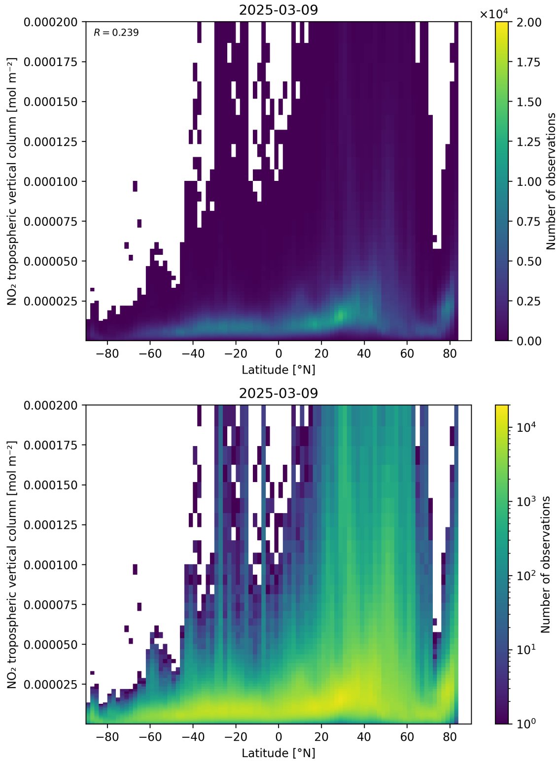
Figure 92: Scatter density plot of “Latitude” against “NO 2 tropospheric vertical column” for 2025-03-09 to 2025-03-10.
