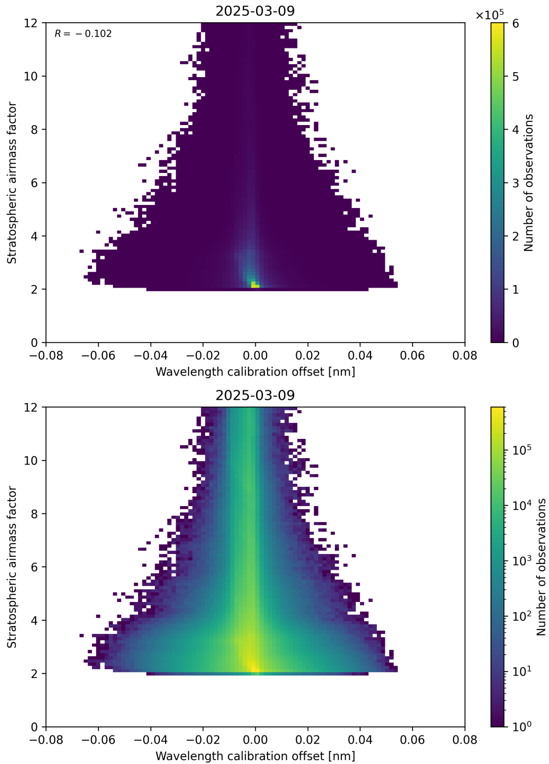
Figure 174: Scatter density plot of “Wavelength calibration offset” against “Stratospheric airmass factor” for 2025-03-09 to 2025-03-10.
