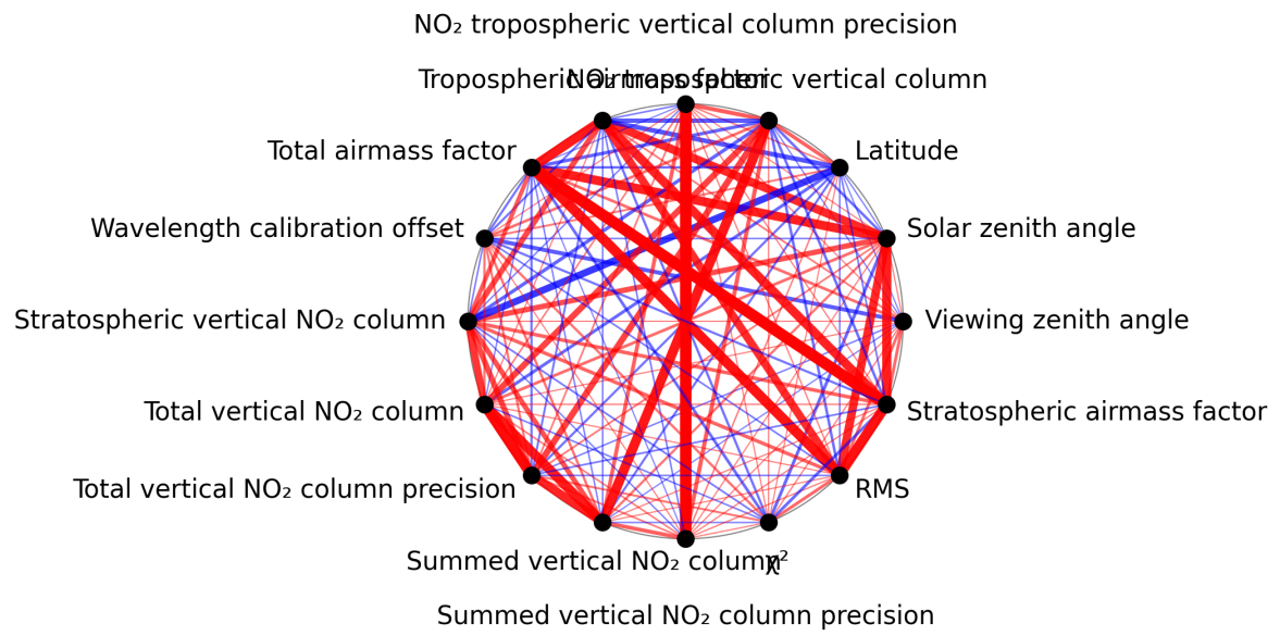
Figure 1: Map of correlation graph for 2025-03-09 to 2025-03-10.
