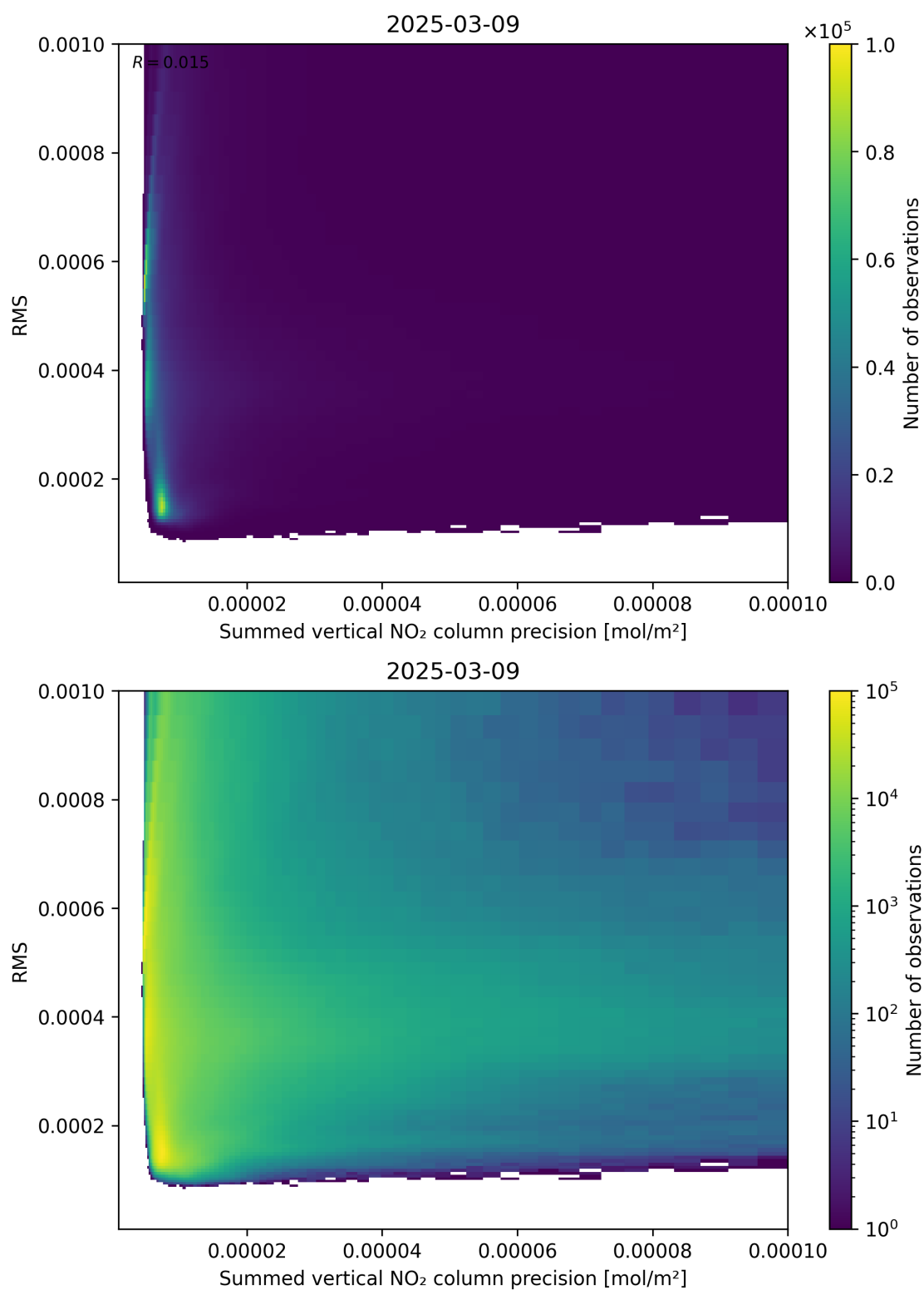
Figure 108: Scatter density plot of “Summed vertical NO 2 column precision” against “RMS” for 2025-03-09 to 2025-03-10.
