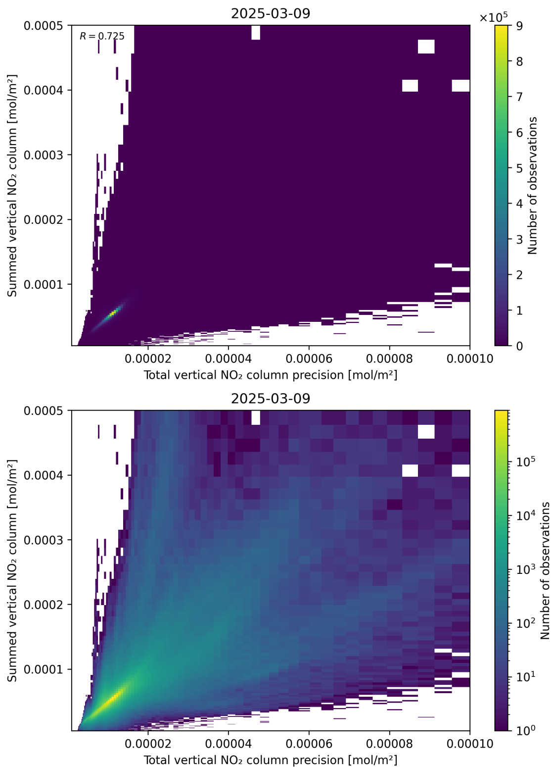
Figure 117: Scatter density plot of “Total vertical NO 2 column precision” against “Summed vertical NO 2 column” for 2025-03-09 to 2025-03-10.
