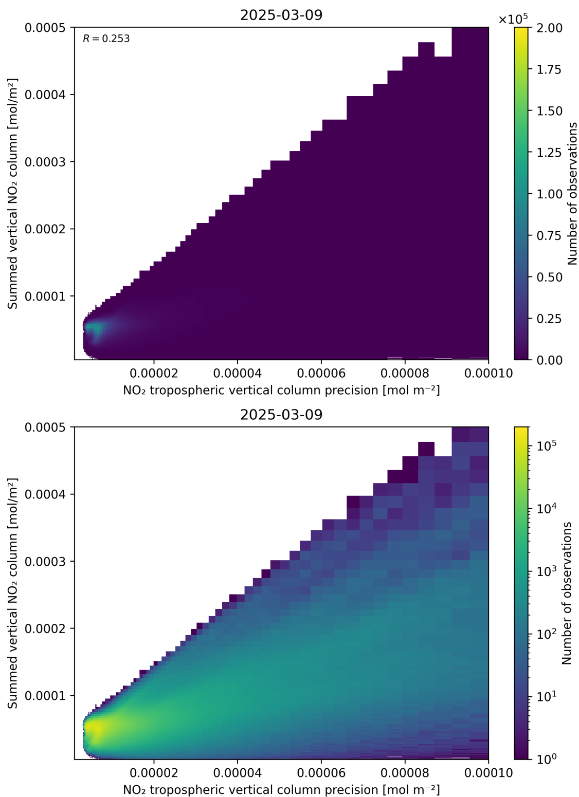
Figure 136: Scatter density plot of “NO 2 tropospheric vertical column precision” against “Summed vertical NO 2 column” for 2025-03-09 to 2025-03-10.
