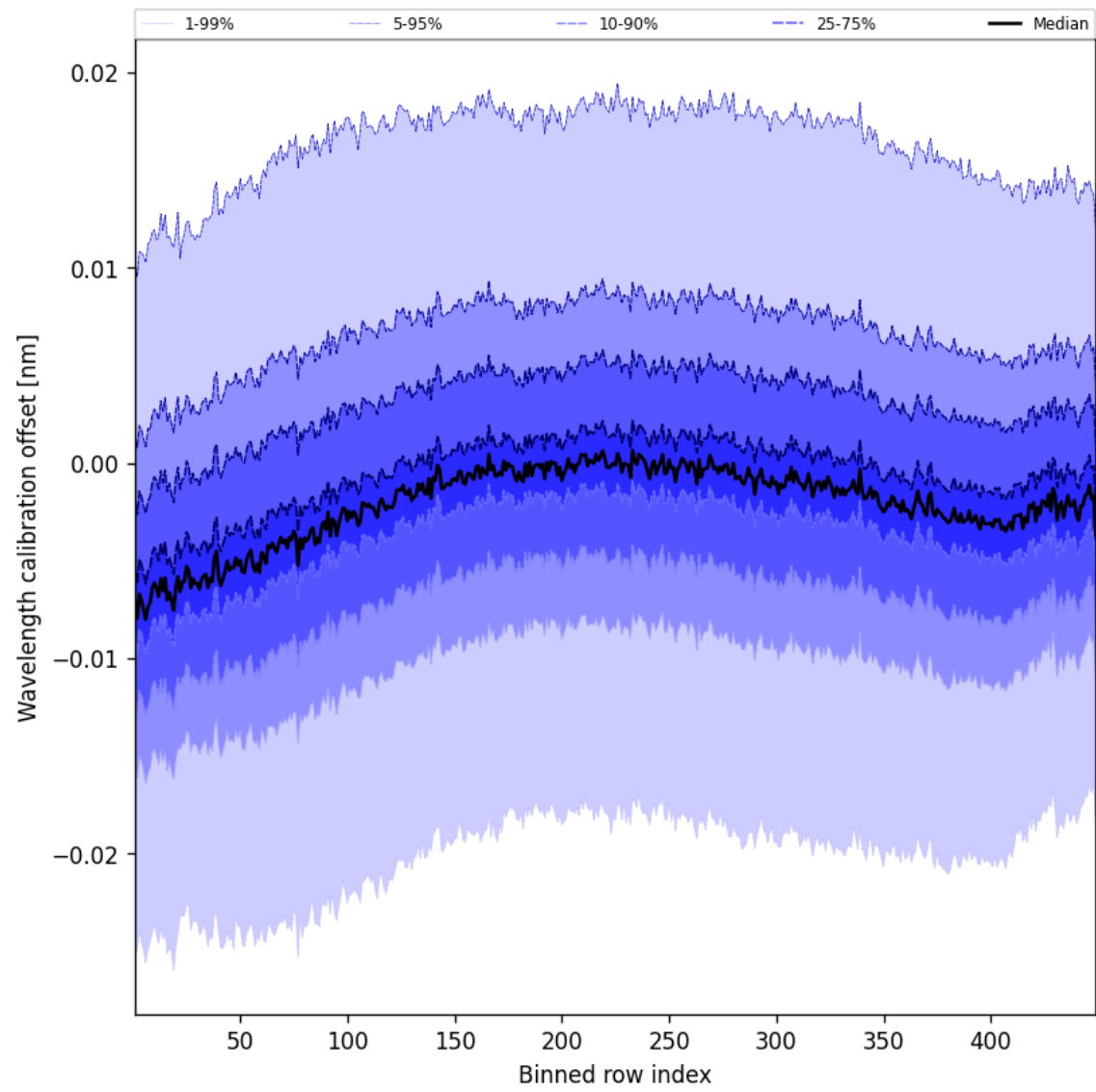
Figure 52: Along track statistics of “Wavelength calibration offset” for 2025-03-09 to 2025-03-10
