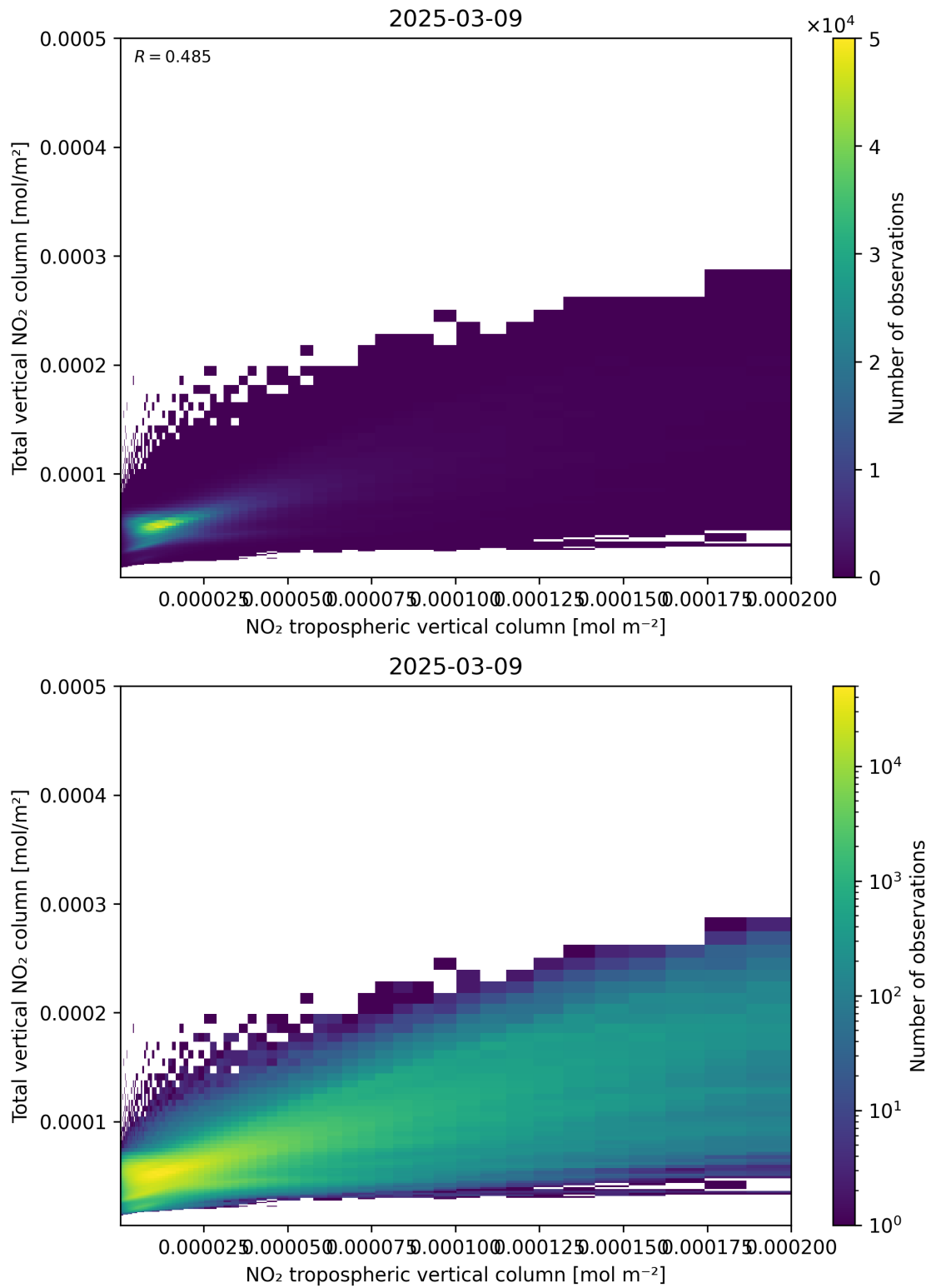
Figure 128: Scatter density plot of “NO 2 tropospheric vertical column” against “Total vertical NO 2 column” for 2025-03-09 to 2025-03-10.
