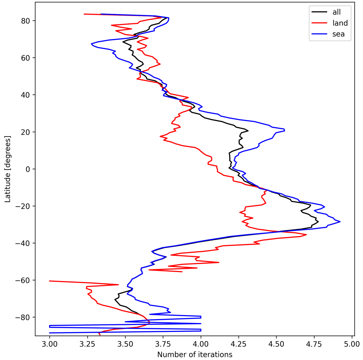
Figure 17: Zonal average of “Number of iterations” for 2025-03-09 to 2025-03-10.
