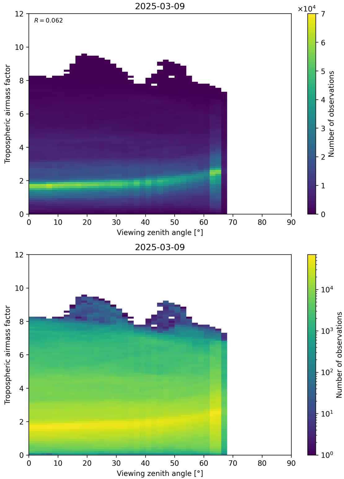
Figure 161: Scatter density plot of “Viewing zenith angle” against “Tropospheric airmass factor” for 2025-03-09 to 2025-03-10.
