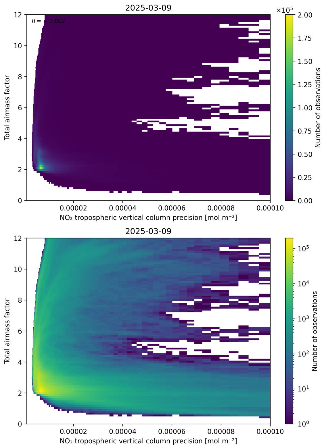
Figure 132: Scatter density plot of “NO 2 tropospheric vertical column precision” against “Total airmass factor” for 2025-03-09 to 2025-03-10.
