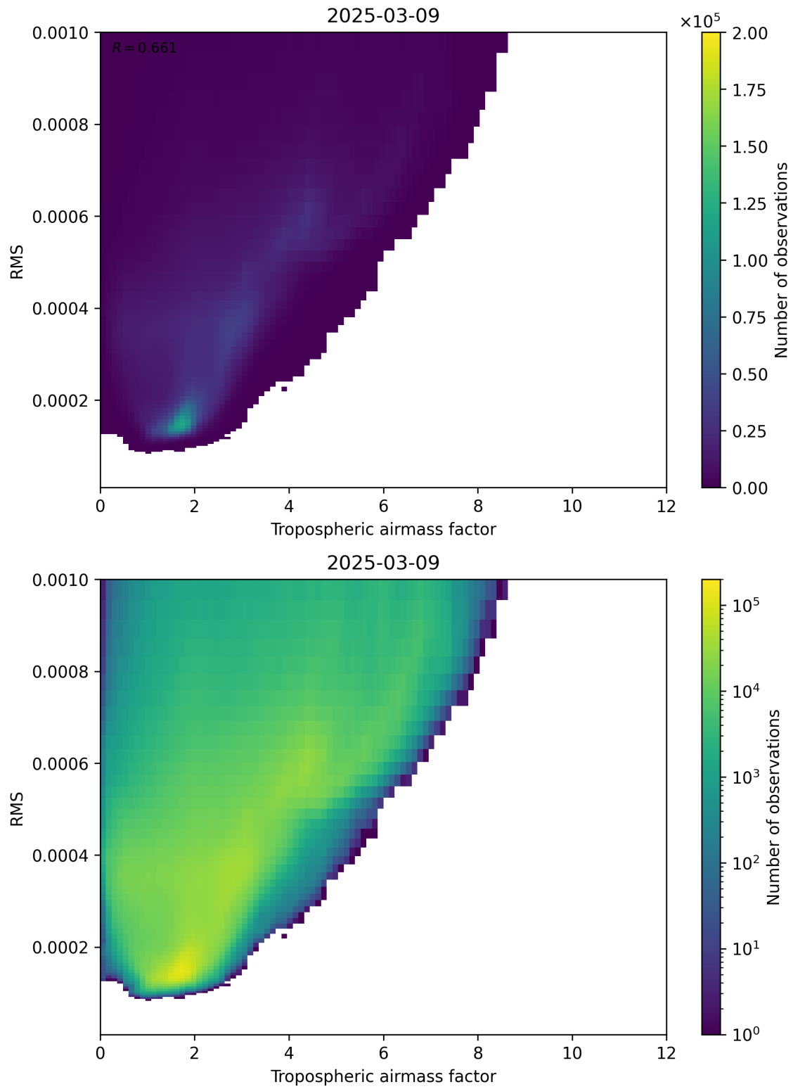
Figure 79: Scatter density plot of “Tropospheric airmass factor” against “RMS” for 2025-03-09 to 2025-03-10.
