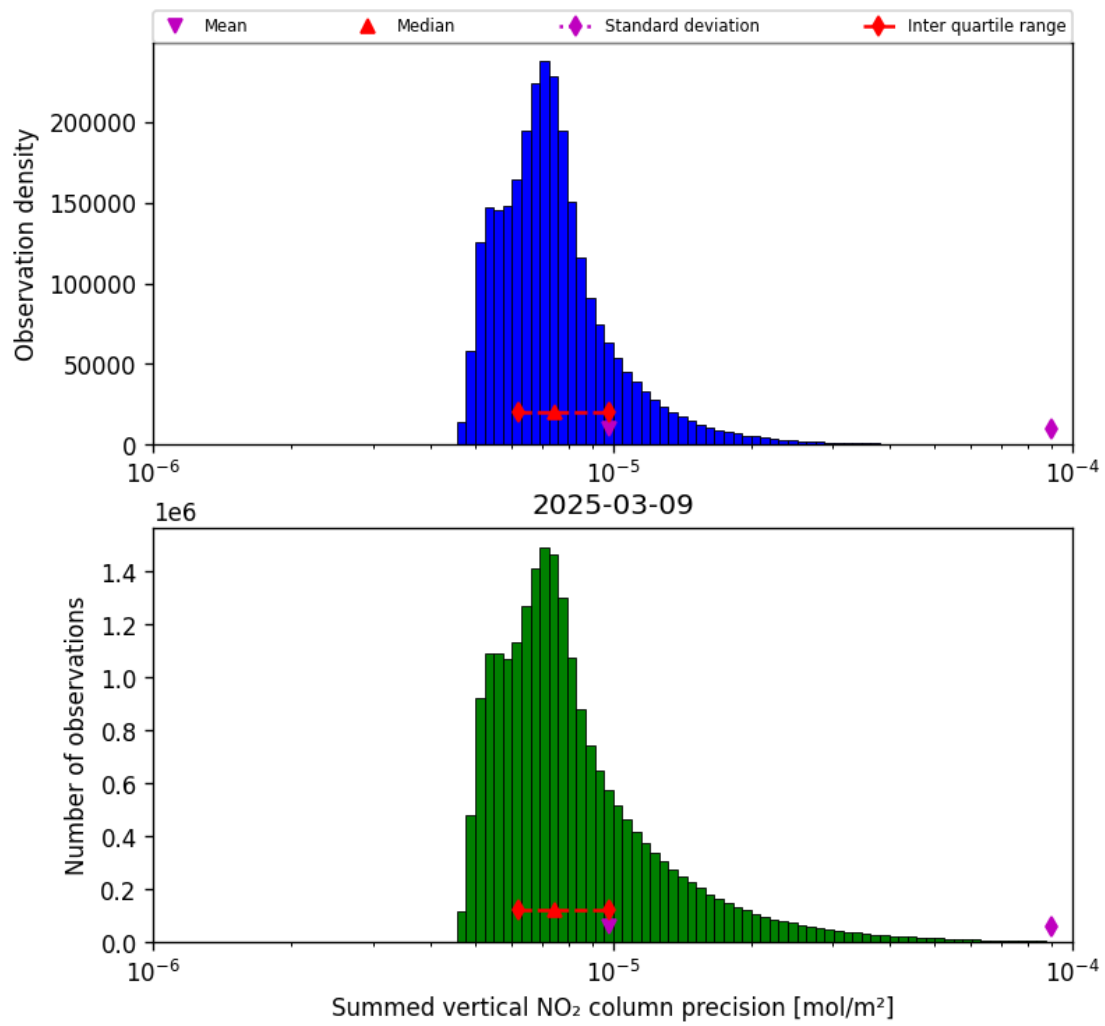
Figure 41: Histogram of "Summed vertical NO 2 column precision" for 2025-03-09 to 2025-03-10
