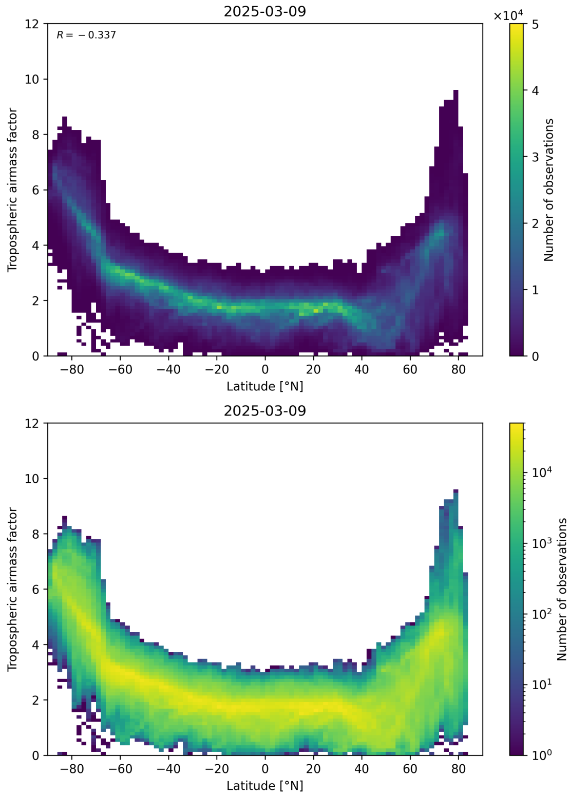
Figure 85: Scatter density plot of “Latitude” against “Tropospheric airmass factor” for 2025-03-09 to 2025-03-10.
