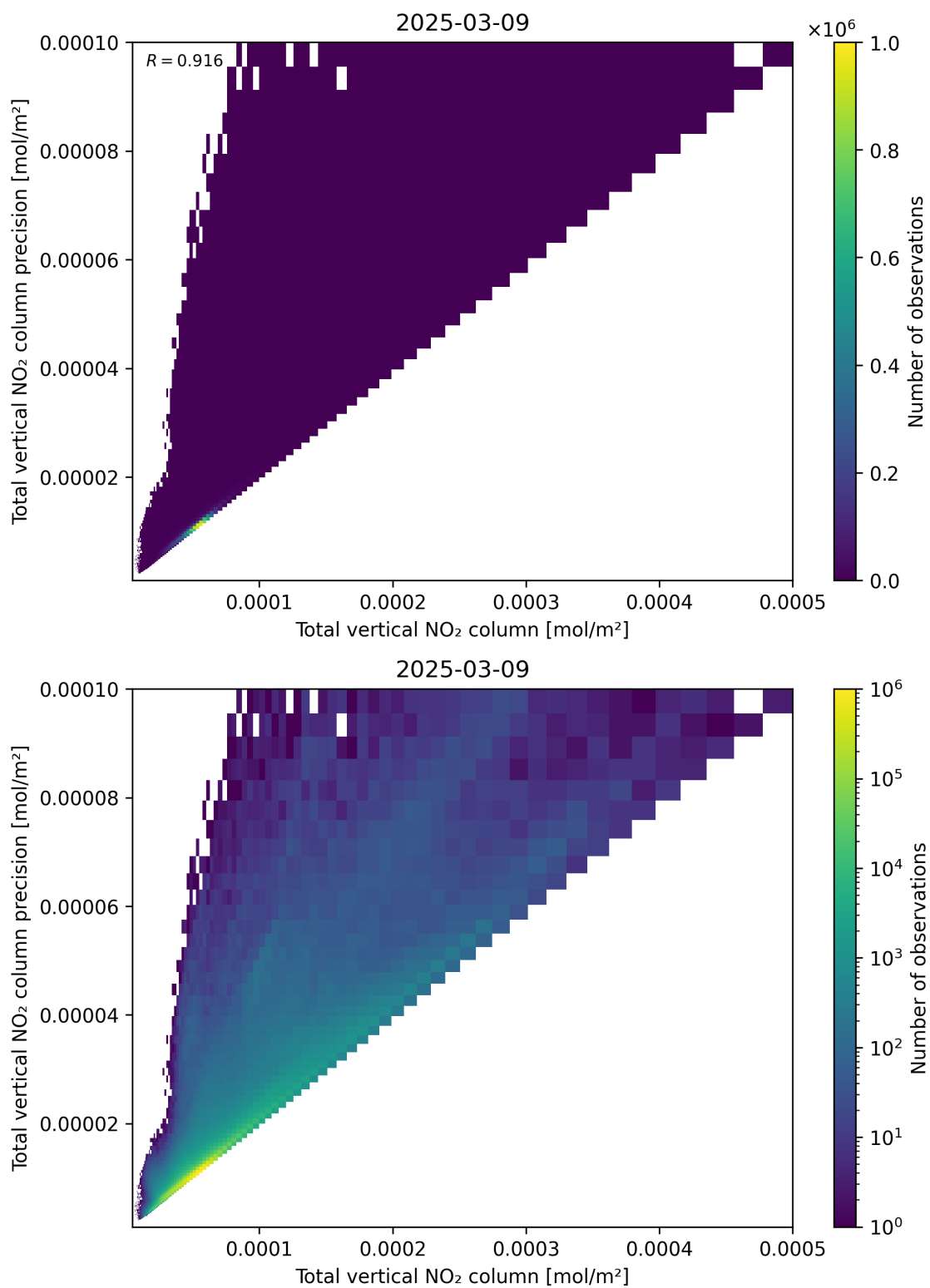
Figure 114: Scatter density plot of “Total vertical NO 2 column” against “Total vertical NO 2 column precision” for 2025-03-09 to 2025-03-10.
