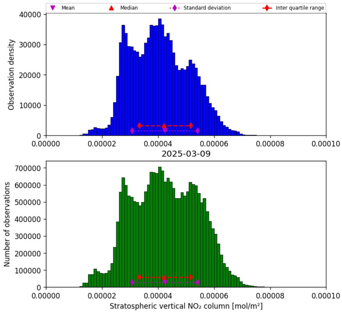
Figure 36: Histogram of “Stratospheric vertical NO 2 column” for 2025-03-09 to 2025-03-10
