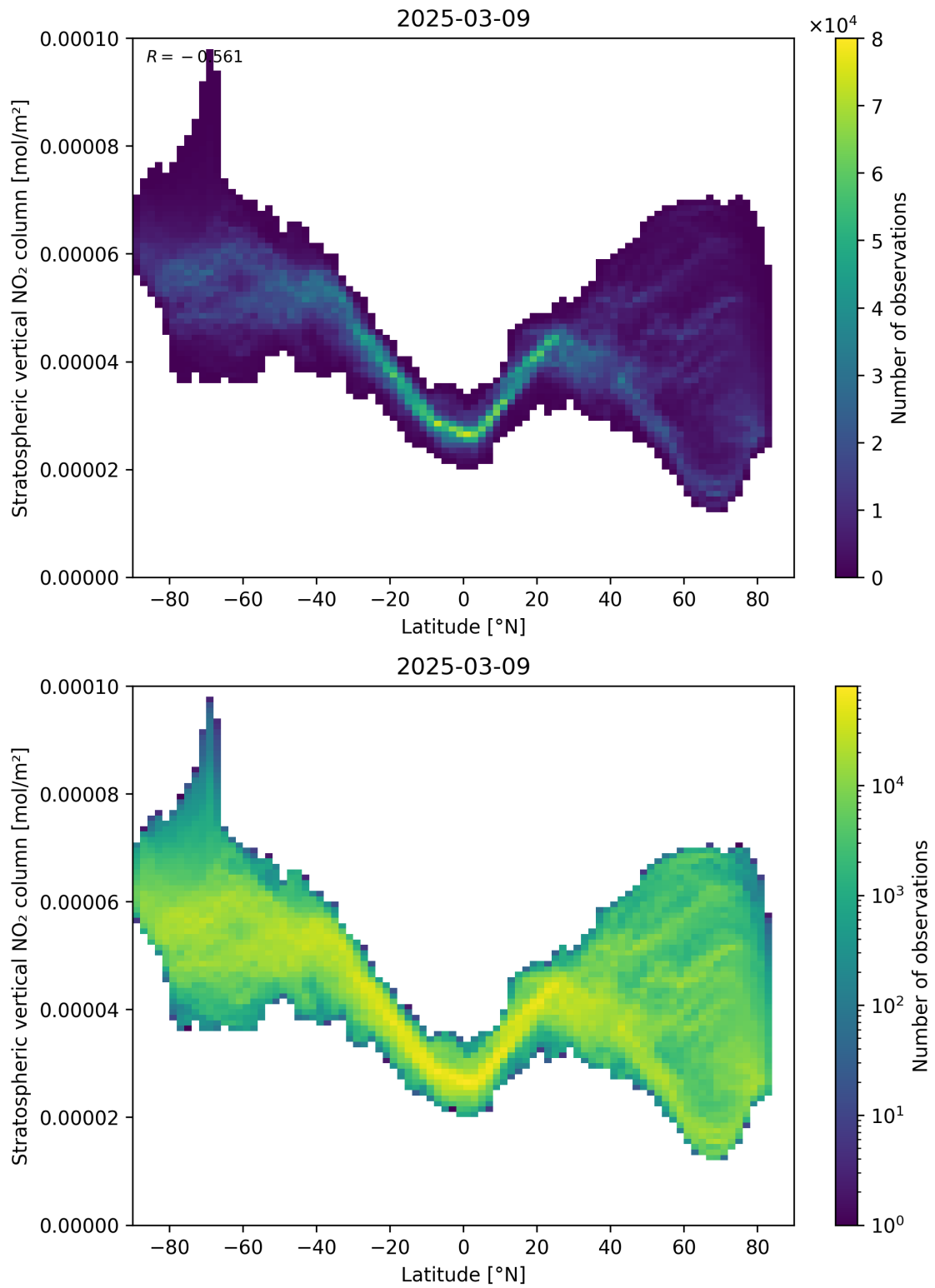
Figure 87: Scatter density plot of “Latitude” against “Stratospheric vertical NO 2 column” for 2025-03-09 to 2025-03-10.
