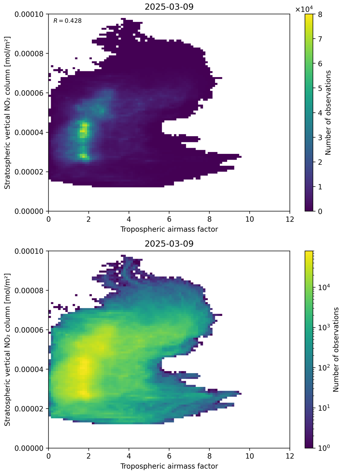
Figure 74: Scatter density plot of “Tropospheric air mass factor” against “Stratospheric vertical NO 2 column” for 2025-03-09 to 2025-03-10.
