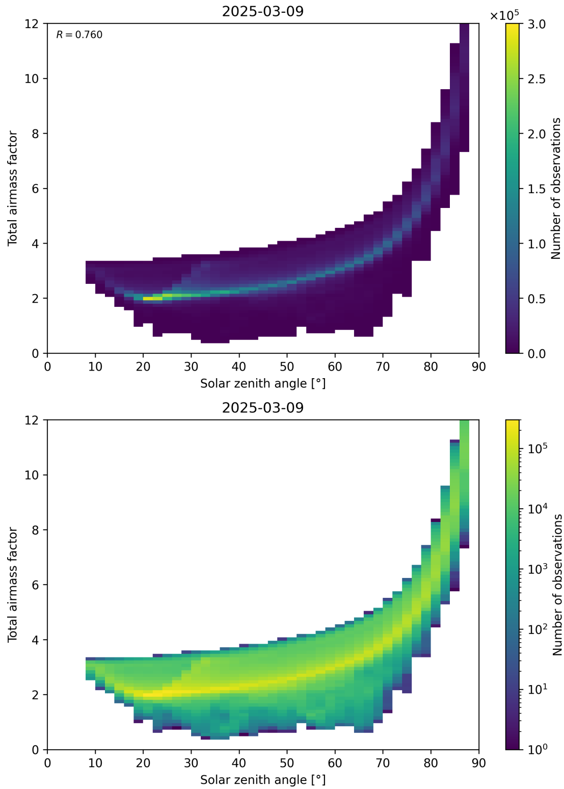
Figure 146: Scatter density plot of “Solar zenith angle” against “Total airmass factor” for 2025-03-09 to 2025-03-10.
