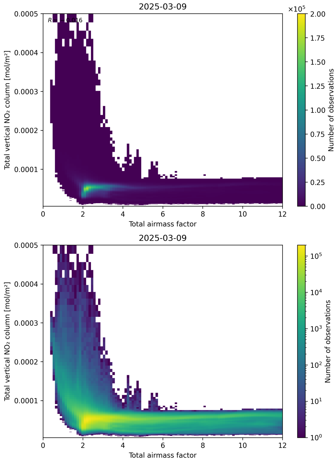
Figure 67: Scatter density plot of “Total airmass factor” against “Total vertical NO 2 column” for 2025-03-09 to 2025-03-10.
