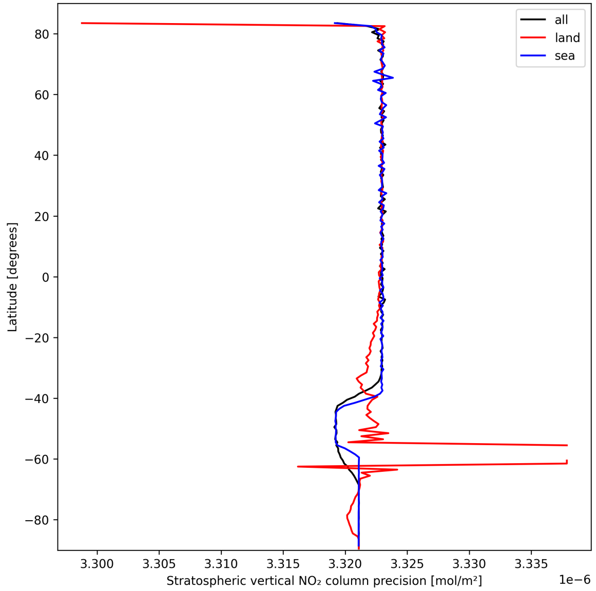
Figure 20: Zonal average of “Stratospheric vertical NO 2 column precision” for 2025-03-09 to 2025-03-10.
