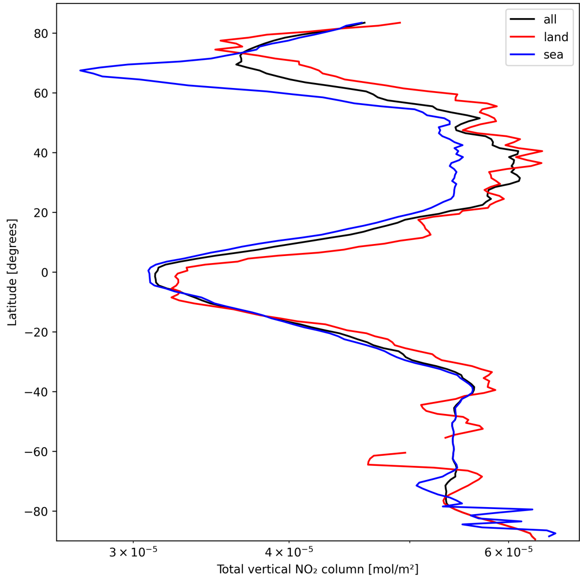
Figure 21: Zonal average of “Total vertical NO 2 column” for 2025-03-09 to 2025-03-10.
