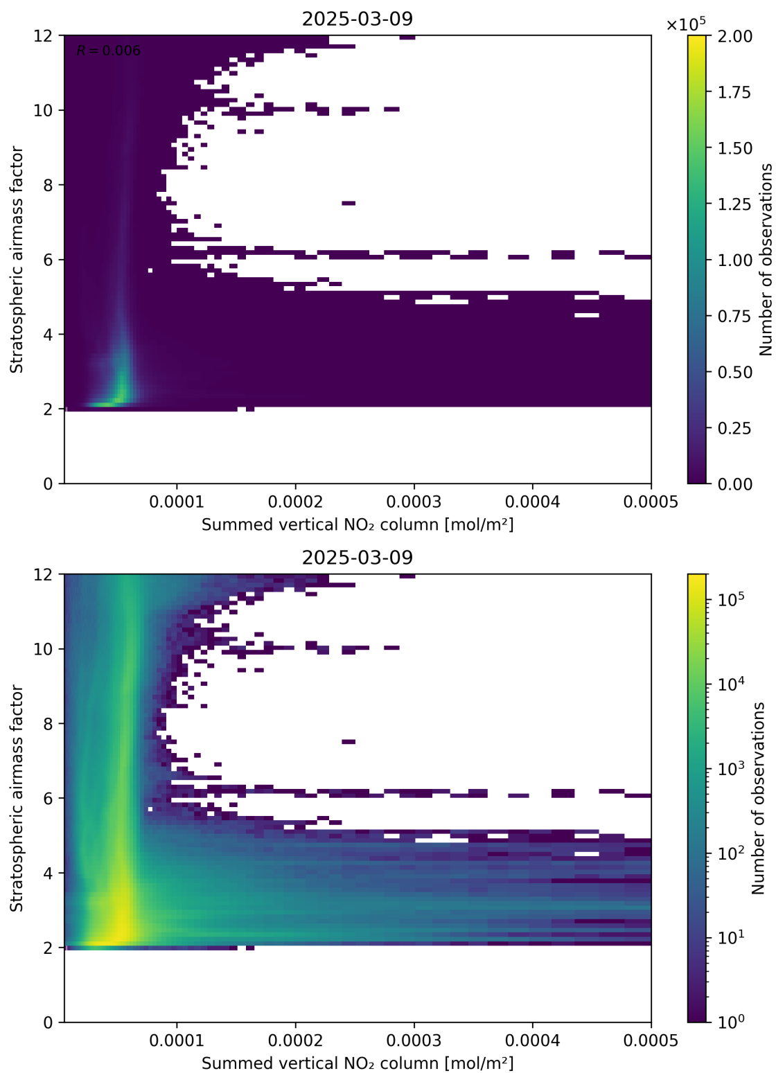
Figure 103: Scatter density plot of “Summed vertical NO 2 column” against “Stratospheric air mass factor” for 2025-03-09 to 2025-03-10.
