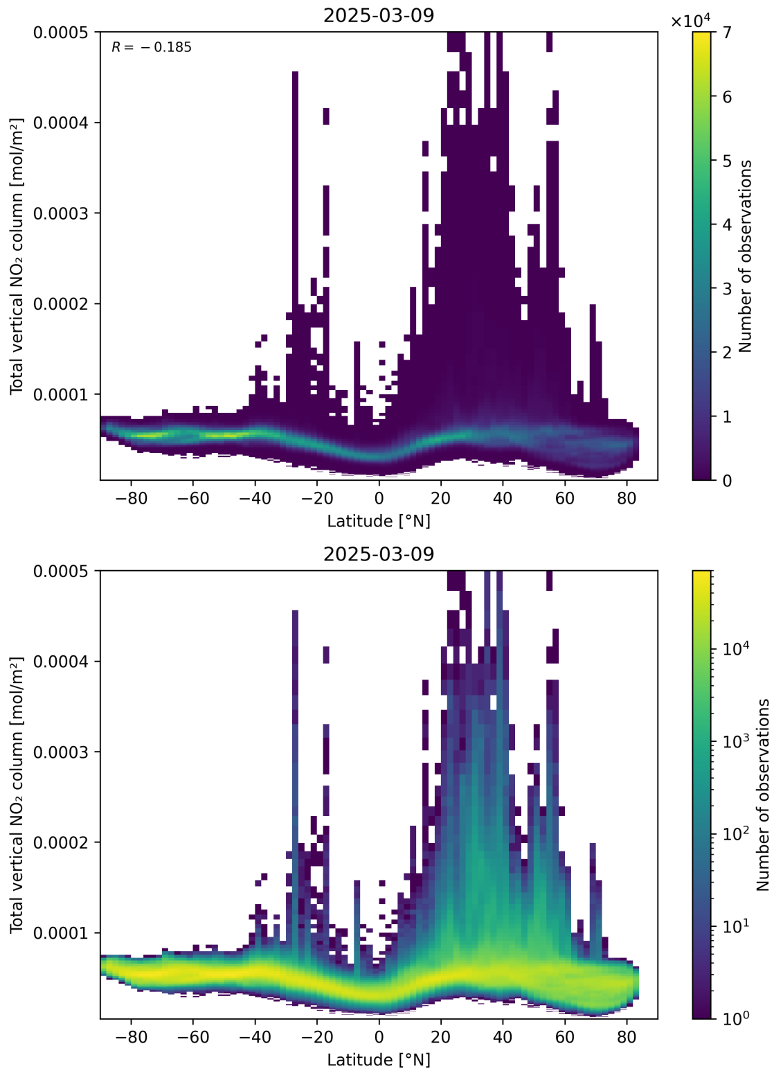
Figure 90: Scatter density plot of “Latitude” against “Total vertical NO 2 column” for 2025-03-09 to 2025-03-10.
