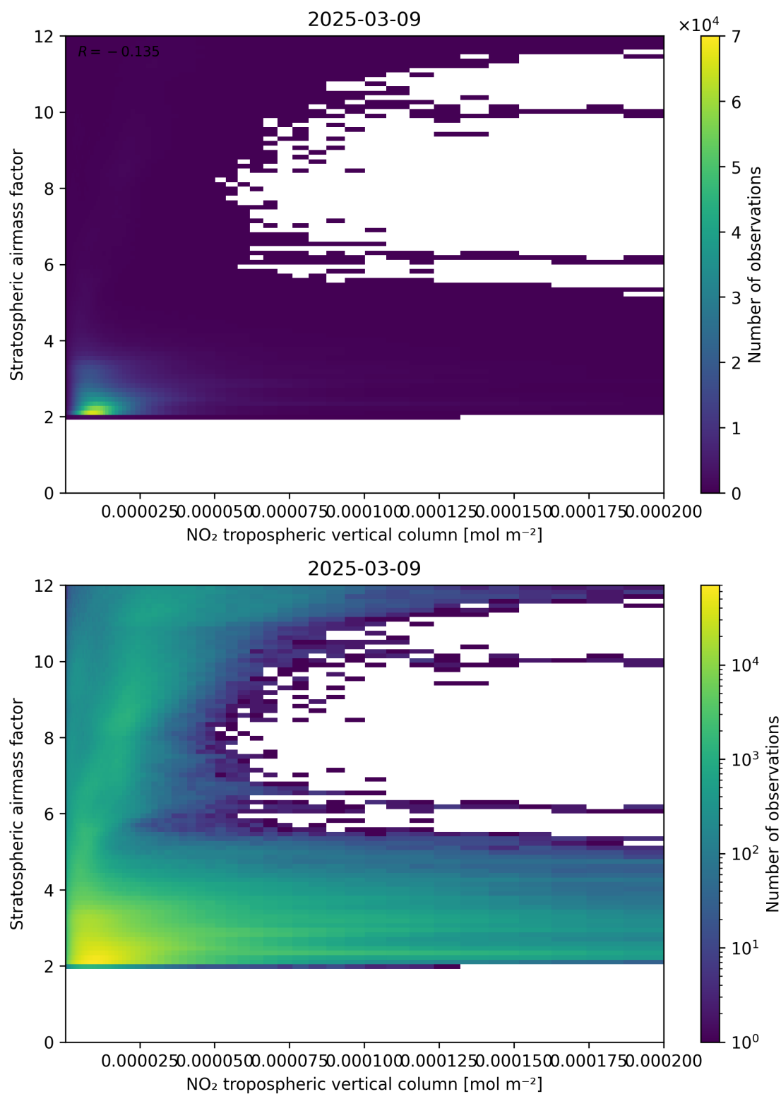
Figure 121: Scatter density plot of “NO 2 tropospheric vertical column” against “Stratospheric air mass factor” for 2025-03-09 to 2025-03-10.
