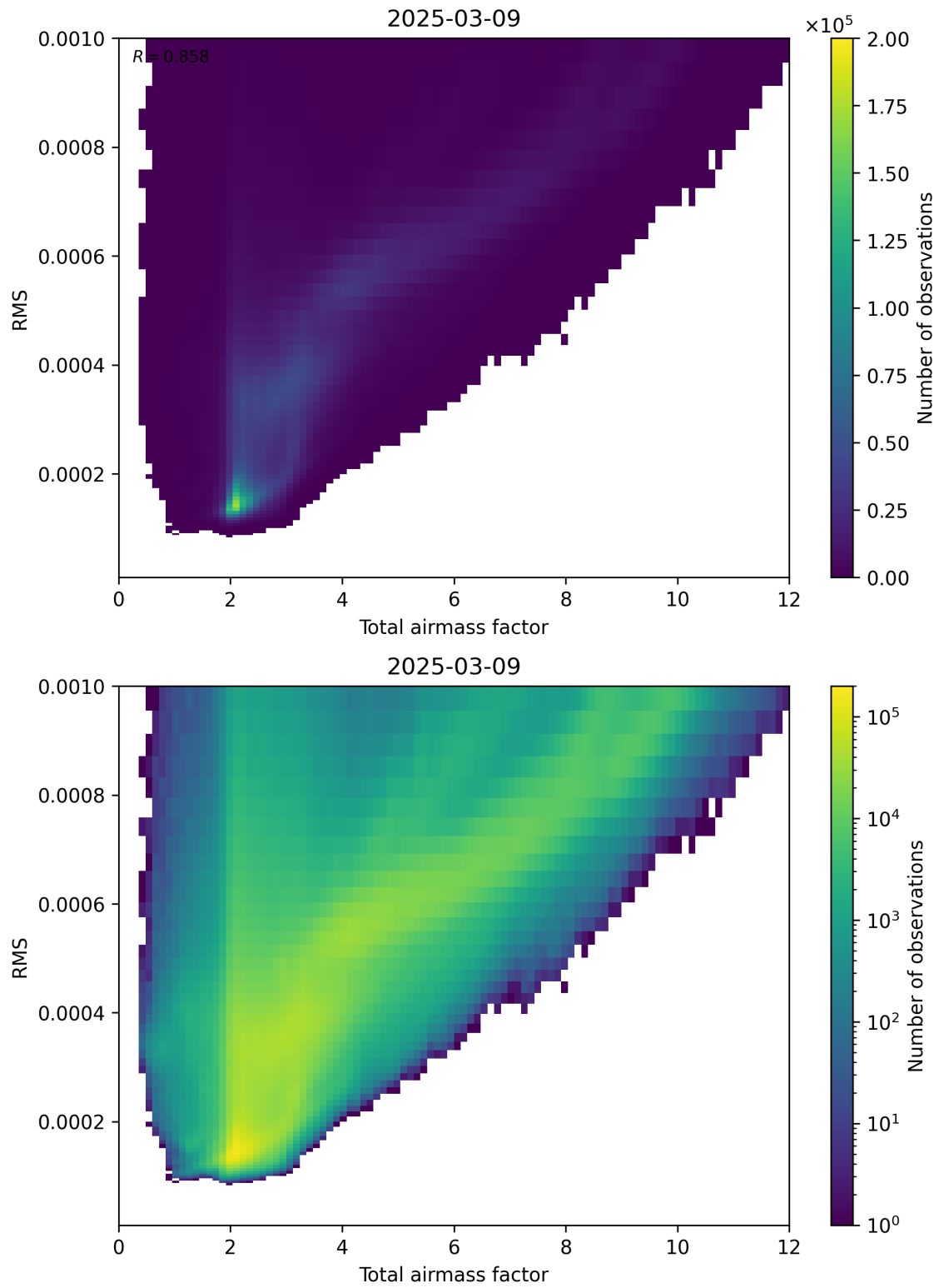
Figure 69: Scatter density plot of “Total airmass factor” against “RMS” for 2025-03-09 to 2025-03-10.
