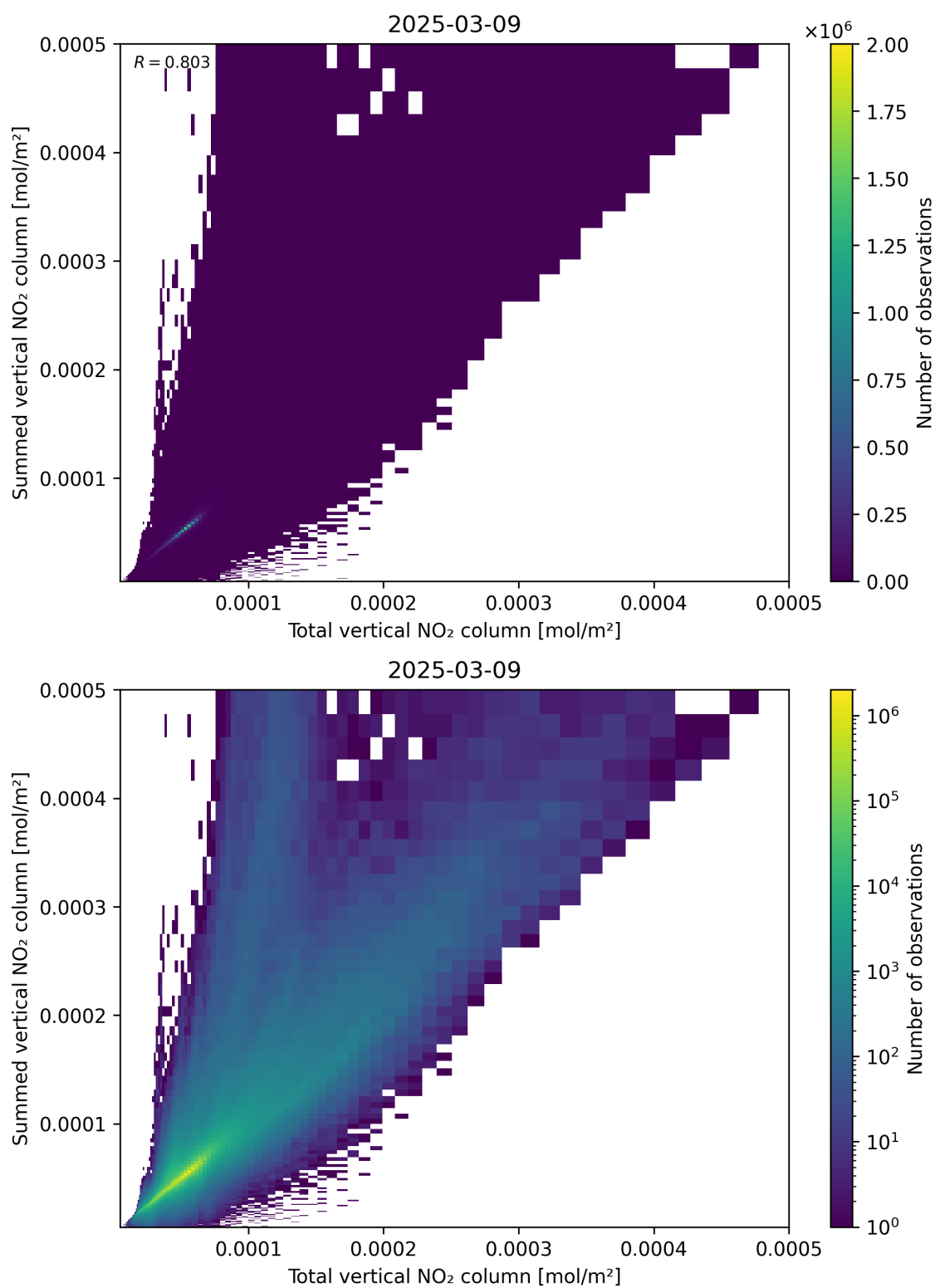
Figure 112: Scatter density plot of “Total vertical NO 2 column” against “Summed vertical NO 2 column” for 2025-03-09 to 2025-03-10.
