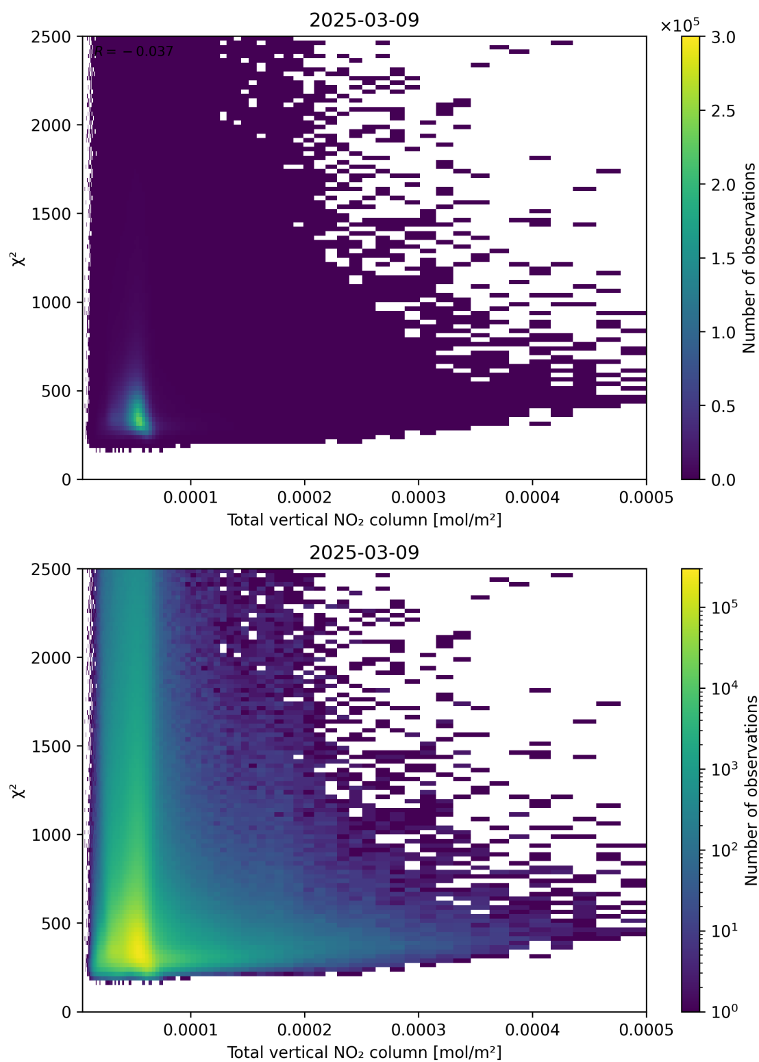
Figure 111: Scatter density plot of “Total vertical NO 2 column” against “ \chi^2 ” for 2025-03-09 to 2025-03-10.
