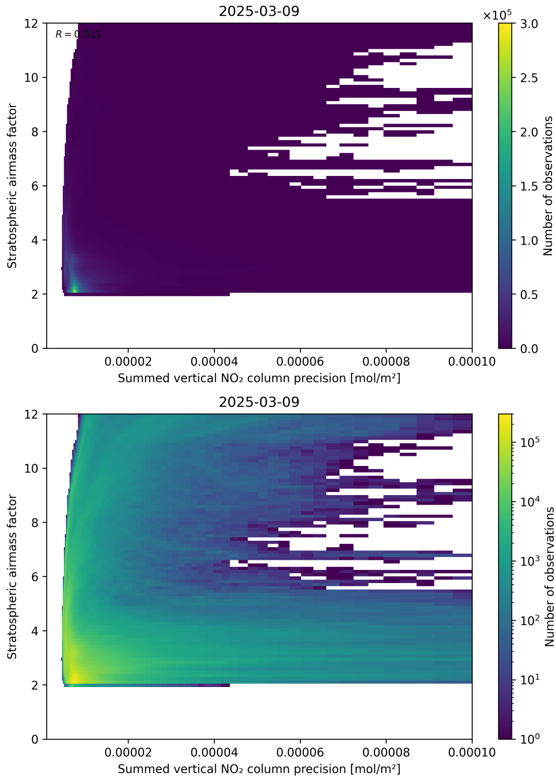
Figure 106: Scatter density plot of “Summed vertical NO 2 column precision” against “Stratospheric airmass factor” for 2025-03-09 to 2025-03-10.
