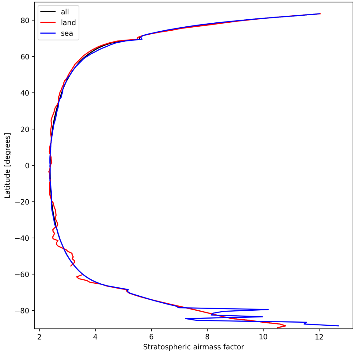
Figure 27: Zonal average of “Stratospheric airmass factor” for 2025-03-09 to 2025-03-10.
