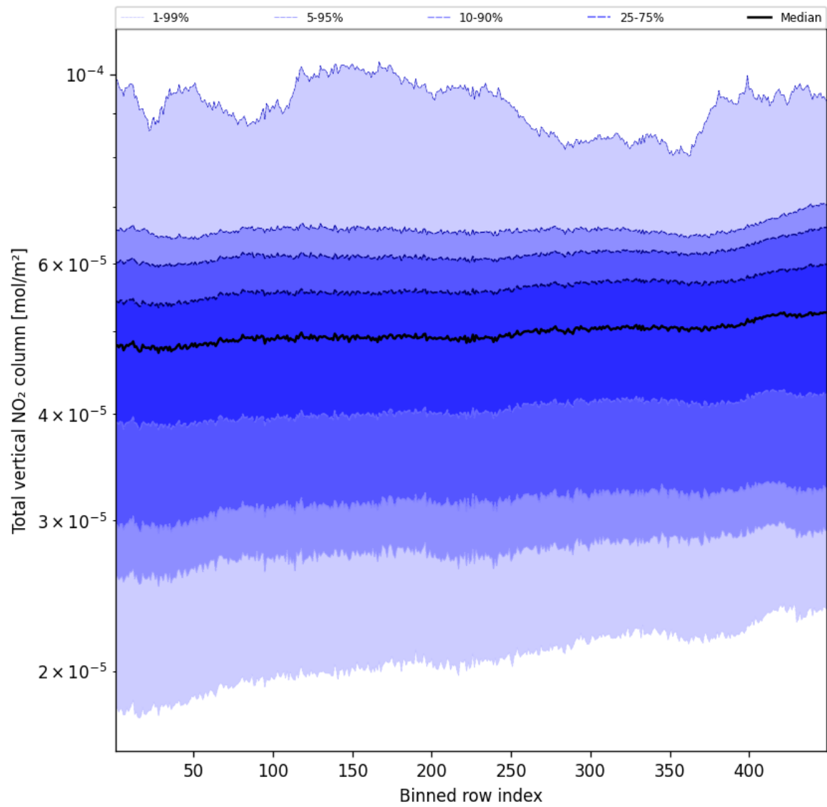
Figure 55: Along track statistics of “Total vertical NO 2 column” for 2025-03-09 to 2025-03-10
