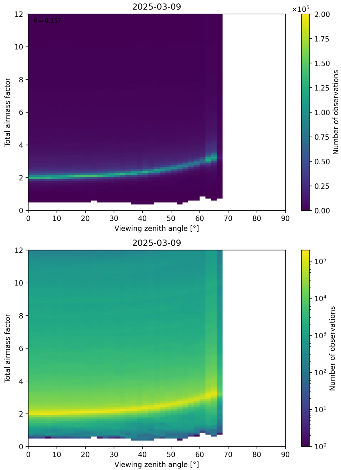
Figure 160: Scatter density plot of “Viewing zenith angle” against “Total airmass factor” for 2025-03-09 to 2025-03-10.
