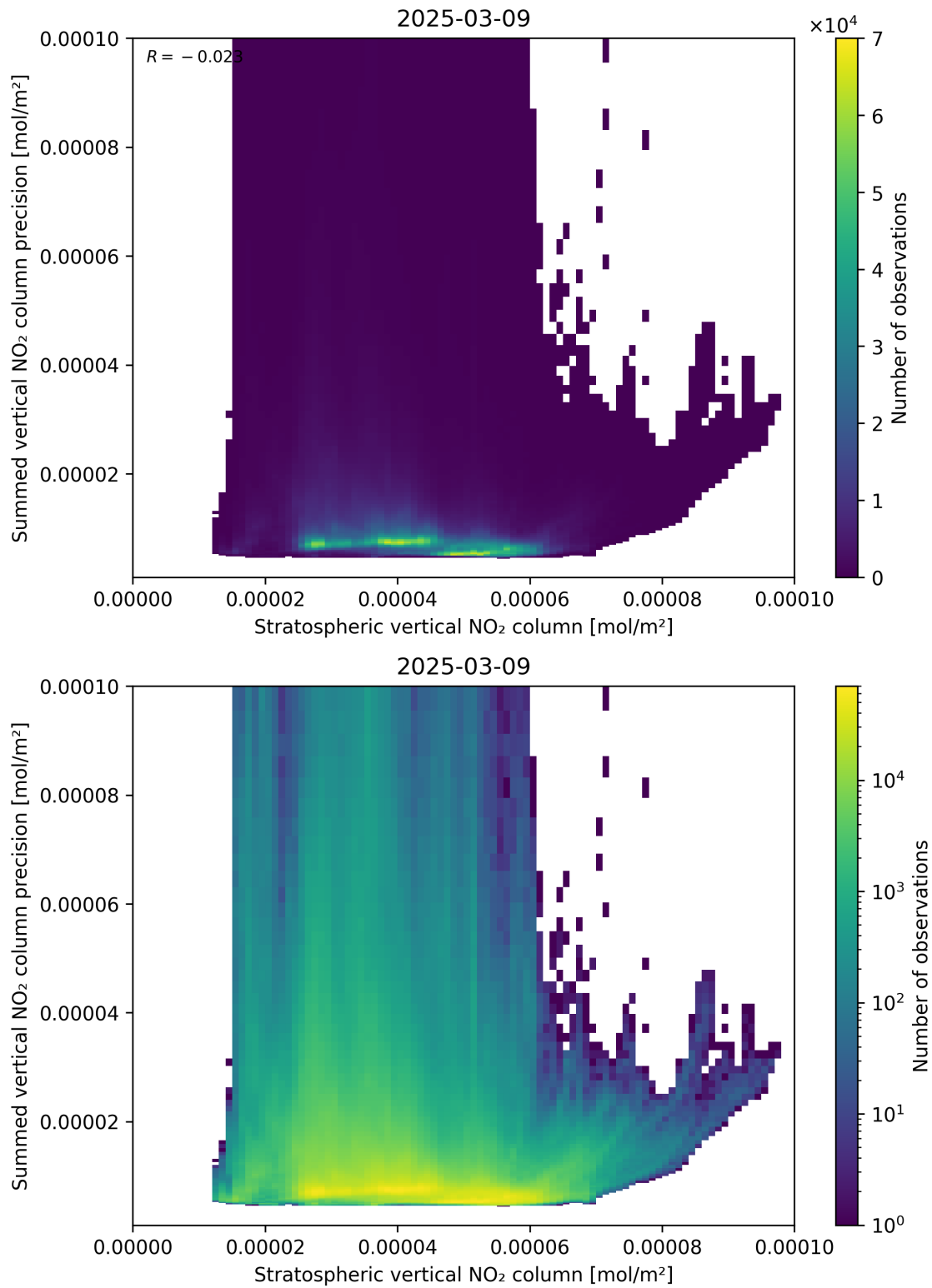
Figure 99: Scatter density plot of “Stratospheric vertical NO 2 column” against “Summed vertical NO 2 column precision” for 2025-03-09 to 2025-03-10.
