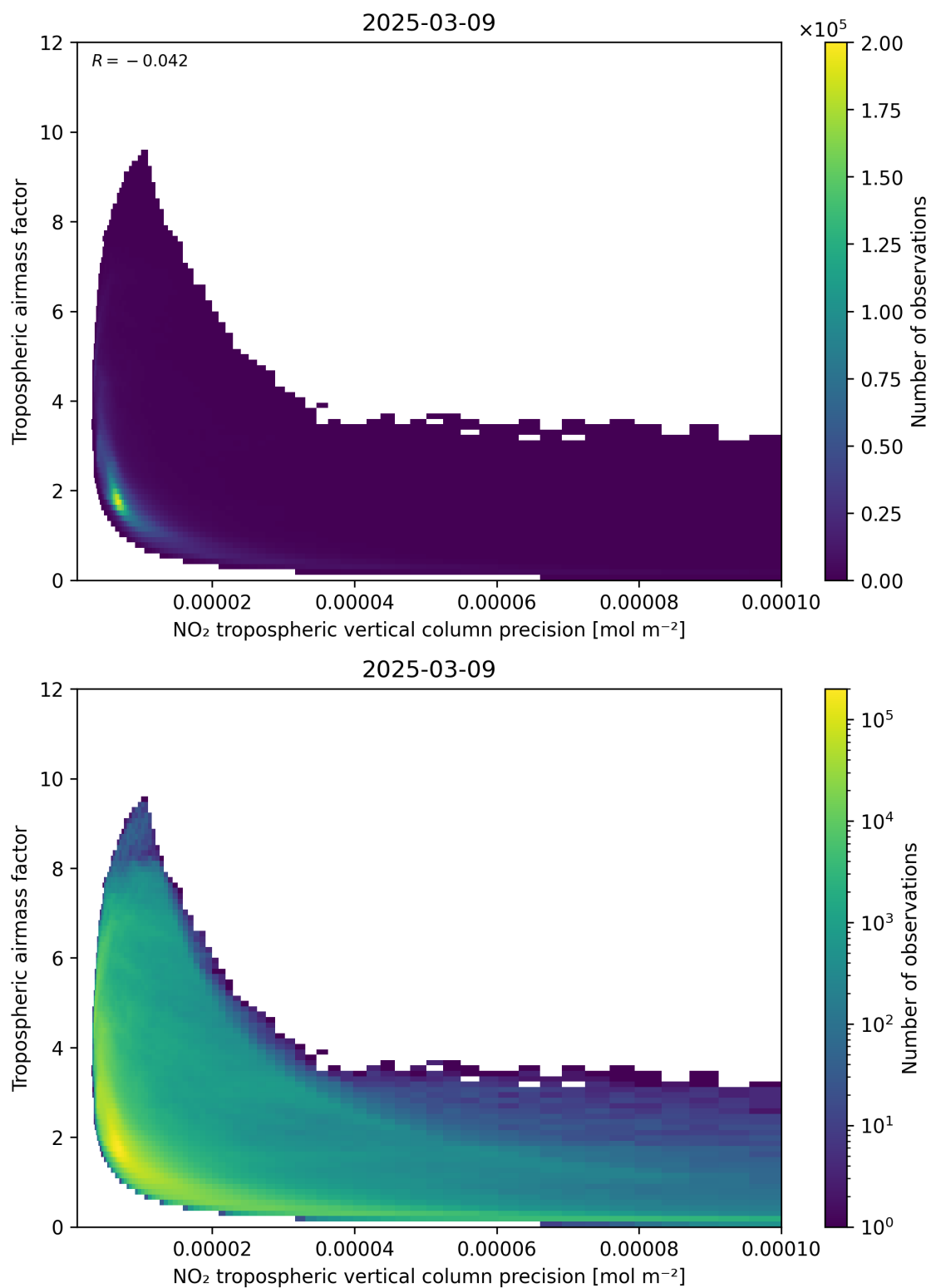
Figure 133: Scatter density plot of “NO 2 tropospheric vertical column precision” against “Tropospheric air mass factor” for 2025-03-09 to 2025-03-10.
