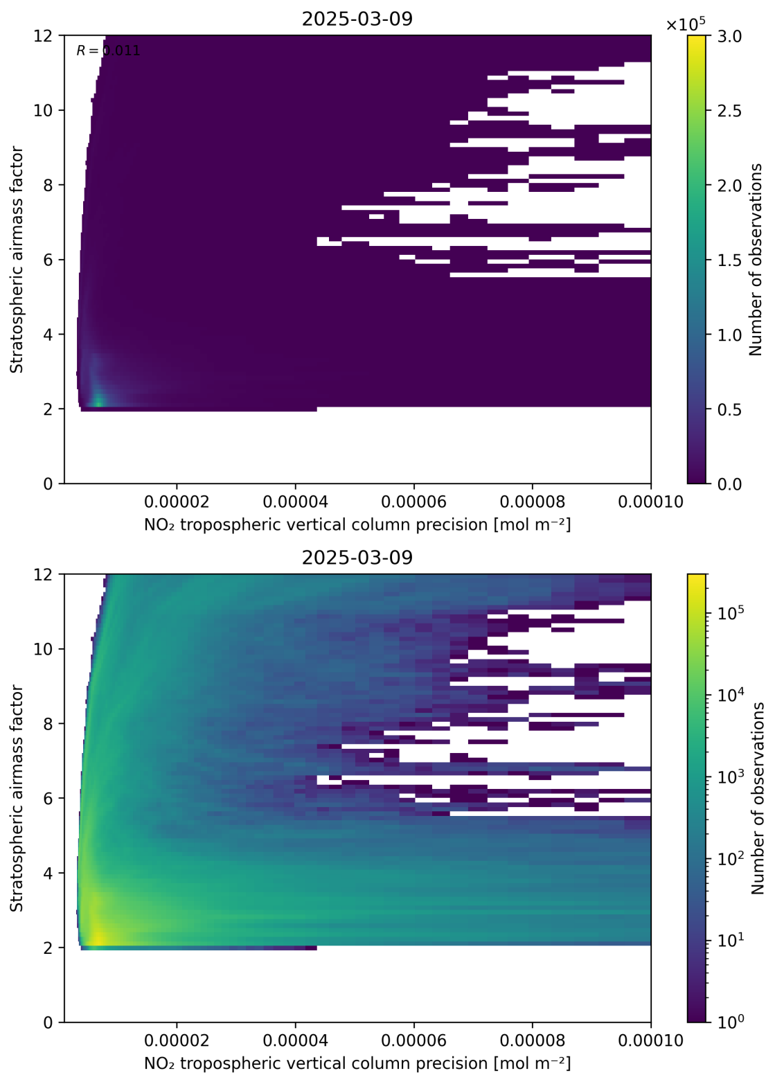
Figure 131: Scatter density plot of “NO 2 tropospheric vertical column precision” against “Stratospheric airmass factor” for 2025-03-09 to 2025-03-10.
