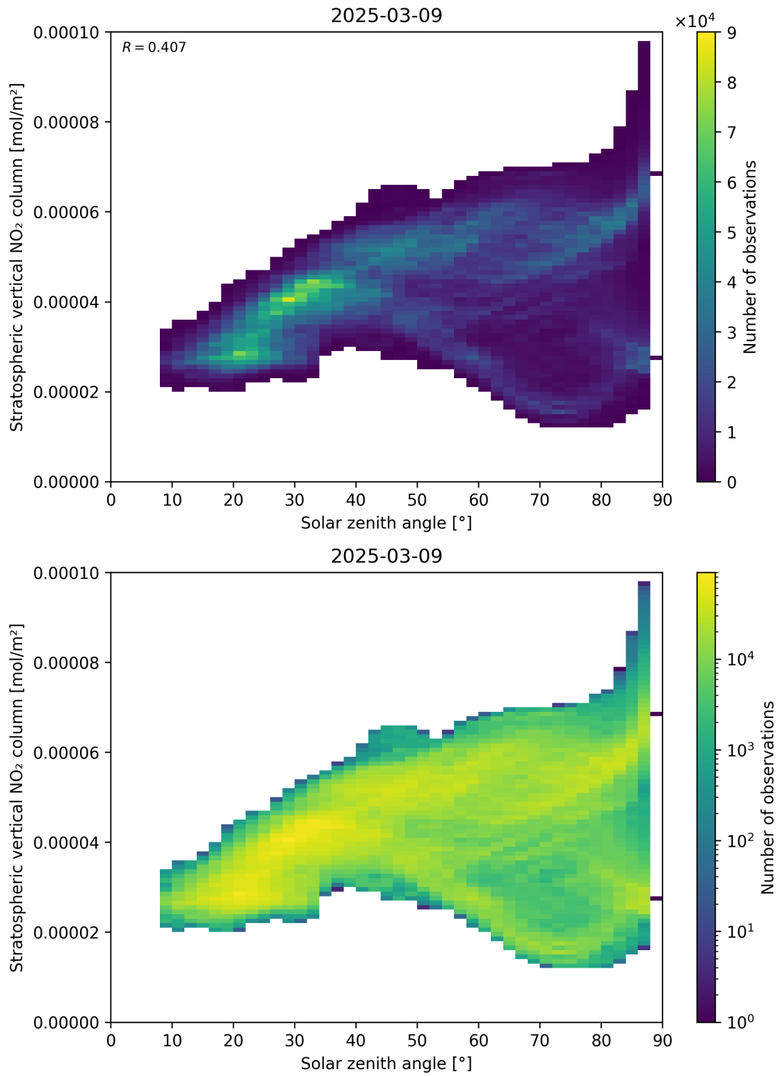
Figure 150: Scatter density plot of “Solar zenith angle” against “Stratospheric vertical NO 2 column” for 2025-03-09 to 2025-03-10.
