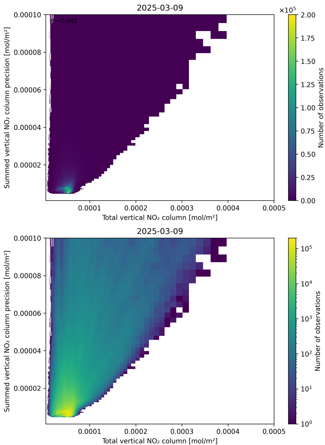
Figure 113: Scatter density plot of “Total vertical NO 2 column” against “Summed vertical NO 2 column precision” for 2025-03-09 to 2025-03-10.
