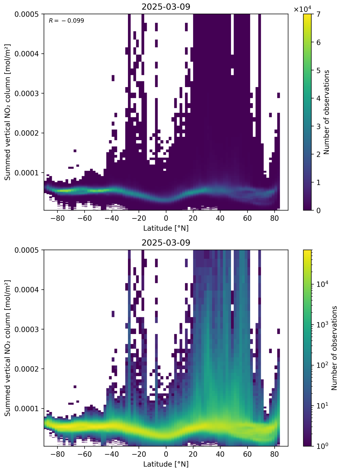
Figure 88: Scatter density plot of “Latitude” against “Summed vertical NO 2 column” for 2025-03-09 to 2025-03-10.
