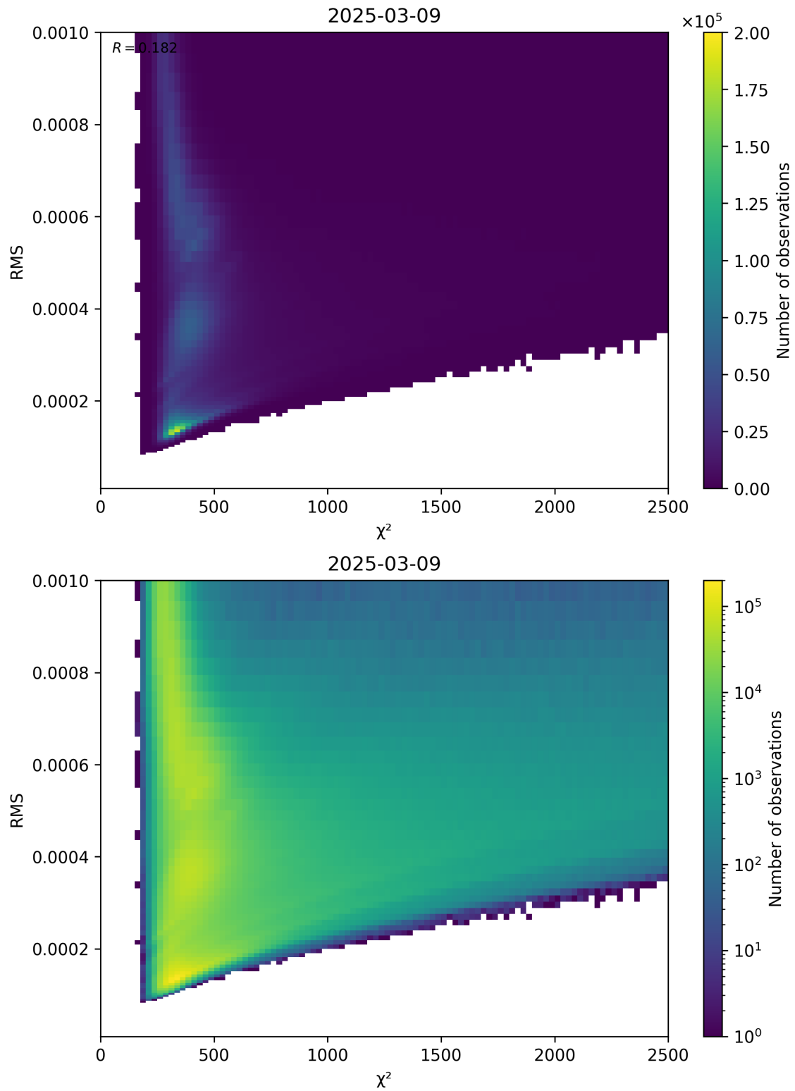
Figure 82: Scatter density plot of “ \chi^2 ” against “RMS” for 2025-03-09 to 2025-03-10.
