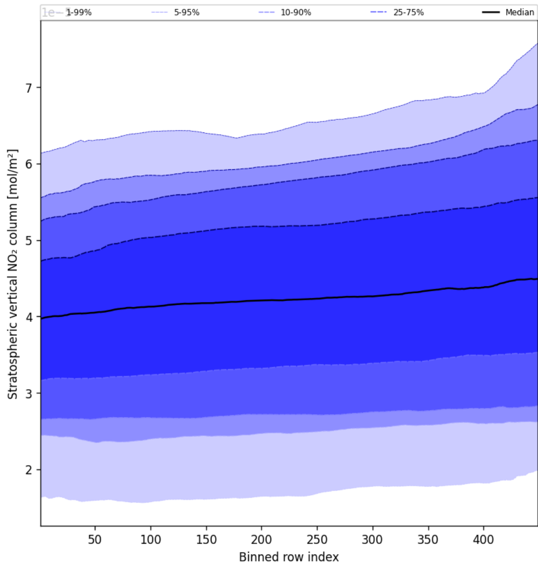
Figure 53: Along track statistics of “Stratospheric vertical NO 2 column” for 2025-03-09 to 2025-03-10
