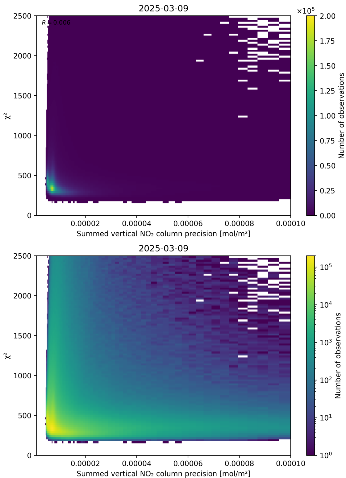
Figure 107: Scatter density plot of “Summed vertical NO 2 column precision” against “ \chi^2 ” for 2025-03-09 to 2025-03-10.
