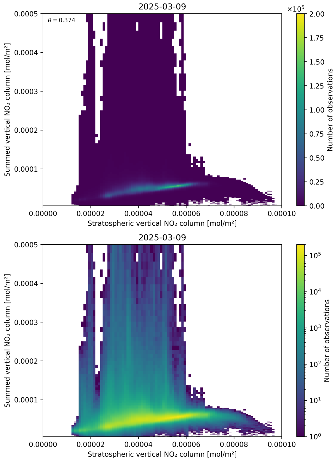
Figure 98: Scatter density plot of “Stratospheric vertical NO 2 column” against “Summed vertical NO 2 column” for 2025-03-09 to 2025-03-10.
