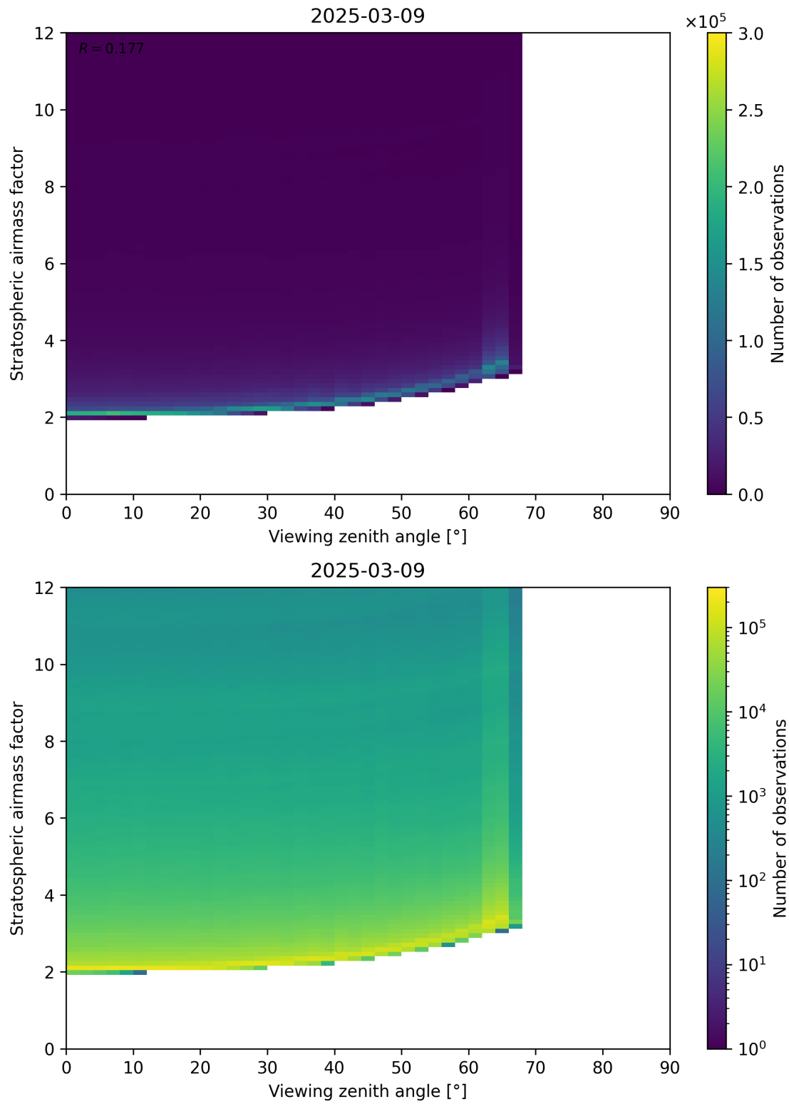
Figure 159: Scatter density plot of “Viewing zenith angle” against “Stratospheric airmass factor” for 2025-03-09 to 2025-03-10.
