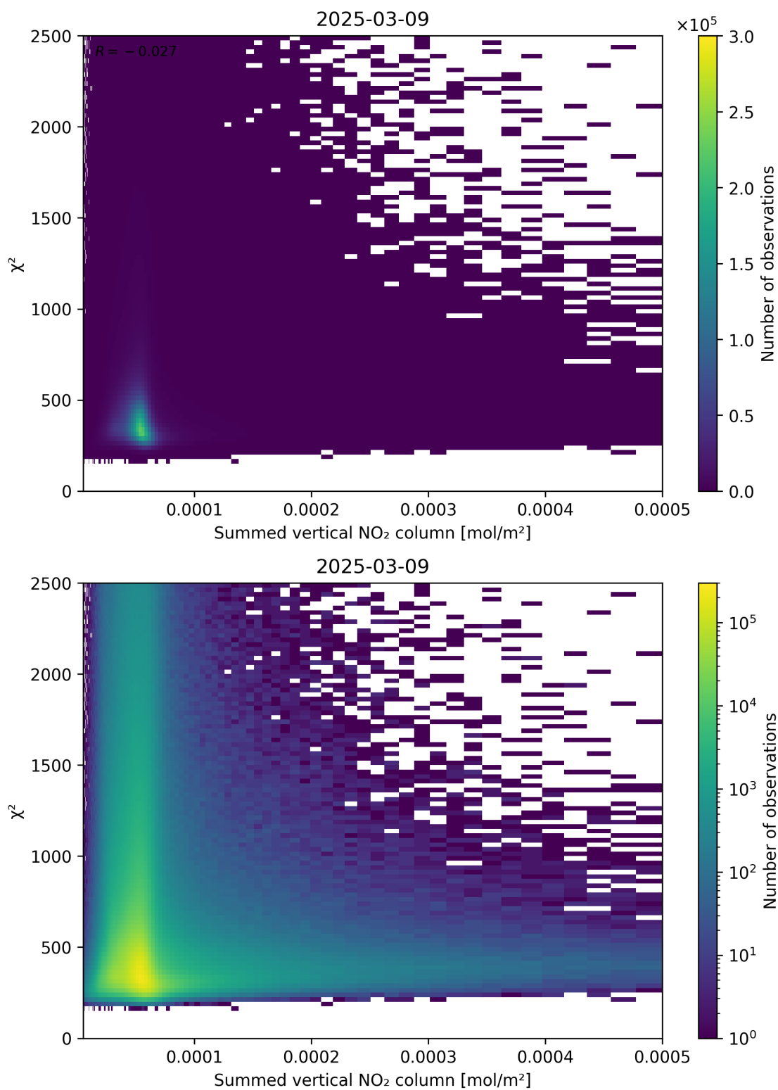
Figure 104: Scatter density plot of “Summed vertical NO 2 column” against “ \chi^2 ” for 2025-03-09 to 2025-03-10.
