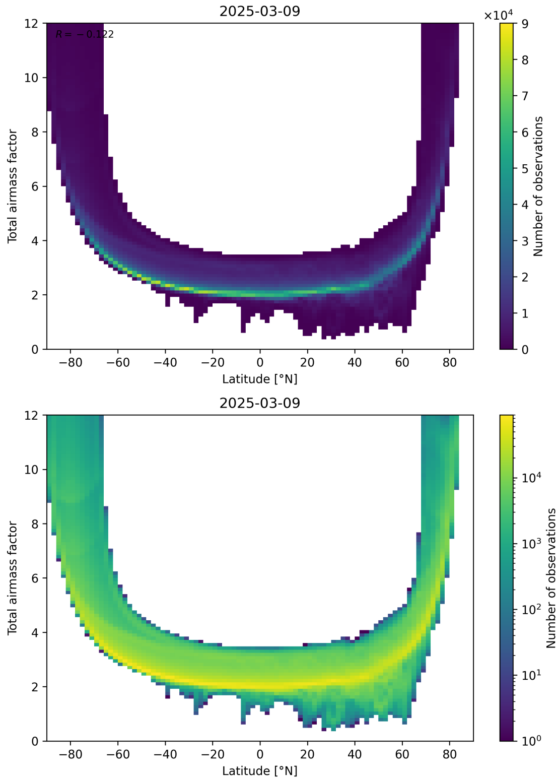
Figure 84: Scatter density plot of “Latitude” against “Total airmass factor” for 2025-03-09 to 2025-03-10.
