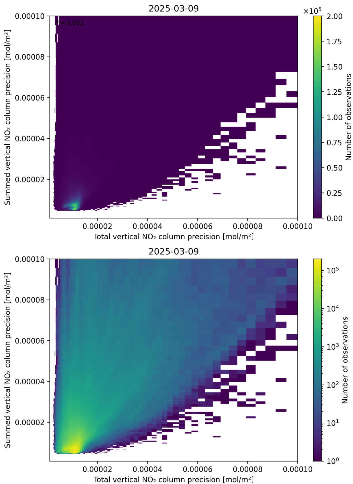
Figure 118: Scatter density plot of “Total vertical NO 2 column precision” against “Summed vertical NO 2 column precision” for 2025-03-09 to 2025-03-10.
