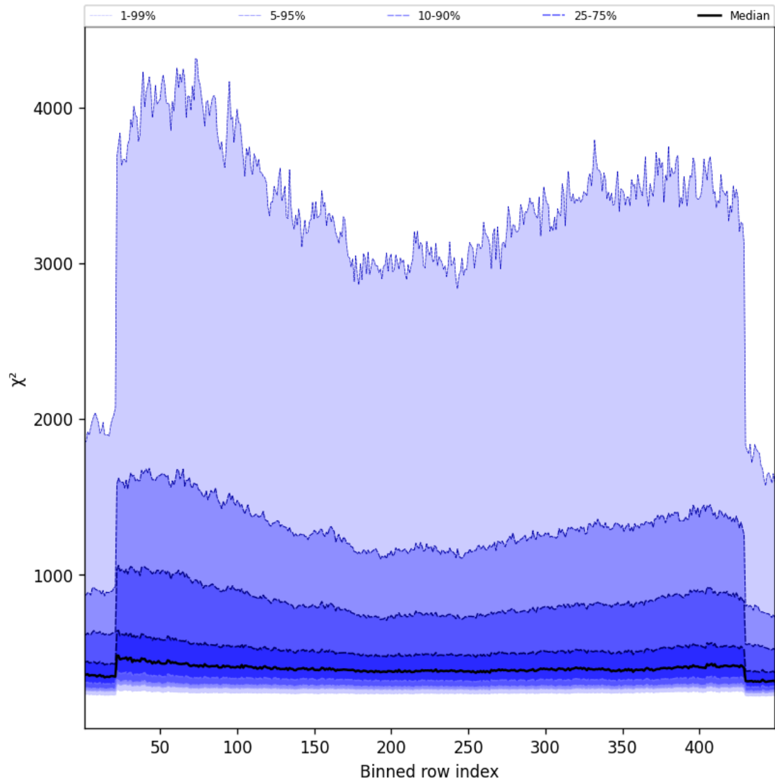
Figure 59: Along track statistics of “ \chi^2 ” for 2025-03-09 to 2025-03-10
