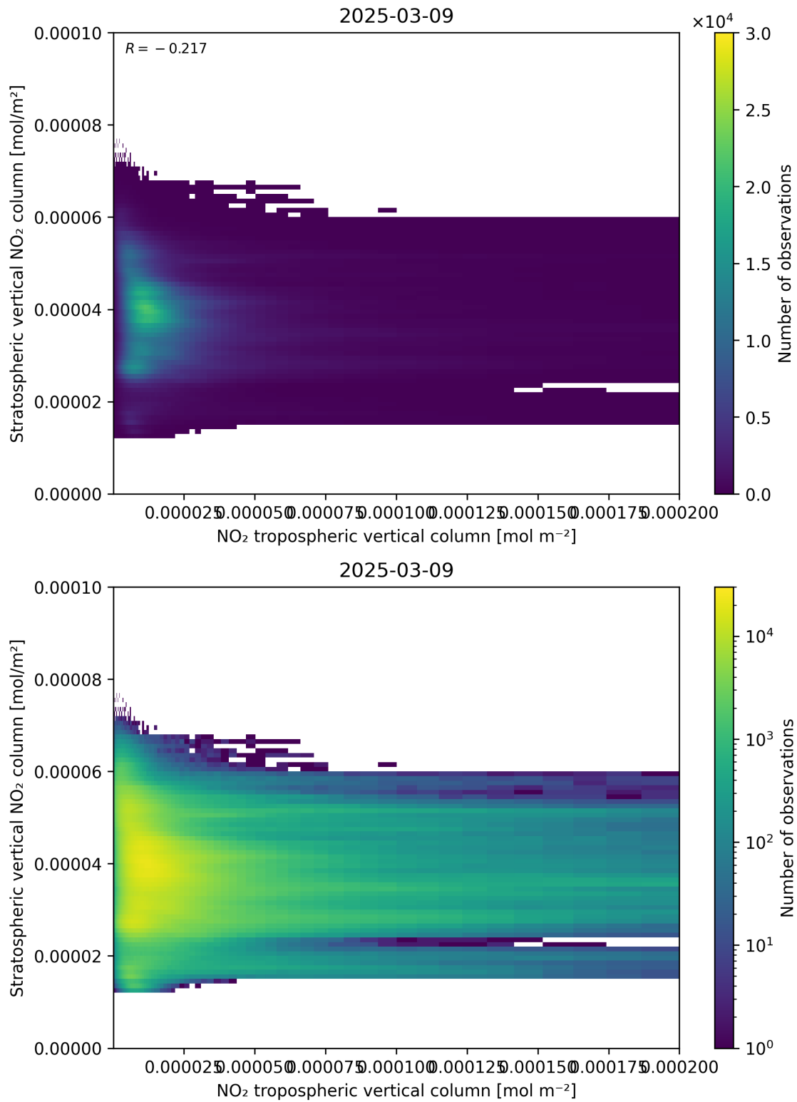
Figure 125: Scatter density plot of “NO 2 tropospheric vertical column” against “Stratospheric vertical NO 2 column” for 2025-03-09 to 2025-03-10.
