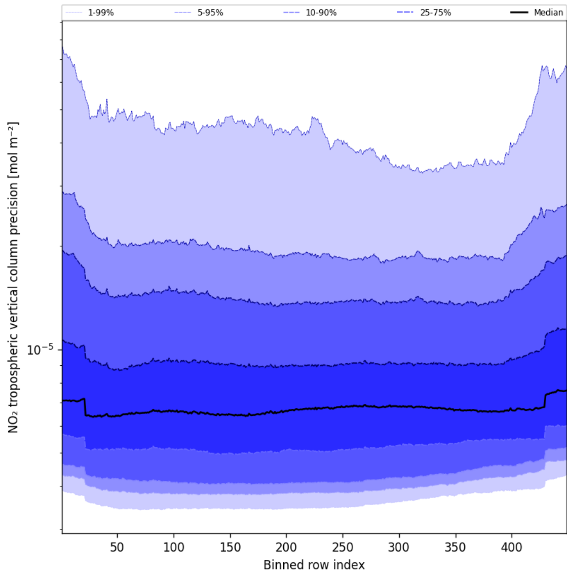
Figure 47: Along track statistics of “NO 2 tropospheric vertical column precision” for 2025-03-09 to 2025-03-10
