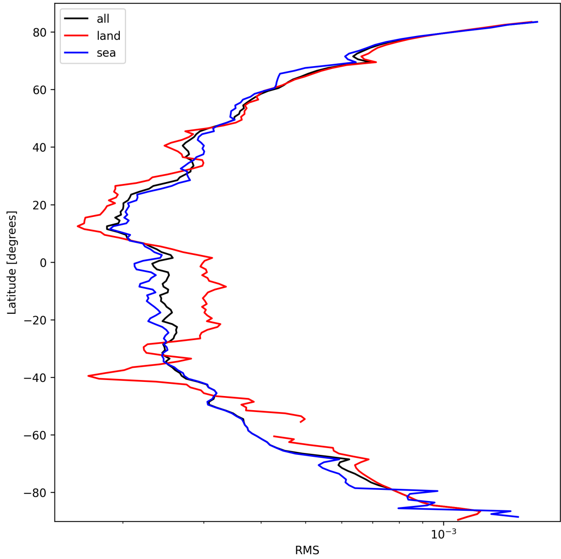
Figure 26: Zonal average of “RMS” for 2025-03-09 to 2025-03-10.
