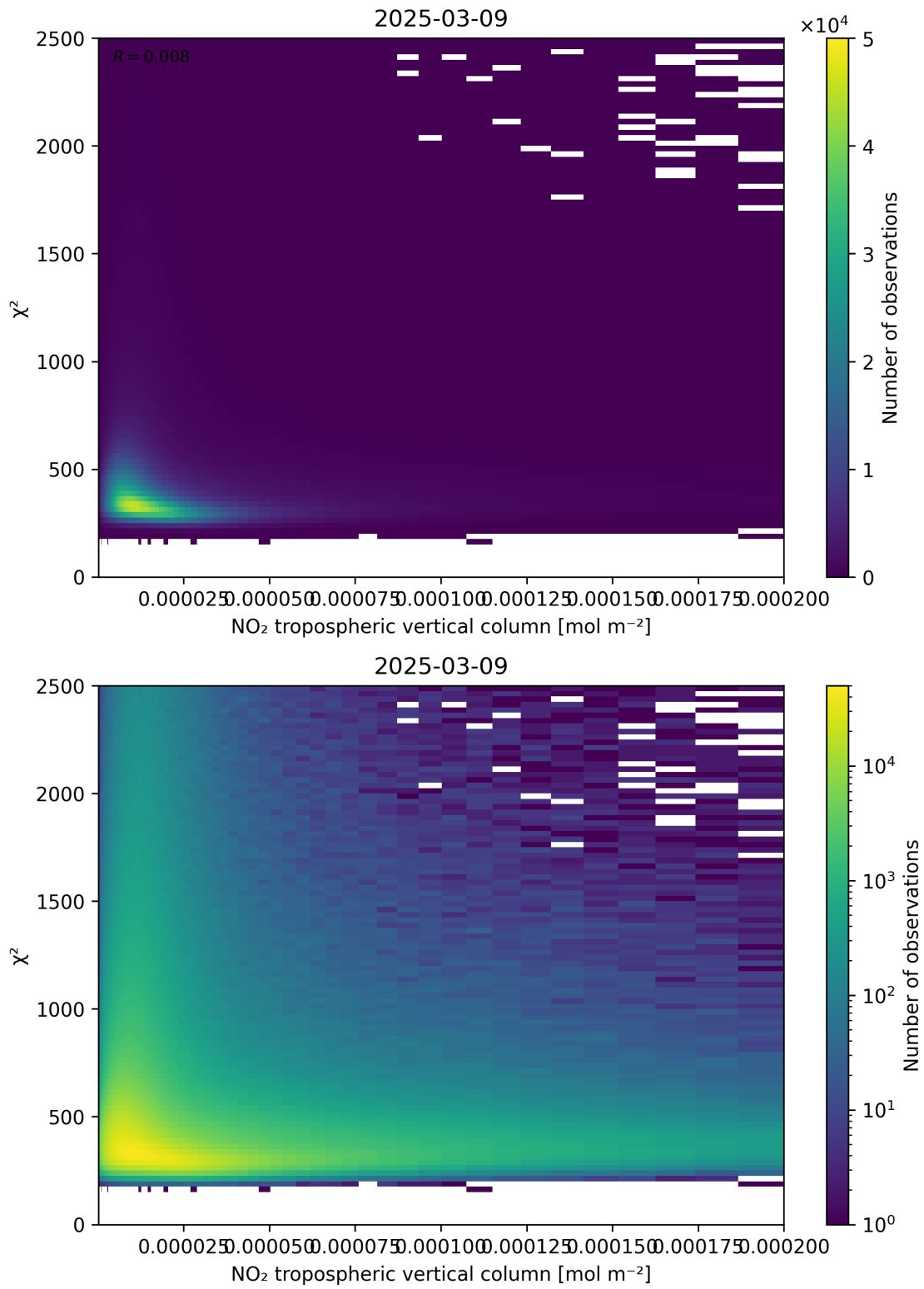
Figure 124: Scatter density plot of “NO 2 tropospheric vertical column” against “ \chi^2 ” for 2025-03-09 to 2025-03-10.
