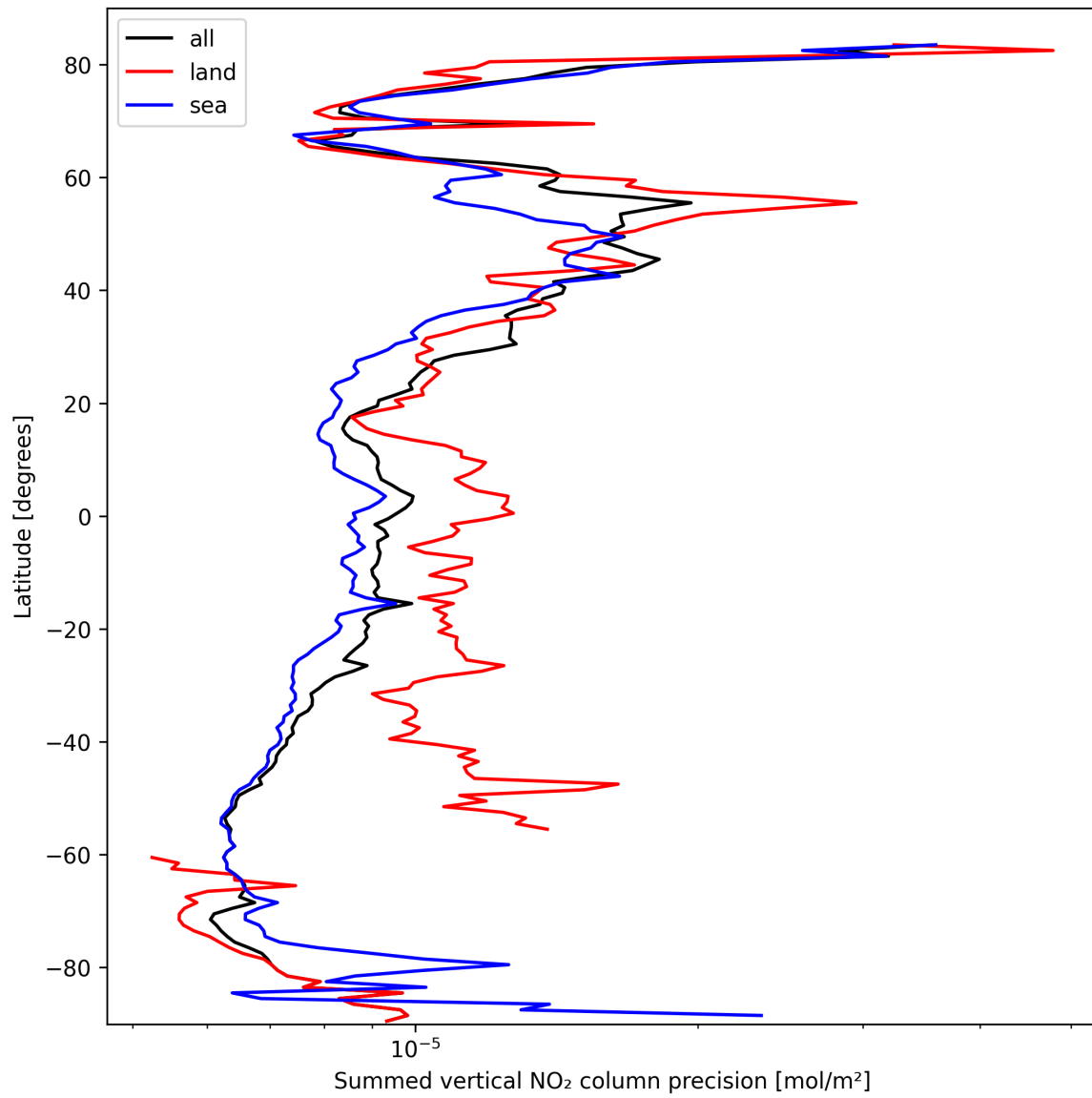
Figure 24: Zonal average of “Summed vertical NO 2 column precision” for 2025-03-09 to 2025-03-10.
