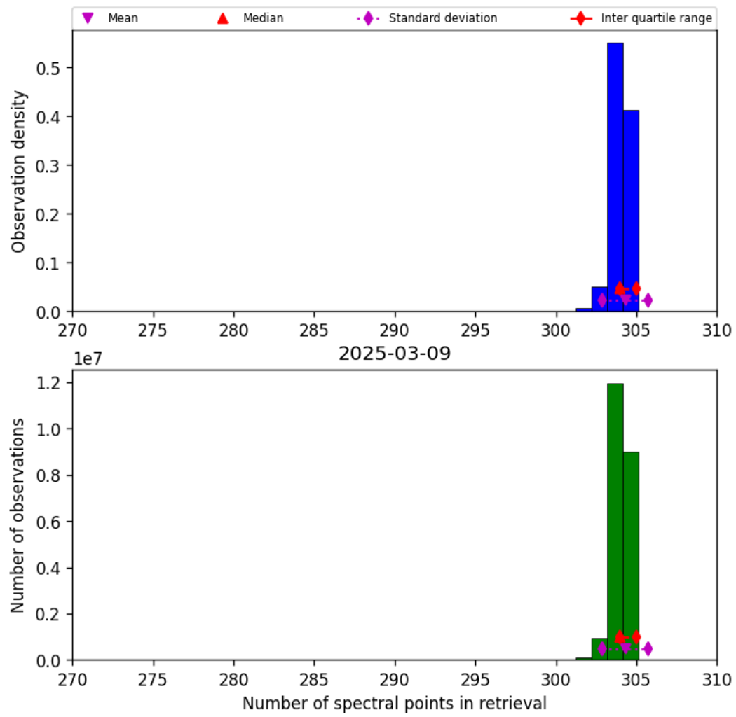
Figure 33: Histogram of “Number of spectral points in retrieval” for 2025-03-09 to 2025-03-10
