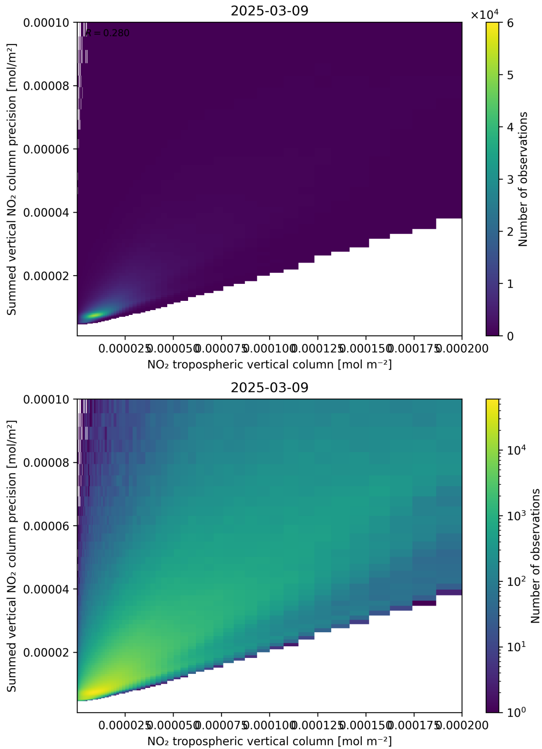
Figure 127: Scatter density plot of “NO 2 tropospheric vertical column” against “Summed vertical NO 2 column precision” for 2025-03-09 to 2025-03-10.
