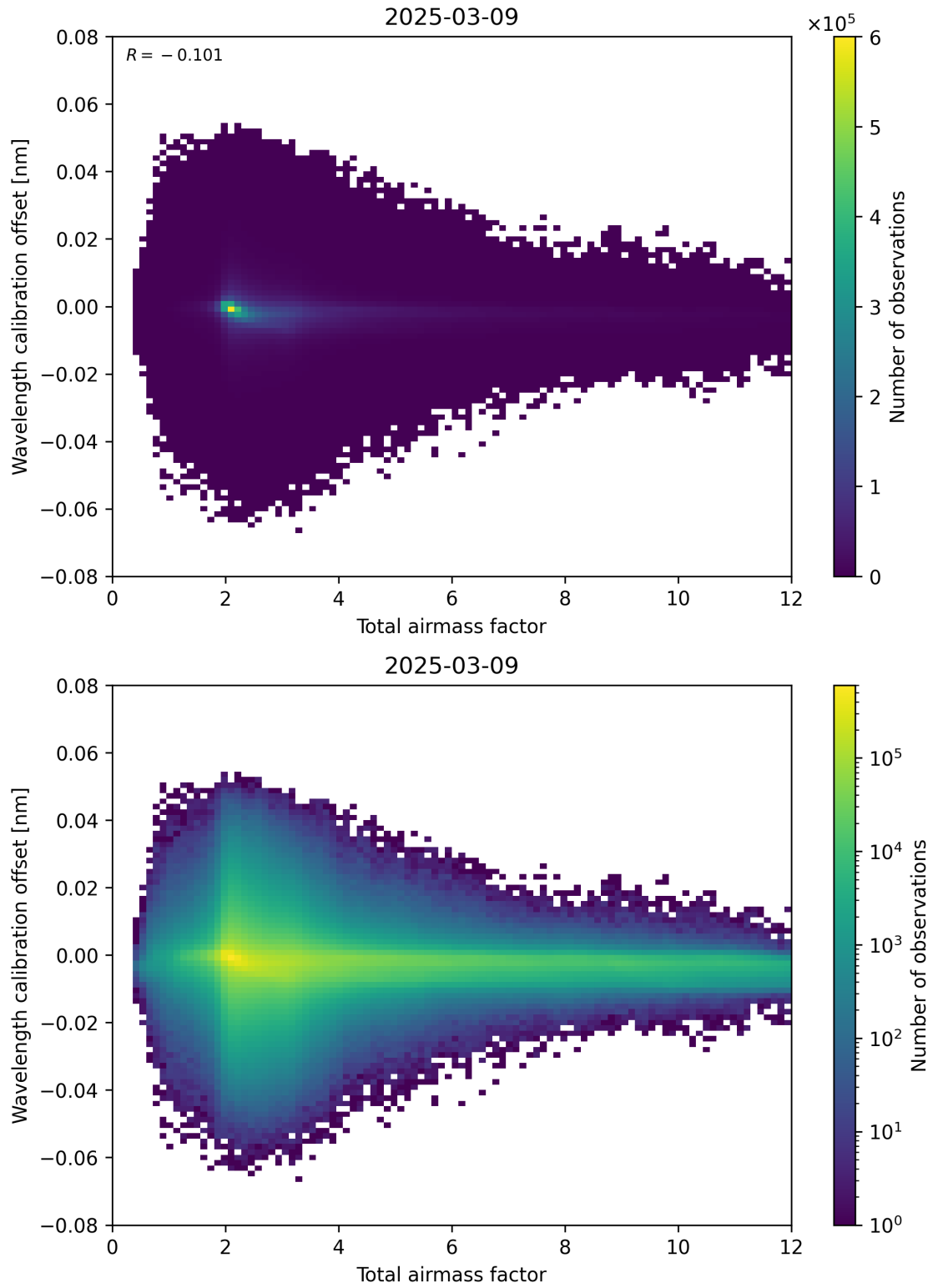
Figure 70: Scatter density plot of “Total airmass factor” against “Wavelength calibration offset” for 2025-03-09 to 2025-03-10.
