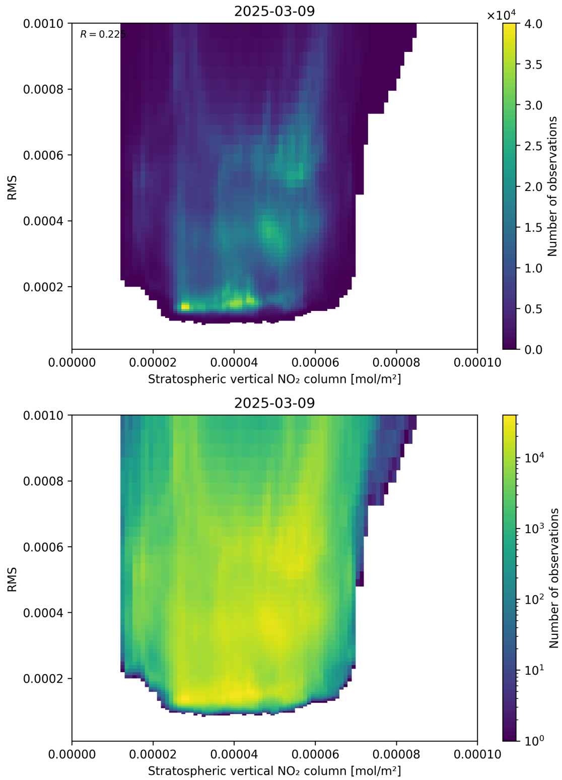
Figure 102: Scatter density plot of “Stratospheric vertical NO 2 column” against “RMS” for 2025-03-09 to 2025-03-10.
