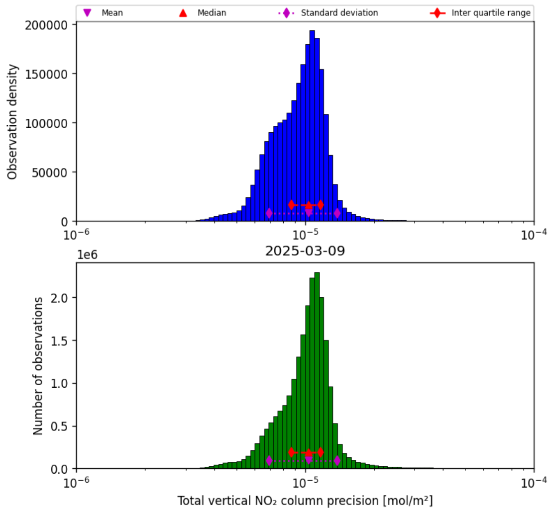
Figure 39: Histogram of “Total vertical NO 2 column precision” for 2025-03-09 to 2025-03-10
