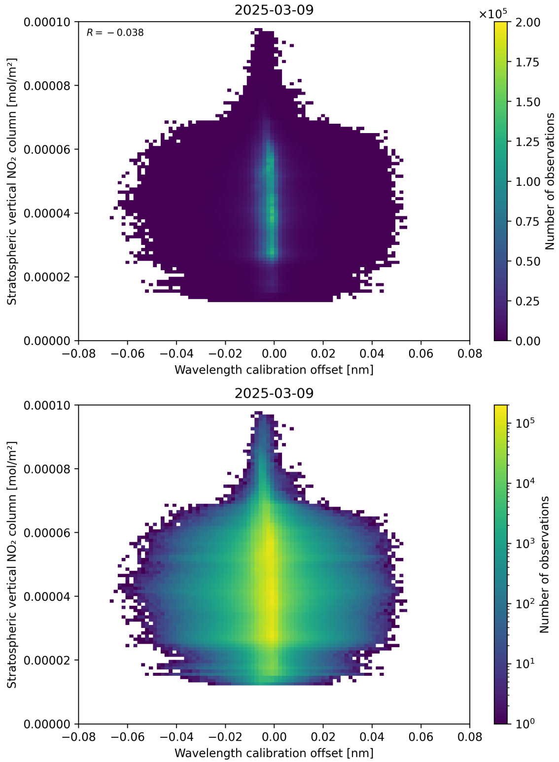
Figure 176: Scatter density plot of “Wavelength calibration offset” against “Stratospheric vertical NO 2 column” for 2025-03-09 to 2025-03-10.
