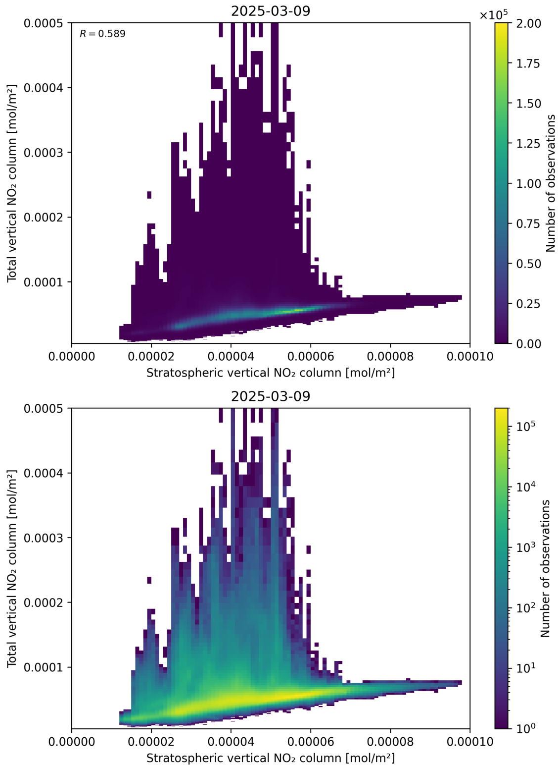
Figure 100: Scatter density plot of “Stratospheric vertical NO 2 column” against “Total vertical NO 2 column” for 2025-03-09 to 2025-03-10.
