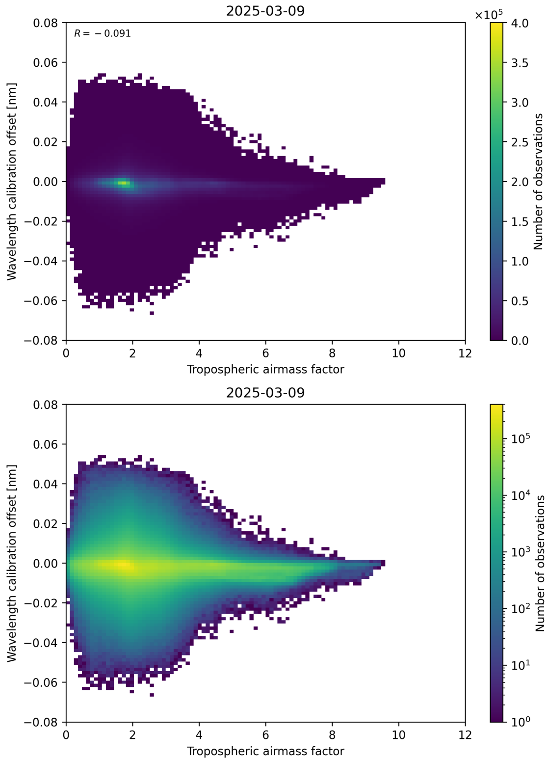
Figure 80: Scatter density plot of “Tropospheric airmass factor” against “Wavelength calibration offset” for 2025-03-09 to 2025-03-10.
