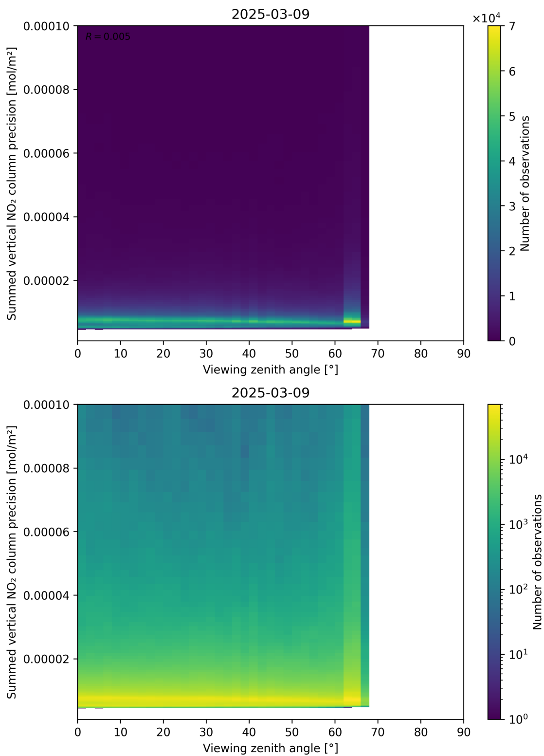
Figure 166: Scatter density plot of “Viewing zenith angle” against “Summed vertical NO 2 column precision” for 2025-03-09 to 2025-03-10.
