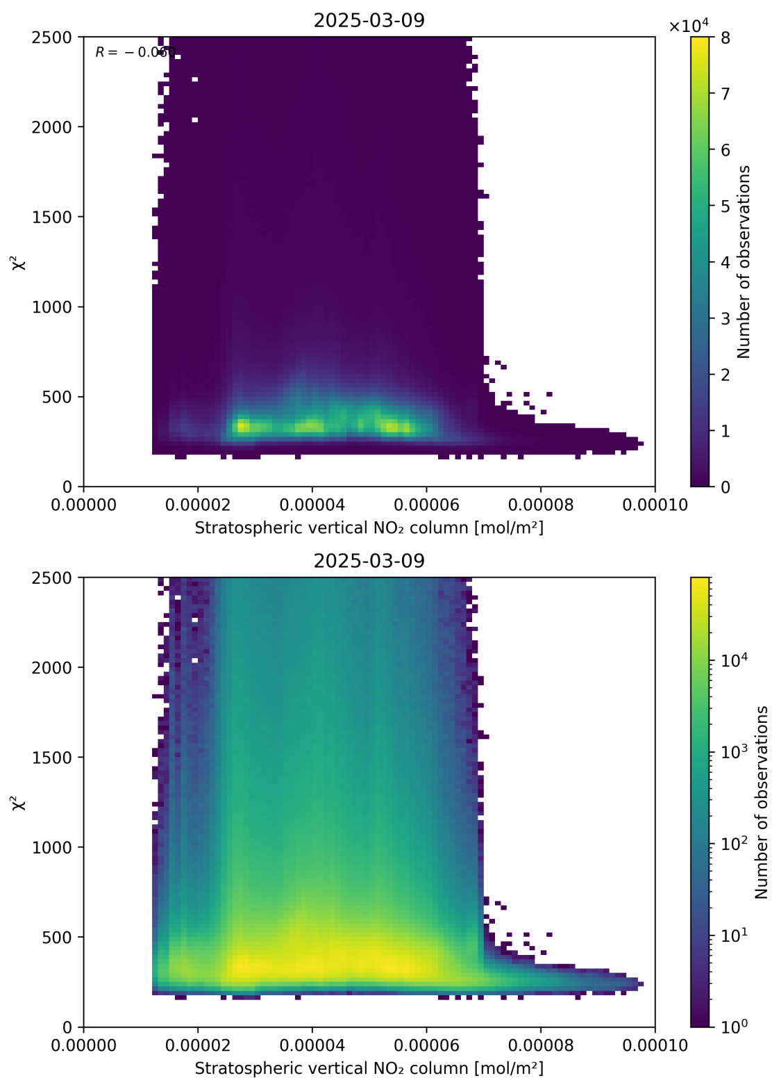
Figure 97: Scatter density plot of “Stratospheric vertical NO 2 column” against “ \chi^2 ” for 2025-03-09 to 2025-03-10.
