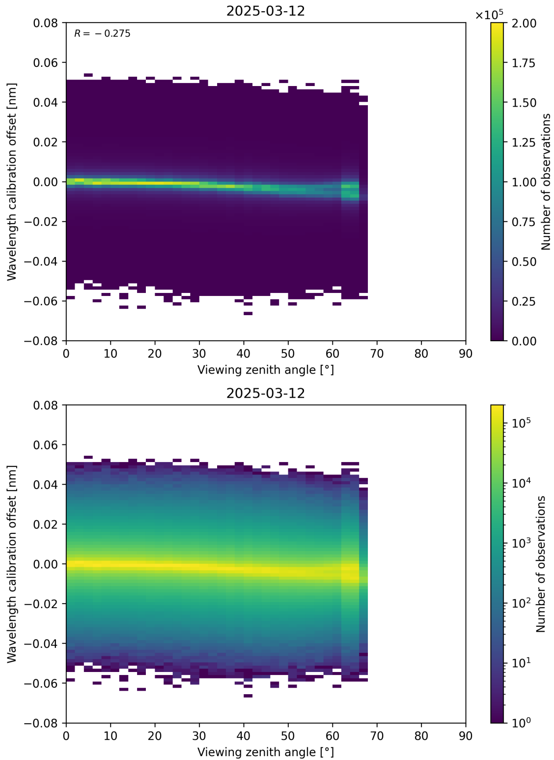
Figure 173: Scatter density plot of “Viewing zenith angle” against “Wavelength calibration offset” for 2025-03-12 to 2025-03-13.
