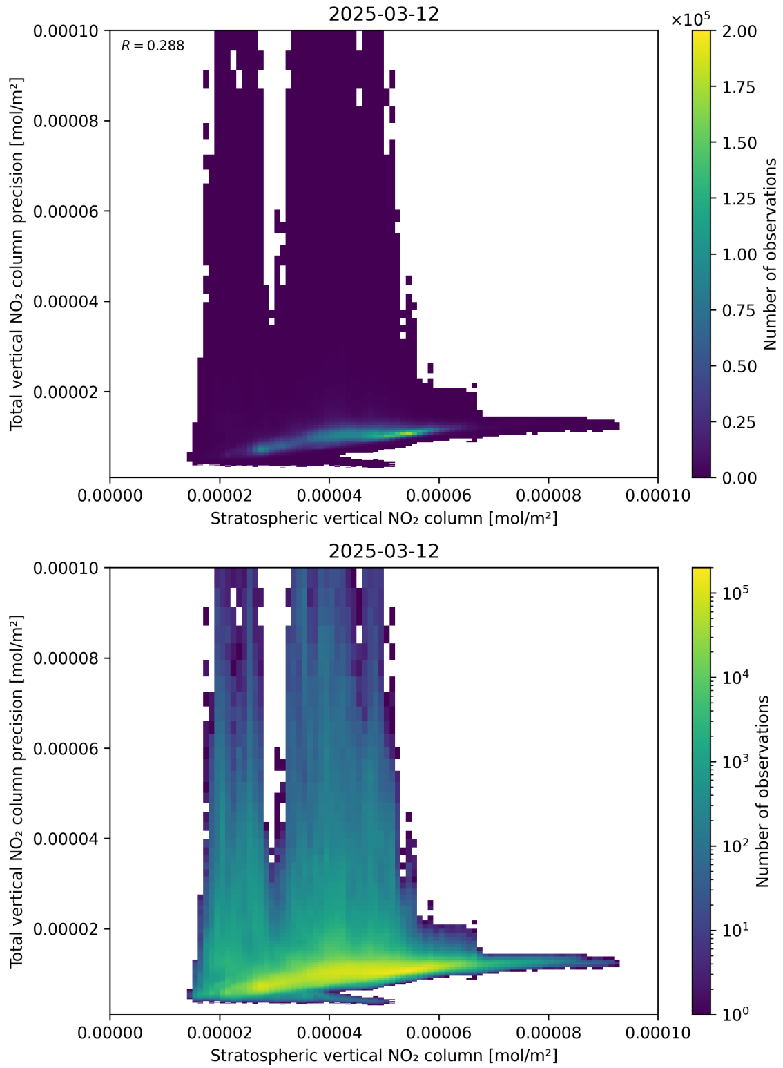
Figure 101: Scatter density plot of “Stratospheric vertical NO 2 column” against “Total vertical NO 2 column precision” for 2025-03-12 to 2025-03-13.
