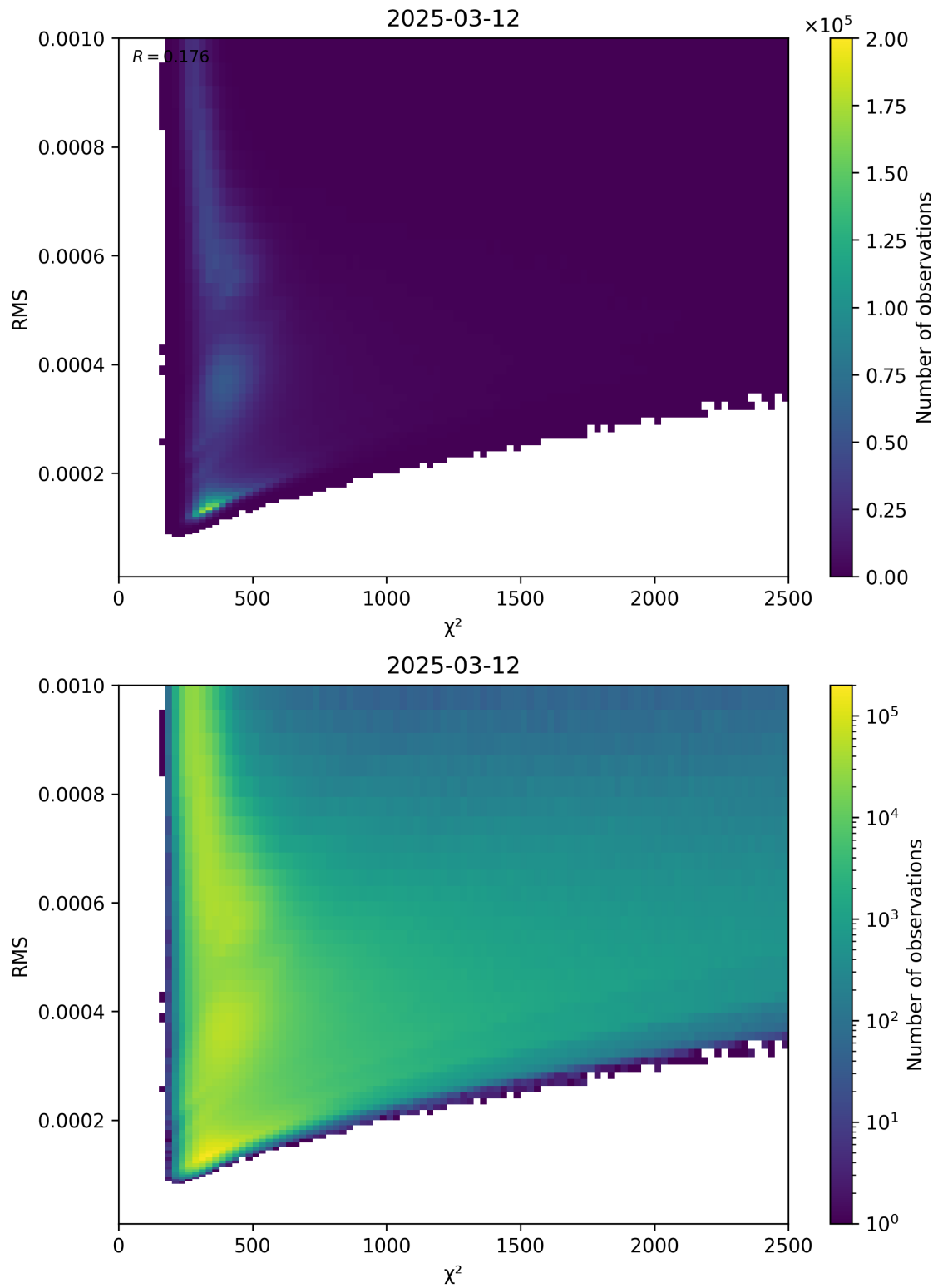
Figure 82: Scatter density plot of “ \chi^2 ” against “RMS” for 2025-03-12 to 2025-03-13.
