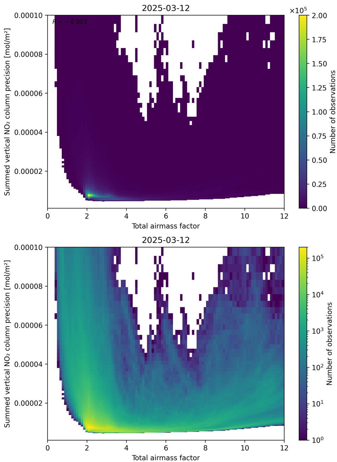
Figure 66: Scatter density plot of “Total airmass factor” against “Summed vertical NO 2 column precision” for 2025-03-12 to 2025-03-13.
