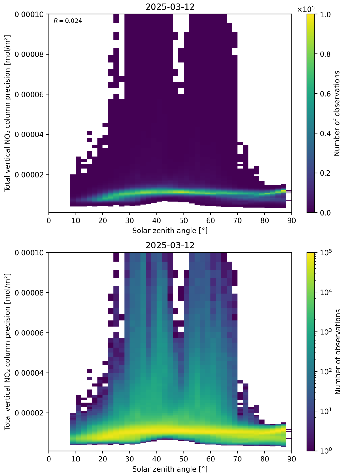
Figure 154: Scatter density plot of “Solar zenith angle” against “Total vertical NO 2 column precision” for 2025-03-12 to 2025-03-13.
