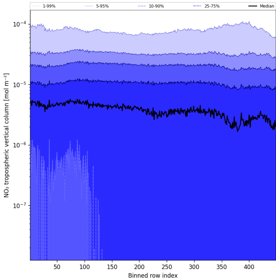
Figure 46: Along track statistics of “NO 2 tropospheric vertical column” for 2025-03-12 to 2025-03-13
