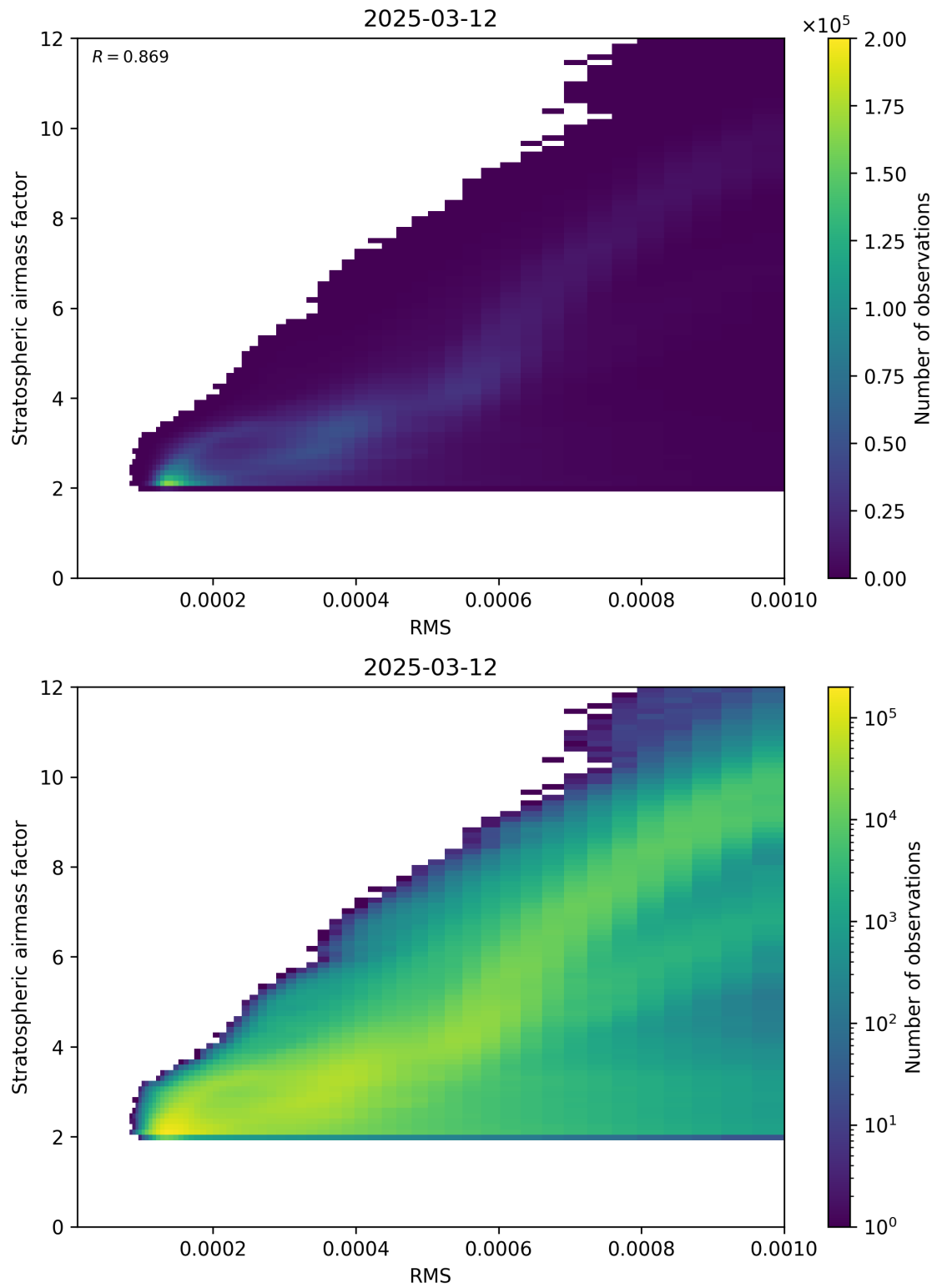
Figure 144: Scatter density plot of “RMS” against “Stratospheric airmass factor” for 2025-03-12 to 2025-03-13.
