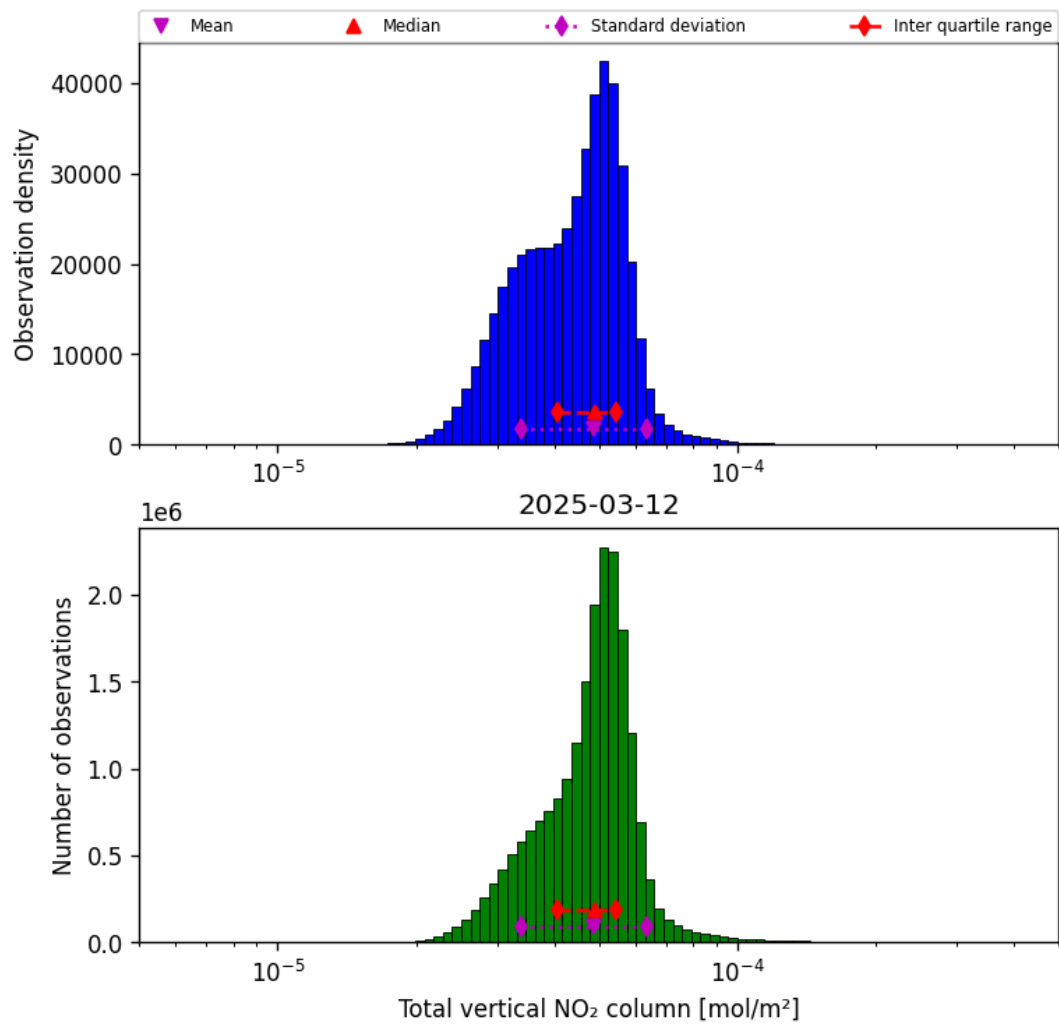
Figure 38: Histogram of “Total vertical NO 2 column” for 2025-03-12 to 2025-03-13
