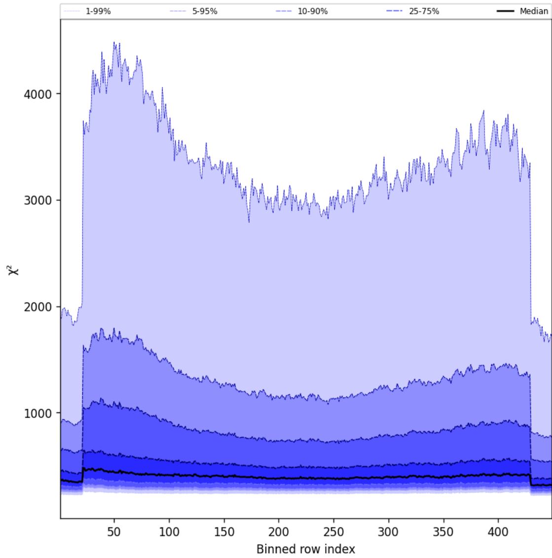
Figure 59: Along track statistics of “ \chi^2 ” for 2025-03-12 to 2025-03-13
