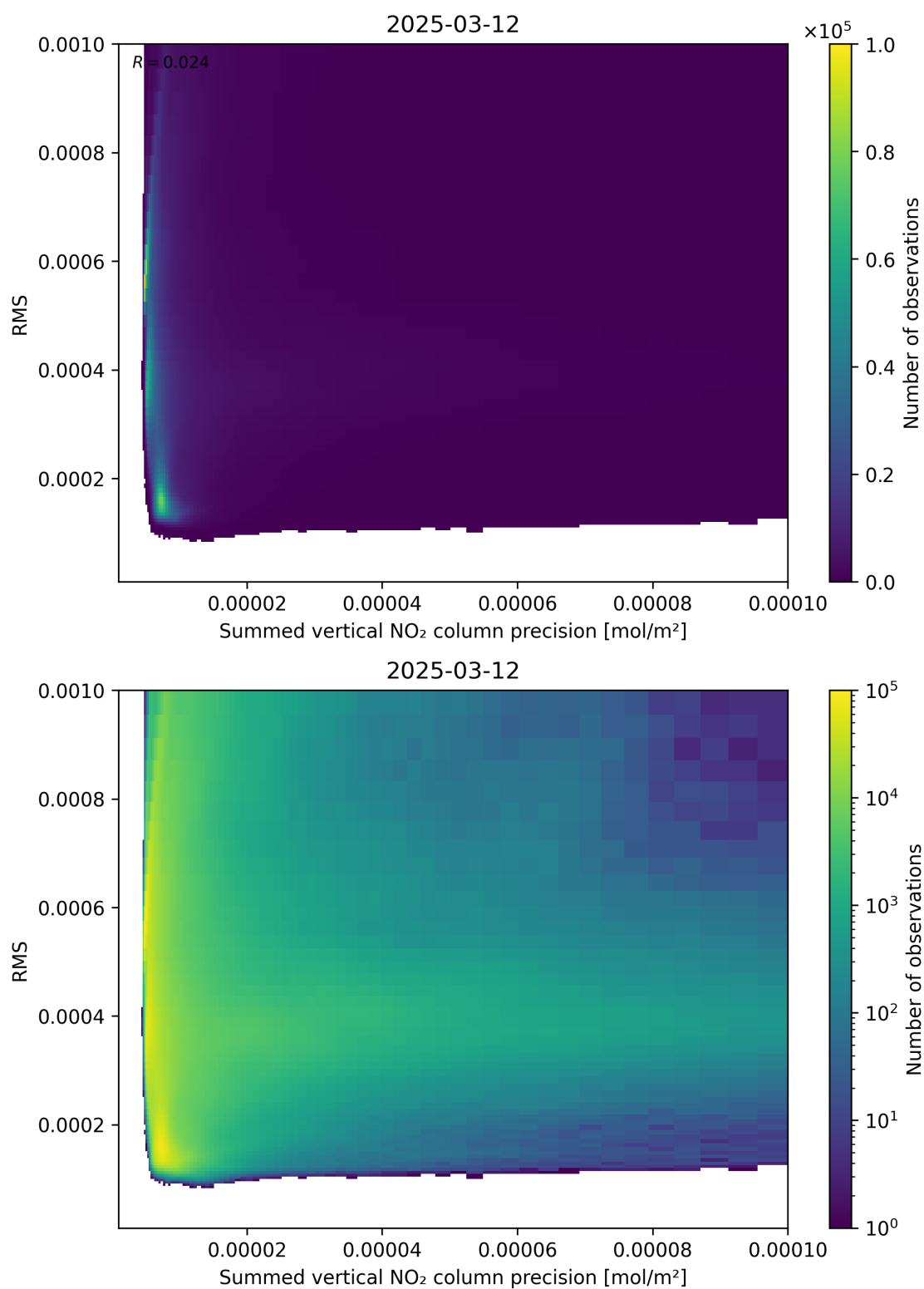
Figure 108: Scatter density plot of “Summed vertical NO 2 column precision” against “RMS” for 2025-03-12 to 2025-03-13.
