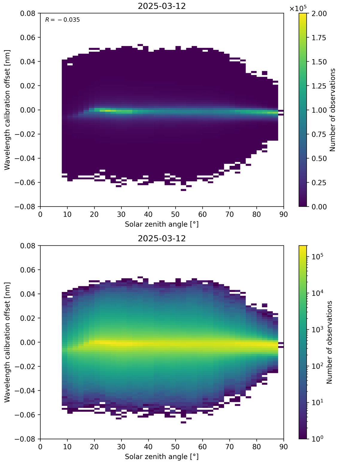
Figure 158: Scatter density plot of “Solar zenith angle” against “Wavelength calibration offset” for 2025-03-12 to 2025-03-13.
