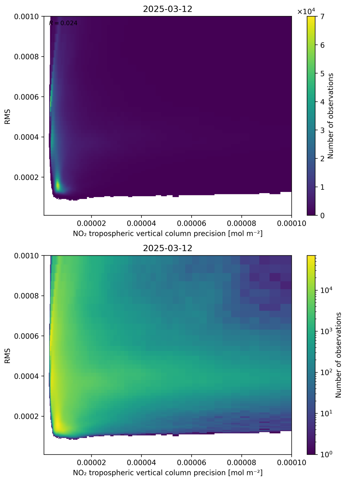
Figure 140: Scatter density plot of “NO 2 tropospheric vertical column precision” against “RMS” for 2025-03-12 to 2025-03-13.
