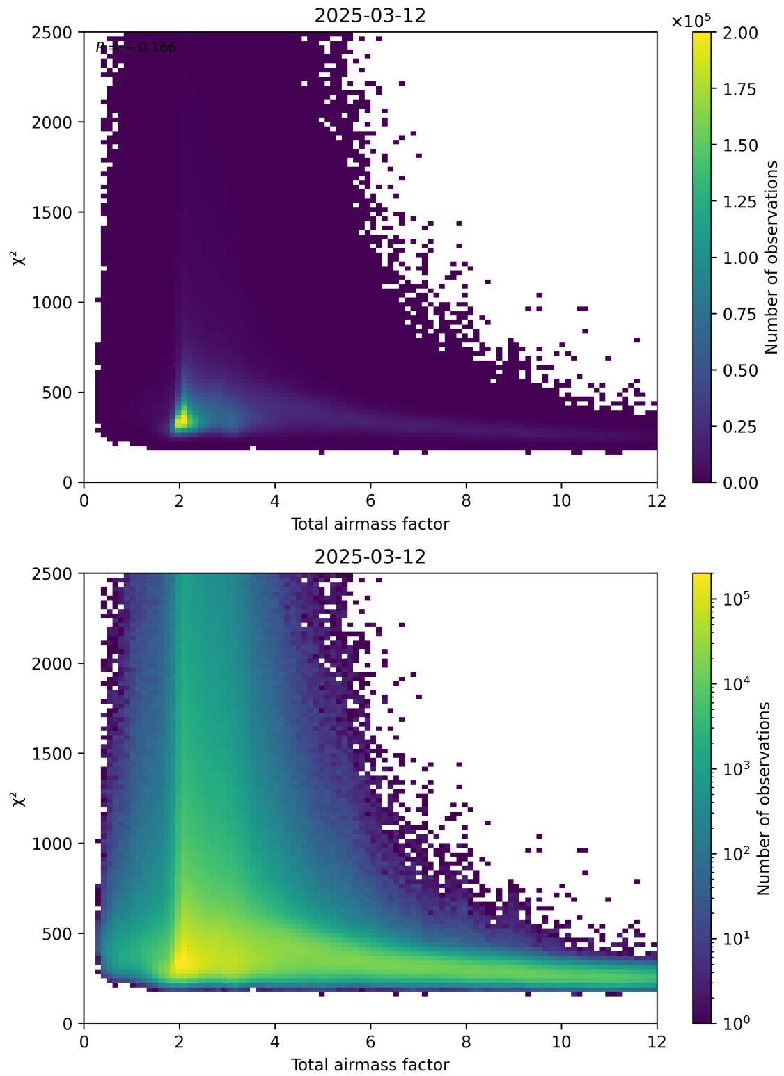
Figure 63: Scatter density plot of “Total airmass factor” against “ \chi^2 ” for 2025-03-12 to 2025-03-13.
