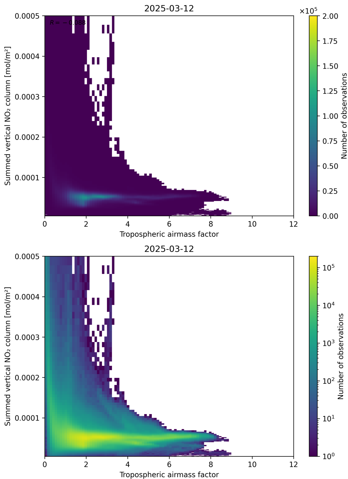
Figure 75: Scatter density plot of “Tropospheric air mass factor” against “Summed vertical NO 2 column” for 2025-03-12 to 2025-03-13.
