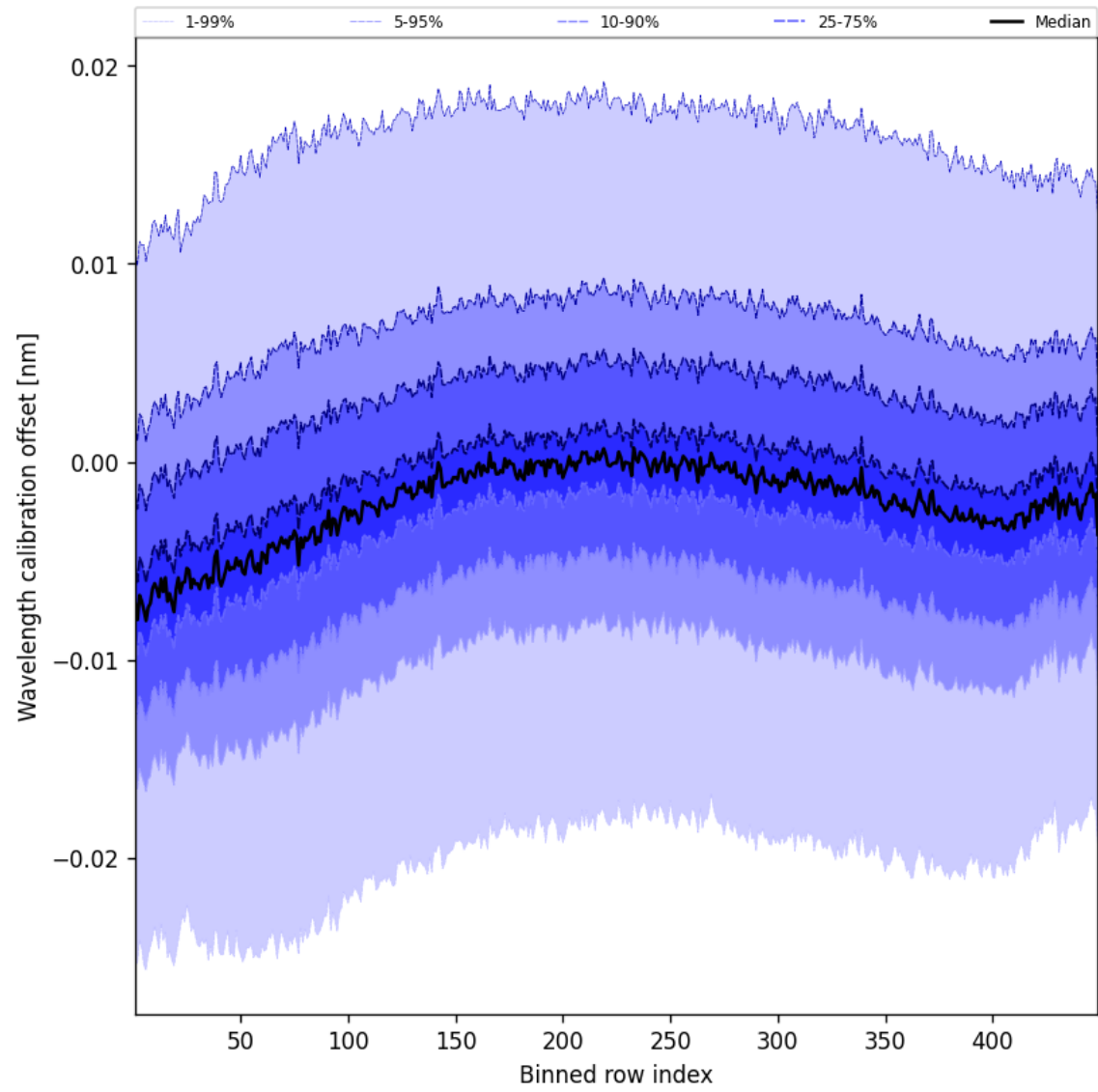
Figure 52: Along track statistics of “Wavelength calibration offset” for 2025-03-12 to 2025-03-13
