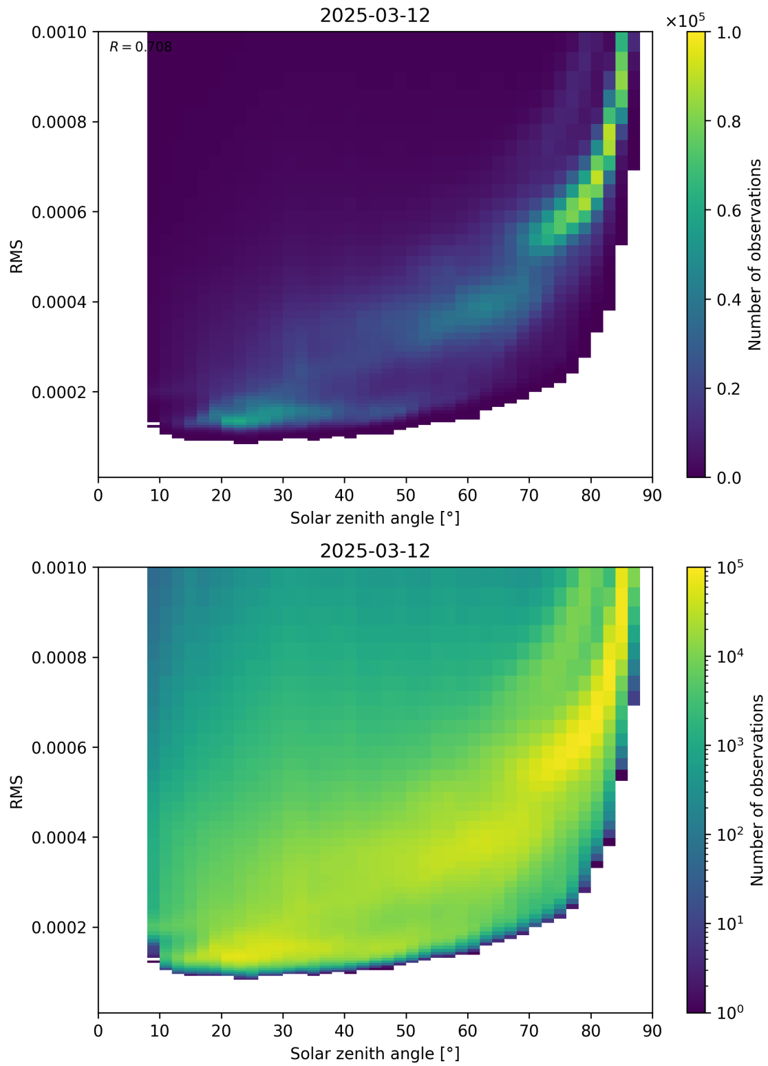
Figure 157: Scatter density plot of “Solar zenith angle” against “RMS” for 2025-03-12 to 2025-03-13.
