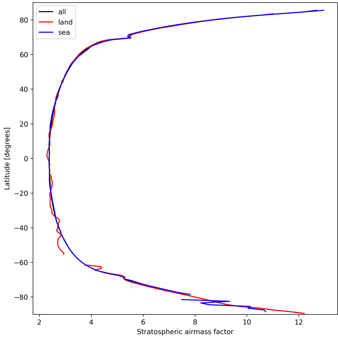
Figure 27: Zonal average of “Stratospheric air mass factor” for 2025-03-12 to 2025-03-13.
