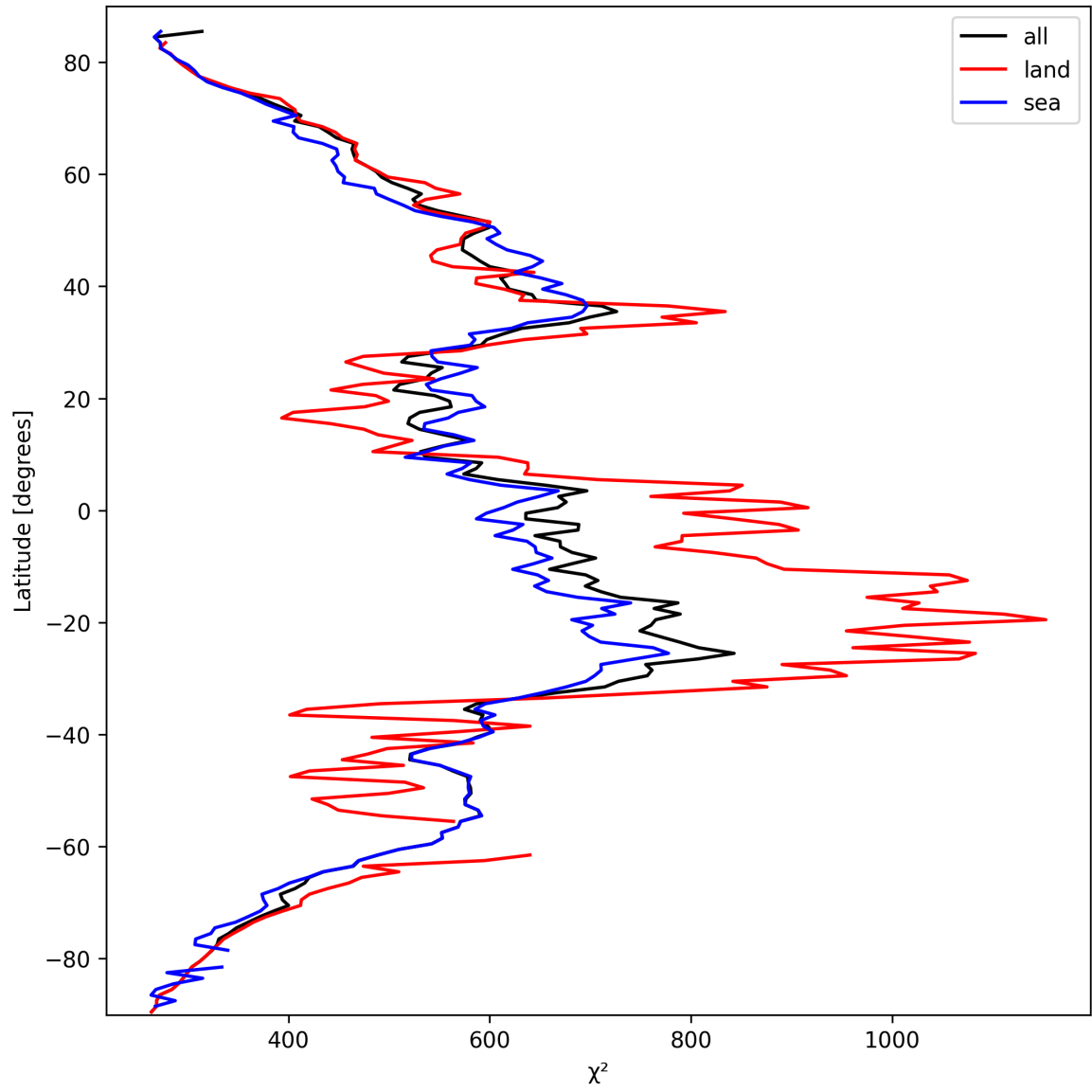
Figure 25: Zonal average of “ \chi^2 ” for 2025-03-12 to 2025-03-13.
