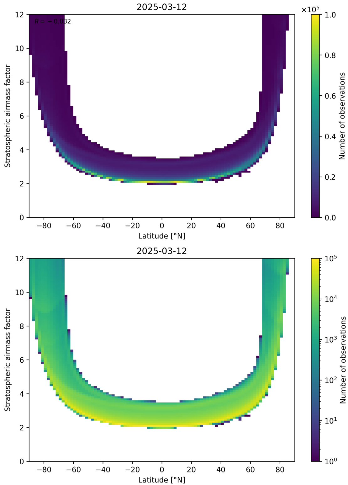
Figure 83: Scatter density plot of “Latitude” against “Stratospheric air mass factor” for 2025-03-12 to 2025-03-13.
