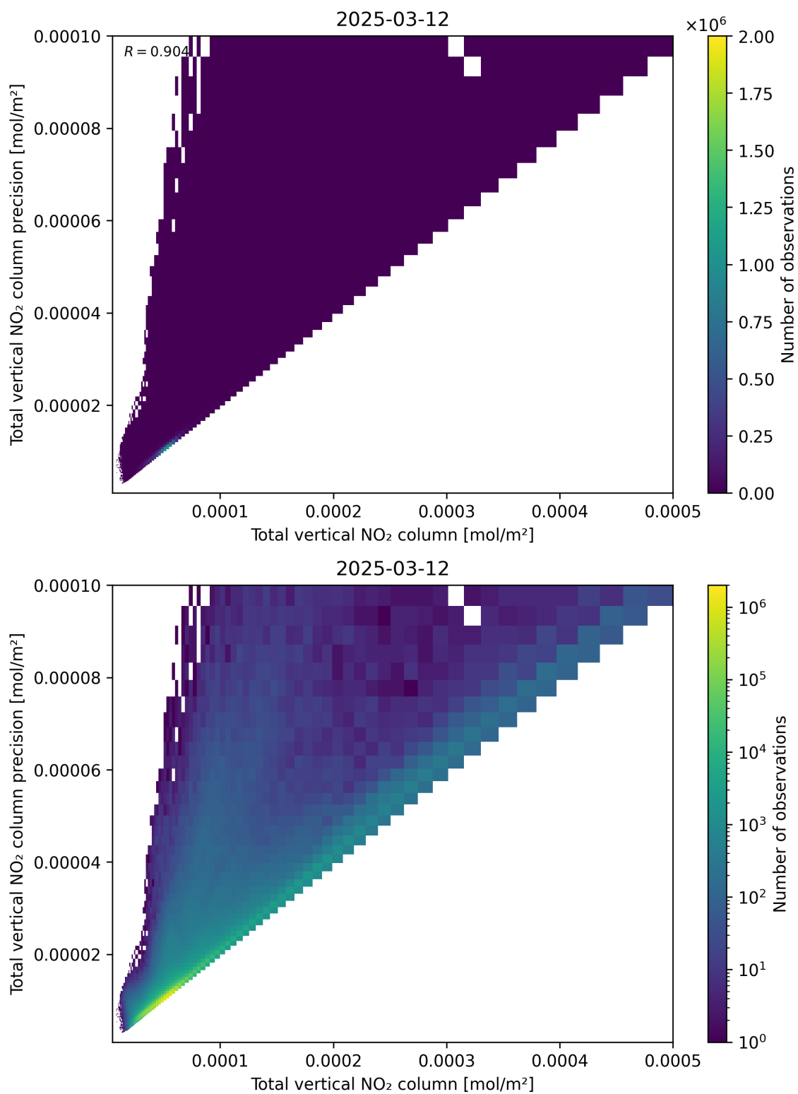
Figure 114: Scatter density plot of “Total vertical NO 2 column” against “Total vertical NO 2 column precision” for 2025-03-12 to 2025-03-13.
