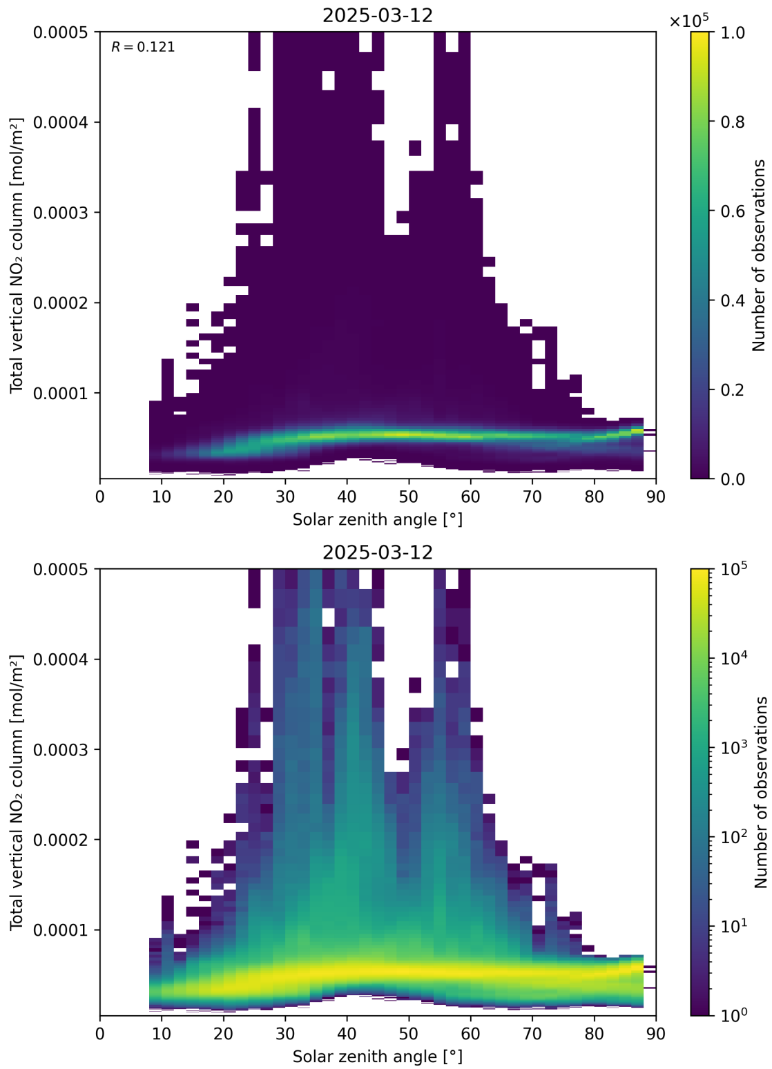
Figure 153: Scatter density plot of “Solar zenith angle” against “Total vertical NO 2 column” for 2025-03-12 to 2025-03-13.
