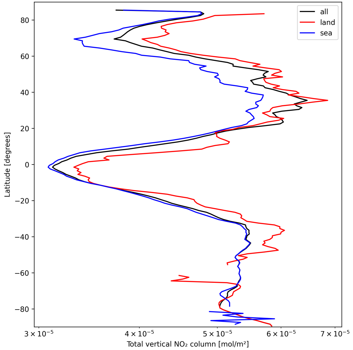
Figure 21: Zonal average of “Total vertical NO 2 column” for 2025-03-12 to 2025-03-13.
