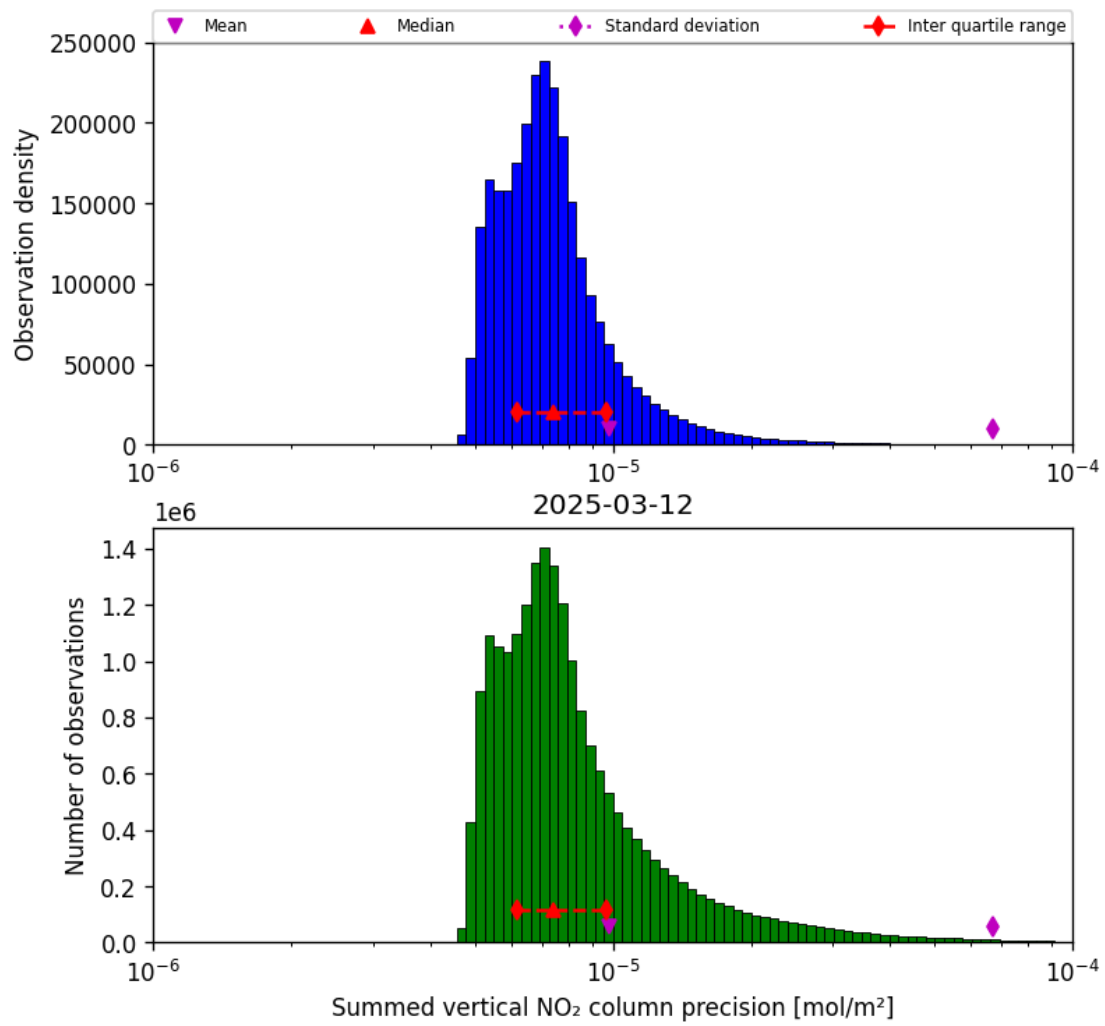
Figure 41: Histogram of “Summed vertical NO 2 column precision” for 2025-03-12 to 2025-03-13
