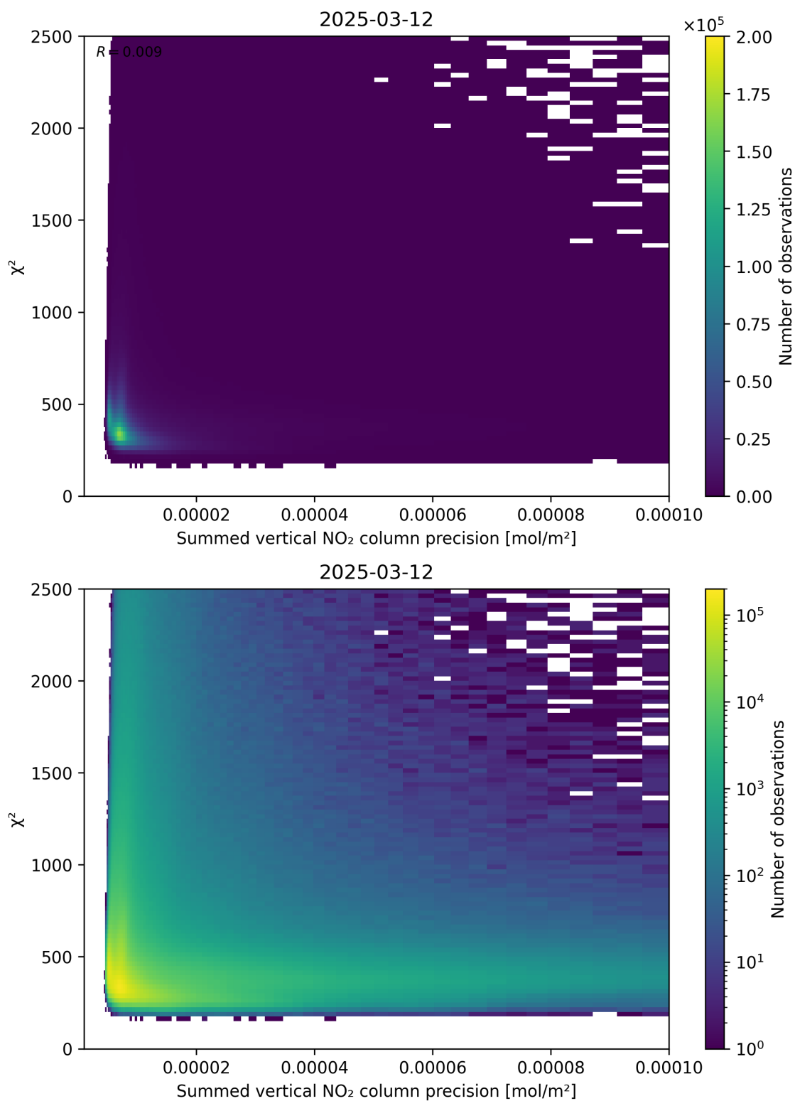
Figure 107: Scatter density plot of “Summed vertical NO 2 column precision” against “ \chi^2 ” for 2025-03-12 to 2025-03-13.
