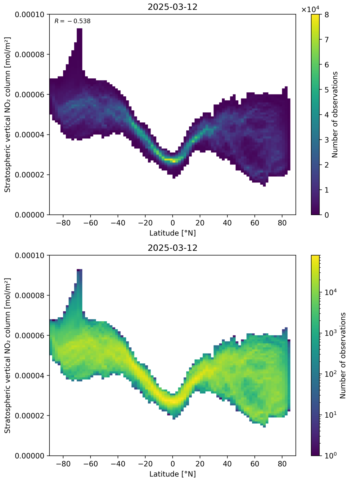
Figure 87: Scatter density plot of “Latitude” against “Stratospheric vertical NO 2 column” for 2025-03-12 to 2025-03-13.
