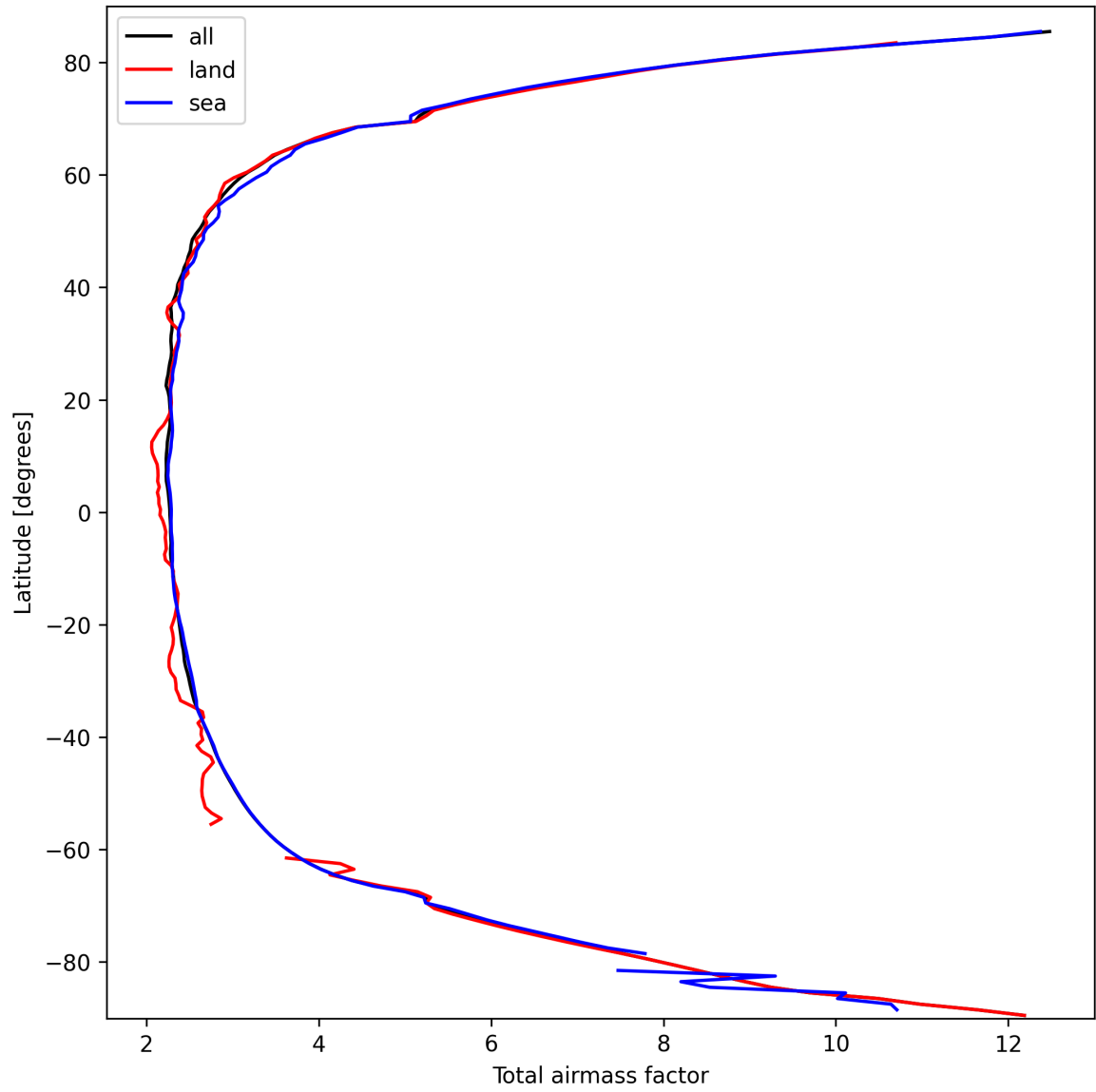
Figure 15: Zonal average of “Total airmass factor” for 2025-03-12 to 2025-03-13.
