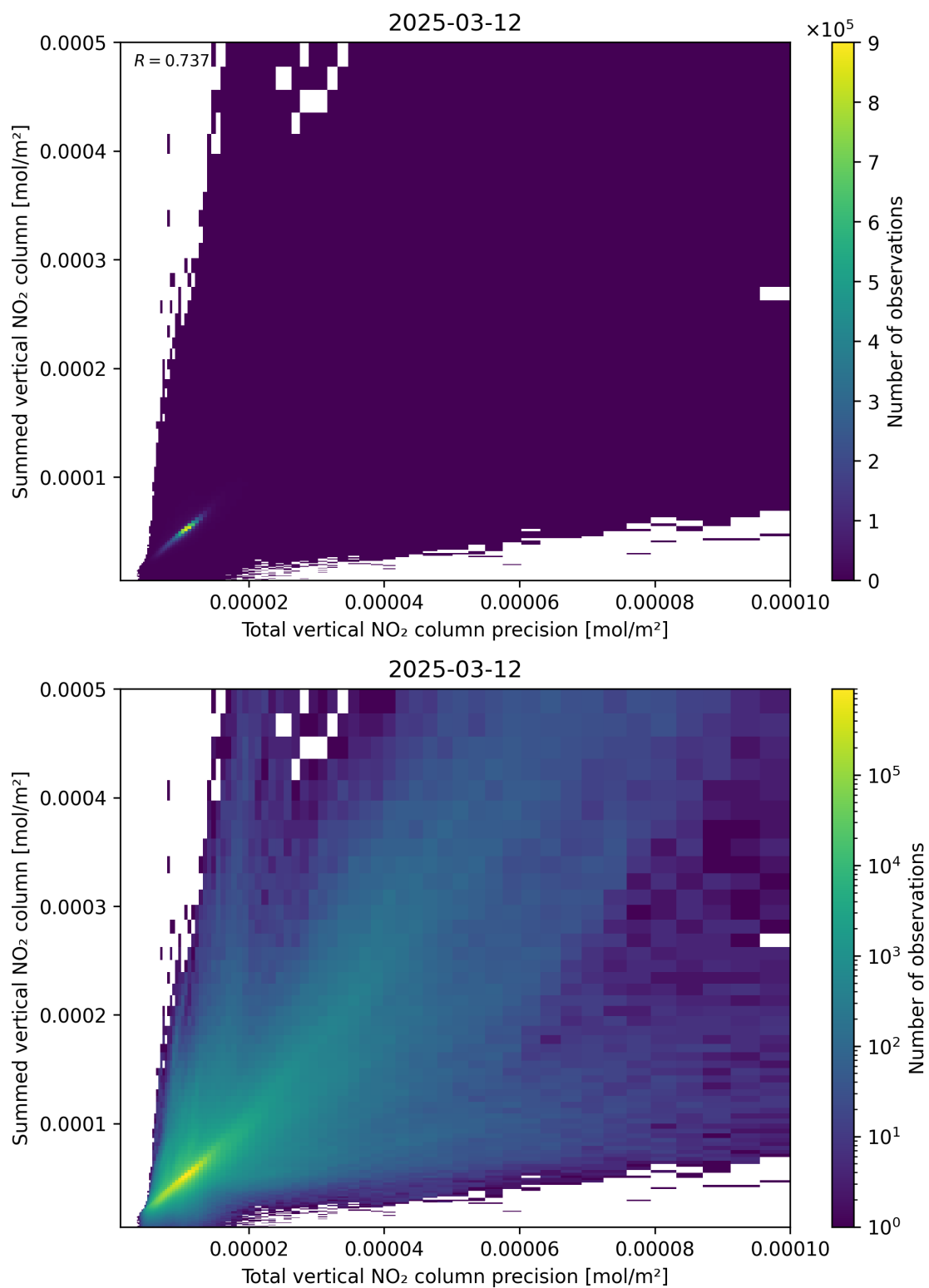
Figure 117: Scatter density plot of “Total vertical NO 2 column precision” against “Summed vertical NO 2 column” for 2025-03-12 to 2025-03-13.
