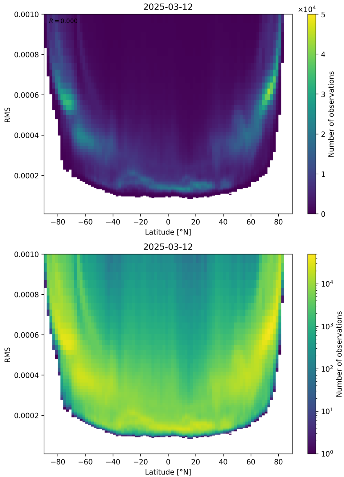
Figure 94: Scatter density plot of “Latitude” against “RMS” for 2025-03-12 to 2025-03-13.
