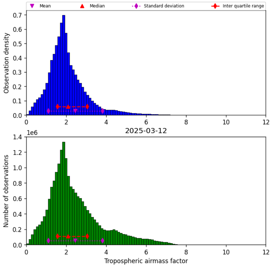
Figure 31: Histogram of “Tropospheric airmass factor” for 2025-03-12 to 2025-03-13
