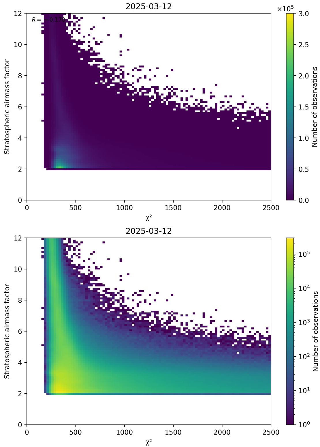
Figure 81: Scatter density plot of “ \chi^2 ” against “Stratospheric airmass factor” for 2025-03-12 to 2025-03-13.
