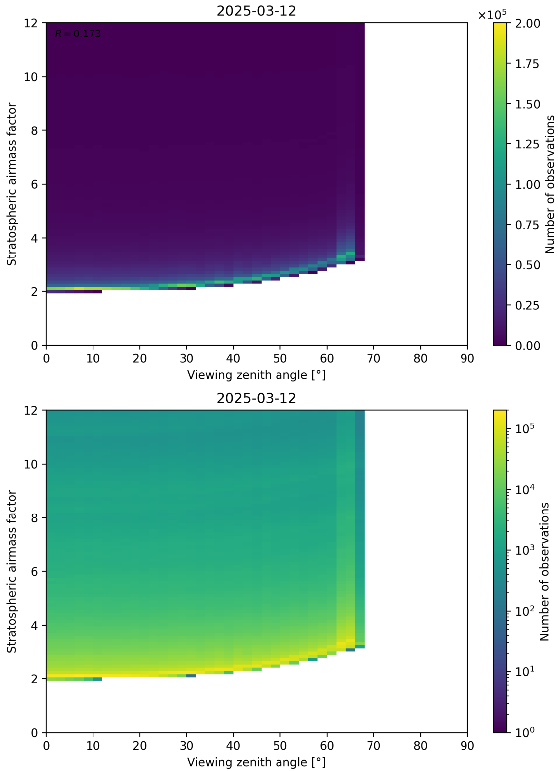
Figure 159: Scatter density plot of “Viewing zenith angle” against “Stratospheric airmass factor” for 2025-03-12 to 2025-03-13.
