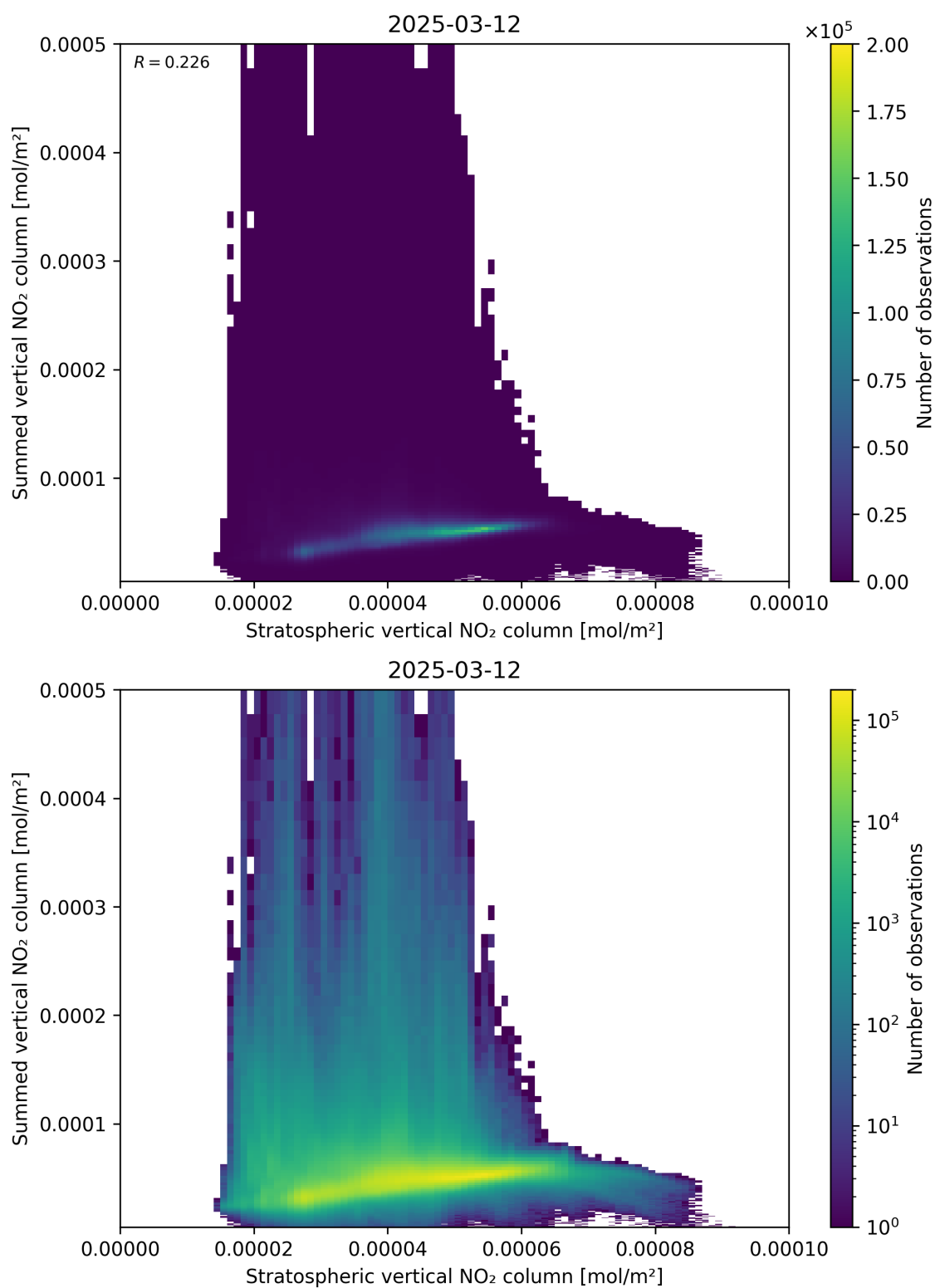
Figure 98: Scatter density plot of “Stratospheric vertical NO 2 column” against “Summed vertical NO 2 column” for 2025-03-12 to 2025-03-13.
