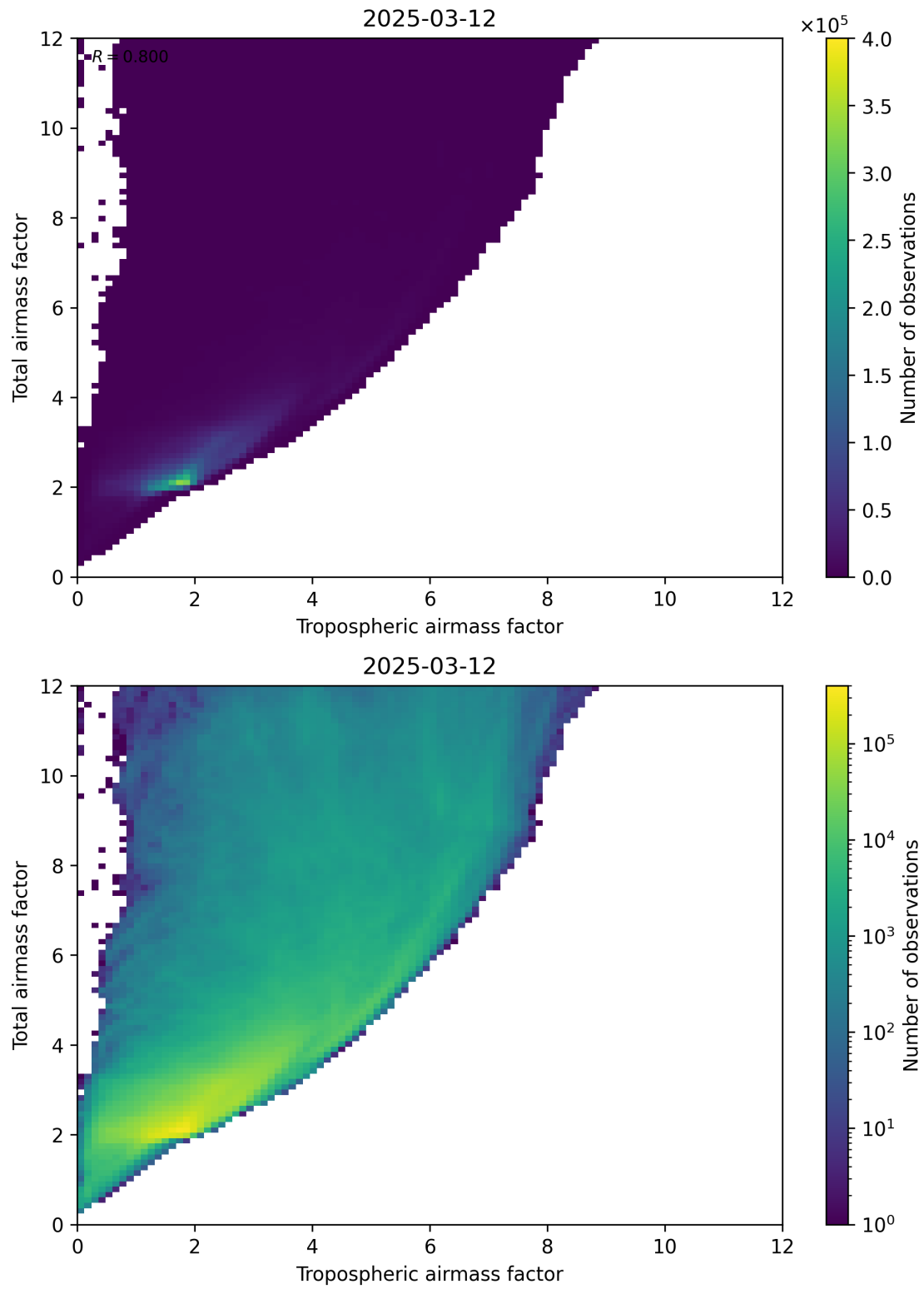
Figure 72: Scatter density plot of “Tropospheric airmass factor” against “Total airmass factor” for 2025-03-12 to 2025-03-13.
