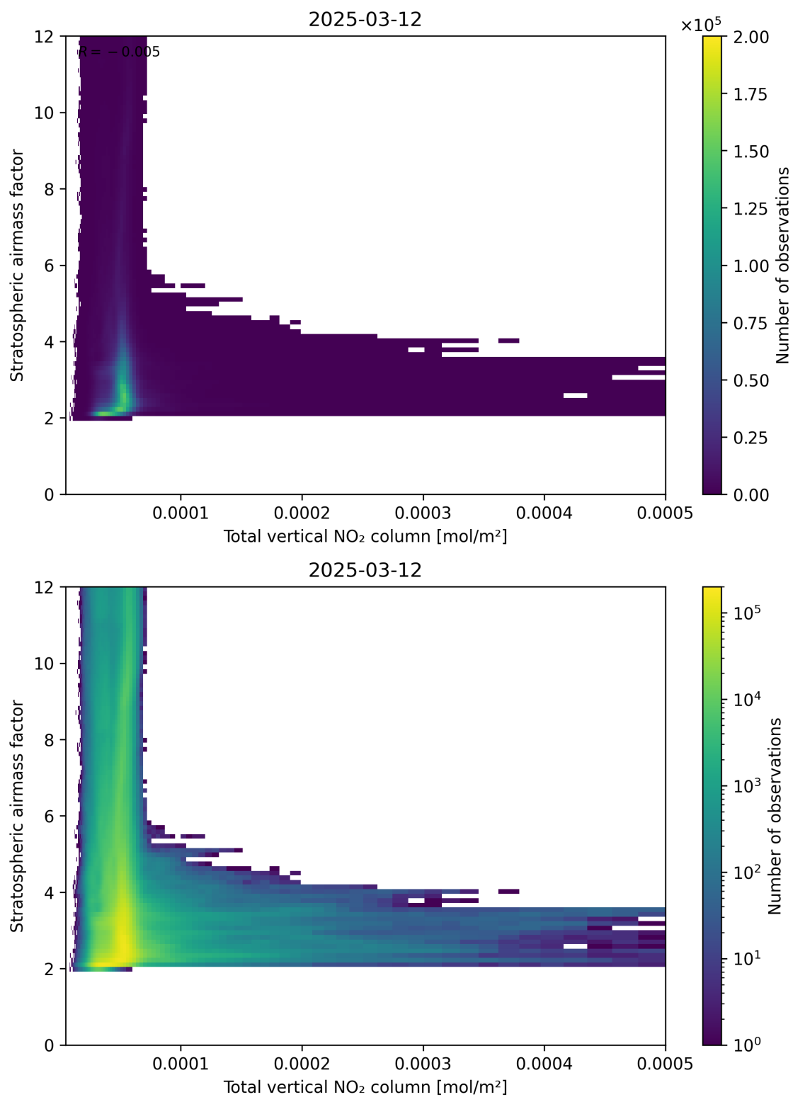
Figure 110: Scatter density plot of “Total vertical NO 2 column” against “Stratospheric airmass factor” for 2025-03-12 to 2025-03-13.
