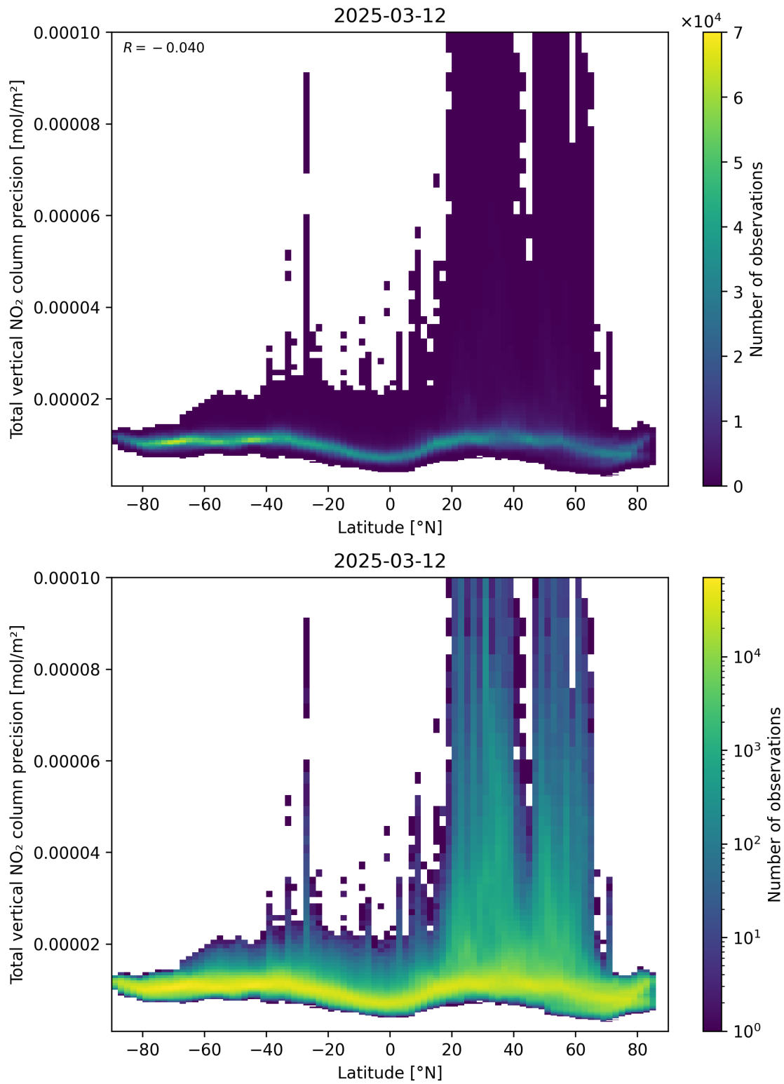
Figure 91: Scatter density plot of “Latitude” against “Total vertical NO 2 column precision” for 2025-03-12 to 2025-03-13.
