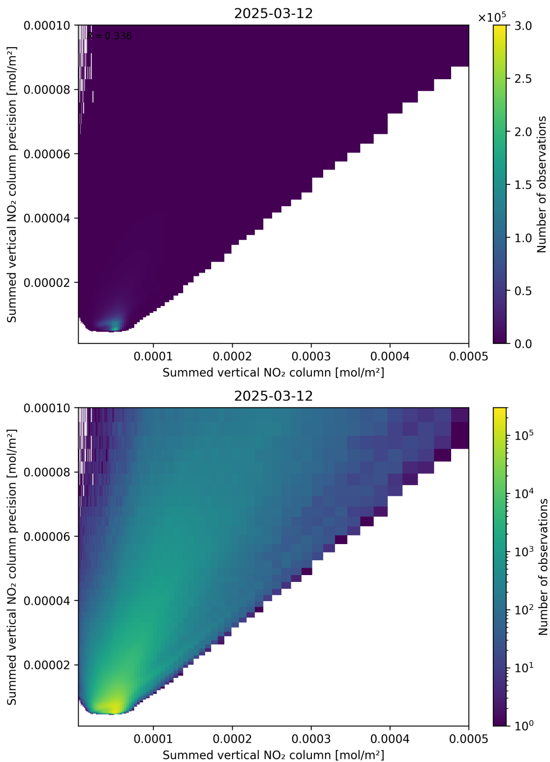
Figure 105: Scatter density plot of “Summed vertical NO 2 column” against “Summed vertical NO 2 column precision” for 2025-03-12 to 2025-03-13.
