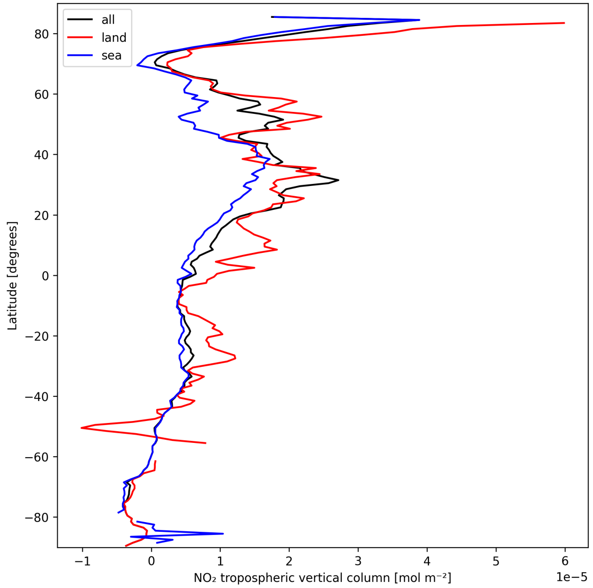
Figure 12: Zonal average of “NO 2 tropospheric vertical column” for 2025-03-12 to 2025-03-13.
