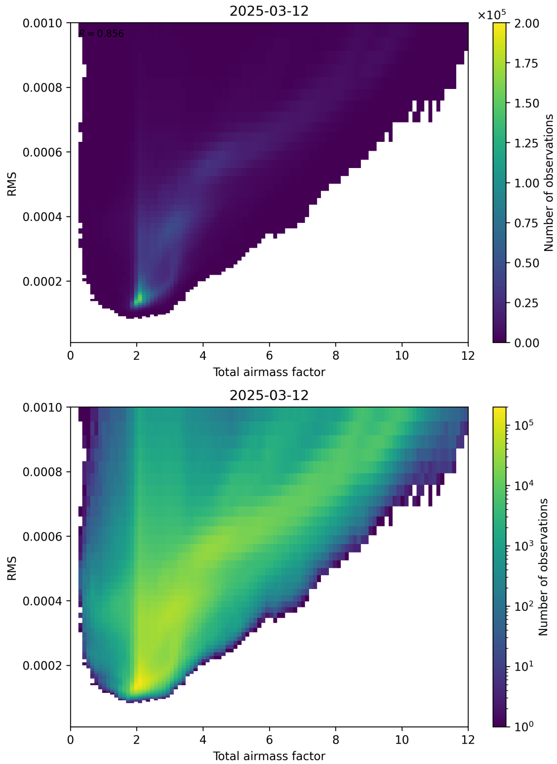
Figure 69: Scatter density plot of “Total airmass factor” against “RMS” for 2025-03-12 to 2025-03-13.
