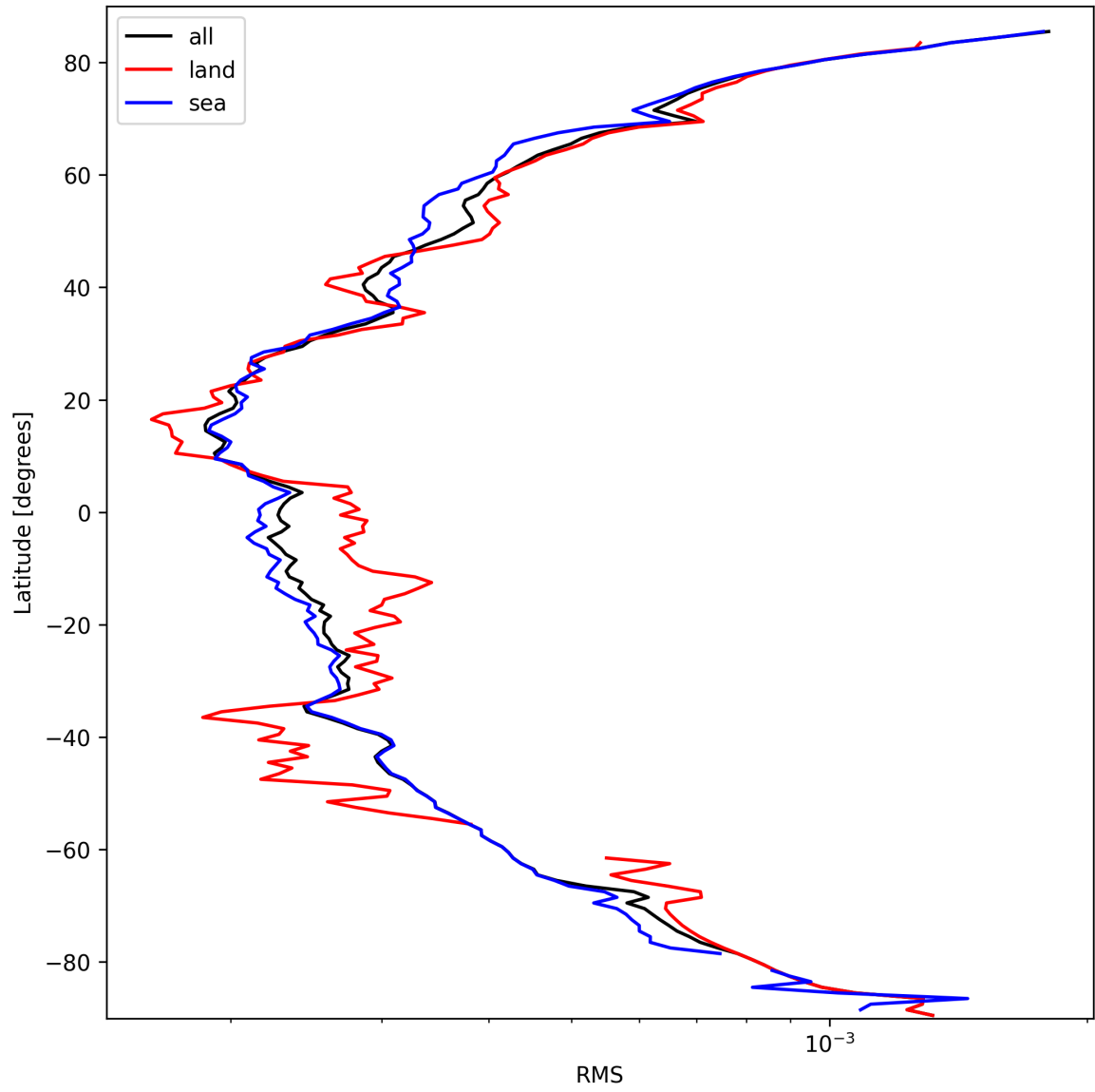
Figure 26: Zonal average of “RMS” for 2025-03-12 to 2025-03-13.
