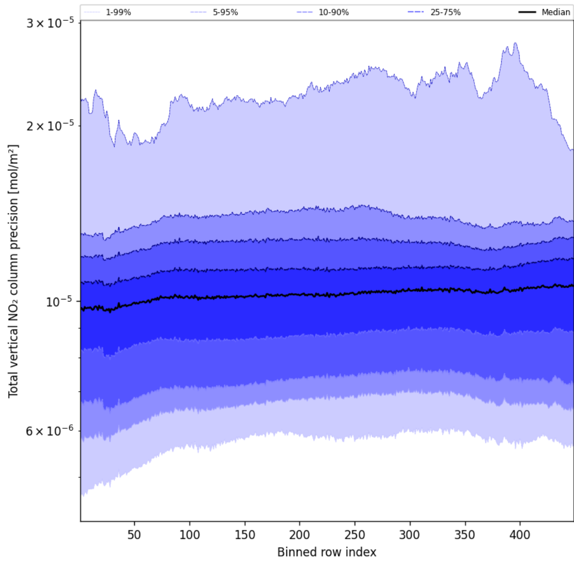
Figure 56: Along track statistics of “Total vertical NO 2 column precision” for 2025-03-12 to 2025-03-13
