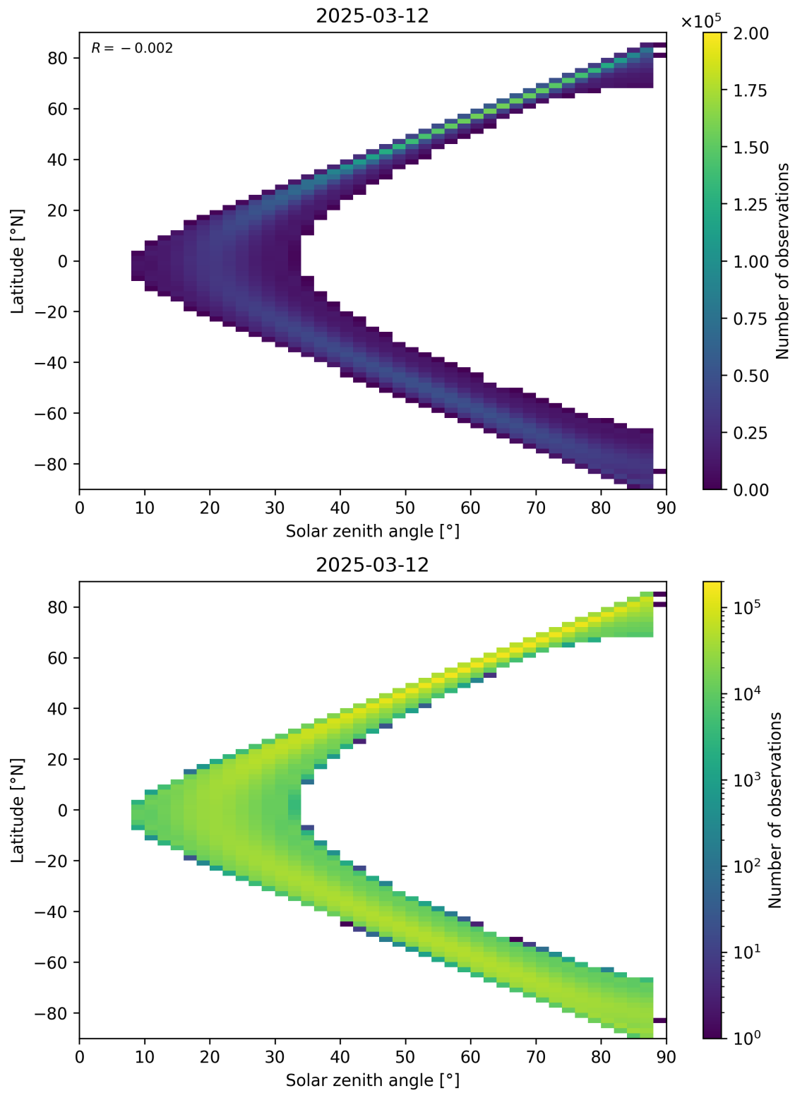
Figure 149: Scatter density plot of “Solar zenith angle” against “Latitude” for 2025-03-12 to 2025-03-13.
