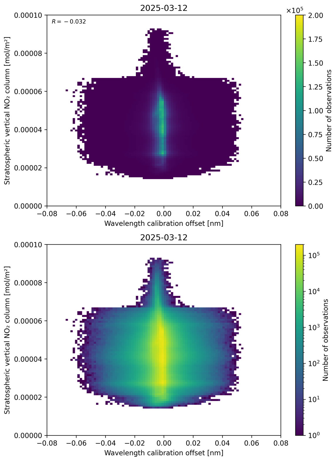
Figure 176: Scatter density plot of “Wavelength calibration offset” against “Stratospheric vertical NO 2 column” for 2025-03-12 to 2025-03-13.
