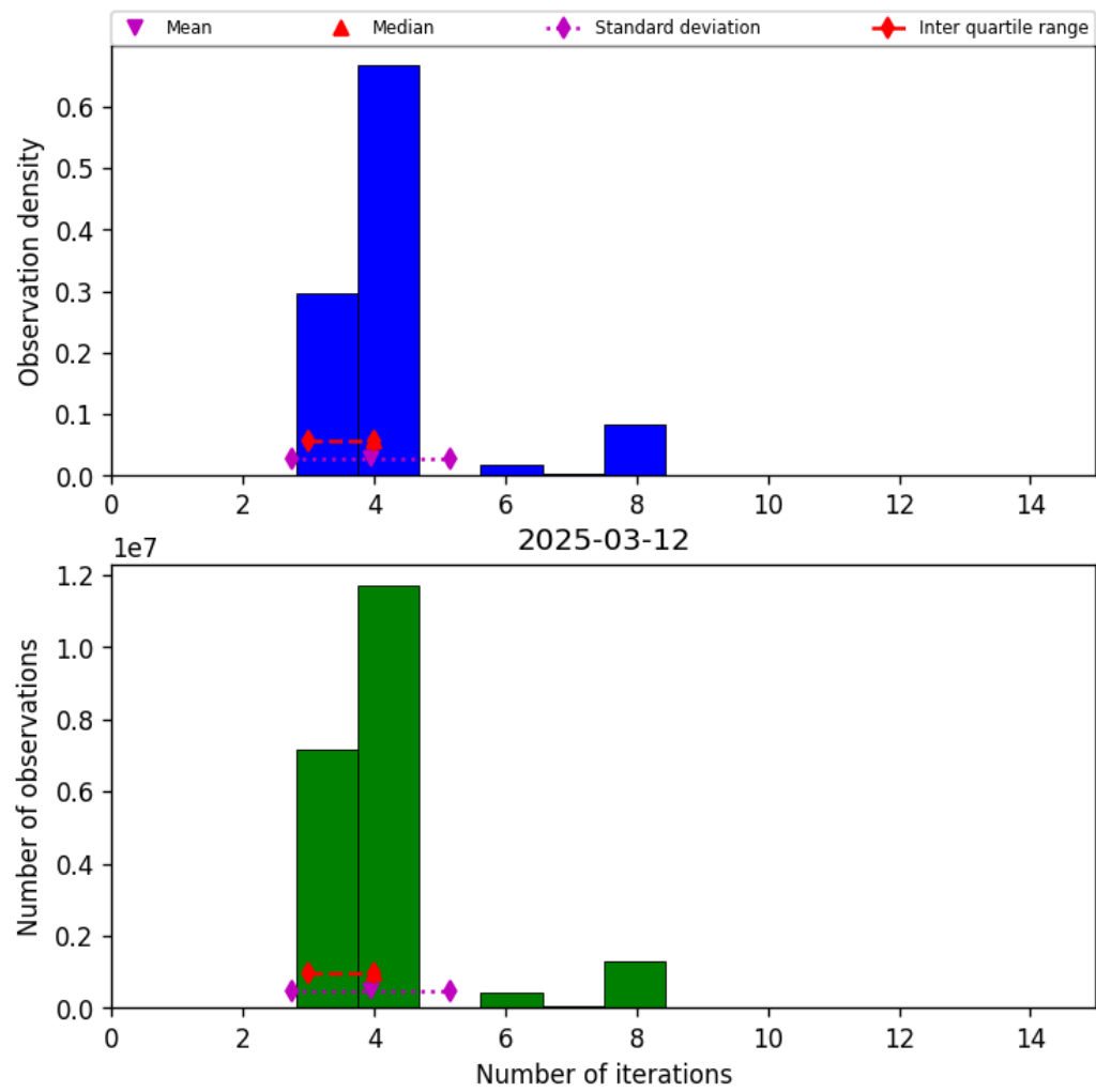
Figure 34: Histogram of “Number of iterations” for 2025-03-12 to 2025-03-13
