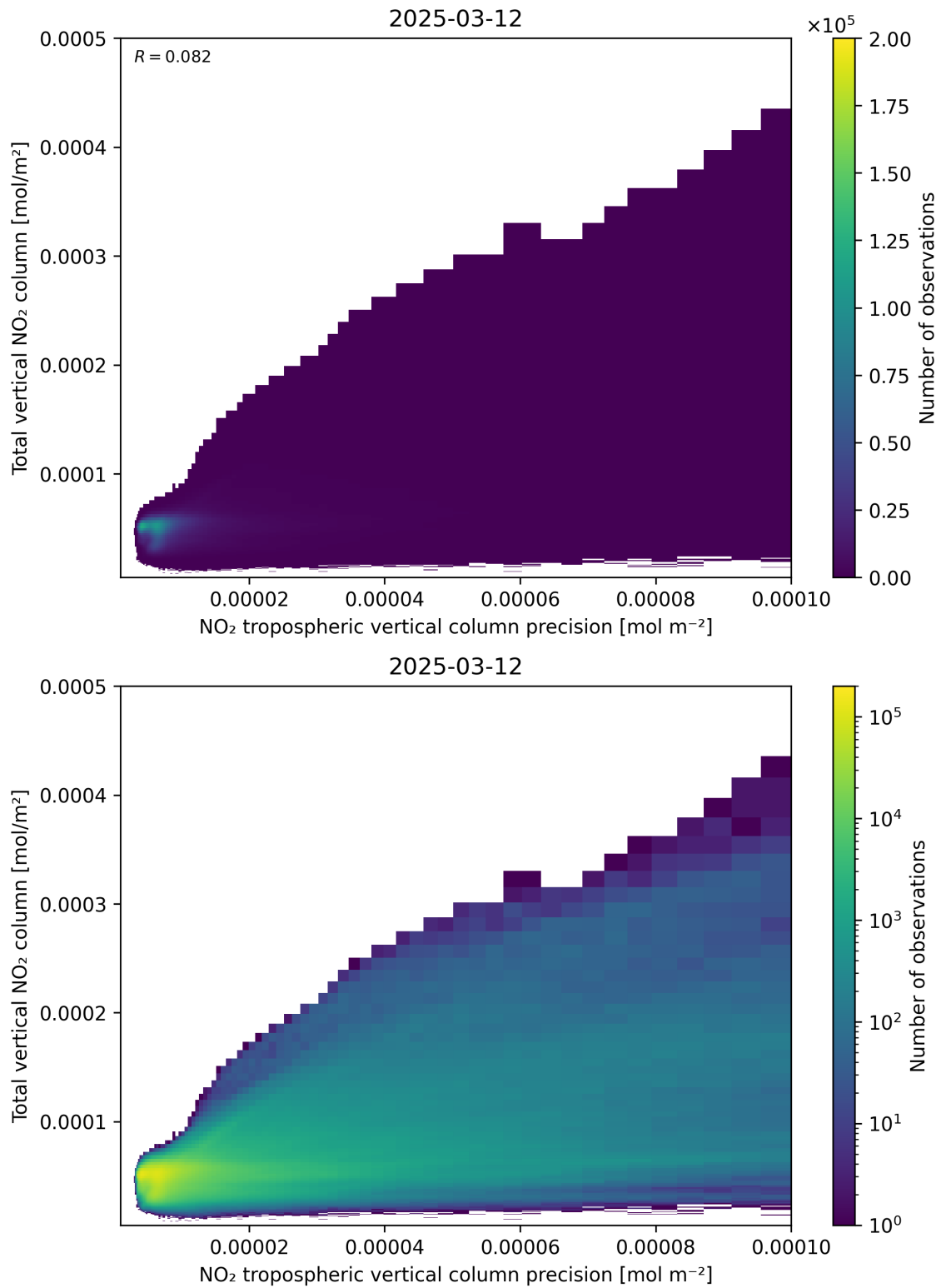
Figure 138: Scatter density plot of “NO 2 tropospheric vertical column precision” against “Total vertical NO 2 column” for 2025-03-12 to 2025-03-13.
