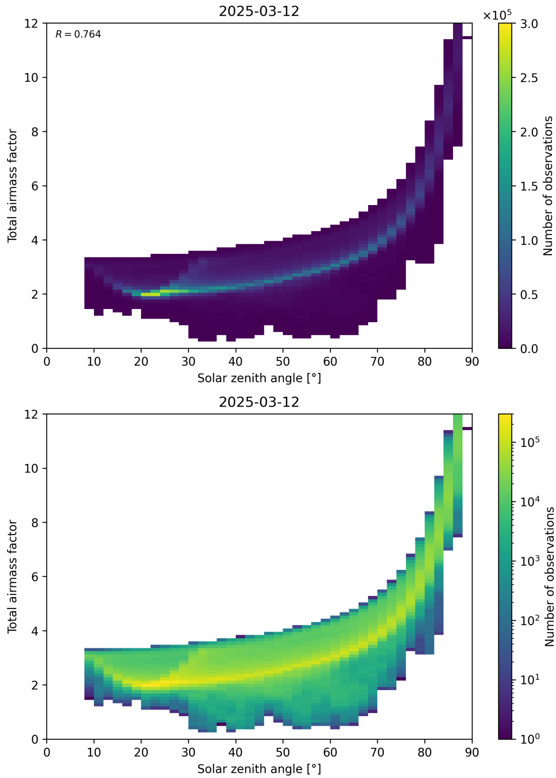
Figure 146: Scatter density plot of “Solar zenith angle” against “Total air mass factor” for 2025-03-12 to 2025-03-13.
