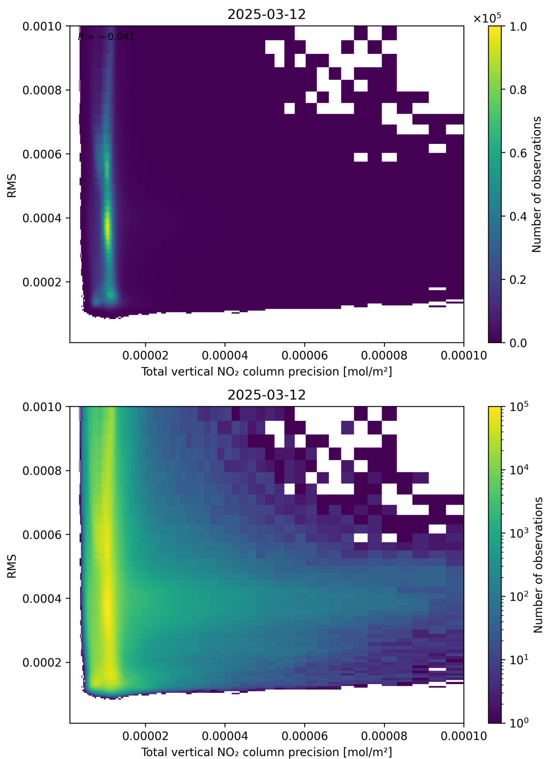
Figure 119: Scatter density plot of “Total vertical NO 2 column precision” against “RMS” for 2025-03-12 to 2025-03-13.
