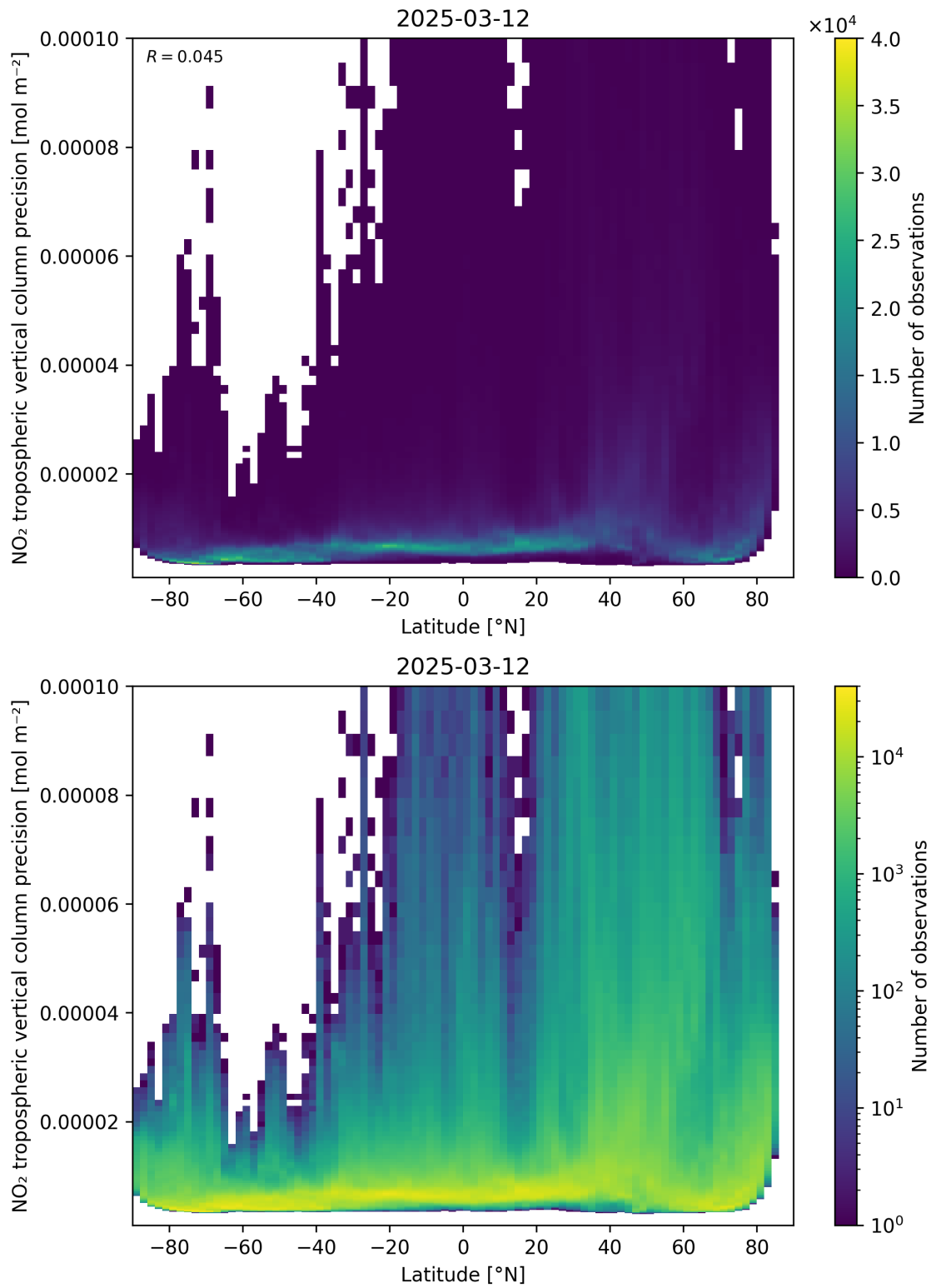
Figure 93: Scatter density plot of “Latitude” against “NO 2 tropospheric vertical column precision” for 2025-03-12 to 2025-03-13.
