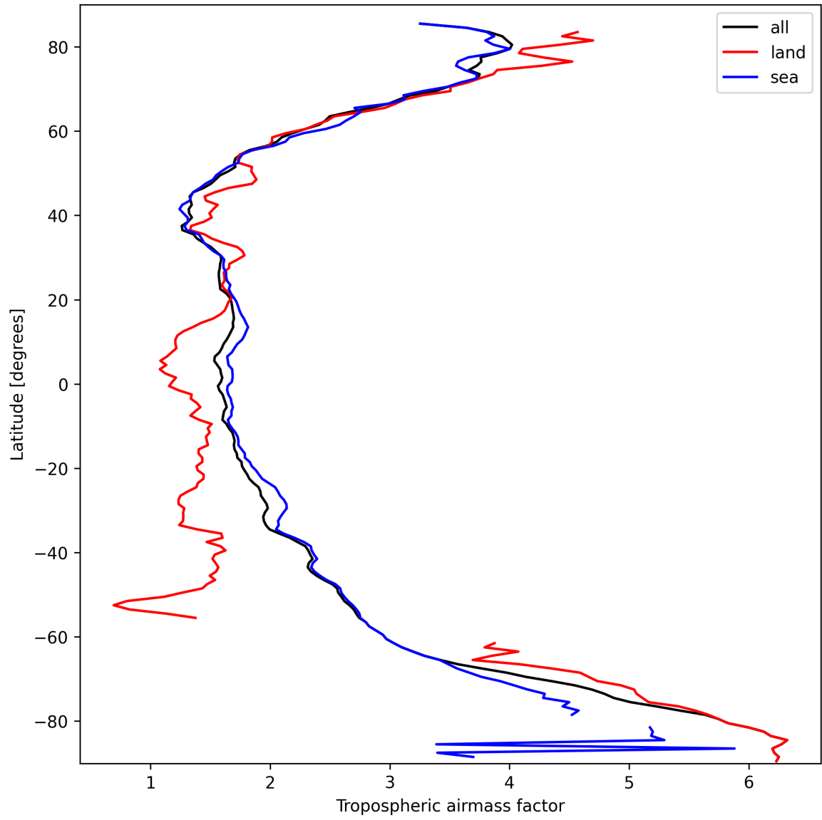
Figure 14: Zonal average of “Tropospheric airmass factor” for 2025-03-12 to 2025-03-13.
