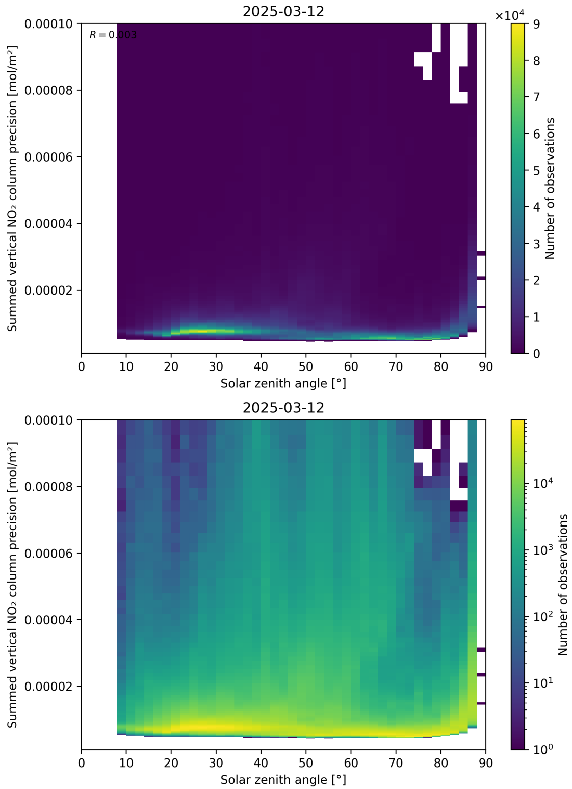
Figure 152: Scatter density plot of “Solar zenith angle” against “Summed vertical NO 2 column precision” for 2025-03-12 to 2025-03-13.
