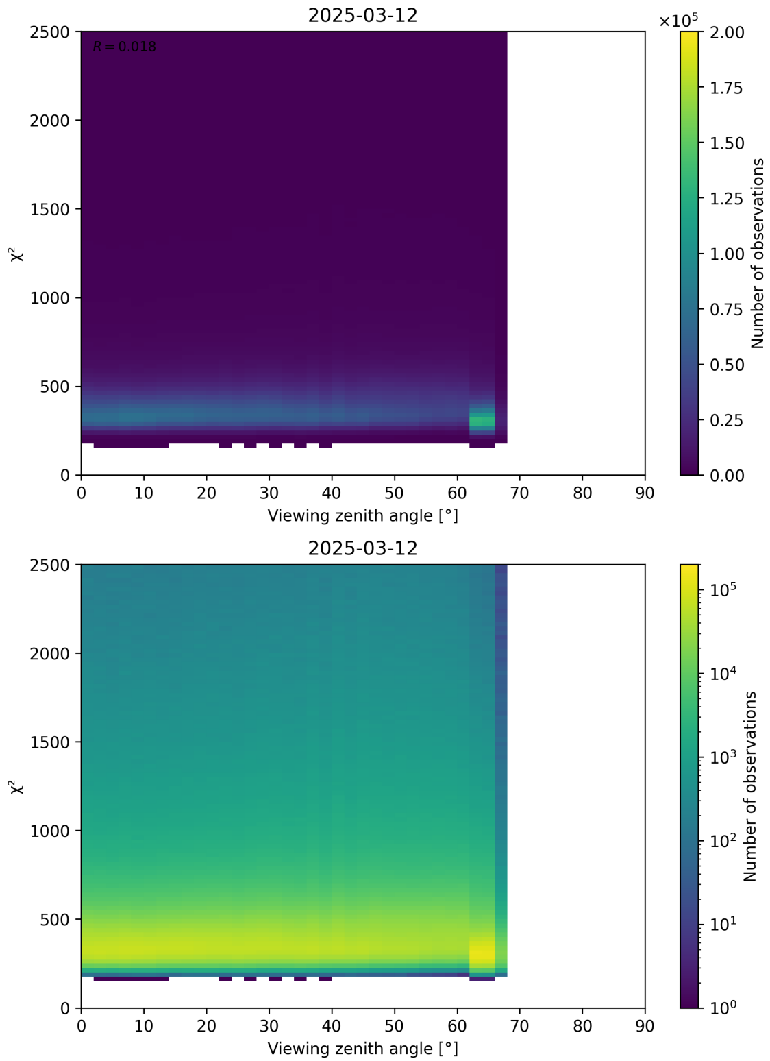
Figure 162: Scatter density plot of “Viewing zenith angle” against “ \chi^2 ” for 2025-03-12 to 2025-03-13.
