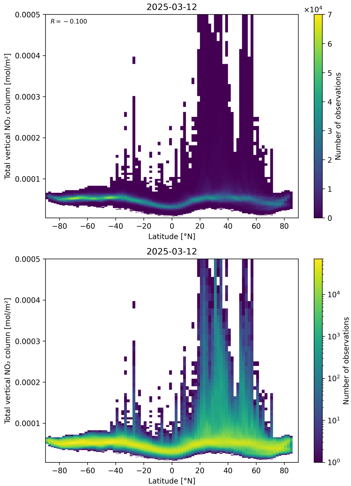
Figure 90: Scatter density plot of “Latitude” against “Total vertical NO 2 column” for 2025-03-12 to 2025-03-13.
