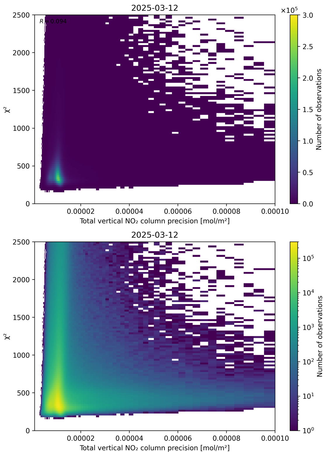
Figure 116: Scatter density plot of “Total vertical NO 2 column precision” against “ \chi^2 ” for 2025-03-12 to 2025-03-13.
