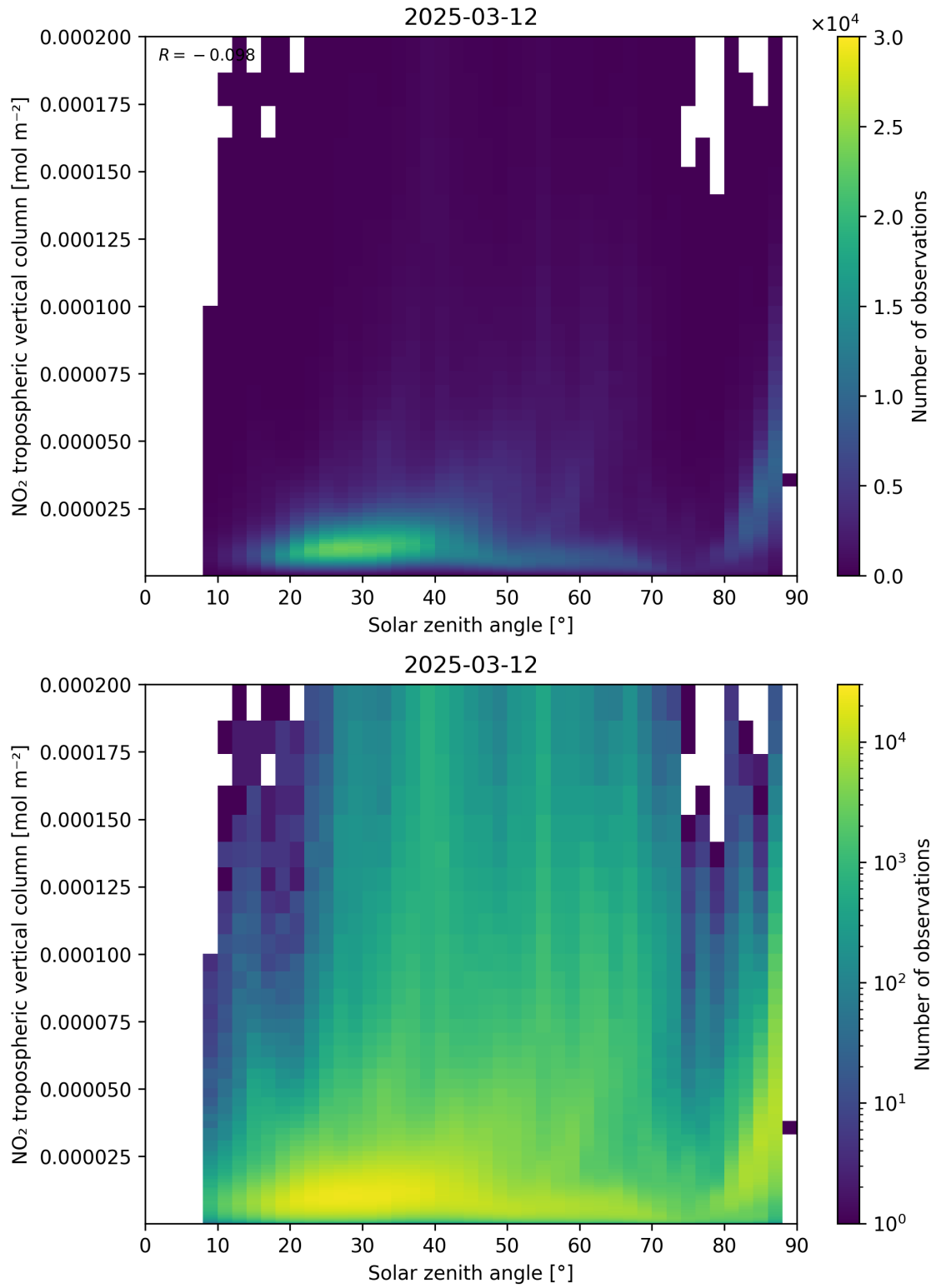
Figure 155: Scatter density plot of “Solar zenith angle” against “NO 2 tropospheric vertical column” for 2025-03-12 to 2025-03-13.
