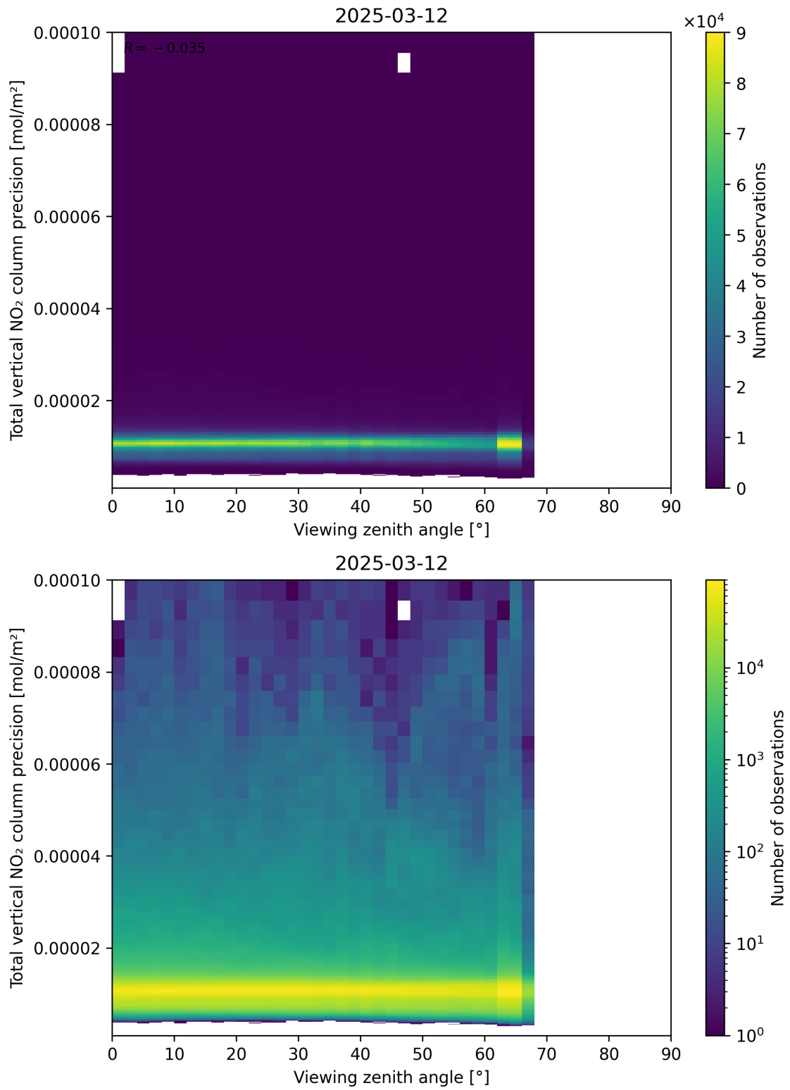
Figure 168: Scatter density plot of “Viewing zenith angle” against “Total vertical NO 2 column precision” for 2025-03-12 to 2025-03-13.
