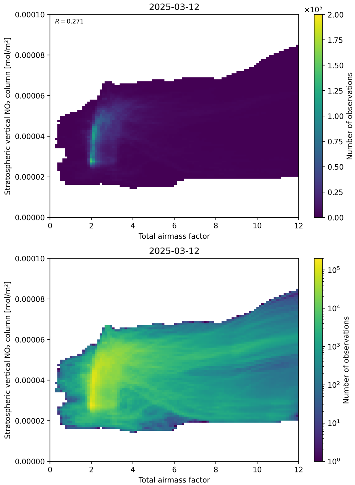
Figure 64: Scatter density plot of “Total airmass factor” against “Stratospheric vertical \text{NO}_2 column” for 2025-03-12 to 2025-03-13.
