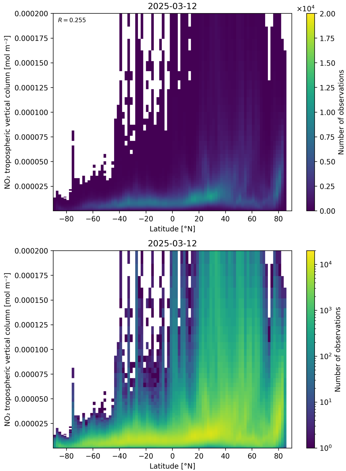
Figure 92: Scatter density plot of “Latitude” against “NO 2 tropospheric vertical column” for 2025-03-12 to 2025-03-13.
