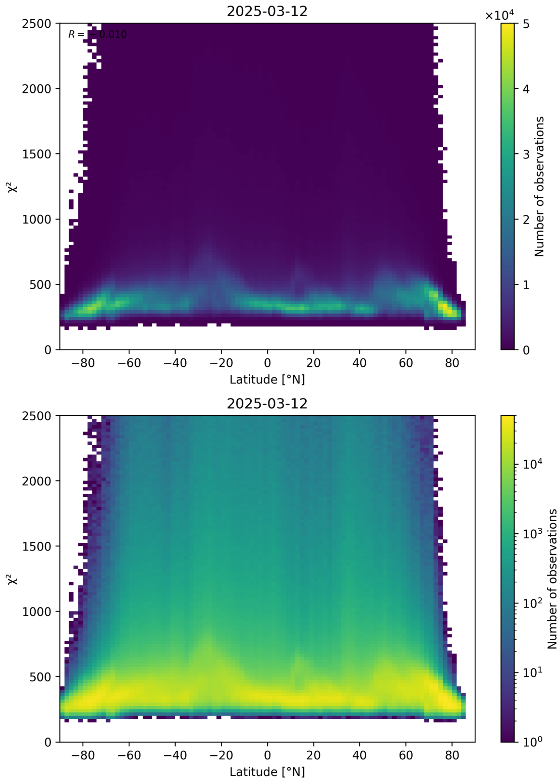
Figure 86: Scatter density plot of “Latitude” against “ \chi^2 ” for 2025-03-12 to 2025-03-13.
