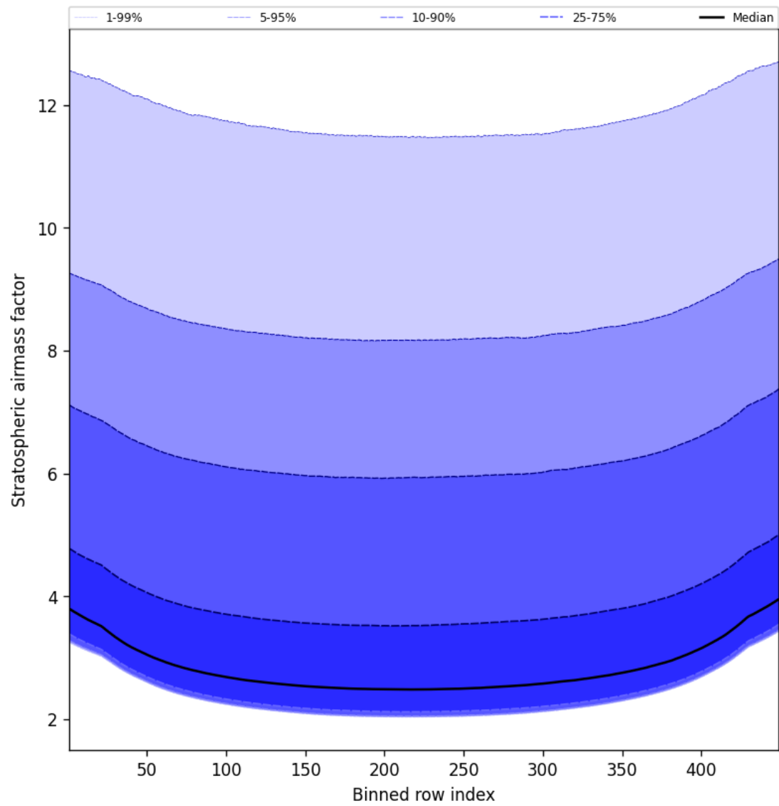
Figure 61: Along track statistics of “Stratospheric airmass factor” for 2025-03-12 to 2025-03-13
