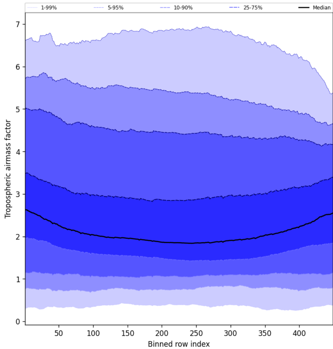
Figure 48: Along track statistics of “Tropospheric air mass factor” for 2025-03-12 to 2025-03-13
