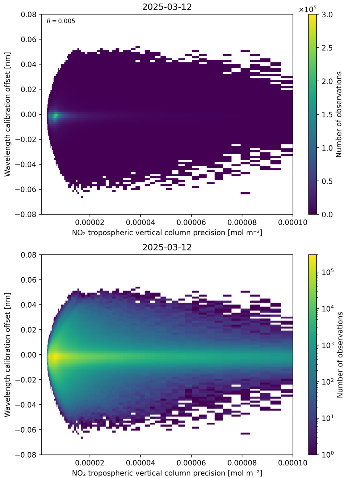
Figure 141: Scatter density plot of “NO 2 tropospheric vertical column precision” against “Wavelength calibration offset” for 2025-03-12 to 2025-03-13.
