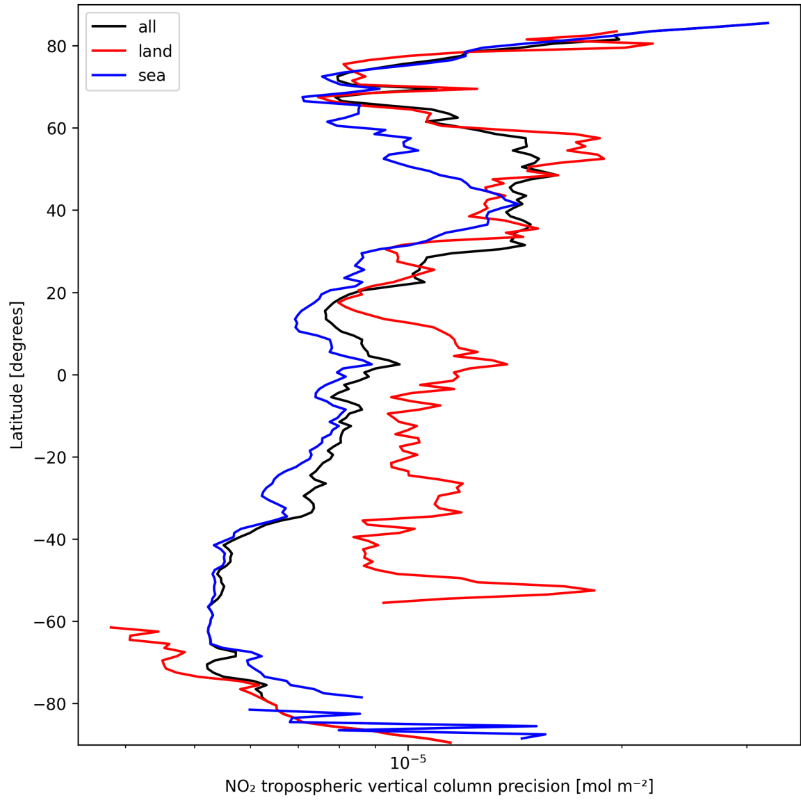
Figure 13: Zonal average of “NO 2 tropospheric vertical column precision” for 2025-03-12 to 2025-03-13.
