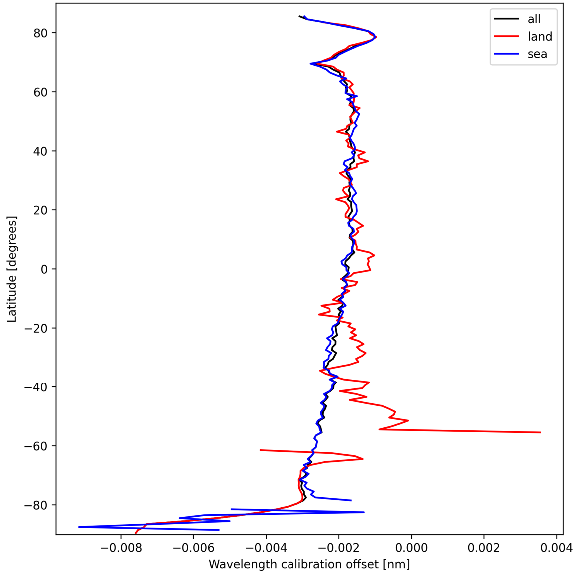
Figure 18: Zonal average of “Wavelength calibration offset” for 2025-03-12 to 2025-03-13.
