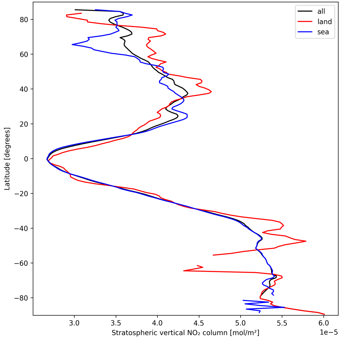
Figure 19: Zonal average of “Stratospheric vertical NO 2 column” for 2025-03-12 to 2025-03-13.
