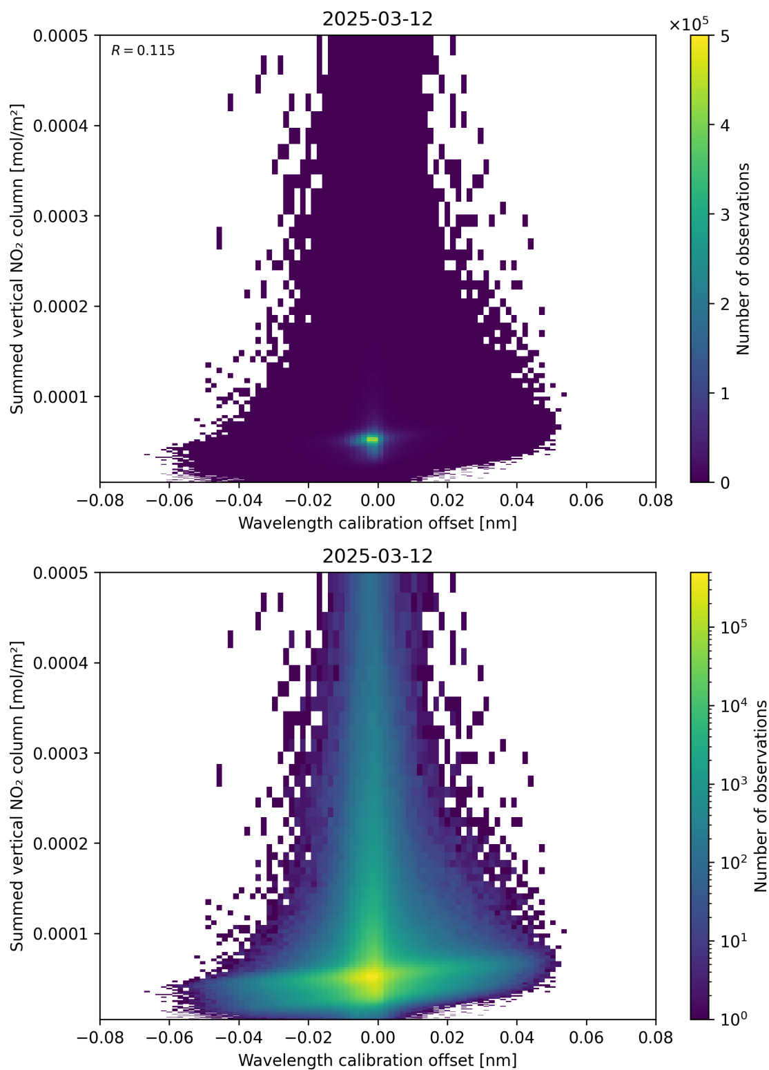
Figure 177: Scatter density plot of “Wavelength calibration offset” against “Summed vertical NO 2 column” for 2025-03-12 to 2025-03-13.
