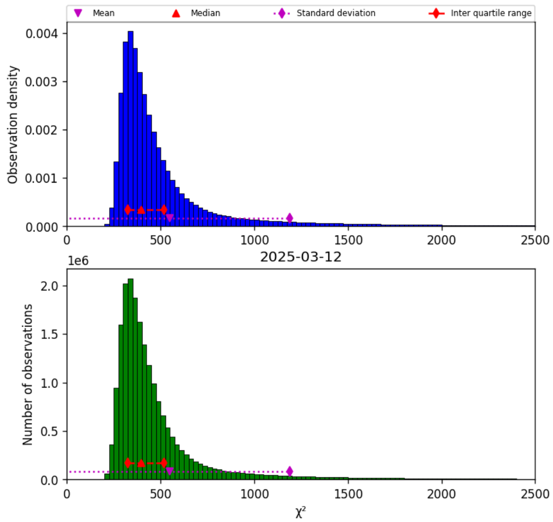
Figure 42: Histogram of “ \chi^2 ” for 2025-03-12 to 2025-03-13
