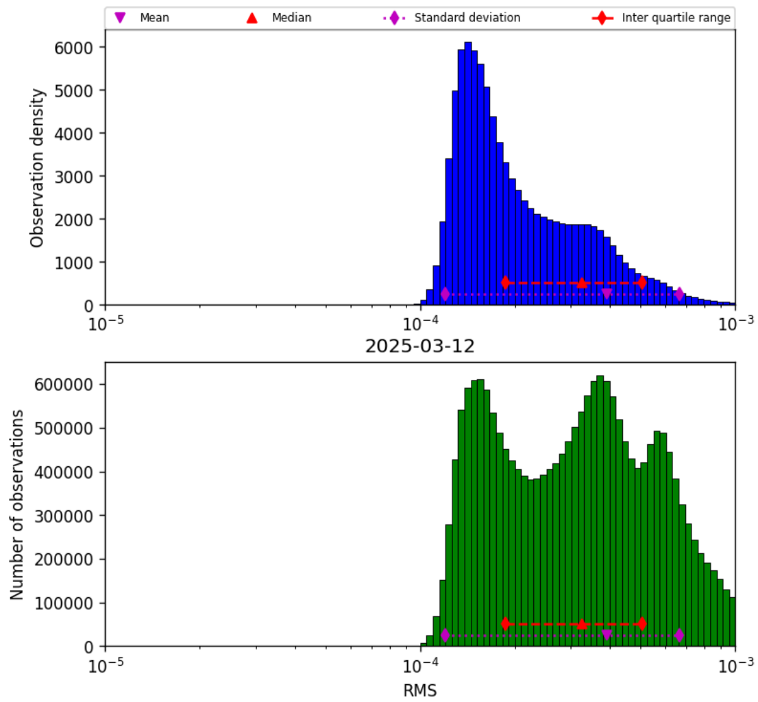
Figure 43: Histogram of “RMS” for 2025-03-12 to 2025-03-13
