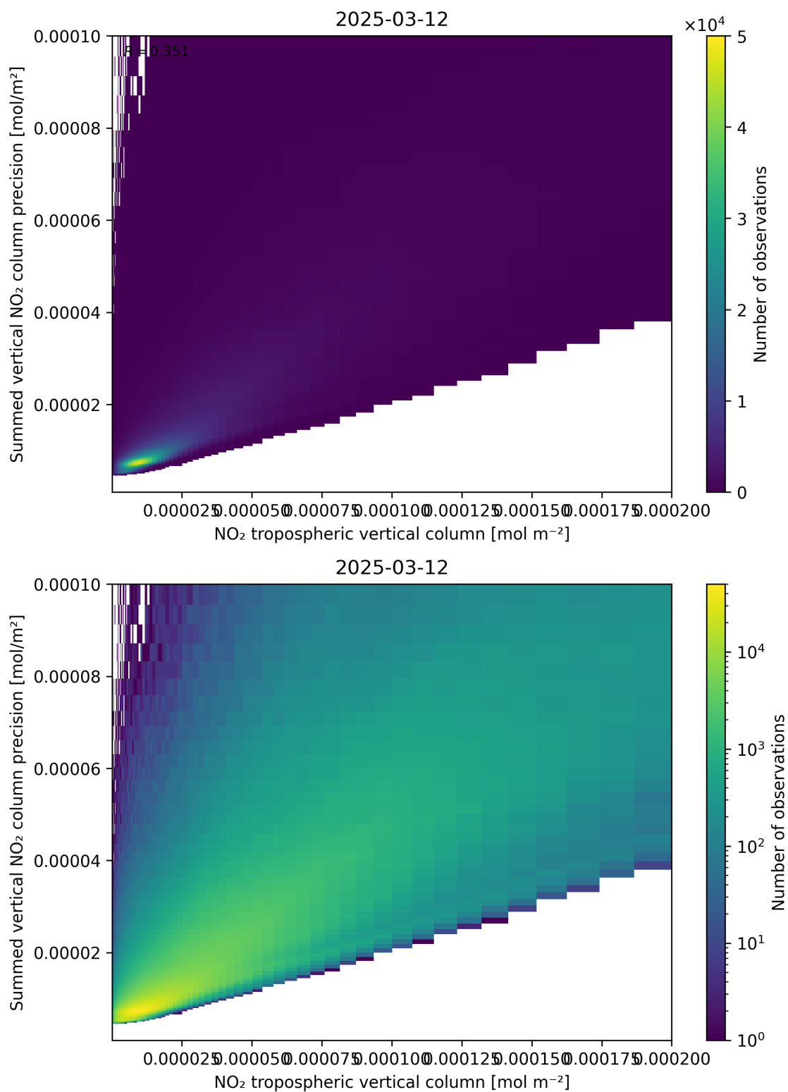
Figure 127: Scatter density plot of “NO 2 tropospheric vertical column” against “Summed vertical NO 2 column precision” for 2025-03-12 to 2025-03-13.
