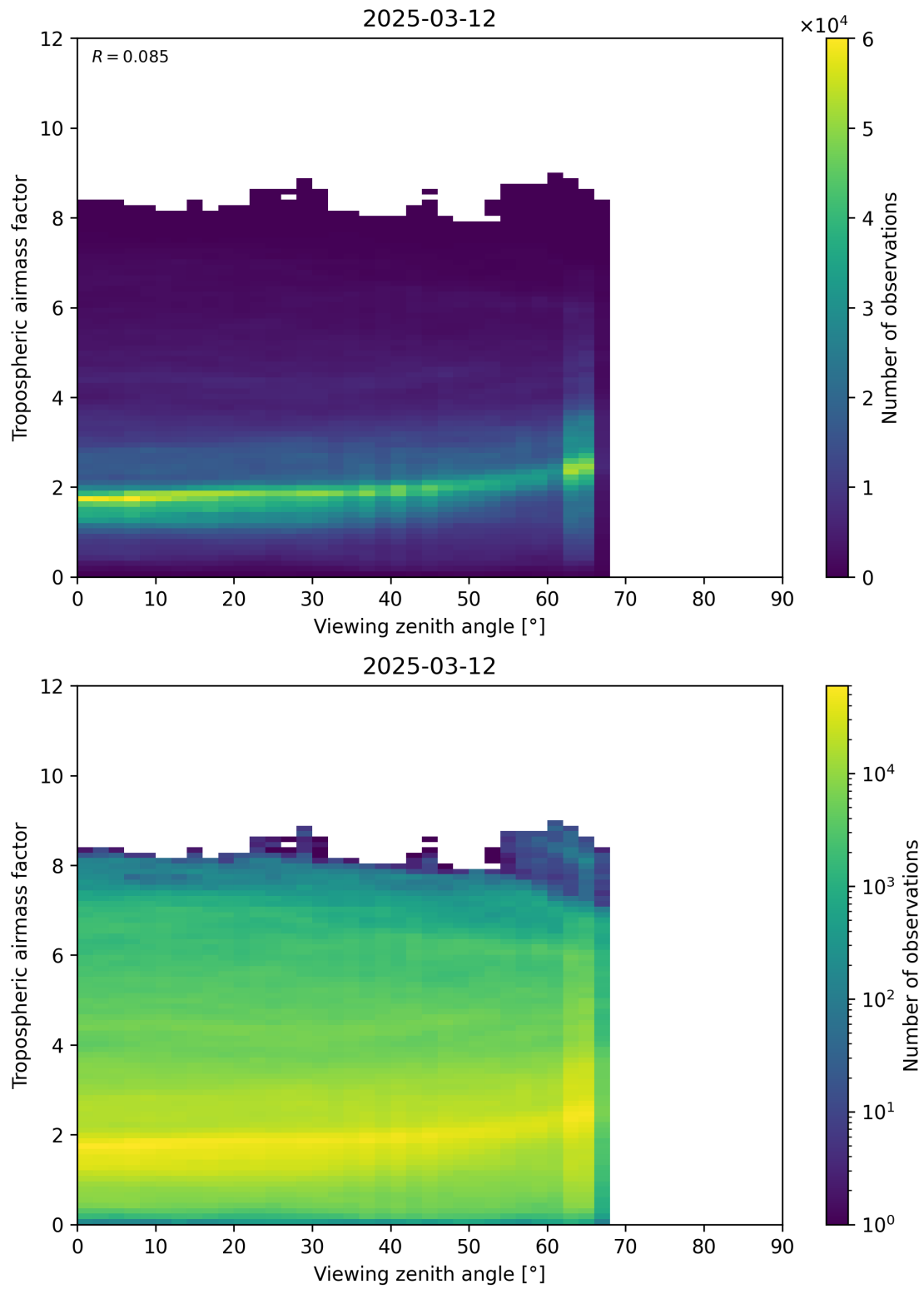
Figure 161: Scatter density plot of “Viewing zenith angle” against “Tropospheric airmass factor” for 2025-03-12 to 2025-03-13.
