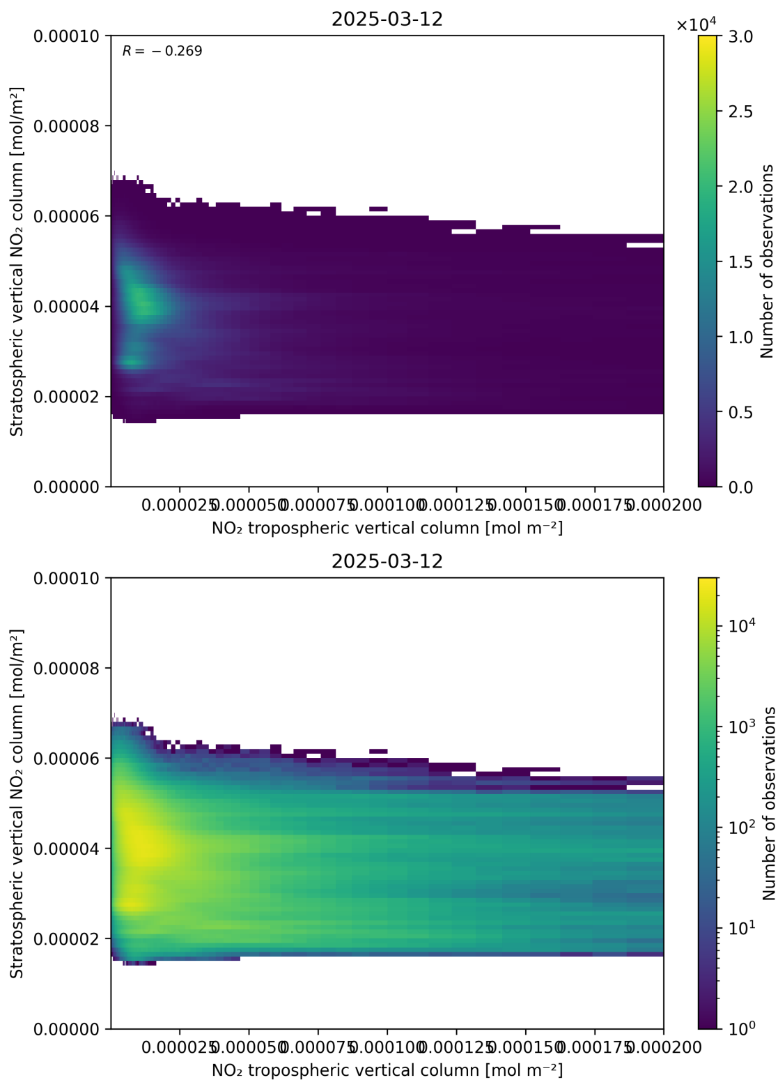
Figure 125: Scatter density plot of “NO 2 tropospheric vertical column” against “Stratospheric vertical NO 2 column” for 2025-03-12 to 2025-03-13.
