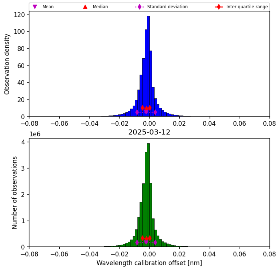
Figure 35: Histogram of “Wavelength calibration offset” for 2025-03-12 to 2025-03-13
