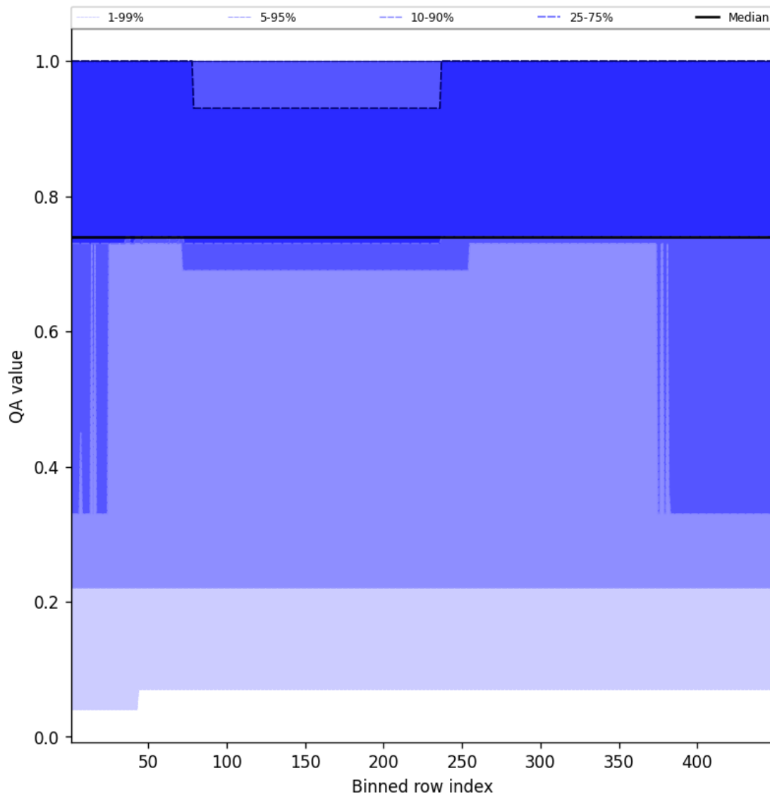
Figure 45: Along track statistics of “QA value” for 2025-03-12 to 2025-03-13
