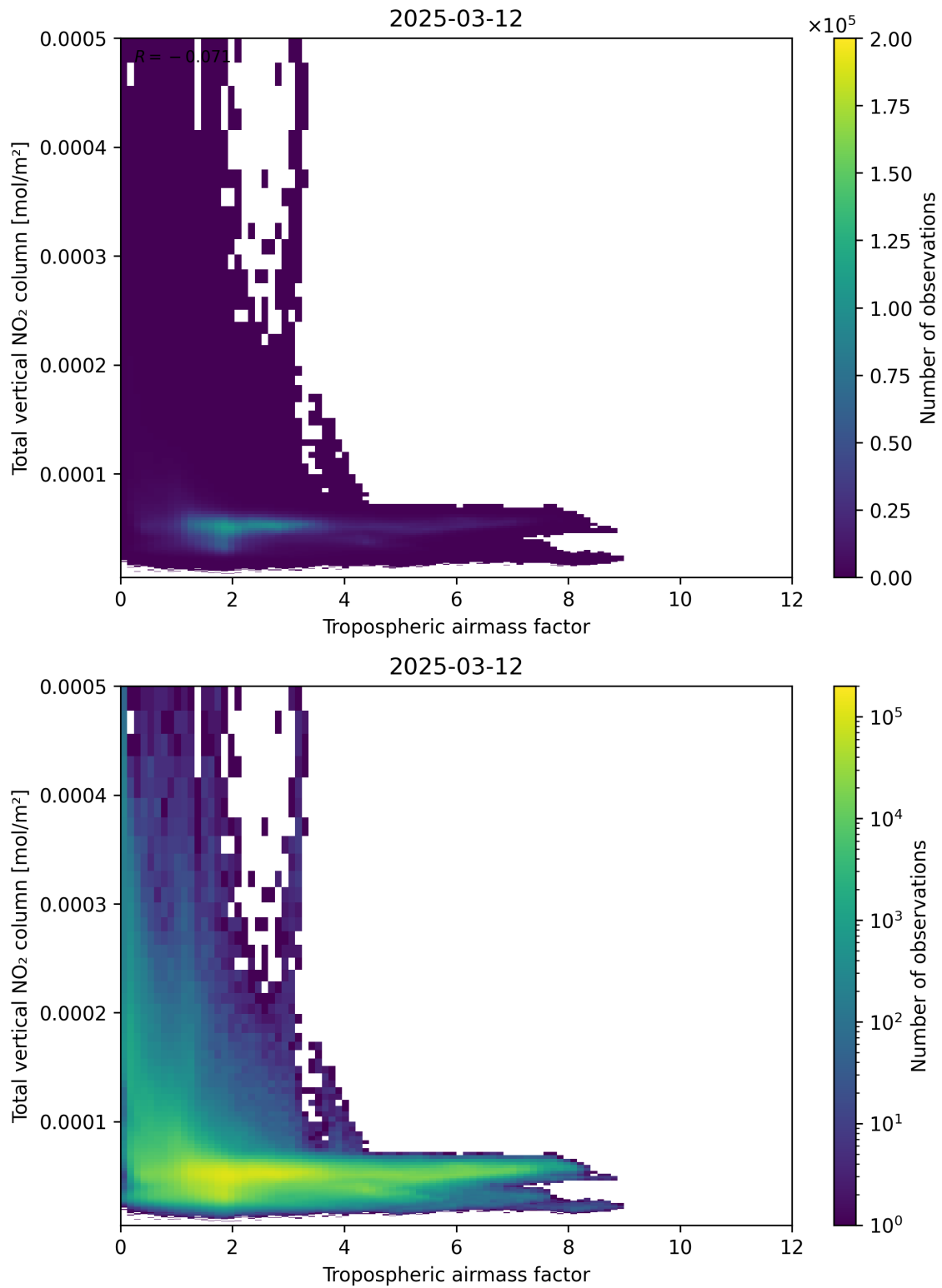
Figure 77: Scatter density plot of “Tropospheric airmass factor” against “Total vertical NO 2 column” for 2025-03-12 to 2025-03-13.
