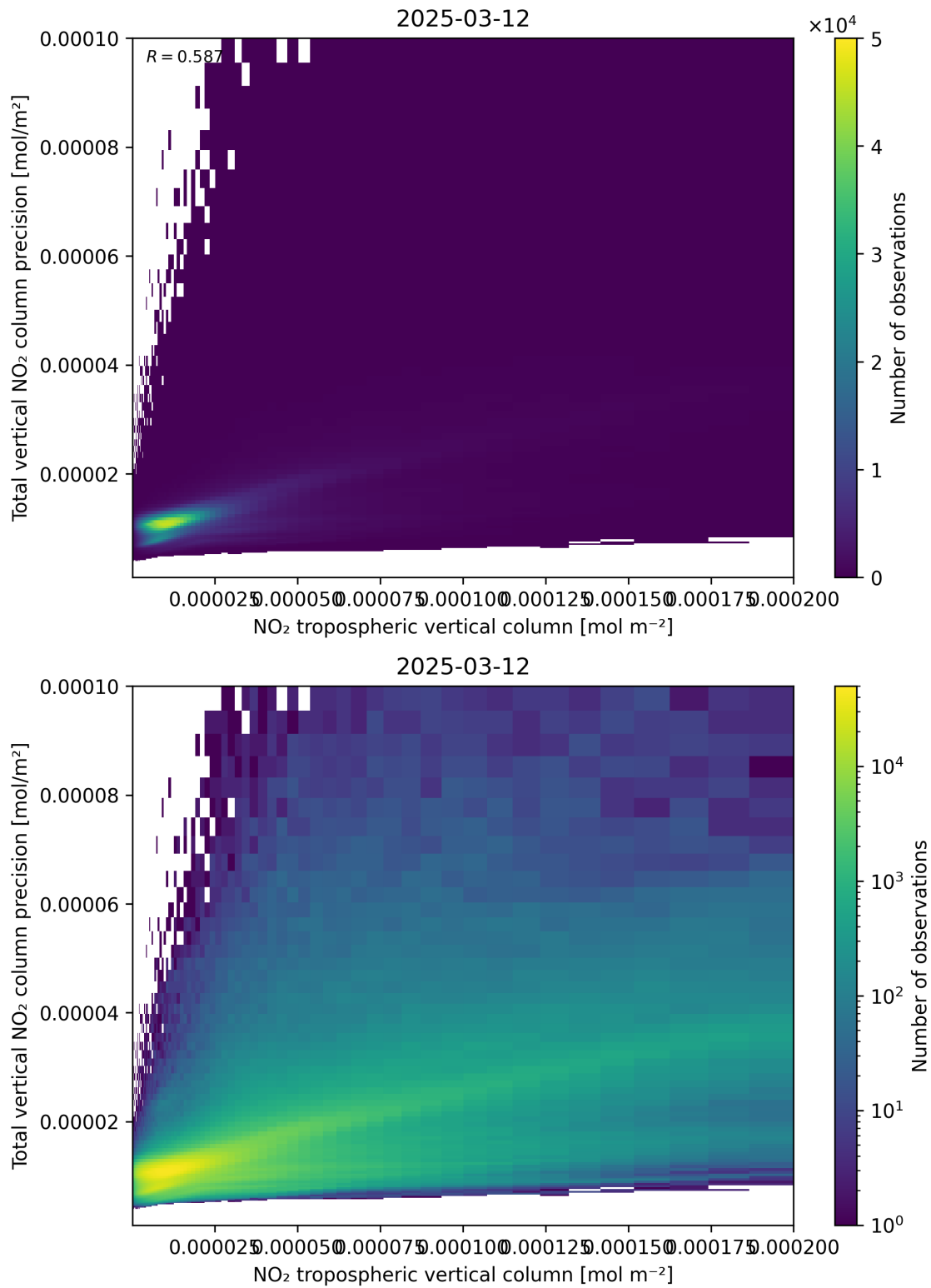
Figure 129: Scatter density plot of “NO 2 tropospheric vertical column” against “Total vertical NO 2 column precision” for 2025-03-12 to 2025-03-13.
