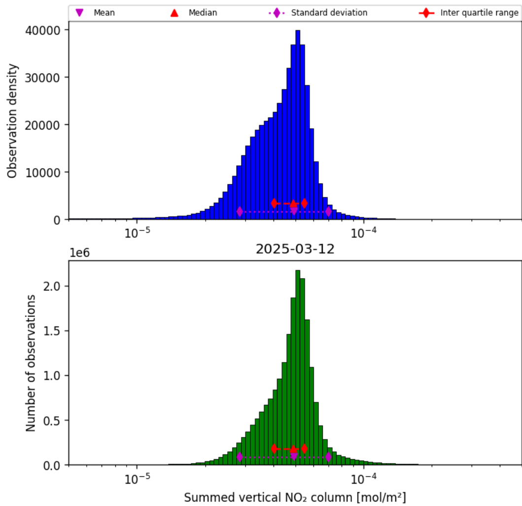
Figure 40: Histogram of “Summed vertical NO 2 column” for 2025-03-12 to 2025-03-13
