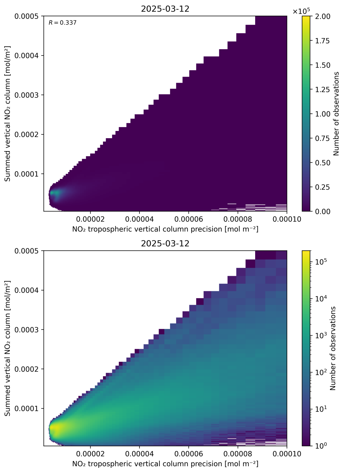
Figure 136: Scatter density plot of “NO 2 tropospheric vertical column precision” against “Summed vertical NO 2 column” for 2025-03-12 to 2025-03-13.
