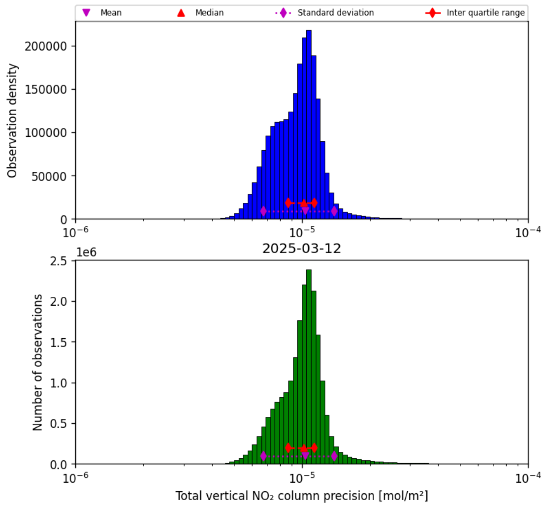
Figure 39: Histogram of “Total vertical NO 2 column precision” for 2025-03-12 to 2025-03-13
