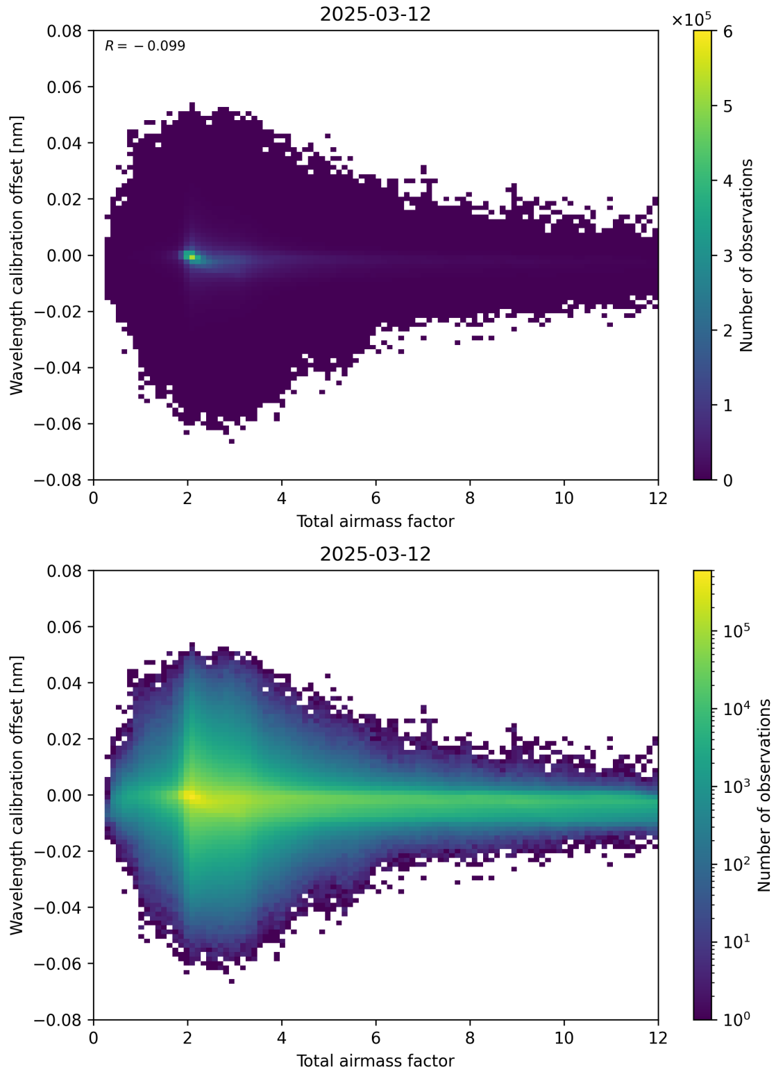
Figure 70: Scatter density plot of “Total airmass factor” against “Wavelength calibration offset” for 2025-03-12 to 2025-03-13.
