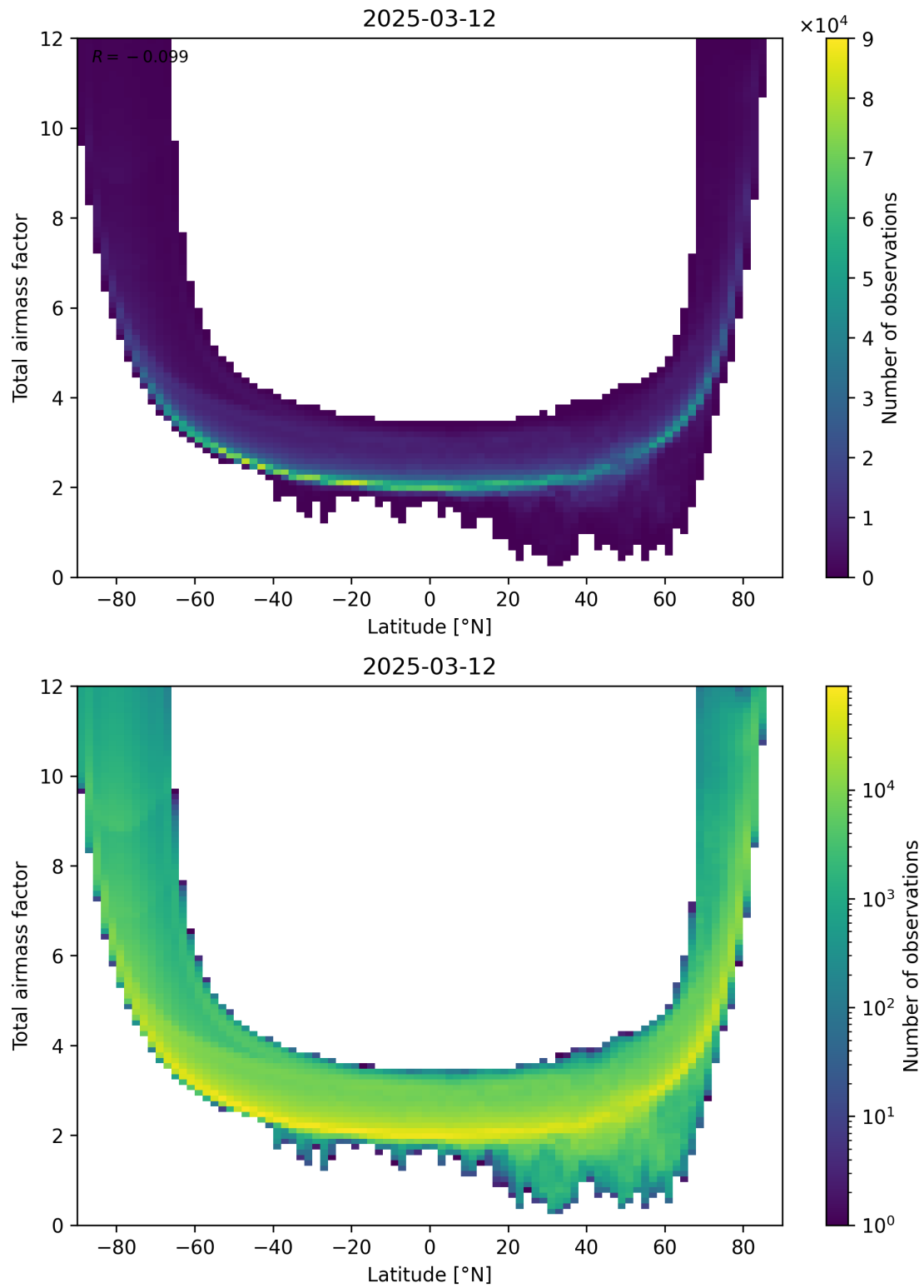
Figure 84: Scatter density plot of “Latitude” against “Total airmass factor” for 2025-03-12 to 2025-03-13.
