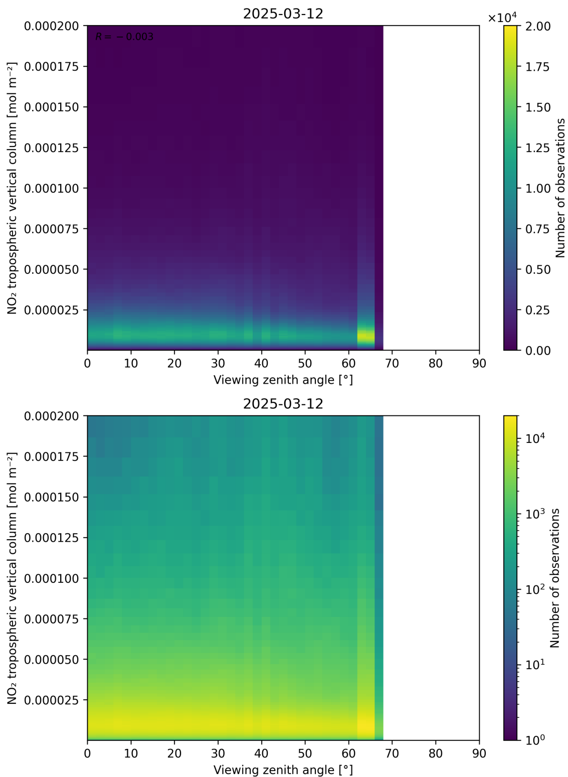
Figure 169: Scatter density plot of “Viewing zenith angle” against “NO 2 tropospheric vertical column” for 2025-03-12 to 2025-03-13.
