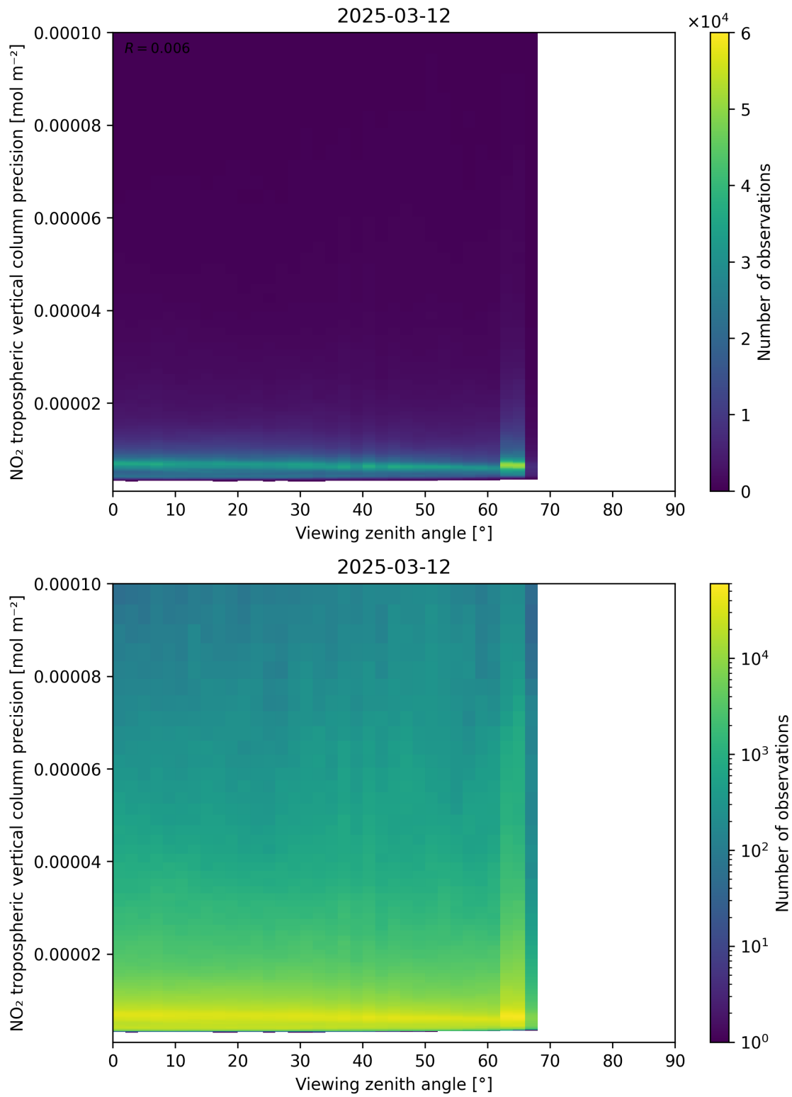
Figure 170: Scatter density plot of “Viewing zenith angle” against “NO 2 tropospheric vertical column precision” for 2025-03-12 to 2025-03-13.
