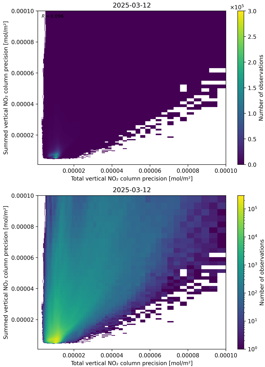
Figure 118: Scatter density plot of “Total vertical NO 2 column precision” against “Summed vertical NO 2 column precision” for 2025-03-12 to 2025-03-13.
