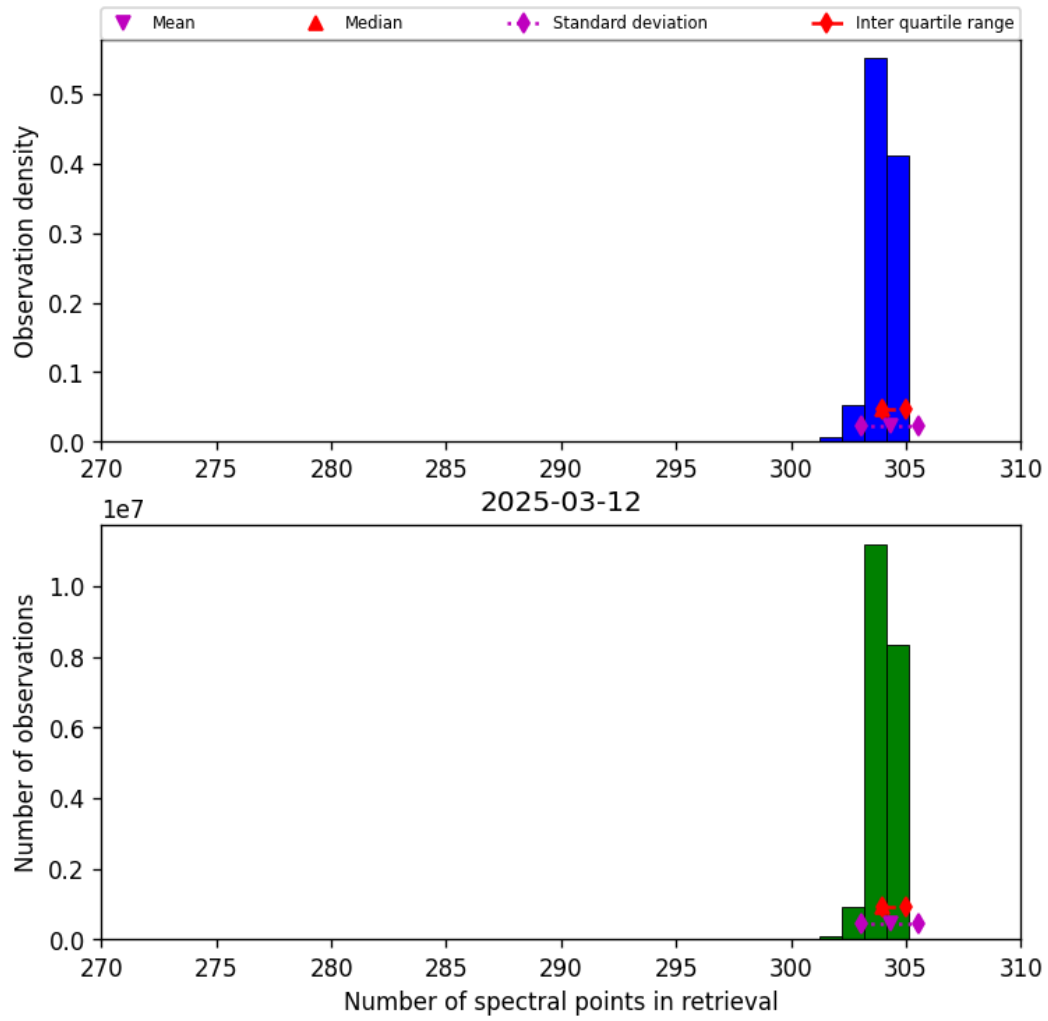
Figure 33: Histogram of “Number of spectral points in retrieval” for 2025-03-12 to 2025-03-13
