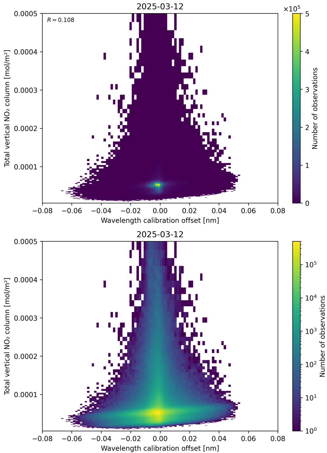
Figure 179: Scatter density plot of “Wavelength calibration offset” against “Total vertical NO 2 column” for 2025-03-12 to 2025-03-13.
