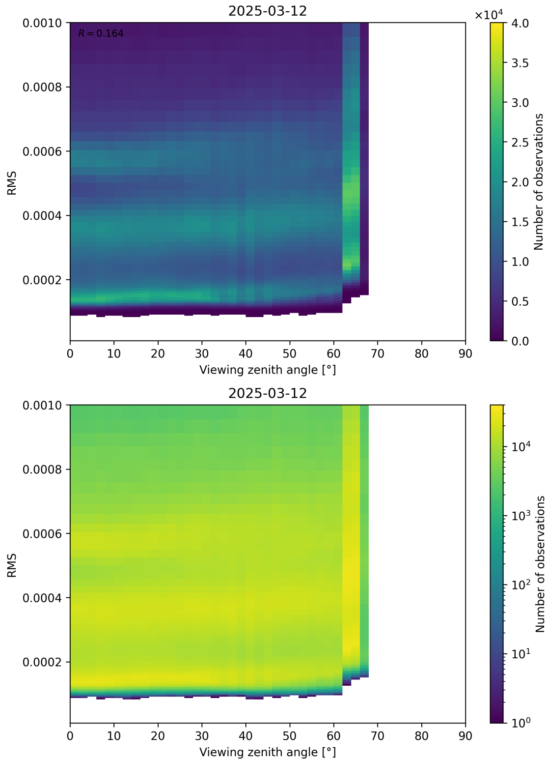
Figure 171: Scatter density plot of “Viewing zenith angle” against “RMS” for 2025-03-12 to 2025-03-13.
