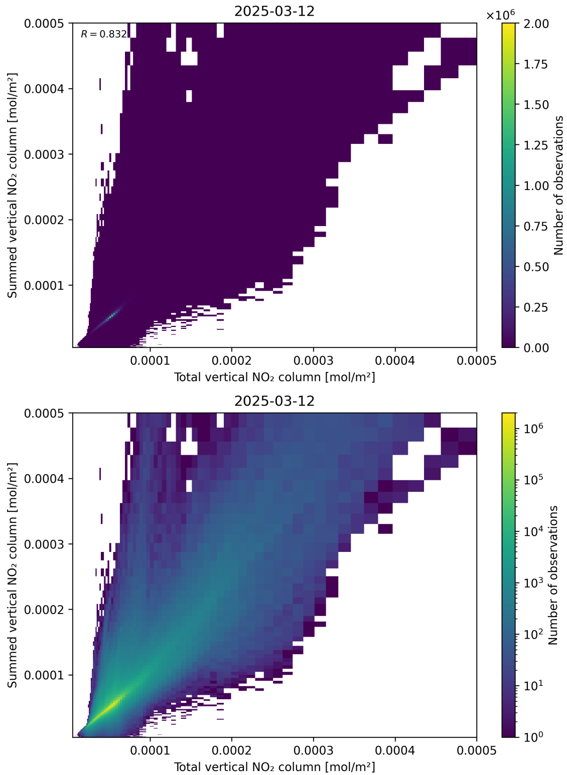
Figure 112: Scatter density plot of “Total vertical NO 2 column” against “Summed vertical NO 2 column” for 2025-03-12 to 2025-03-13.
