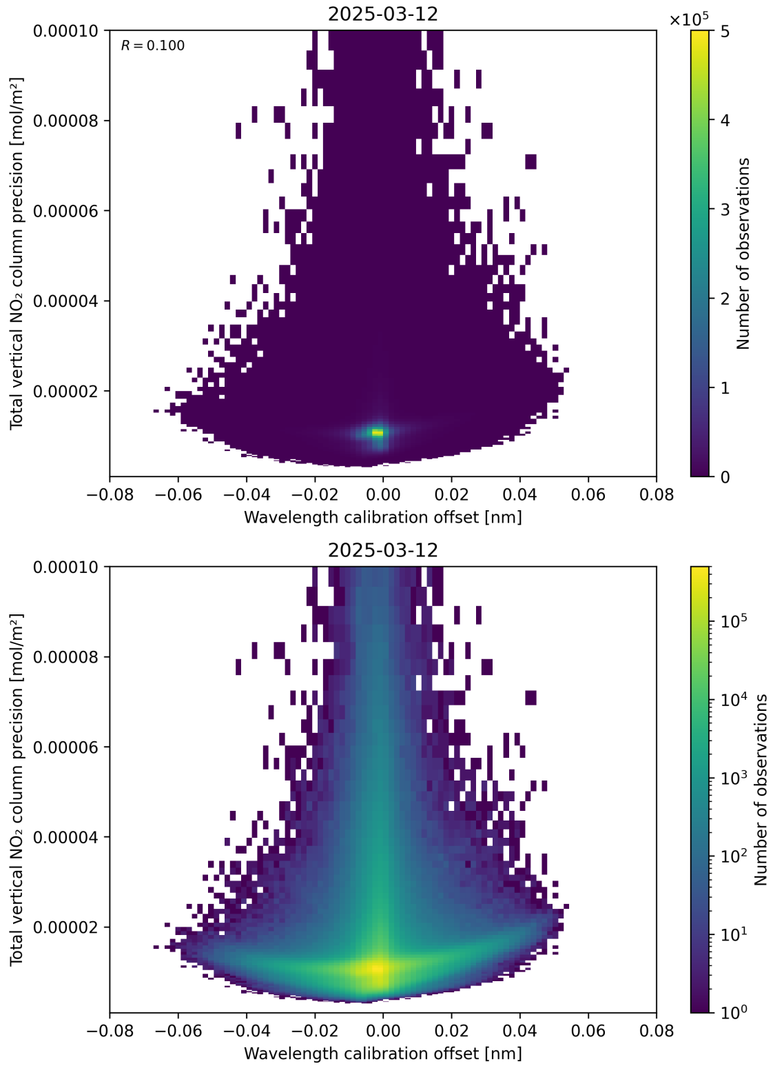
Figure 180: Scatter density plot of “Wavelength calibration offset” against “Total vertical NO 2 column precision” for 2025-03-12 to 2025-03-13.
