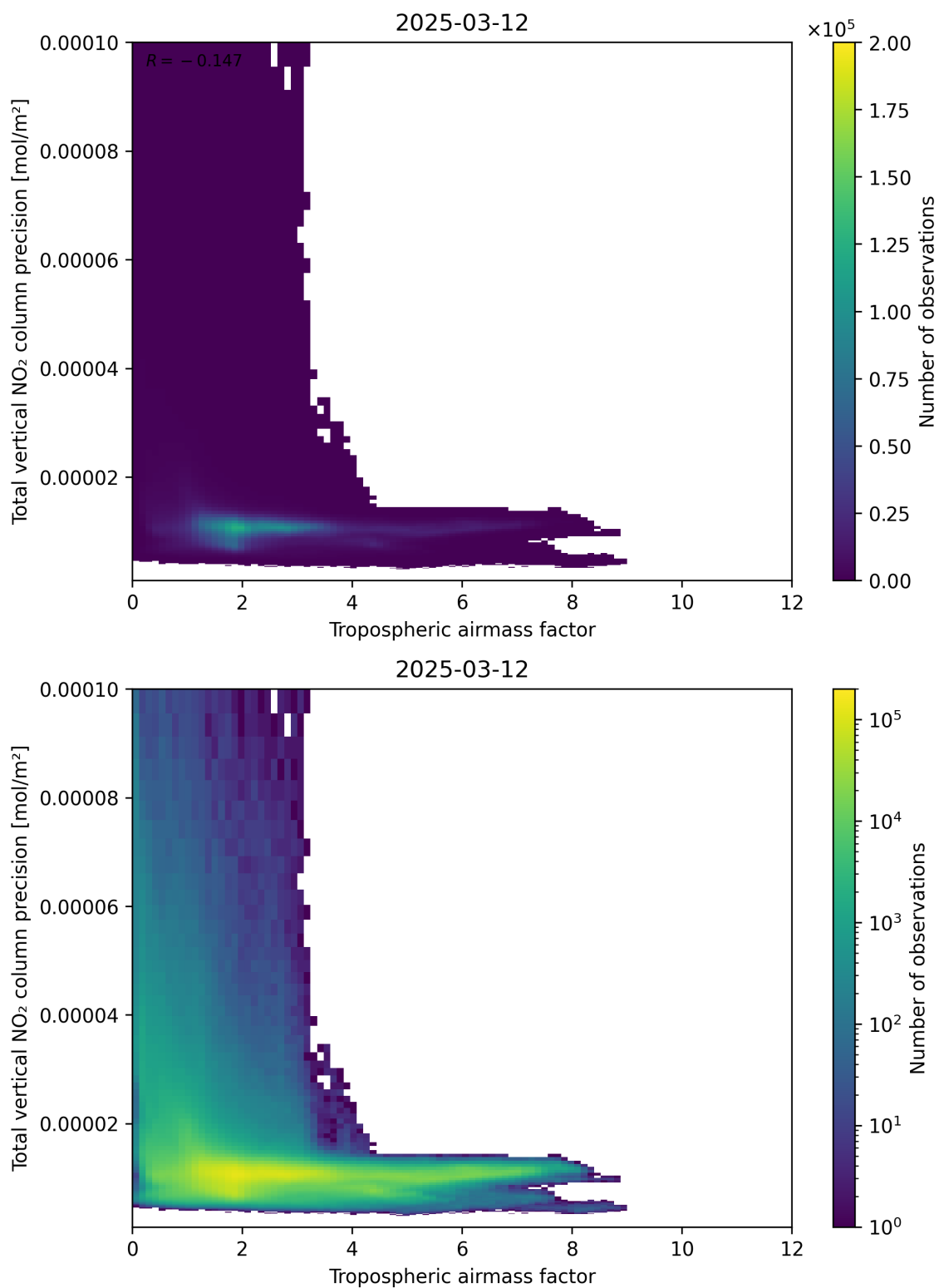
Figure 78: Scatter density plot of “Tropospheric air mass factor” against “Total vertical NO 2 column precision” for 2025-03-12 to 2025-03-13.
