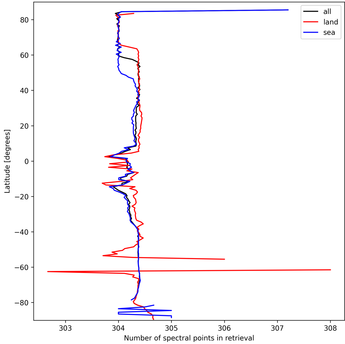
Figure 16: Zonal average of “Number of spectral points in retrieval” for 2025-03-12 to 2025-03-13.
