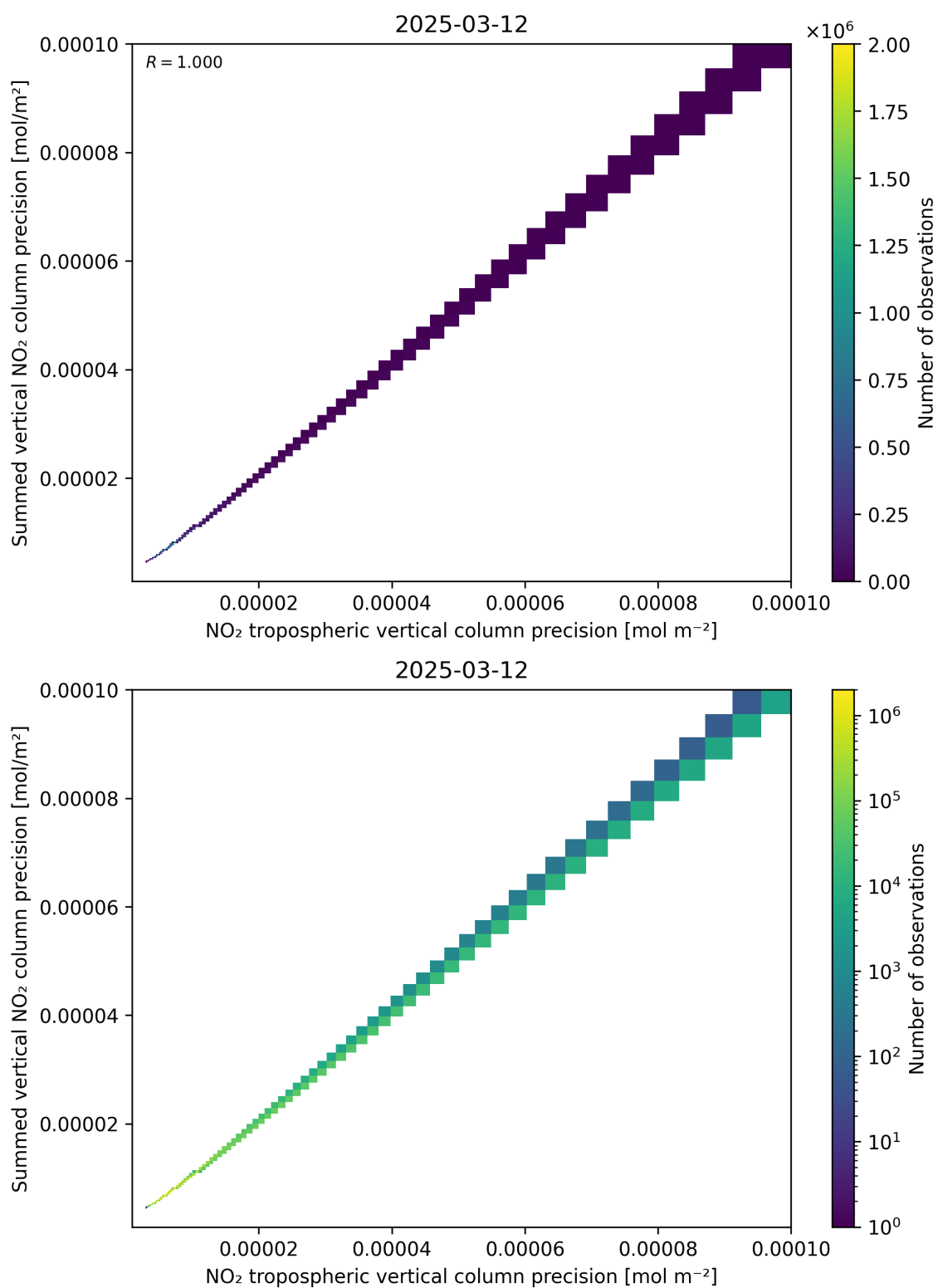
Figure 137: Scatter density plot of “NO 2 tropospheric vertical column precision” against “Summed vertical NO 2 column precision” for 2025-03-12 to 2025-03-13.
