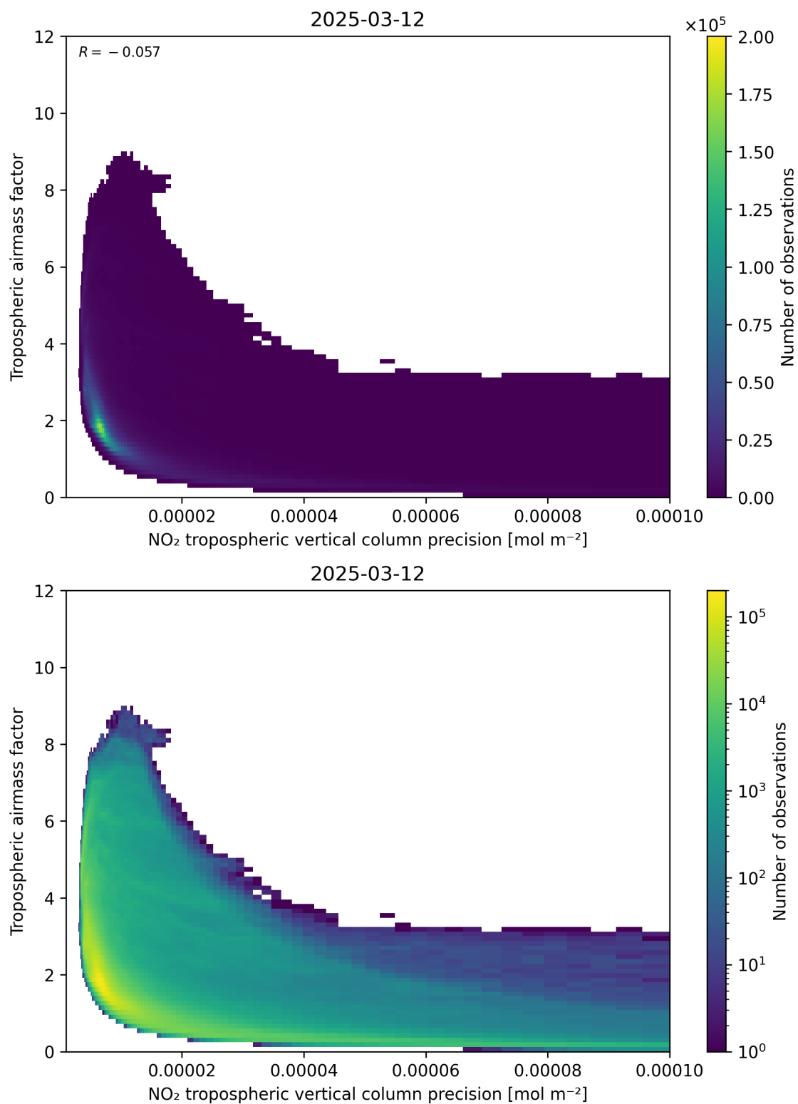
Figure 133: Scatter density plot of “NO 2 tropospheric vertical column precision” against “Tropospheric airmass factor” for 2025-03-12 to 2025-03-13.
