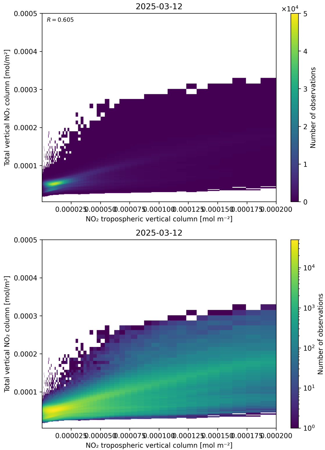
Figure 128: Scatter density plot of “NO 2 tropospheric vertical column” against “Total vertical NO 2 column” for 2025-03-12 to 2025-03-13.
