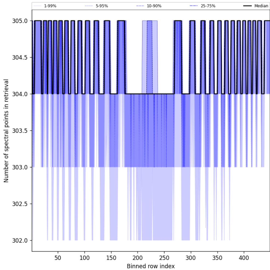
Figure 50: Along track statistics of “Number of spectral points in retrieval” for 2025-03-12 to 2025-03-13
