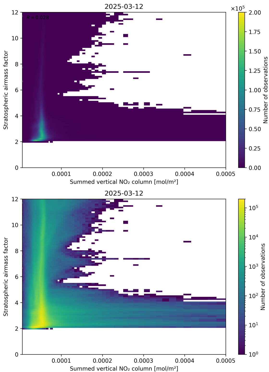
Figure 103: Scatter density plot of “Summed vertical NO 2 column” against “Stratospheric air mass factor” for 2025-03-12 to 2025-03-13.
