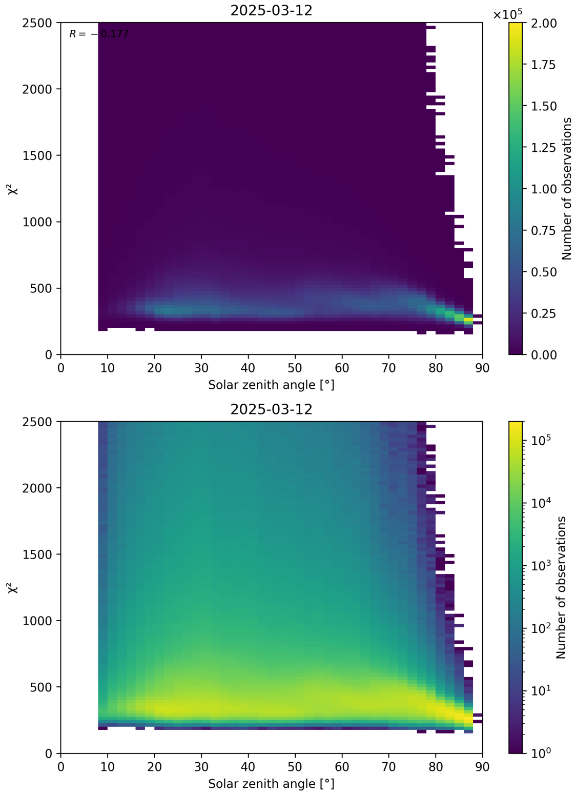
Figure 148: Scatter density plot of “Solar zenith angle” against “ \chi^2 ” for 2025-03-12 to 2025-03-13.
