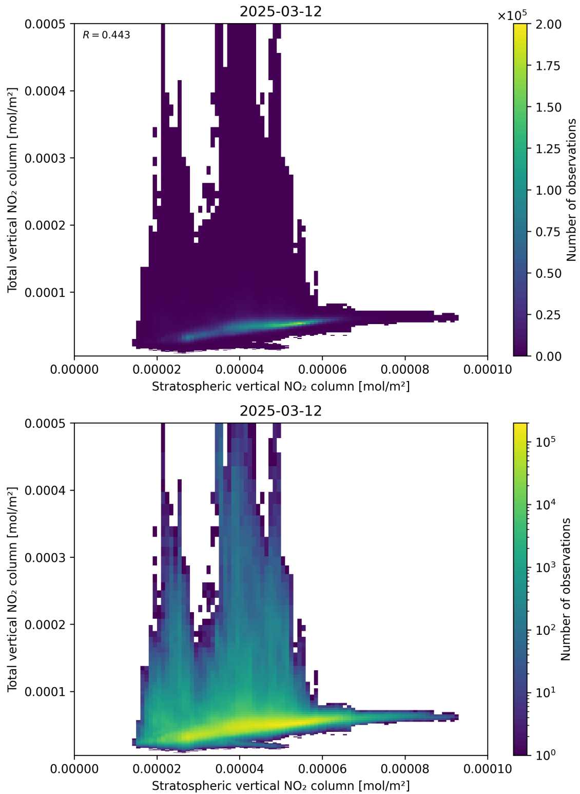
Figure 100: Scatter density plot of “Stratospheric vertical NO 2 column” against “Total vertical NO 2 column” for 2025-03-12 to 2025-03-13.
