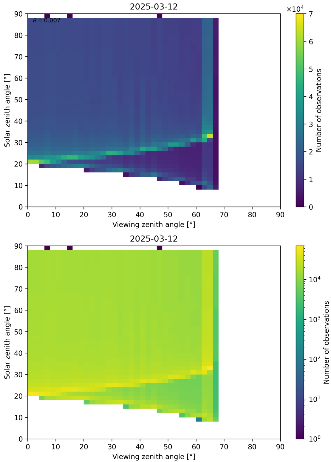
Figure 172: Scatter density plot of “Viewing zenith angle” against “Solar zenith angle” for 2025-03-12 to 2025-03-13.
