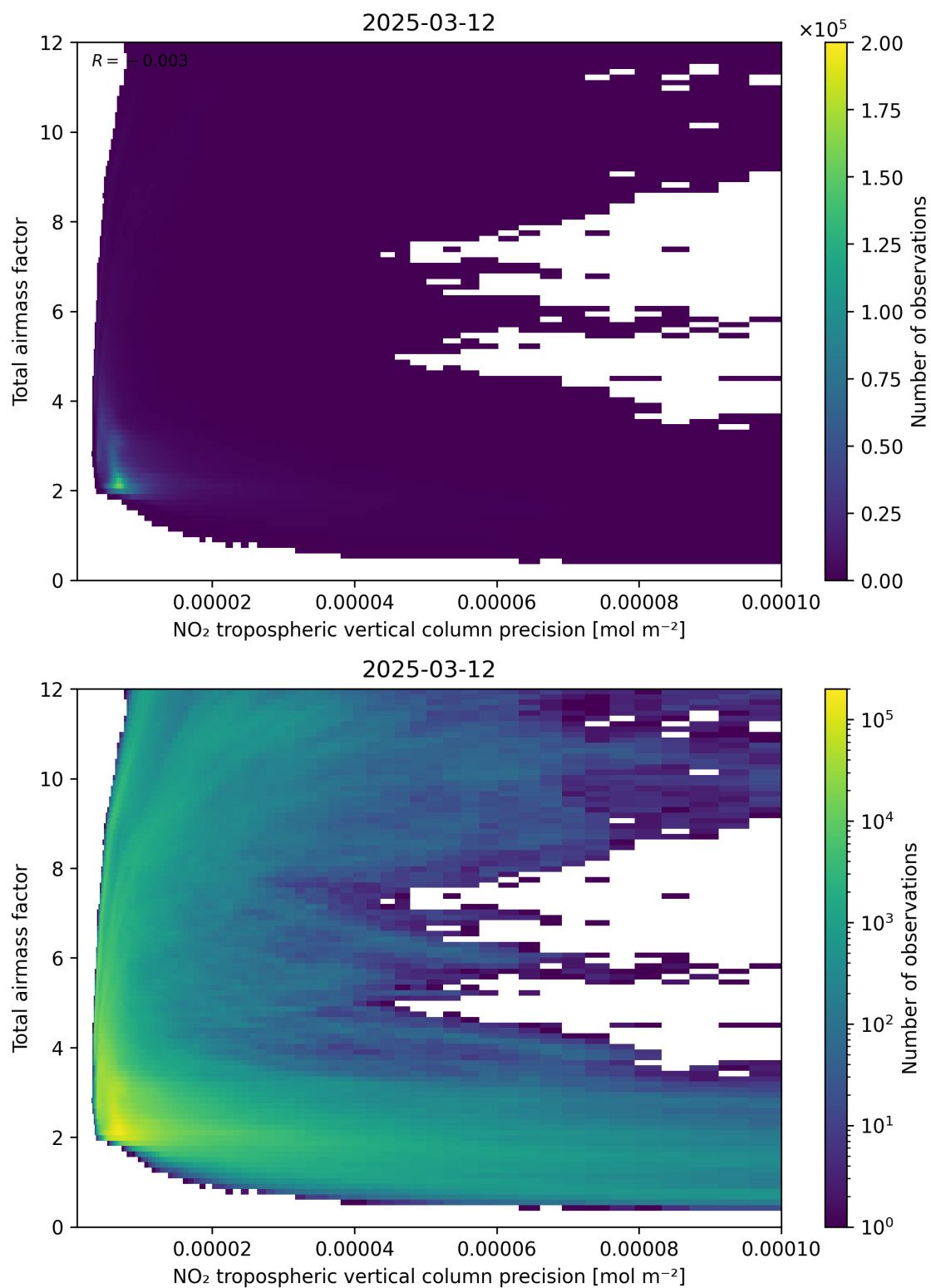
Figure 132: Scatter density plot of “NO 2 tropospheric vertical column precision” against “Total air mass factor” for 2025-03-12 to 2025-03-13.
