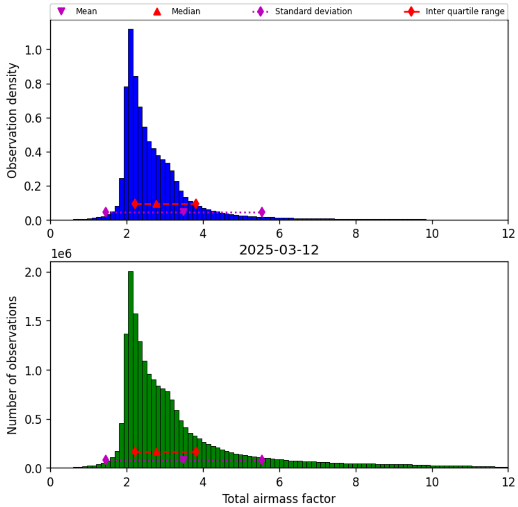
Figure 32: Histogram of “Total airmass factor” for 2025-03-12 to 2025-03-13
