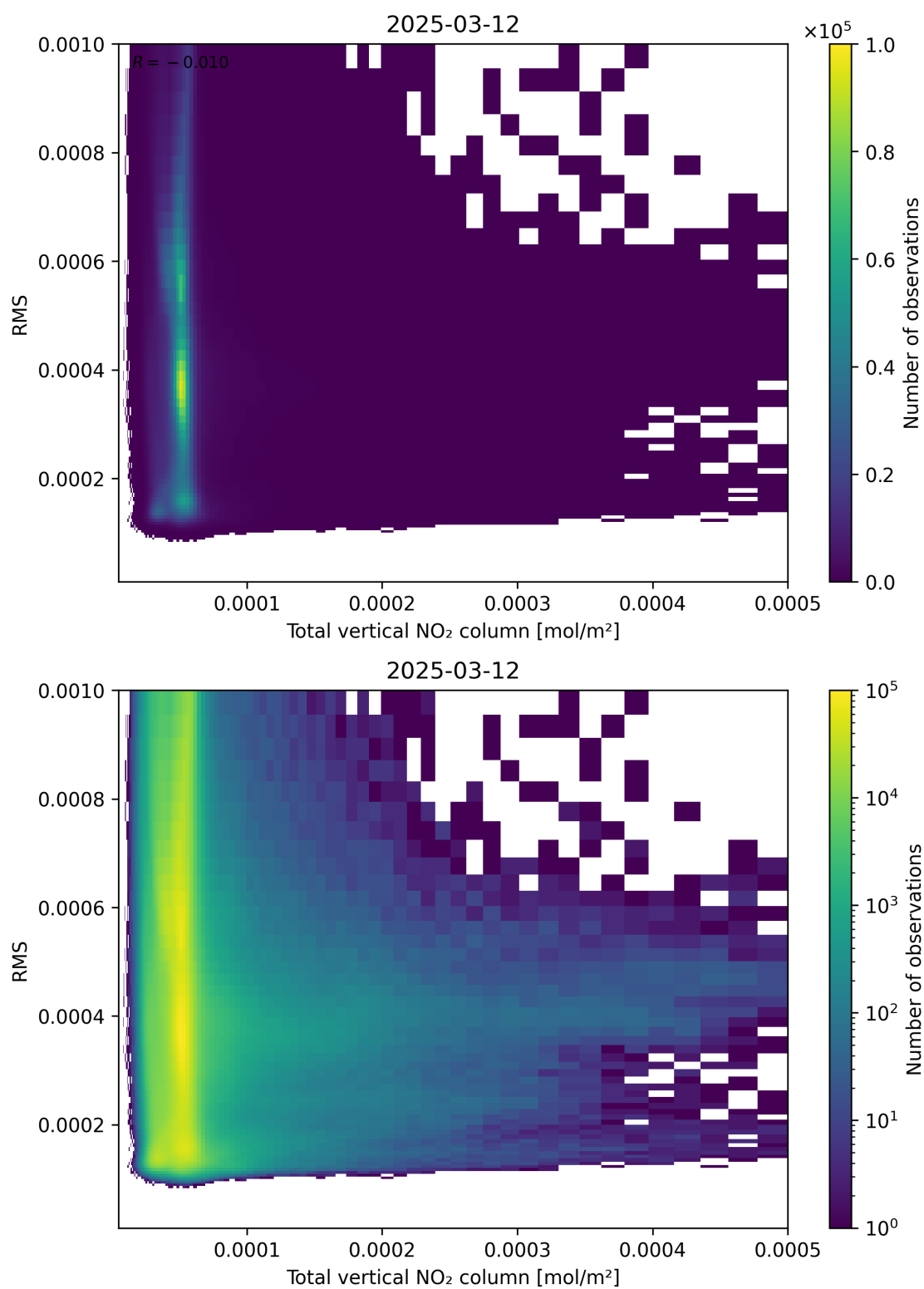
Figure 120: Scatter density plot of “Total vertical NO 2 column” against “RMS” for 2025-03-12 to 2025-03-13.
