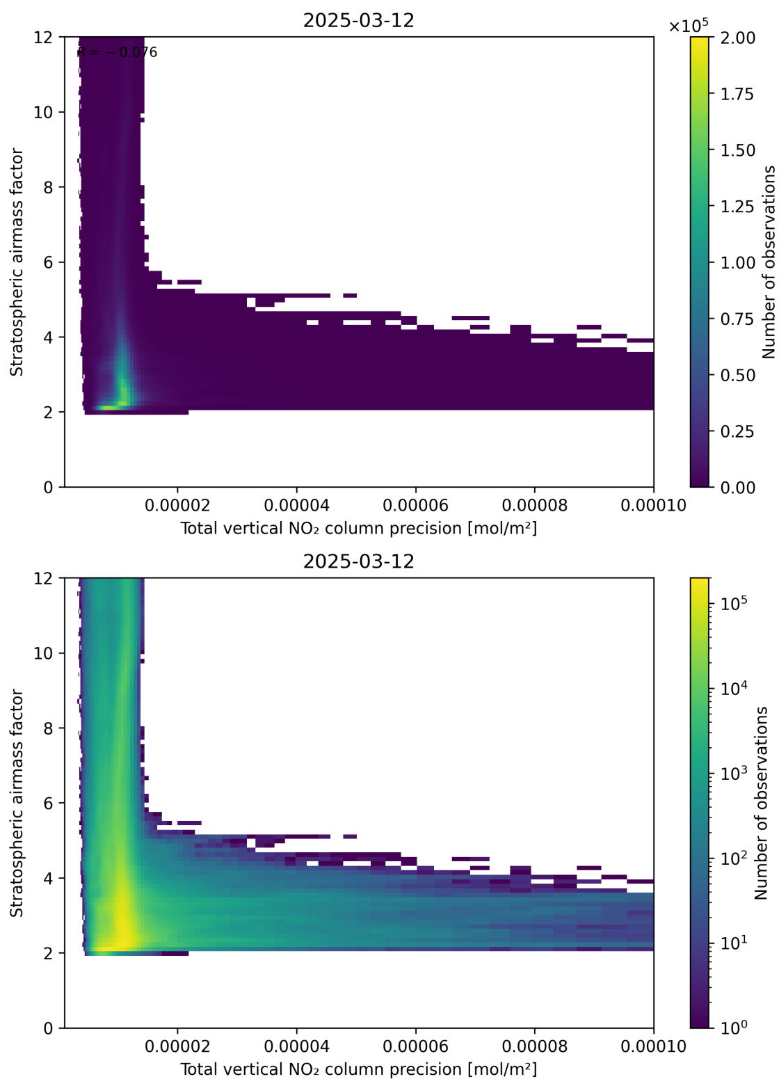
Figure 115: Scatter density plot of “Total vertical NO 2 column precision” against “Stratospheric air mass factor” for 2025-03-12 to 2025-03-13.
