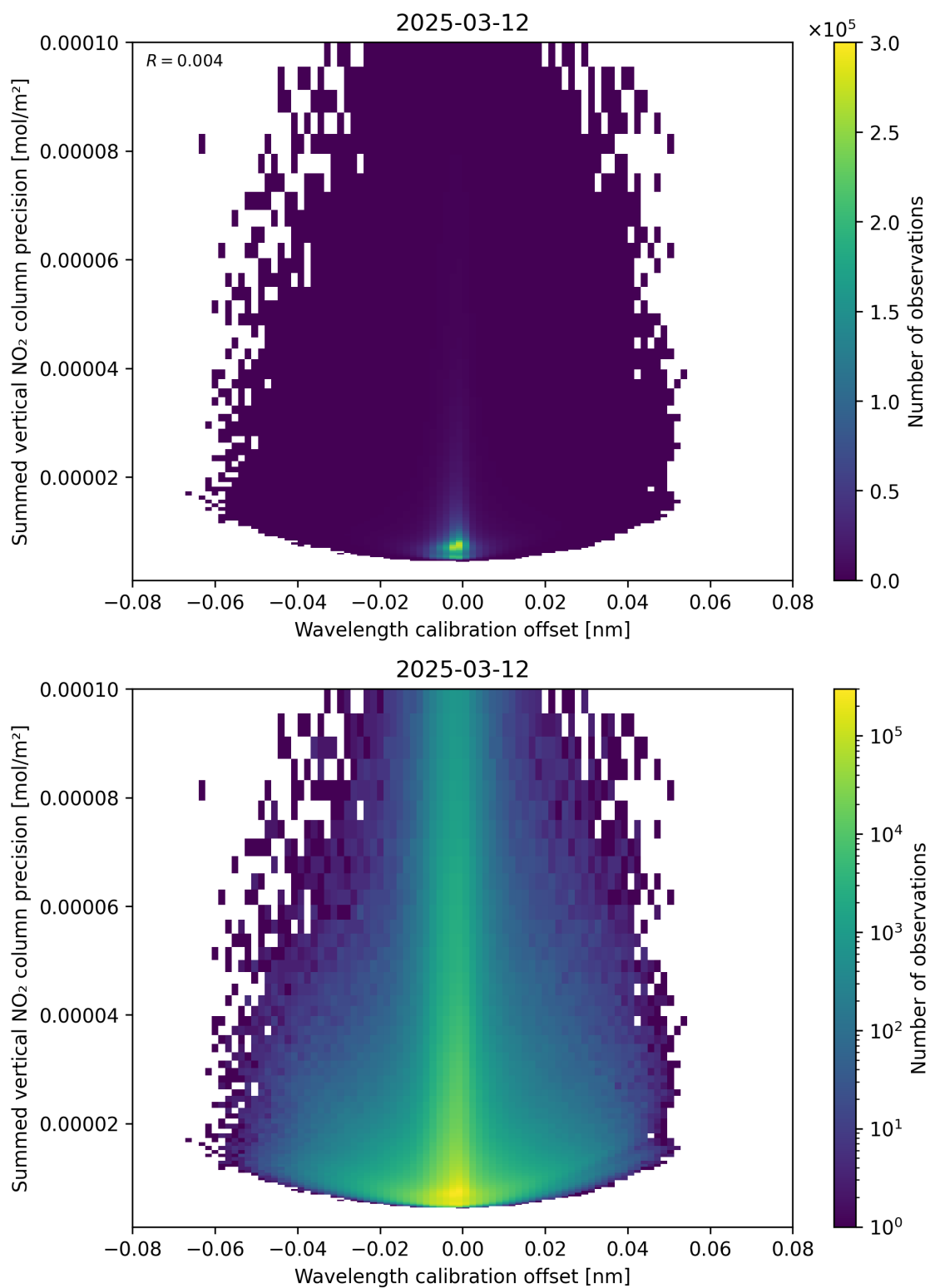
Figure 178: Scatter density plot of “Wavelength calibration offset” against “Summed vertical NO 2 column precision” for 2025-03-12 to 2025-03-13.
