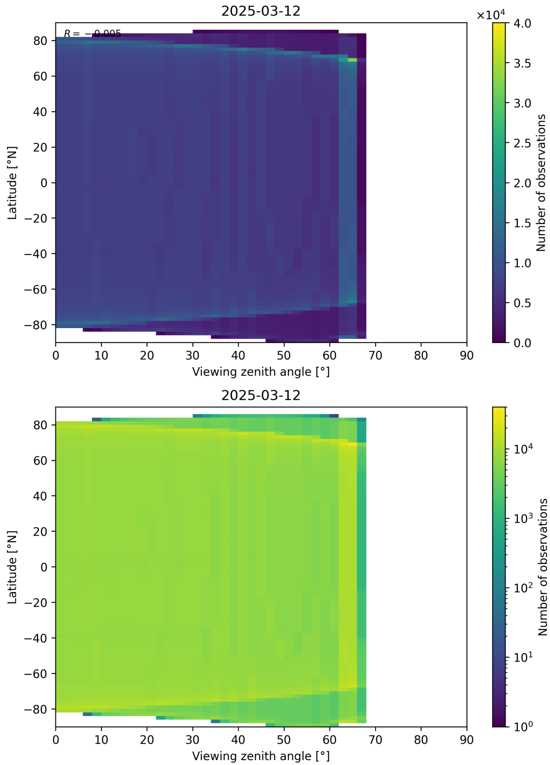
Figure 163: Scatter density plot of “Viewing zenith angle” against “Latitude” for 2025-03-12 to 2025-03-13.
