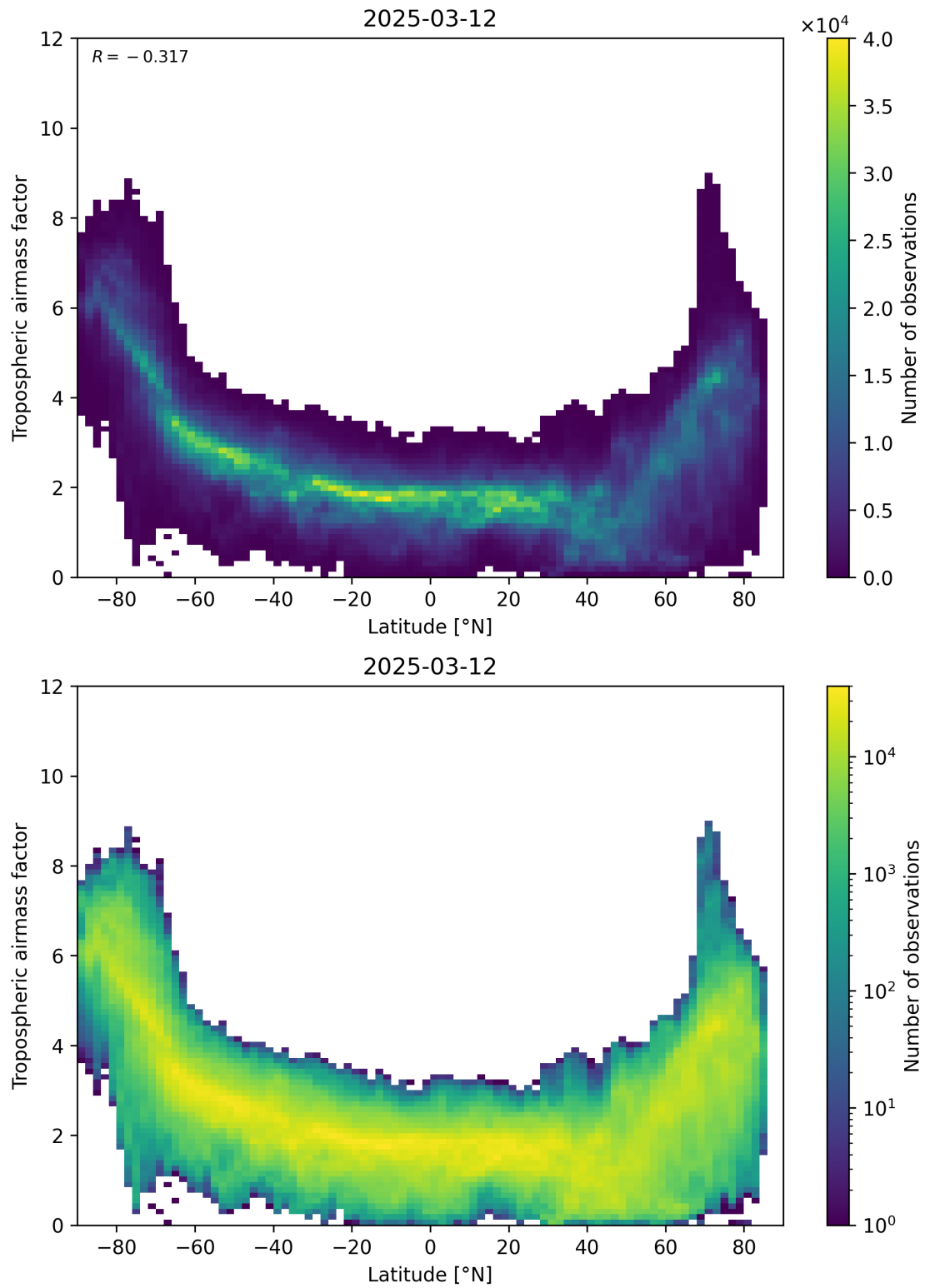
Figure 85: Scatter density plot of “Latitude” against “Tropospheric airmass factor” for 2025-03-12 to 2025-03-13.
