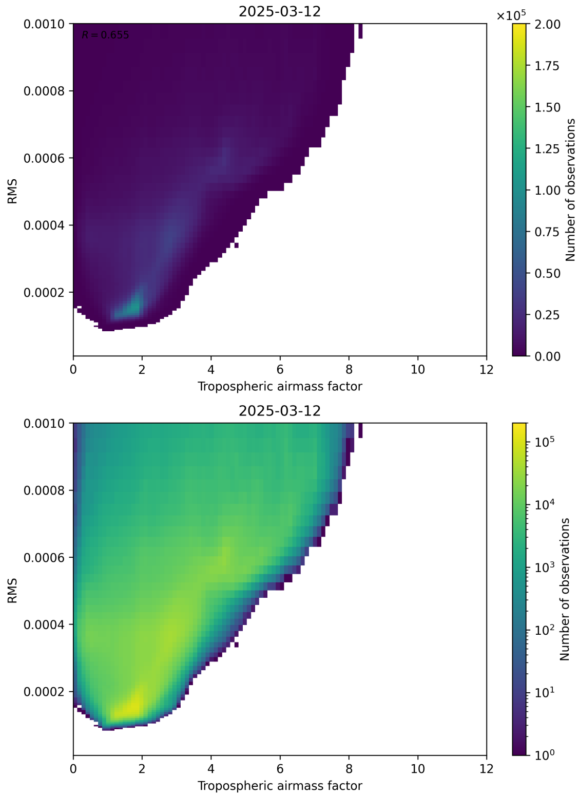
Figure 79: Scatter density plot of “Tropospheric airmass factor” against “RMS” for 2025-03-12 to 2025-03-13.
