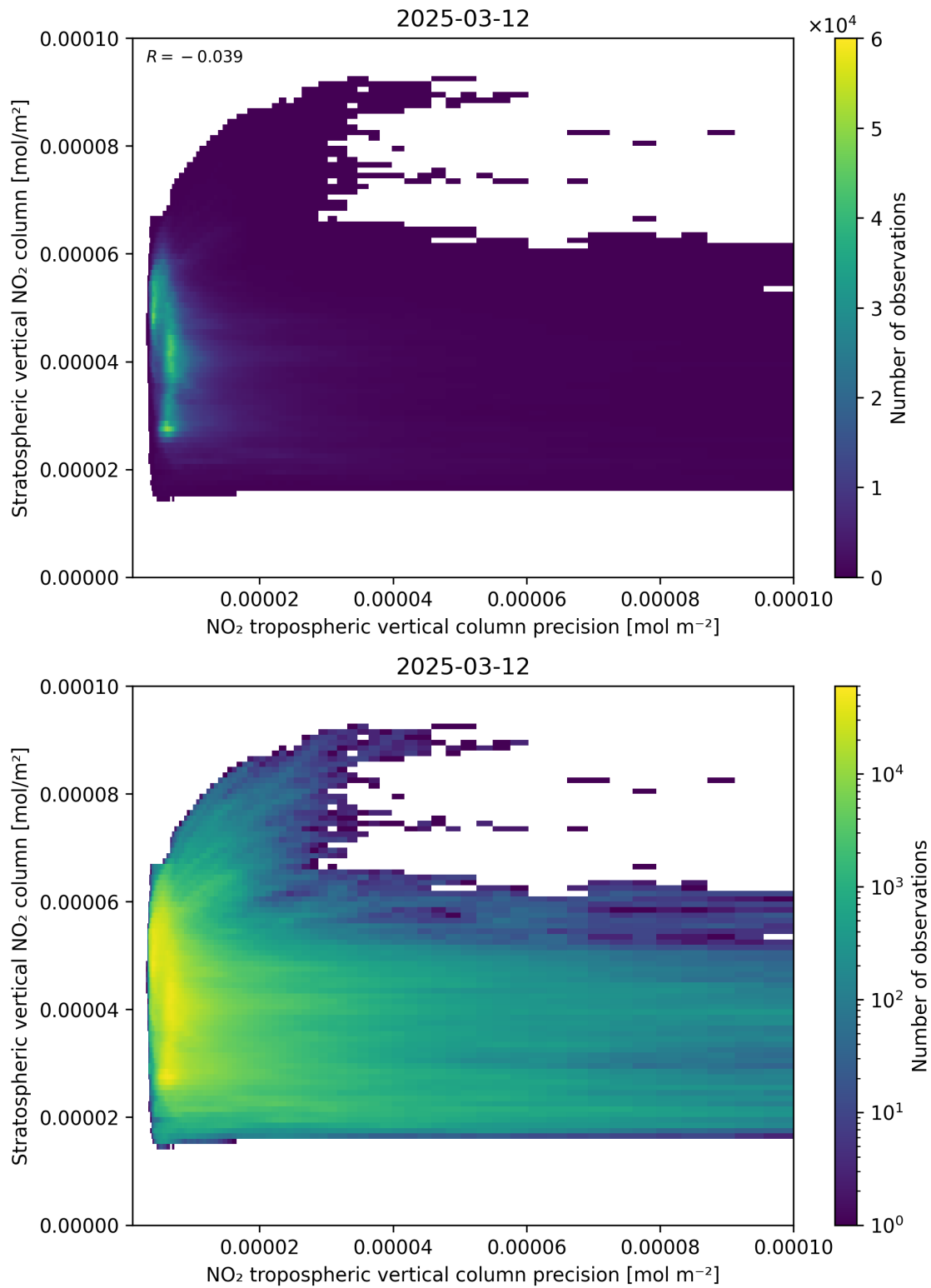
Figure 135: Scatter density plot of “NO 2 tropospheric vertical column precision” against “Stratospheric vertical NO 2 column” for 2025-03-12 to 2025-03-13.
