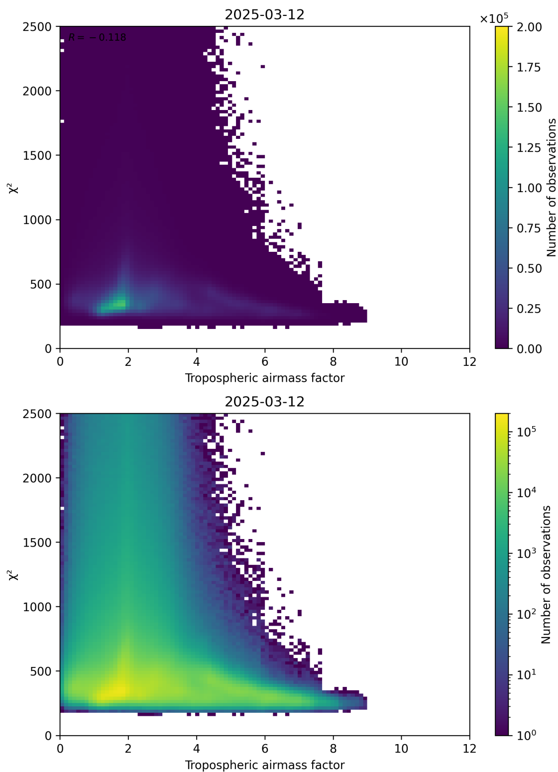
Figure 73: Scatter density plot of “Tropospheric airmass factor” against “ \chi^2 ” for 2025-03-12 to 2025-03-13.
