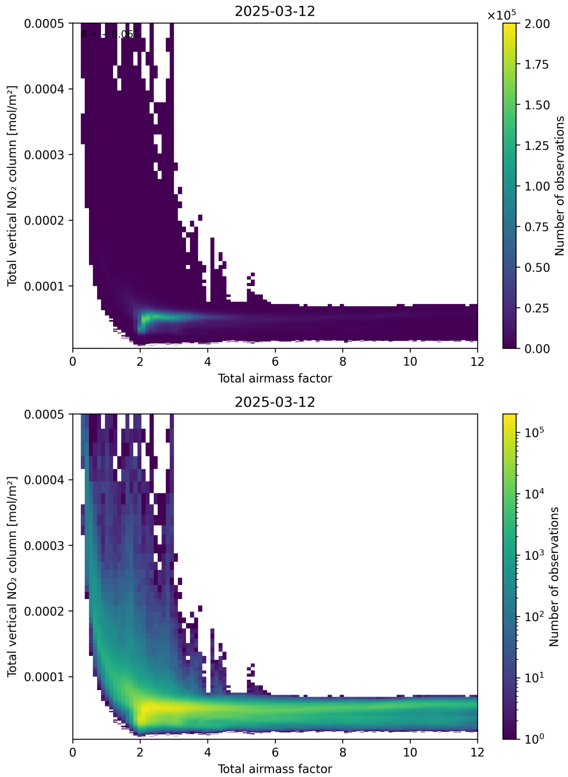
Figure 67: Scatter density plot of “Total airmass factor” against “Total vertical NO 2 column” for 2025-03-12 to 2025-03-13.
