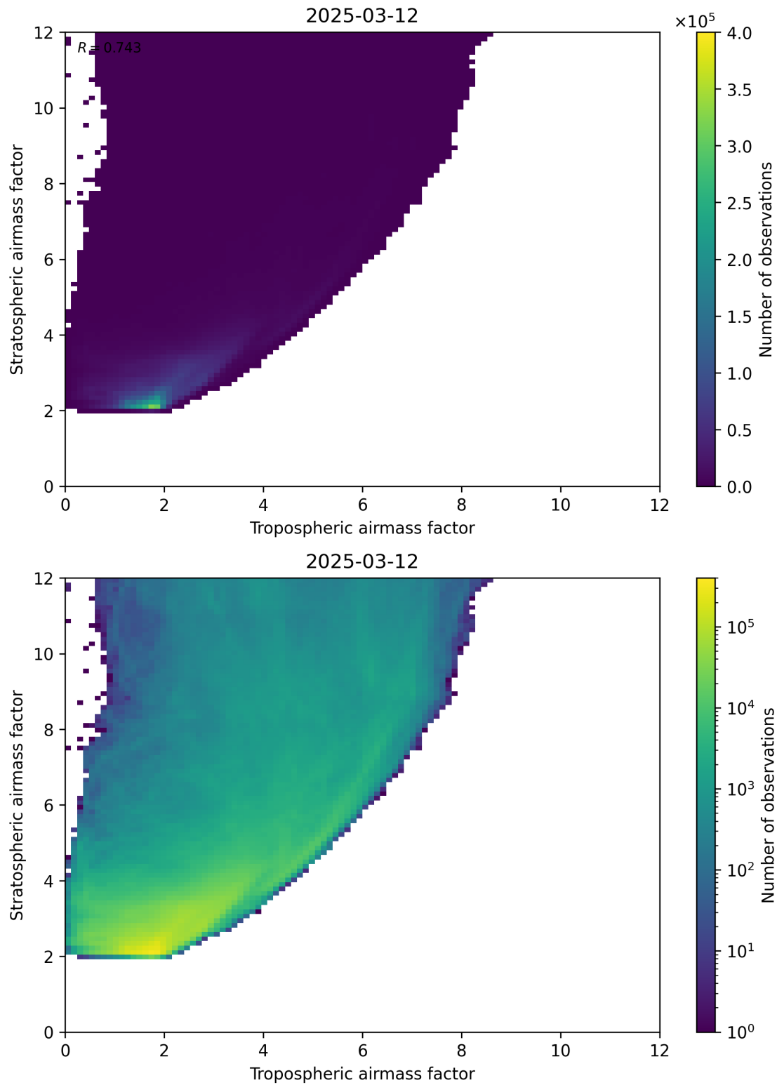
Figure 71: Scatter density plot of “Tropospheric airmass factor” against “Stratospheric airmass factor” for 2025-03-12 to 2025-03-13.
