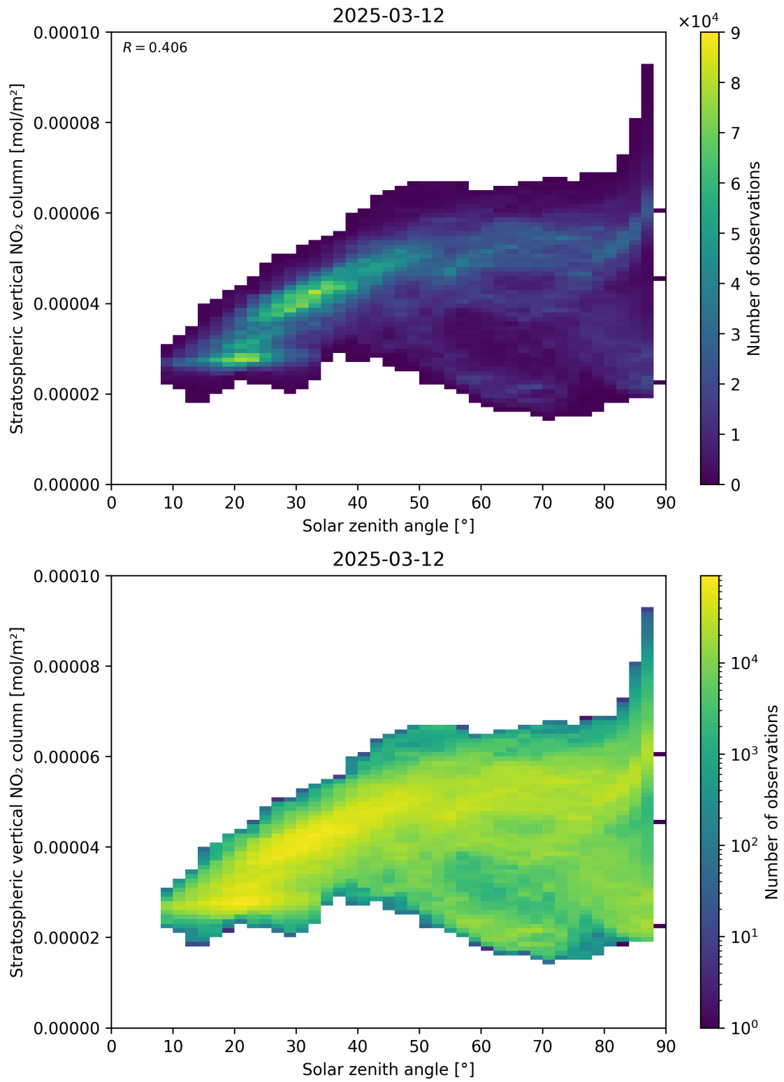
Figure 150: Scatter density plot of “Solar zenith angle” against “Stratospheric vertical \text{NO}_2 column” for 2025-03-12 to 2025-03-13.
