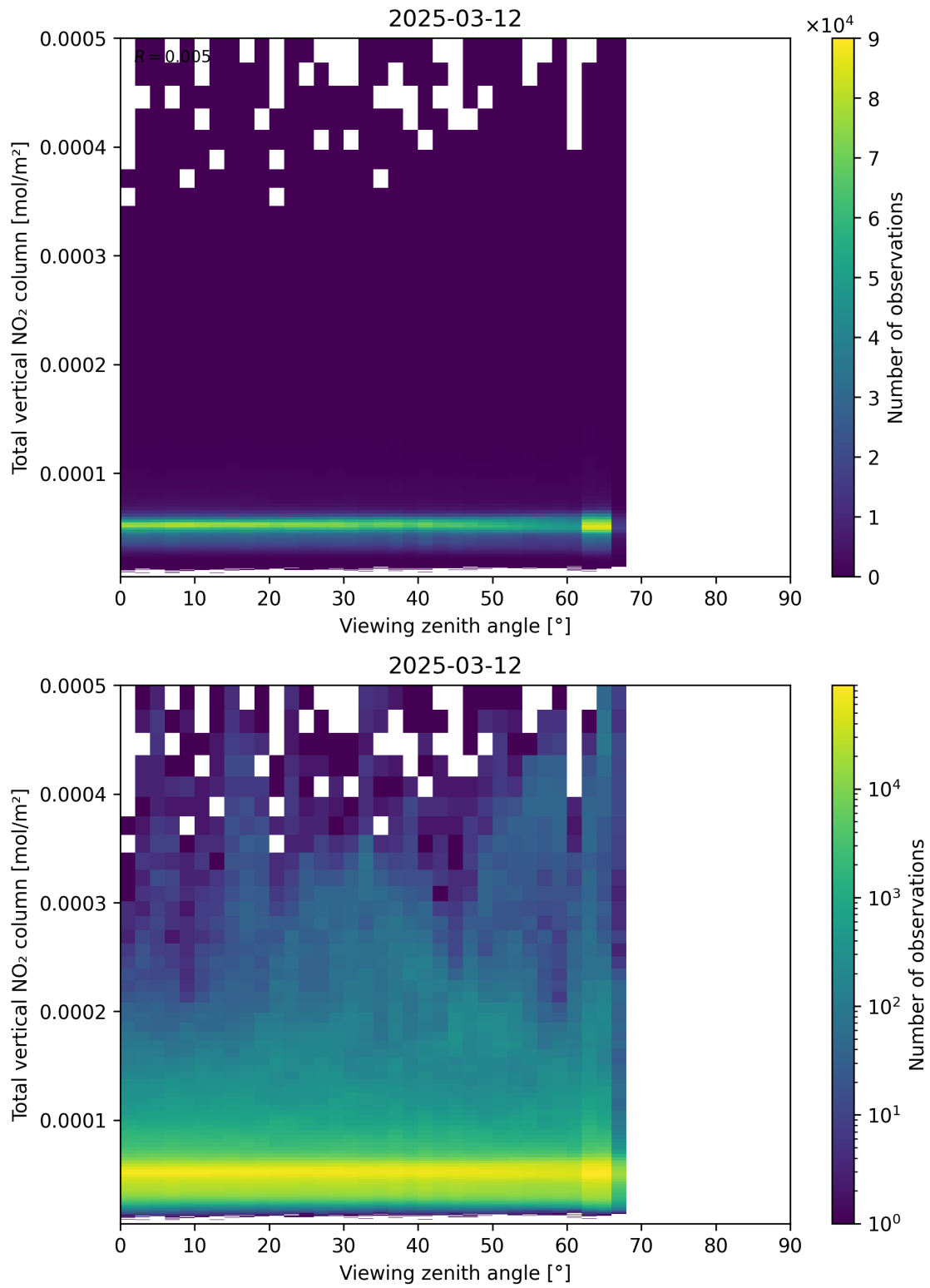
Figure 167: Scatter density plot of “Viewing zenith angle” against “Total vertical NO 2 column” for 2025-03-12 to 2025-03-13.
