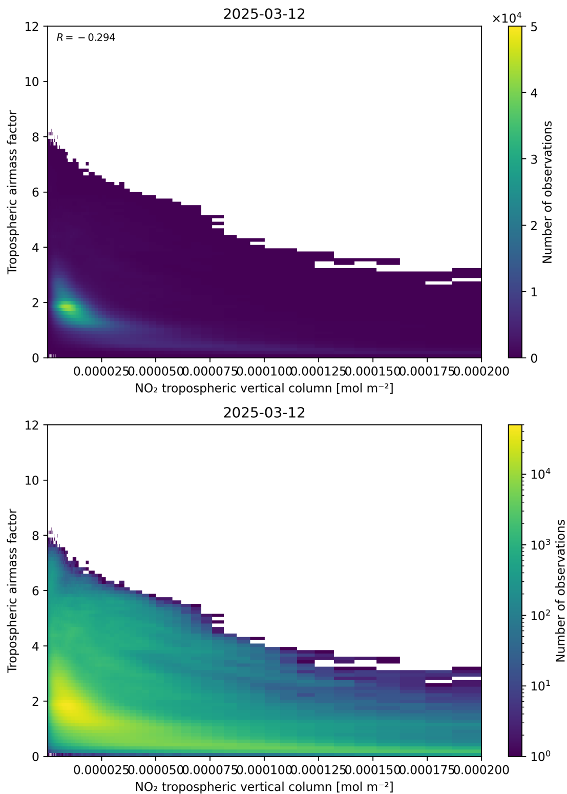
Figure 123: Scatter density plot of “NO 2 tropospheric vertical column” against “Tropospheric air mass factor” for 2025-03-12 to 2025-03-13.
