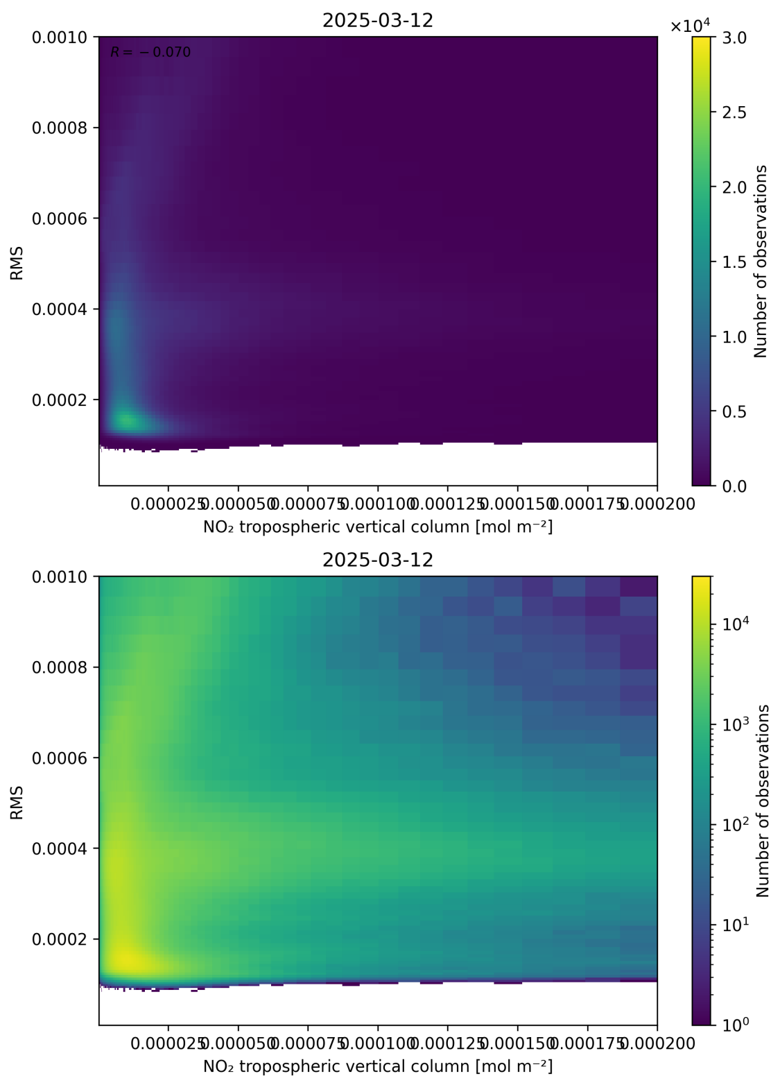
Figure 142: Scatter density plot of “NO 2 tropospheric vertical column” against “RMS” for 2025-03-12 to 2025-03-13.
