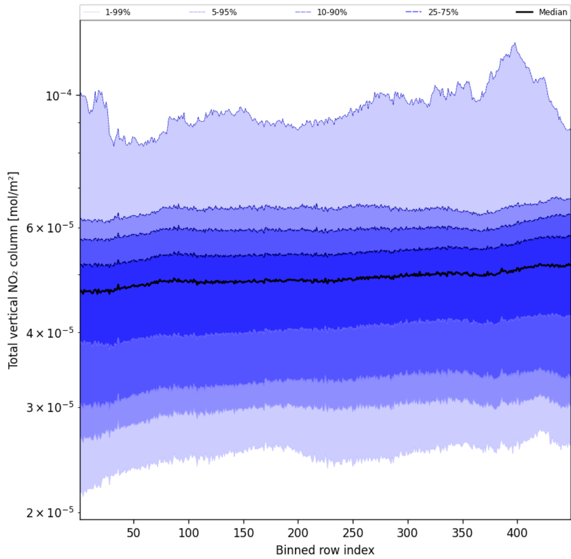
Figure 55: Along track statistics of “Total vertical NO 2 column” for 2025-03-12 to 2025-03-13
