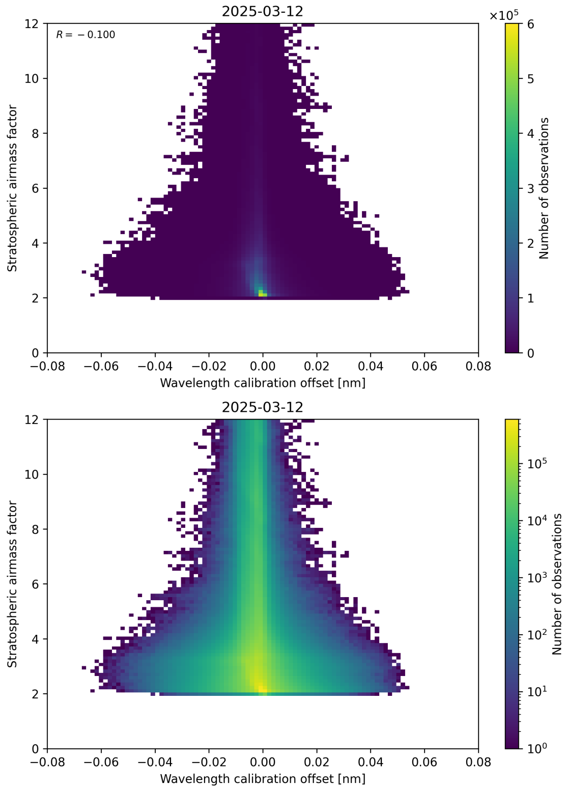
Figure 174: Scatter density plot of “Wavelength calibration offset” against “Stratospheric air mass factor” for 2025-03-12 to 2025-03-13.
