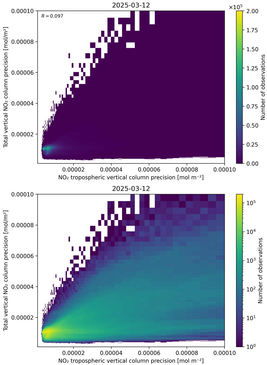
Figure 139: Scatter density plot of “NO 2 tropospheric vertical column precision” against “Total vertical NO 2 column precision” for 2025-03-12 to 2025-03-13.
