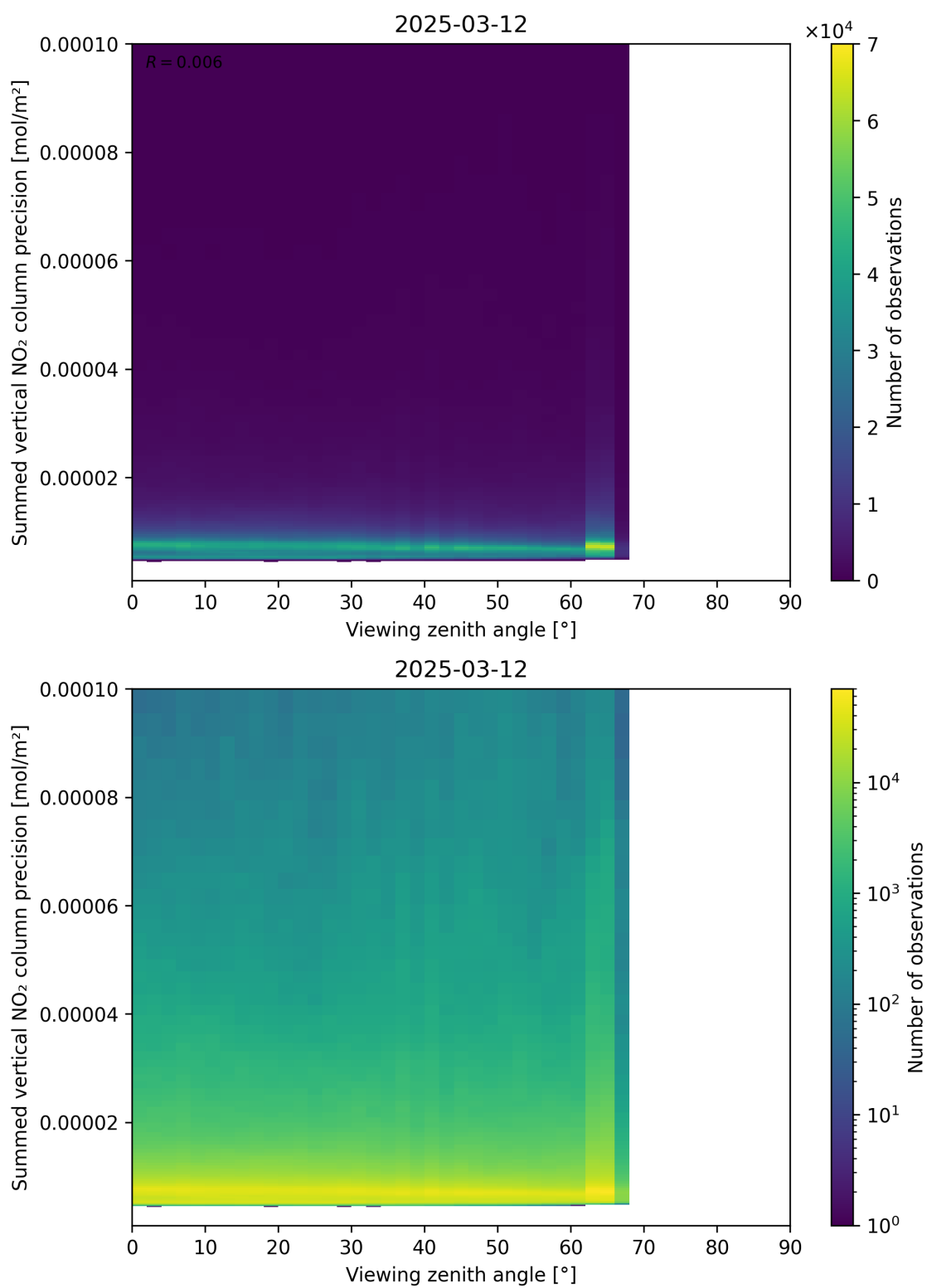
Figure 166: Scatter density plot of “Viewing zenith angle” against “Summed vertical NO 2 column precision” for 2025-03-12 to 2025-03-13.
