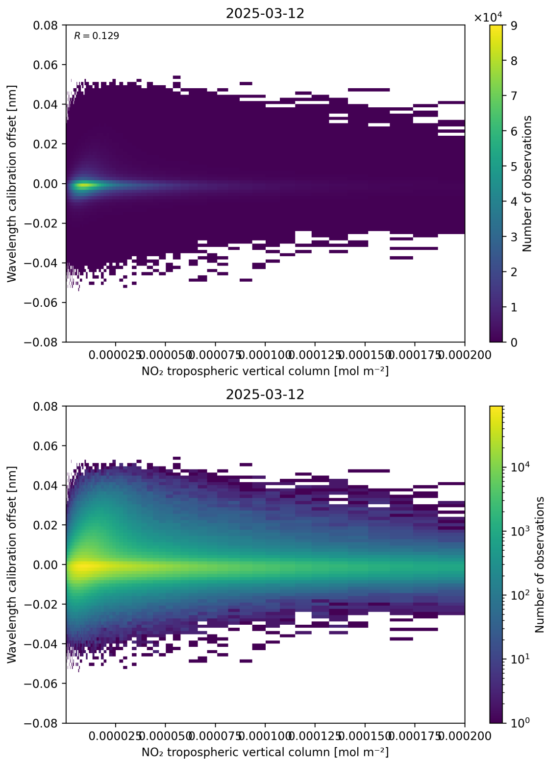
Figure 143: Scatter density plot of “NO 2 tropospheric vertical column” against “Wavelength calibration offset” for 2025-03-12 to 2025-03-13.
