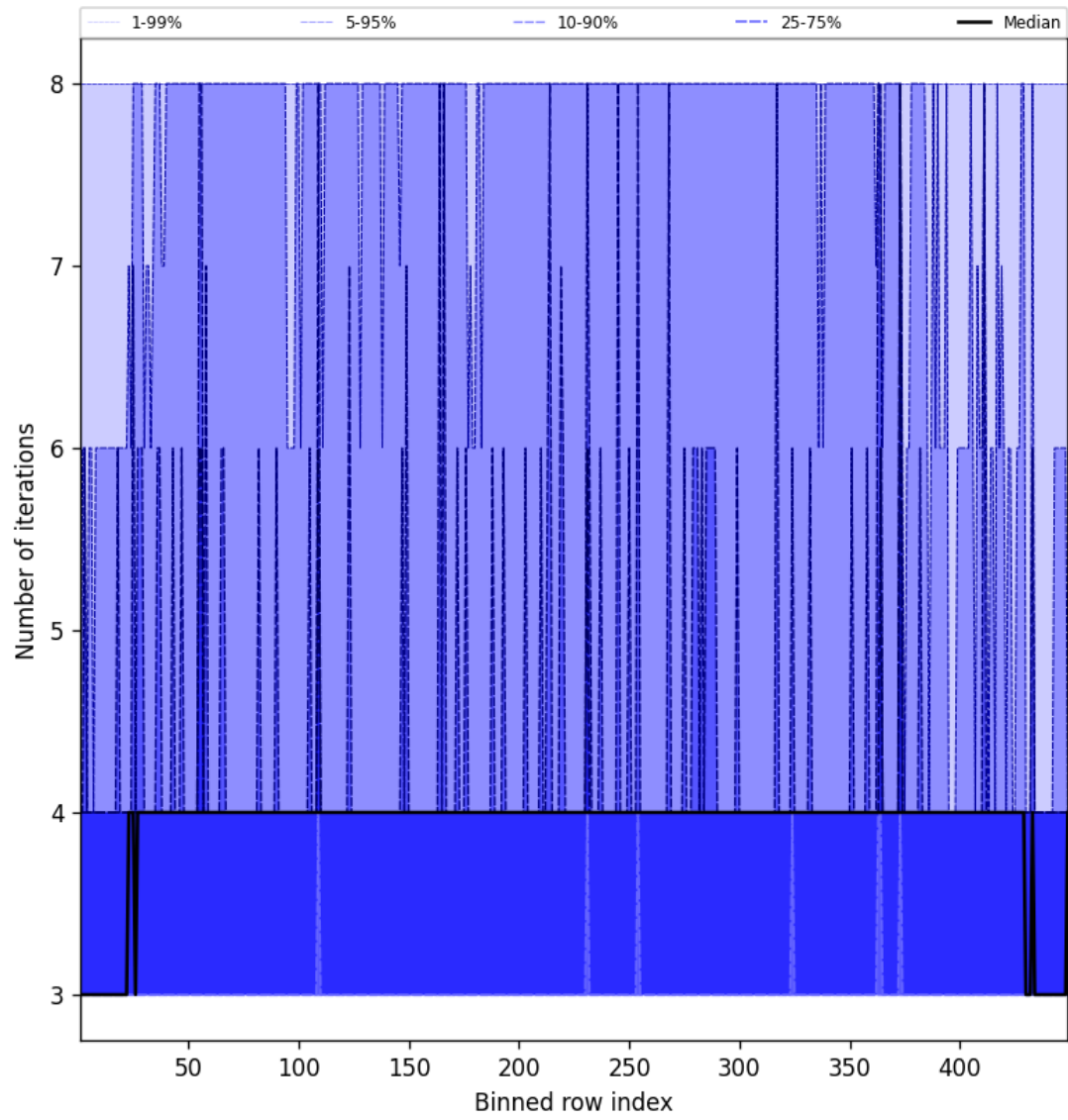
Figure 51: Along track statistics of “Number of iterations” for 2025-03-12 to 2025-03-13
