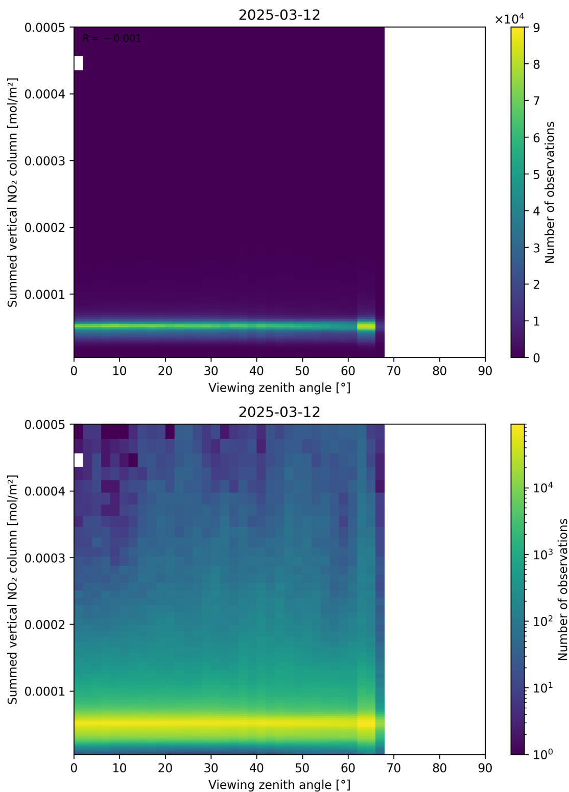
Figure 165: Scatter density plot of “Viewing zenith angle” against “Summed vertical NO 2 column” for 2025-03-12 to 2025-03-13.
