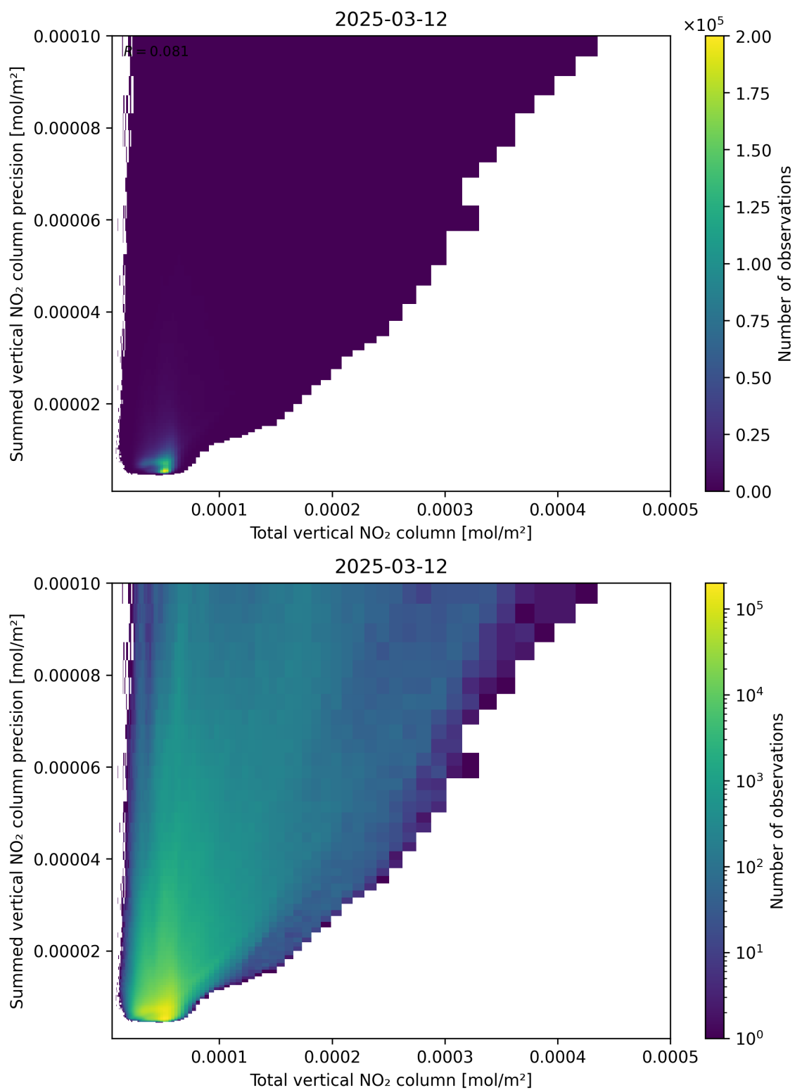
Figure 113: Scatter density plot of “Total vertical NO 2 column” against “Summed vertical NO 2 column precision” for 2025-03-12 to 2025-03-13.
