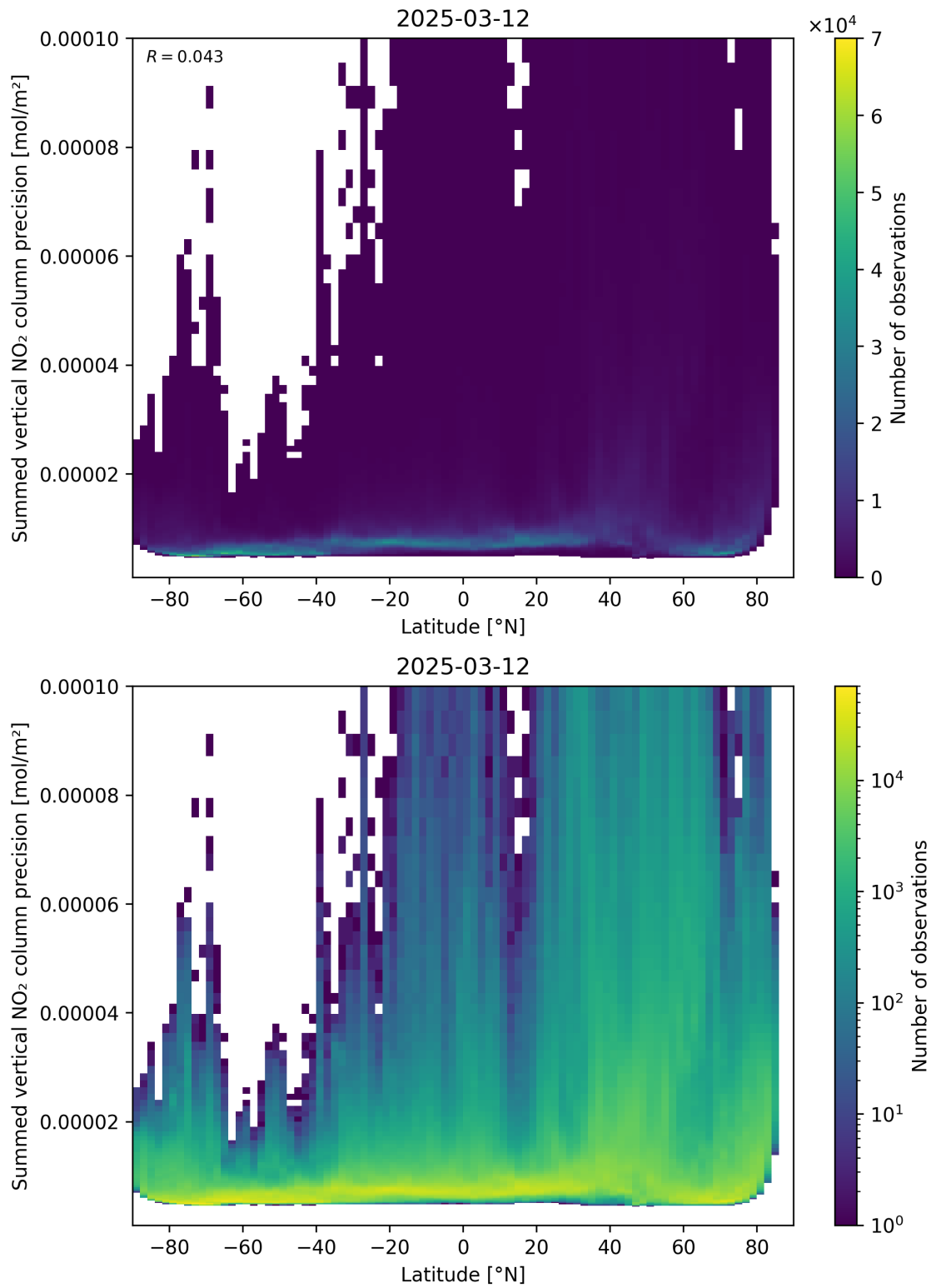
Figure 89: Scatter density plot of “Latitude” against “Summed vertical NO 2 column precision” for 2025-03-12 to 2025-03-13.
