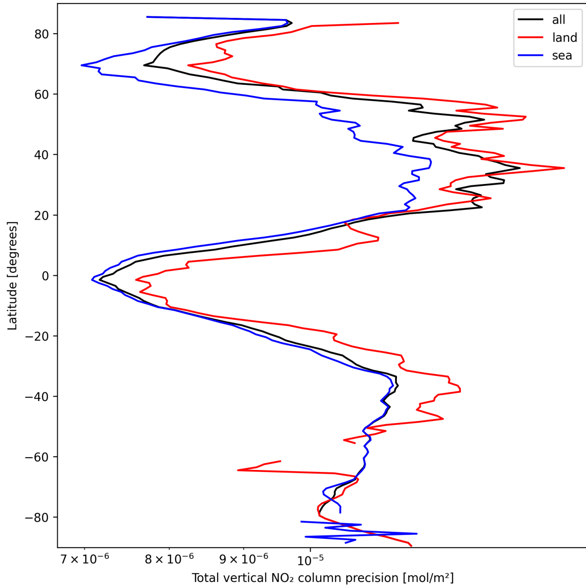
Figure 22: Zonal average of “Total vertical NO 2 column precision” for 2025-03-12 to 2025-03-13.
