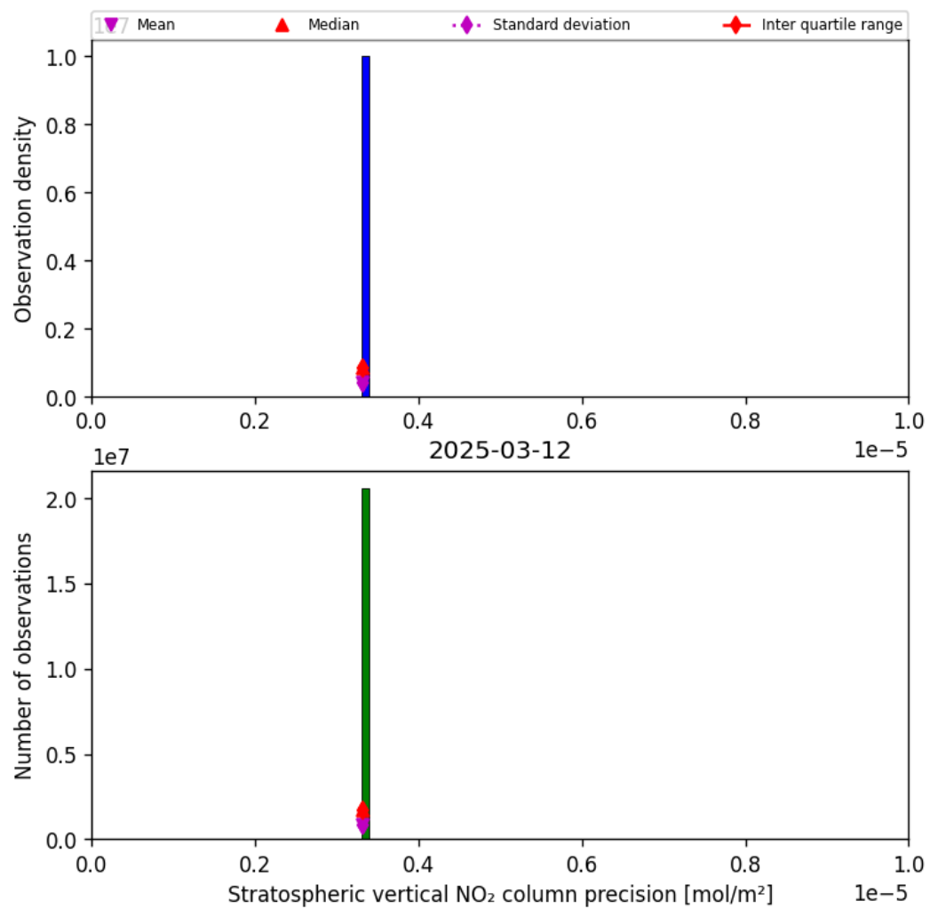
Figure 37: Histogram of “Stratospheric vertical NO 2 column precision” for 2025-03-12 to 2025-03-13
