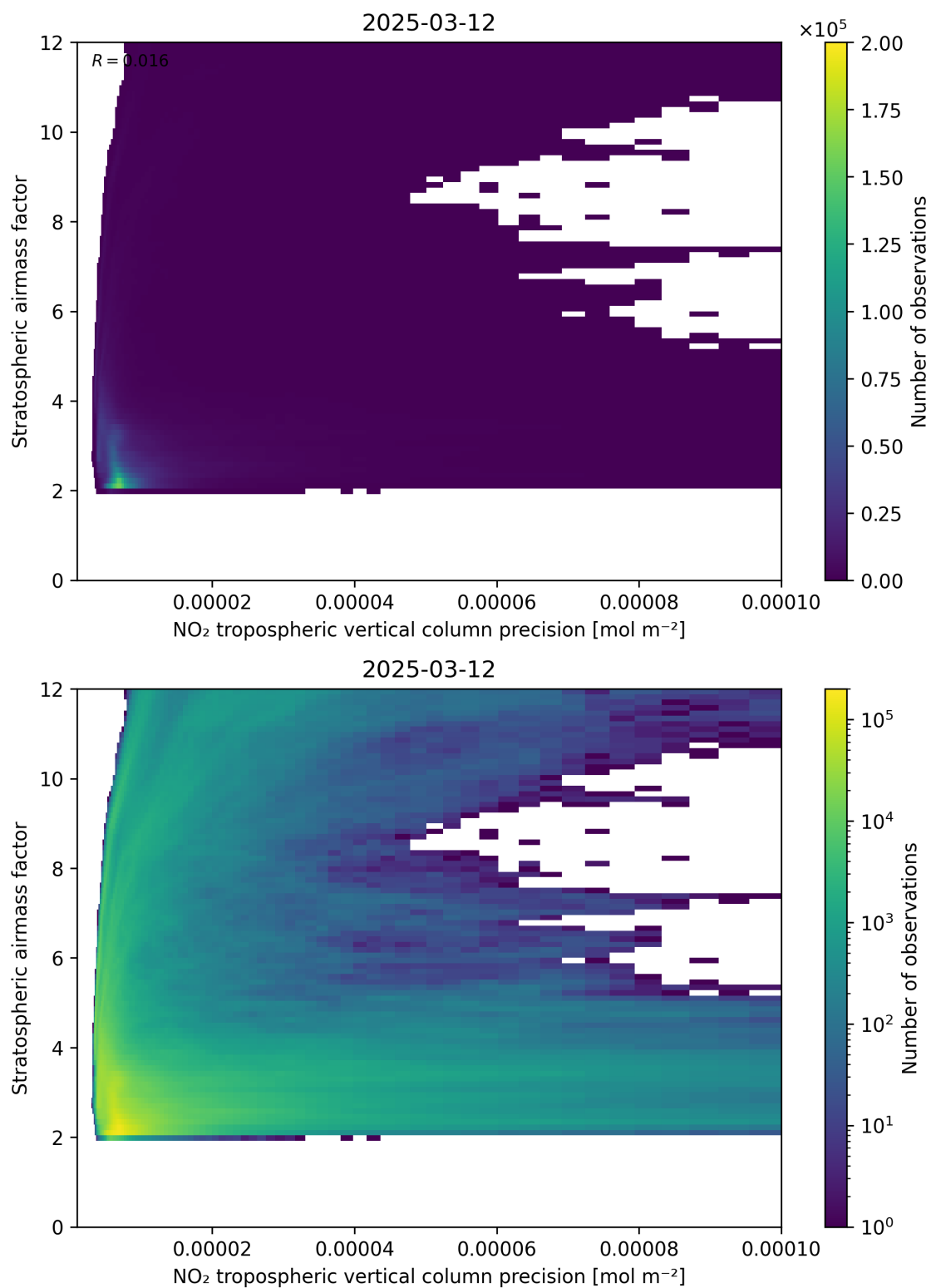
Figure 131: Scatter density plot of “NO 2 tropospheric vertical column precision” against “Stratospheric airmass factor” for 2025-03-12 to 2025-03-13.
