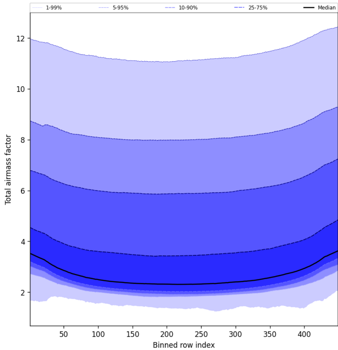
Figure 49: Along track statistics of “Total airmass factor” for 2025-03-12 to 2025-03-13
