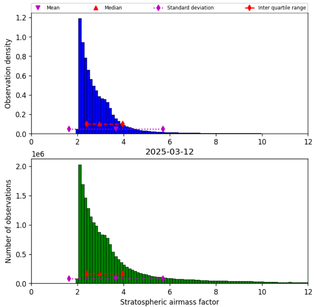
Figure 44: Histogram of “Stratospheric airmass factor” for 2025-03-12 to 2025-03-13
