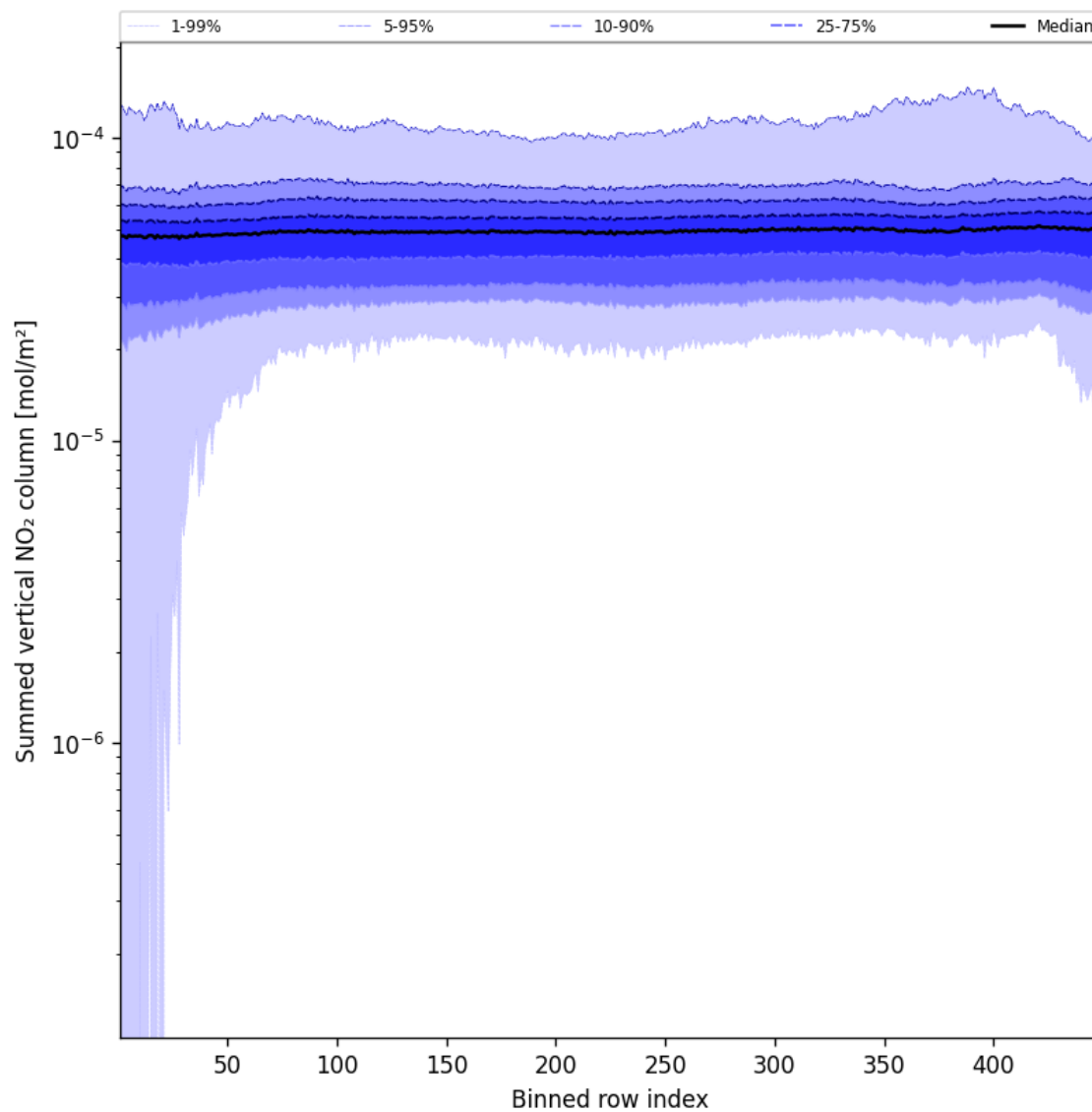
Figure 57: Along track statistics of “Summed vertical NO 2 column” for 2025-03-12 to 2025-03-13
