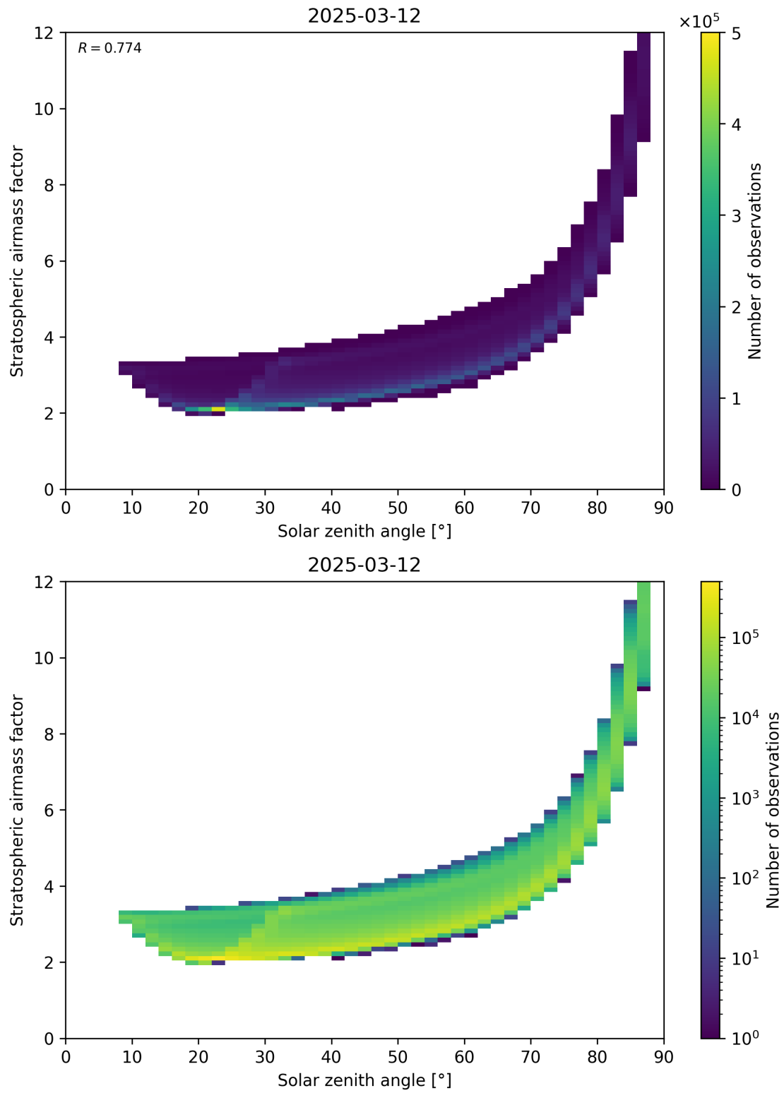
Figure 145: Scatter density plot of “Solar zenith angle” against “Stratospheric airmass factor” for 2025-03-12 to 2025-03-13.
