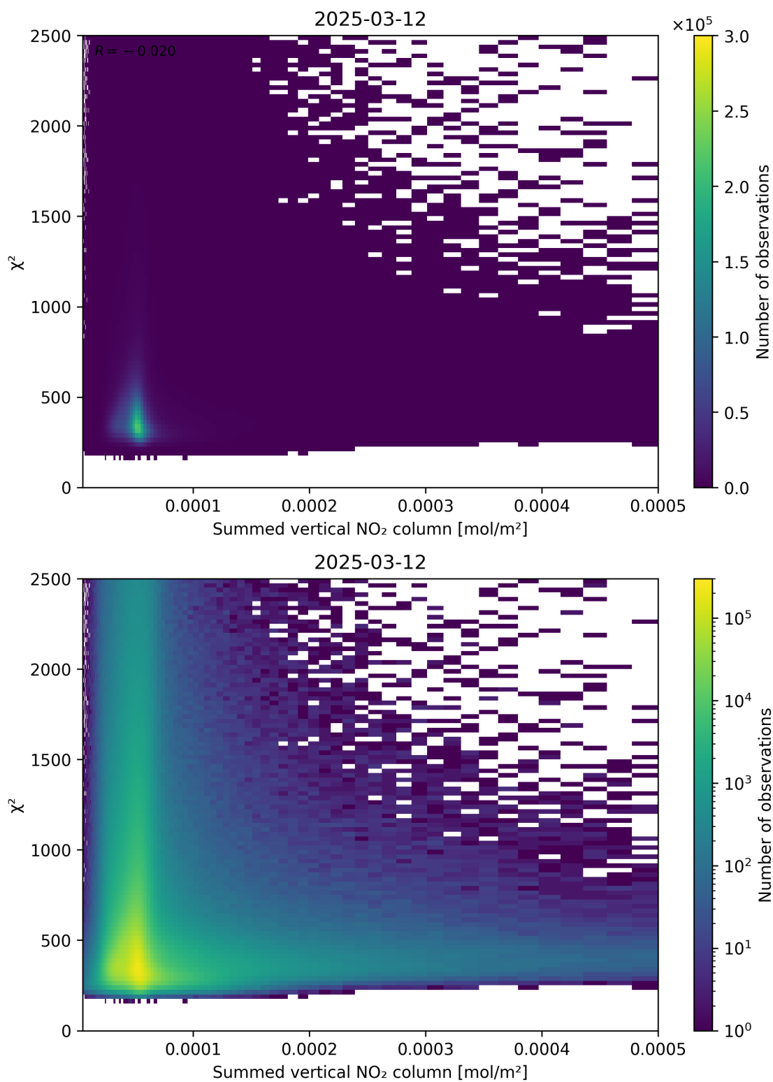
Figure 104: Scatter density plot of “Summed vertical NO 2 column” against “ \chi^2 ” for 2025-03-12 to 2025-03-13.
