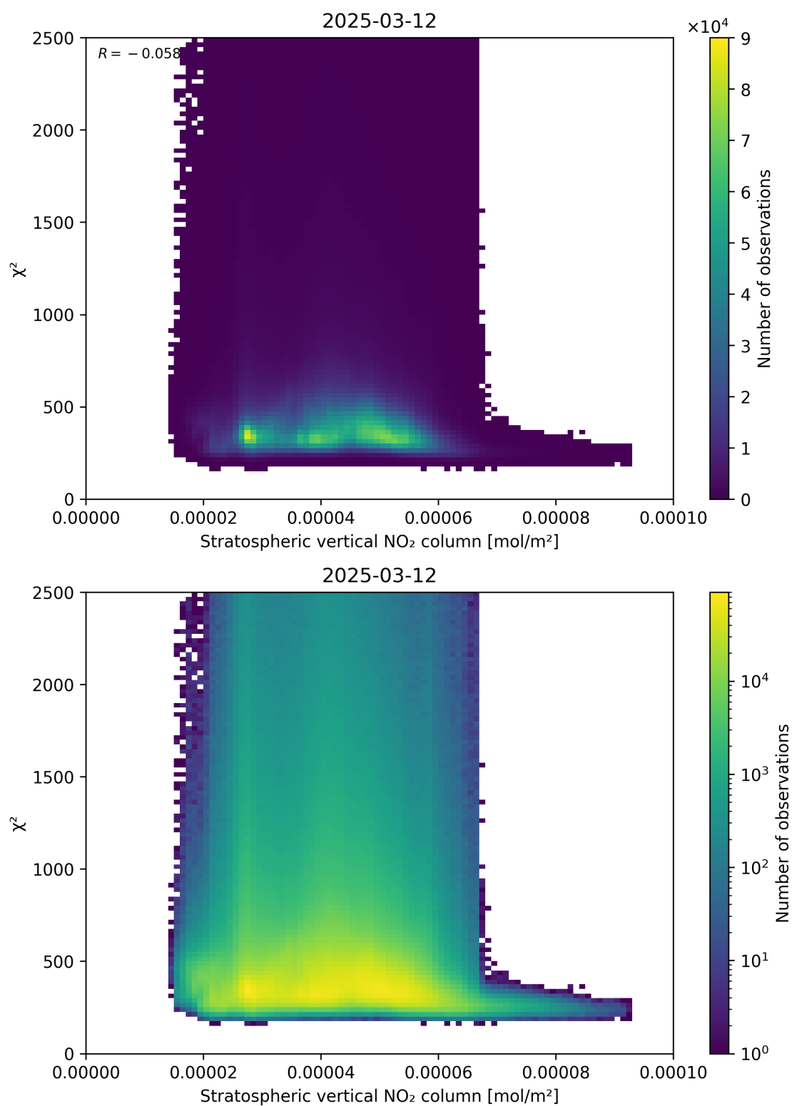
Figure 97: Scatter density plot of “Stratospheric vertical NO 2 column” against “ \chi^2 ” for 2025-03-12 to 2025-03-13.
