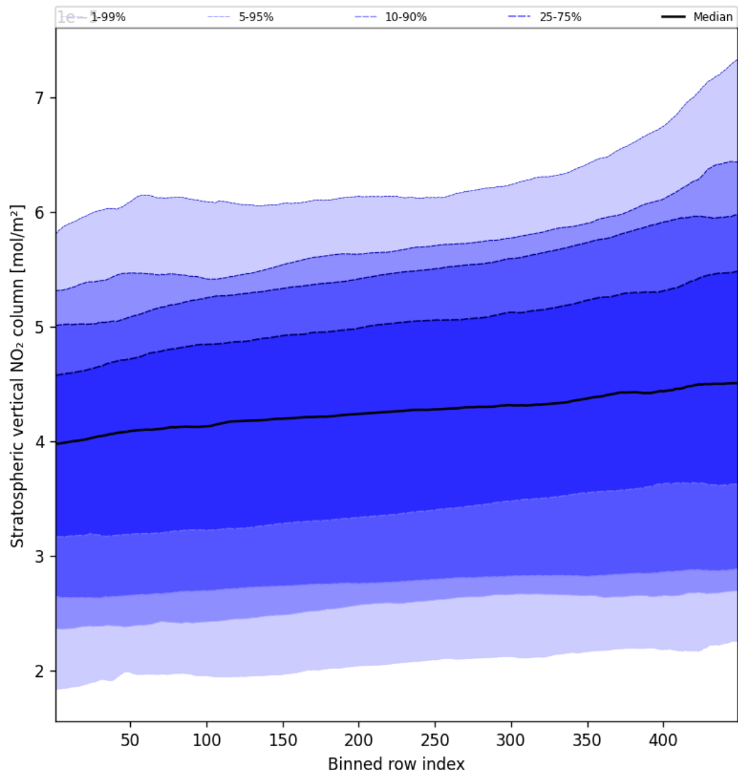
Figure 53: Along track statistics of “Stratospheric vertical NO 2 column” for 2025-03-12 to 2025-03-13
