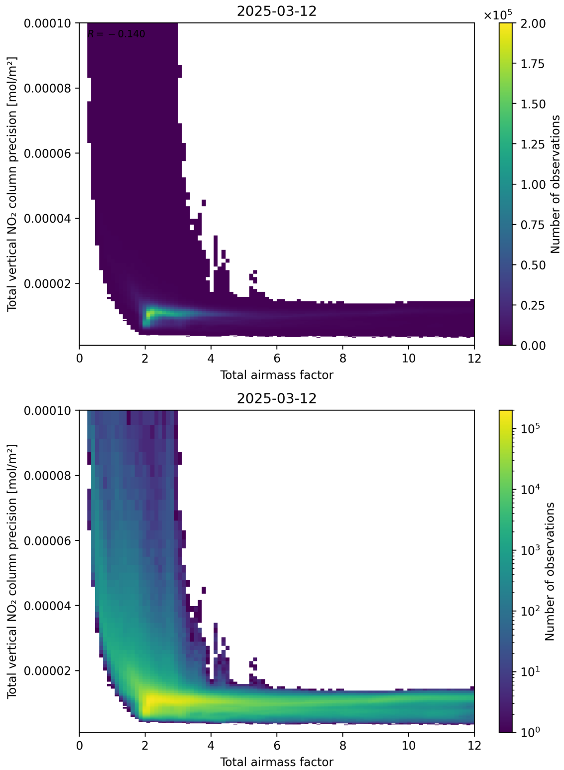
Figure 68: Scatter density plot of “Total airmass factor” against “Total vertical NO 2 column precision” for 2025-03-12 to 2025-03-13.
