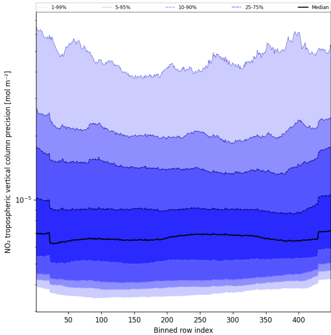
Figure 47: Along track statistics of “NO 2 tropospheric vertical column precision” for 2025-03-12 to 2025-03-13
