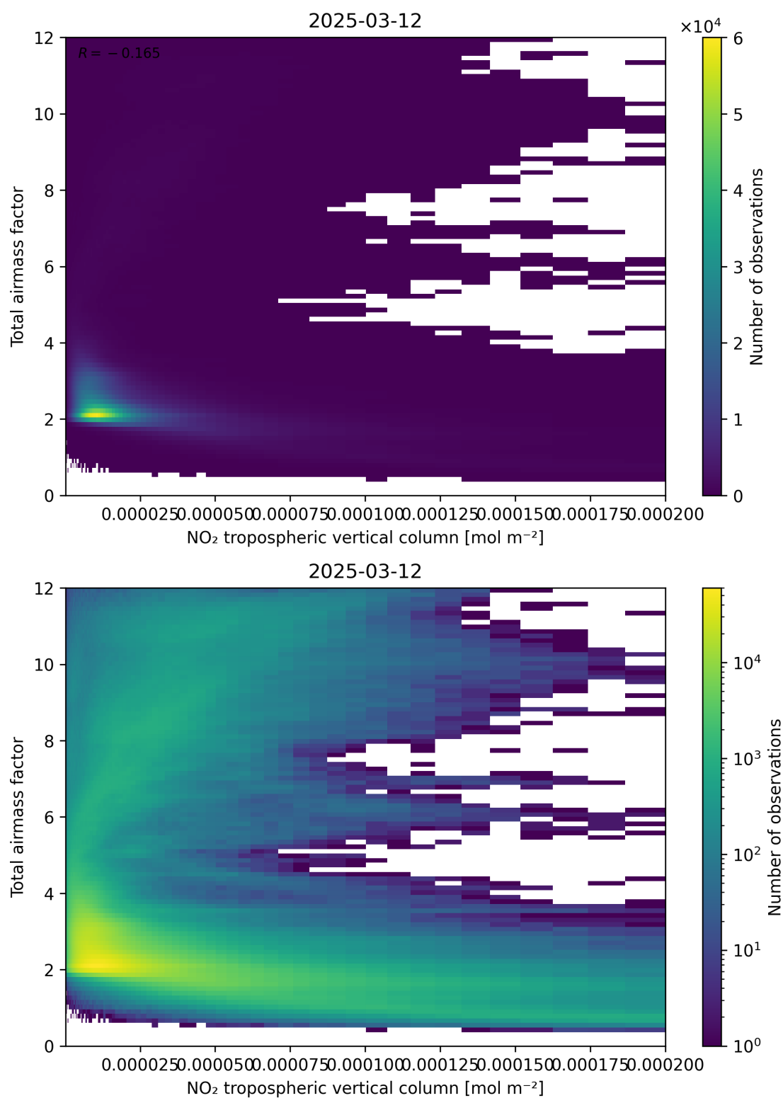
Figure 122: Scatter density plot of “NO 2 tropospheric vertical column” against “Total air mass factor” for 2025-03-12 to 2025-03-13.
