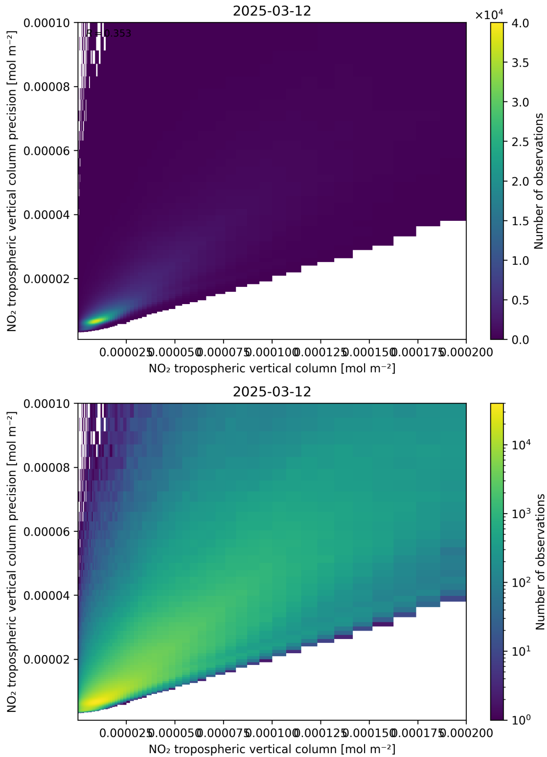
Figure 130: Scatter density plot of “NO 2 tropospheric vertical column” against “NO 2 tropospheric vertical column precision” for 2025-03-12 to 2025-03-13.
