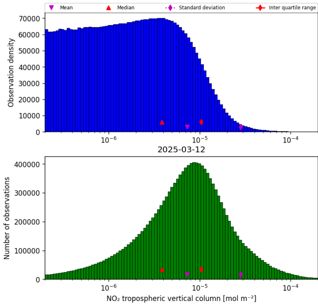
Figure 29: Histogram of “NO 2 tropospheric vertical column” for 2025-03-12 to 2025-03-13
