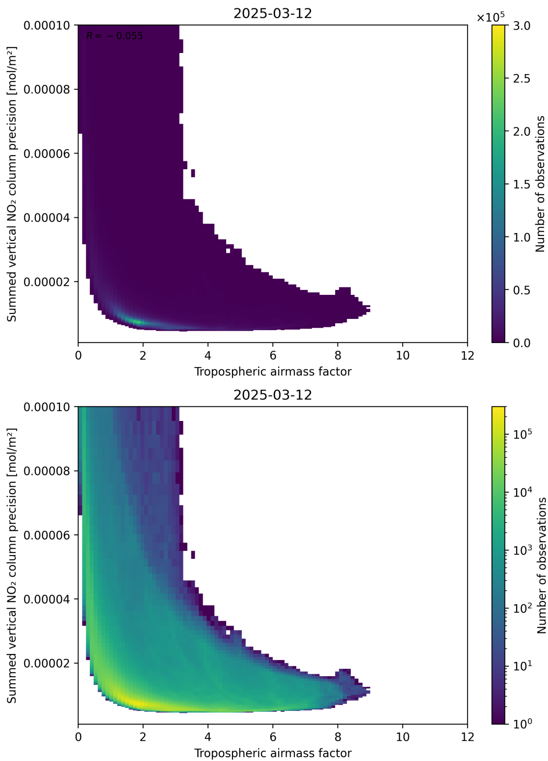
Figure 76: Scatter density plot of “Tropospheric air mass factor” against “Summed vertical NO 2 column precision” for 2025-03-12 to 2025-03-13.
