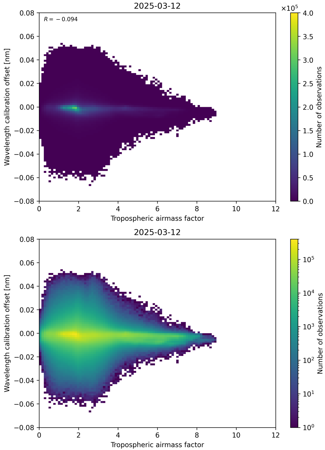
Figure 80: Scatter density plot of “Tropospheric airmass factor” against “Wavelength calibration offset” for 2025-03-12 to 2025-03-13.
