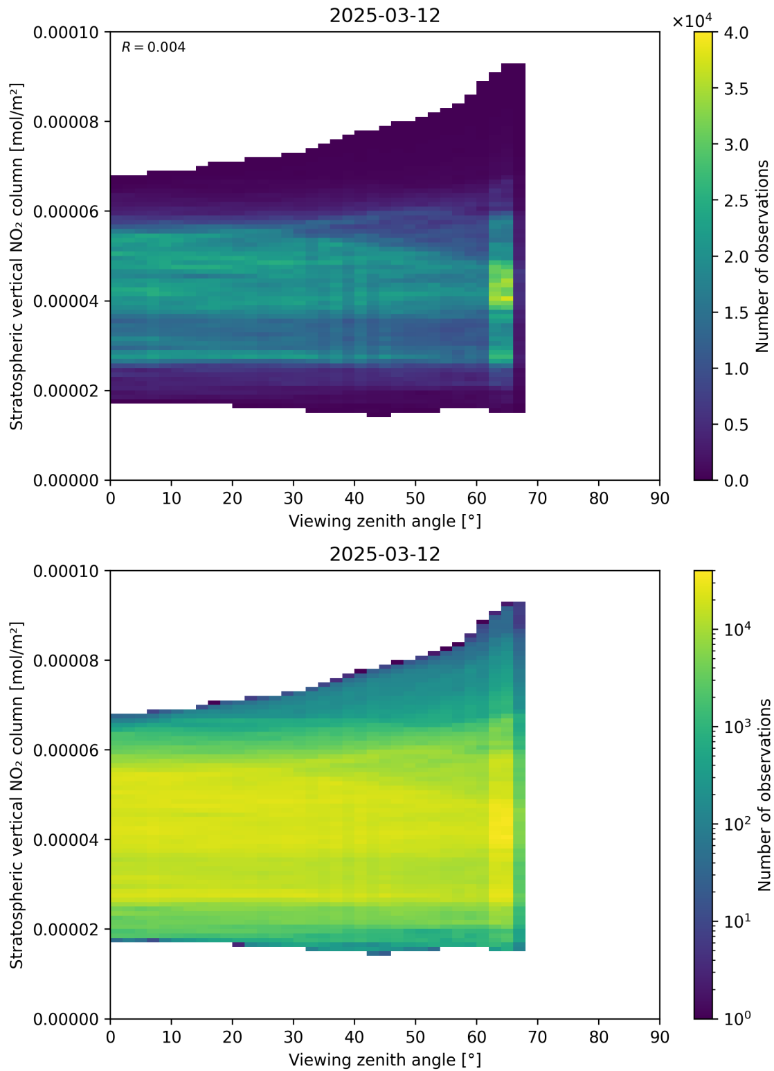
Figure 164: Scatter density plot of “Viewing zenith angle” against “Stratospheric vertical \text{NO}_2 column” for 2025-03-12 to 2025-03-13.
