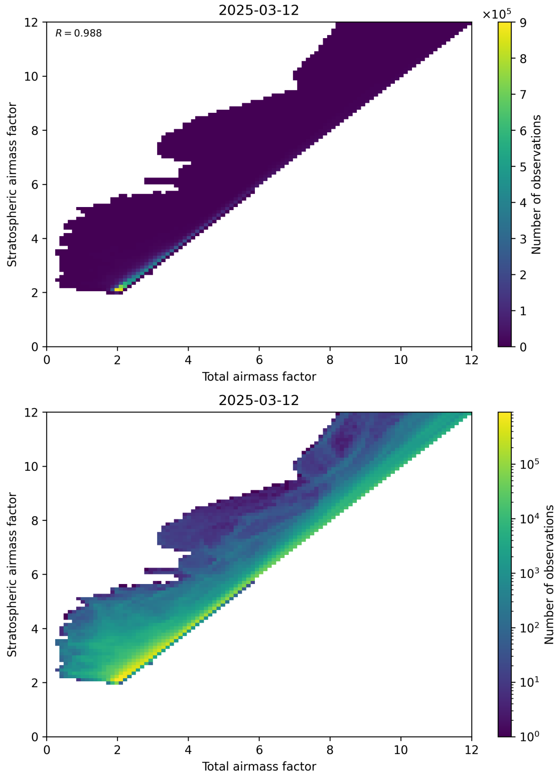
Figure 62: Scatter density plot of “Total airmass factor” against “Stratospheric airmass factor” for 2025-03-12 to 2025-03-13.
