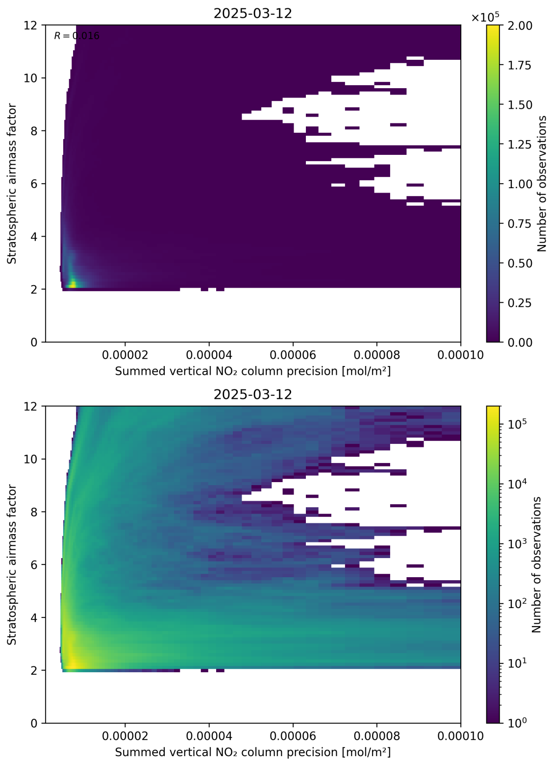
Figure 106: Scatter density plot of “Summed vertical NO 2 column precision” against “Stratospheric airmass factor” for 2025-03-12 to 2025-03-13.
