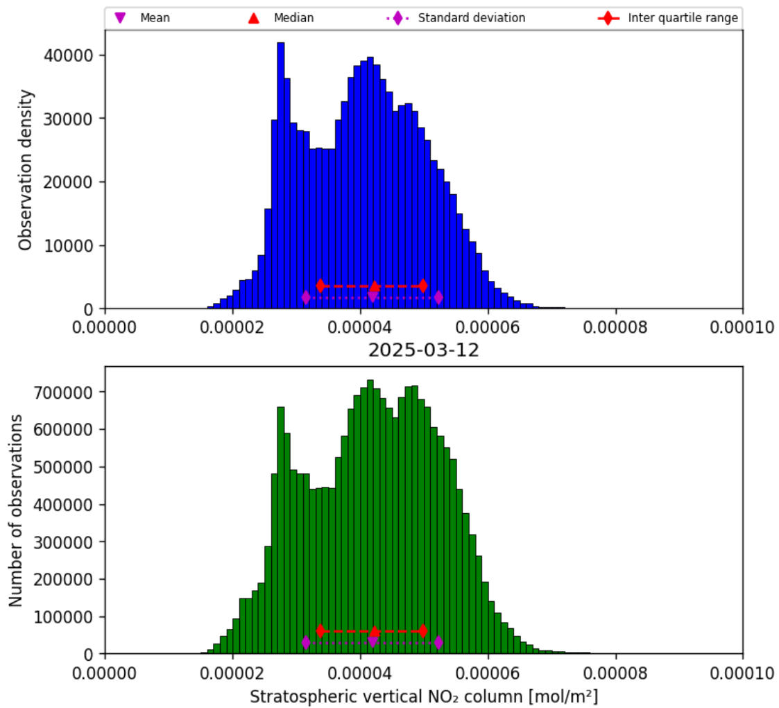
Figure 36: Histogram of “Stratospheric vertical NO 2 column” for 2025-03-12 to 2025-03-13
