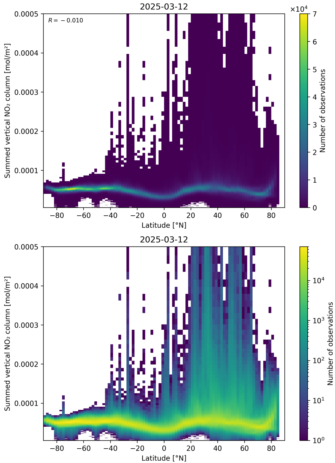
Figure 88: Scatter density plot of “Latitude” against “Summed vertical NO 2 column” for 2025-03-12 to 2025-03-13.
