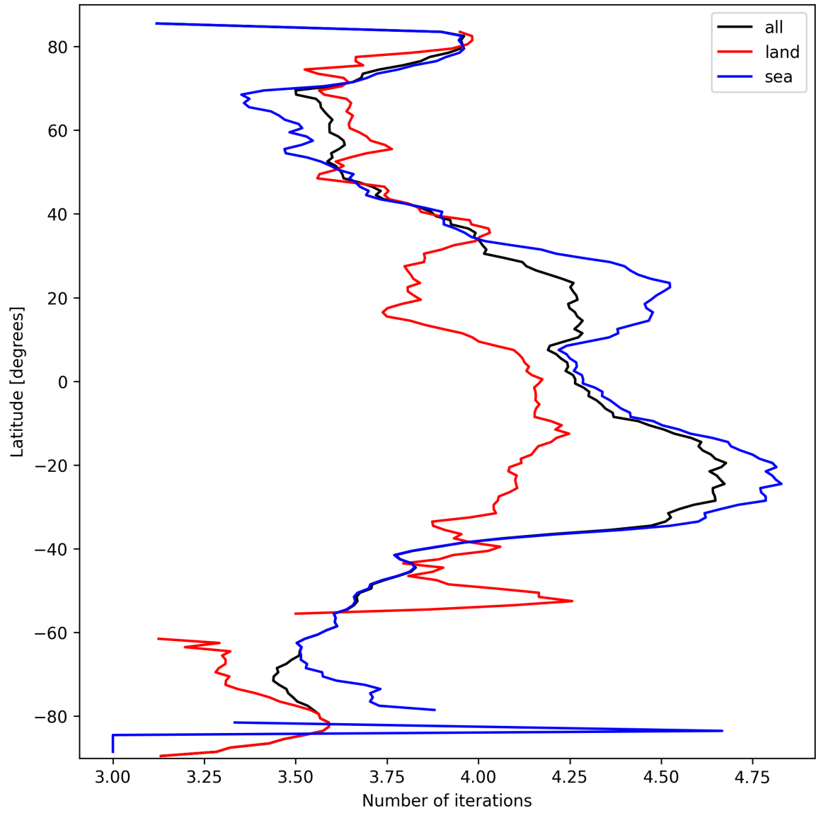
Figure 17: Zonal average of “Number of iterations” for 2025-03-12 to 2025-03-13.
