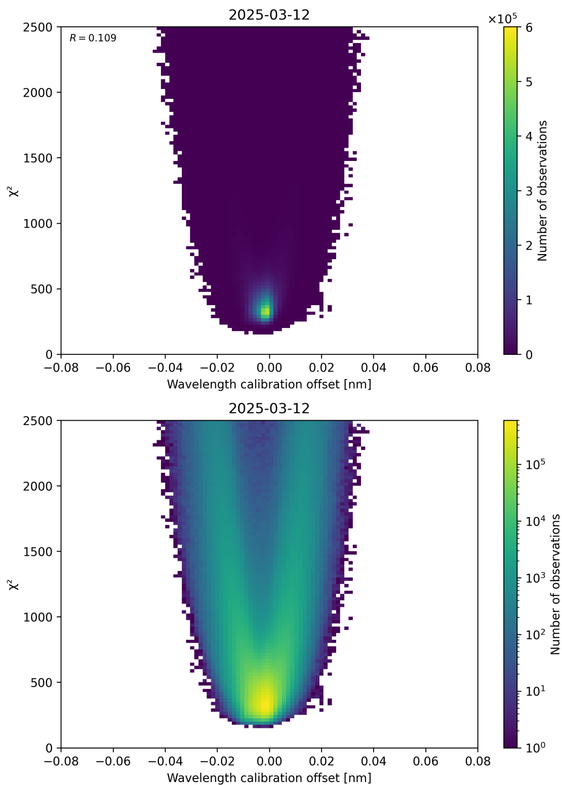
Figure 175: Scatter density plot of “Wavelength calibration offset” against “ \chi^2 ” for 2025-03-12 to 2025-03-13.
