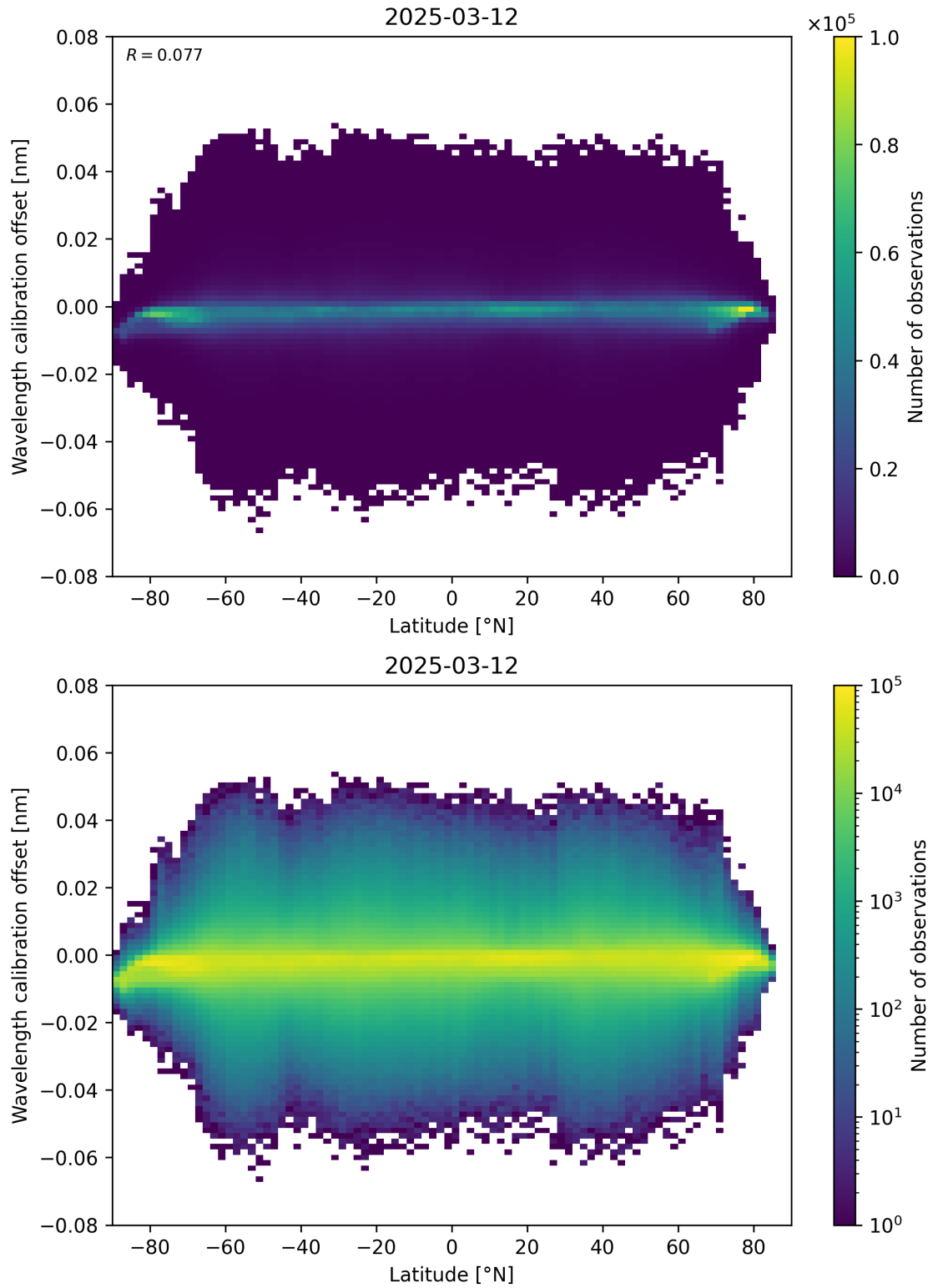
Figure 95: Scatter density plot of “Latitude” against “Wavelength calibration offset” for 2025-03-12 to 2025-03-13.
