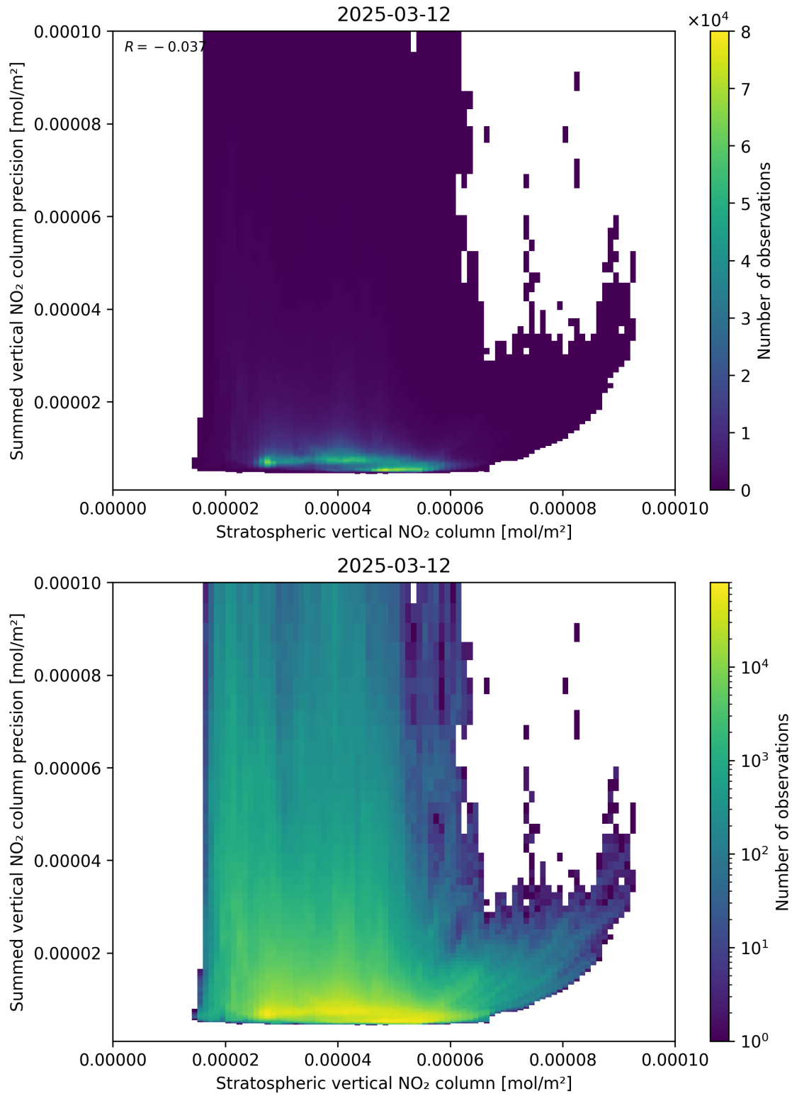
Figure 99: Scatter density plot of “Stratospheric vertical NO 2 column” against “Summed vertical NO 2 column precision” for 2025-03-12 to 2025-03-13.
