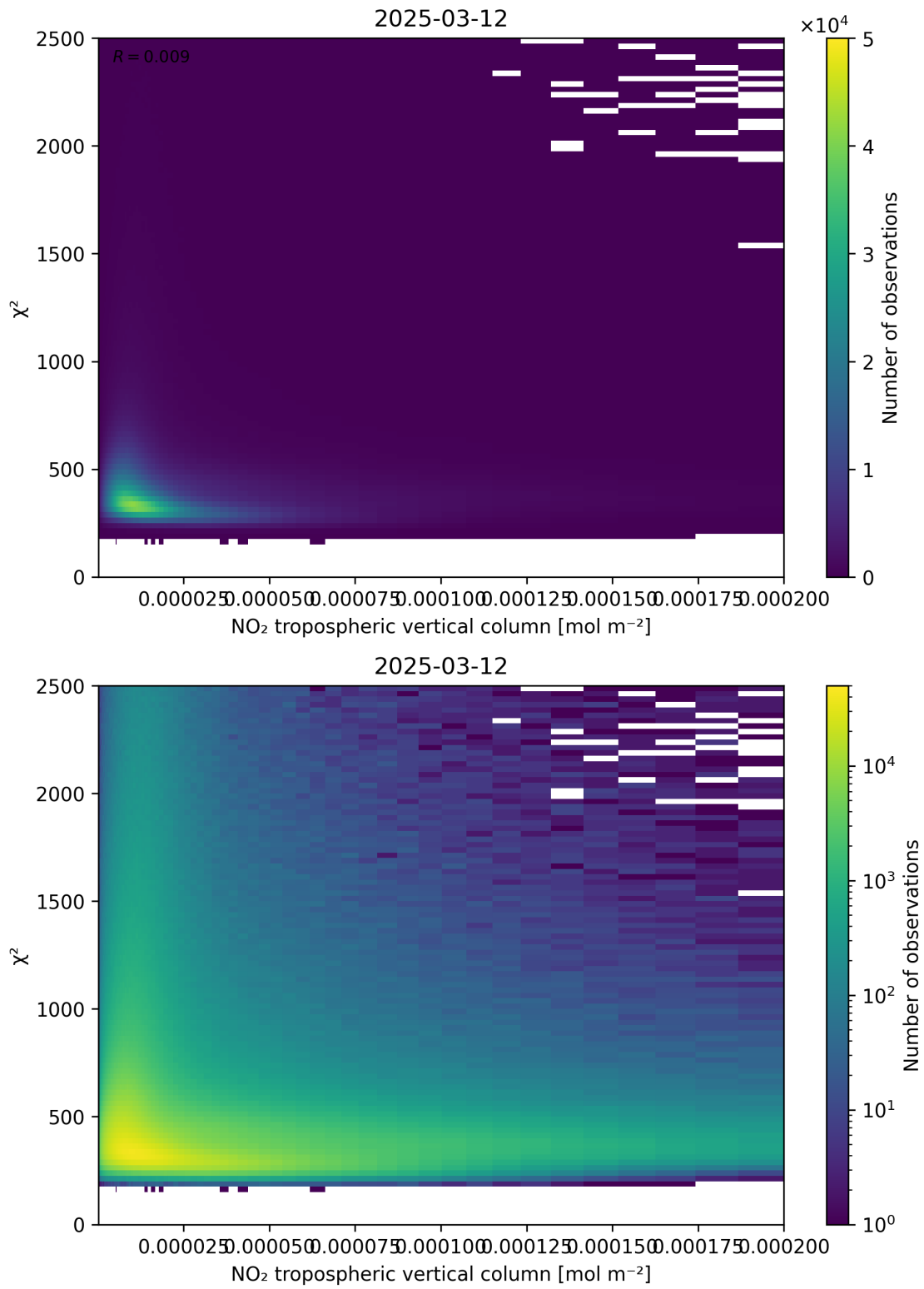
Figure 124: Scatter density plot of “NO 2 tropospheric vertical column” against “ \chi^2 ” for 2025-03-12 to 2025-03-13.
