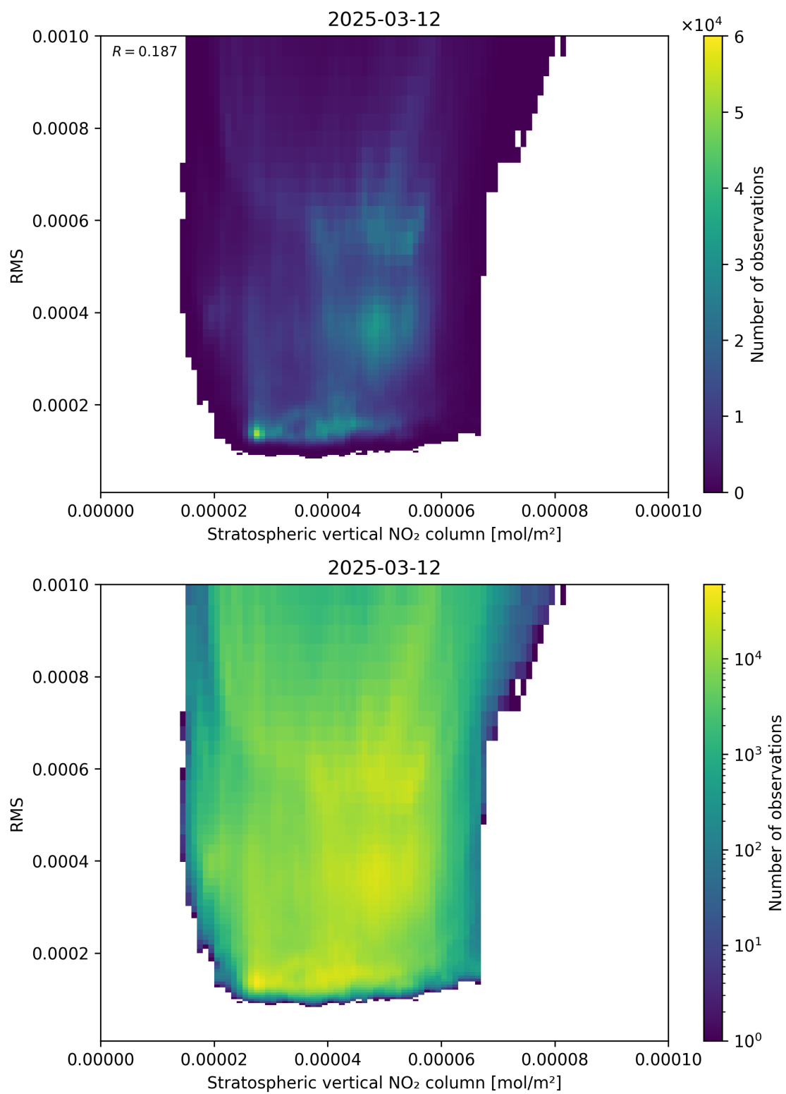
Figure 102: Scatter density plot of “Stratospheric vertical NO 2 column” against “RMS” for 2025-03-12 to 2025-03-13.
