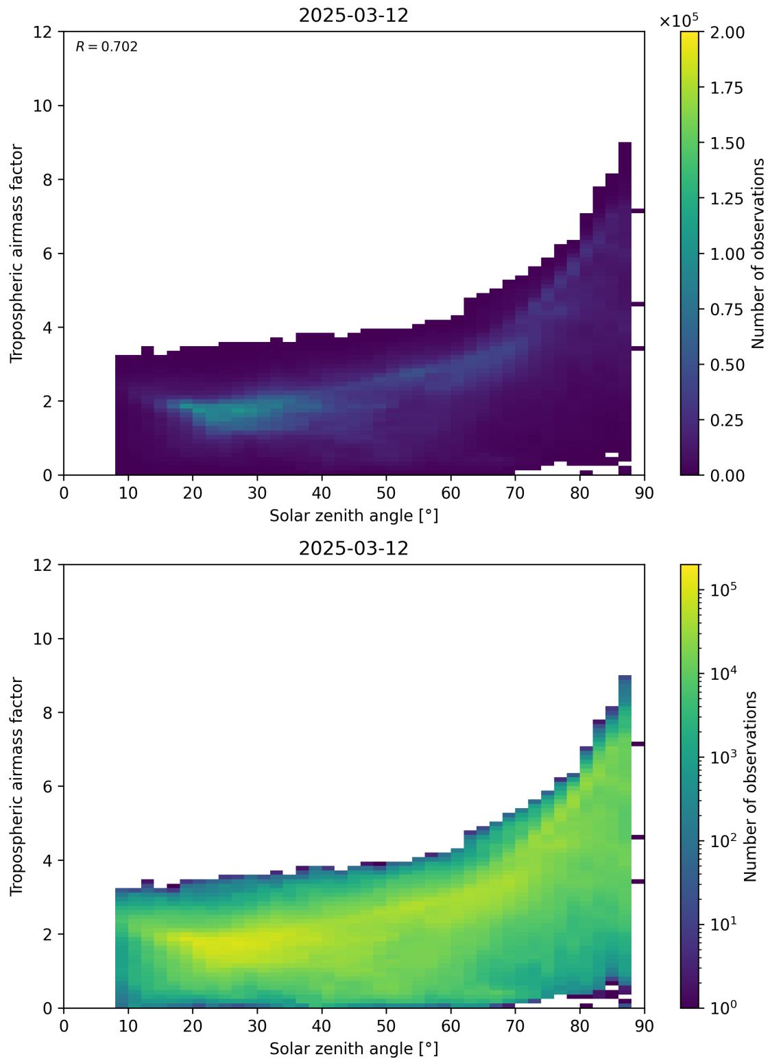
Figure 147: Scatter density plot of “Solar zenith angle” against “Tropospheric airmass factor” for 2025-03-12 to 2025-03-13.
