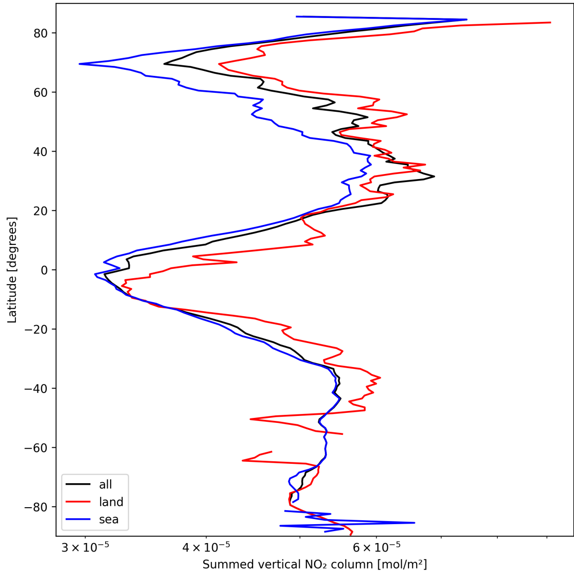
Figure 23: Zonal average of “Summed vertical NO 2 column” for 2025-03-12 to 2025-03-13.
