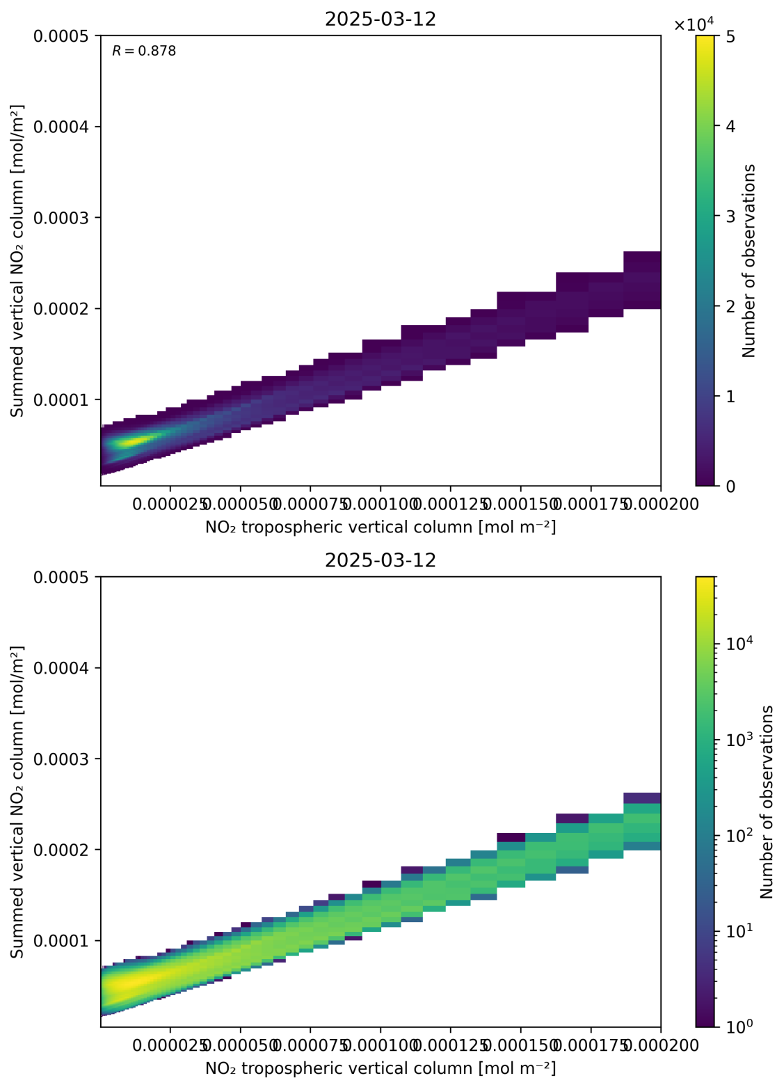
Figure 126: Scatter density plot of “NO 2 tropospheric vertical column” against “Summed vertical NO 2 column” for 2025-03-12 to 2025-03-13.
