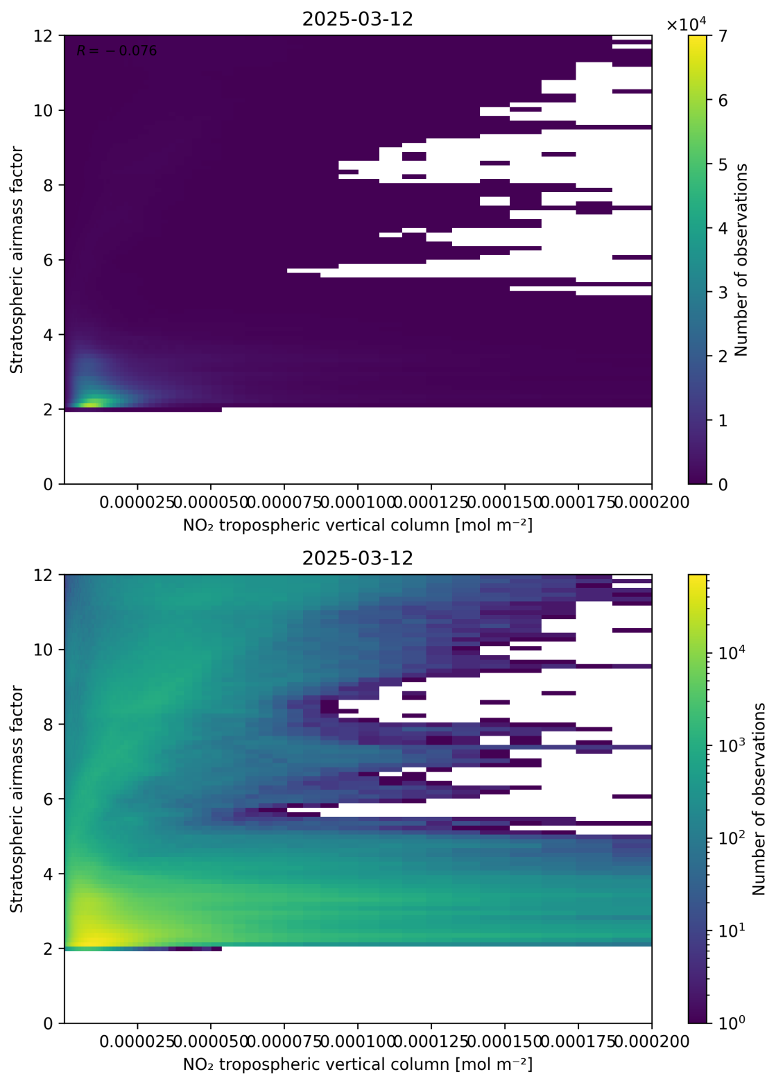
Figure 121: Scatter density plot of “NO 2 tropospheric vertical column” against “Stratospheric air mass factor” for 2025-03-12 to 2025-03-13.
