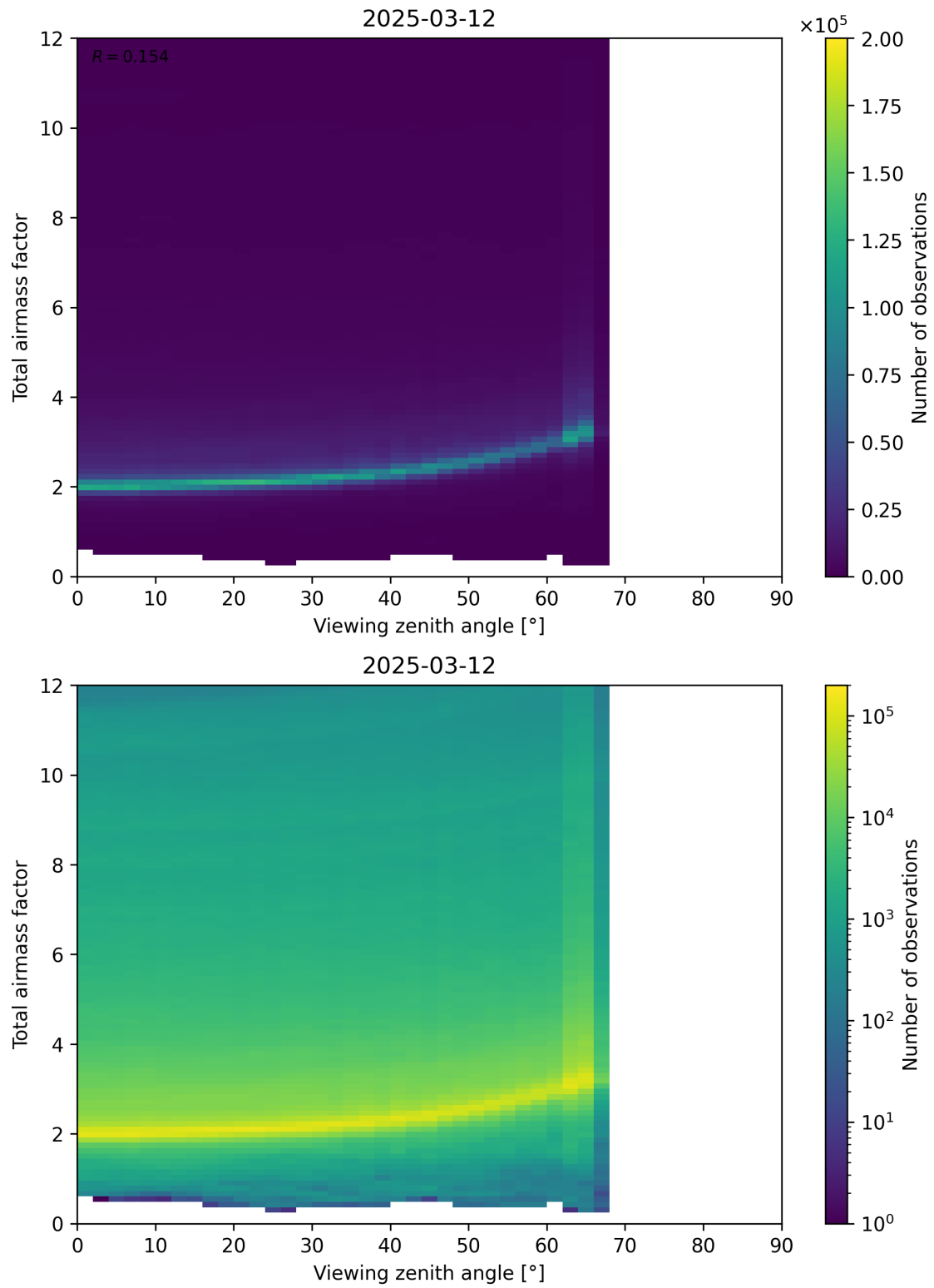
Figure 160: Scatter density plot of “Viewing zenith angle” against “Total airmass factor” for 2025-03-12 to 2025-03-13.
