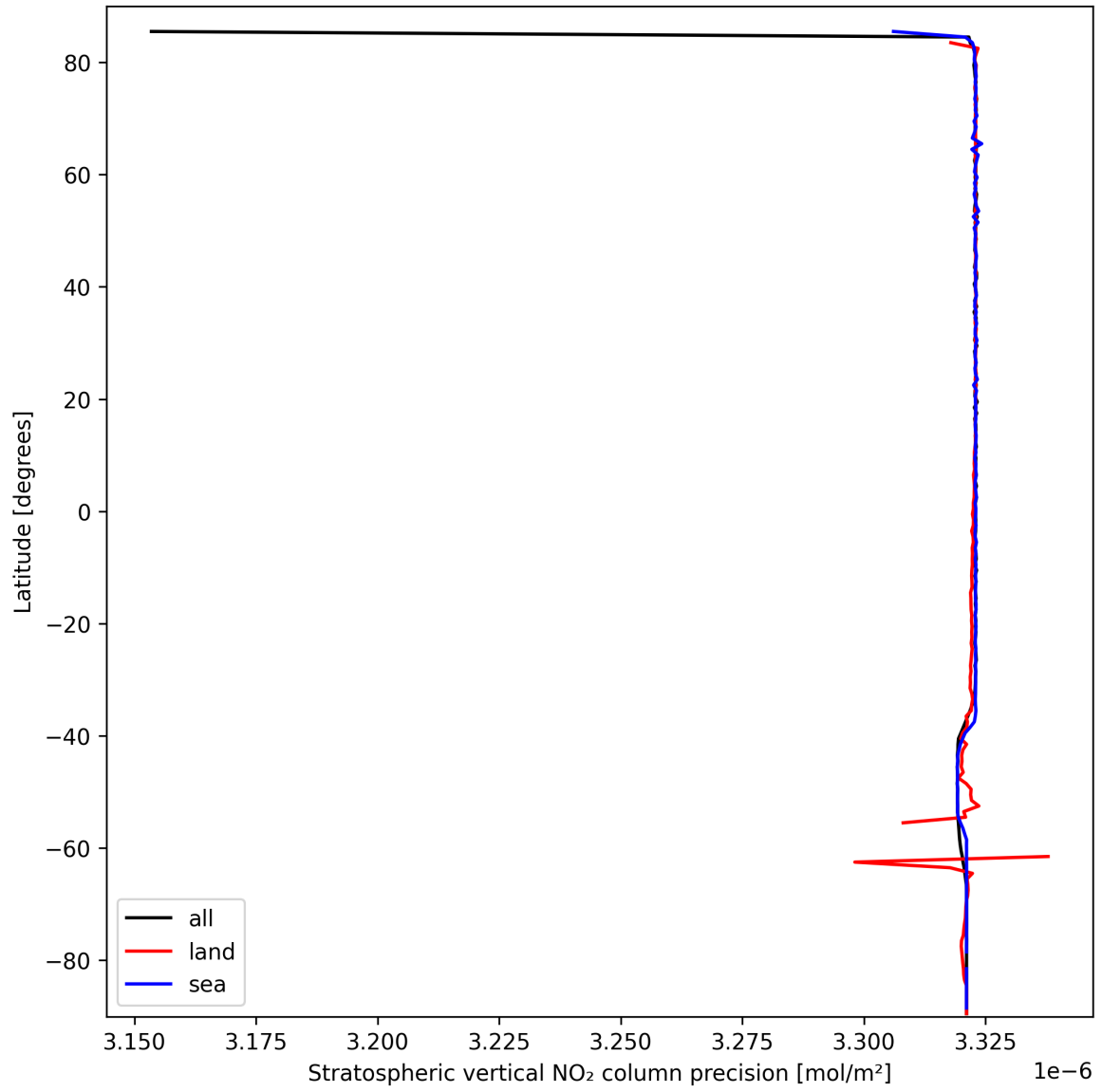
Figure 20: Zonal average of “Stratospheric vertical NO 2 column precision” for 2025-03-12 to 2025-03-13.
