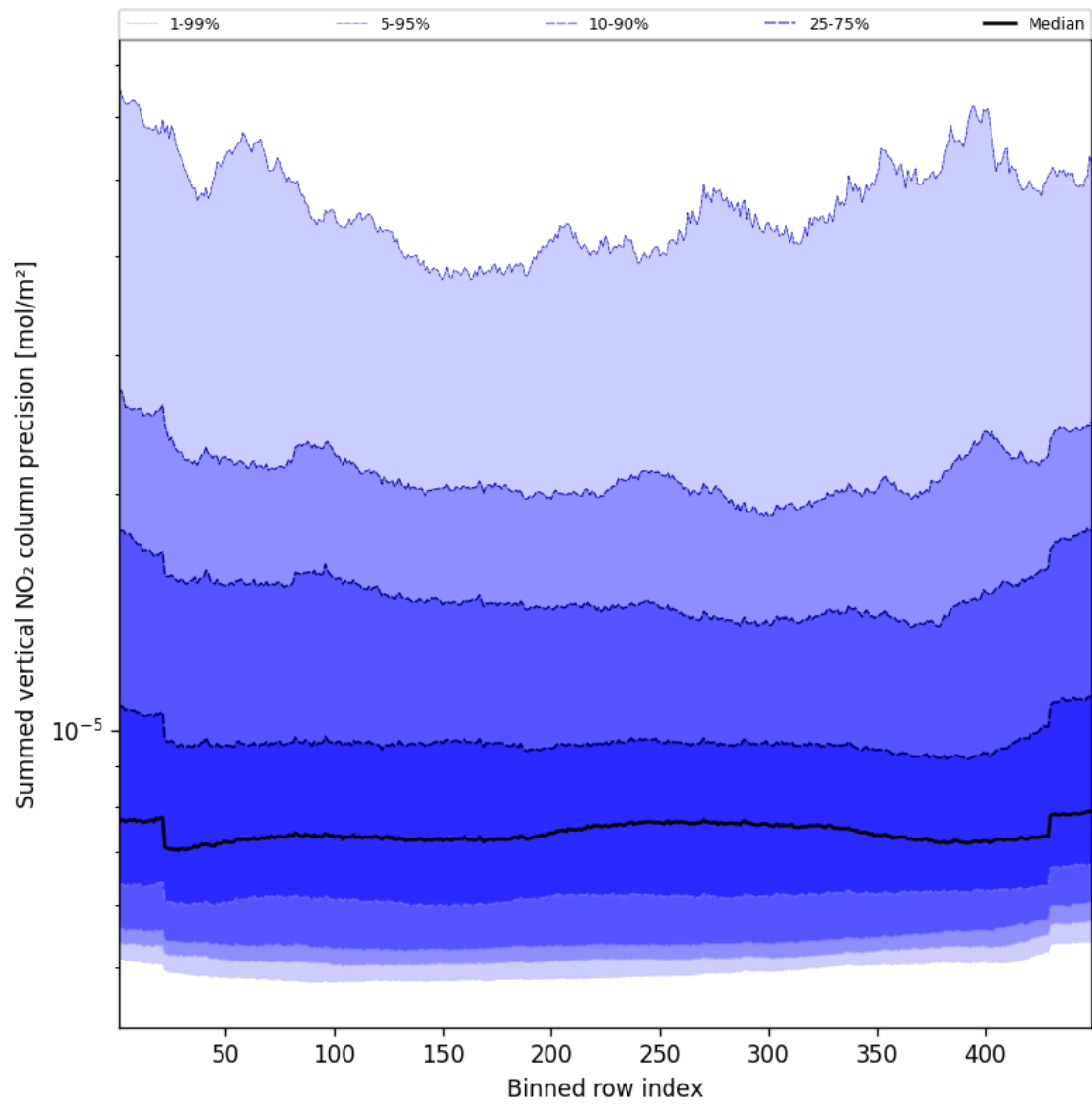
Figure 58: Along track statistics of “Summed vertical NO 2 column precision” for 2025-03-12 to 2025-03-13
