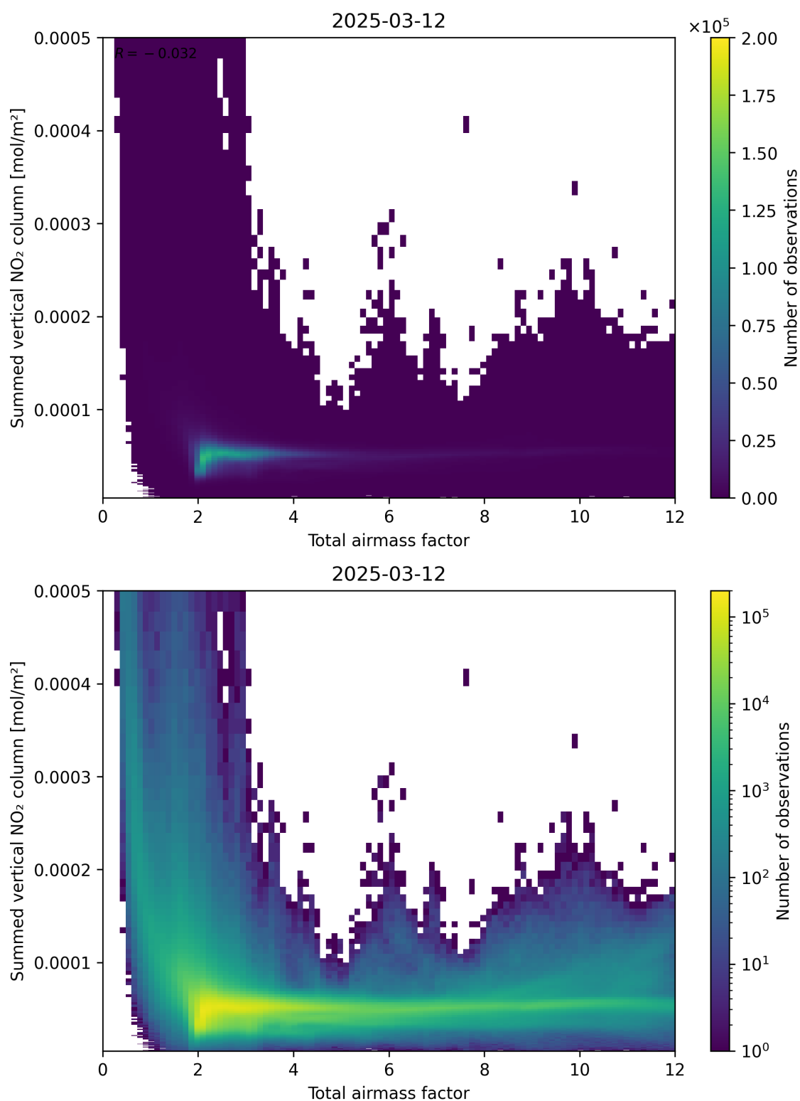
Figure 65: Scatter density plot of “Total airmass factor” against “Summed vertical NO 2 column” for 2025-03-12 to 2025-03-13.
