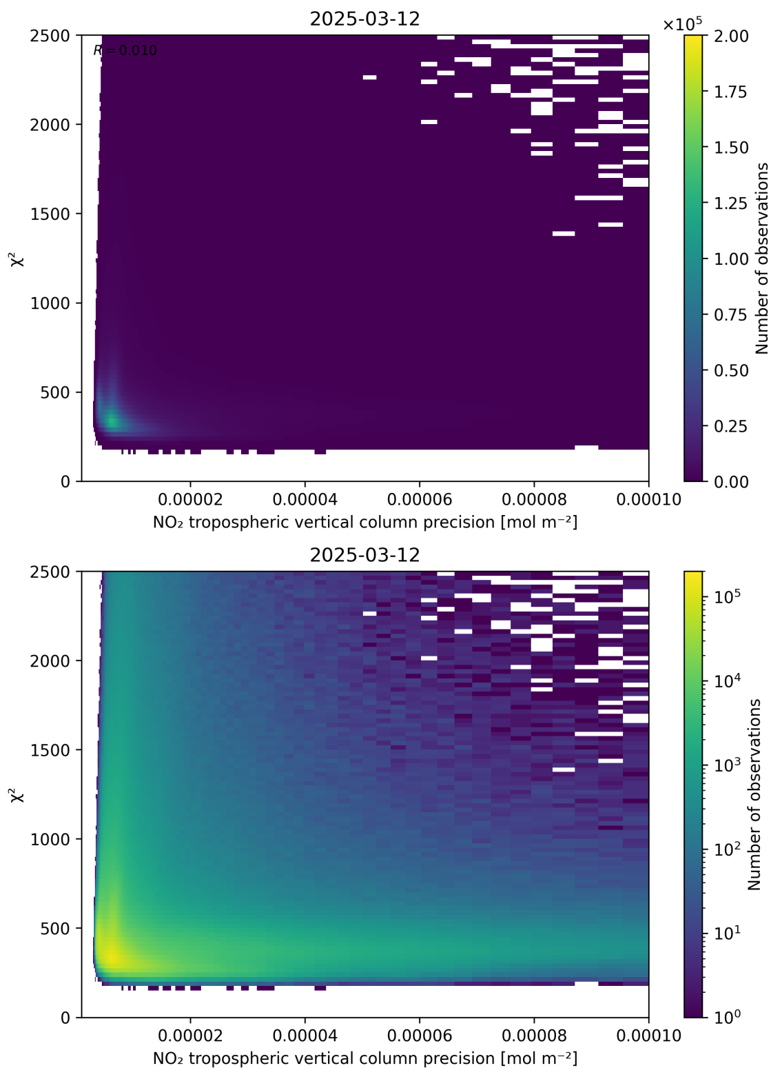
Figure 134: Scatter density plot of “NO 2 tropospheric vertical column precision” against “ \chi^2 ” for 2025-03-12 to 2025-03-13.
