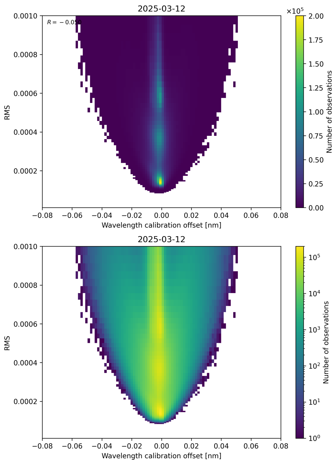
Figure 181: Scatter density plot of “Wavelength calibration offset” against “RMS” for 2025-03-12 to 2025-03-13.
