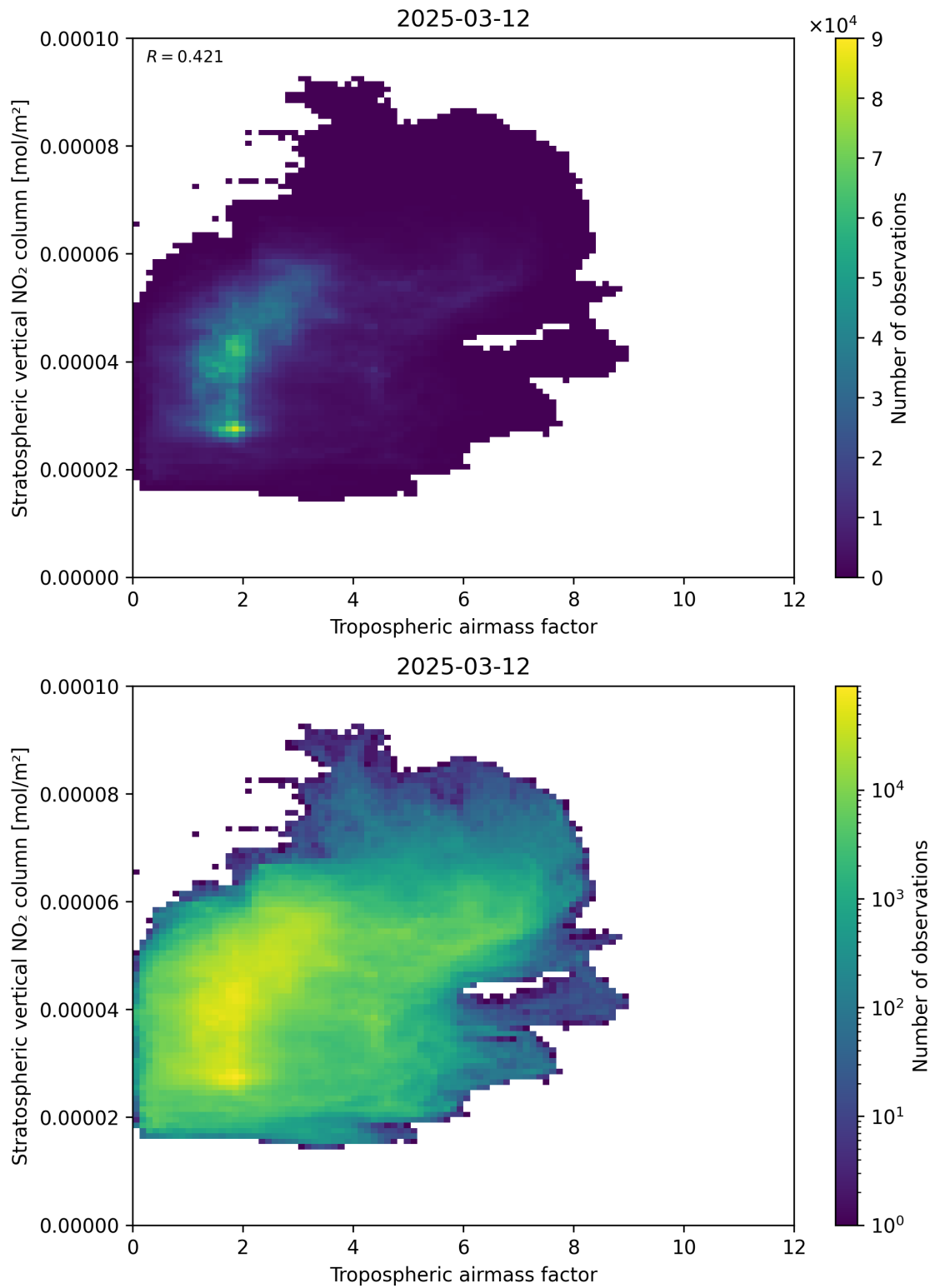
Figure 74: Scatter density plot of “Tropospheric air mass factor” against “Stratospheric vertical NO 2 column” for 2025-03-12 to 2025-03-13.
