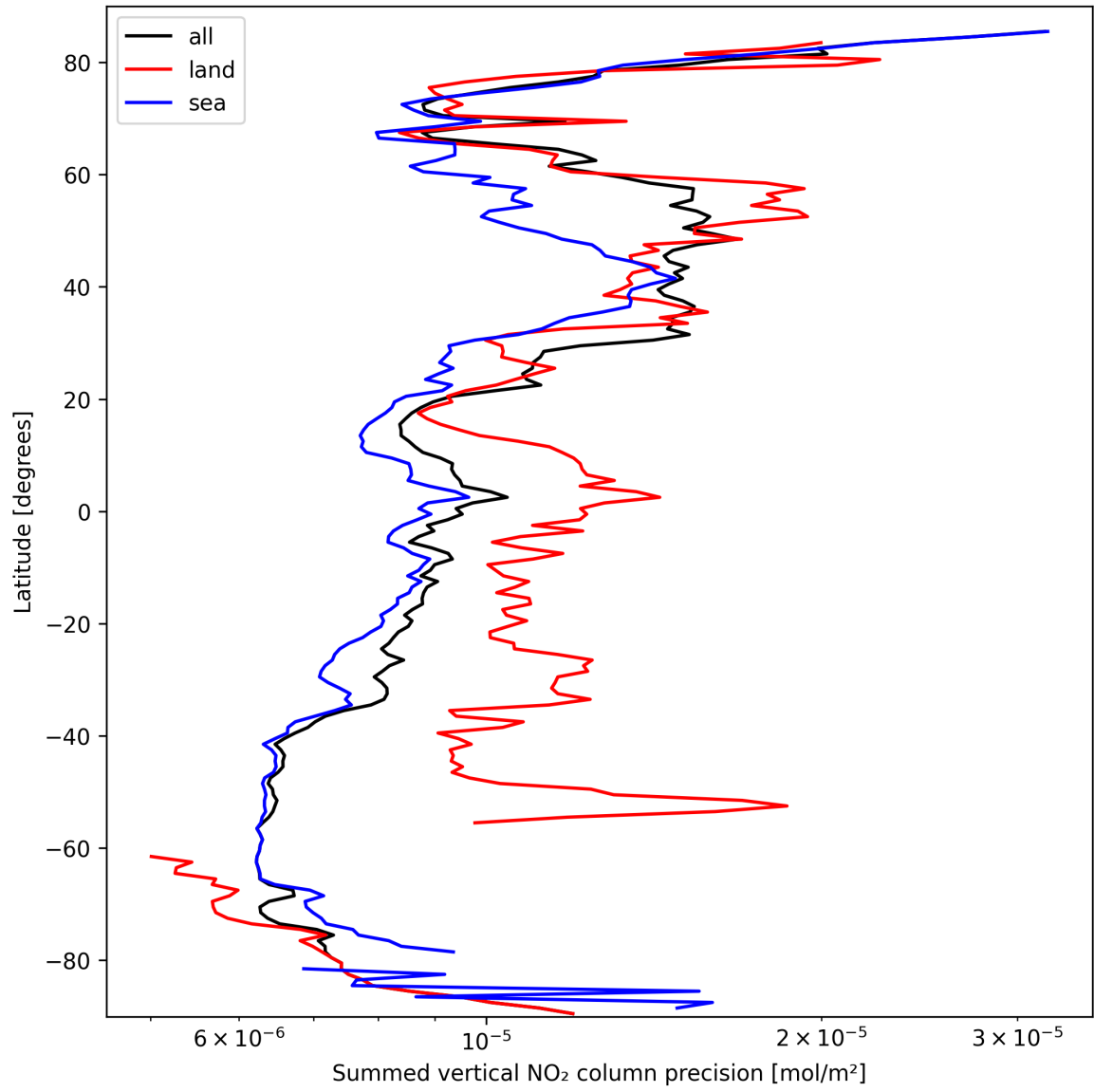
Figure 24: Zonal average of “Summed vertical NO 2 column precision” for 2025-03-12 to 2025-03-13.
