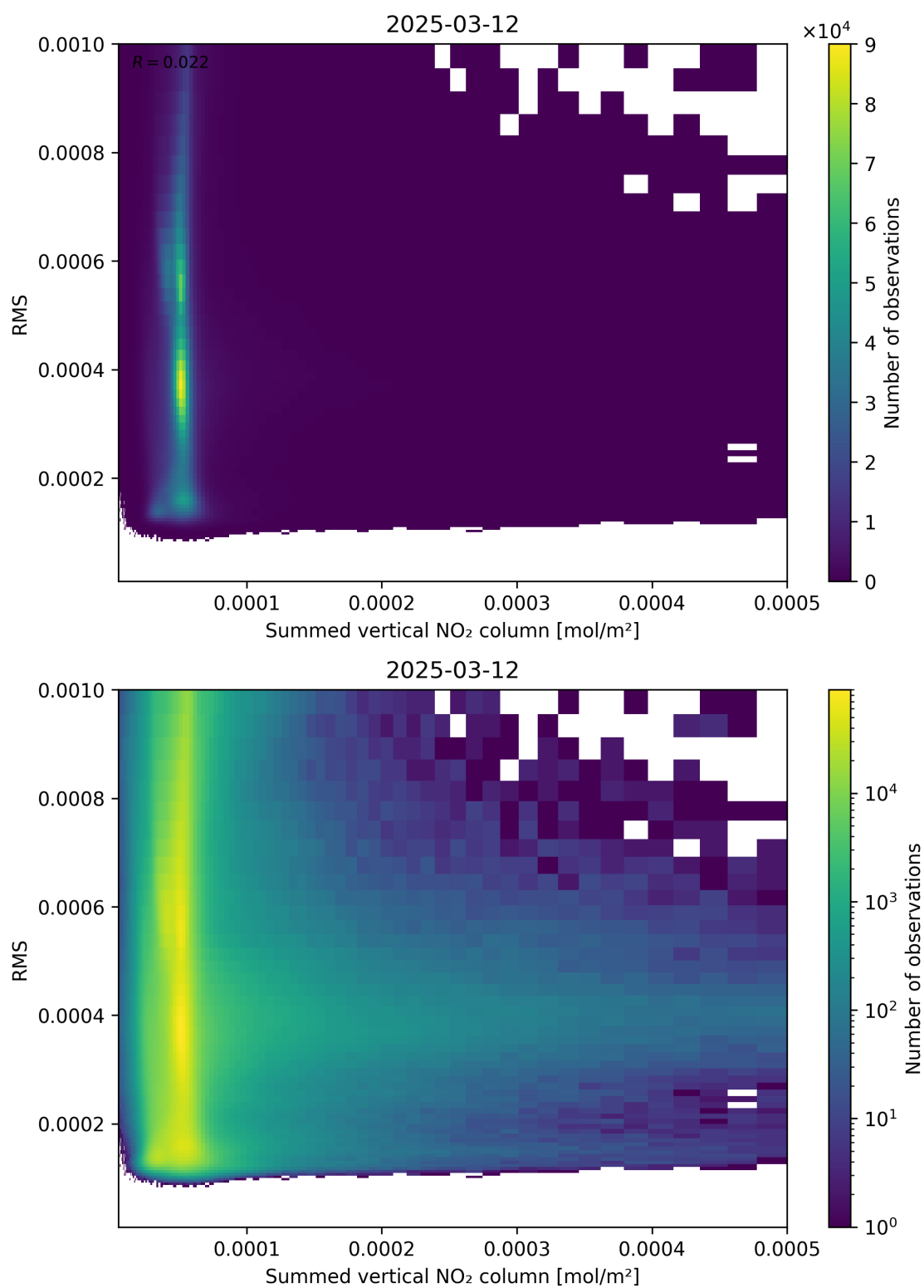
Figure 109: Scatter density plot of “Summed vertical NO 2 column” against “RMS” for 2025-03-12 to 2025-03-13.
