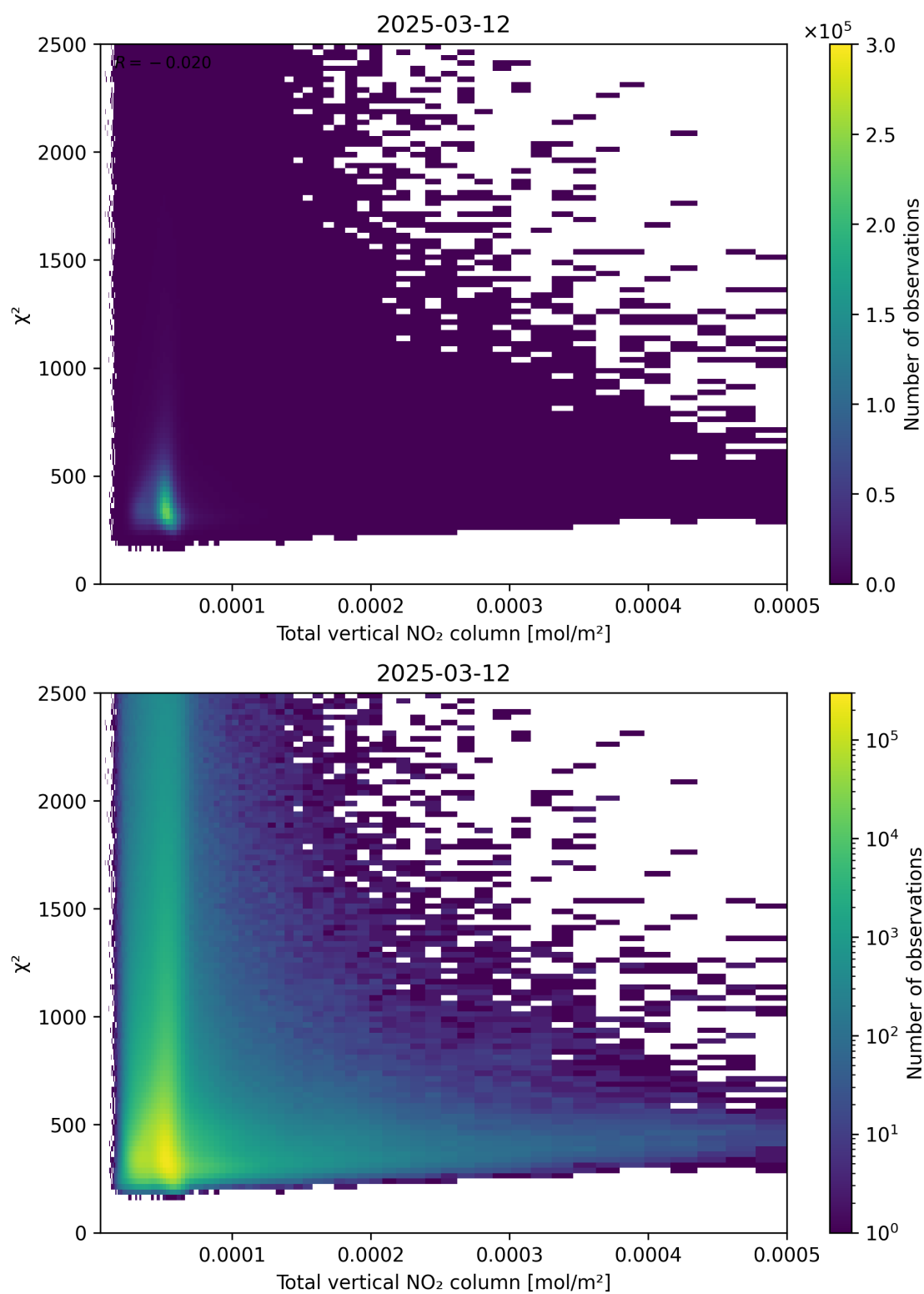
Figure 111: Scatter density plot of “Total vertical NO 2 column” against “ \chi^2 ” for 2025-03-12 to 2025-03-13.
