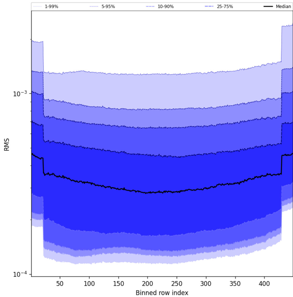
Figure 60: Along track statistics of “RMS” for 2025-03-12 to 2025-03-13
