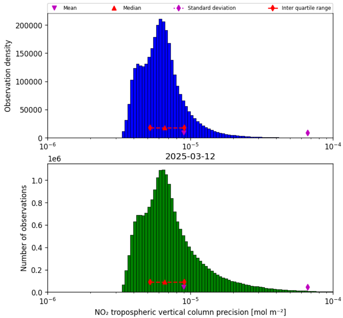
Figure 30: Histogram of “NO 2 tropospheric vertical column precision” for 2025-03-12 to 2025-03-13
