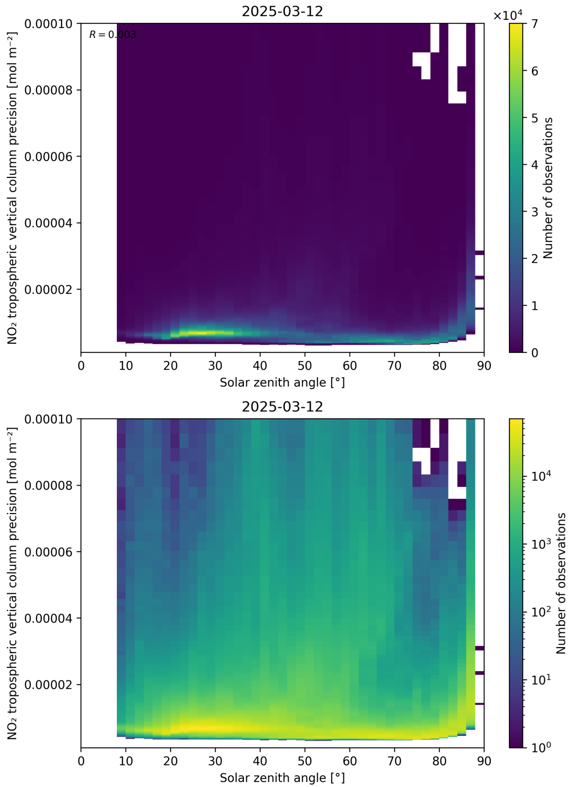
Figure 156: Scatter density plot of “Solar zenith angle” against “NO 2 tropospheric vertical column precision” for 2025-03-12 to 2025-03-13.
