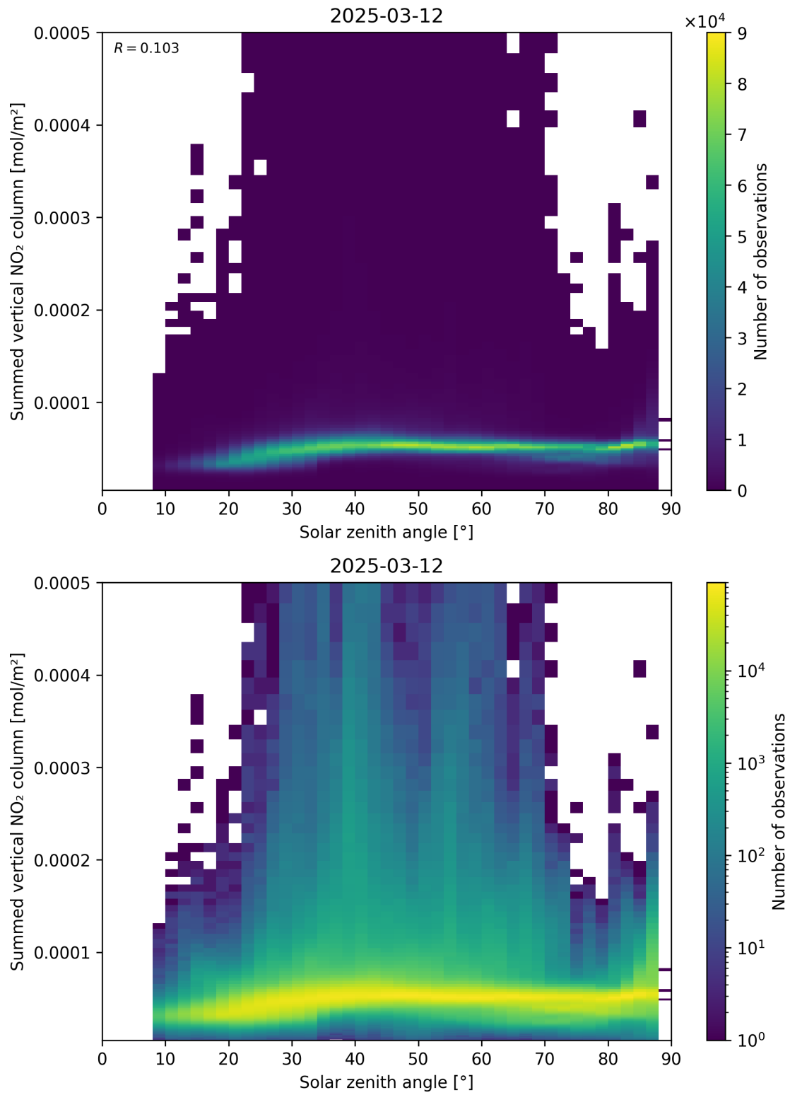
Figure 151: Scatter density plot of “Solar zenith angle” against “Summed vertical NO 2 column” for 2025-03-12 to 2025-03-13.
