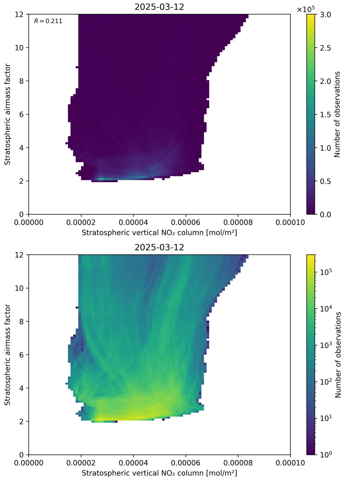
Figure 96: Scatter density plot of “Stratospheric vertical NO 2 column” against “Stratospheric airmass factor” for 2025-03-12 to 2025-03-13.
