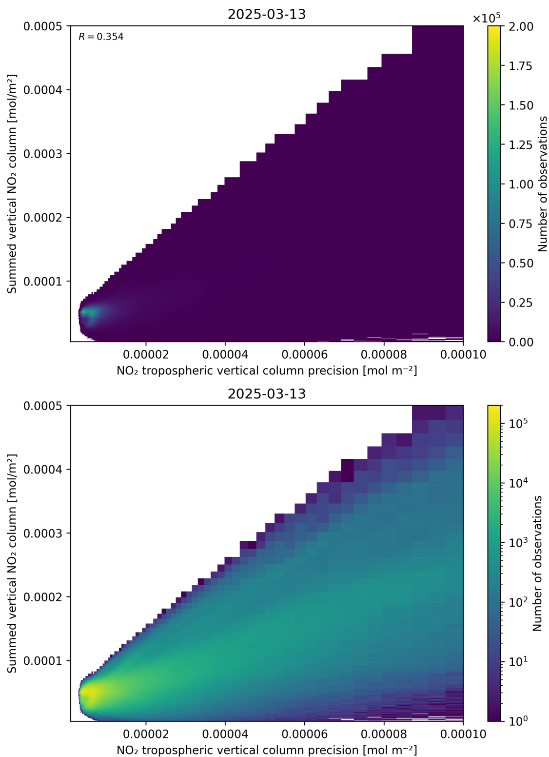
Figure 136: Scatter density plot of “NO 2 tropospheric vertical column precision” against “Summed vertical NO 2 column” for 2025-03-13 to 2025-03-14.
