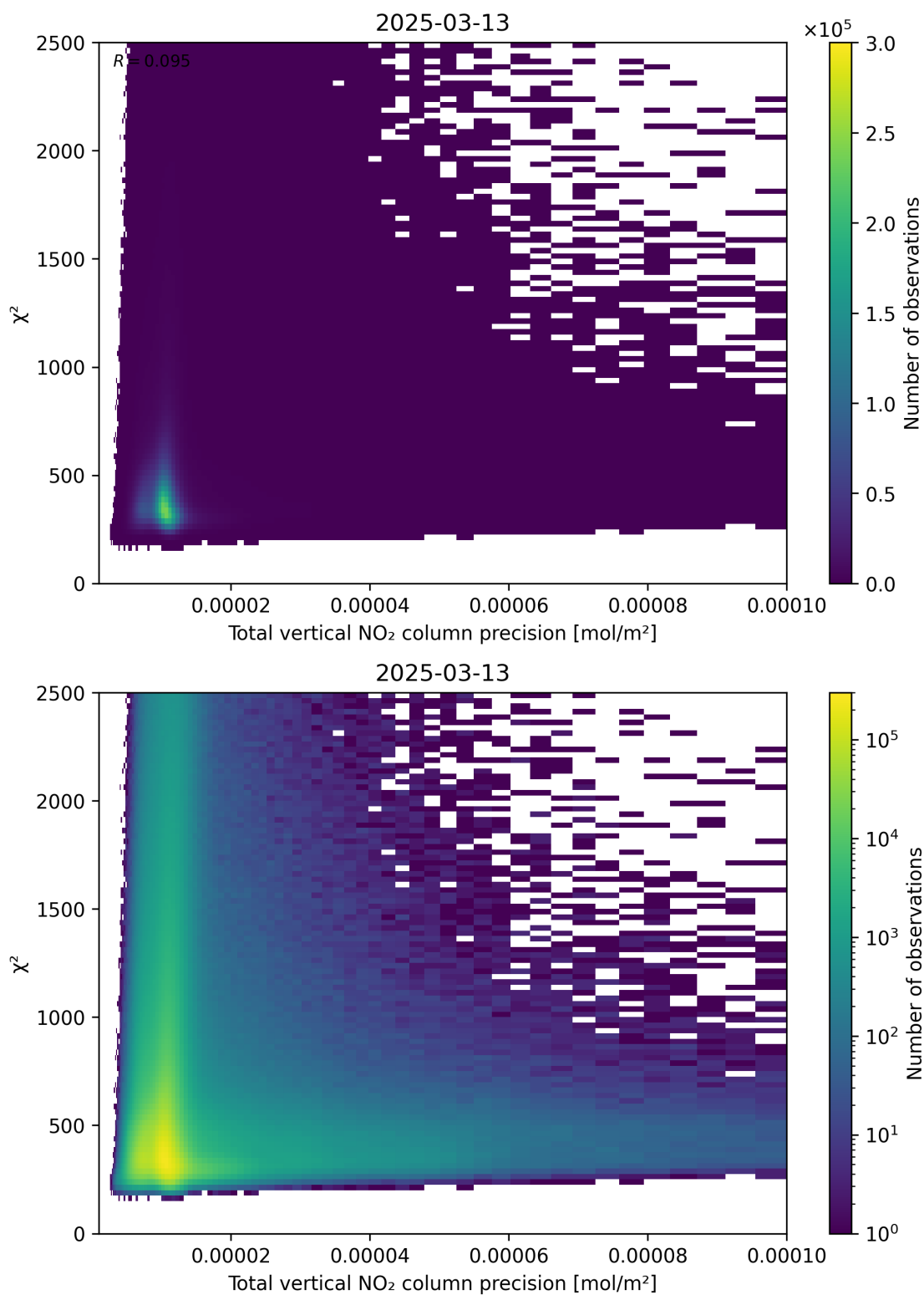
Figure 116: Scatter density plot of “Total vertical NO 2 column precision” against “ \chi^2 ” for 2025-03-13 to 2025-03-14.
