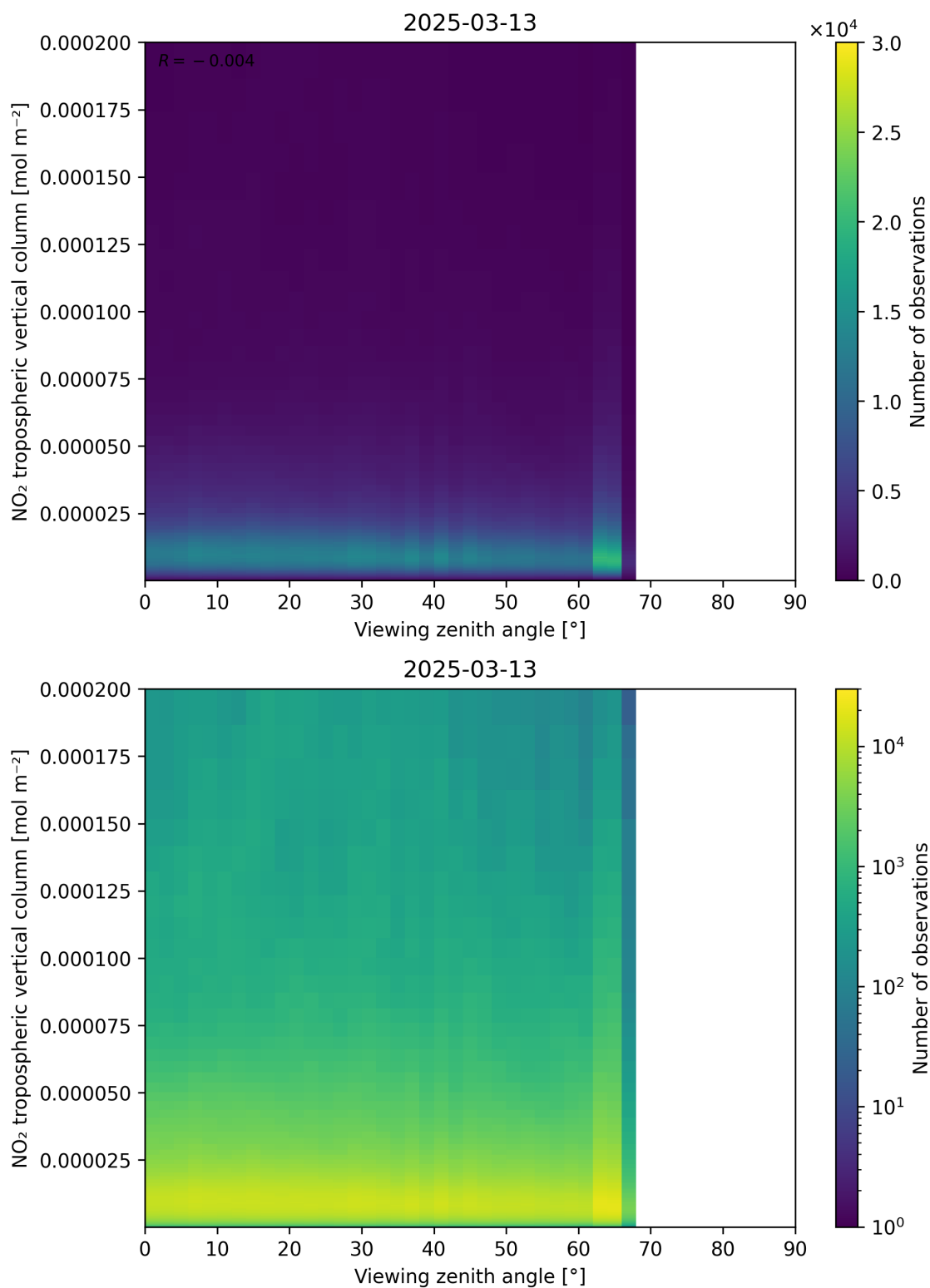
Figure 169: Scatter density plot of “Viewing zenith angle” against “NO 2 tropospheric vertical column” for 2025-03-13 to 2025-03-14.
