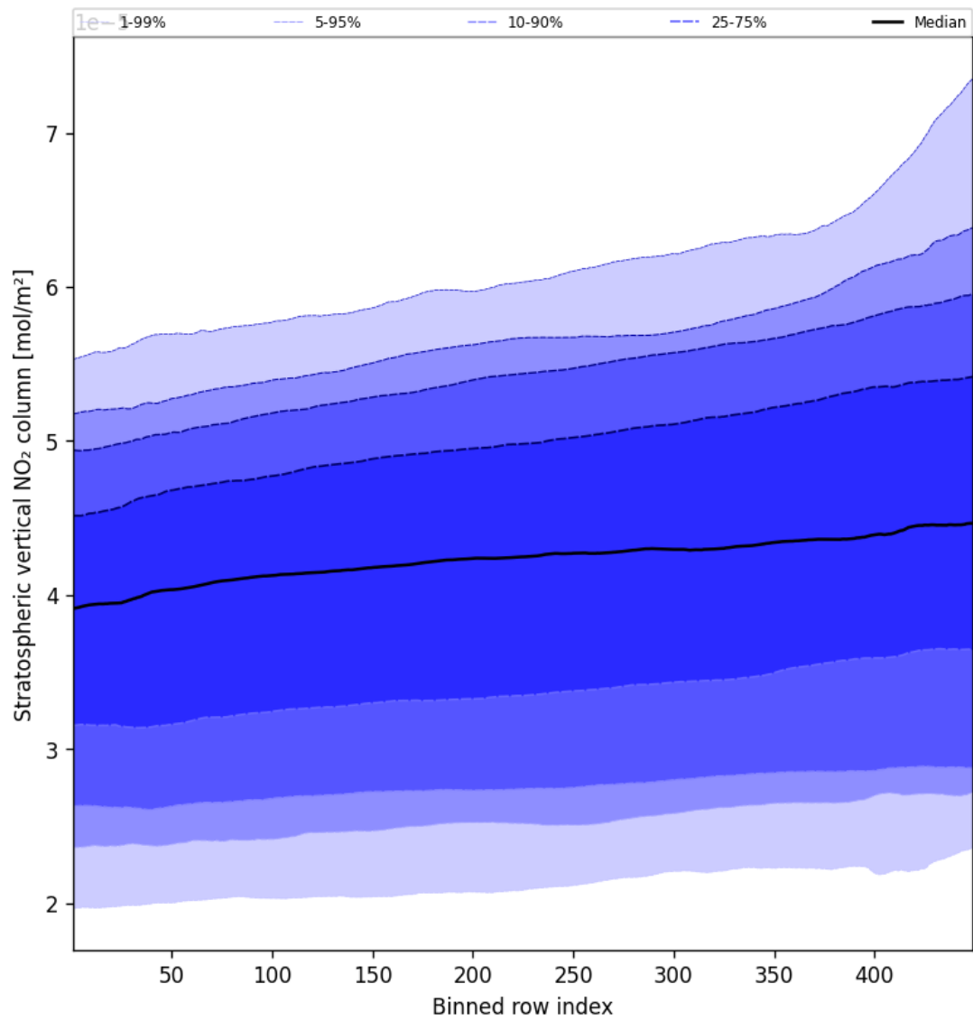
Figure 53: Along track statistics of “Stratospheric vertical NO 2 column” for 2025-03-13 to 2025-03-14
