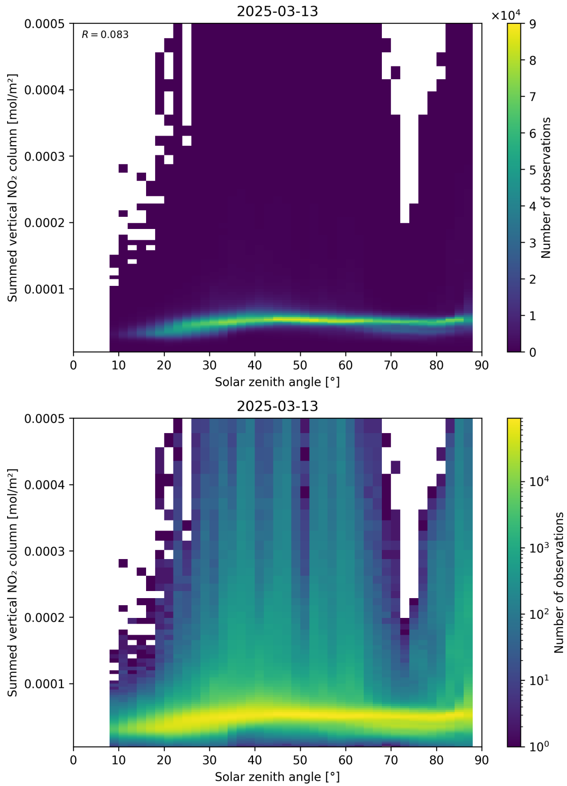
Figure 151: Scatter density plot of “Solar zenith angle” against “Summed vertical NO 2 column” for 2025-03-13 to 2025-03-14.
