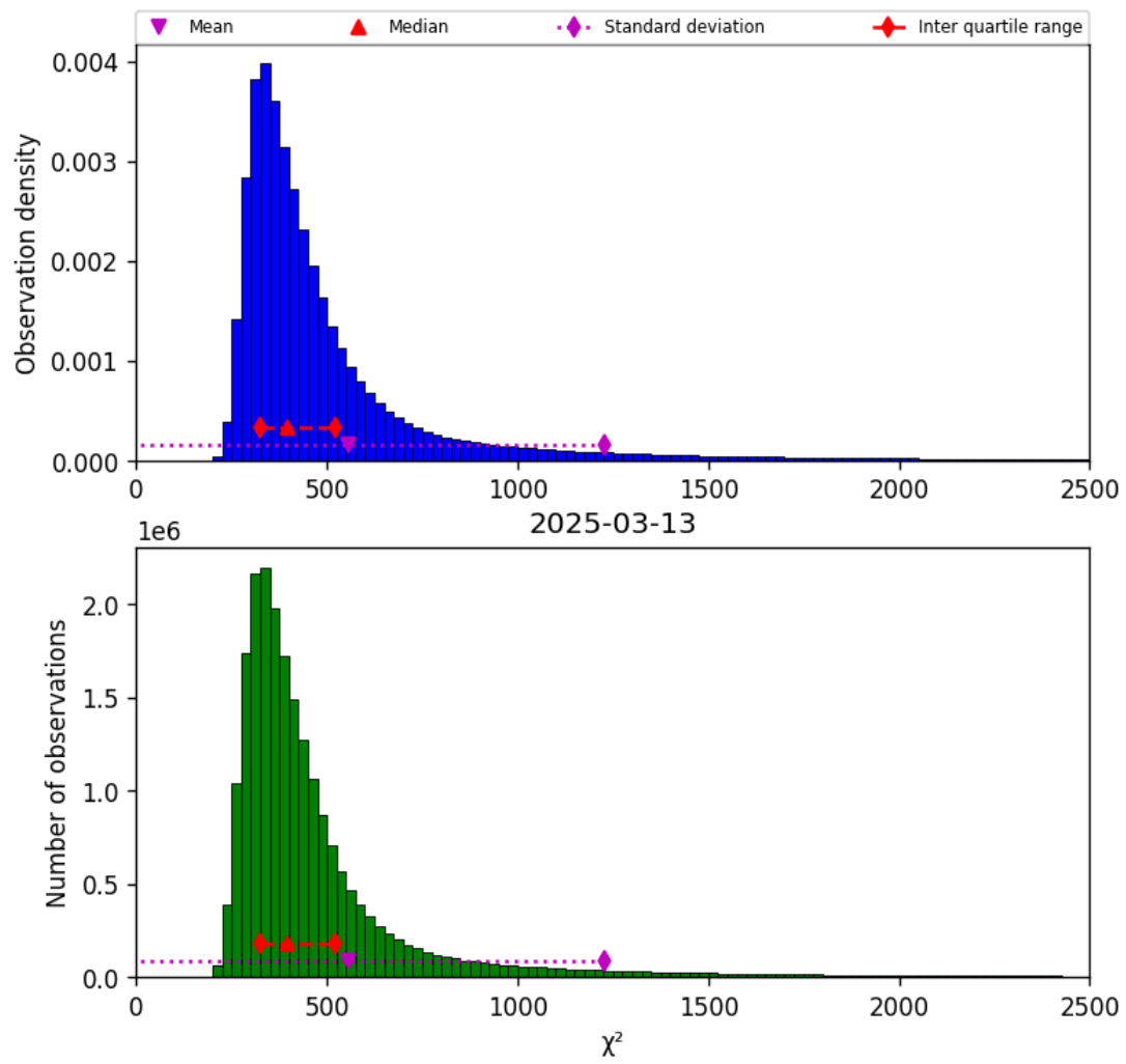
Figure 42: Histogram of “ \chi^2 ” for 2025-03-13 to 2025-03-14
