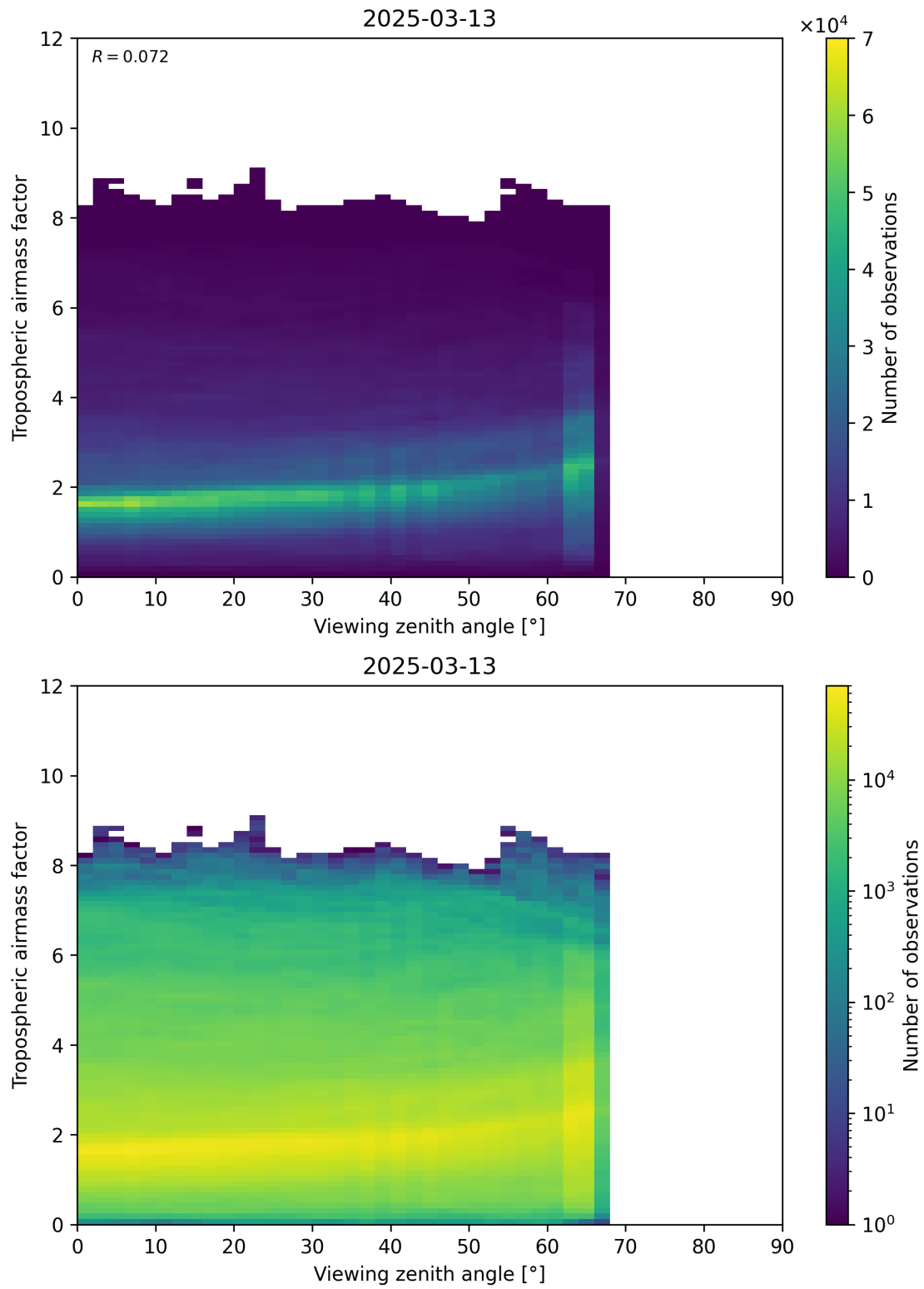
Figure 161: Scatter density plot of “Viewing zenith angle” against “Tropospheric airmass factor” for 2025-03-13 to 2025-03-14.
