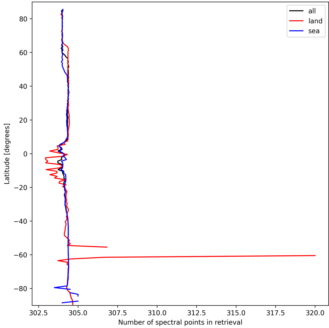
Figure 16: Zonal average of “Number of spectral points in retrieval” for 2025-03-13 to 2025-03-14.
