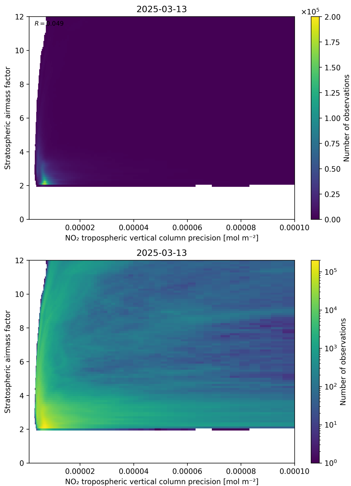
Figure 131: Scatter density plot of “NO 2 tropospheric vertical column precision” against “Stratospheric airmass factor” for 2025-03-13 to 2025-03-14.
