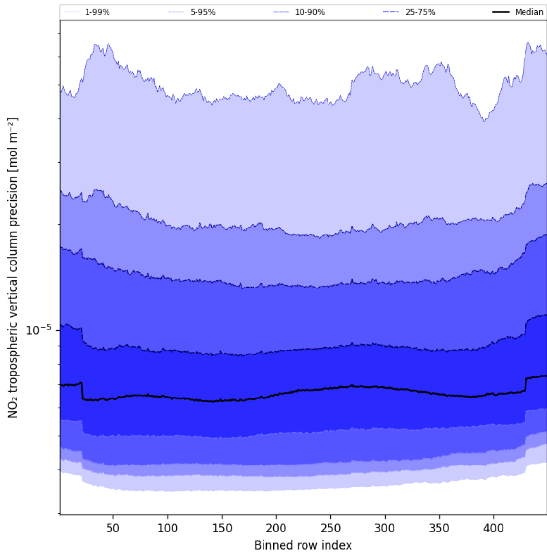
Figure 47: Along track statistics of “NO 2 tropospheric vertical column precision” for 2025-03-13 to 2025-03-14
