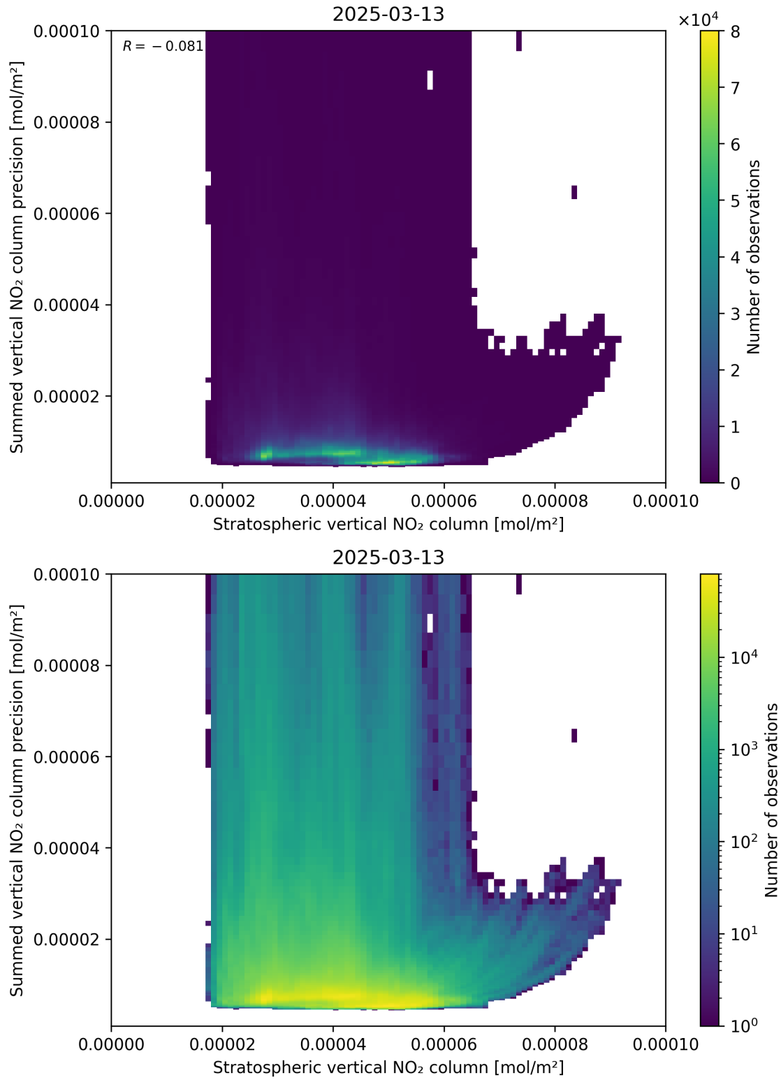
Figure 99: Scatter density plot of “Stratospheric vertical NO 2 column” against “Summed vertical NO 2 column precision” for 2025-03-13 to 2025-03-14.
