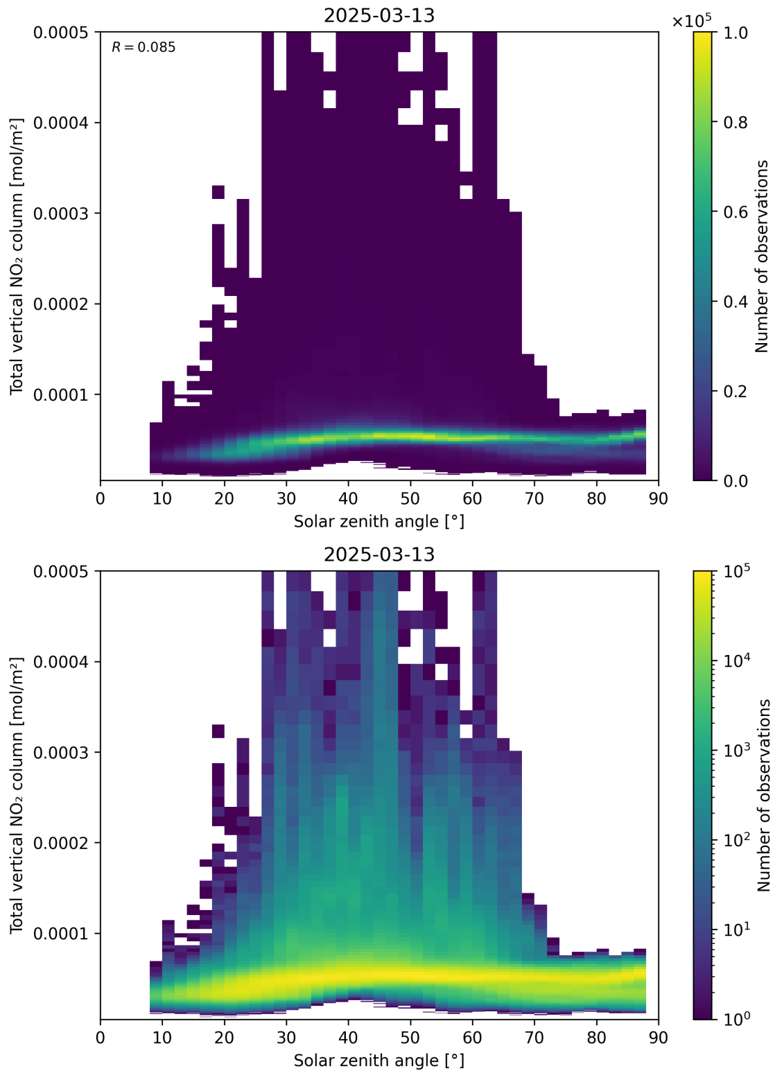
Figure 153: Scatter density plot of “Solar zenith angle” against “Total vertical NO 2 column” for 2025-03-13 to 2025-03-14.
