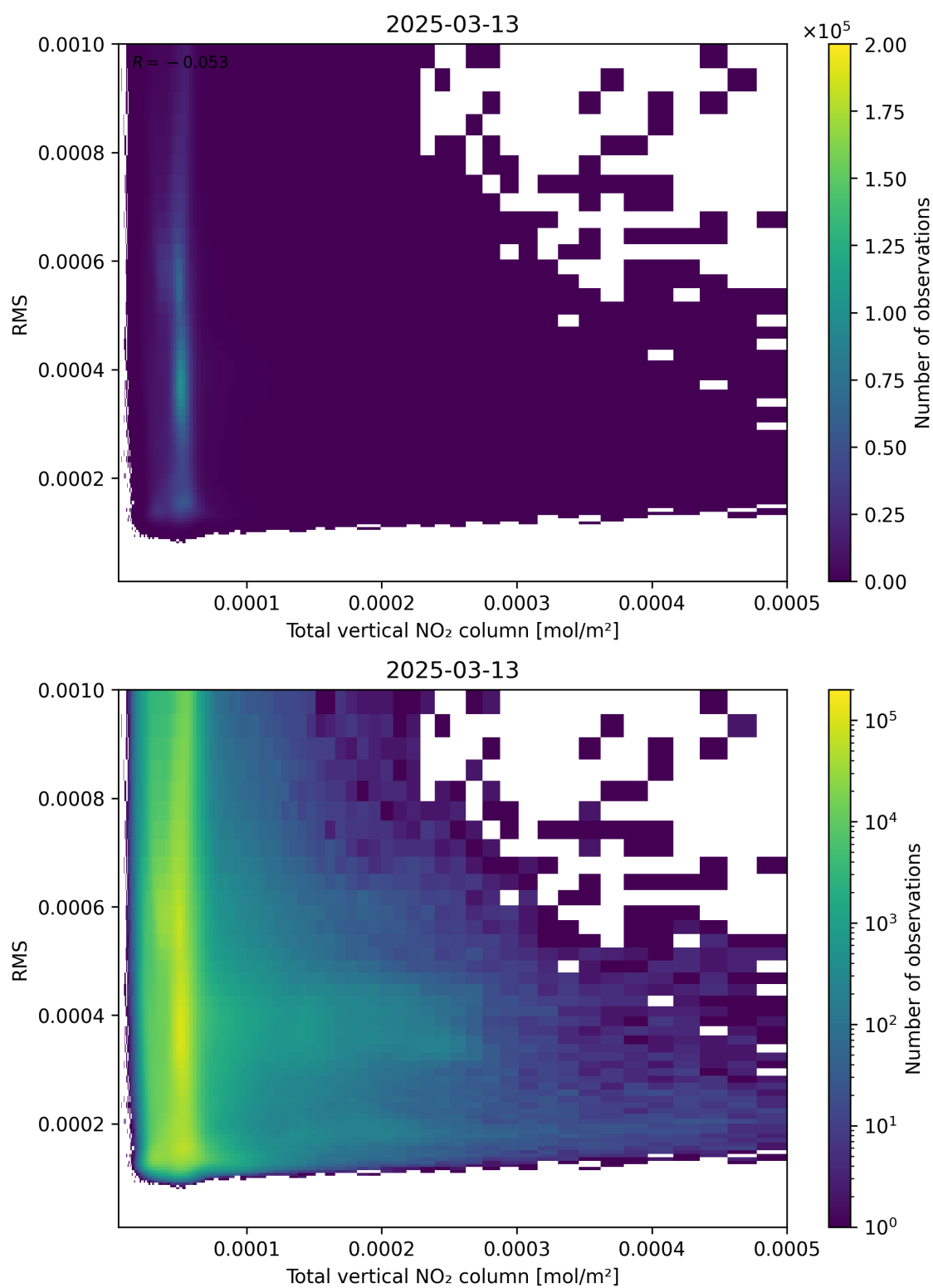
Figure 120: Scatter density plot of “Total vertical NO 2 column” against “RMS” for 2025-03-13 to 2025-03-14.
