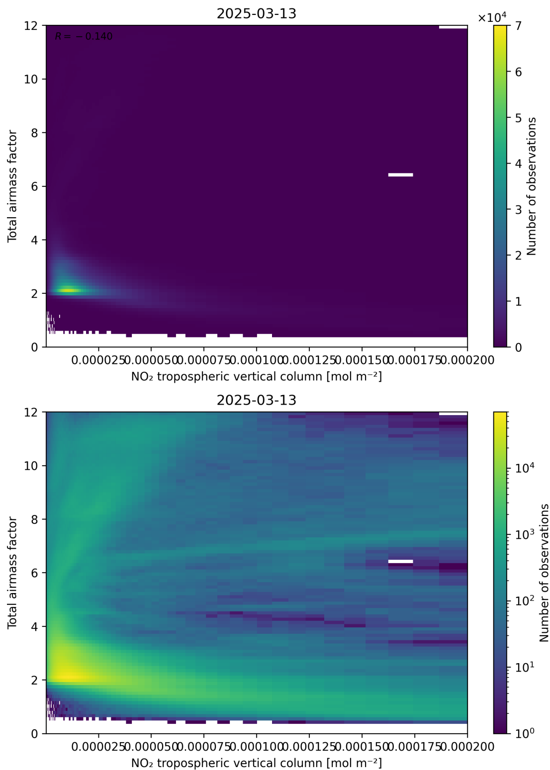
Figure 122: Scatter density plot of “NO 2 tropospheric vertical column” against “Total air mass factor” for 2025-03-13 to 2025-03-14.
