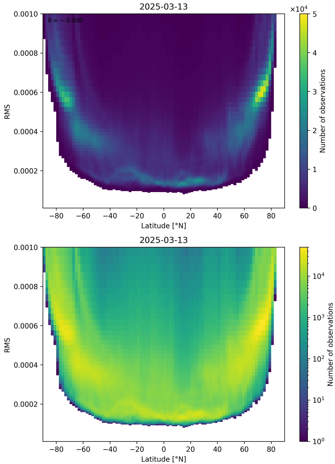
Figure 94: Scatter density plot of “Latitude” against “RMS” for 2025-03-13 to 2025-03-14.
