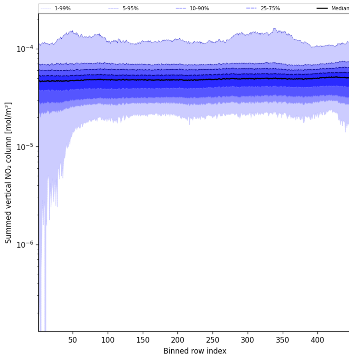
Figure 57: Along track statistics of “Summed vertical NO 2 column” for 2025-03-13 to 2025-03-14
