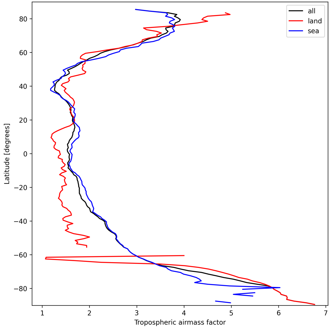
Figure 14: Zonal average of “Tropospheric air mass factor” for 2025-03-13 to 2025-03-14.
