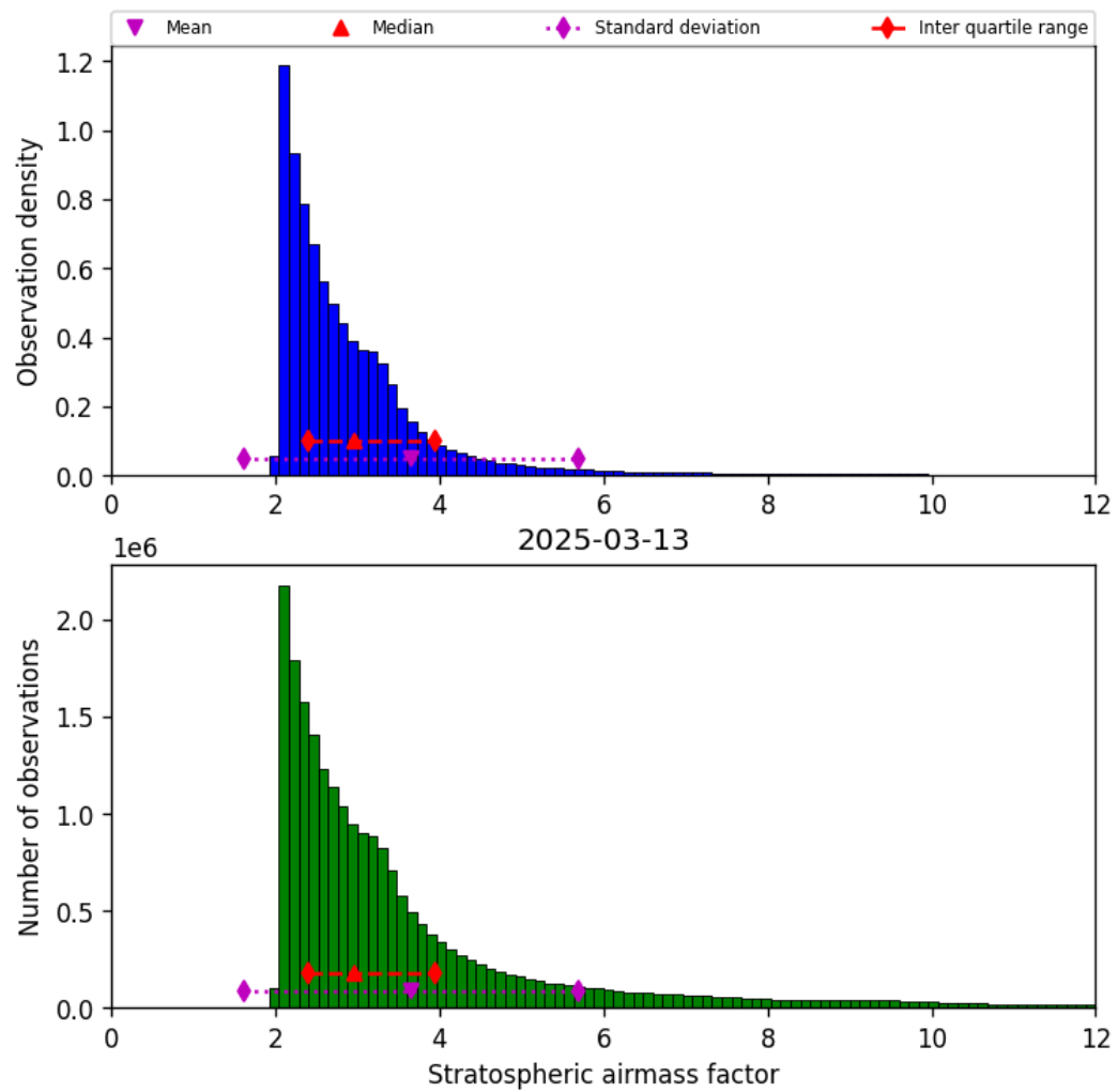
Figure 44: Histogram of “Stratospheric airmass factor” for 2025-03-13 to 2025-03-14
