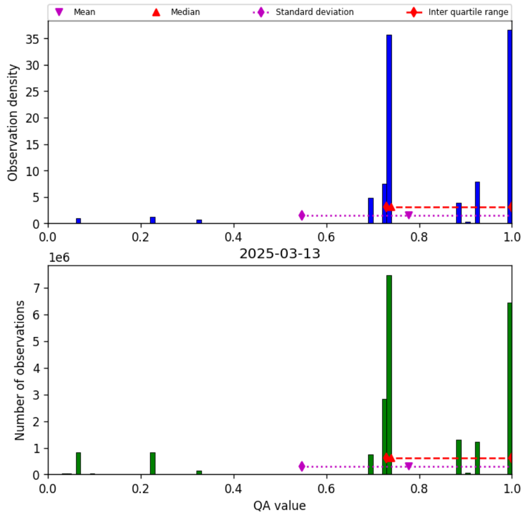
Figure 28: Histogram of “QA value” for 2025-03-13 to 2025-03-14
