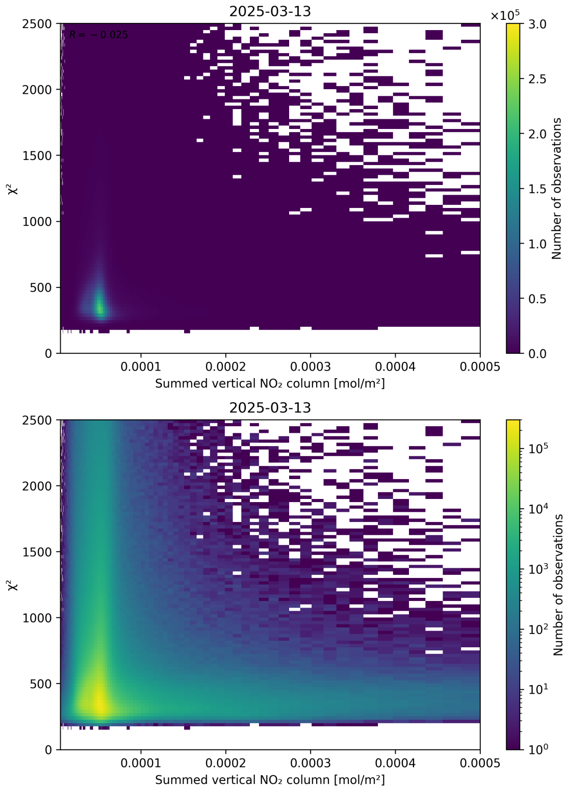
Figure 104: Scatter density plot of “Summed vertical NO 2 column” against “ \chi^2 ” for 2025-03-13 to 2025-03-14.
