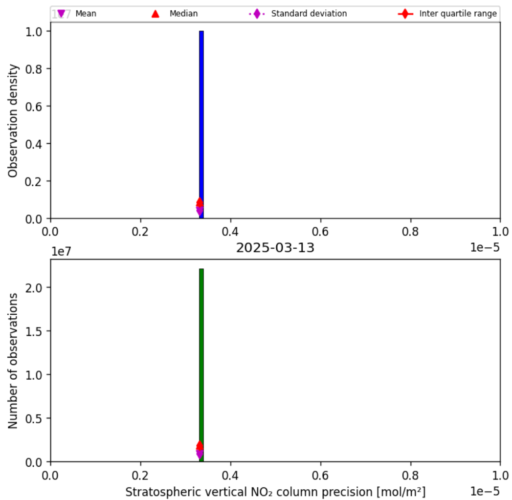
Figure 37: Histogram of “Stratospheric vertical NO 2 column precision” for 2025-03-13 to 2025-03-14
