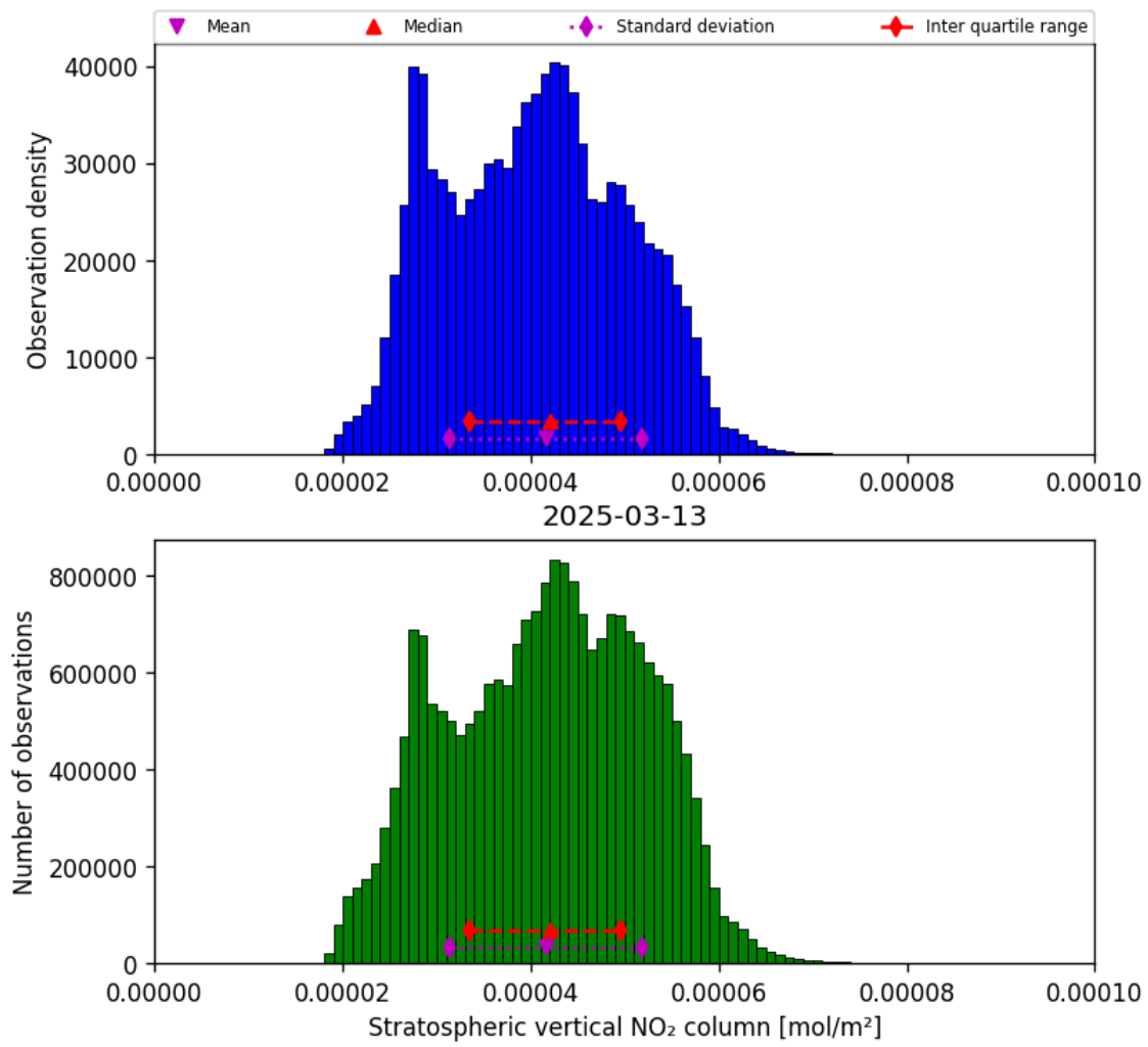
Figure 36: Histogram of “Stratospheric vertical NO 2 column” for 2025-03-13 to 2025-03-14
