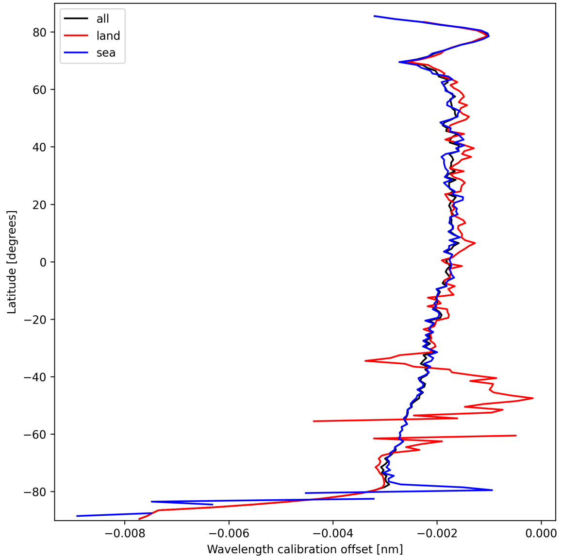
Figure 18: Zonal average of “Wavelength calibration offset” for 2025-03-13 to 2025-03-14.
