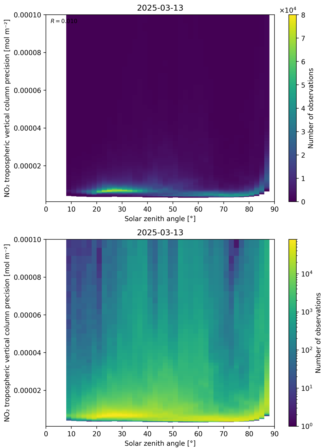
Figure 156: Scatter density plot of “Solar zenith angle” against “NO 2 tropospheric vertical column precision” for 2025-03-13 to 2025-03-14.
