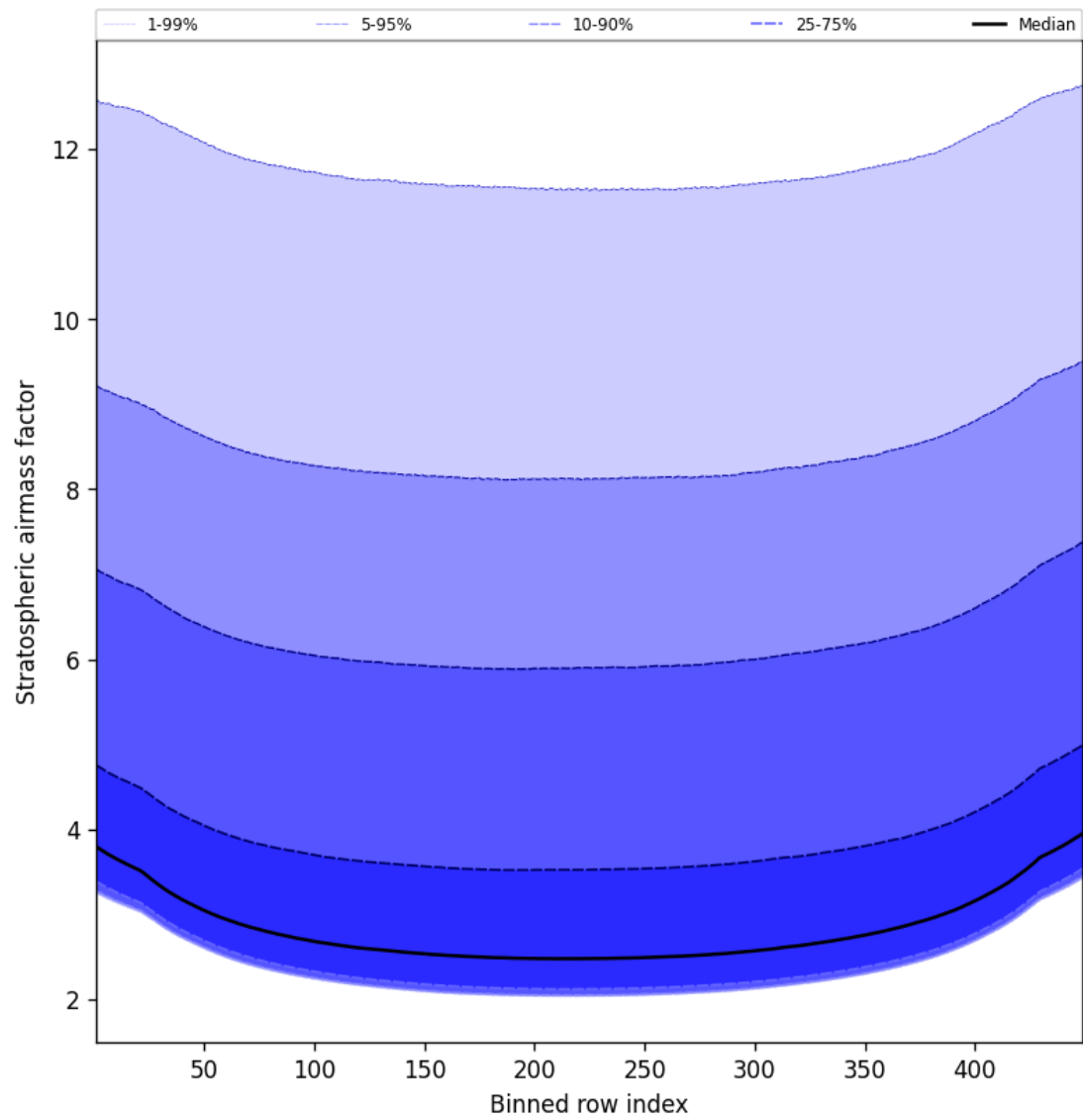
Figure 61: Along track statistics of “Stratospheric air mass factor” for 2025-03-13 to 2025-03-14
