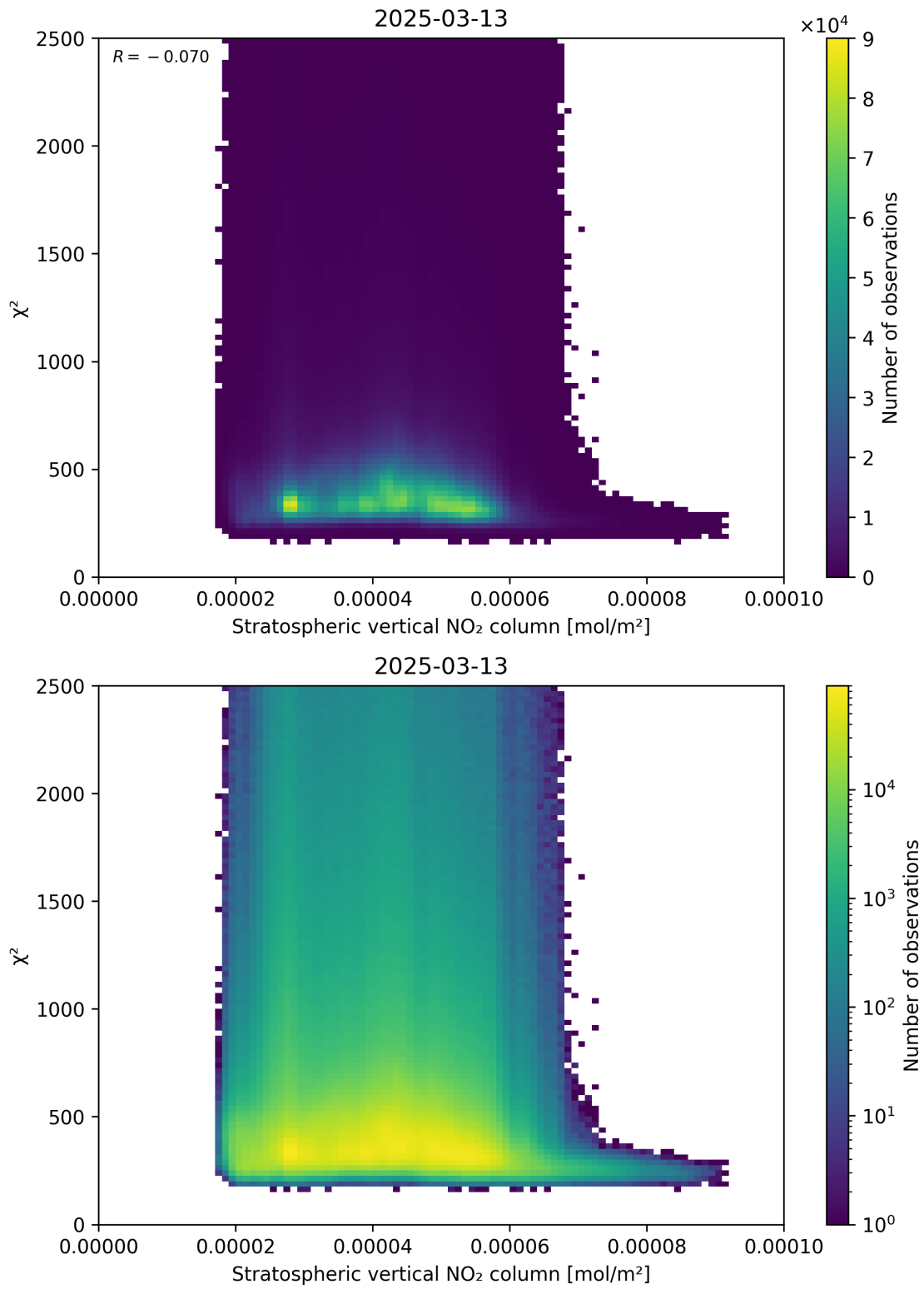
Figure 97: Scatter density plot of “Stratospheric vertical NO 2 column” against “ \chi^2 ” for 2025-03-13 to 2025-03-14.
