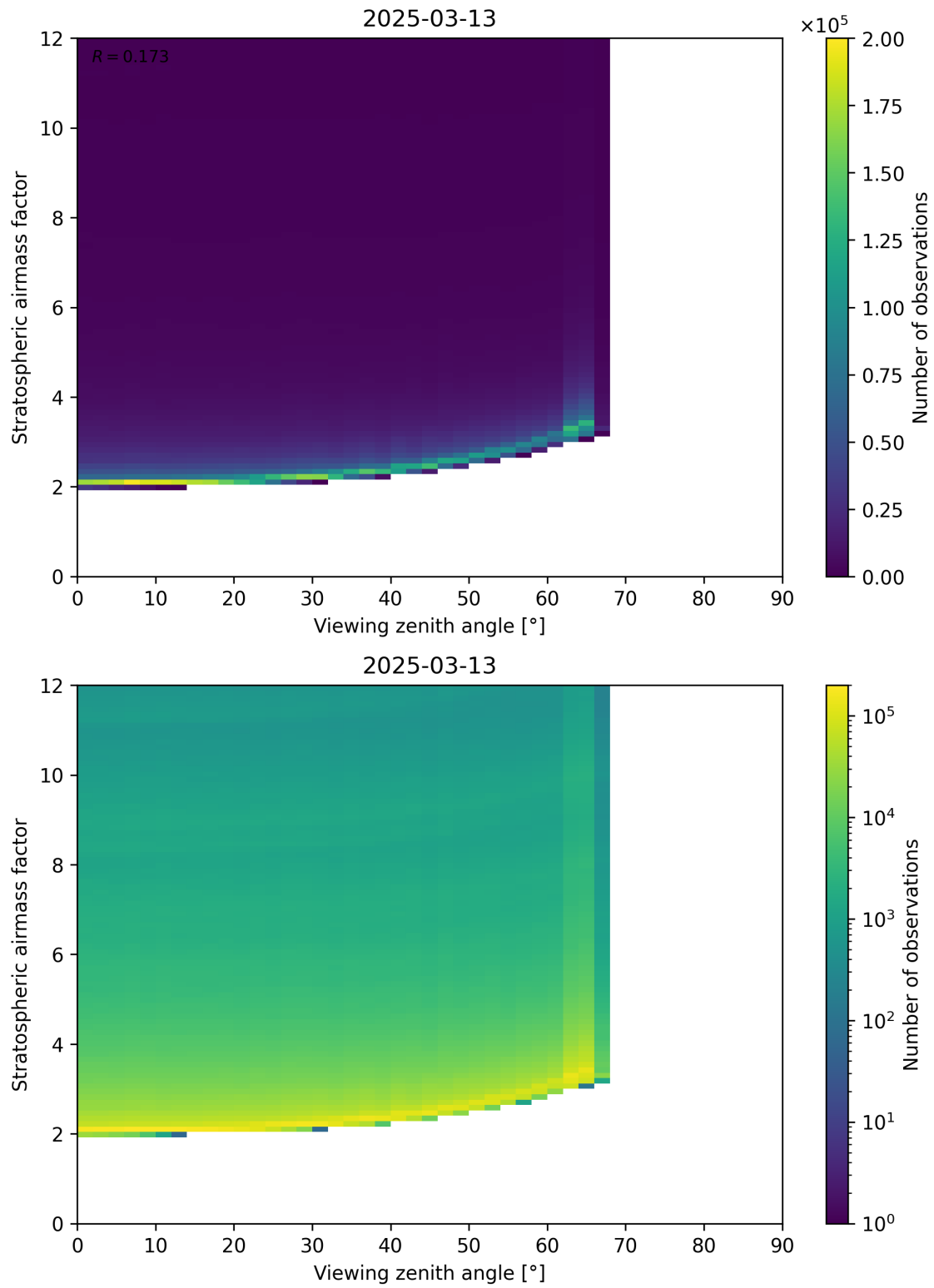
Figure 159: Scatter density plot of “Viewing zenith angle” against “Stratospheric airmass factor” for 2025-03-13 to 2025-03-14.
