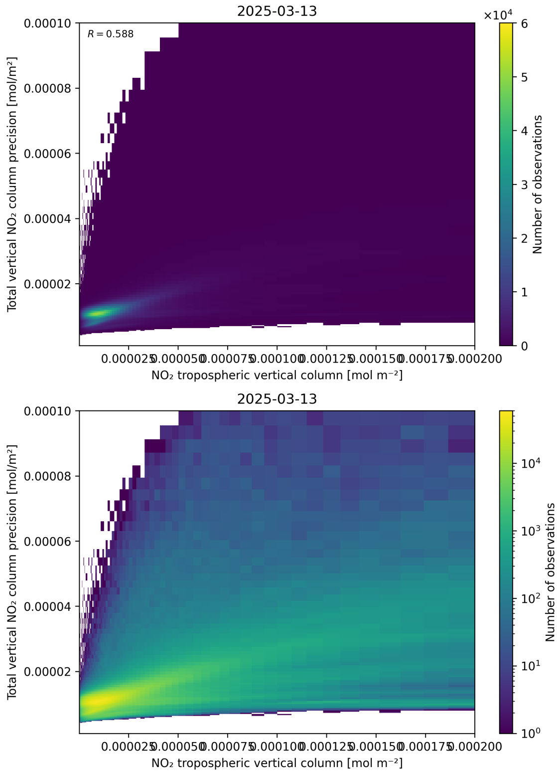
Figure 129: Scatter density plot of “NO 2 tropospheric vertical column” against “Total vertical NO 2 column precision” for 2025-03-13 to 2025-03-14.
