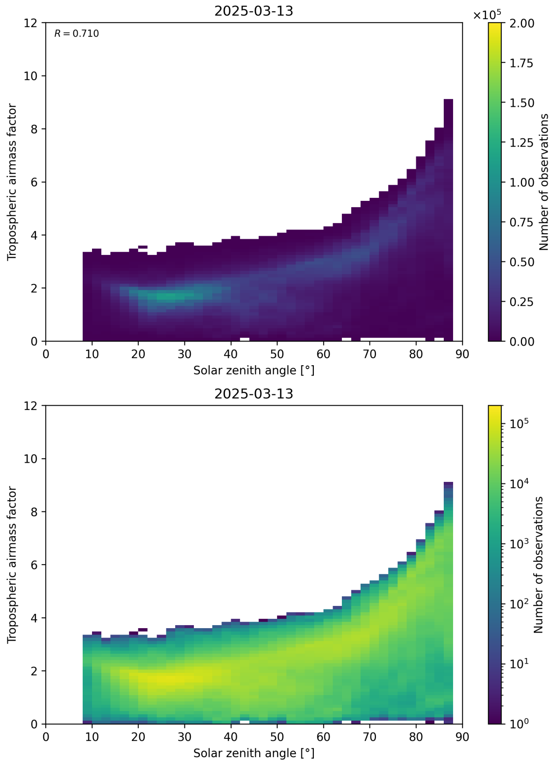
Figure 147: Scatter density plot of “Solar zenith angle” against “Tropospheric airmass factor” for 2025-03-13 to 2025-03-14.
