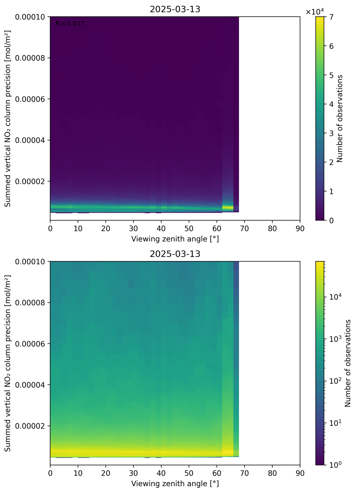
Figure 166: Scatter density plot of “Viewing zenith angle” against “Summed vertical NO 2 column precision” for 2025-03-13 to 2025-03-14.
