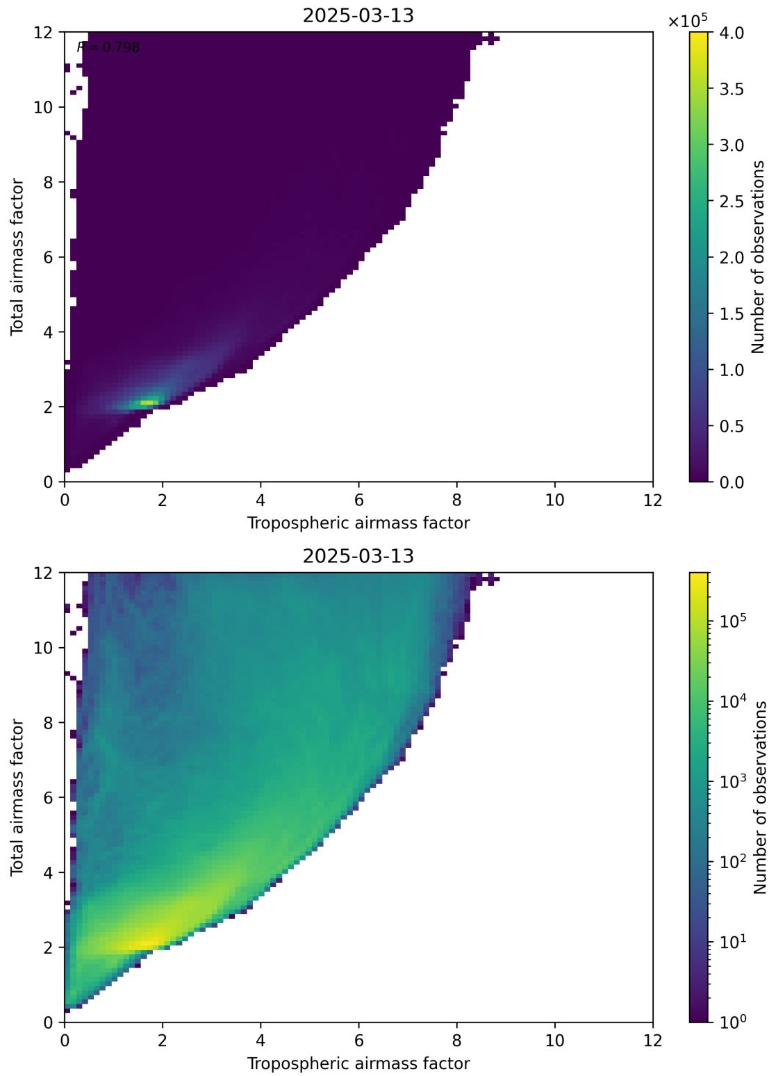
Figure 72: Scatter density plot of “Tropospheric airmass factor” against “Total airmass factor” for 2025-03-13 to 2025-03-14.
