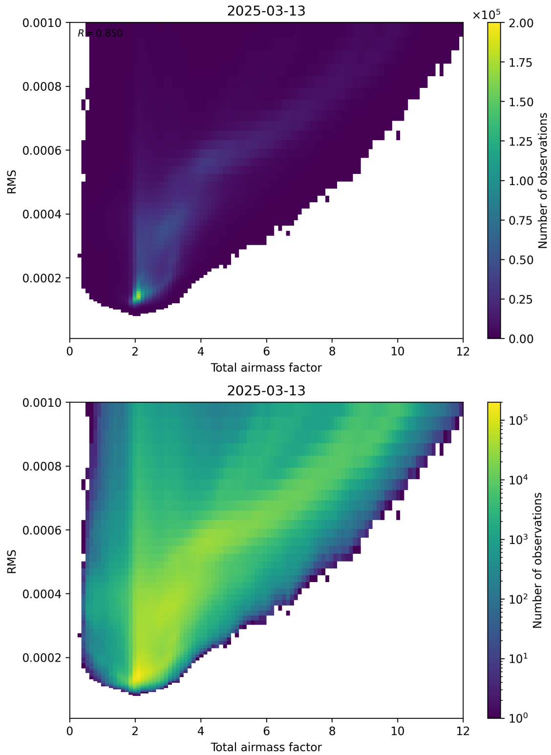
Figure 69: Scatter density plot of “Total airmass factor” against “RMS” for 2025-03-13 to 2025-03-14.
