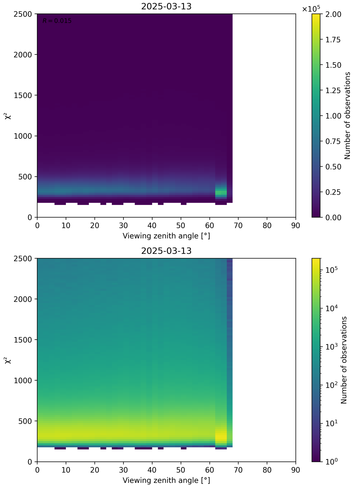
Figure 162: Scatter density plot of “Viewing zenith angle” against “ \chi^2 ” for 2025-03-13 to 2025-03-14.
