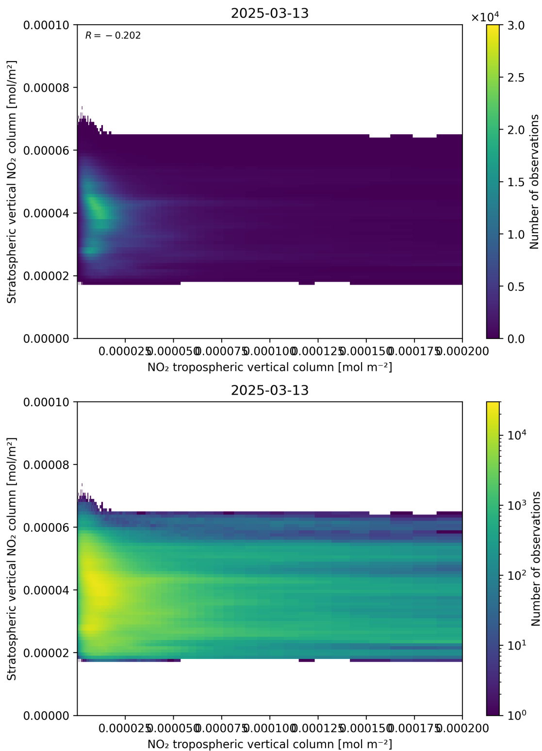
Figure 125: Scatter density plot of “NO 2 tropospheric vertical column” against “Stratospheric vertical NO 2 column” for 2025-03-13 to 2025-03-14.
