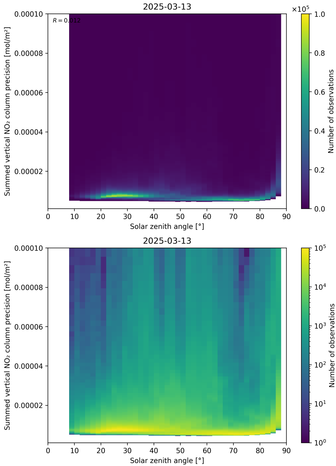
Figure 152: Scatter density plot of “Solar zenith angle” against “Summed vertical NO 2 column precision” for 2025-03-13 to 2025-03-14.
