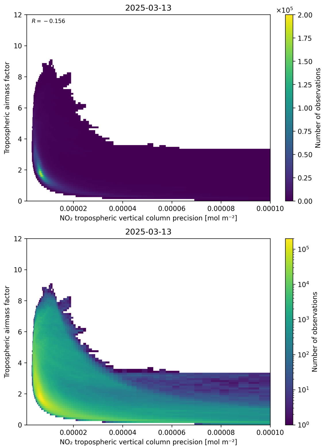
Figure 133: Scatter density plot of “NO 2 tropospheric vertical column precision” against “Tropospheric airmass factor” for 2025-03-13 to 2025-03-14.
