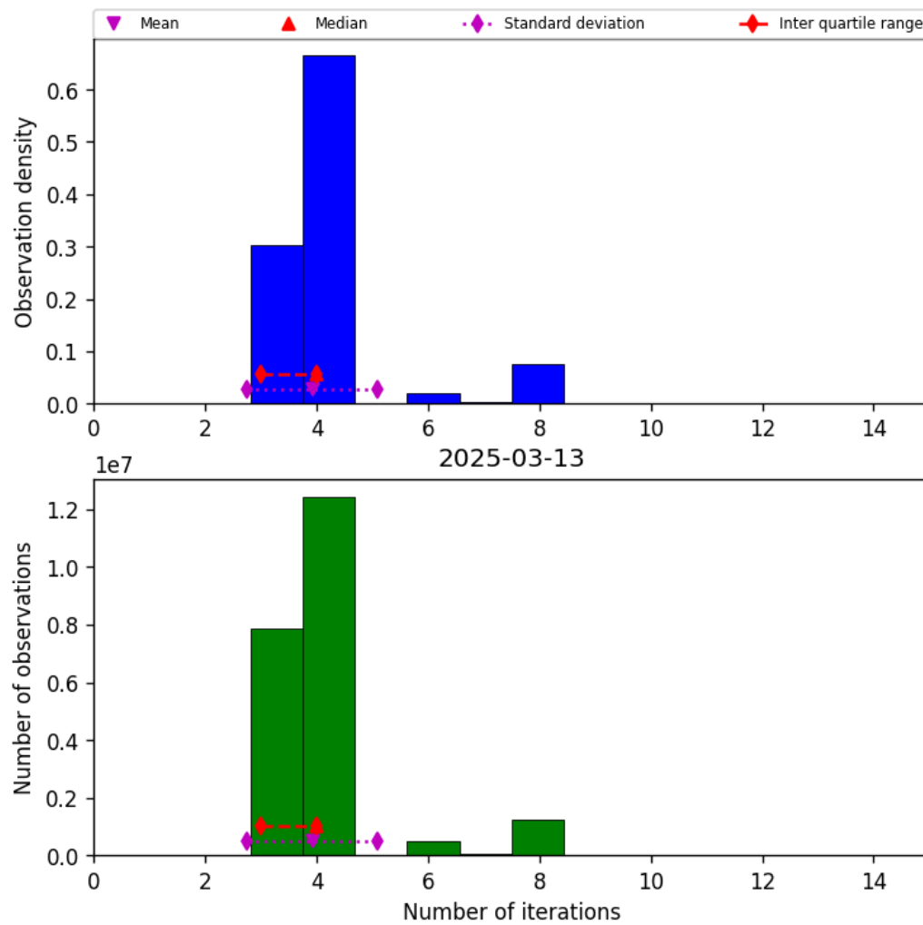
Figure 34: Histogram of “Number of iterations” for 2025-03-13 to 2025-03-14
