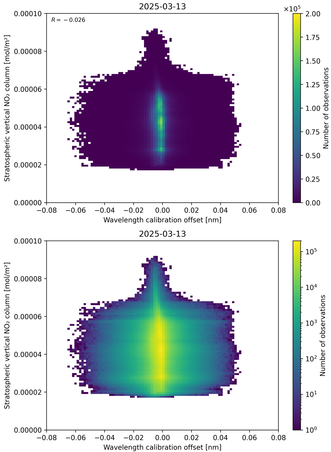
Figure 176: Scatter density plot of “Wavelength calibration offset” against “Stratospheric vertical NO 2 column” for 2025-03-13 to 2025-03-14.
