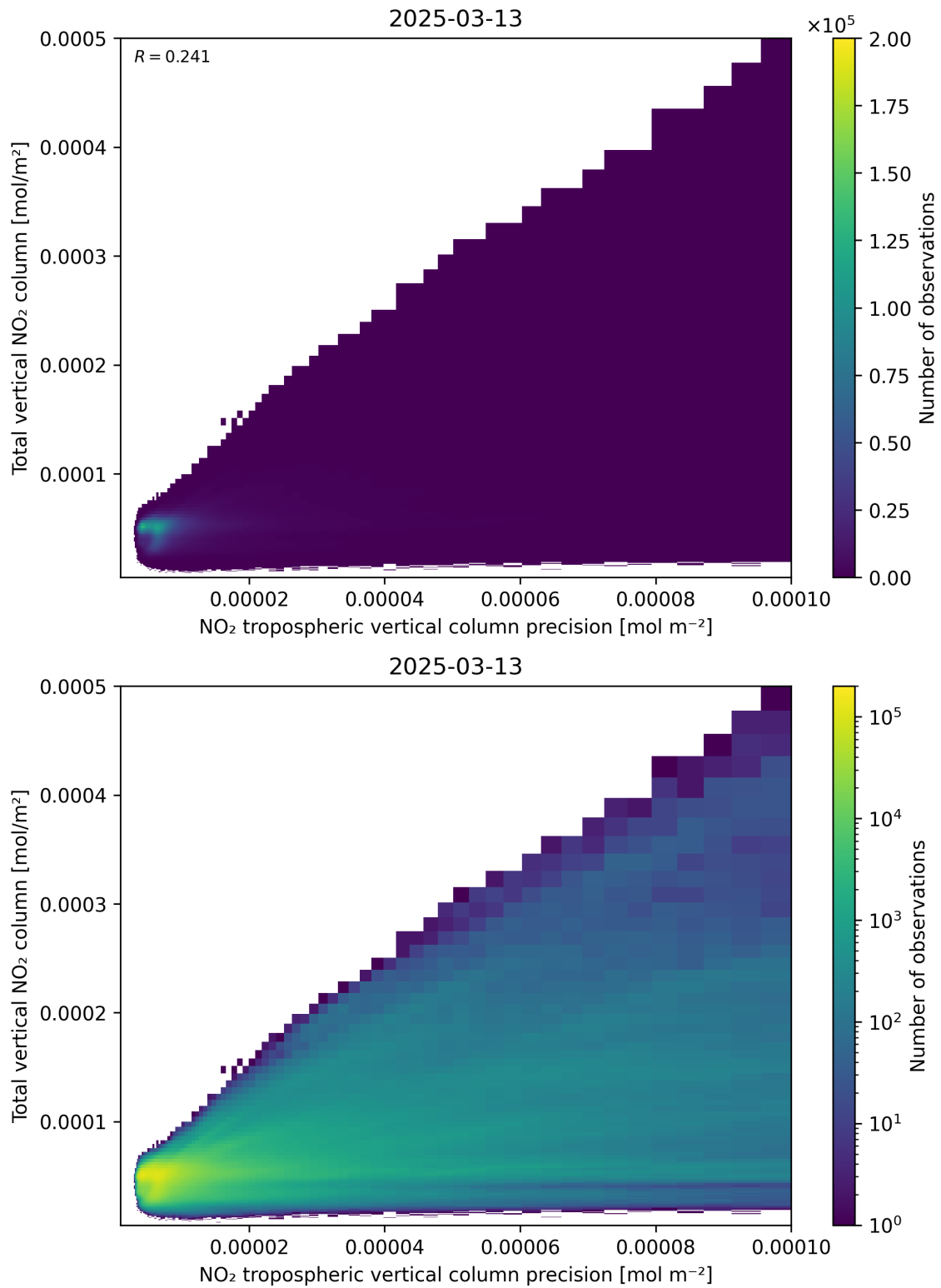
Figure 138: Scatter density plot of “NO 2 tropospheric vertical column precision” against “Total vertical NO 2 column” for 2025-03-13 to 2025-03-14.
