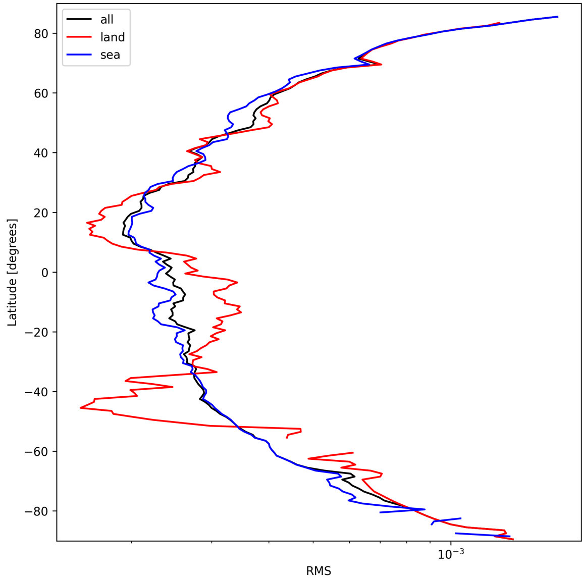
Figure 26: Zonal average of “RMS” for 2025-03-13 to 2025-03-14.
