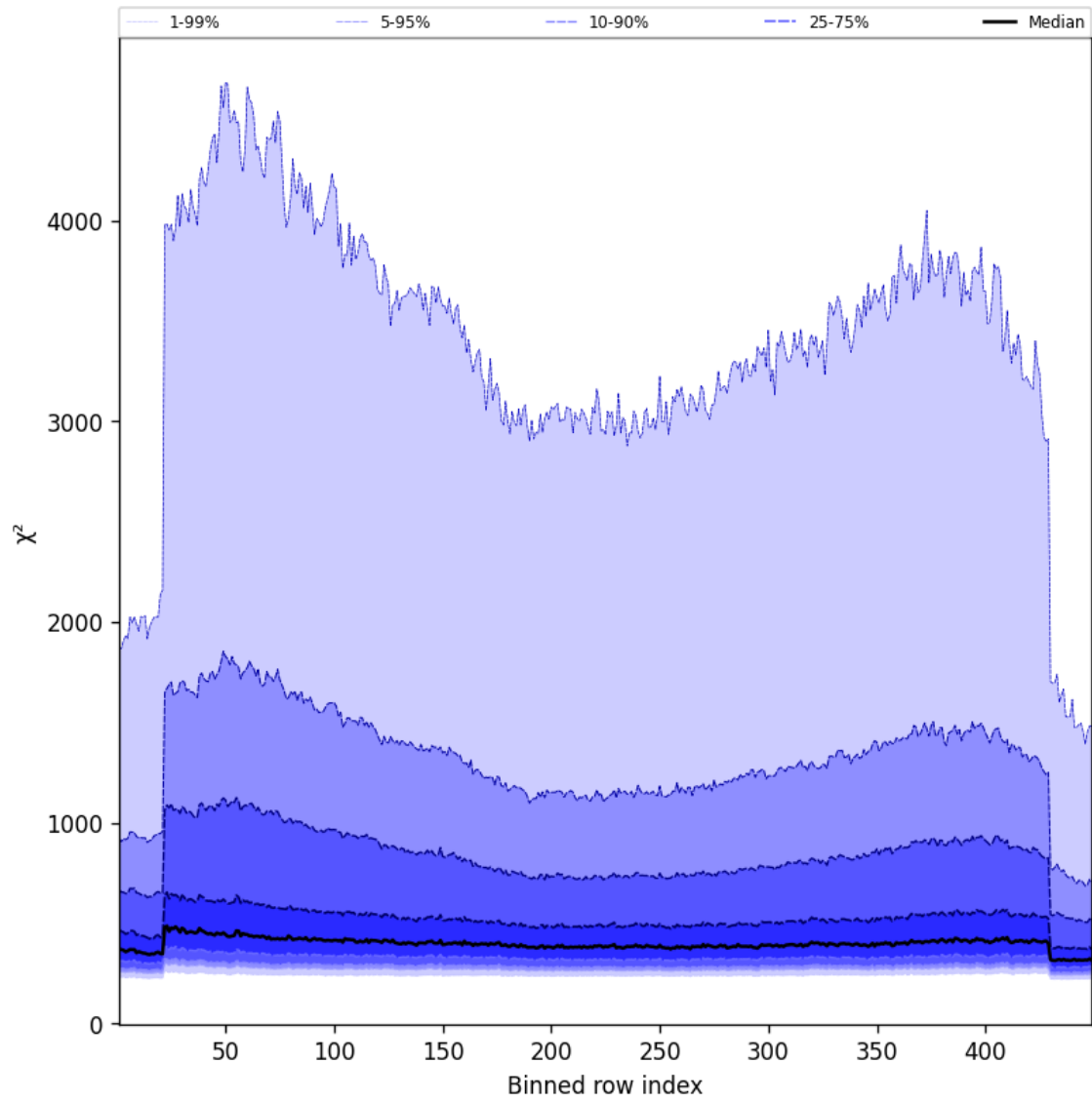
Figure 59: Along track statistics of “ \chi^2 ” for 2025-03-13 to 2025-03-14
