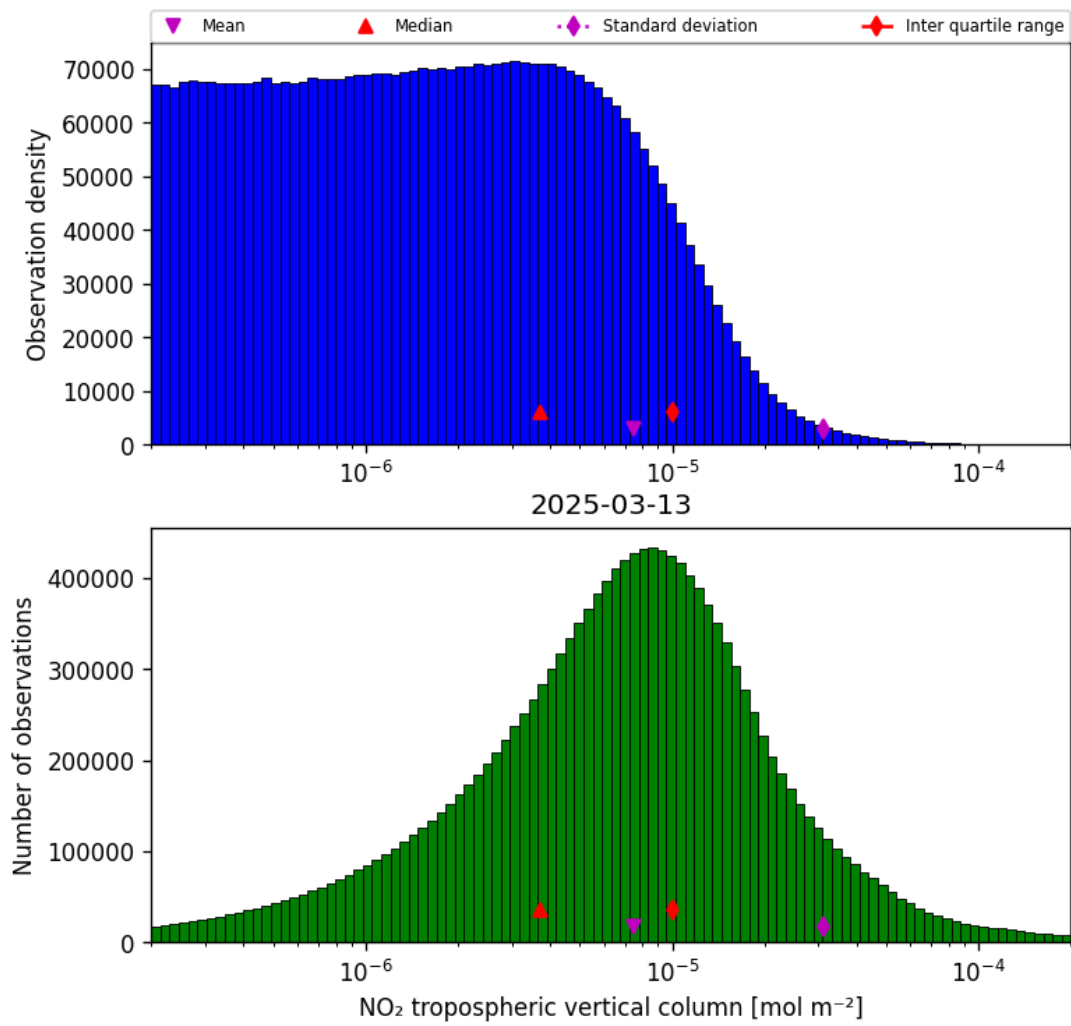
Figure 29: Histogram of “NO 2 tropospheric vertical column” for 2025-03-13 to 2025-03-14
