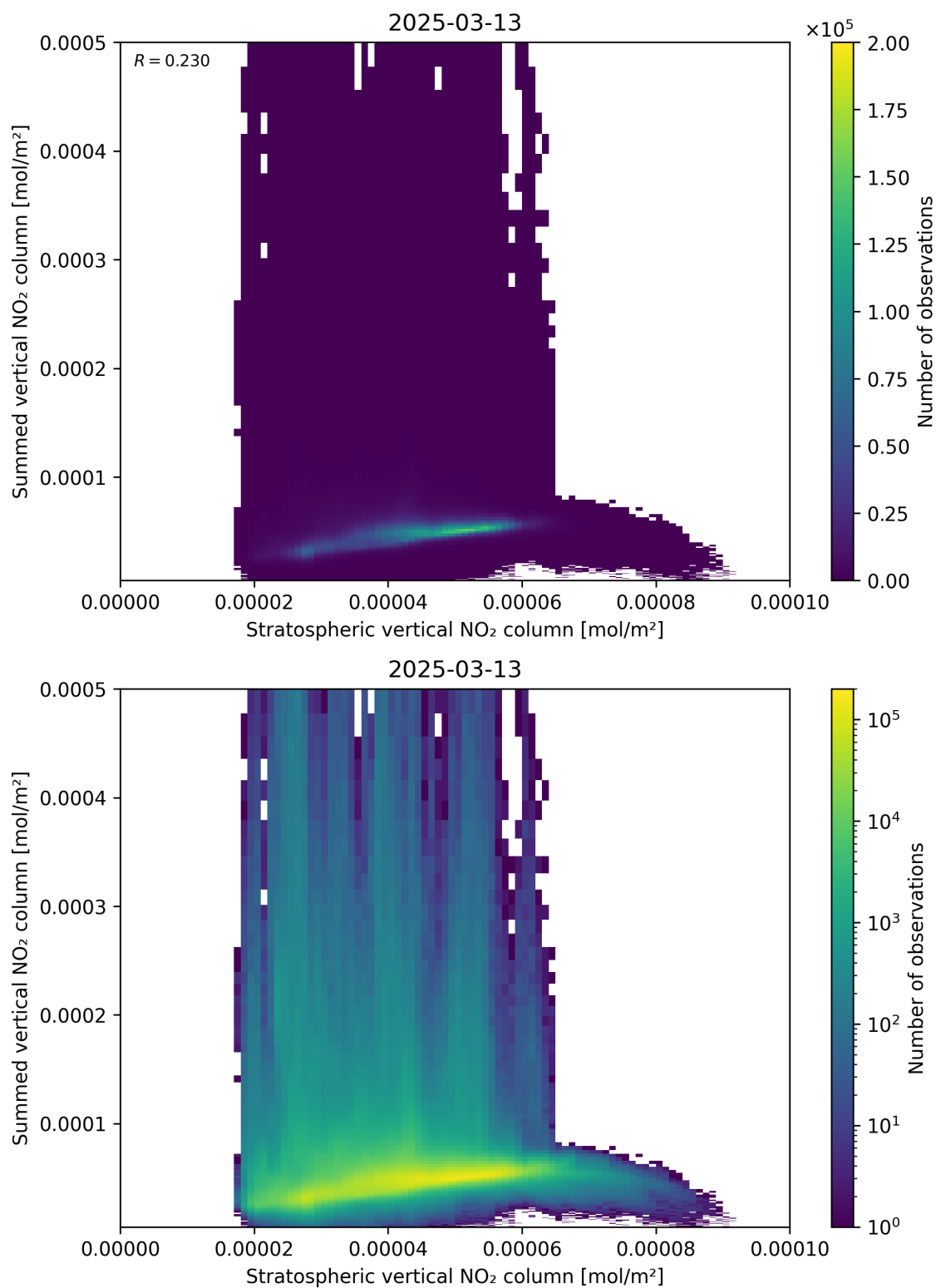
Figure 98: Scatter density plot of “Stratospheric vertical NO 2 column” against “Summed vertical NO 2 column” for 2025-03-13 to 2025-03-14.
