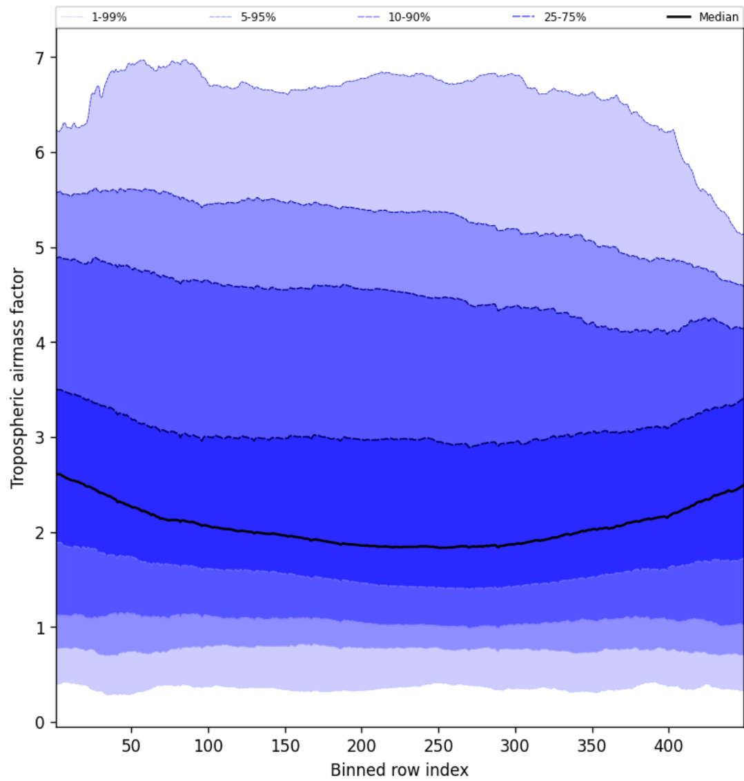
Figure 48: Along track statistics of “Tropospheric air mass factor” for 2025-03-13 to 2025-03-14
