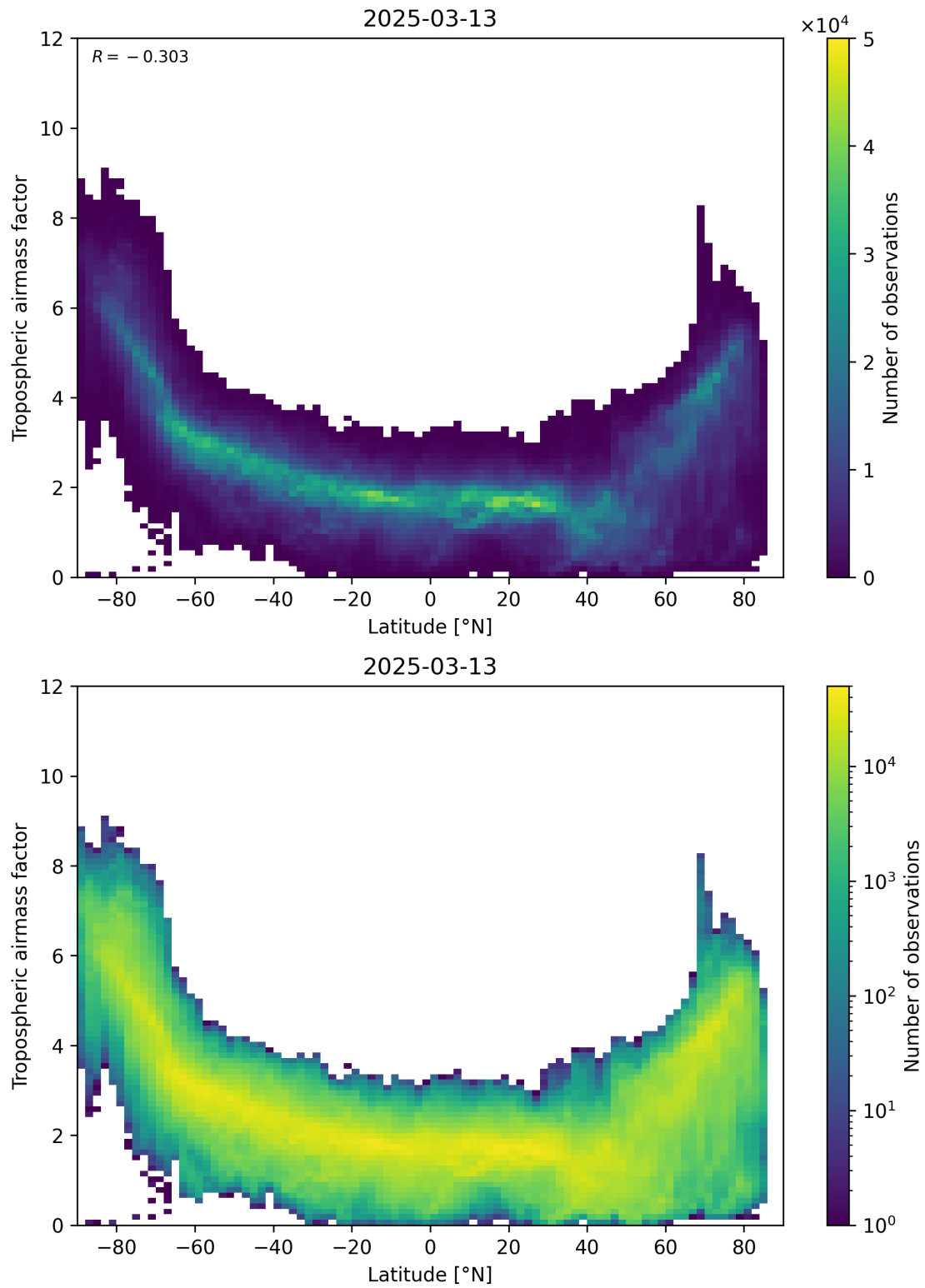
Figure 85: Scatter density plot of “Latitude” against “Tropospheric airmass factor” for 2025-03-13 to 2025-03-14.
