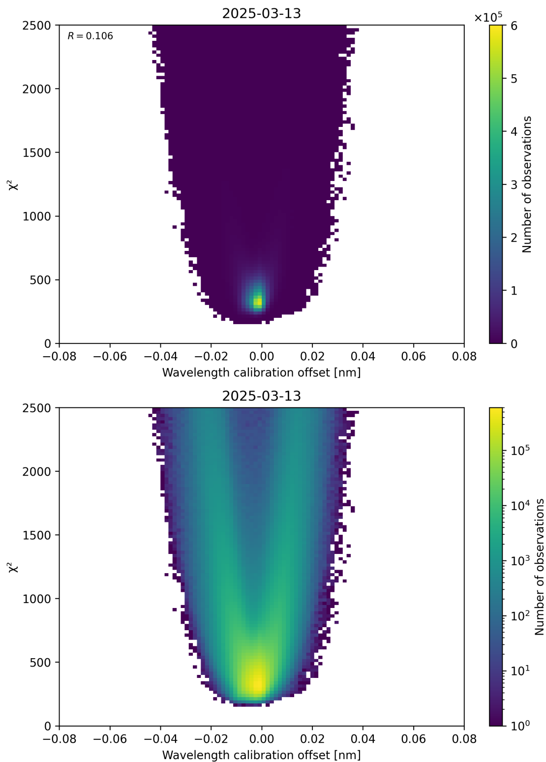
Figure 175: Scatter density plot of “Wavelength calibration offset” against “ \chi^2 ” for 2025-03-13 to 2025-03-14.
