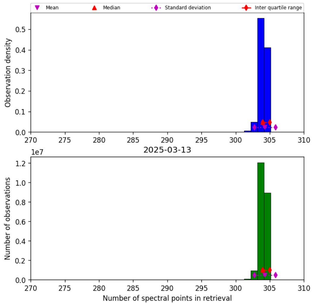
Figure 33: Histogram of “Number of spectral points in retrieval” for 2025-03-13 to 2025-03-14
