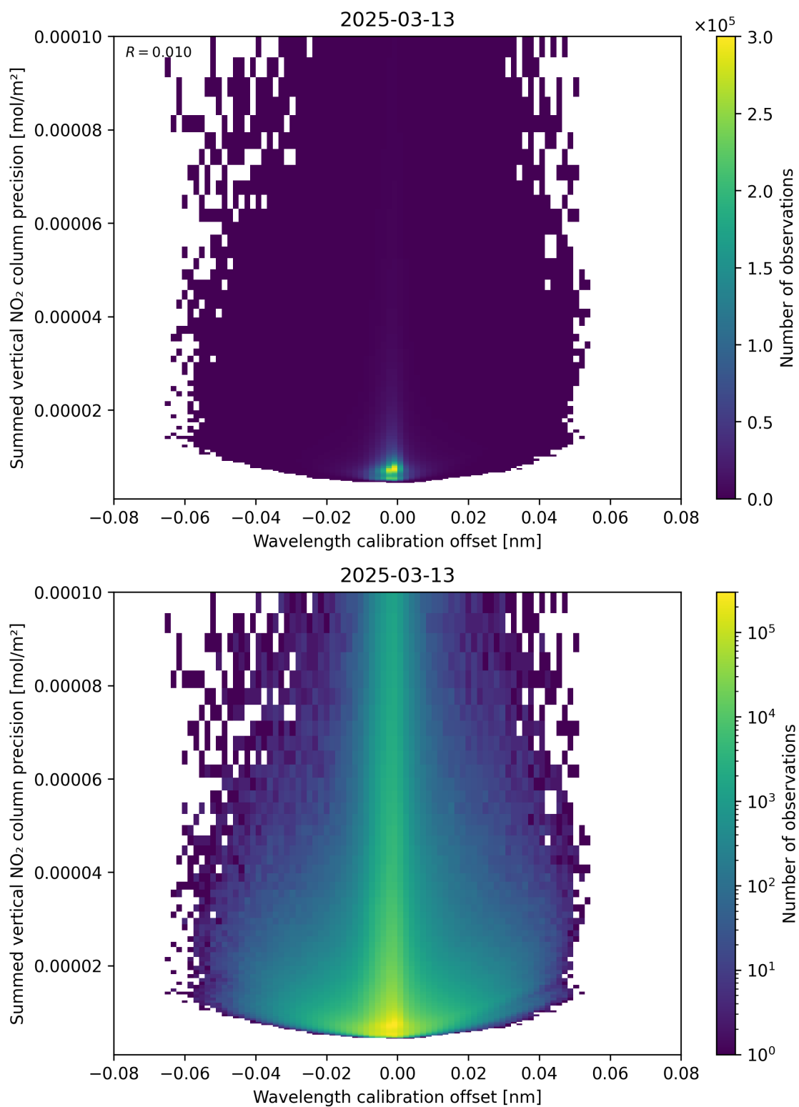
Figure 178: Scatter density plot of “Wavelength calibration offset” against “Summed vertical NO 2 column precision” for 2025-03-13 to 2025-03-14.
