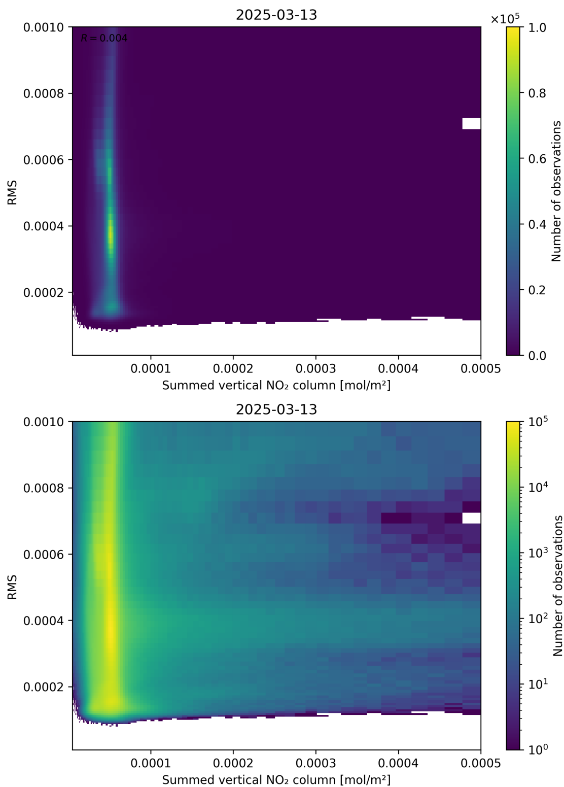
Figure 109: Scatter density plot of “Summed vertical NO 2 column” against “RMS” for 2025-03-13 to 2025-03-14.
