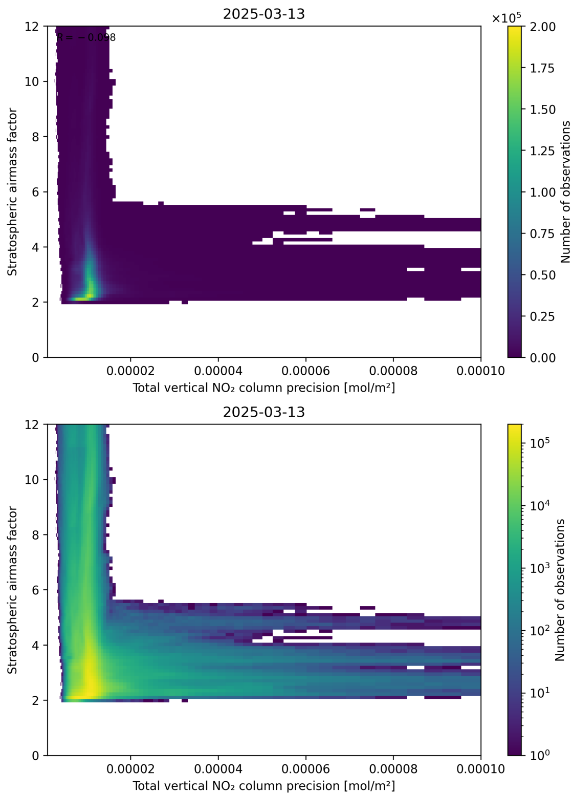
Figure 115: Scatter density plot of “Total vertical NO 2 column precision” against “Stratospheric air mass factor” for 2025-03-13 to 2025-03-14.
