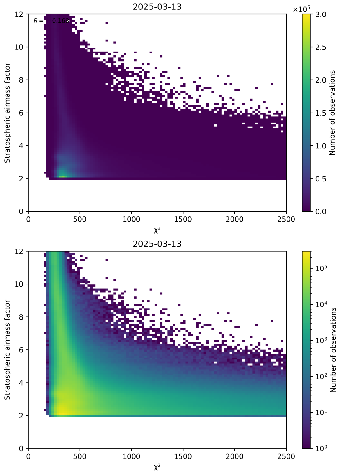
Figure 81: Scatter density plot of “ \chi^2 ” against “Stratospheric airmass factor” for 2025-03-13 to 2025-03-14.
