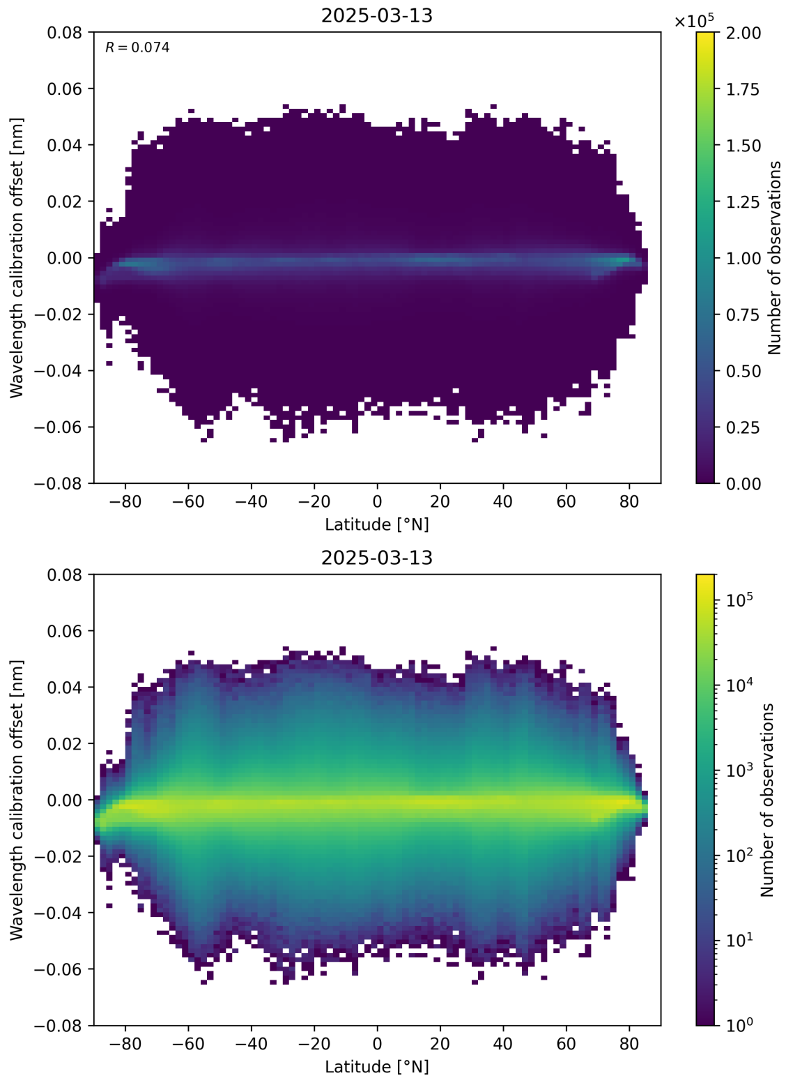
Figure 95: Scatter density plot of “Latitude” against “Wavelength calibration offset” for 2025-03-13 to 2025-03-14.
