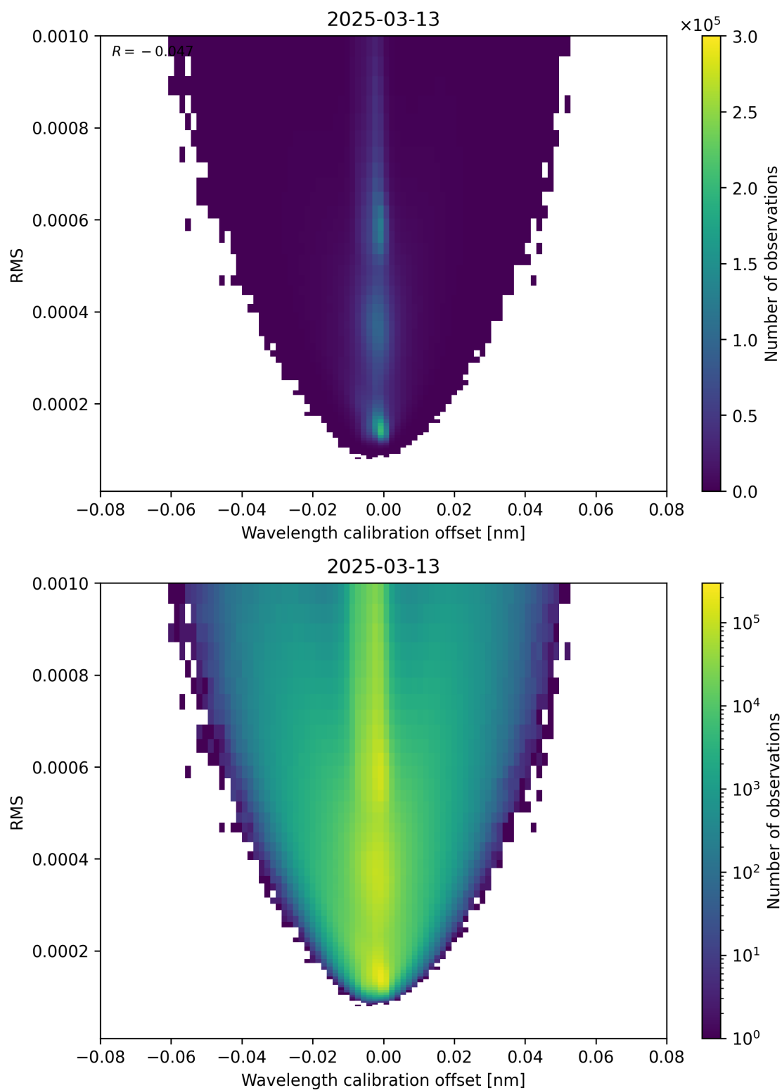
Figure 181: Scatter density plot of “Wavelength calibration offset” against “RMS” for 2025-03-13 to 2025-03-14.
