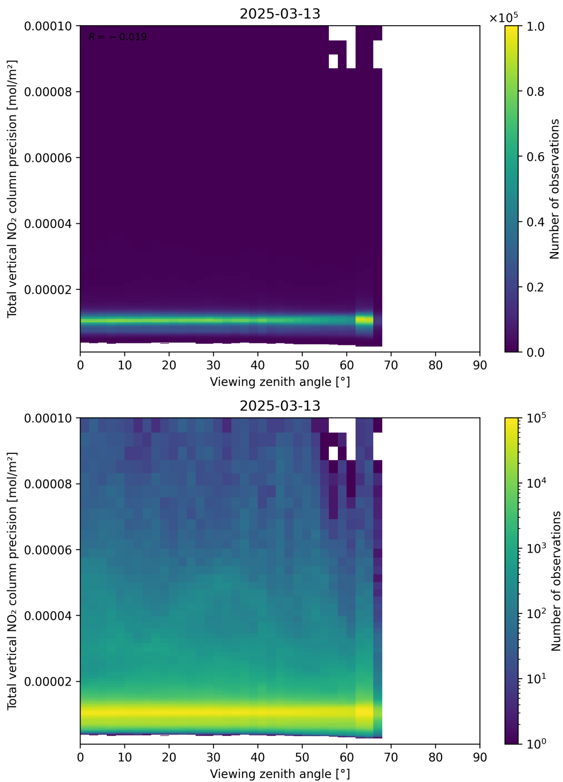
Figure 168: Scatter density plot of “Viewing zenith angle” against “Total vertical NO 2 column precision” for 2025-03-13 to 2025-03-14.
