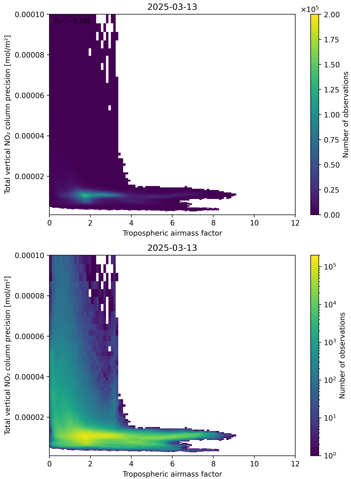
Figure 78: Scatter density plot of “Tropospheric airmass factor” against “Total vertical NO 2 column precision” for 2025-03-13 to 2025-03-14.
