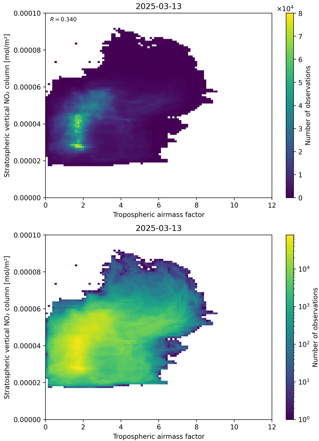
Figure 74: Scatter density plot of “Tropospheric airmass factor” against “Stratospheric vertical NO 2 column” for 2025-03-13 to 2025-03-14.
