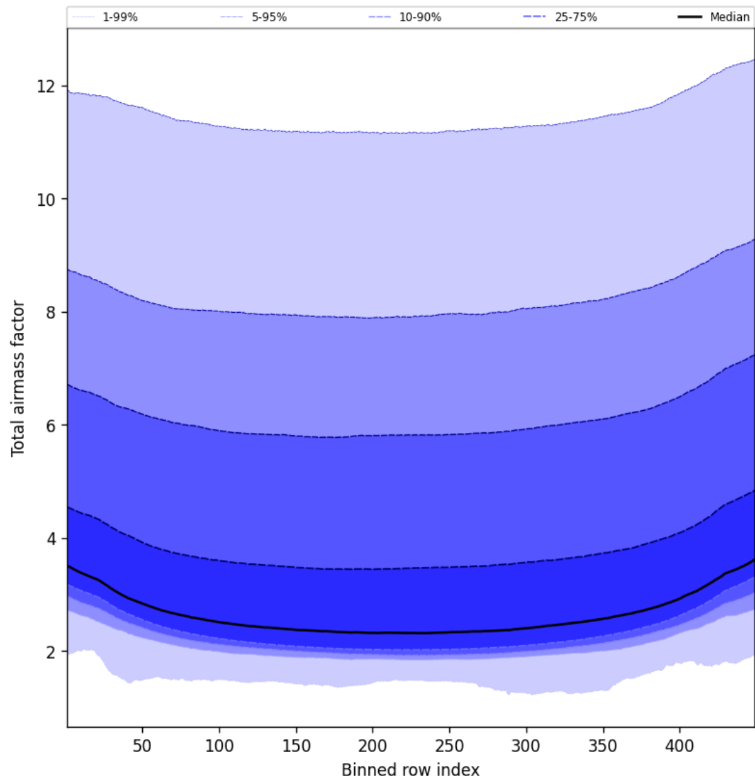
Figure 49: Along track statistics of “Total airmass factor” for 2025-03-13 to 2025-03-14
