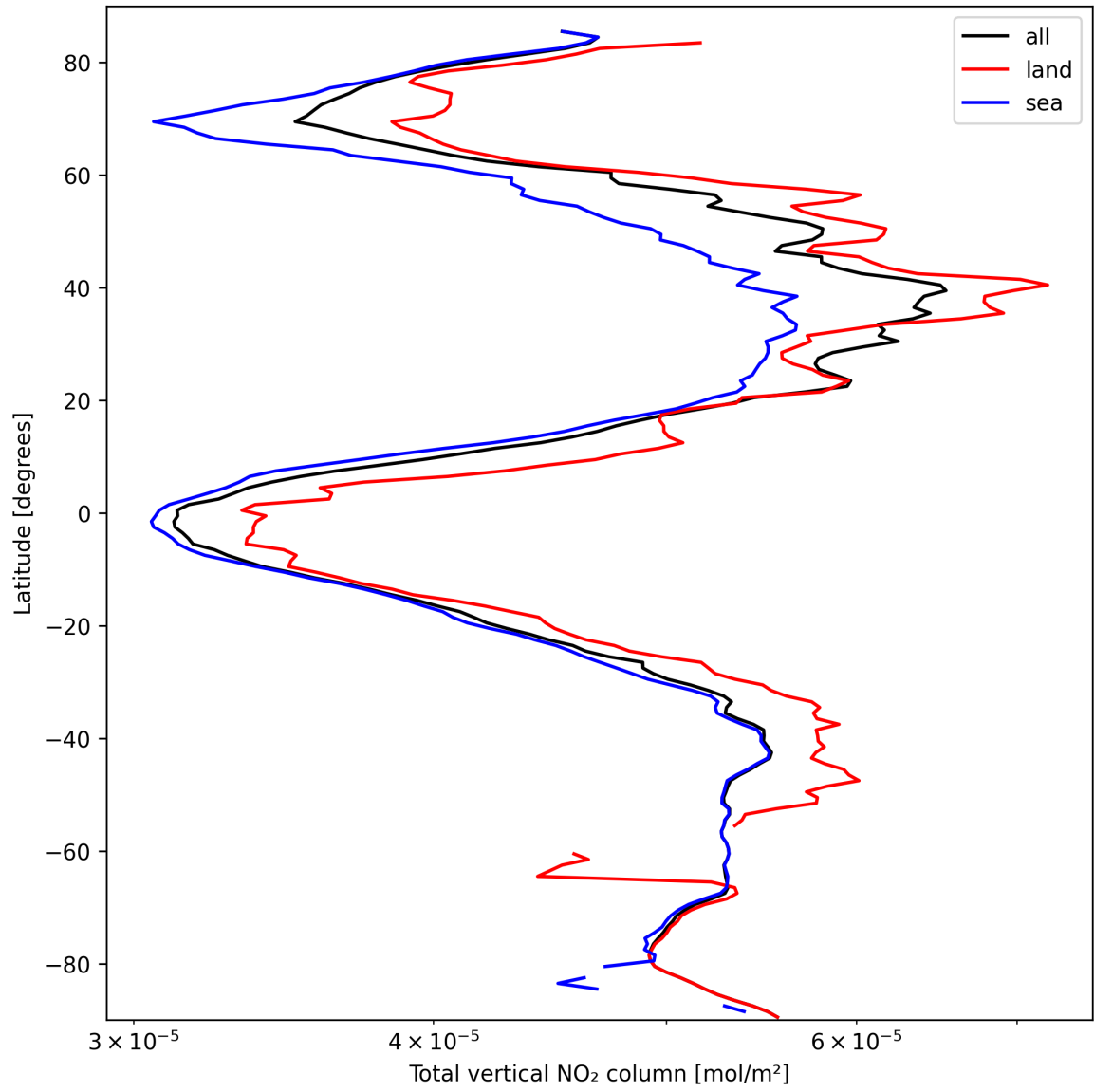
Figure 21: Zonal average of “Total vertical NO 2 column” for 2025-03-13 to 2025-03-14.
