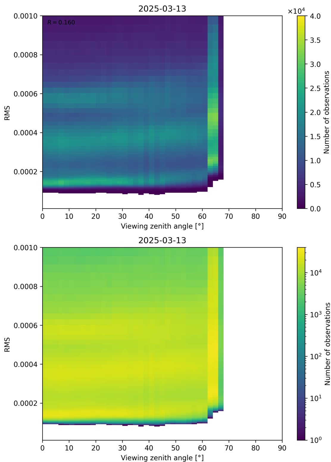
Figure 171: Scatter density plot of “Viewing zenith angle” against “RMS” for 2025-03-13 to 2025-03-14.
