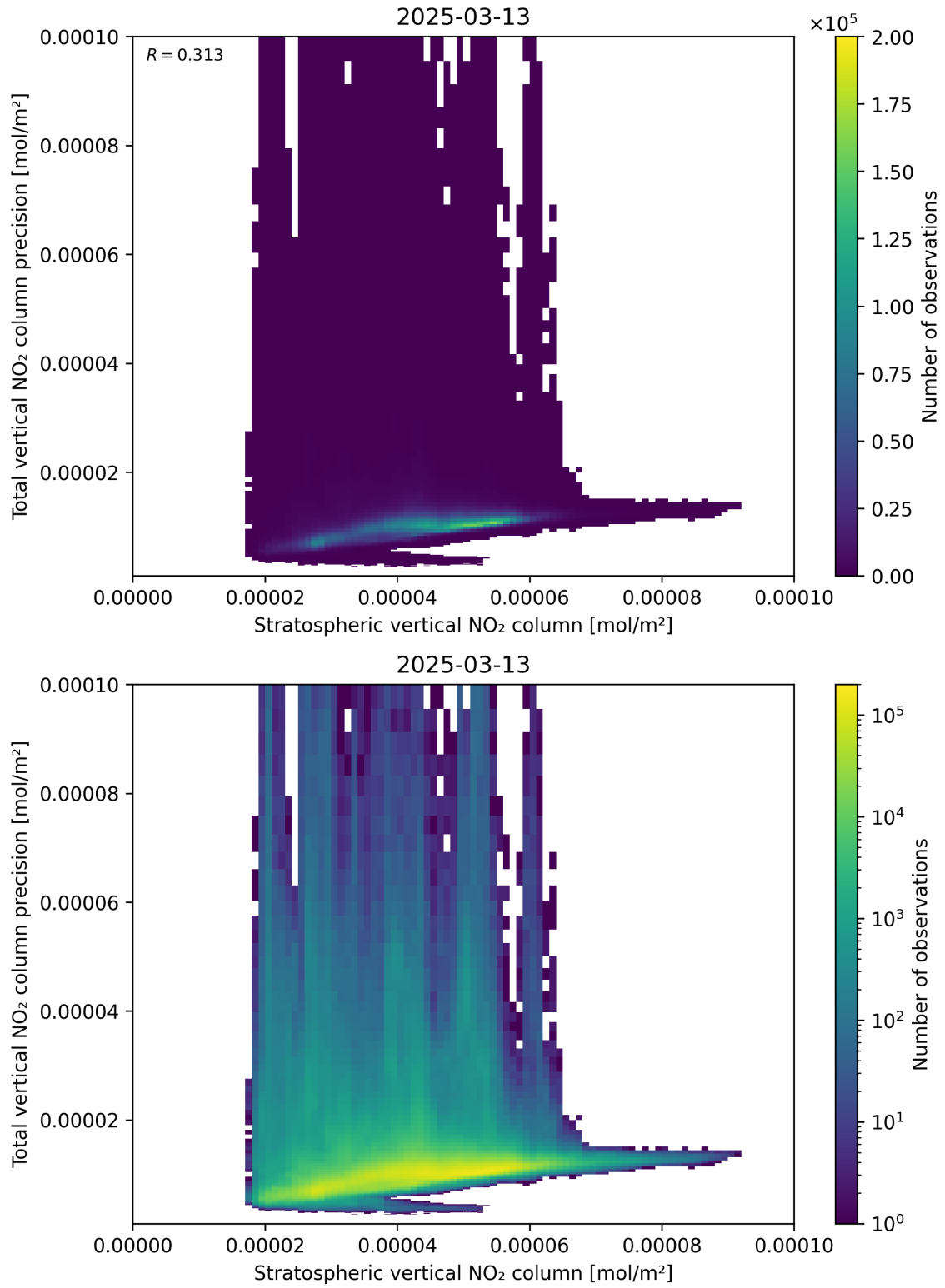
Figure 101: Scatter density plot of “Stratospheric vertical NO 2 column” against “Total vertical NO 2 column precision” for 2025-03-13 to 2025-03-14.
