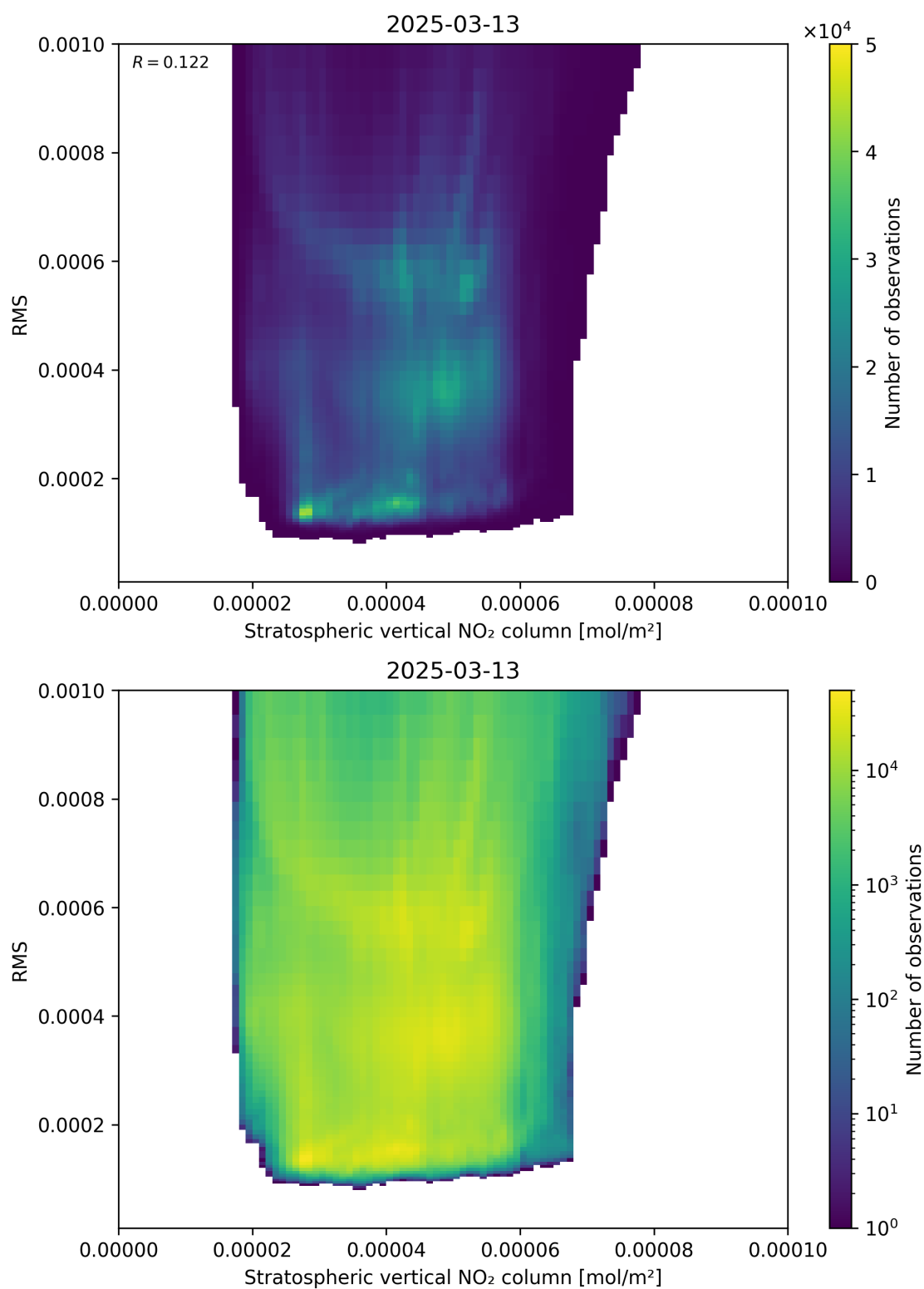
Figure 102: Scatter density plot of “Stratospheric vertical NO 2 column” against “RMS” for 2025-03-13 to 2025-03-14.
