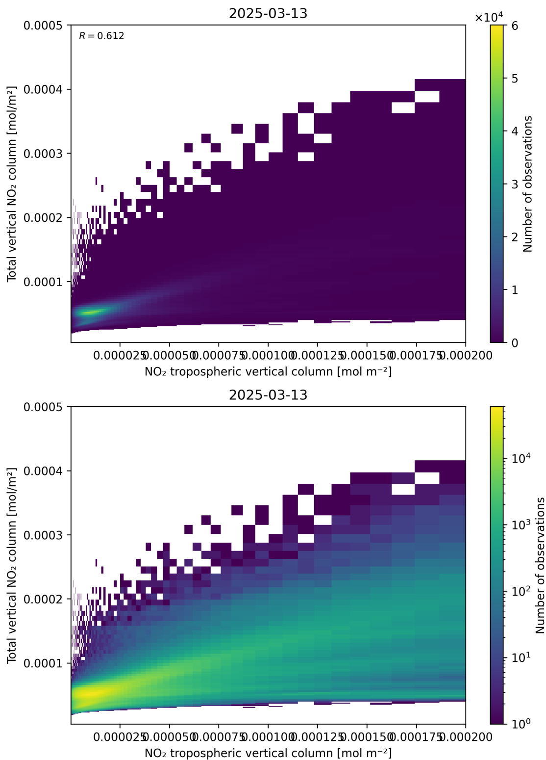
Figure 128: Scatter density plot of “NO 2 tropospheric vertical column” against “Total vertical NO 2 column” for 2025-03-13 to 2025-03-14.
