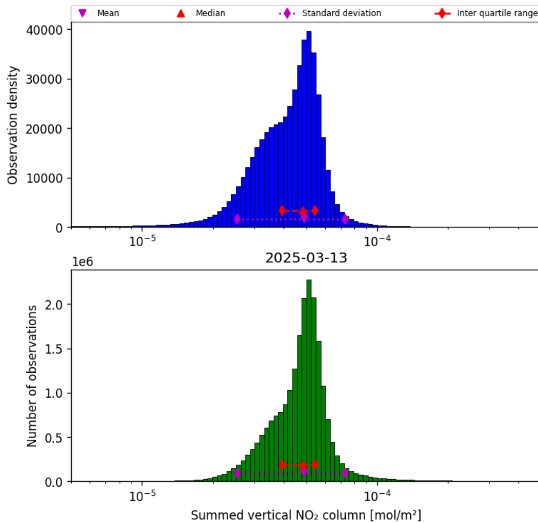
Figure 40: Histogram of “Summed vertical NO 2 column” for 2025-03-13 to 2025-03-14
