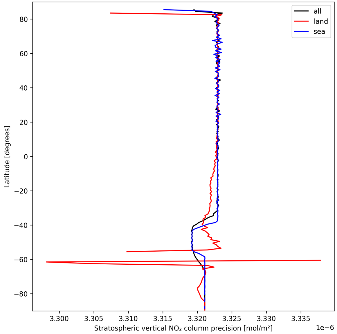
Figure 20: Zonal average of “Stratospheric vertical NO 2 column precision” for 2025-03-13 to 2025-03-14.
