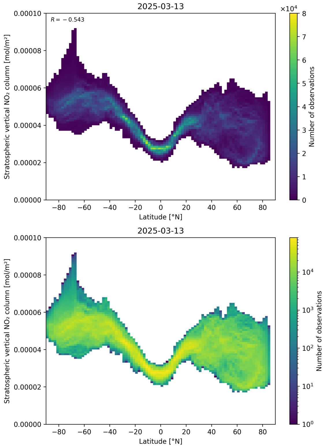
Figure 87: Scatter density plot of “Latitude” against “Stratospheric vertical NO 2 column” for 2025-03-13 to 2025-03-14.
