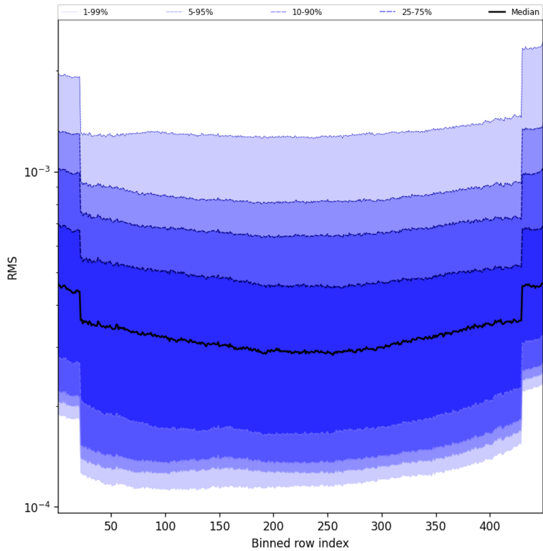
Figure 60: Along track statistics of “RMS” for 2025-03-13 to 2025-03-14
