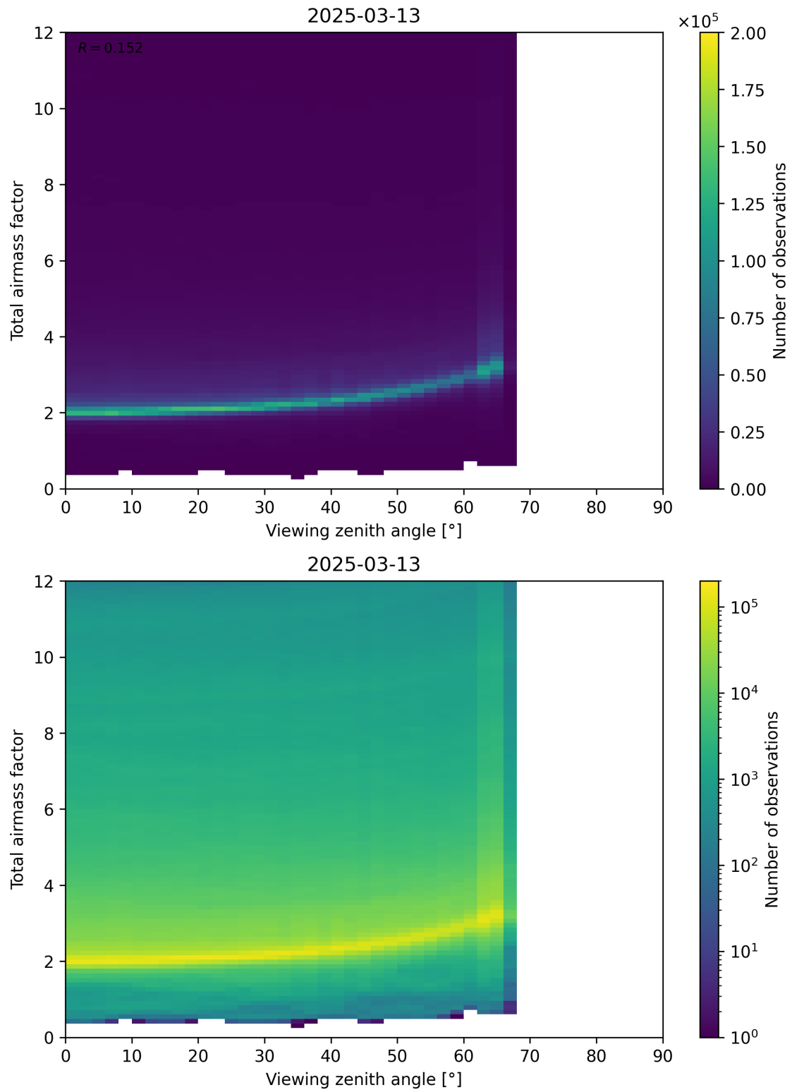
Figure 160: Scatter density plot of “Viewing zenith angle” against “Total airmass factor” for 2025-03-13 to 2025-03-14.
