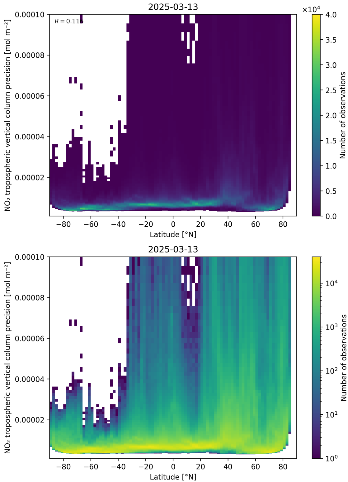
Figure 93: Scatter density plot of “Latitude” against “NO 2 tropospheric vertical column precision” for 2025-03-13 to 2025-03-14.
