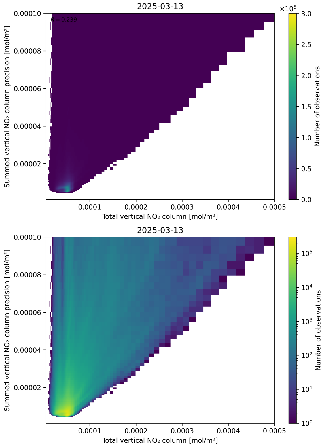
Figure 113: Scatter density plot of “Total vertical NO 2 column” against “Summed vertical NO 2 column precision” for 2025-03-13 to 2025-03-14.
