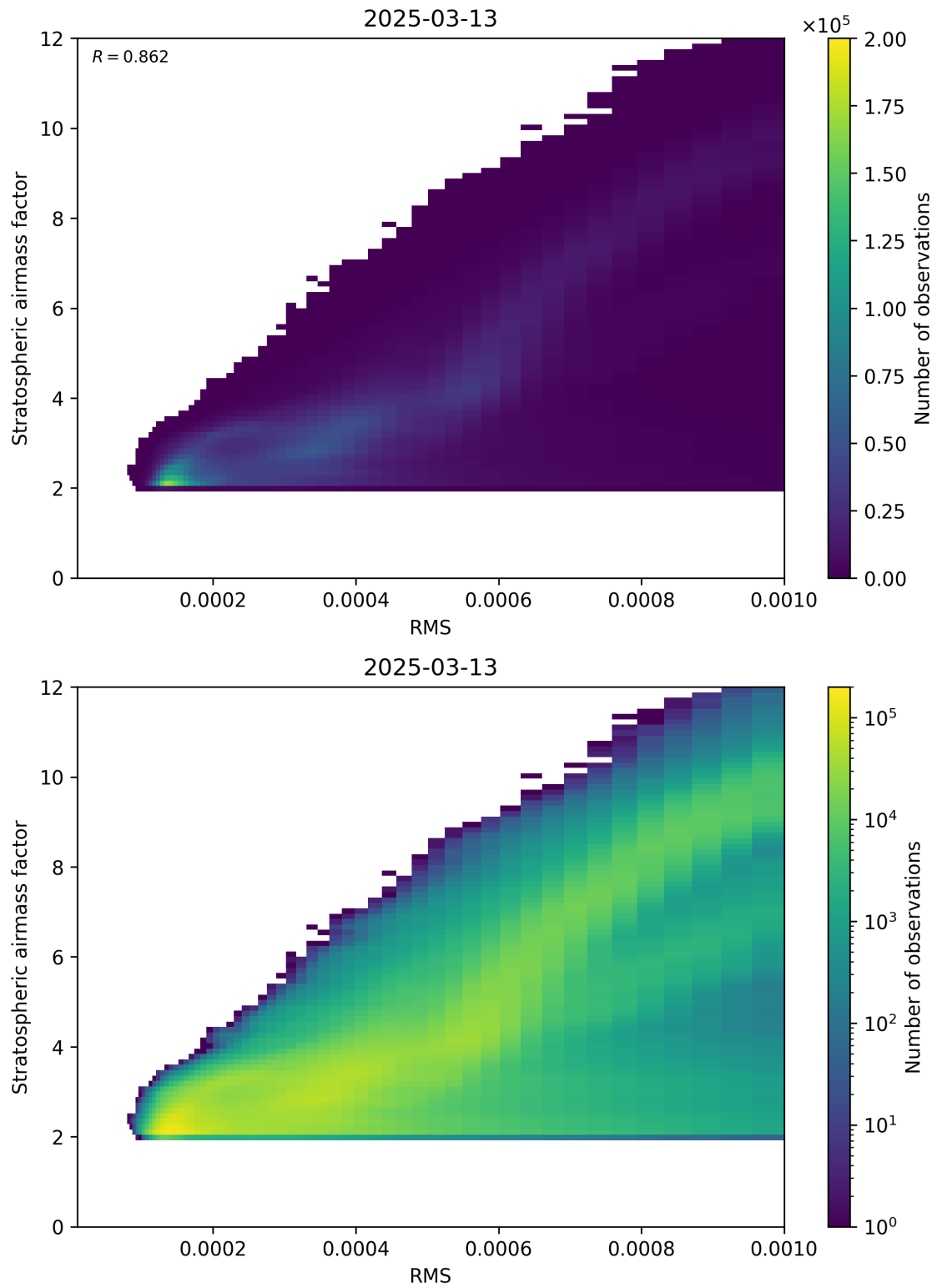
Figure 144: Scatter density plot of “RMS” against “Stratospheric airmass factor” for 2025-03-13 to 2025-03-14.
