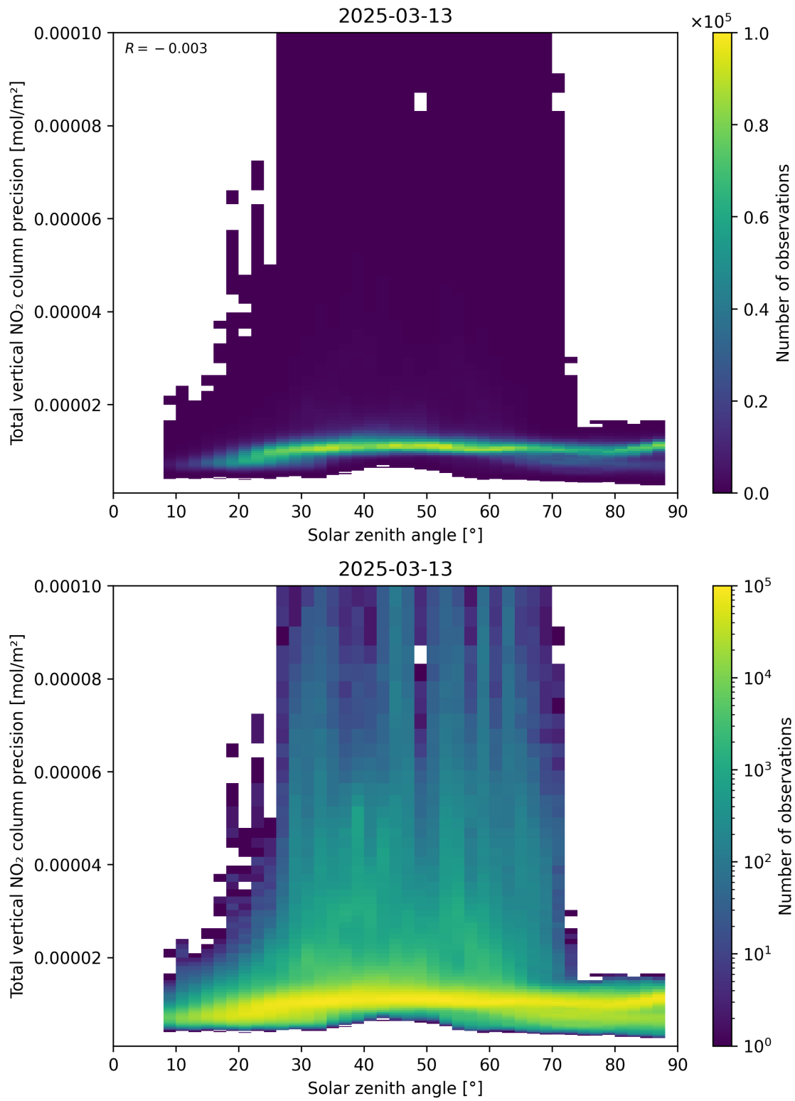
Figure 154: Scatter density plot of “Solar zenith angle” against “Total vertical NO 2 column precision” for 2025-03-13 to 2025-03-14.
