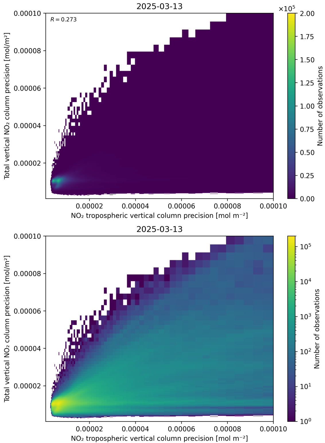
Figure 139: Scatter density plot of “NO 2 tropospheric vertical column precision” against “Total vertical NO 2 column precision” for 2025-03-13 to 2025-03-14.
