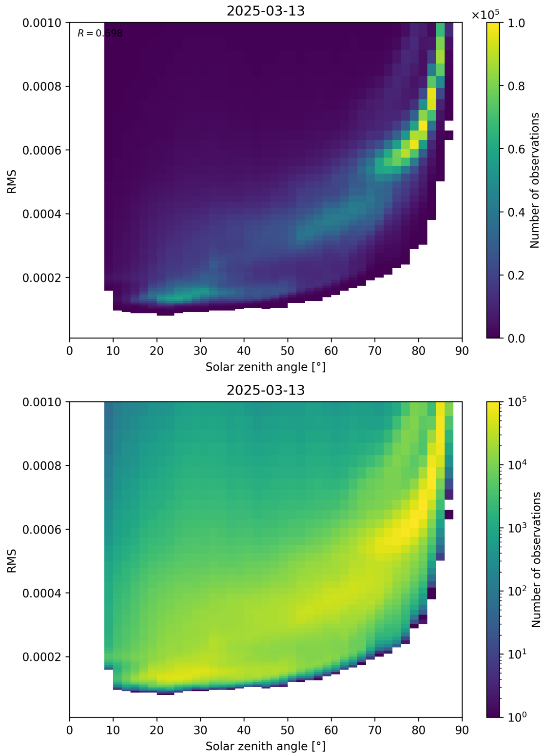
Figure 157: Scatter density plot of “Solar zenith angle” against “RMS” for 2025-03-13 to 2025-03-14.
