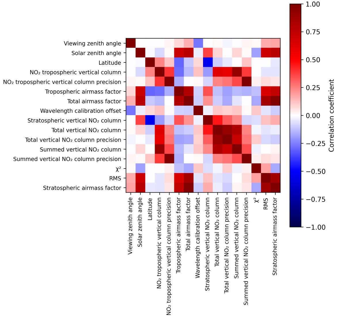
Figure 2: Map of correlation matrix for 2025-03-13 to 2025-03-14.
