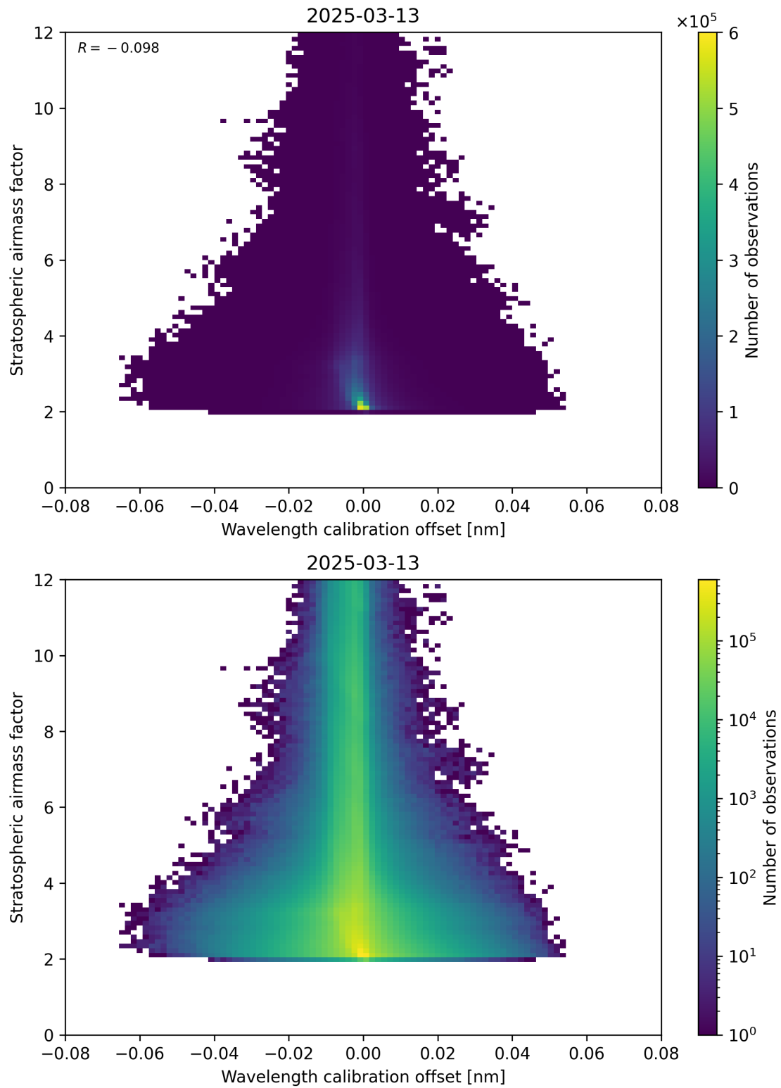
Figure 174: Scatter density plot of “Wavelength calibration offset” against “Stratospheric airmass factor” for 2025-03-13 to 2025-03-14.
