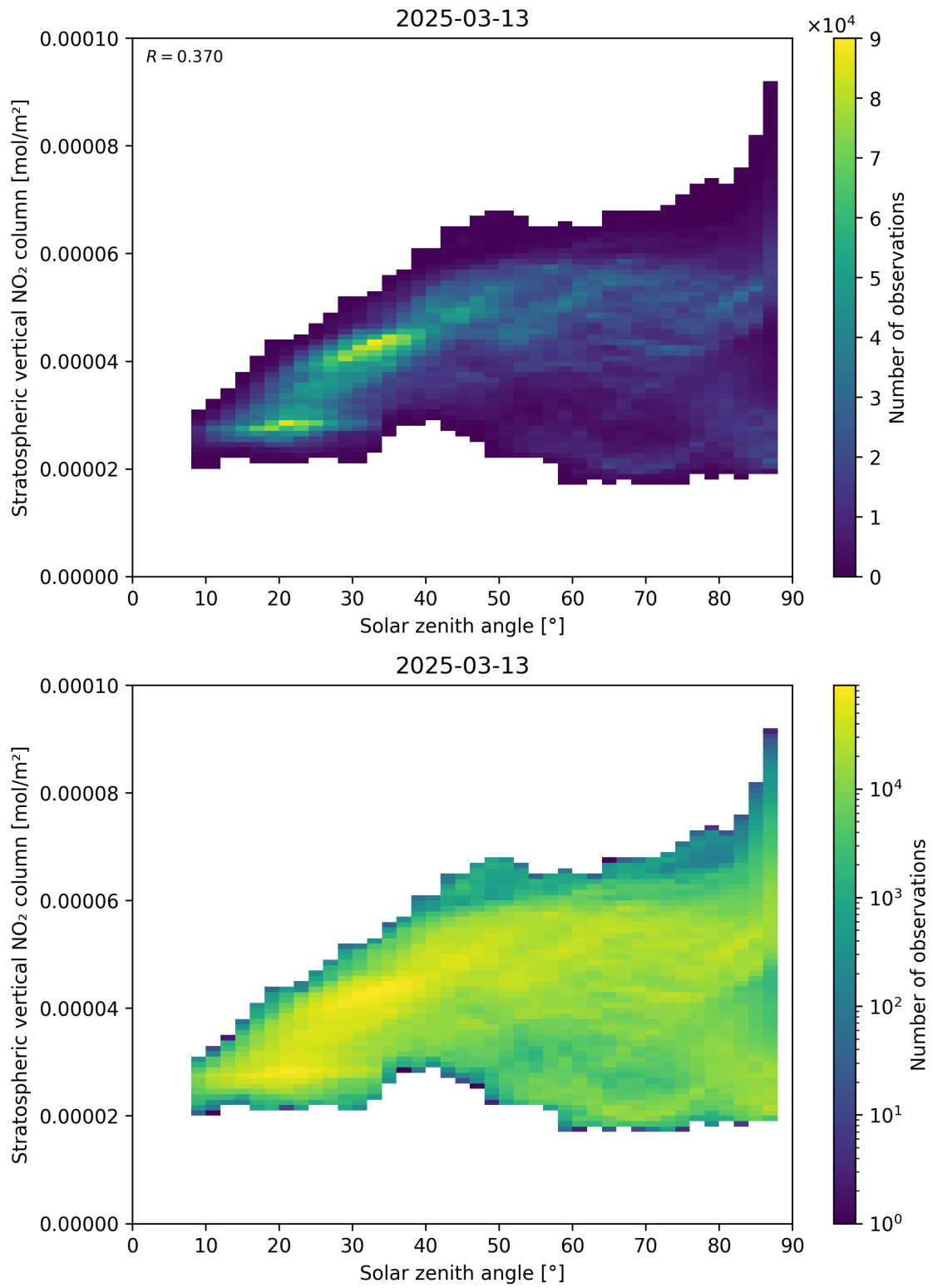
Figure 150: Scatter density plot of “Solar zenith angle” against “Stratospheric vertical NO 2 column” for 2025-03-13 to 2025-03-14.
