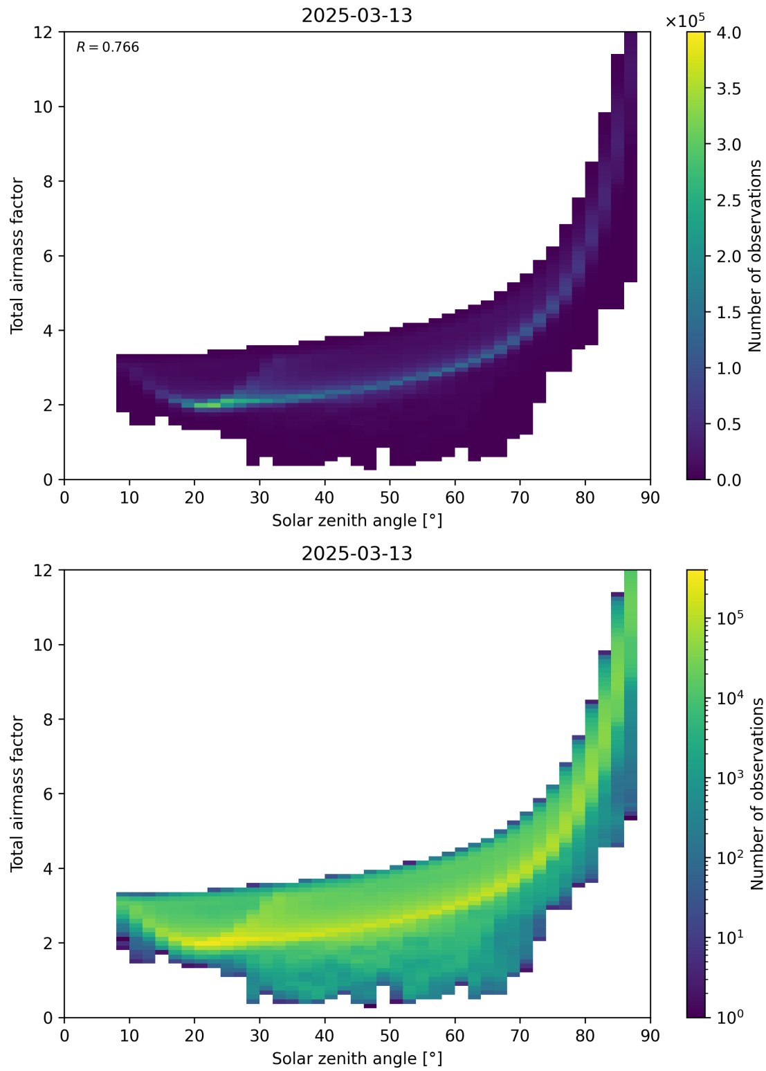
Figure 146: Scatter density plot of “Solar zenith angle” against “Total air mass factor” for 2025-03-13 to 2025-03-14.
