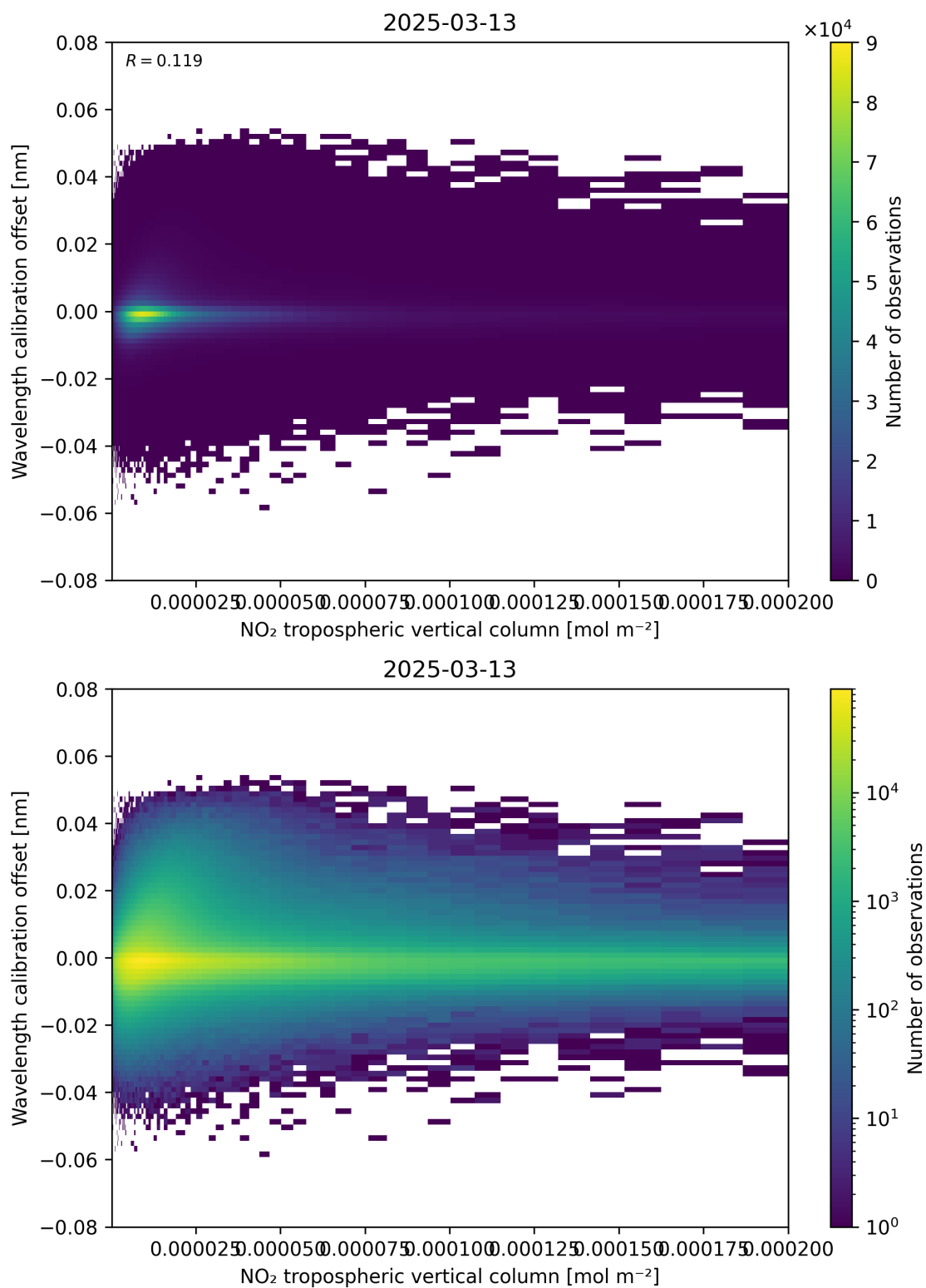
Figure 143: Scatter density plot of “NO 2 tropospheric vertical column” against “Wavelength calibration offset” for 2025-03-13 to 2025-03-14.
