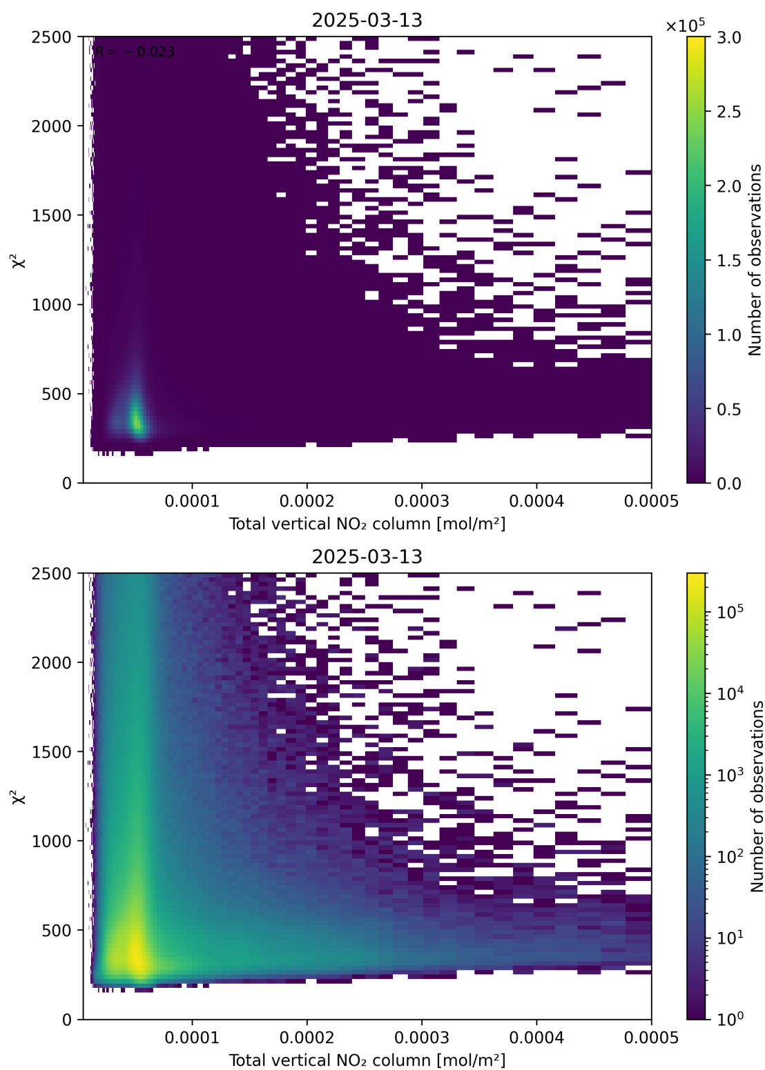
Figure 111: Scatter density plot of “Total vertical NO 2 column” against “ \chi^2 ” for 2025-03-13 to 2025-03-14.
