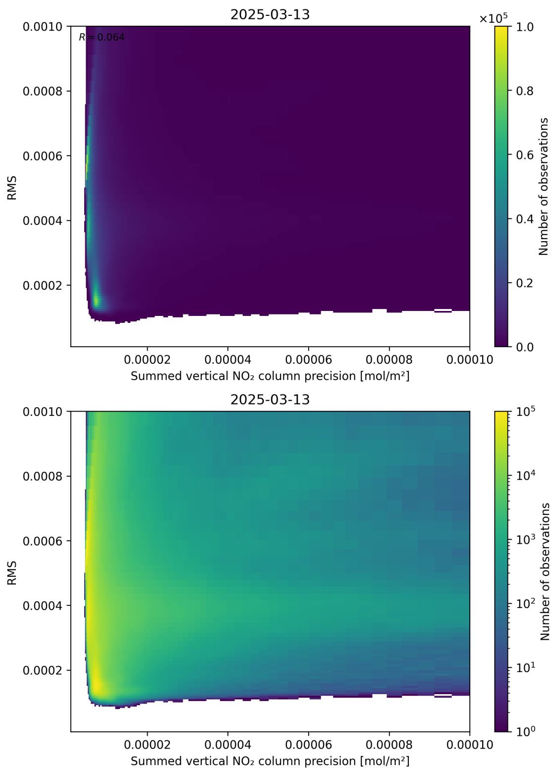
Figure 108: Scatter density plot of “Summed vertical NO 2 column precision” against “RMS” for 2025-03-13 to 2025-03-14.
