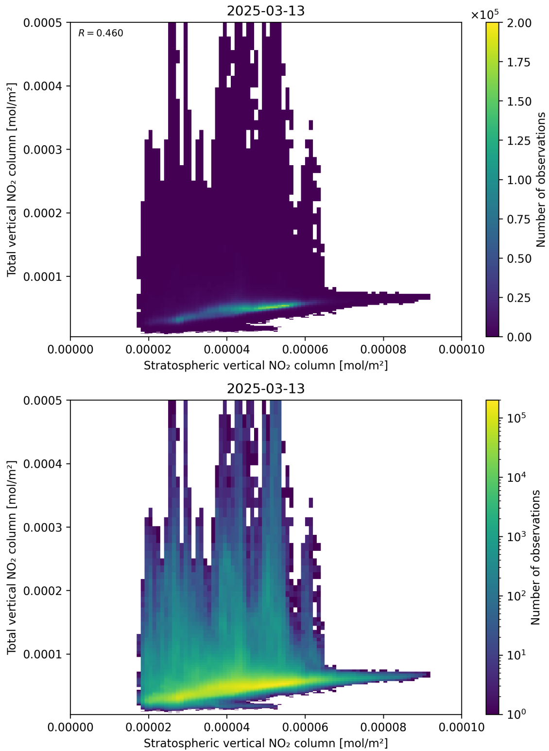
Figure 100: Scatter density plot of “Stratospheric vertical NO 2 column” against “Total vertical NO 2 column” for 2025-03-13 to 2025-03-14.
