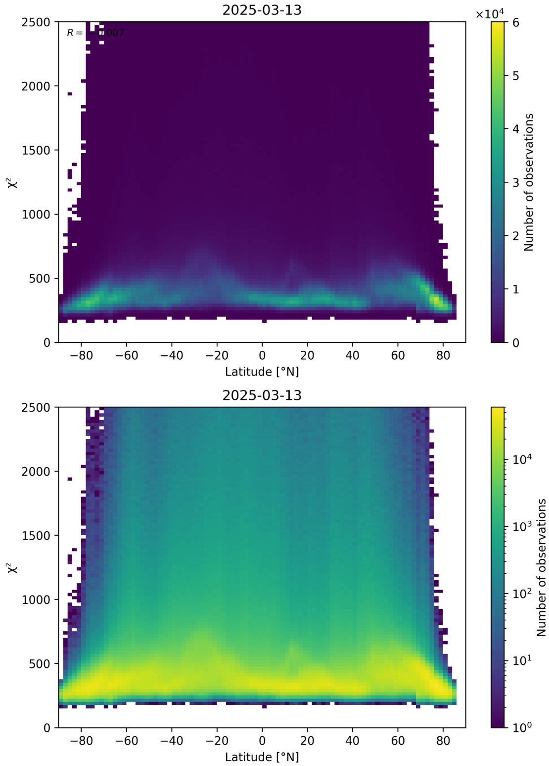
Figure 86: Scatter density plot of “Latitude” against “ \chi^2 ” for 2025-03-13 to 2025-03-14.
