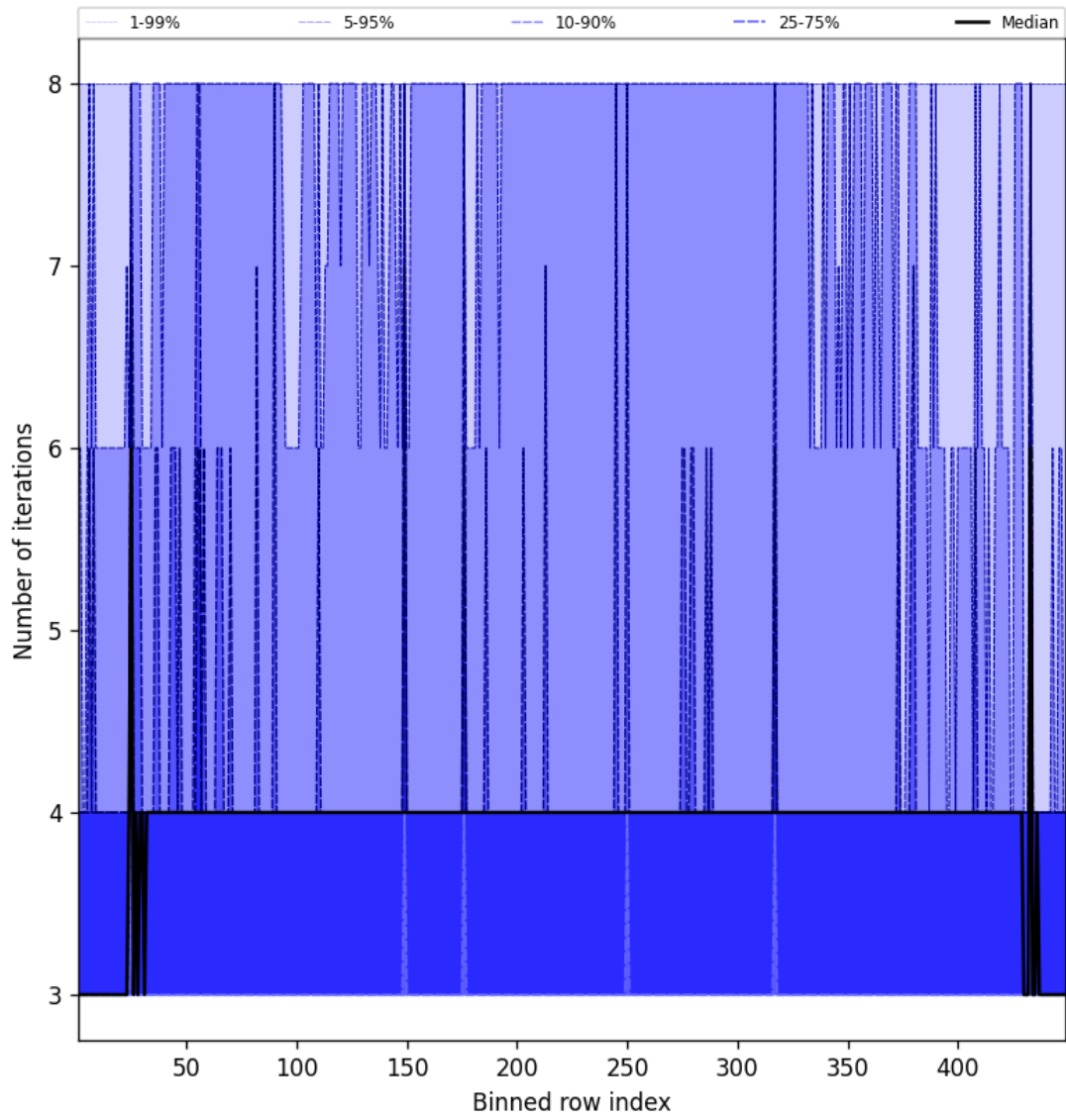
Figure 51: Along track statistics of “Number of iterations” for 2025-03-13 to 2025-03-14
