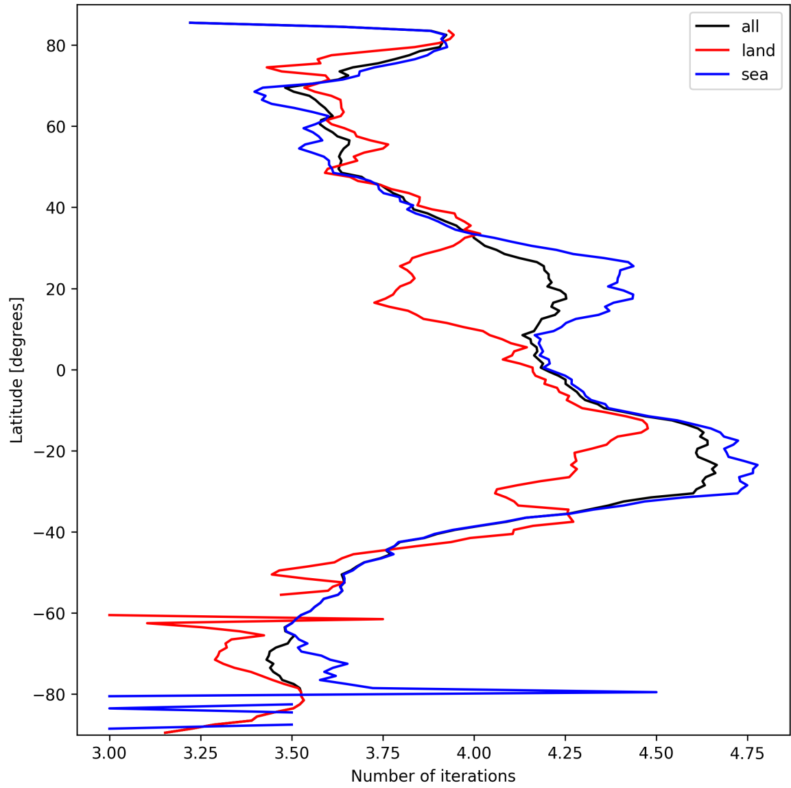
Figure 17: Zonal average of “Number of iterations” for 2025-03-13 to 2025-03-14.
