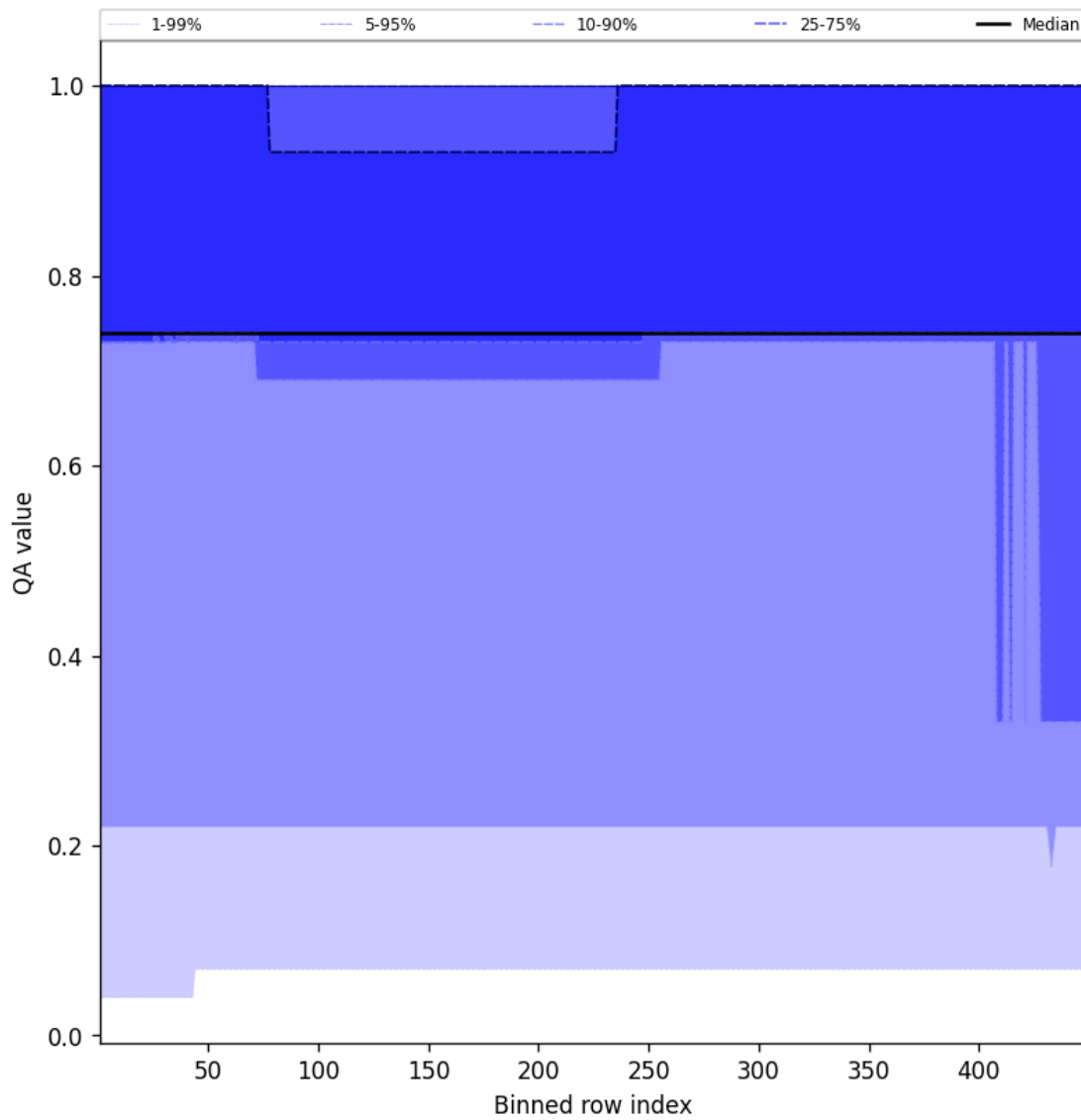
Figure 45: Along track statistics of "QA value" for 2025-03-13 to 2025-03-14
