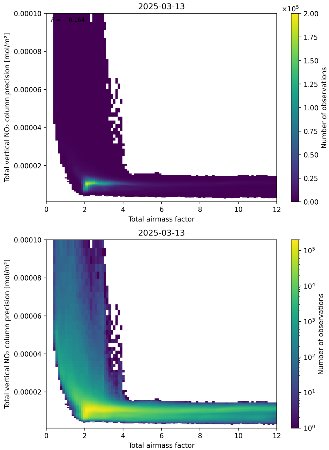
Figure 68: Scatter density plot of “Total airmass factor” against “Total vertical NO 2 column precision” for 2025-03-13 to 2025-03-14.
