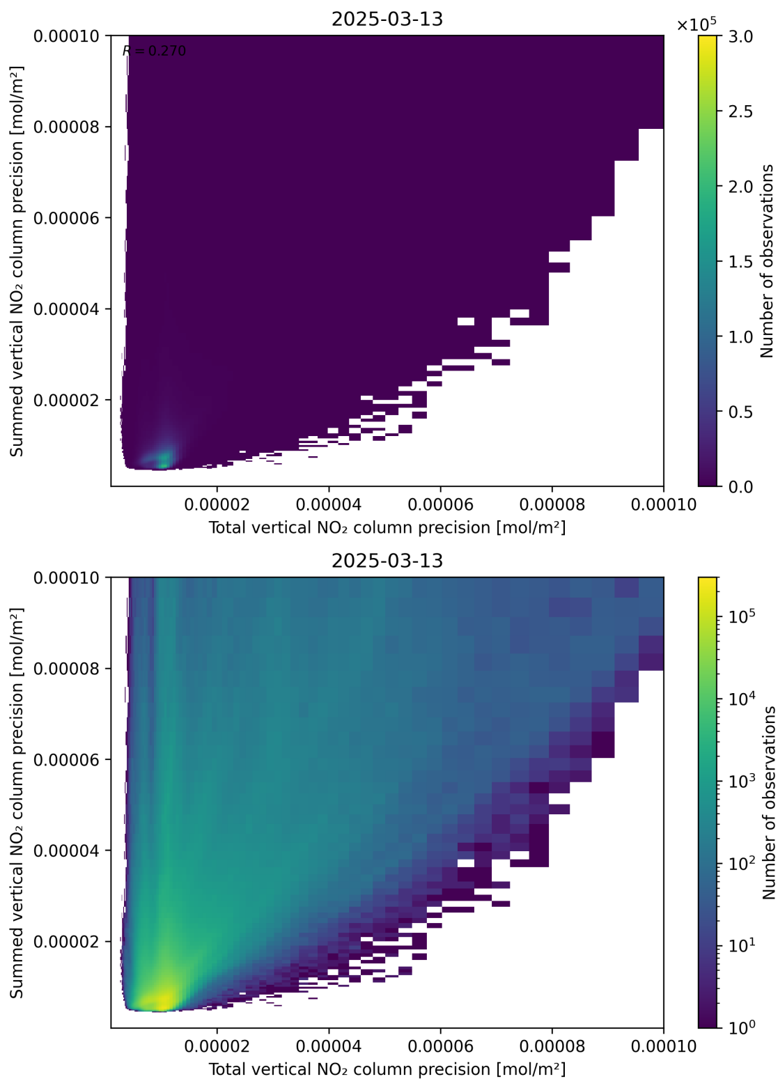
Figure 118: Scatter density plot of “Total vertical NO 2 column precision” against “Summed vertical NO 2 column precision” for 2025-03-13 to 2025-03-14.
