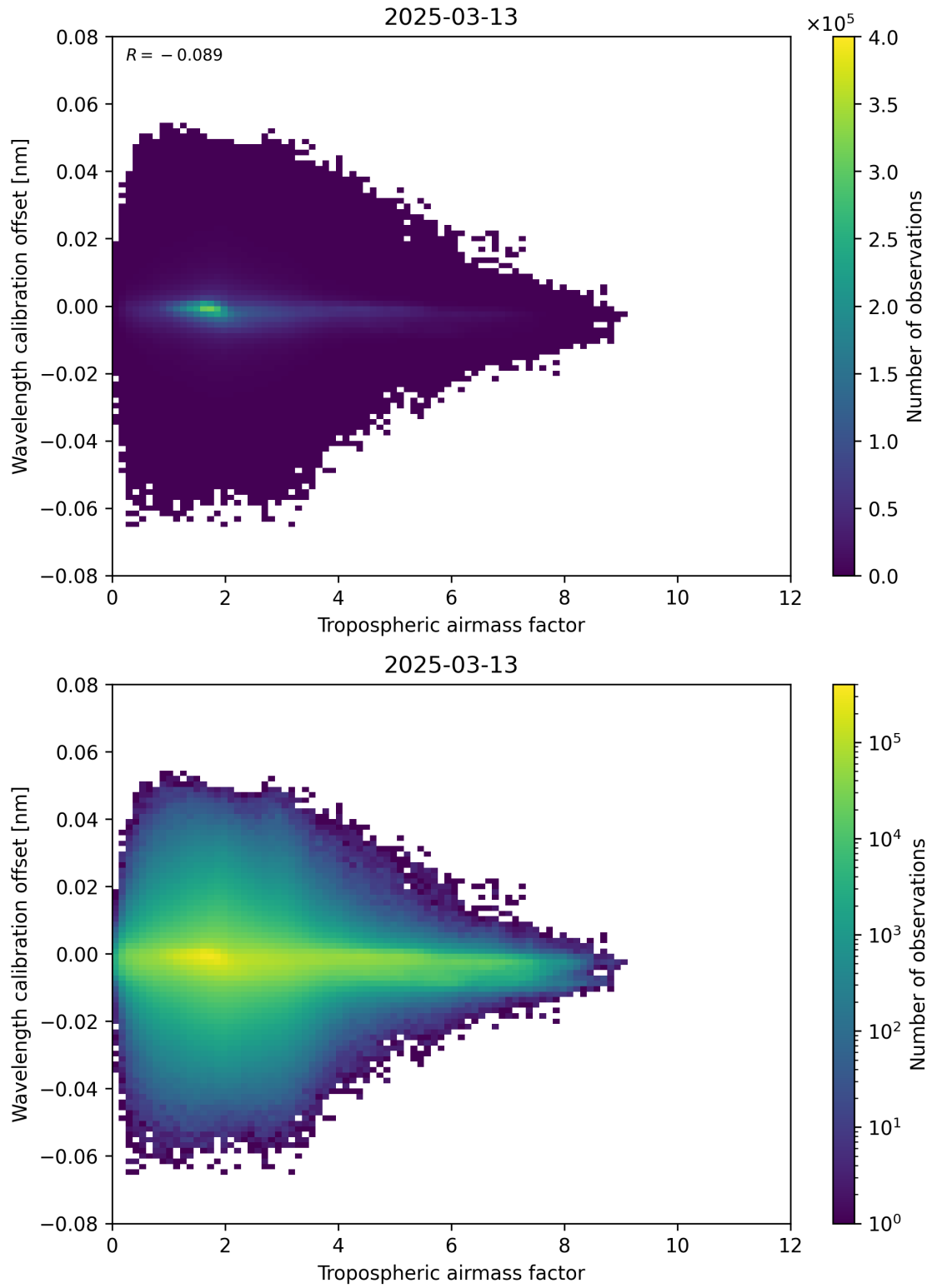
Figure 80: Scatter density plot of “Tropospheric airmass factor” against “Wavelength calibration offset” for 2025-03-13 to 2025-03-14.
