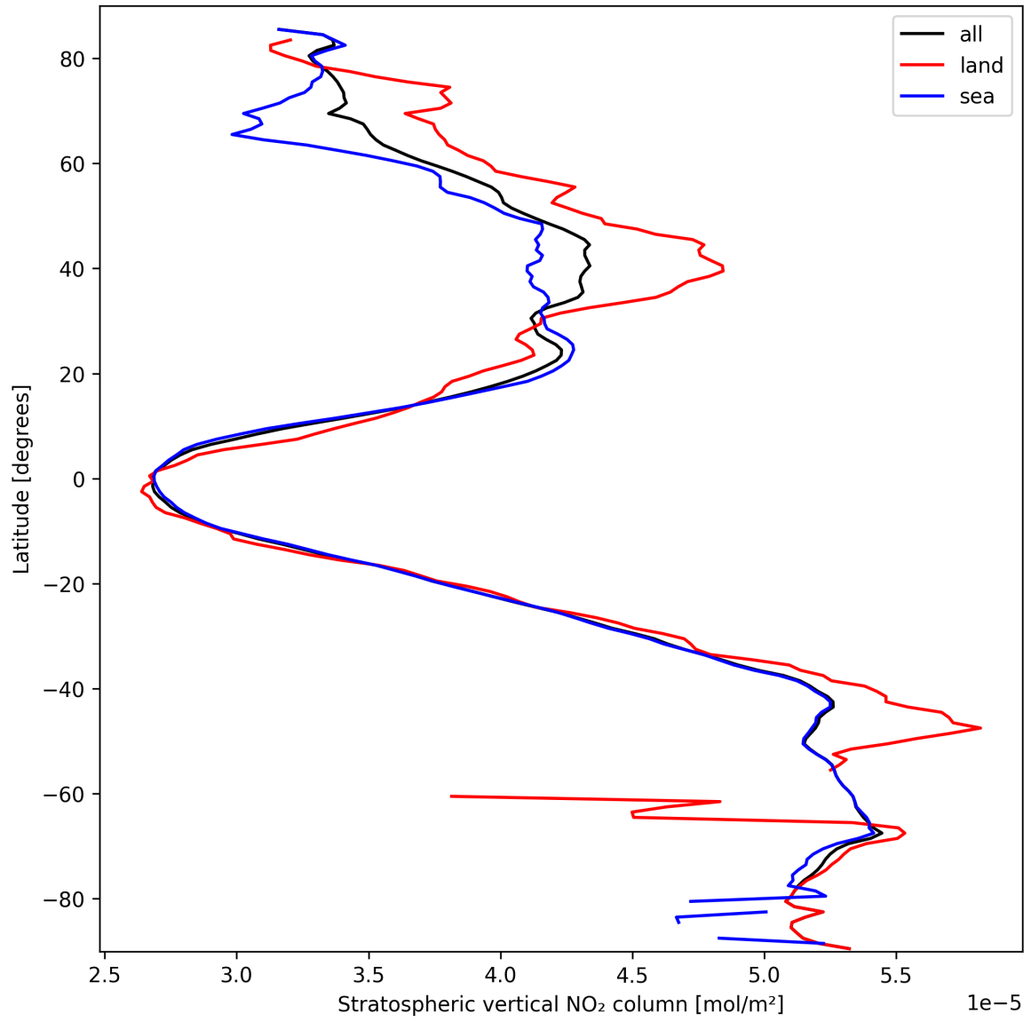
Figure 19: Zonal average of “Stratospheric vertical NO 2 column” for 2025-03-13 to 2025-03-14.
