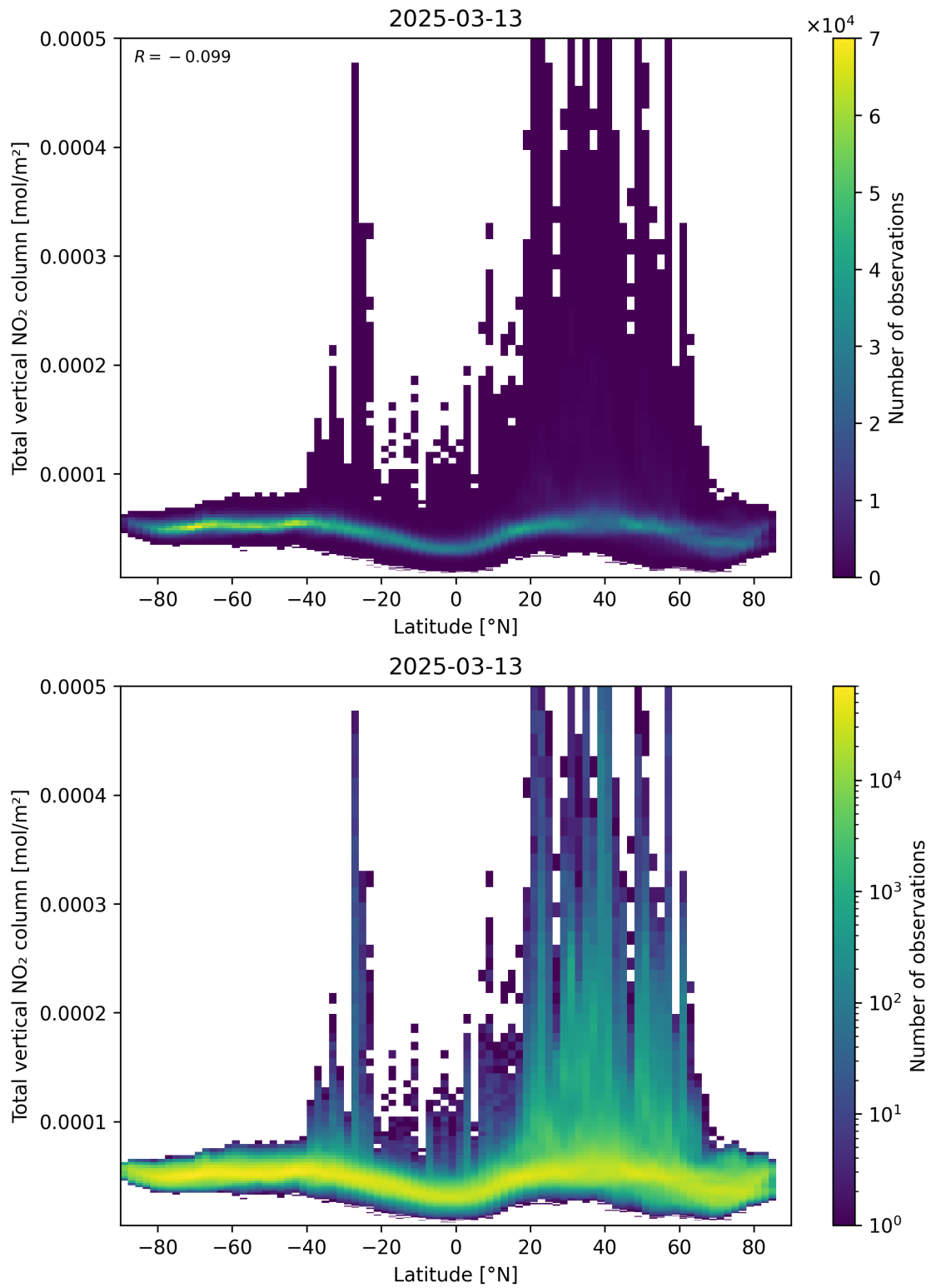
Figure 90: Scatter density plot of “Latitude” against “Total vertical NO 2 column” for 2025-03-13 to 2025-03-14.
