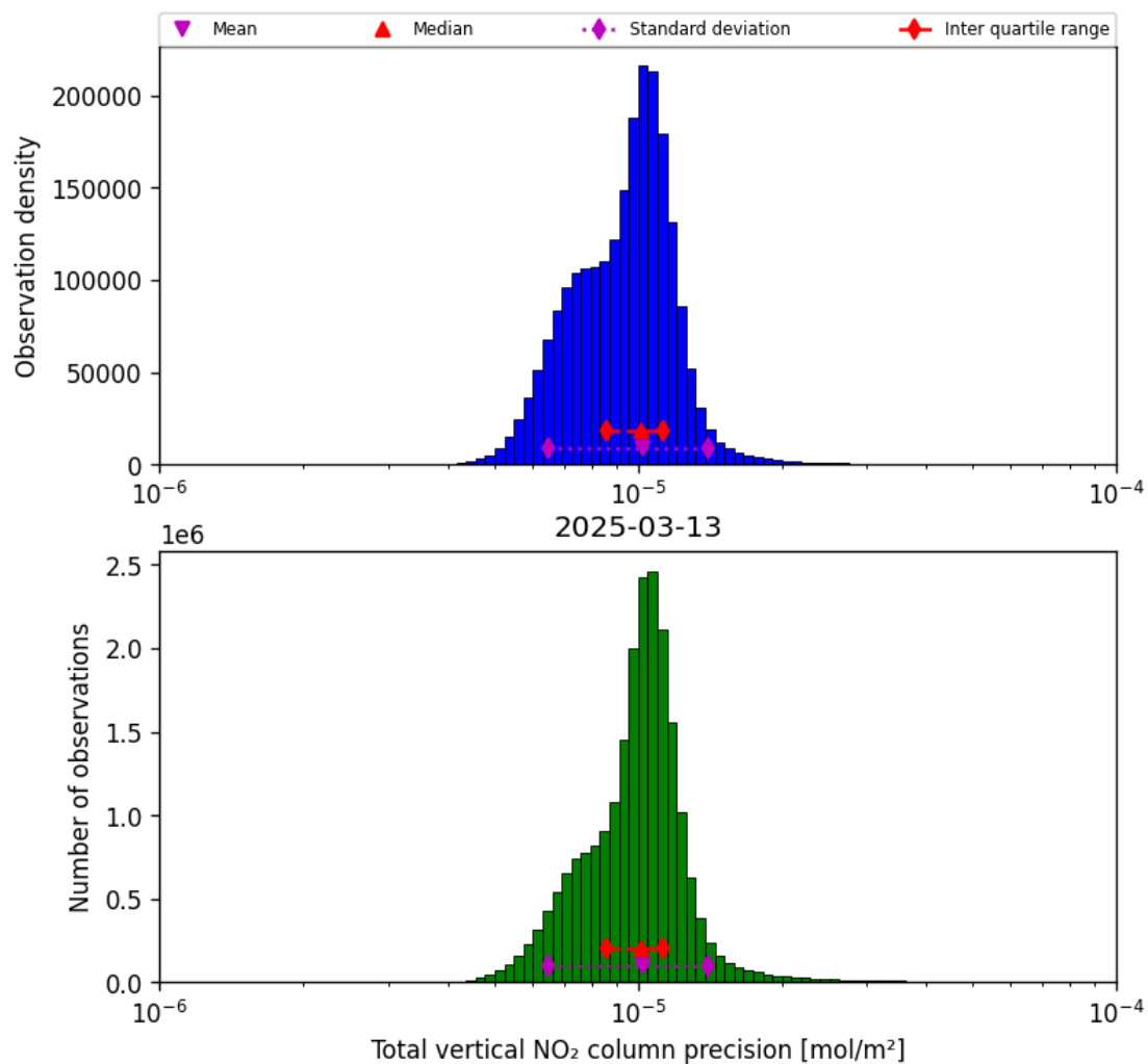
Figure 39: Histogram of “Total vertical NO 2 column precision” for 2025-03-13 to 2025-03-14
