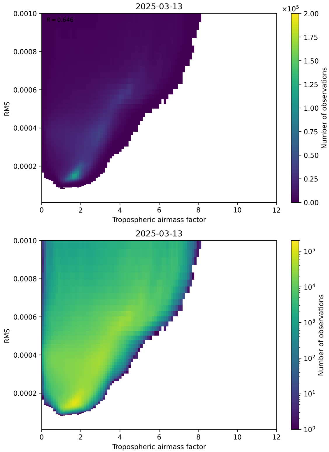
Figure 79: Scatter density plot of “Tropospheric airmass factor” against “RMS” for 2025-03-13 to 2025-03-14.
