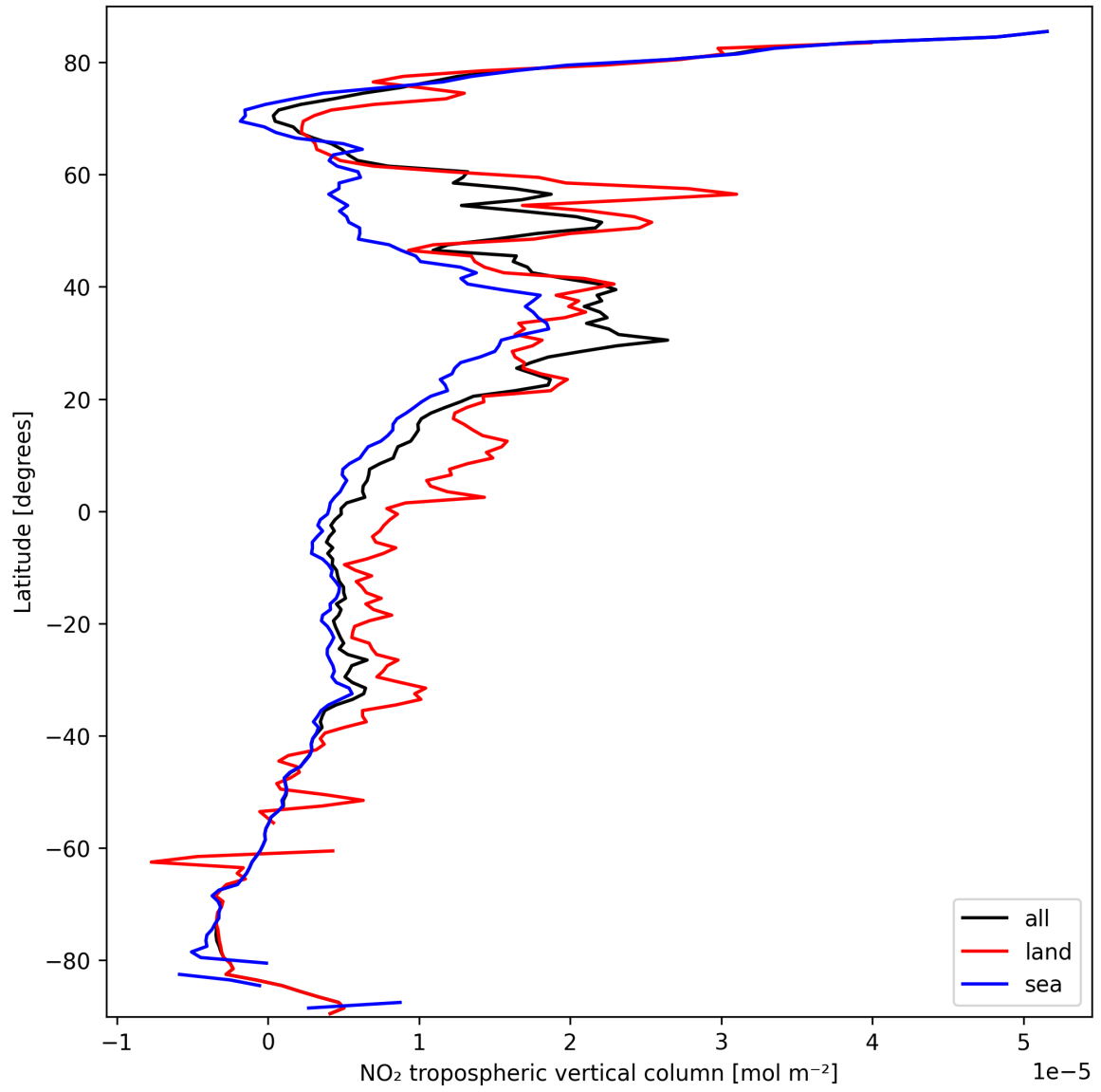
Figure 12: Zonal average of “NO 2 tropospheric vertical column” for 2025-03-13 to 2025-03-14.
