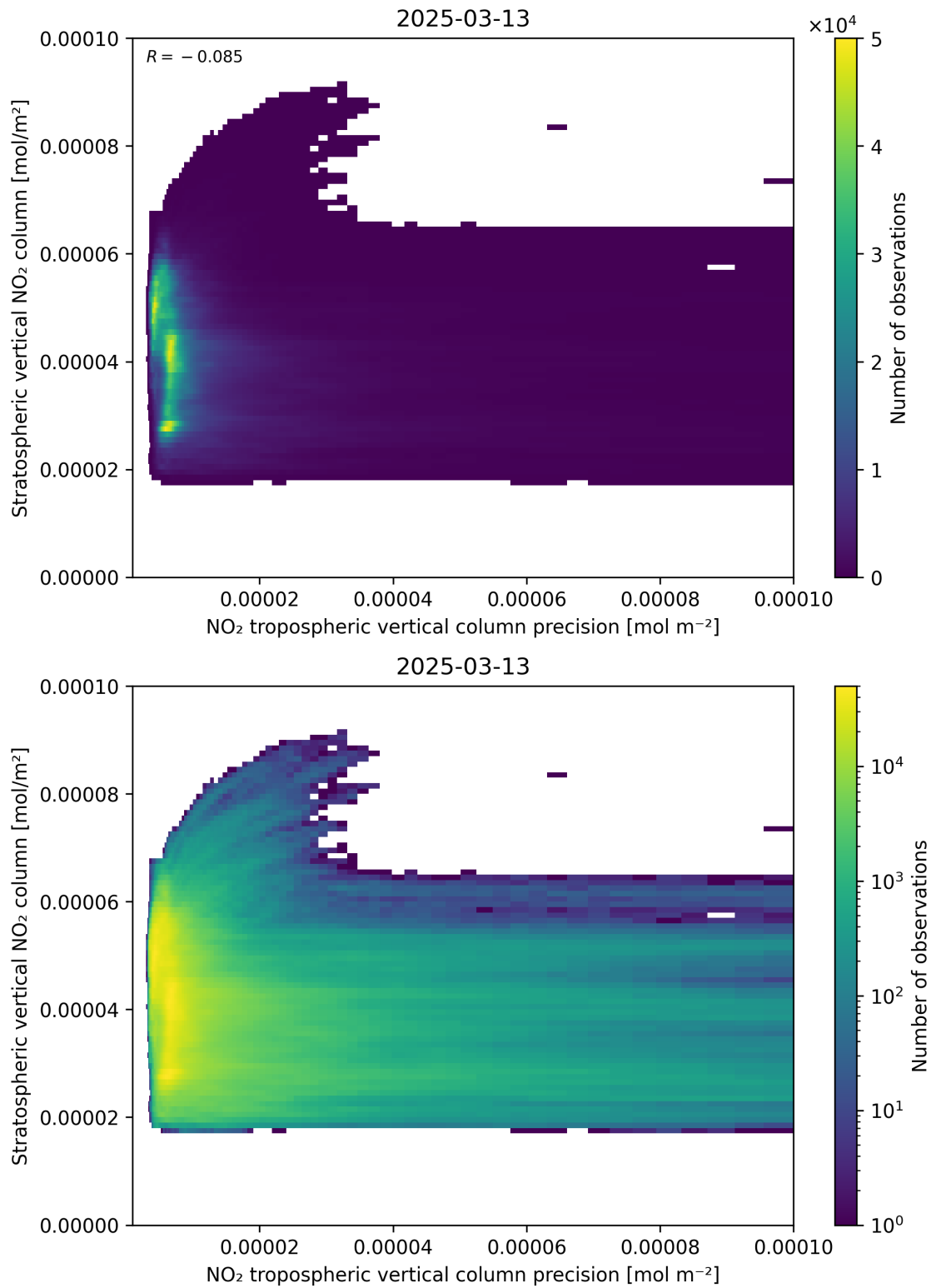
Figure 135: Scatter density plot of “NO 2 tropospheric vertical column precision” against “Stratospheric vertical NO 2 column” for 2025-03-13 to 2025-03-14.
