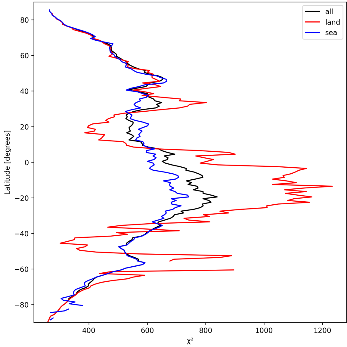
Figure 25: Zonal average of “ \chi^2 ” for 2025-03-13 to 2025-03-14.
