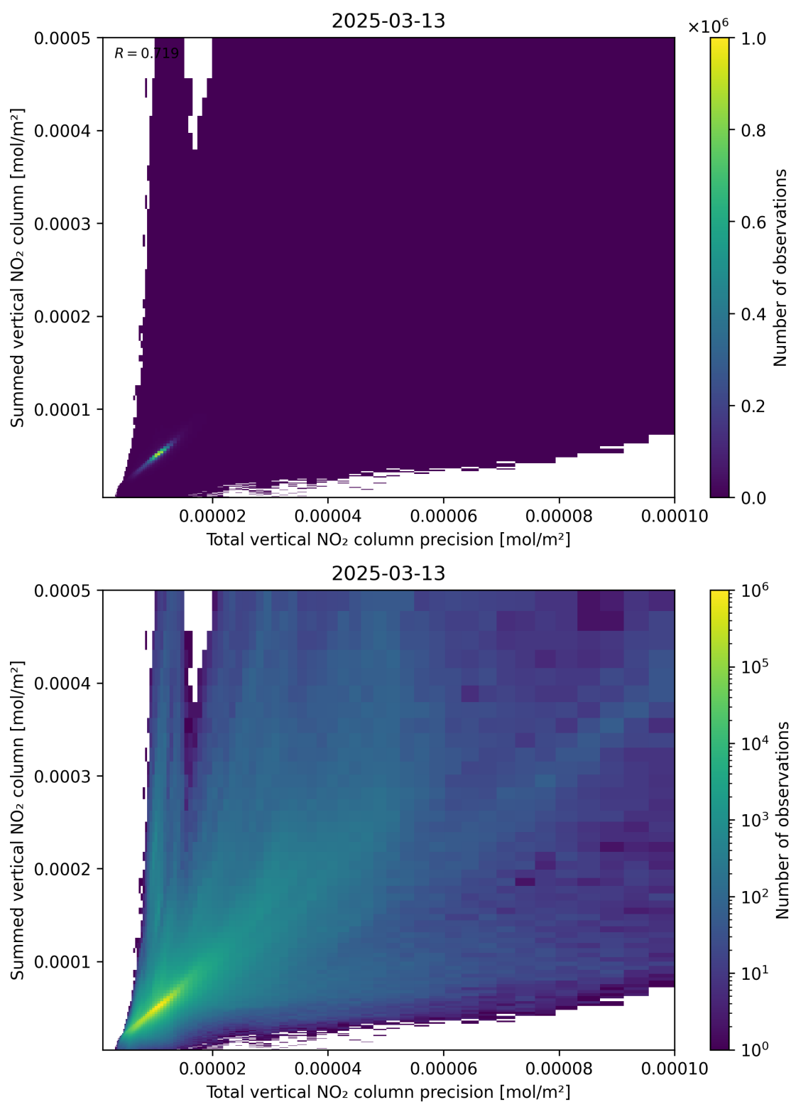
Figure 117: Scatter density plot of “Total vertical NO 2 column precision” against “Summed vertical NO 2 column” for 2025-03-13 to 2025-03-14.
