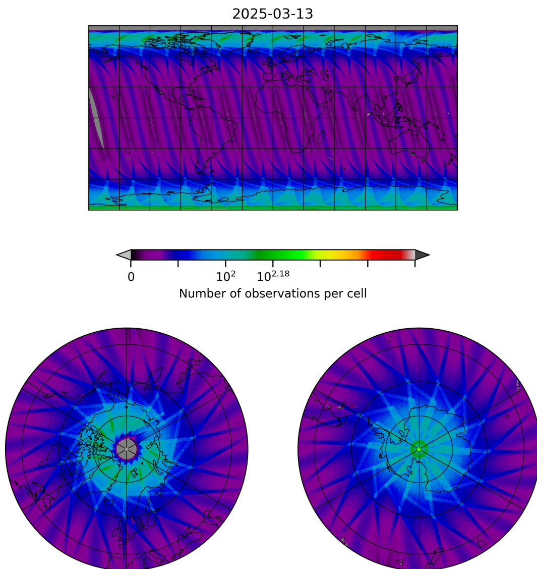
Figure 10: Map of the number of observations for 2025-03-13 to 2025-03-14
