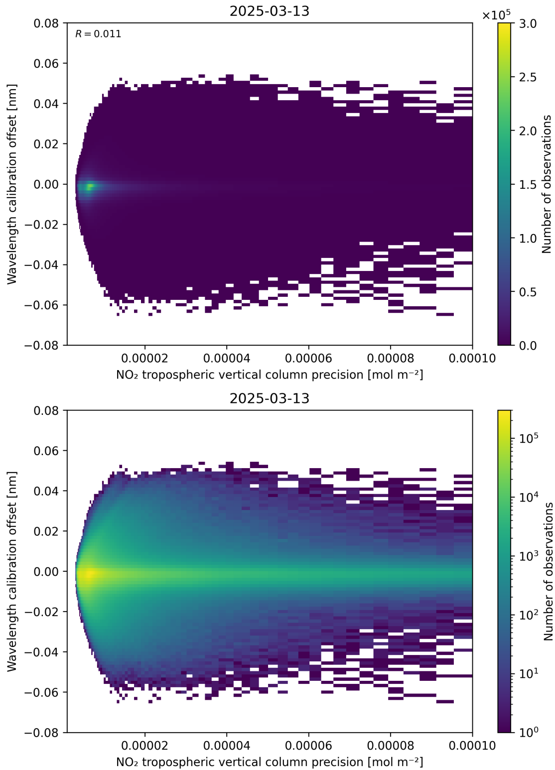
Figure 141: Scatter density plot of “NO 2 tropospheric vertical column precision” against “Wavelength calibration offset” for 2025-03-13 to 2025-03-14.
