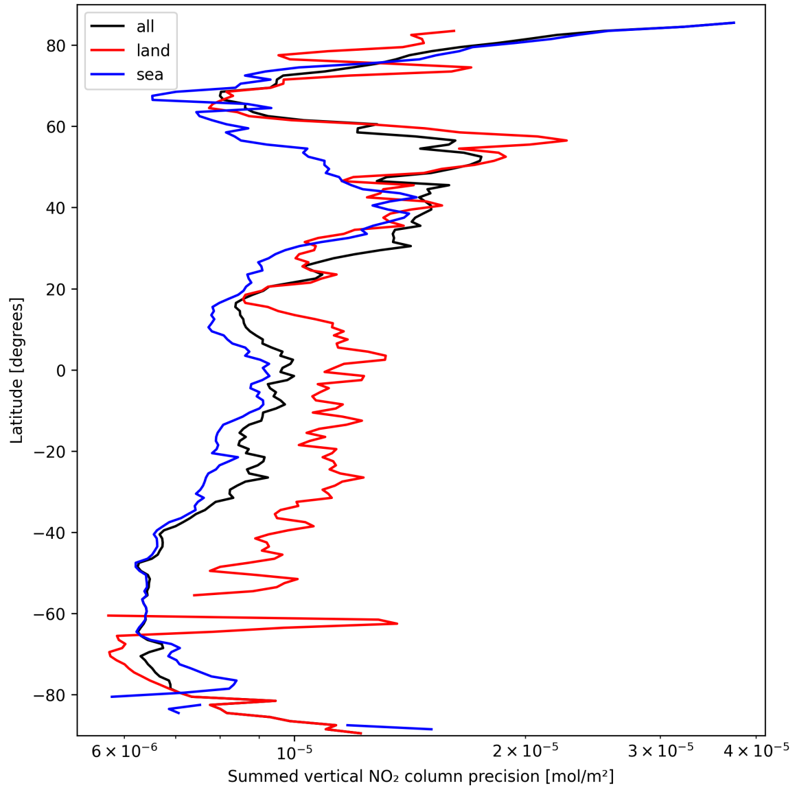
Figure 24: Zonal average of “Summed vertical NO 2 column precision” for 2025-03-13 to 2025-03-14.
