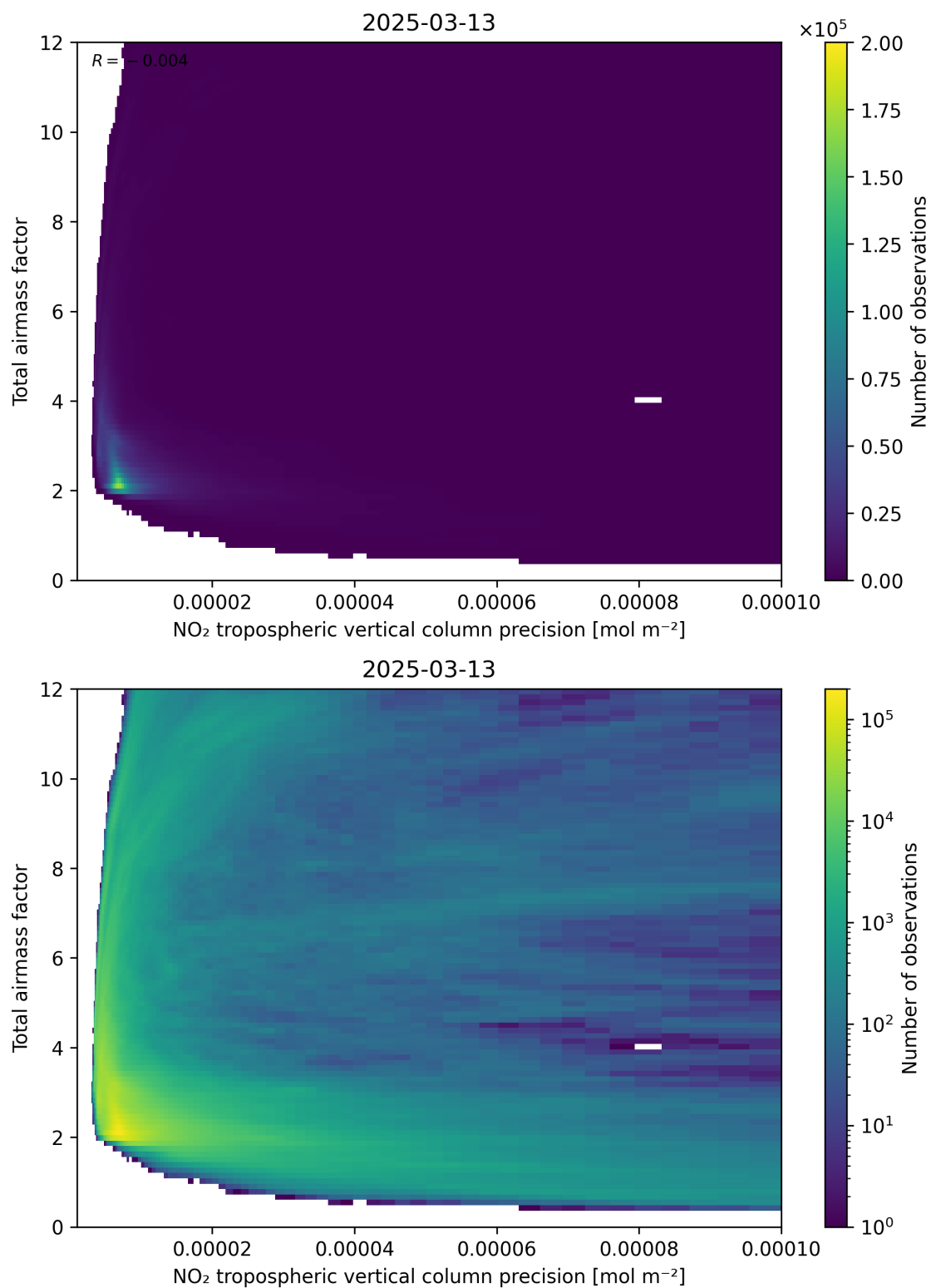
Figure 132: Scatter density plot of “NO 2 tropospheric vertical column precision” against “Total airmass factor” for 2025-03-13 to 2025-03-14.
