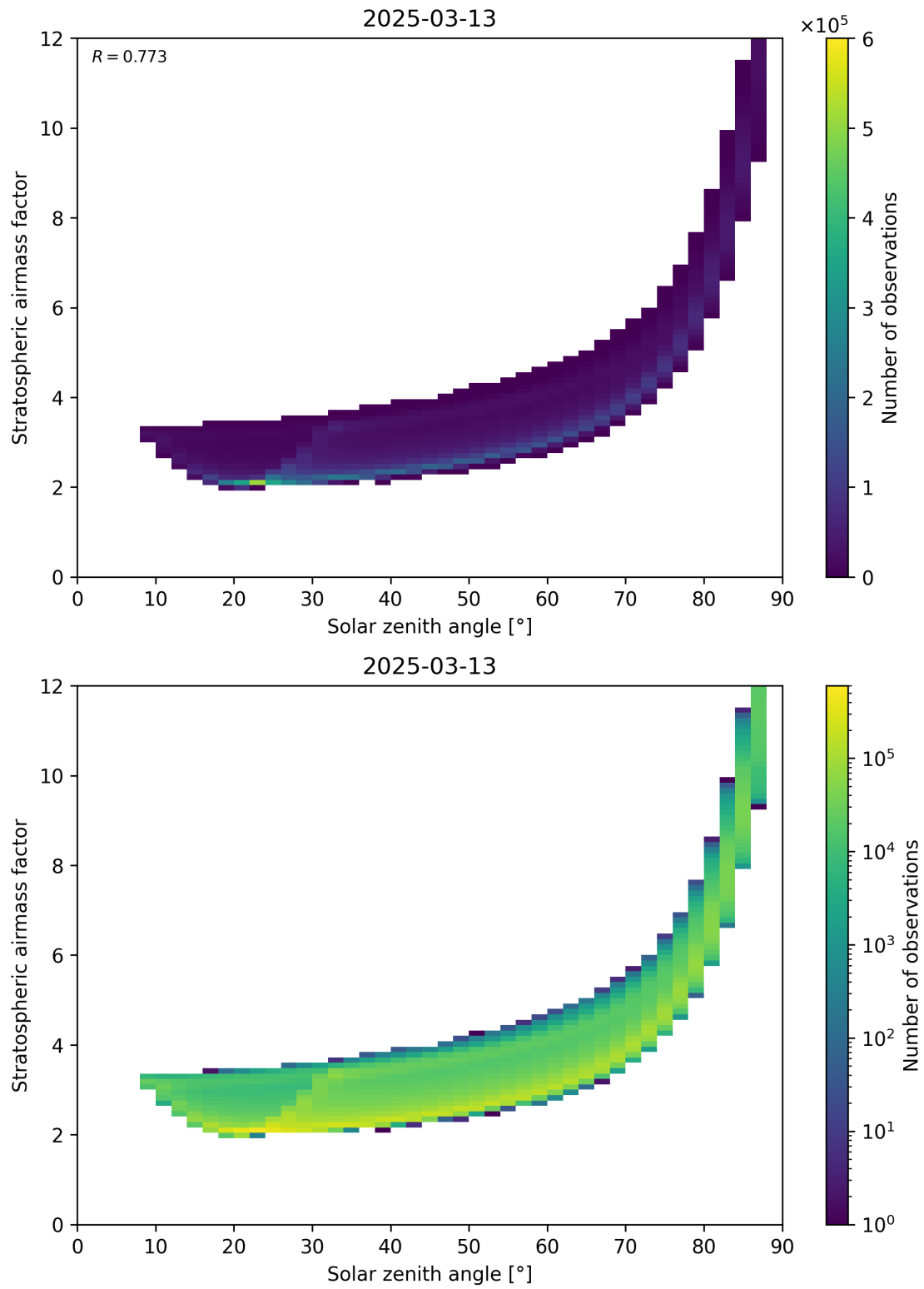
Figure 145: Scatter density plot of “Solar zenith angle” against “Stratospheric airmass factor” for 2025-03-13 to 2025-03-14.
