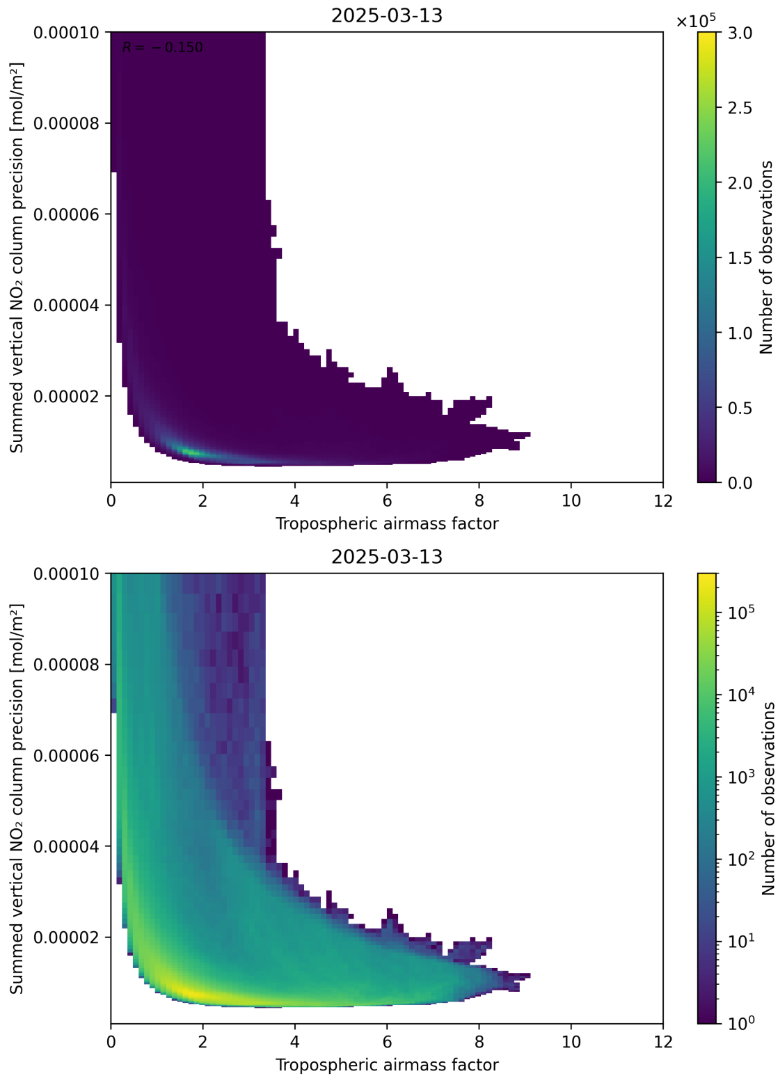
Figure 76: Scatter density plot of “Tropospheric air mass factor” against “Summed vertical NO 2 column precision” for 2025-03-13 to 2025-03-14.
