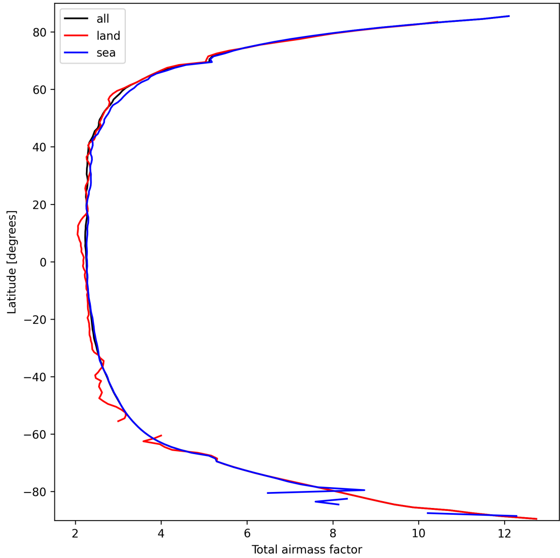
Figure 15: Zonal average of “Total airmass factor” for 2025-03-13 to 2025-03-14.
