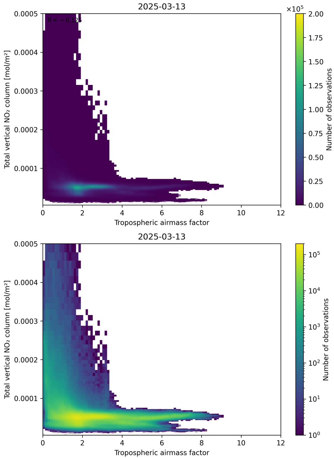
Figure 77: Scatter density plot of “Tropospheric airmass factor” against “Total vertical NO 2 column” for 2025-03-13 to 2025-03-14.
