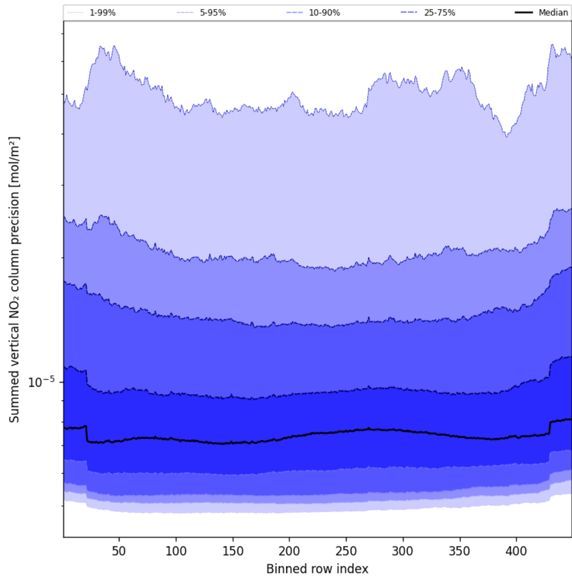
Figure 58: Along track statistics of “Summed vertical NO 2 column precision” for 2025-03-13 to 2025-03-14
