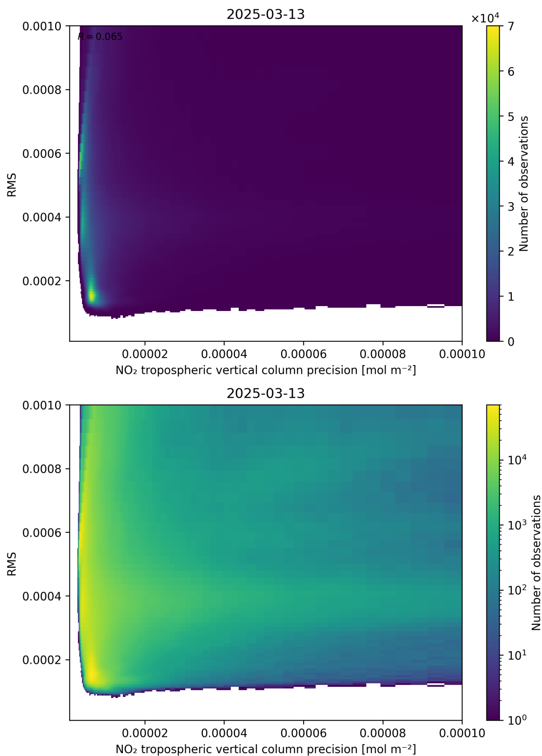
Figure 140: Scatter density plot of “NO 2 tropospheric vertical column precision” against “RMS” for 2025-03-13 to 2025-03-14.
