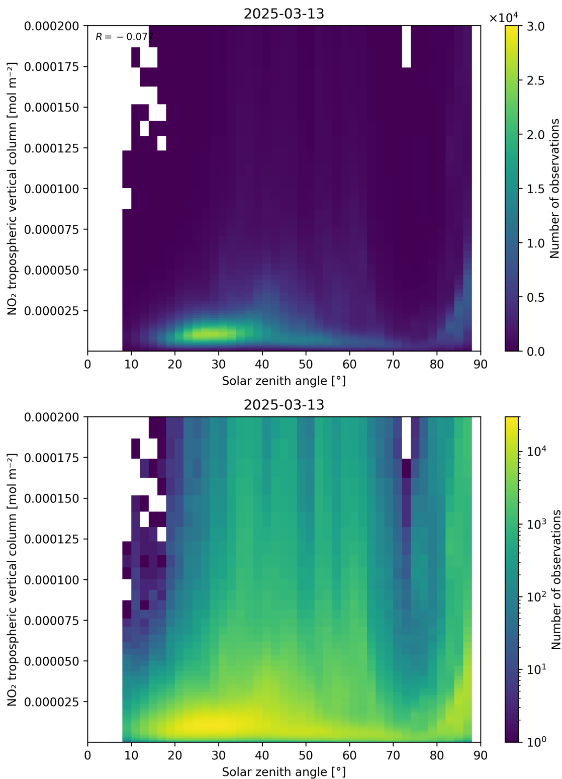
Figure 155: Scatter density plot of “Solar zenith angle” against “NO 2 tropospheric vertical column” for 2025-03-13 to 2025-03-14.
