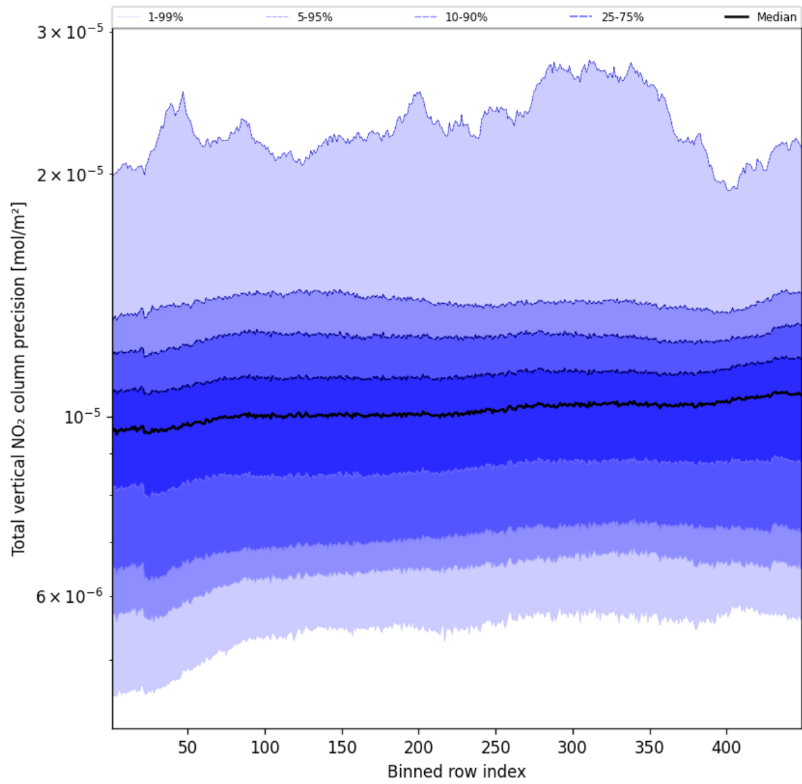
Figure 56: Along track statistics of “Total vertical NO 2 column precision” for 2025-03-13 to 2025-03-14
