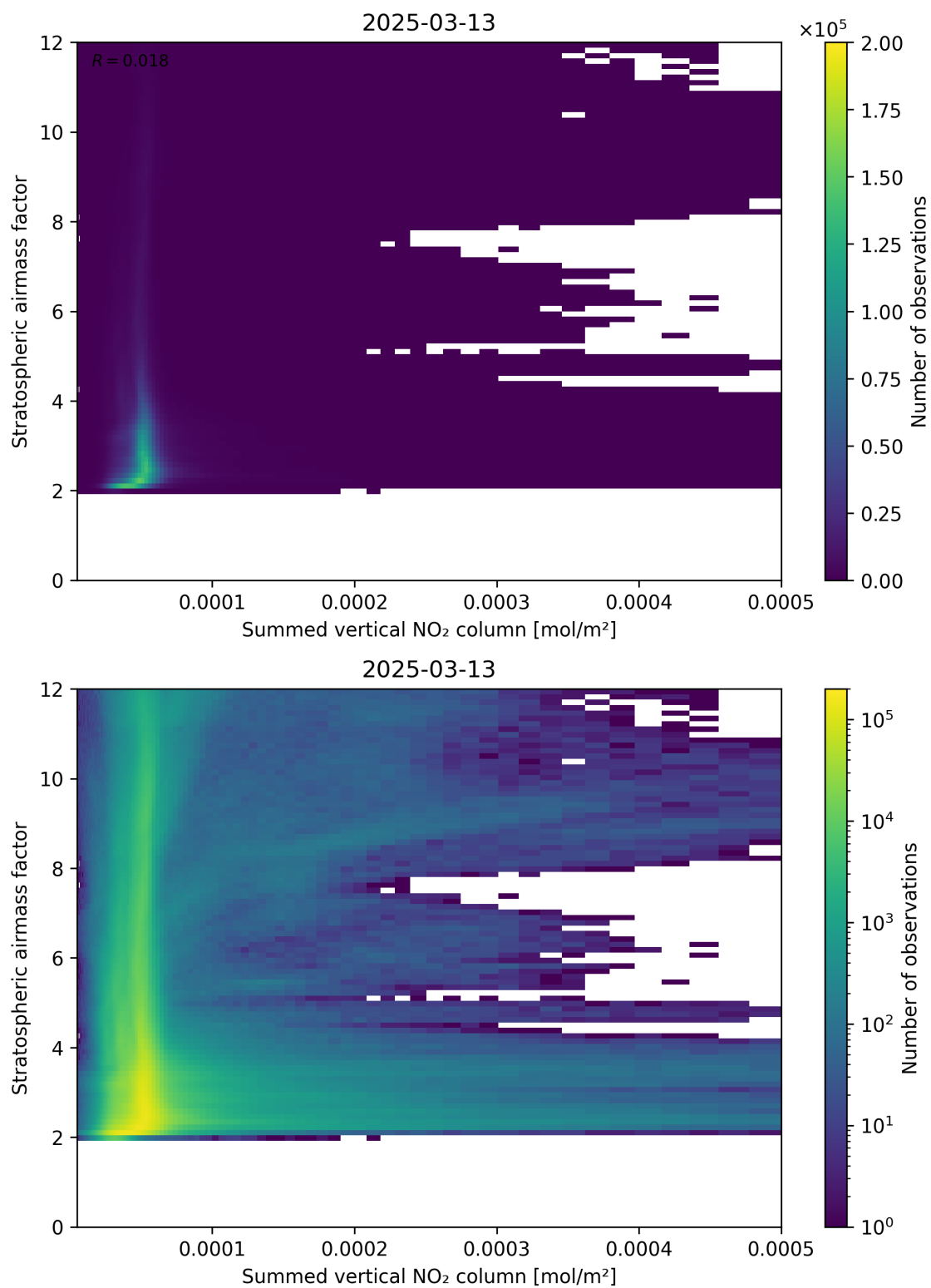
Figure 103: Scatter density plot of “Summed vertical NO 2 column” against “Stratospheric airmass factor” for 2025-03-13 to 2025-03-14.
