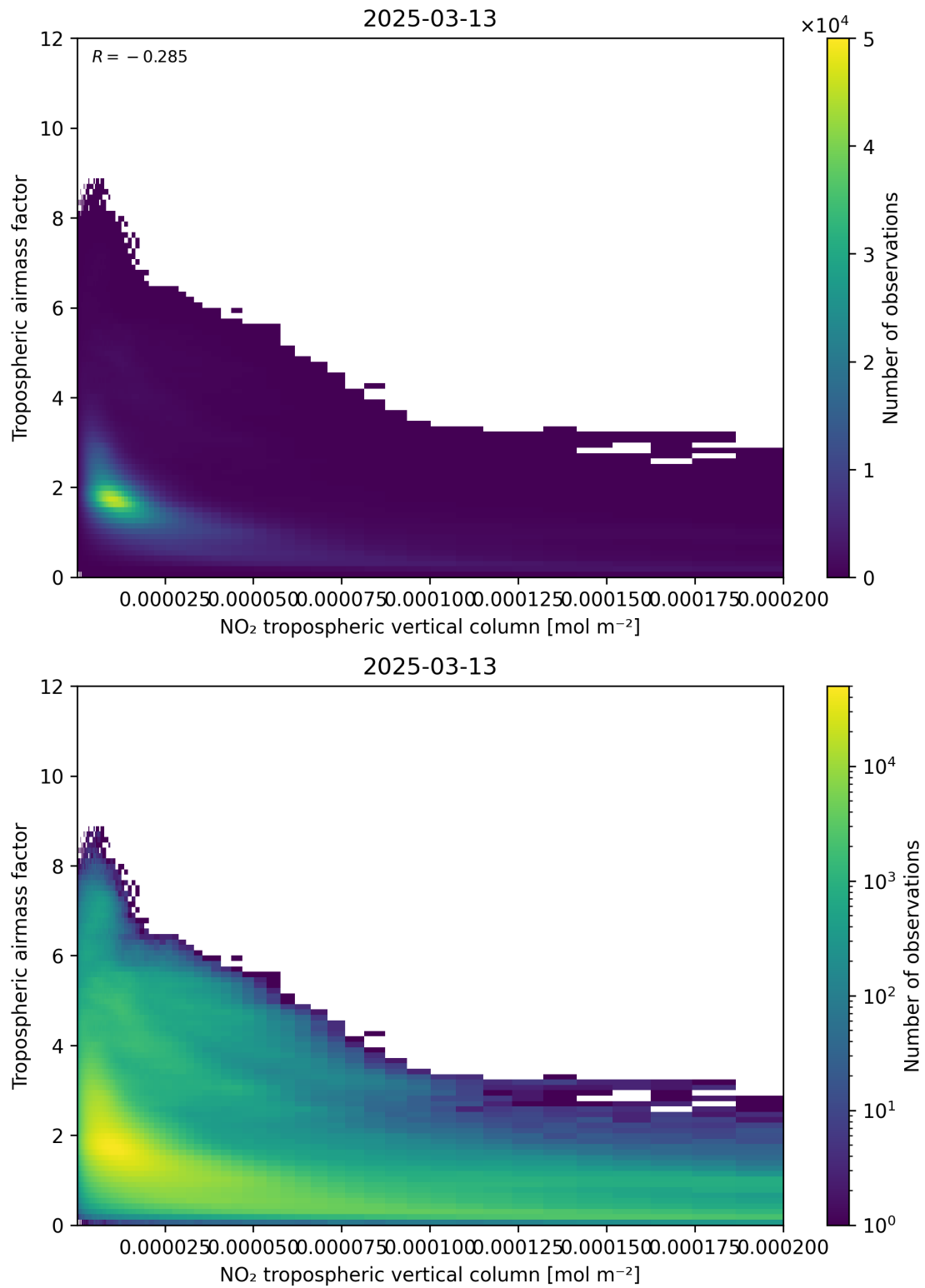
Figure 123: Scatter density plot of “NO 2 tropospheric vertical column” against “Tropospheric air mass factor” for 2025-03-13 to 2025-03-14.
