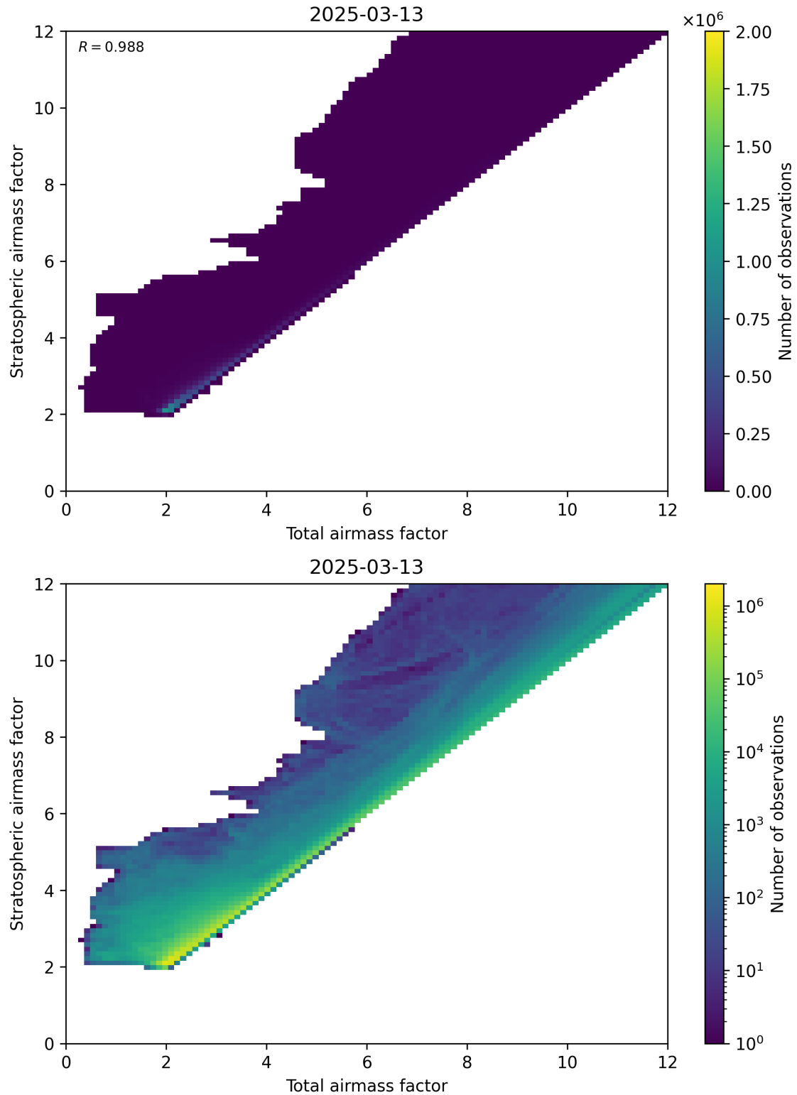
Figure 62: Scatter density plot of “Total airmass factor” against “Stratospheric airmass factor” for 2025-03-13 to 2025-03-14.
