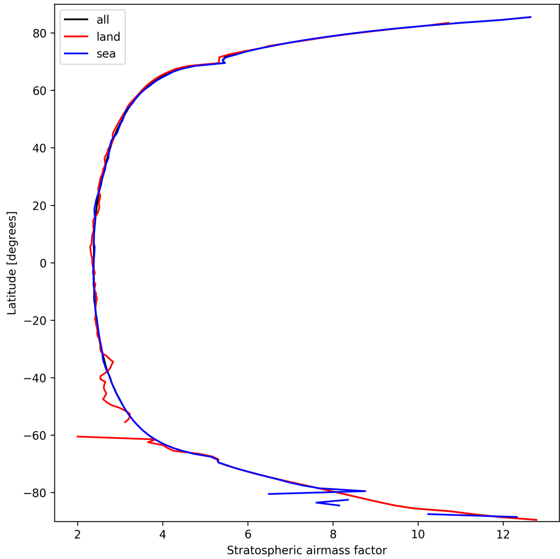
Figure 27: Zonal average of “Stratospheric airmass factor” for 2025-03-13 to 2025-03-14.
