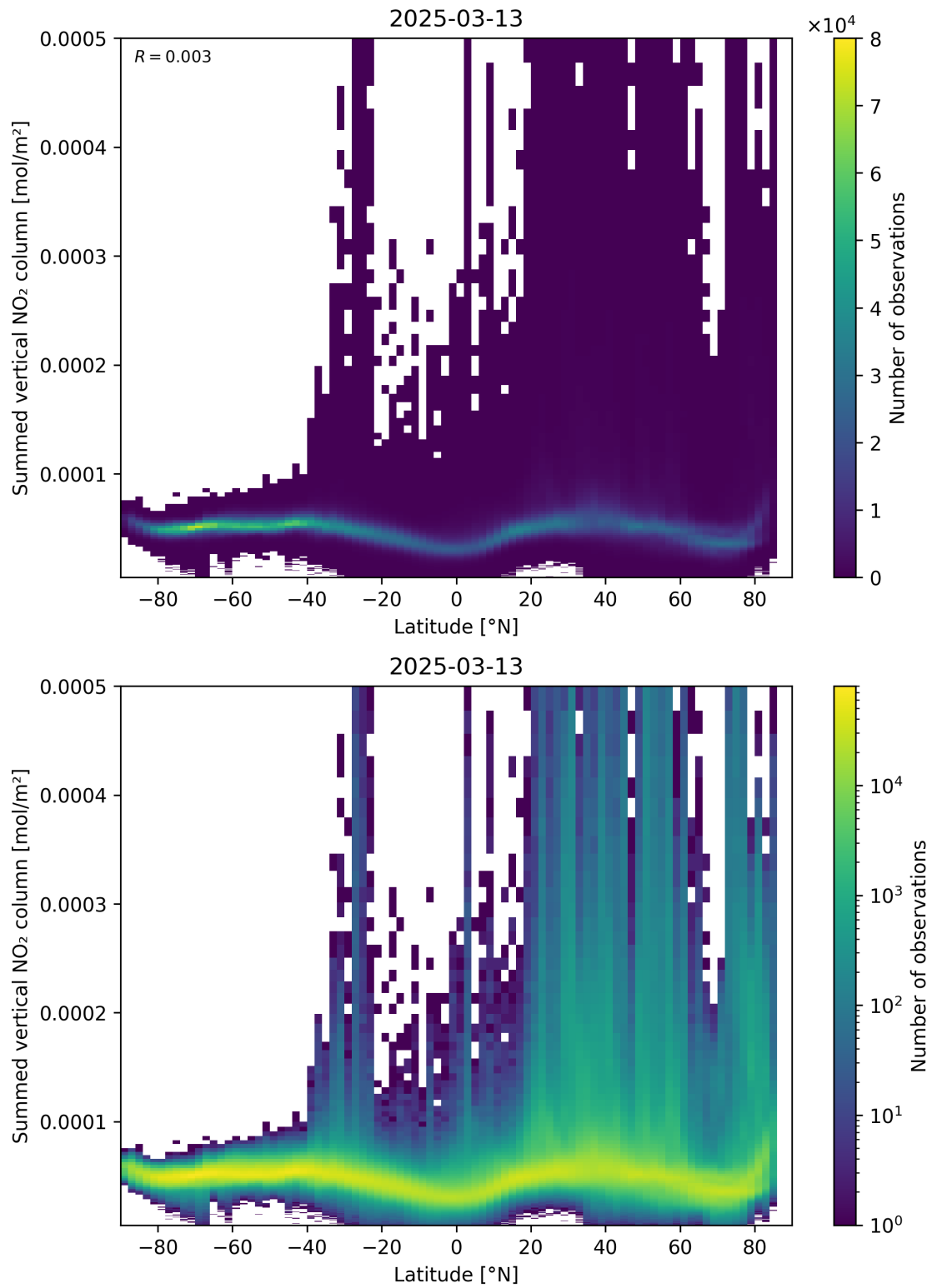
Figure 88: Scatter density plot of “Latitude” against “Summed vertical NO 2 column” for 2025-03-13 to 2025-03-14.
