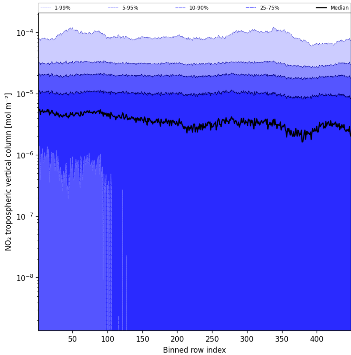
Figure 46: Along track statistics of “NO 2 tropospheric vertical column” for 2025-03-13 to 2025-03-14
