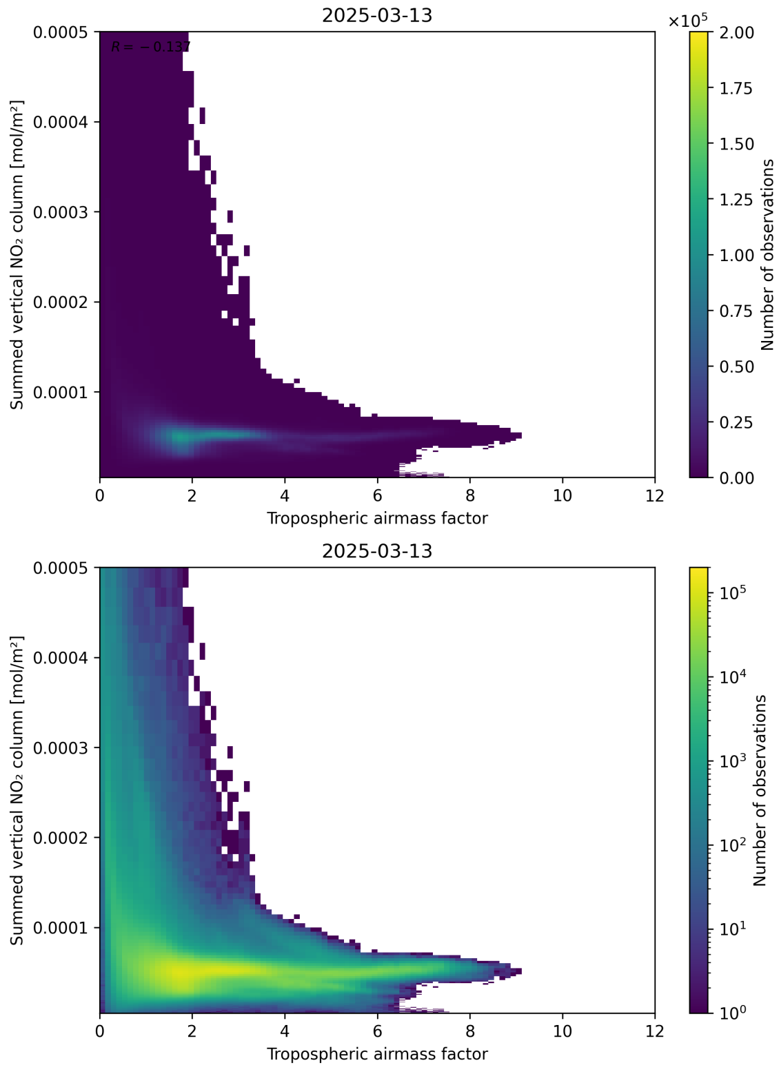
Figure 75: Scatter density plot of “Tropospheric airmass factor” against “Summed vertical NO 2 column” for 2025-03-13 to 2025-03-14.
