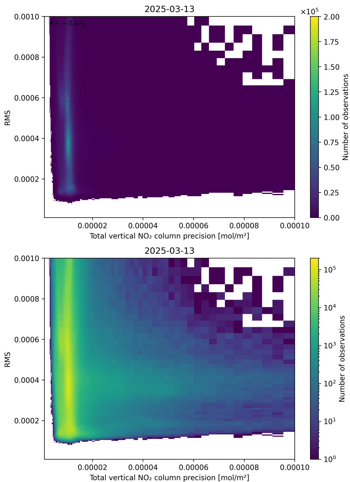
Figure 119: Scatter density plot of “Total vertical NO 2 column precision” against “RMS” for 2025-03-13 to 2025-03-14.
