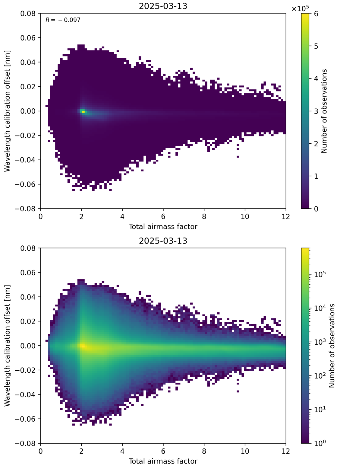
Figure 70: Scatter density plot of “Total airmass factor” against “Wavelength calibration offset” for 2025-03-13 to 2025-03-14.
