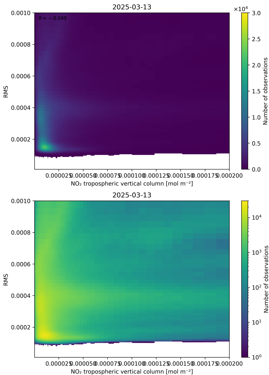
Figure 142: Scatter density plot of “NO 2 tropospheric vertical column” against “RMS” for 2025-03-13 to 2025-03-14.
