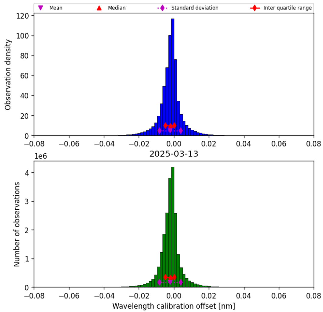
Figure 35: Histogram of “Wavelength calibration offset” for 2025-03-13 to 2025-03-14
