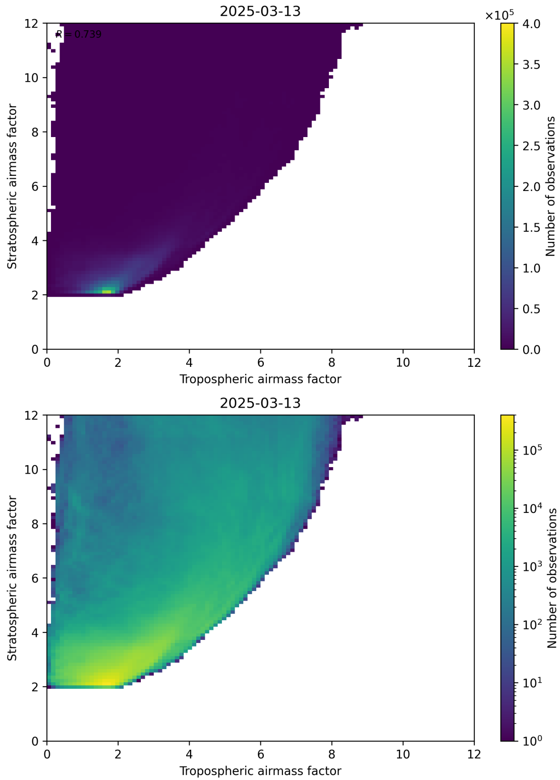
Figure 71: Scatter density plot of “Tropospheric airmass factor” against “Stratospheric airmass factor” for 2025-03-13 to 2025-03-14.
