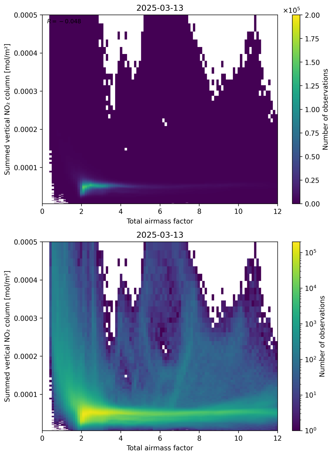
Figure 65: Scatter density plot of “Total airmass factor” against “Summed vertical NO 2 column” for 2025-03-13 to 2025-03-14.
