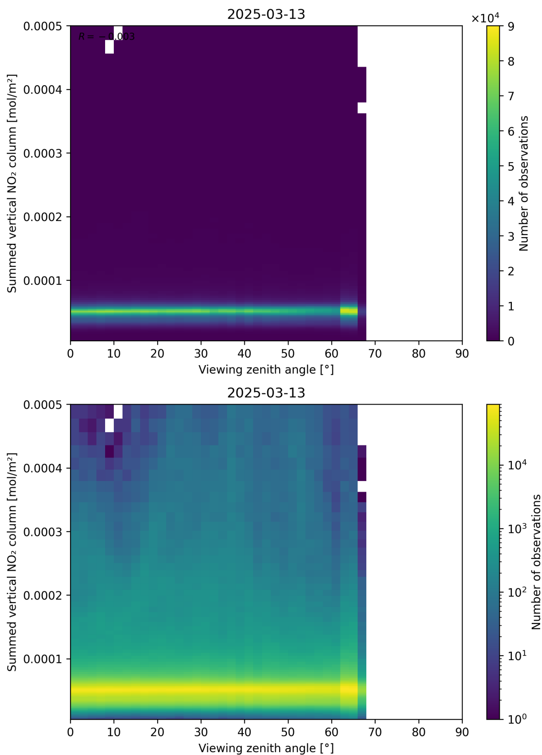
Figure 165: Scatter density plot of “Viewing zenith angle” against “Summed vertical NO 2 column” for 2025-03-13 to 2025-03-14.
