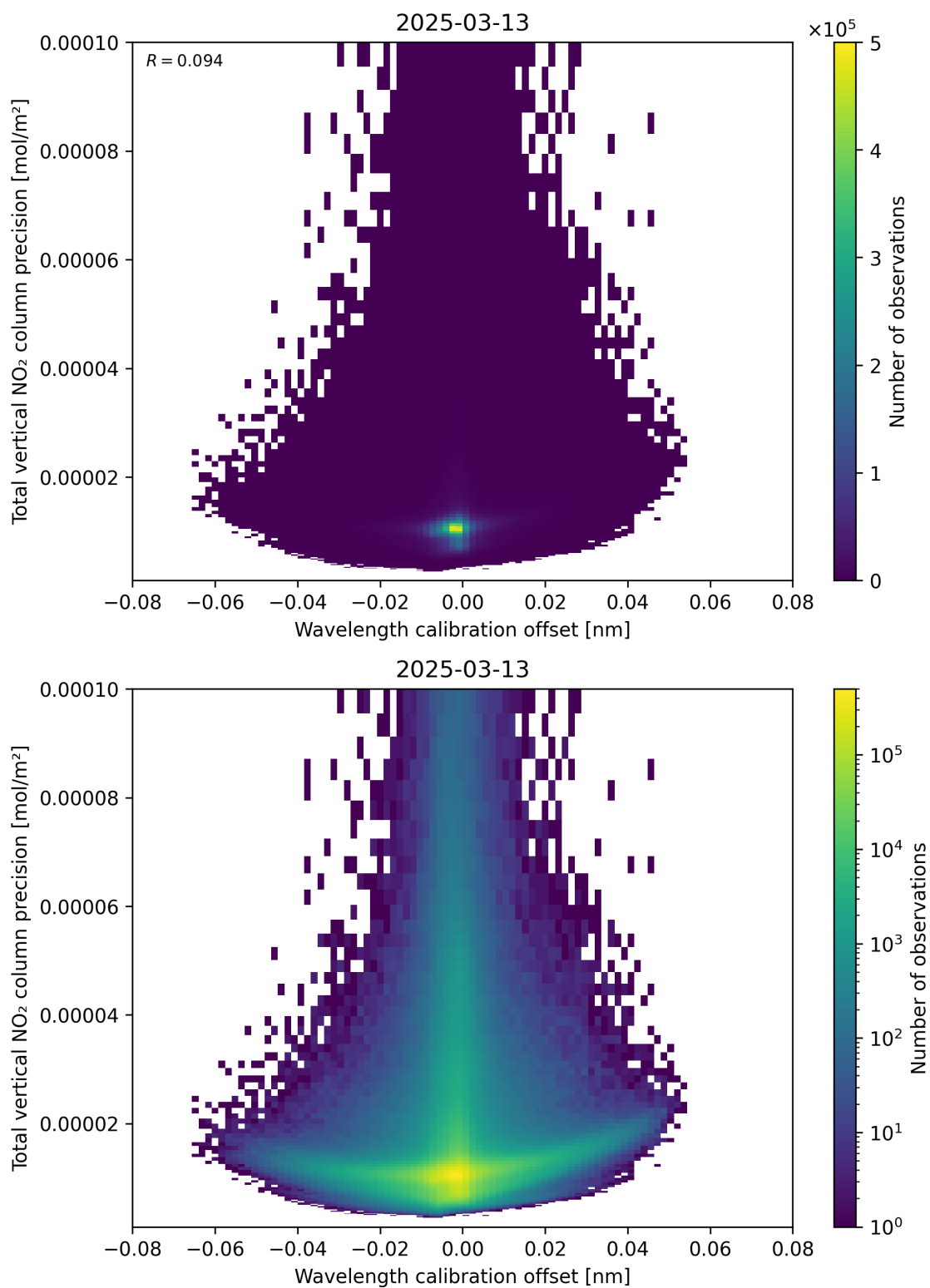
Figure 180: Scatter density plot of “Wavelength calibration offset” against “Total vertical NO 2 column precision” for 2025-03-13 to 2025-03-14.
