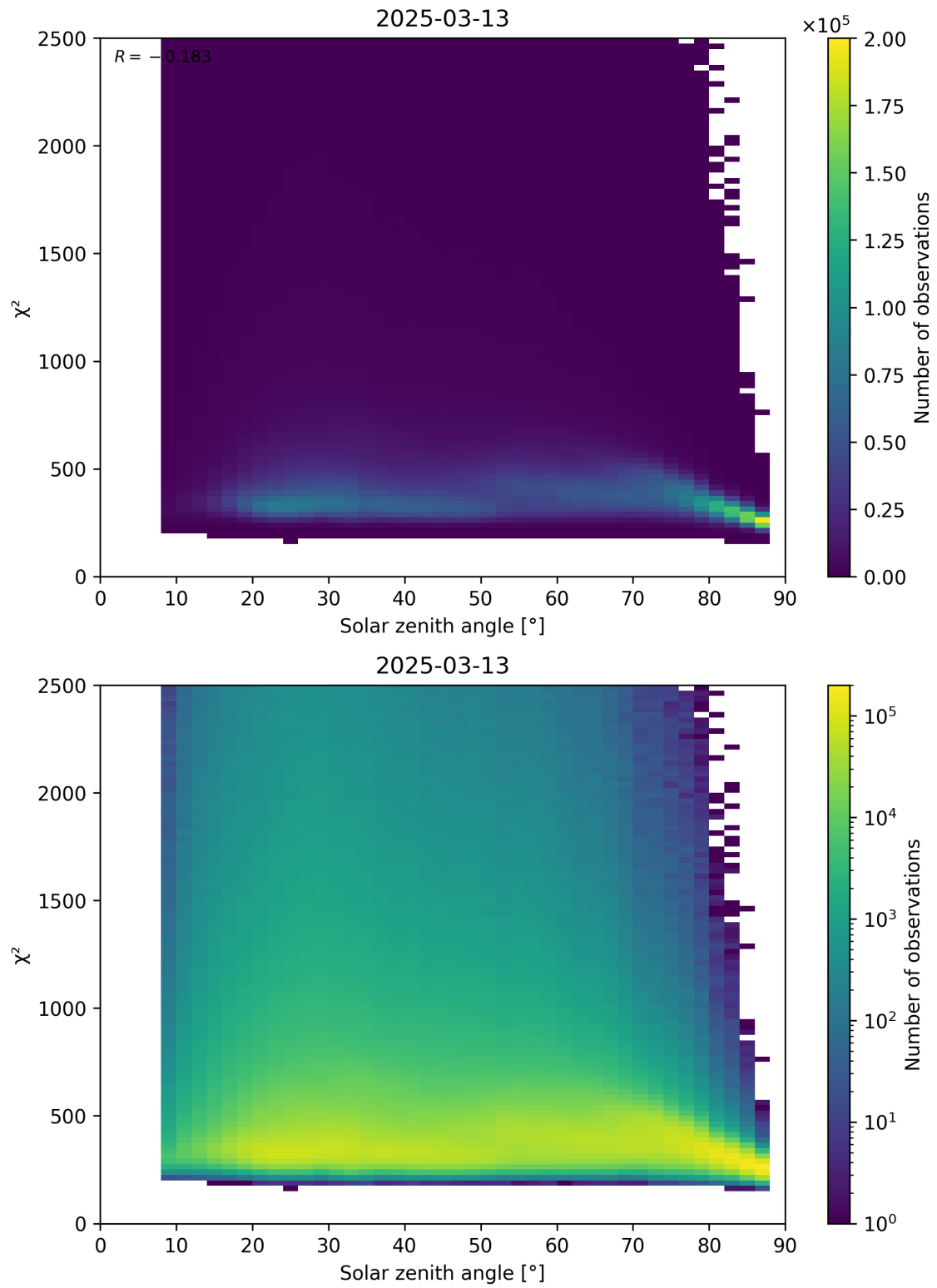
Figure 148: Scatter density plot of “Solar zenith angle” against “ \chi^2 ” for 2025-03-13 to 2025-03-14.
