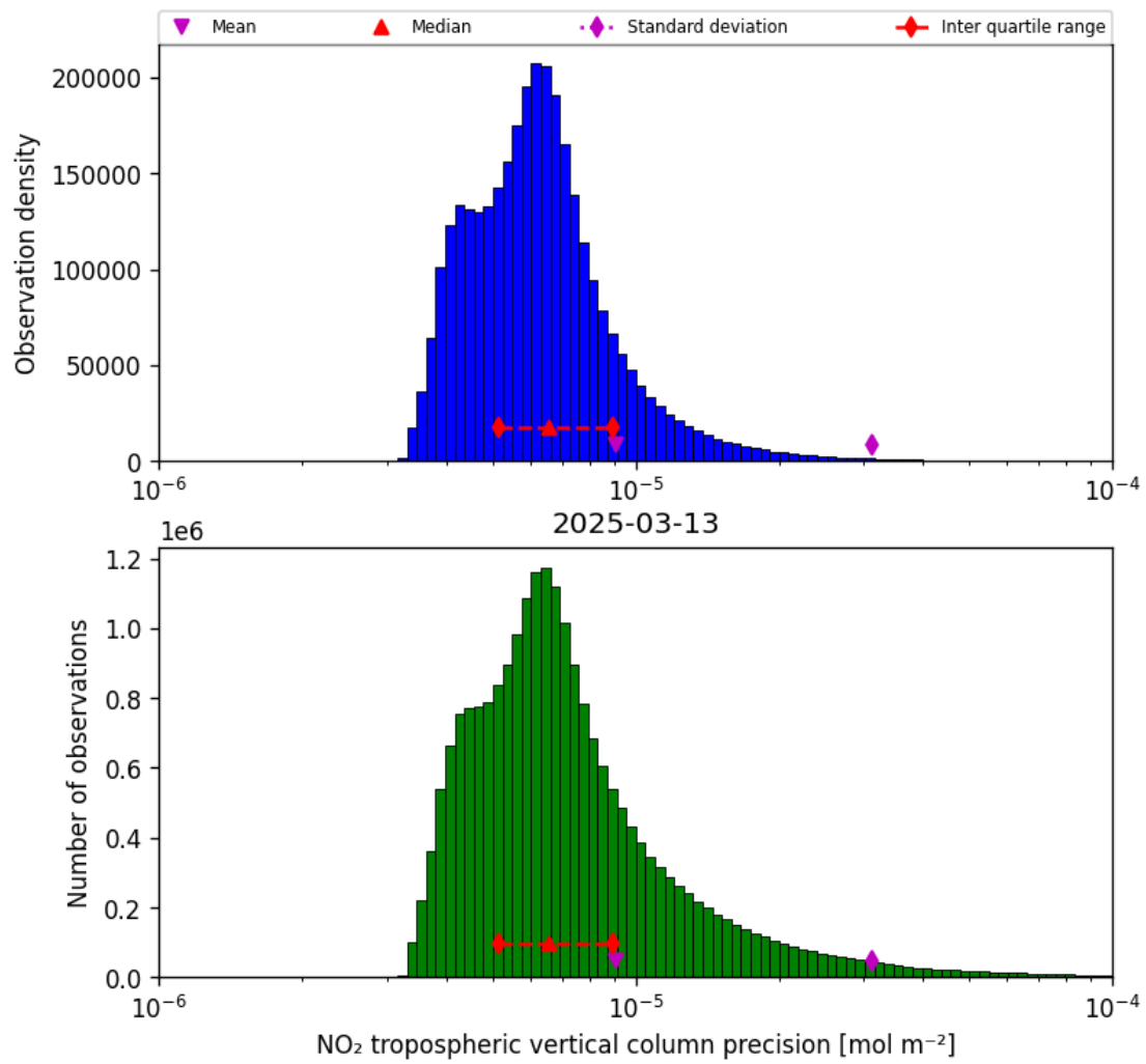
Figure 30: Histogram of “NO 2 tropospheric vertical column precision” for 2025-03-13 to 2025-03-14
