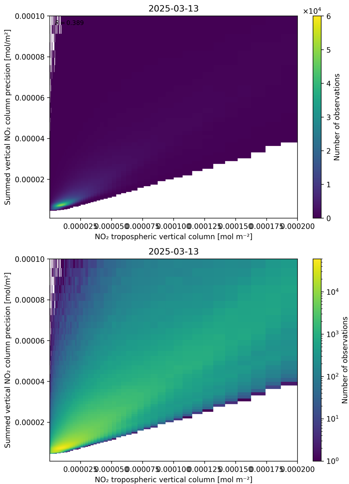
Figure 127: Scatter density plot of “NO 2 tropospheric vertical column” against “Summed vertical NO 2 column precision” for 2025-03-13 to 2025-03-14.
