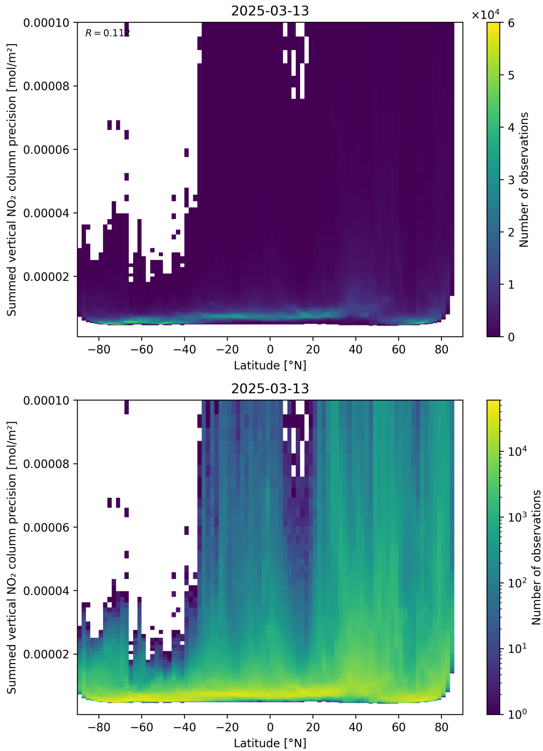
Figure 89: Scatter density plot of “Latitude” against “Summed vertical NO 2 column precision” for 2025-03-13 to 2025-03-14.
