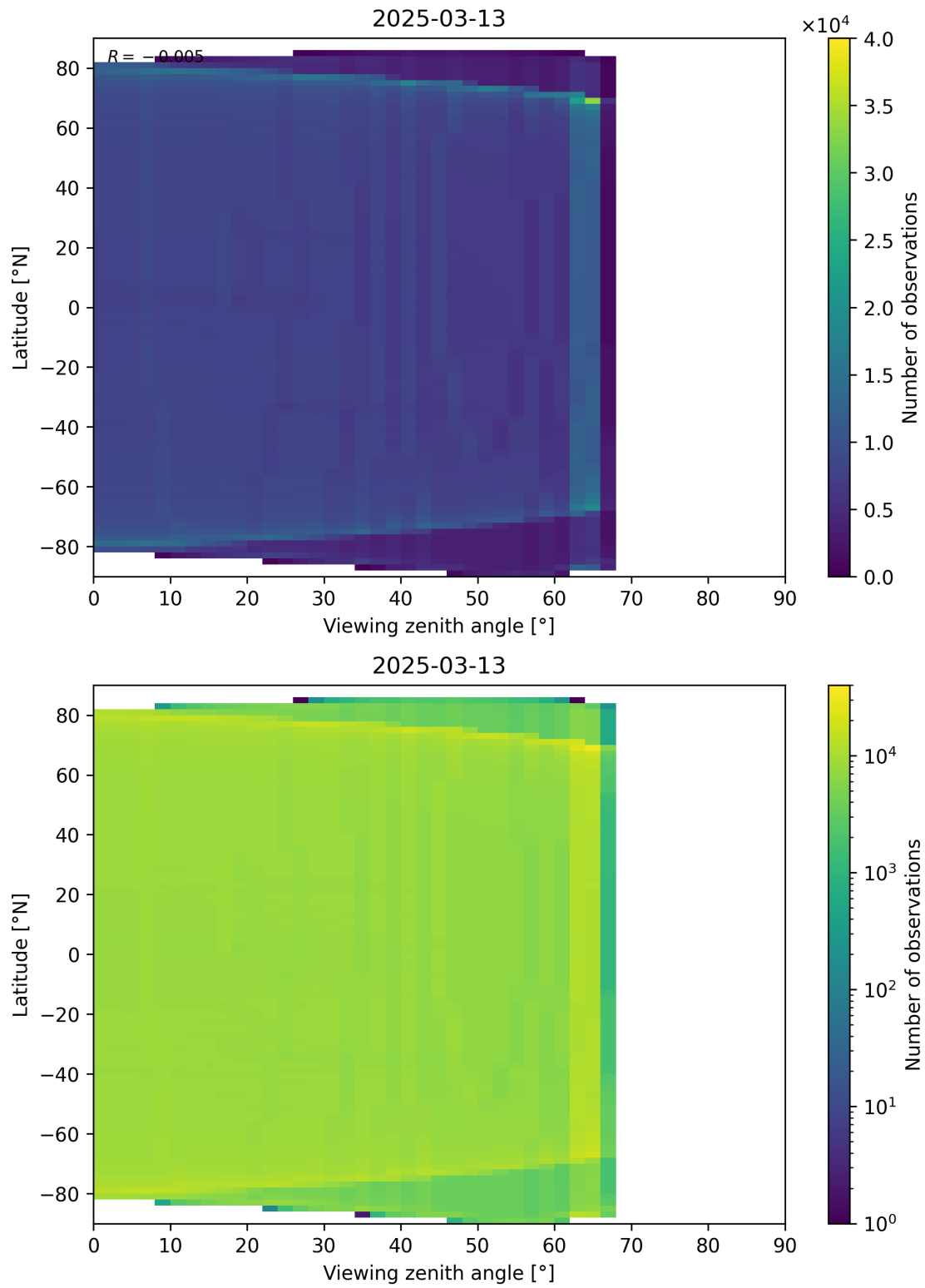
Figure 163: Scatter density plot of “Viewing zenith angle” against “Latitude” for 2025-03-13 to 2025-03-14.
