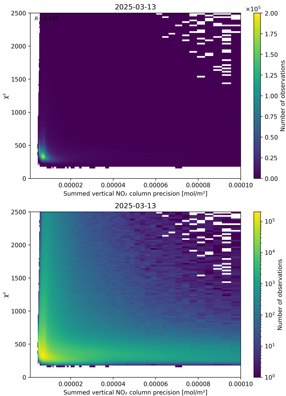
Figure 107: Scatter density plot of “Summed vertical NO 2 column precision” against “ \chi^2 ” for 2025-03-13 to 2025-03-14.
