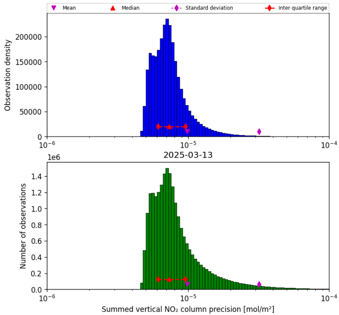
Figure 41: Histogram of "Summed vertical NO 2 column precision" for 2025-03-13 to 2025-03-14
