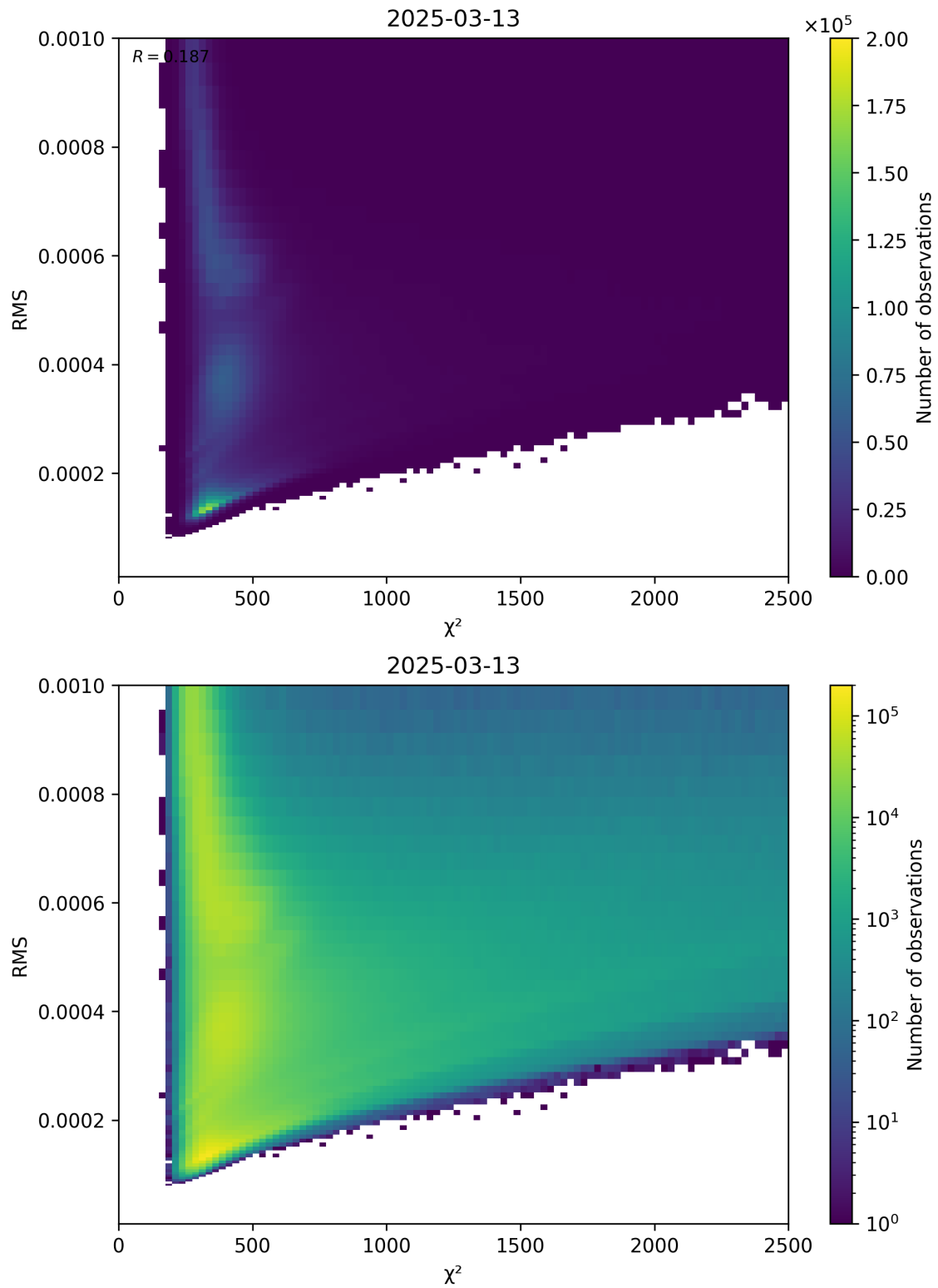
Figure 82: Scatter density plot of “ \chi^2 ” against “RMS” for 2025-03-13 to 2025-03-14.
