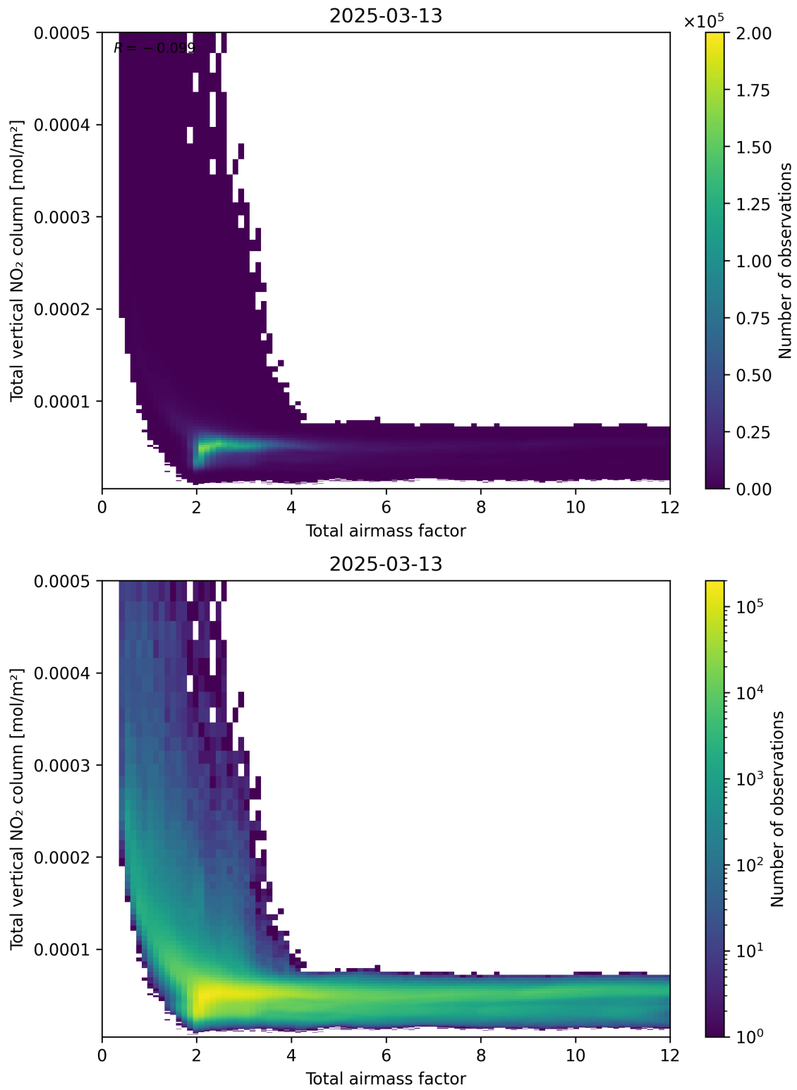
Figure 67: Scatter density plot of “Total airmass factor” against “Total vertical NO 2 column” for 2025-03-13 to 2025-03-14.
