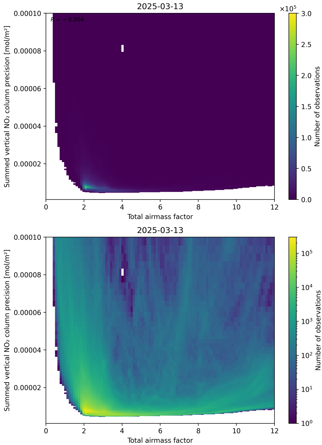
Figure 66: Scatter density plot of “Total airmass factor” against “Summed vertical NO 2 column precision” for 2025-03-13 to 2025-03-14.
