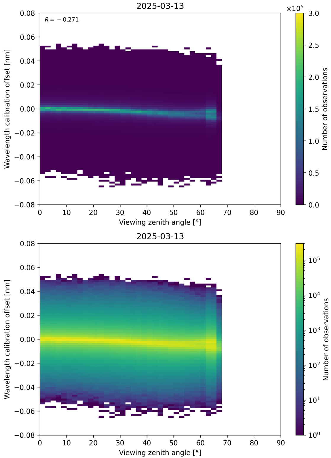
Figure 173: Scatter density plot of “Viewing zenith angle” against “Wavelength calibration offset” for 2025-03-13 to 2025-03-14.
