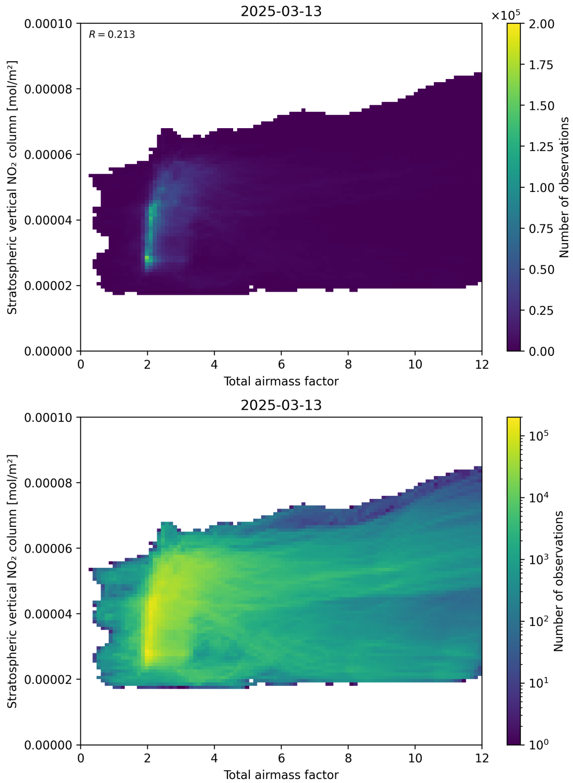
Figure 64: Scatter density plot of “Total airmass factor” against “Stratospheric vertical \text{NO}_2 column” for 2025-03-13 to 2025-03-14.
