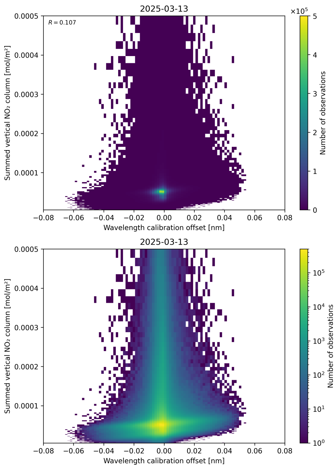
Figure 177: Scatter density plot of “Wavelength calibration offset” against “Summed vertical NO 2 column” for 2025-03-13 to 2025-03-14.
