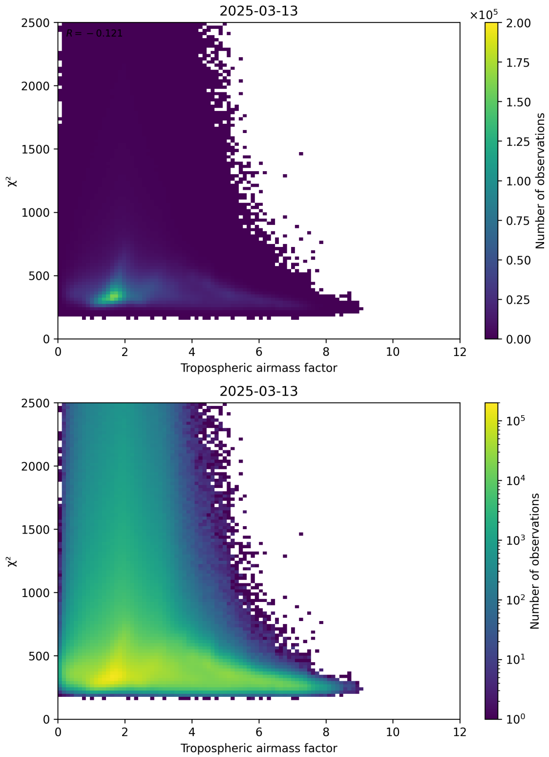
Figure 73: Scatter density plot of “Tropospheric airmass factor” against “ \chi^2 ” for 2025-03-13 to 2025-03-14.
