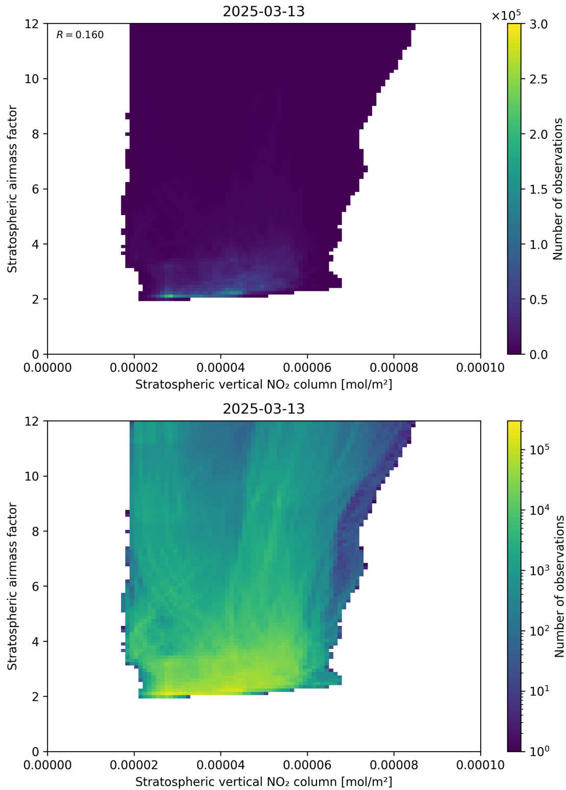
Figure 96: Scatter density plot of “Stratospheric vertical NO 2 column” against “Stratospheric airmass factor” for 2025-03-13 to 2025-03-14.
