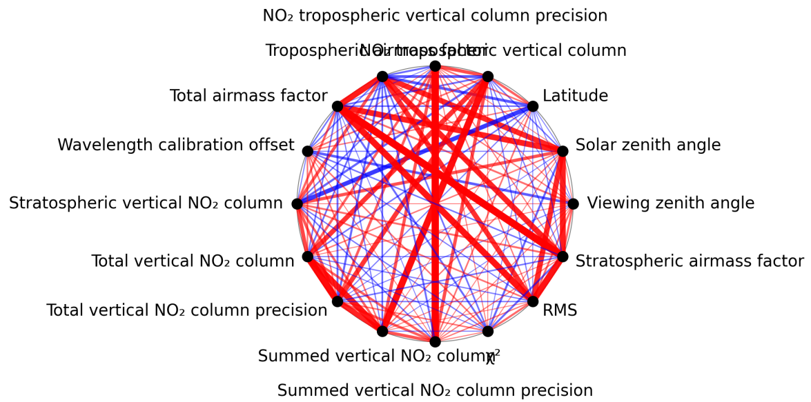
Figure 1: Map of correlation graph for 2025-03-13 to 2025-03-14.
