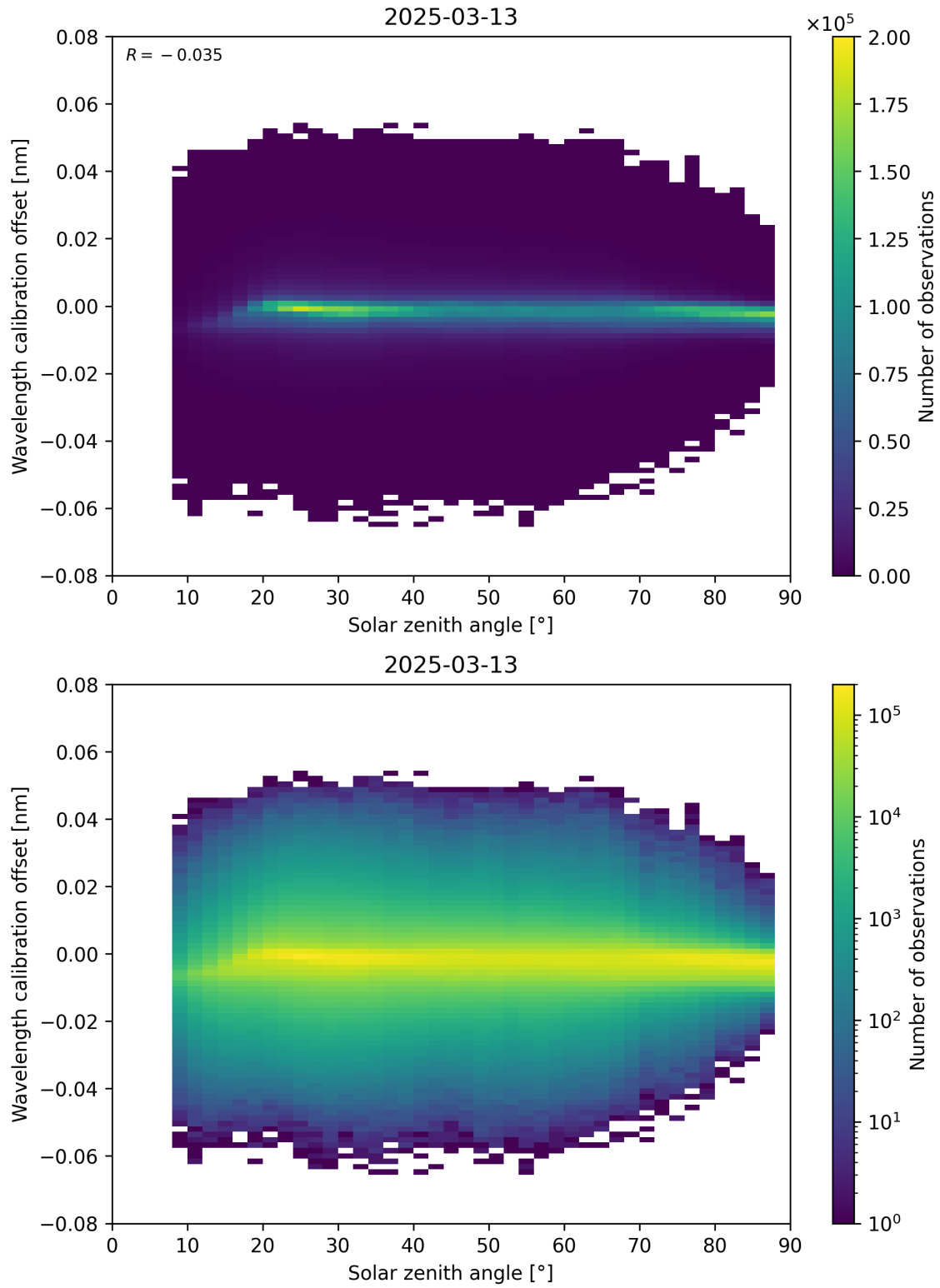
Figure 158: Scatter density plot of “Solar zenith angle” against “Wavelength calibration offset” for 2025-03-13 to 2025-03-14.
