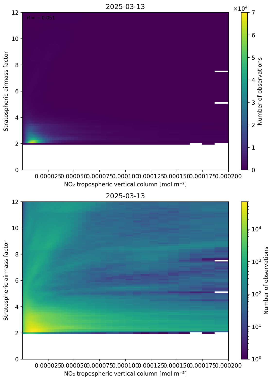
Figure 121: Scatter density plot of “NO 2 tropospheric vertical column” against “Stratospheric airmass factor” for 2025-03-13 to 2025-03-14.
