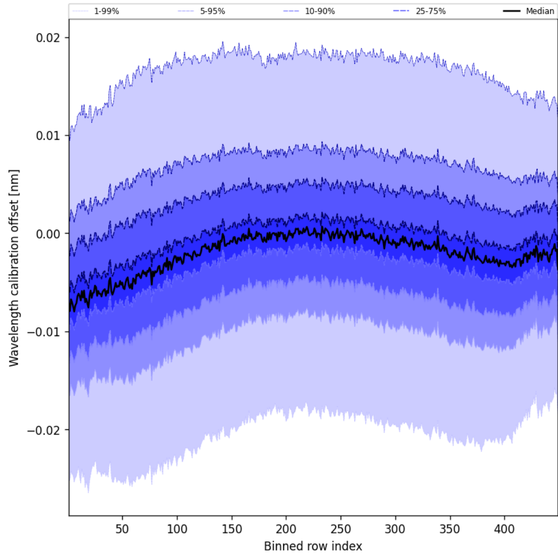
Figure 52: Along track statistics of “Wavelength calibration offset” for 2025-03-13 to 2025-03-14
