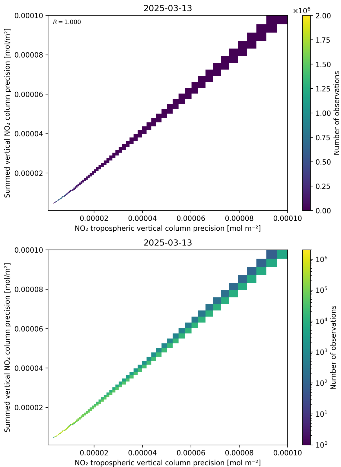
Figure 137: Scatter density plot of “NO 2 tropospheric vertical column precision” against “Summed vertical NO 2 column precision” for 2025-03-13 to 2025-03-14.
