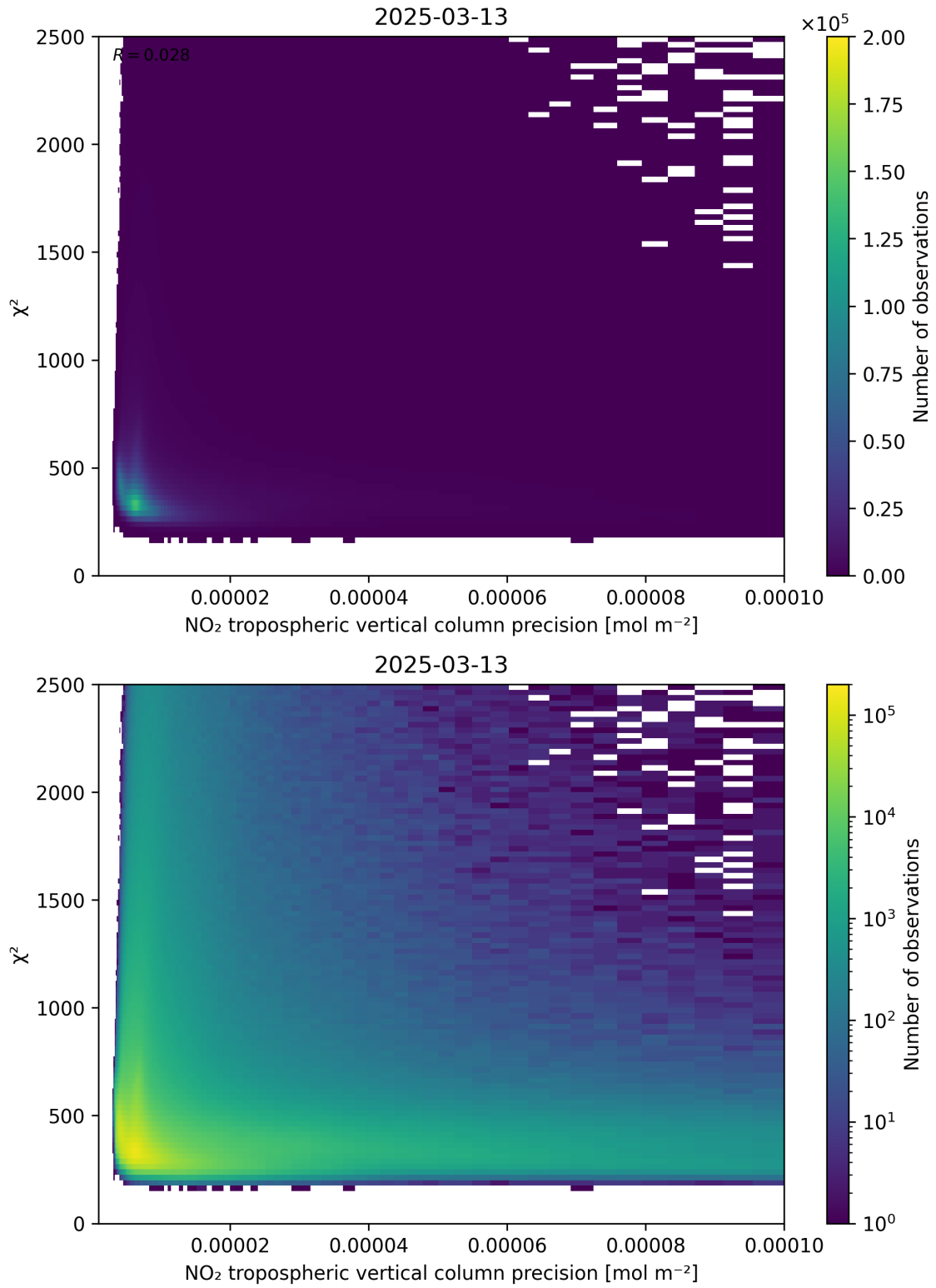
Figure 134: Scatter density plot of “NO 2 tropospheric vertical column precision” against “ \chi^2 ” for 2025-03-13 to 2025-03-14.
