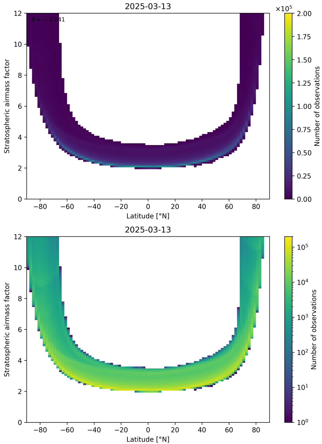
Figure 83: Scatter density plot of “Latitude” against “Stratospheric air mass factor” for 2025-03-13 to 2025-03-14.
