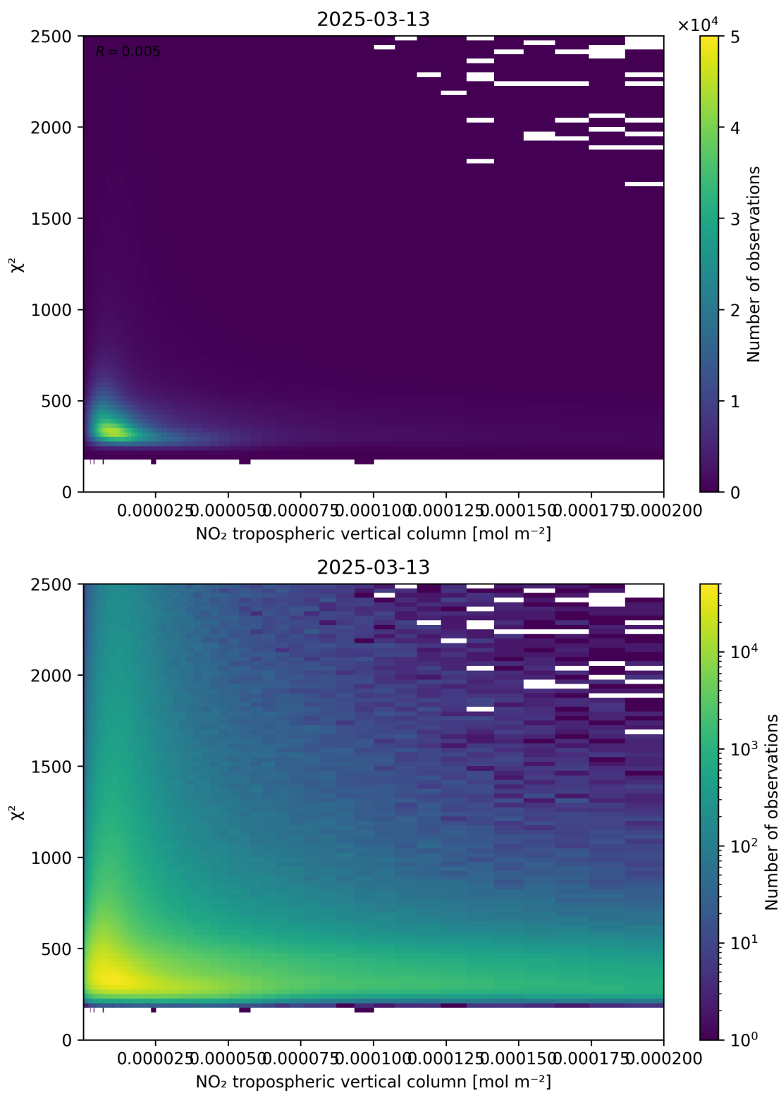
Figure 124: Scatter density plot of “NO 2 tropospheric vertical column” against “ \chi^2 ” for 2025-03-13 to 2025-03-14.
