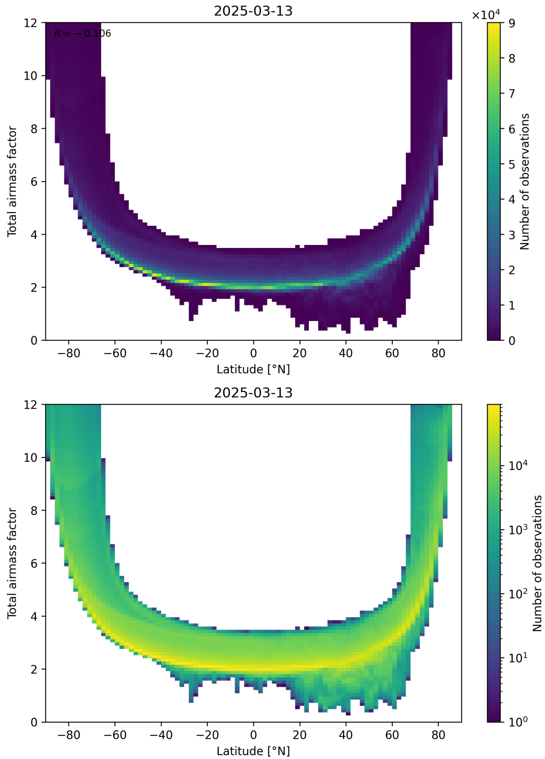
Figure 84: Scatter density plot of “Latitude” against “Total airmass factor” for 2025-03-13 to 2025-03-14.
