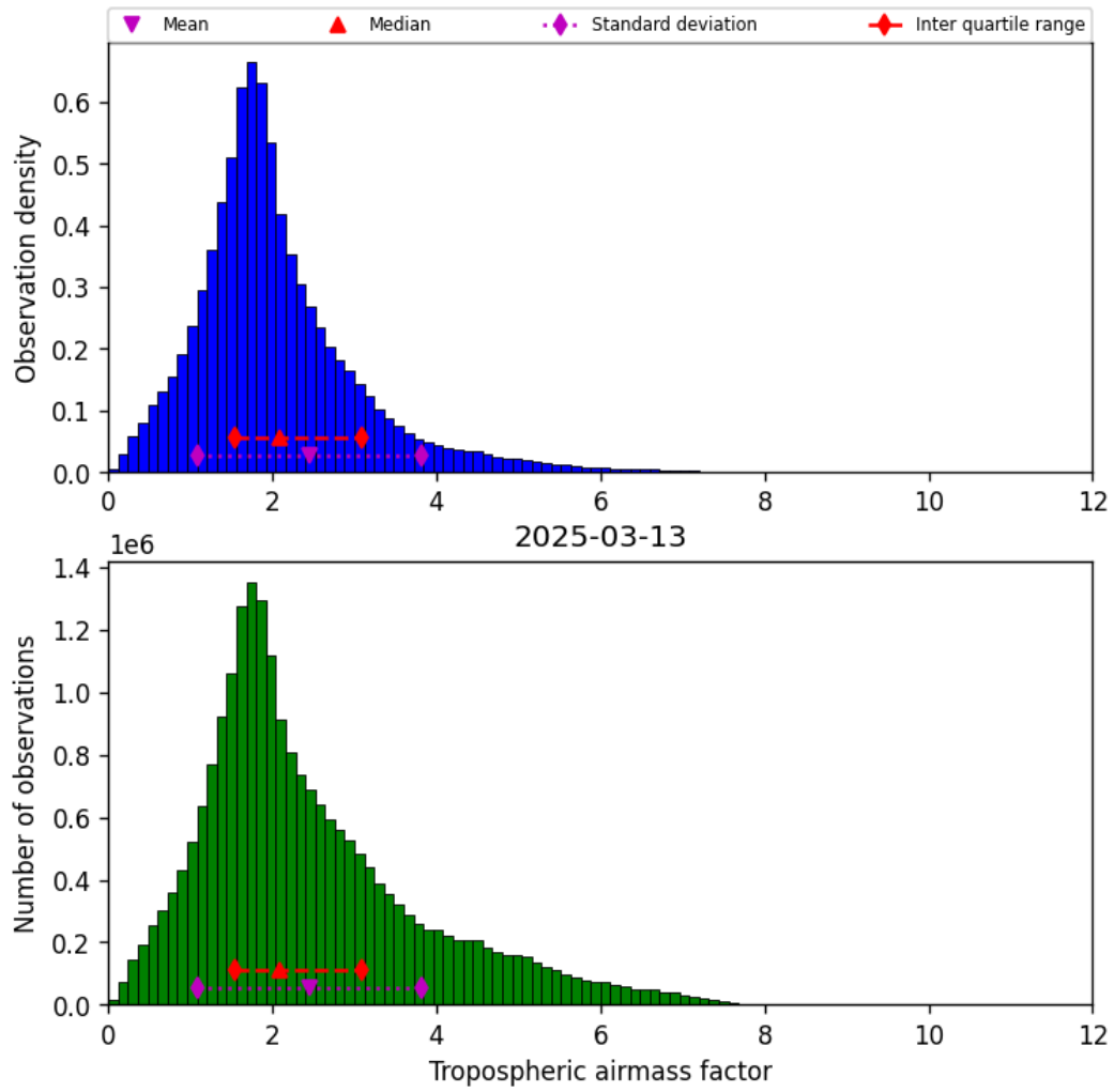
Figure 31: Histogram of “Tropospheric airmass factor” for 2025-03-13 to 2025-03-14
