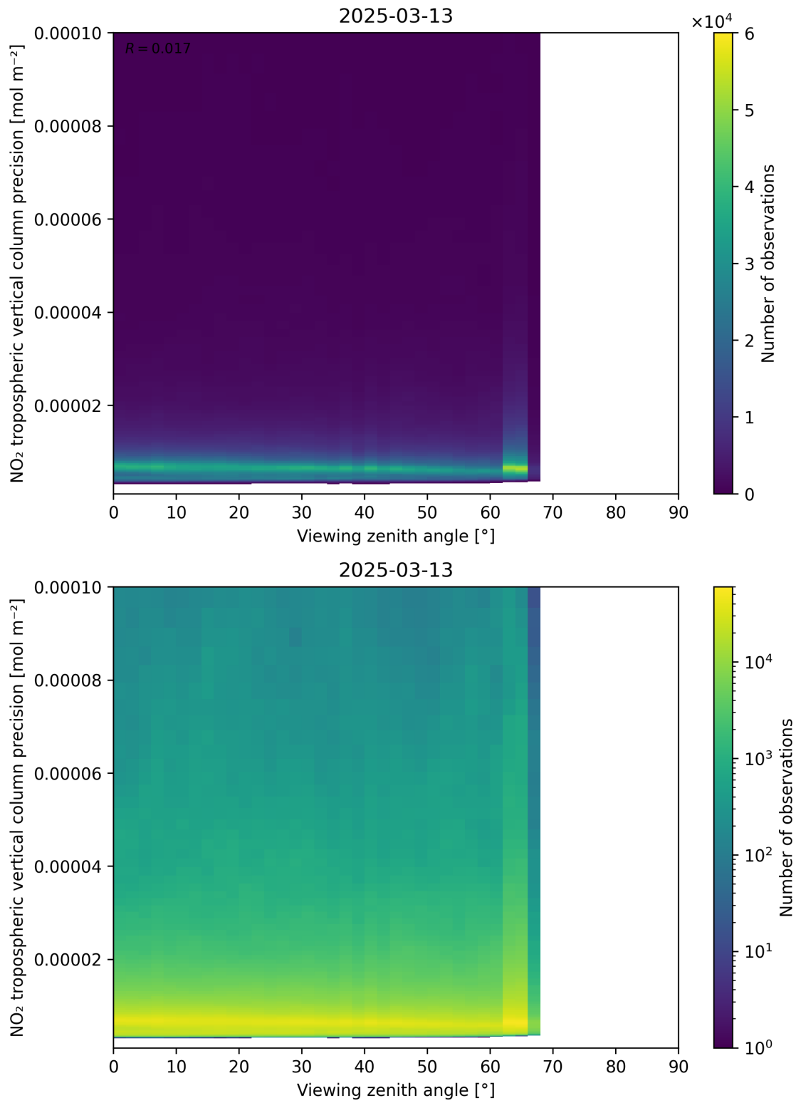
Figure 170: Scatter density plot of “Viewing zenith angle” against “NO 2 tropospheric vertical column precision” for 2025-03-13 to 2025-03-14.
