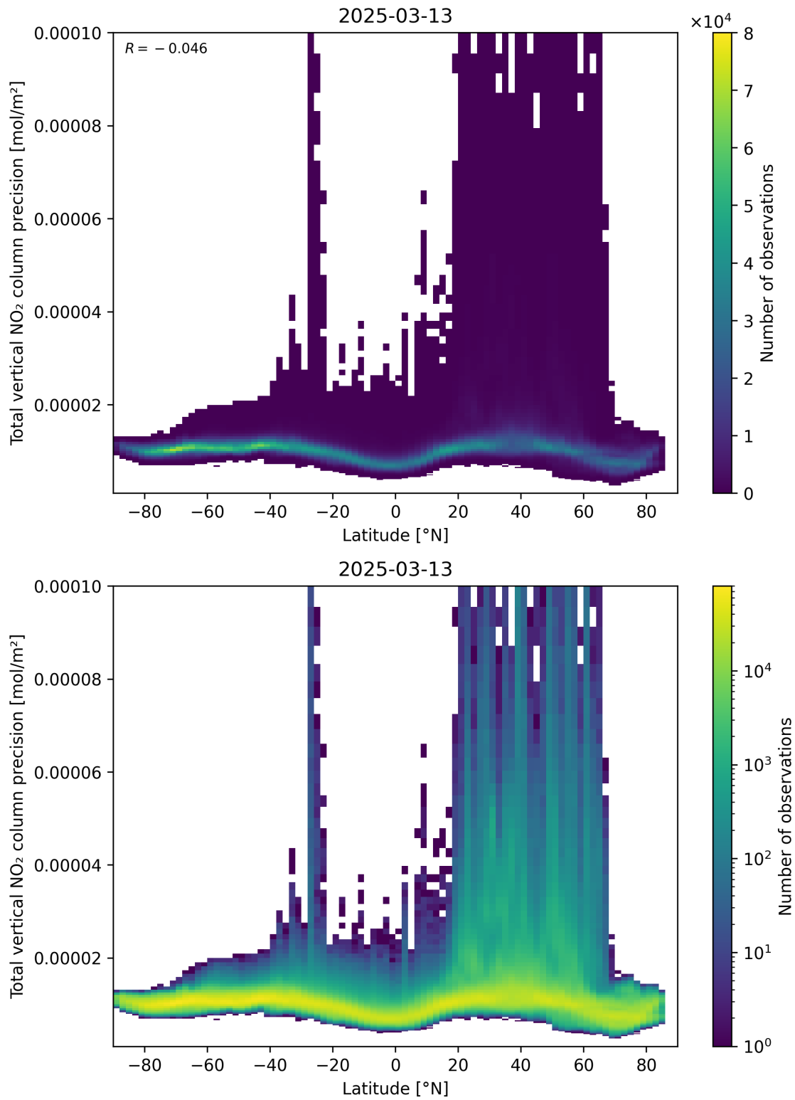
Figure 91: Scatter density plot of “Latitude” against “Total vertical NO 2 column precision” for 2025-03-13 to 2025-03-14.
