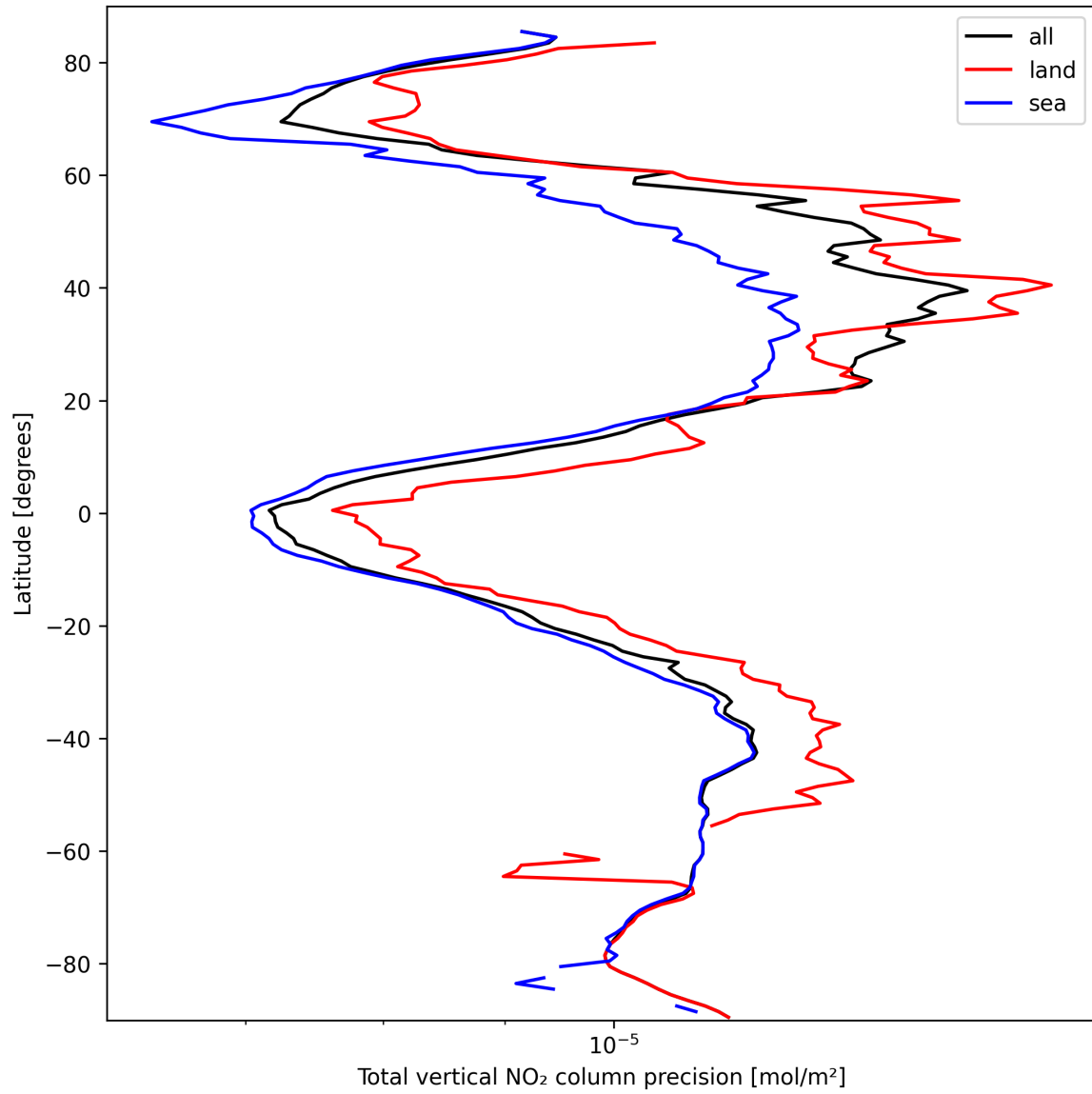
Figure 22: Zonal average of “Total vertical NO 2 column precision” for 2025-03-13 to 2025-03-14.
