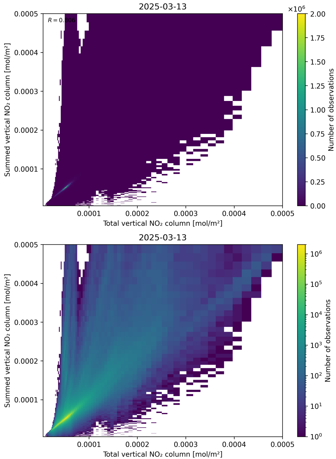
Figure 112: Scatter density plot of “Total vertical NO 2 column” against “Summed vertical NO 2 column” for 2025-03-13 to 2025-03-14.
