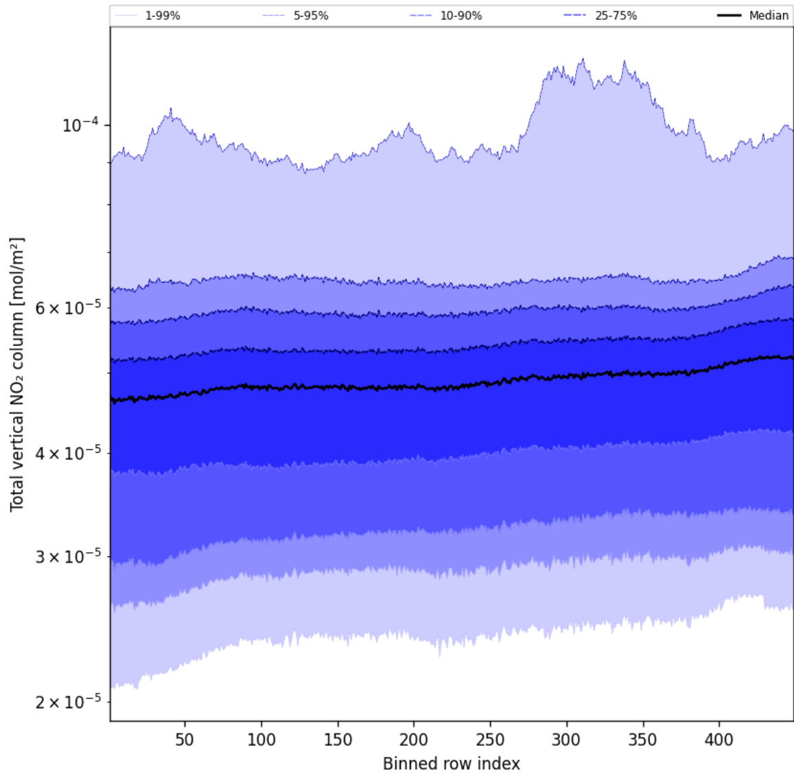
Figure 55: Along track statistics of “Total vertical NO 2 column” for 2025-03-13 to 2025-03-14
