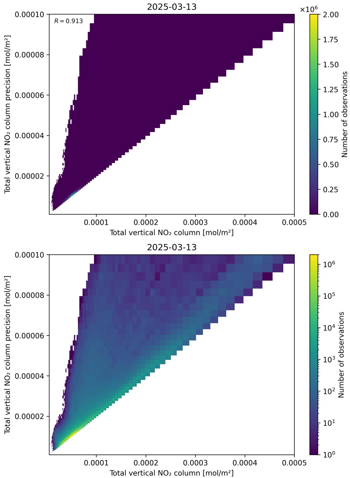
Figure 114: Scatter density plot of “Total vertical NO 2 column” against “Total vertical NO 2 column precision” for 2025-03-13 to 2025-03-14.
