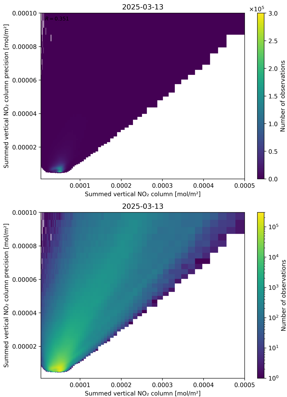
Figure 105: Scatter density plot of “Summed vertical NO 2 column” against “Summed vertical NO 2 column precision” for 2025-03-13 to 2025-03-14.
