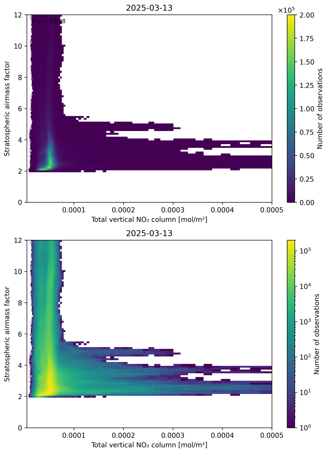
Figure 110: Scatter density plot of “Total vertical NO 2 column” against “Stratospheric airmass factor” for 2025-03-13 to 2025-03-14.
