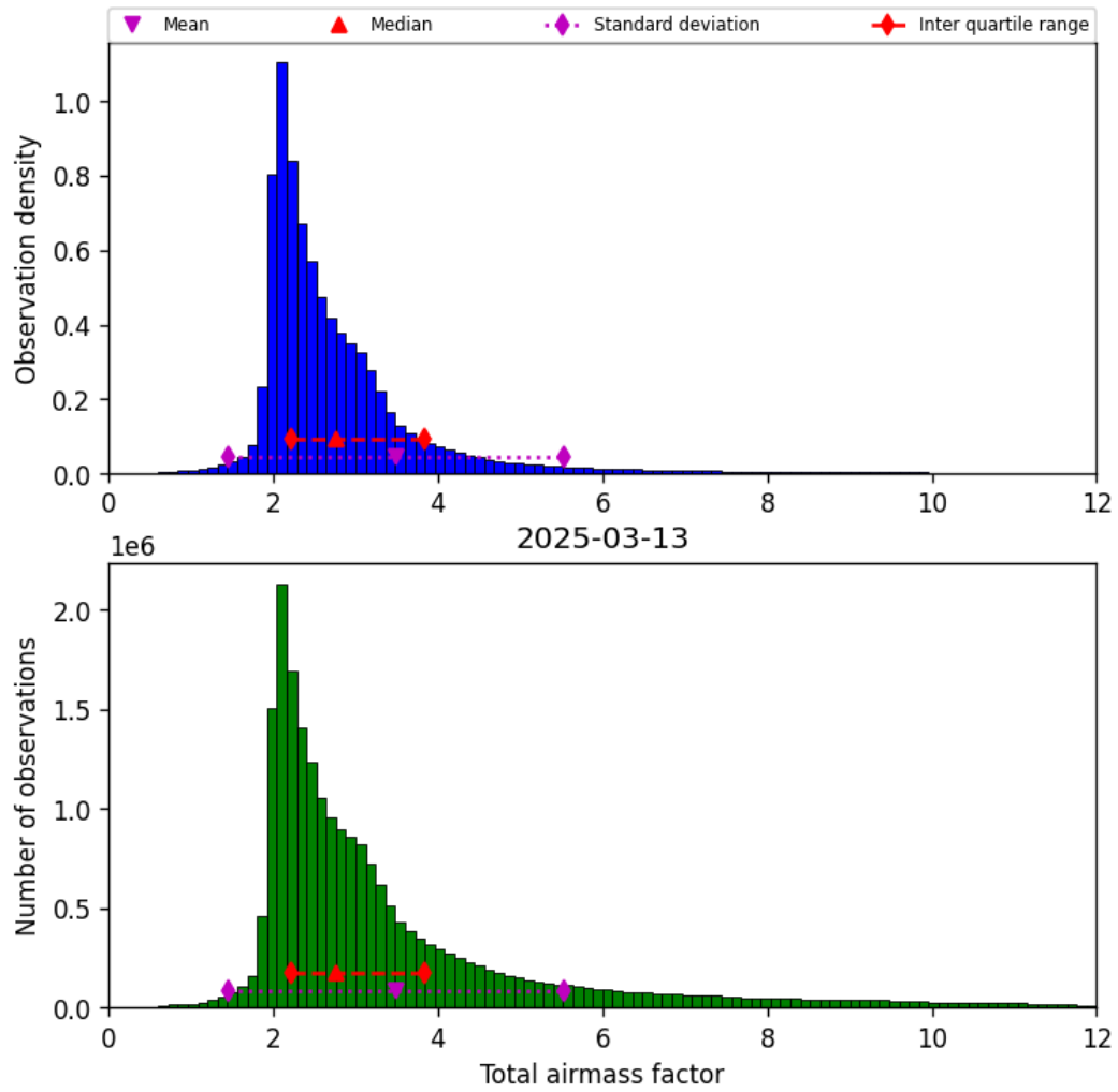
Figure 32: Histogram of “Total airmass factor” for 2025-03-13 to 2025-03-14
