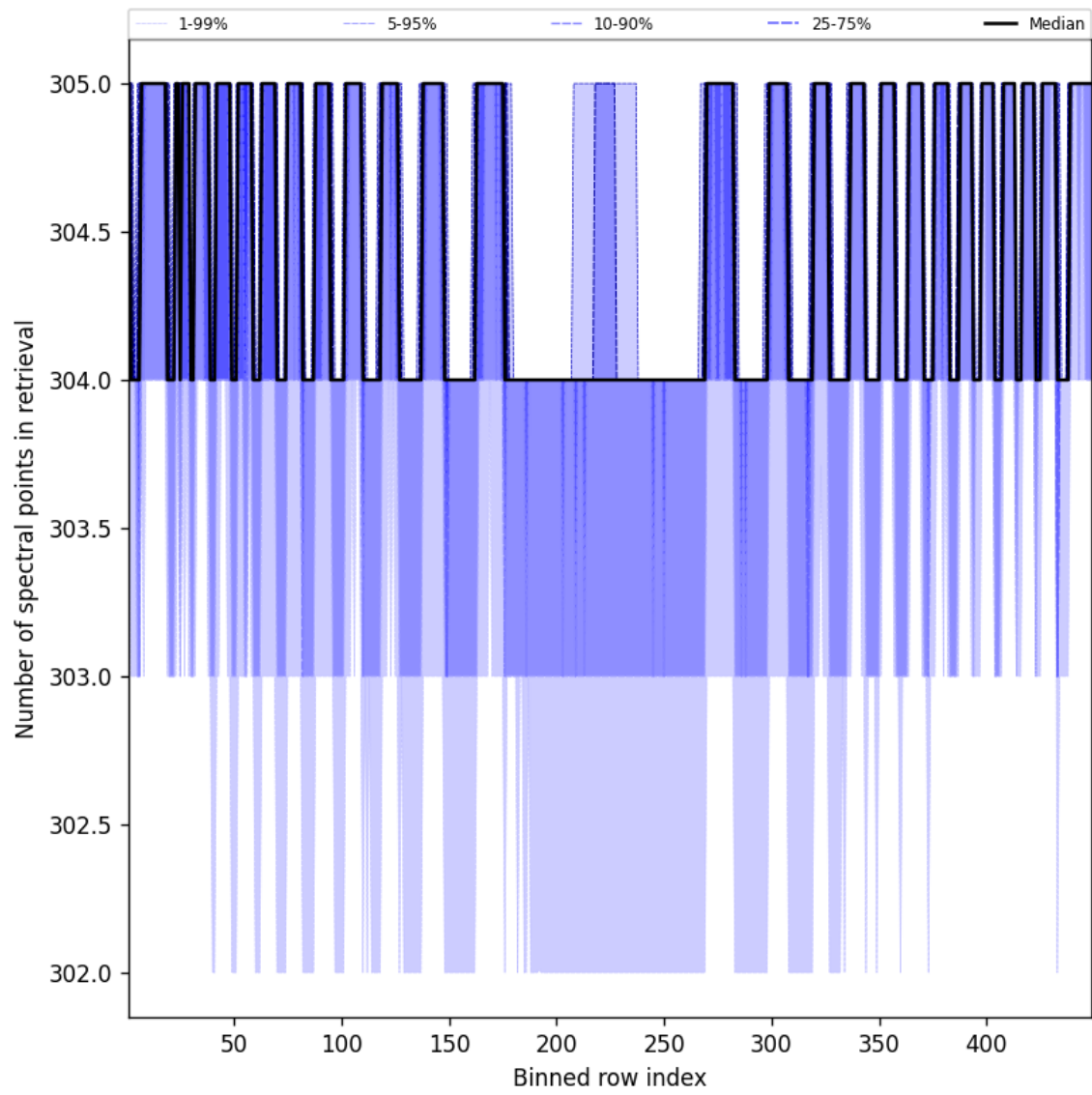
Figure 50: Along track statistics of “Number of spectral points in retrieval” for 2025-03-13 to 2025-03-14
