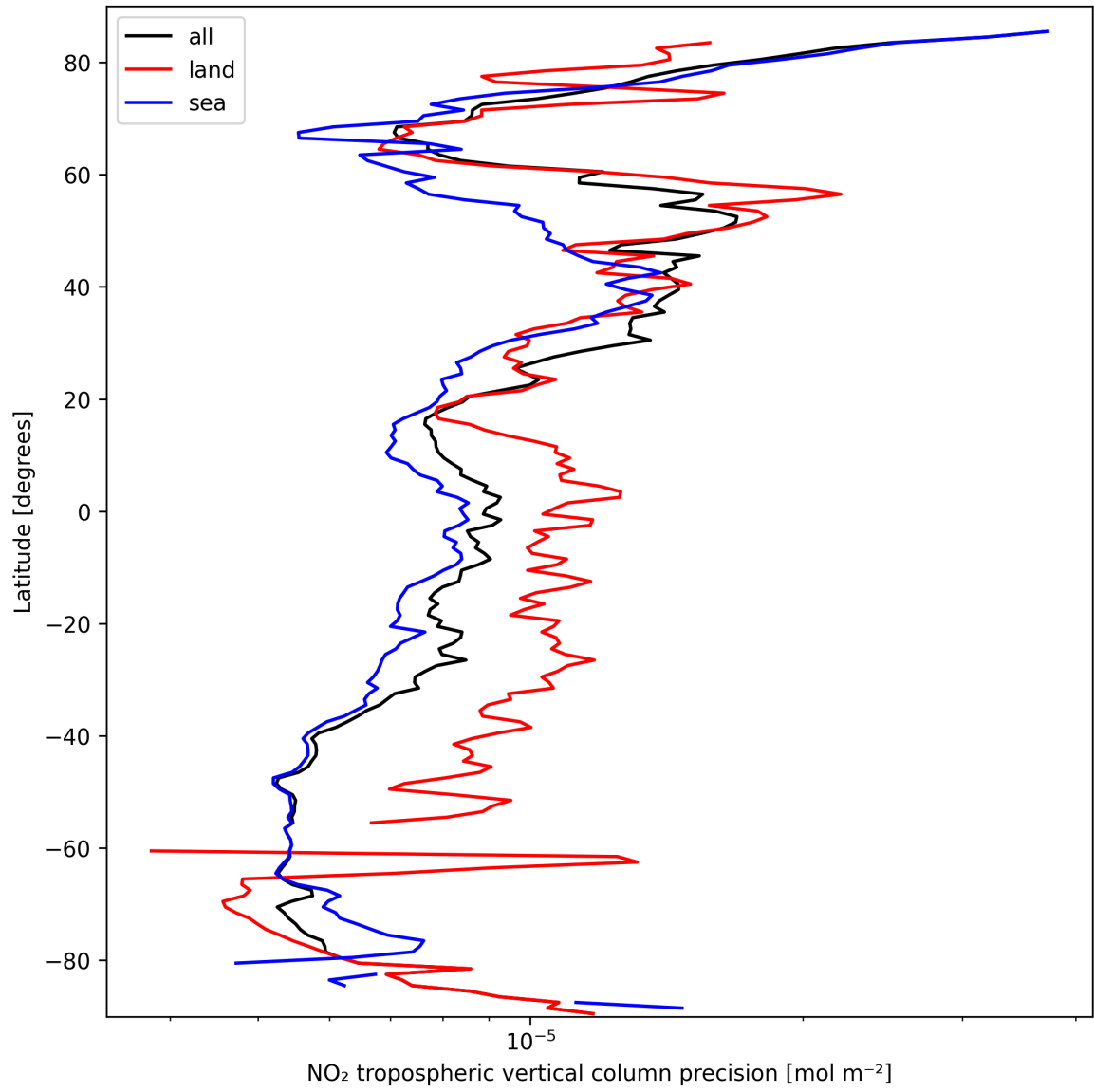
Figure 13: Zonal average of “NO 2 tropospheric vertical column precision” for 2025-03-13 to 2025-03-14.
