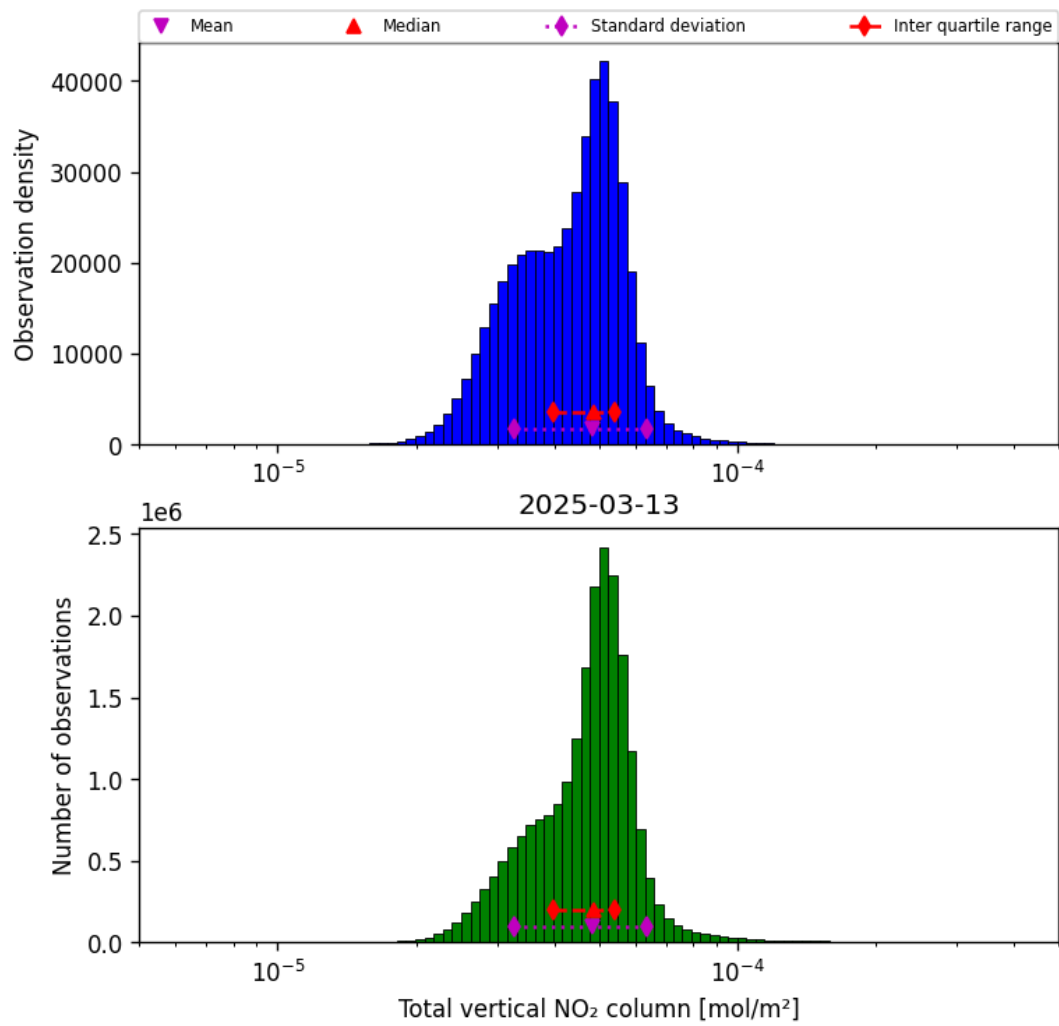
Figure 38: Histogram of “Total vertical NO 2 column” for 2025-03-13 to 2025-03-14
