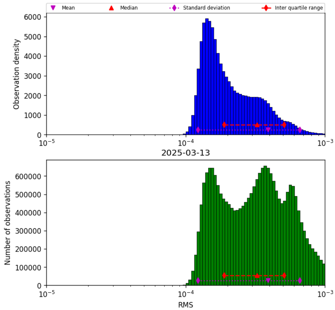
Figure 43: Histogram of “RMS” for 2025-03-13 to 2025-03-14
