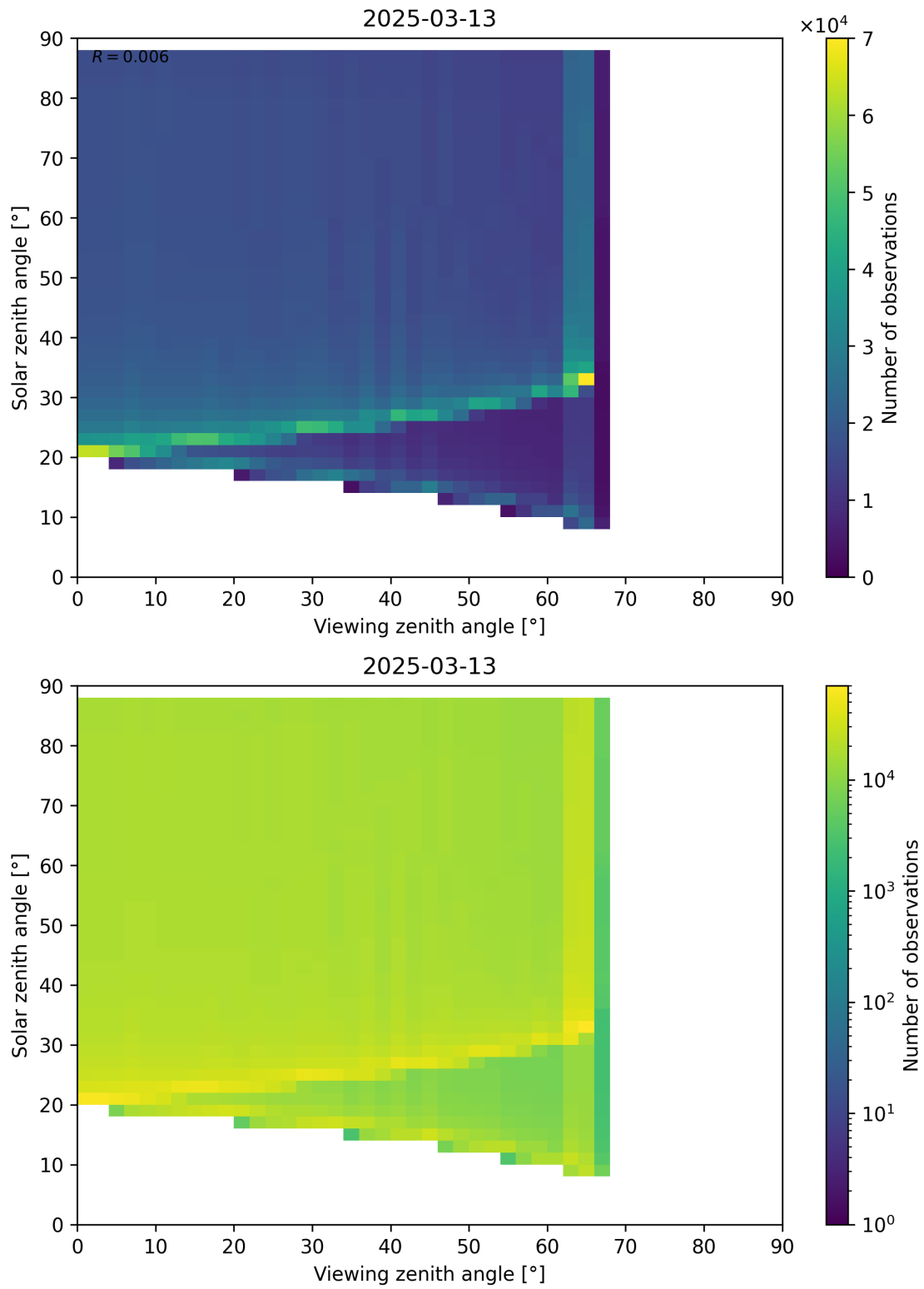
Figure 172: Scatter density plot of “Viewing zenith angle” against “Solar zenith angle” for 2025-03-13 to 2025-03-14.
