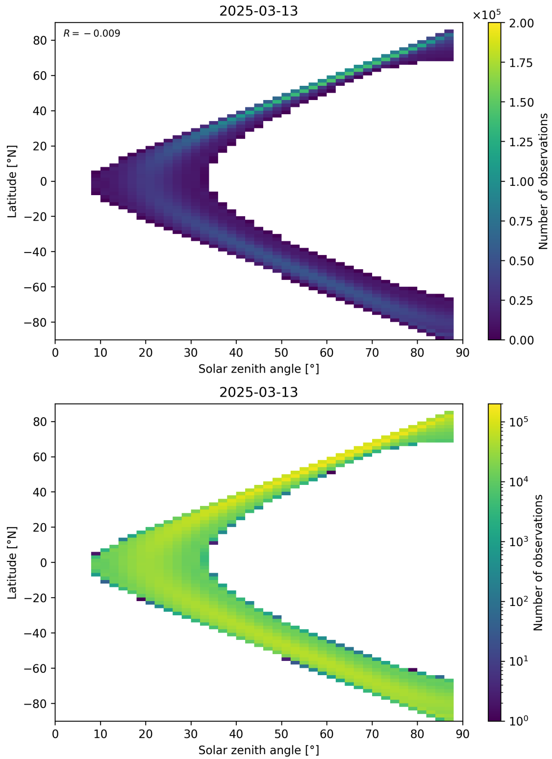
Figure 149: Scatter density plot of “Solar zenith angle” against “Latitude” for 2025-03-13 to 2025-03-14.
