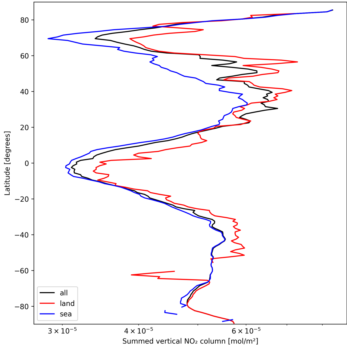
Figure 23: Zonal average of “Summed vertical NO 2 column” for 2025-03-13 to 2025-03-14.
