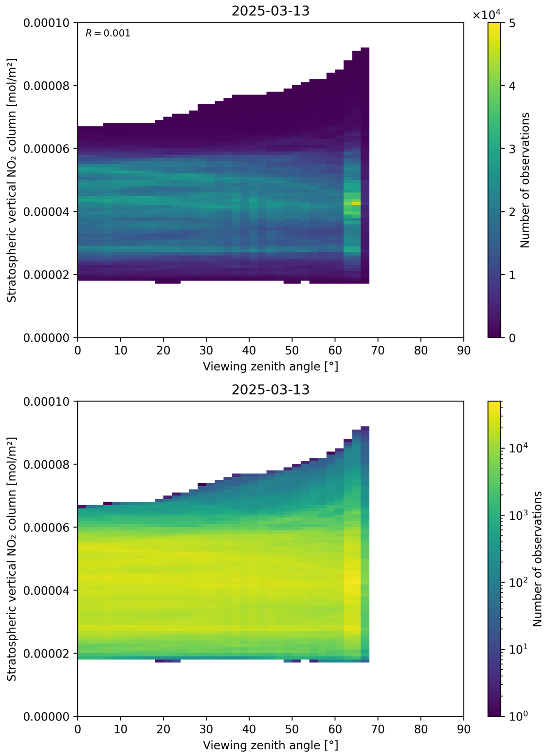
Figure 164: Scatter density plot of “Viewing zenith angle” against “Stratospheric vertical NO 2 column” for 2025-03-13 to 2025-03-14.
