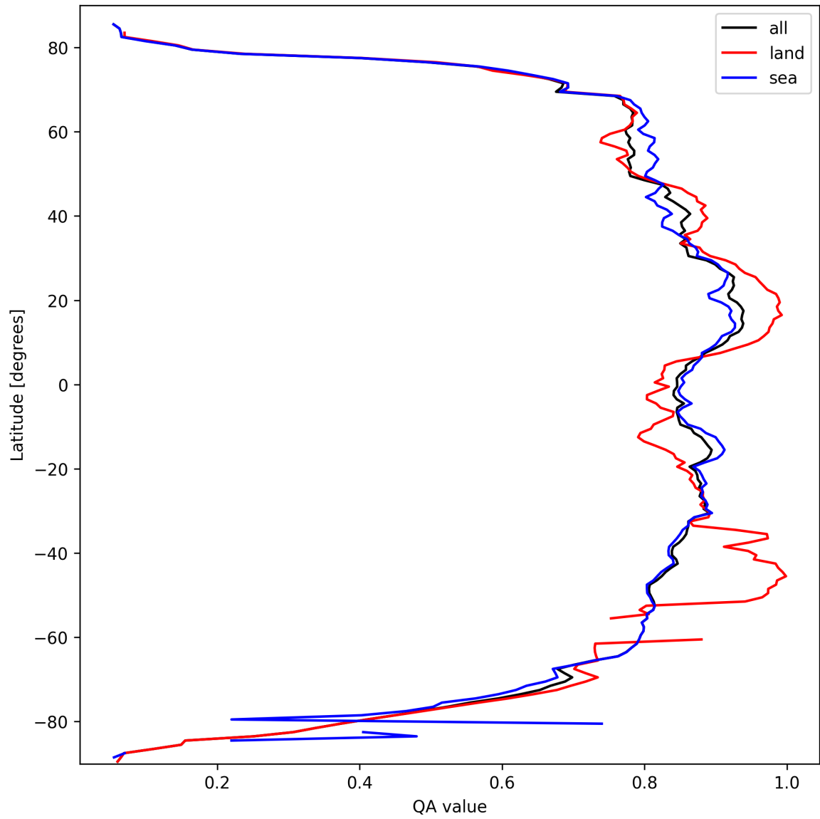
Figure 11: Zonal average of “QA value” for 2025-03-13 to 2025-03-14.
