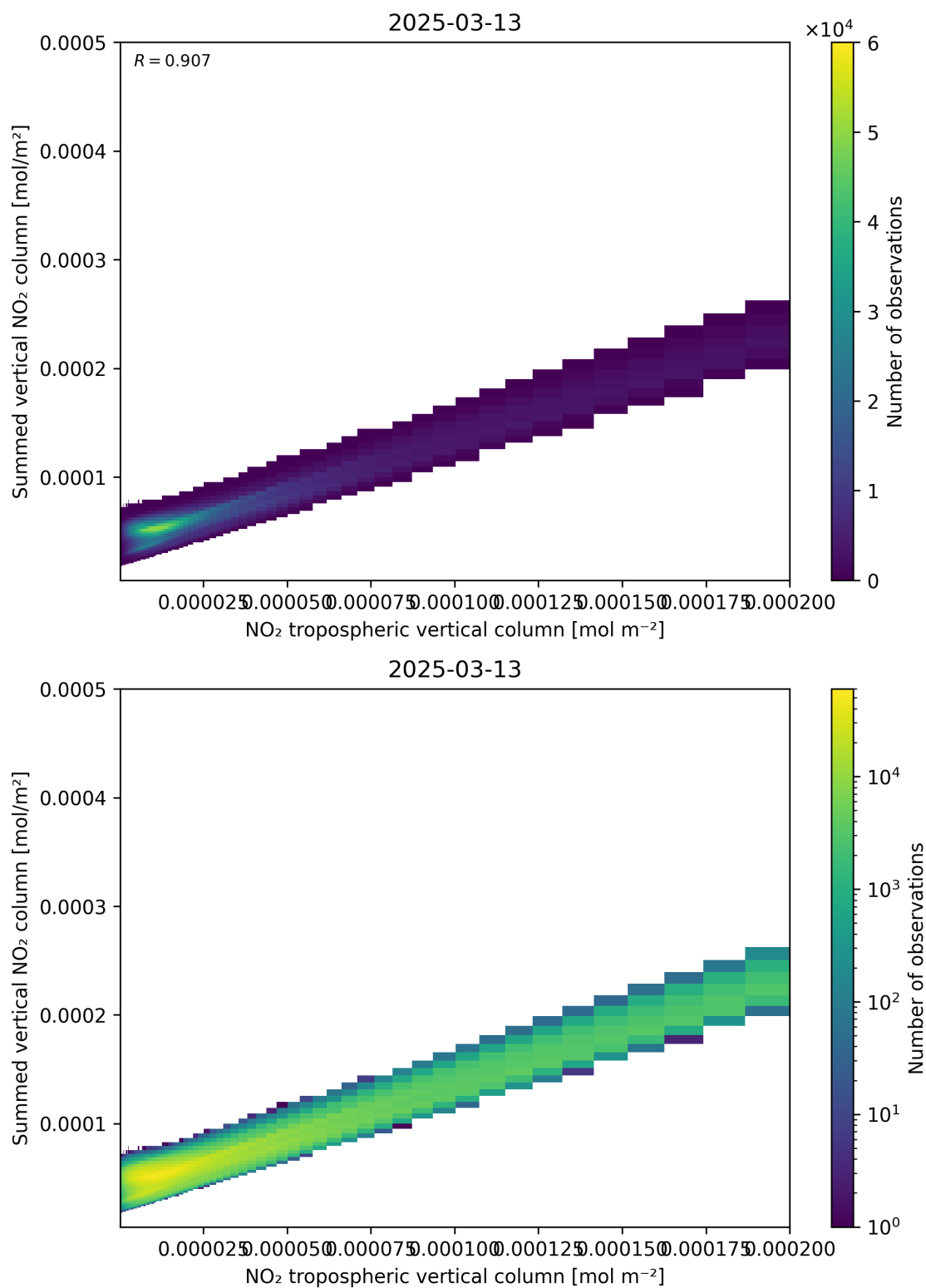
Figure 126: Scatter density plot of “NO 2 tropospheric vertical column” against “Summed vertical NO 2 column” for 2025-03-13 to 2025-03-14.
