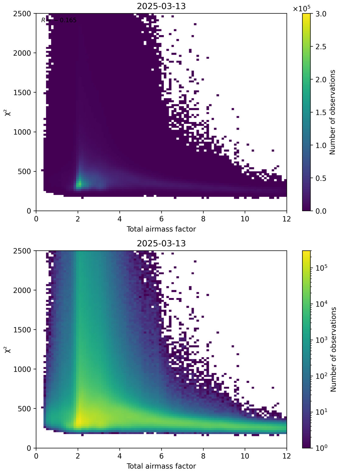
Figure 63: Scatter density plot of “Total airmass factor” against “ \chi^2 ” for 2025-03-13 to 2025-03-14.
