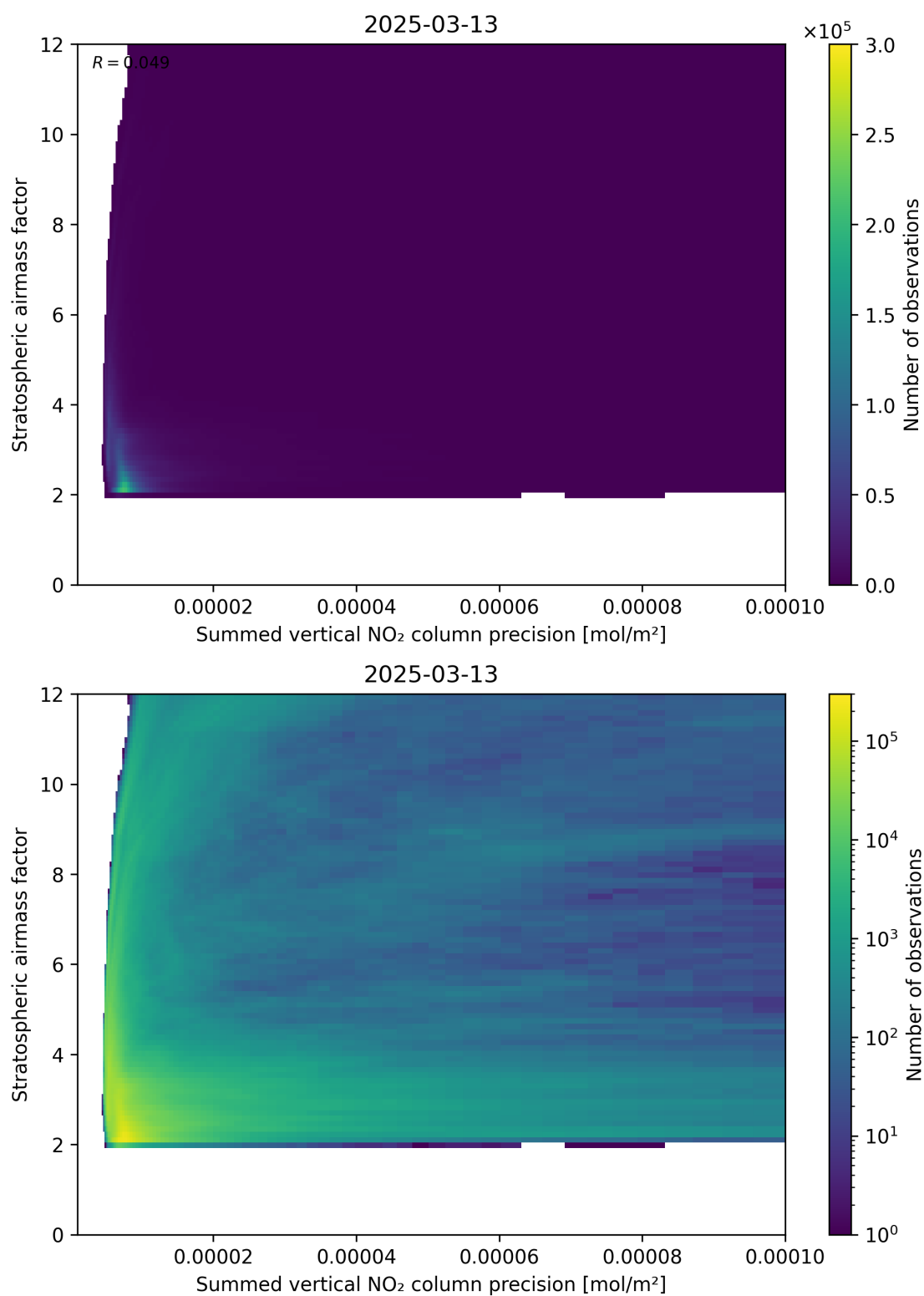
Figure 106: Scatter density plot of “Summed vertical NO 2 column precision” against “Stratospheric airmass factor” for 2025-03-13 to 2025-03-14.
