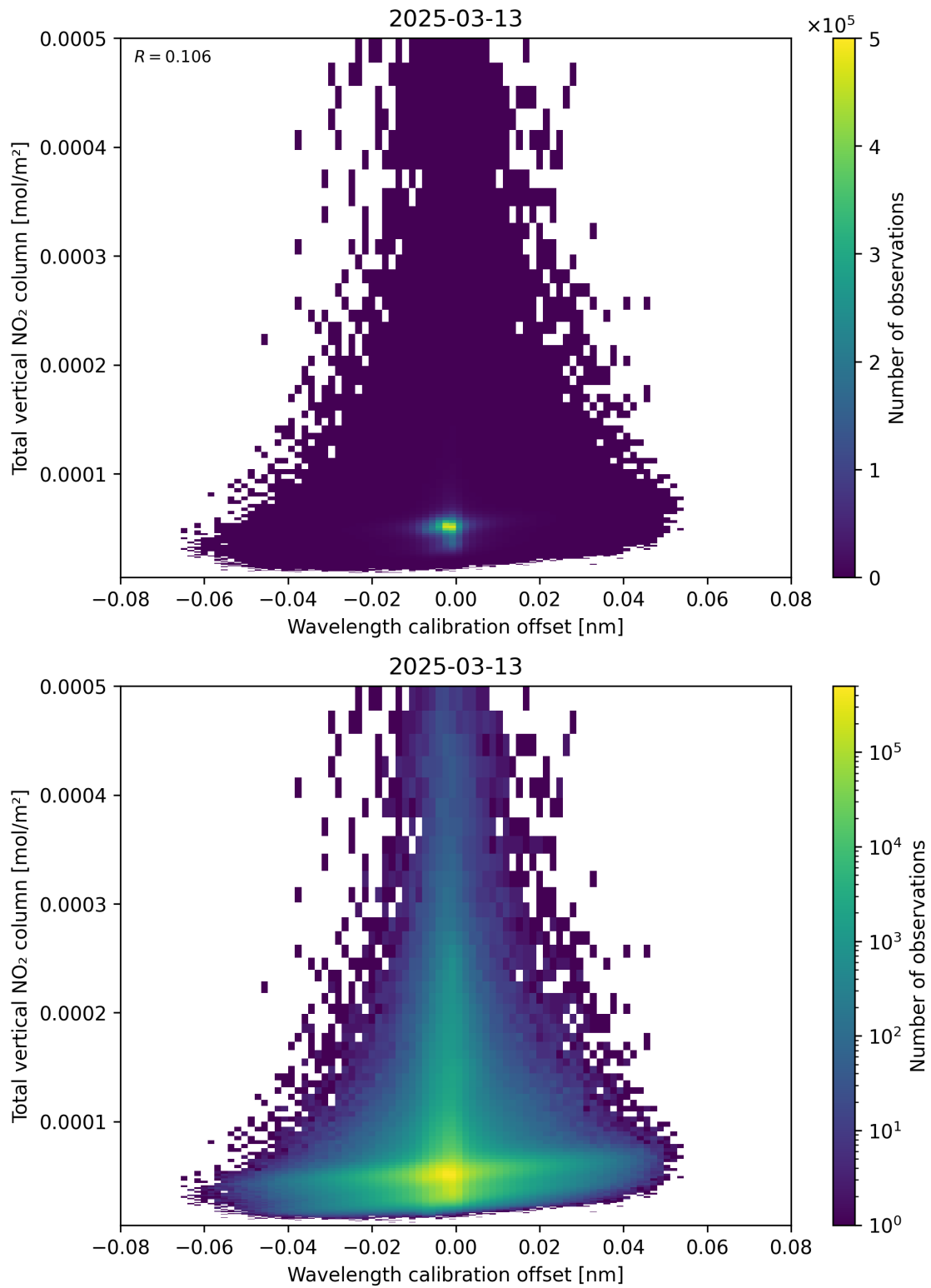
Figure 179: Scatter density plot of “Wavelength calibration offset” against “Total vertical NO 2 column” for 2025-03-13 to 2025-03-14.
