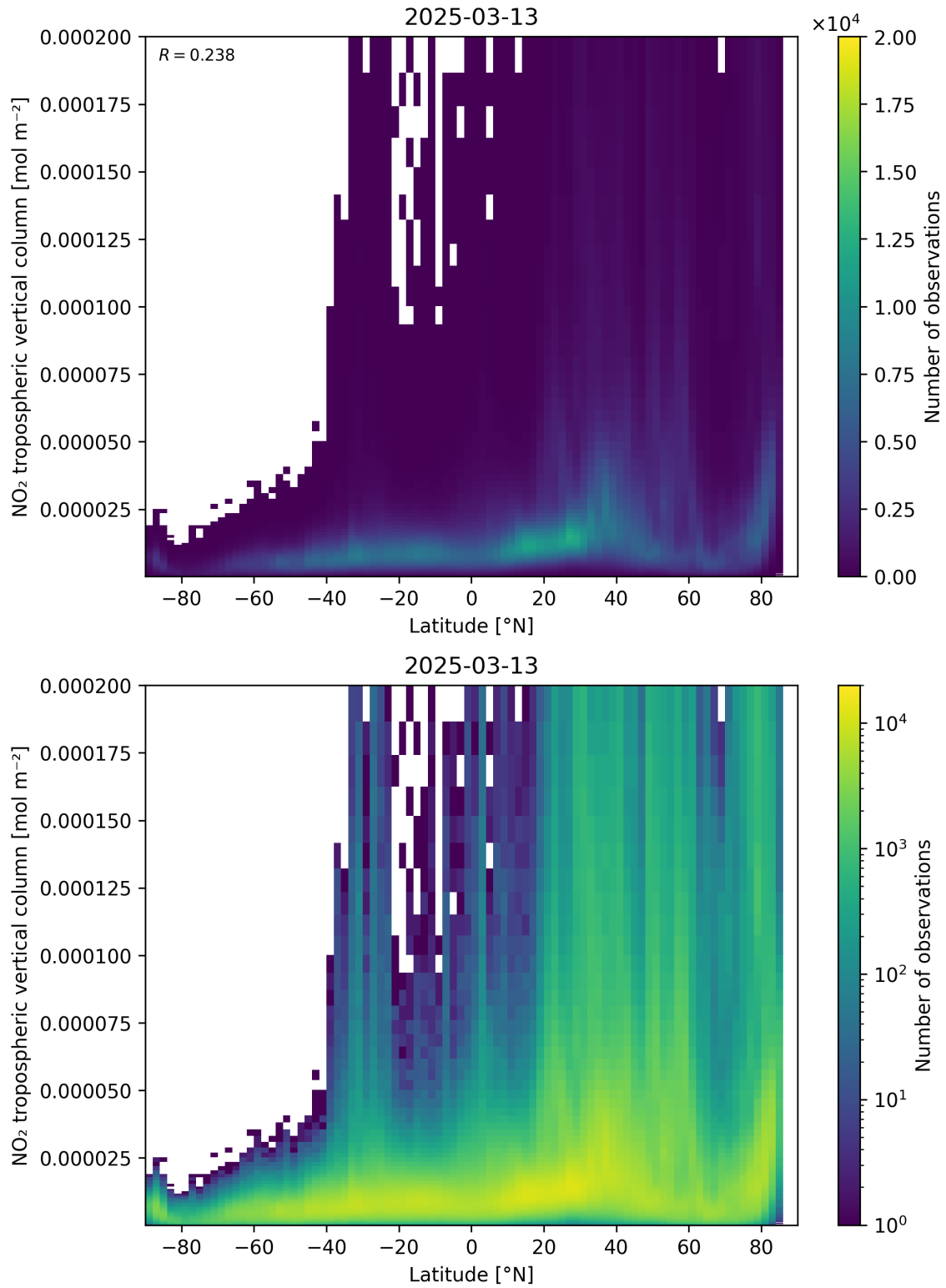
Figure 92: Scatter density plot of “Latitude” against “NO 2 tropospheric vertical column” for 2025-03-13 to 2025-03-14.
