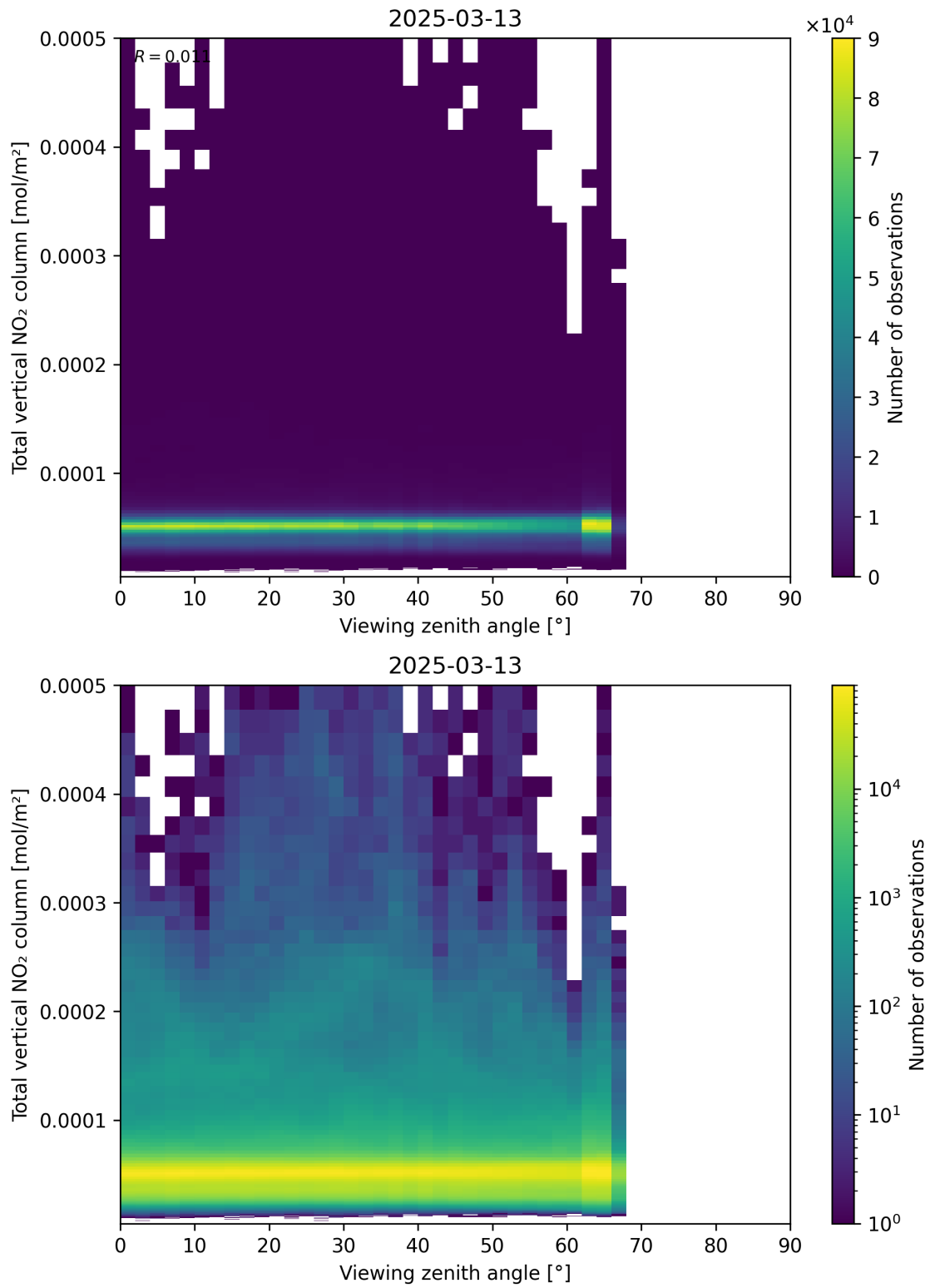
Figure 167: Scatter density plot of “Viewing zenith angle” against “Total vertical NO 2 column” for 2025-03-13 to 2025-03-14.
