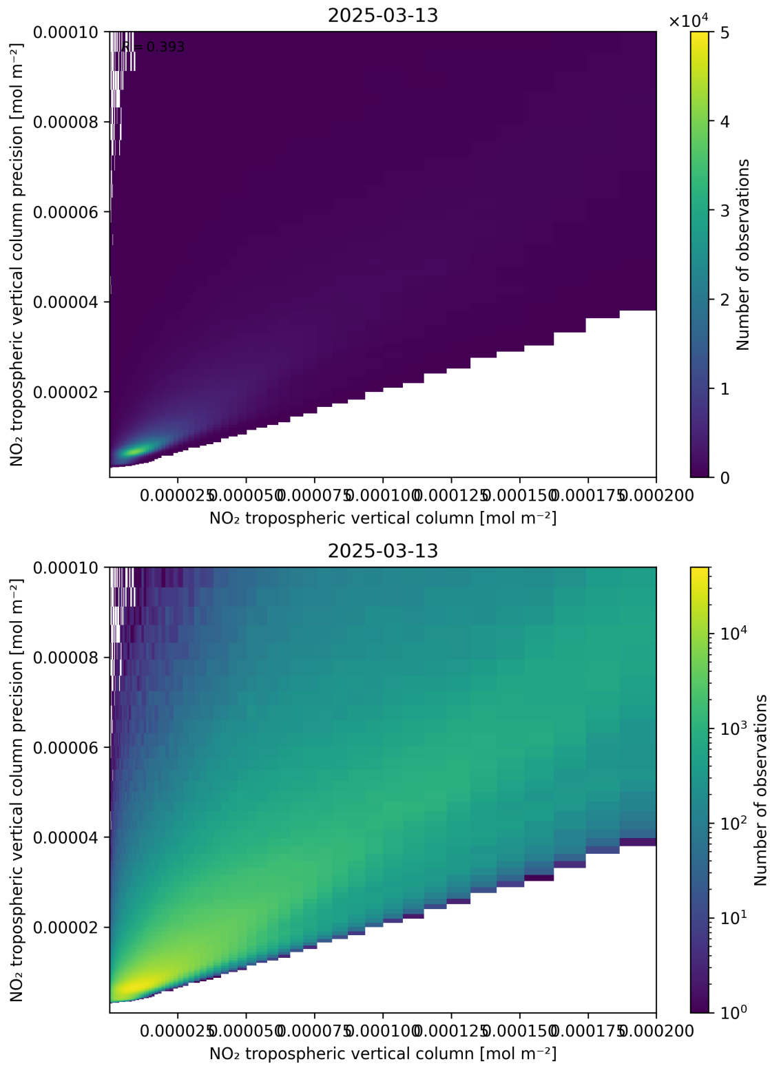
Figure 130: Scatter density plot of “NO 2 tropospheric vertical column” against “NO 2 tropospheric vertical column precision” for 2025-03-13 to 2025-03-14.
