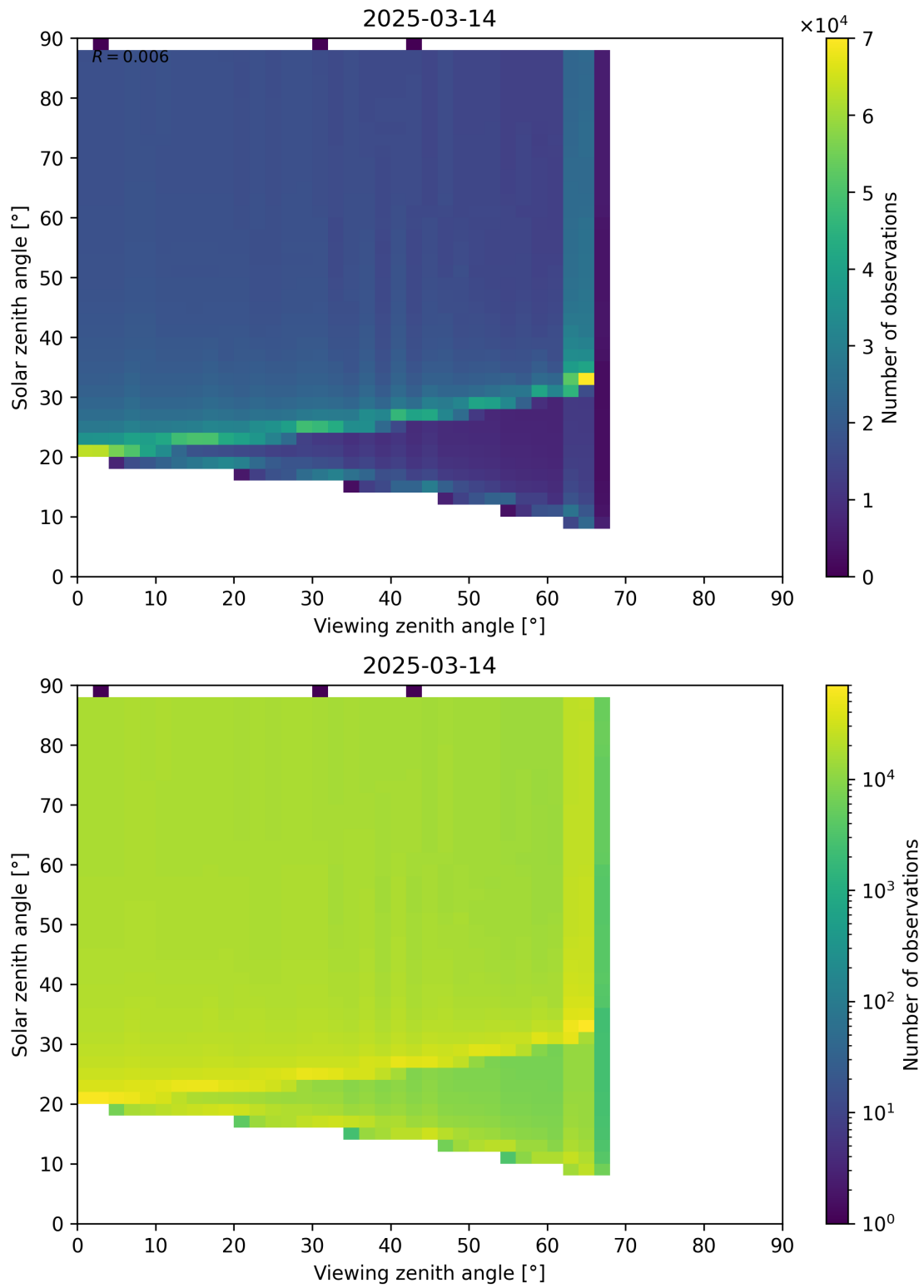
Figure 172: Scatter density plot of “Viewing zenith angle” against “Solar zenith angle” for 2025-03-14 to 2025-03-15.
