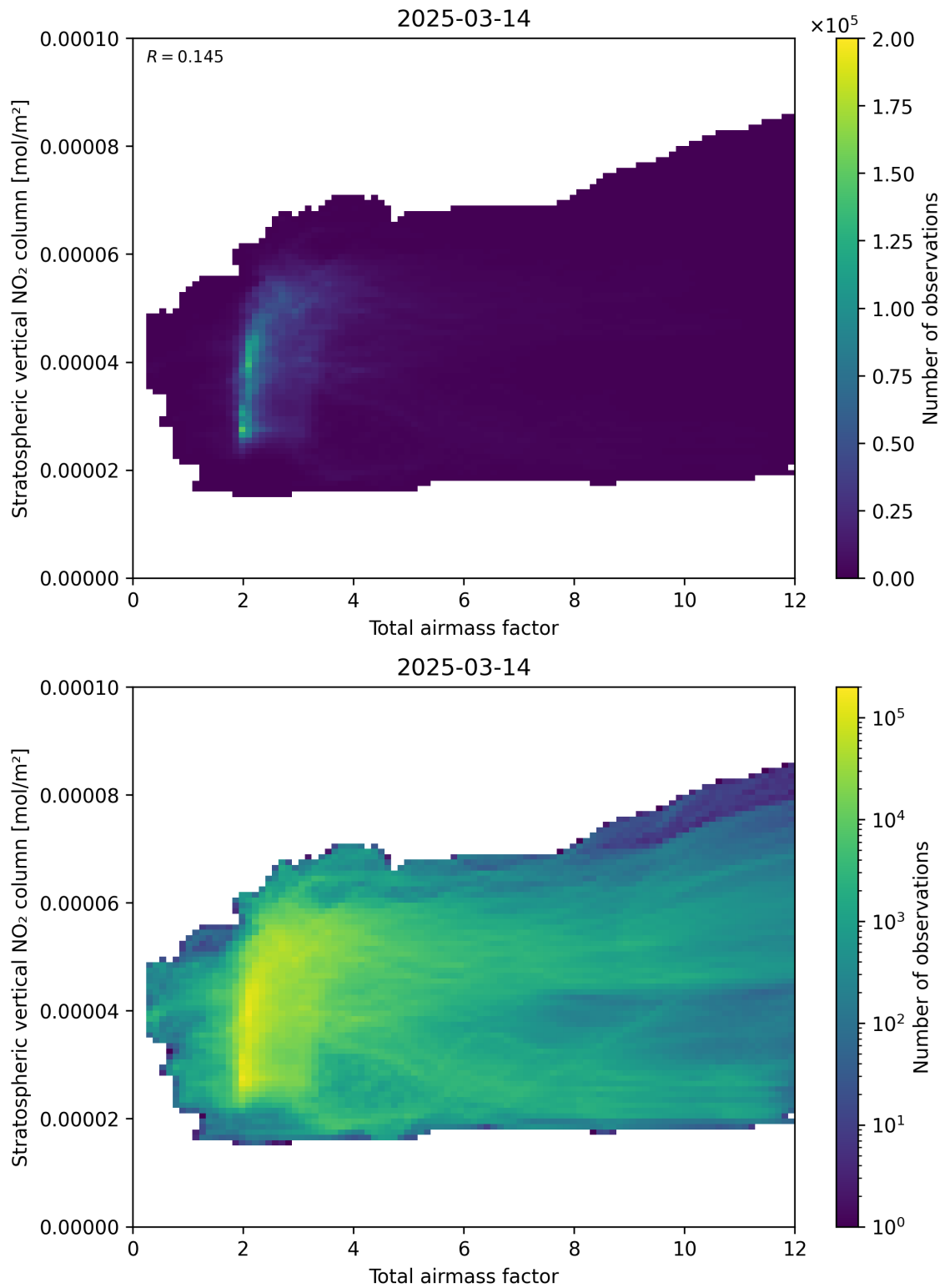
Figure 64: Scatter density plot of “Total airmass factor” against “Stratospheric vertical NO 2 column” for 2025-03-14 to 2025-03-15.
