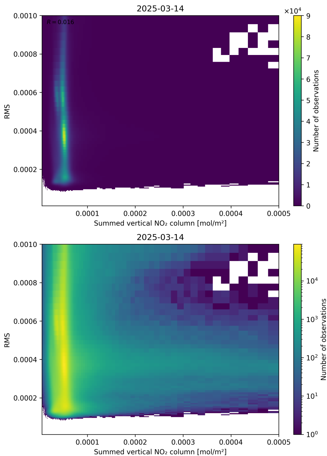
Figure 109: Scatter density plot of “Summed vertical NO 2 column” against “RMS” for 2025-03-14 to 2025-03-15.
