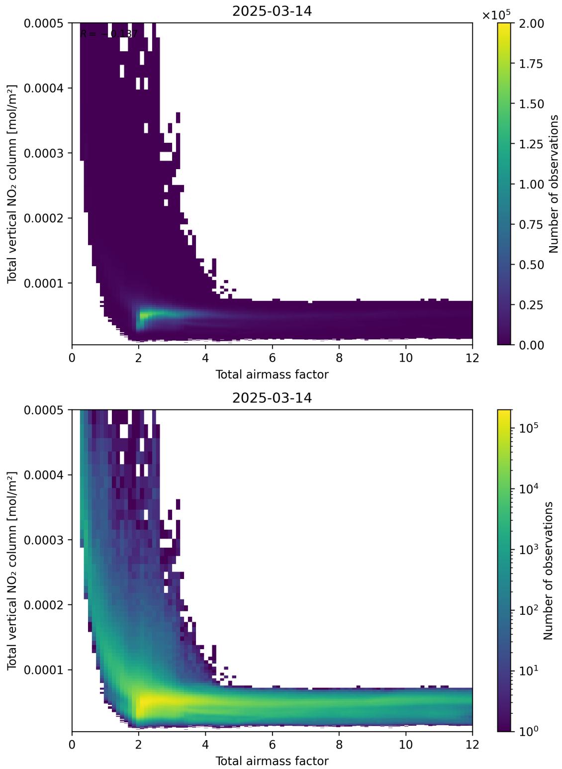
Figure 67: Scatter density plot of “Total airmass factor” against “Total vertical NO 2 column” for 2025-03-14 to 2025-03-15.
