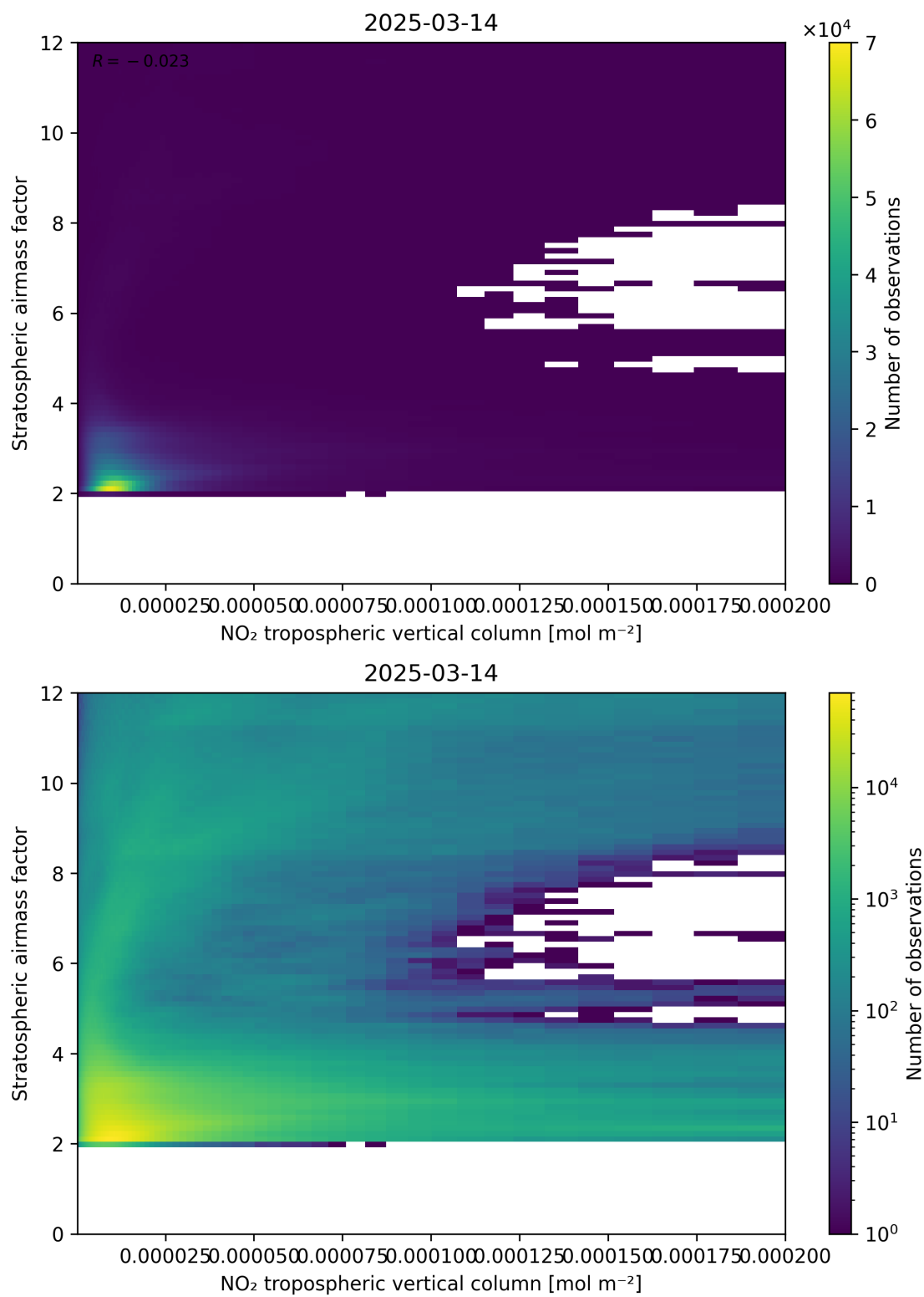
Figure 121: Scatter density plot of “NO 2 tropospheric vertical column” against “Stratospheric airmass factor” for 2025-03-14 to 2025-03-15.
