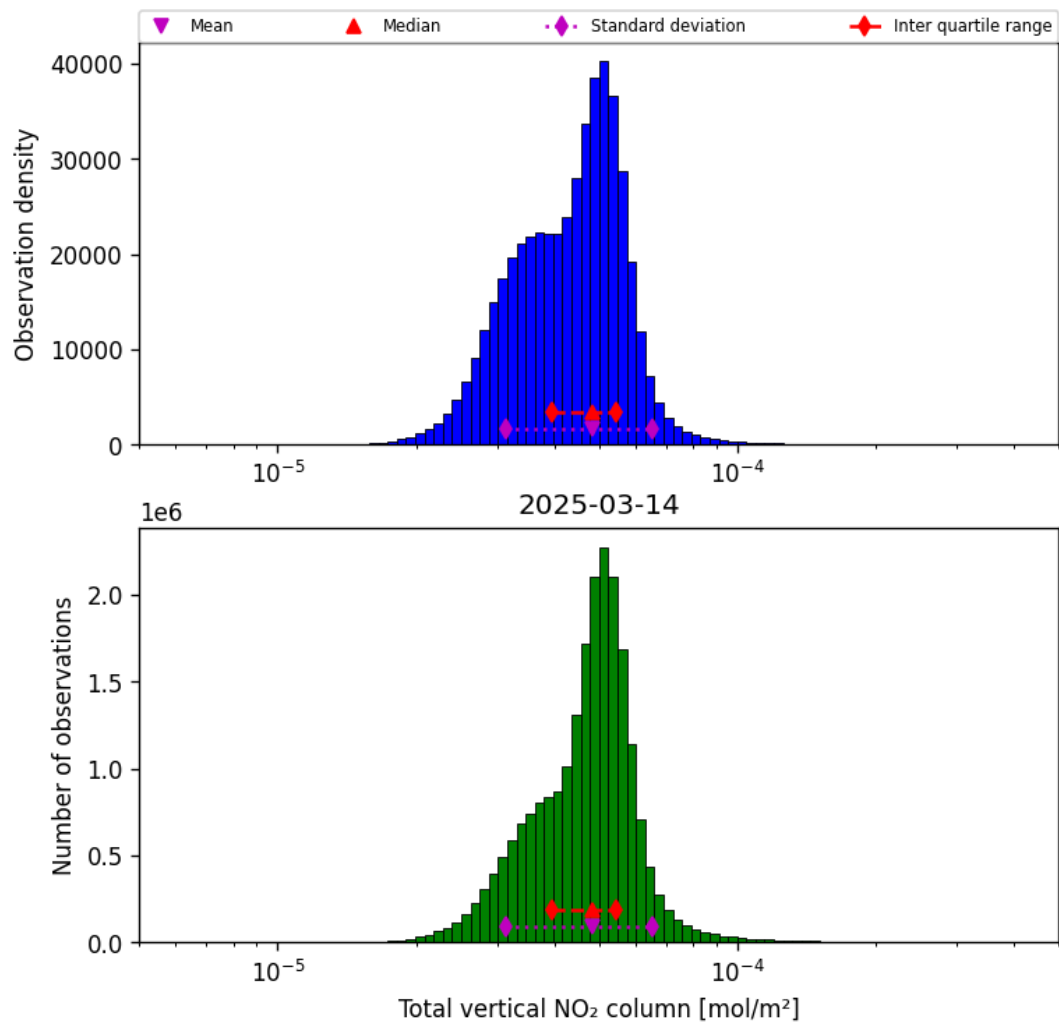
Figure 38: Histogram of “Total vertical NO 2 column” for 2025-03-14 to 2025-03-15
