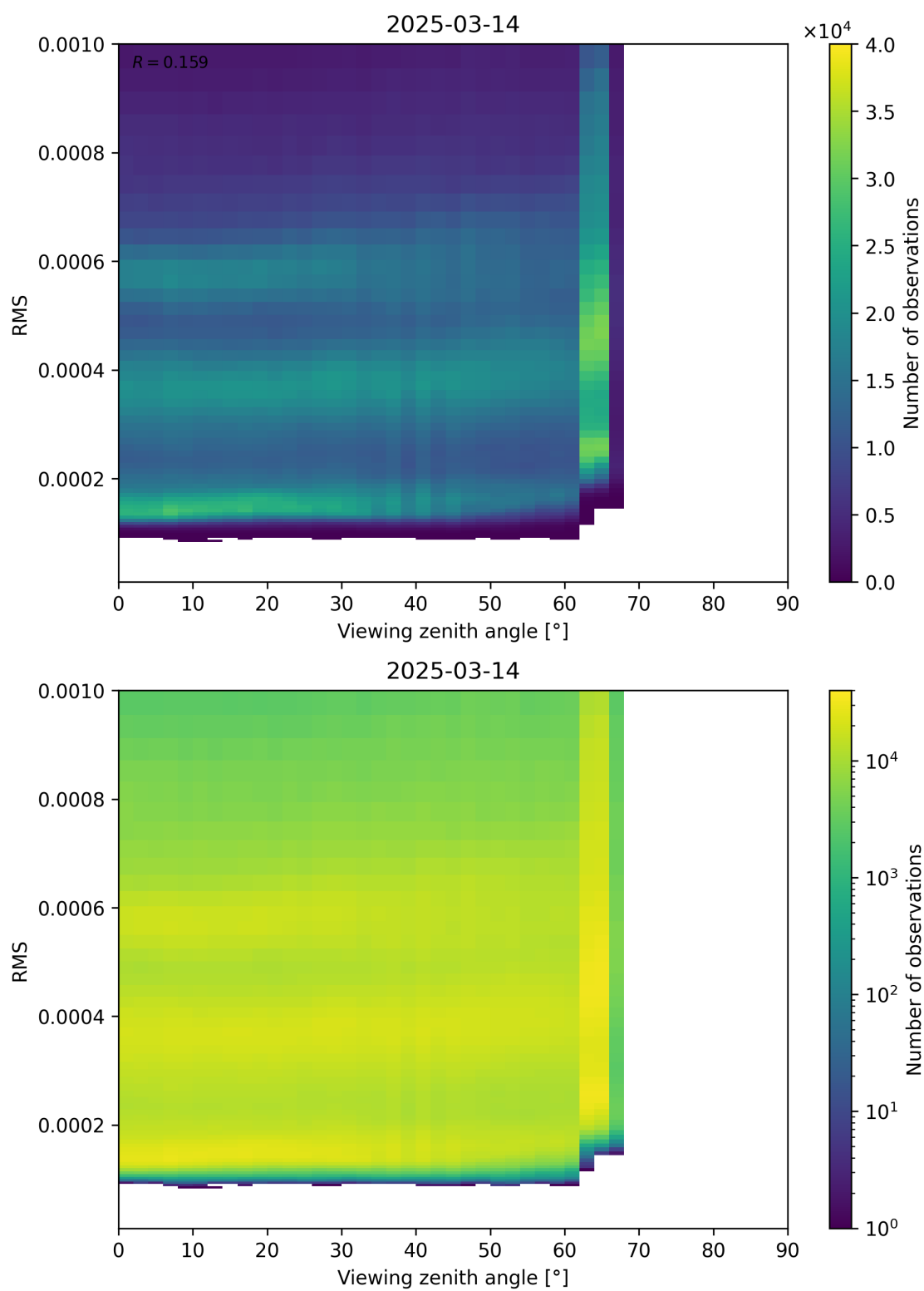
Figure 171: Scatter density plot of “Viewing zenith angle” against “RMS” for 2025-03-14 to 2025-03-15.
