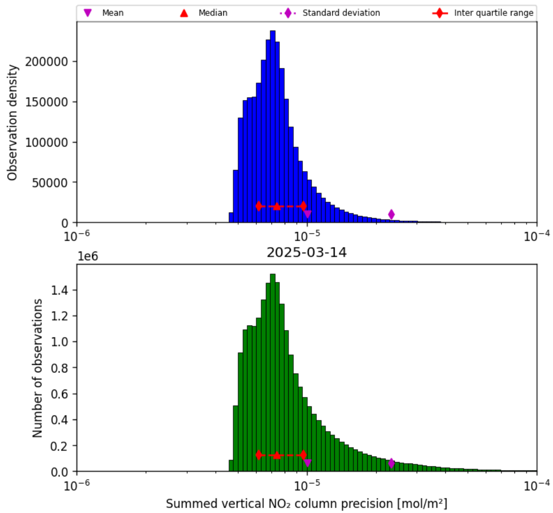
Figure 41: Histogram of "Summed vertical NO 2 column precision" for 2025-03-14 to 2025-03-15
