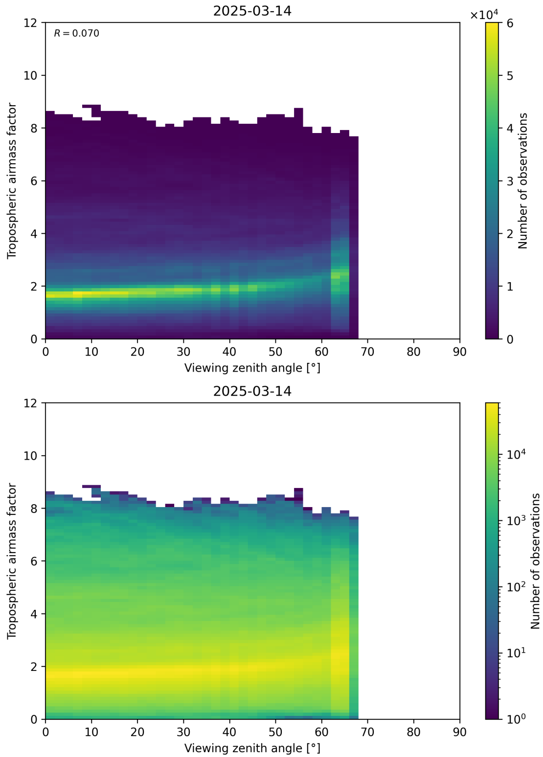
Figure 161: Scatter density plot of “Viewing zenith angle” against “Tropospheric airmass factor” for 2025-03-14 to 2025-03-15.
