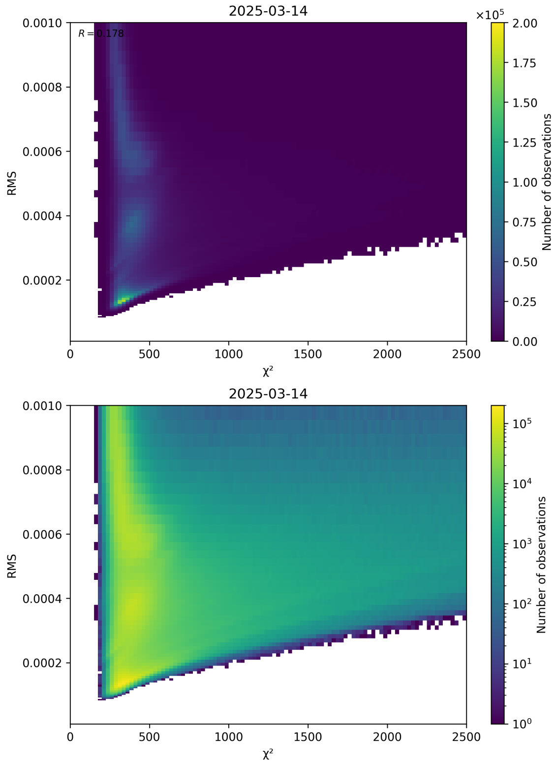
Figure 82: Scatter density plot of “ \chi^2 ” against “RMS” for 2025-03-14 to 2025-03-15.
