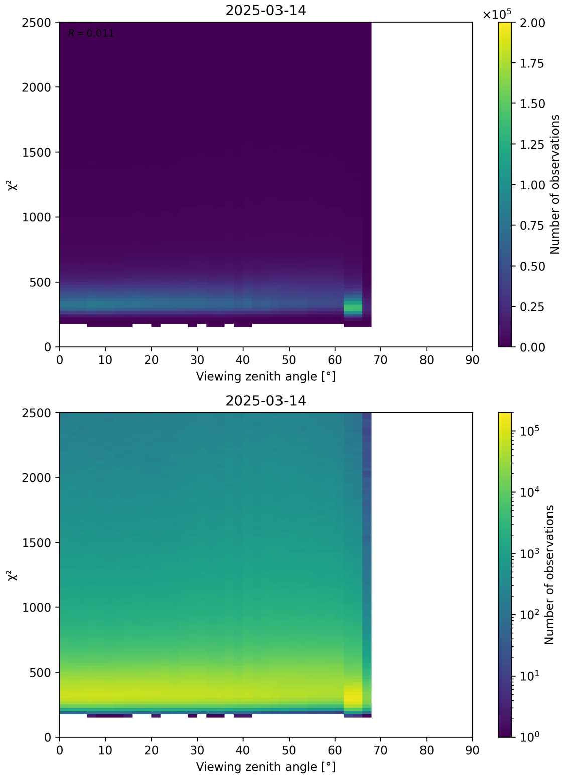
Figure 162: Scatter density plot of “Viewing zenith angle” against “ \chi^2 ” for 2025-03-14 to 2025-03-15.
