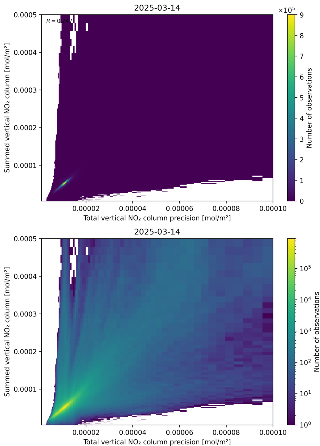
Figure 117: Scatter density plot of “Total vertical NO 2 column precision” against “Summed vertical NO 2 column” for 2025-03-14 to 2025-03-15.
