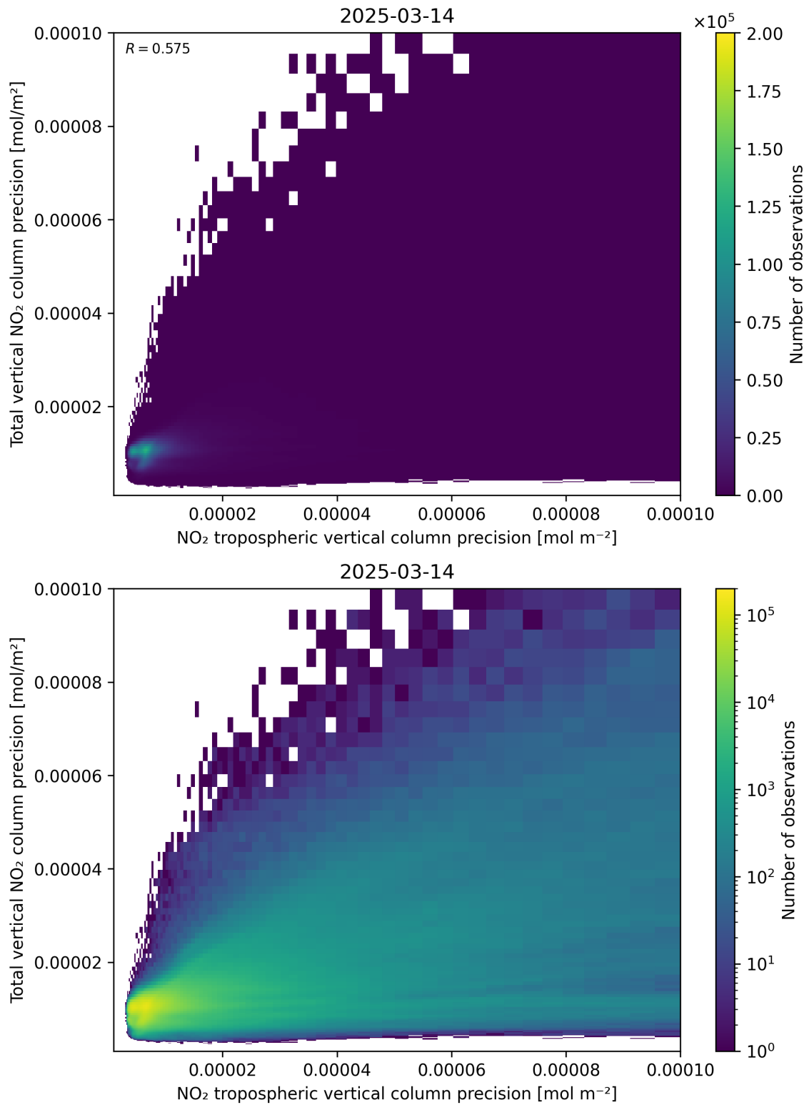
Figure 139: Scatter density plot of “NO 2 tropospheric vertical column precision” against “Total vertical NO 2 column precision” for 2025-03-14 to 2025-03-15.
