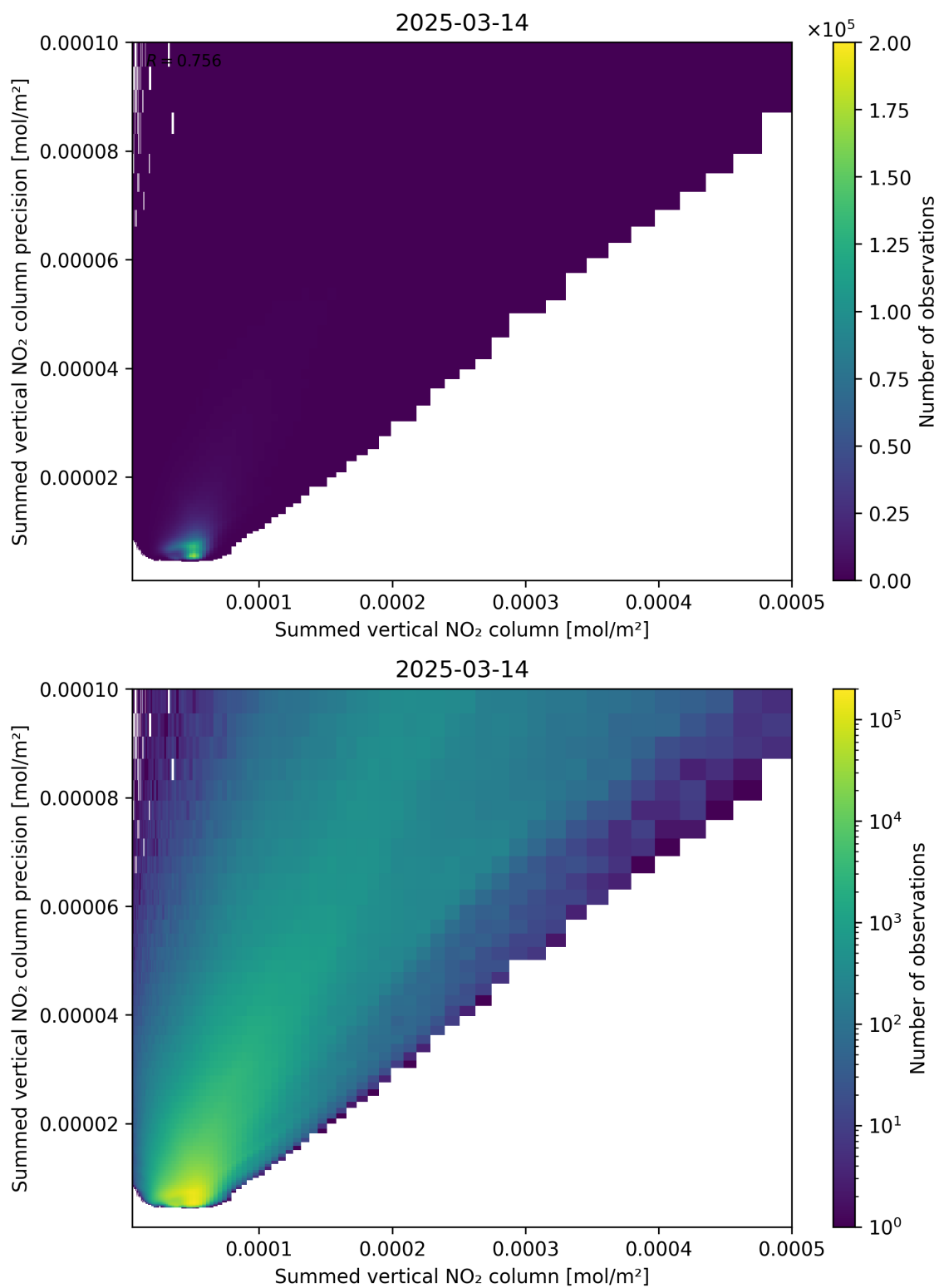
Figure 105: Scatter density plot of “Summed vertical NO 2 column” against “Summed vertical NO 2 column precision” for 2025-03-14 to 2025-03-15.
