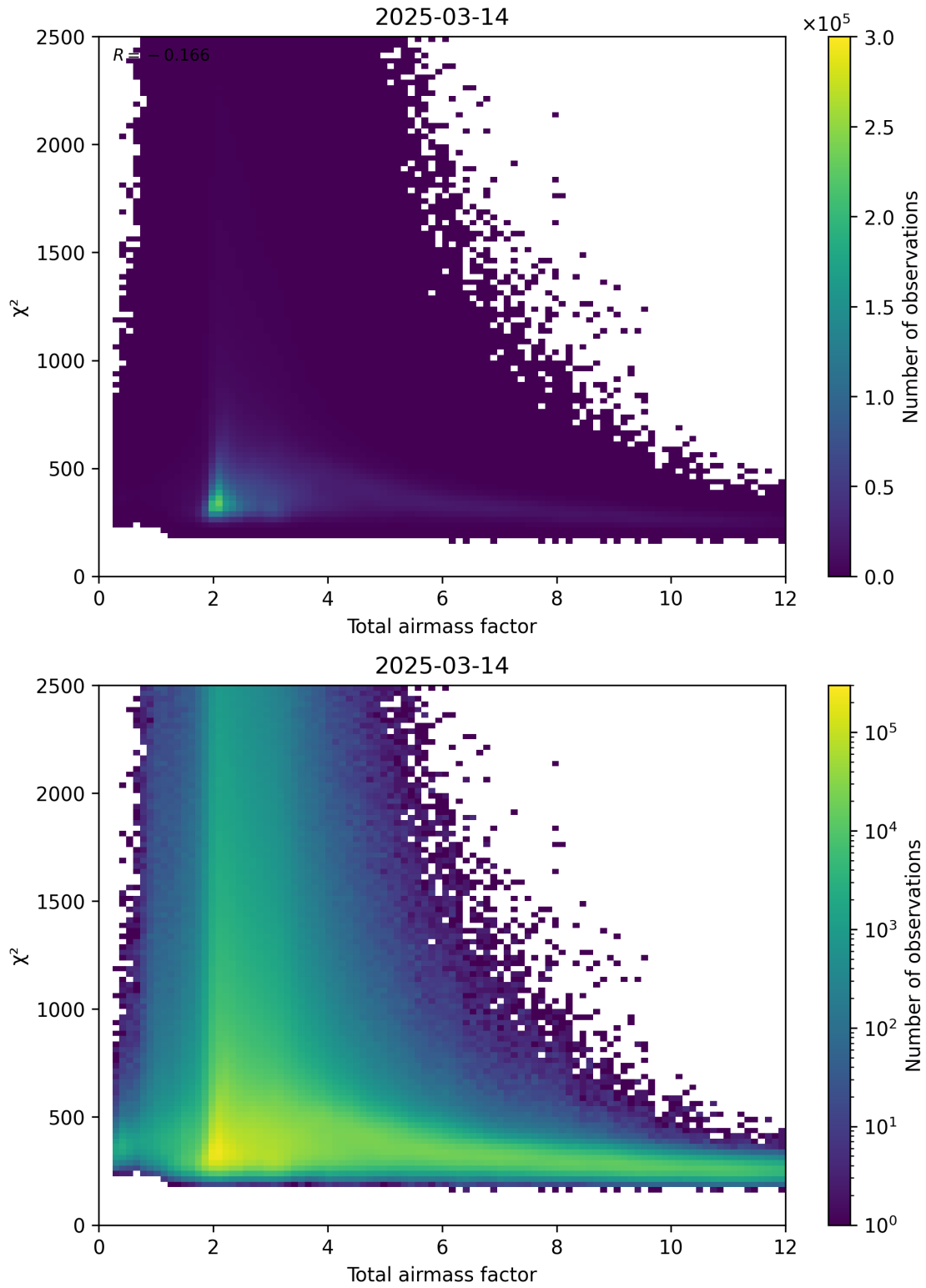
Figure 63: Scatter density plot of “Total airmass factor” against “ \chi^2 ” for 2025-03-14 to 2025-03-15.
