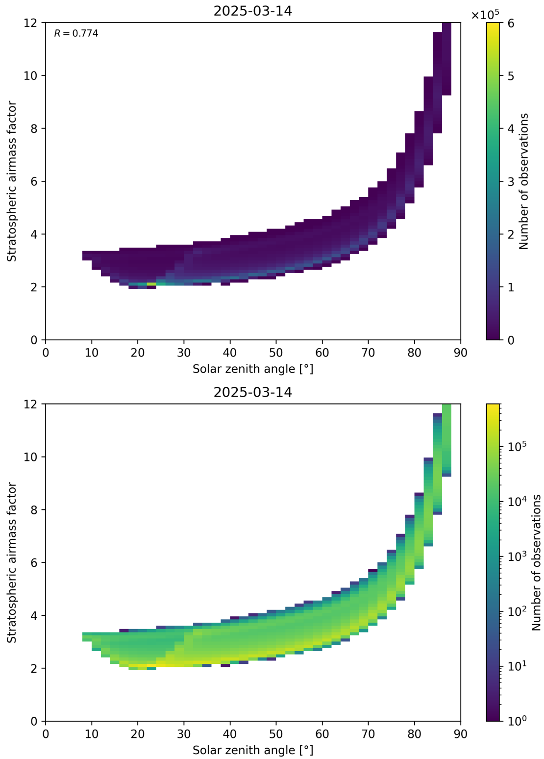
Figure 145: Scatter density plot of “Solar zenith angle” against “Stratospheric airmass factor” for 2025-03-14 to 2025-03-15.
