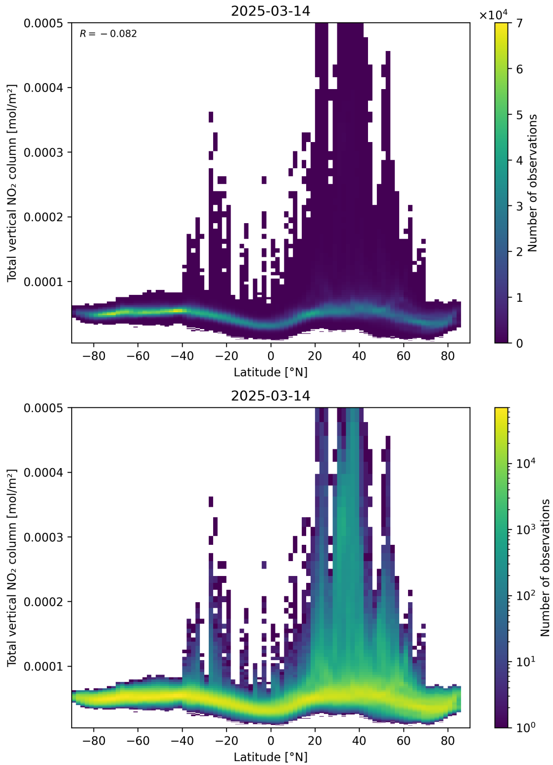
Figure 90: Scatter density plot of “Latitude” against “Total vertical NO 2 column” for 2025-03-14 to 2025-03-15.
