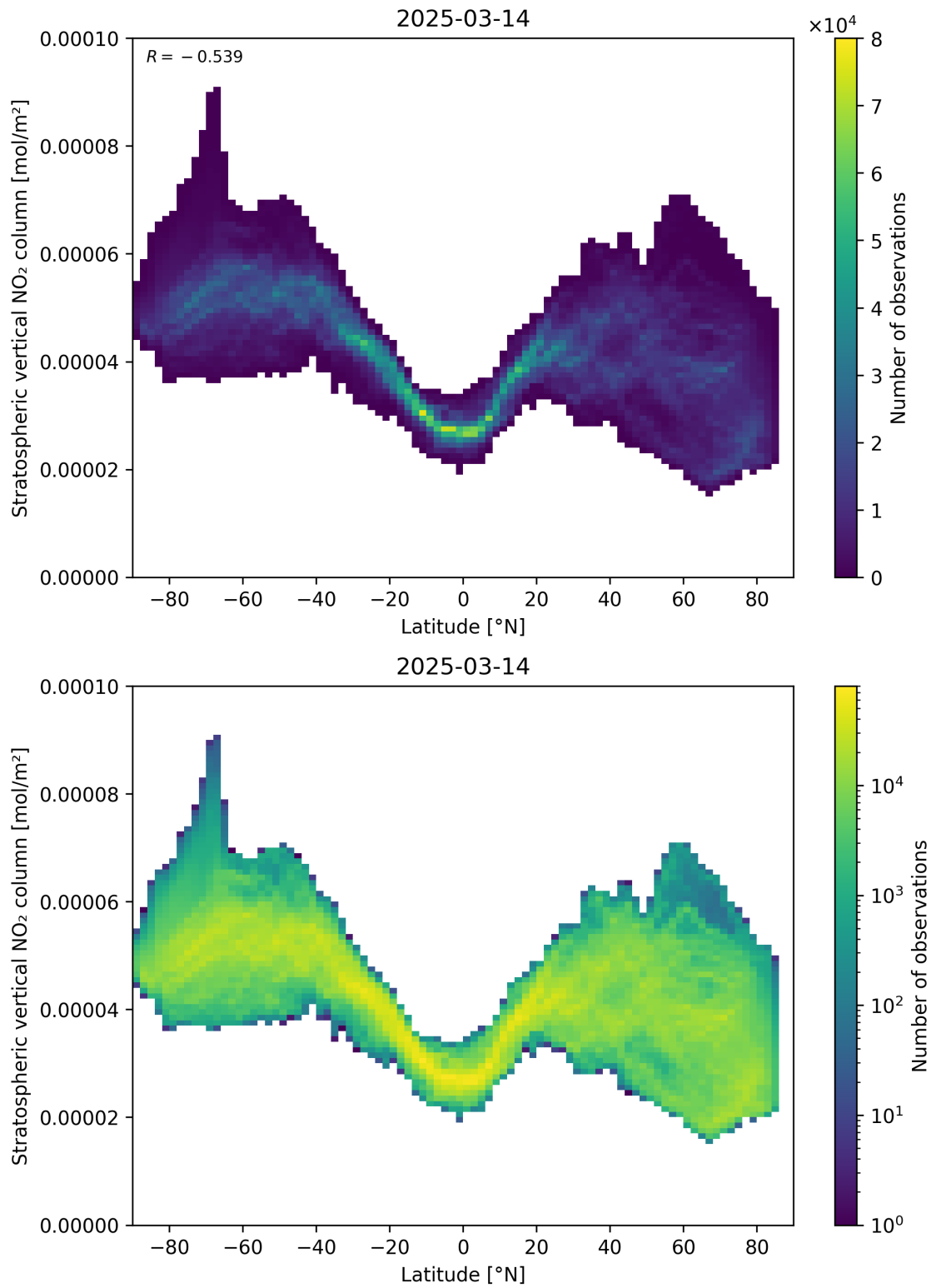
Figure 87: Scatter density plot of “Latitude” against “Stratospheric vertical NO 2 column” for 2025-03-14 to 2025-03-15.
