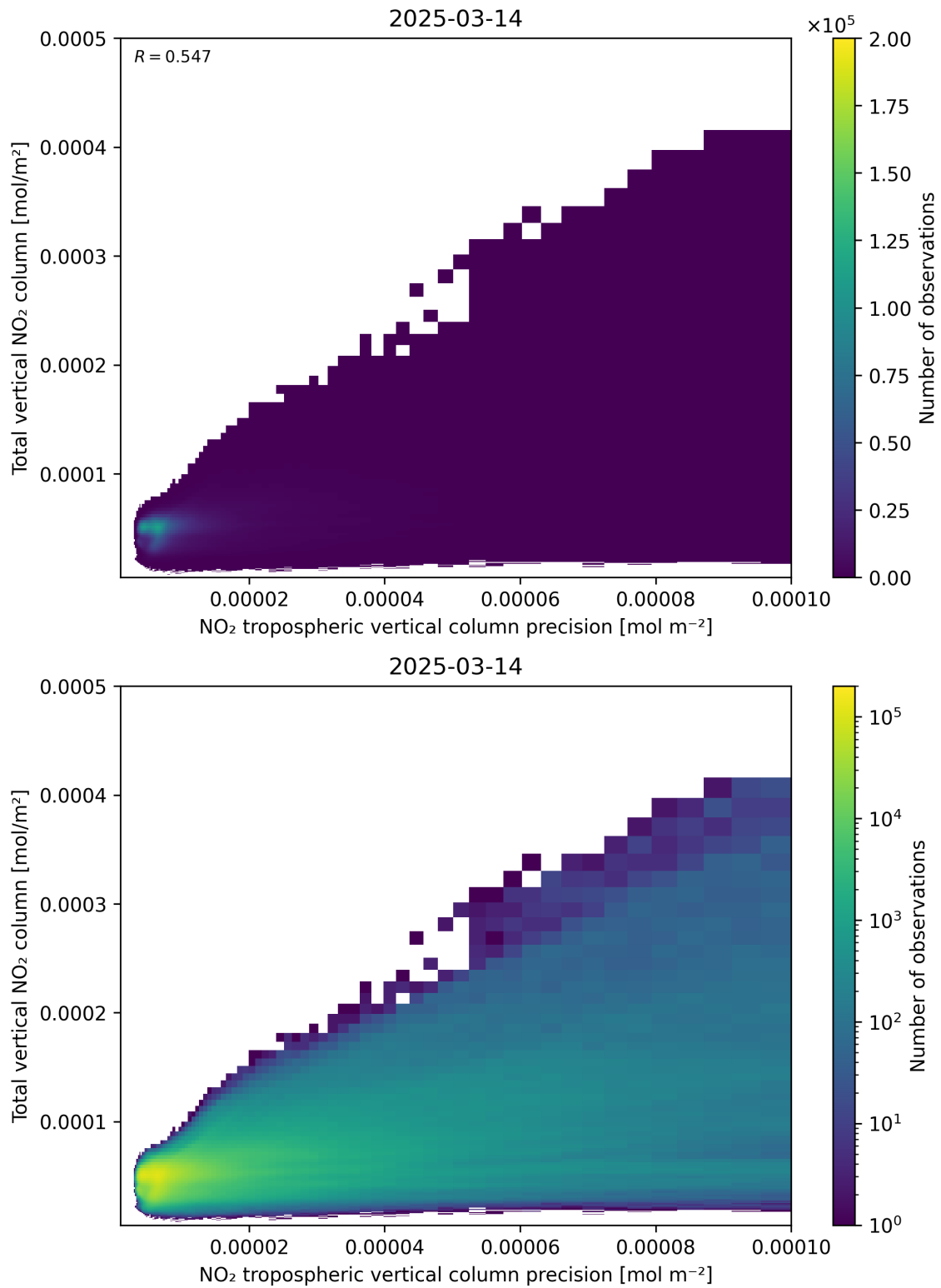
Figure 138: Scatter density plot of “NO 2 tropospheric vertical column precision” against “Total vertical NO 2 column” for 2025-03-14 to 2025-03-15.
