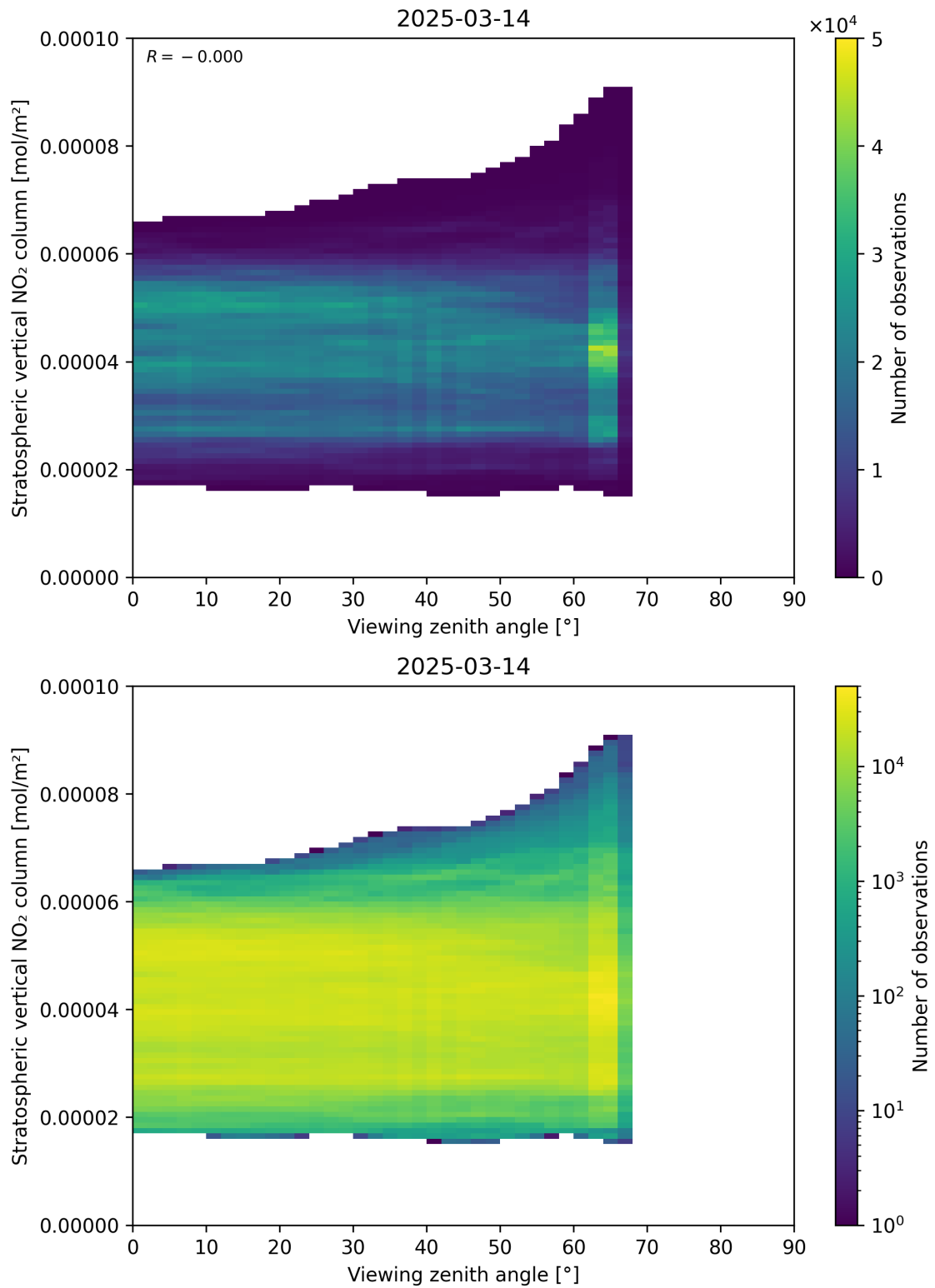
Figure 164: Scatter density plot of “Viewing zenith angle” against “Stratospheric vertical NO 2 column” for 2025-03-14 to 2025-03-15.
