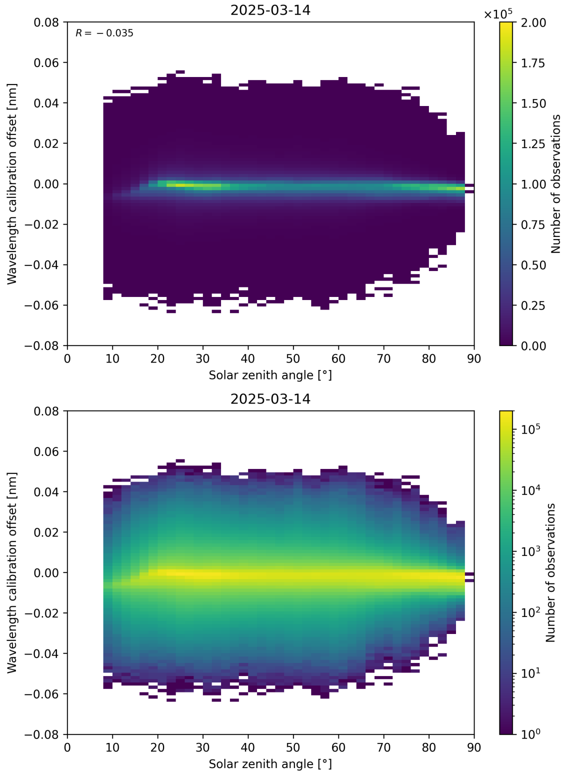
Figure 158: Scatter density plot of “Solar zenith angle” against “Wavelength calibration offset” for 2025-03-14 to 2025-03-15.
