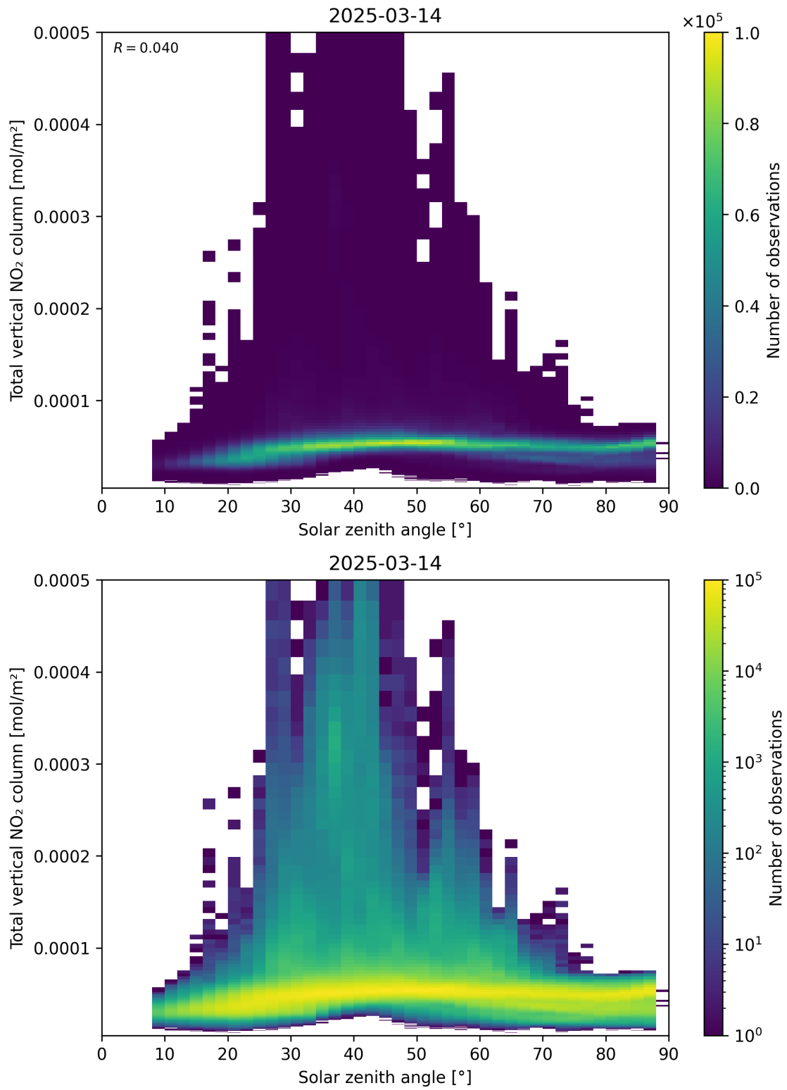
Figure 153: Scatter density plot of “Solar zenith angle” against “Total vertical NO 2 column” for 2025-03-14 to 2025-03-15.
