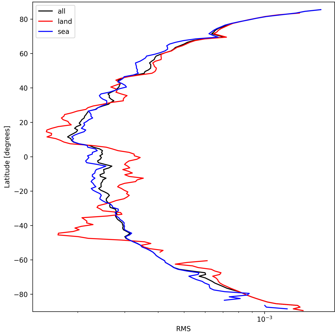
Figure 26: Zonal average of “RMS” for 2025-03-14 to 2025-03-15.
