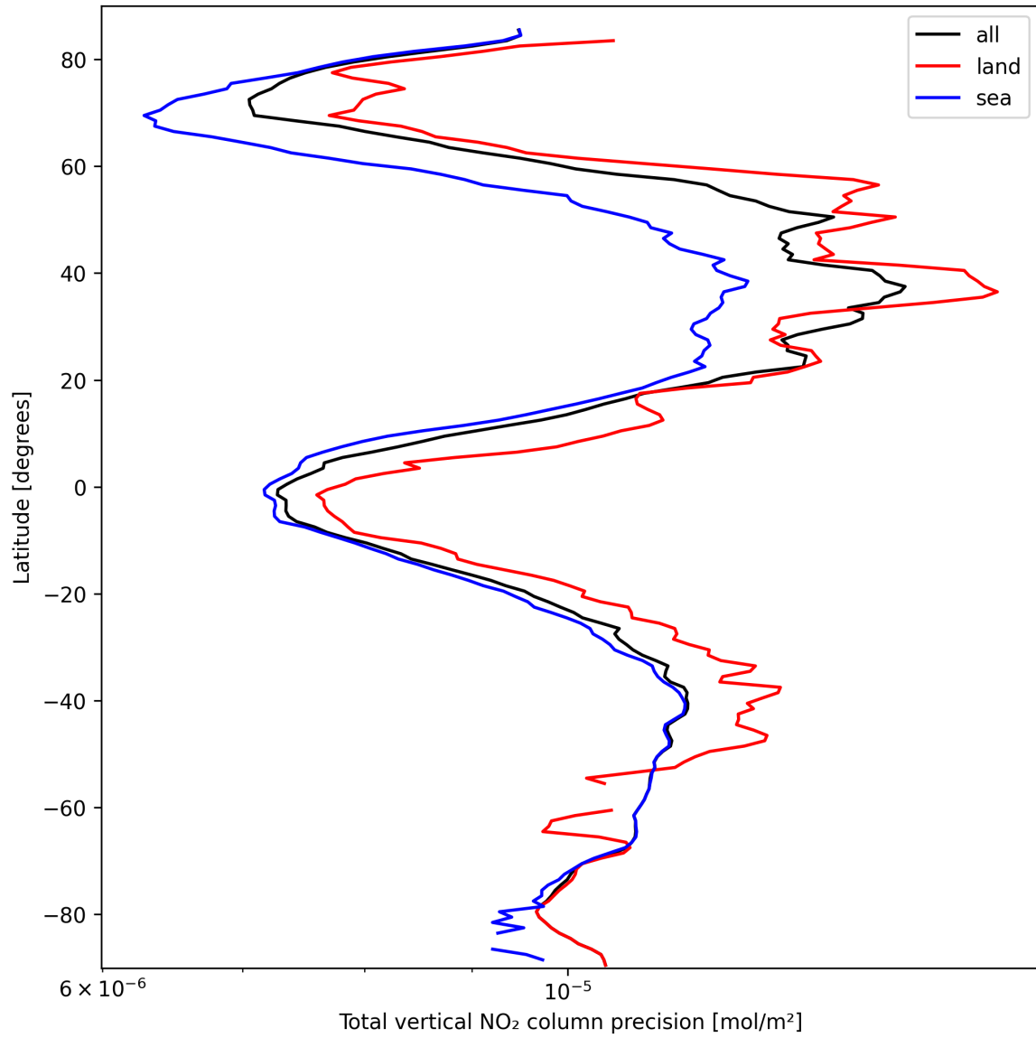
Figure 22: Zonal average of “Total vertical NO 2 column precision” for 2025-03-14 to 2025-03-15.
