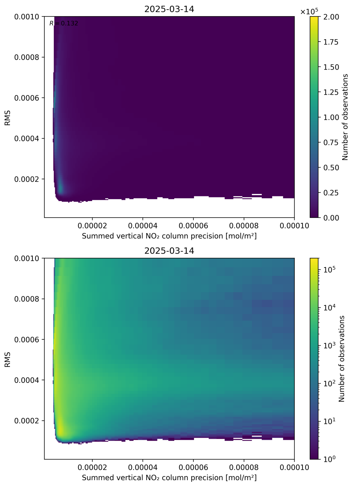
Figure 108: Scatter density plot of “Summed vertical NO 2 column precision” against “RMS” for 2025-03-14 to 2025-03-15.
