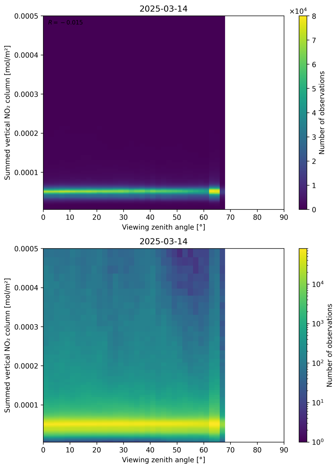
Figure 165: Scatter density plot of “Viewing zenith angle” against “Summed vertical NO 2 column” for 2025-03-14 to 2025-03-15.
