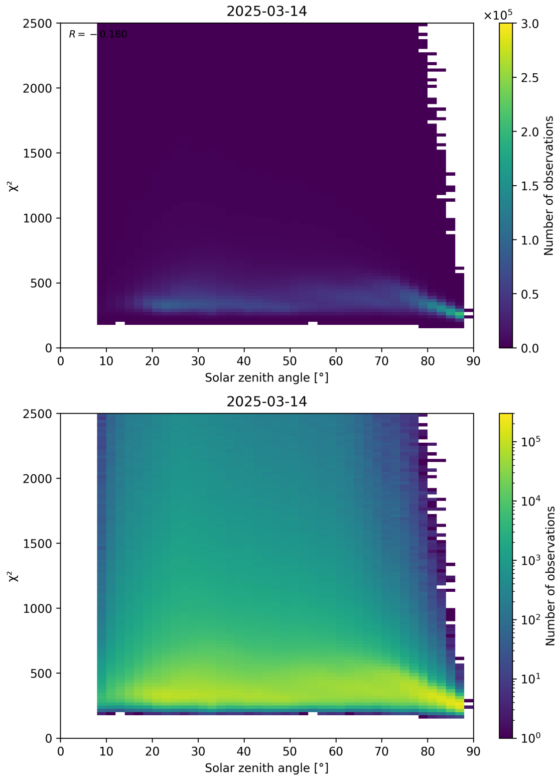
Figure 148: Scatter density plot of “Solar zenith angle” against “ \chi^2 ” for 2025-03-14 to 2025-03-15.
