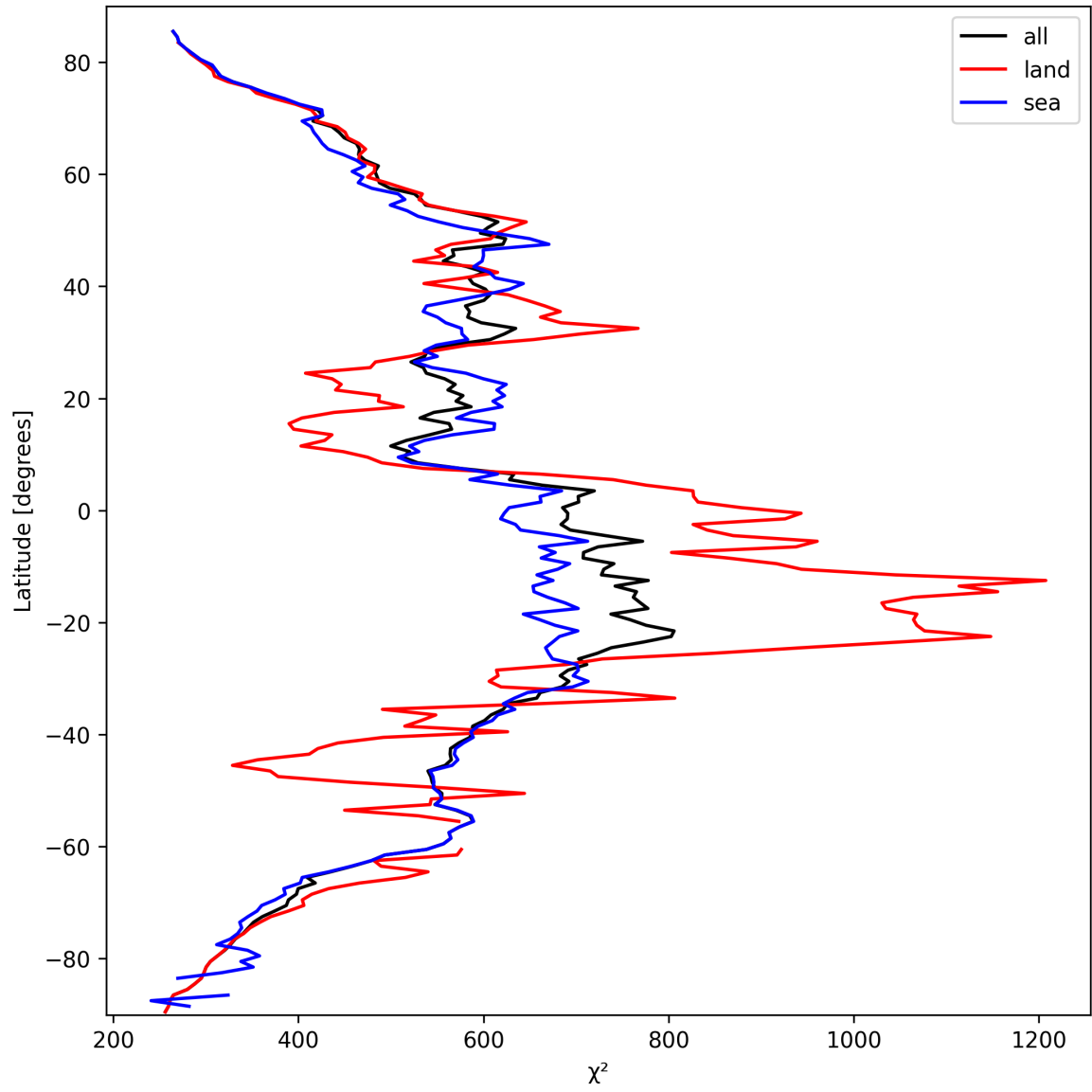
Figure 25: Zonal average of “ \chi^2 ” for 2025-03-14 to 2025-03-15.
