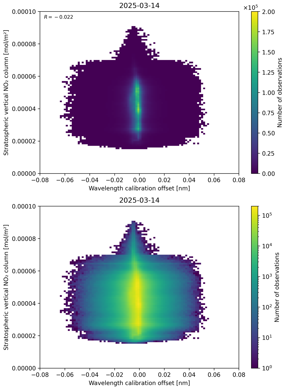
Figure 176: Scatter density plot of “Wavelength calibration offset” against “Stratospheric vertical NO 2 column” for 2025-03-14 to 2025-03-15.
