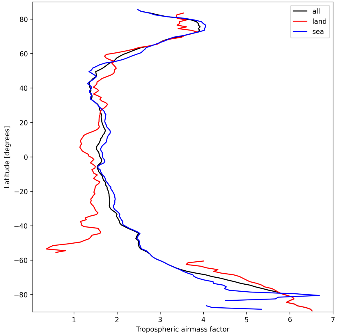
Figure 14: Zonal average of “Tropospheric airmass factor” for 2025-03-14 to 2025-03-15.
