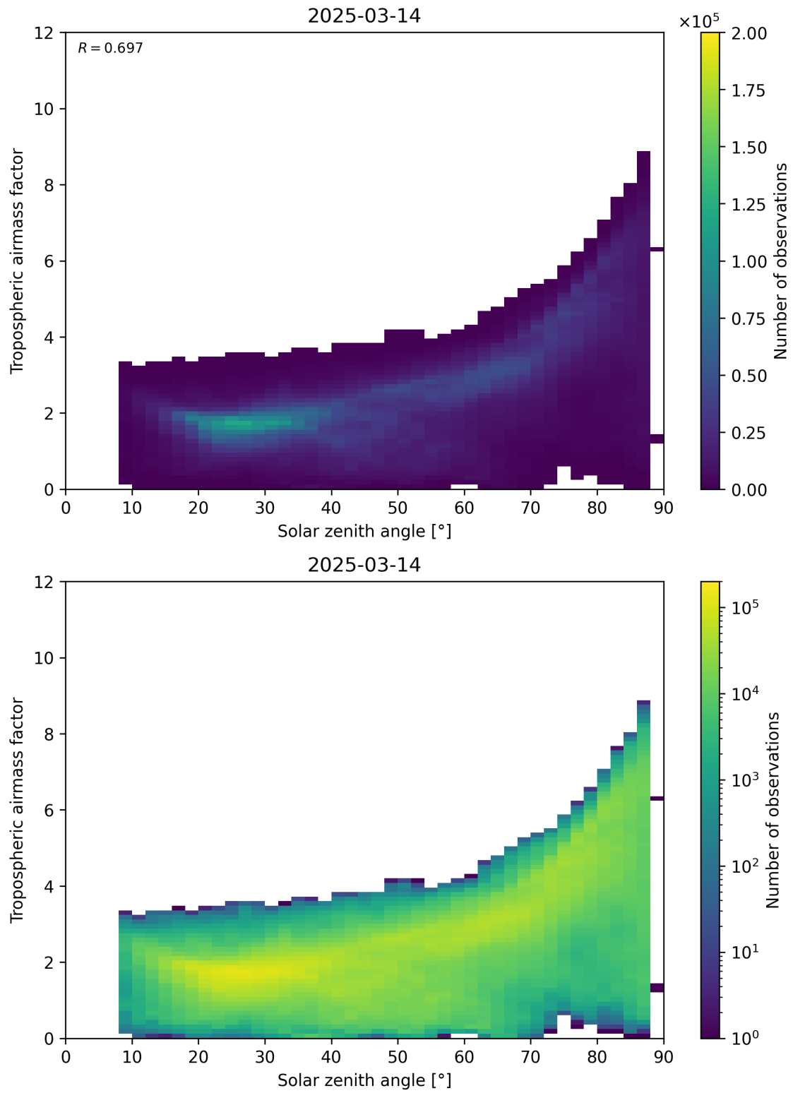
Figure 147: Scatter density plot of “Solar zenith angle” against “Tropospheric airmass factor” for 2025-03-14 to 2025-03-15.
