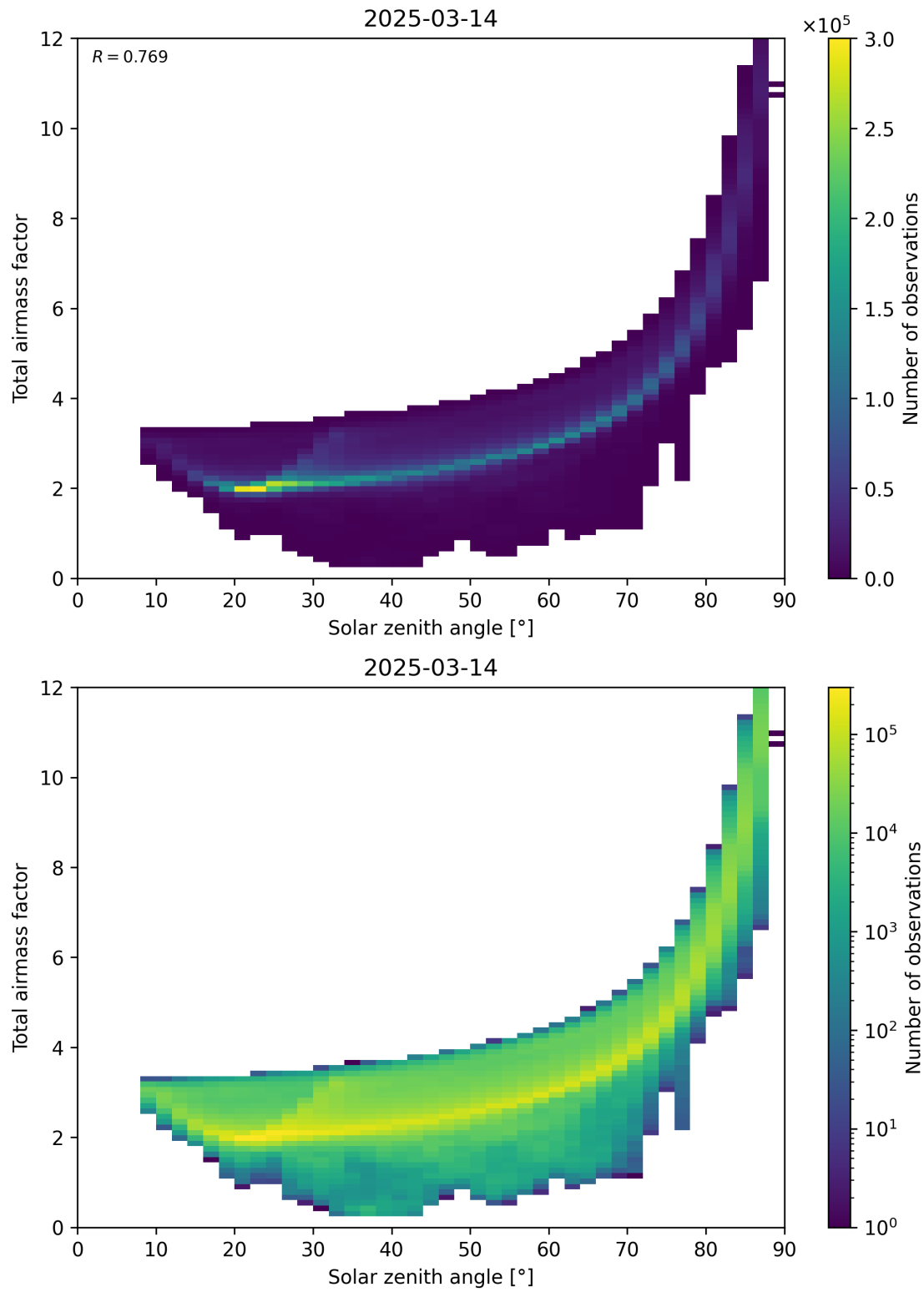
Figure 146: Scatter density plot of “Solar zenith angle” against “Total airmass factor” for 2025-03-14 to 2025-03-15.
