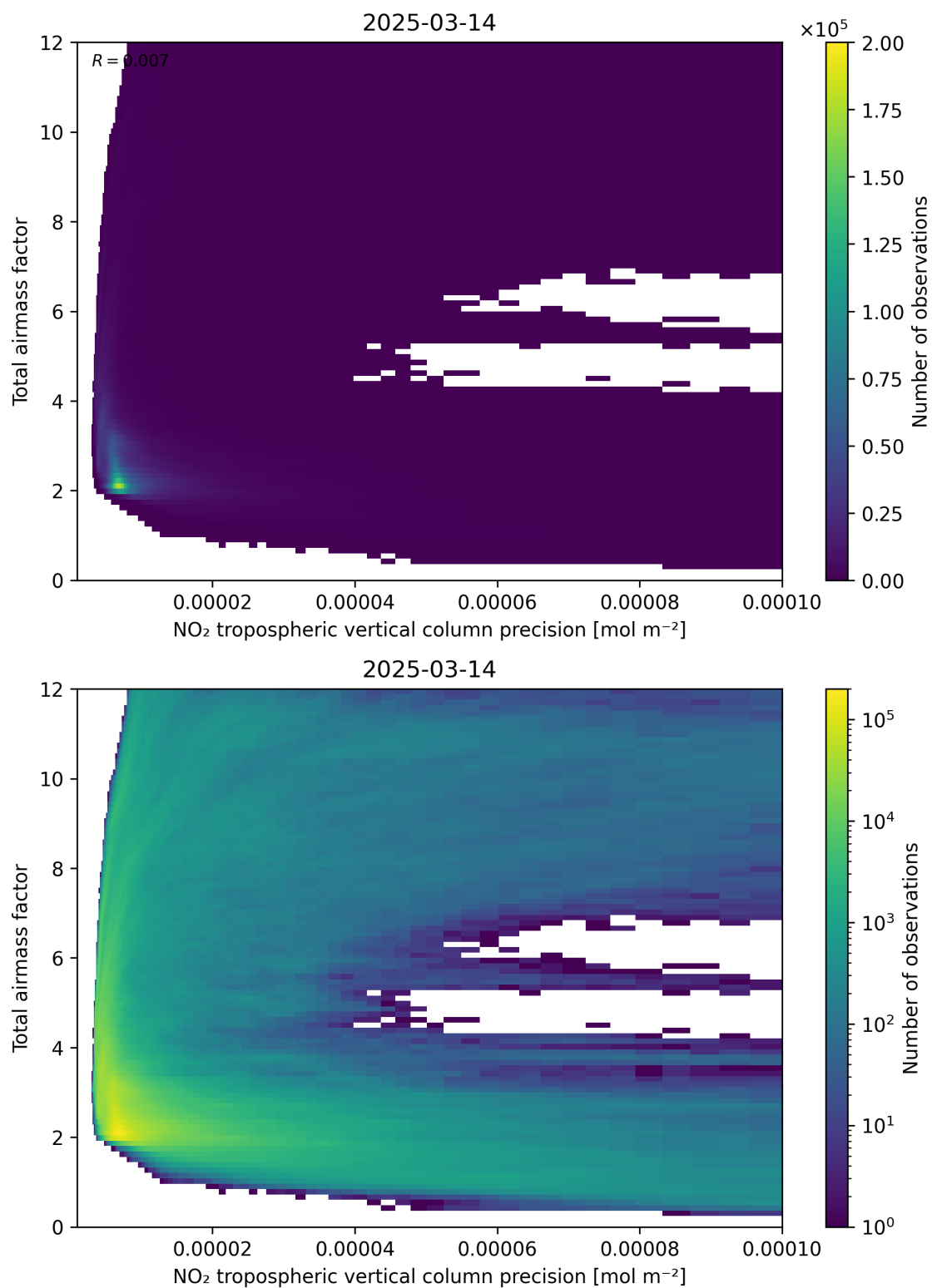
Figure 132: Scatter density plot of “NO 2 tropospheric vertical column precision” against “Total air mass factor” for 2025-03-14 to 2025-03-15.
