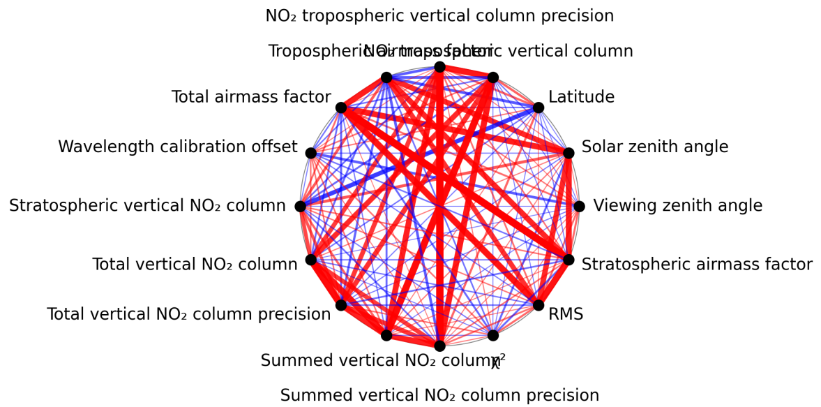
Figure 1: Map of correlation graph for 2025-03-14 to 2025-03-15.
