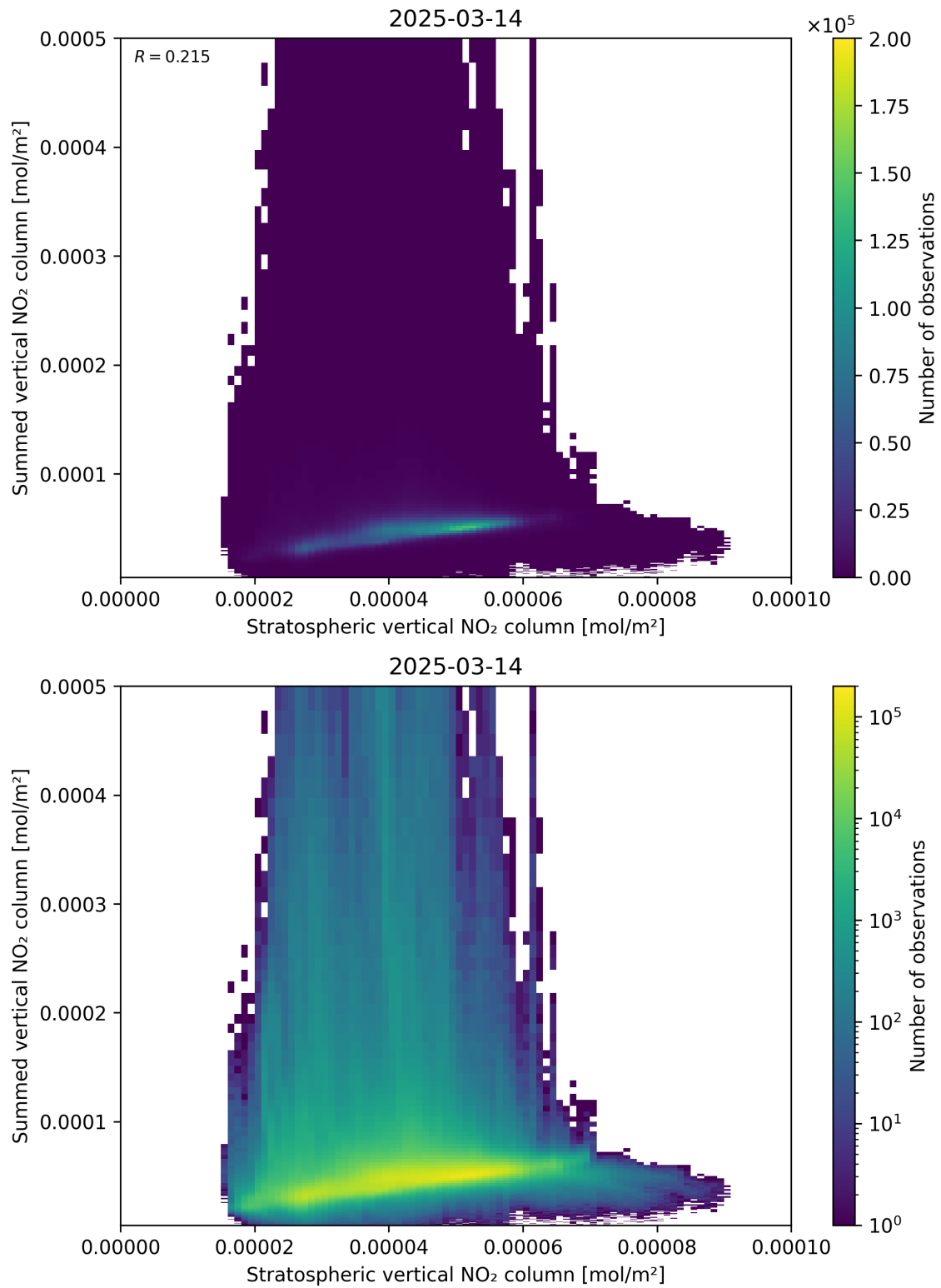
Figure 98: Scatter density plot of “Stratospheric vertical NO 2 column” against “Summed vertical NO 2 column” for 2025-03-14 to 2025-03-15.
