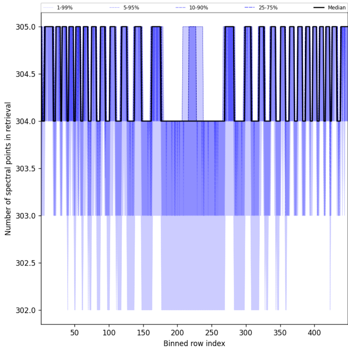
Figure 50: Along track statistics of “Number of spectral points in retrieval” for 2025-03-14 to 2025-03-15
