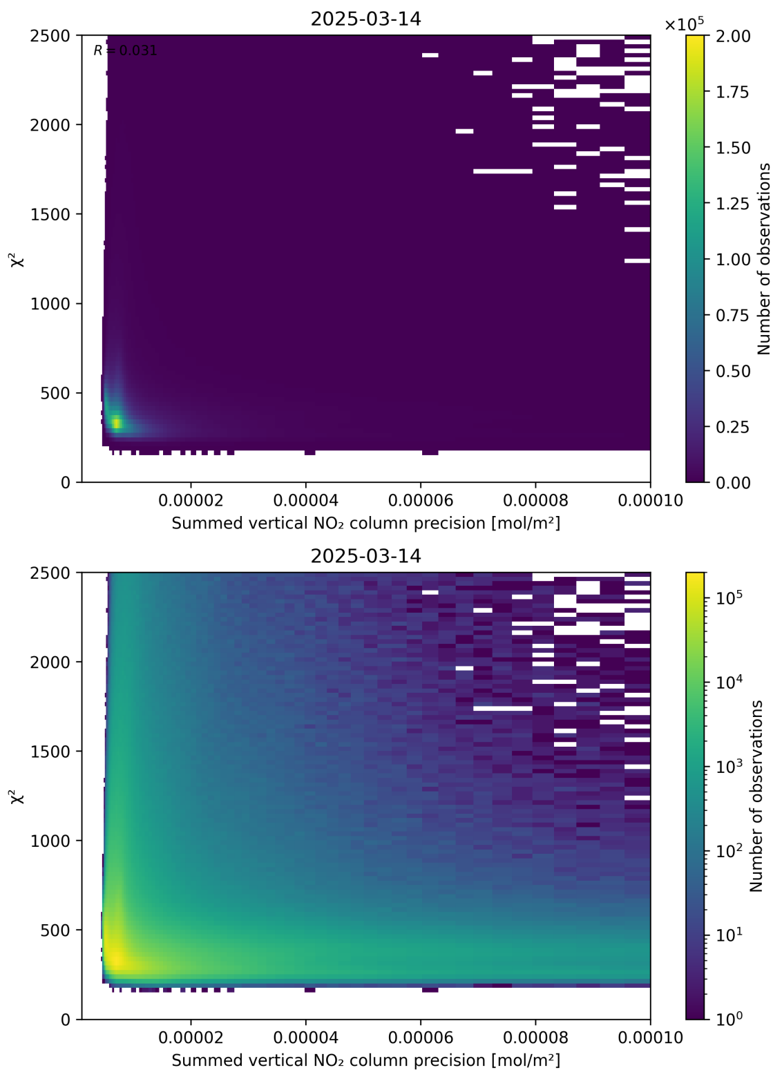
Figure 107: Scatter density plot of “Summed vertical NO 2 column precision” against “ \chi^2 ” for 2025-03-14 to 2025-03-15.
