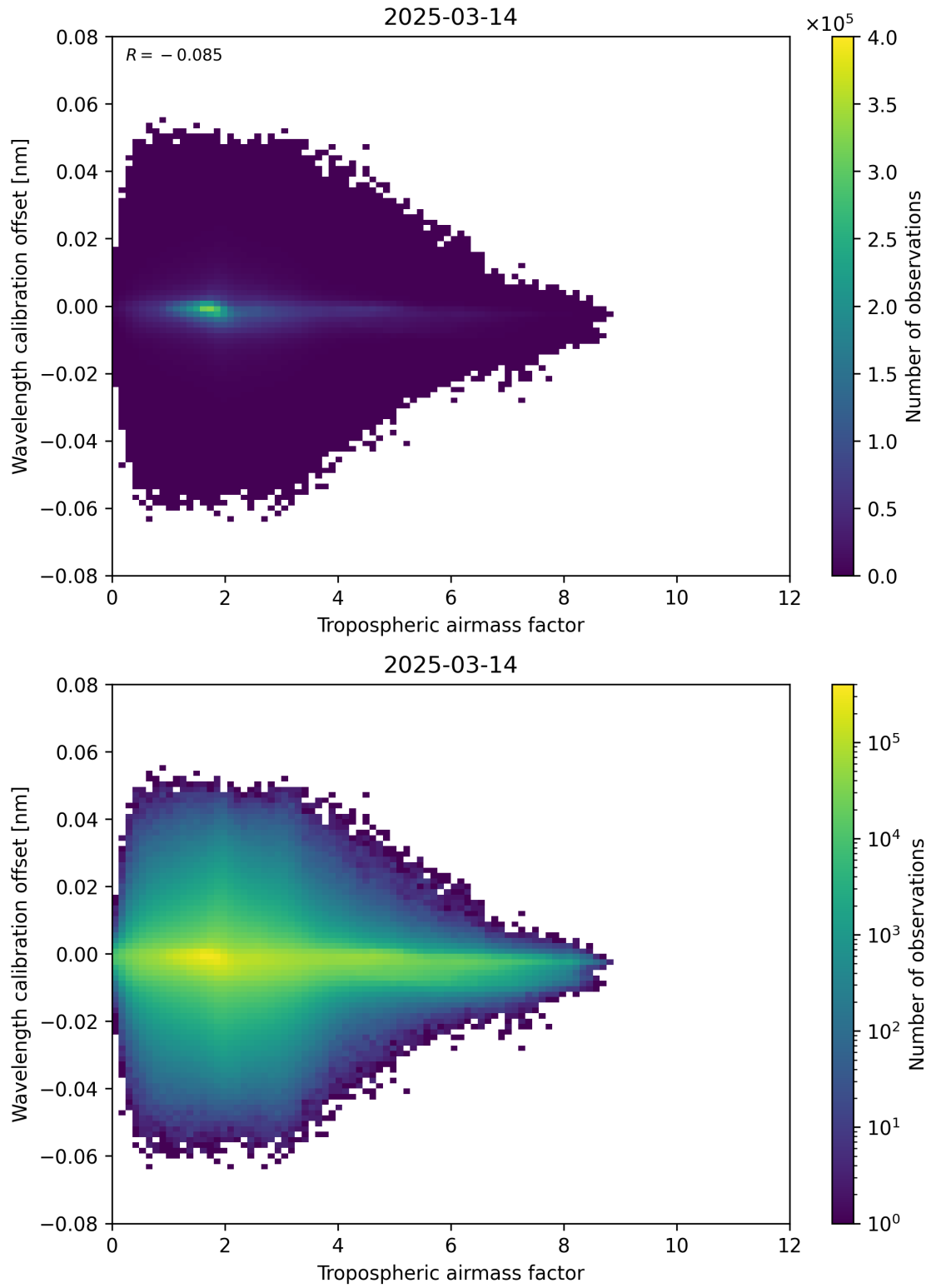
Figure 80: Scatter density plot of “Tropospheric airmass factor” against “Wavelength calibration offset” for 2025-03-14 to 2025-03-15.
