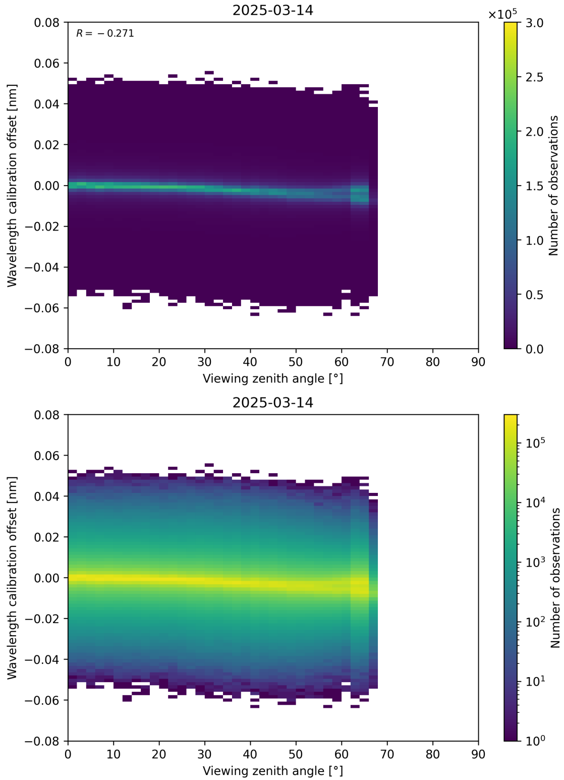
Figure 173: Scatter density plot of “Viewing zenith angle” against “Wavelength calibration offset” for 2025-03-14 to 2025-03-15.
