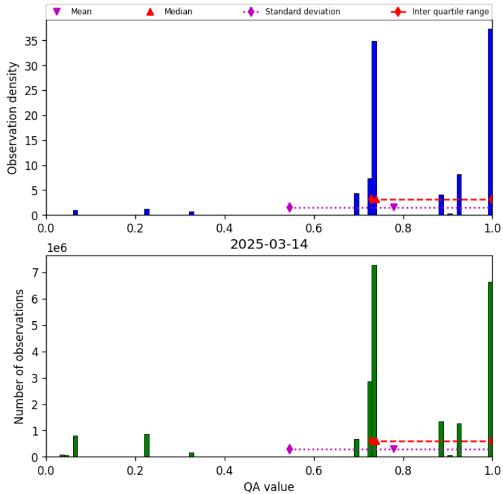
Figure 28: Histogram of “QA value” for 2025-03-14 to 2025-03-15
