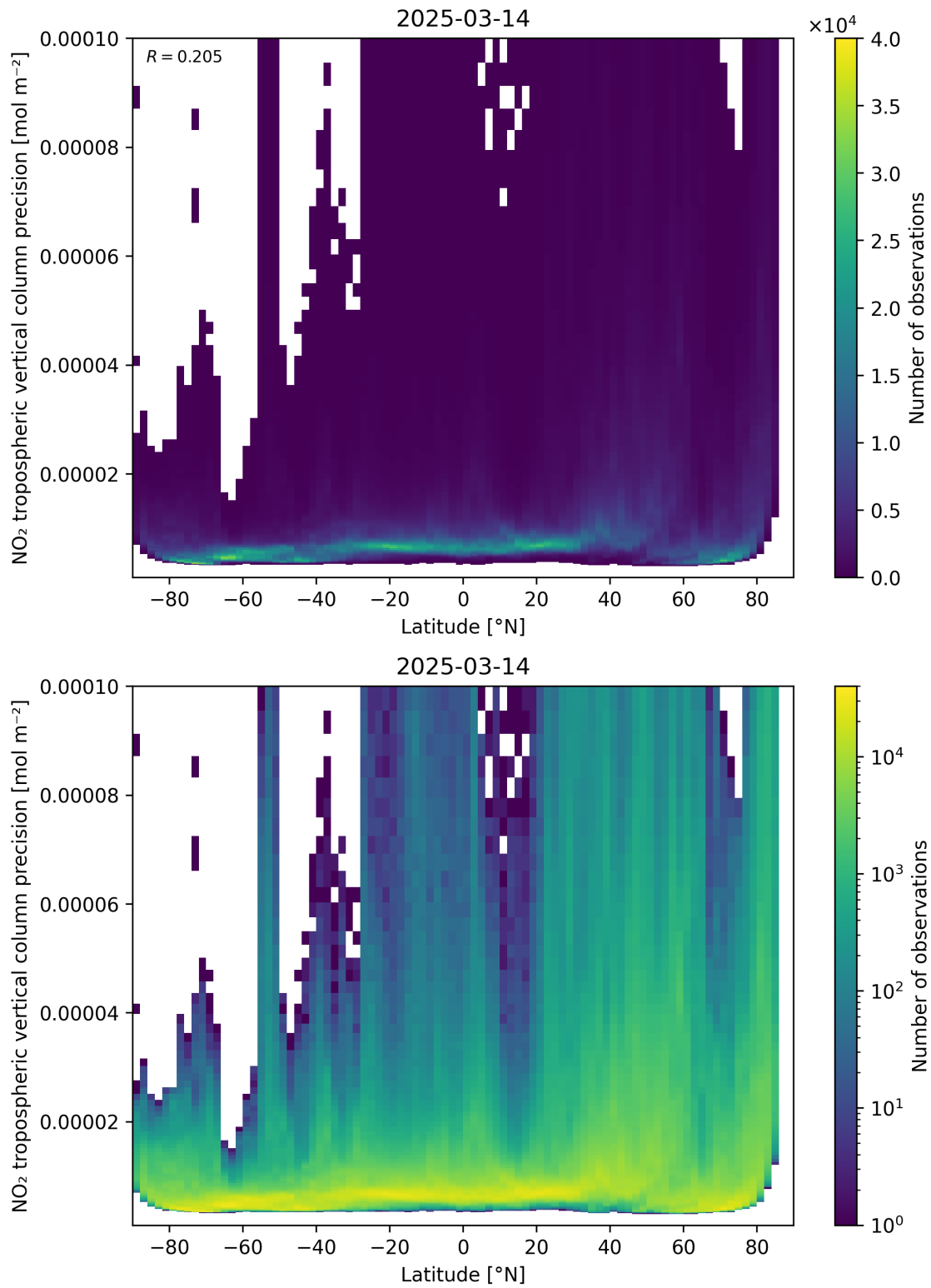
Figure 93: Scatter density plot of “Latitude” against “NO 2 tropospheric vertical column precision” for 2025-03-14 to 2025-03-15.
