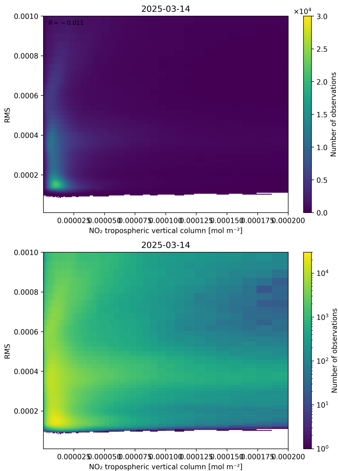
Figure 142: Scatter density plot of “NO 2 tropospheric vertical column” against “RMS” for 2025-03-14 to 2025-03-15.
