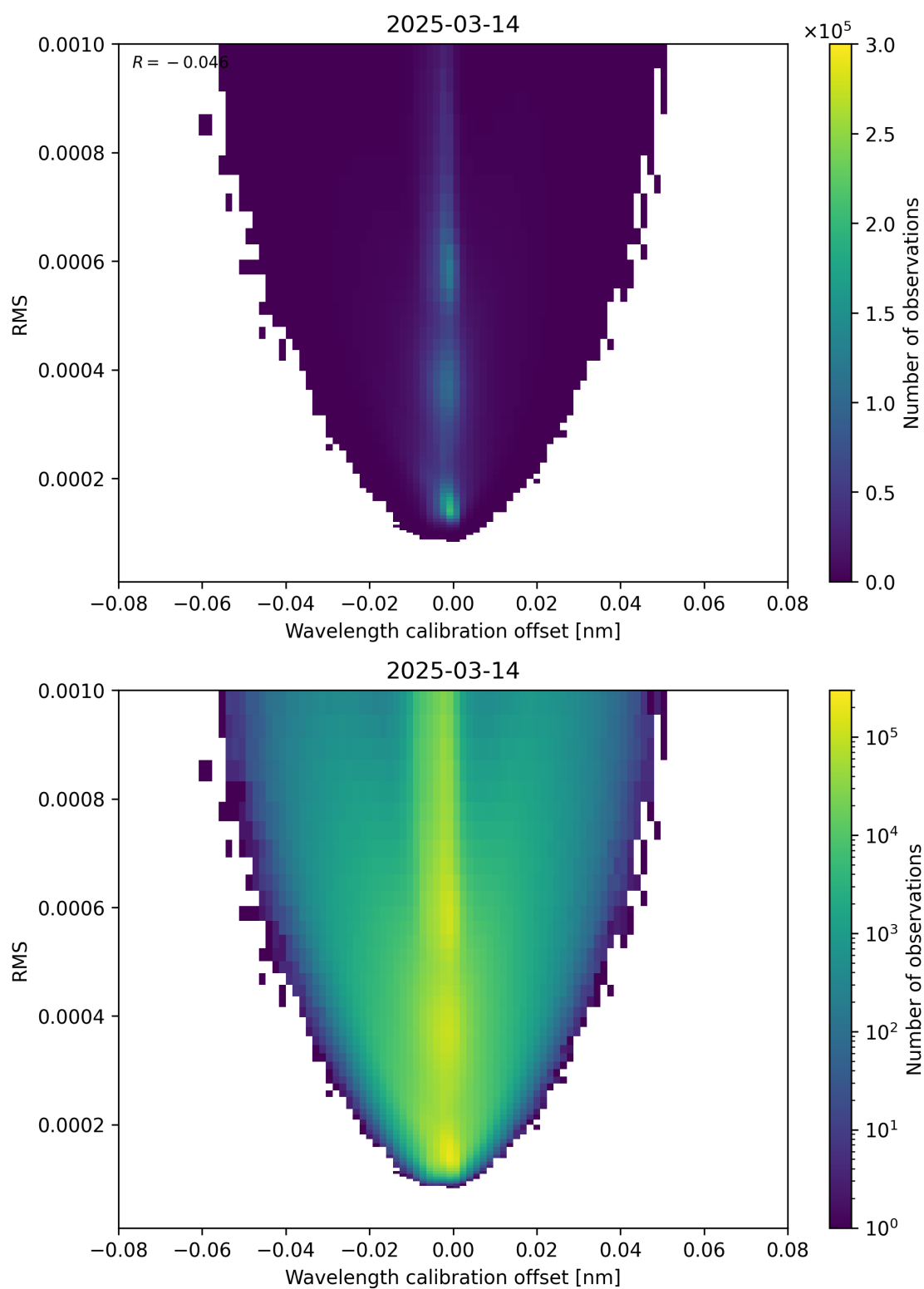
Figure 181: Scatter density plot of “Wavelength calibration offset” against “RMS” for 2025-03-14 to 2025-03-15.
