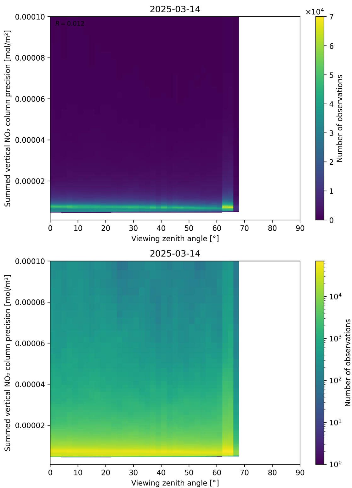
Figure 166: Scatter density plot of “Viewing zenith angle” against “Summed vertical NO 2 column precision” for 2025-03-14 to 2025-03-15.
