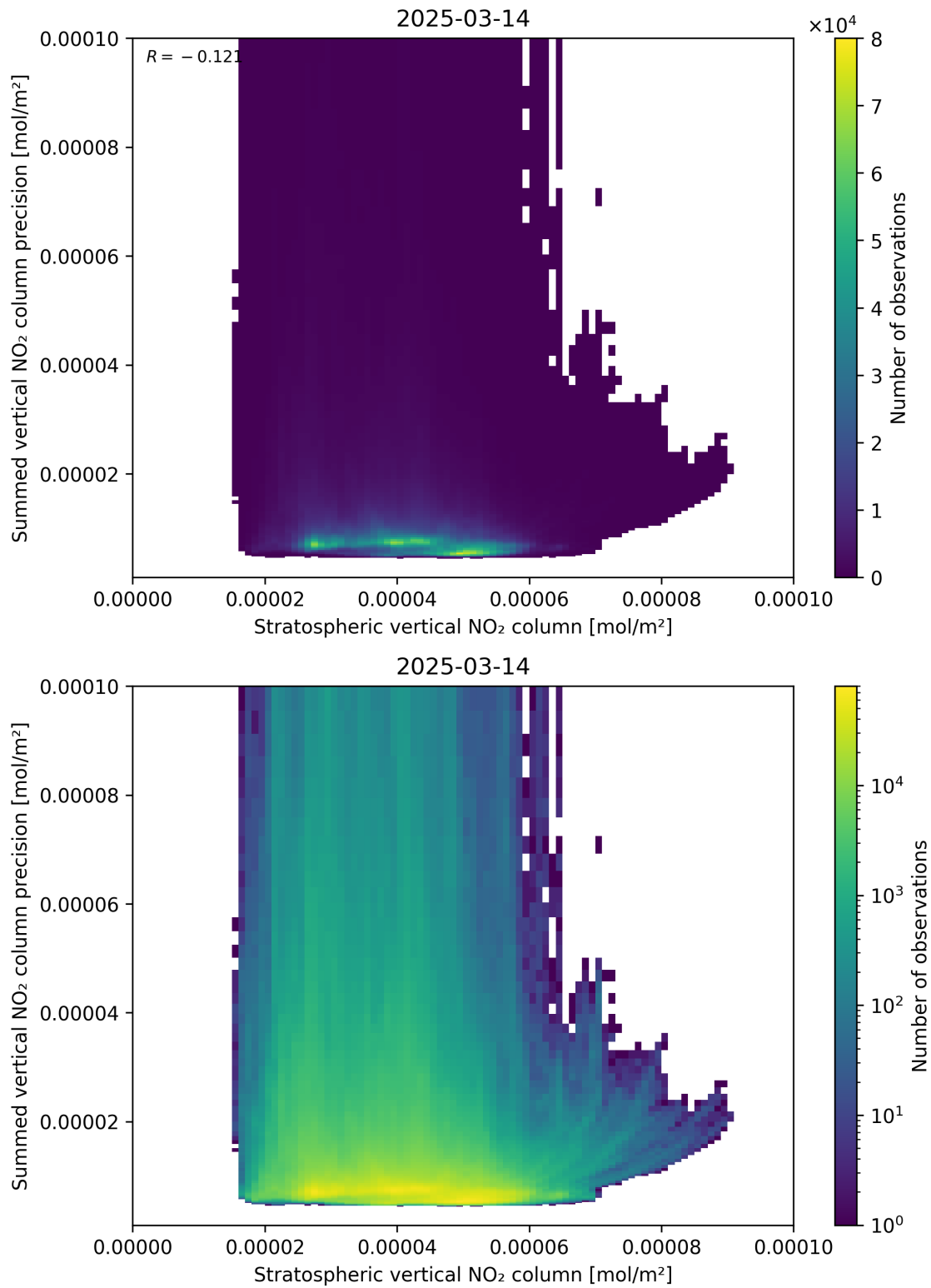
Figure 99: Scatter density plot of “Stratospheric vertical NO 2 column” against “Summed vertical NO 2 column precision” for 2025-03-14 to 2025-03-15.
