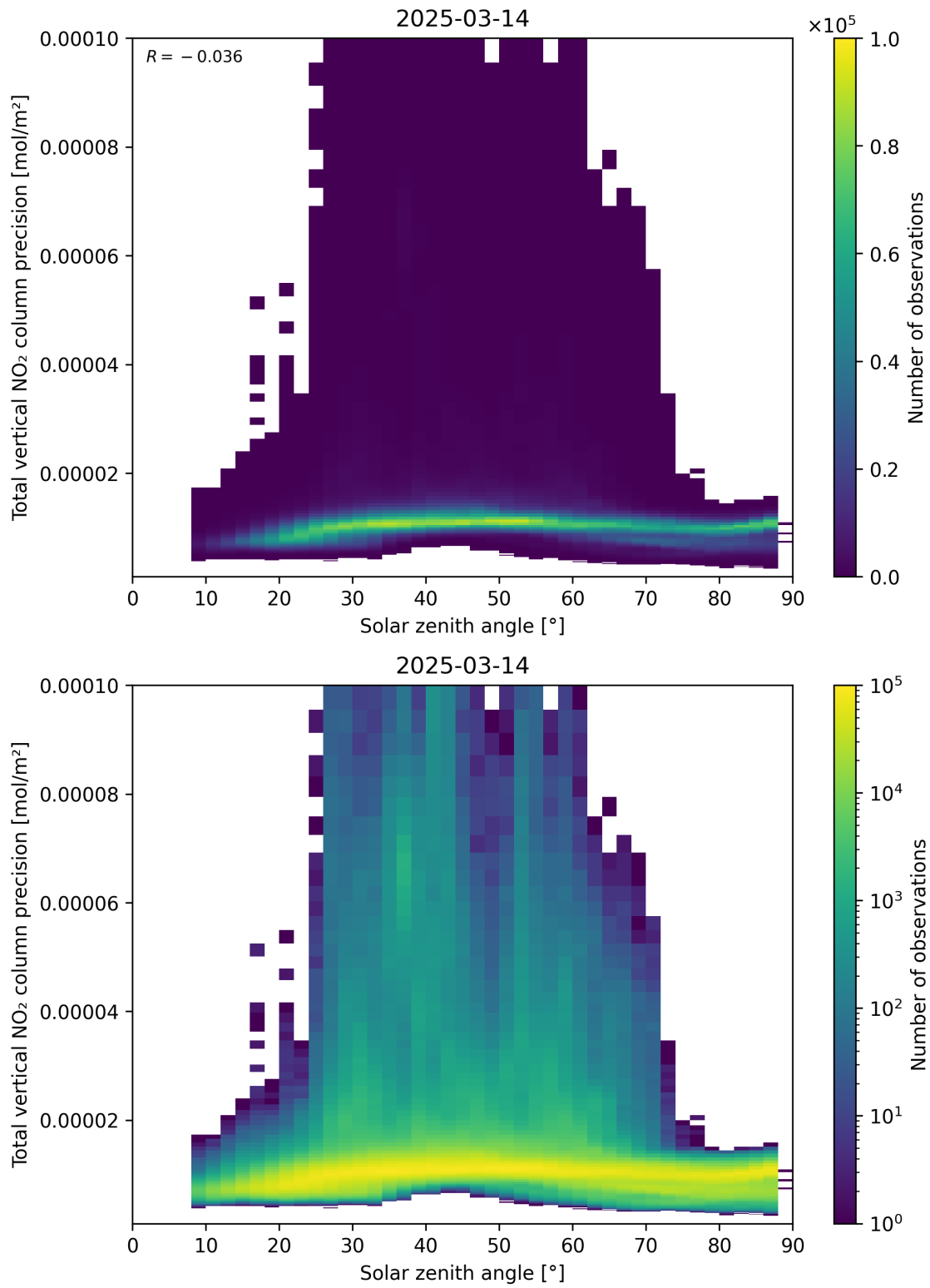
Figure 154: Scatter density plot of “Solar zenith angle” against “Total vertical NO 2 column precision” for 2025-03-14 to 2025-03-15.
