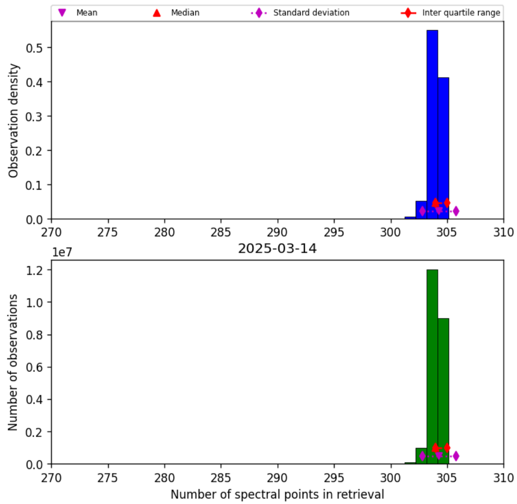
Figure 33: Histogram of “Number of spectral points in retrieval” for 2025-03-14 to 2025-03-15
