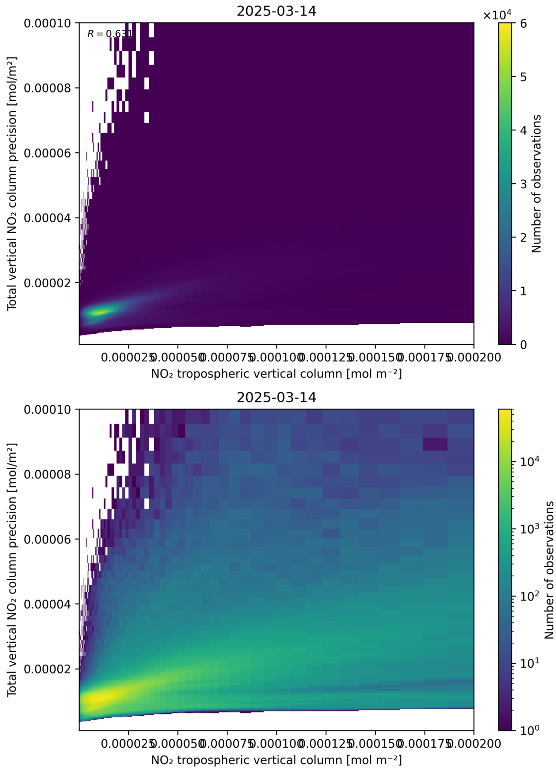
Figure 129: Scatter density plot of “NO 2 tropospheric vertical column” against “Total vertical NO 2 column precision” for 2025-03-14 to 2025-03-15.
