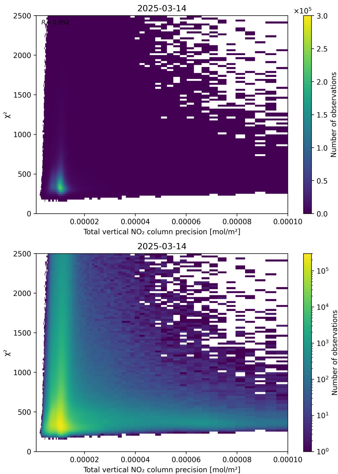
Figure 116: Scatter density plot of “Total vertical NO 2 column precision” against “ \chi^2 ” for 2025-03-14 to 2025-03-15.
