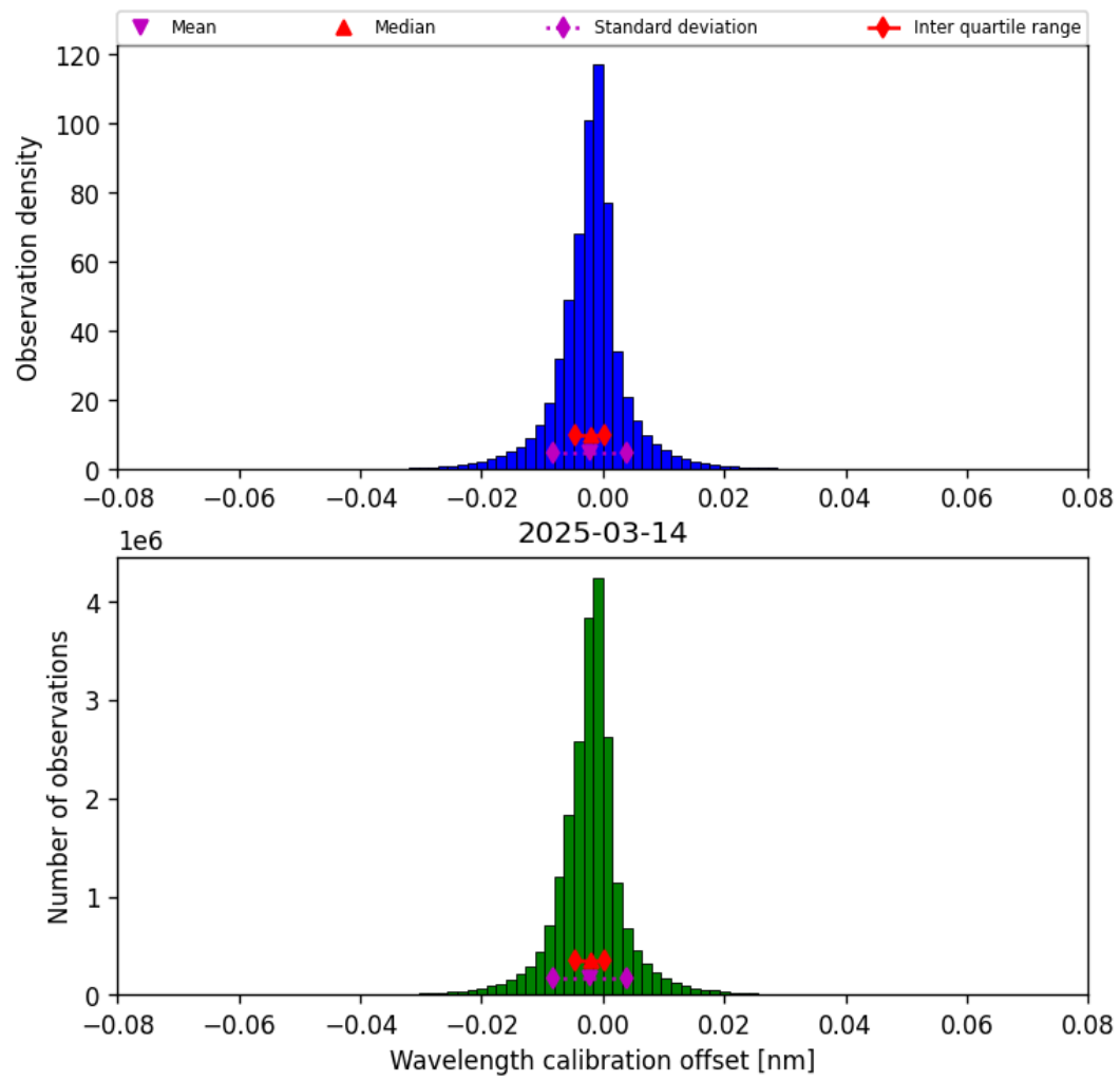
Figure 35: Histogram of “Wavelength calibration offset” for 2025-03-14 to 2025-03-15
