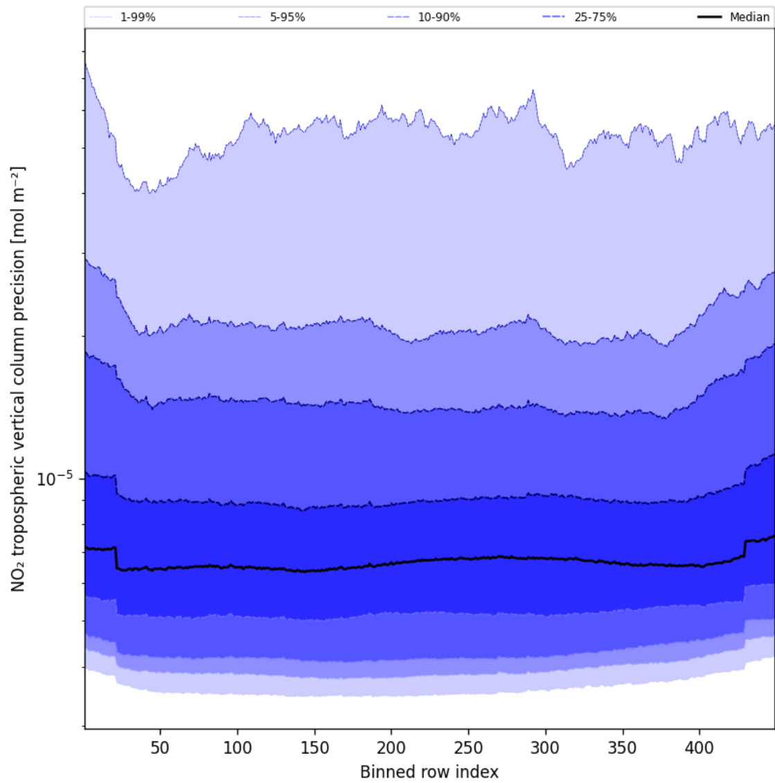
Figure 47: Along track statistics of “NO 2 tropospheric vertical column precision” for 2025-03-14 to 2025-03-15
