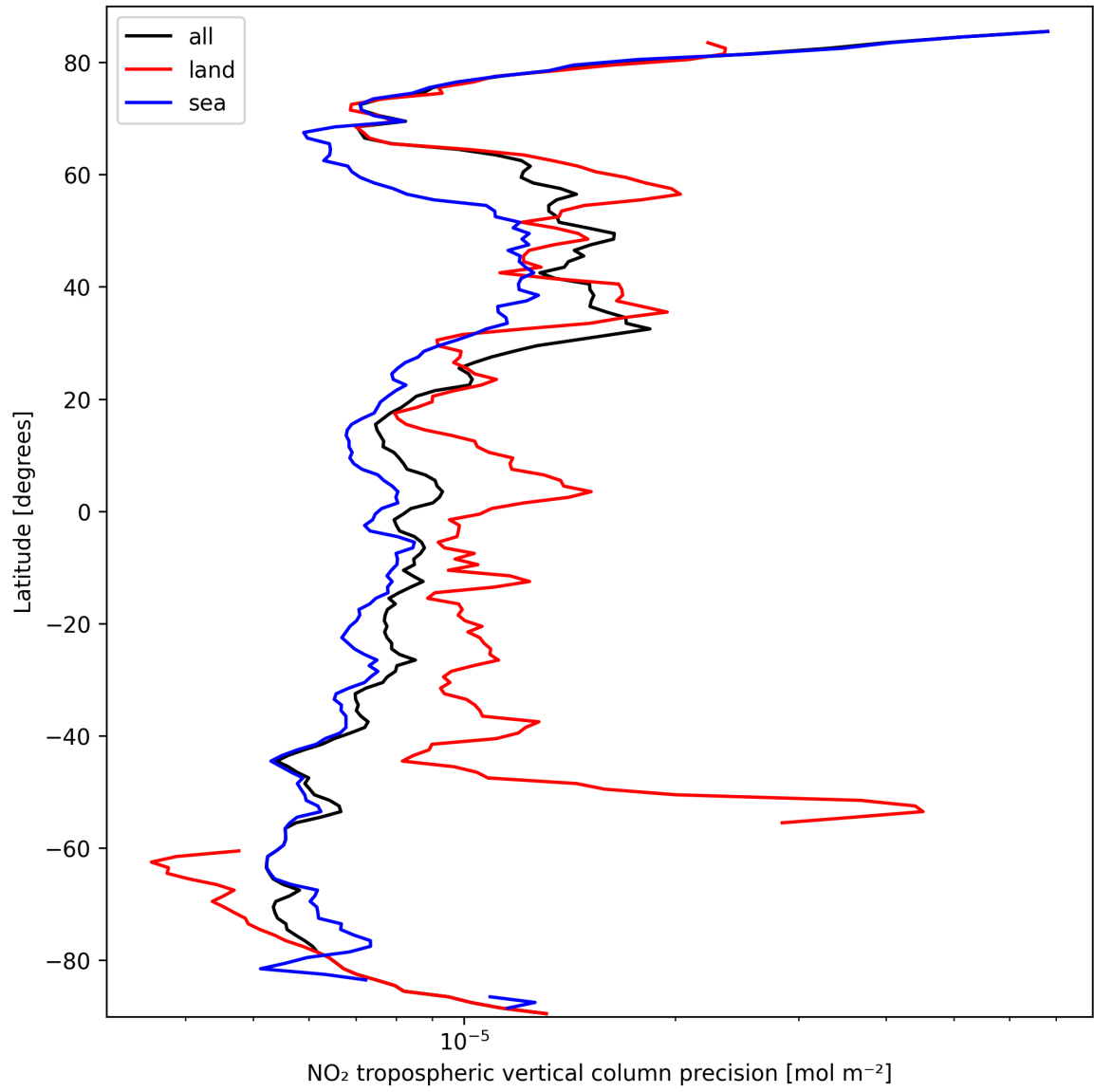
Figure 13: Zonal average of “NO 2 tropospheric vertical column precision” for 2025-03-14 to 2025-03-15.
