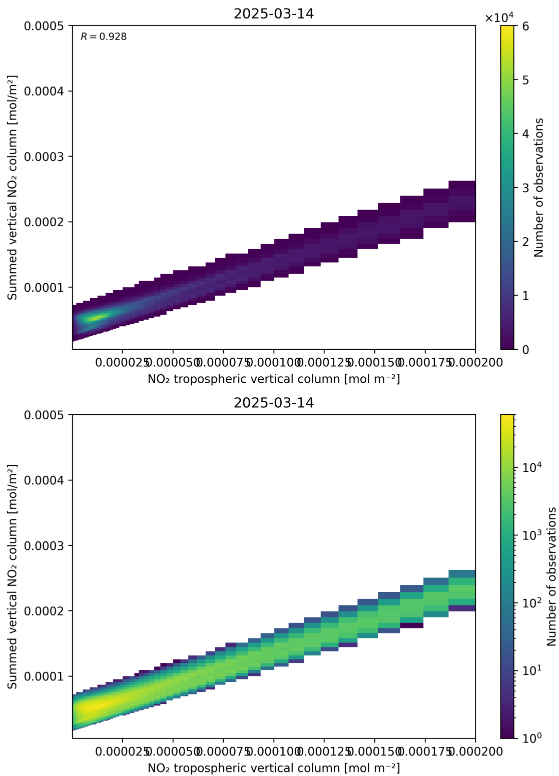
Figure 126: Scatter density plot of “NO 2 tropospheric vertical column” against “Summed vertical NO 2 column” for 2025-03-14 to 2025-03-15.
