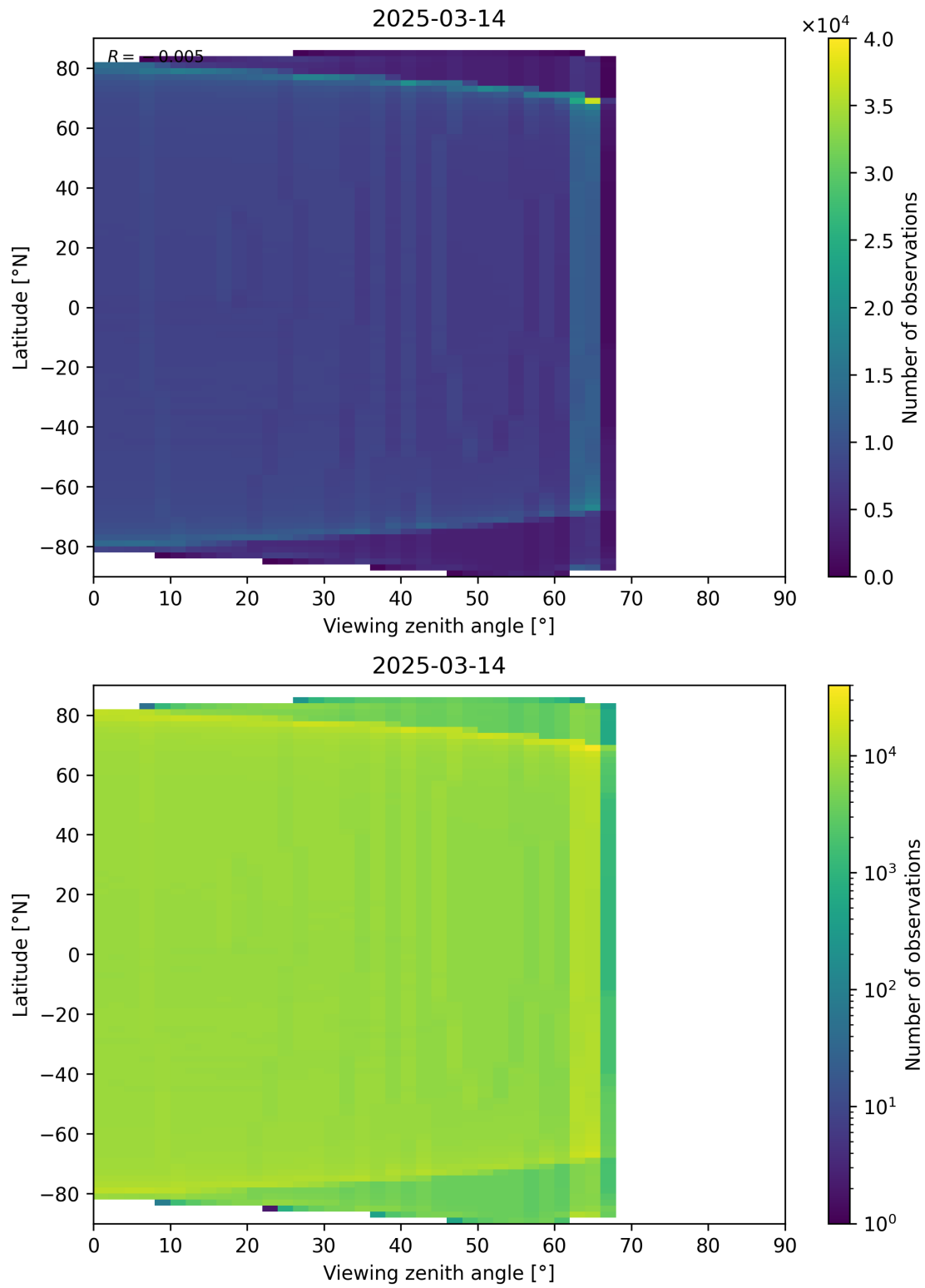
Figure 163: Scatter density plot of “Viewing zenith angle” against “Latitude” for 2025-03-14 to 2025-03-15.
