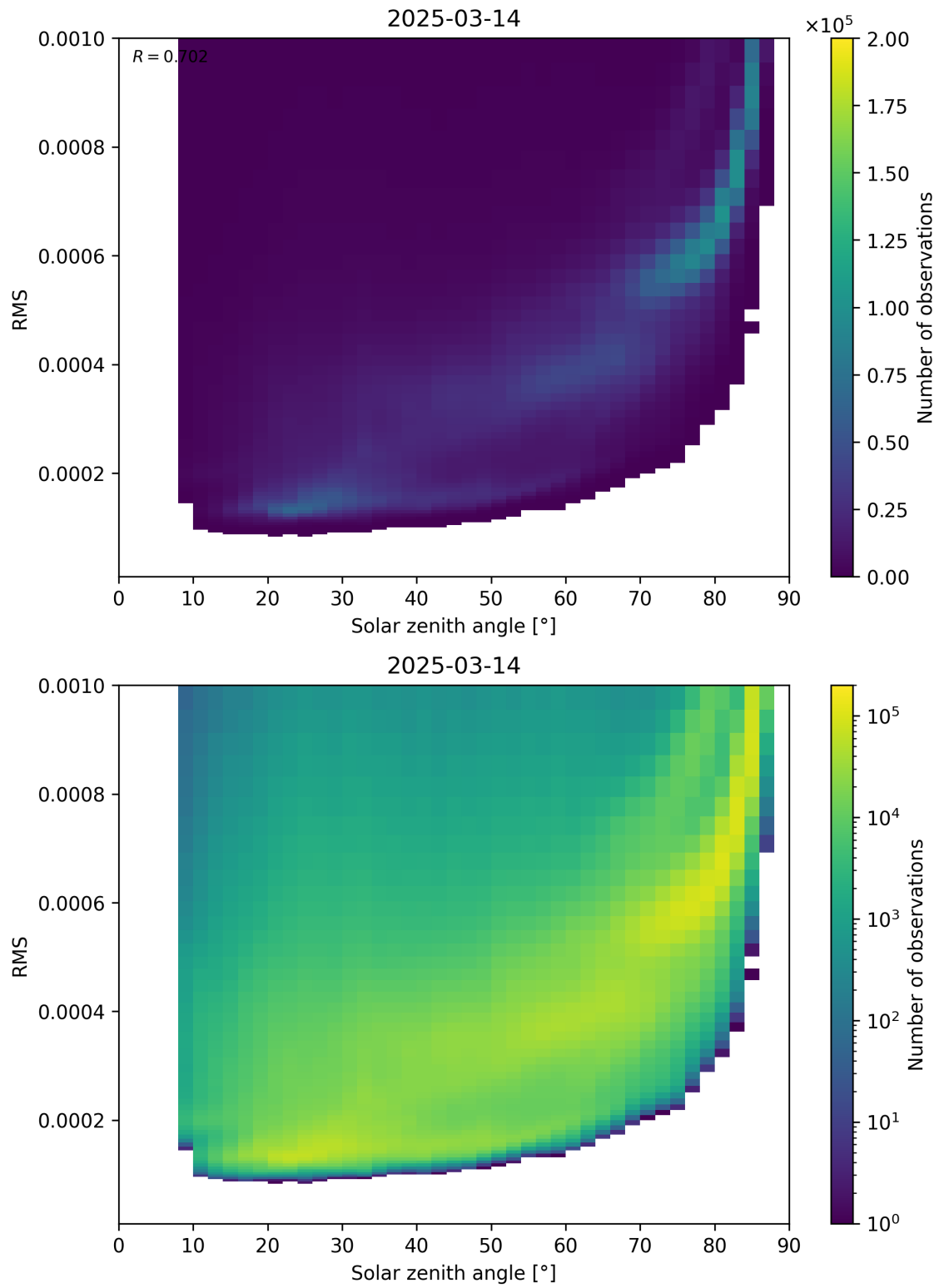
Figure 157: Scatter density plot of “Solar zenith angle” against “RMS” for 2025-03-14 to 2025-03-15.
