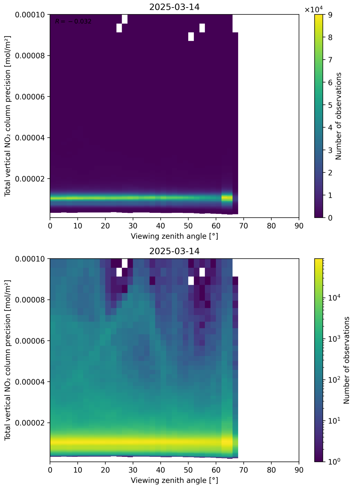
Figure 168: Scatter density plot of “Viewing zenith angle” against “Total vertical NO 2 column precision” for 2025-03-14 to 2025-03-15.
