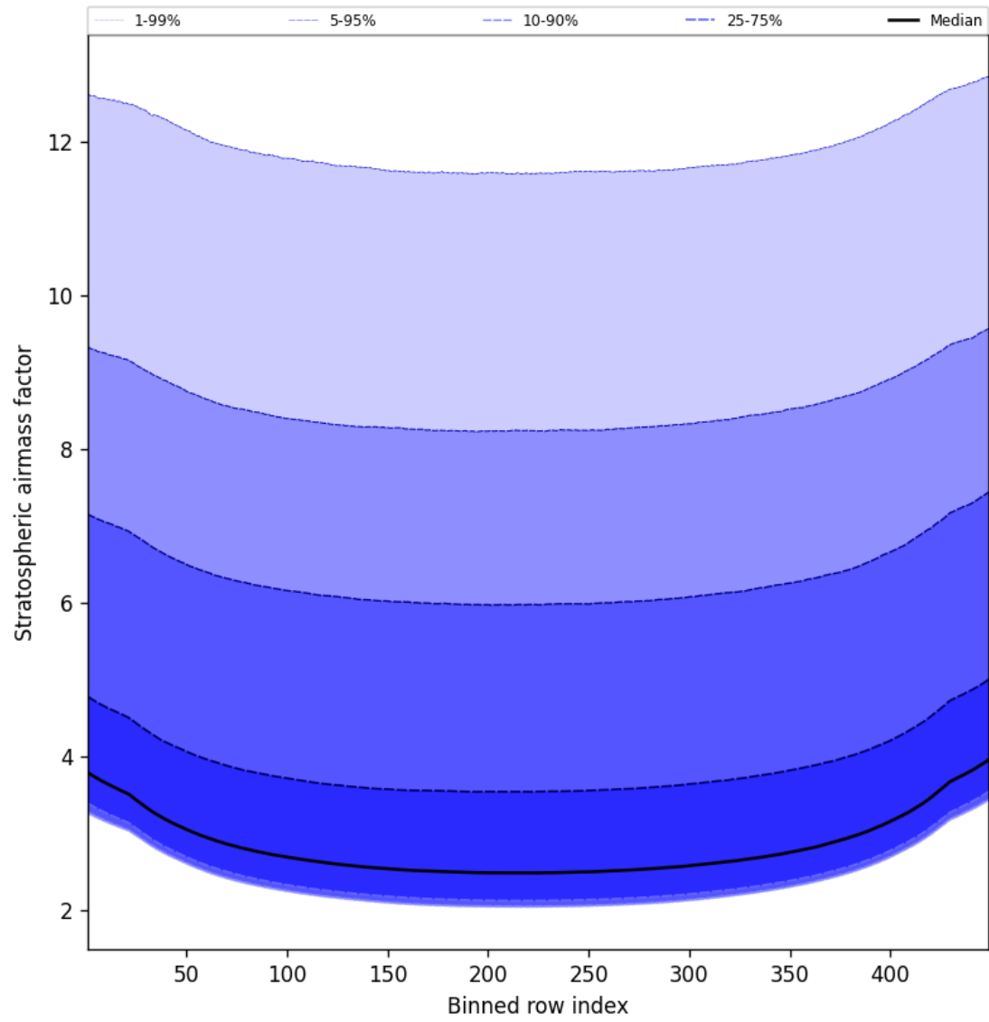
Figure 61: Along track statistics of “Stratospheric airmass factor” for 2025-03-14 to 2025-03-15
