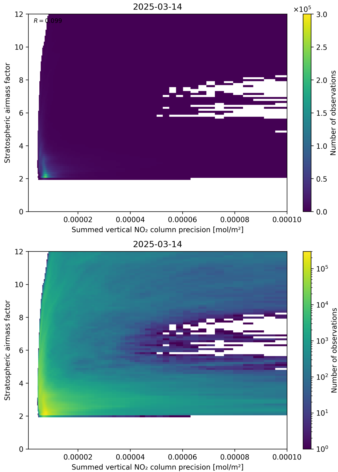
Figure 106: Scatter density plot of “Summed vertical NO 2 column precision” against “Stratospheric airmass factor” for 2025-03-14 to 2025-03-15.
