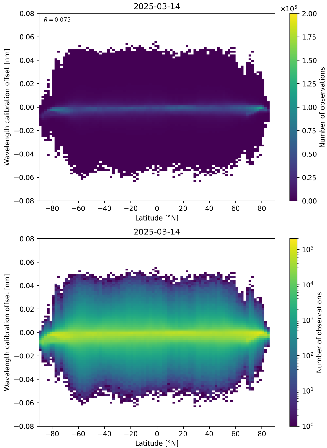
Figure 95: Scatter density plot of “Latitude” against “Wavelength calibration offset” for 2025-03-14 to 2025-03-15.
