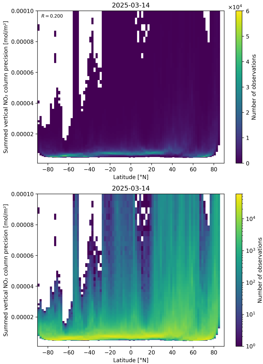
Figure 89: Scatter density plot of “Latitude” against “Summed vertical NO 2 column precision” for 2025-03-14 to 2025-03-15.
