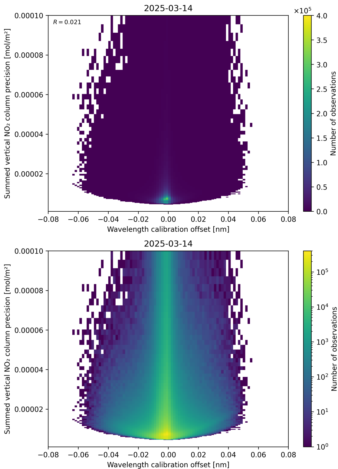
Figure 178: Scatter density plot of “Wavelength calibration offset” against “Summed vertical NO 2 column precision” for 2025-03-14 to 2025-03-15.
