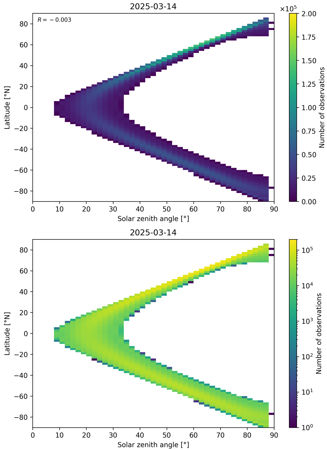
Figure 149: Scatter density plot of “Solar zenith angle” against “Latitude” for 2025-03-14 to 2025-03-15.
