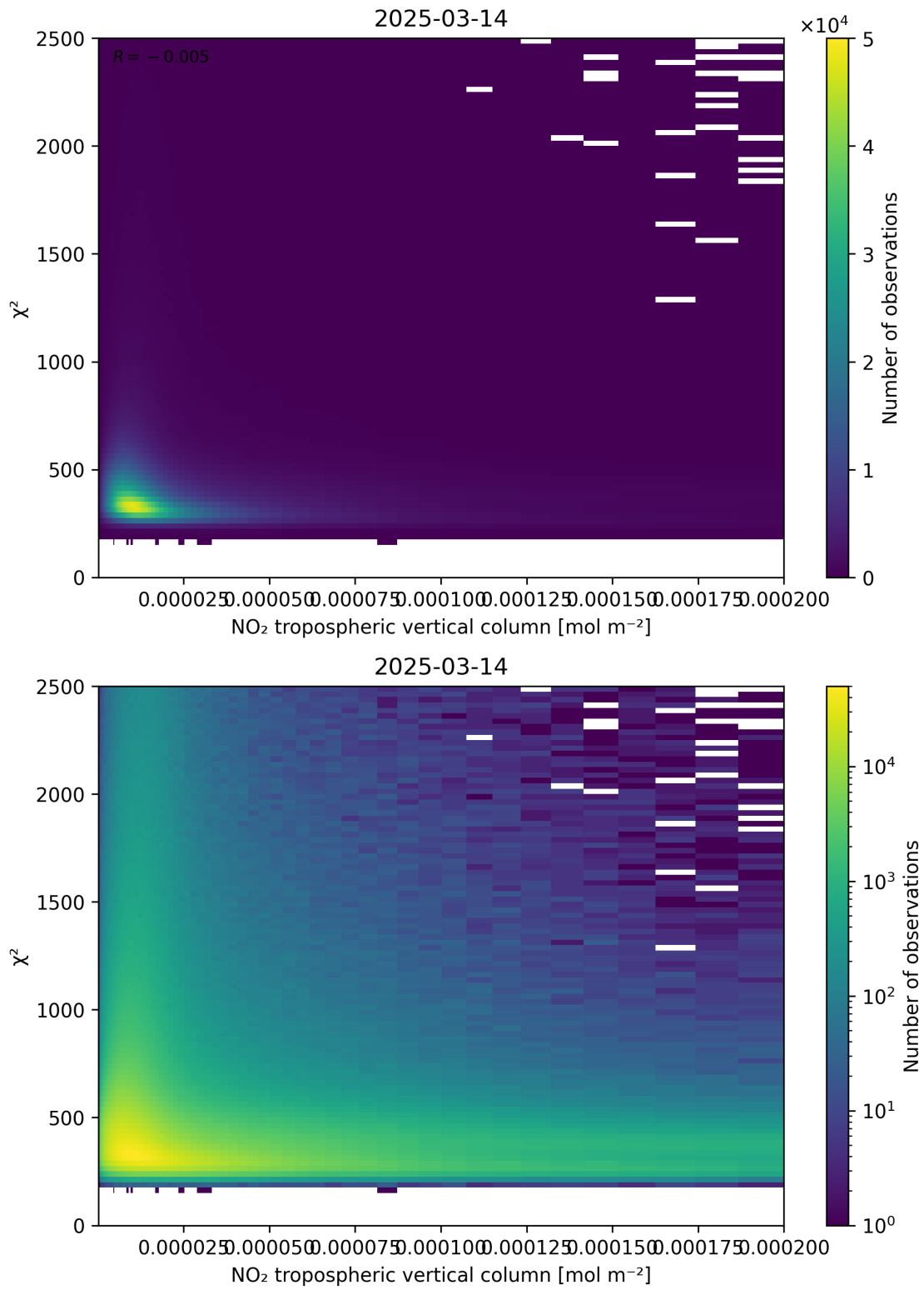
Figure 124: Scatter density plot of “NO 2 tropospheric vertical column” against “ \chi^2 ” for 2025-03-14 to 2025-03-15.
