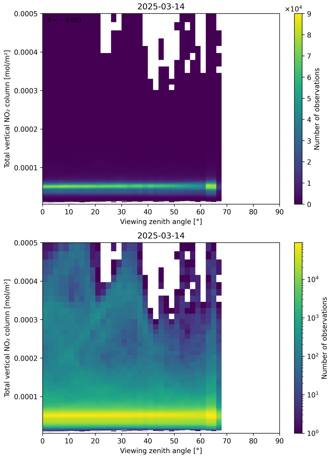
Figure 167: Scatter density plot of “Viewing zenith angle” against “Total vertical NO 2 column” for 2025-03-14 to 2025-03-15.
