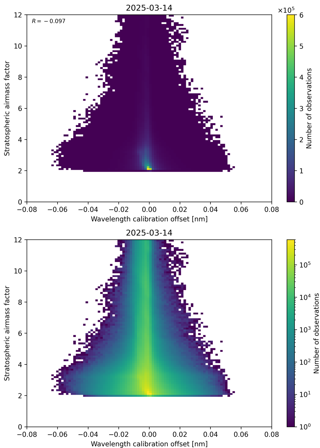
Figure 174: Scatter density plot of “Wavelength calibration offset” against “Stratospheric airmass factor” for 2025-03-14 to 2025-03-15.
