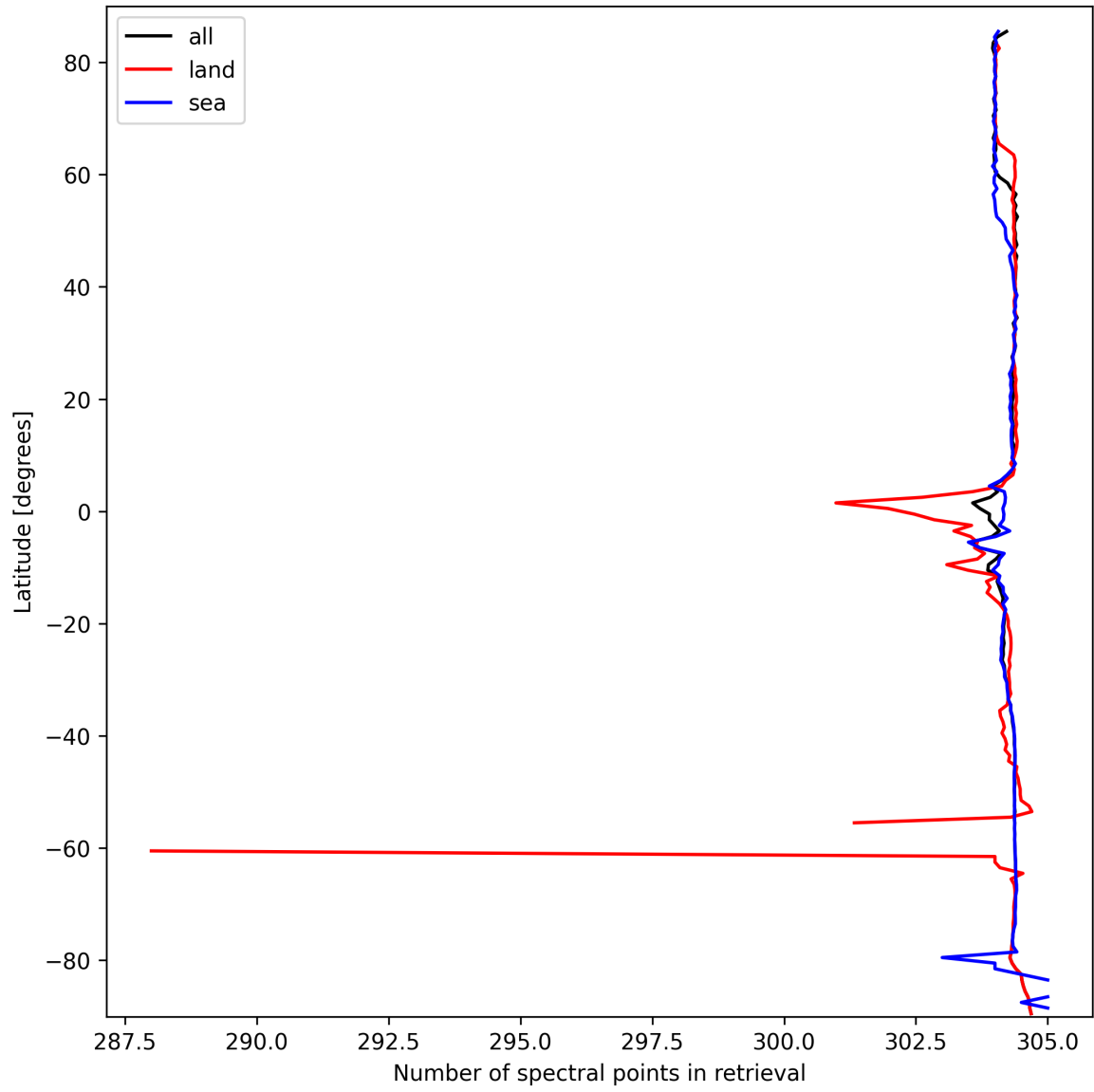
Figure 16: Zonal average of “Number of spectral points in retrieval” for 2025-03-14 to 2025-03-15.
