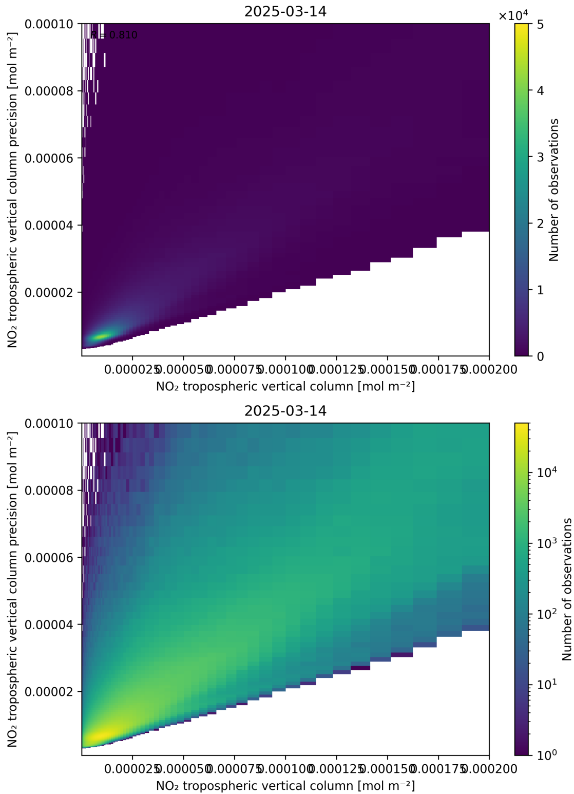
Figure 130: Scatter density plot of “NO 2 tropospheric vertical column” against “NO 2 tropospheric vertical column precision” for 2025-03-14 to 2025-03-15.
