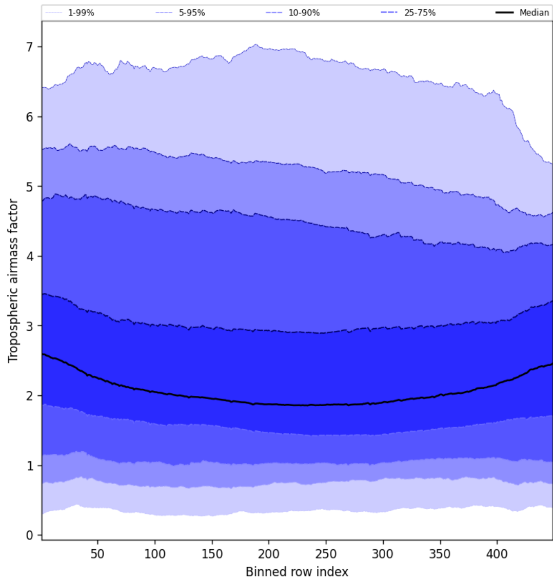
Figure 48: Along track statistics of “Tropospheric air mass factor” for 2025-03-14 to 2025-03-15
