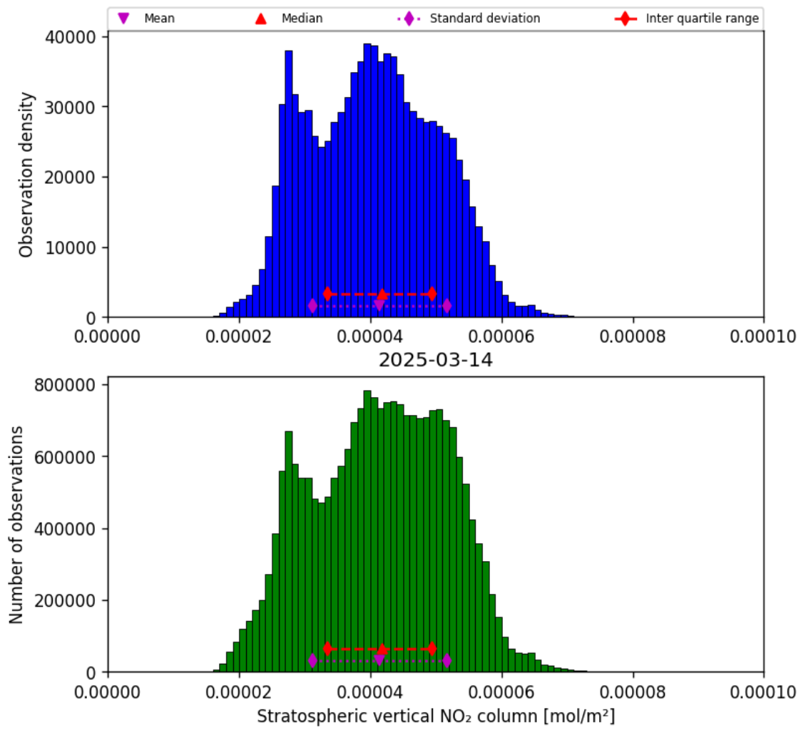
Figure 36: Histogram of “Stratospheric vertical NO 2 column” for 2025-03-14 to 2025-03-15
