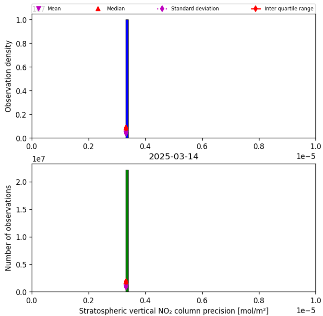
Figure 37: Histogram of “Stratospheric vertical NO 2 column precision” for 2025-03-14 to 2025-03-15
