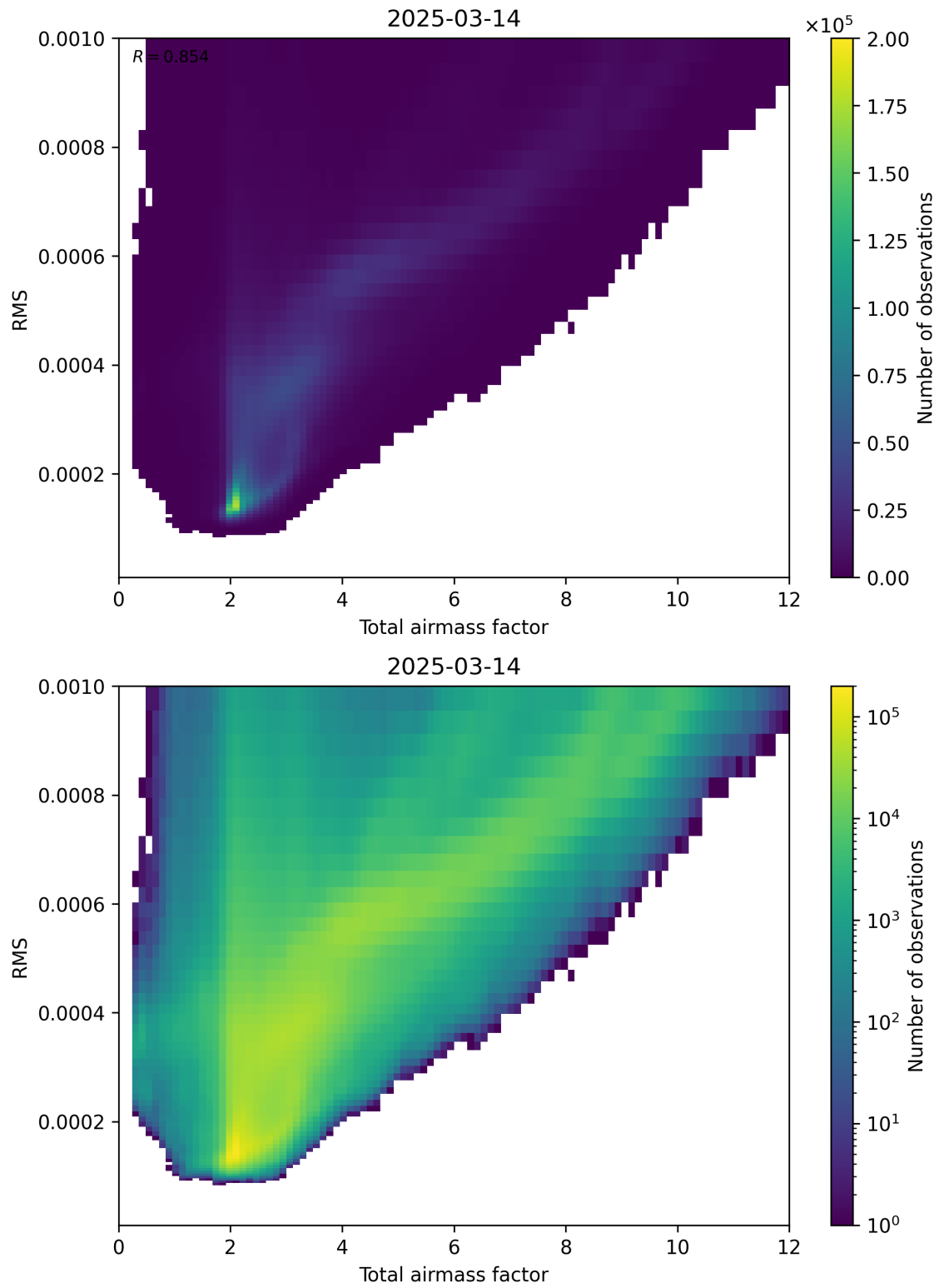
Figure 69: Scatter density plot of “Total airmass factor” against “RMS” for 2025-03-14 to 2025-03-15.
