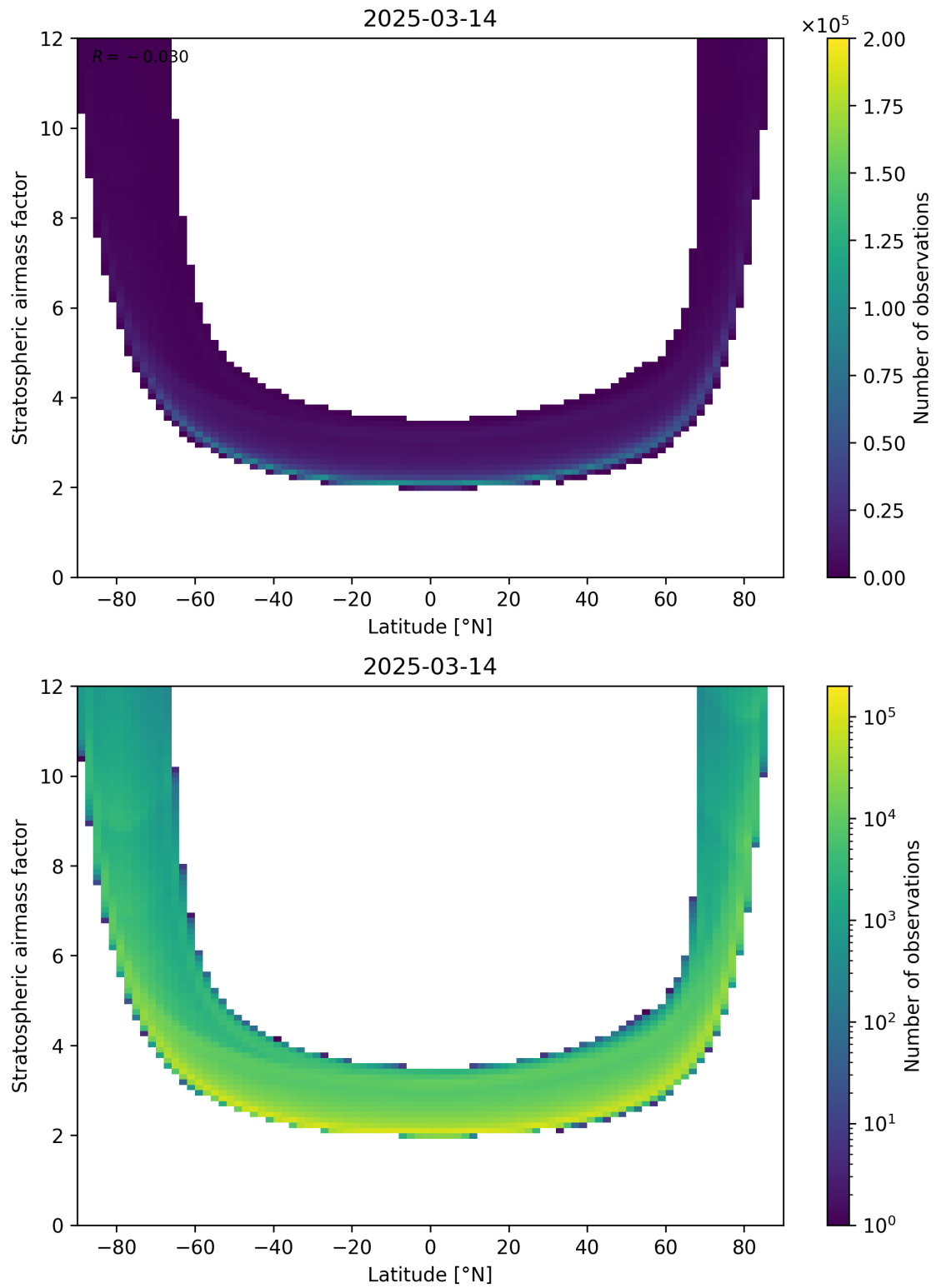
Figure 83: Scatter density plot of “Latitude” against “Stratospheric air mass factor” for 2025-03-14 to 2025-03-15.
