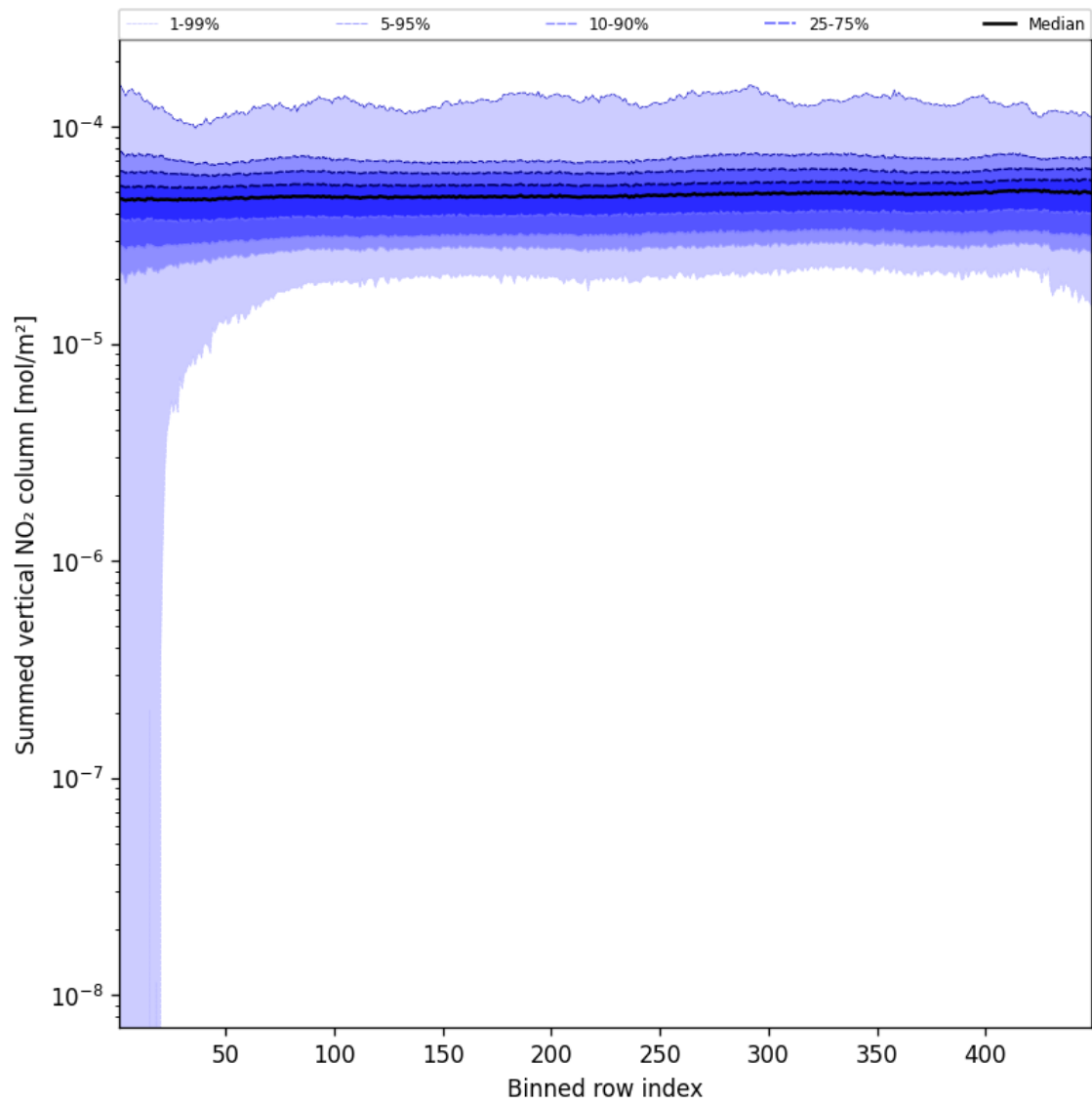
Figure 57: Along track statistics of “Summed vertical NO 2 column” for 2025-03-14 to 2025-03-15
