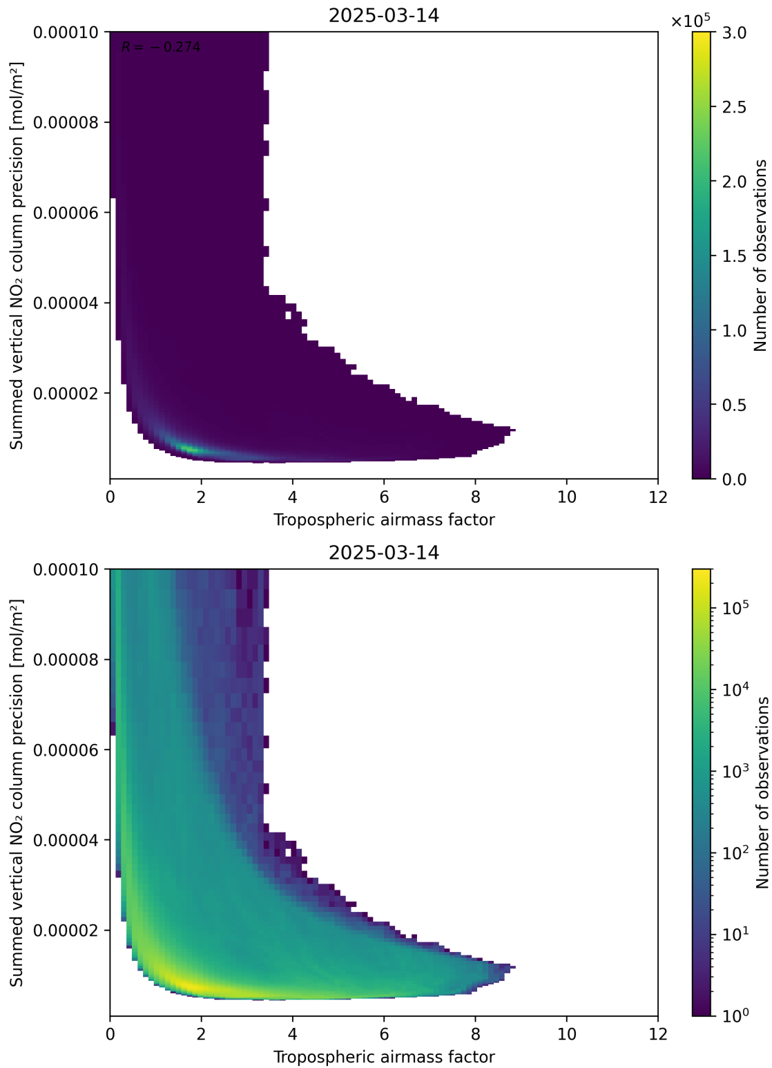
Figure 76: Scatter density plot of “Tropospheric airmass factor” against “Summed vertical NO 2 column precision” for 2025-03-14 to 2025-03-15.
