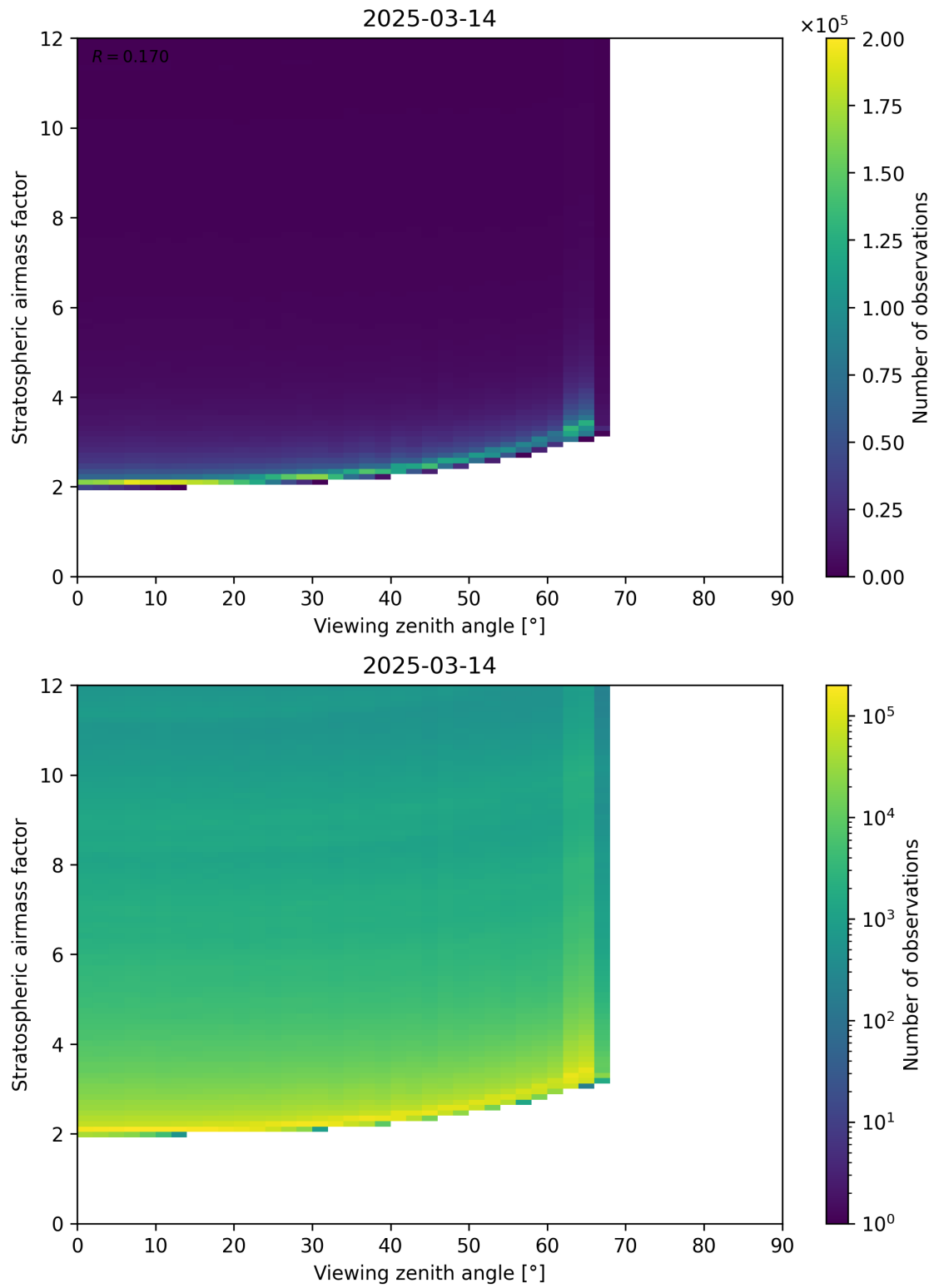
Figure 159: Scatter density plot of “Viewing zenith angle” against “Stratospheric airmass factor” for 2025-03-14 to 2025-03-15.
