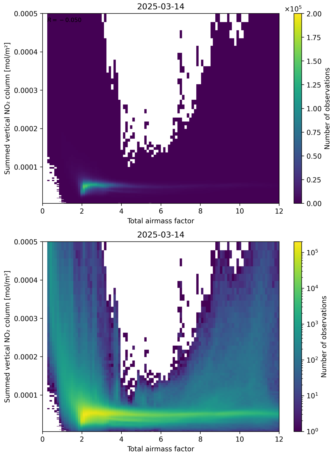
Figure 65: Scatter density plot of “Total airmass factor” against “Summed vertical NO 2 column” for 2025-03-14 to 2025-03-15.
