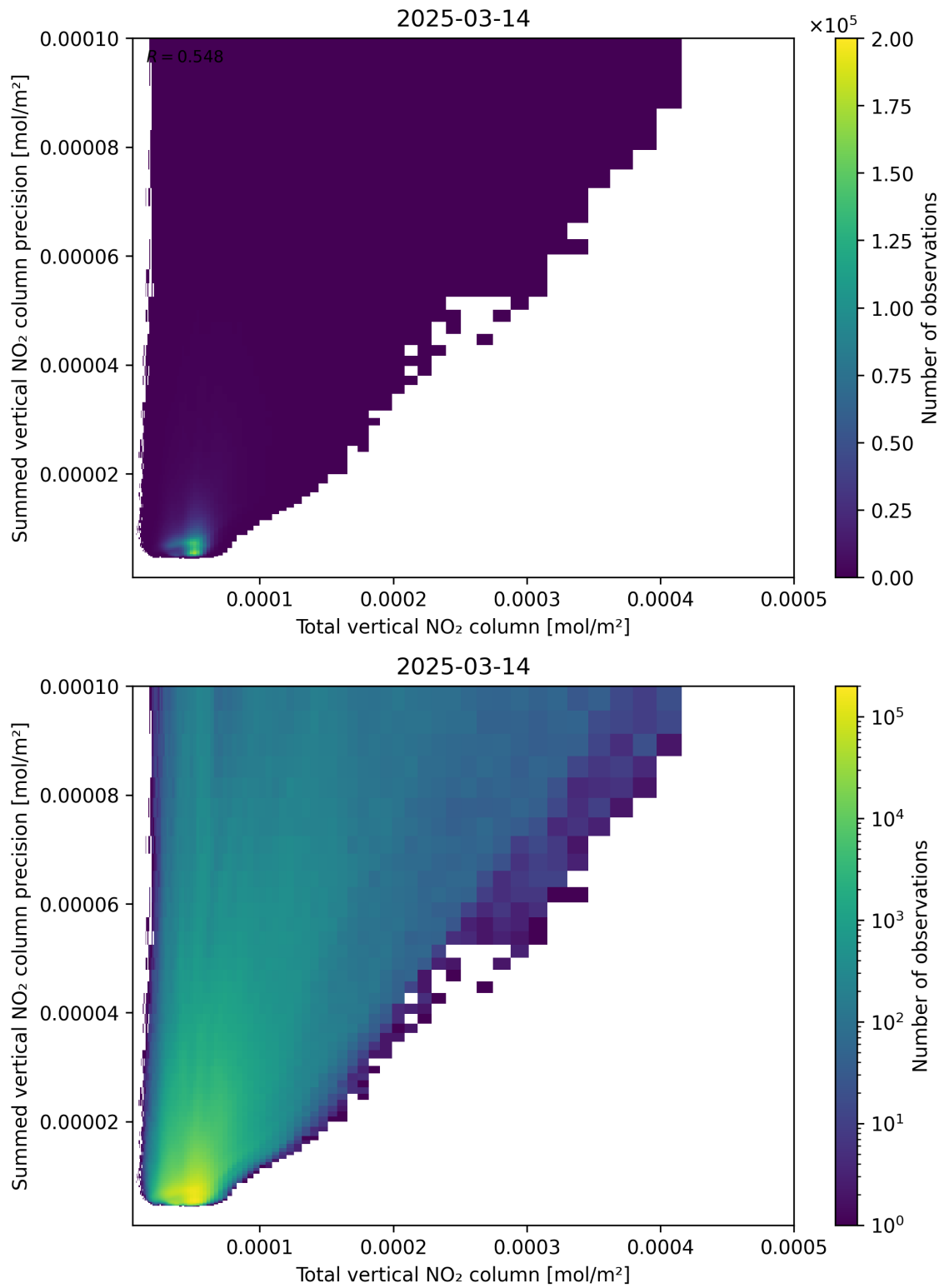
Figure 113: Scatter density plot of “Total vertical NO 2 column” against “Summed vertical NO 2 column precision” for 2025-03-14 to 2025-03-15.
