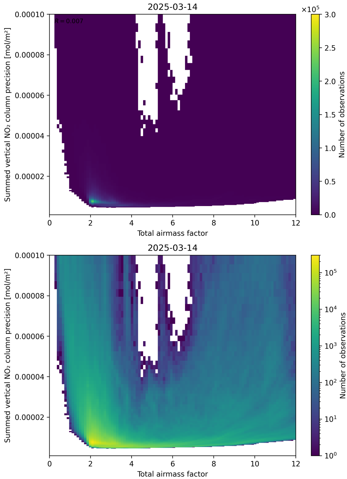
Figure 66: Scatter density plot of “Total airmass factor” against “Summed vertical NO 2 column precision” for 2025-03-14 to 2025-03-15.
