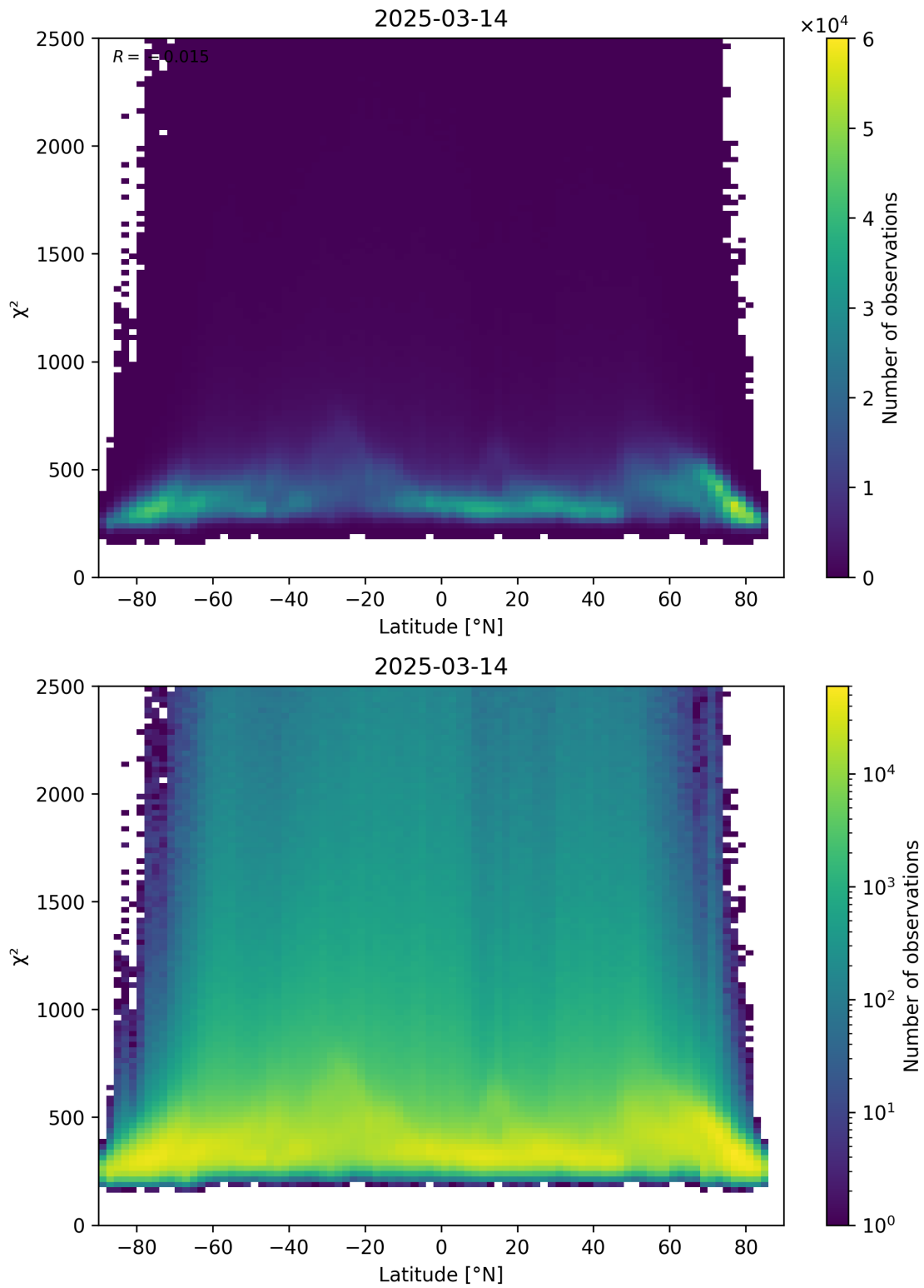
Figure 86: Scatter density plot of “Latitude” against “ \chi^2 ” for 2025-03-14 to 2025-03-15.
