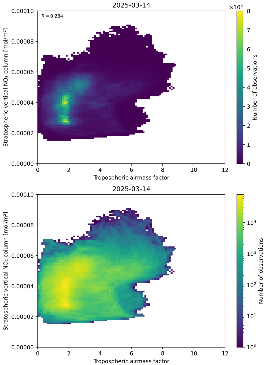
Figure 74: Scatter density plot of “Tropospheric air mass factor” against “Stratospheric vertical NO 2 column” for 2025-03-14 to 2025-03-15.
