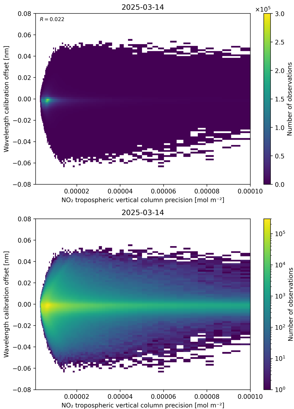
Figure 141: Scatter density plot of “NO 2 tropospheric vertical column precision” against “Wavelength calibration offset” for 2025-03-14 to 2025-03-15.
