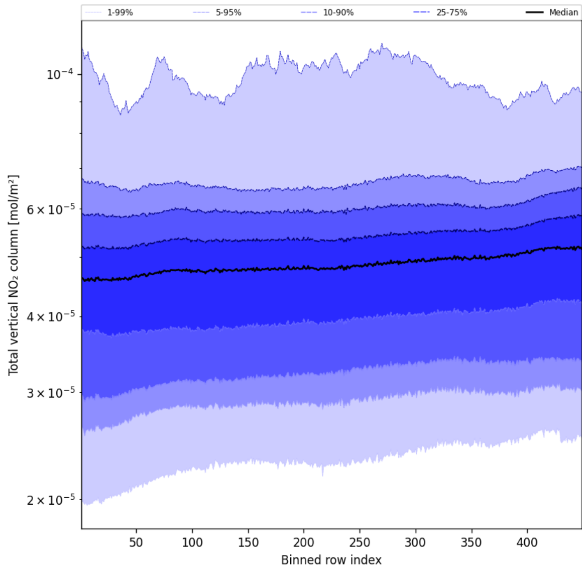
Figure 55: Along track statistics of “Total vertical NO 2 column” for 2025-03-14 to 2025-03-15
