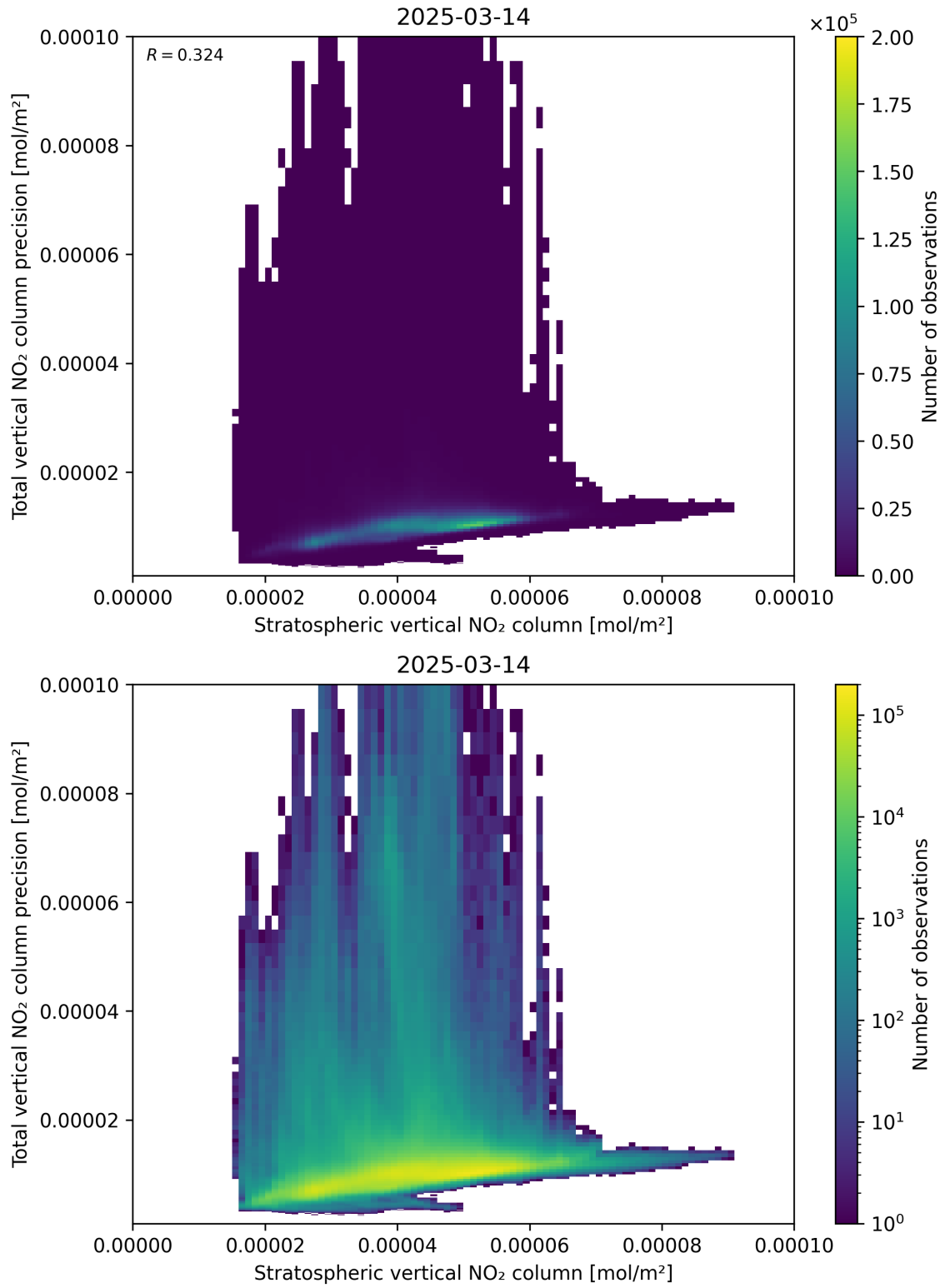
Figure 101: Scatter density plot of “Stratospheric vertical NO 2 column” against “Total vertical NO 2 column precision” for 2025-03-14 to 2025-03-15.
