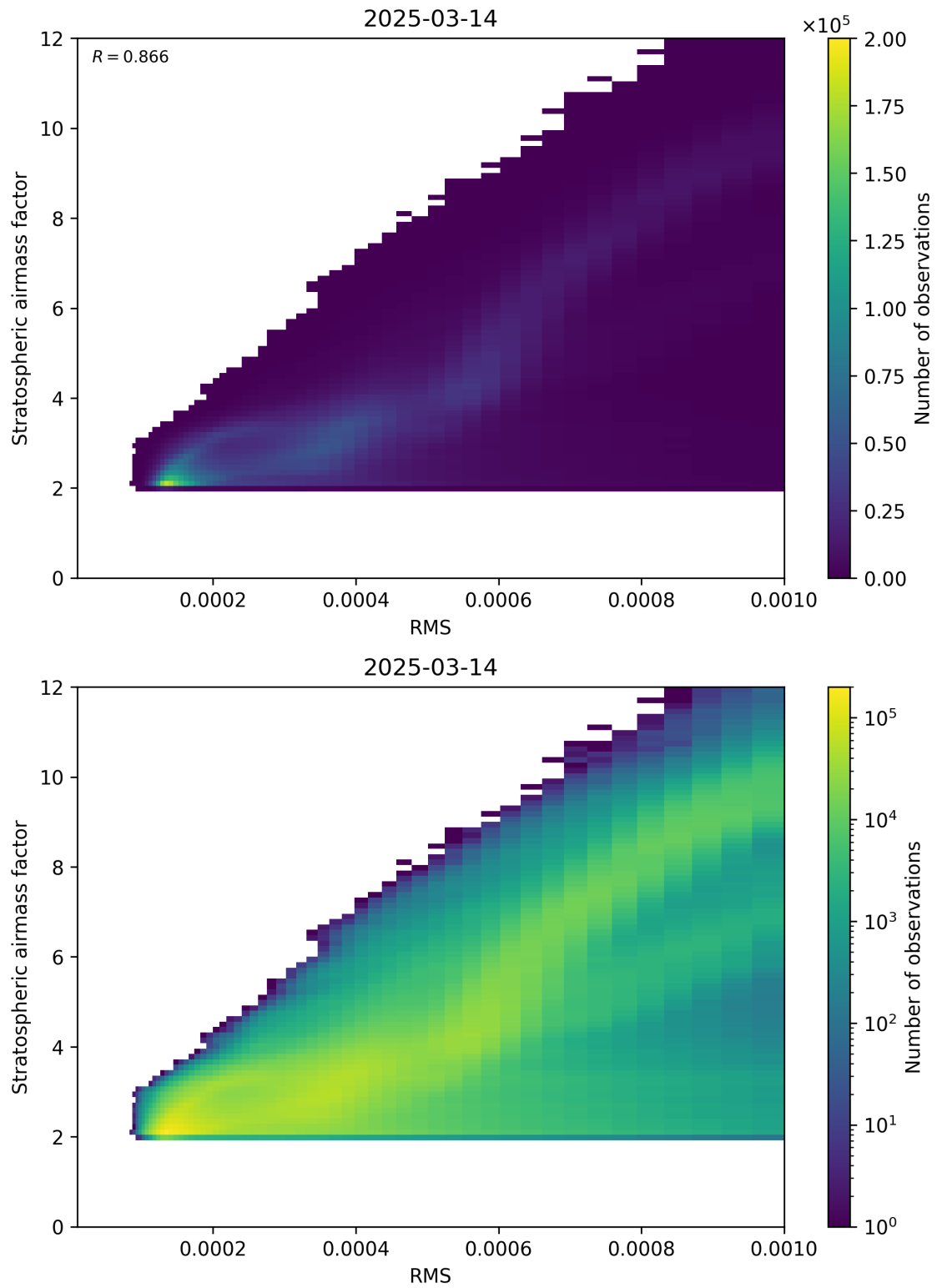
Figure 144: Scatter density plot of “RMS” against “Stratospheric airmass factor” for 2025-03-14 to 2025-03-15.
