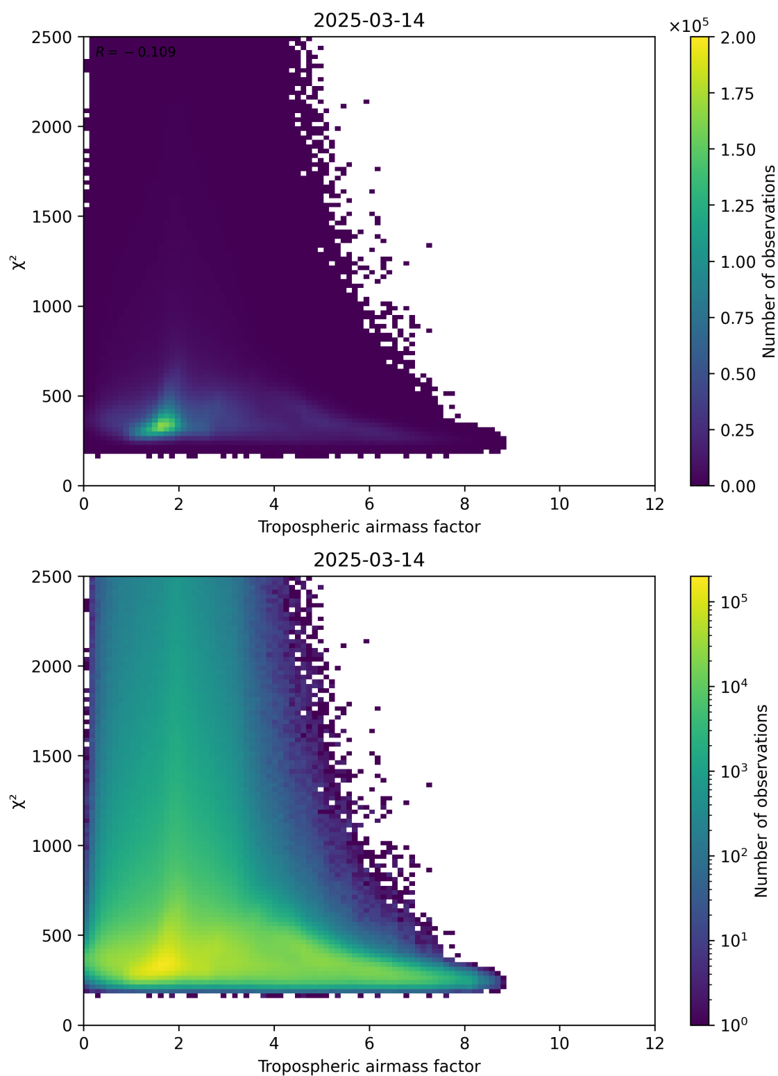
Figure 73: Scatter density plot of “Tropospheric airmass factor” against “ \chi^2 ” for 2025-03-14 to 2025-03-15.
