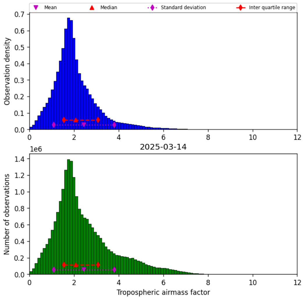
Figure 31: Histogram of “Tropospheric airmass factor” for 2025-03-14 to 2025-03-15
