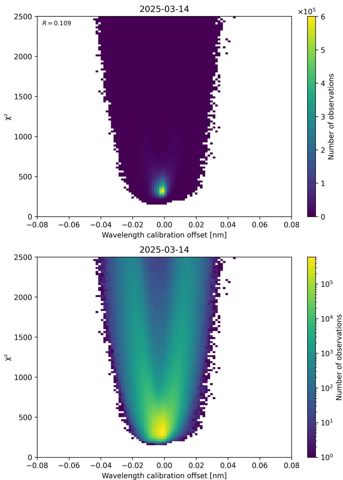
Figure 175: Scatter density plot of “Wavelength calibration offset” against “ \chi^2 ” for 2025-03-14 to 2025-03-15.
