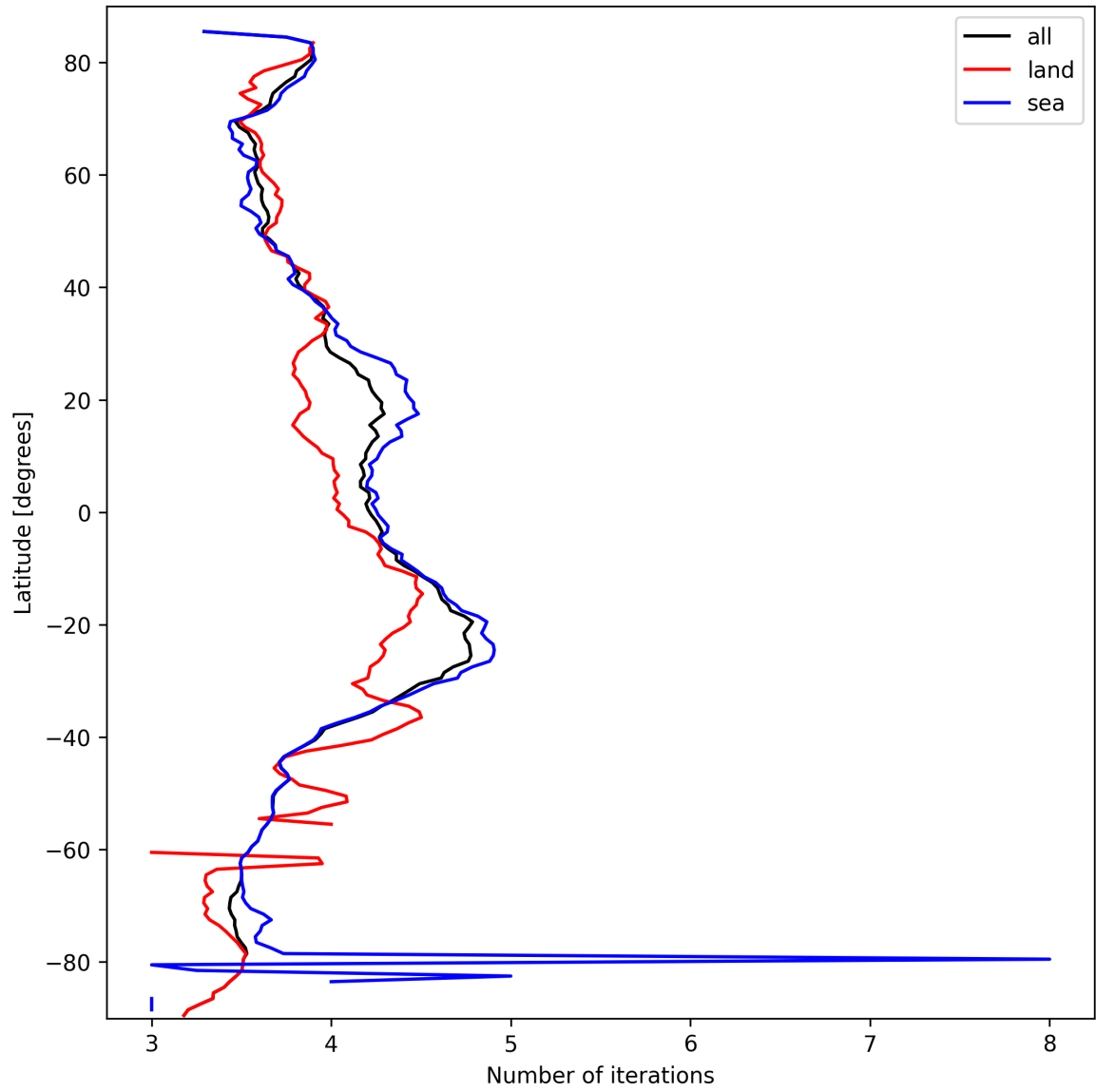
Figure 17: Zonal average of “Number of iterations” for 2025-03-14 to 2025-03-15.
