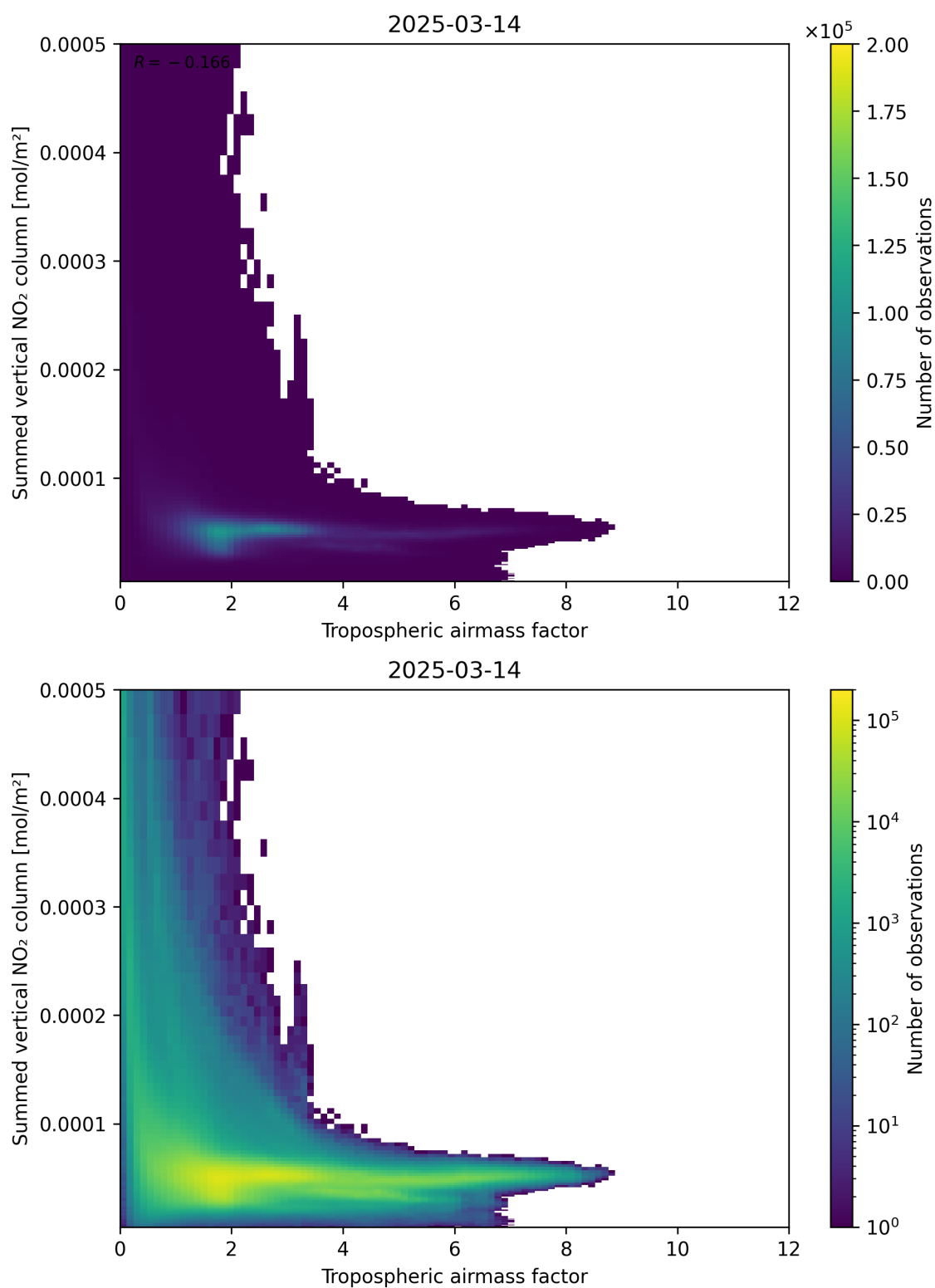
Figure 75: Scatter density plot of “Tropospheric air mass factor” against “Summed vertical NO 2 column” for 2025-03-14 to 2025-03-15.
