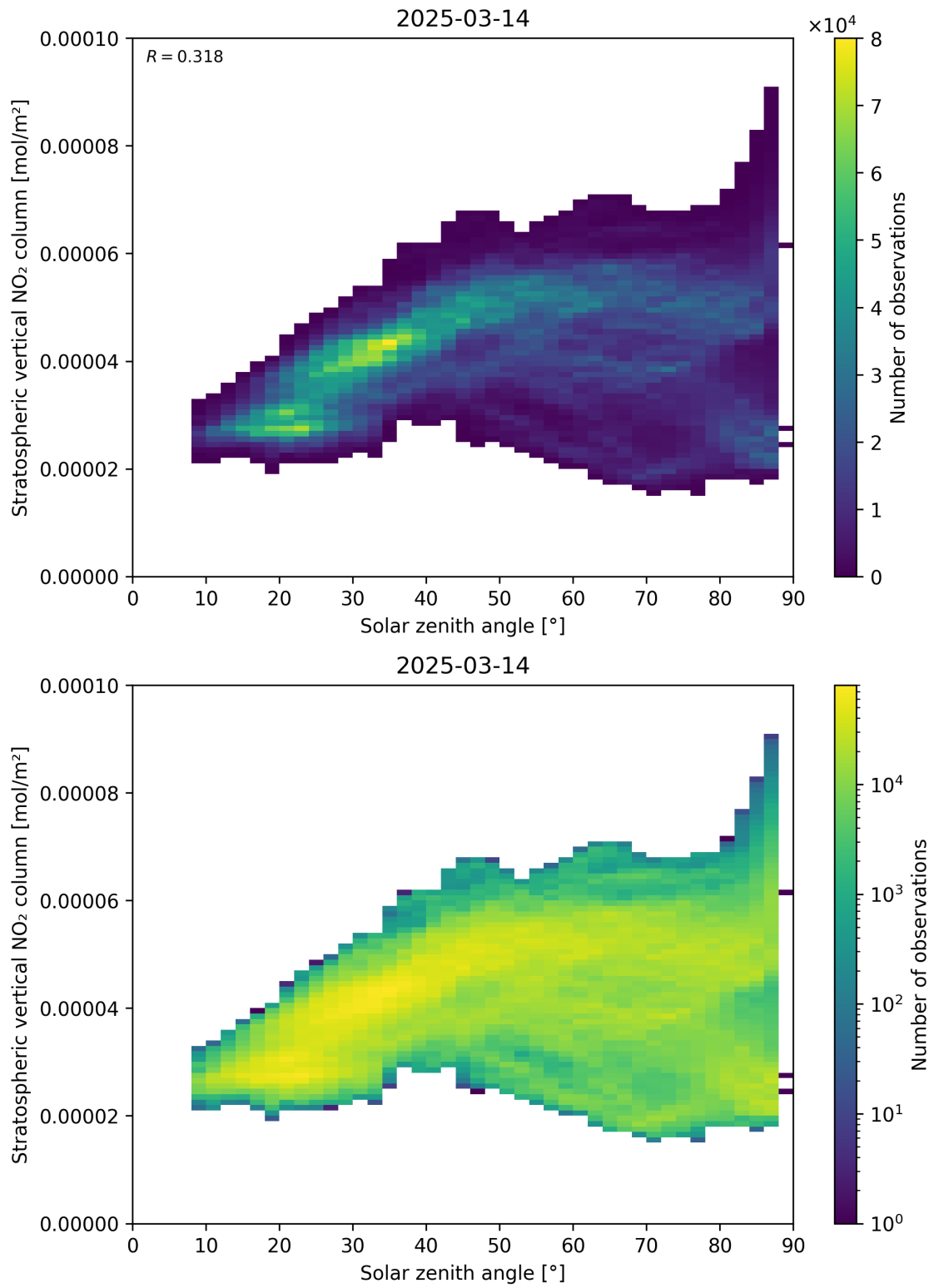
Figure 150: Scatter density plot of “Solar zenith angle” against “Stratospheric vertical NO 2 column” for 2025-03-14 to 2025-03-15.
