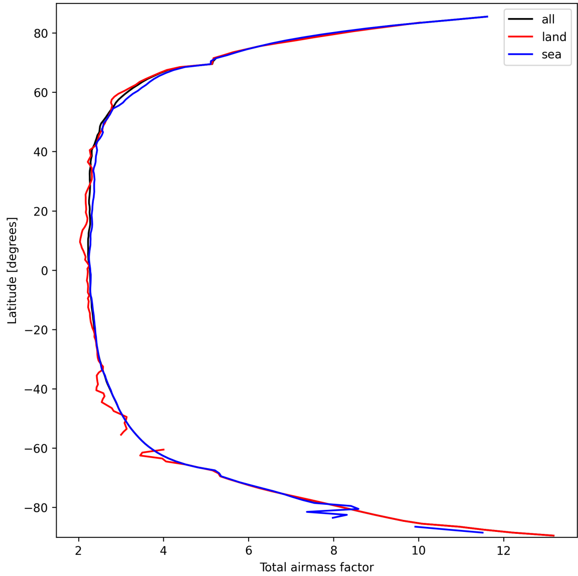
Figure 15: Zonal average of “Total airmass factor” for 2025-03-14 to 2025-03-15.
