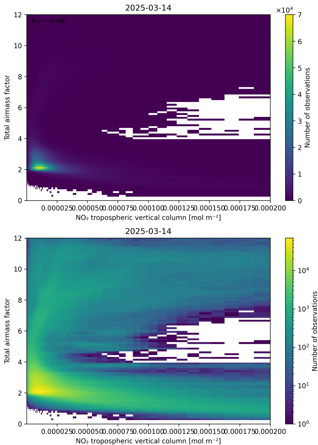
Figure 122: Scatter density plot of “NO 2 tropospheric vertical column” against “Total air mass factor” for 2025-03-14 to 2025-03-15.
