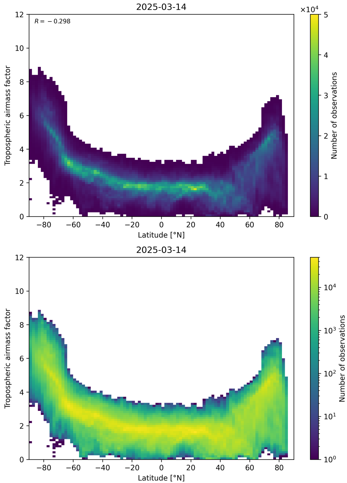
Figure 85: Scatter density plot of “Latitude” against “Tropospheric airmass factor” for 2025-03-14 to 2025-03-15.
