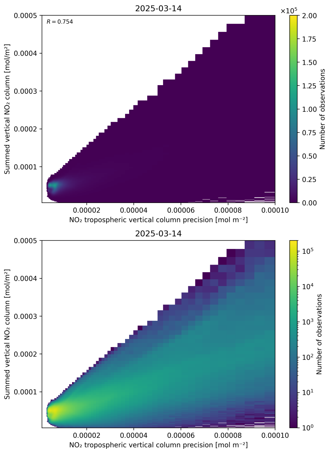
Figure 136: Scatter density plot of “NO 2 tropospheric vertical column precision” against “Summed vertical NO 2 column” for 2025-03-14 to 2025-03-15.
