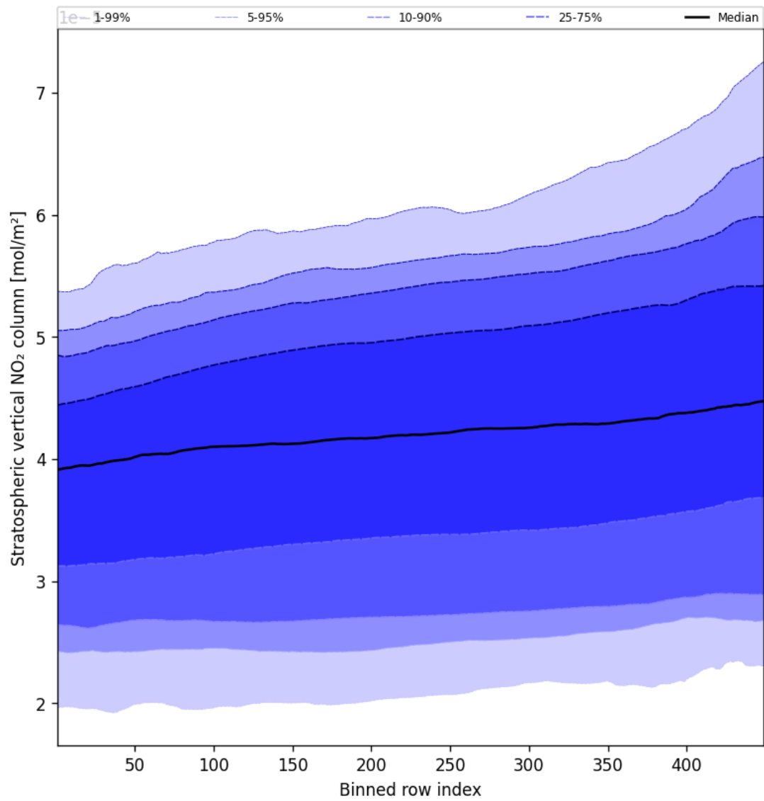
Figure 53: Along track statistics of “Stratospheric vertical NO 2 column” for 2025-03-14 to 2025-03-15
