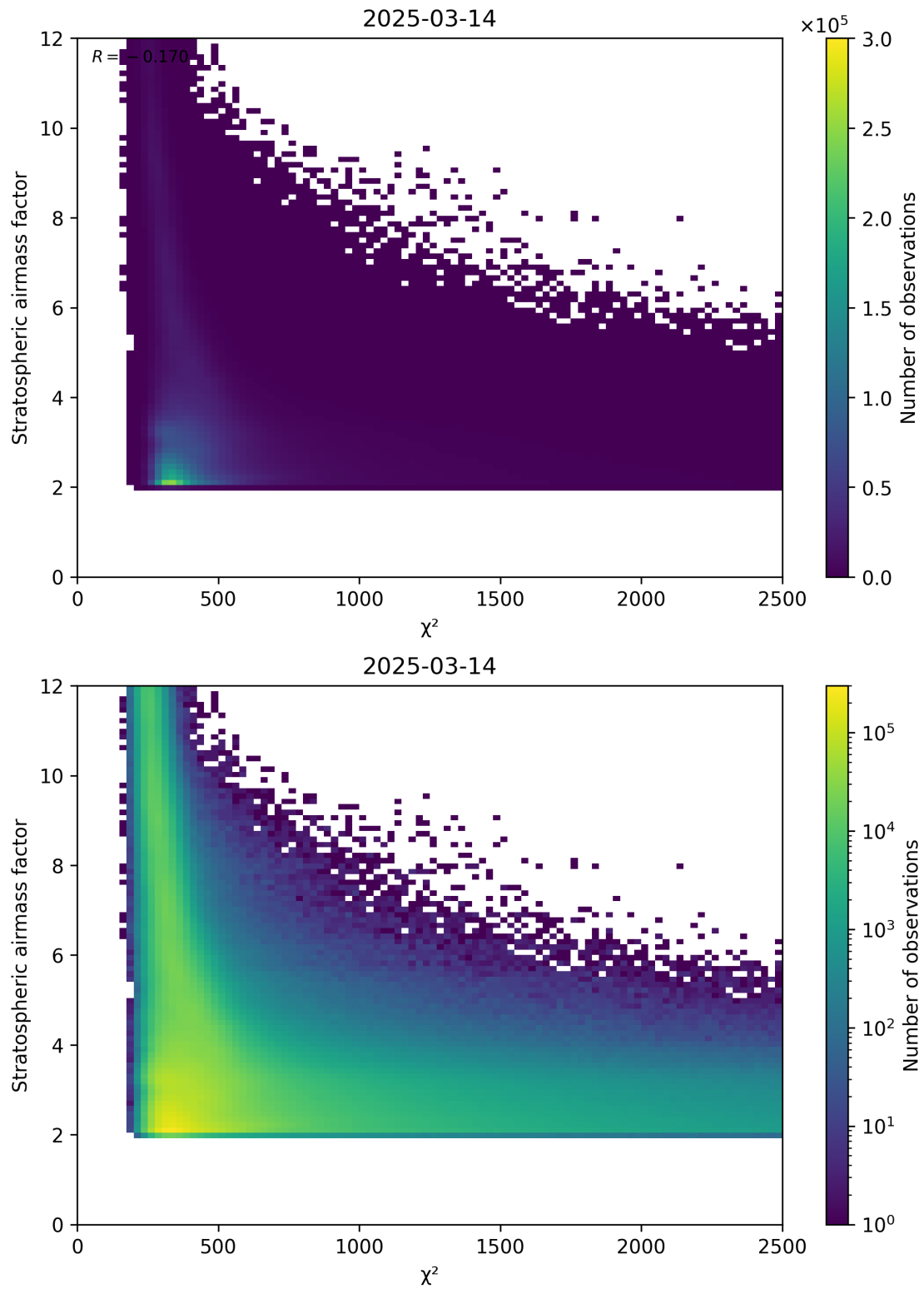
Figure 81: Scatter density plot of “ \chi^2 ” against “Stratospheric airmass factor” for 2025-03-14 to 2025-03-15.
