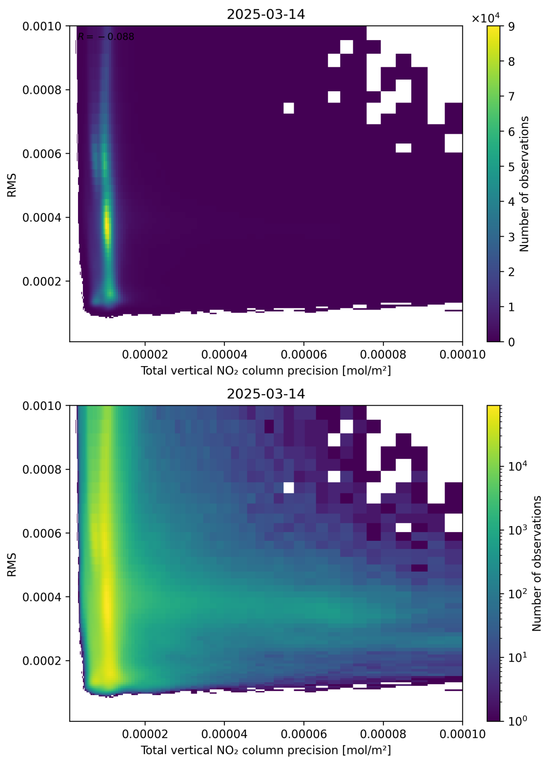
Figure 119: Scatter density plot of “Total vertical NO 2 column precision” against “RMS” for 2025-03-14 to 2025-03-15.
