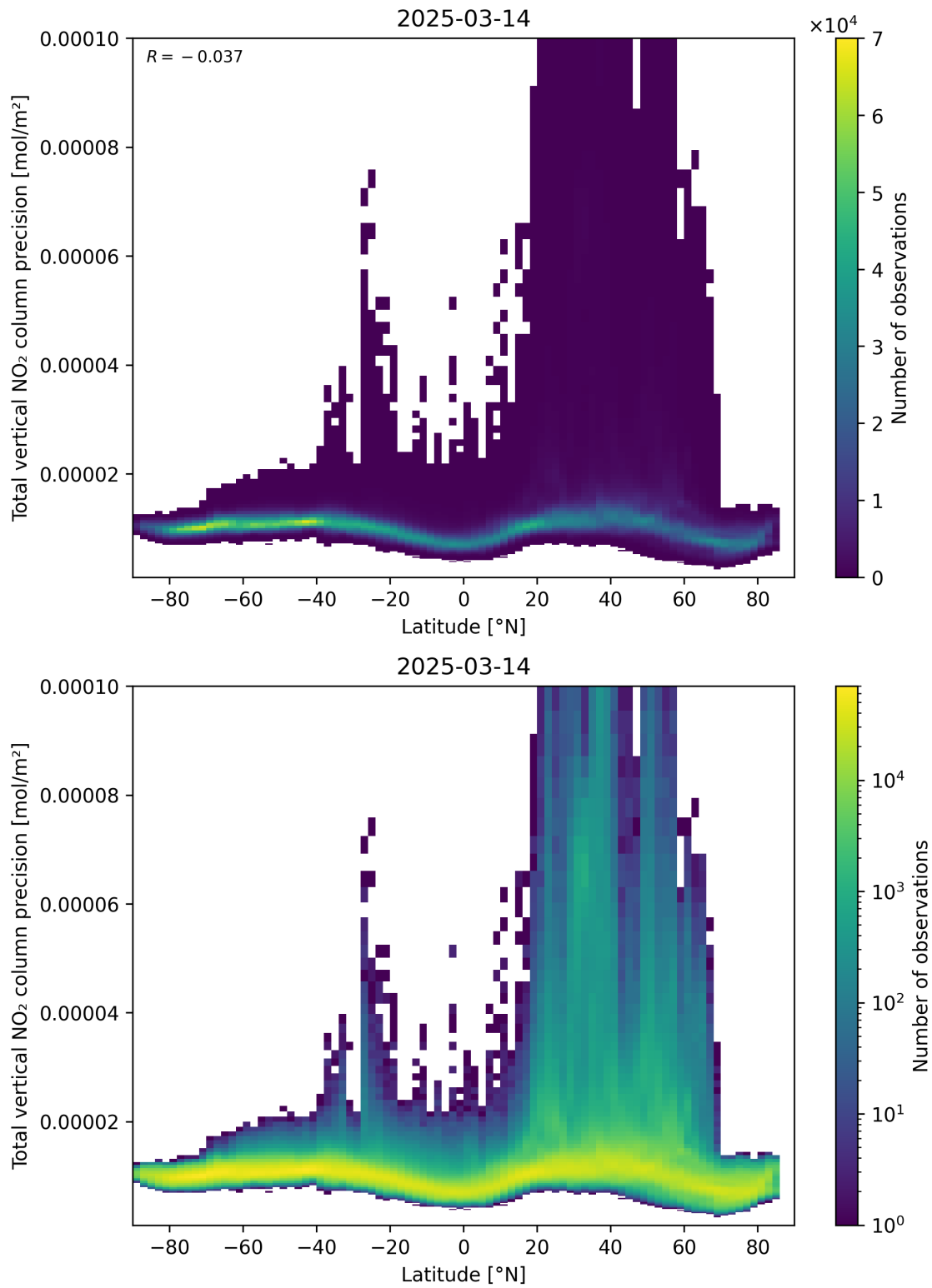
Figure 91: Scatter density plot of “Latitude” against “Total vertical NO 2 column precision” for 2025-03-14 to 2025-03-15.
