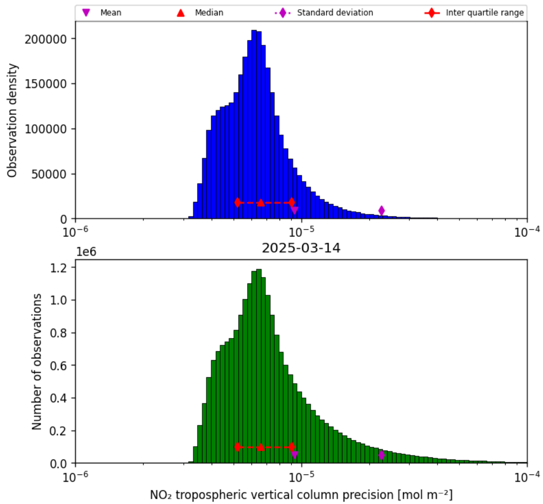
Figure 30: Histogram of “NO 2 tropospheric vertical column precision” for 2025-03-14 to 2025-03-15
