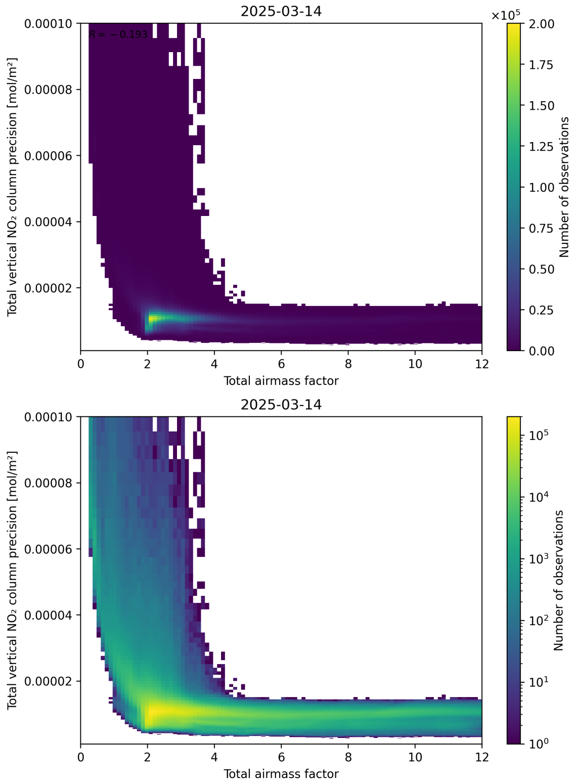
Figure 68: Scatter density plot of “Total airmass factor” against “Total vertical NO 2 column precision” for 2025-03-14 to 2025-03-15.
