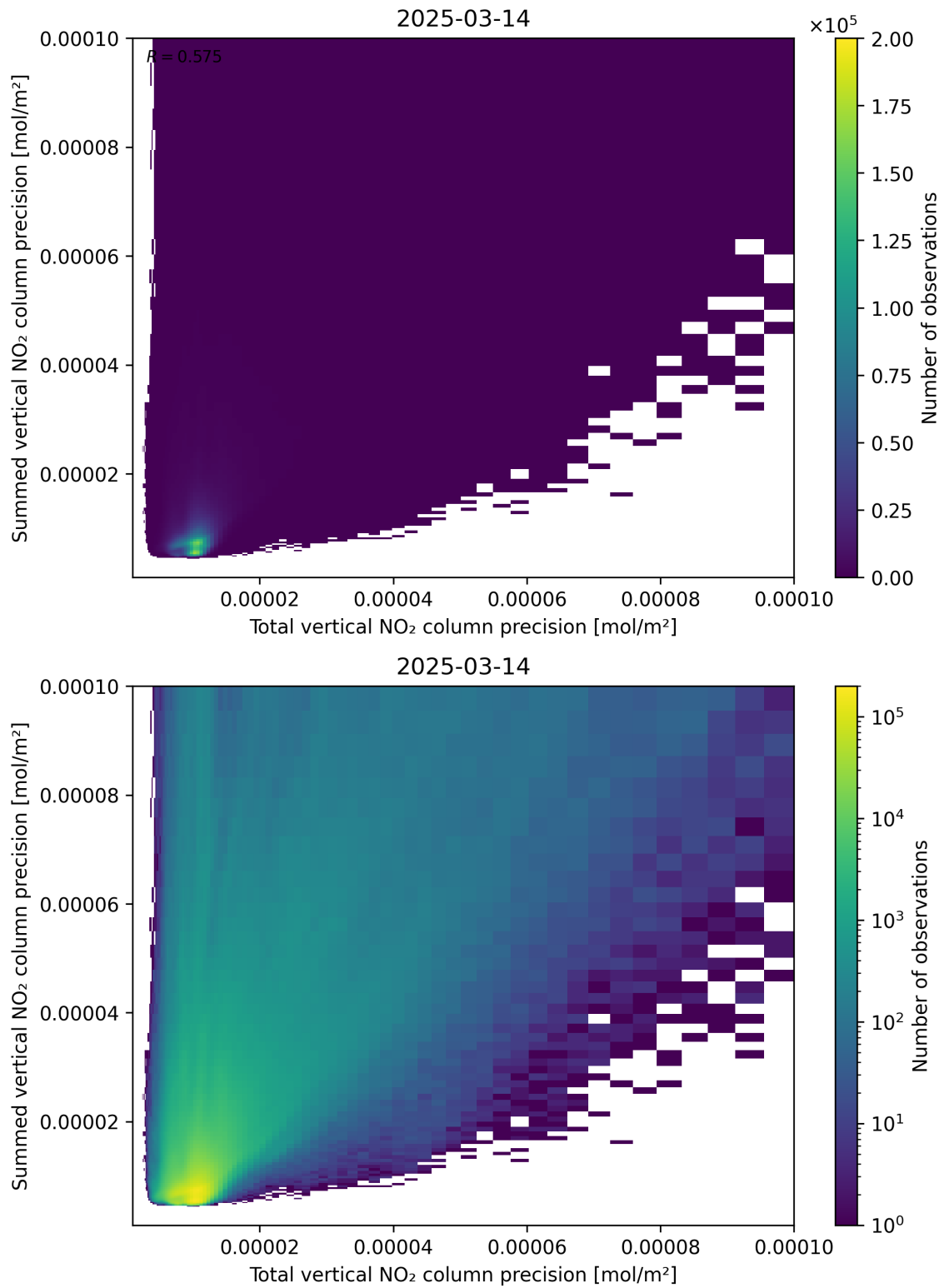
Figure 118: Scatter density plot of “Total vertical NO 2 column precision” against “Summed vertical NO 2 column precision” for 2025-03-14 to 2025-03-15.
