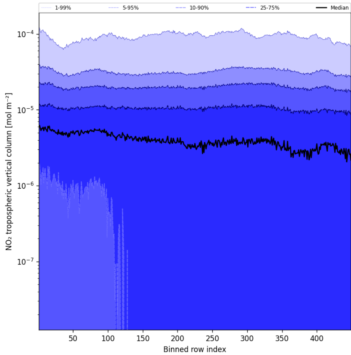
Figure 46: Along track statistics of “NO 2 tropospheric vertical column” for 2025-03-14 to 2025-03-15
