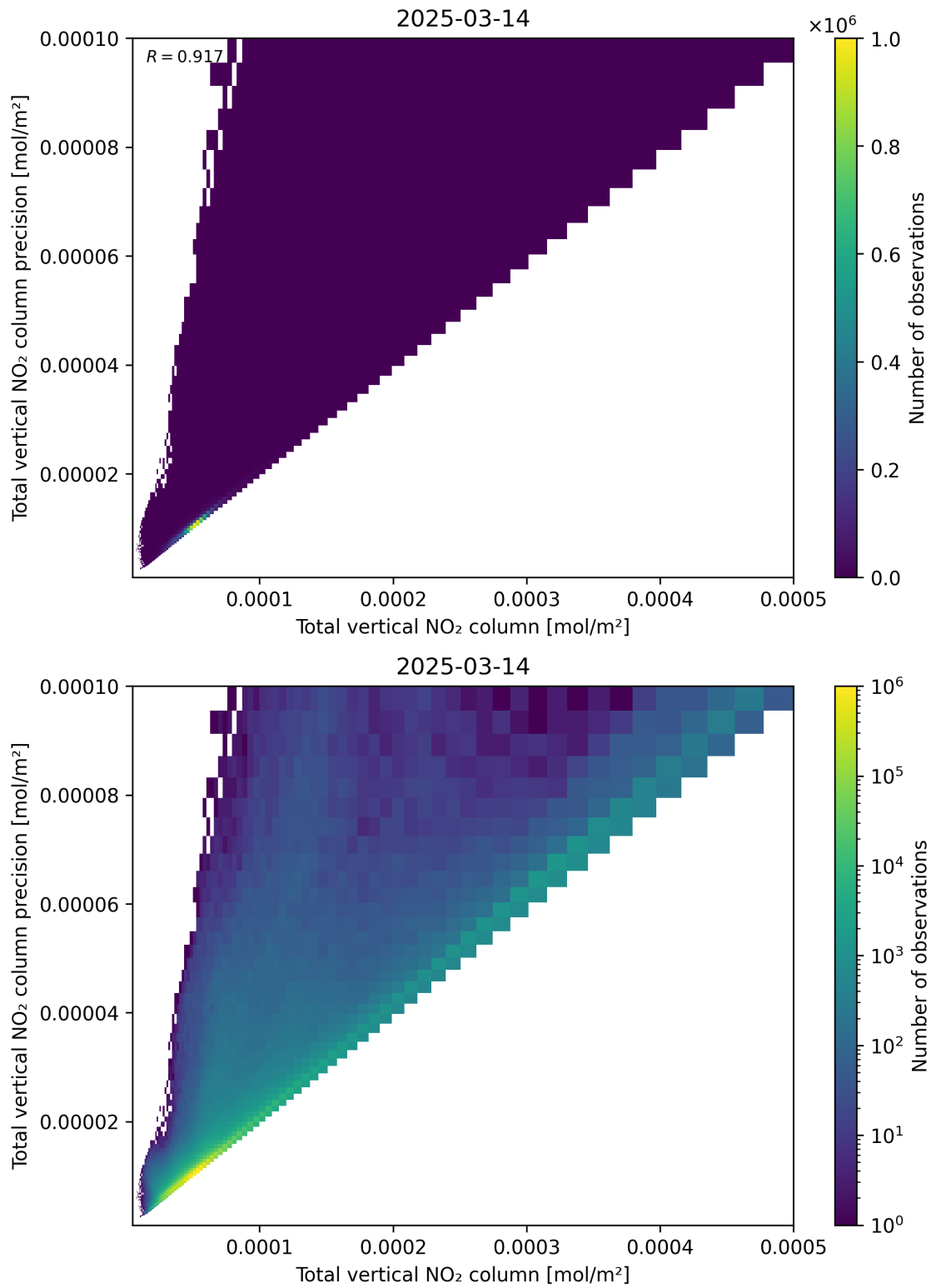
Figure 114: Scatter density plot of “Total vertical NO 2 column” against “Total vertical NO 2 column precision” for 2025-03-14 to 2025-03-15.
