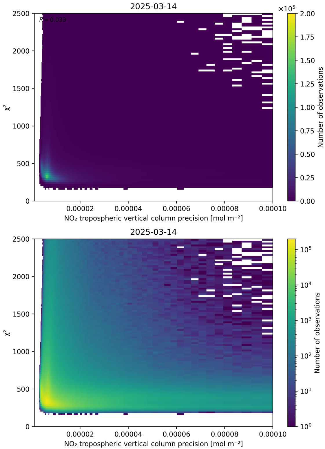
Figure 134: Scatter density plot of “NO 2 tropospheric vertical column precision” against “ \chi^2 ” for 2025-03-14 to 2025-03-15.
