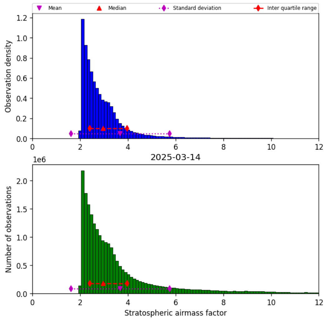
Figure 44: Histogram of “Stratospheric airmass factor” for 2025-03-14 to 2025-03-15
