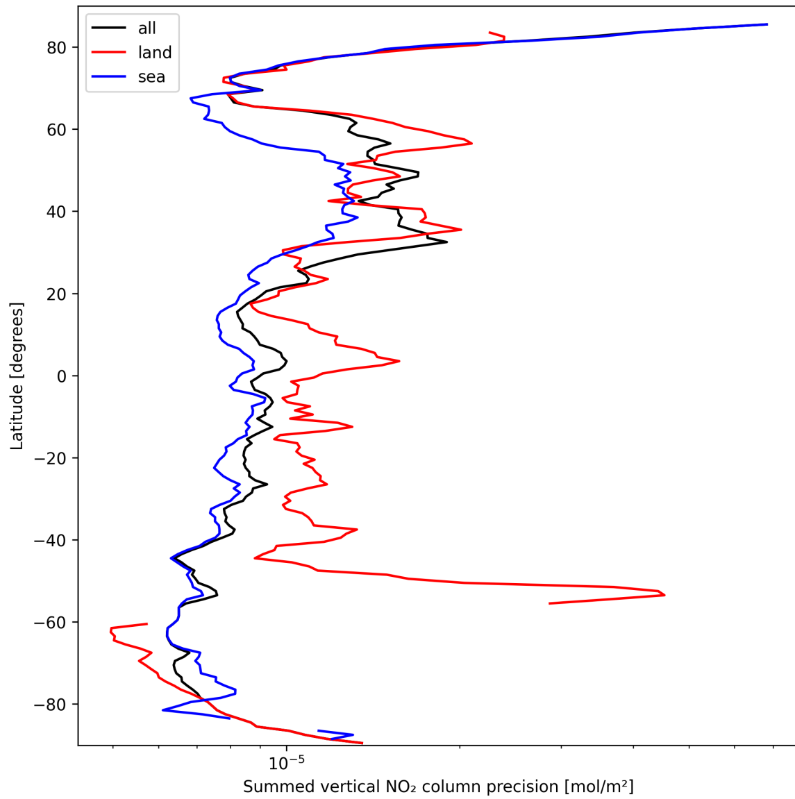
Figure 24: Zonal average of “Summed vertical NO 2 column precision” for 2025-03-14 to 2025-03-15.
