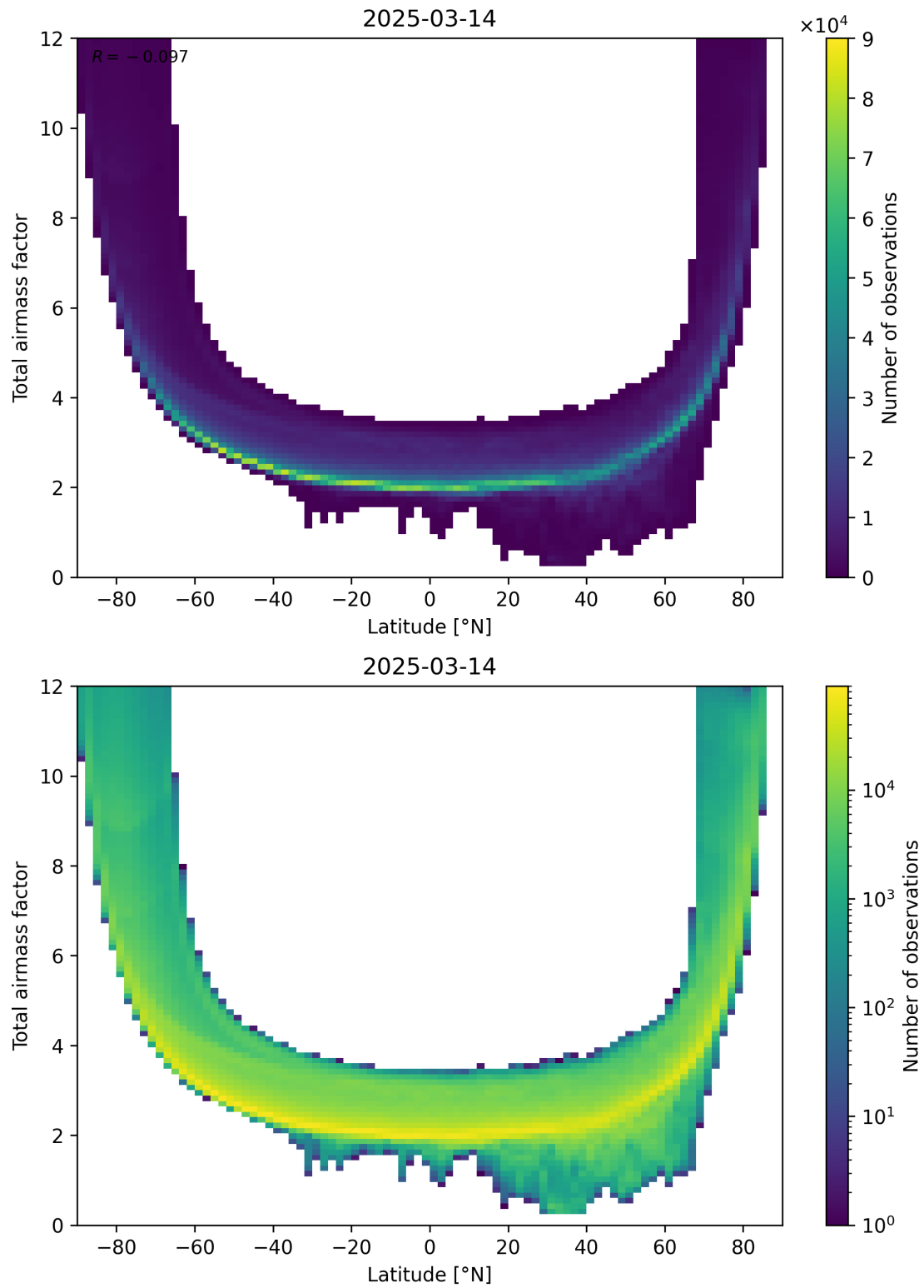
Figure 84: Scatter density plot of “Latitude” against “Total airmass factor” for 2025-03-14 to 2025-03-15.
