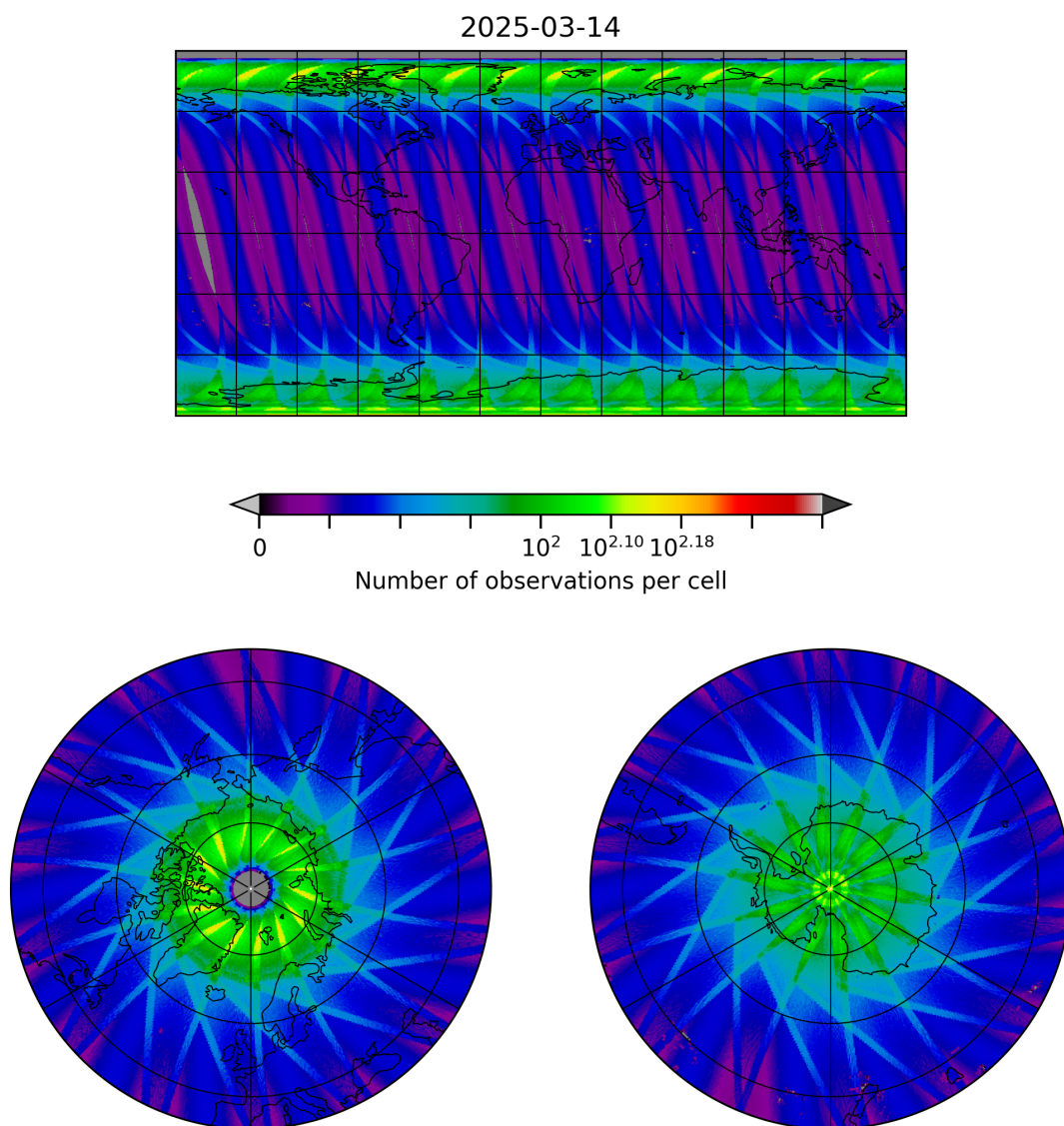
Figure 10: Map of the number of observations for 2025-03-14 to 2025-03-15
