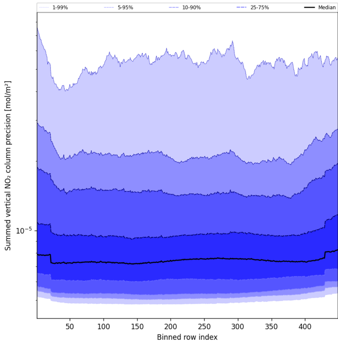
Figure 58: Along track statistics of “Summed vertical NO 2 column precision” for 2025-03-14 to 2025-03-15
