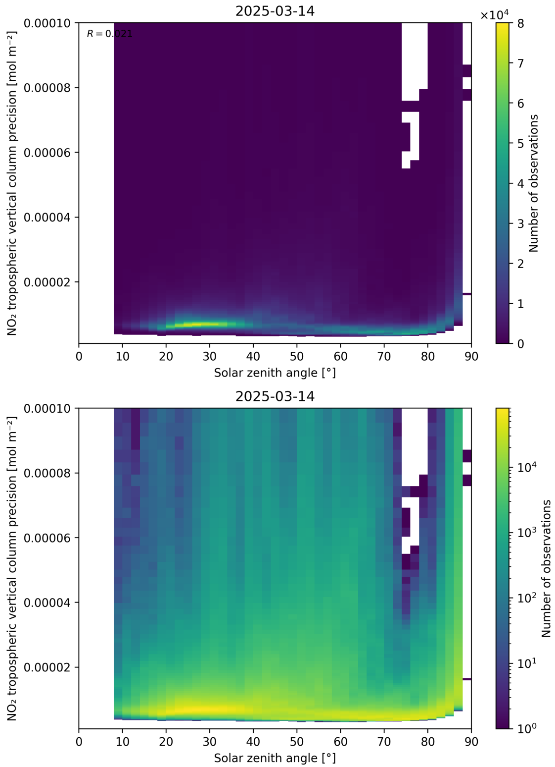
Figure 156: Scatter density plot of “Solar zenith angle” against “NO 2 tropospheric vertical column precision” for 2025-03-14 to 2025-03-15.
