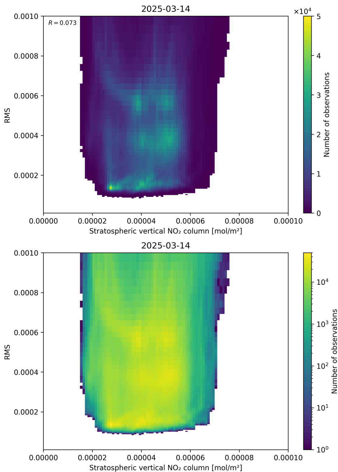
Figure 102: Scatter density plot of “Stratospheric vertical NO 2 column” against “RMS” for 2025-03-14 to 2025-03-15.
