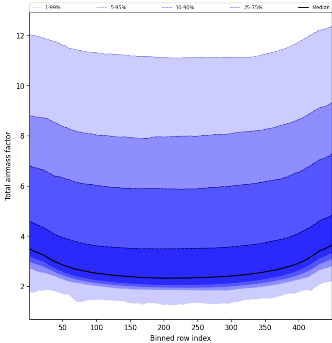
Figure 49: Along track statistics of “Total airmass factor” for 2025-03-14 to 2025-03-15
