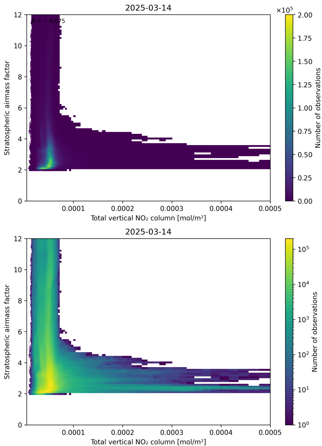
Figure 110: Scatter density plot of “Total vertical NO 2 column” against “Stratospheric airmass factor” for 2025-03-14 to 2025-03-15.
