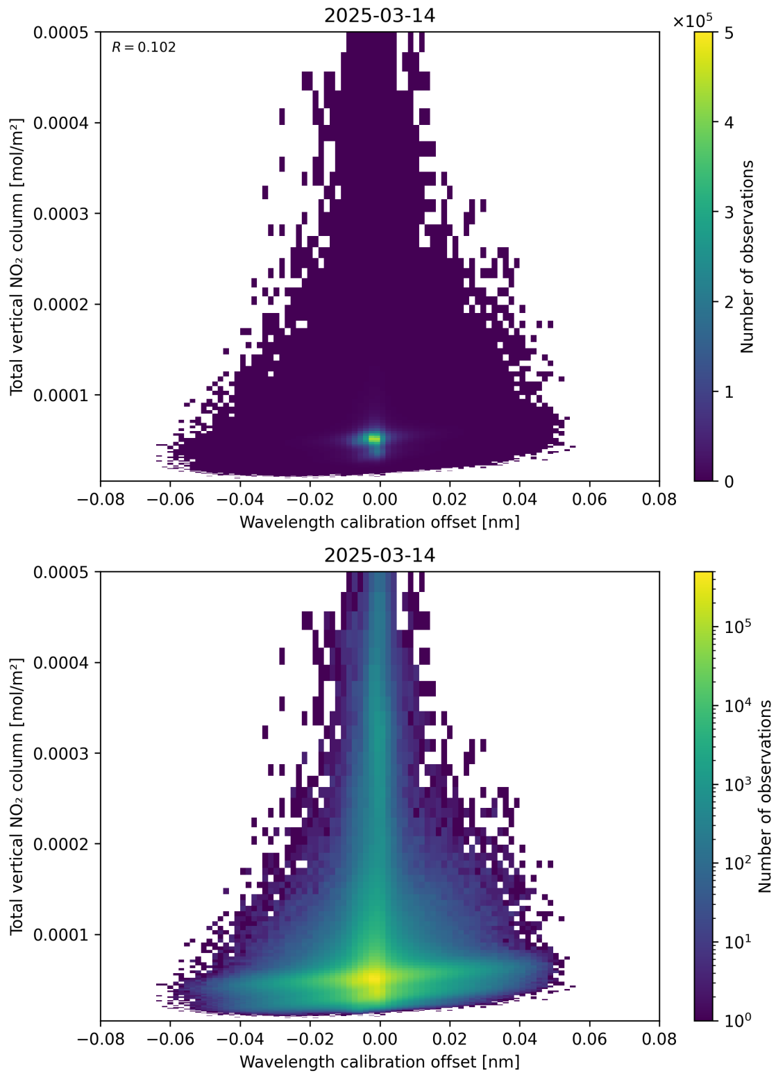
Figure 179: Scatter density plot of “Wavelength calibration offset” against “Total vertical NO 2 column” for 2025-03-14 to 2025-03-15.
