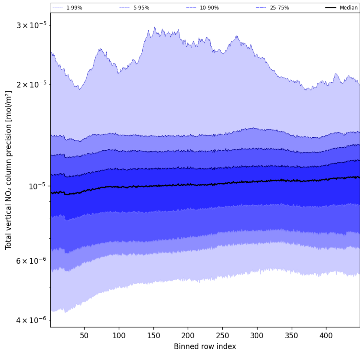
Figure 56: Along track statistics of “Total vertical NO 2 column precision” for 2025-03-14 to 2025-03-15
