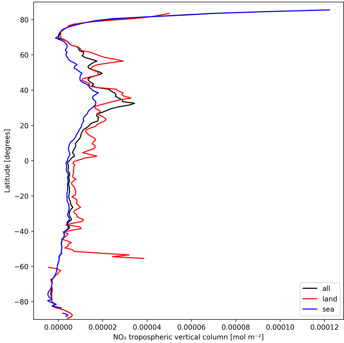
Figure 12: Zonal average of “NO 2 tropospheric vertical column” for 2025-03-14 to 2025-03-15.
