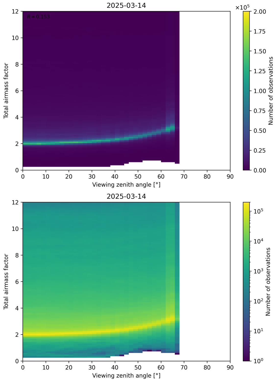
Figure 160: Scatter density plot of “Viewing zenith angle” against “Total airmass factor” for 2025-03-14 to 2025-03-15.
