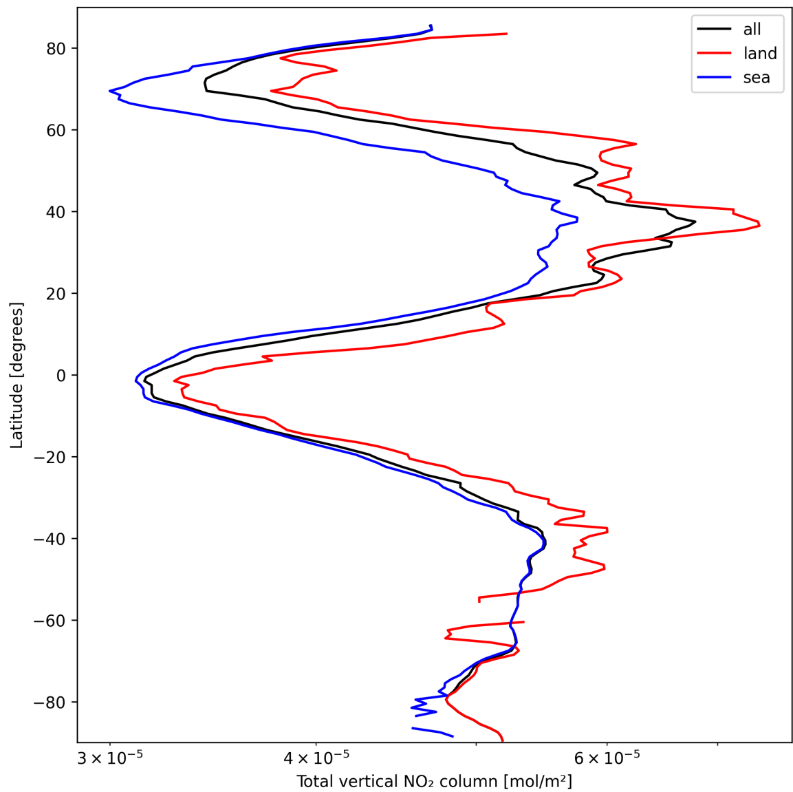
Figure 21: Zonal average of “Total vertical NO 2 column” for 2025-03-14 to 2025-03-15.
