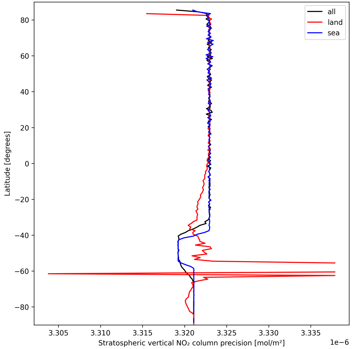
Figure 20: Zonal average of "Stratospheric vertical NO 2 column precision" for 2025-03-14 to 2025-03-15.
