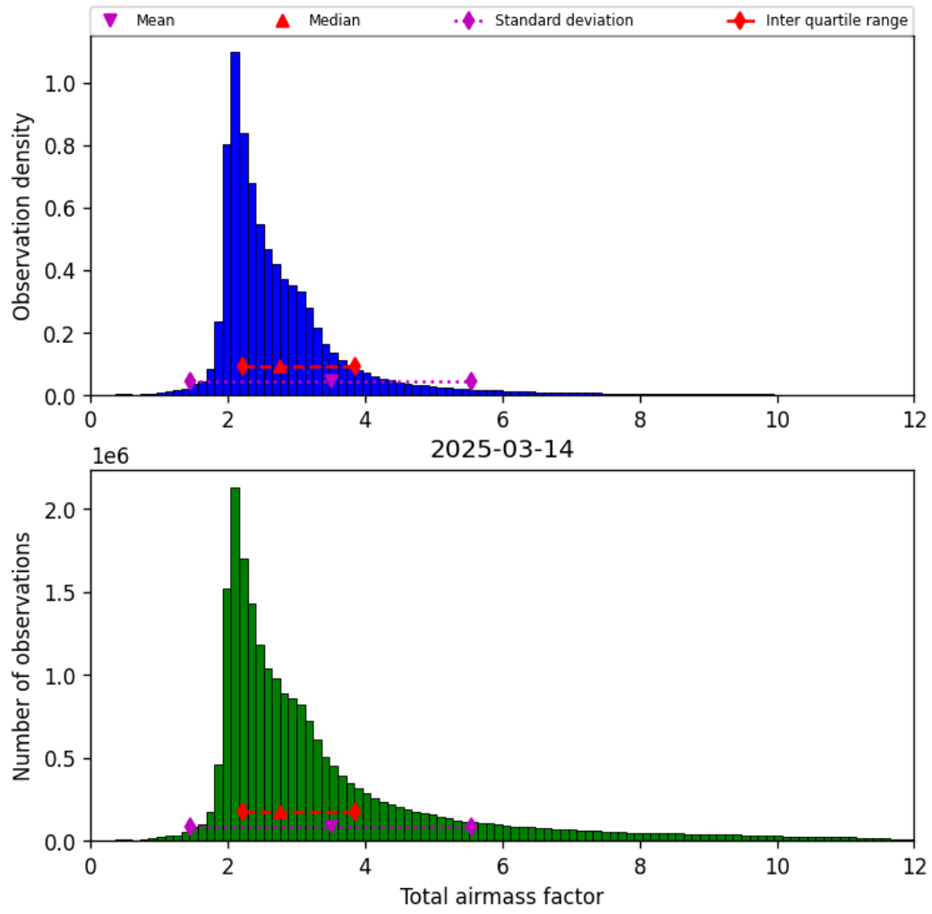
Figure 32: Histogram of “Total airmass factor” for 2025-03-14 to 2025-03-15
