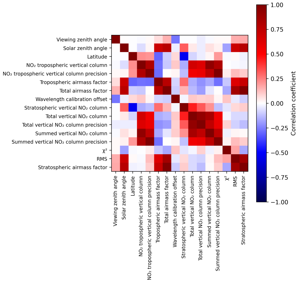
Figure 2: Map of correlation matrix for 2025-03-14 to 2025-03-15.
