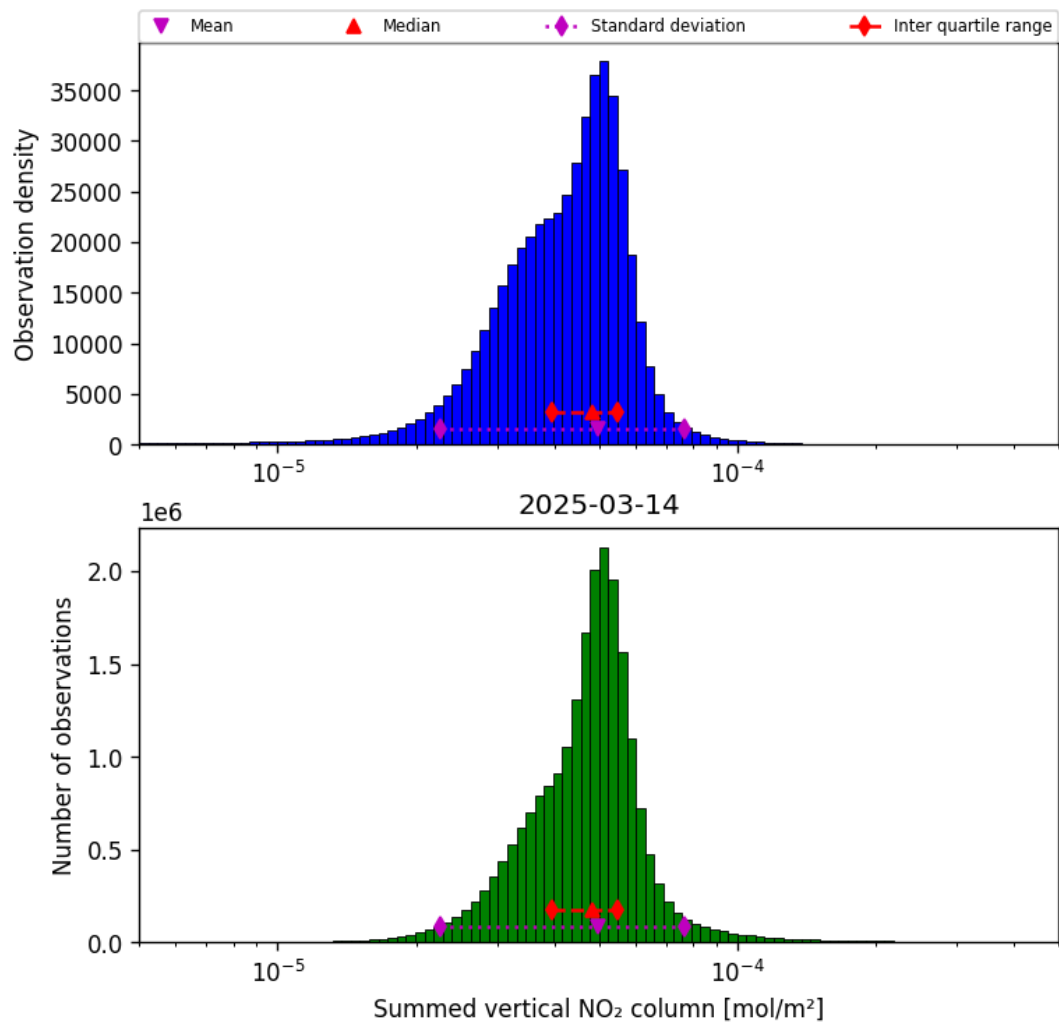
Figure 40: Histogram of “Summed vertical NO 2 column” for 2025-03-14 to 2025-03-15
