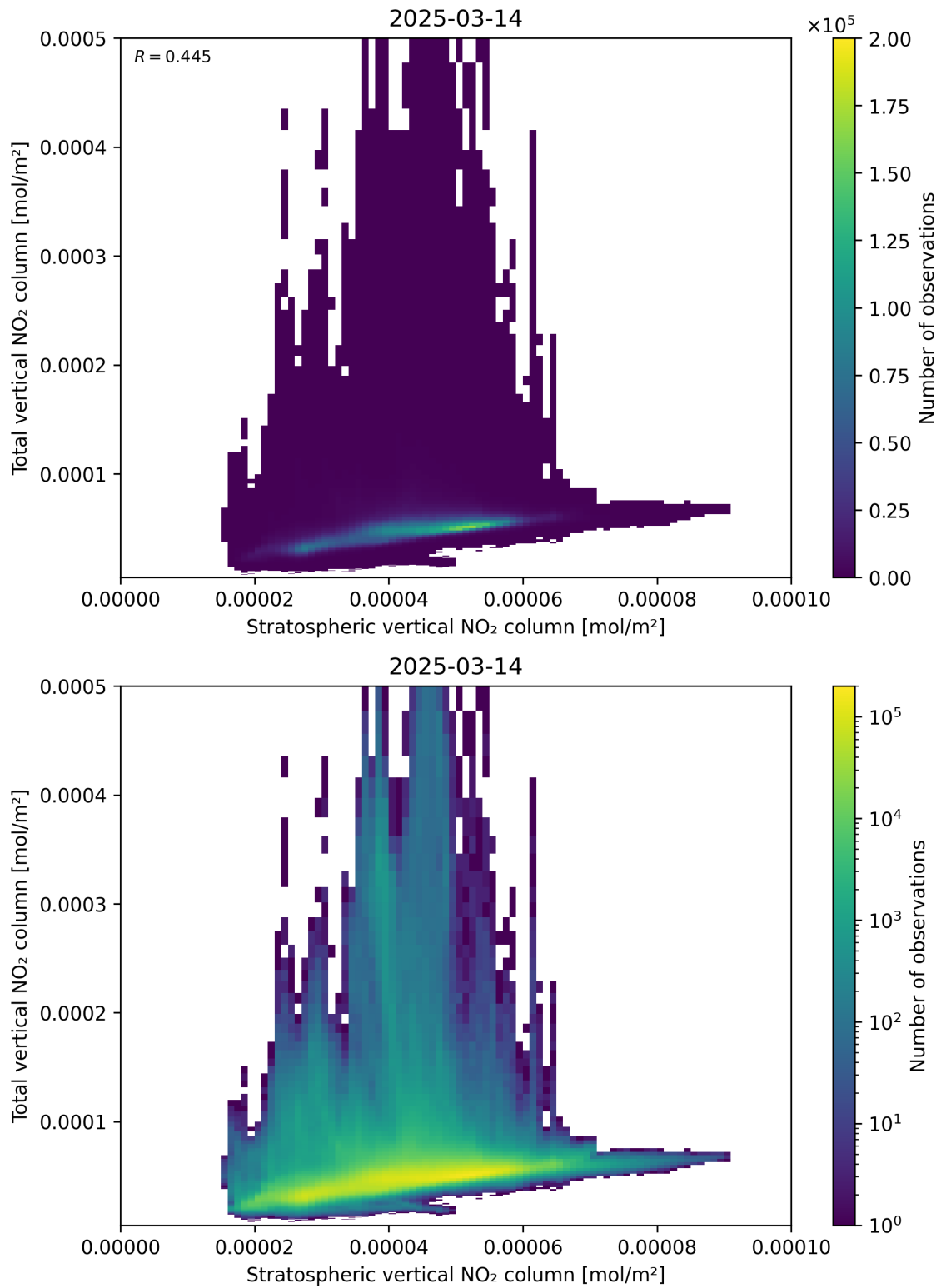
Figure 100: Scatter density plot of “Stratospheric vertical NO 2 column” against “Total vertical NO 2 column” for 2025-03-14 to 2025-03-15.
