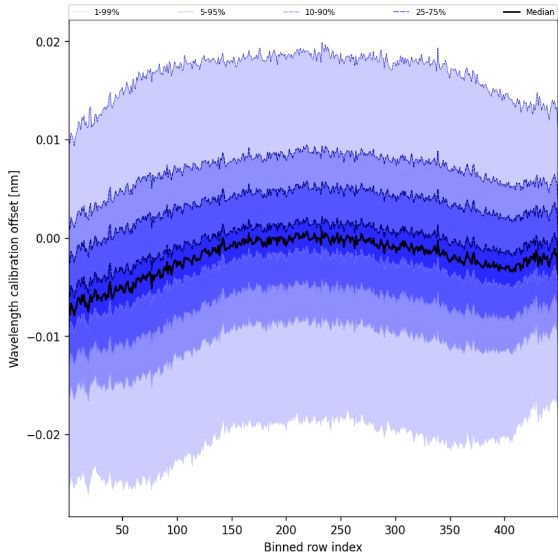
Figure 52: Along track statistics of “Wavelength calibration offset” for 2025-03-14 to 2025-03-15
