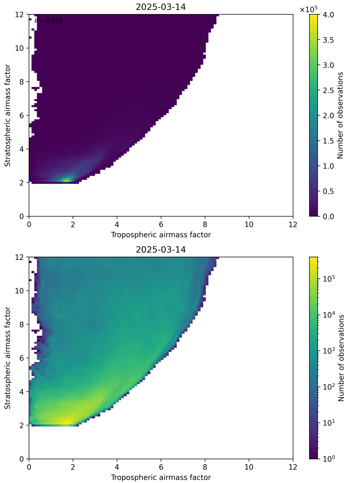
Figure 71: Scatter density plot of “Tropospheric airmass factor” against “Stratospheric airmass factor” for 2025-03-14 to 2025-03-15.
