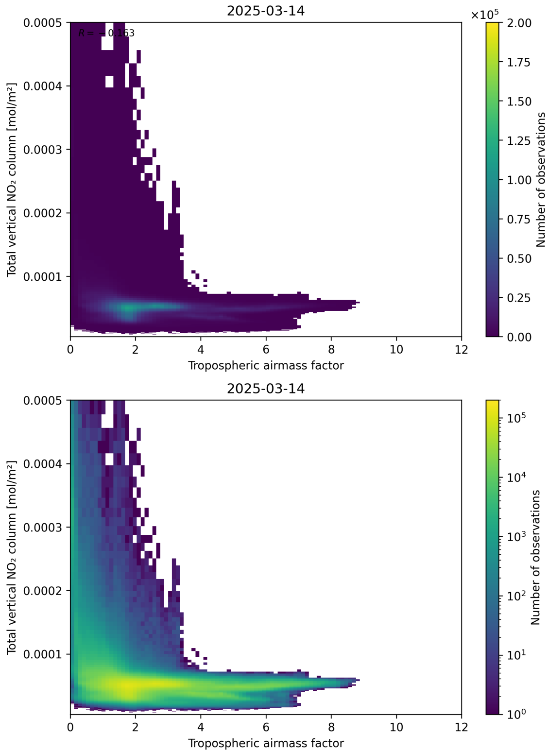
Figure 77: Scatter density plot of “Tropospheric airmass factor” against “Total vertical NO 2 column” for 2025-03-14 to 2025-03-15.
