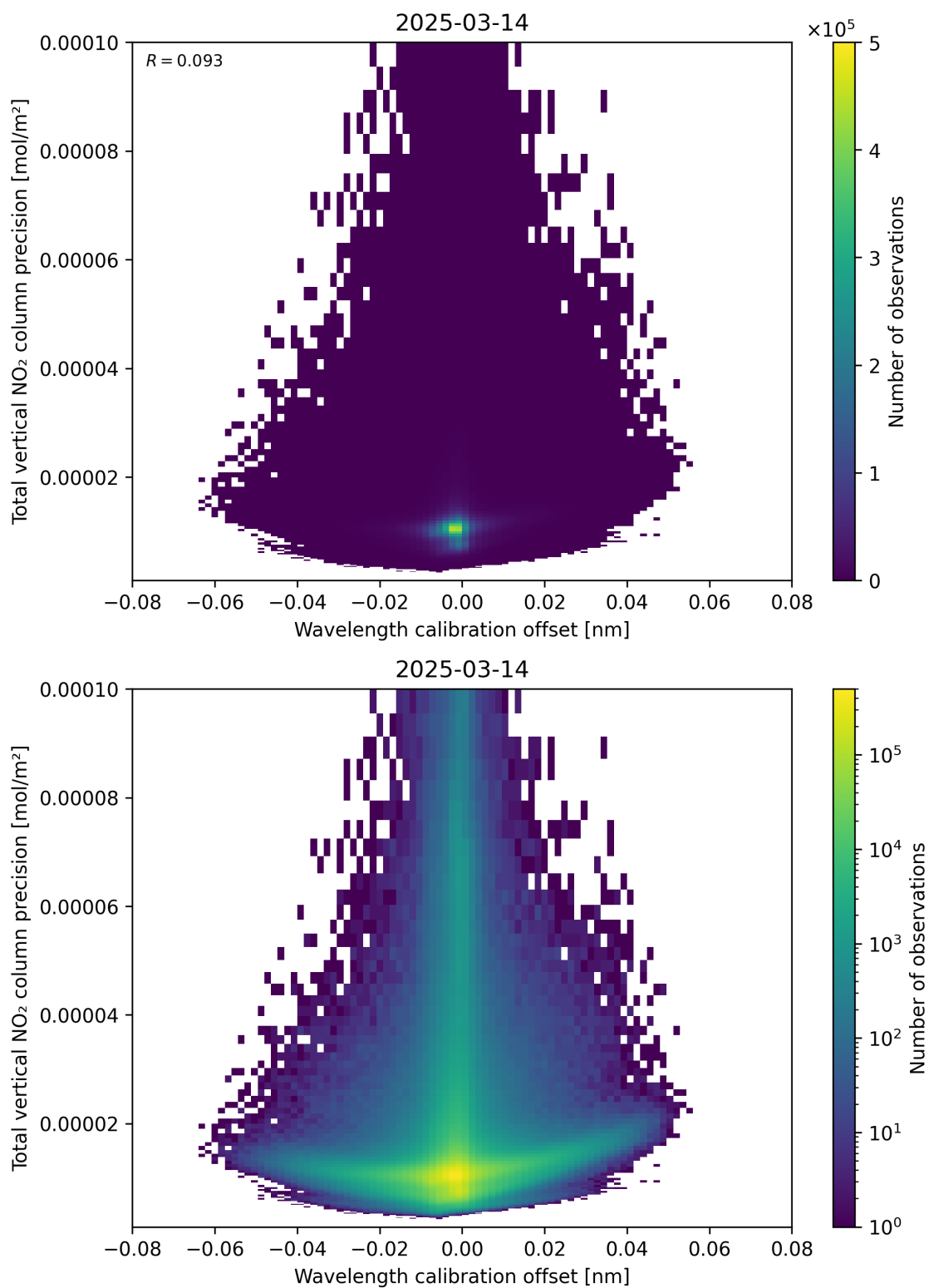
Figure 180: Scatter density plot of “Wavelength calibration offset” against “Total vertical NO 2 column precision” for 2025-03-14 to 2025-03-15.
