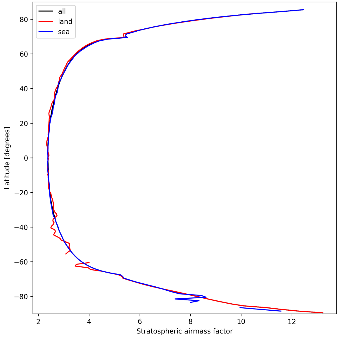
Figure 27: Zonal average of “Stratospheric airmass factor” for 2025-03-14 to 2025-03-15.
