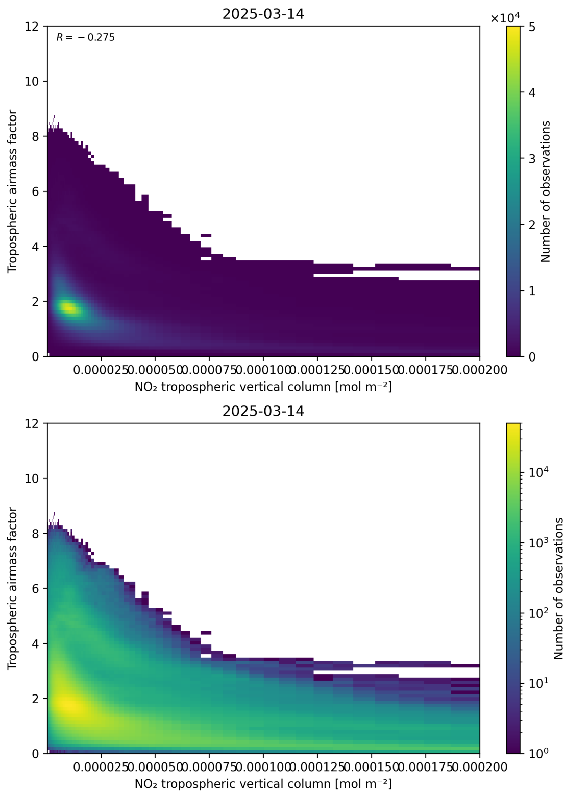
Figure 123: Scatter density plot of “NO 2 tropospheric vertical column” against “Tropospheric air mass factor” for 2025-03-14 to 2025-03-15.
