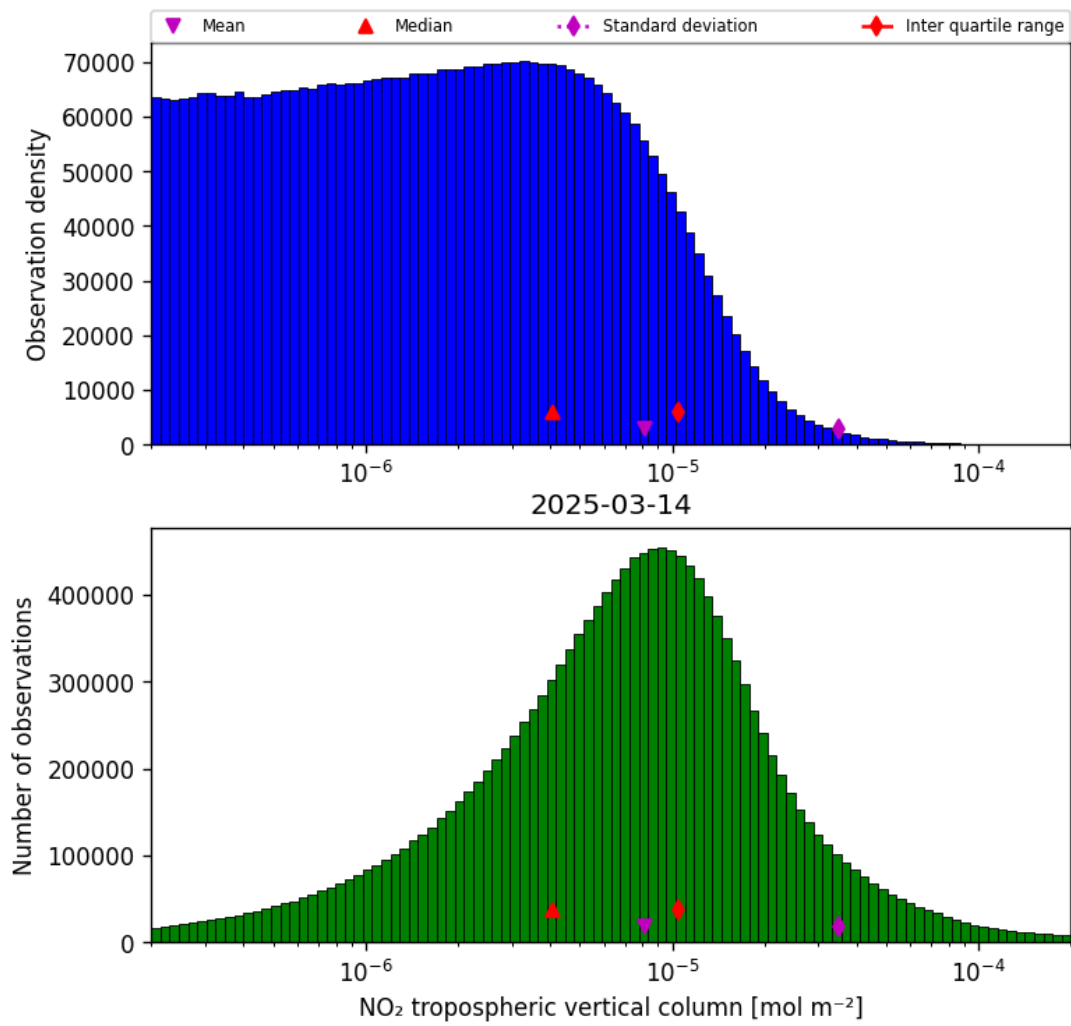
Figure 29: Histogram of “NO 2 tropospheric vertical column” for 2025-03-14 to 2025-03-15
