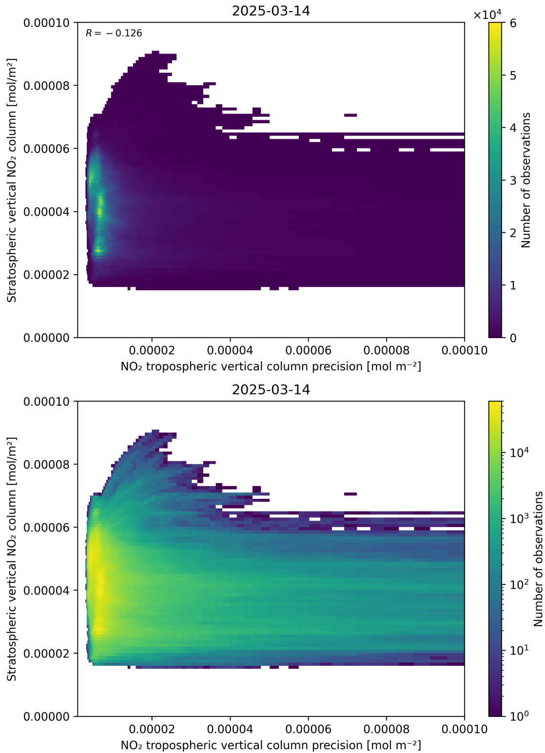
Figure 135: Scatter density plot of “NO 2 tropospheric vertical column precision” against “Stratospheric vertical NO 2 column” for 2025-03-14 to 2025-03-15.
