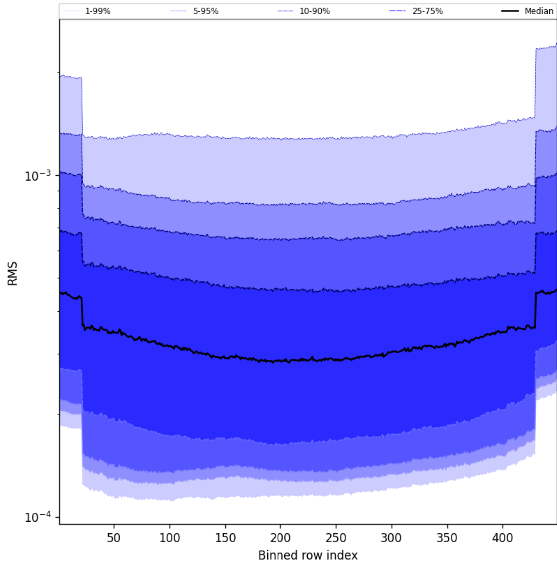
Figure 60: Along track statistics of “RMS” for 2025-03-14 to 2025-03-15
