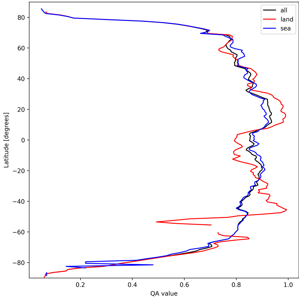
Figure 11: Zonal average of “QA value” for 2025-03-14 to 2025-03-15.
