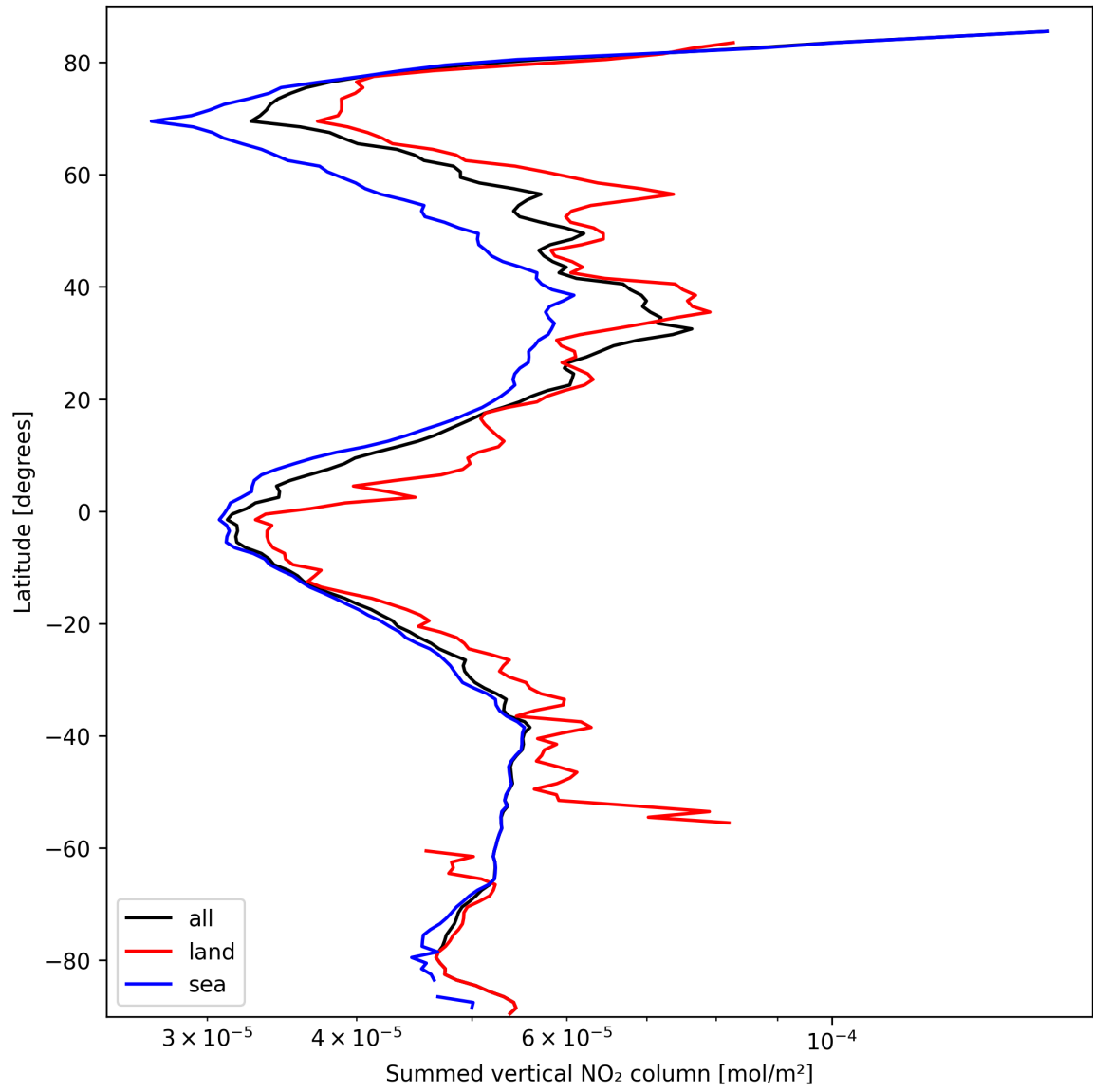
Figure 23: Zonal average of “Summed vertical NO 2 column” for 2025-03-14 to 2025-03-15.
