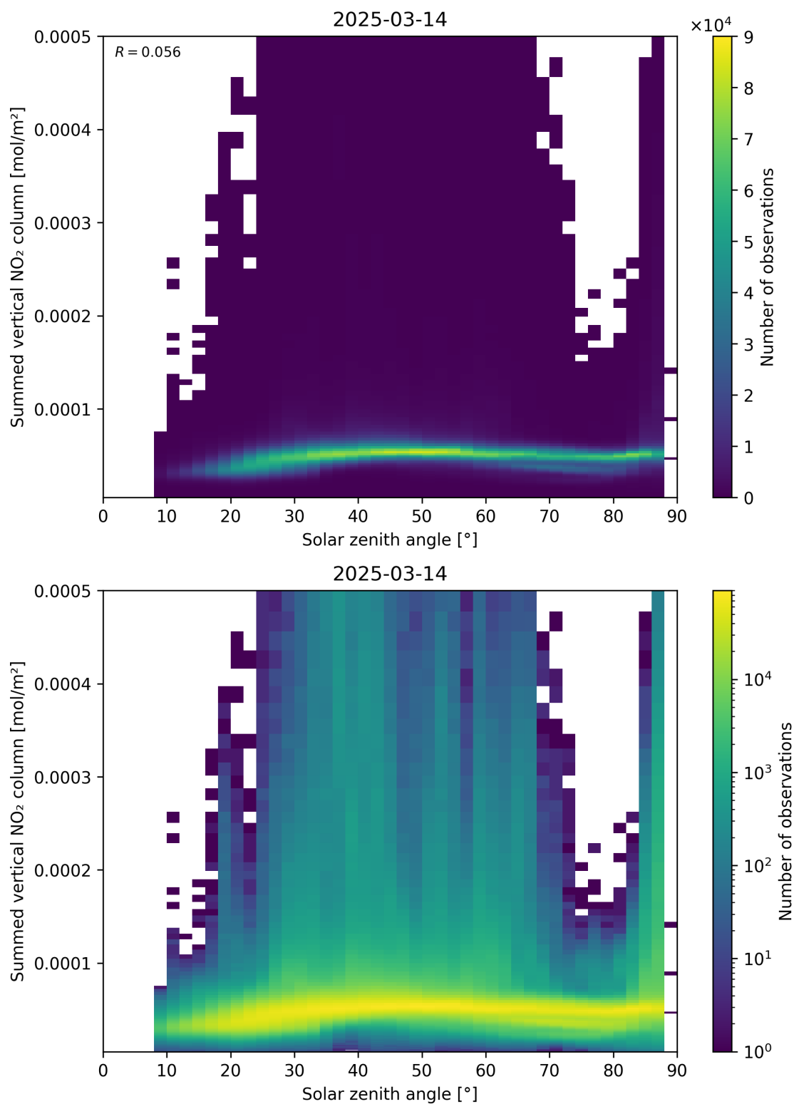
Figure 151: Scatter density plot of “Solar zenith angle” against “Summed vertical NO 2 column” for 2025-03-14 to 2025-03-15.
