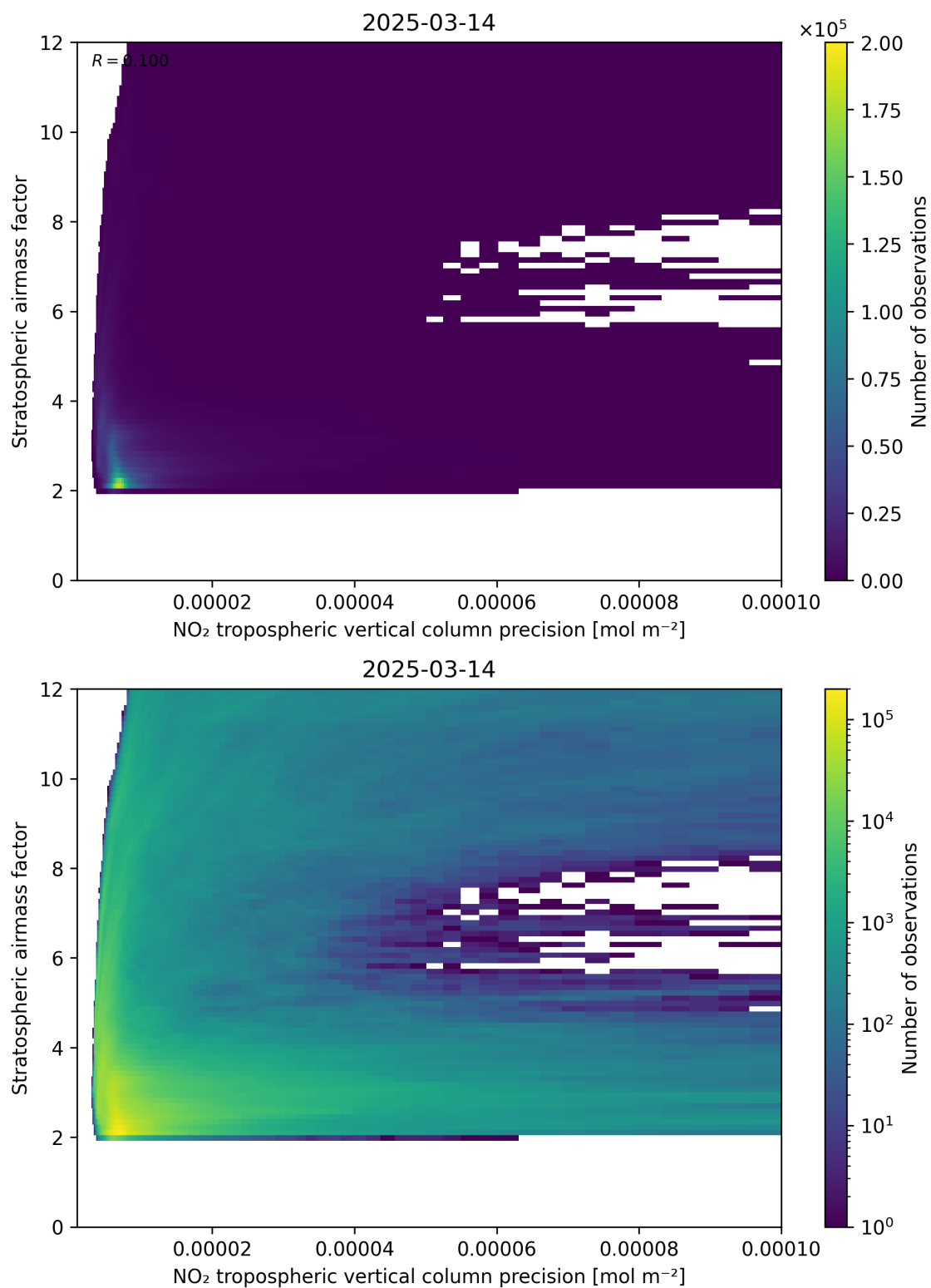
Figure 131: Scatter density plot of “NO 2 tropospheric vertical column precision” against “Stratospheric airmass factor” for 2025-03-14 to 2025-03-15.
