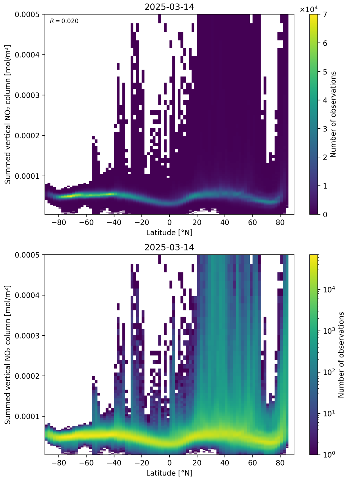
Figure 88: Scatter density plot of “Latitude” against “Summed vertical NO 2 column” for 2025-03-14 to 2025-03-15.
