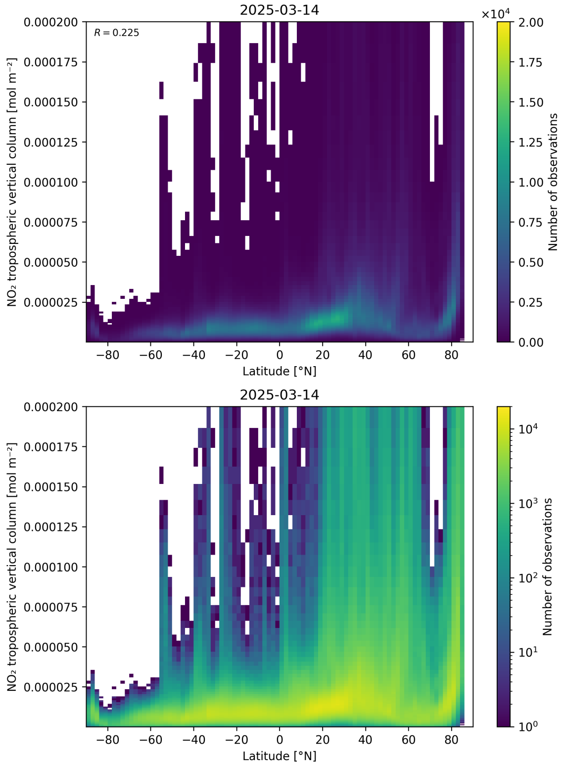
Figure 92: Scatter density plot of “Latitude” against “NO 2 tropospheric vertical column” for 2025-03-14 to 2025-03-15.
