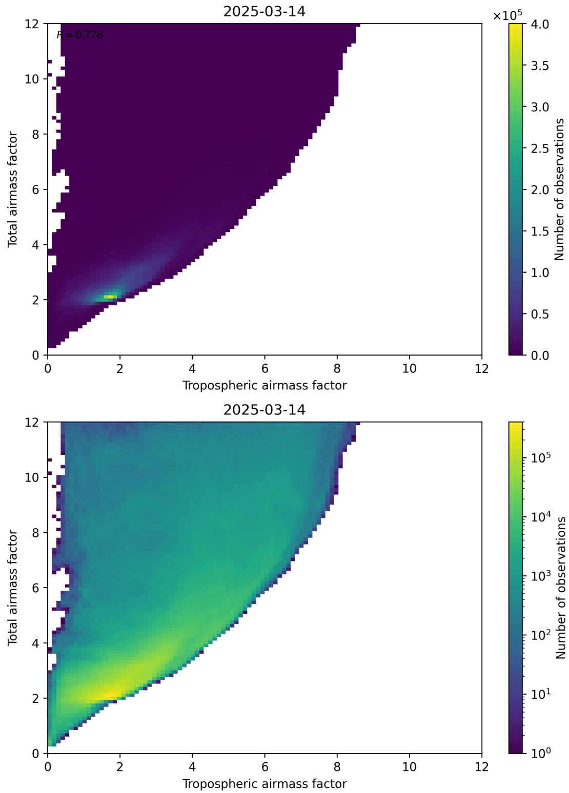
Figure 72: Scatter density plot of “Tropospheric airmass factor” against “Total airmass factor” for 2025-03-14 to 2025-03-15.
