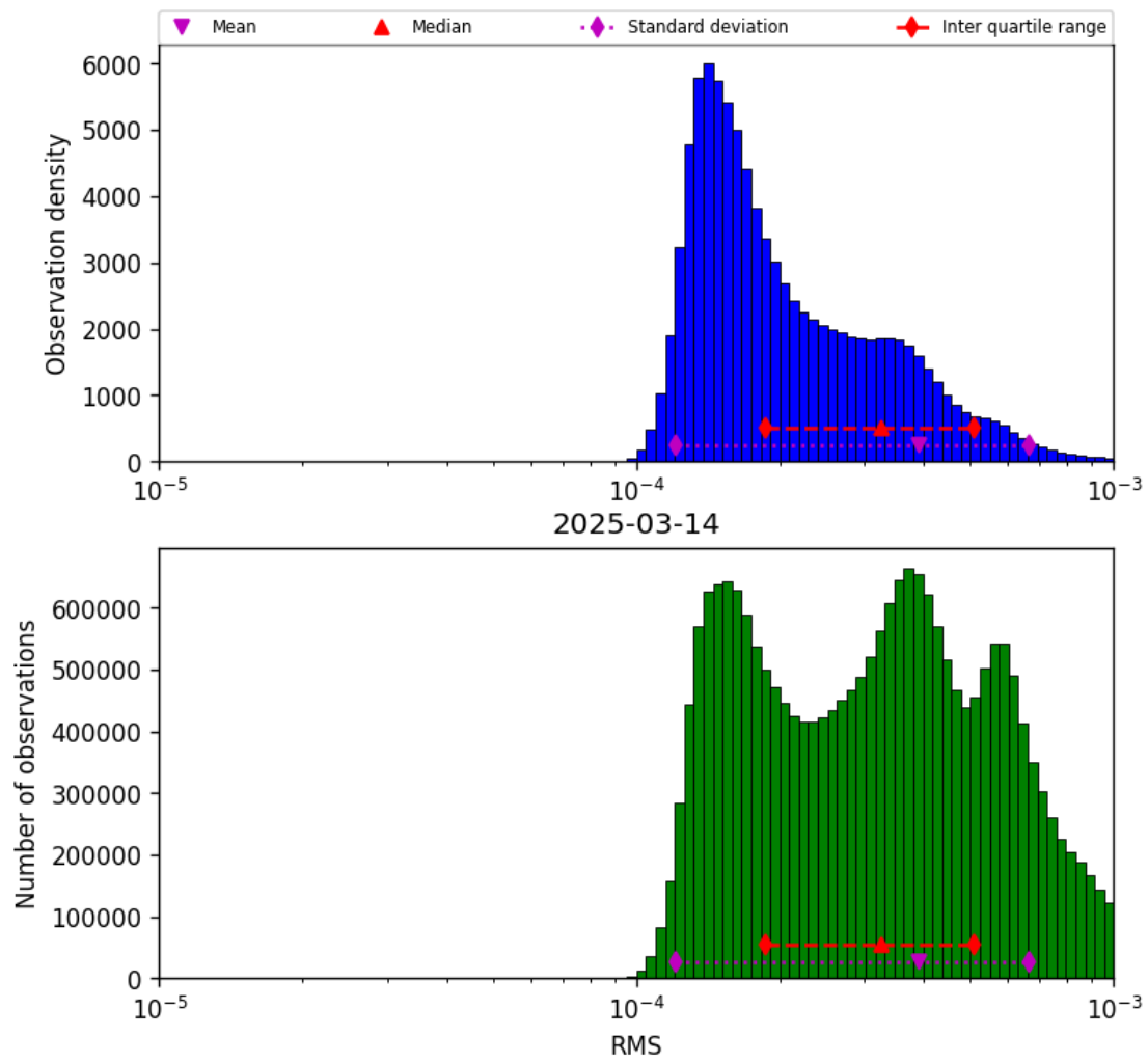
Figure 43: Histogram of “RMS” for 2025-03-14 to 2025-03-15
