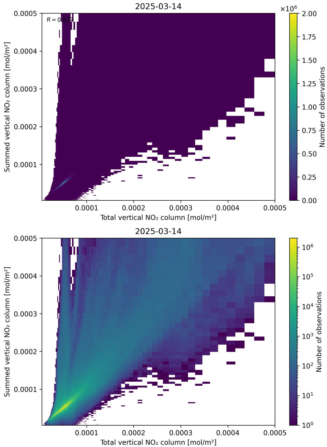
Figure 112: Scatter density plot of “Total vertical NO 2 column” against “Summed vertical NO 2 column” for 2025-03-14 to 2025-03-15.
