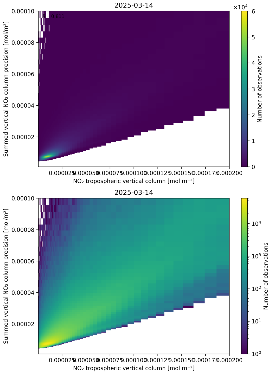
Figure 127: Scatter density plot of “NO 2 tropospheric vertical column” against “Summed vertical NO 2 column precision” for 2025-03-14 to 2025-03-15.
