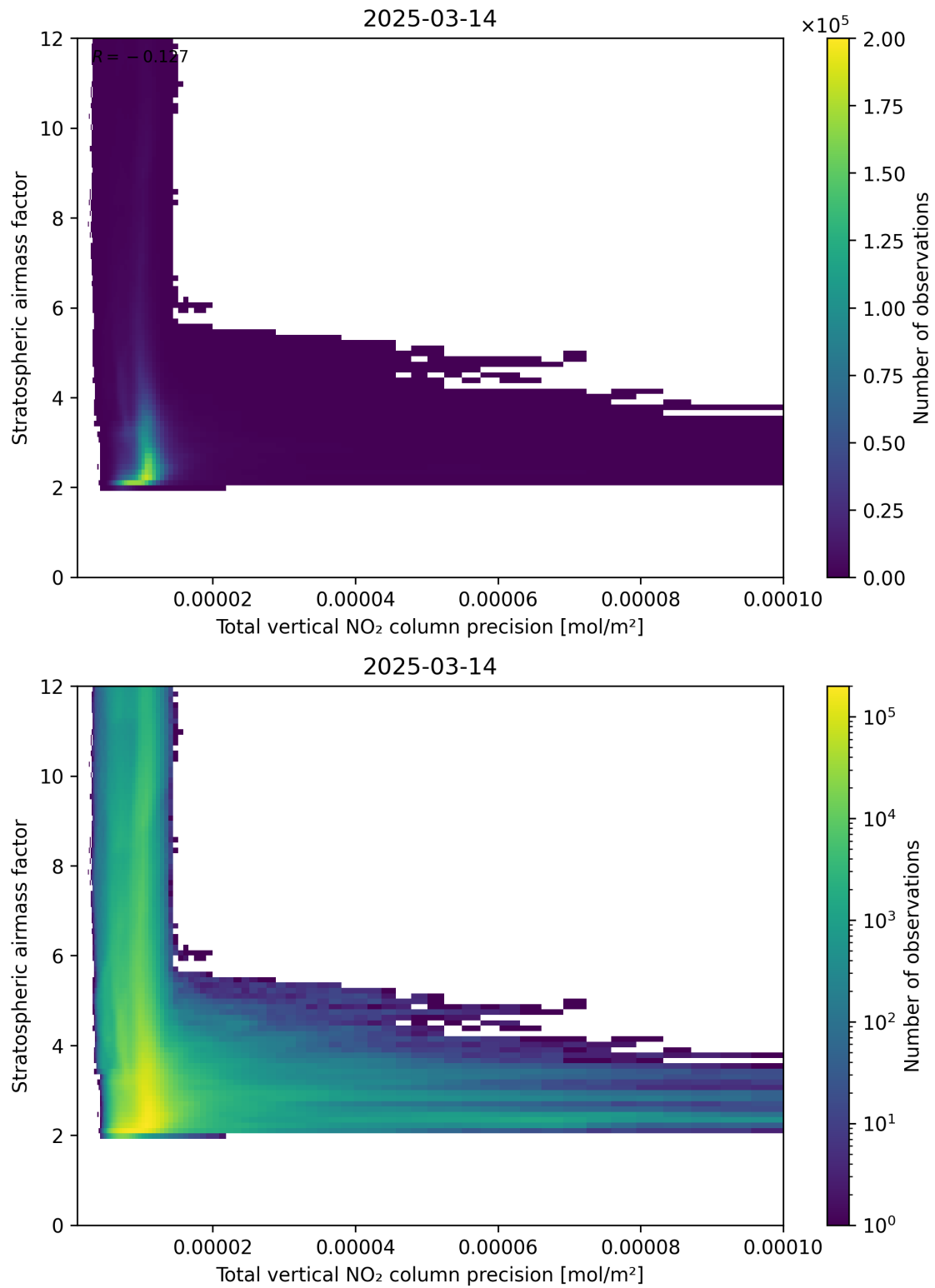
Figure 115: Scatter density plot of “Total vertical NO 2 column precision” against “Stratospheric air mass factor” for 2025-03-14 to 2025-03-15.
