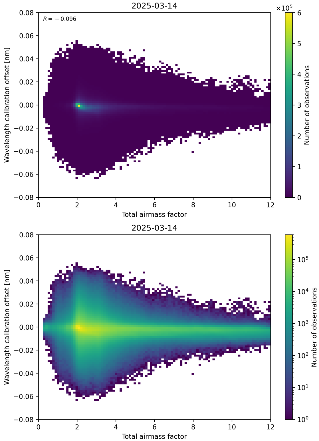
Figure 70: Scatter density plot of “Total airmass factor” against “Wavelength calibration offset” for 2025-03-14 to 2025-03-15.
