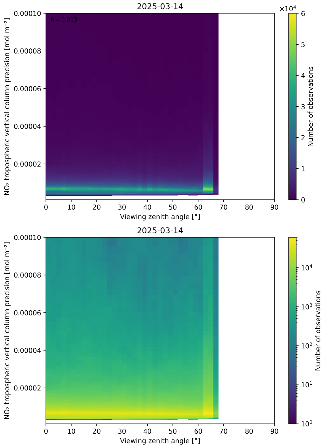
Figure 170: Scatter density plot of “Viewing zenith angle” against “NO 2 tropospheric vertical column precision” for 2025-03-14 to 2025-03-15.
