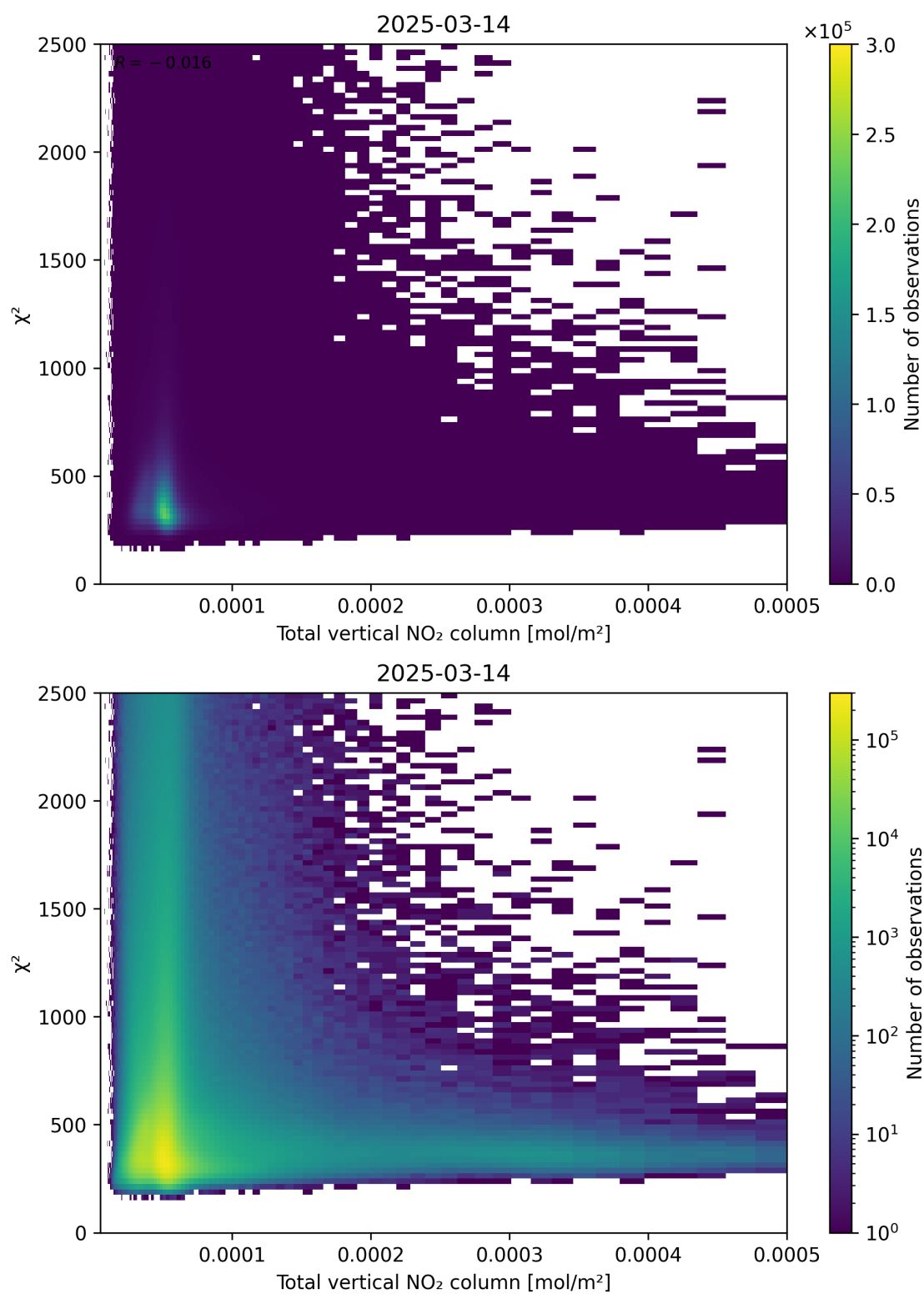
Figure 111: Scatter density plot of “Total vertical NO 2 column” against “ \chi^2 ” for 2025-03-14 to 2025-03-15.
