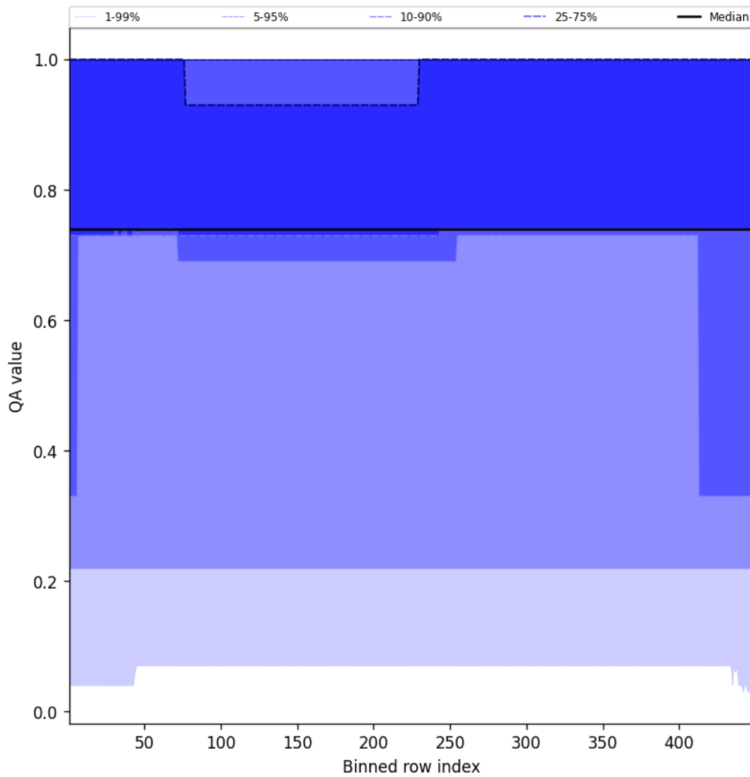
Figure 45: Along track statistics of “QA value” for 2025-03-14 to 2025-03-15
