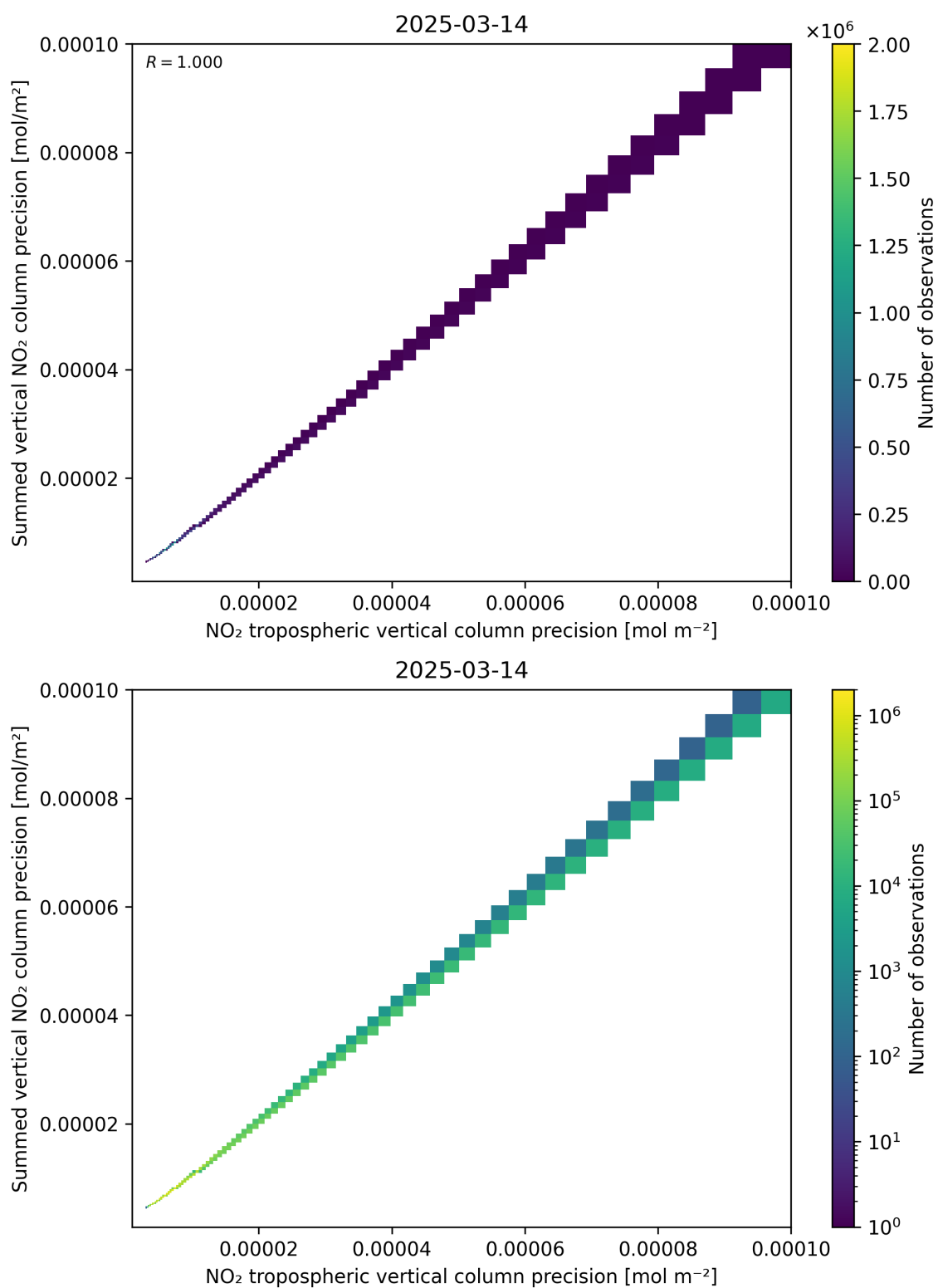
Figure 137: Scatter density plot of “NO 2 tropospheric vertical column precision” against “Summed vertical NO 2 column precision” for 2025-03-14 to 2025-03-15.
