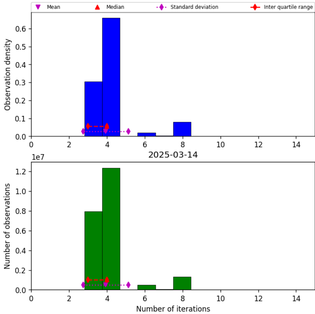
Figure 34: Histogram of “Number of iterations” for 2025-03-14 to 2025-03-15
