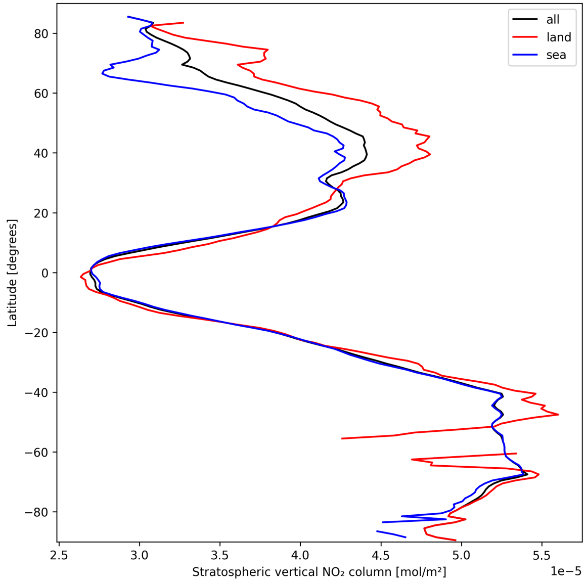
Figure 19: Zonal average of “Stratospheric vertical NO 2 column” for 2025-03-14 to 2025-03-15.
