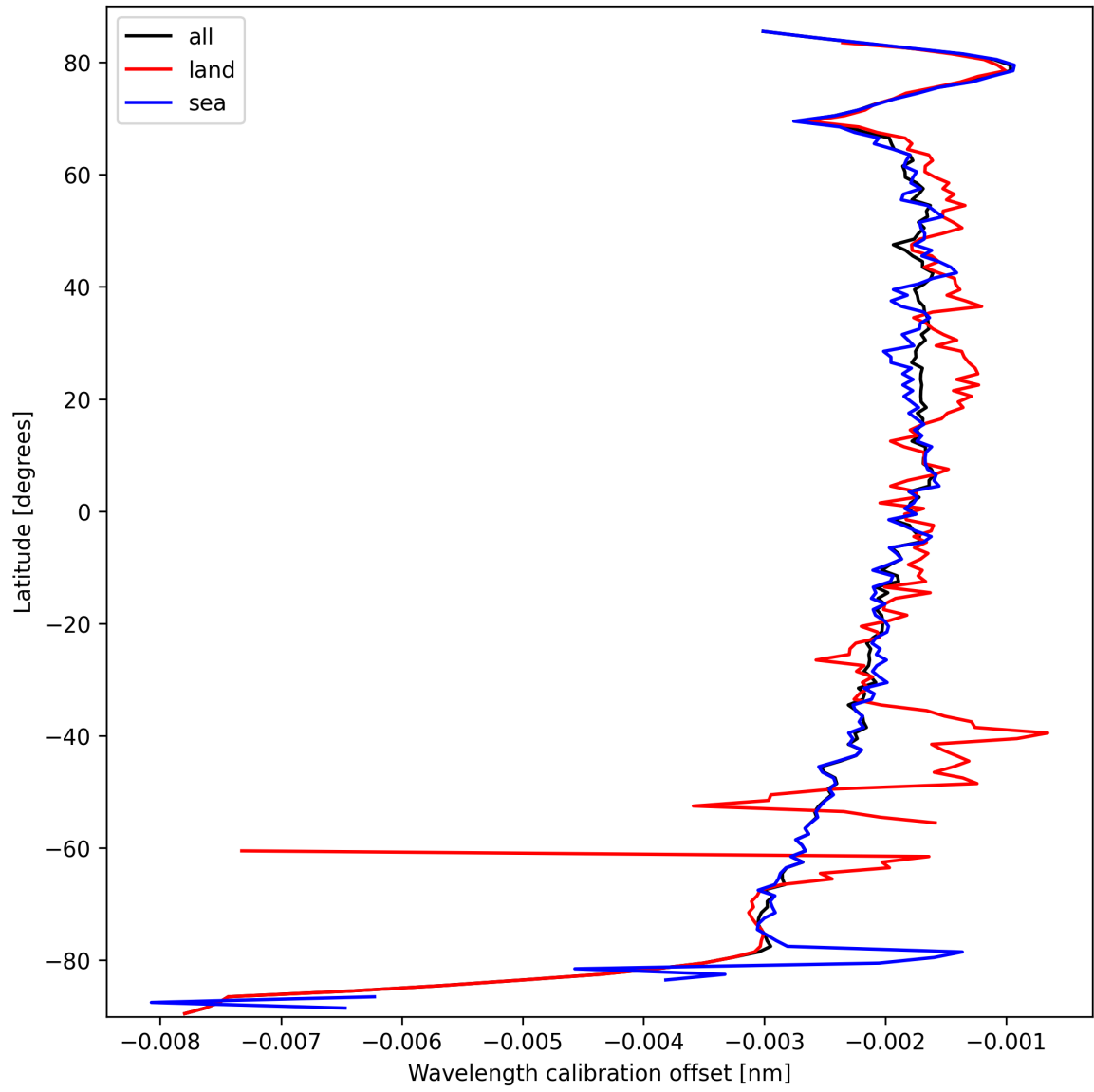
Figure 18: Zonal average of “Wavelength calibration offset” for 2025-03-14 to 2025-03-15.
