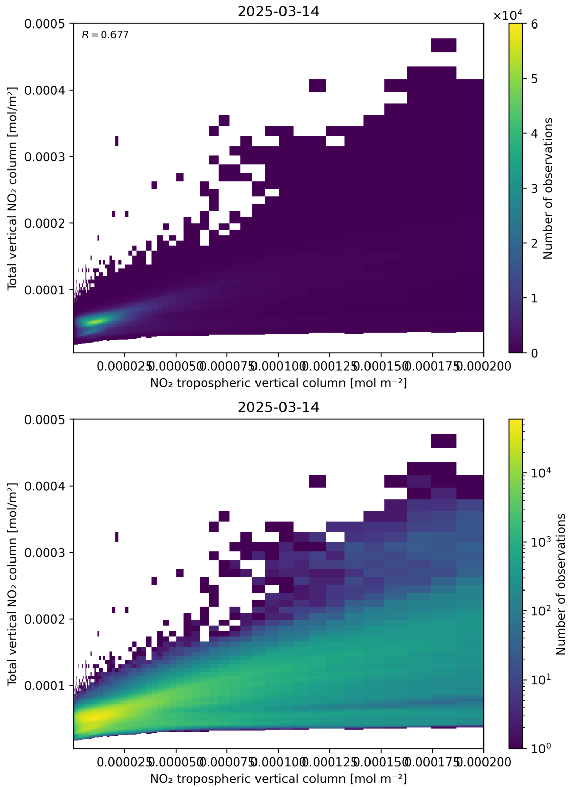
Figure 128: Scatter density plot of “NO 2 tropospheric vertical column” against “Total vertical NO 2 column” for 2025-03-14 to 2025-03-15.
