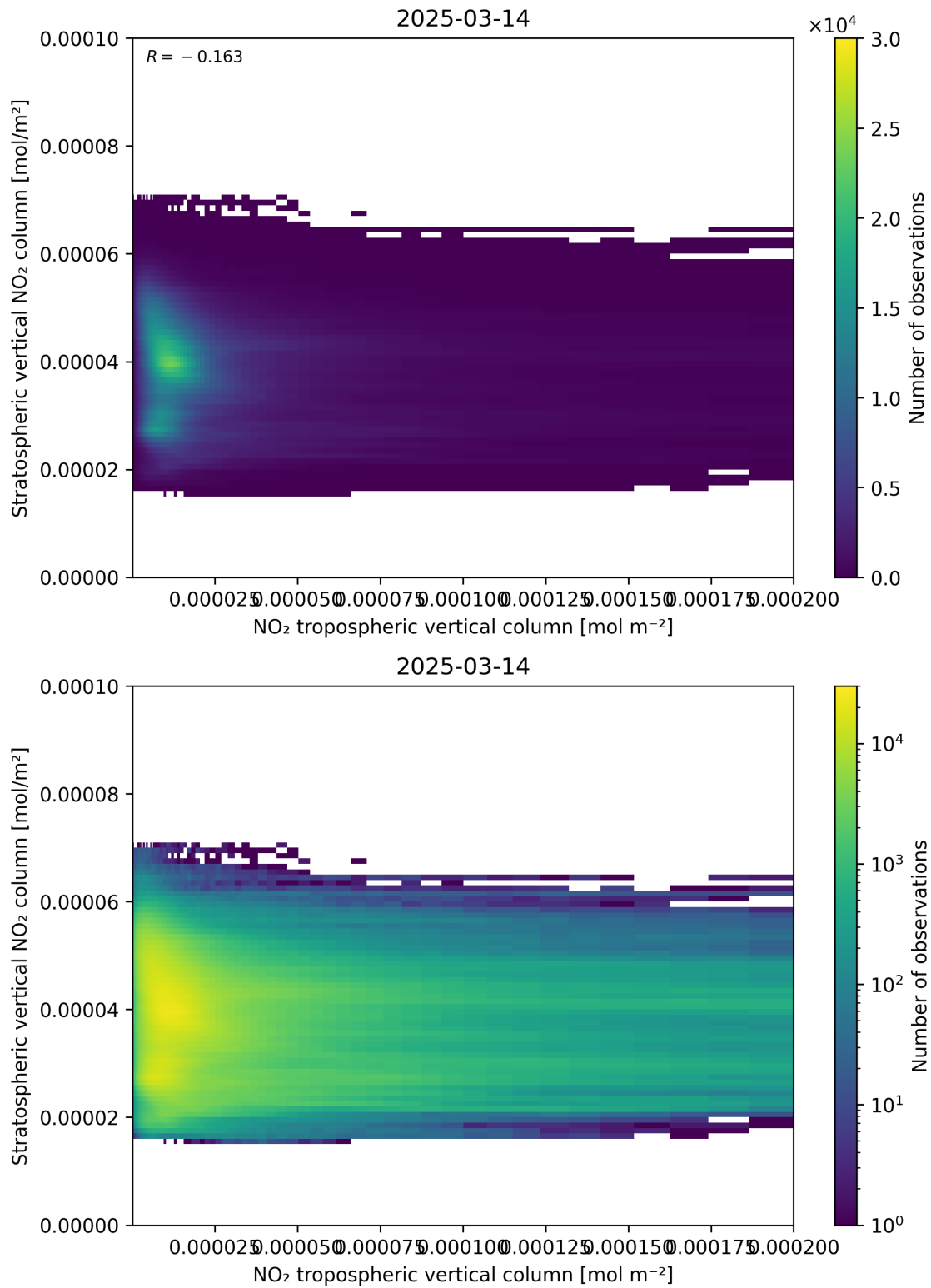
Figure 125: Scatter density plot of “NO 2 tropospheric vertical column” against “Stratospheric vertical NO 2 column” for 2025-03-14 to 2025-03-15.
