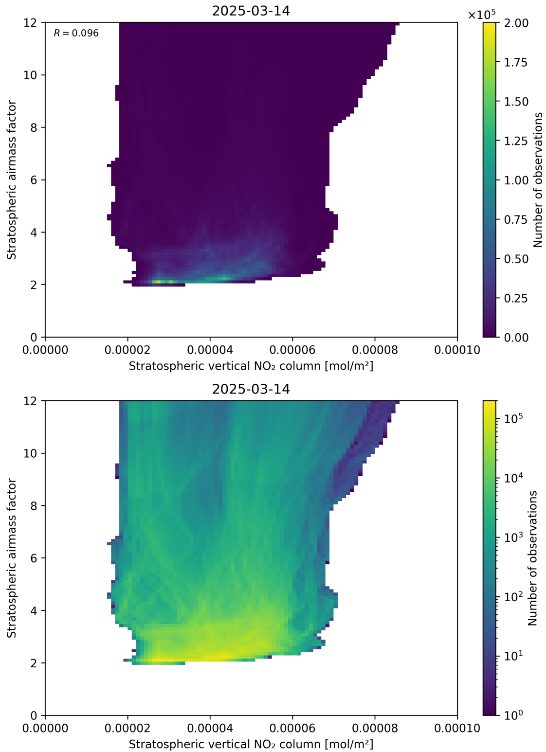
Figure 96: Scatter density plot of “Stratospheric vertical NO 2 column” against “Stratospheric airmass factor” for 2025-03-14 to 2025-03-15.
