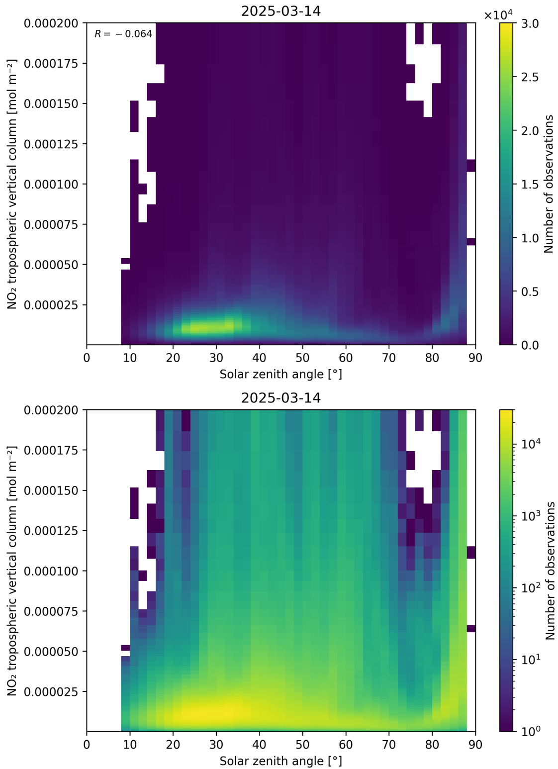
Figure 155: Scatter density plot of “Solar zenith angle” against “NO 2 tropospheric vertical column” for 2025-03-14 to 2025-03-15.
