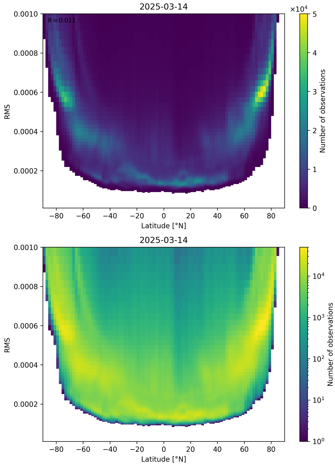
Figure 94: Scatter density plot of “Latitude” against “RMS” for 2025-03-14 to 2025-03-15.
