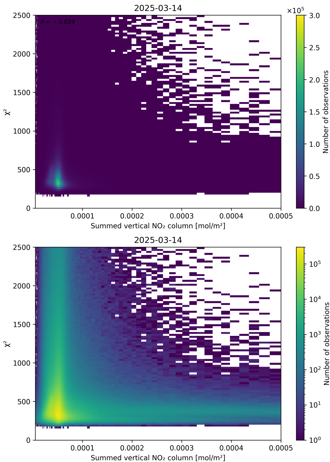
Figure 104: Scatter density plot of “Summed vertical NO 2 column” against “ \chi^2 ” for 2025-03-14 to 2025-03-15.
