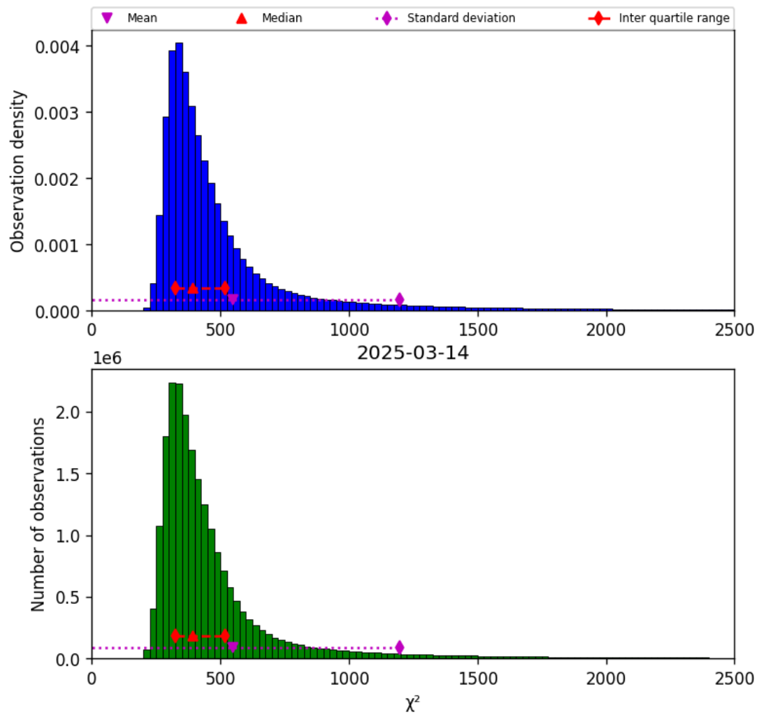
Figure 42: Histogram of “ \chi^2 ” for 2025-03-14 to 2025-03-15
