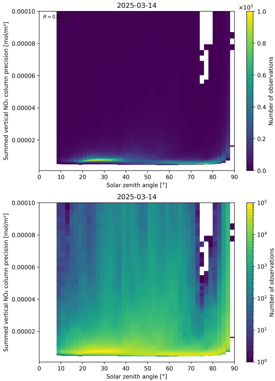
Figure 152: Scatter density plot of “Solar zenith angle” against “Summed vertical NO 2 column precision” for 2025-03-14 to 2025-03-15.
