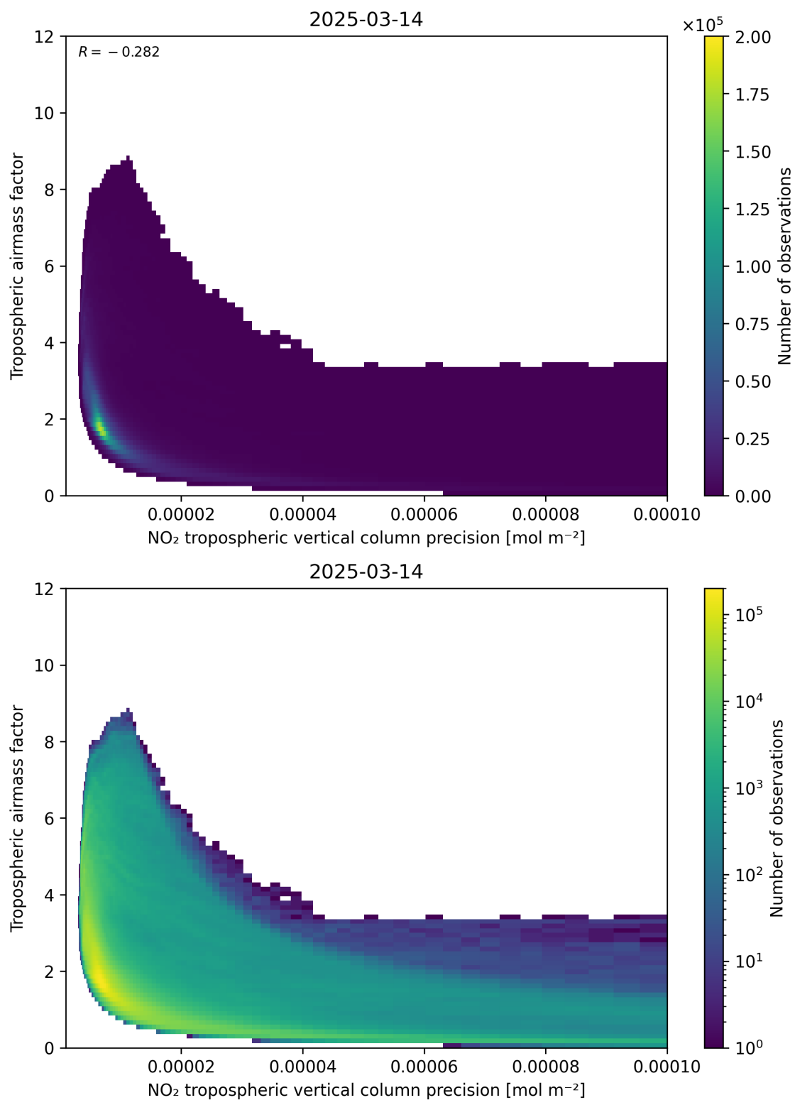
Figure 133: Scatter density plot of “NO 2 tropospheric vertical column precision” against “Tropospheric air mass factor” for 2025-03-14 to 2025-03-15.
