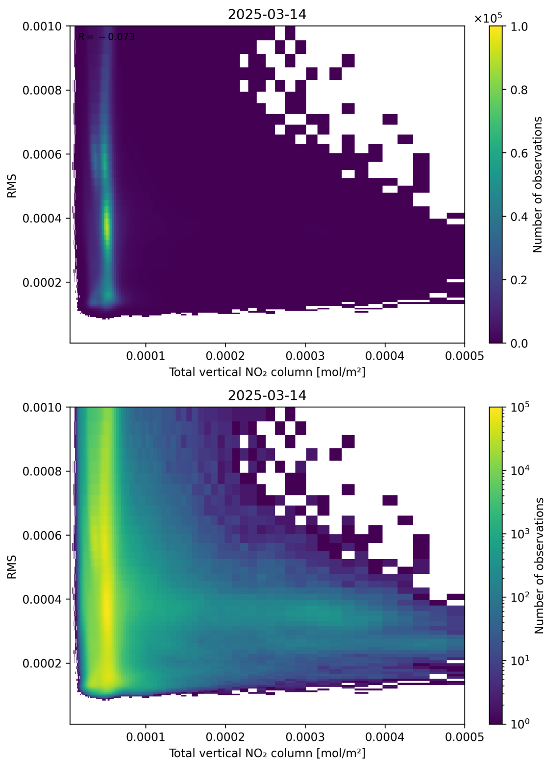
Figure 120: Scatter density plot of “Total vertical NO 2 column” against “RMS” for 2025-03-14 to 2025-03-15.
