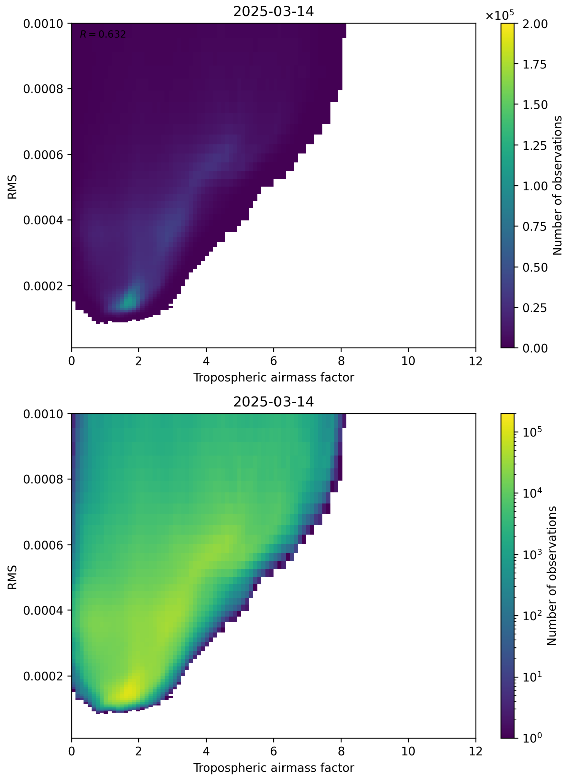
Figure 79: Scatter density plot of “Tropospheric airmass factor” against “RMS” for 2025-03-14 to 2025-03-15.
