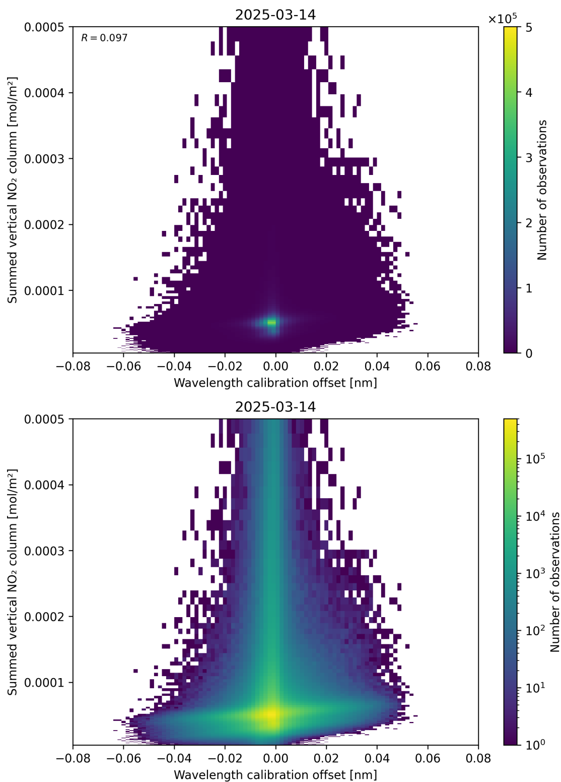
Figure 177: Scatter density plot of “Wavelength calibration offset” against “Summed vertical NO 2 column” for 2025-03-14 to 2025-03-15.
