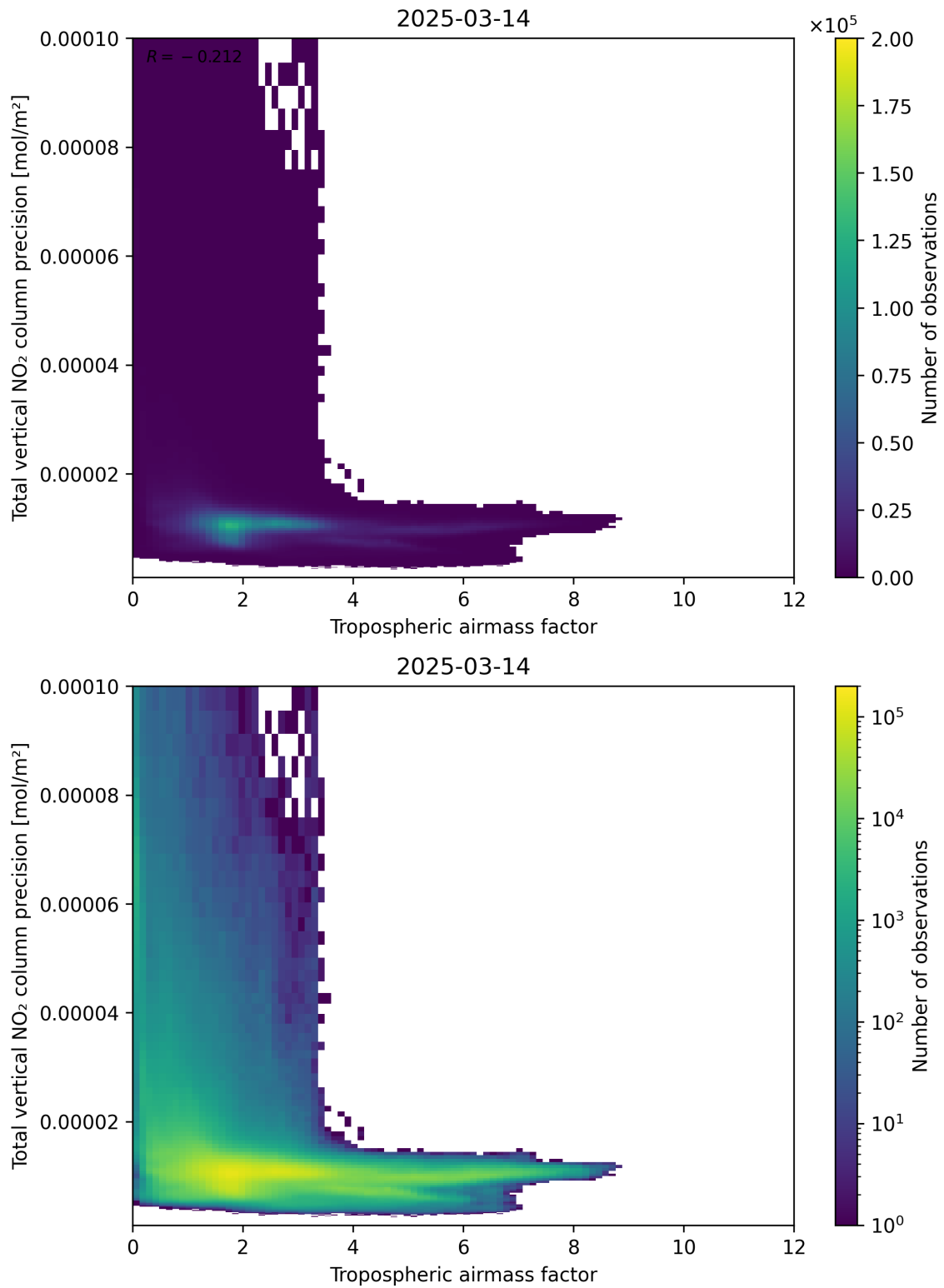
Figure 78: Scatter density plot of “Tropospheric air mass factor” against “Total vertical NO 2 column precision” for 2025-03-14 to 2025-03-15.
