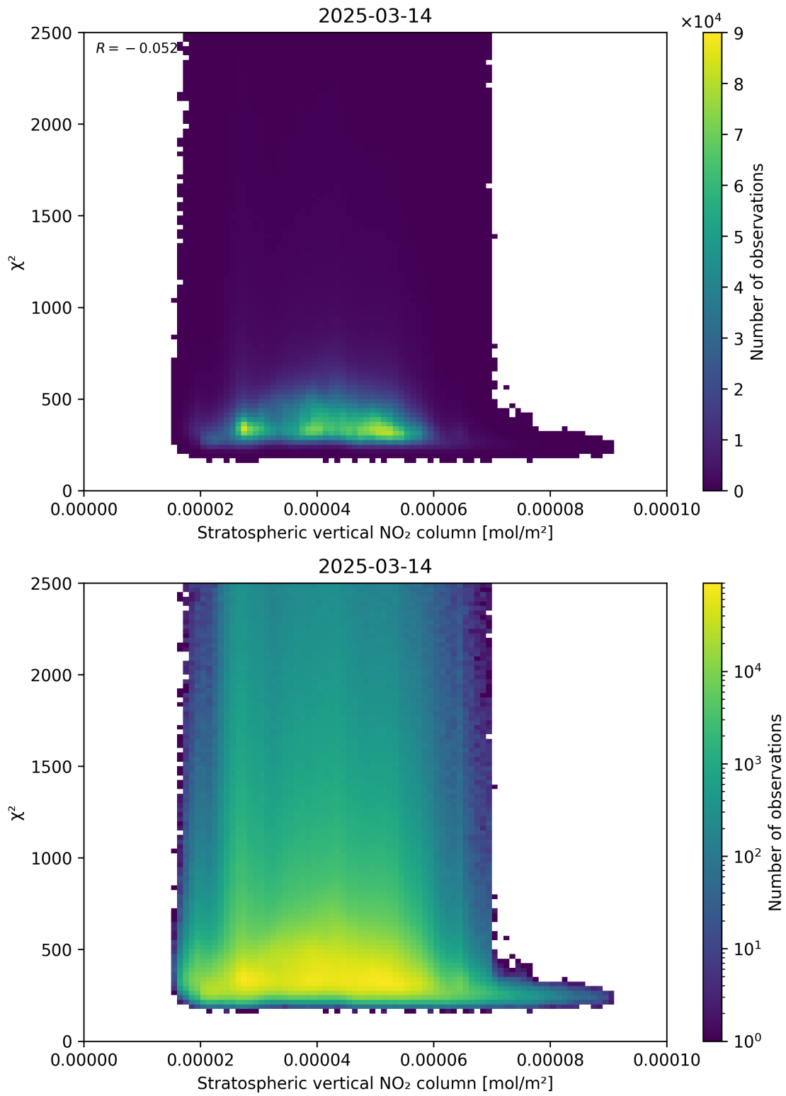
Figure 97: Scatter density plot of “Stratospheric vertical NO 2 column” against “ \chi^2 ” for 2025-03-14 to 2025-03-15.
