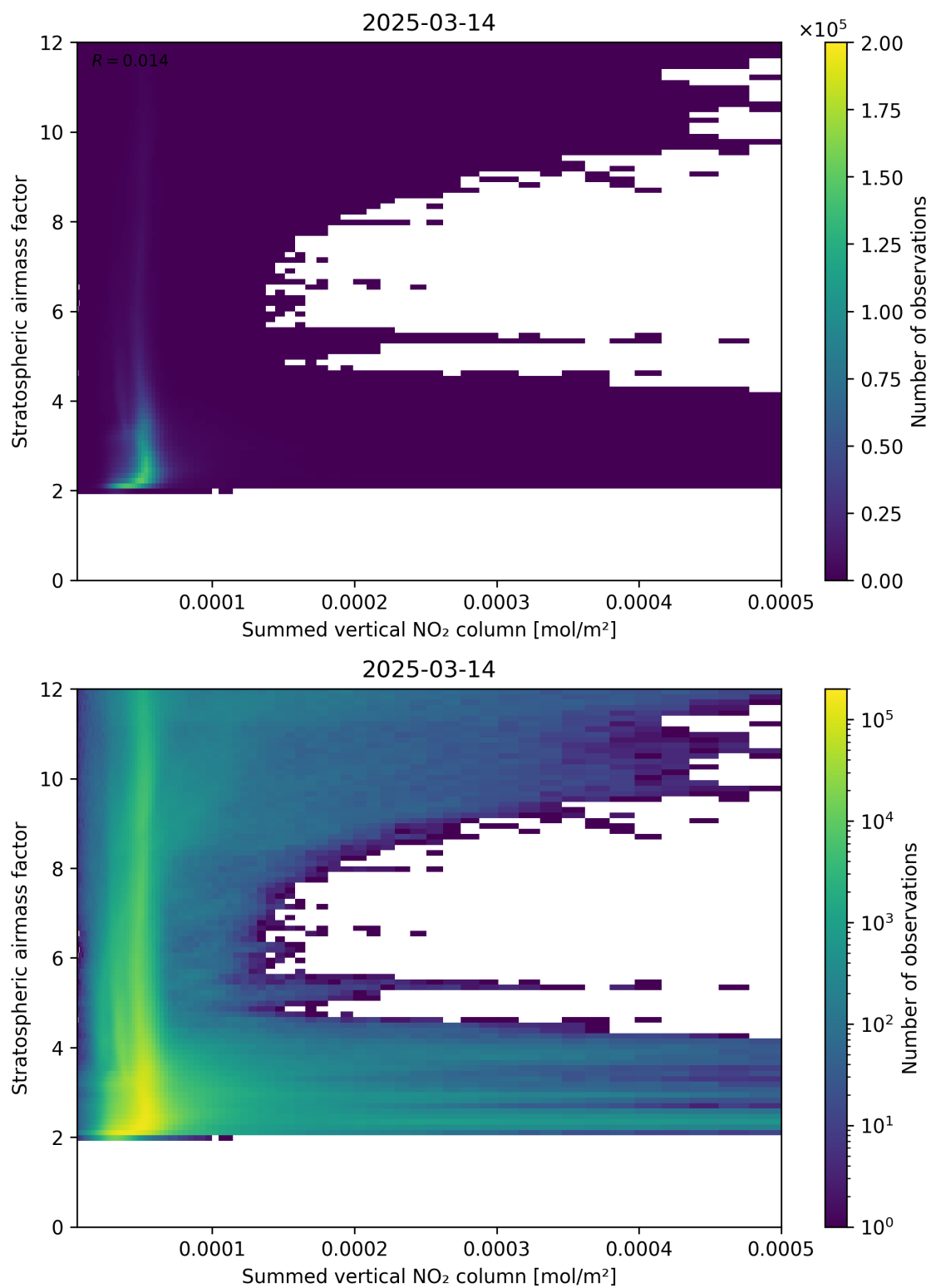
Figure 103: Scatter density plot of “Summed vertical NO 2 column” against “Stratospheric air mass factor” for 2025-03-14 to 2025-03-15.
