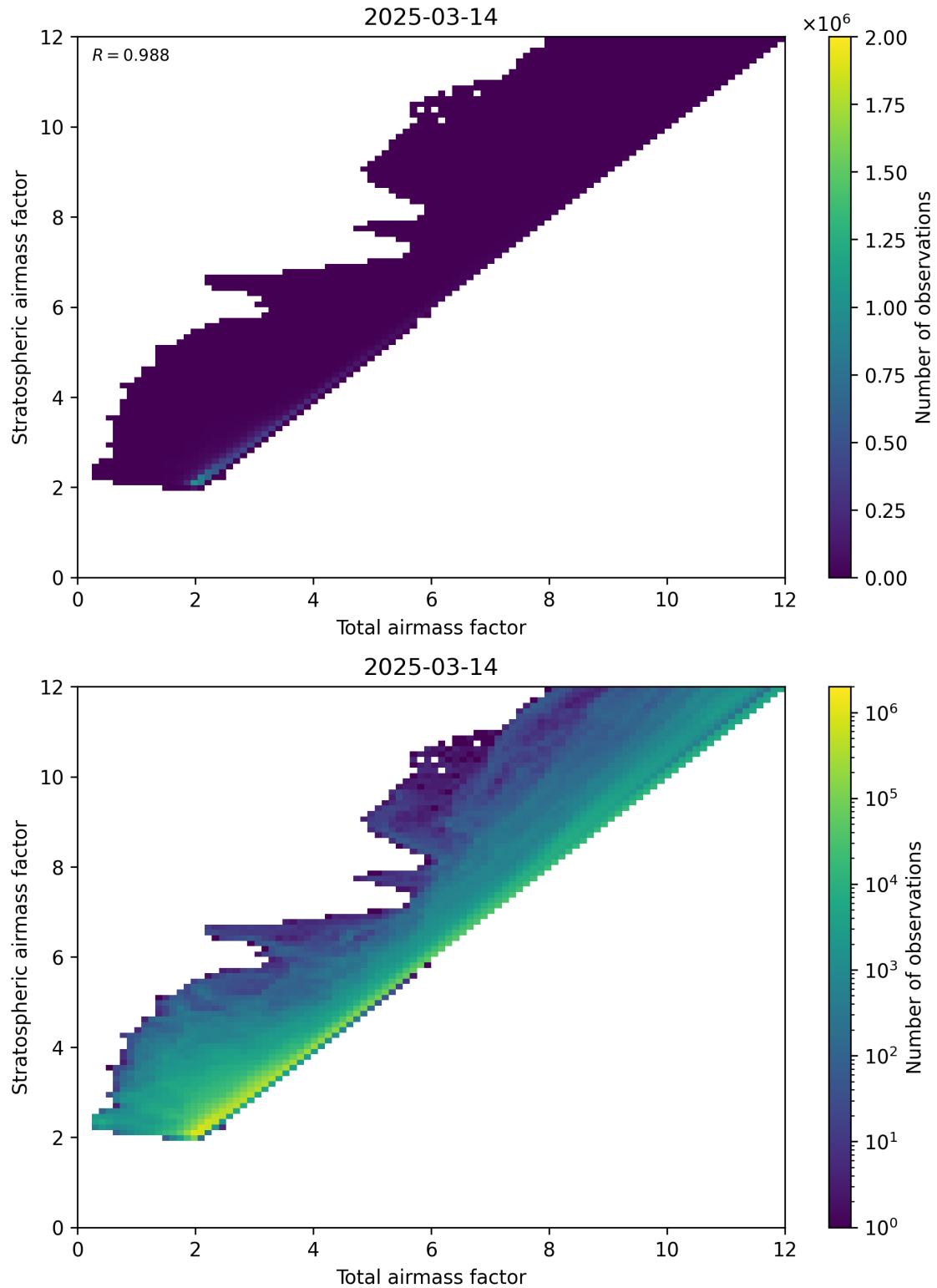
Figure 62: Scatter density plot of “Total airmass factor” against “Stratospheric airmass factor” for 2025-03-14 to 2025-03-15.
