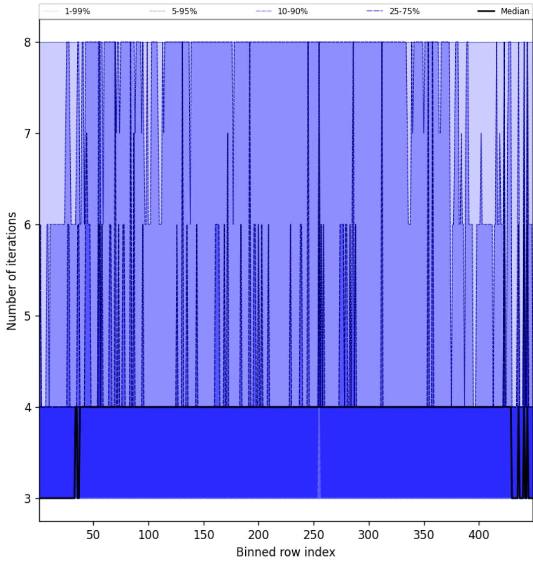
Figure 51: Along track statistics of “Number of iterations” for 2025-03-14 to 2025-03-15
