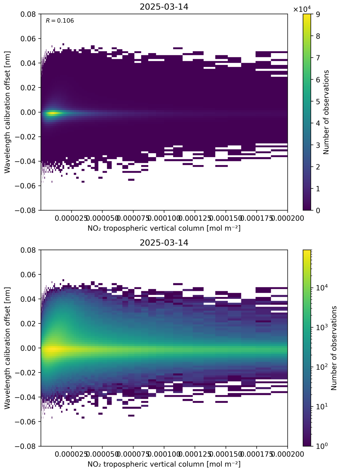
Figure 143: Scatter density plot of “NO 2 tropospheric vertical column” against “Wavelength calibration offset” for 2025-03-14 to 2025-03-15.
