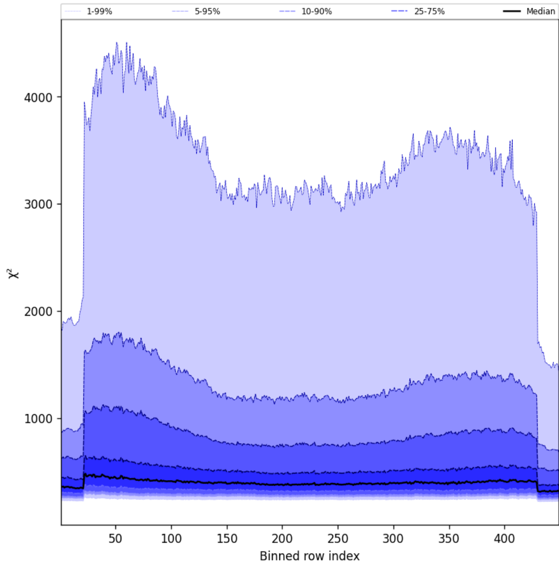
Figure 59: Along track statistics of “ \chi^2 ” for 2025-03-14 to 2025-03-15
