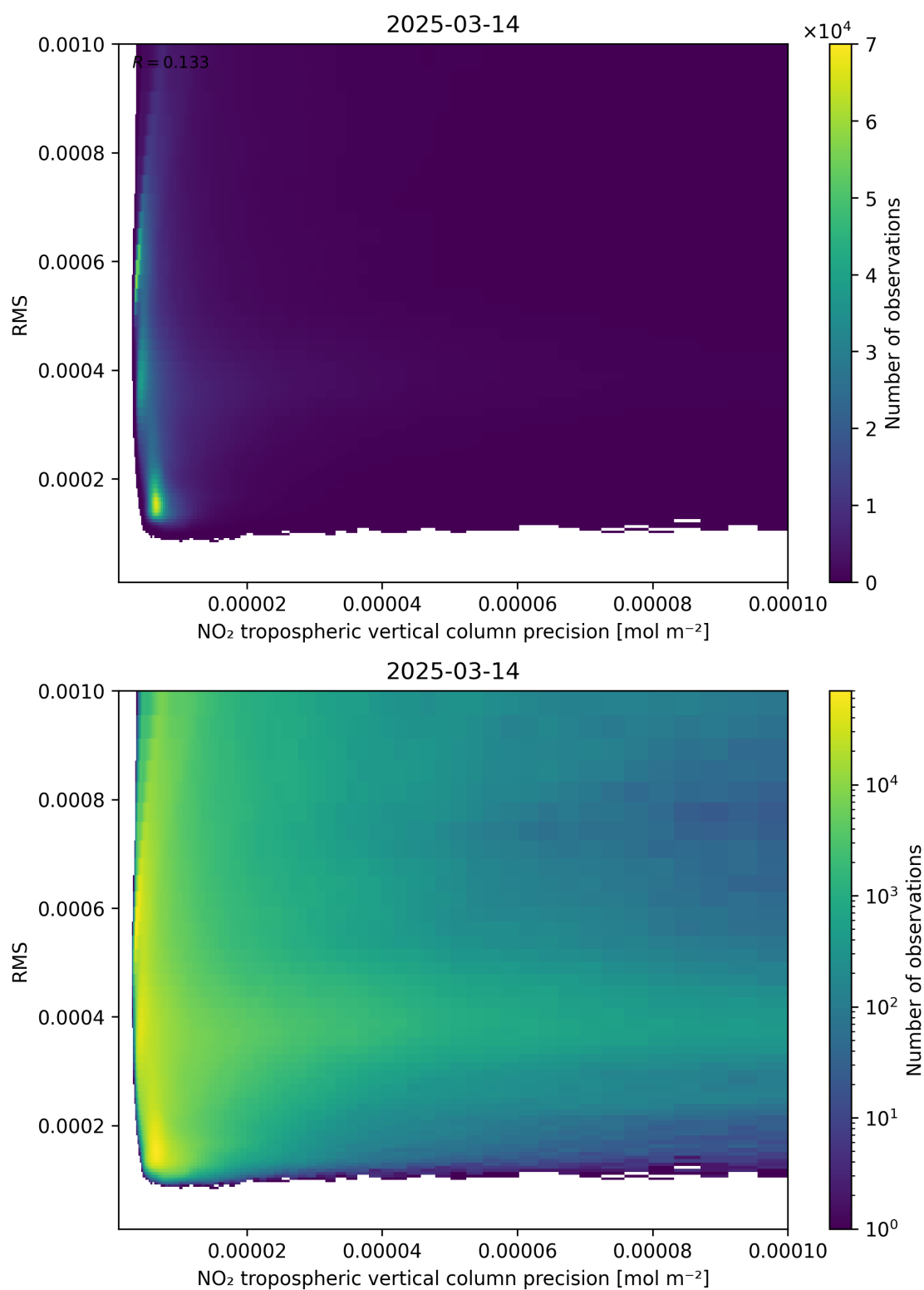
Figure 140: Scatter density plot of “NO 2 tropospheric vertical column precision” against “RMS” for 2025-03-14 to 2025-03-15.
