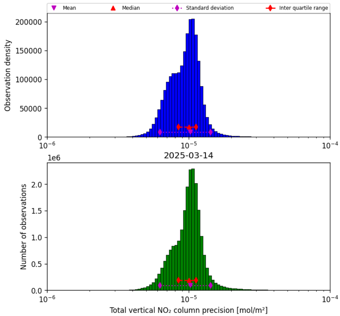
Figure 39: Histogram of “Total vertical NO 2 column precision” for 2025-03-14 to 2025-03-15
