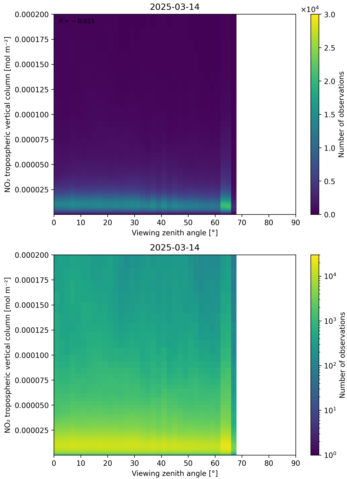
Figure 169: Scatter density plot of “Viewing zenith angle” against “NO 2 tropospheric vertical column” for 2025-03-14 to 2025-03-15.
