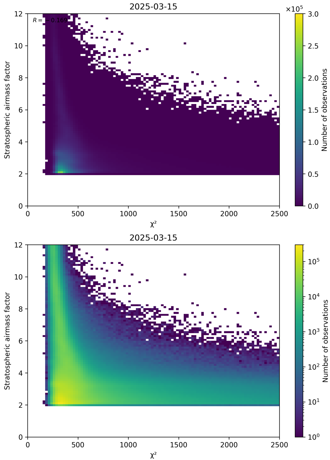
Figure 81: Scatter density plot of " \chi^2 " against "Stratospheric airmass factor" for 2025-03-15 to 2025-03-15.
