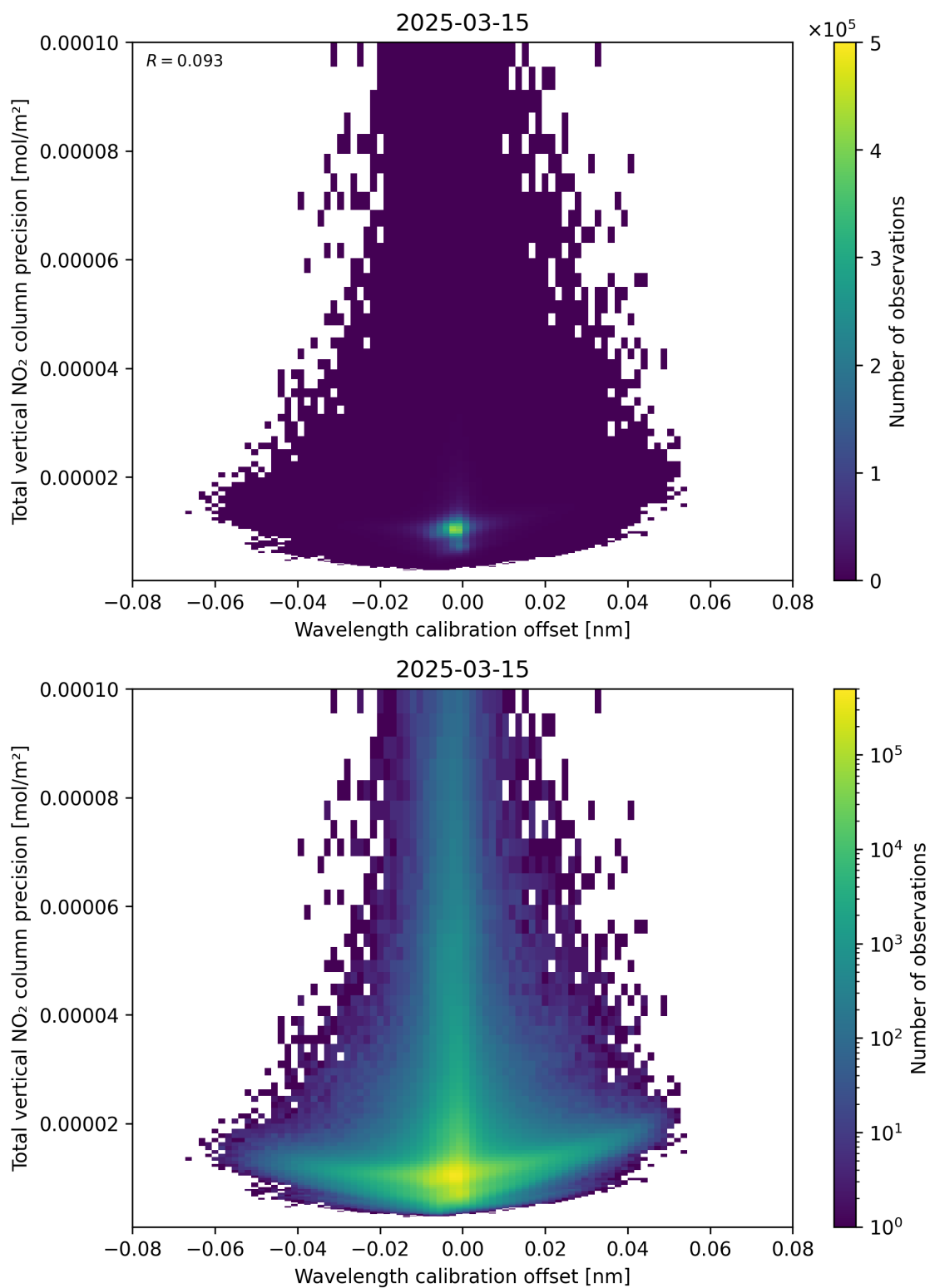
Figure 180: Scatter density plot of “Wavelength calibration offset” against “Total vertical NO 2 column precision” for 2025-03-15 to 2025-03-15.
