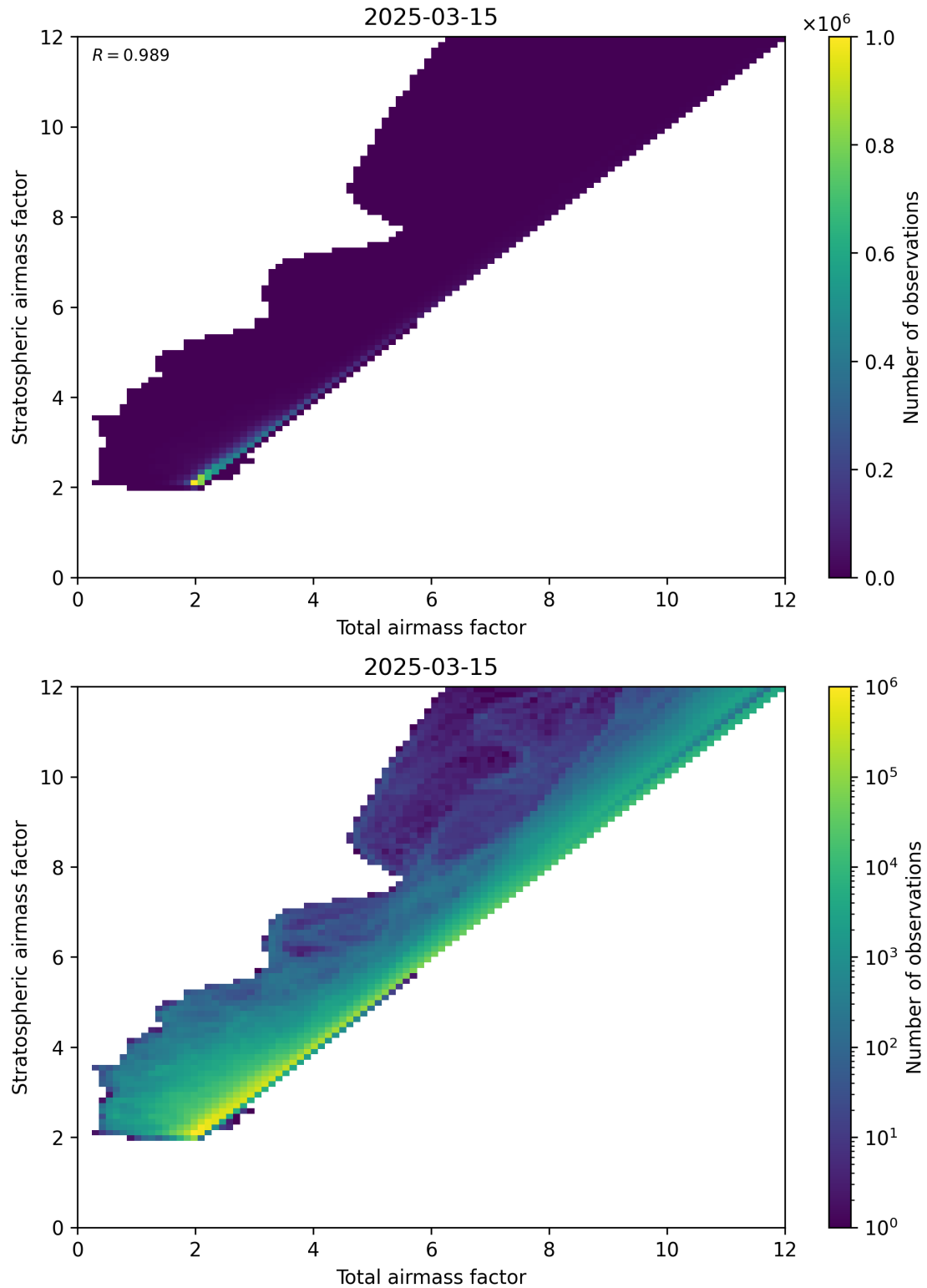
Figure 62: Scatter density plot of “Total airmass factor” against “Stratospheric airmass factor” for 2025-03-15 to 2025-03-15.
