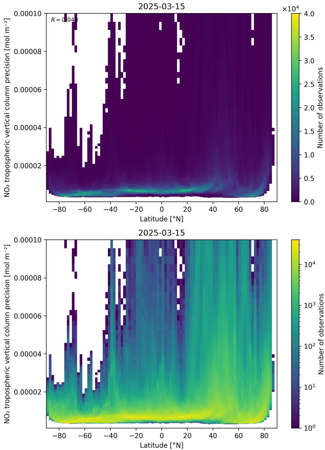
Figure 93: Scatter density plot of “Latitude” against “NO 2 tropospheric vertical column precision” for 2025-03-15 to 2025-03-15.
