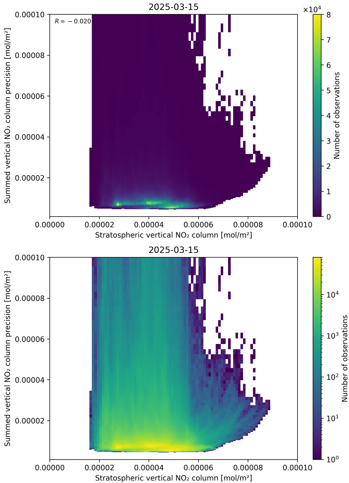
Figure 99: Scatter density plot of “Stratospheric vertical NO 2 column” against “Summed vertical NO 2 column precision” for 2025-03-15 to 2025-03-15.
