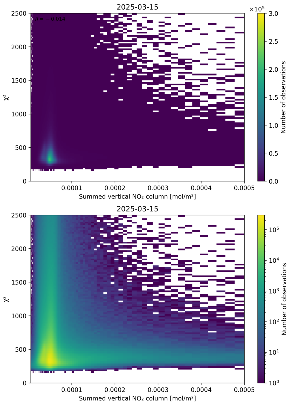
Figure 104: Scatter density plot of “Summed vertical NO 2 column” against “ \chi^2 ” for 2025-03-15 to 2025-03-15.
