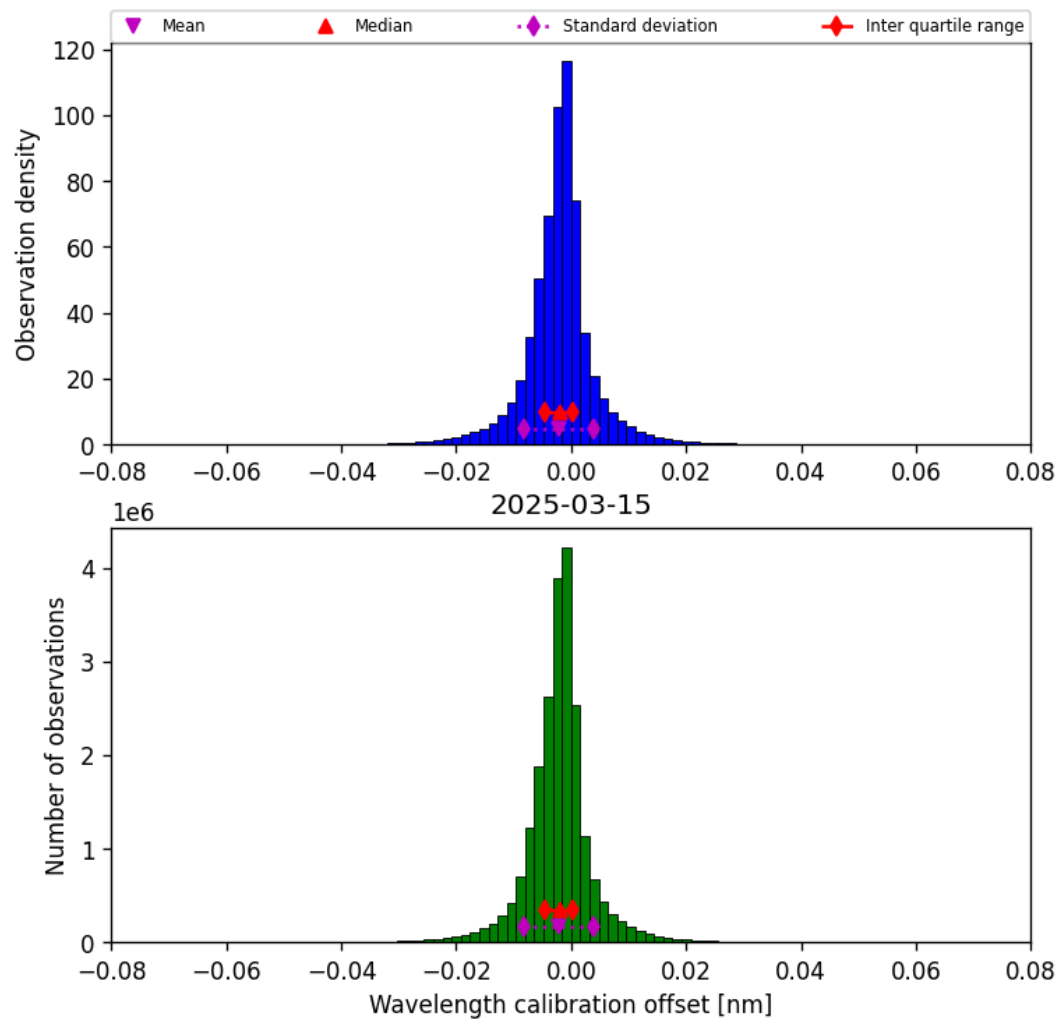
Figure 35: Histogram of “Wavelength calibration offset” for 2025-03-15 to 2025-03-15
