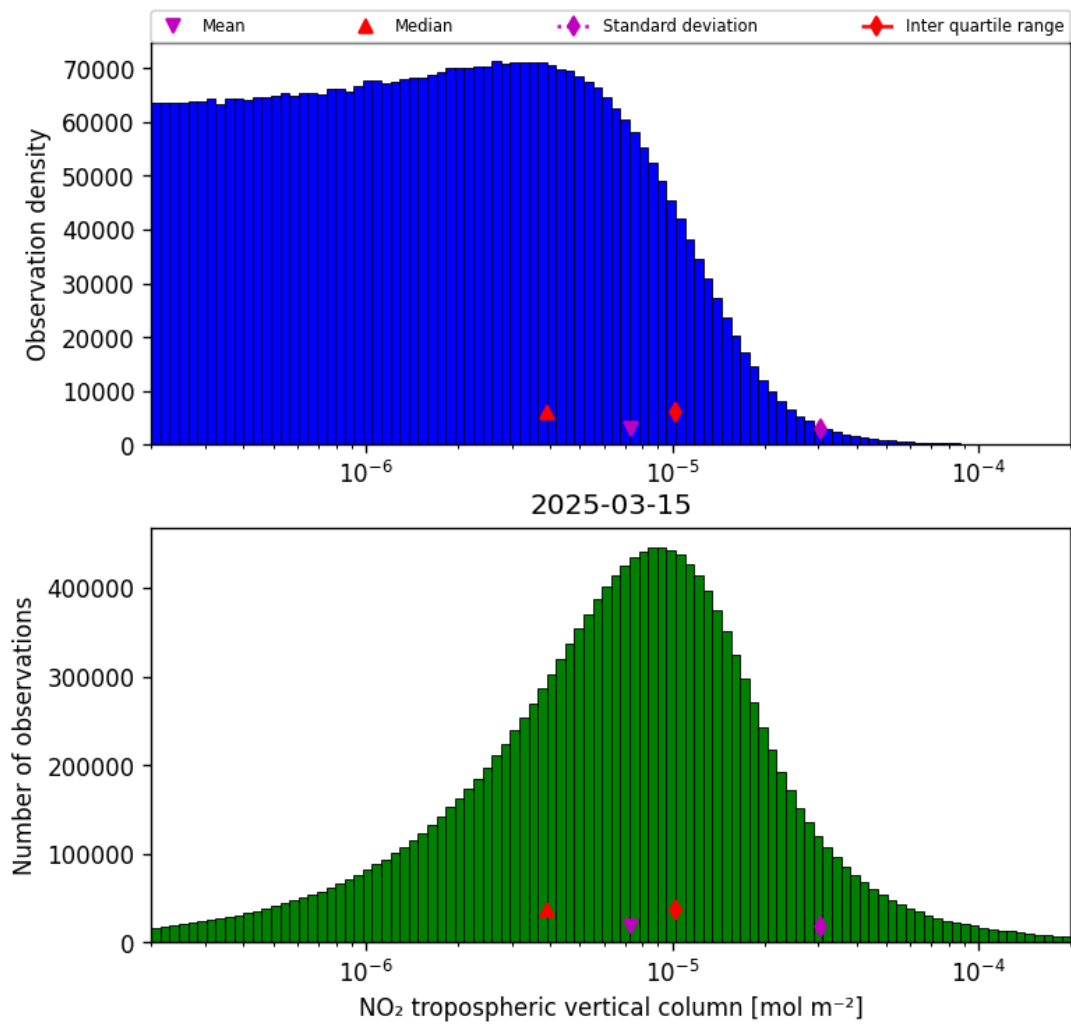
Figure 29: Histogram of “NO 2 tropospheric vertical column” for 2025-03-15 to 2025-03-15
