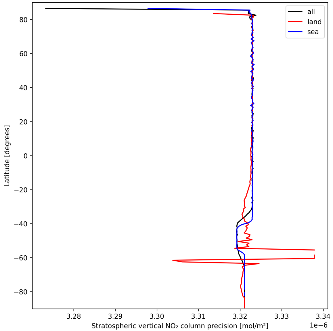
Figure 20: Zonal average of “Stratospheric vertical NO 2 column precision” for 2025-03-15 to 2025-03-15.
