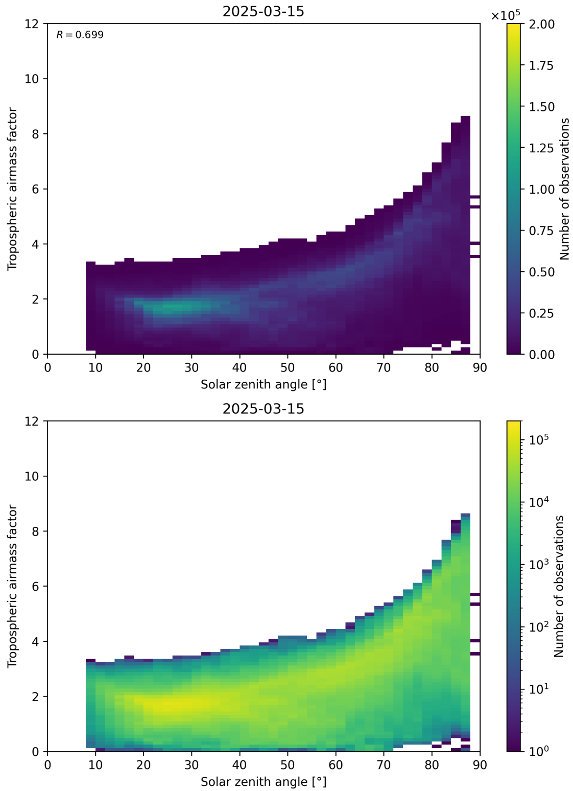
Figure 147: Scatter density plot of “Solar zenith angle” against “Tropospheric airmass factor” for 2025-03-15 to 2025-03-15.
