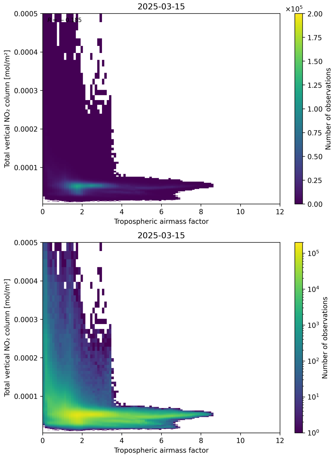
Figure 77: Scatter density plot of “Tropospheric airmass factor” against “Total vertical NO 2 column” for 2025-03-15 to 2025-03-15.
