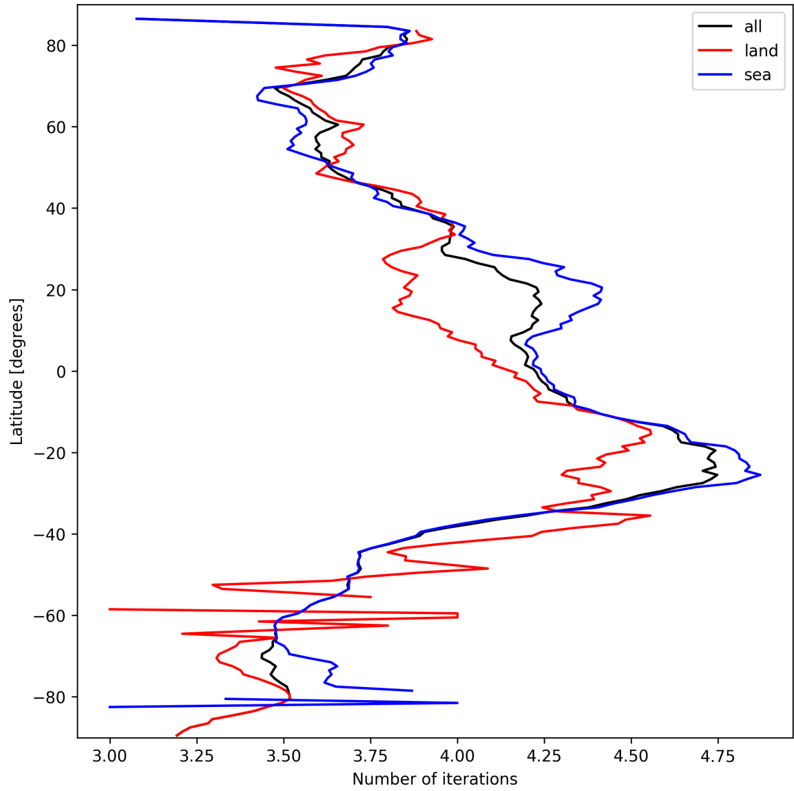
Figure 17: Zonal average of “Number of iterations” for 2025-03-15 to 2025-03-15.
