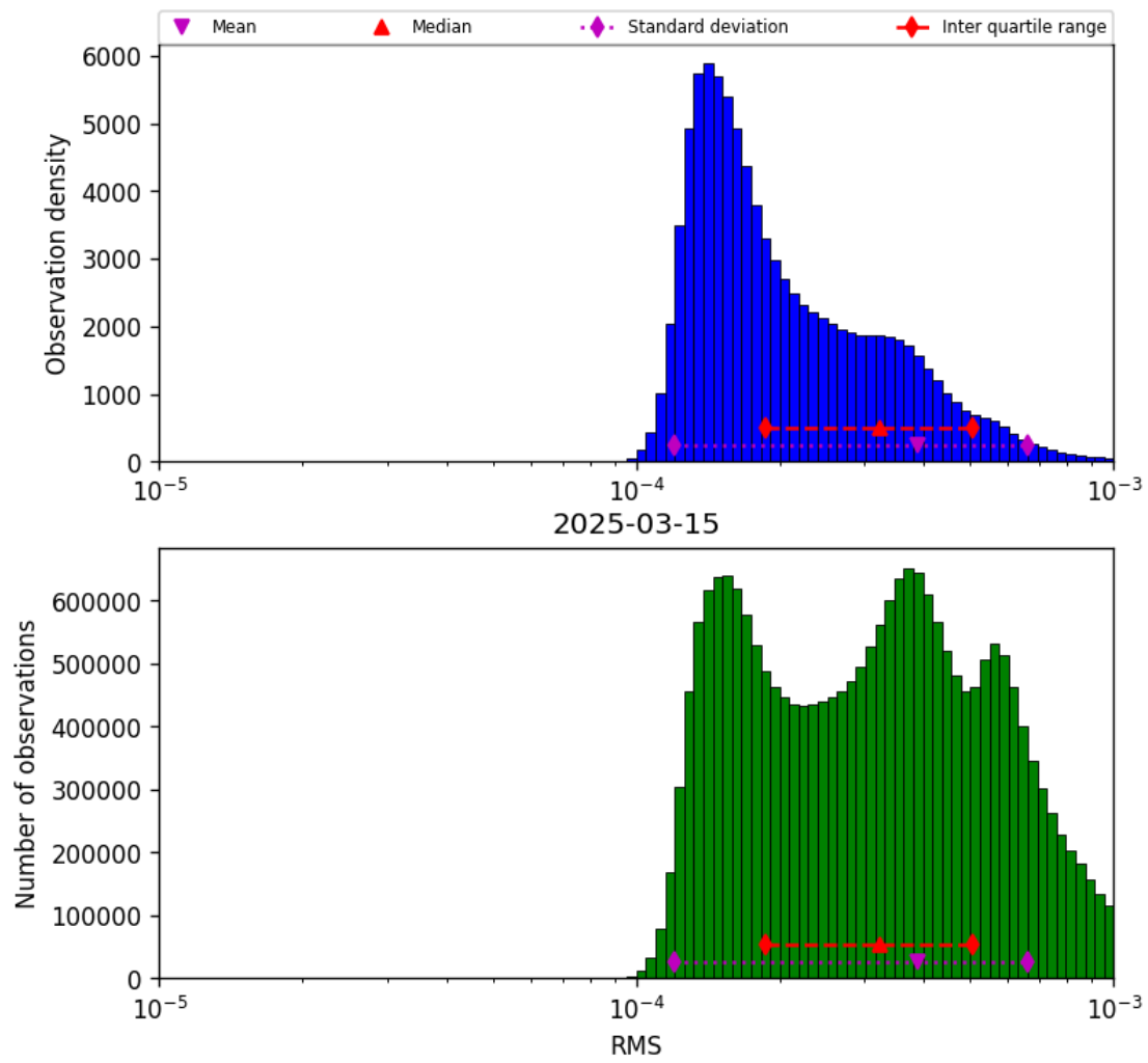
Figure 43: Histogram of “RMS” for 2025-03-15 to 2025-03-15
