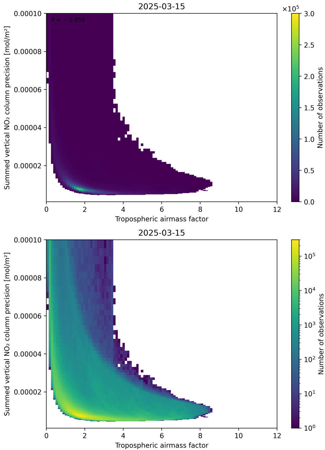
Figure 76: Scatter density plot of “Tropospheric air mass factor” against “Summed vertical NO 2 column precision” for 2025-03-15 to 2025-03-15.
