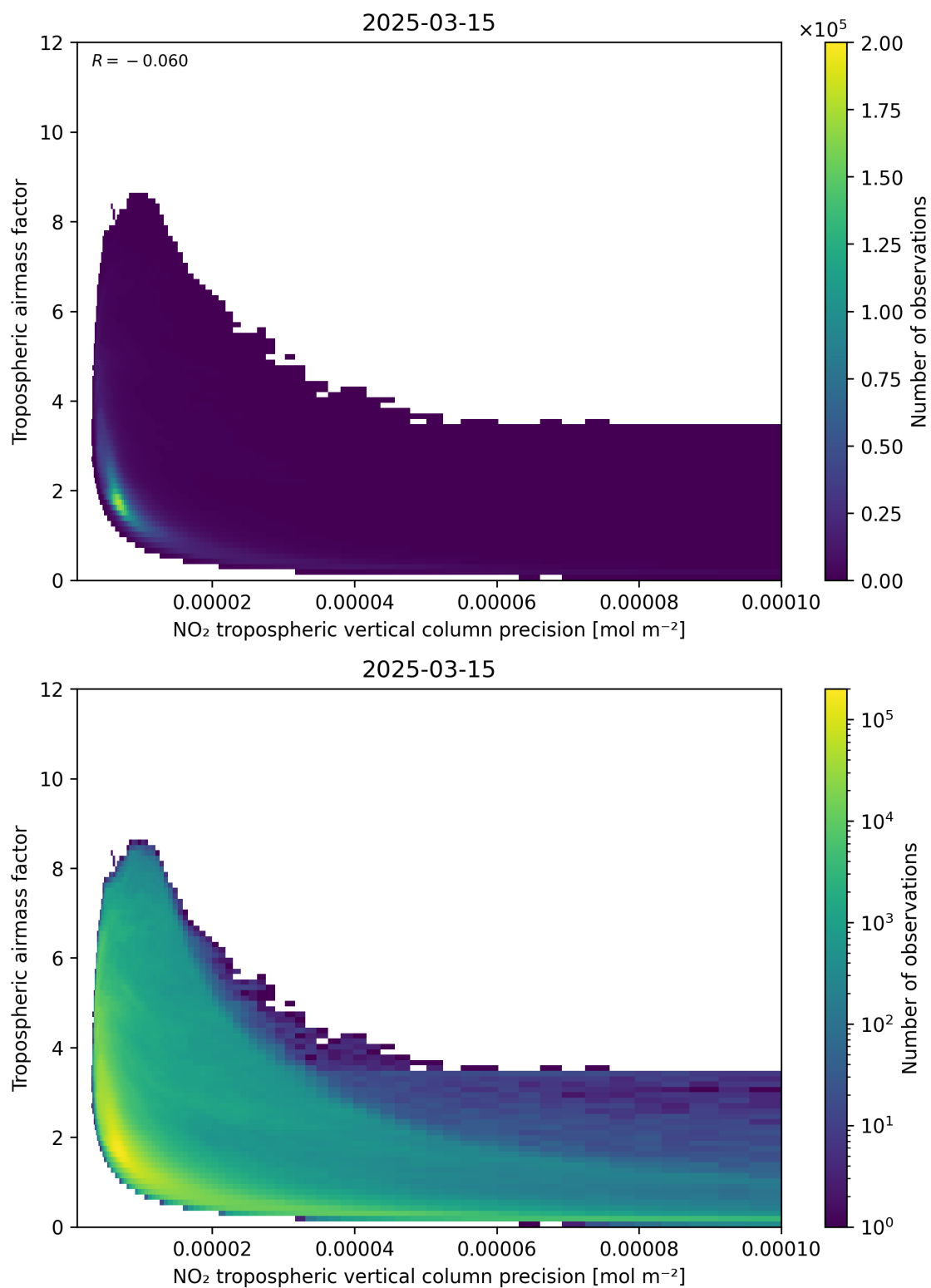
Figure 133: Scatter density plot of “NO 2 tropospheric vertical column precision” against “Tropospheric airmass factor” for 2025-03-15 to 2025-03-15.
