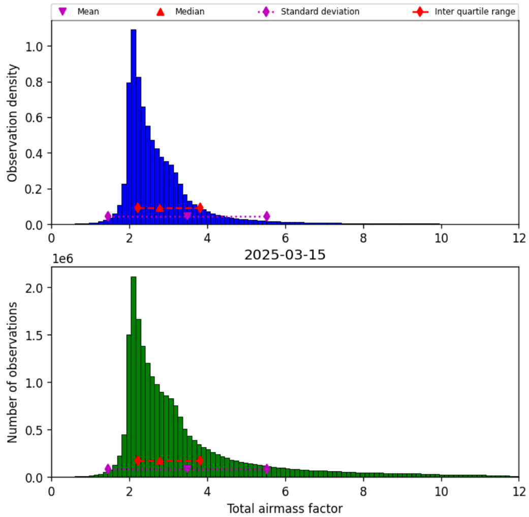
Figure 32: Histogram of “Total airmass factor” for 2025-03-15 to 2025-03-15
