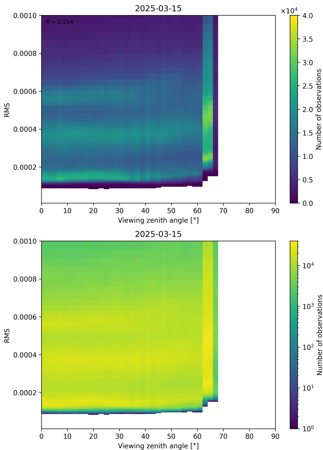
Figure 171: Scatter density plot of “Viewing zenith angle” against “RMS” for 2025-03-15 to 2025-03-15.
