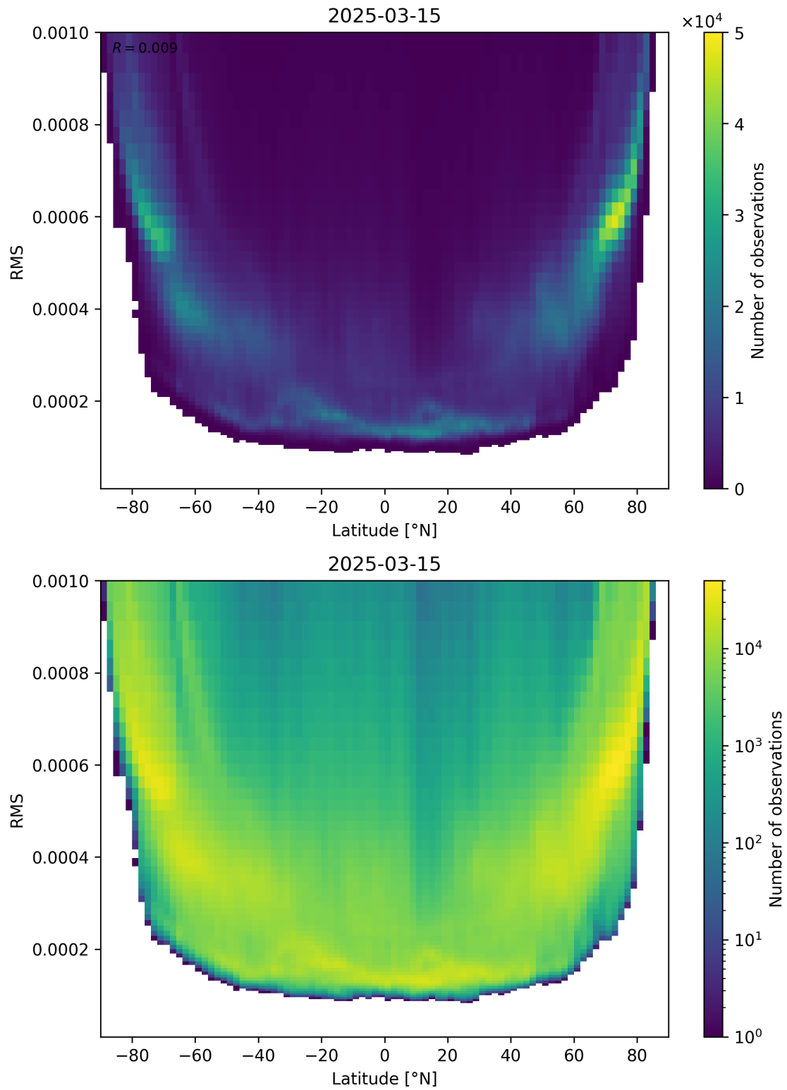
Figure 94: Scatter density plot of “Latitude” against “RMS” for 2025-03-15 to 2025-03-15.
