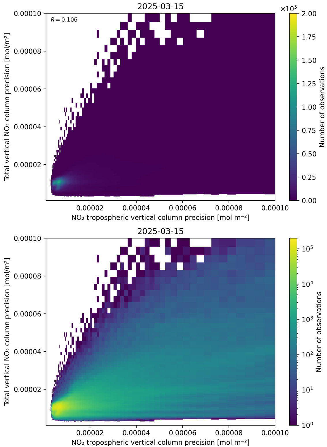
Figure 139: Scatter density plot of “NO 2 tropospheric vertical column precision” against “Total vertical NO 2 column precision” for 2025-03-15 to 2025-03-15.
