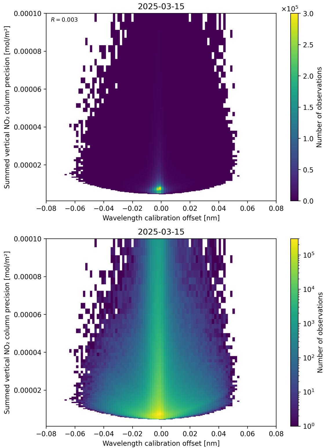
Figure 178: Scatter density plot of “Wavelength calibration offset” against “Summed vertical NO 2 column precision” for 2025-03-15 to 2025-03-15.
