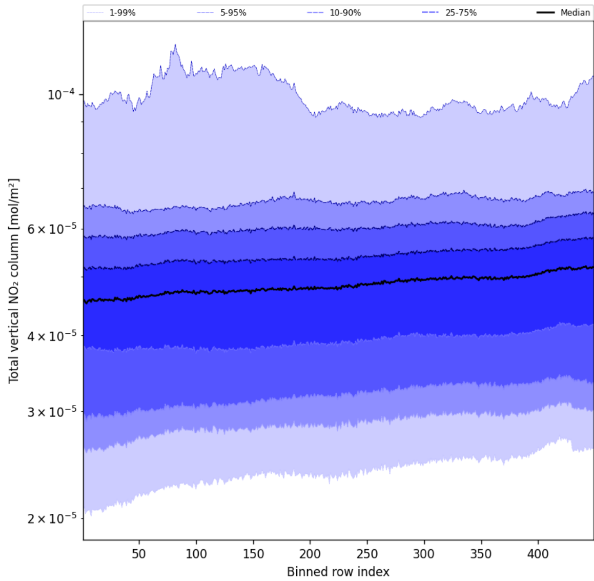
Figure 55: Along track statistics of “Total vertical NO 2 column” for 2025-03-15 to 2025-03-15
