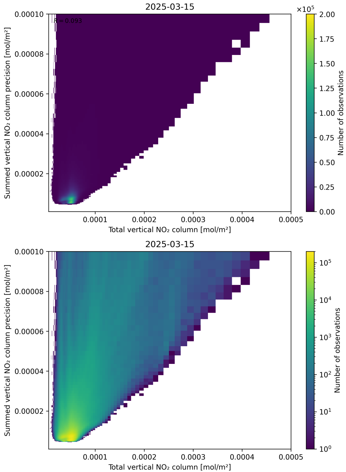
Figure 113: Scatter density plot of “Total vertical NO 2 column” against “Summed vertical NO 2 column precision” for 2025-03-15 to 2025-03-15.
