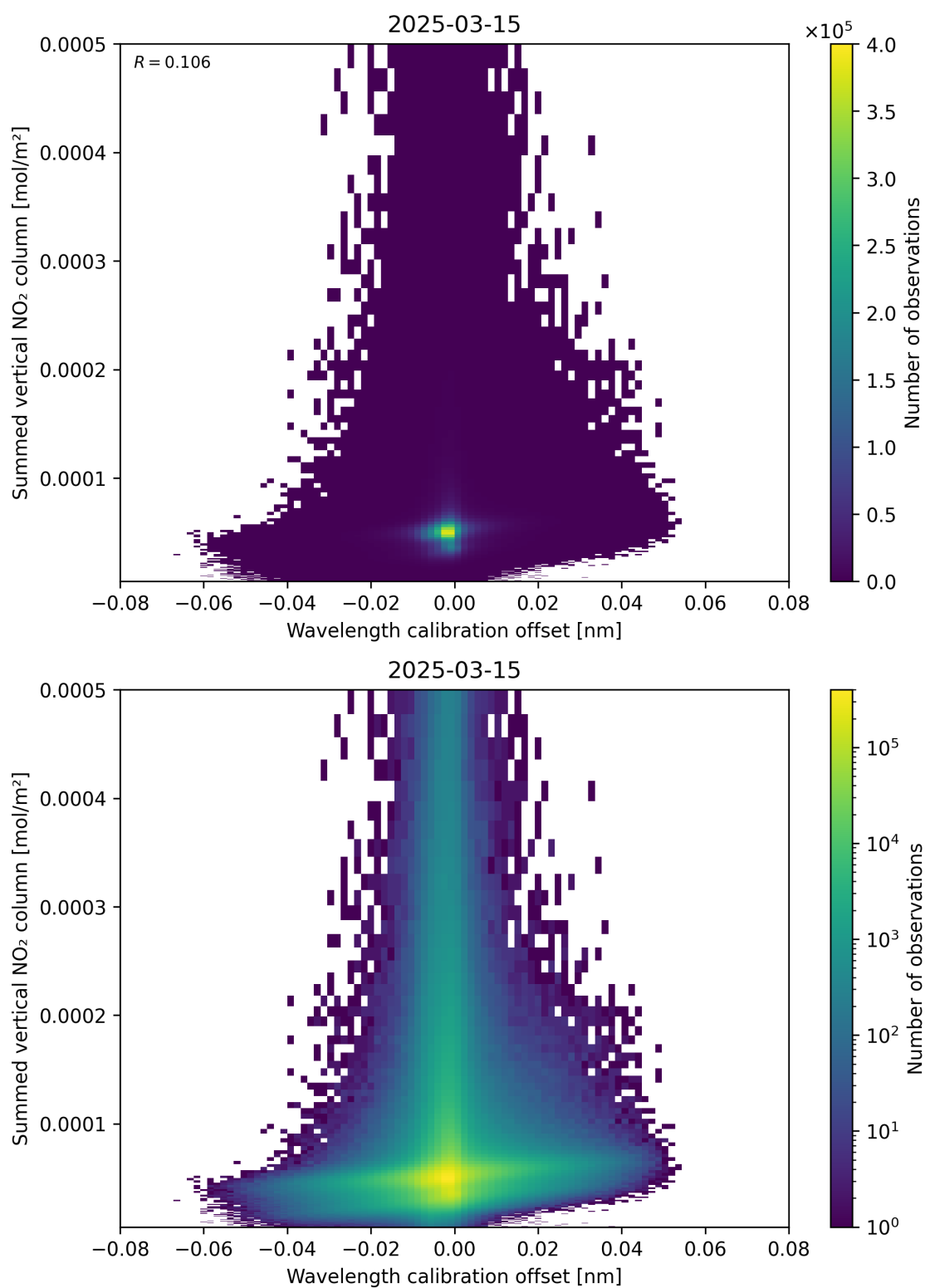
Figure 177: Scatter density plot of “Wavelength calibration offset” against “Summed vertical NO 2 column” for 2025-03-15 to 2025-03-15.
