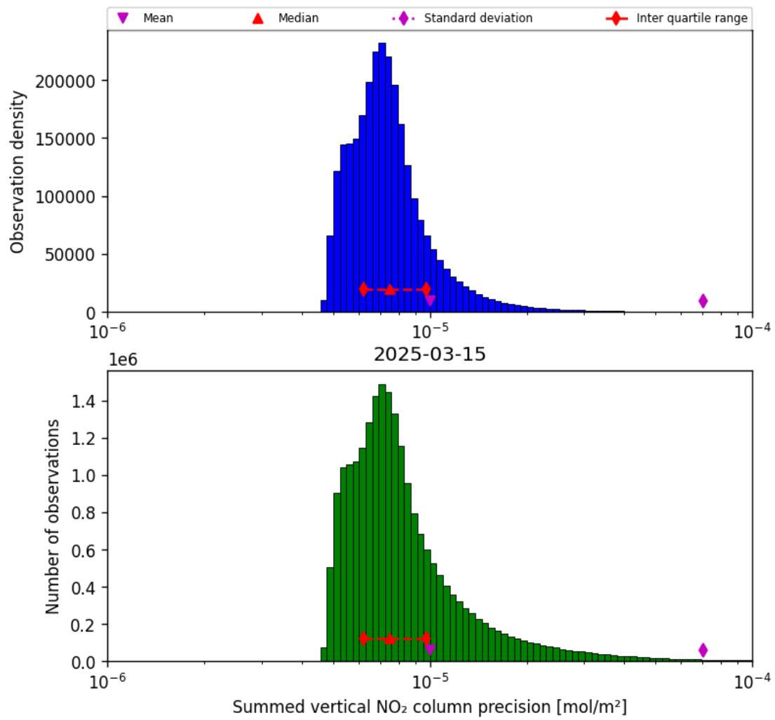
Figure 41: Histogram of "Summed vertical NO 2 column precision" for 2025-03-15 to 2025-03-15
