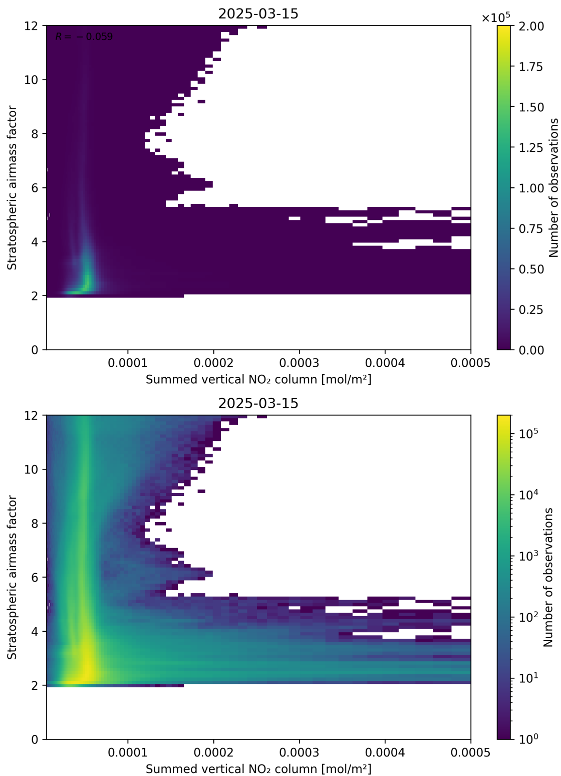
Figure 103: Scatter density plot of “Summed vertical NO 2 column” against “Stratospheric airmass factor” for 2025-03-15 to 2025-03-15.
