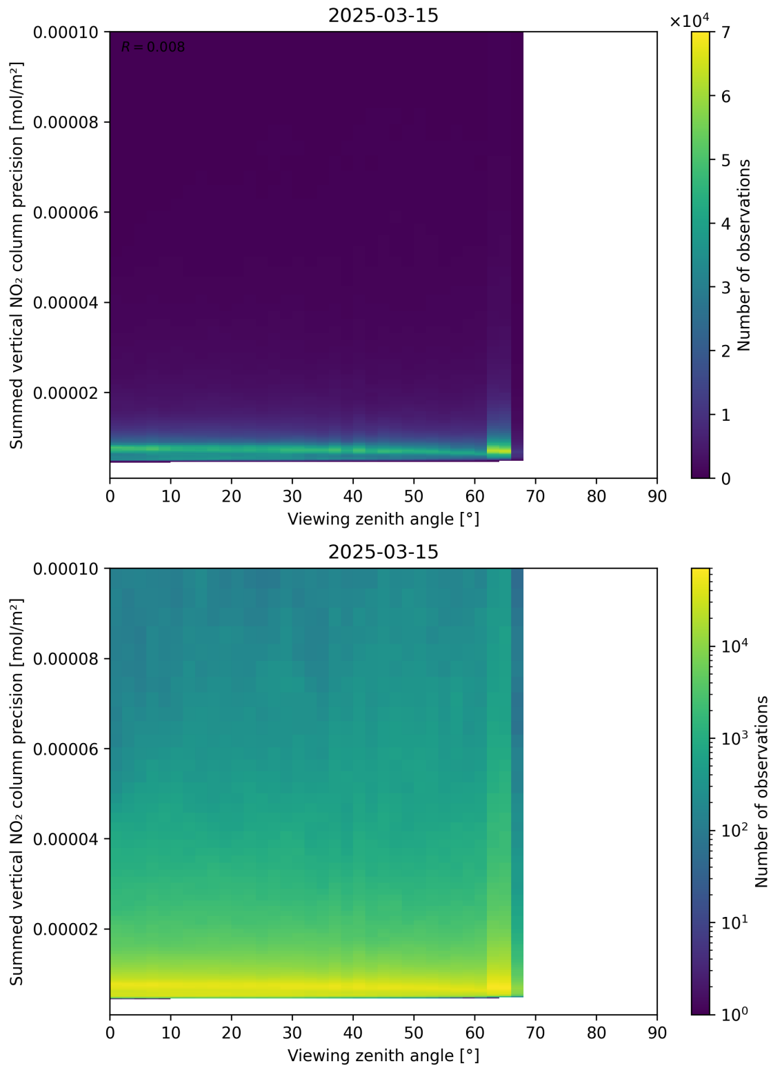
Figure 166: Scatter density plot of “Viewing zenith angle” against “Summed vertical NO 2 column precision” for 2025-03-15 to 2025-03-15.
