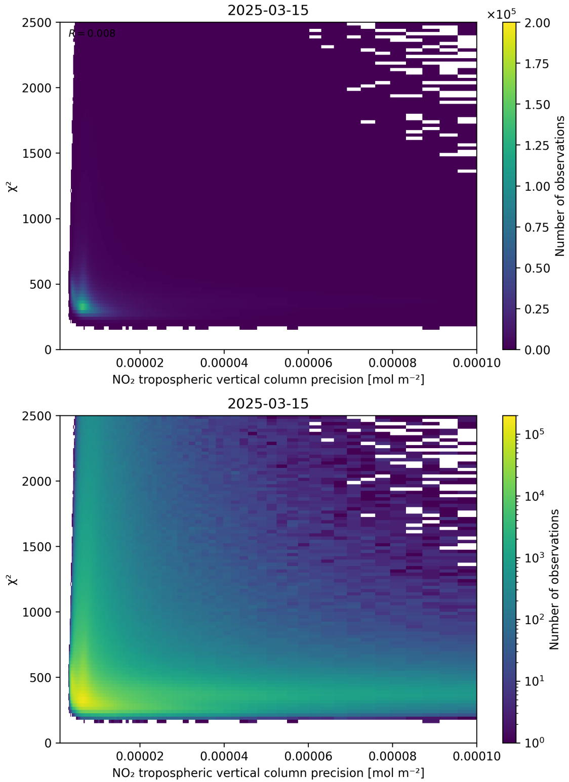
Figure 134: Scatter density plot of “NO 2 tropospheric vertical column precision” against “ \chi^2 ” for 2025-03-15 to 2025-03-15.
