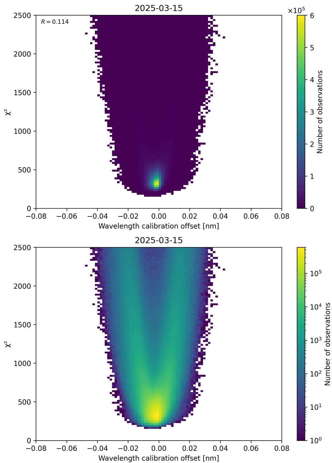
Figure 175: Scatter density plot of “Wavelength calibration offset” against “ \chi^2 ” for 2025-03-15 to 2025-03-15.
