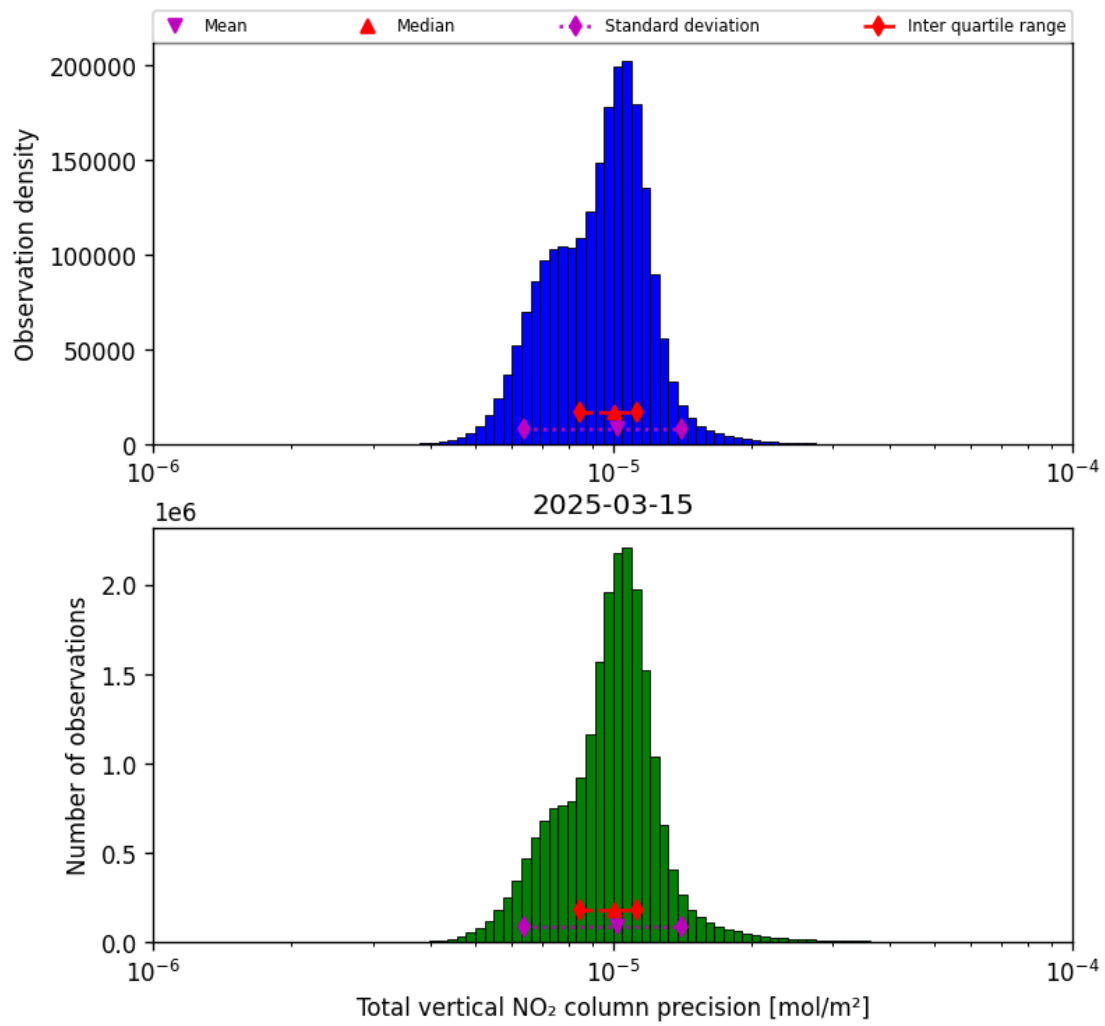
Figure 39: Histogram of "Total vertical NO 2 column precision" for 2025-03-15 to 2025-03-15
