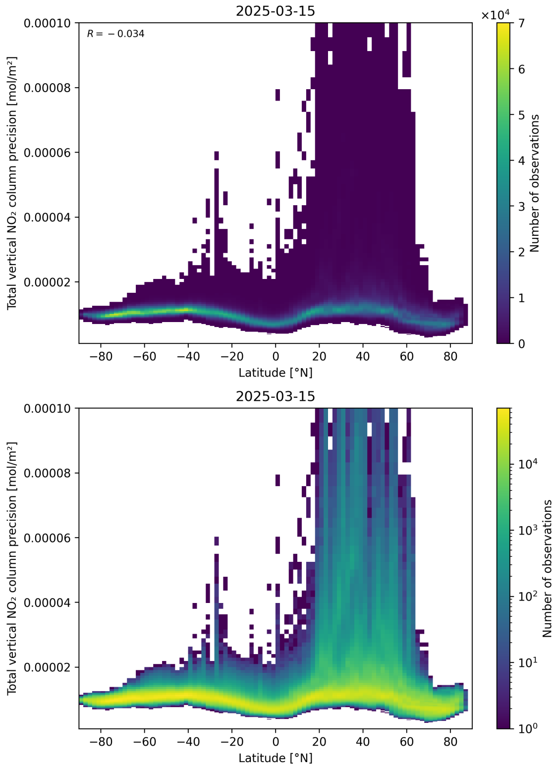
Figure 91: Scatter density plot of “Latitude” against “Total vertical NO 2 column precision” for 2025-03-15 to 2025-03-15.
