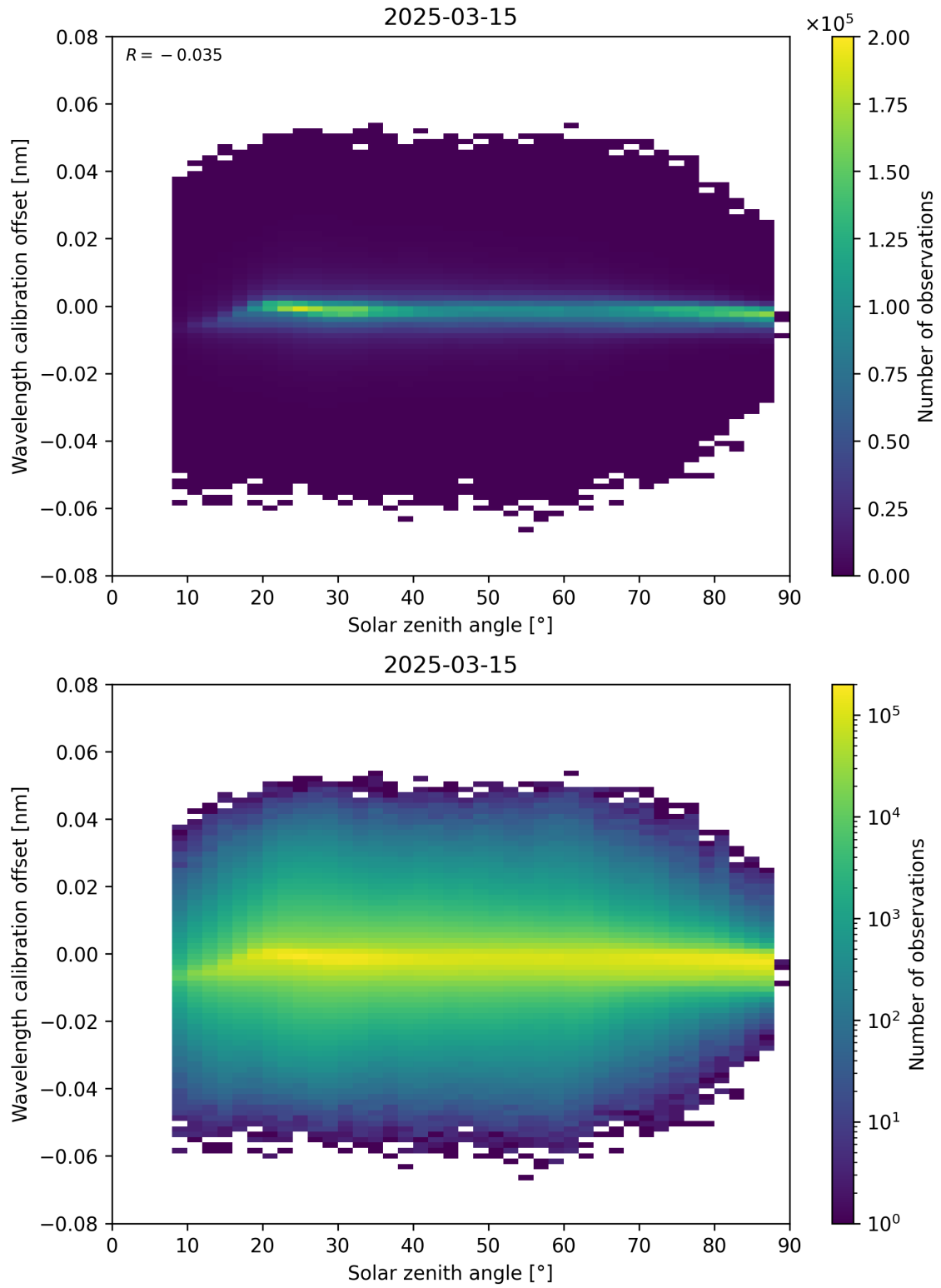
Figure 158: Scatter density plot of “Solar zenith angle” against “Wavelength calibration offset” for 2025-03-15 to 2025-03-15.
