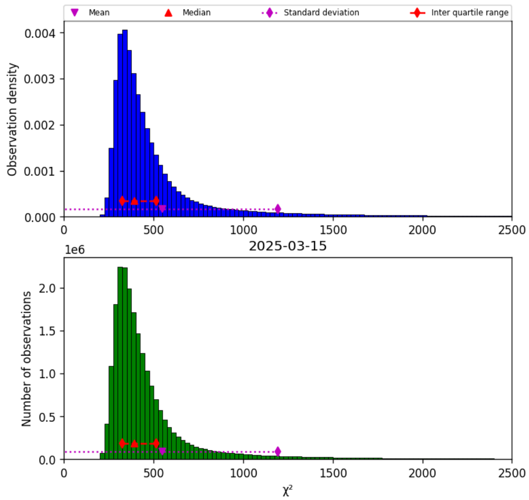
Figure 42: Histogram of “ \chi^2 ” for 2025-03-15 to 2025-03-15
