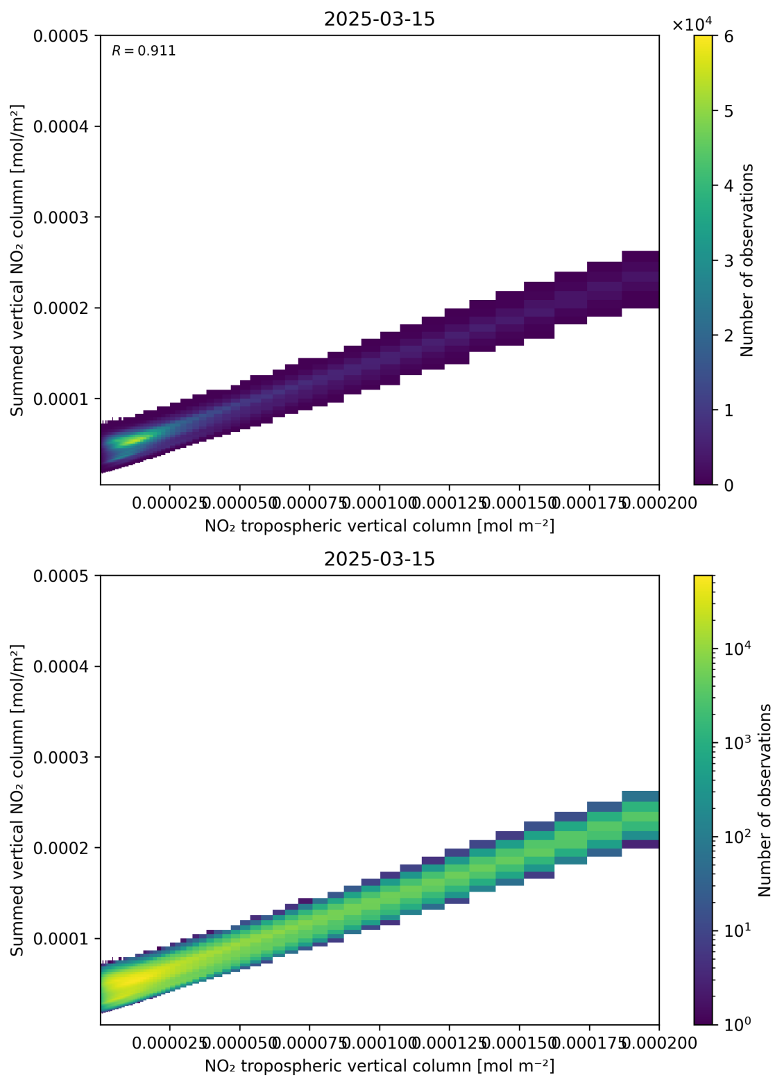
Figure 126: Scatter density plot of “NO 2 tropospheric vertical column” against “Summed vertical NO 2 column” for 2025-03-15 to 2025-03-15.
