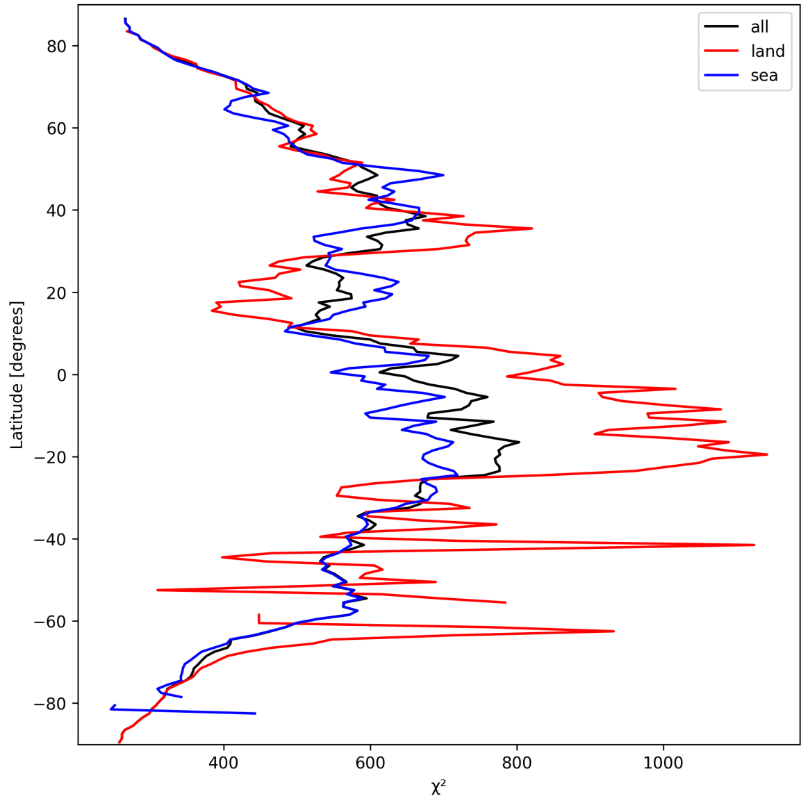
Figure 25: Zonal average of “ \chi^2 ” for 2025-03-15 to 2025-03-15.
