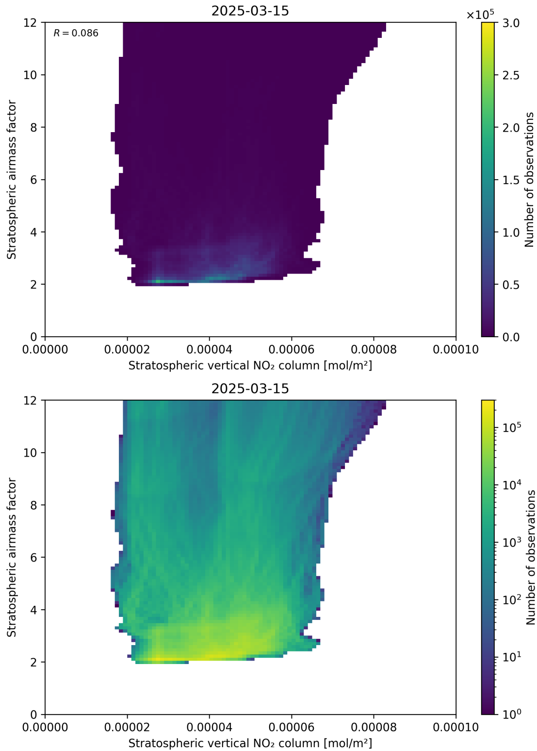
Figure 96: Scatter density plot of “Stratospheric vertical NO 2 column” against “Stratospheric airmass factor” for 2025-03-15 to 2025-03-15.
