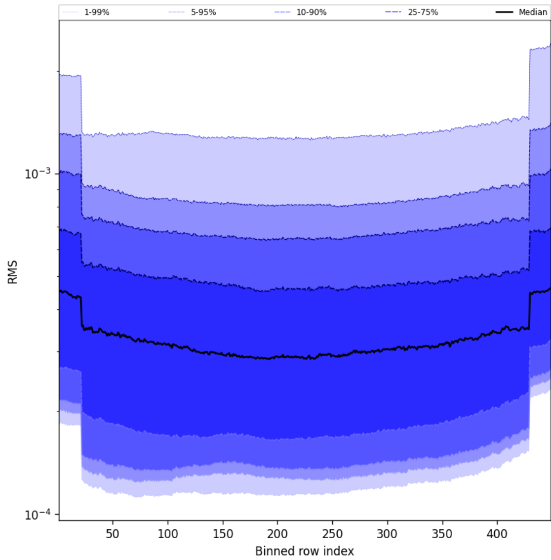
Figure 60: Along track statistics of “RMS” for 2025-03-15 to 2025-03-15
