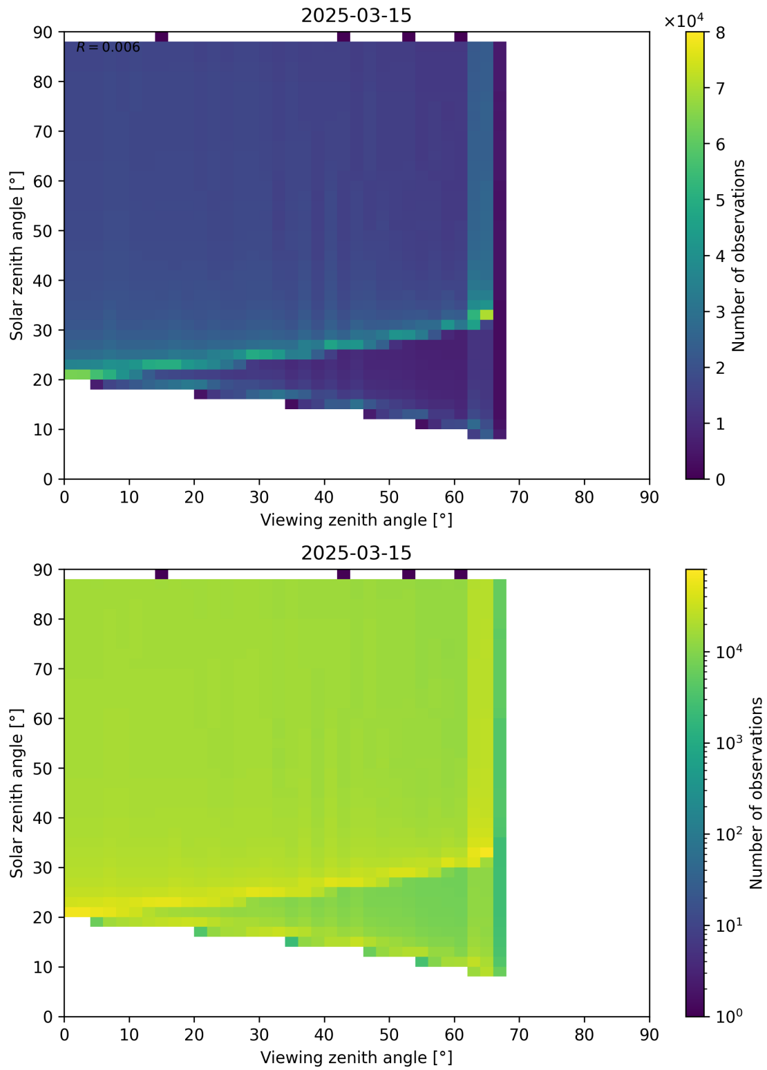
Figure 172: Scatter density plot of “Viewing zenith angle” against “Solar zenith angle” for 2025-03-15 to 2025-03-15.
