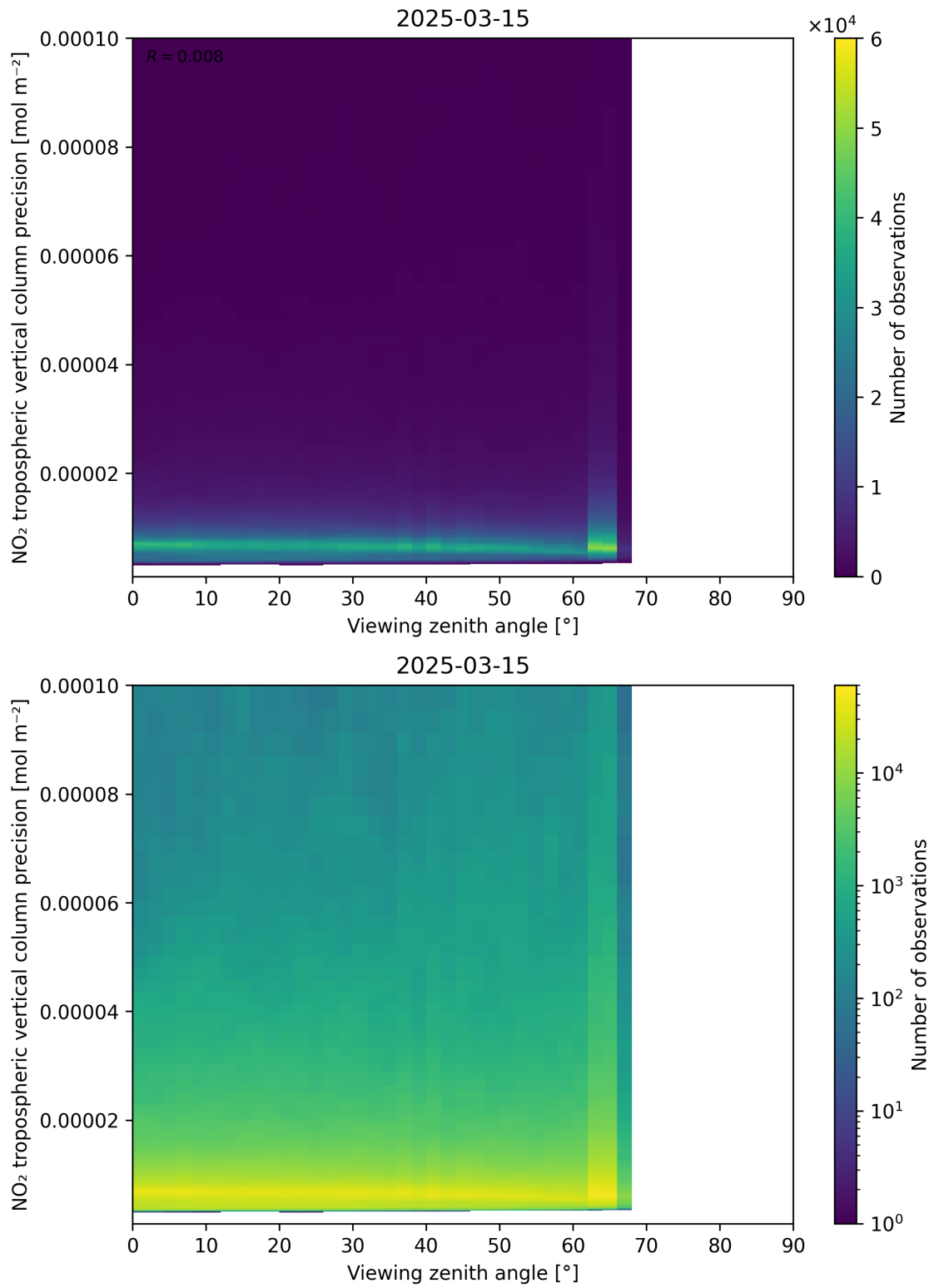
Figure 170: Scatter density plot of “Viewing zenith angle” against “NO 2 tropospheric vertical column precision” for 2025-03-15 to 2025-03-15.
