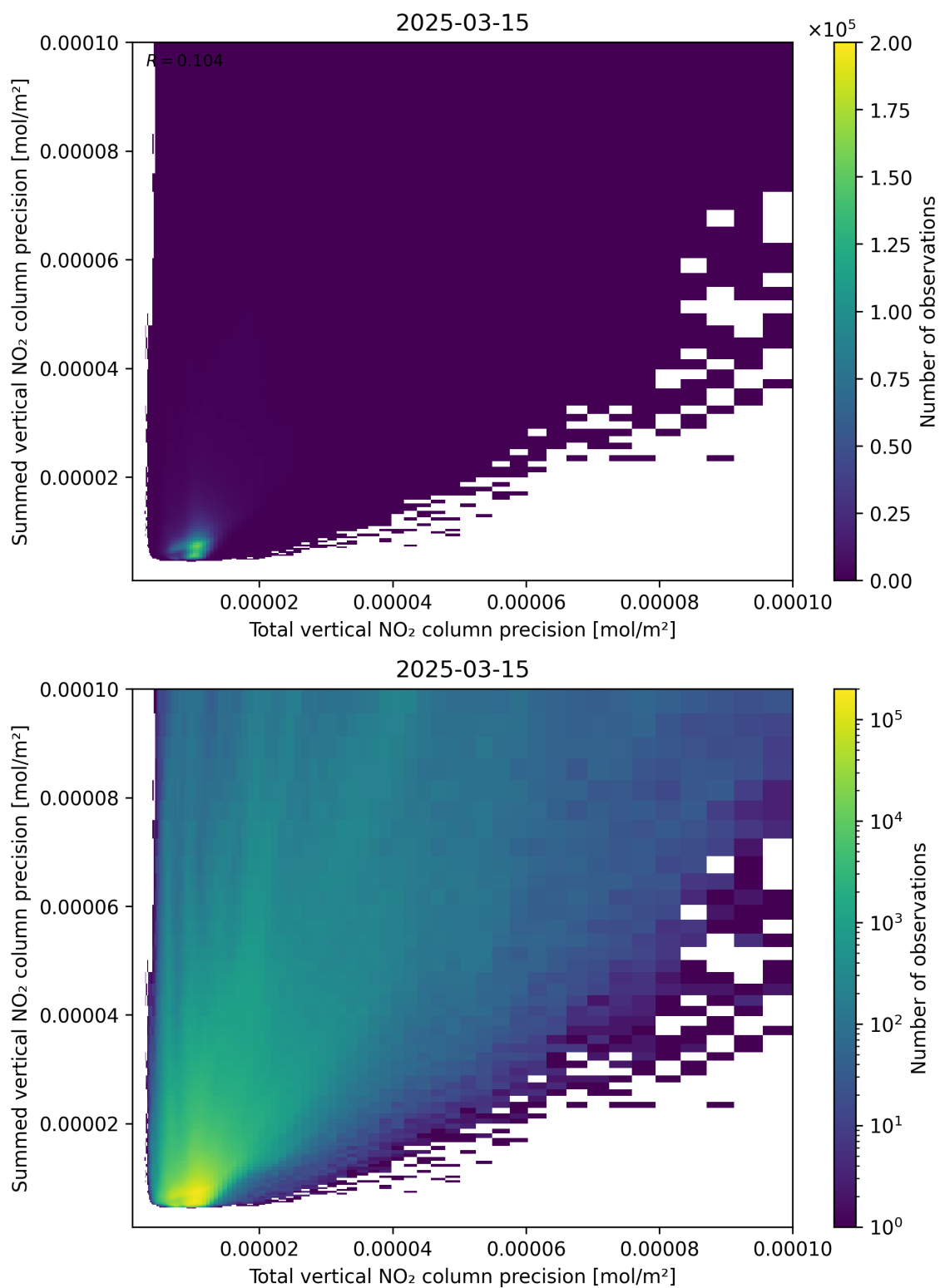
Figure 118: Scatter density plot of “Total vertical NO 2 column precision” against “Summed vertical NO 2 column precision” for 2025-03-15 to 2025-03-15.
