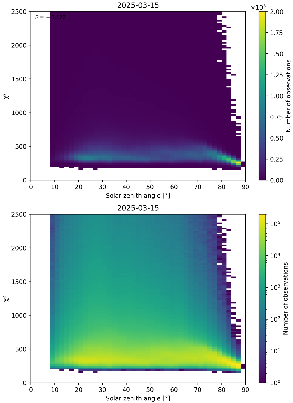
Figure 148: Scatter density plot of “Solar zenith angle” against “ \chi^2 ” for 2025-03-15 to 2025-03-15.
