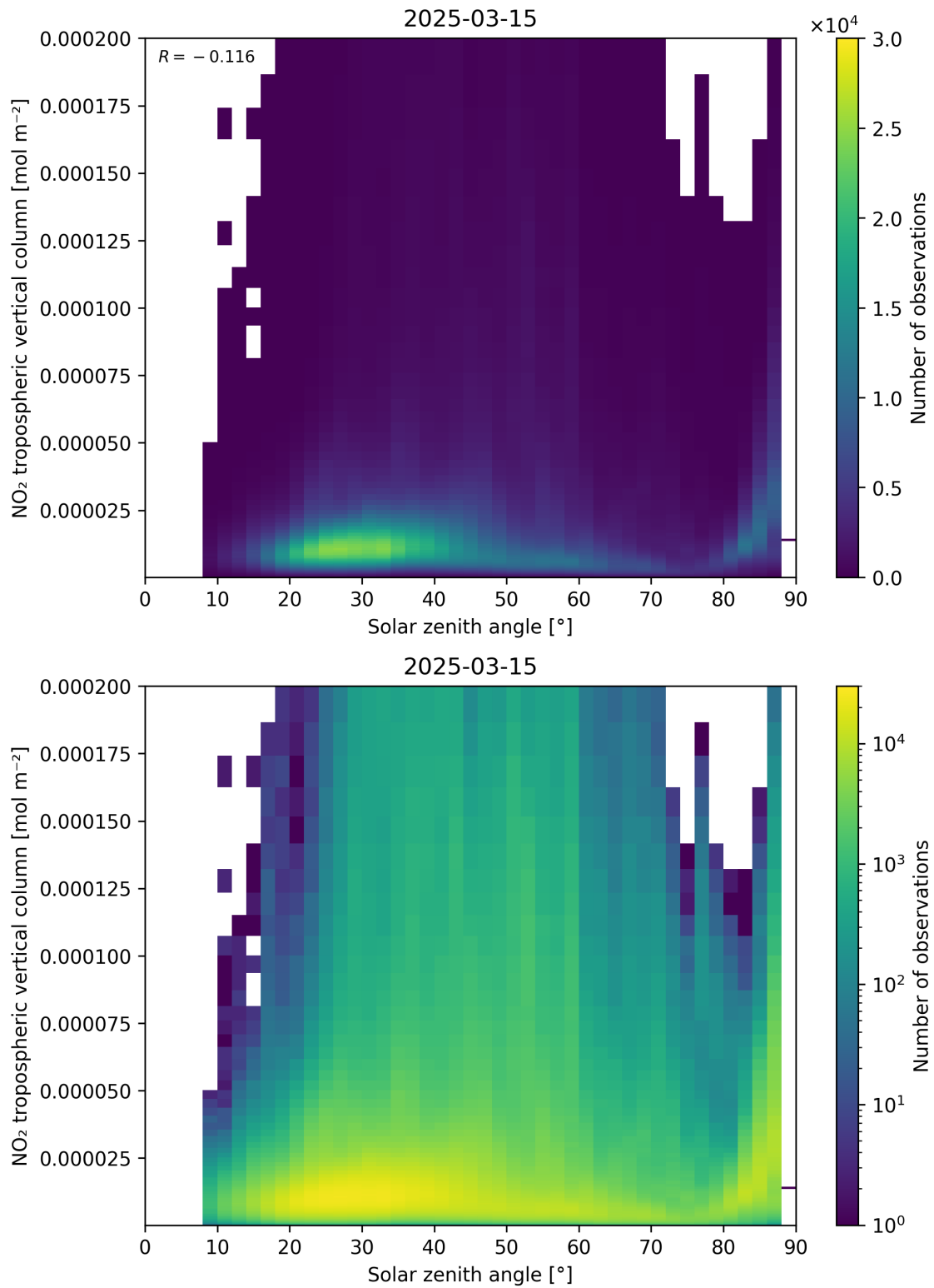
Figure 155: Scatter density plot of “Solar zenith angle” against “NO 2 tropospheric vertical column” for 2025-03-15 to 2025-03-15.
