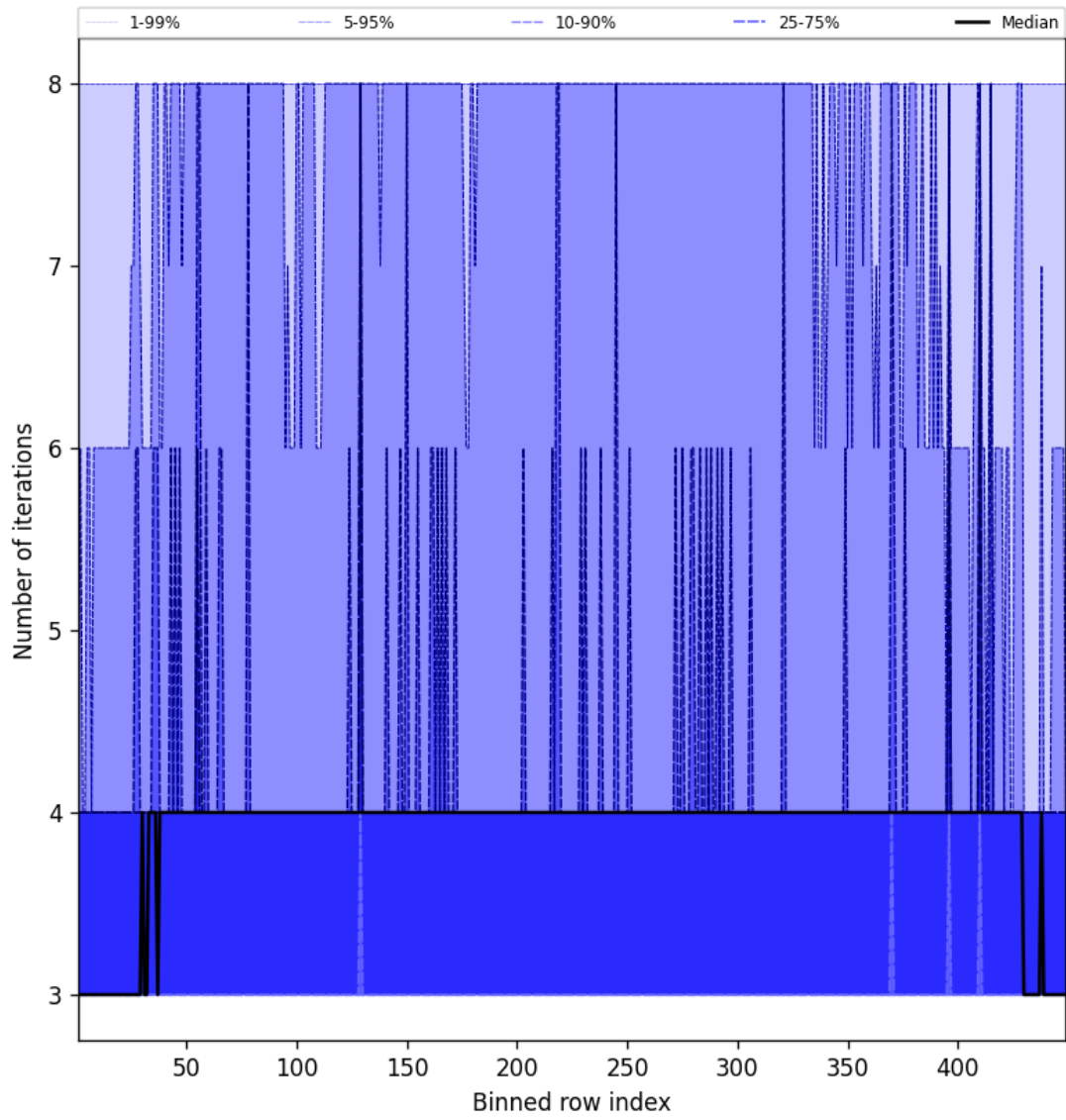
Figure 51: Along track statistics of “Number of iterations” for 2025-03-15 to 2025-03-15
