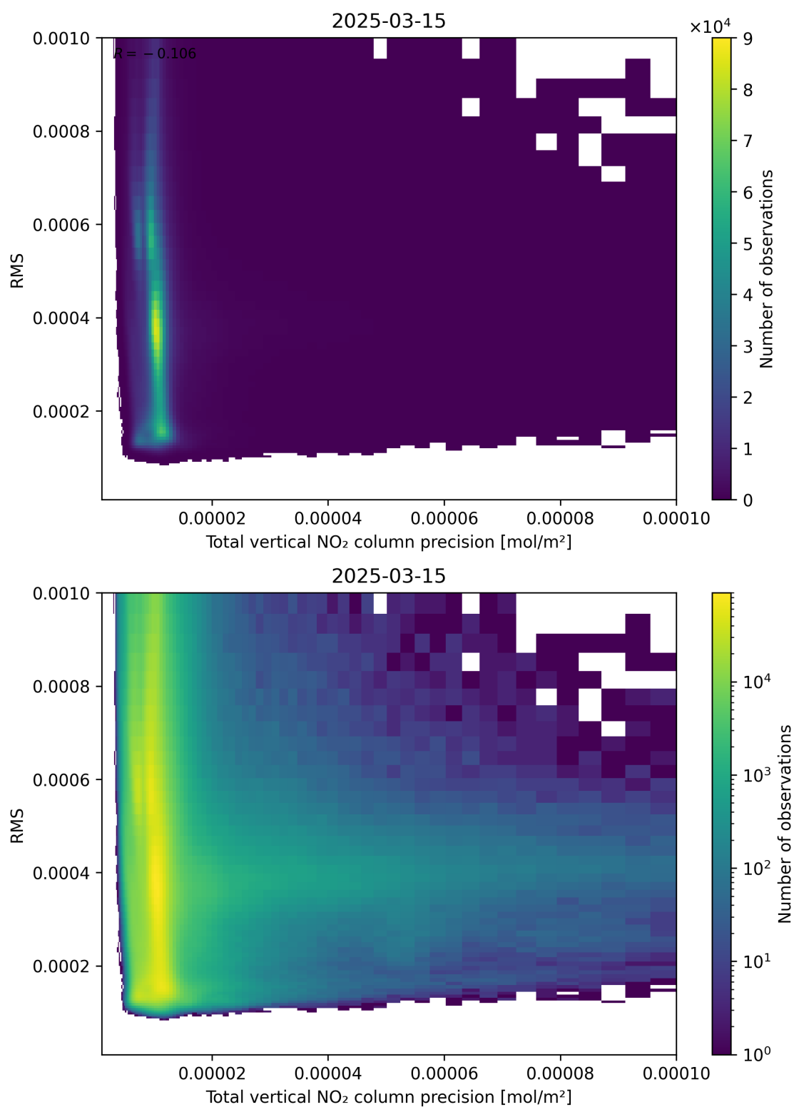
Figure 119: Scatter density plot of “Total vertical NO 2 column precision” against “RMS” for 2025-03-15 to 2025-03-15.
