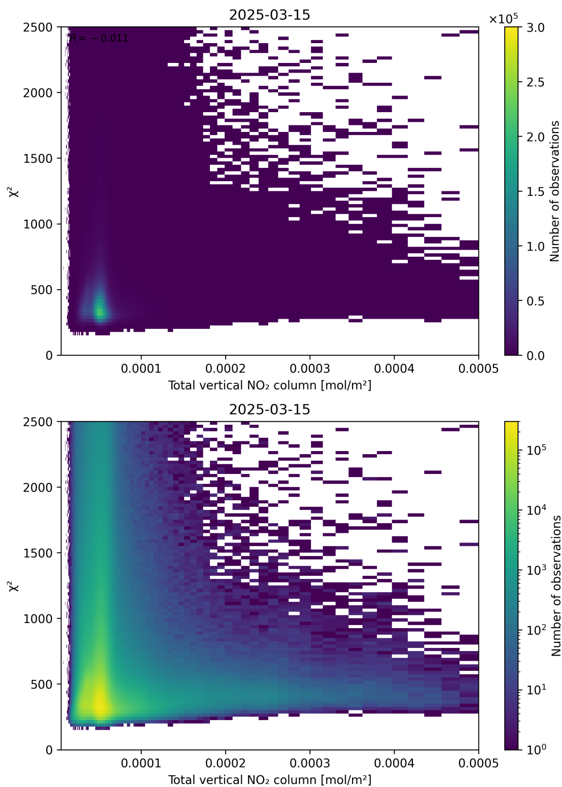
Figure 111: Scatter density plot of “Total vertical NO 2 column” against “ \chi^2 ” for 2025-03-15 to 2025-03-15.
