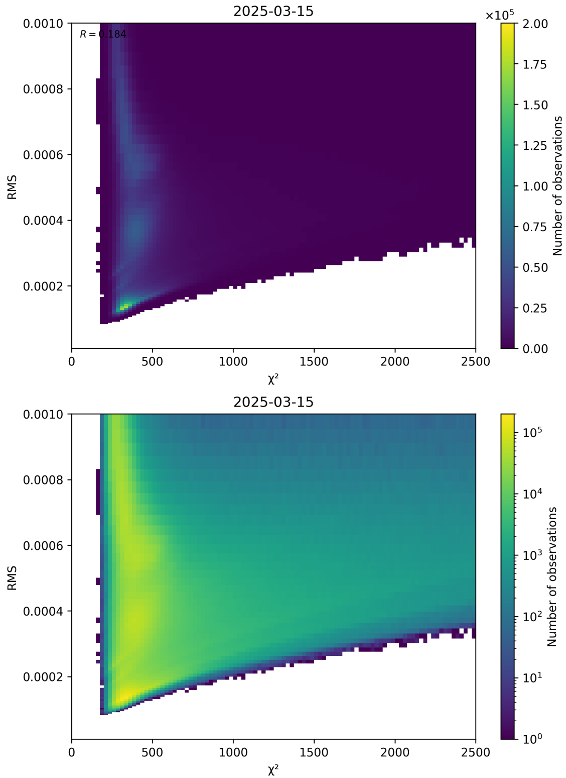
Figure 82: Scatter density plot of “ \chi^2 ” against “RMS” for 2025-03-15 to 2025-03-15.
