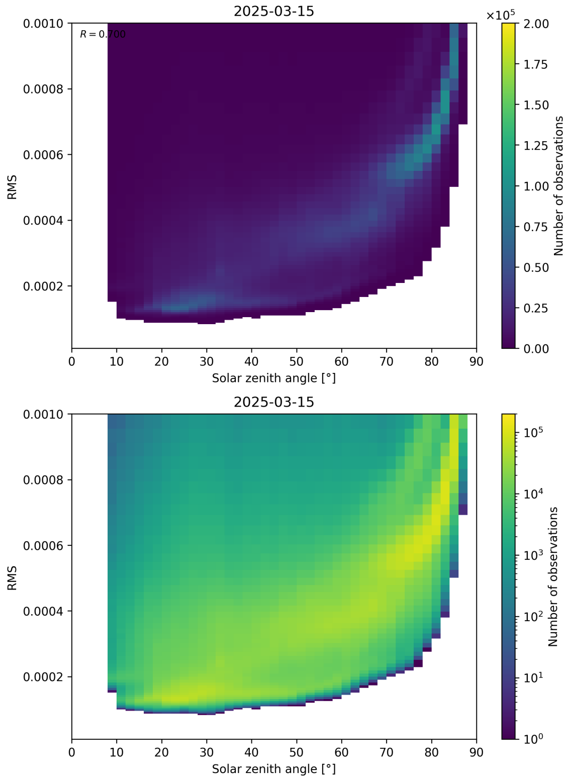
Figure 157: Scatter density plot of “Solar zenith angle” against “RMS” for 2025-03-15 to 2025-03-15.
