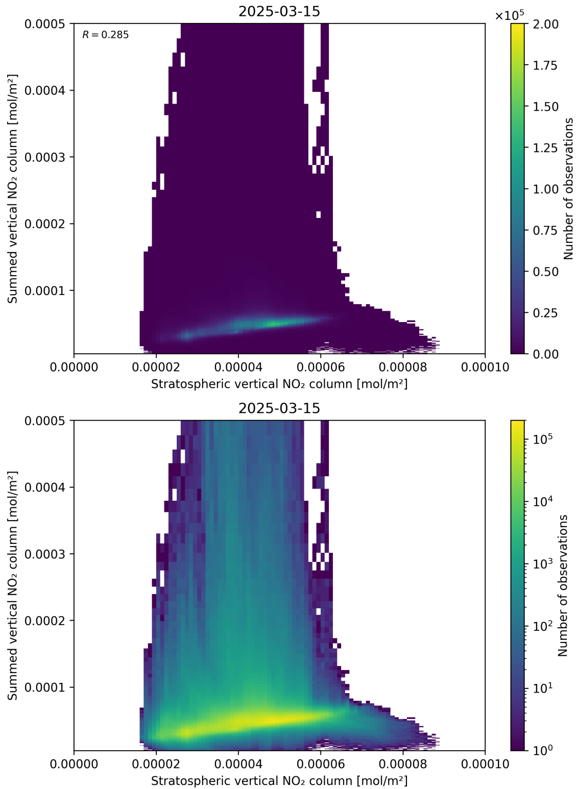
Figure 98: Scatter density plot of “Stratospheric vertical NO 2 column” against “Summed vertical NO 2 column” for 2025-03-15 to 2025-03-15.
