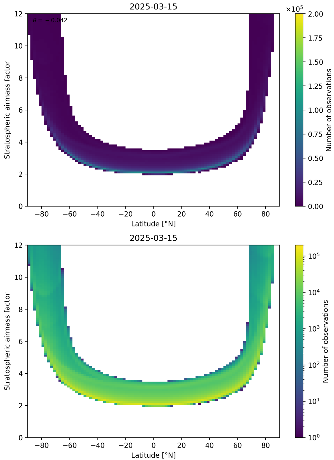
Figure 83: Scatter density plot of “Latitude” against “Stratospheric airmass factor” for 2025-03-15 to 2025-03-15.
