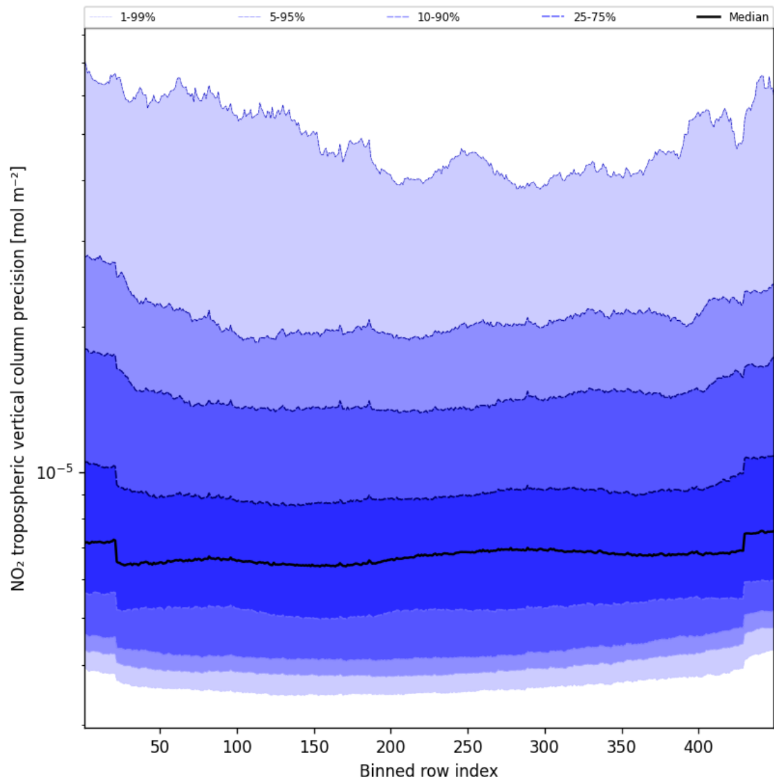
Figure 47: Along track statistics of “NO 2 tropospheric vertical column precision” for 2025-03-15 to 2025-03-15
