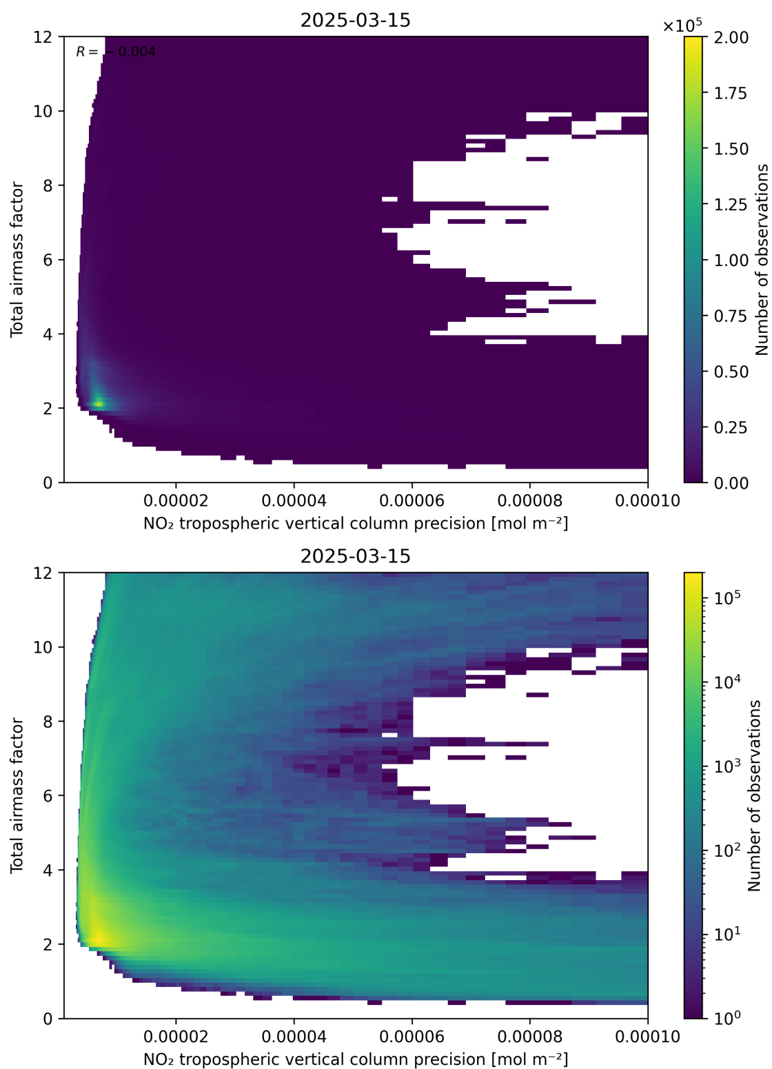
Figure 132: Scatter density plot of “NO 2 tropospheric vertical column precision” against “Total airmass factor” for 2025-03-15 to 2025-03-15.
