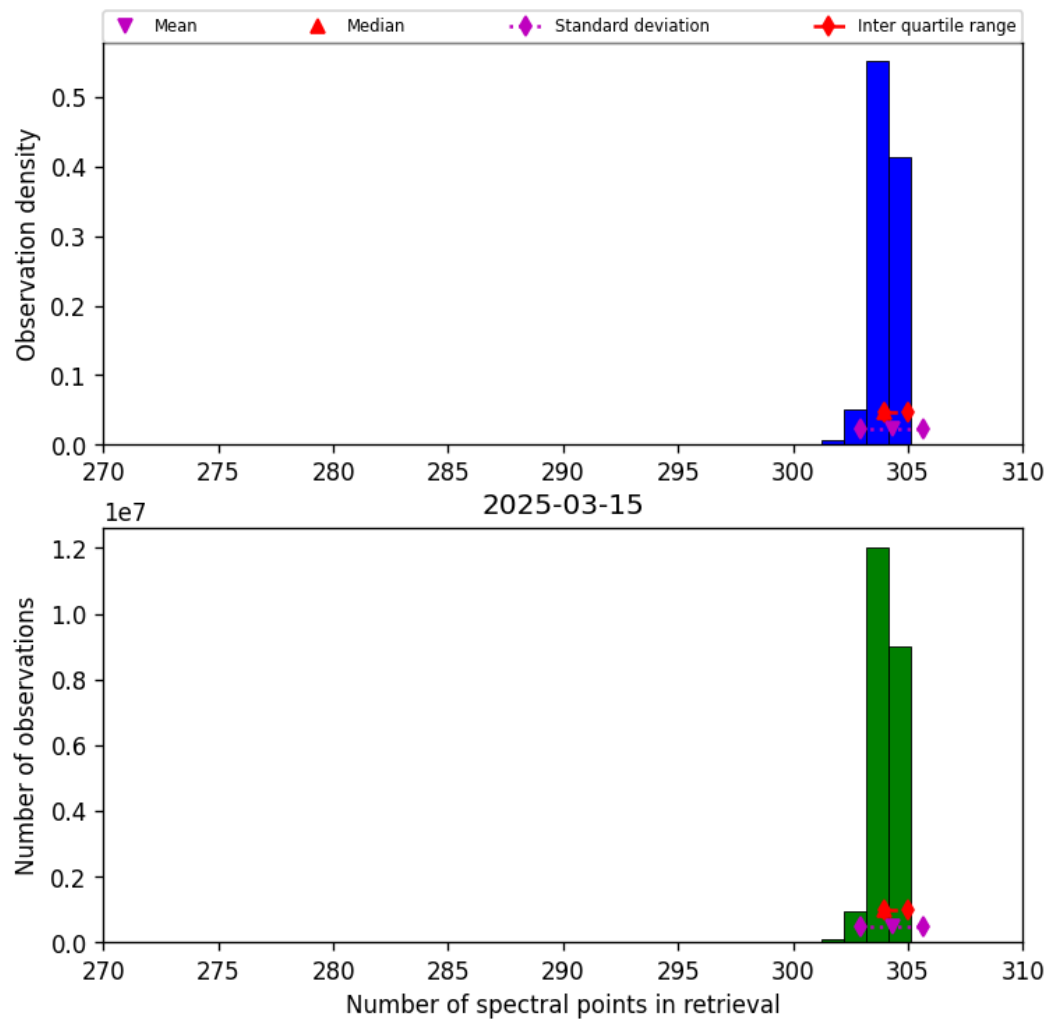
Figure 33: Histogram of “Number of spectral points in retrieval” for 2025-03-15 to 2025-03-15
