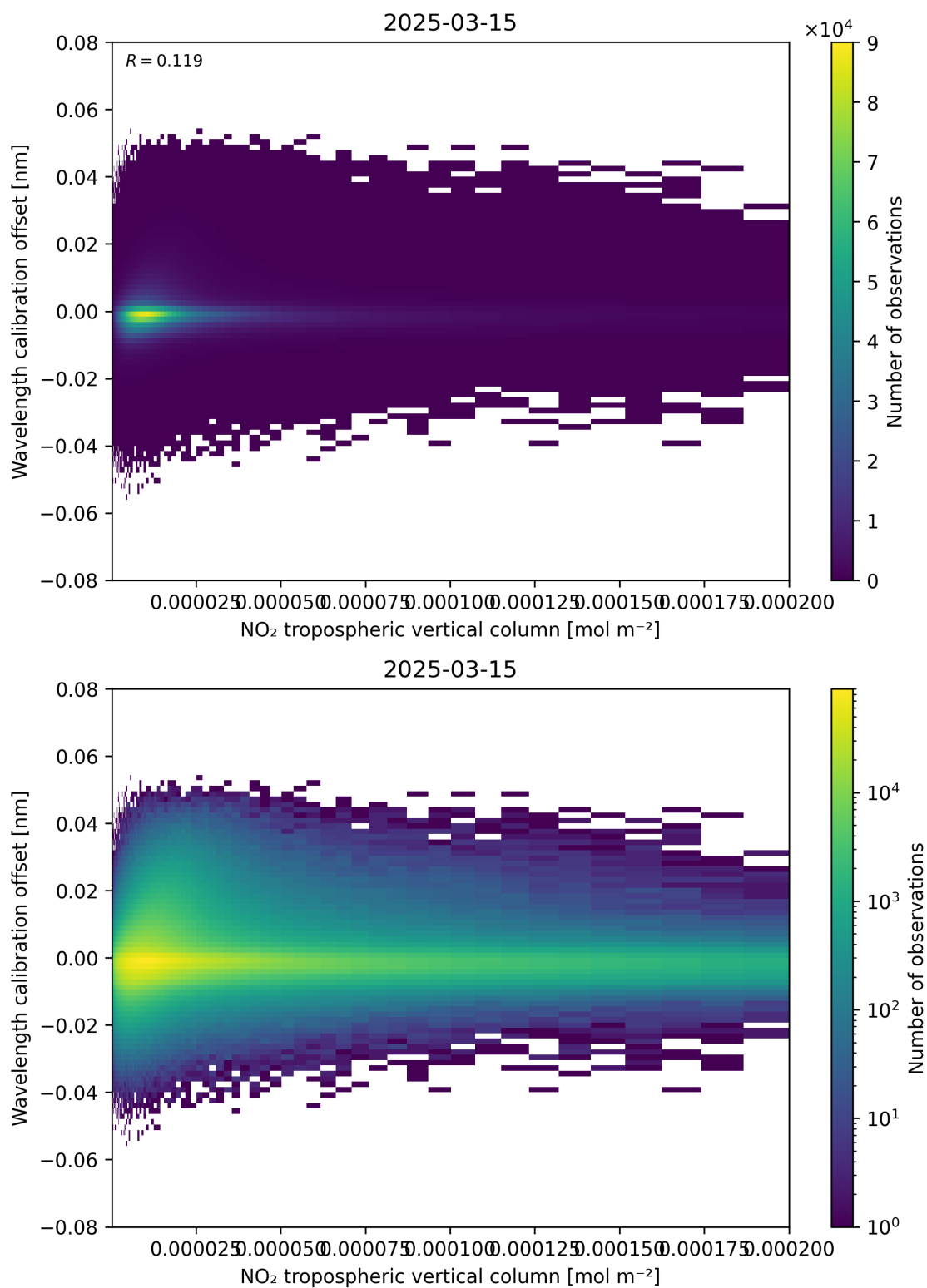
Figure 143: Scatter density plot of “NO 2 tropospheric vertical column” against “Wavelength calibration offset” for 2025-03-15 to 2025-03-15.
