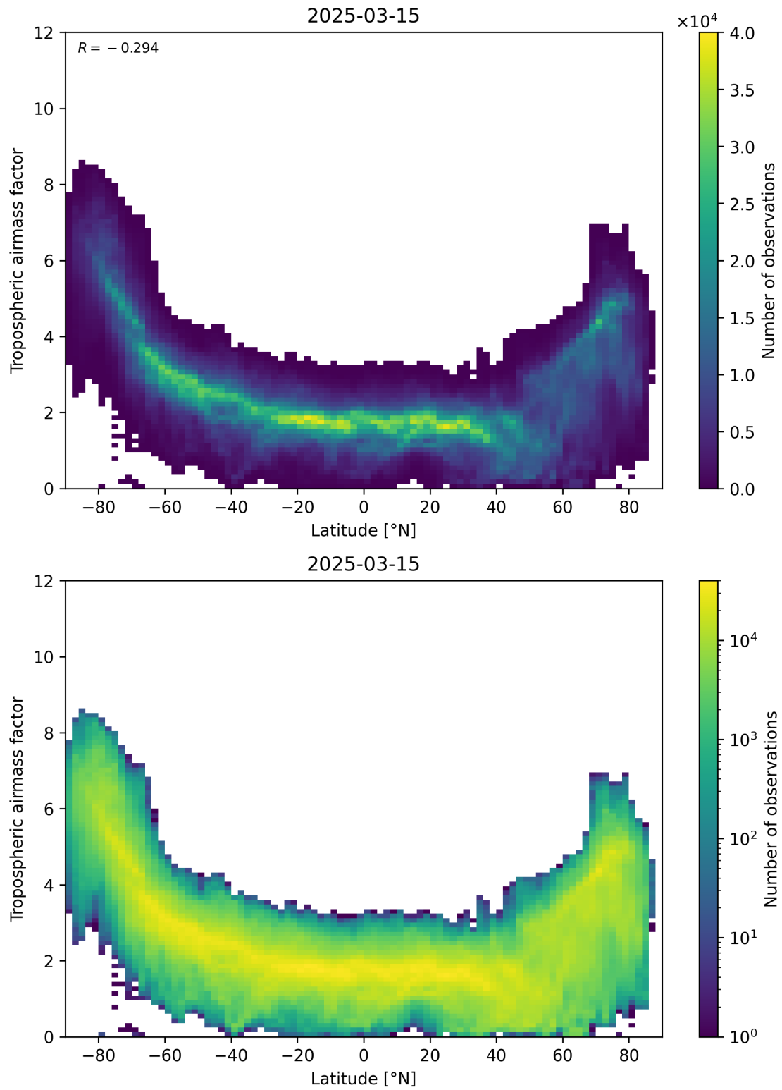
Figure 85: Scatter density plot of “Latitude” against “Tropospheric airmass factor” for 2025-03-15 to 2025-03-15.
