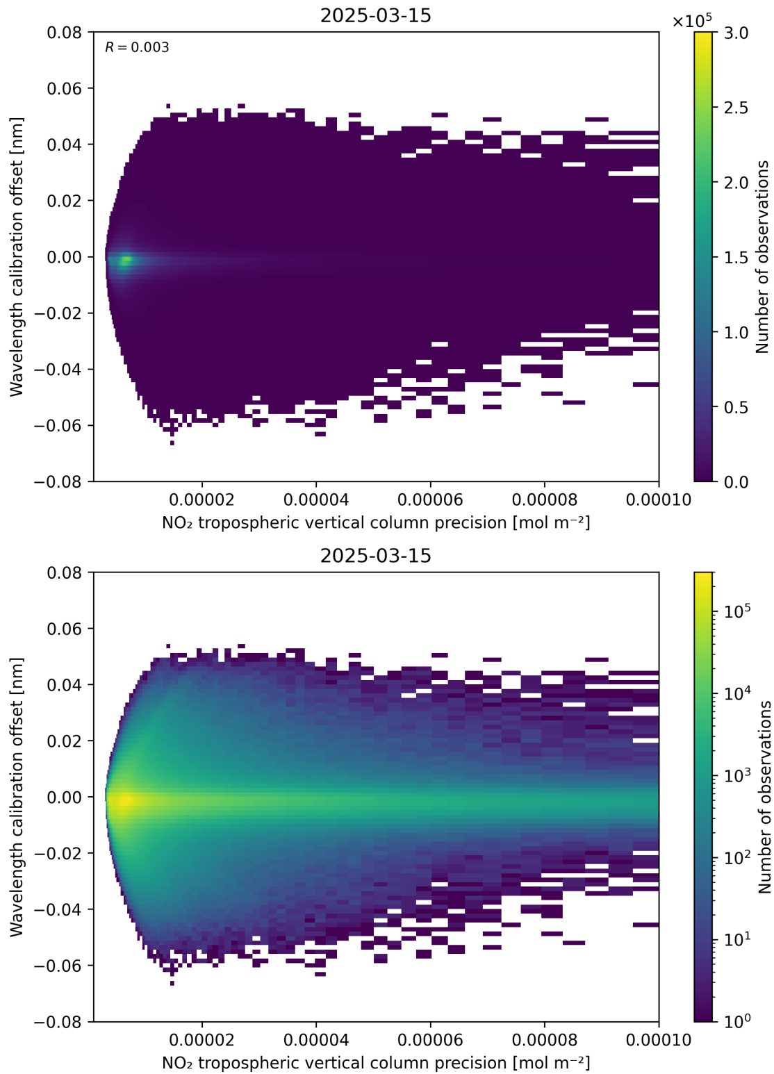
Figure 141: Scatter density plot of “NO 2 tropospheric vertical column precision” against “Wavelength calibration offset” for 2025-03-15 to 2025-03-15.
