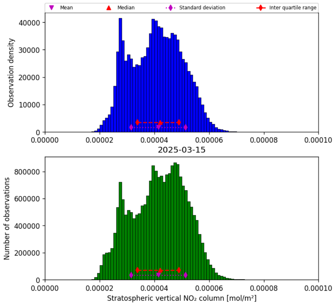
Figure 36: Histogram of “Stratospheric vertical NO 2 column” for 2025-03-15 to 2025-03-15
