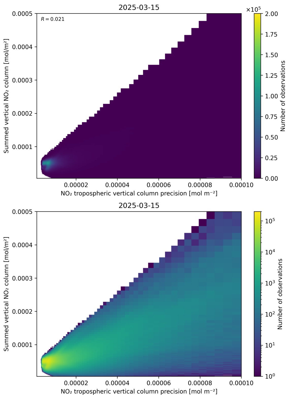
Figure 136: Scatter density plot of “NO 2 tropospheric vertical column precision” against “Summed vertical NO 2 column” for 2025-03-15 to 2025-03-15.
