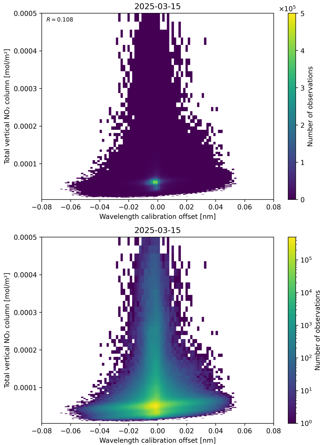
Figure 179: Scatter density plot of “Wavelength calibration offset” against “Total vertical NO 2 column” for 2025-03-15 to 2025-03-15.
