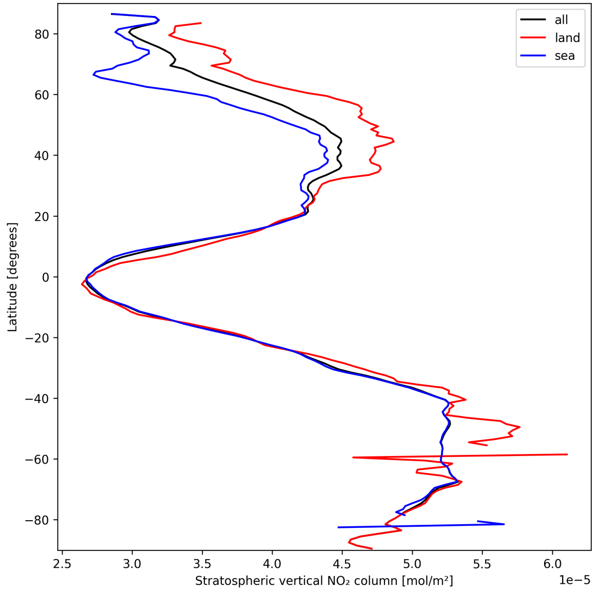
Figure 19: Zonal average of “Stratospheric vertical NO 2 column” for 2025-03-15 to 2025-03-15.
