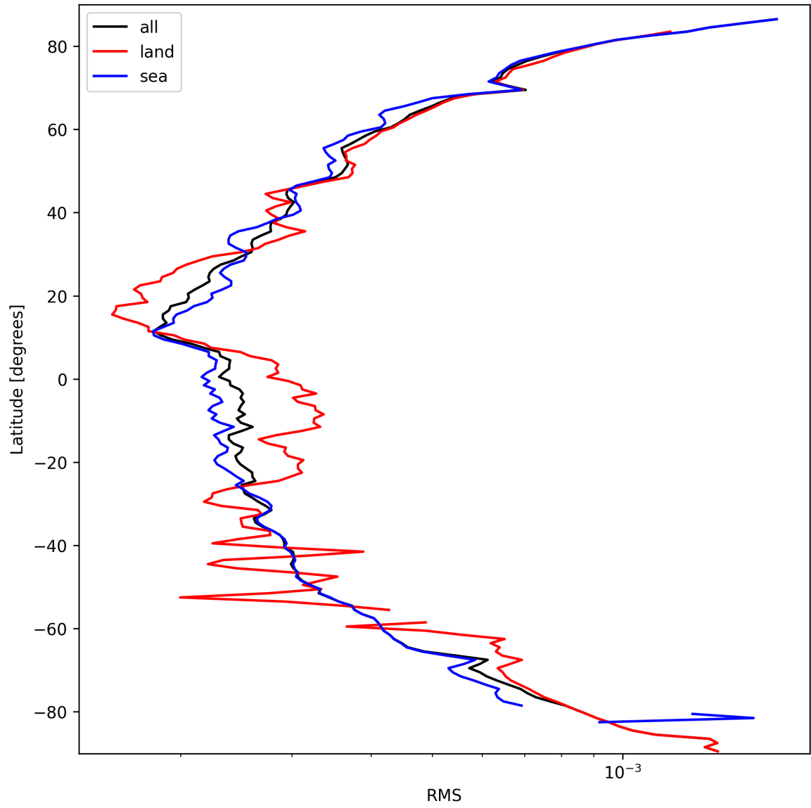
Figure 26: Zonal average of “RMS” for 2025-03-15 to 2025-03-15.
