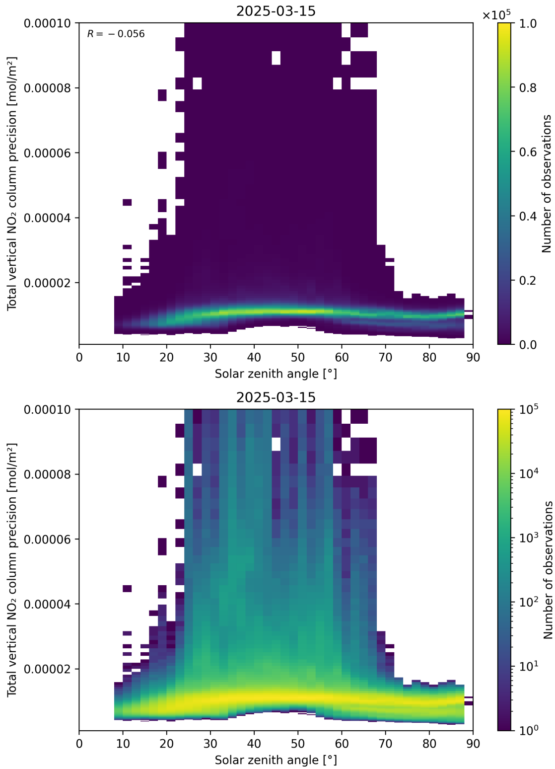
Figure 154: Scatter density plot of “Solar zenith angle” against “Total vertical NO 2 column precision” for 2025-03-15 to 2025-03-15.
