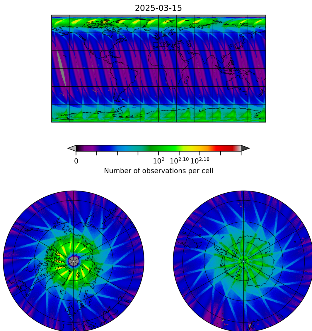
Figure 10: Map of the number of observations for 2025-03-15 to 2025-03-15
