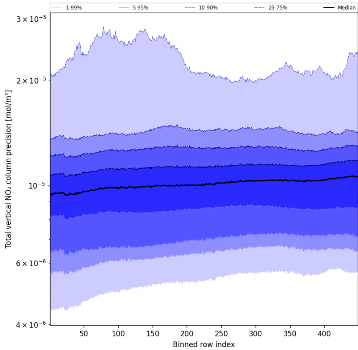
Figure 56: Along track statistics of “Total vertical NO 2 column precision” for 2025-03-15 to 2025-03-15
