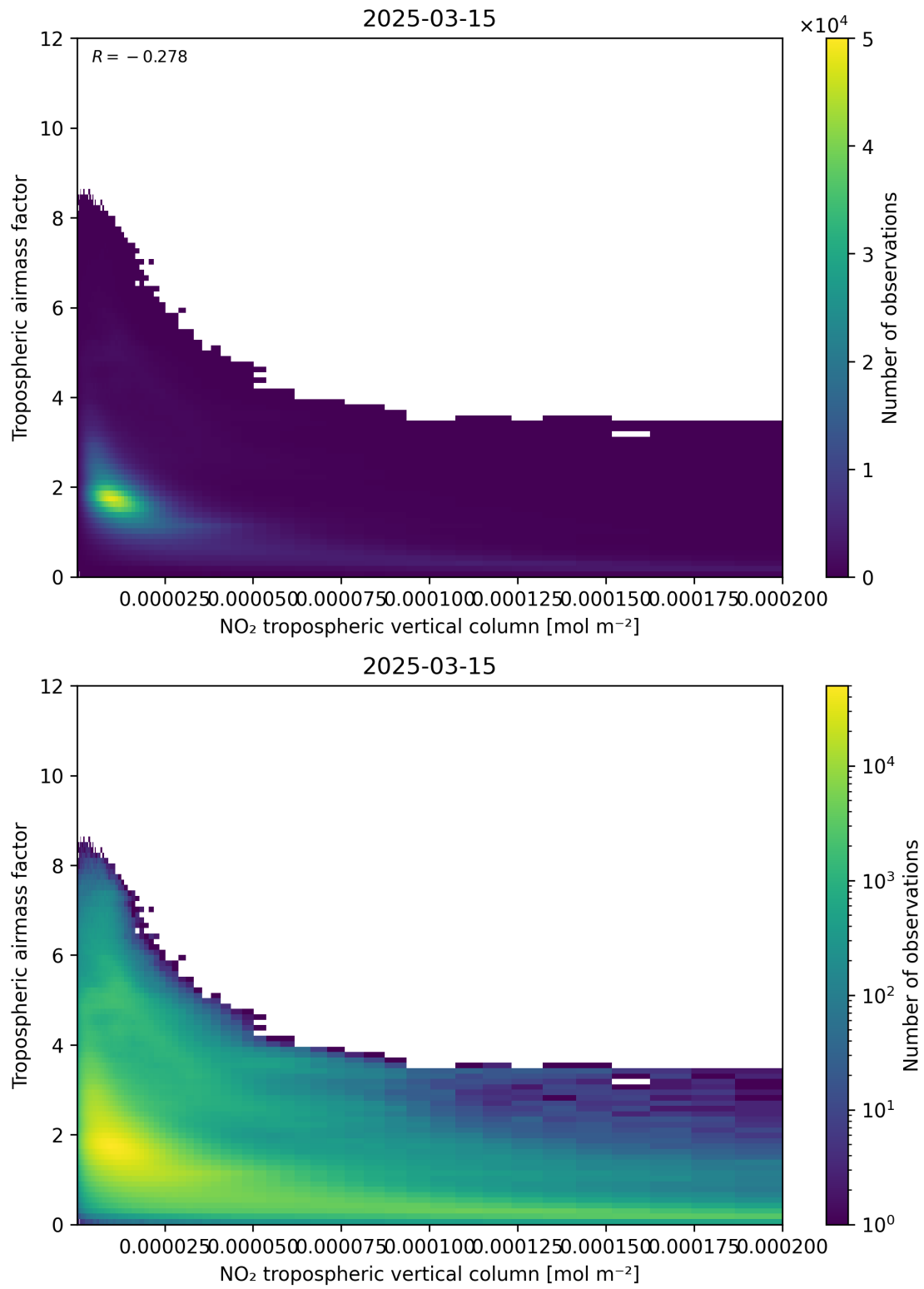
Figure 123: Scatter density plot of “NO 2 tropospheric vertical column” against “Tropospheric air mass factor” for 2025-03-15 to 2025-03-15.
