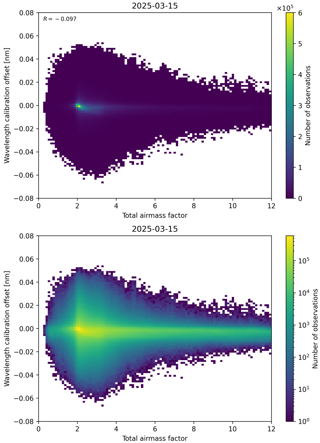
Figure 70: Scatter density plot of “Total airmass factor” against “Wavelength calibration offset” for 2025-03-15 to 2025-03-15.
