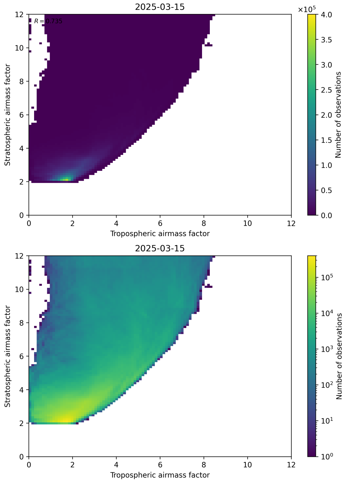
Figure 71: Scatter density plot of “Tropospheric airmass factor” against “Stratospheric airmass factor” for 2025-03-15 to 2025-03-15.
