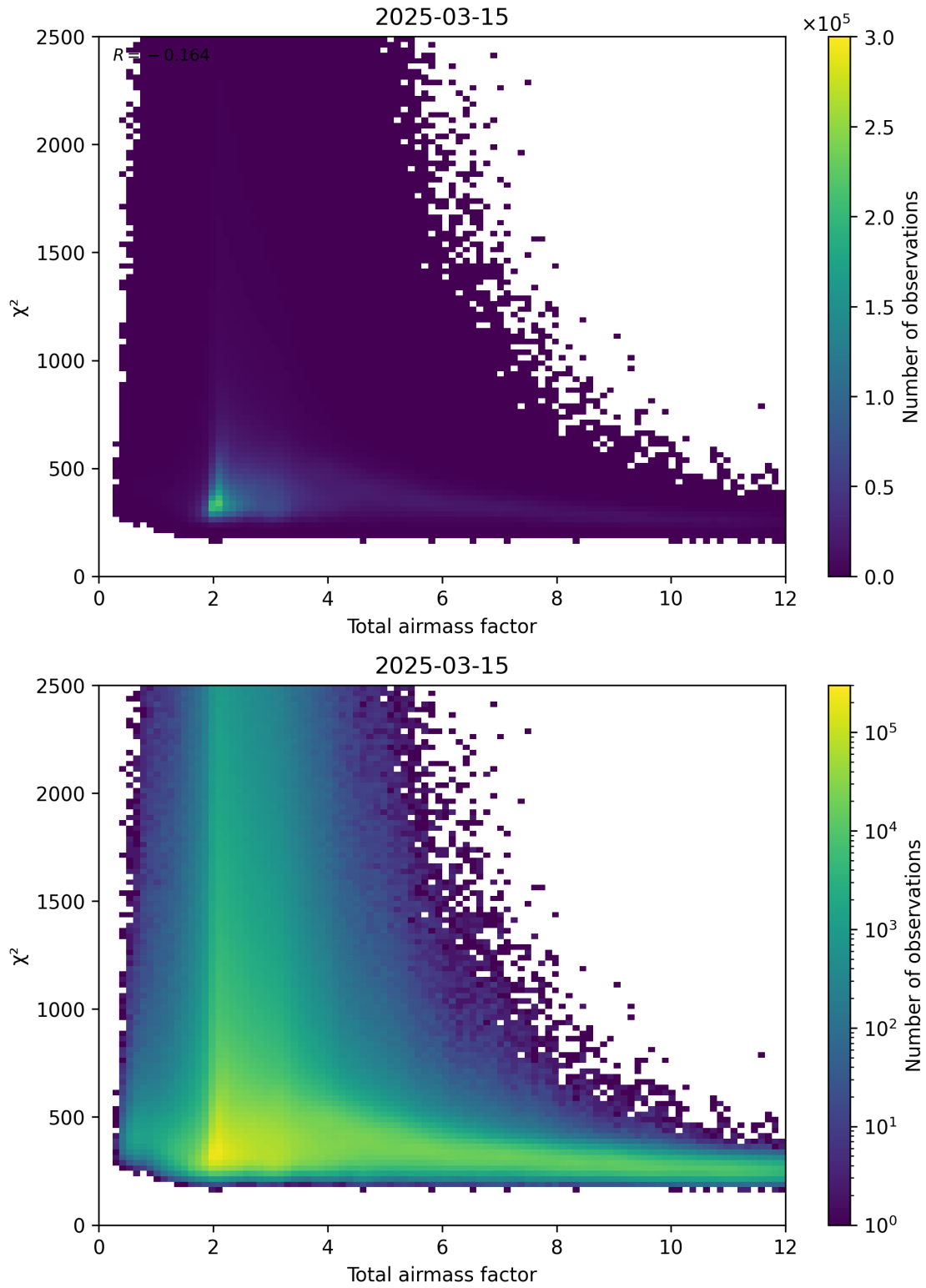
Figure 63: Scatter density plot of “Total airmass factor” against “ \chi^2 ” for 2025-03-15 to 2025-03-15.
