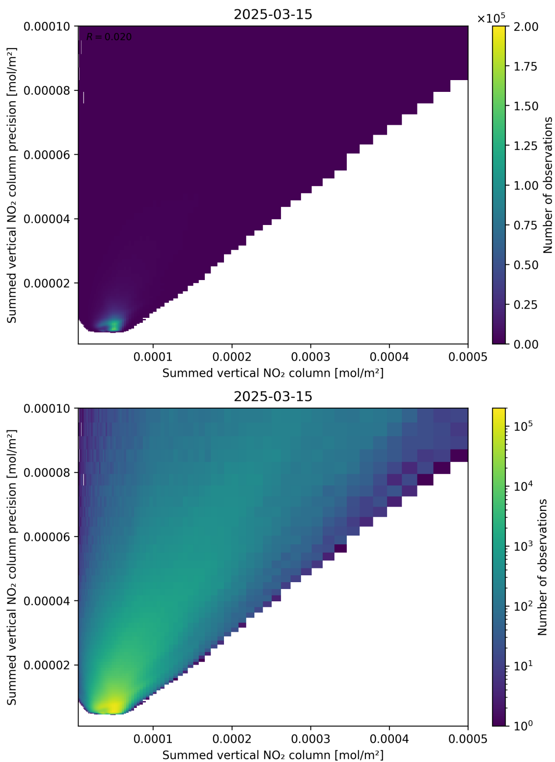
Figure 105: Scatter density plot of “Summed vertical NO 2 column” against “Summed vertical NO 2 column precision” for 2025-03-15 to 2025-03-15.
