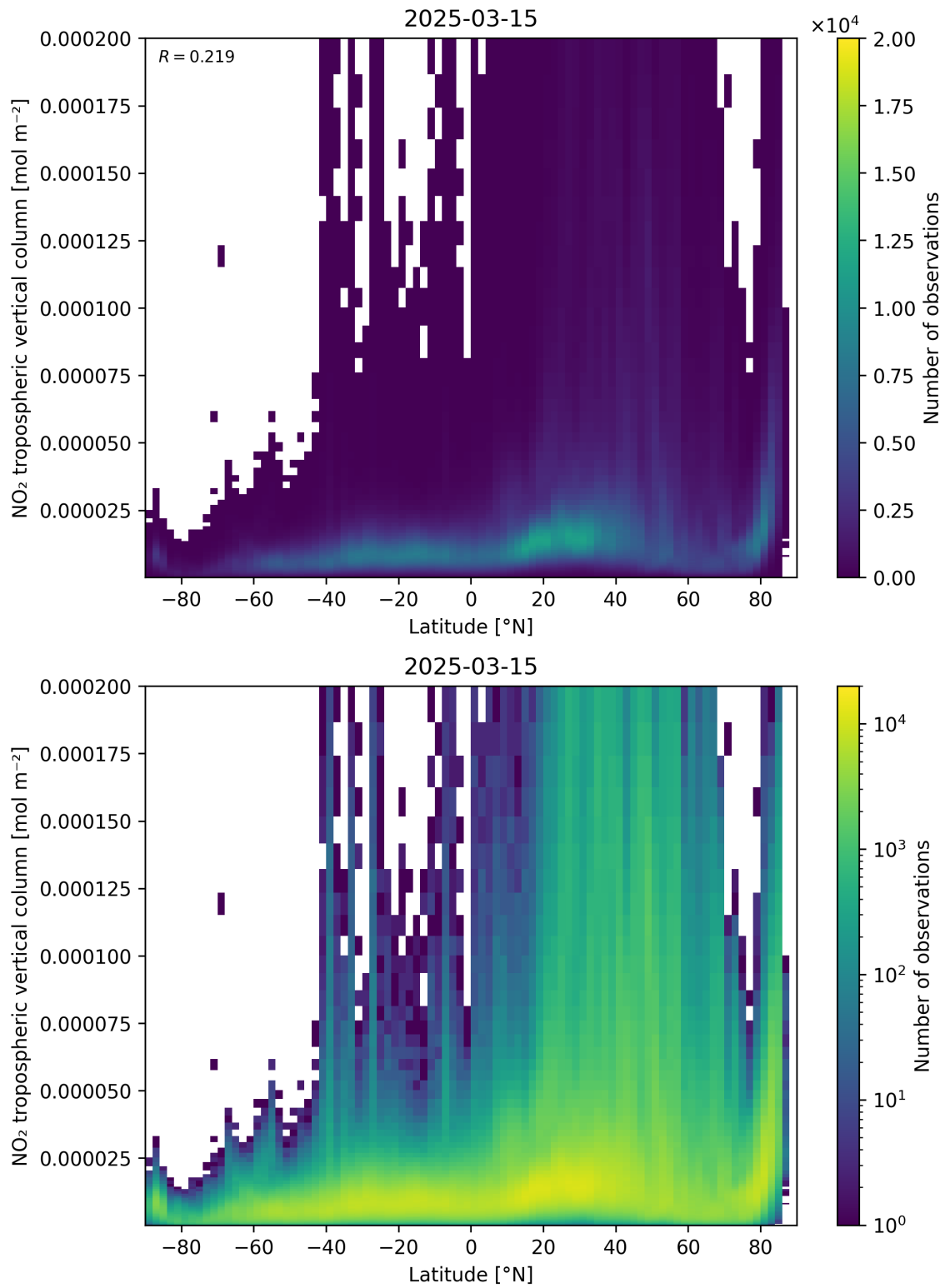
Figure 92: Scatter density plot of “Latitude” against “NO 2 tropospheric vertical column” for 2025-03-15 to 2025-03-15.
