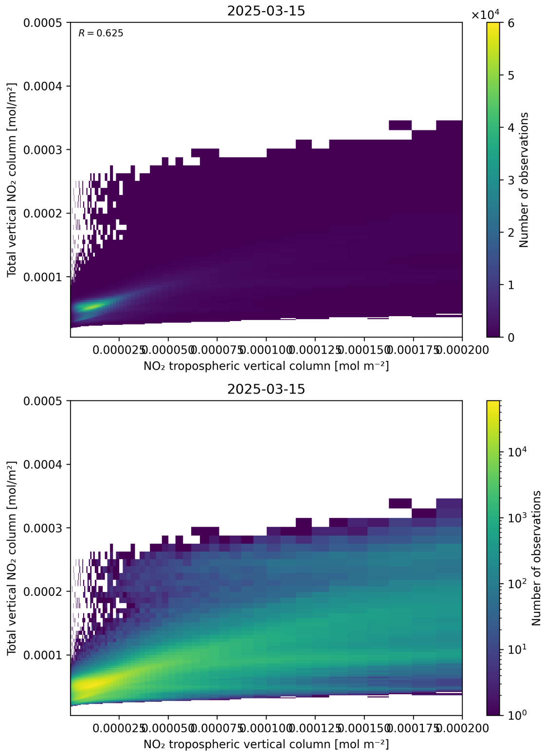
Figure 128: Scatter density plot of “NO 2 tropospheric vertical column” against “Total vertical NO 2 column” for 2025-03-15 to 2025-03-15.
