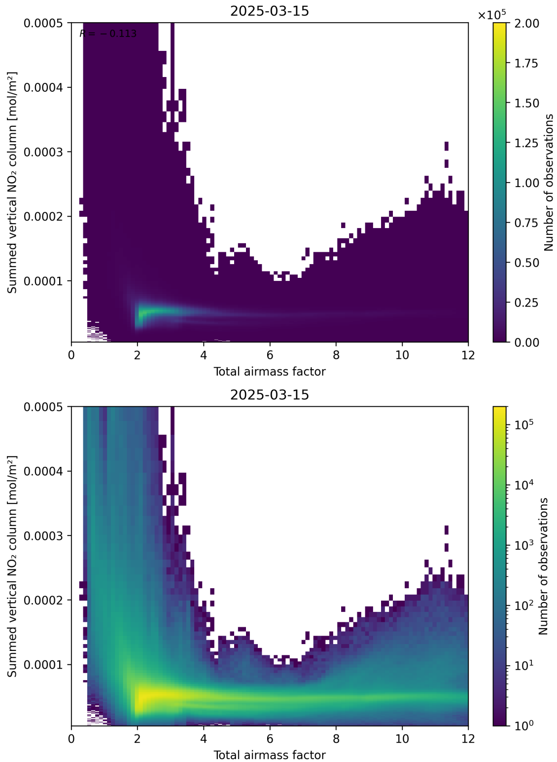
Figure 65: Scatter density plot of “Total airmass factor” against “Summed vertical NO 2 column” for 2025-03-15 to 2025-03-15.
