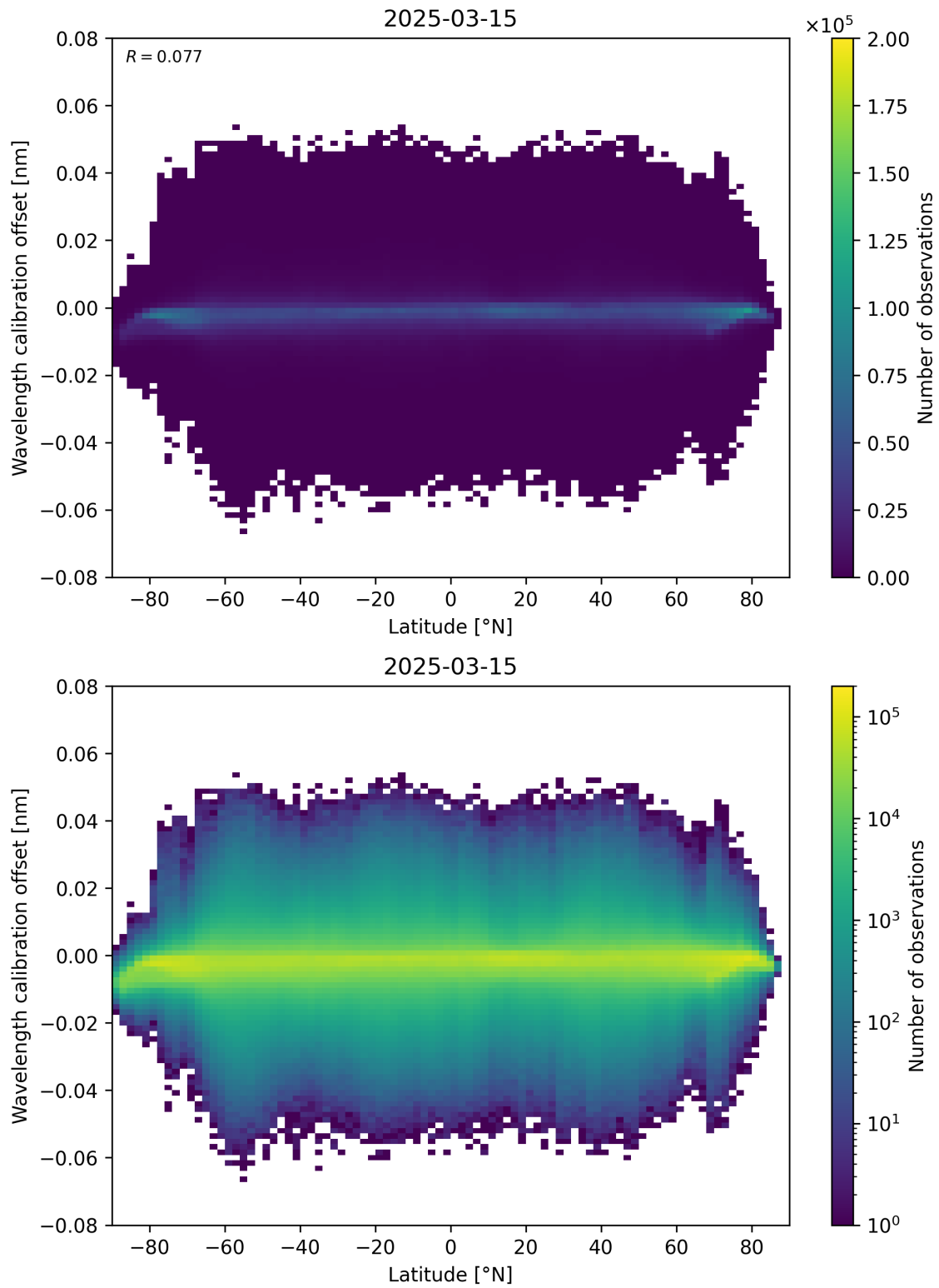
Figure 95: Scatter density plot of “Latitude” against “Wavelength calibration offset” for 2025-03-15 to 2025-03-15.
