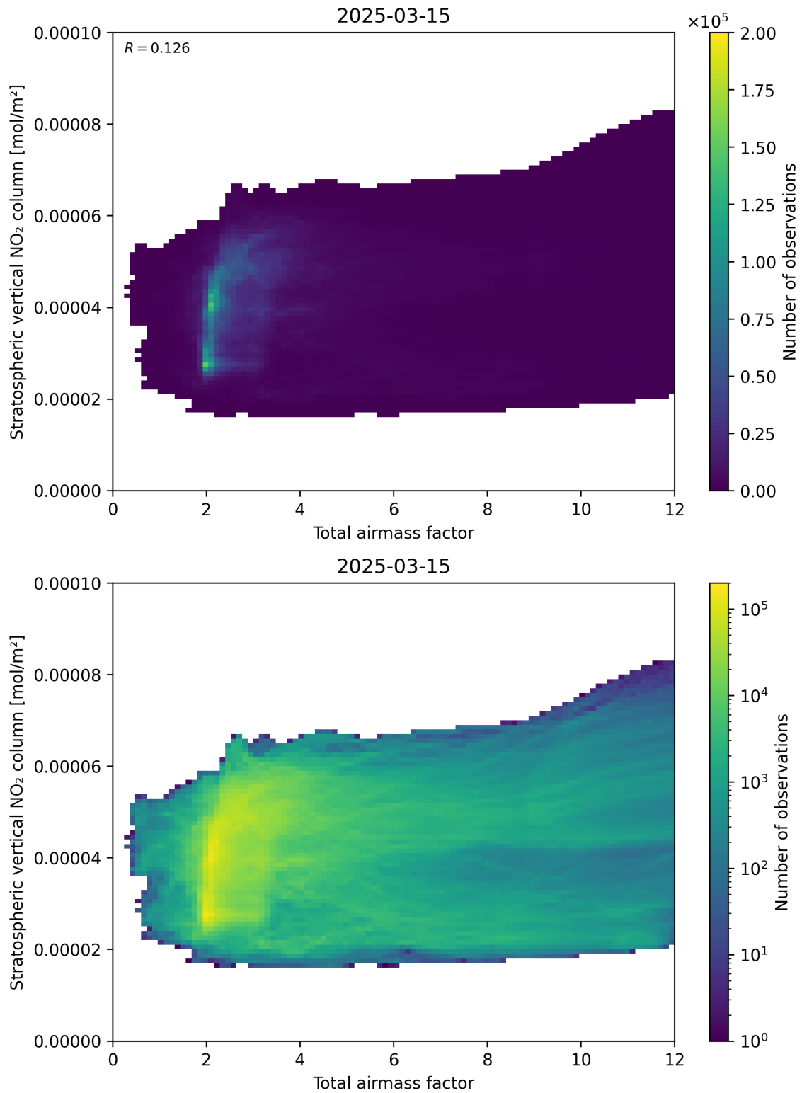
Figure 64: Scatter density plot of “Total airmass factor” against “Stratospheric vertical NO 2 column” for 2025-03-15 to 2025-03-15.
