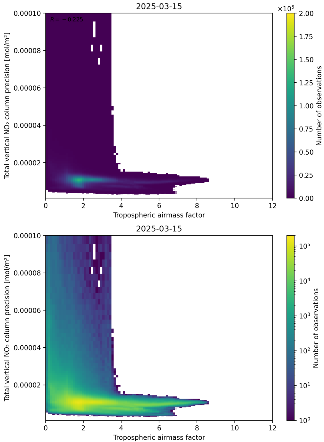
Figure 78: Scatter density plot of “Tropospheric air mass factor” against “Total vertical NO 2 column precision” for 2025-03-15 to 2025-03-15.
