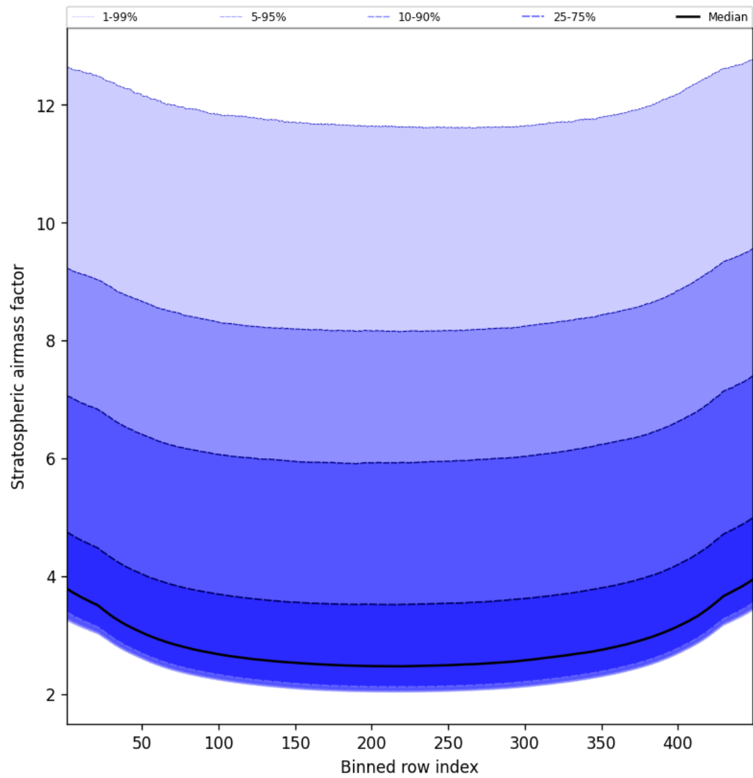
Figure 61: Along track statistics of “Stratospheric air mass factor” for 2025-03-15 to 2025-03-15
