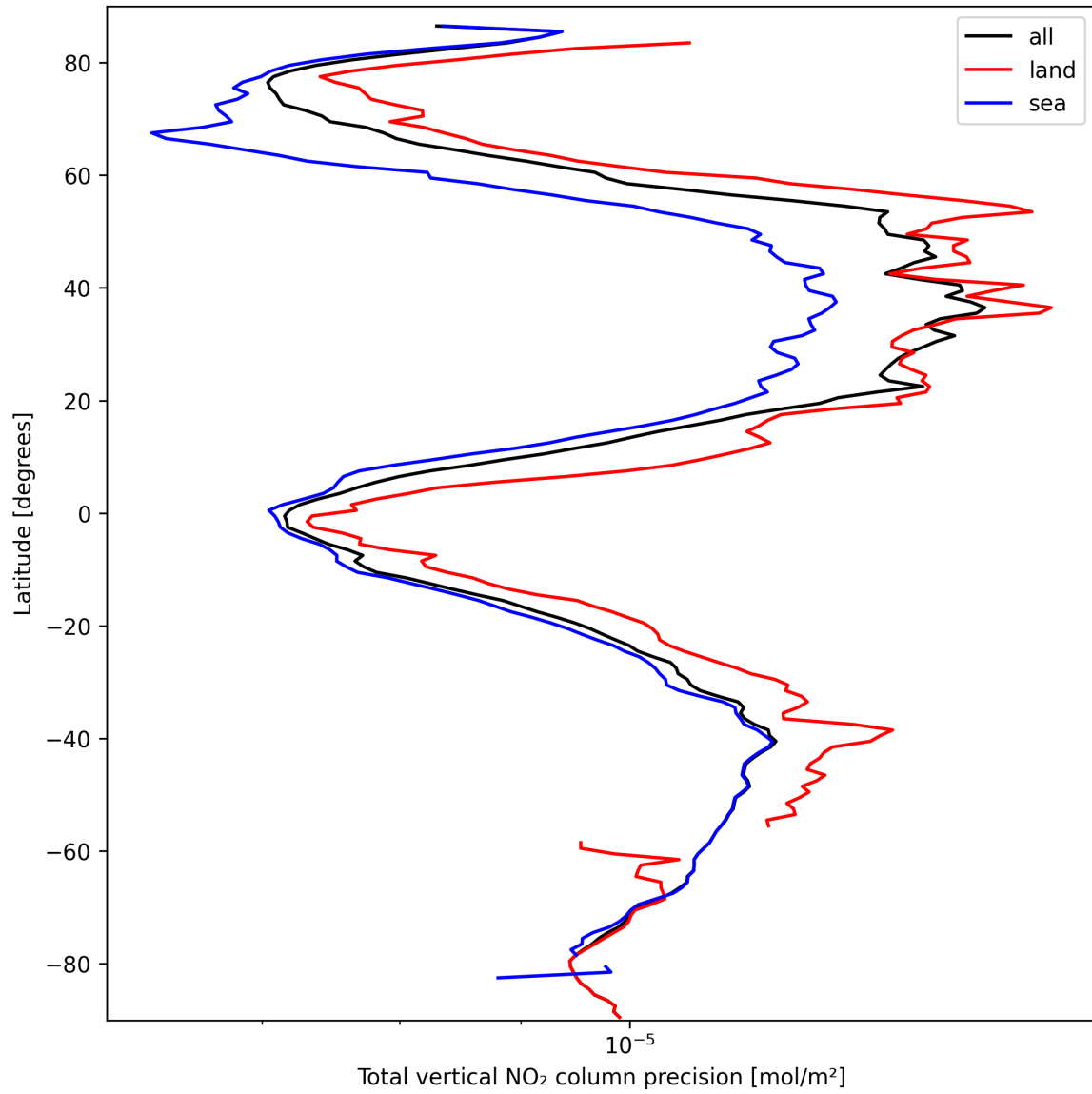
Figure 22: Zonal average of “Total vertical NO 2 column precision” for 2025-03-15 to 2025-03-15.
