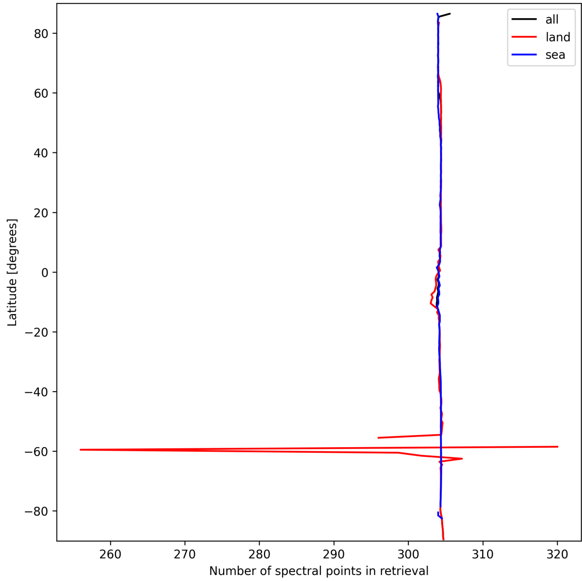
Figure 16: Zonal average of “Number of spectral points in retrieval” for 2025-03-15 to 2025-03-15.
