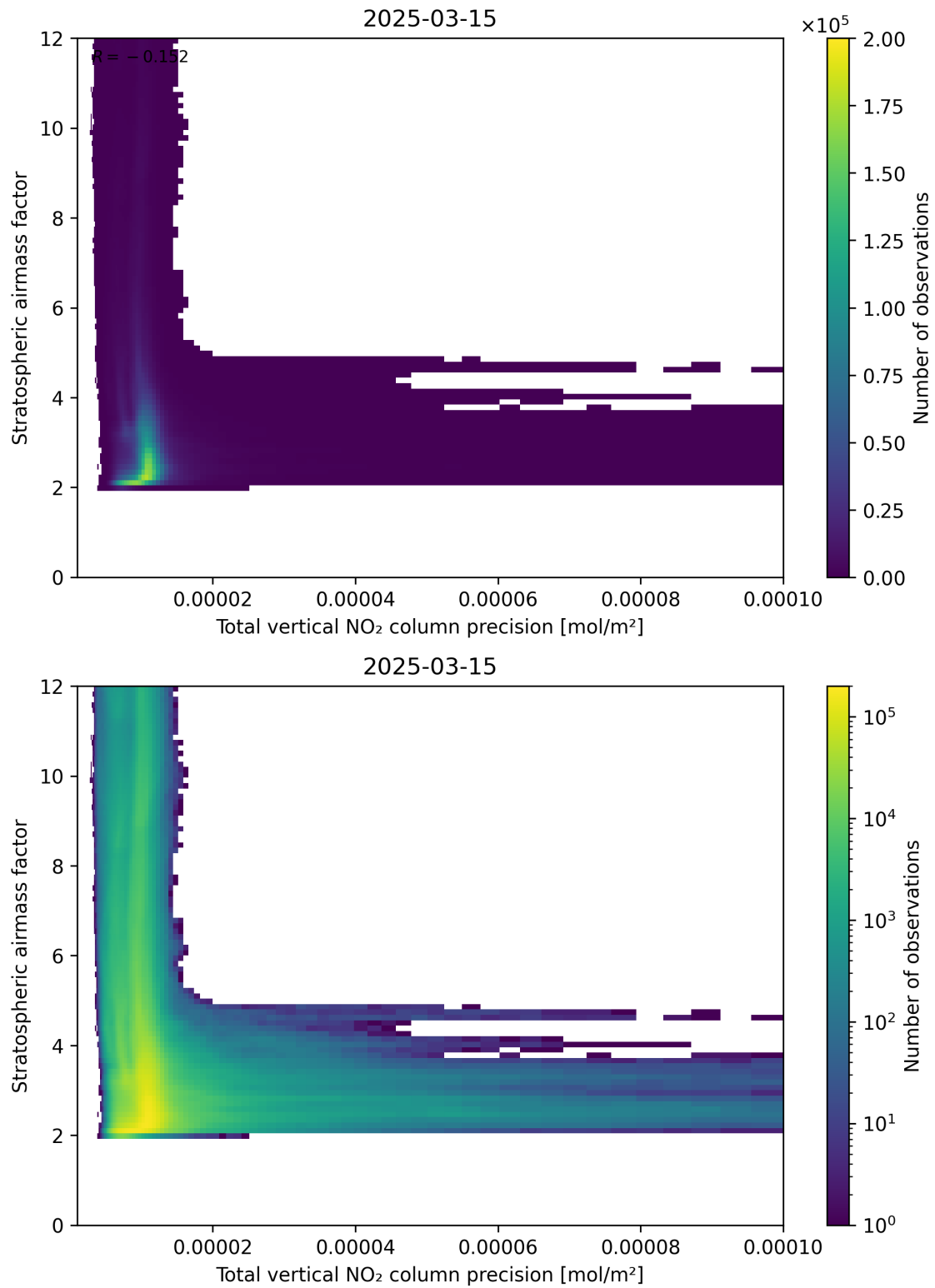
Figure 115: Scatter density plot of “Total vertical NO 2 column precision” against “Stratospheric air mass factor” for 2025-03-15 to 2025-03-15.
