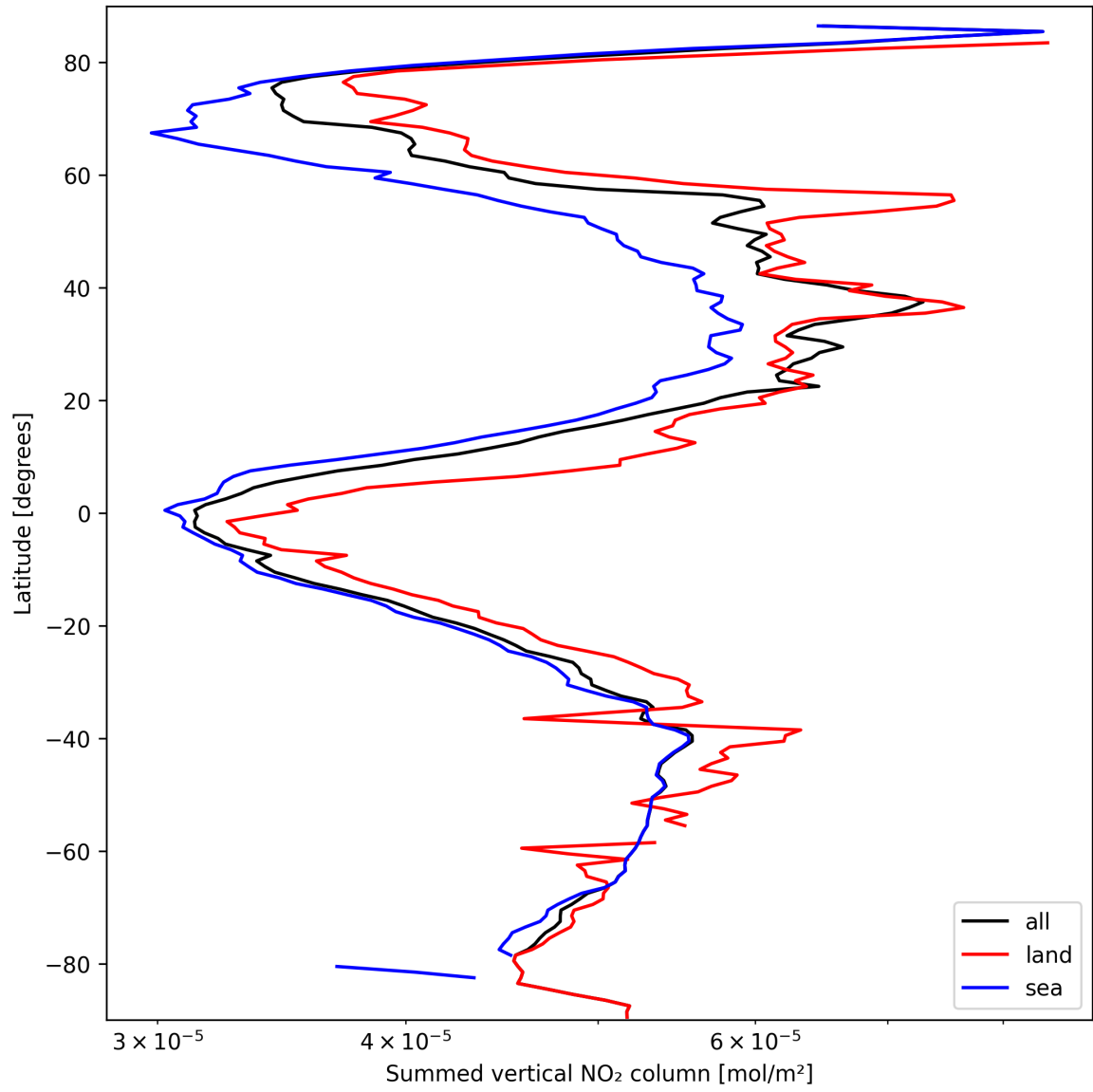
Figure 23: Zonal average of “Summed vertical NO 2 column” for 2025-03-15 to 2025-03-15.
