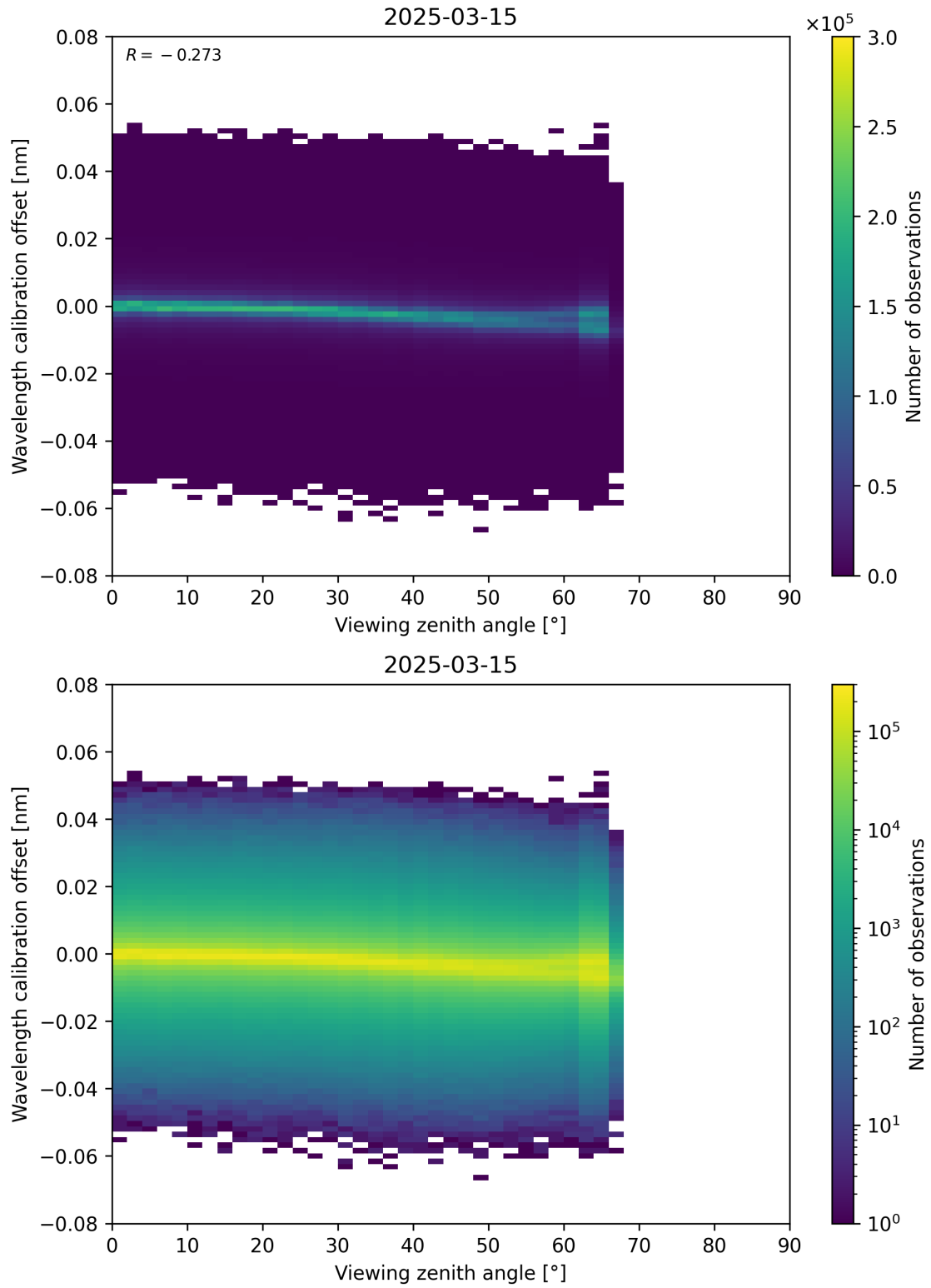
Figure 173: Scatter density plot of “Viewing zenith angle” against “Wavelength calibration offset” for 2025-03-15 to 2025-03-15.
