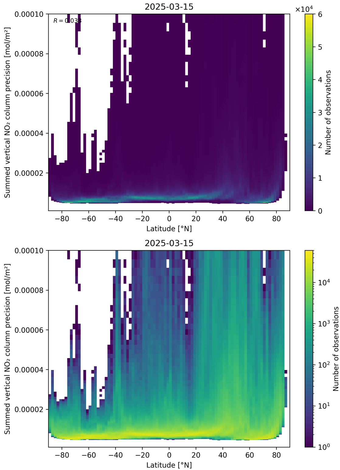
Figure 89: Scatter density plot of “Latitude” against “Summed vertical NO 2 column precision” for 2025-03-15 to 2025-03-15.
