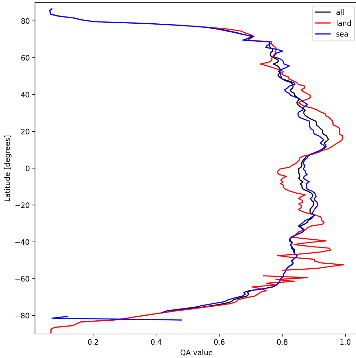
Figure 11: Zonal average of “QA value” for 2025-03-15 to 2025-03-15.
