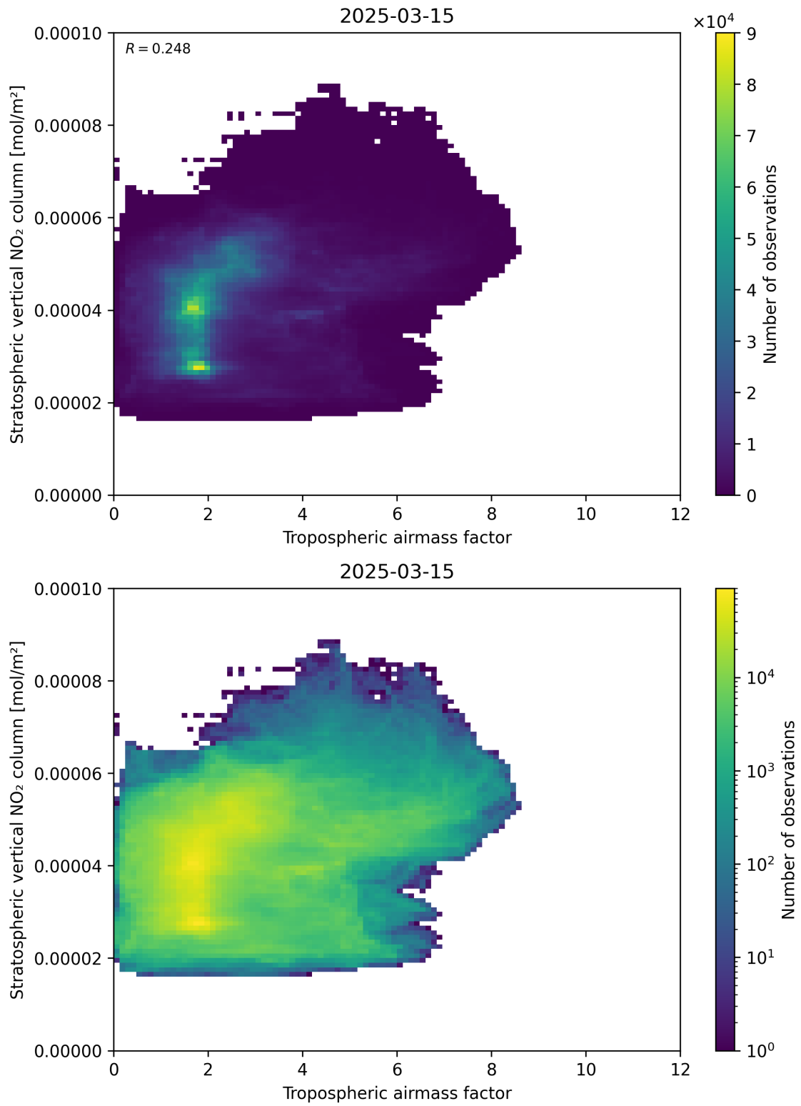
Figure 74: Scatter density plot of “Tropospheric air mass factor” against “Stratospheric vertical NO 2 column” for 2025-03-15 to 2025-03-15.
