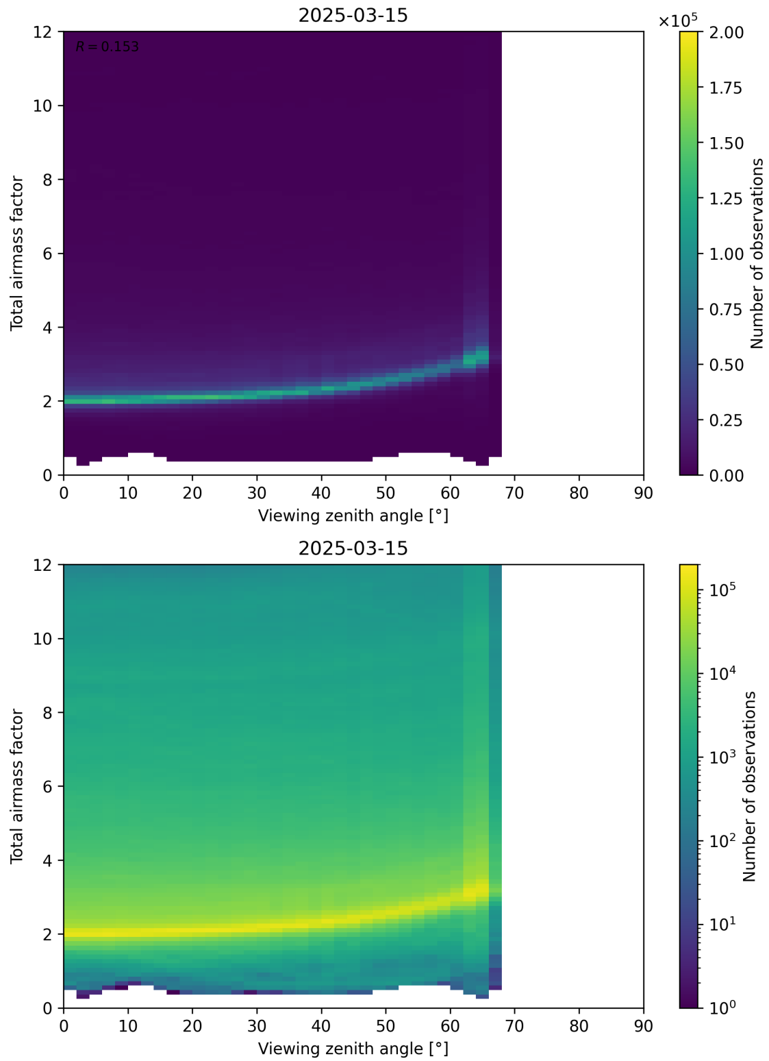
Figure 160: Scatter density plot of “Viewing zenith angle” against “Total airmass factor” for 2025-03-15 to 2025-03-15.
