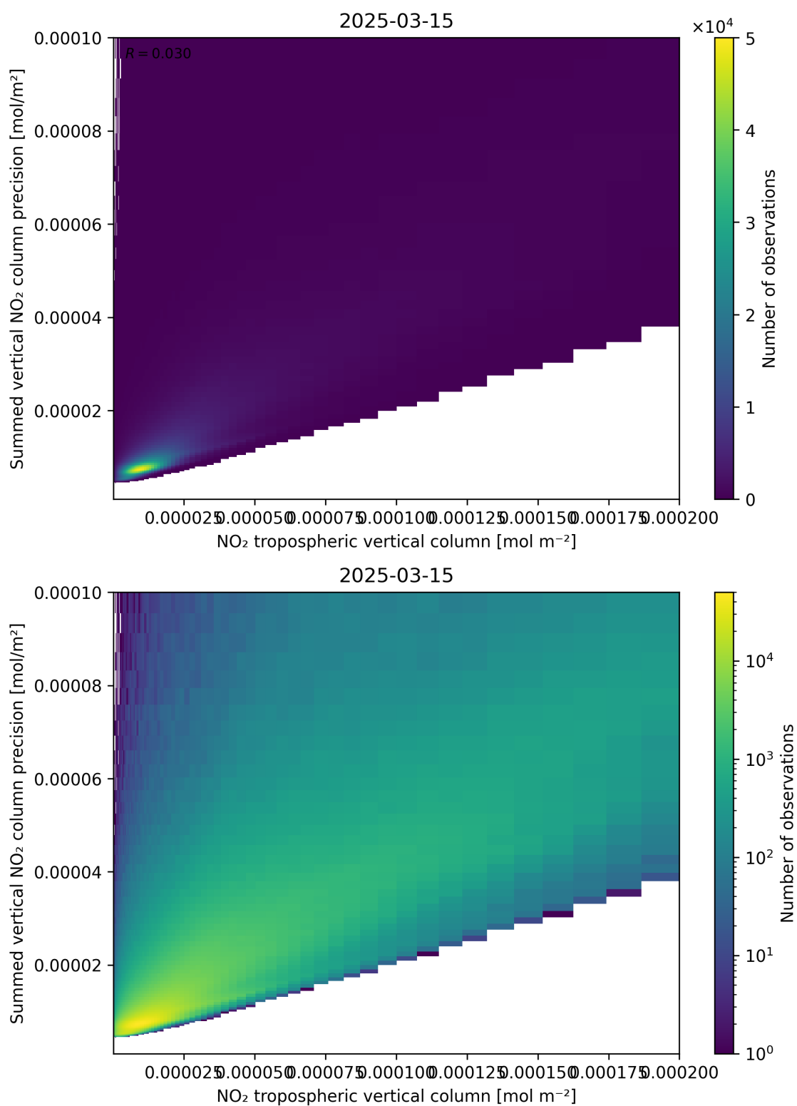
Figure 127: Scatter density plot of “NO 2 tropospheric vertical column” against “Summed vertical NO 2 column precision” for 2025-03-15 to 2025-03-15.
