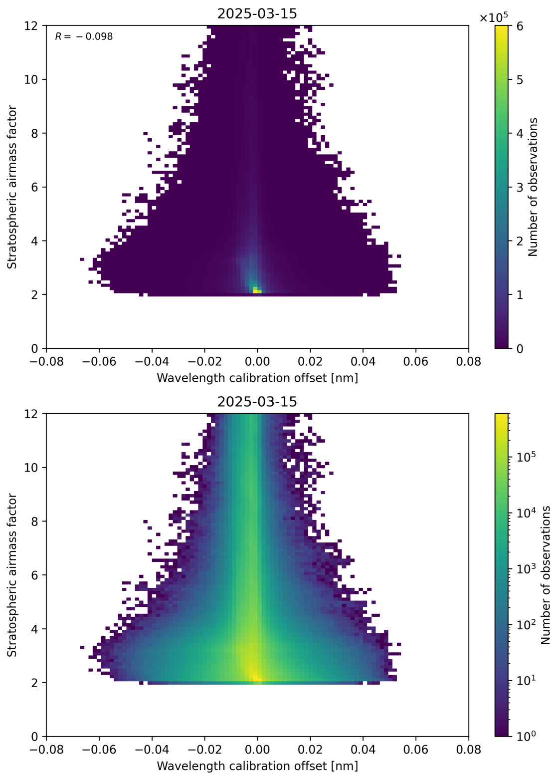
Figure 174: Scatter density plot of “Wavelength calibration offset” against “Stratospheric airmass factor” for 2025-03-15 to 2025-03-15.
