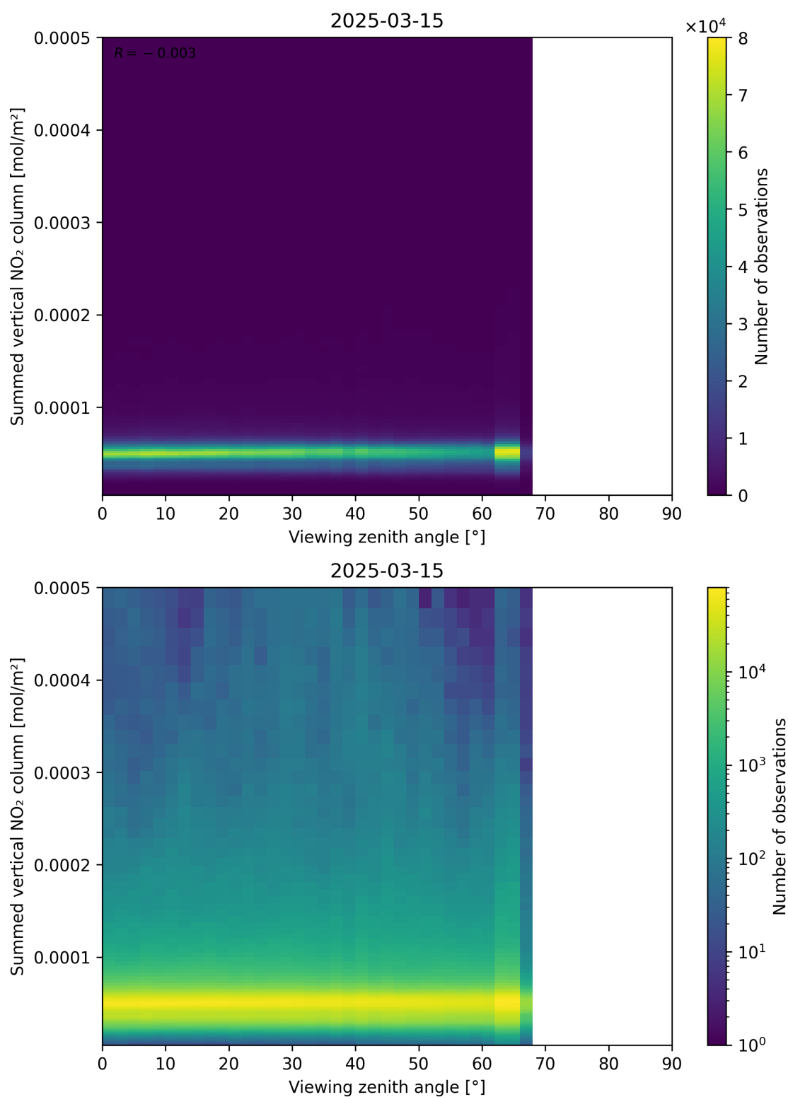
Figure 165: Scatter density plot of “Viewing zenith angle” against “Summed vertical NO 2 column” for 2025-03-15 to 2025-03-15.
