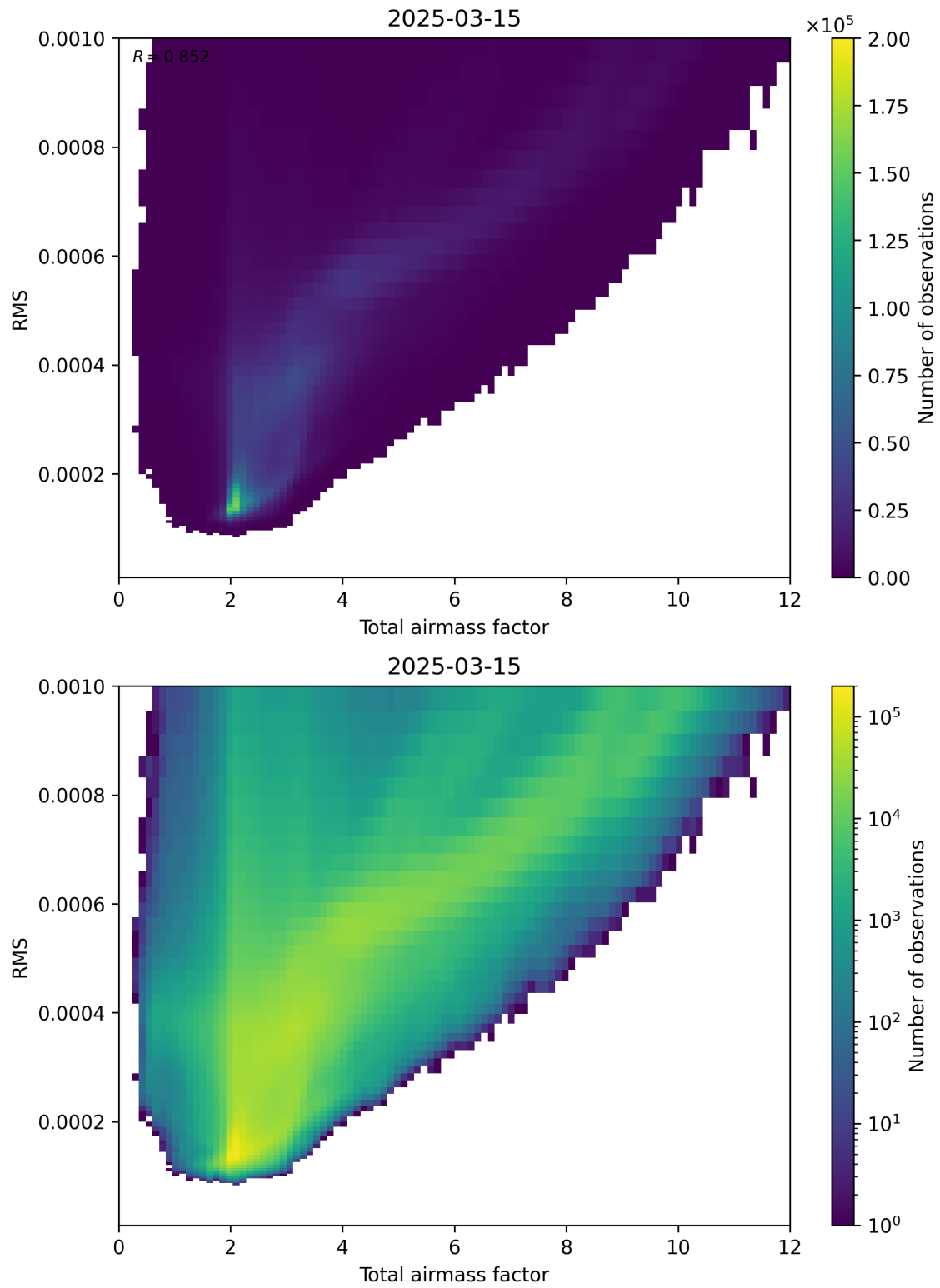
Figure 69: Scatter density plot of “Total airmass factor” against “RMS” for 2025-03-15 to 2025-03-15.
