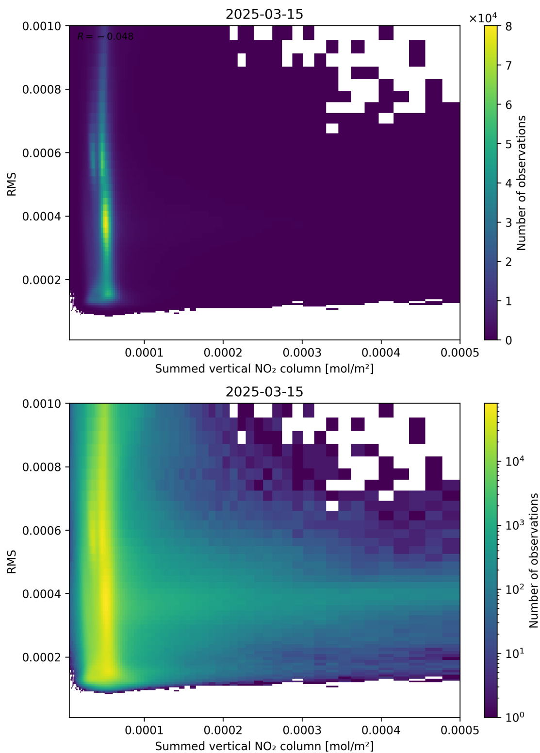
Figure 109: Scatter density plot of “Summed vertical NO 2 column” against “RMS” for 2025-03-15 to 2025-03-15.
