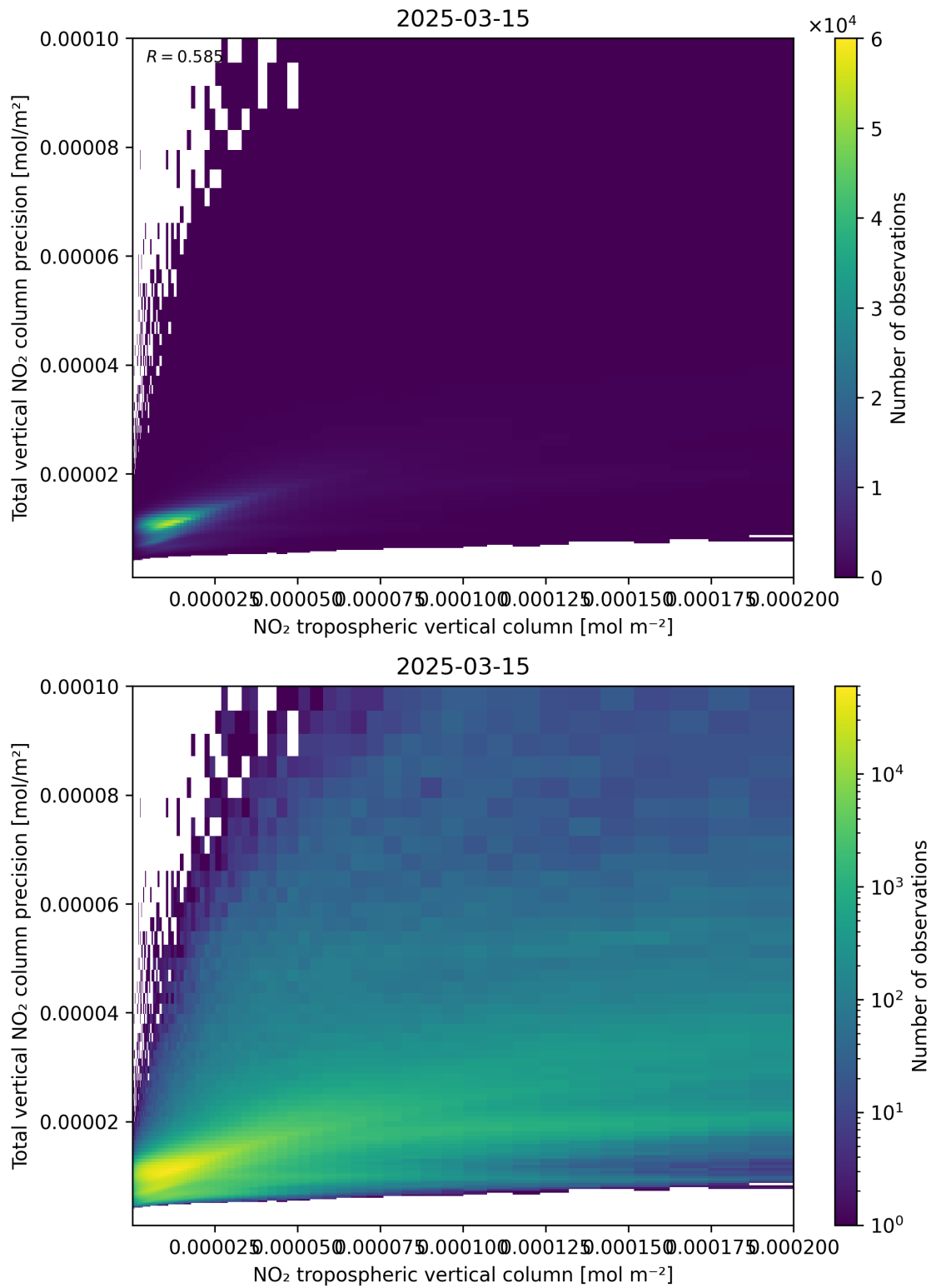
Figure 129: Scatter density plot of “NO 2 tropospheric vertical column” against “Total vertical NO 2 column precision” for 2025-03-15 to 2025-03-15.
