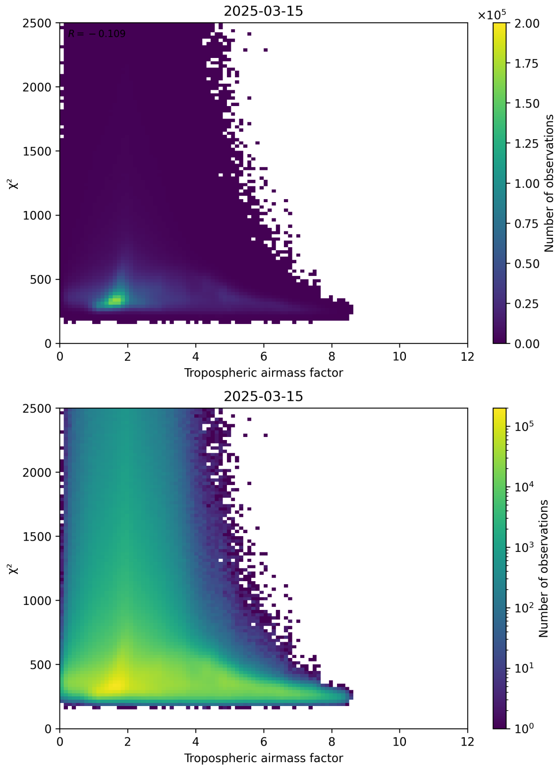
Figure 73: Scatter density plot of “Tropospheric airmass factor” against “ \chi^2 ” for 2025-03-15 to 2025-03-15.
