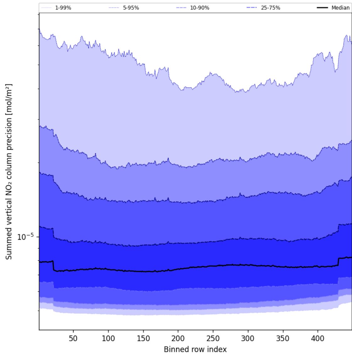
Figure 58: Along track statistics of “Summed vertical NO 2 column precision” for 2025-03-15 to 2025-03-15
