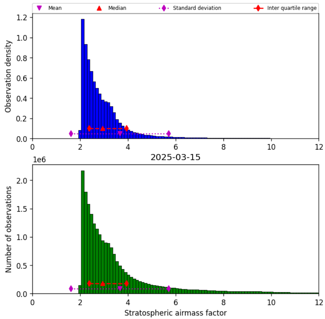
Figure 44: Histogram of “Stratospheric airmass factor” for 2025-03-15 to 2025-03-15
