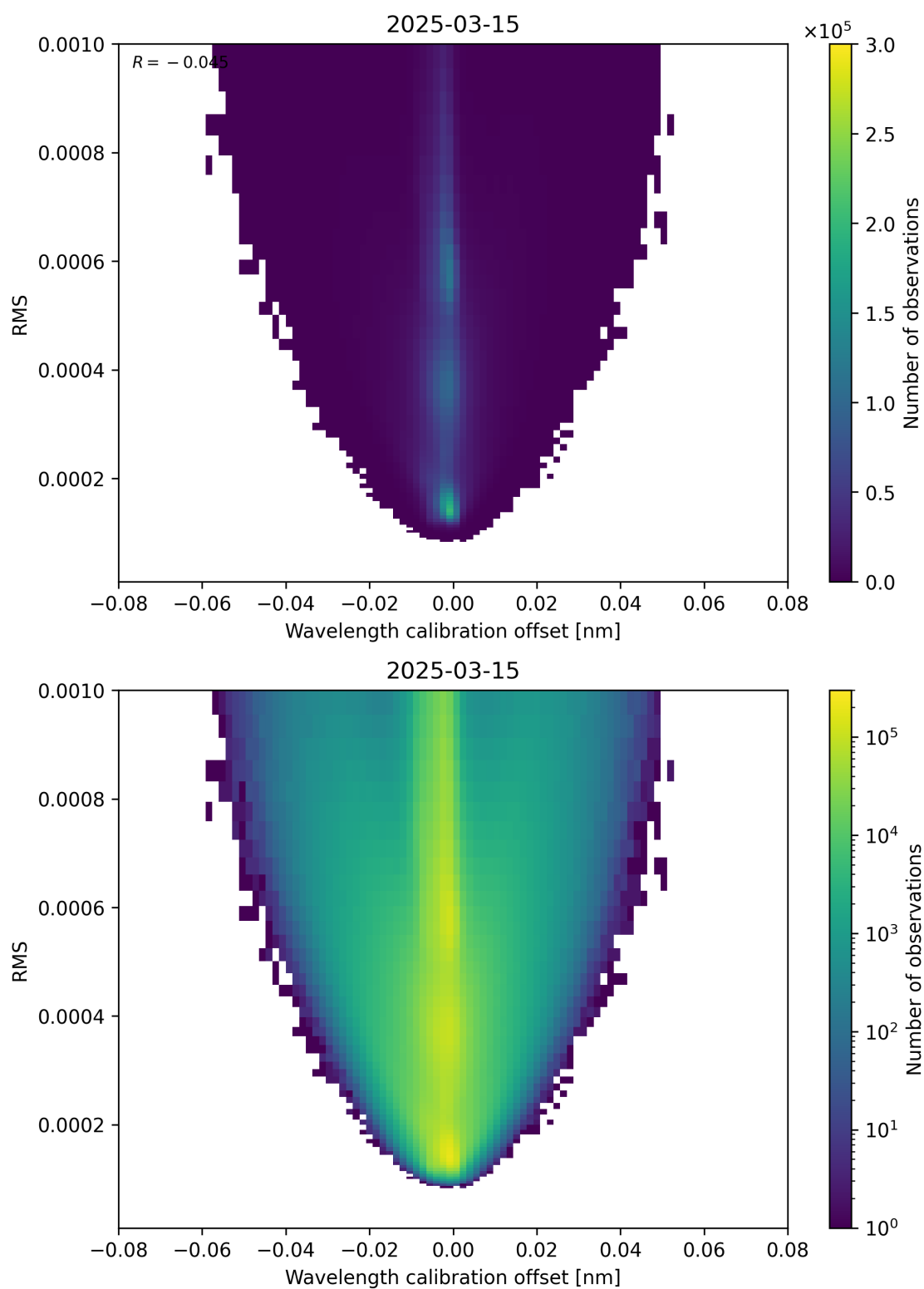
Figure 181: Scatter density plot of “Wavelength calibration offset” against “RMS” for 2025-03-15 to 2025-03-15.
