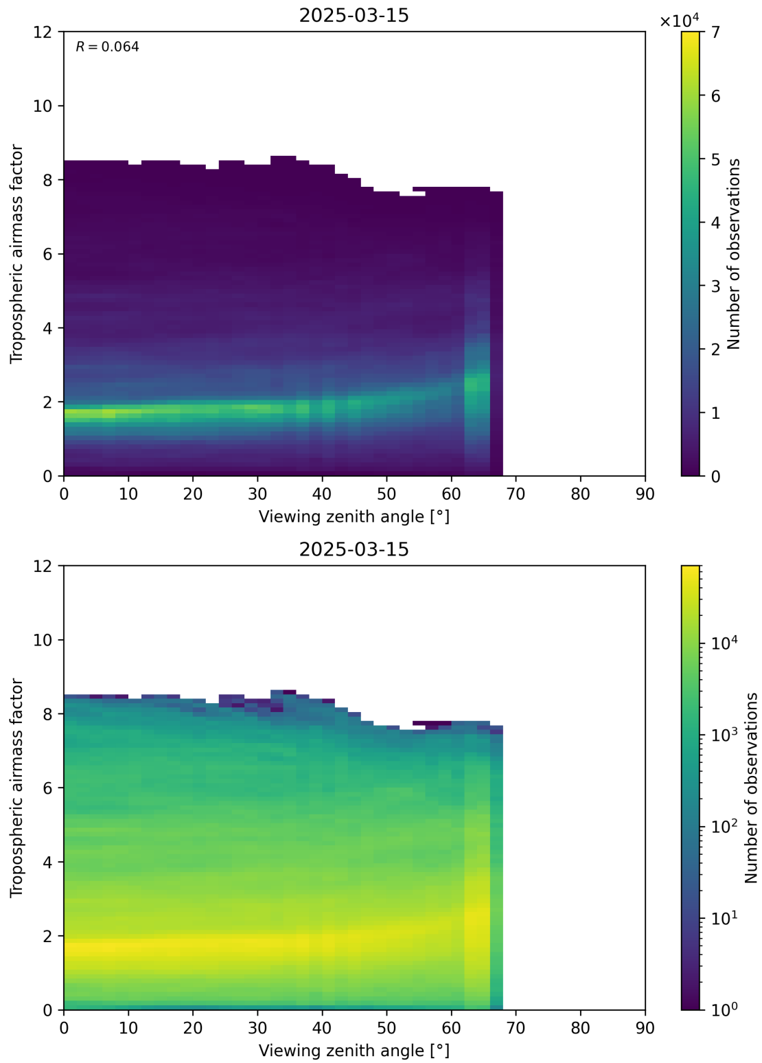
Figure 161: Scatter density plot of “Viewing zenith angle” against “Tropospheric airmass factor” for 2025-03-15 to 2025-03-15.
