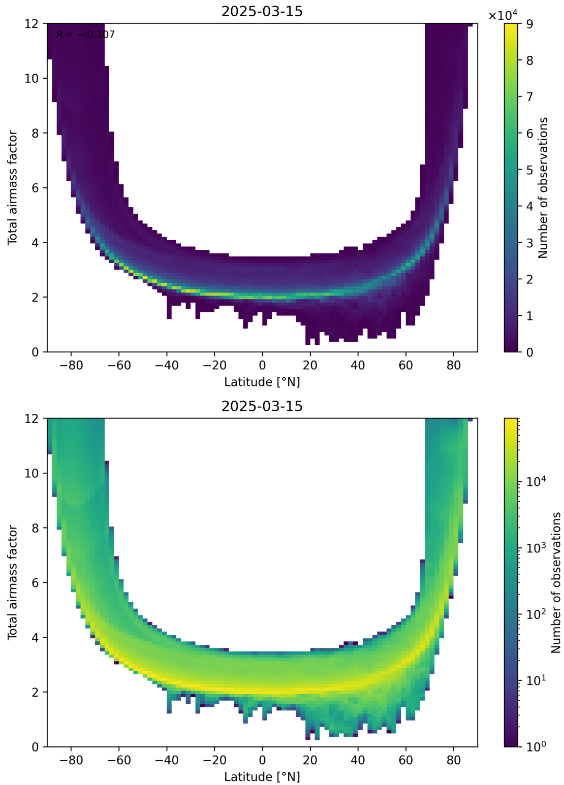
Figure 84: Scatter density plot of “Latitude” against “Total airmass factor” for 2025-03-15 to 2025-03-15.
