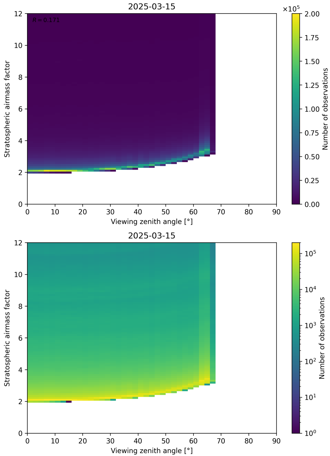
Figure 159: Scatter density plot of “Viewing zenith angle” against “Stratospheric airmass factor” for 2025-03-15 to 2025-03-15.
