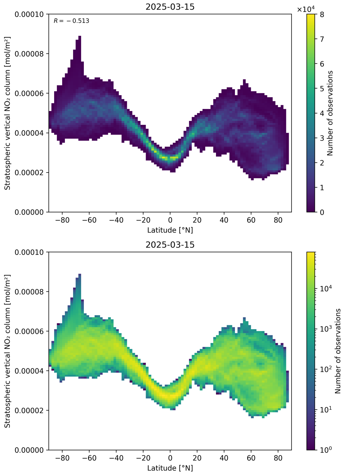
Figure 87: Scatter density plot of “Latitude” against “Stratospheric vertical NO 2 column” for 2025-03-15 to 2025-03-15.
