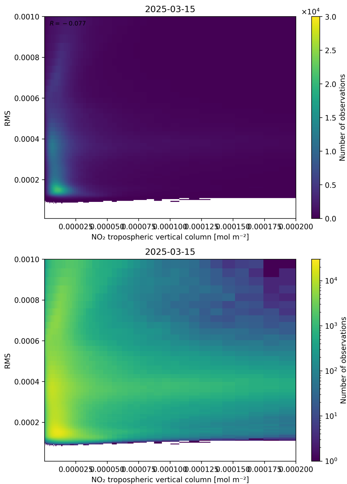
Figure 142: Scatter density plot of “NO 2 tropospheric vertical column” against “RMS” for 2025-03-15 to 2025-03-15.
