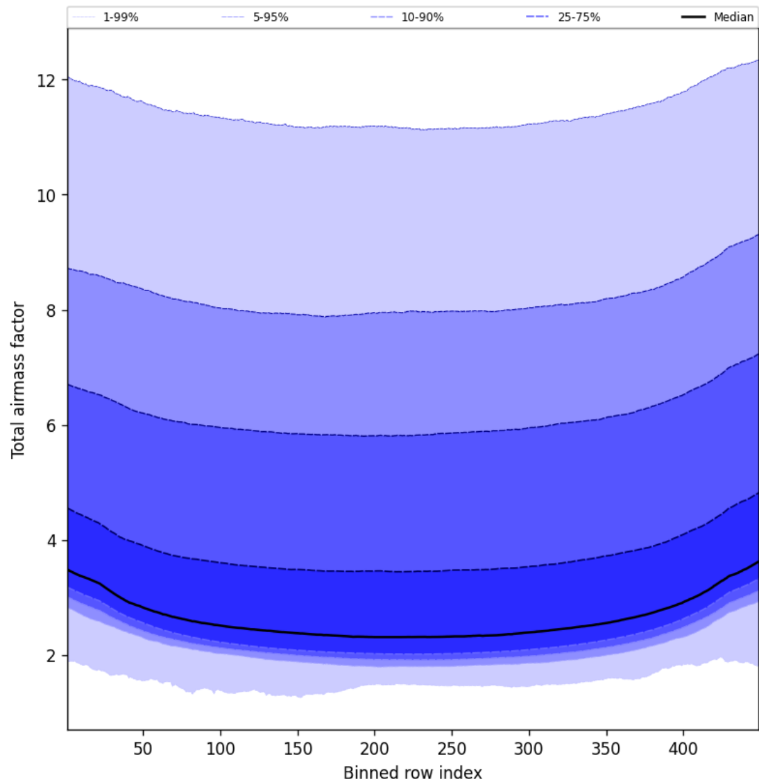
Figure 49: Along track statistics of “Total airmass factor” for 2025-03-15 to 2025-03-15
