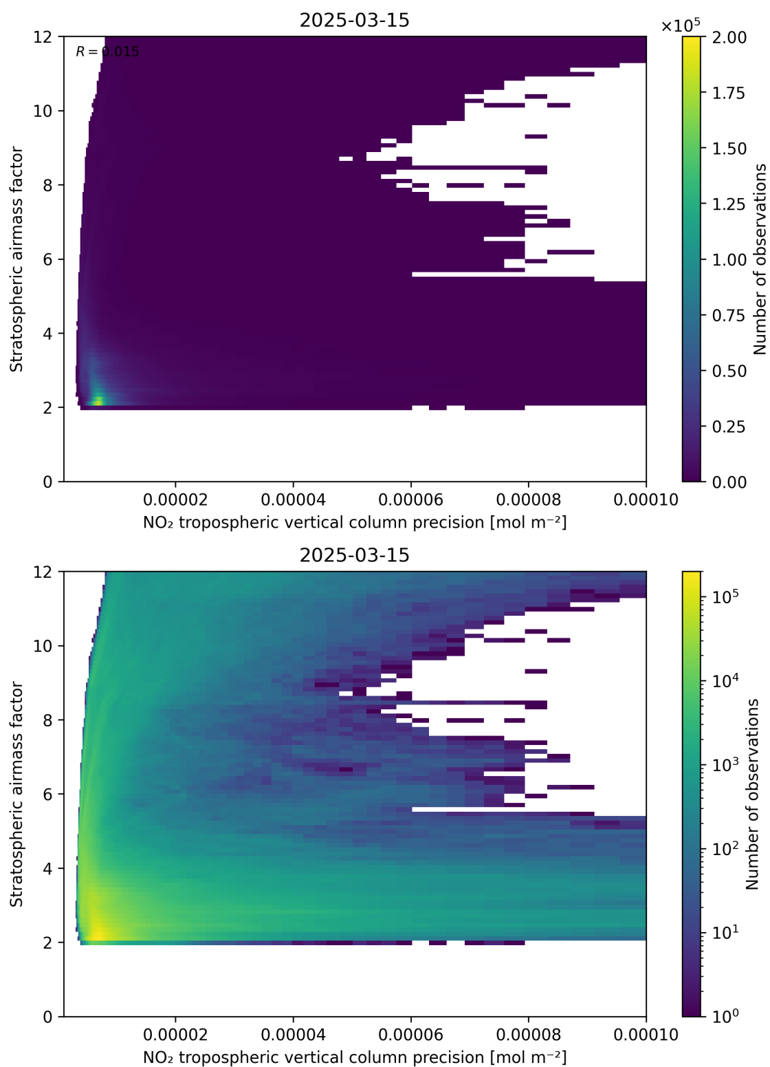
Figure 131: Scatter density plot of “NO 2 tropospheric vertical column precision” against “Stratospheric airmass factor” for 2025-03-15 to 2025-03-15.
