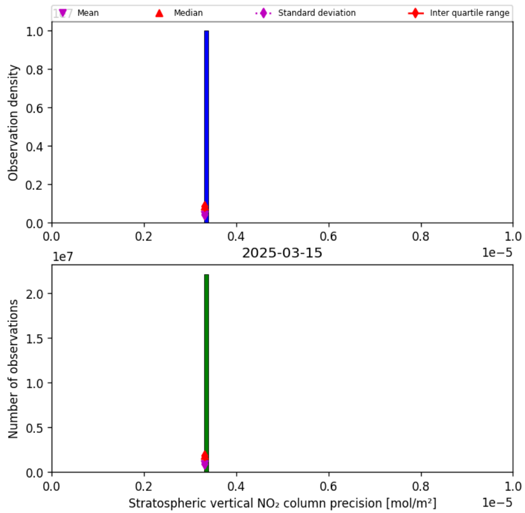
Figure 37: Histogram of “Stratospheric vertical NO 2 column precision” for 2025-03-15 to 2025-03-15
