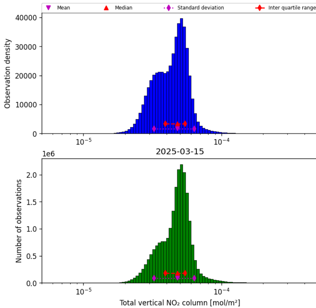
Figure 38: Histogram of “Total vertical NO 2 column” for 2025-03-15 to 2025-03-15
