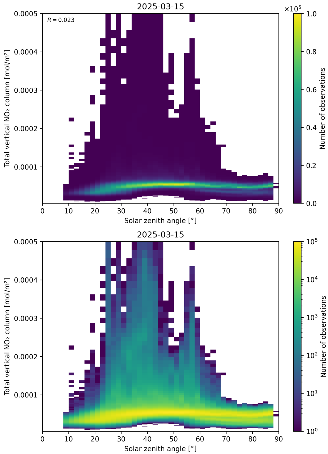
Figure 153: Scatter density plot of “Solar zenith angle” against “Total vertical NO 2 column” for 2025-03-15 to 2025-03-15.
