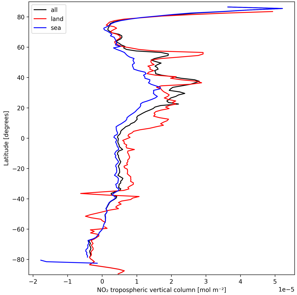
Figure 12: Zonal average of “NO 2 tropospheric vertical column” for 2025-03-15 to 2025-03-15.
