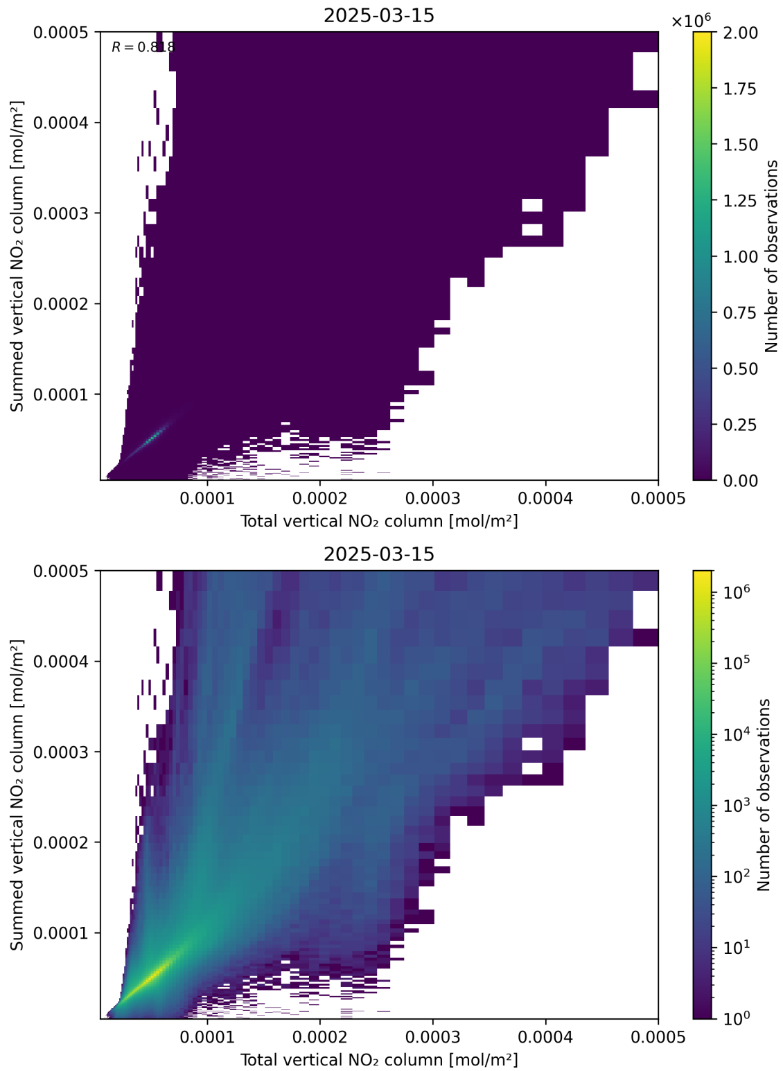
Figure 112: Scatter density plot of “Total vertical NO 2 column” against “Summed vertical NO 2 column” for 2025-03-15 to 2025-03-15.
