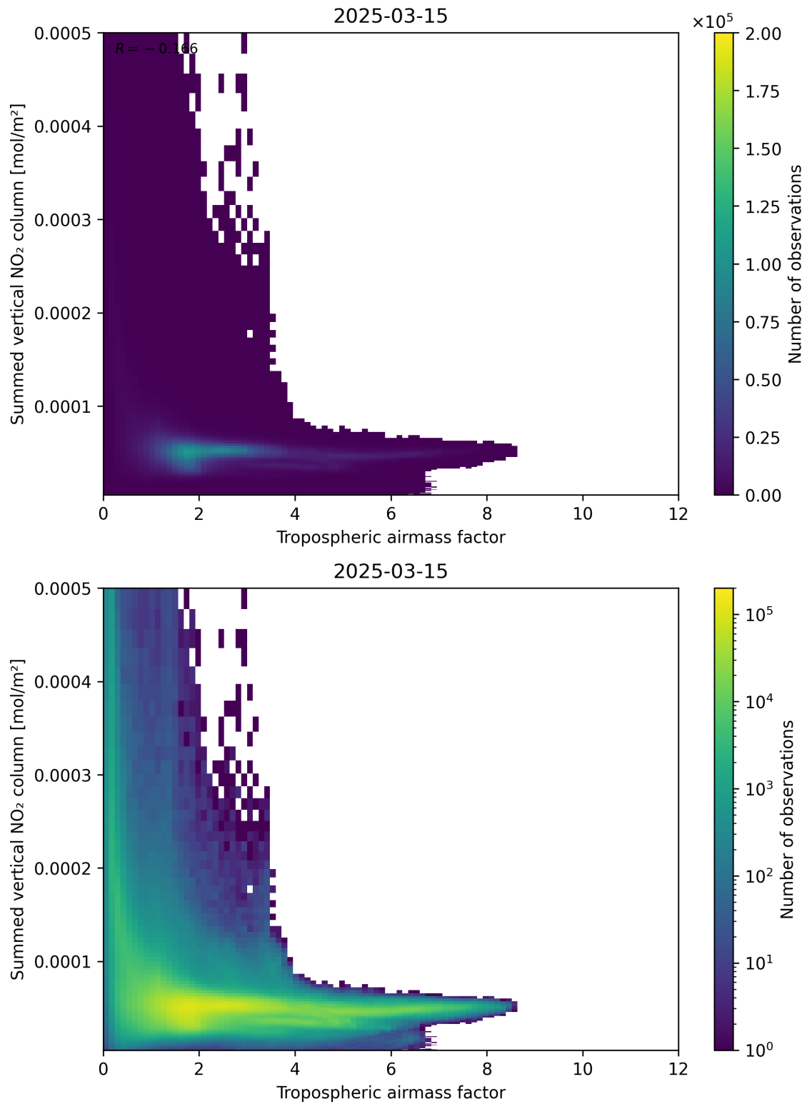
Figure 75: Scatter density plot of “Tropospheric air mass factor” against “Summed vertical NO 2 column” for 2025-03-15 to 2025-03-15.
