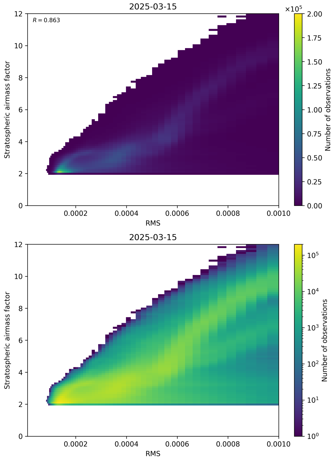
Figure 144: Scatter density plot of “RMS” against “Stratospheric airmass factor” for 2025-03-15 to 2025-03-15.
