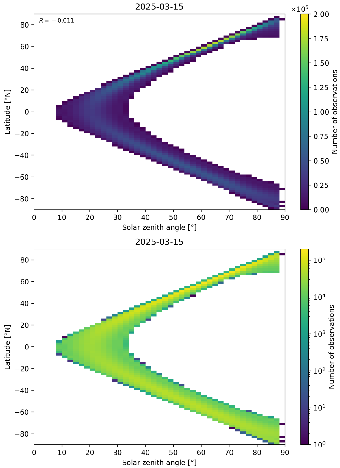
Figure 149: Scatter density plot of “Solar zenith angle” against “Latitude” for 2025-03-15 to 2025-03-15.
