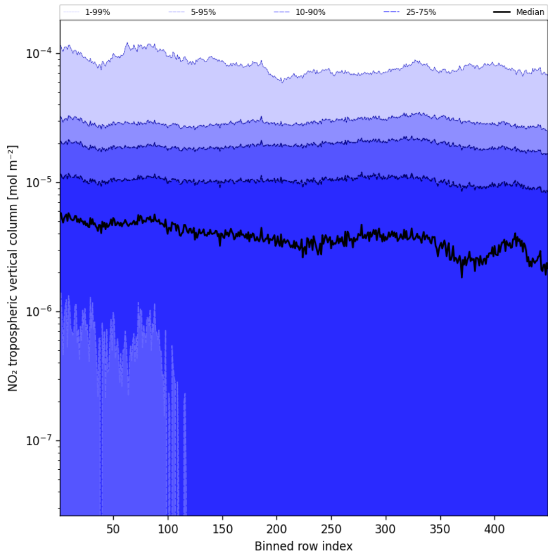
Figure 46: Along track statistics of “NO 2 tropospheric vertical column” for 2025-03-15 to 2025-03-15
