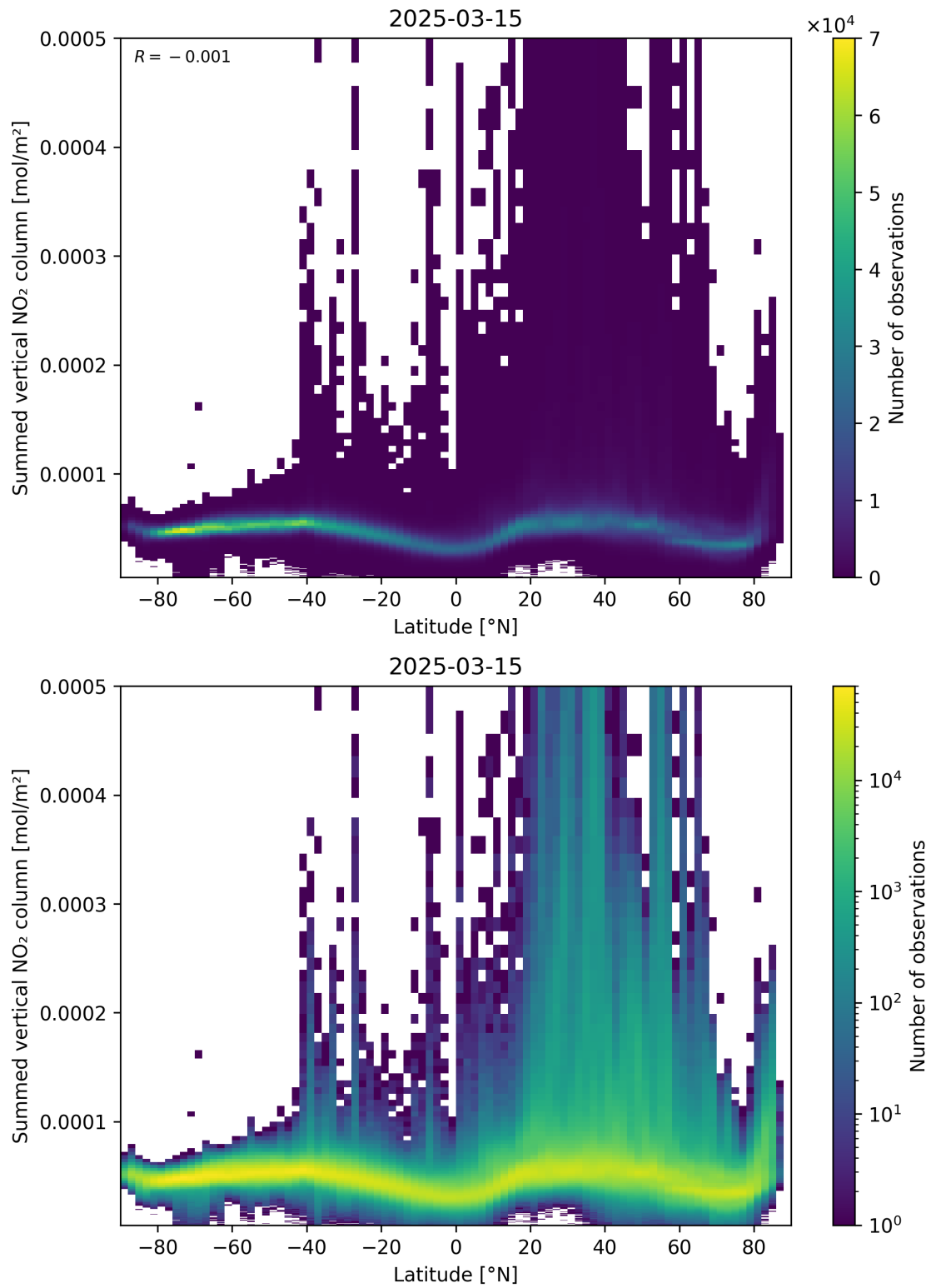
Figure 88: Scatter density plot of “Latitude” against “Summed vertical NO 2 column” for 2025-03-15 to 2025-03-15.
