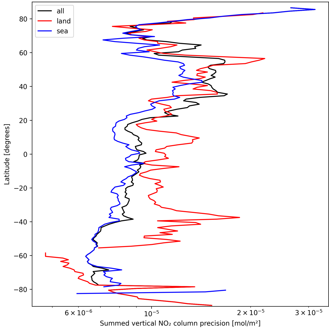
Figure 24: Zonal average of “Summed vertical NO 2 column precision” for 2025-03-15 to 2025-03-15.
