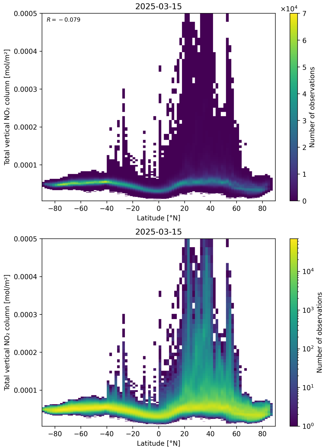
Figure 90: Scatter density plot of “Latitude” against “Total vertical NO 2 column” for 2025-03-15 to 2025-03-15.
