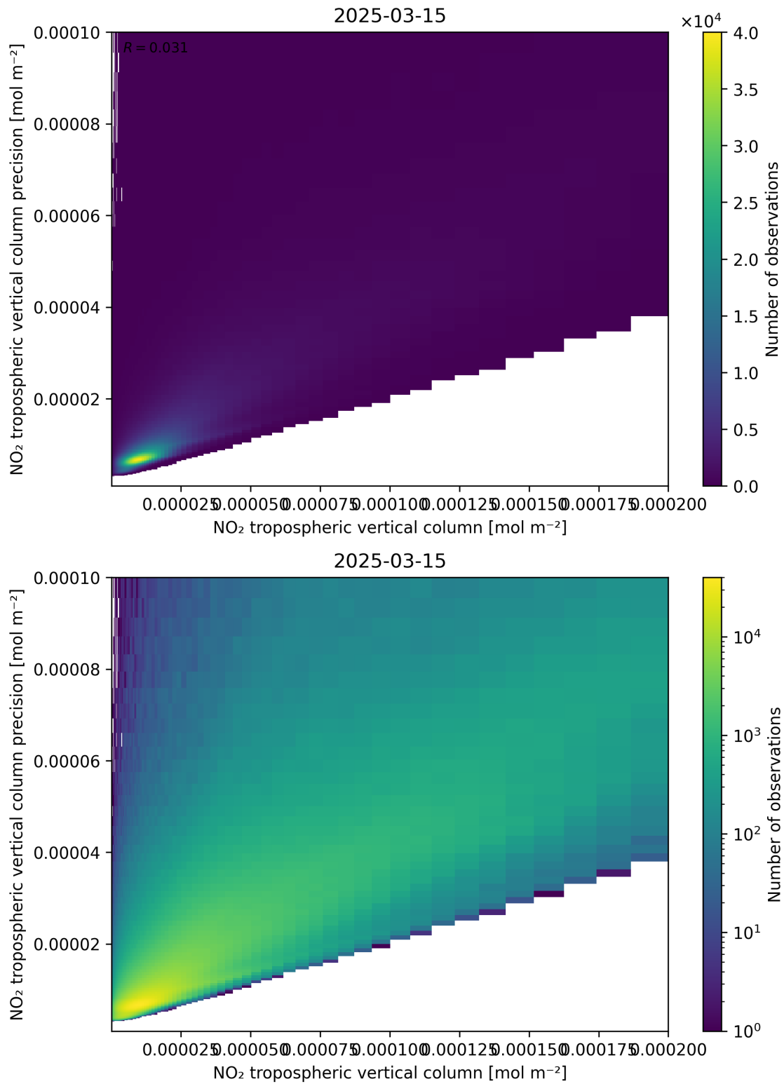
Figure 130: Scatter density plot of “NO 2 tropospheric vertical column” against “NO 2 tropospheric vertical column precision” for 2025-03-15 to 2025-03-15.
