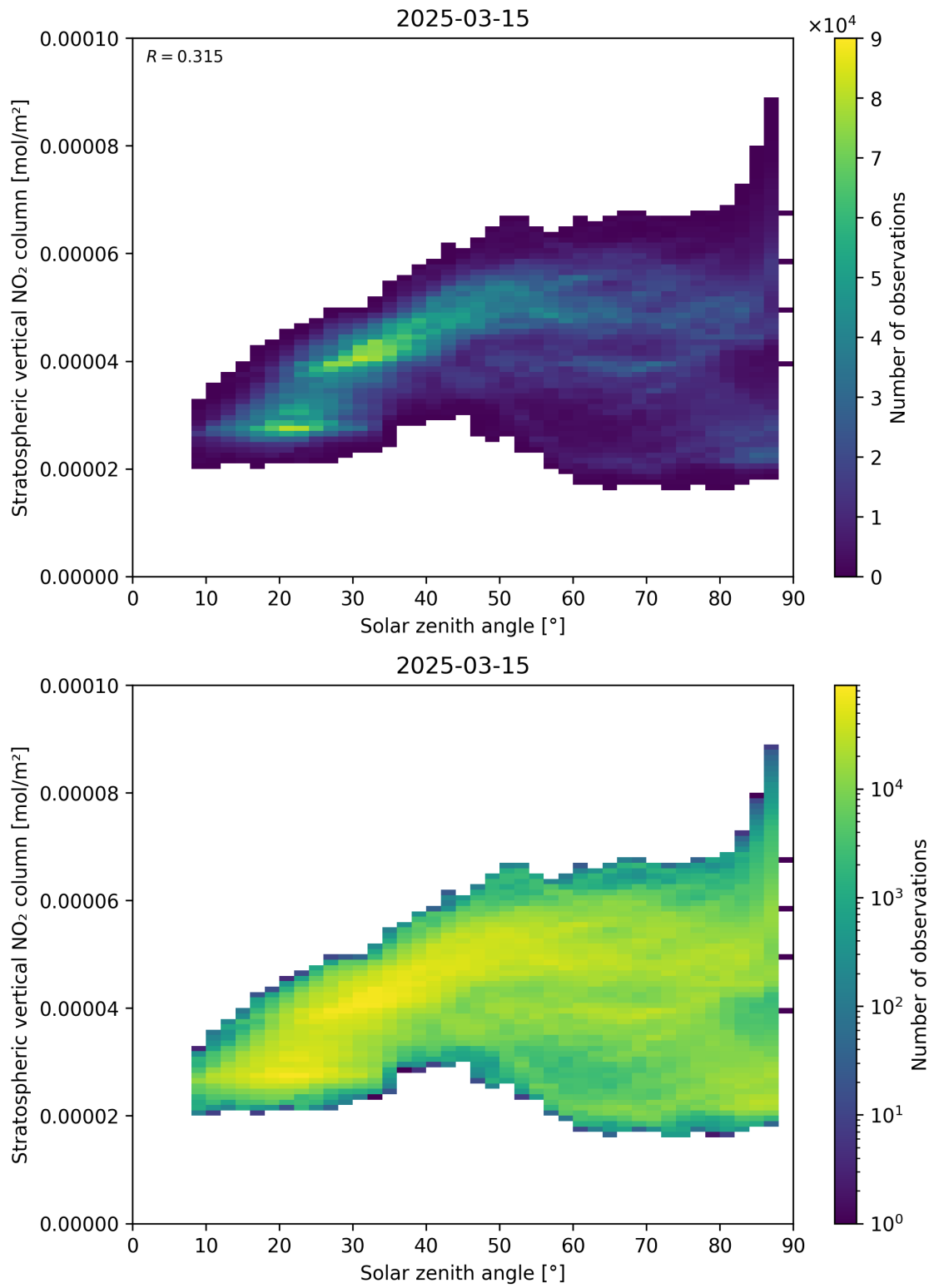
Figure 150: Scatter density plot of “Solar zenith angle” against “Stratospheric vertical NO 2 column” for 2025-03-15 to 2025-03-15.
