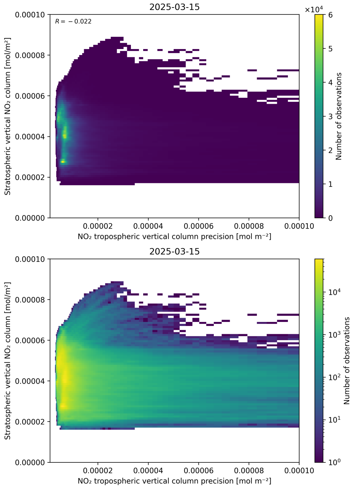
Figure 135: Scatter density plot of “NO 2 tropospheric vertical column precision” against “Stratospheric vertical NO 2 column” for 2025-03-15 to 2025-03-15.
