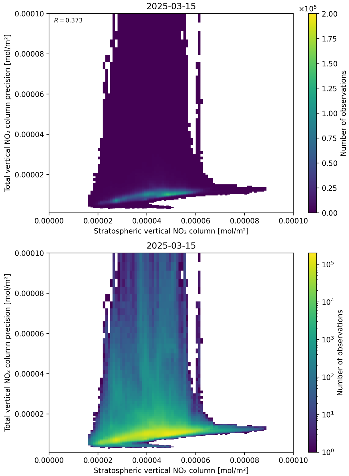
Figure 101: Scatter density plot of “Stratospheric vertical NO 2 column” against “Total vertical NO 2 column precision” for 2025-03-15 to 2025-03-15.
