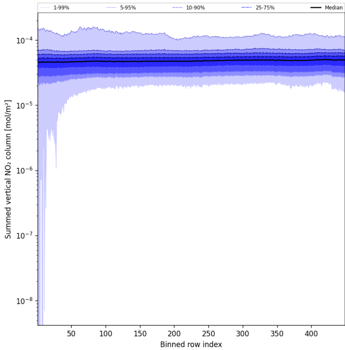
Figure 57: Along track statistics of “Summed vertical NO 2 column” for 2025-03-15 to 2025-03-15
