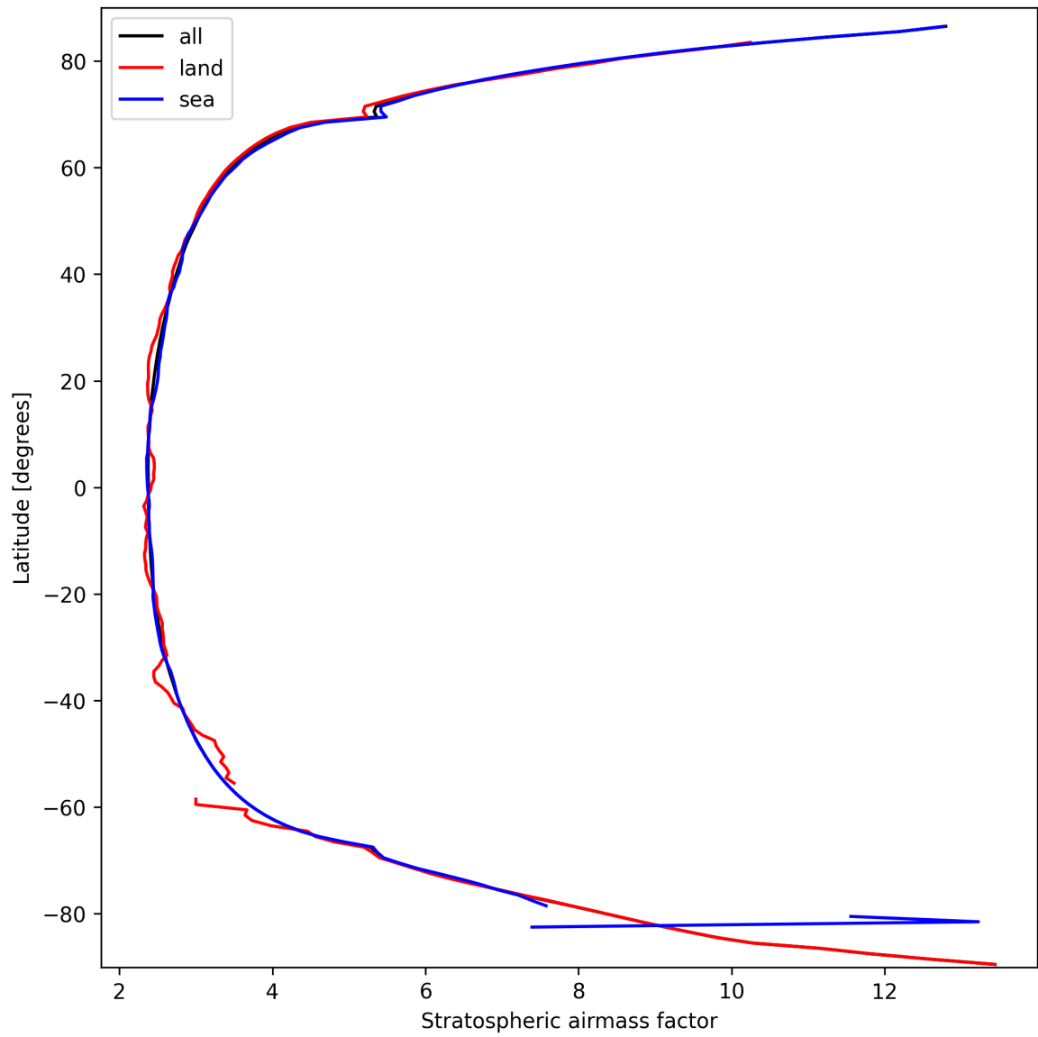
Figure 27: Zonal average of “Stratospheric air mass factor” for 2025-03-15 to 2025-03-15.
