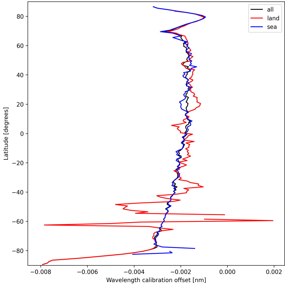
Figure 18: Zonal average of “Wavelength calibration offset” for 2025-03-15 to 2025-03-15.
