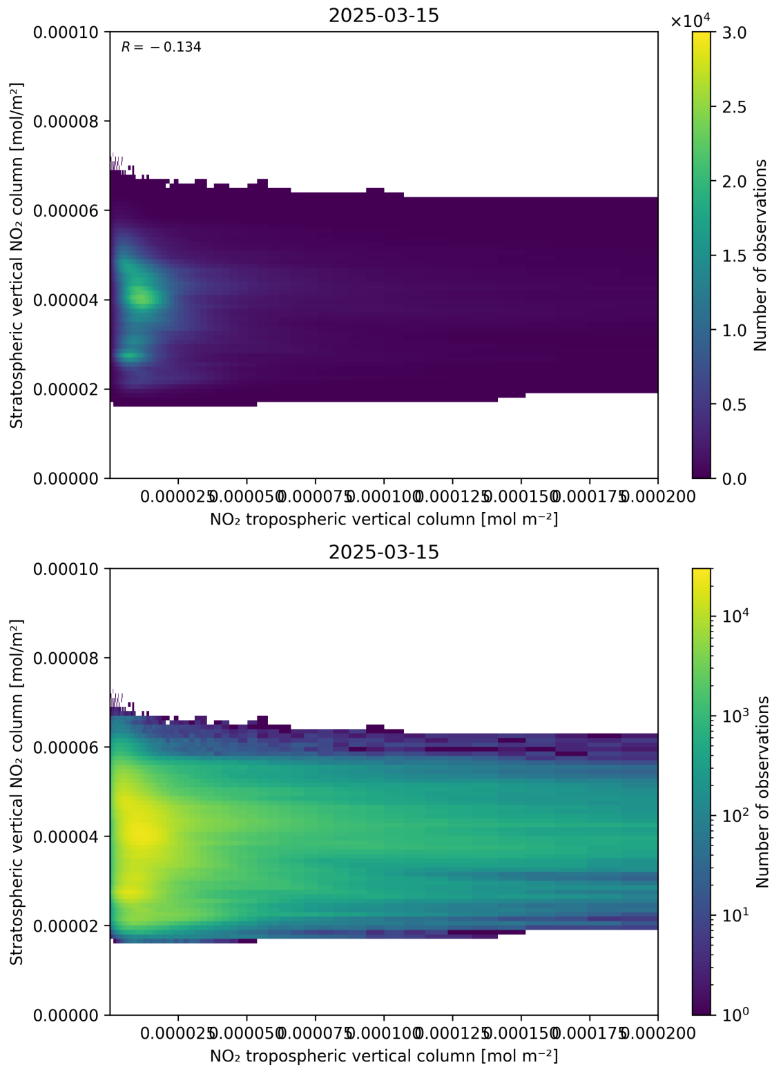
Figure 125: Scatter density plot of “NO 2 tropospheric vertical column” against “Stratospheric vertical NO 2 column” for 2025-03-15 to 2025-03-15.
