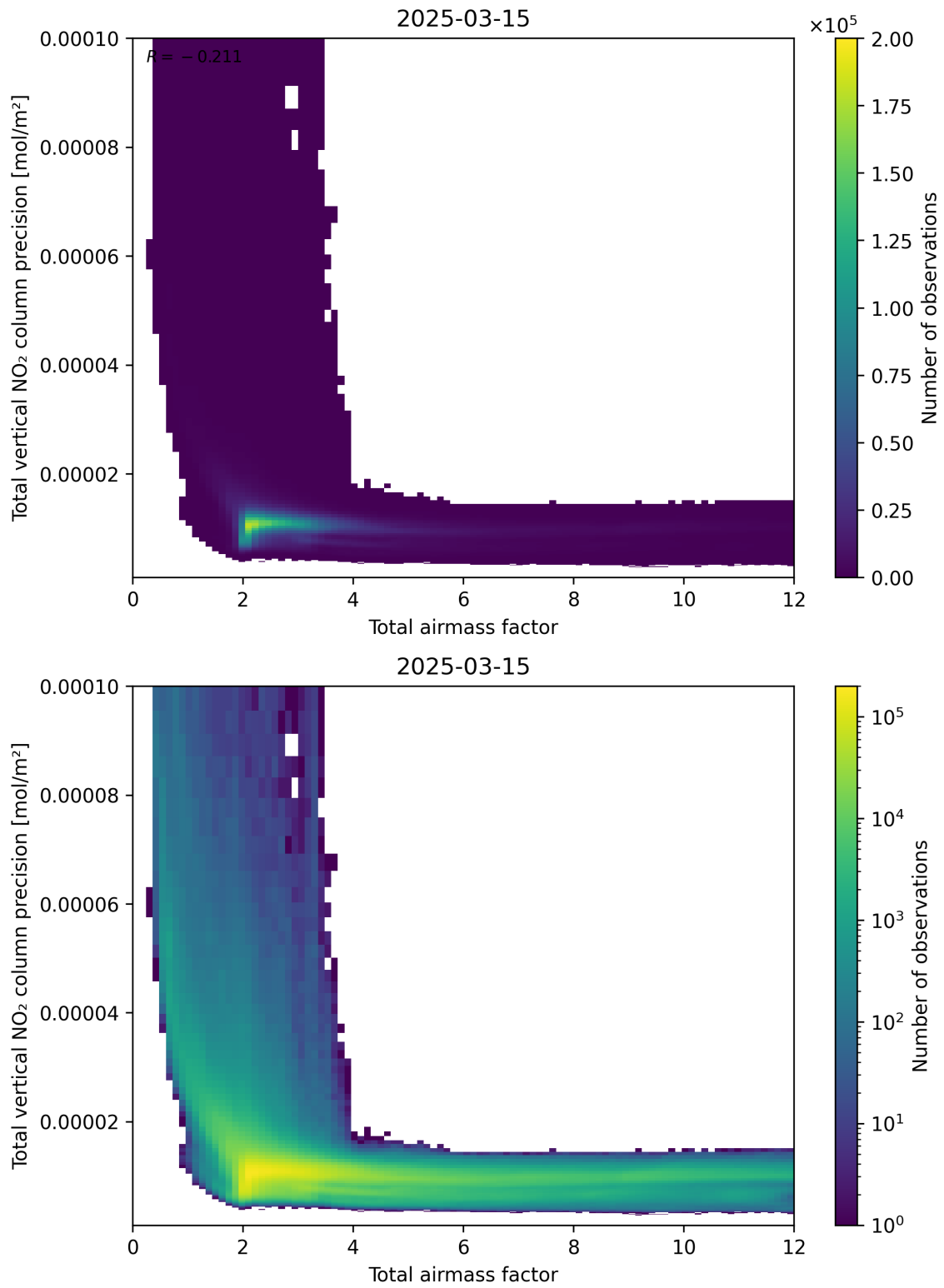
Figure 68: Scatter density plot of “Total airmass factor” against “Total vertical NO 2 column precision” for 2025-03-15 to 2025-03-15.
