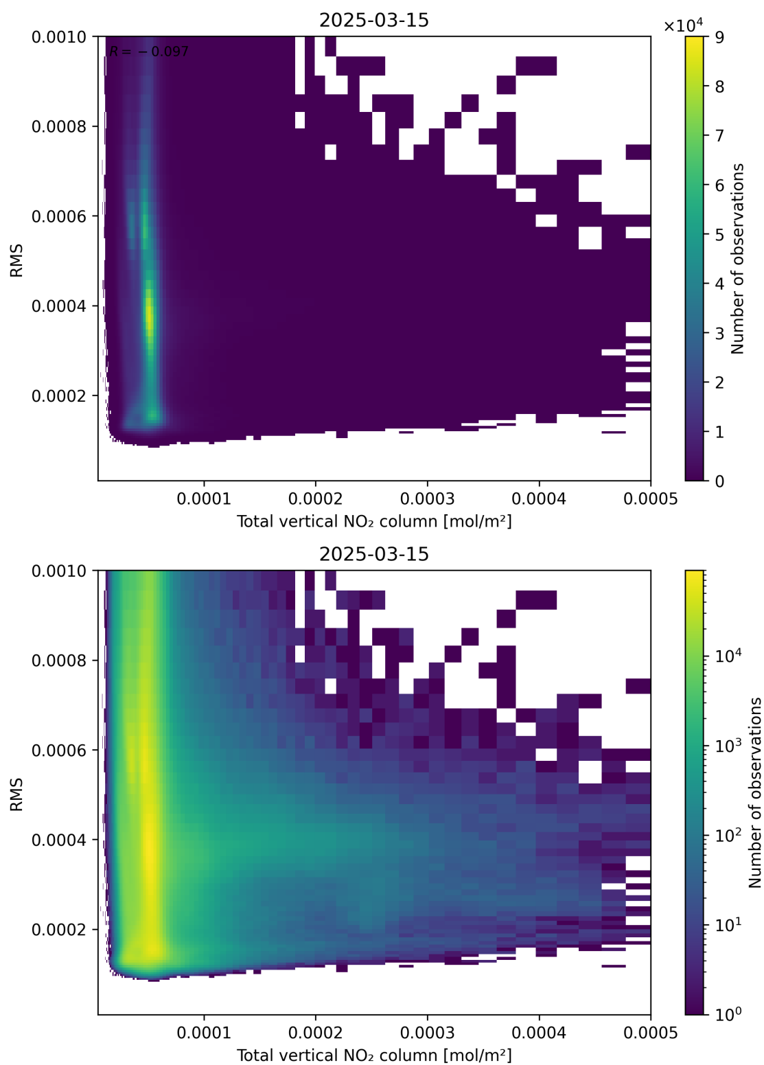
Figure 120: Scatter density plot of “Total vertical NO 2 column” against “RMS” for 2025-03-15 to 2025-03-15.
