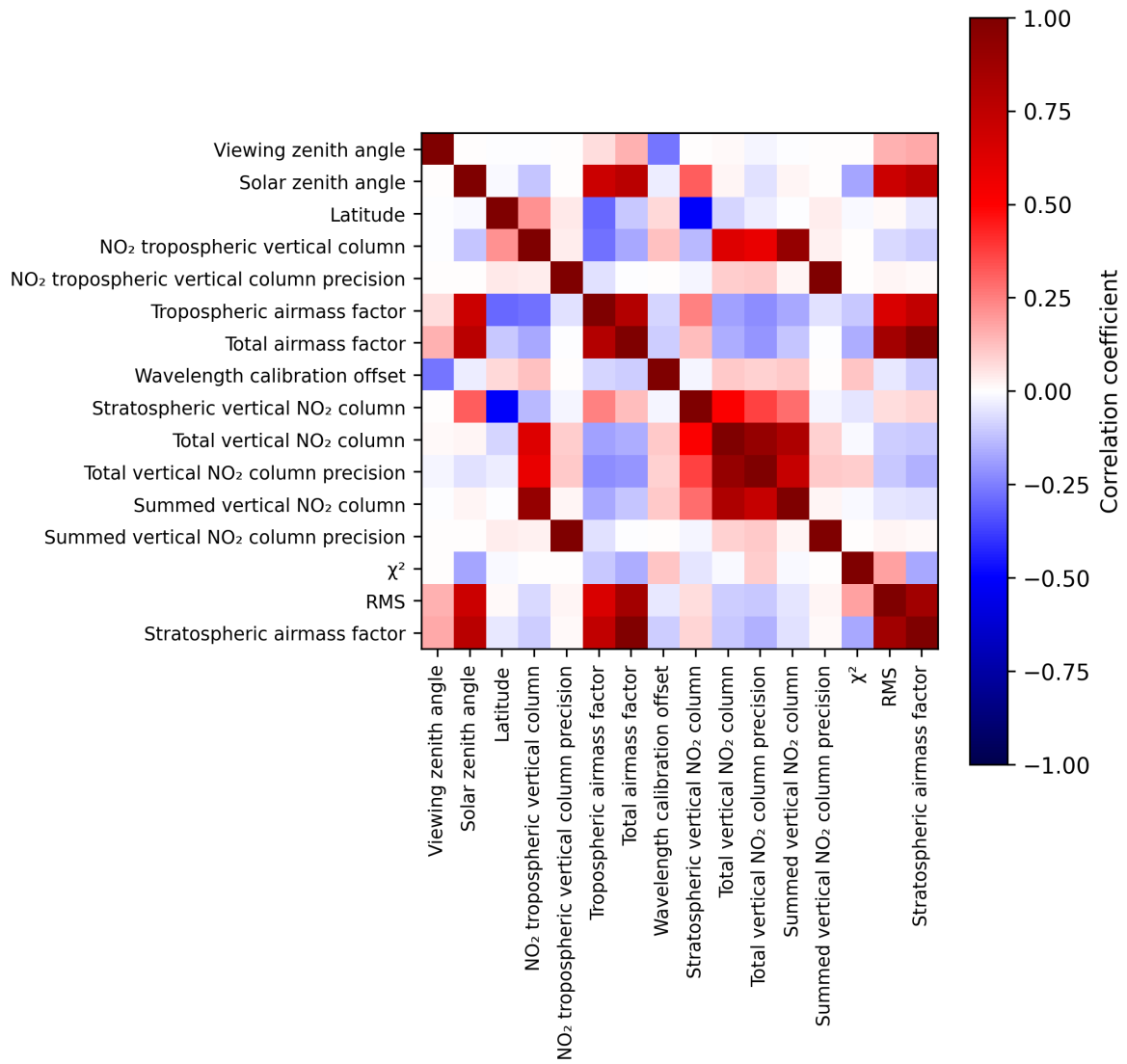
Figure 2: Map of correlation matrix for 2025-03-15 to 2025-03-15.
