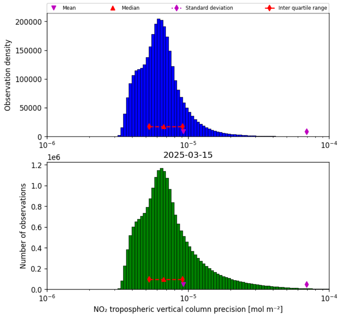
Figure 30: Histogram of “NO 2 tropospheric vertical column precision” for 2025-03-15 to 2025-03-15
