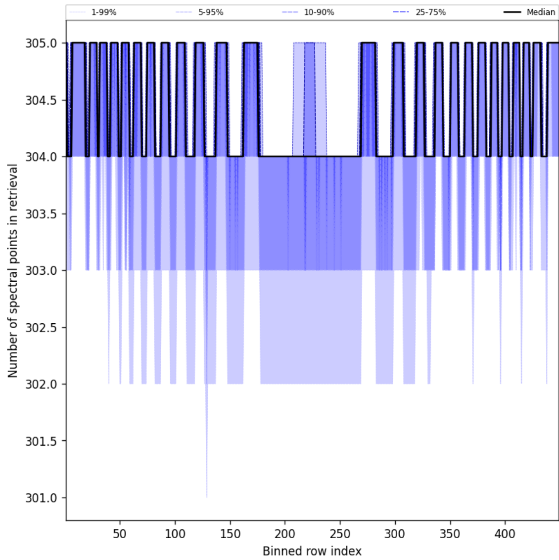
Figure 50: Along track statistics of “Number of spectral points in retrieval” for 2025-03-15 to 2025-03-15
