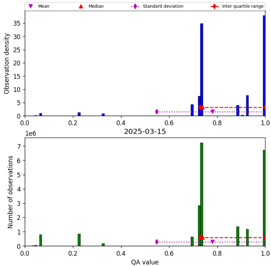
Figure 28: Histogram of “QA value” for 2025-03-15 to 2025-03-15
