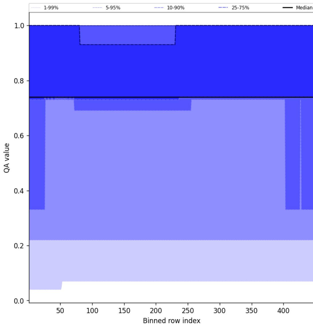
Figure 45: Along track statistics of “QA value” for 2025-03-15 to 2025-03-15
