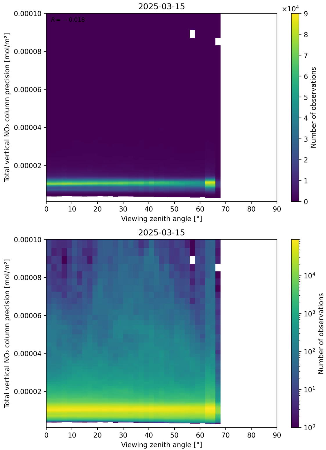
Figure 168: Scatter density plot of “Viewing zenith angle” against “Total vertical NO 2 column precision” for 2025-03-15 to 2025-03-15.
