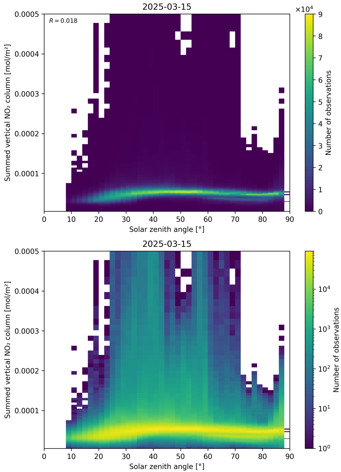
Figure 151: Scatter density plot of “Solar zenith angle” against “Summed vertical NO 2 column” for 2025-03-15 to 2025-03-15.
