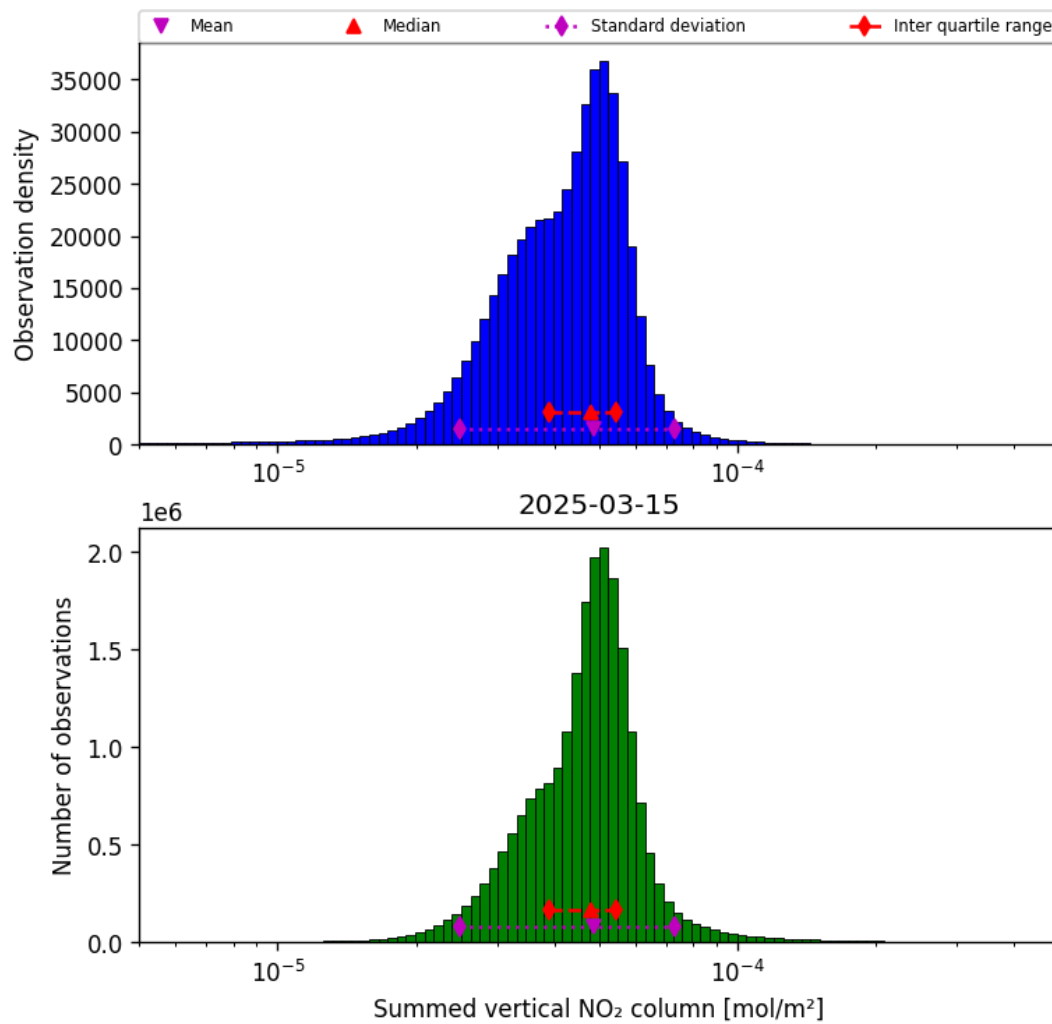
Figure 40: Histogram of “Summed vertical NO 2 column” for 2025-03-15 to 2025-03-15
