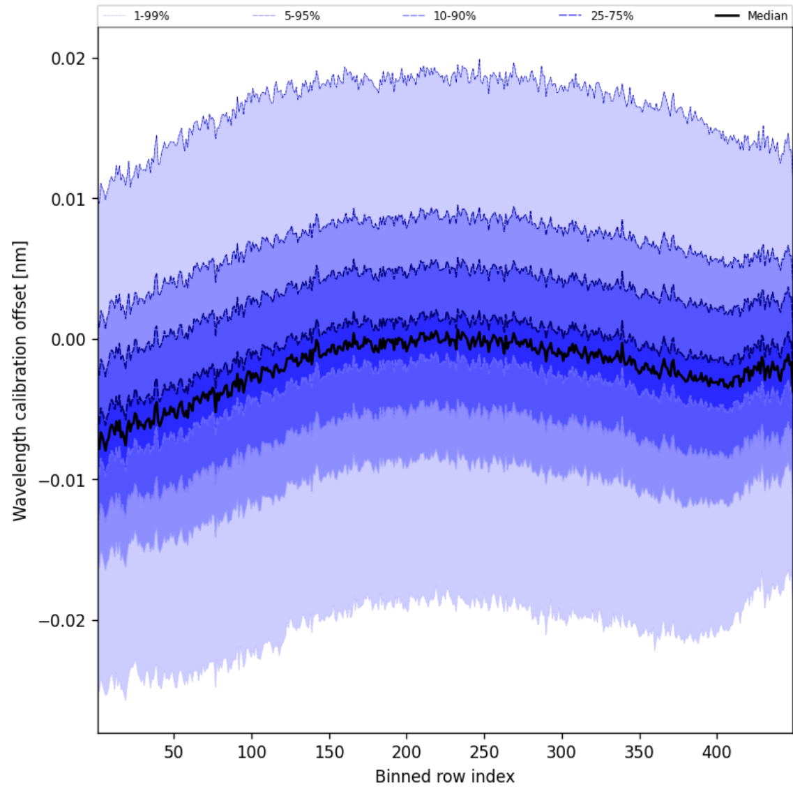
Figure 52: Along track statistics of “Wavelength calibration offset” for 2025-03-15 to 2025-03-15
