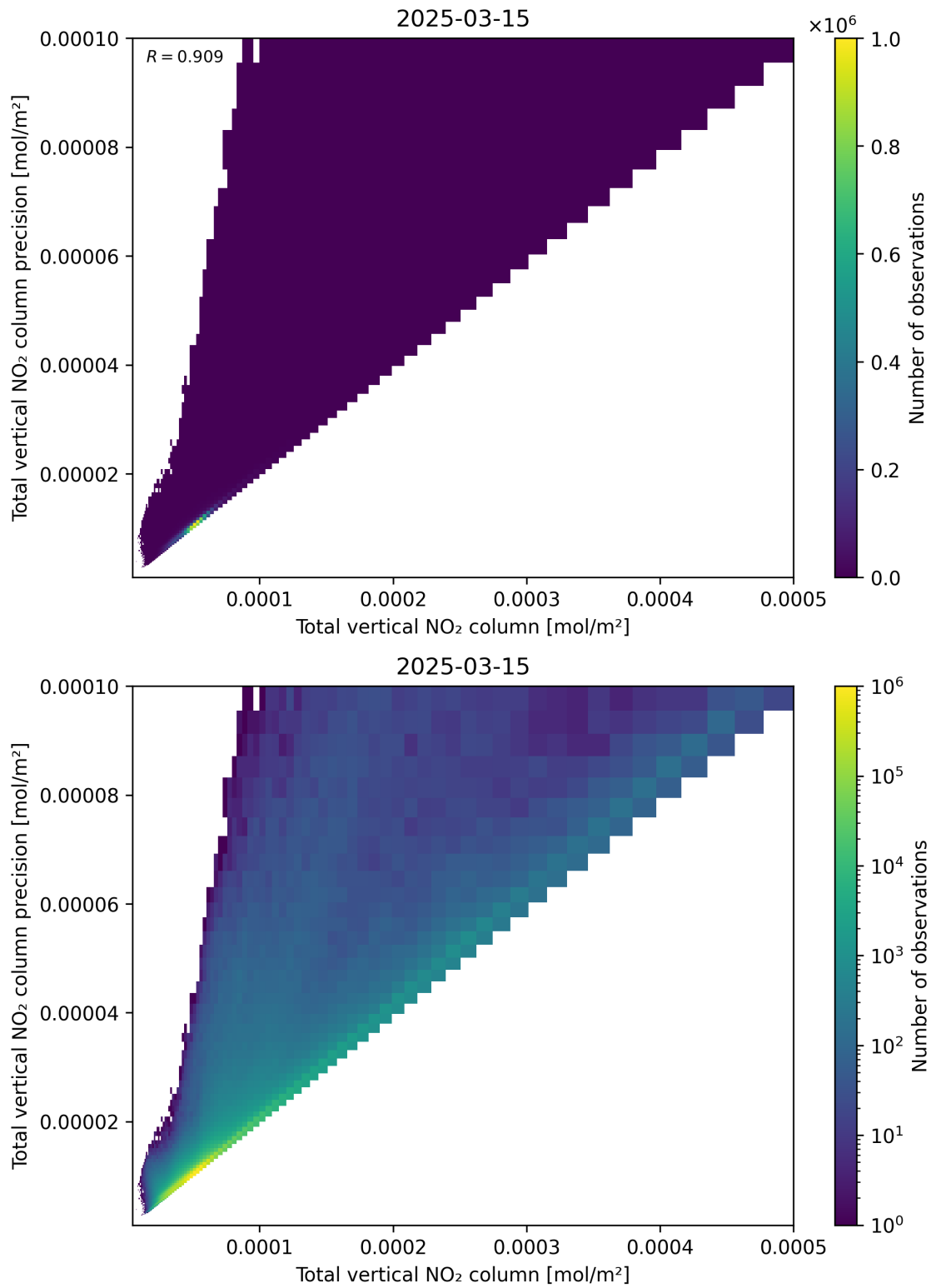
Figure 114: Scatter density plot of “Total vertical NO 2 column” against “Total vertical NO 2 column precision” for 2025-03-15 to 2025-03-15.
