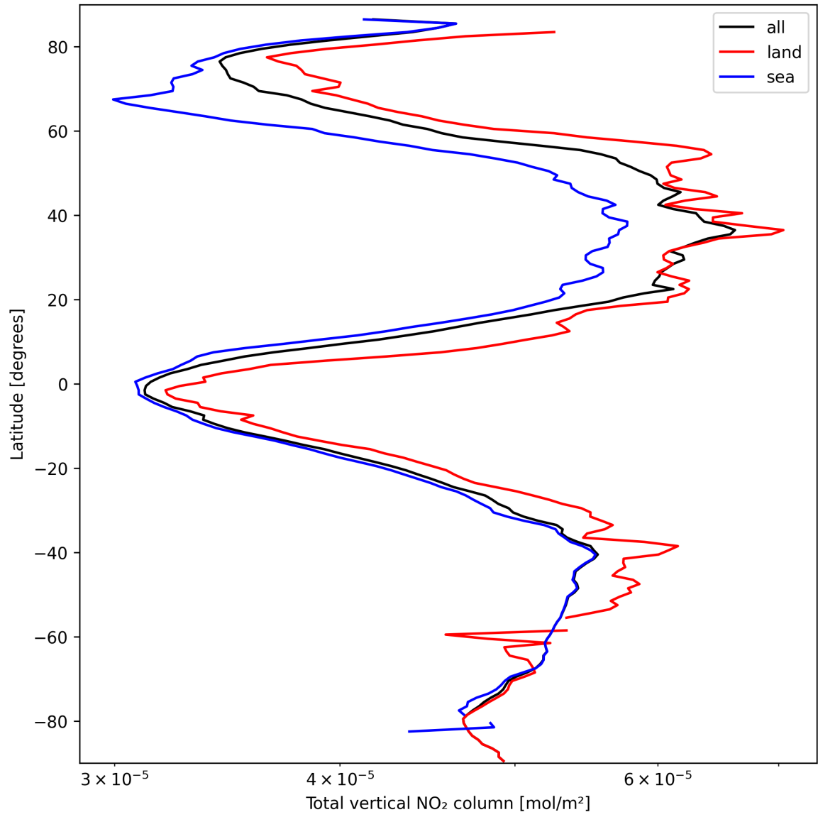
Figure 21: Zonal average of “Total vertical NO 2 column” for 2025-03-15 to 2025-03-15.
