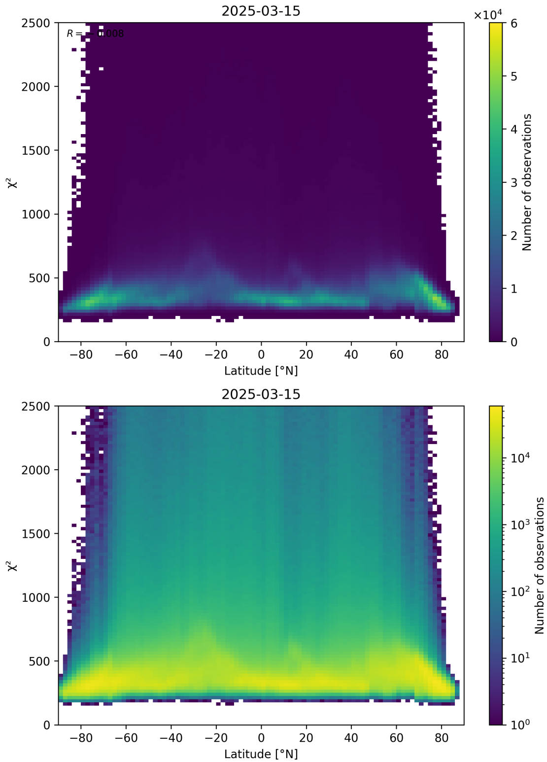
Figure 86: Scatter density plot of “Latitude” against “ \chi^2 ” for 2025-03-15 to 2025-03-15.
