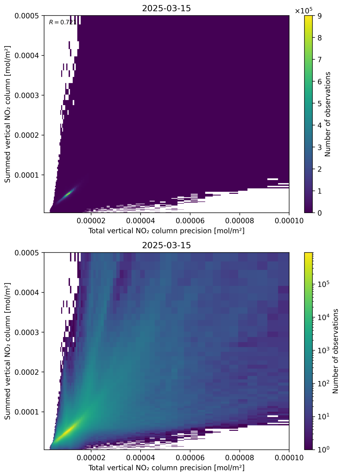
Figure 117: Scatter density plot of “Total vertical NO 2 column precision” against “Summed vertical NO 2 column” for 2025-03-15 to 2025-03-15.
