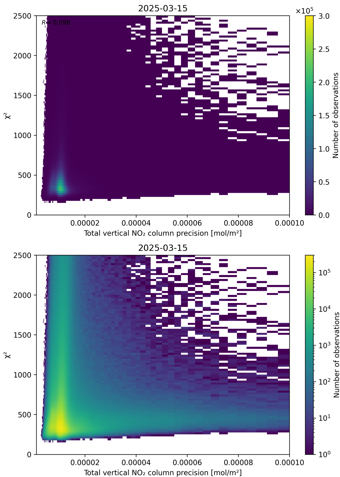
Figure 116: Scatter density plot of “Total vertical NO 2 column precision” against “ \chi^2 ” for 2025-03-15 to 2025-03-15.
