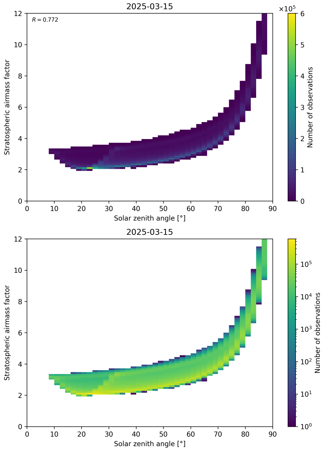
Figure 145: Scatter density plot of “Solar zenith angle” against “Stratospheric airmass factor” for 2025-03-15 to 2025-03-15.
