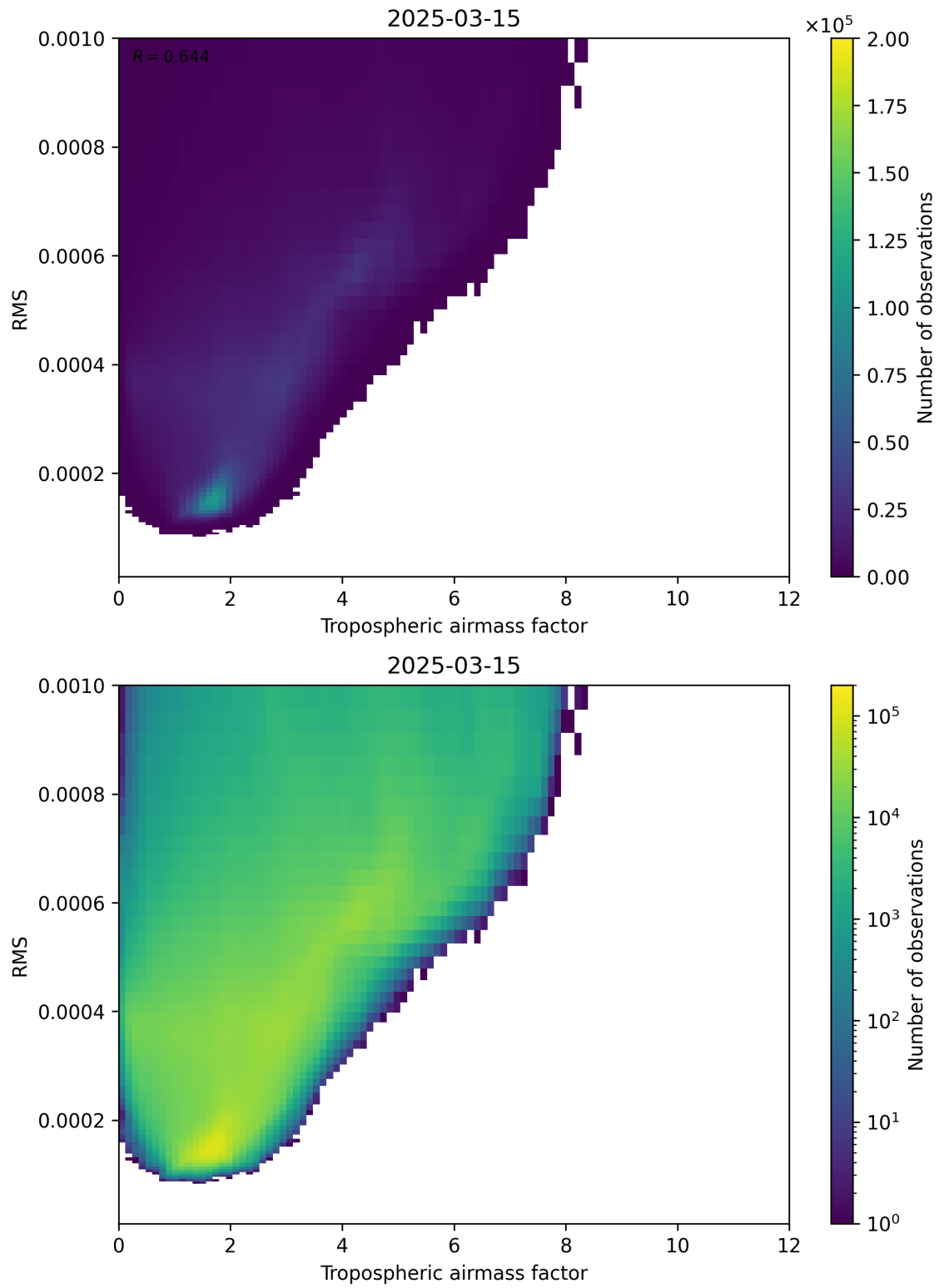
Figure 79: Scatter density plot of “Tropospheric airmass factor” against “RMS” for 2025-03-15 to 2025-03-15.
