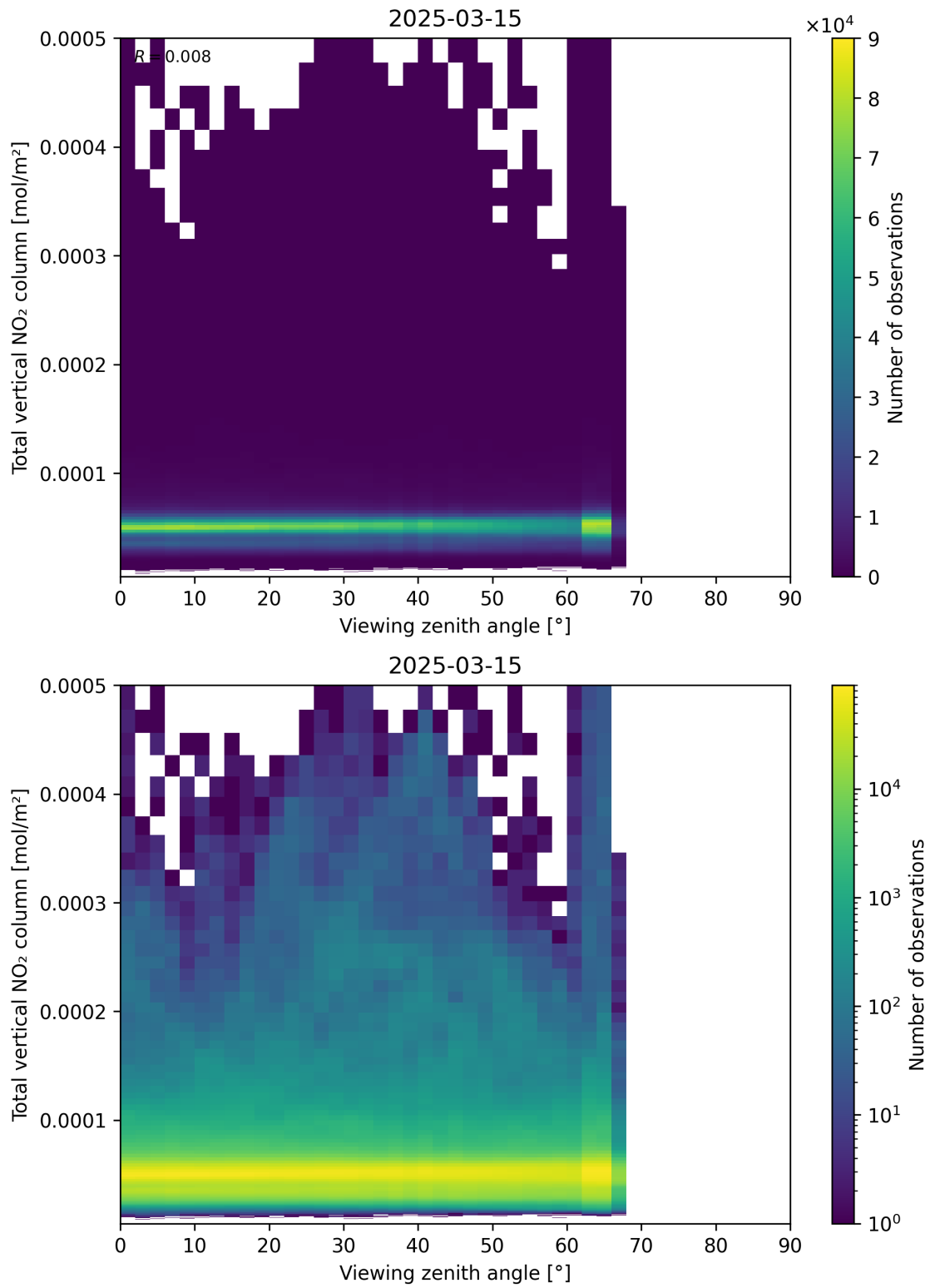
Figure 167: Scatter density plot of “Viewing zenith angle” against “Total vertical NO 2 column” for 2025-03-15 to 2025-03-15.
