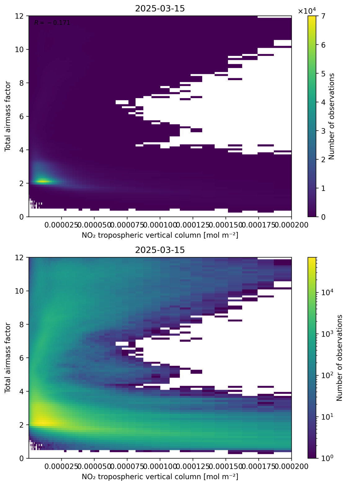
Figure 122: Scatter density plot of “NO 2 tropospheric vertical column” against “Total air mass factor” for 2025-03-15 to 2025-03-15.
