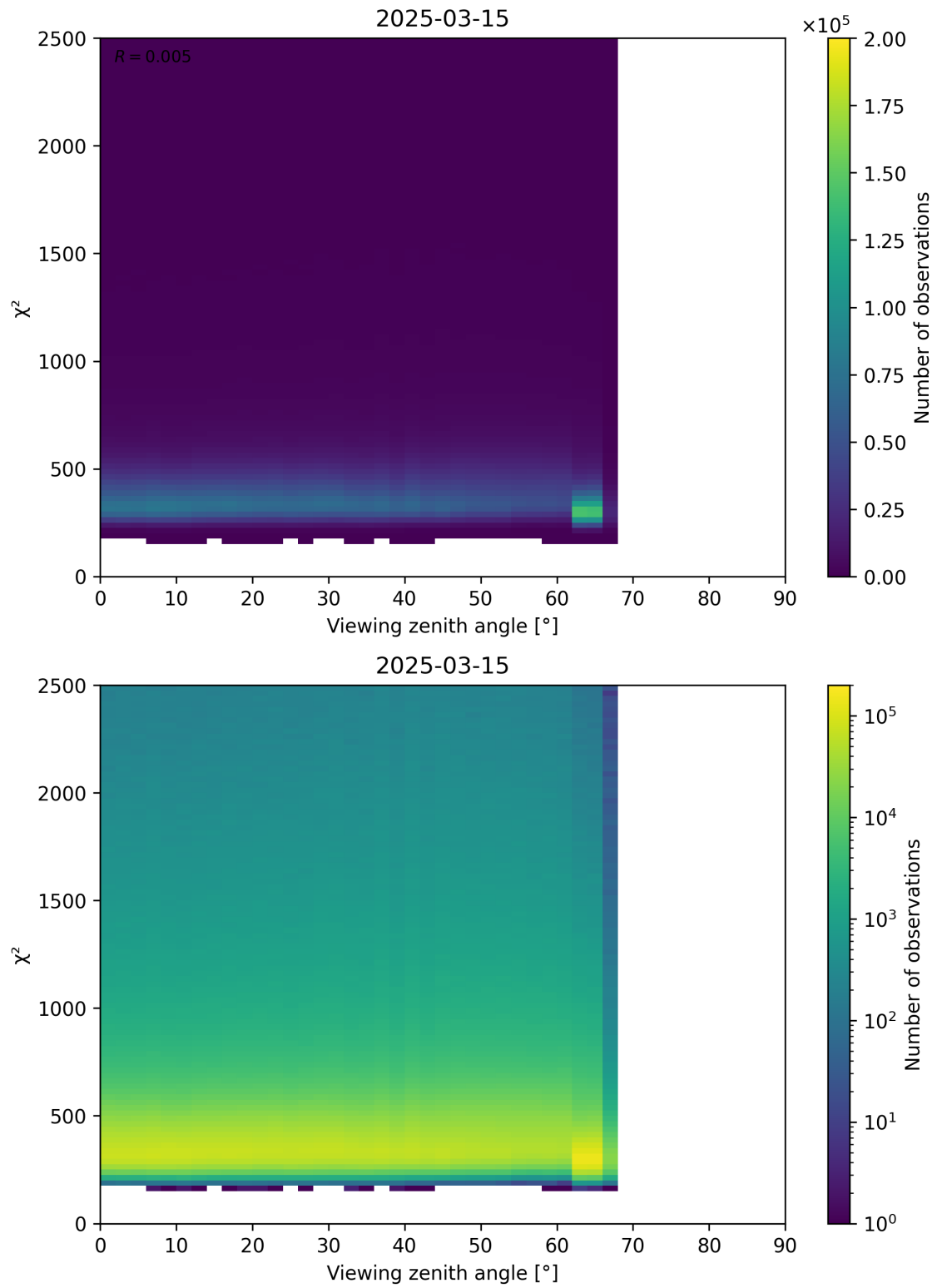
Figure 162: Scatter density plot of “Viewing zenith angle” against “ \chi^2 ” for 2025-03-15 to 2025-03-15.
