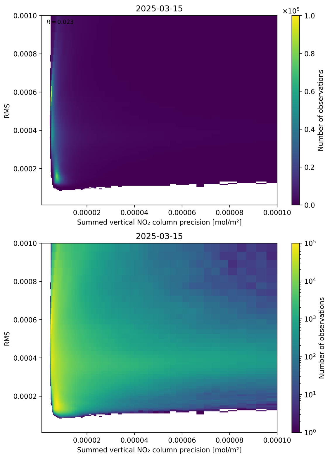
Figure 108: Scatter density plot of “Summed vertical NO 2 column precision” against “RMS” for 2025-03-15 to 2025-03-15.
