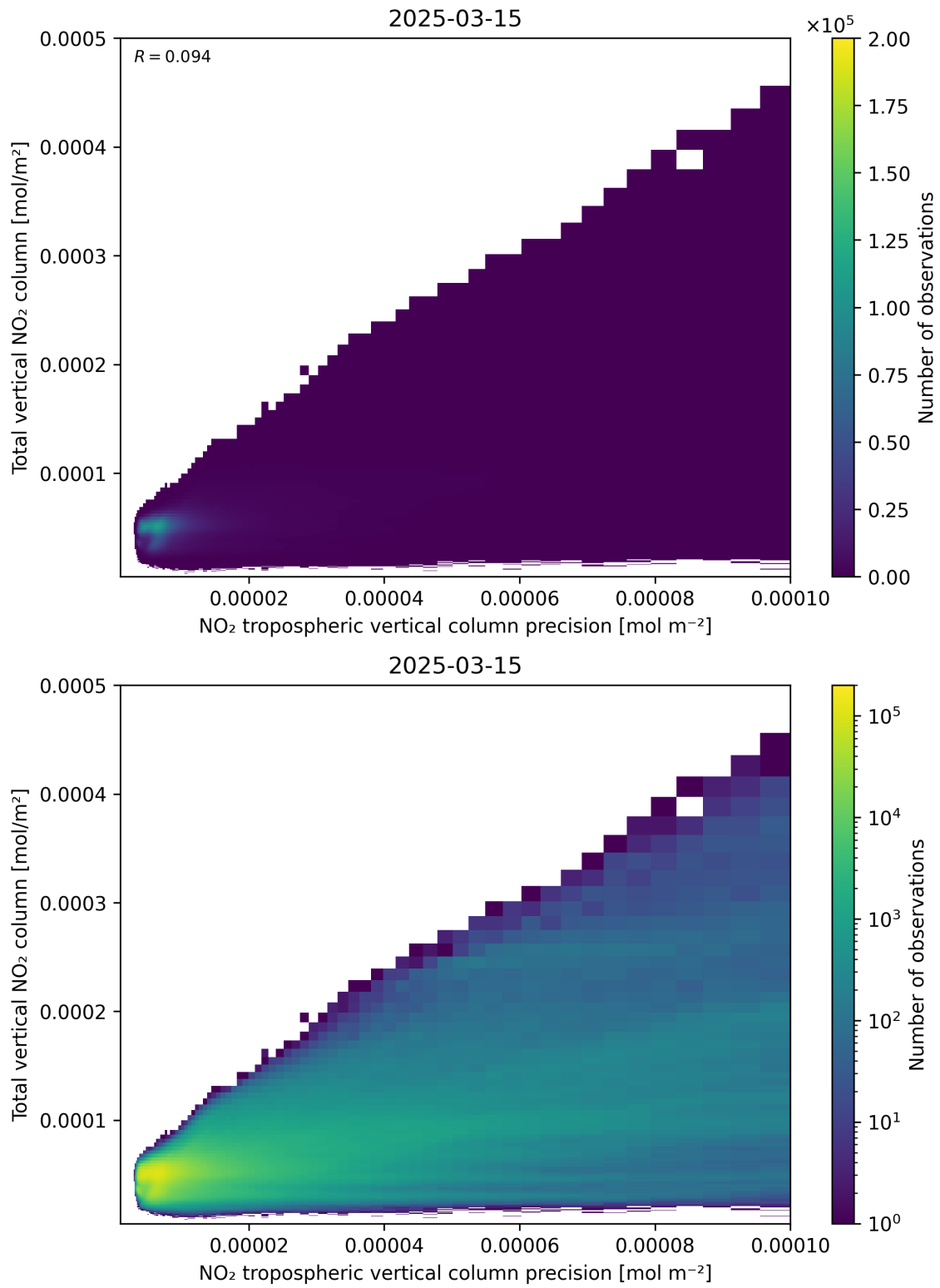
Figure 138: Scatter density plot of “NO 2 tropospheric vertical column precision” against “Total vertical NO 2 column” for 2025-03-15 to 2025-03-15.
