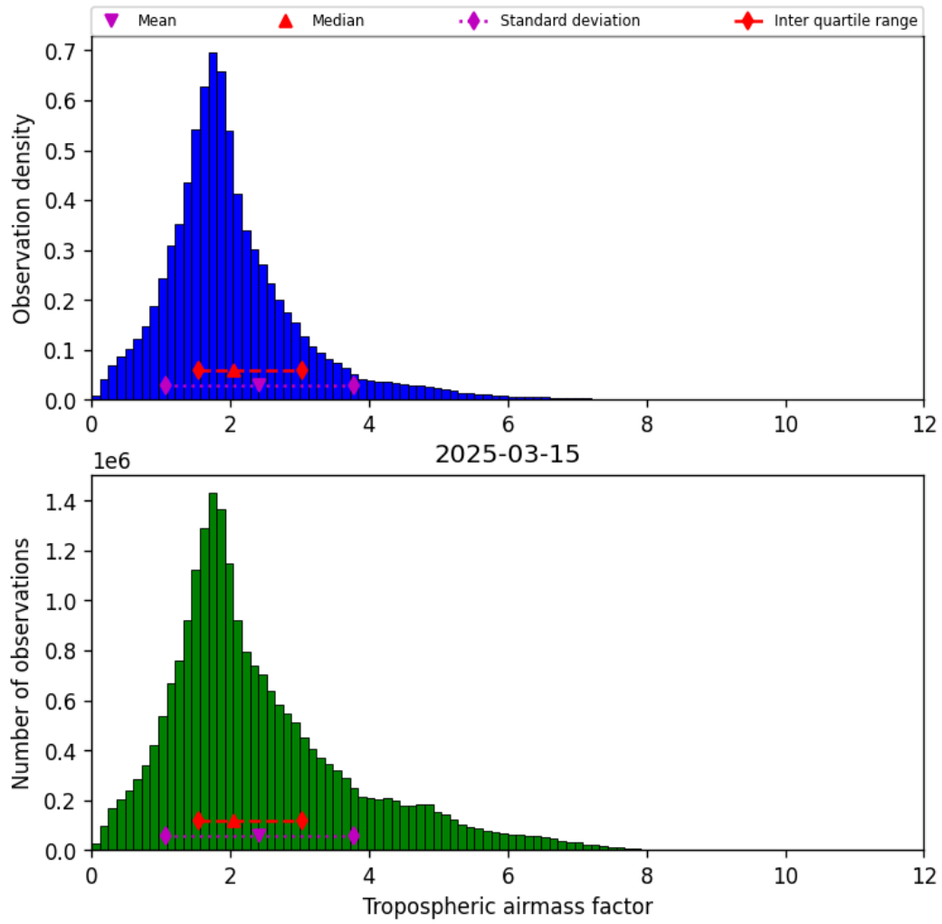
Figure 31: Histogram of “Tropospheric airmass factor” for 2025-03-15 to 2025-03-15
