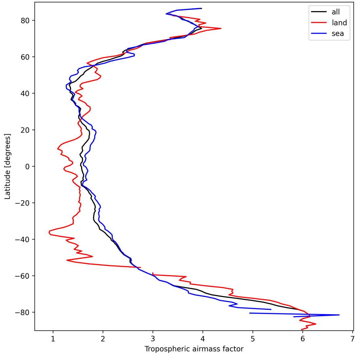
Figure 14: Zonal average of “Tropospheric airmass factor” for 2025-03-15 to 2025-03-15.
