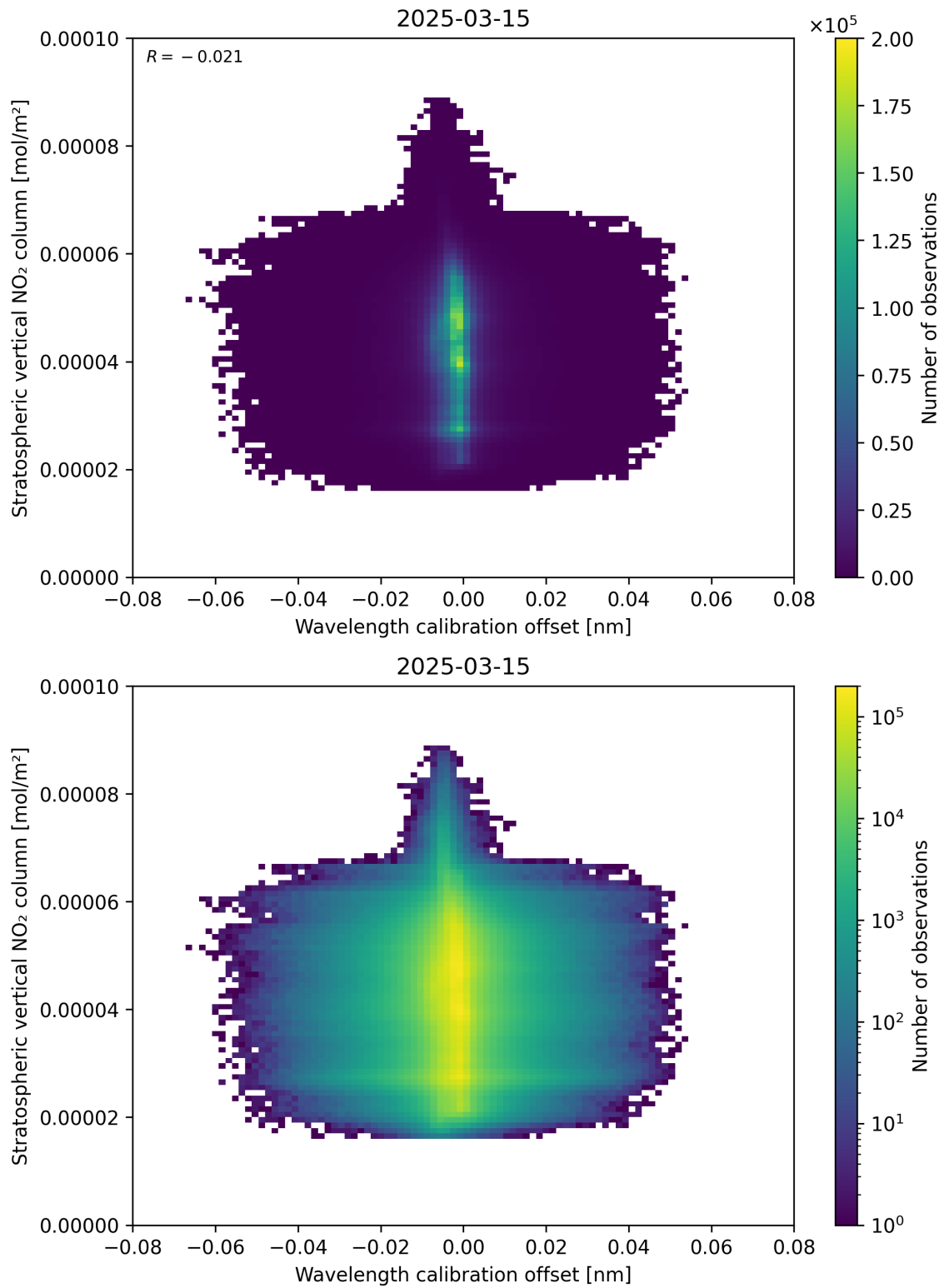
Figure 176: Scatter density plot of “Wavelength calibration offset” against “Stratospheric vertical NO 2 column” for 2025-03-15 to 2025-03-15.
