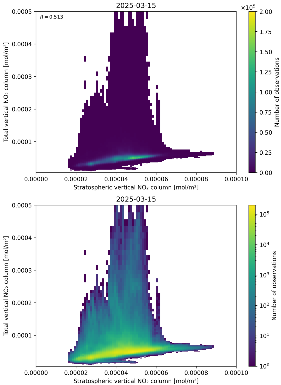
Figure 100: Scatter density plot of “Stratospheric vertical NO 2 column” against “Total vertical NO 2 column” for 2025-03-15 to 2025-03-15.
