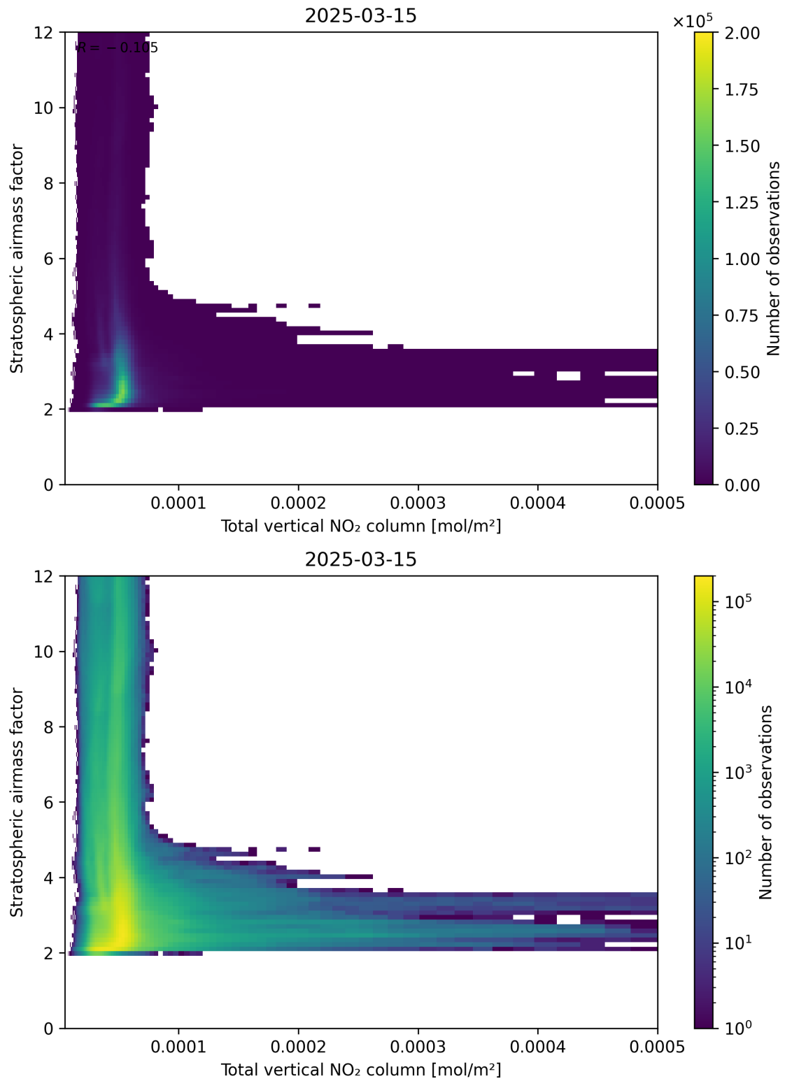
Figure 110: Scatter density plot of “Total vertical NO 2 column” against “Stratospheric airmass factor” for 2025-03-15 to 2025-03-15.
