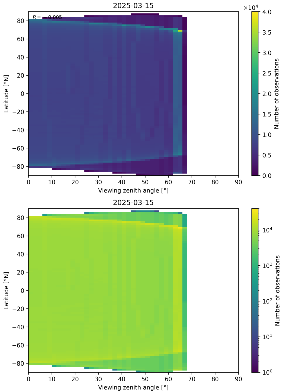
Figure 163: Scatter density plot of “Viewing zenith angle” against “Latitude” for 2025-03-15 to 2025-03-15.
