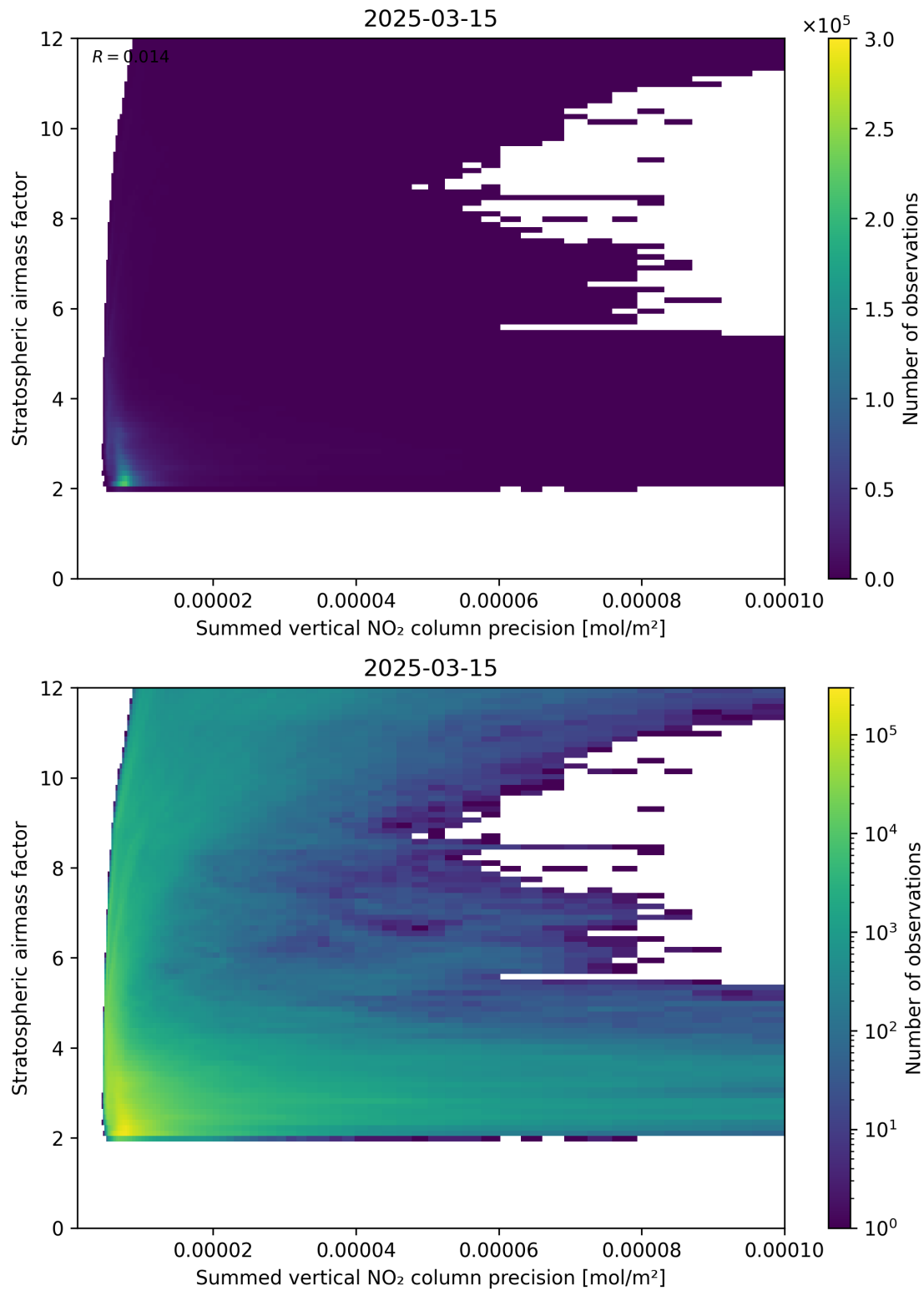
Figure 106: Scatter density plot of “Summed vertical NO 2 column precision” against “Stratospheric airmass factor” for 2025-03-15 to 2025-03-15.
