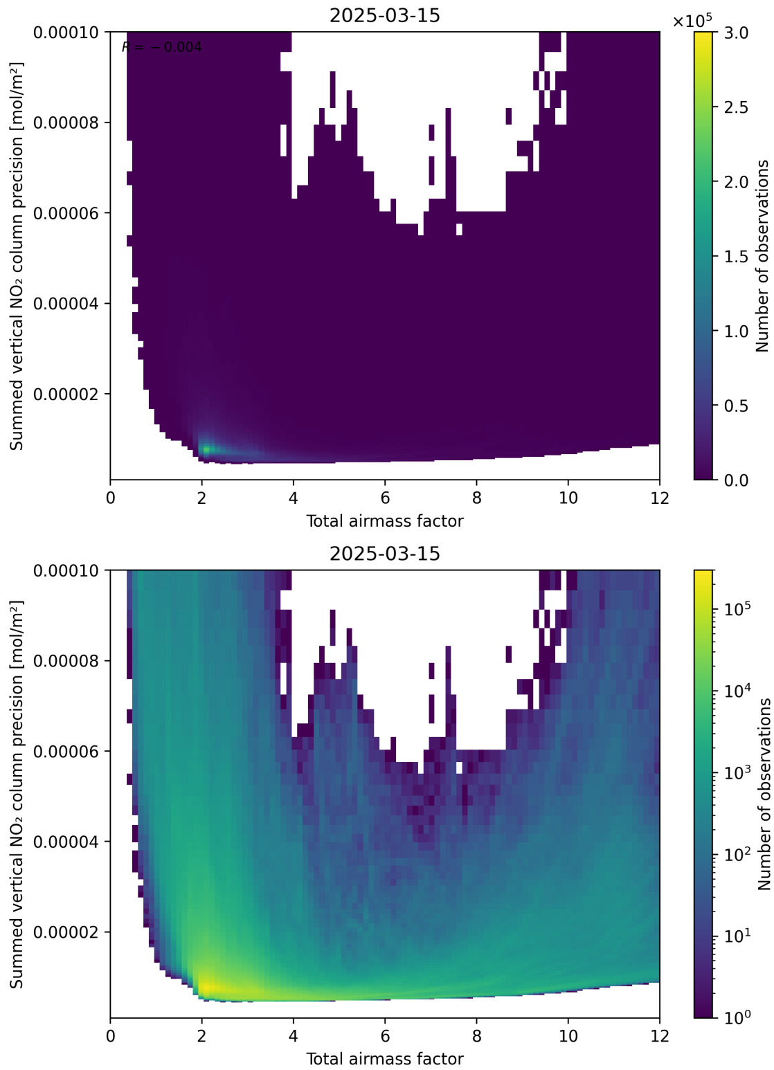
Figure 66: Scatter density plot of “Total airmass factor” against “Summed vertical NO 2 column precision” for 2025-03-15 to 2025-03-15.
