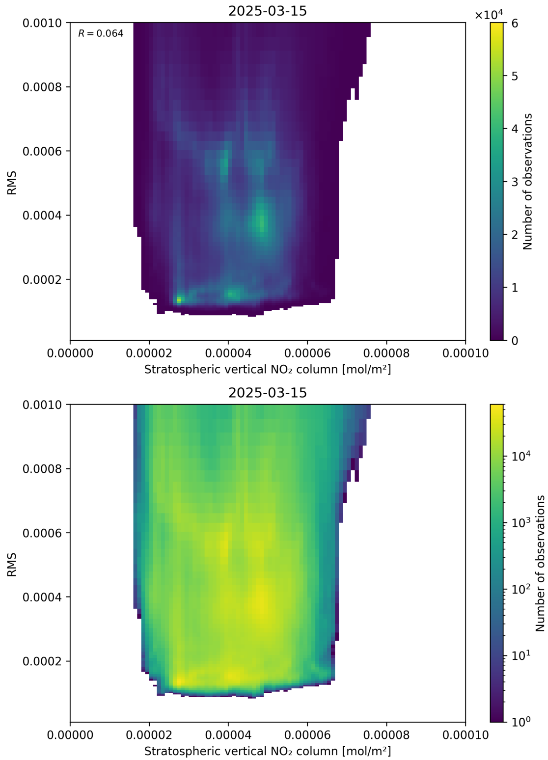
Figure 102: Scatter density plot of “Stratospheric vertical NO 2 column” against “RMS” for 2025-03-15 to 2025-03-15.
