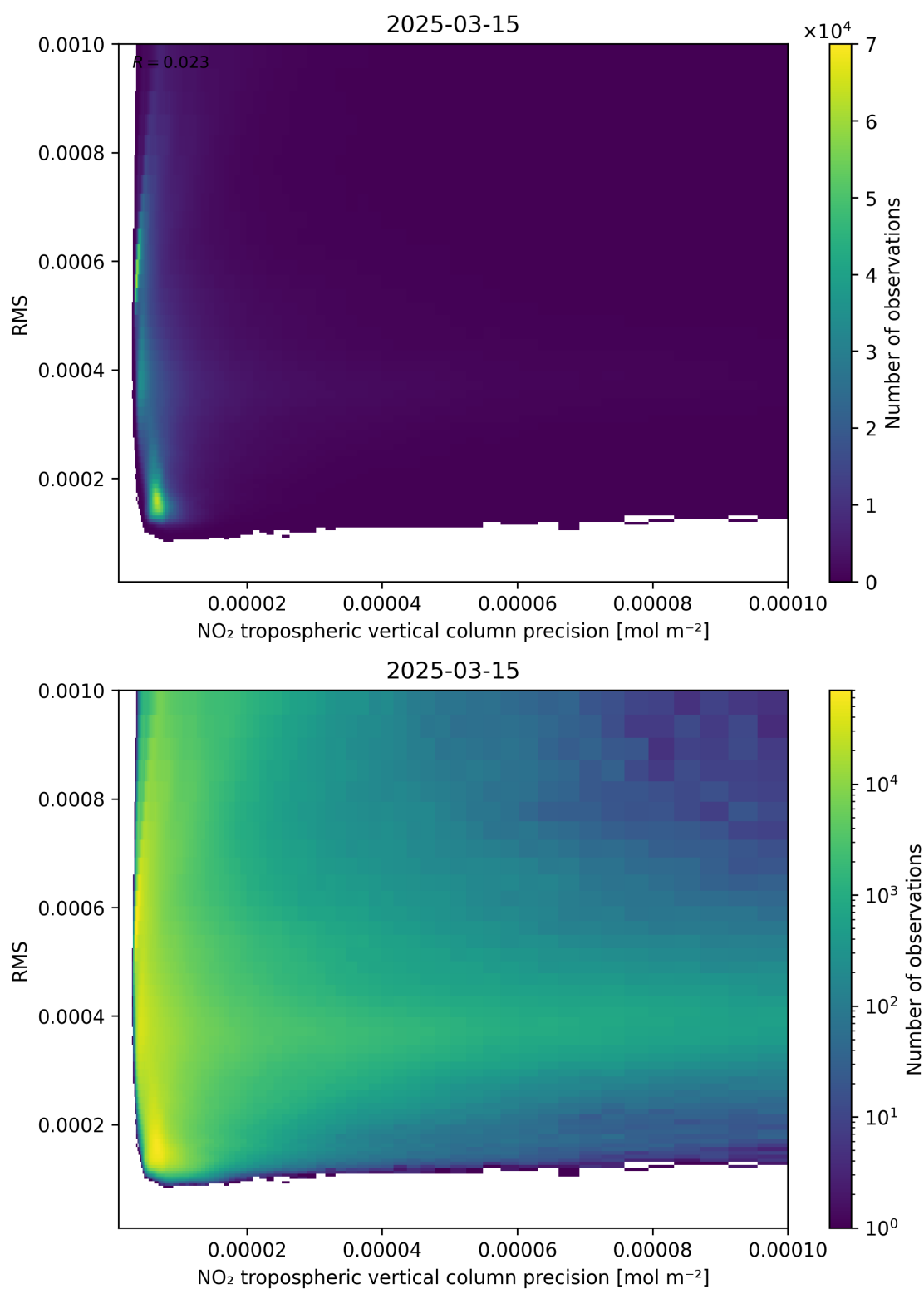
Figure 140: Scatter density plot of “NO 2 tropospheric vertical column precision” against “RMS” for 2025-03-15 to 2025-03-15.
