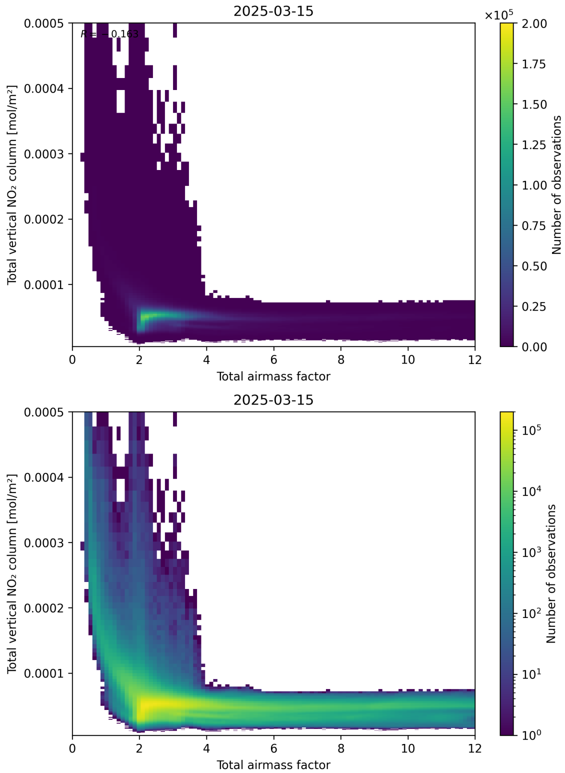
Figure 67: Scatter density plot of “Total airmass factor” against “Total vertical NO 2 column” for 2025-03-15 to 2025-03-15.
