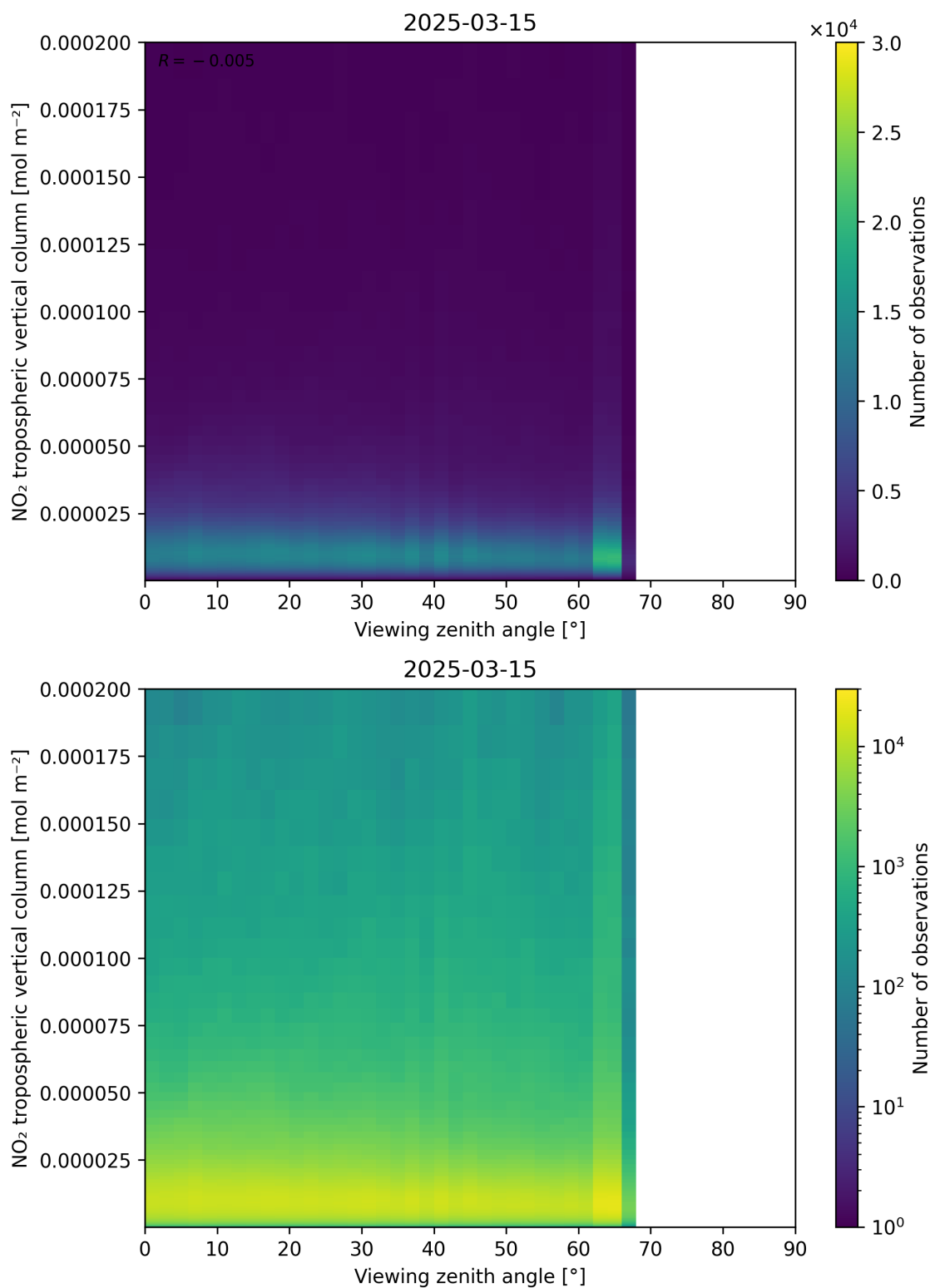
Figure 169: Scatter density plot of “Viewing zenith angle” against “NO 2 tropospheric vertical column” for 2025-03-15 to 2025-03-15.
