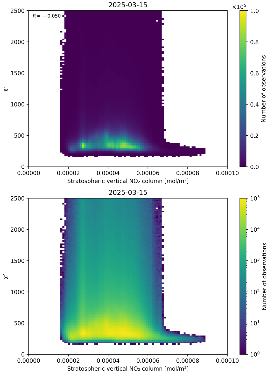
Figure 97: Scatter density plot of “Stratospheric vertical NO 2 column” against “ \chi^2 ” for 2025-03-15 to 2025-03-15.
