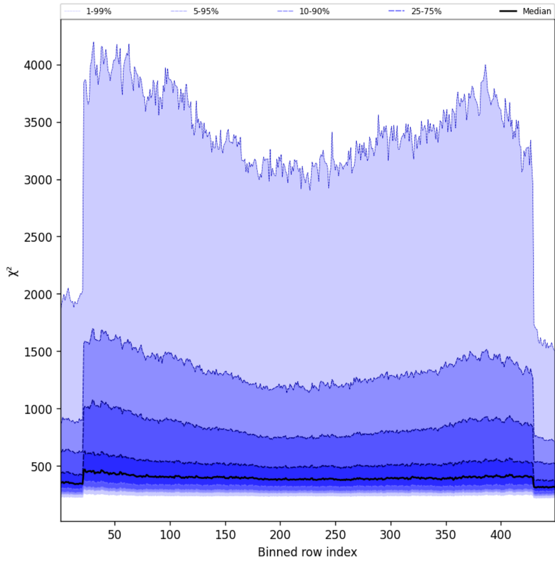
Figure 59: Along track statistics of “ \chi^2 ” for 2025-03-15 to 2025-03-15
