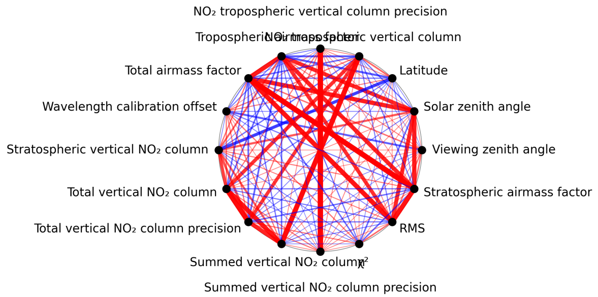
Figure 1: Map of correlation graph for 2025-03-15 to 2025-03-15.
