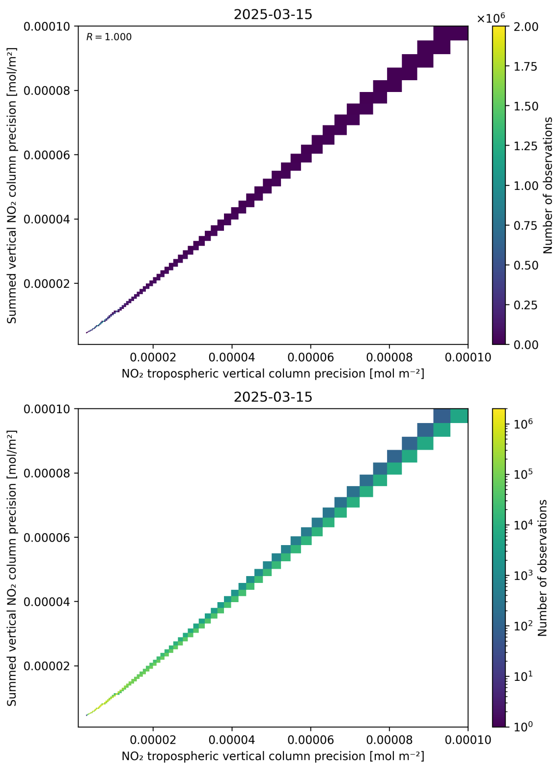
Figure 137: Scatter density plot of “NO 2 tropospheric vertical column precision” against “Summed vertical NO 2 column precision” for 2025-03-15 to 2025-03-15.
