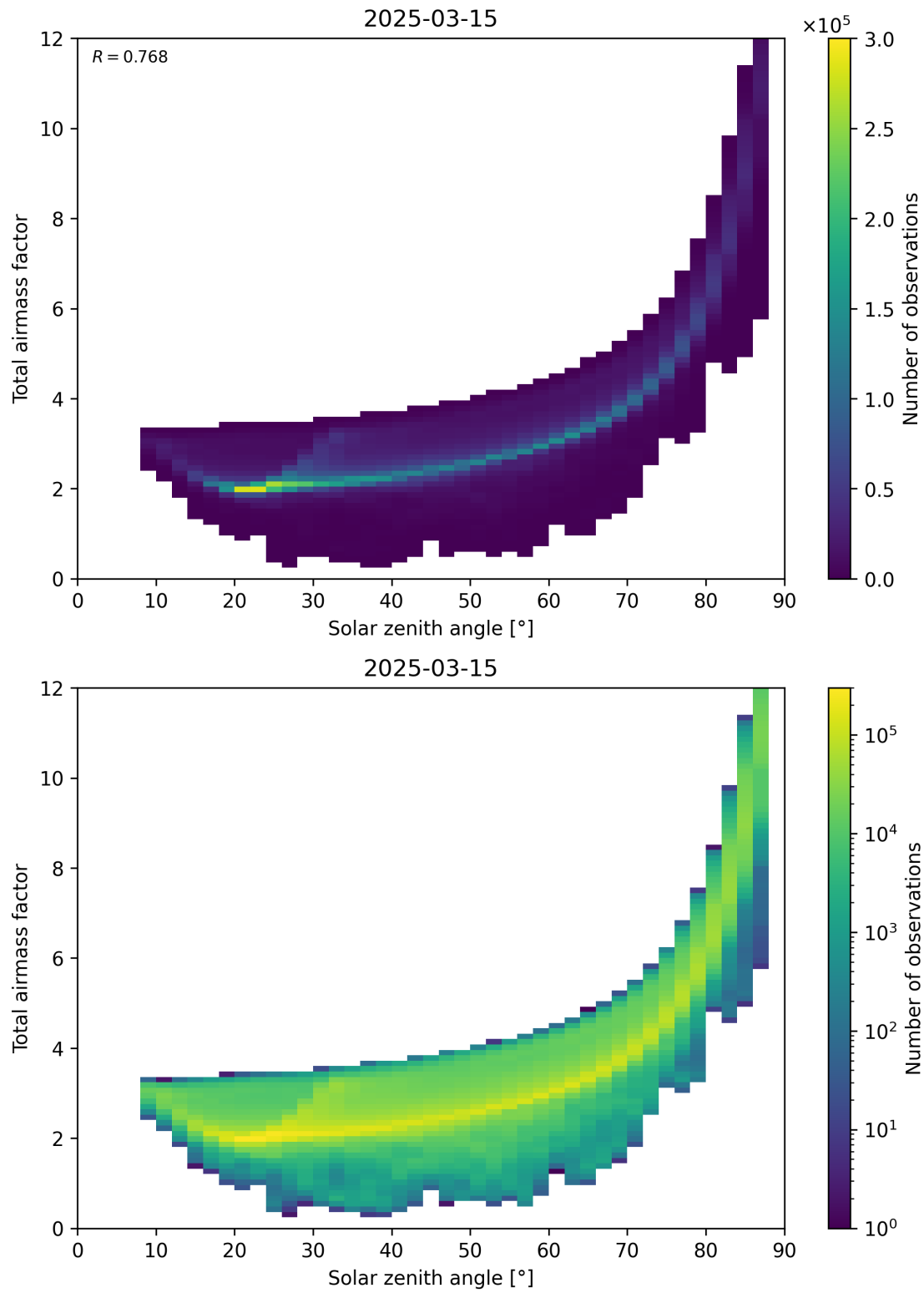
Figure 146: Scatter density plot of “Solar zenith angle” against “Total airmass factor” for 2025-03-15 to 2025-03-15.
