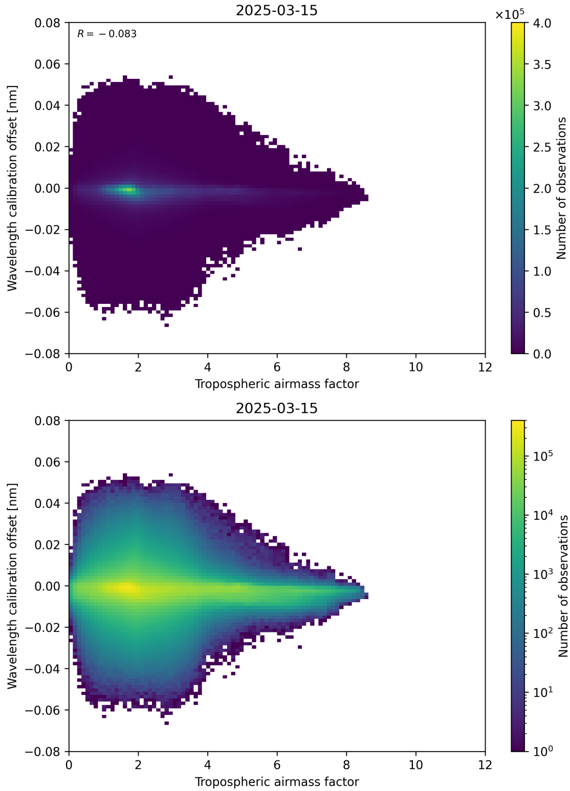
Figure 80: Scatter density plot of “Tropospheric airmass factor” against “Wavelength calibration offset” for 2025-03-15 to 2025-03-15.
