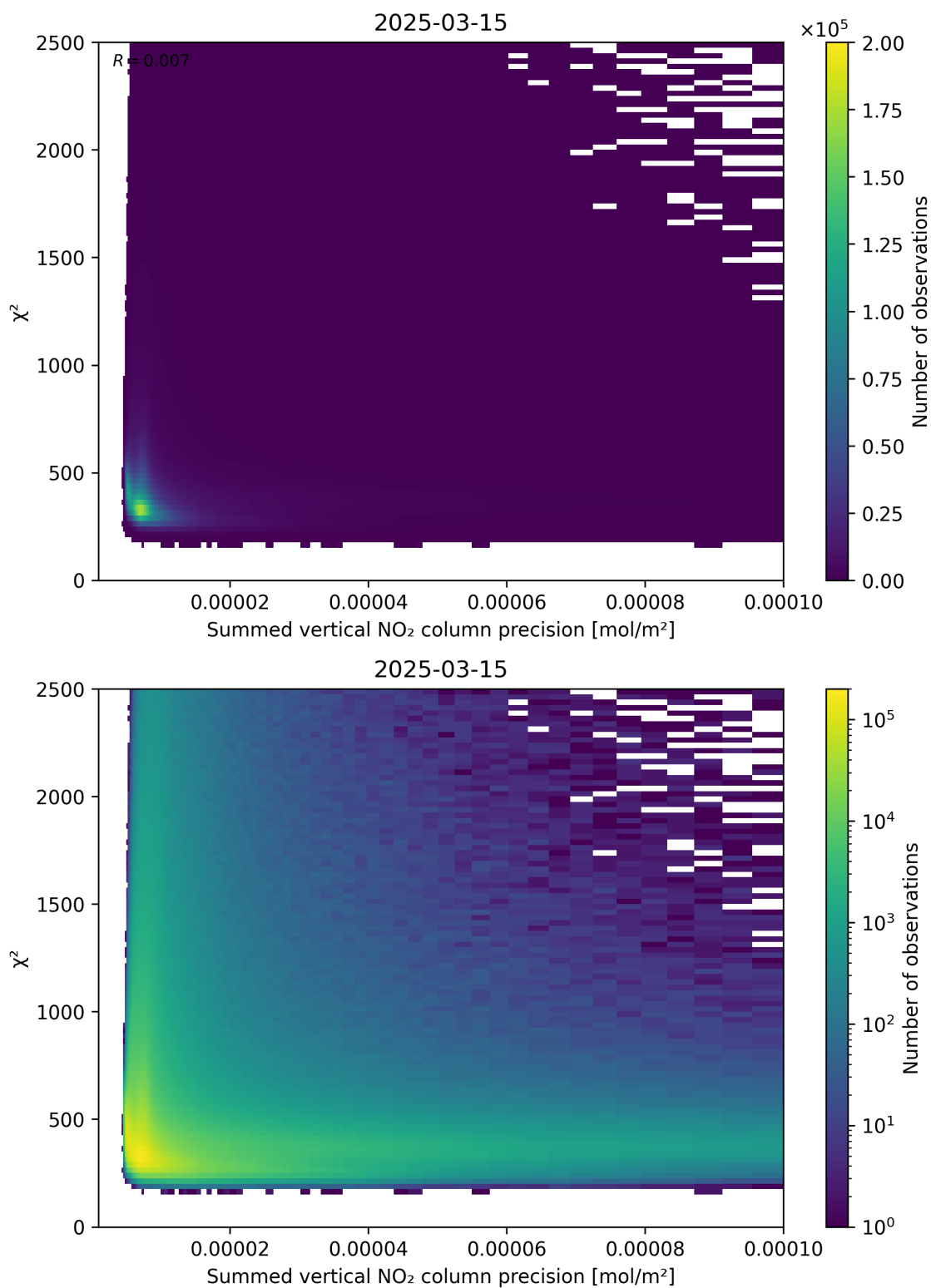
Figure 107: Scatter density plot of “Summed vertical NO 2 column precision” against “ \chi^2 ” for 2025-03-15 to 2025-03-15.
