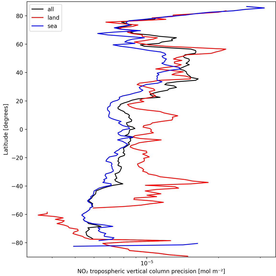
Figure 13: Zonal average of “NO 2 tropospheric vertical column precision” for 2025-03-15 to 2025-03-15.
