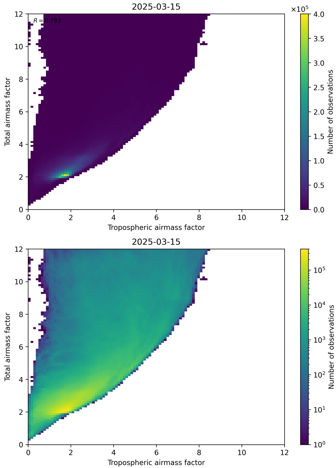
Figure 72: Scatter density plot of “Tropospheric airmass factor” against “Total airmass factor” for 2025-03-15 to 2025-03-15.
