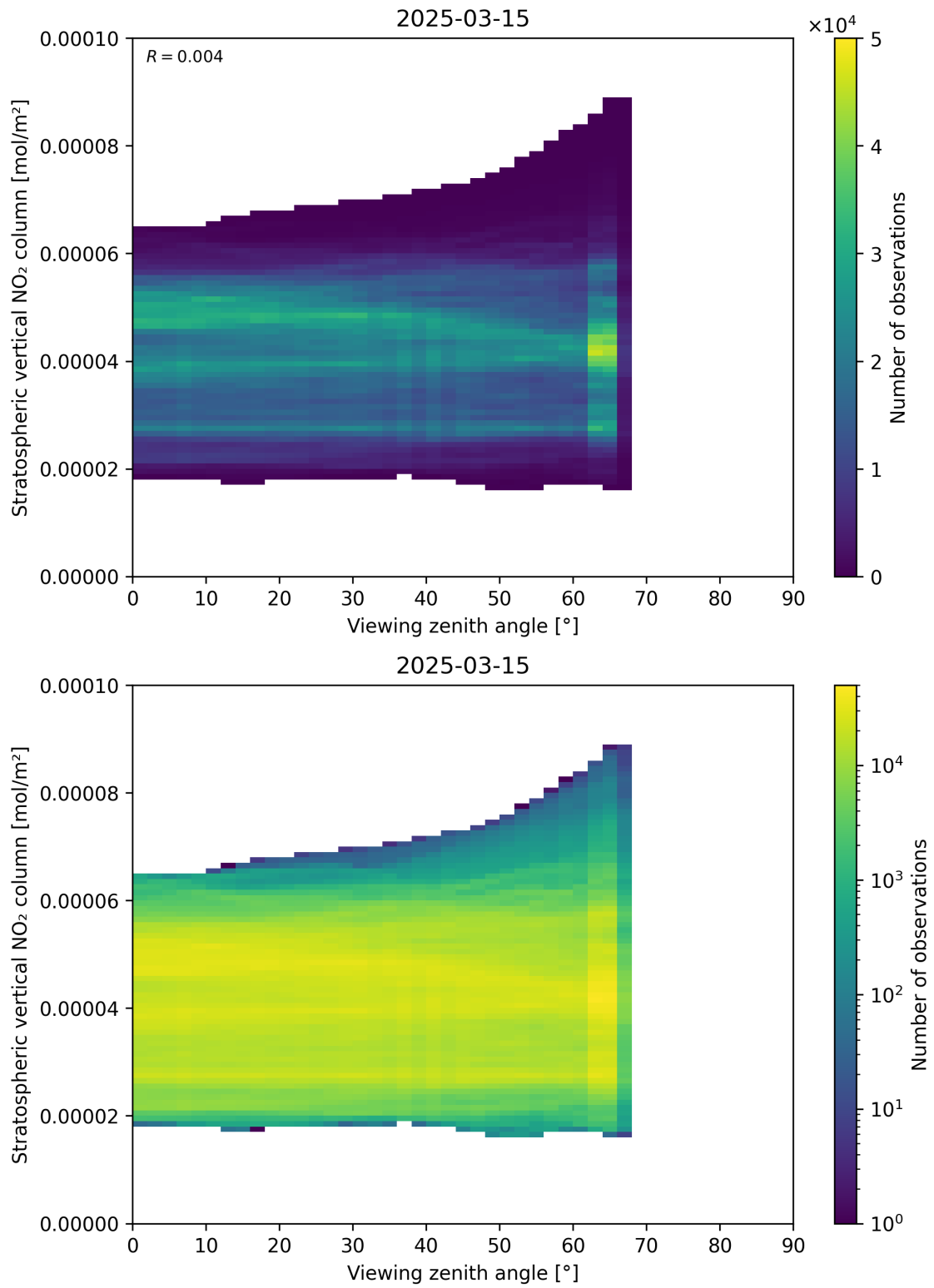
Figure 164: Scatter density plot of “Viewing zenith angle” against “Stratospheric vertical NO 2 column” for 2025-03-15 to 2025-03-15.
