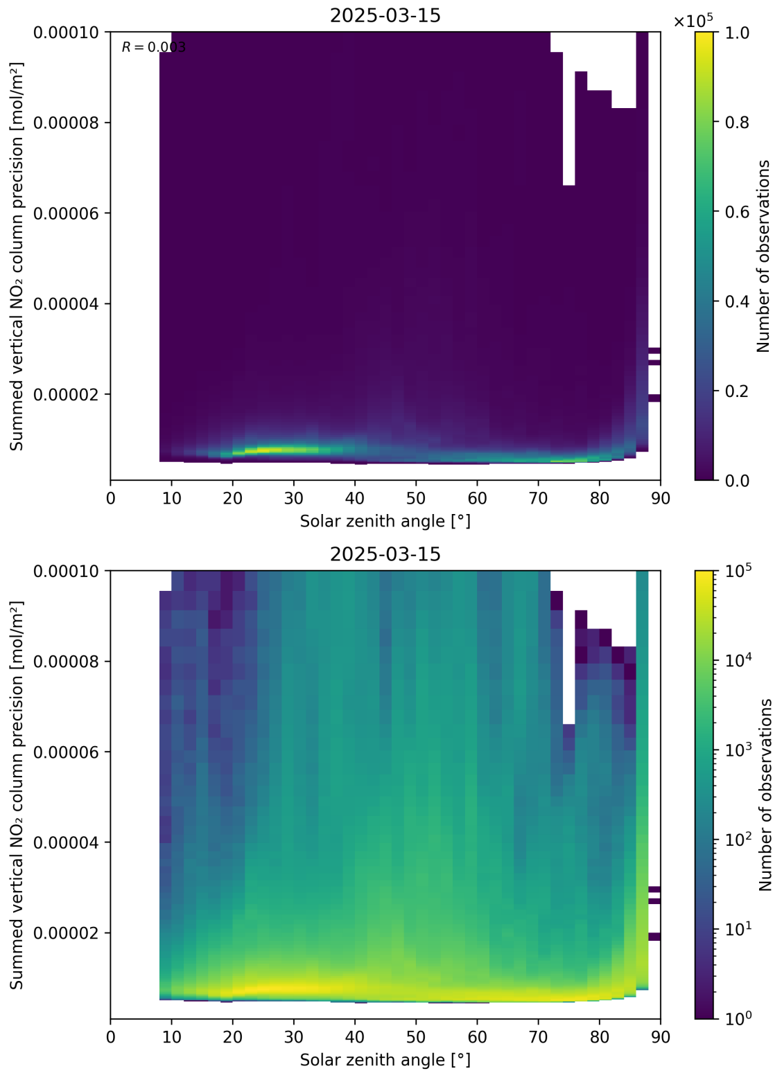
Figure 152: Scatter density plot of “Solar zenith angle” against “Summed vertical NO 2 column precision” for 2025-03-15 to 2025-03-15.
