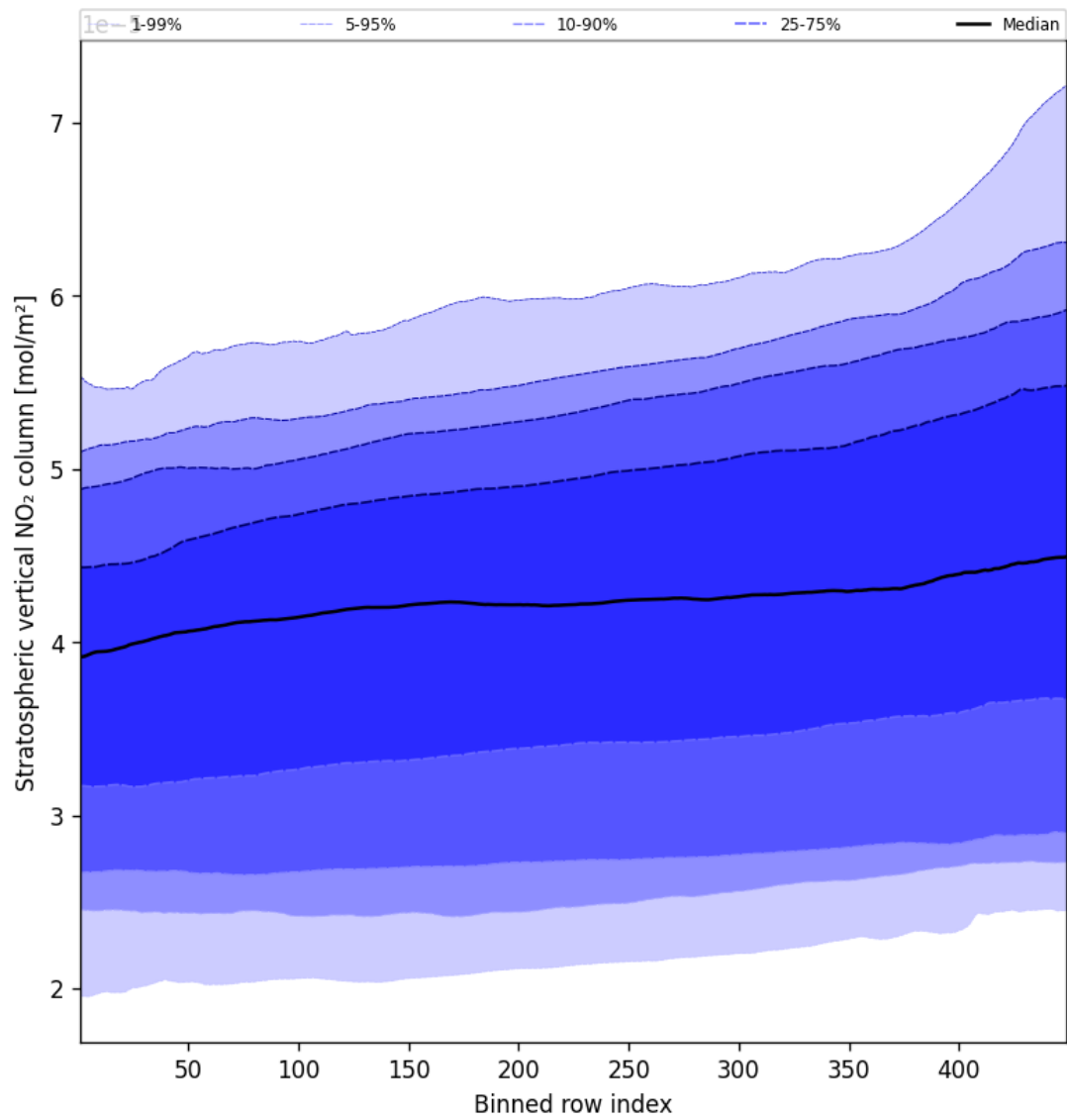
Figure 53: Along track statistics of “Stratospheric vertical NO 2 column” for 2025-03-15 to 2025-03-15
