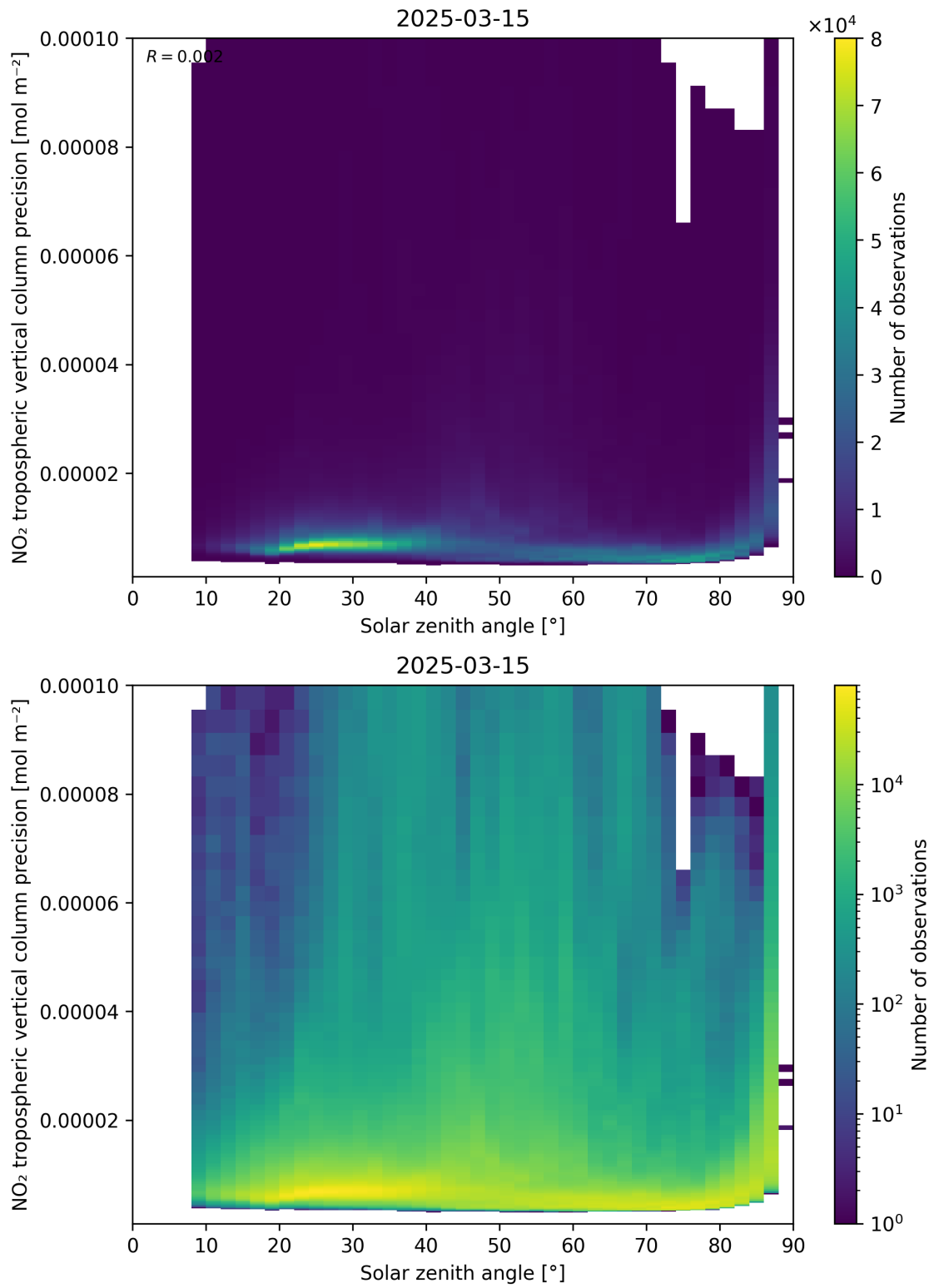
Figure 156: Scatter density plot of “Solar zenith angle” against “NO 2 tropospheric vertical column precision” for 2025-03-15 to 2025-03-15.
