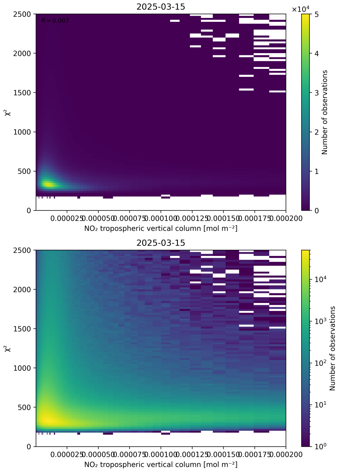
Figure 124: Scatter density plot of “NO 2 tropospheric vertical column” against “ \chi^2 ” for 2025-03-15 to 2025-03-15.
