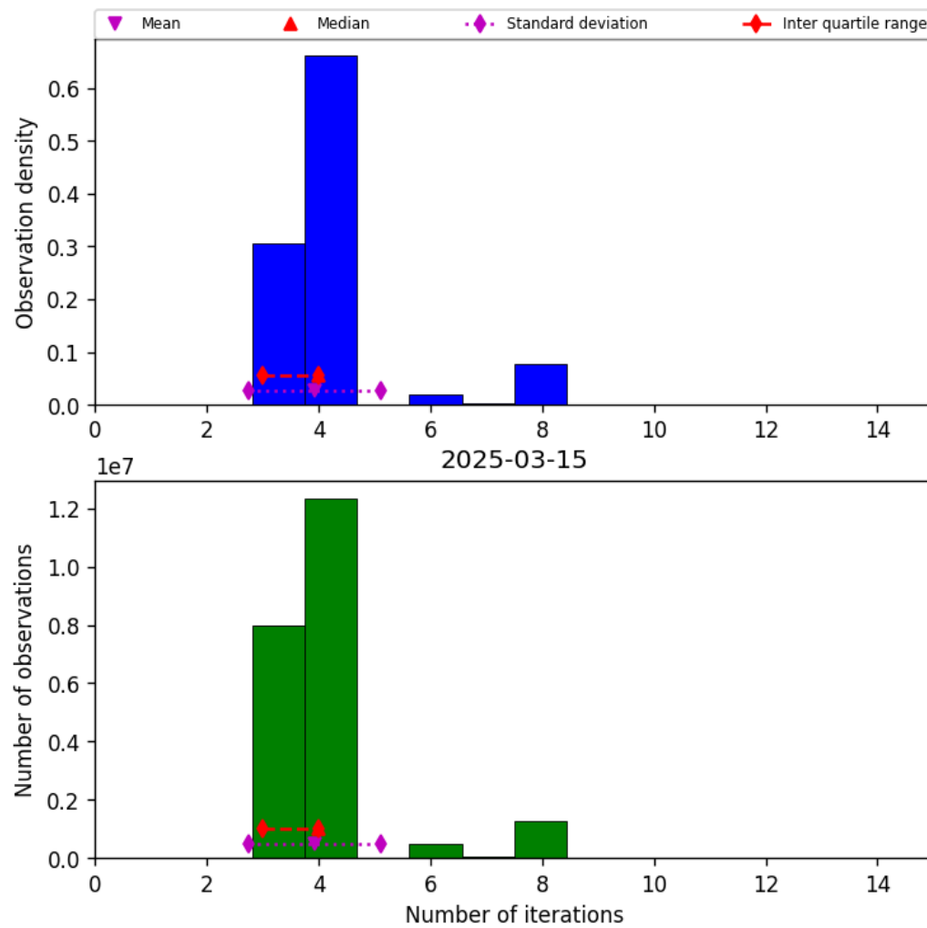
Figure 34: Histogram of “Number of iterations” for 2025-03-15 to 2025-03-15
