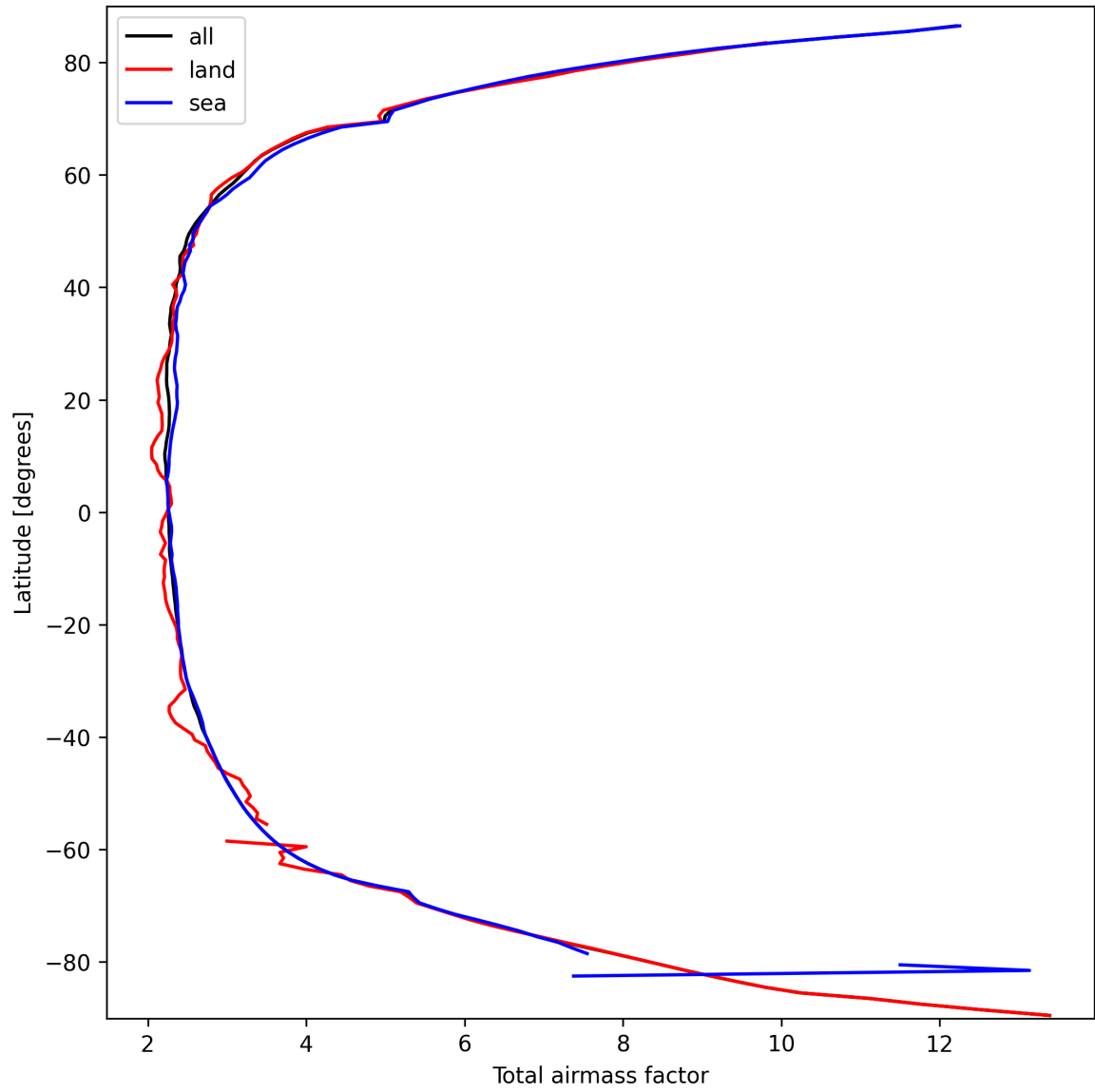
Figure 15: Zonal average of “Total airmass factor” for 2025-03-15 to 2025-03-15.
