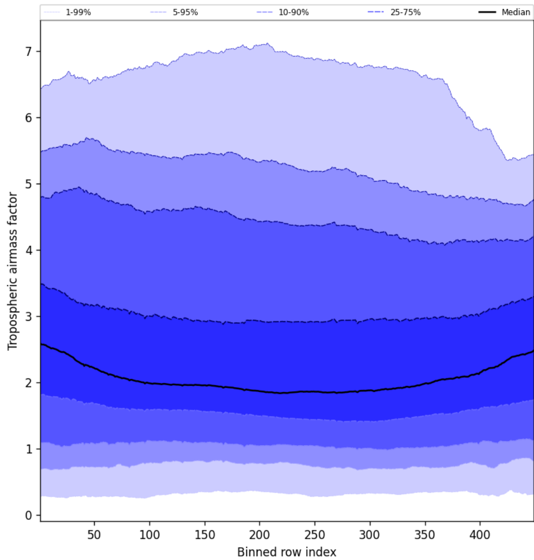
Figure 48: Along track statistics of “Tropospheric airmass factor” for 2025-03-15 to 2025-03-15
