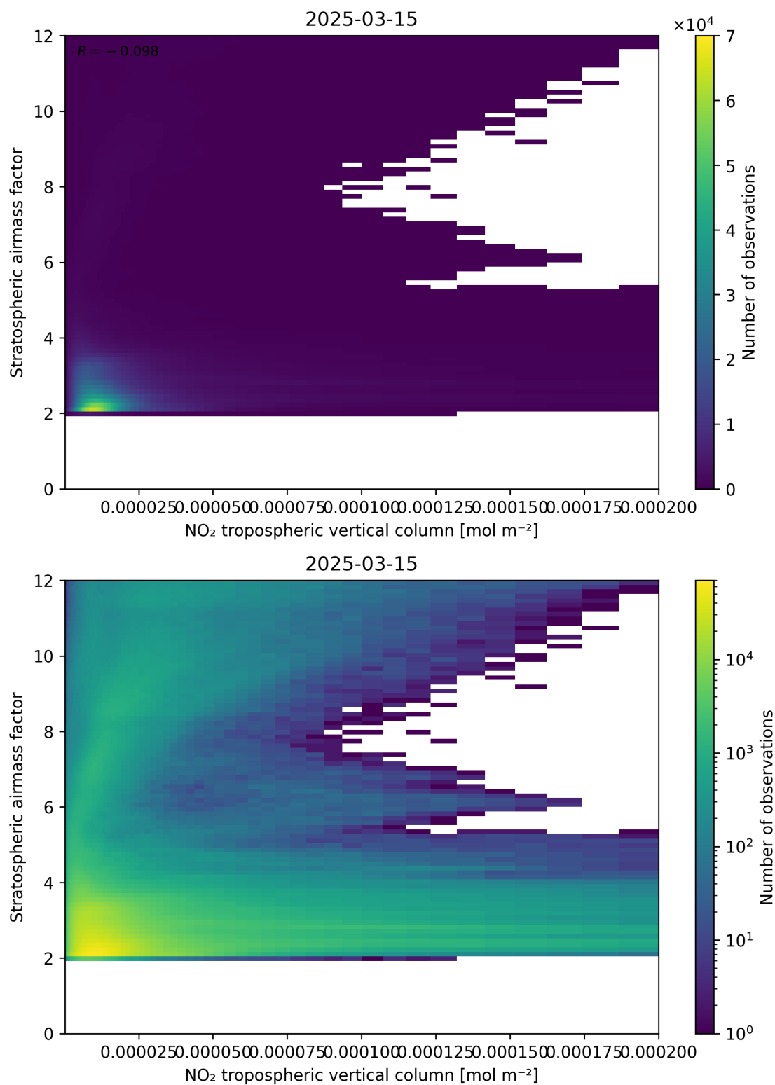
Figure 121: Scatter density plot of “NO 2 tropospheric vertical column” against “Stratospheric air mass factor” for 2025-03-15 to 2025-03-15.
